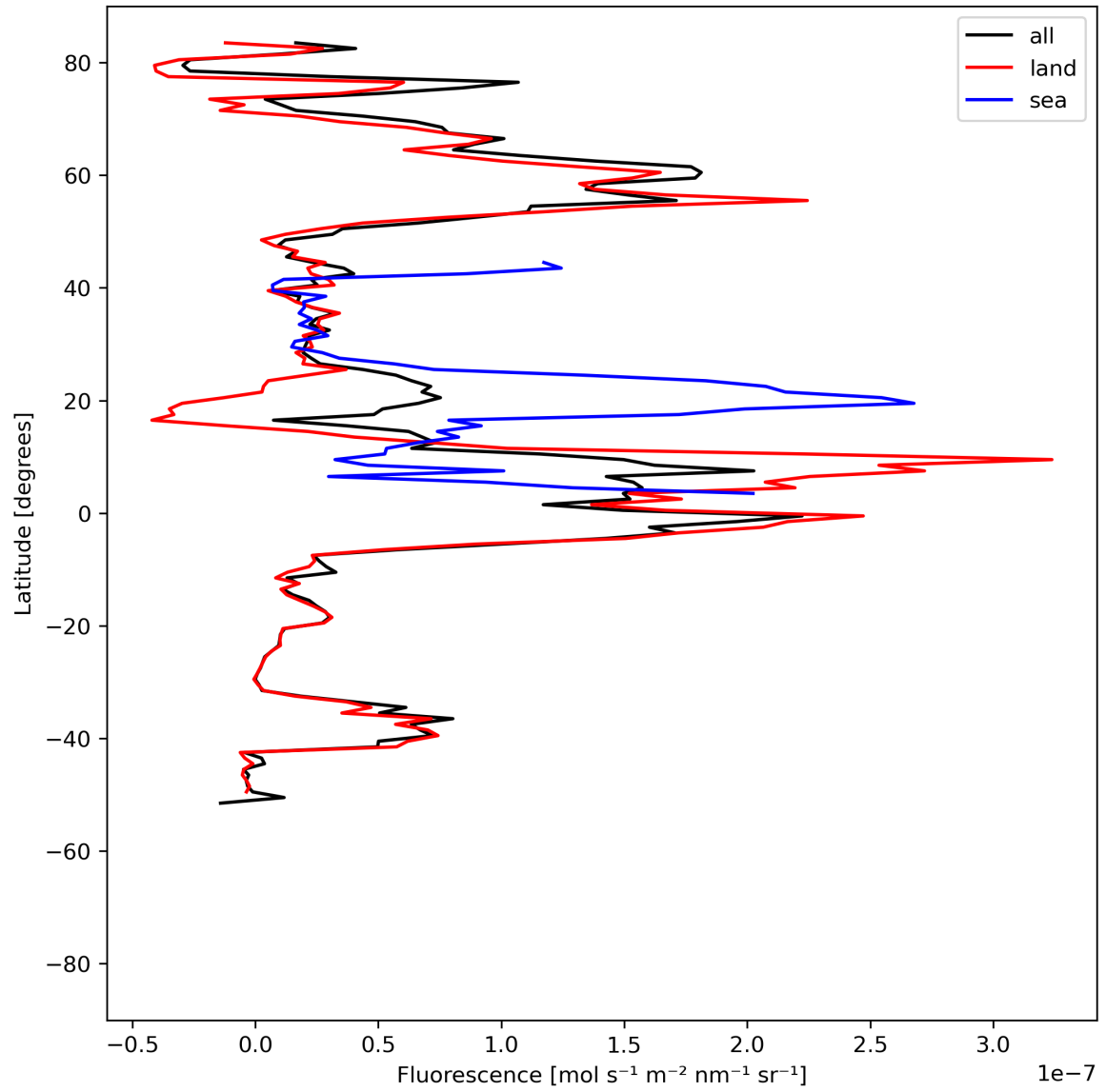
Figure 21: Zonal average of “Fluorescence” for 2023-07-30 to 2023-08-01.
