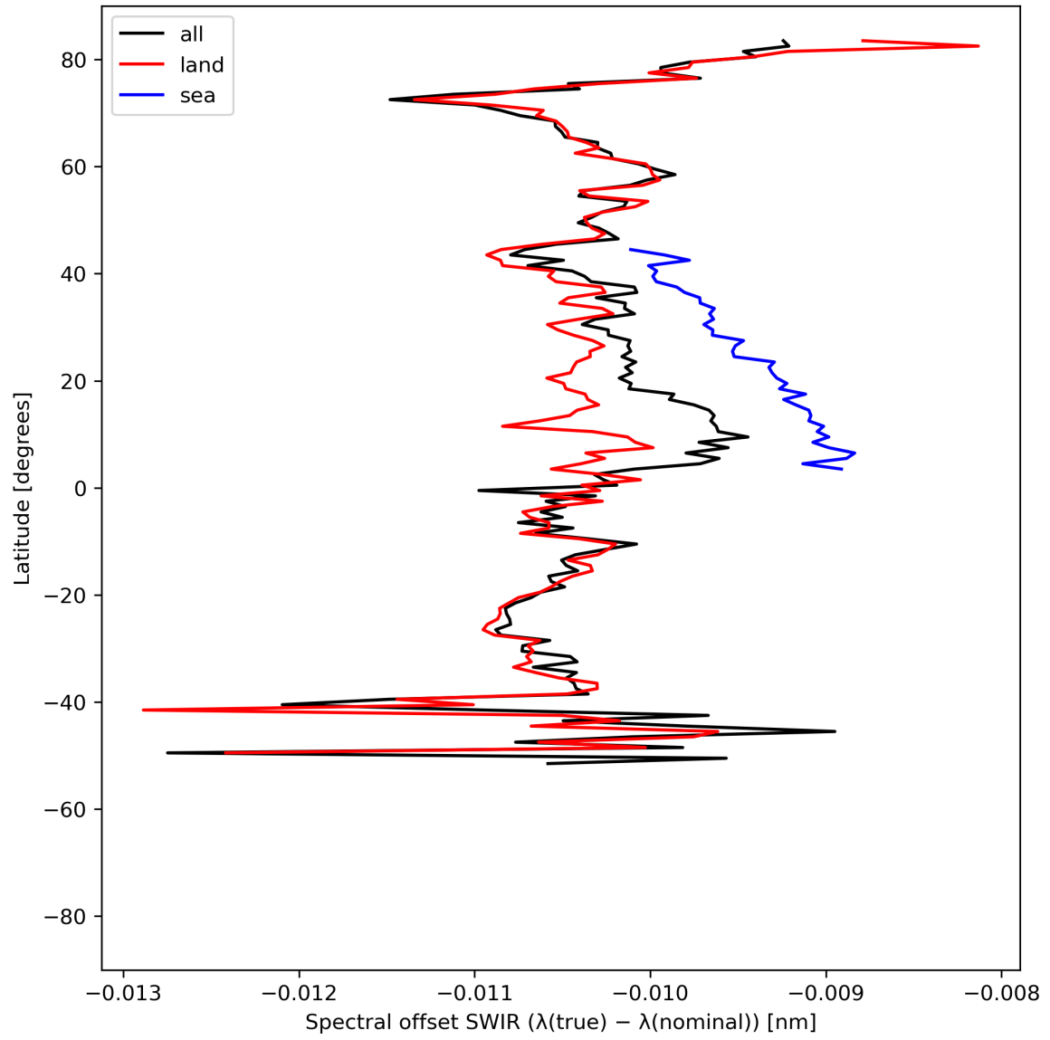
Figure 16: Zonal average of “Spectral offset SWIR ( \lambda(\text{true}) - \lambda(\text{nominal}) )” for 2023-07-30 to 2023-08-01.
