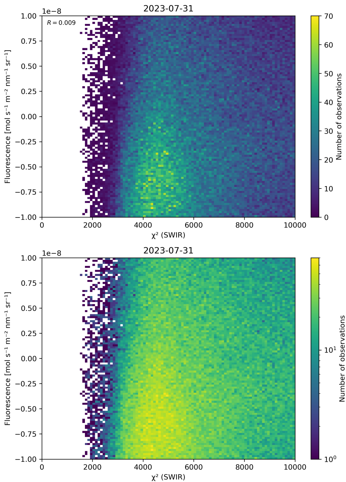
Figure 49: Scatter density plot of “ \chi^2 (SWIR)” against “Fluorescence” for 2023-07-30 to 2023-08-01.
