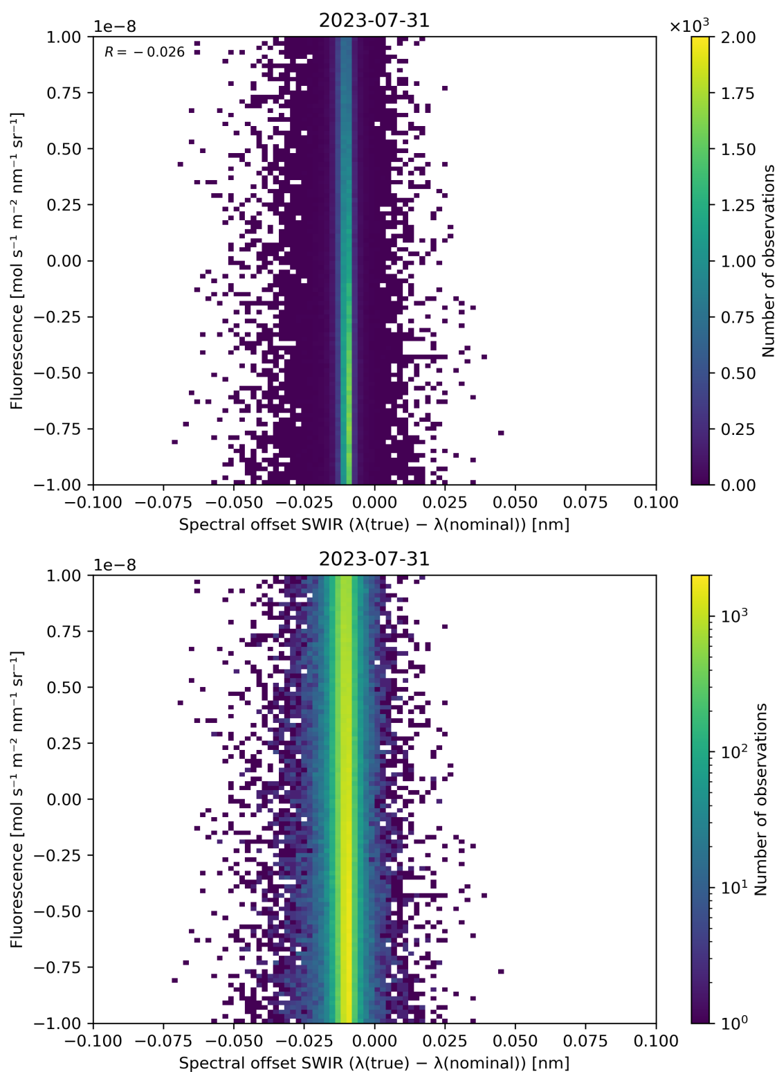
Figure 120: Scatter density plot of “Spectral offset SWIR ( \lambda(\text{true}) - \lambda(\text{nominal}) )” against “Fluorescence” for 2023-07-30 to 2023-08-01.
