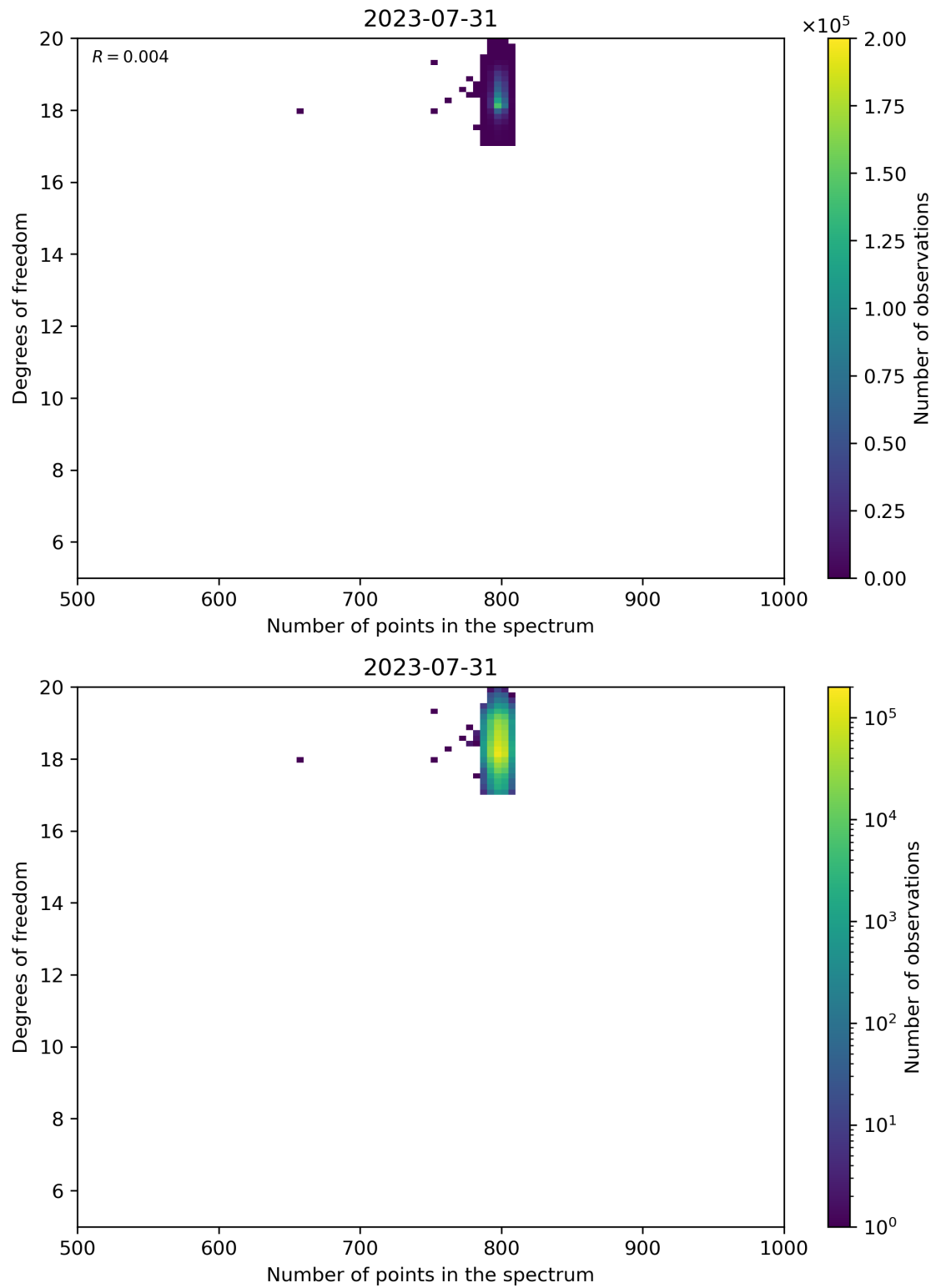
Figure 90: Scatter density plot of “Number of points in the spectrum” against “Degrees of freedom” for 2023-07-30 to 2023-08-01.
