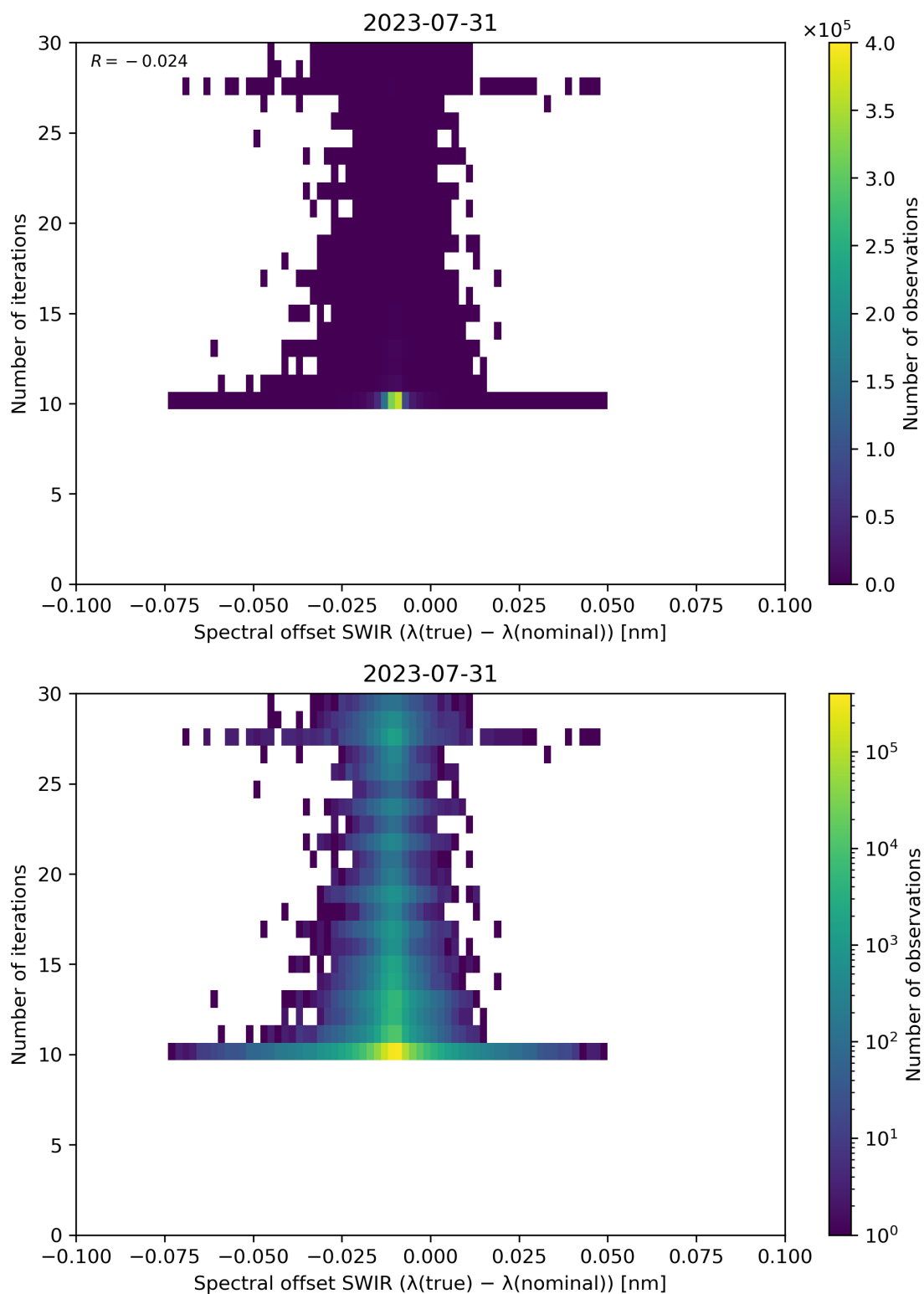
Figure 121: Scatter density plot of “Spectral offset SWIR ( \lambda(\text{true}) - \lambda(\text{nominal}) )” against “Number of iterations” for 2023-07-30 to 2023-08-01.
