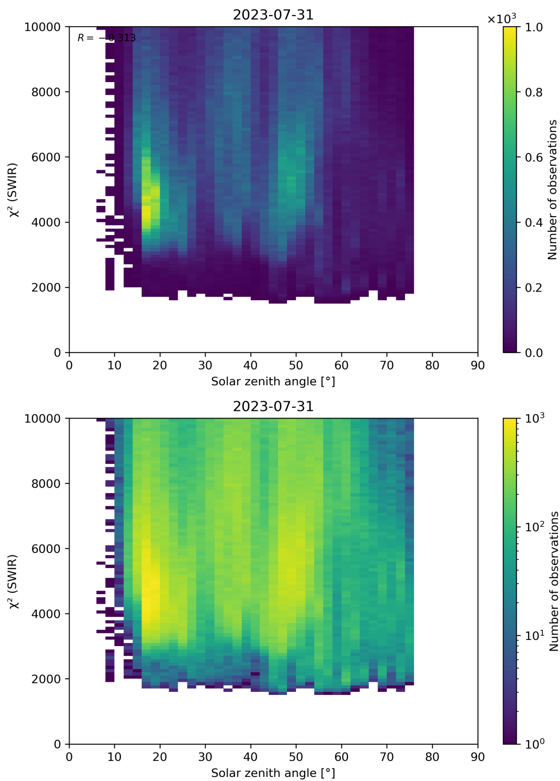
Figure 95: Scatter density plot of “Solar zenith angle” against “ \chi^2 (SWIR)” for 2023-07-30 to 2023-08-01.
