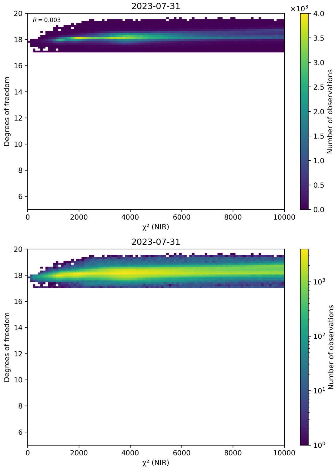
Figure 44: Scatter density plot of “ \chi^2 (NIR)” against “Degrees of freedom” for 2023-07-30 to 2023-08-01.
