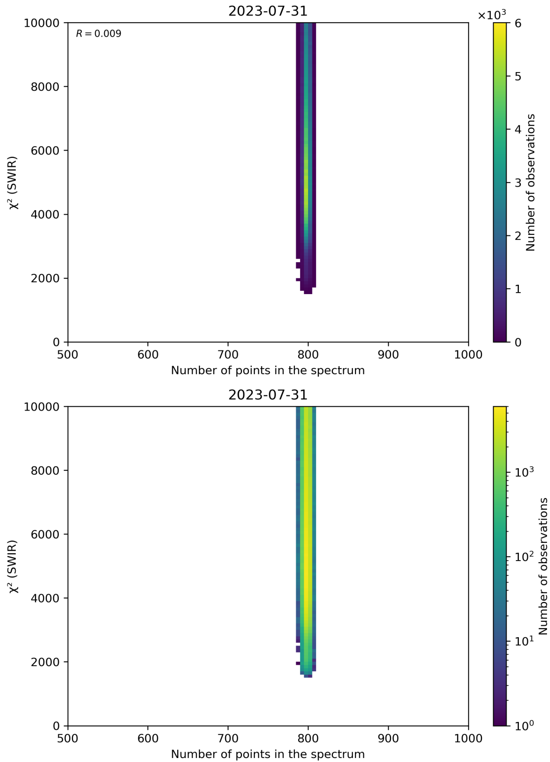
Figure 89: Scatter density plot of “Number of points in the spectrum” against “ \chi^2 (SWIR)” for 2023-07-30 to 2023-08-01.
