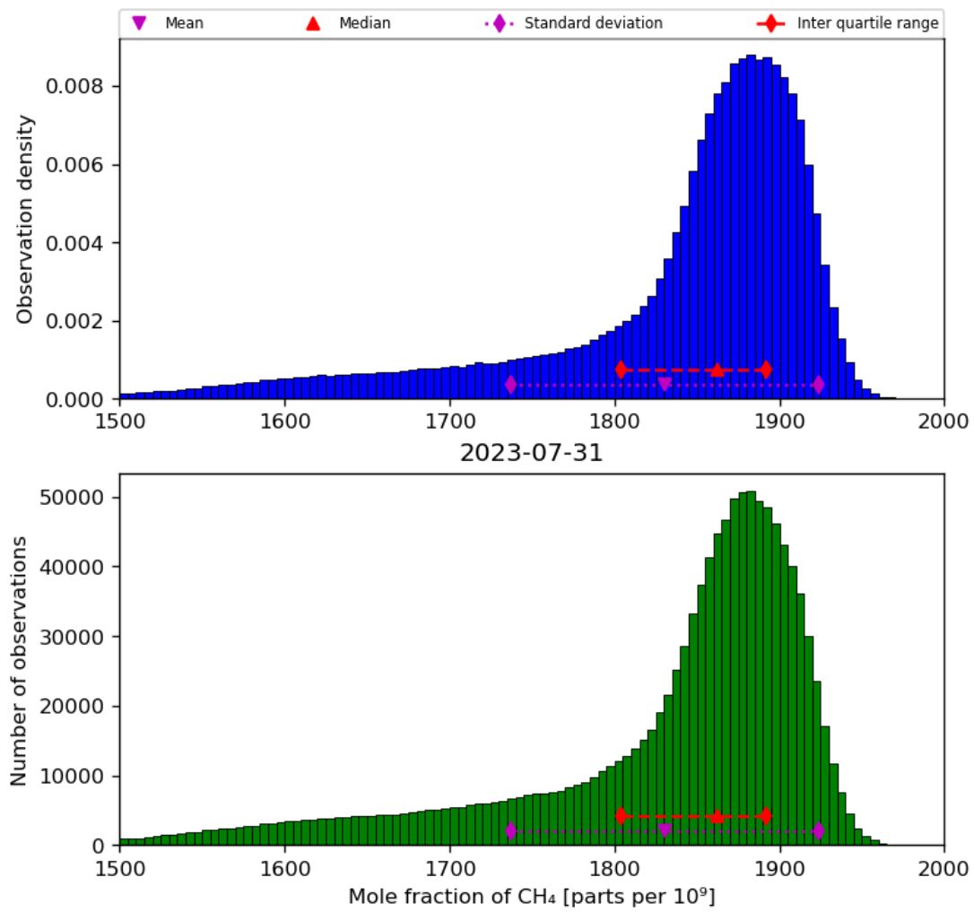
Figure 23: Histogram of “Mole fraction of CH 4 ” for 2023-07-30 to 2023-08-01
