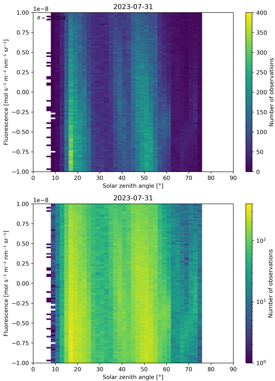
Figure 97: Scatter density plot of “Solar zenith angle” against “Fluorescence” for 2023-07-30 to 2023-08-01.
