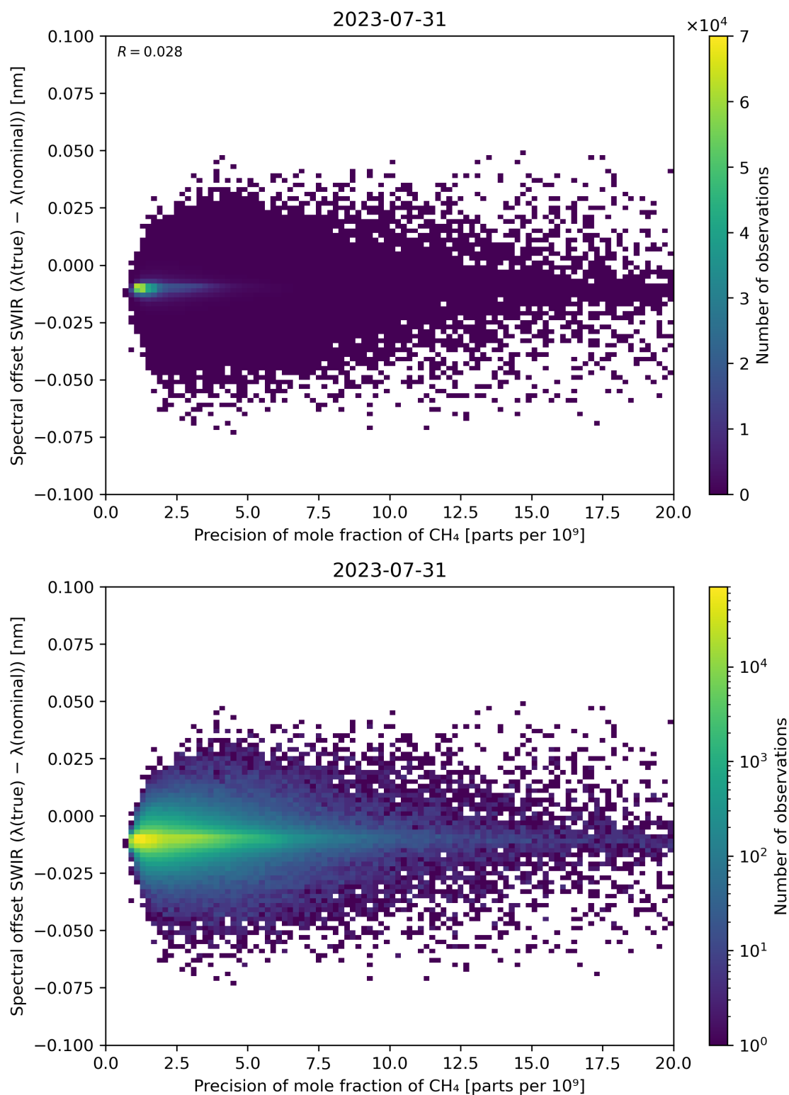
Figure 85: Scatter density plot of “Precision of mole fraction of \text{CH}_4 ” against “Spectral offset SWIR ( \lambda(\text{true}) - \lambda(\text{nominal}) )” for 2023-07-30 to 2023-08-01.
