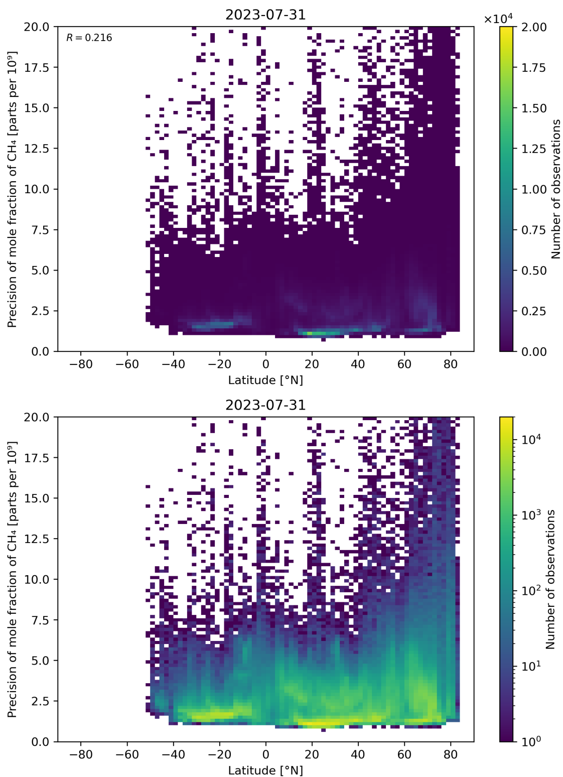
Figure 59: Scatter density plot of “Latitude” against “Precision of mole fraction of \text{CH}_4 ” for 2023-07-30 to 2023-08-01.
