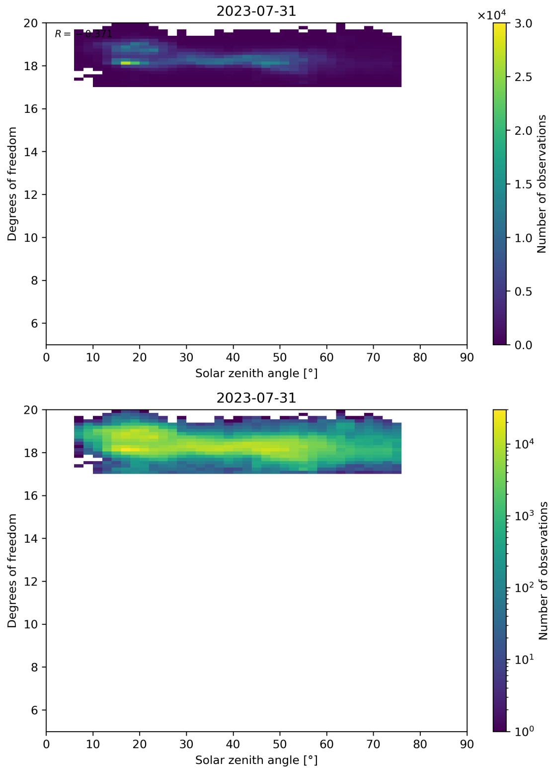
Figure 96: Scatter density plot of “Solar zenith angle” against “Degrees of freedom” for 2023-07-30 to 2023-08-01.
