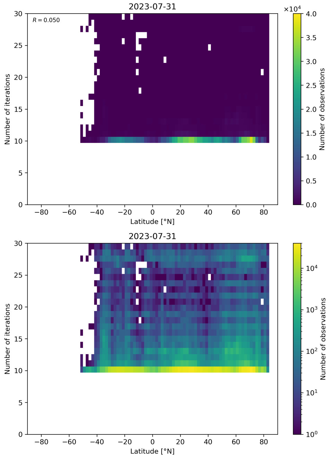
Figure 60: Scatter density plot of “Latitude” against “Number of iterations” for 2023-07-30 to 2023-08-01.
