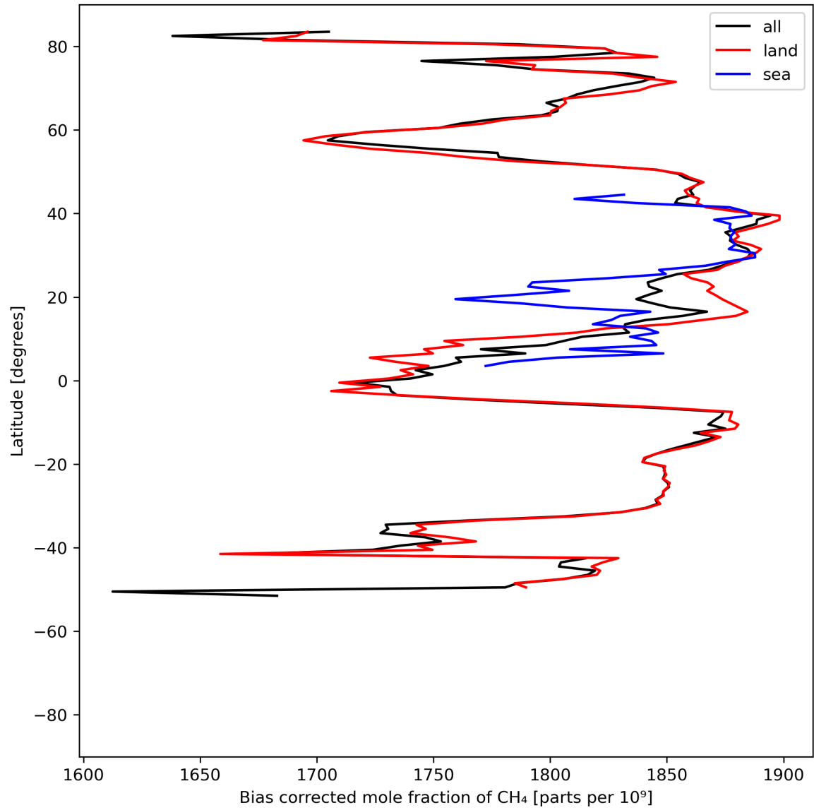
Figure 14: Zonal average of “Bias corrected mole fraction of CH 4 ” for 2023-07-30 to 2023-08-01.
