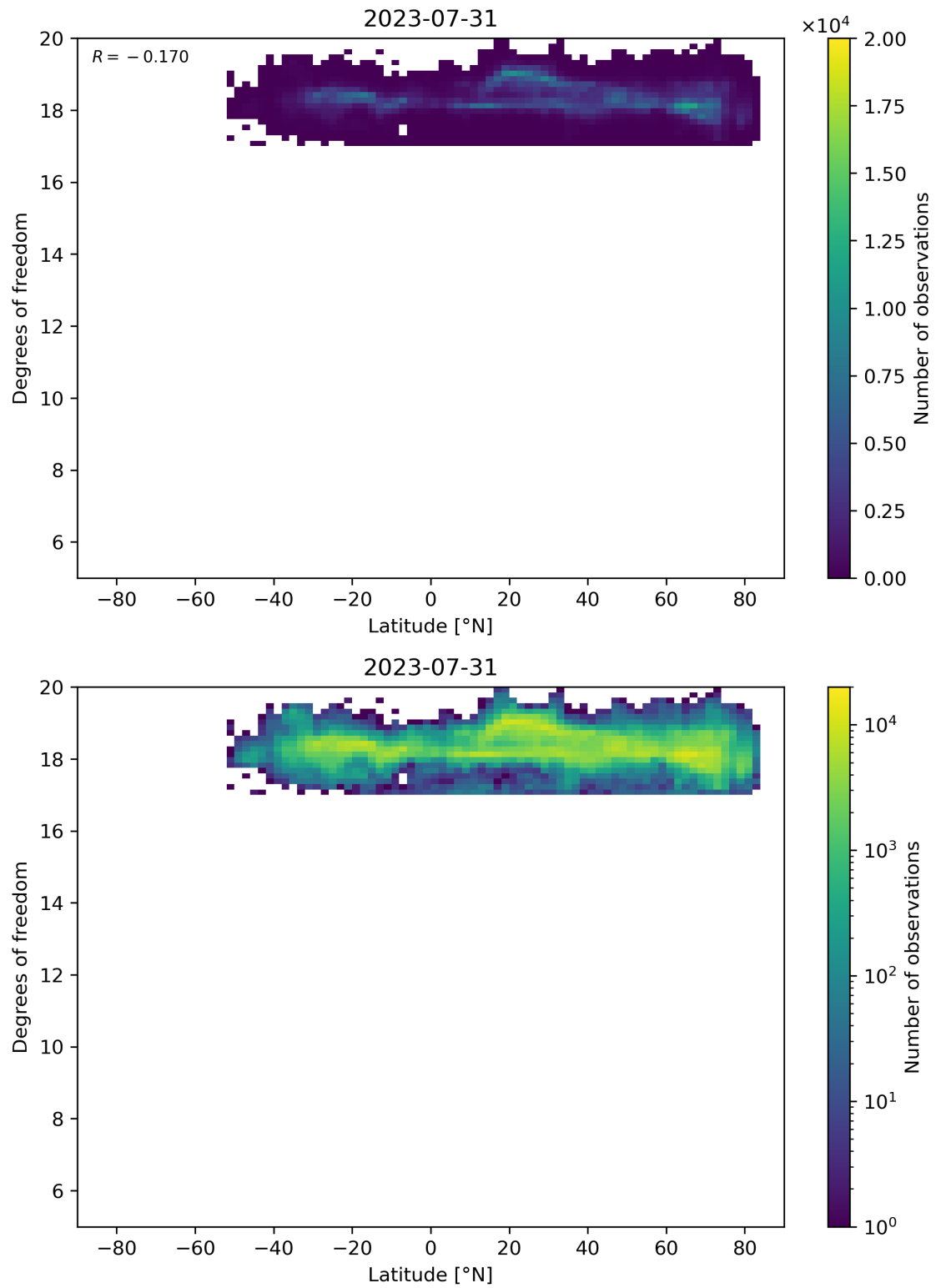
Figure 55: Scatter density plot of “Latitude” against “Degrees of freedom” for 2023-07-30 to 2023-08-01.
