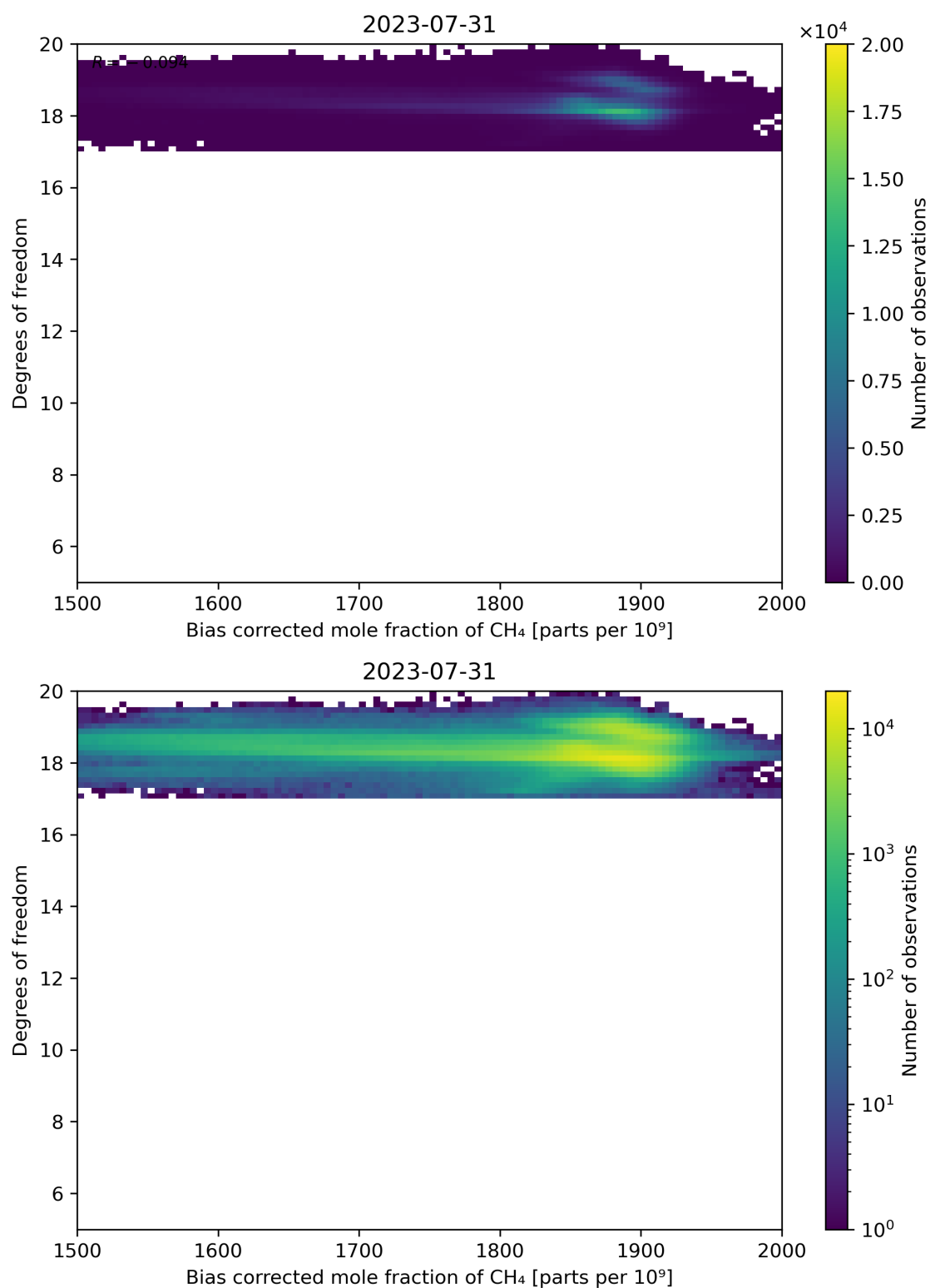
Figure 65: Scatter density plot of “Bias corrected mole fraction of CH 4 ” against “Degrees of freedom” for 2023-07-30 to 2023-08-01.
