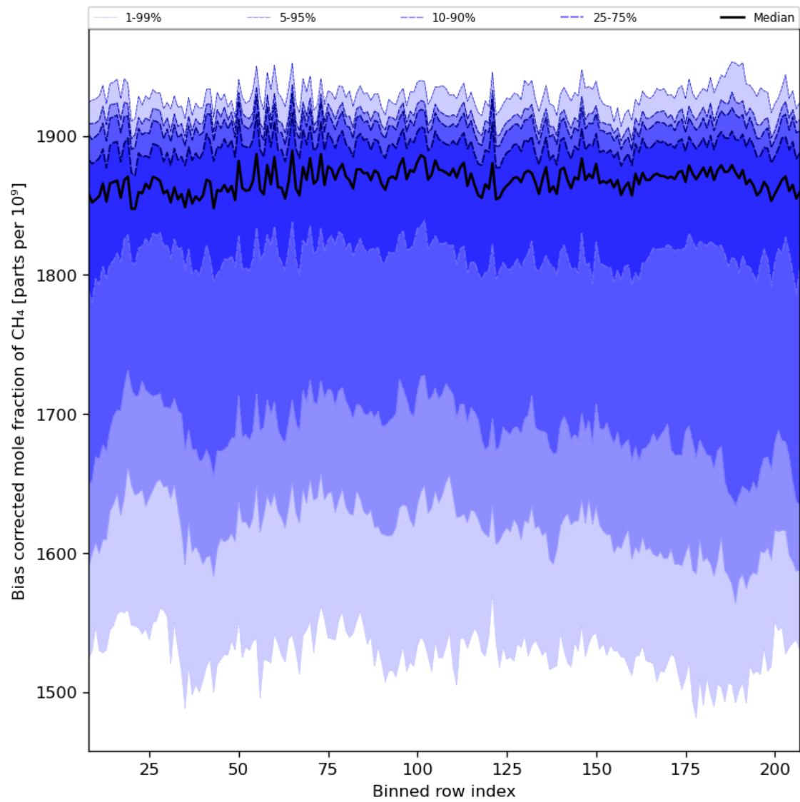
Figure 36: Along track statistics of “Bias corrected mole fraction of CH 4 ” for 2023-07-30 to 2023-08-01
