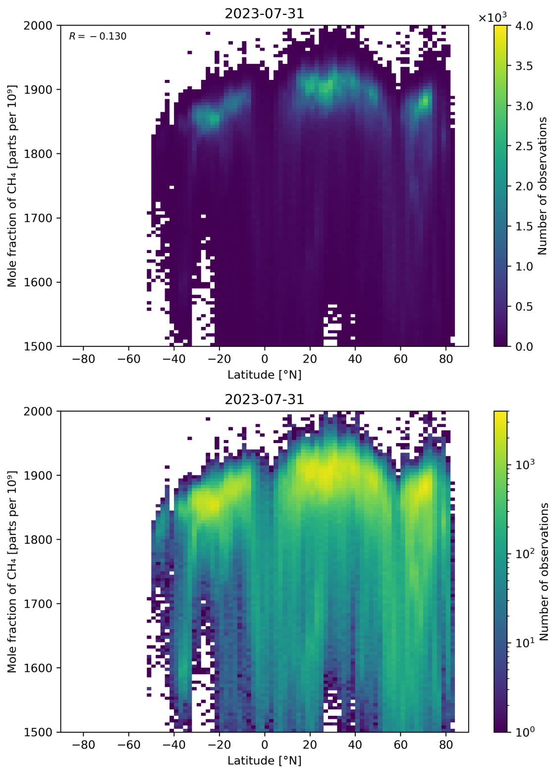
Figure 57: Scatter density plot of “Latitude” against “Mole fraction of CH 4 ” for 2023-07-30 to 2023-08-01.
