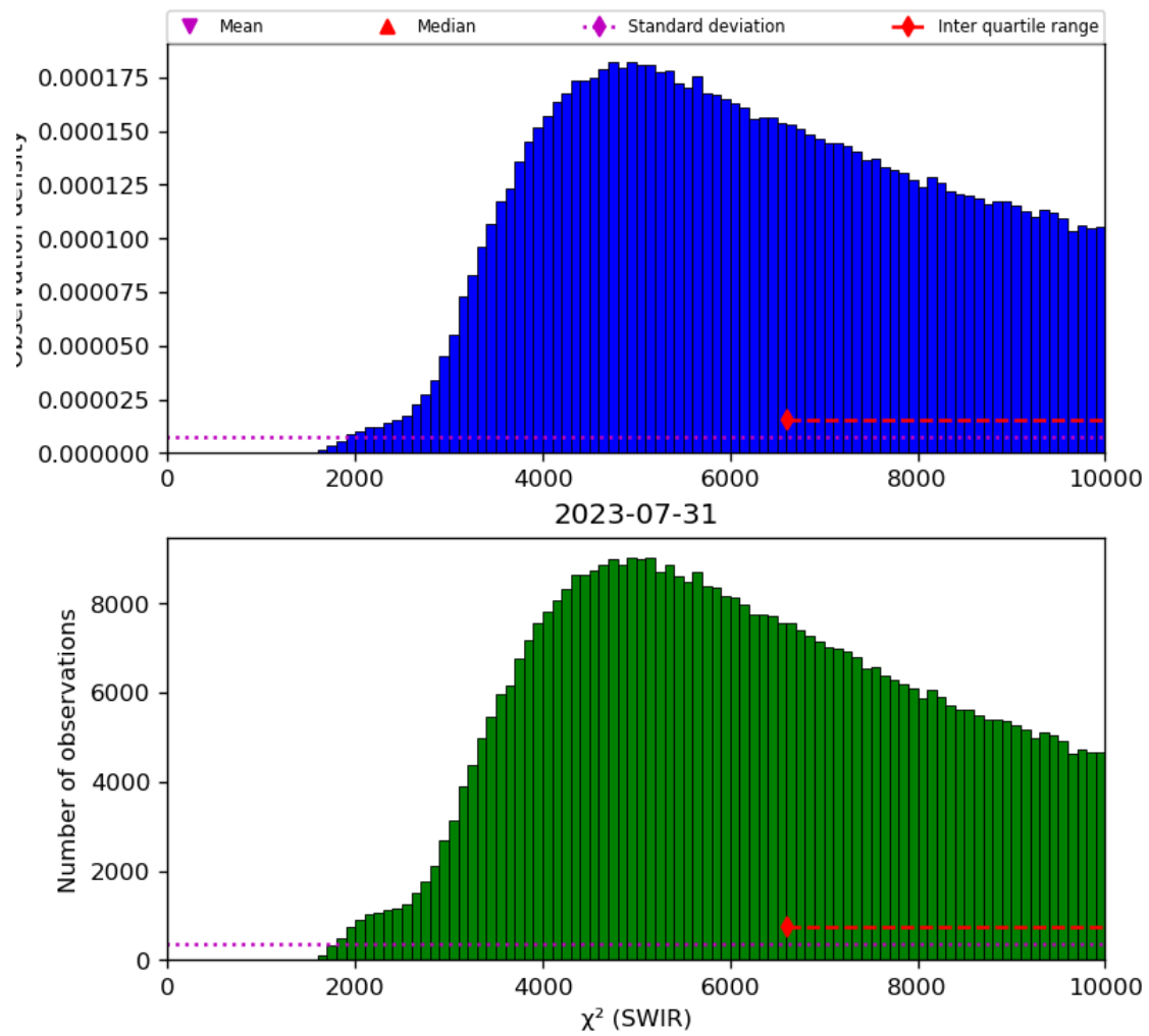
Figure 28: Histogram of “ \chi^2 (SWIR)” for 2023-07-30 to 2023-08-01
