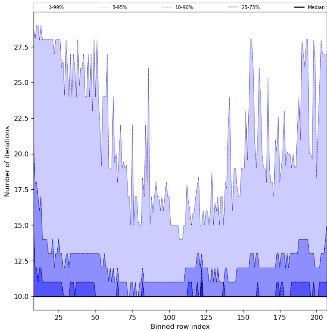
Figure 42: Along track statistics of “Number of iterations” for 2023-07-30 to 2023-08-01
