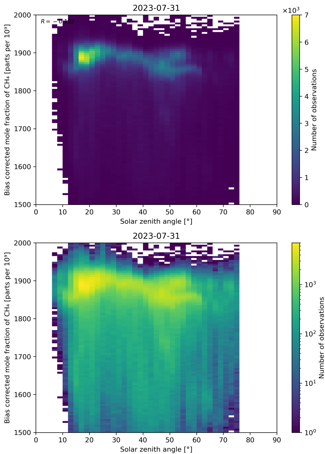
Figure 100: Scatter density plot of “Solar zenith angle” against “Bias corrected mole fraction of CH 4 ” for 2023-07-30 to 2023-08-01.
