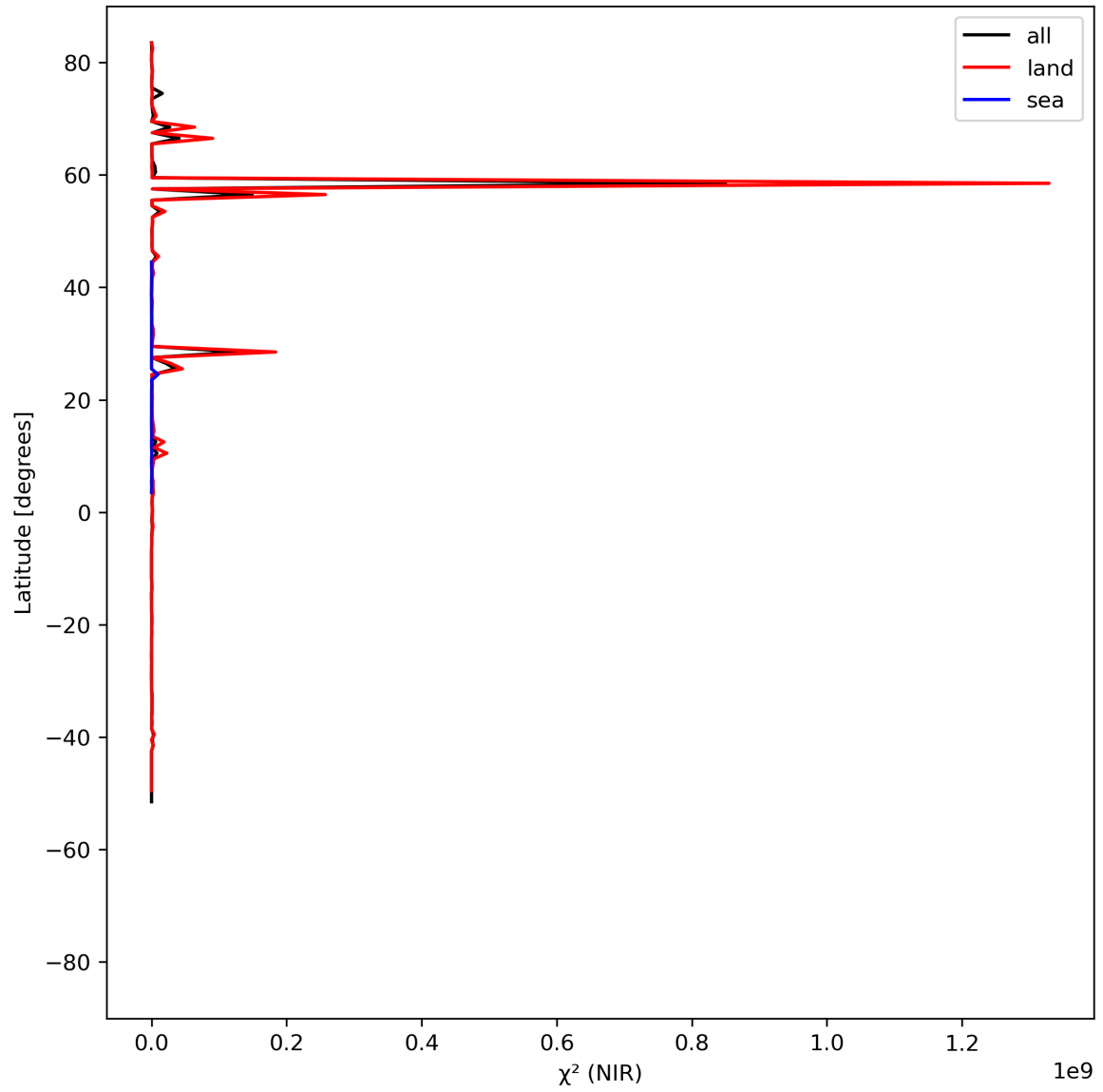
Figure 18: Zonal average of “ \chi^2 (NIR)” for 2023-07-30 to 2023-08-01.
