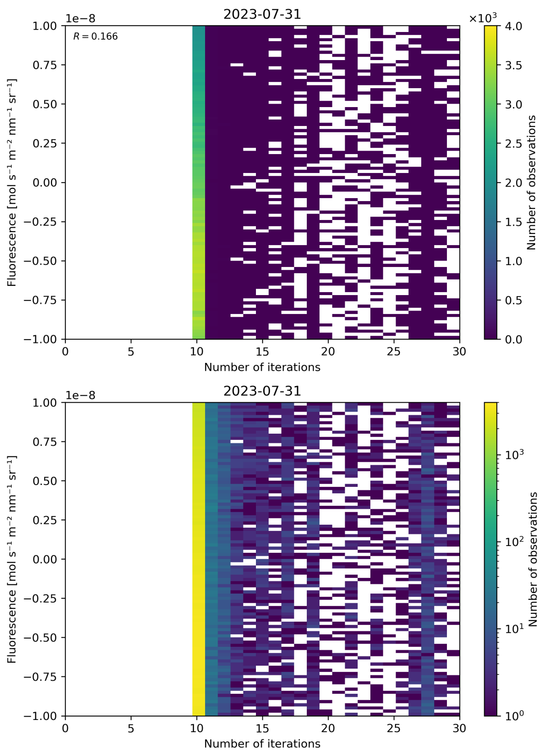
Figure 87: Scatter density plot of “Number of iterations” against “Fluorescence” for 2023-07-30 to 2023-08-01.
