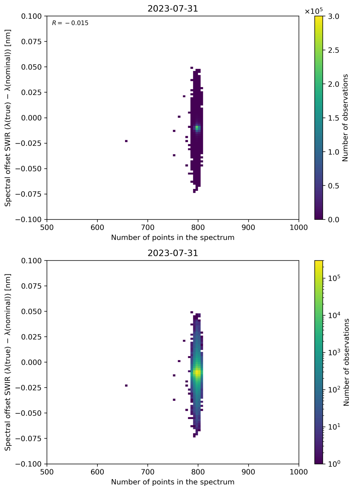
Figure 93: Scatter density plot of “Number of points in the spectrum” against “Spectral offset SWIR ( \lambda(\text{true}) - \lambda(\text{nominal}) )” for 2023-07-30 to 2023-08-01.
