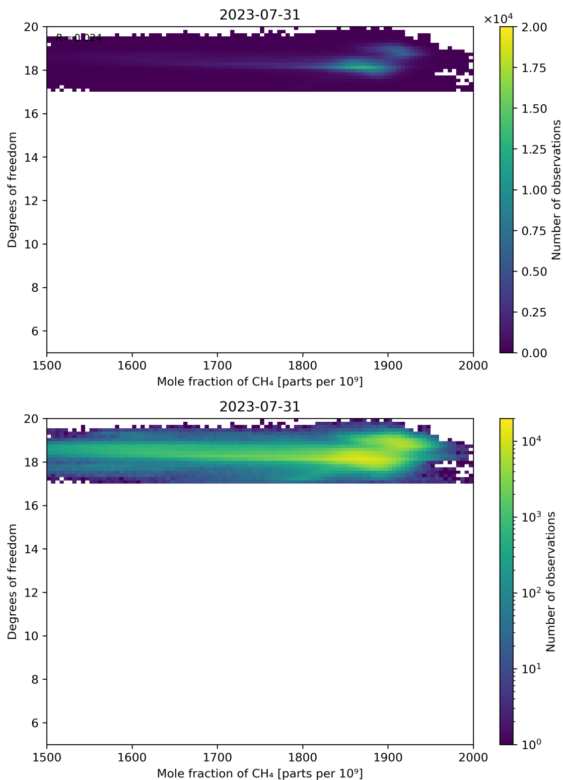
Figure 72: Scatter density plot of “Mole fraction of CH 4 ” against “Degrees of freedom” for 2023-07-30 to 2023-08-01.
