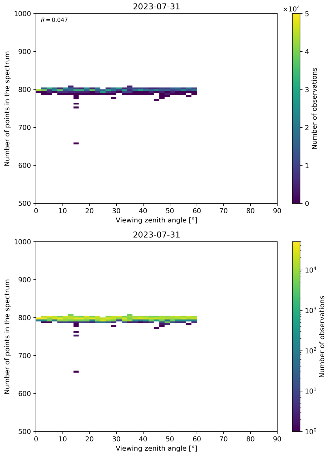
Figure 114: Scatter density plot of “Viewing zenith angle” against “Number of points in the spectrum” for 2023-07-30 to 2023-08-01.
