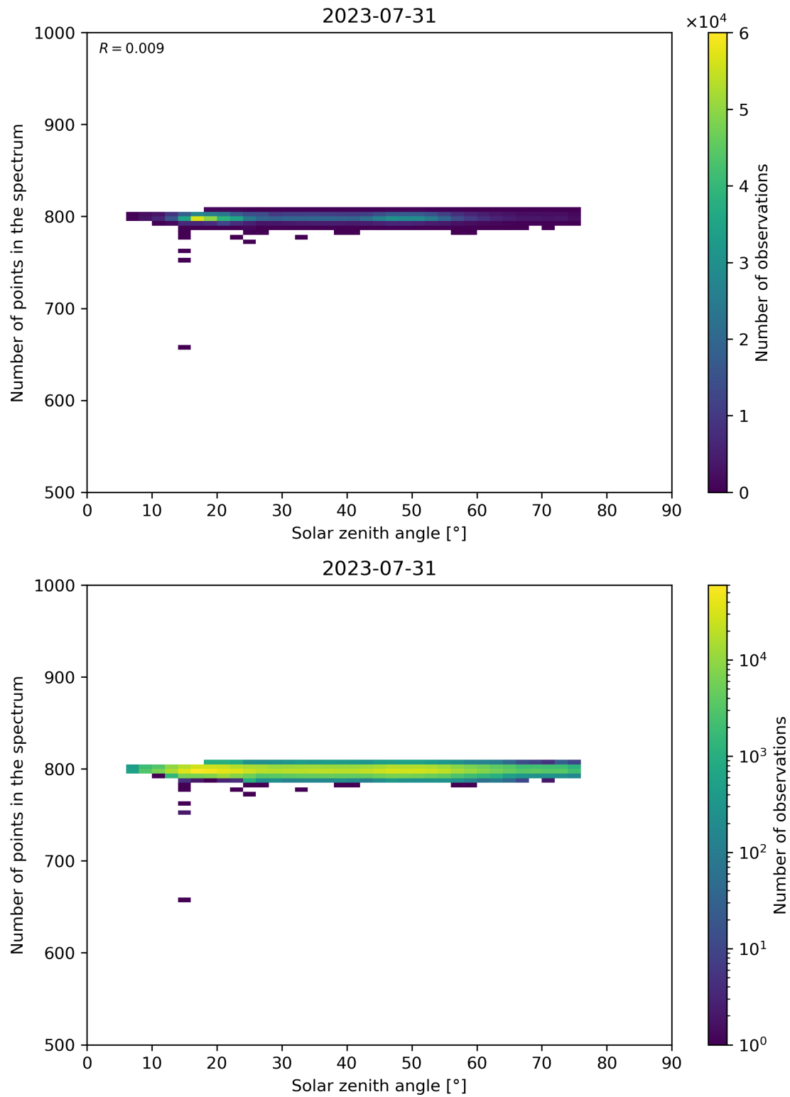
Figure 103: Scatter density plot of “Solar zenith angle” against “Number of points in the spectrum” for 2023-07-30 to 2023-08-01.
