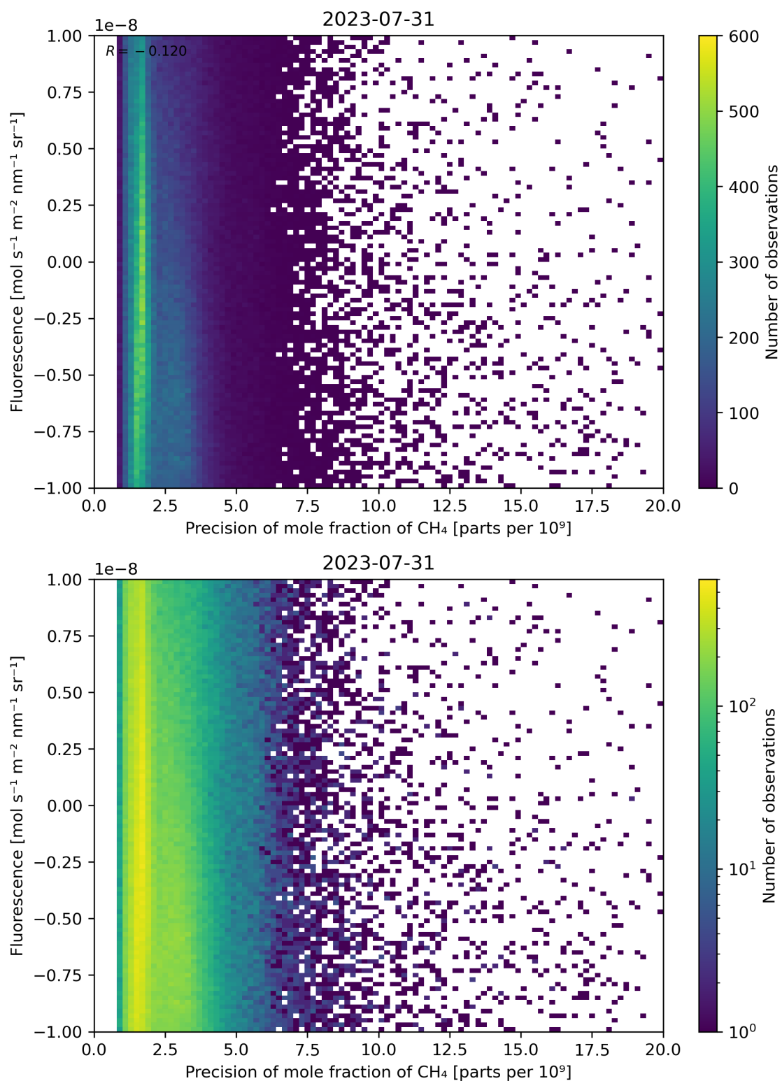
Figure 81: Scatter density plot of “Precision of mole fraction of \text{CH}_4 ” against “Fluorescence” for 2023-07-30 to 2023-08-01.
