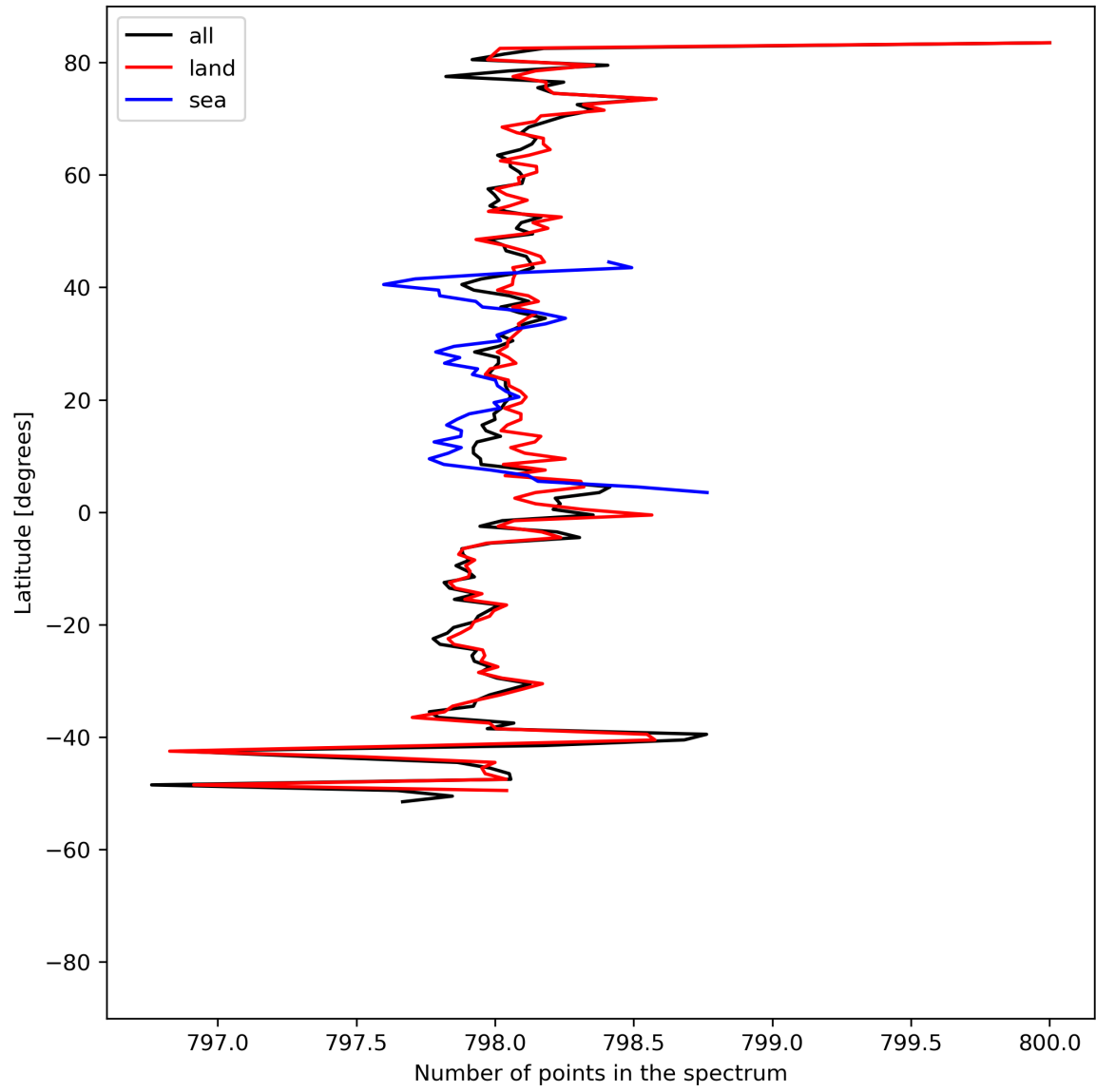
Figure 15: Zonal average of “Number of points in the spectrum” for 2023-07-30 to 2023-08-01.
