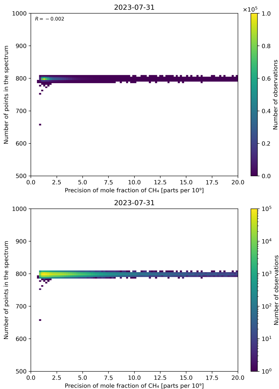
Figure 84: Scatter density plot of “Precision of mole fraction of CH 4 ” against “Number of points in the spectrum” for 2023-07-30 to 2023-08-01.
