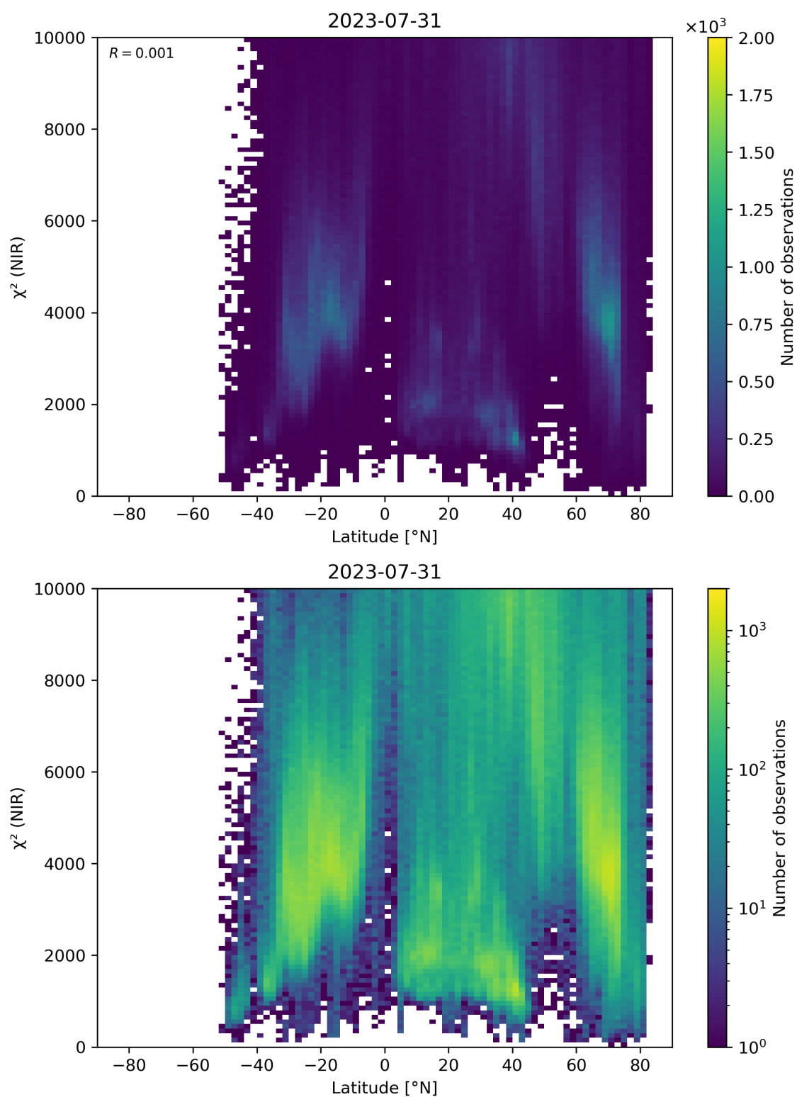
Figure 53: Scatter density plot of “Latitude” against “ \chi^2 (NIR)” for 2023-07-30 to 2023-08-01.
