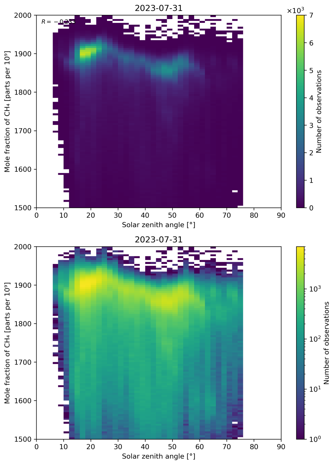
Figure 99: Scatter density plot of “Solar zenith angle” against “Mole fraction of CH 4 ” for 2023-07-30 to 2023-08-01.
