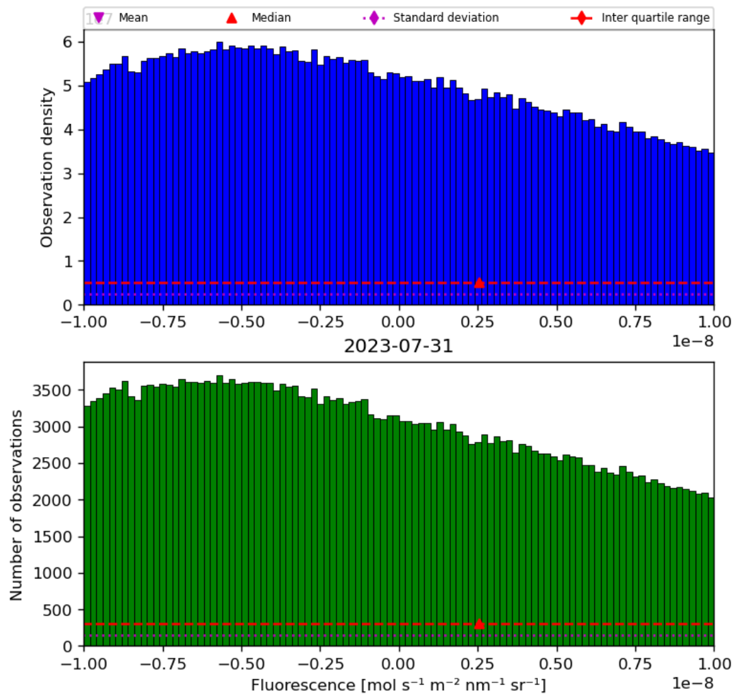
Figure 32: Histogram of “Fluorescence” for 2023-07-30 to 2023-08-01
