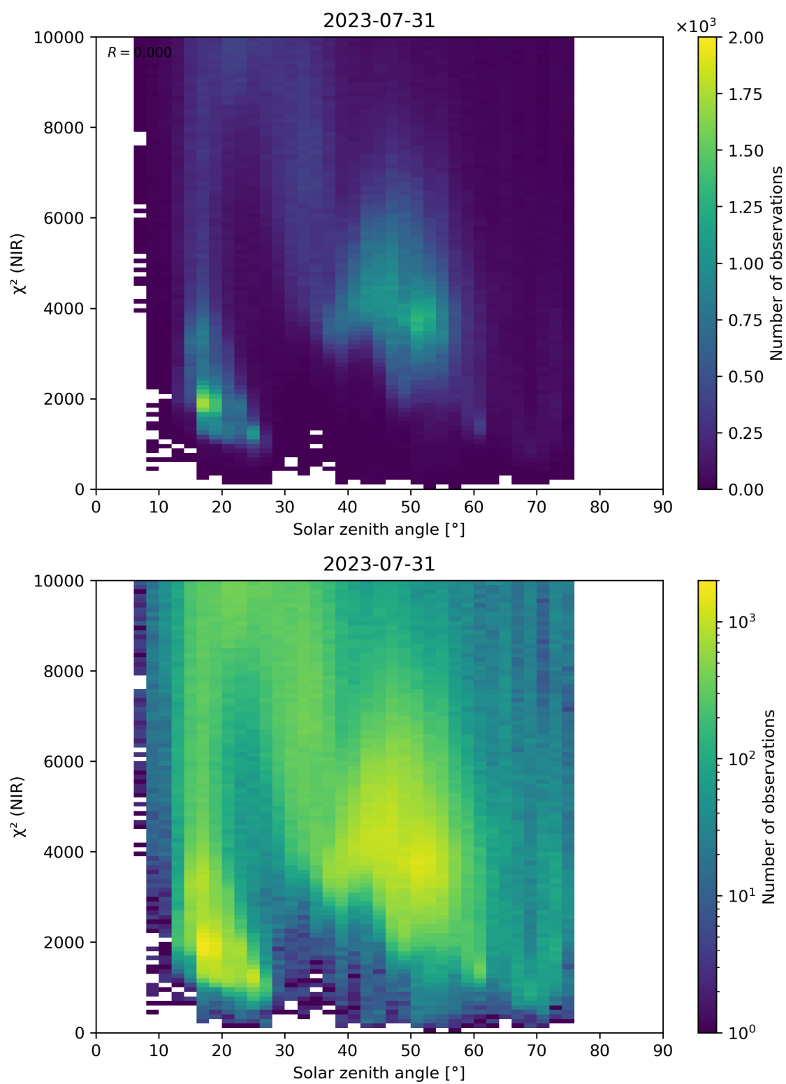
Figure 94: Scatter density plot of “Solar zenith angle” against “ \chi^2 (NIR)” for 2023-07-30 to 2023-08-01.
