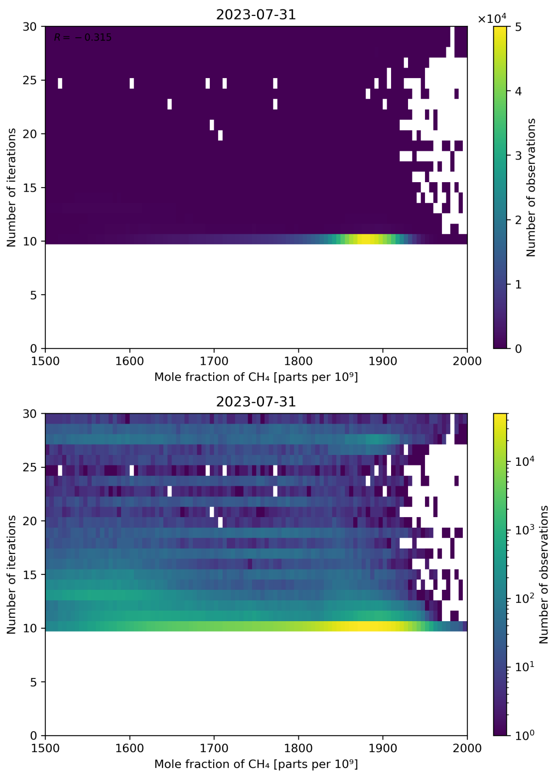
Figure 76: Scatter density plot of “Mole fraction of CH 4 ” against “Number of iterations” for 2023-07-30 to 2023-08-01.
