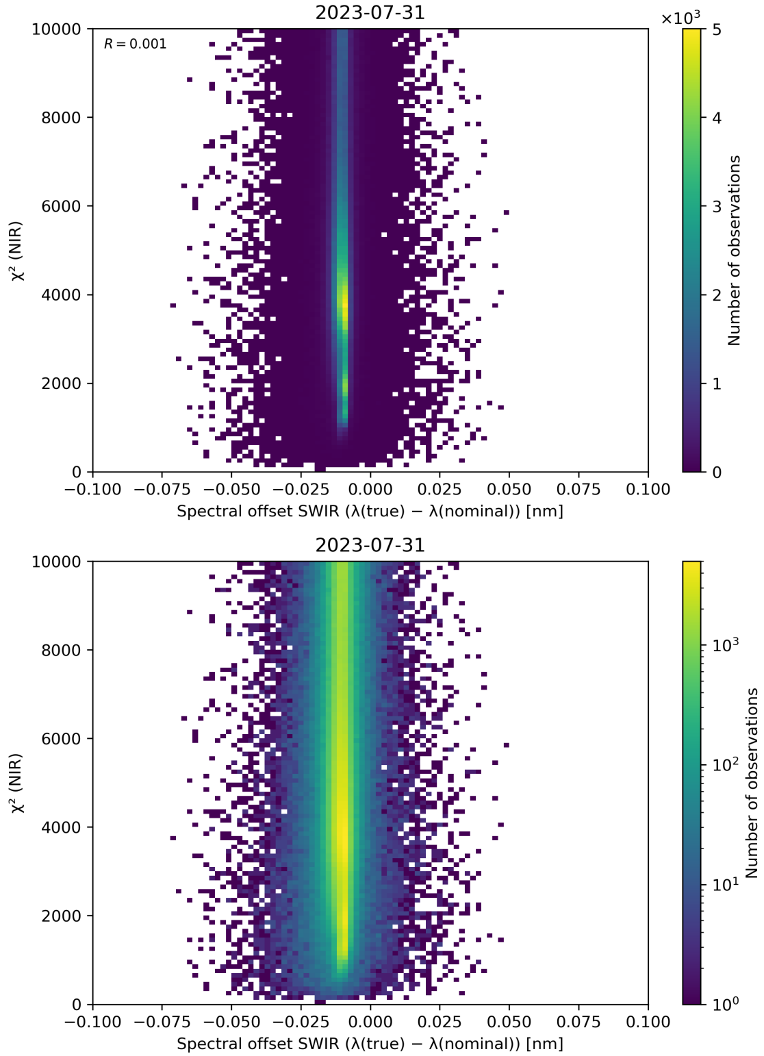
Figure 117: Scatter density plot of “Spectral offset SWIR ( \lambda(\text{true}) - \lambda(\text{nominal}) )” against “ \chi^2 (NIR)” for 2023-07-30 to 2023-08-01.
