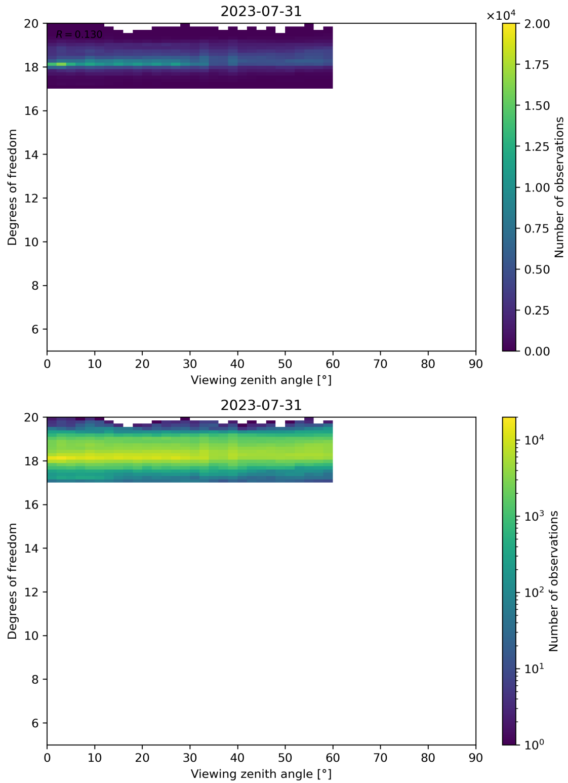
Figure 107: Scatter density plot of “Viewing zenith angle” against “Degrees of freedom” for 2023-07-30 to 2023-08-01.
