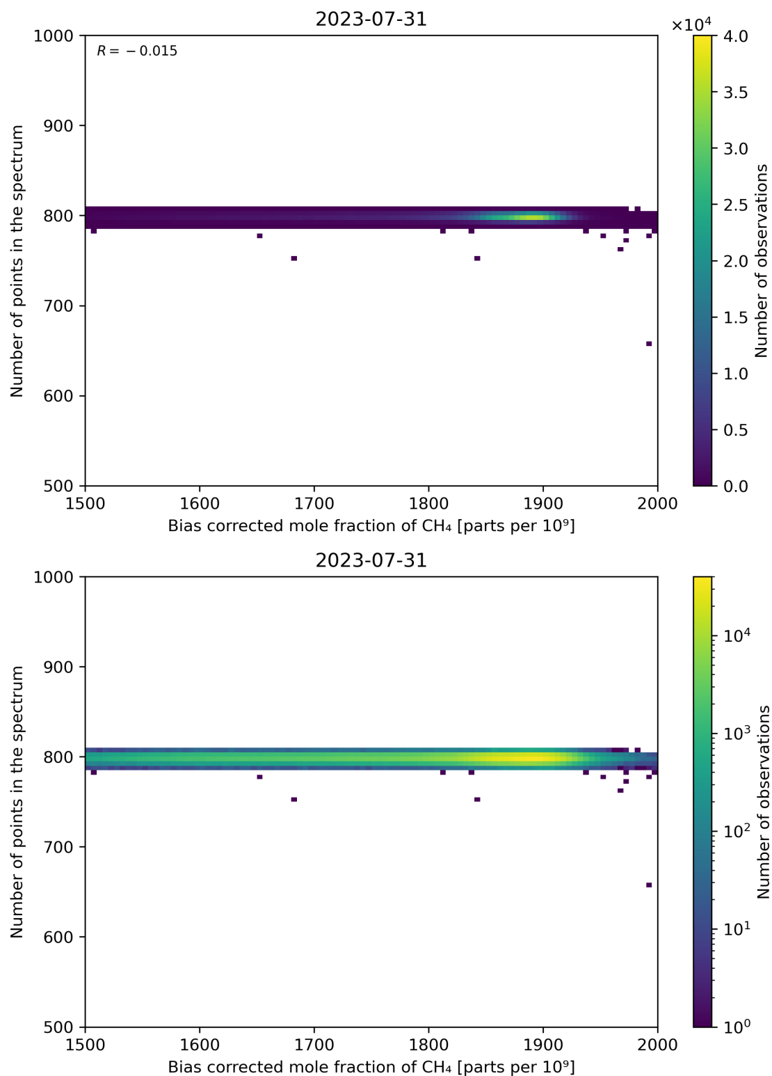
Figure 68: Scatter density plot of “Bias corrected mole fraction of CH 4 ” against “Number of points in the spectrum” for 2023-07-30 to 2023-08-01.
