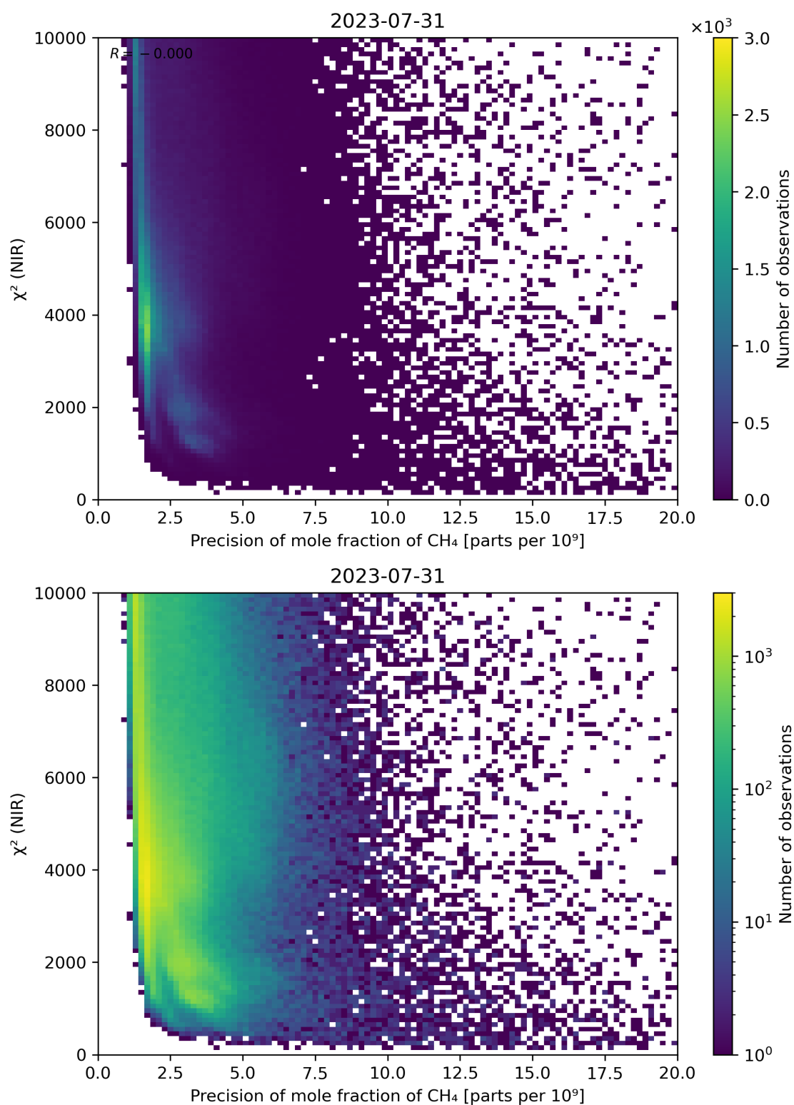
Figure 78: Scatter density plot of “Precision of mole fraction of CH 4 ” against “ \chi^2 (NIR)” for 2023-07-30 to 2023-08-01.
