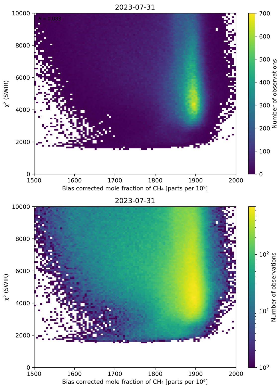
Figure 64: Scatter density plot of “Bias corrected mole fraction of CH 4 ” against “ \chi^2 (SWIR)” for 2023-07-30 to 2023-08-01.
