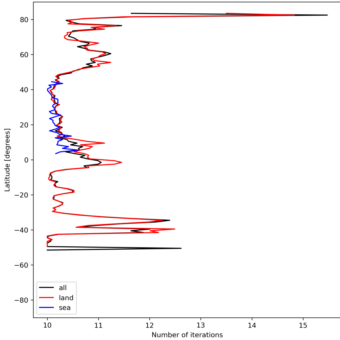
Figure 20: Zonal average of “Number of iterations” for 2023-07-30 to 2023-08-01.
