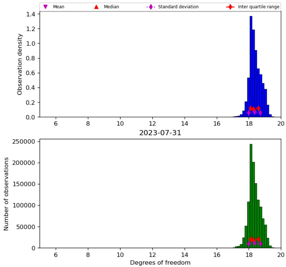
Figure 30: Histogram of “Degrees of freedom” for 2023-07-30 to 2023-08-01
