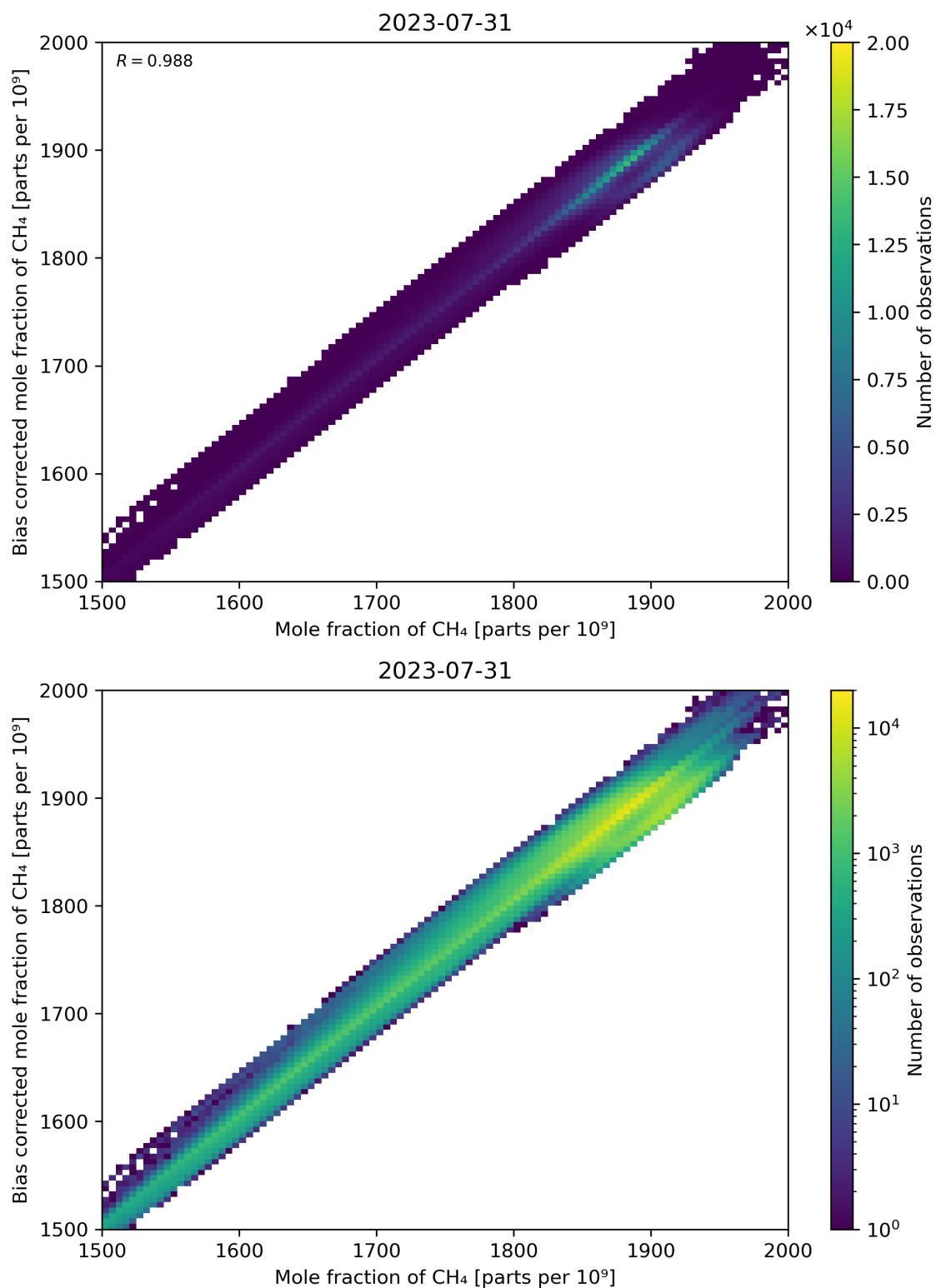
Figure 74: Scatter density plot of “Mole fraction of CH 4 ” against “Bias corrected mole fraction of CH 4 ” for 2023-07-30 to 2023-08-01.
