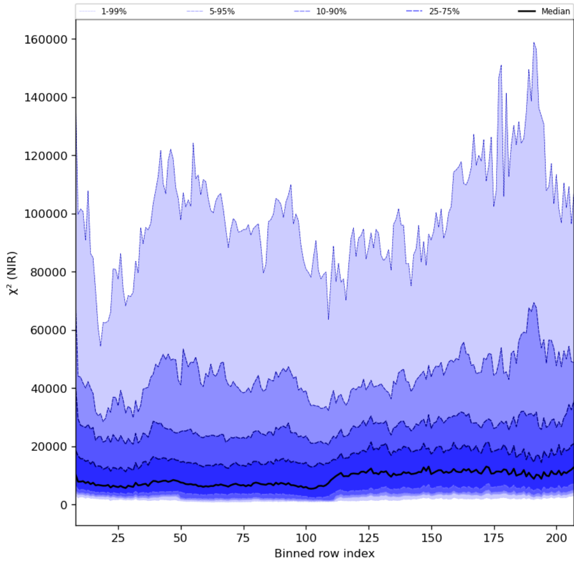
Figure 40: Along track statistics of " \chi^2 (NIR)" for 2023-07-30 to 2023-08-01
