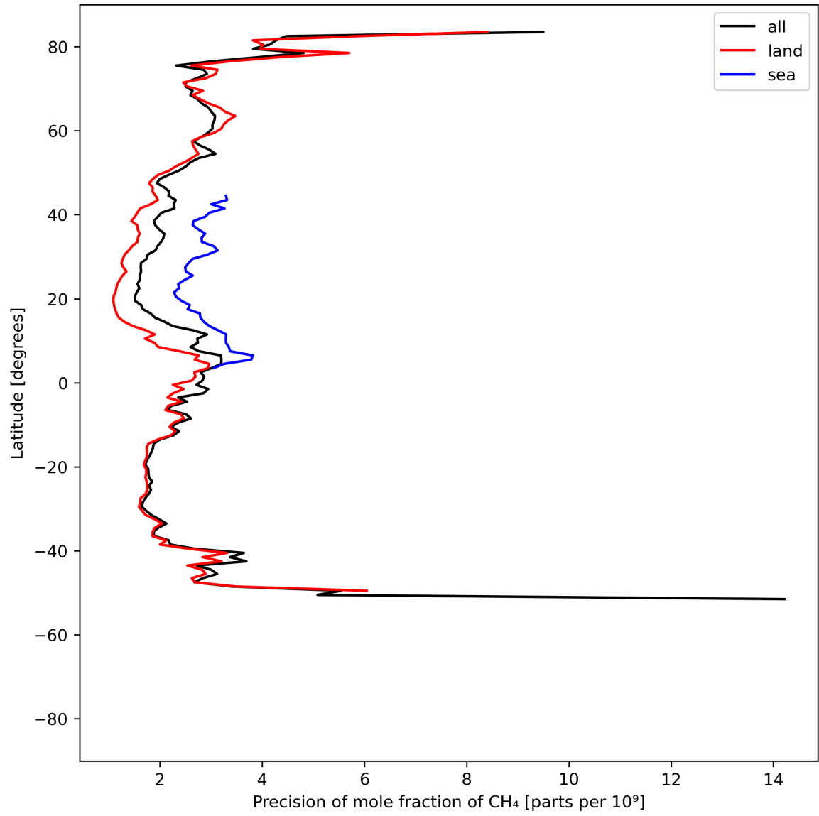
Figure 13: Zonal average of “Precision of mole fraction of CH 4 ” for 2023-07-30 to 2023-08-01.
