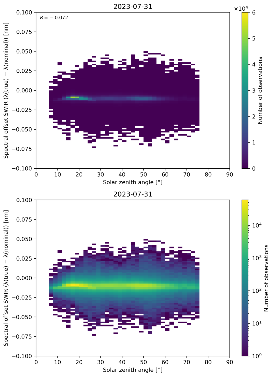
Figure 104: Scatter density plot of “Solar zenith angle” against “Spectral offset SWIR ( \lambda(\text{true}) - \lambda(\text{nominal}) )” for 2023-07-30 to 2023-08-01.
