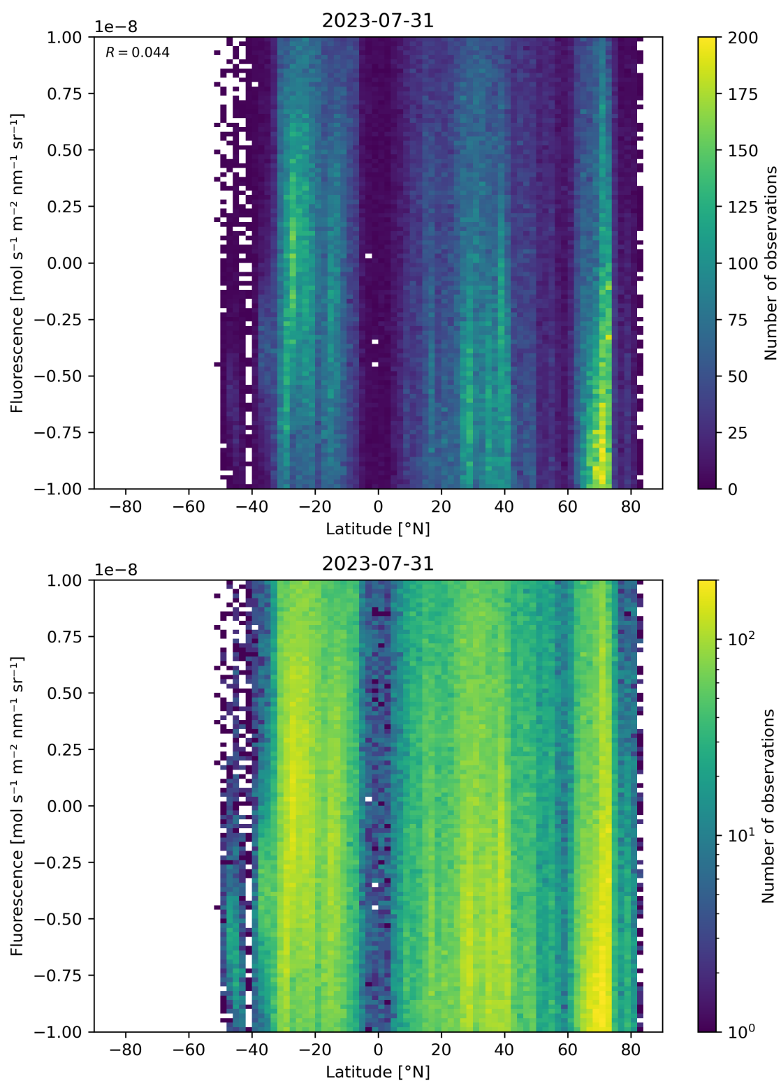
Figure 56: Scatter density plot of “Latitude” against “Fluorescence” for 2023-07-30 to 2023-08-01.
