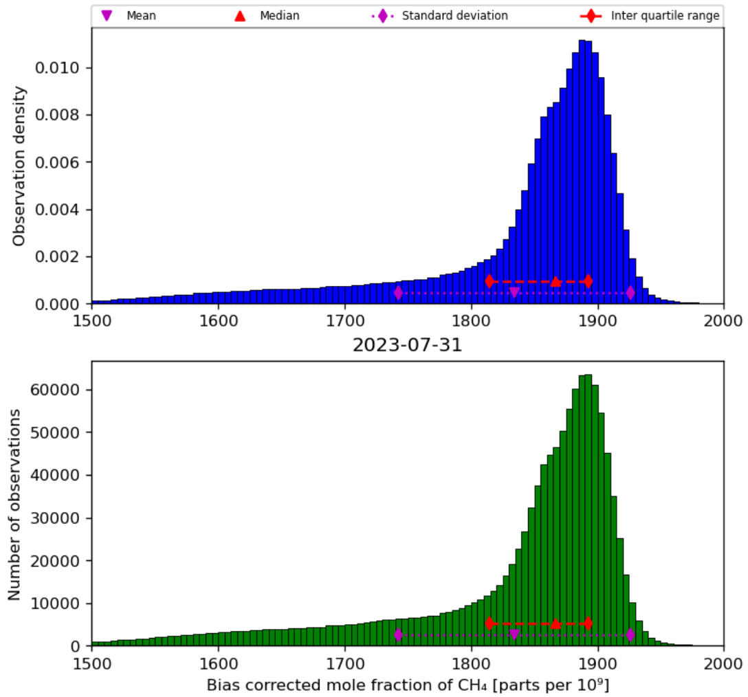
Figure 25: Histogram of “Bias corrected mole fraction of CH 4 ” for 2023-07-30 to 2023-08-01
