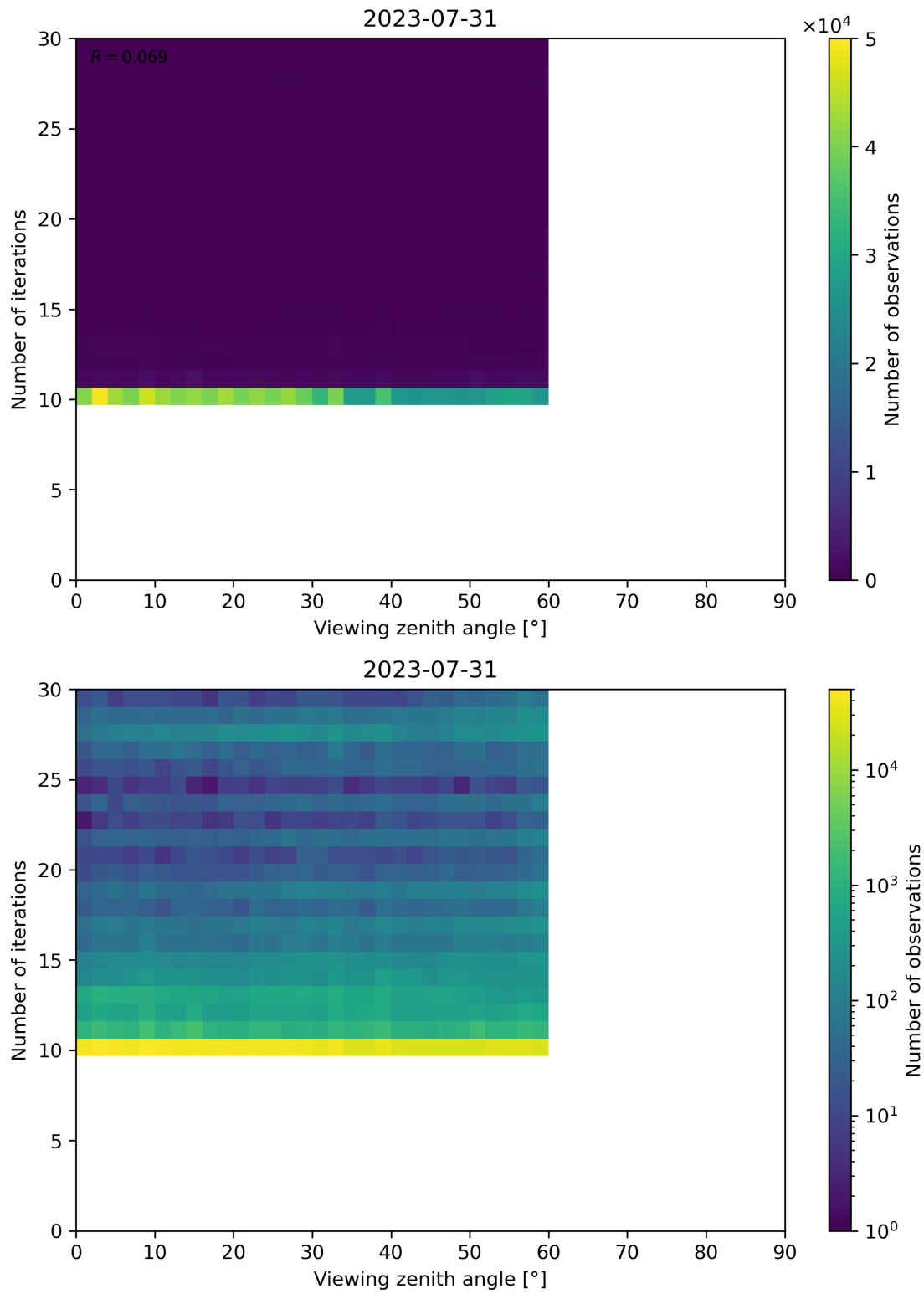
Figure 113: Scatter density plot of “Viewing zenith angle” against “Number of iterations” for 2023-07-30 to 2023-08-01.
