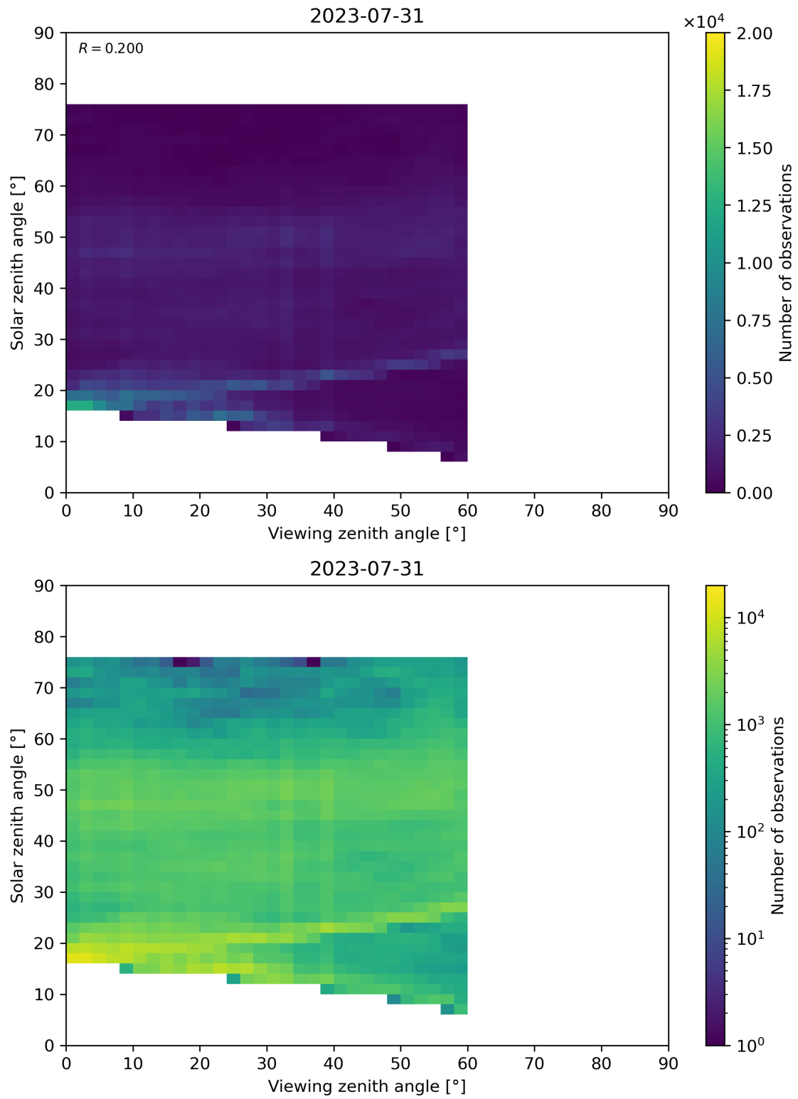
Figure 115: Scatter density plot of “Viewing zenith angle” against “Solar zenith angle” for 2023-07-30 to 2023-08-01.
