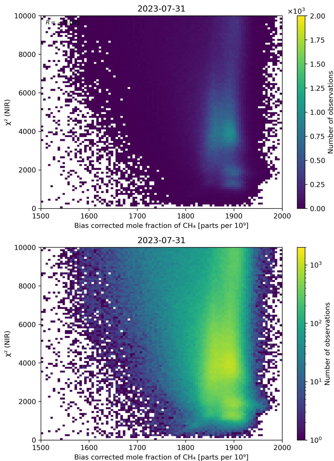
Figure 63: Scatter density plot of “Bias corrected mole fraction of CH 4 ” against “ \chi^2 (NIR)” for 2023-07-30 to 2023-08-01.
