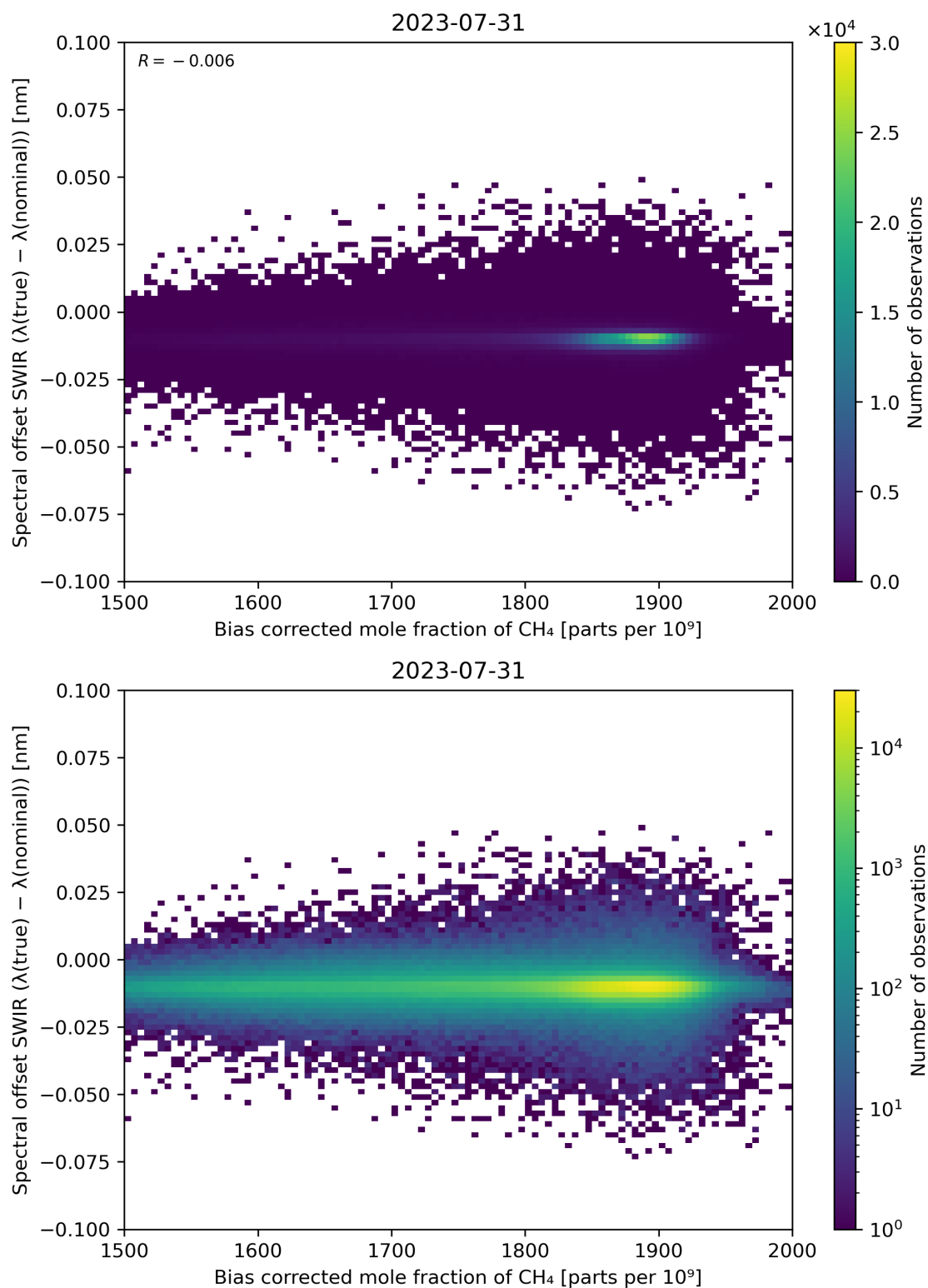
Figure 69: Scatter density plot of “Bias corrected mole fraction of \text{CH}_4 ” against “Spectral offset SWIR ( \lambda(\text{true}) - \lambda(\text{nominal}) )” for 2023-07-30 to 2023-08-01.
