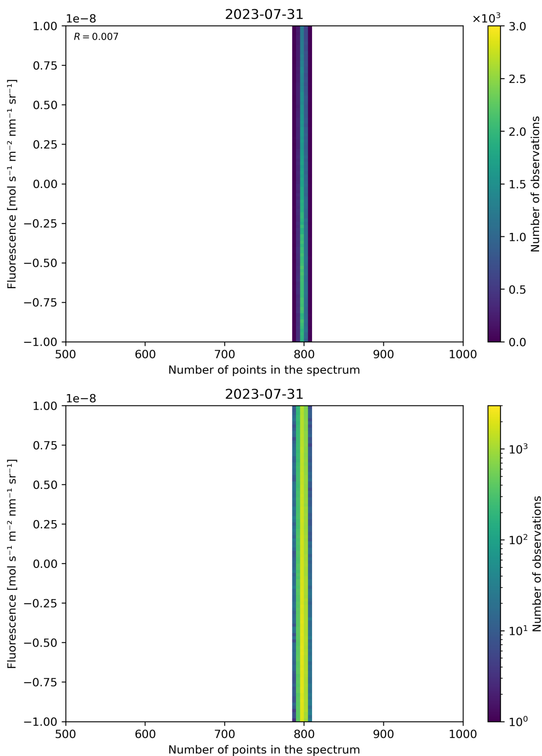
Figure 91: Scatter density plot of “Number of points in the spectrum” against “Fluorescence” for 2023-07-30 to 2023-08-01.
