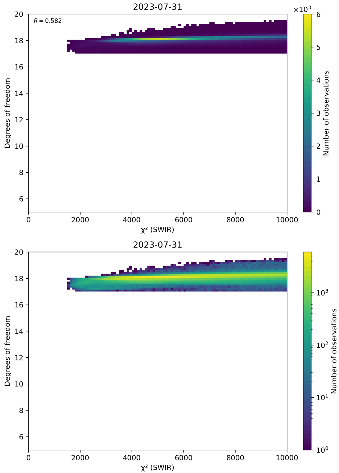
Figure 48: Scatter density plot of " \chi^2 (SWIR)" against "Degrees of freedom" for 2023-07-30 to 2023-08-01.
