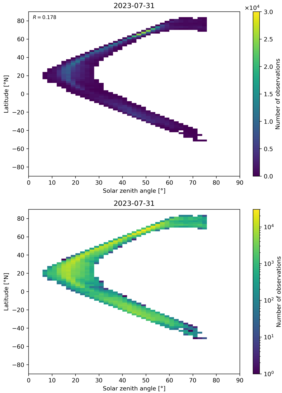
Figure 98: Scatter density plot of “Solar zenith angle” against “Latitude” for 2023-07-30 to 2023-08-01.
