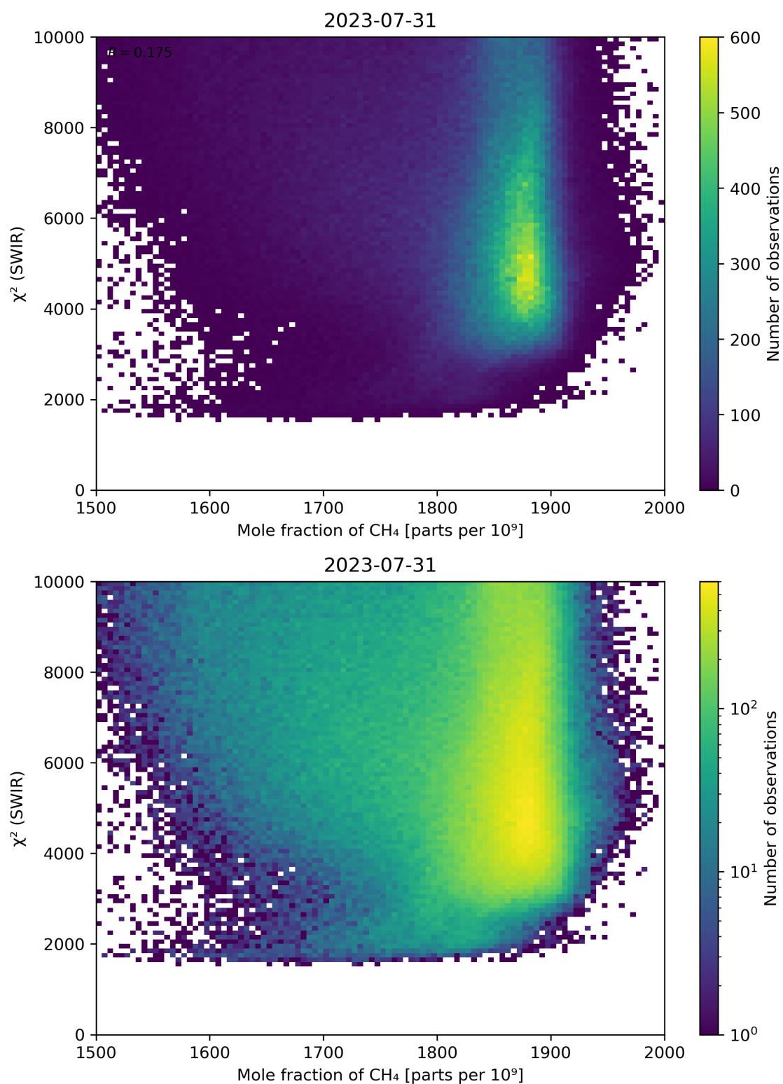
Figure 71: Scatter density plot of “Mole fraction of \text{CH}_4 ” against “ \chi^2 (SWIR)” for 2023-07-30 to 2023-08-01.
