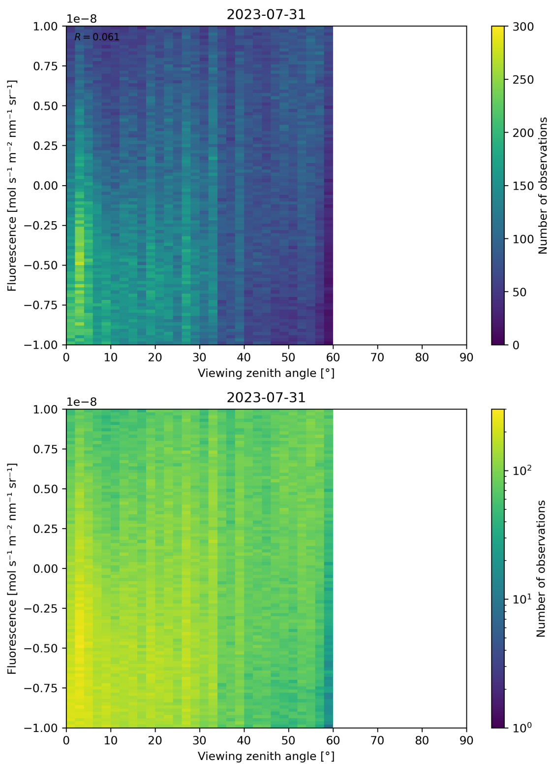
Figure 108: Scatter density plot of “Viewing zenith angle” against “Fluorescence” for 2023-07-30 to 2023-08-01.
