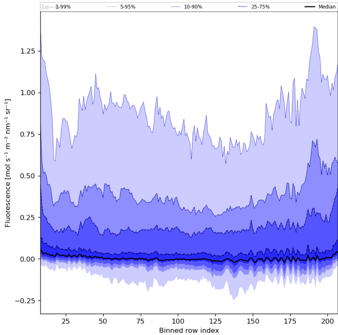
Figure 43: Along track statistics of “Fluorescence” for 2023-07-30 to 2023-08-01
