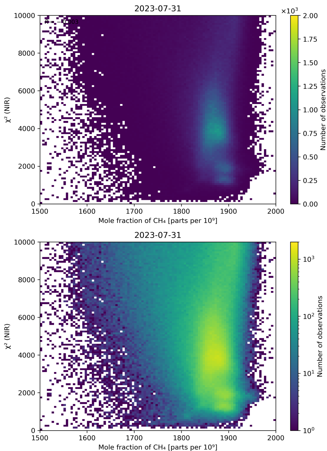
Figure 70: Scatter density plot of “Mole fraction of CH 4 ” against “ \chi^2 (NIR)” for 2023-07-30 to 2023-08-01.
