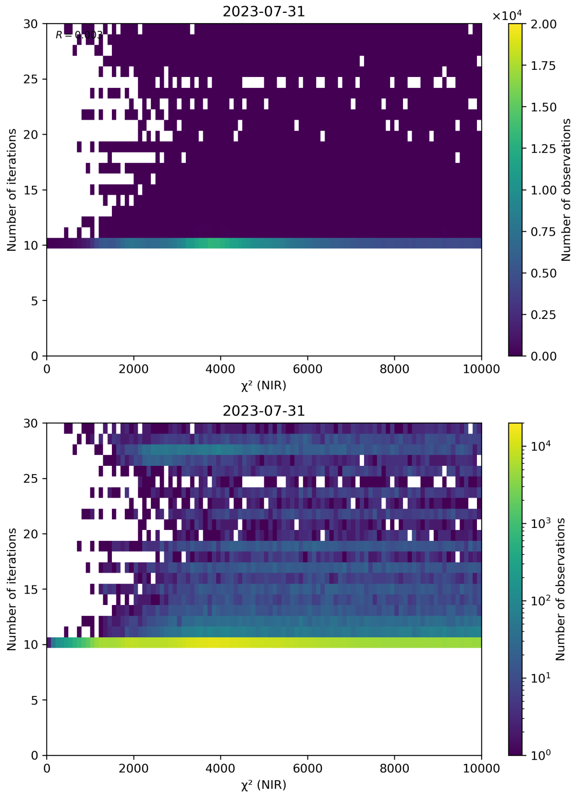
Figure 46: Scatter density plot of “ \chi^2 (NIR)” against “Number of iterations” for 2023-07-30 to 2023-08-01.
