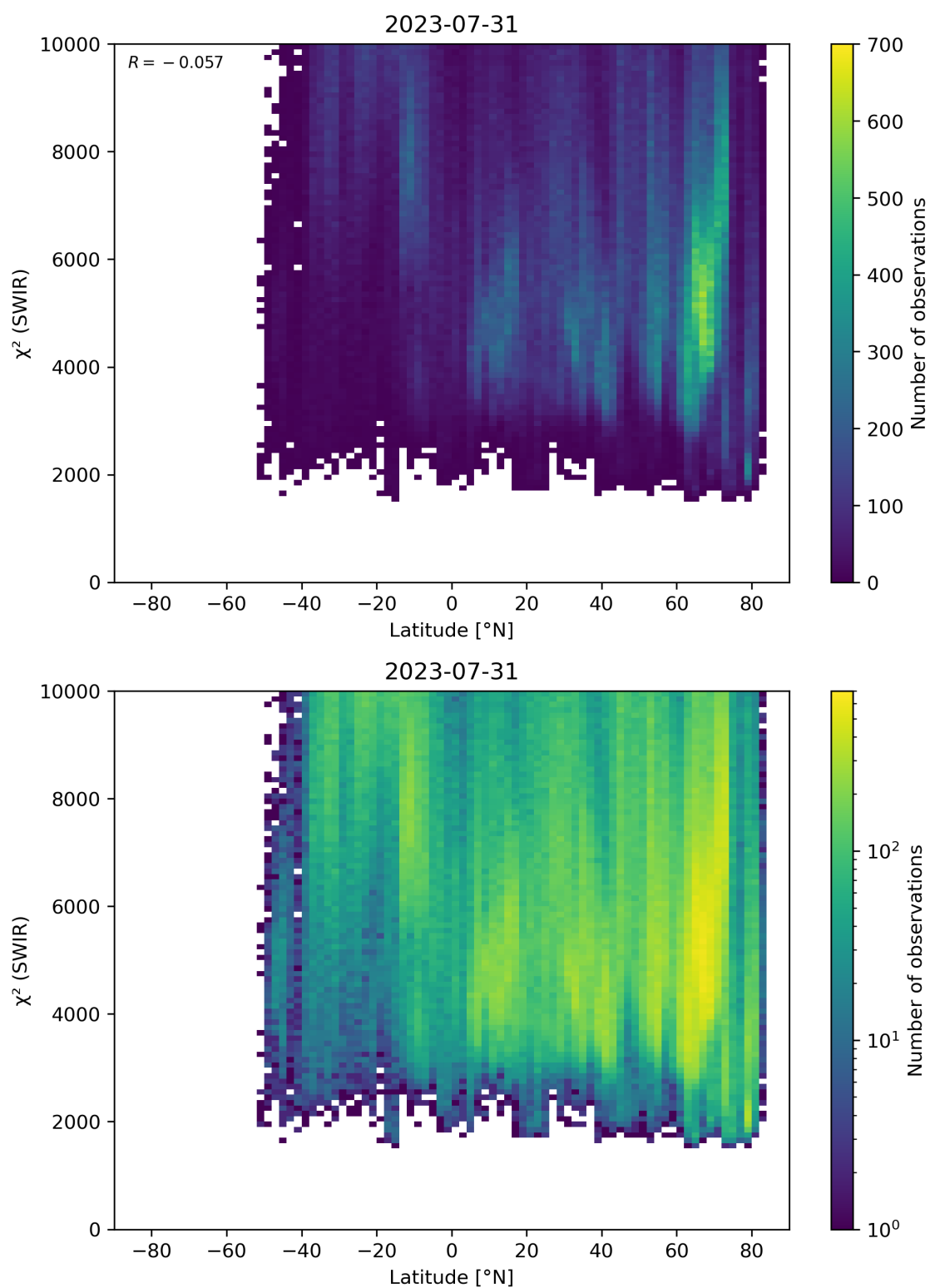
Figure 54: Scatter density plot of “Latitude” against “ \chi^2 (SWIR)” for 2023-07-30 to 2023-08-01.
