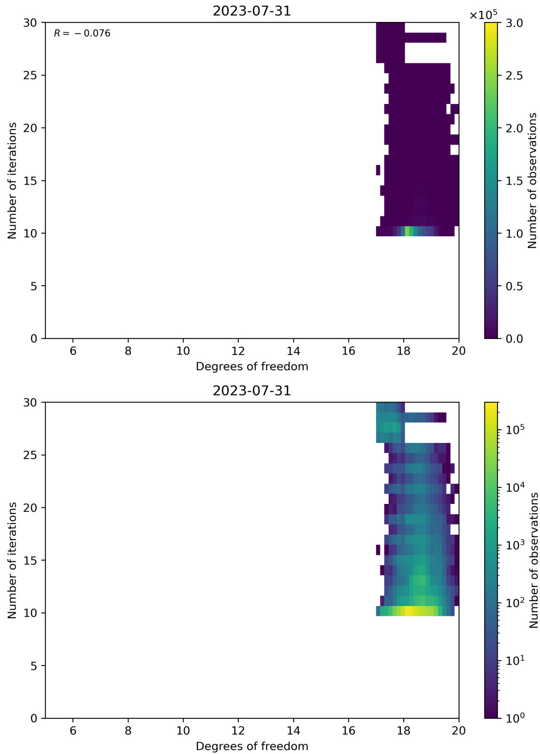
Figure 52: Scatter density plot of “Degrees of freedom” against “Number of iterations” for 2023-07-30 to 2023-08-01.
