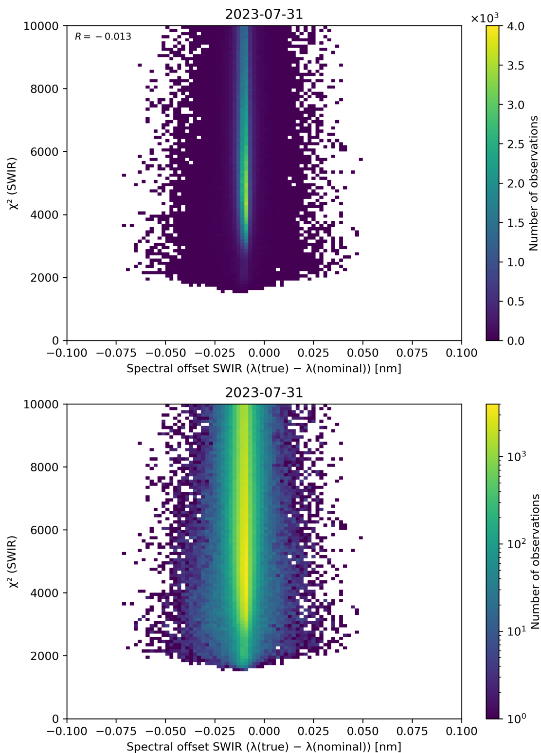
Figure 118: Scatter density plot of “Spectral offset SWIR ( \lambda(\text{true}) - \lambda(\text{nominal}) )” against “ \chi^2 (SWIR)” for 2023-07-30 to 2023-08-01.
