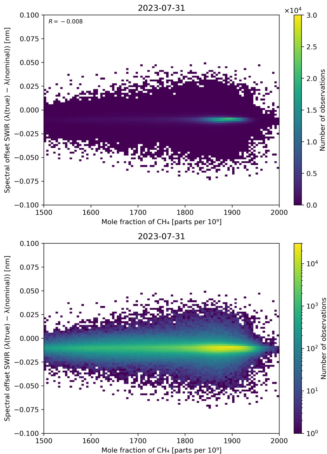
Figure 86: Scatter density plot of “Mole fraction of CH 4 ” against “Spectral offset SWIR ( \lambda(\text{true}) - \lambda(\text{nominal}) )” for 2023-07-30 to 2023-08-01.
