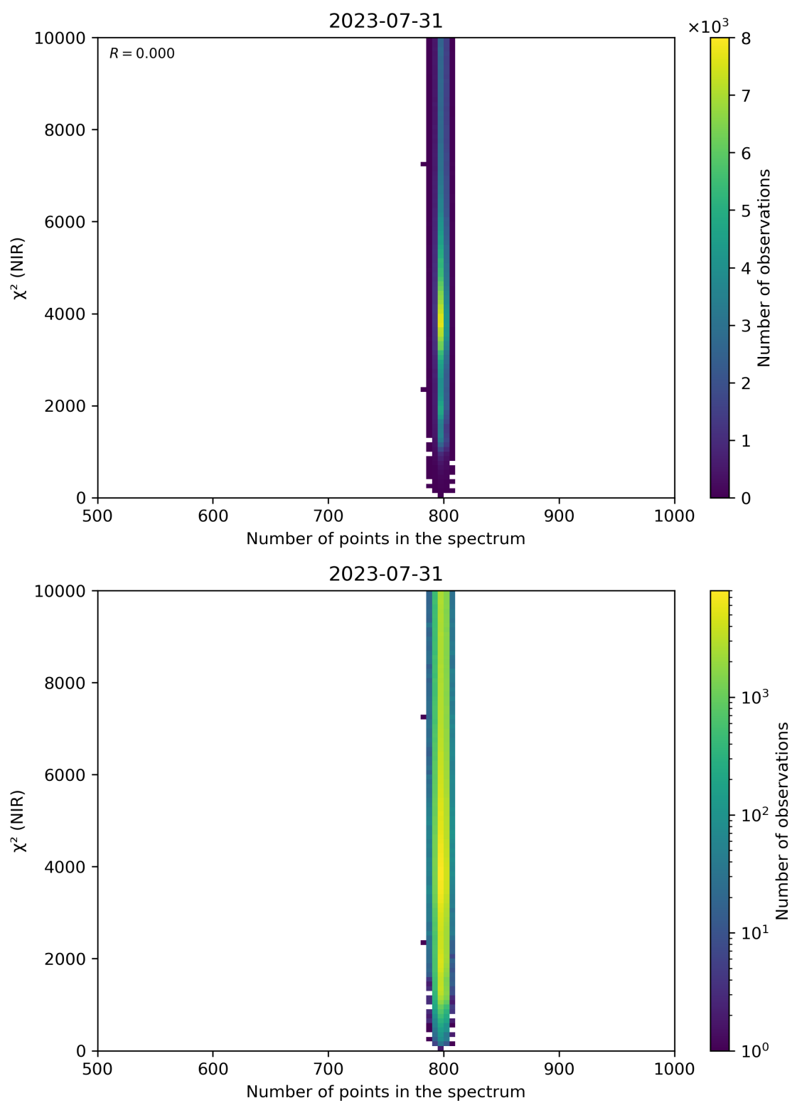
Figure 88: Scatter density plot of “Number of points in the spectrum” against “ \chi^2 (NIR)” for 2023-07-30 to 2023-08-01.
