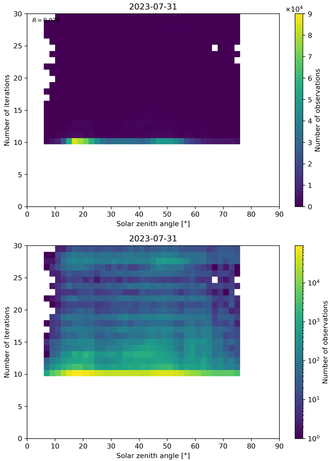
Figure 102: Scatter density plot of “Solar zenith angle” against “Number of iterations” for 2023-07-30 to 2023-08-01.
