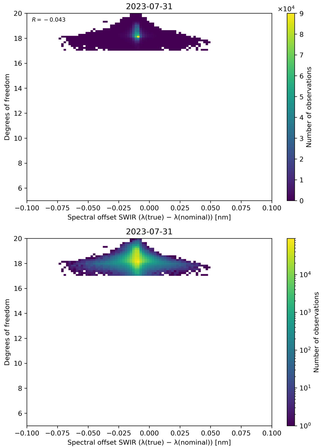
Figure 119: Scatter density plot of “Spectral offset SWIR ( \lambda(\text{true}) - \lambda(\text{nominal}) )” against “Degrees of freedom” for 2023-07-30 to 2023-08-01.
