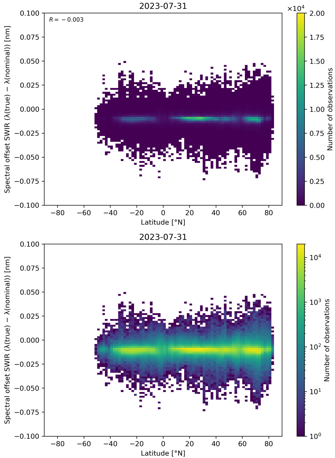
Figure 62: Scatter density plot of “Latitude” against “Spectral offset SWIR ( \lambda(\text{true}) - \lambda(\text{nominal}) )” for 2023-07-30 to 2023-08-01.
