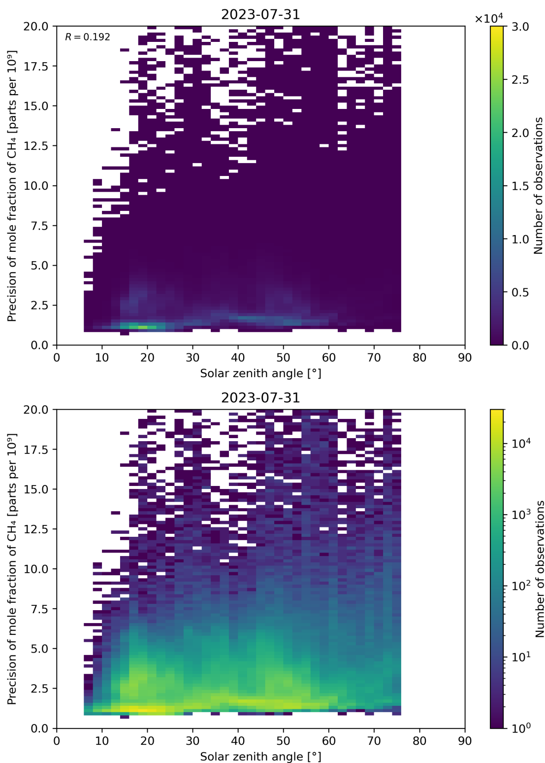
Figure 101: Scatter density plot of “Solar zenith angle” against “Precision of mole fraction of CH 4 ” for 2023-07-30 to 2023-08-01.
