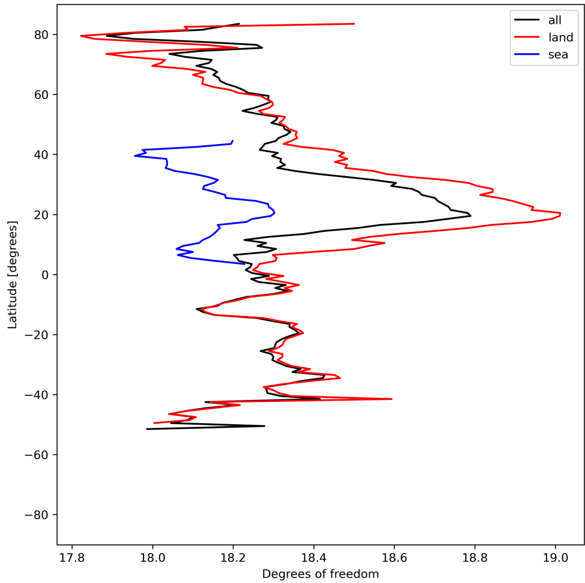
Figure 19: Zonal average of “Degrees of freedom” for 2023-07-30 to 2023-08-01.
