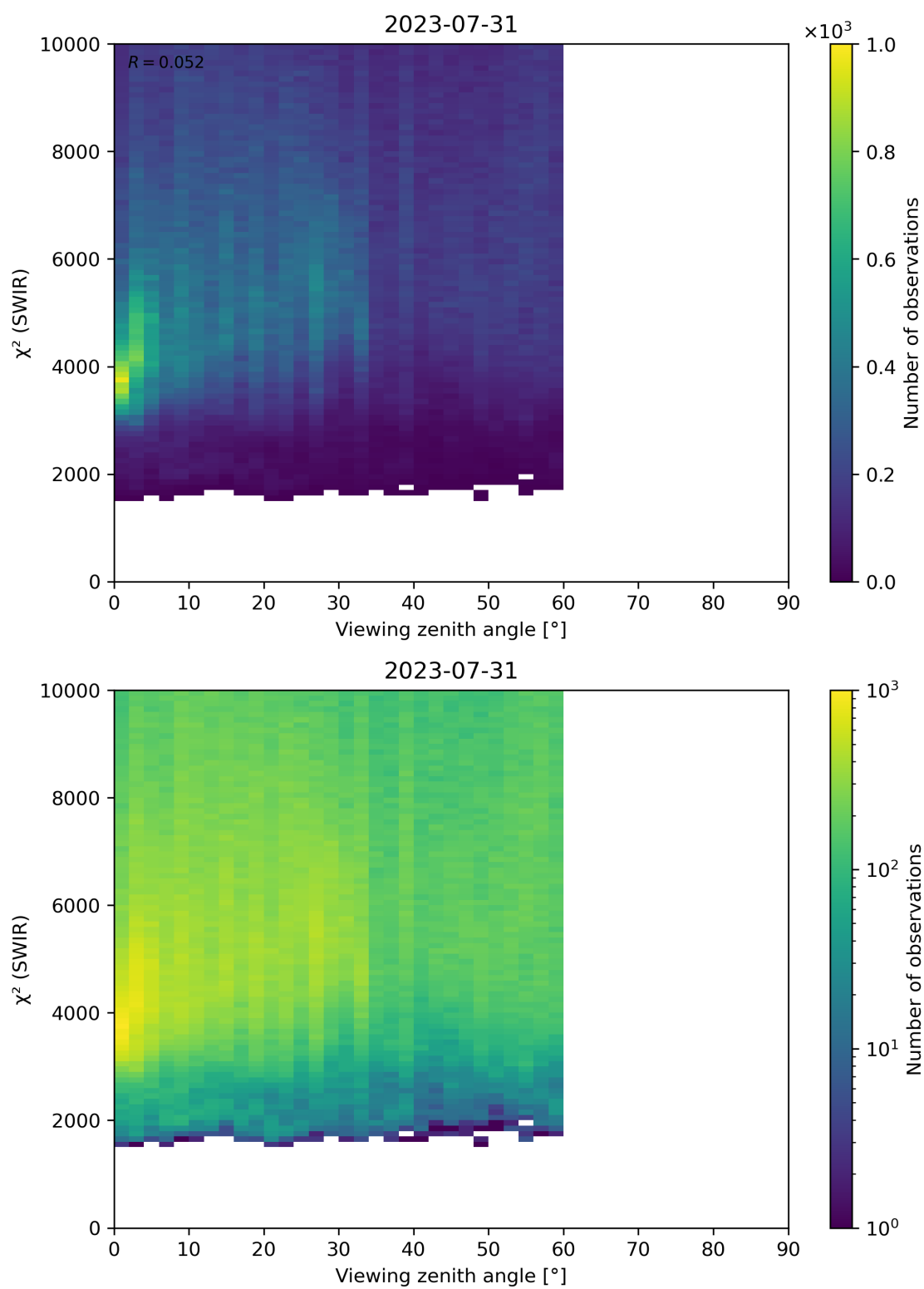
Figure 106: Scatter density plot of “Viewing zenith angle” against “ \chi^2 (SWIR)” for 2023-07-30 to 2023-08-01.
