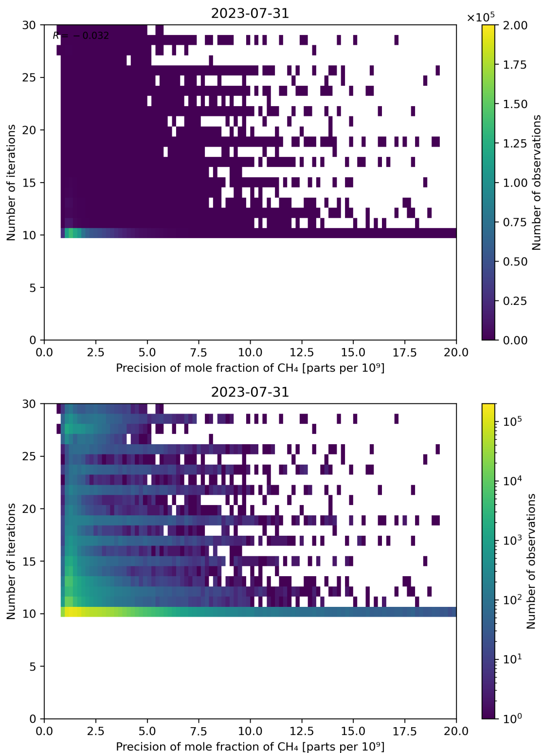
Figure 83: Scatter density plot of “Precision of mole fraction of CH 4 ” against “Number of iterations” for 2023-07-30 to 2023-08-01.
