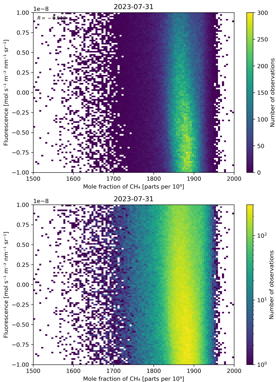
Figure 73: Scatter density plot of “Mole fraction of CH 4 ” against “Fluorescence” for 2023-07-30 to 2023-08-01.
