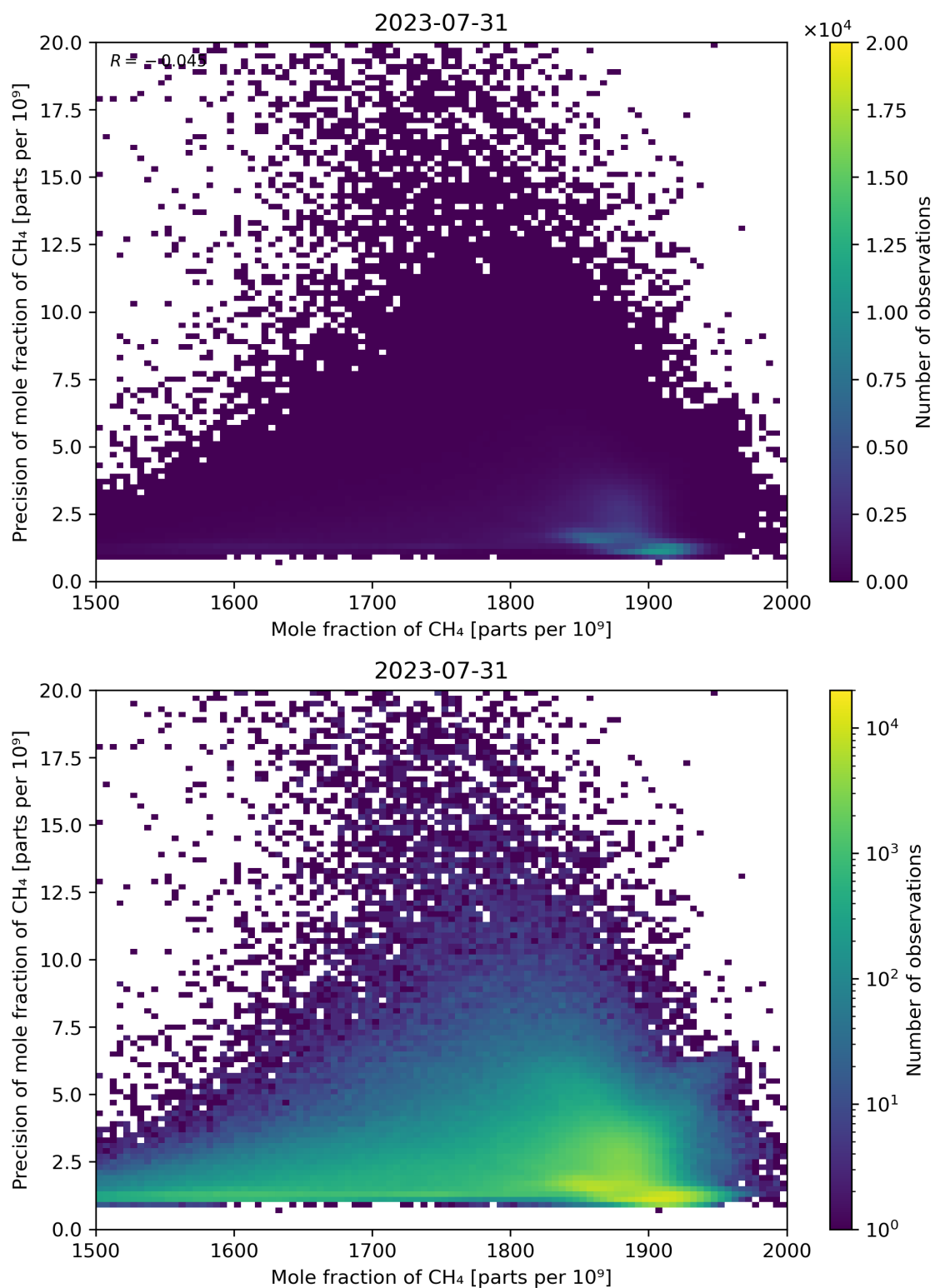
Figure 75: Scatter density plot of “Mole fraction of CH 4 ” against “Precision of mole fraction of CH 4 ” for 2023-07-30 to 2023-08-01.
