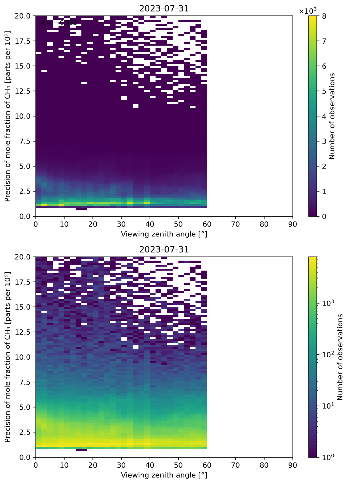
Figure 112: Scatter density plot of “Viewing zenith angle” against “Precision of mole fraction of CH 4 ” for 2023-07-30 to 2023-08-01.
