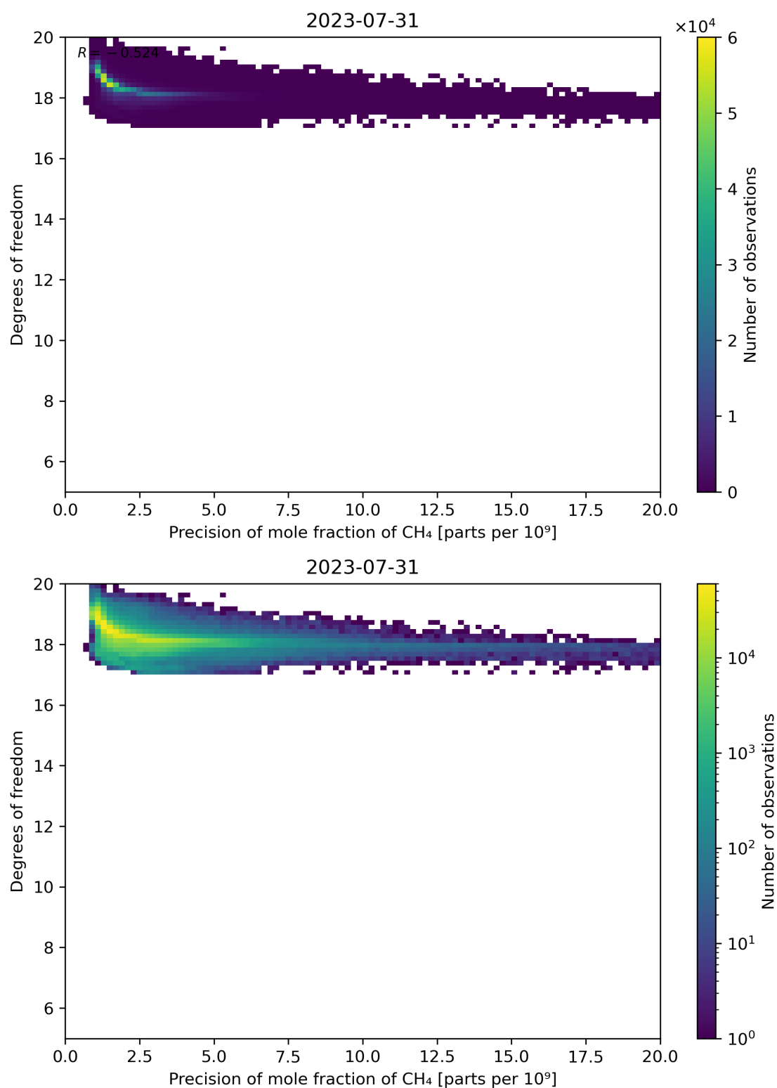
Figure 80: Scatter density plot of “Precision of mole fraction of CH 4 ” against “Degrees of freedom” for 2023-07-30 to 2023-08-01.
