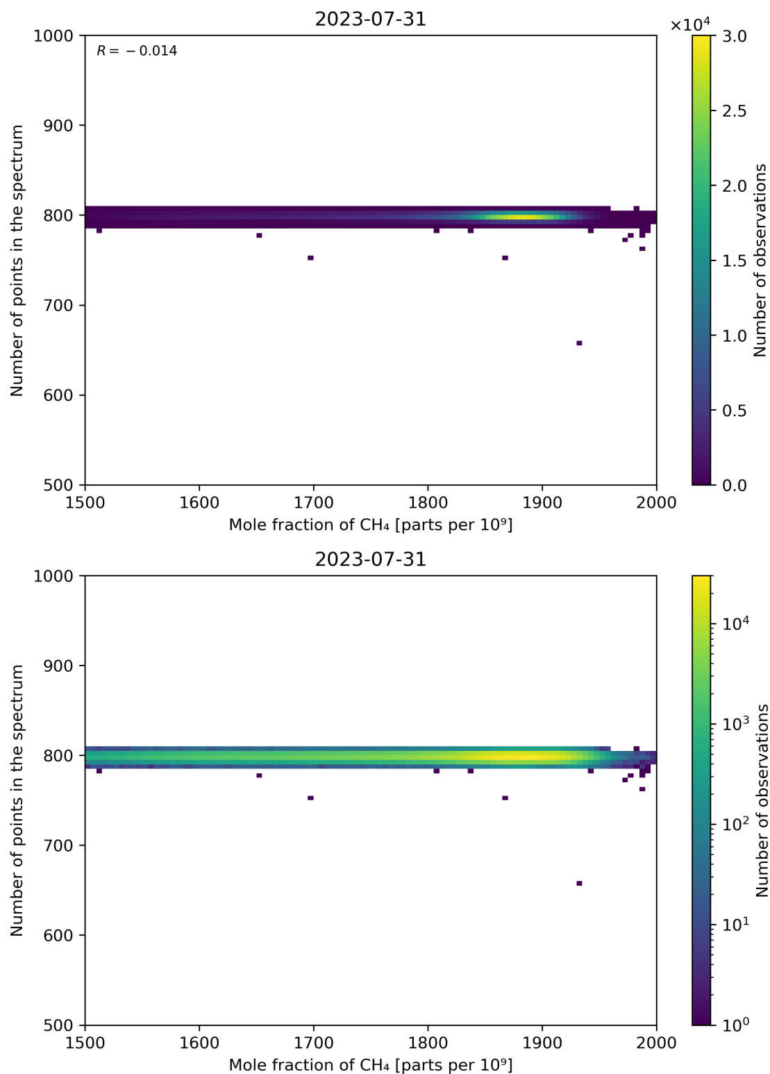
Figure 77: Scatter density plot of “Mole fraction of CH 4 ” against “Number of points in the spectrum” for 2023-07-30 to 2023-08-01.
