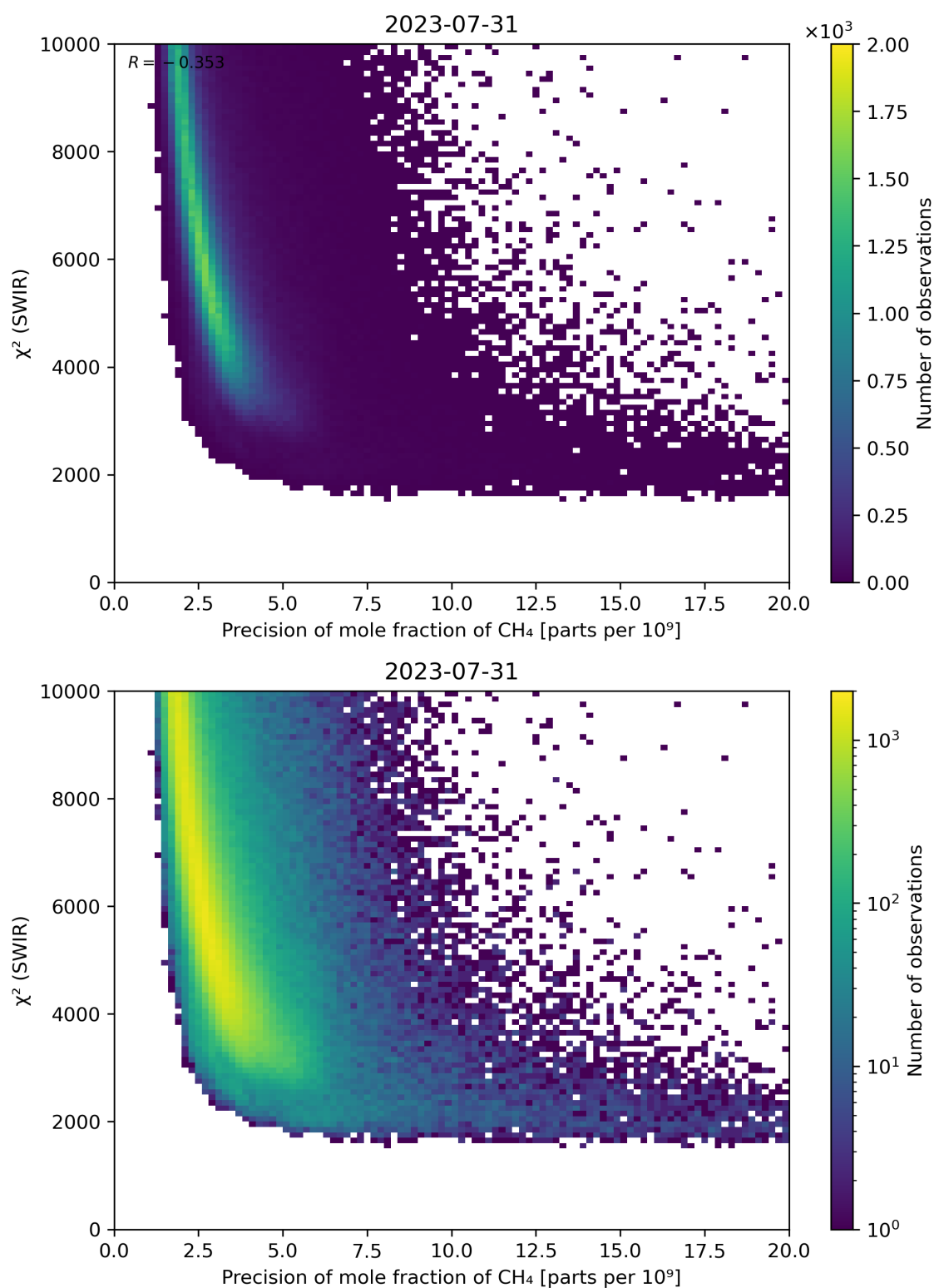
Figure 79: Scatter density plot of “Precision of mole fraction of \text{CH}_4 ” against “ \chi^2 (SWIR)” for 2023-07-30 to 2023-08-01.
