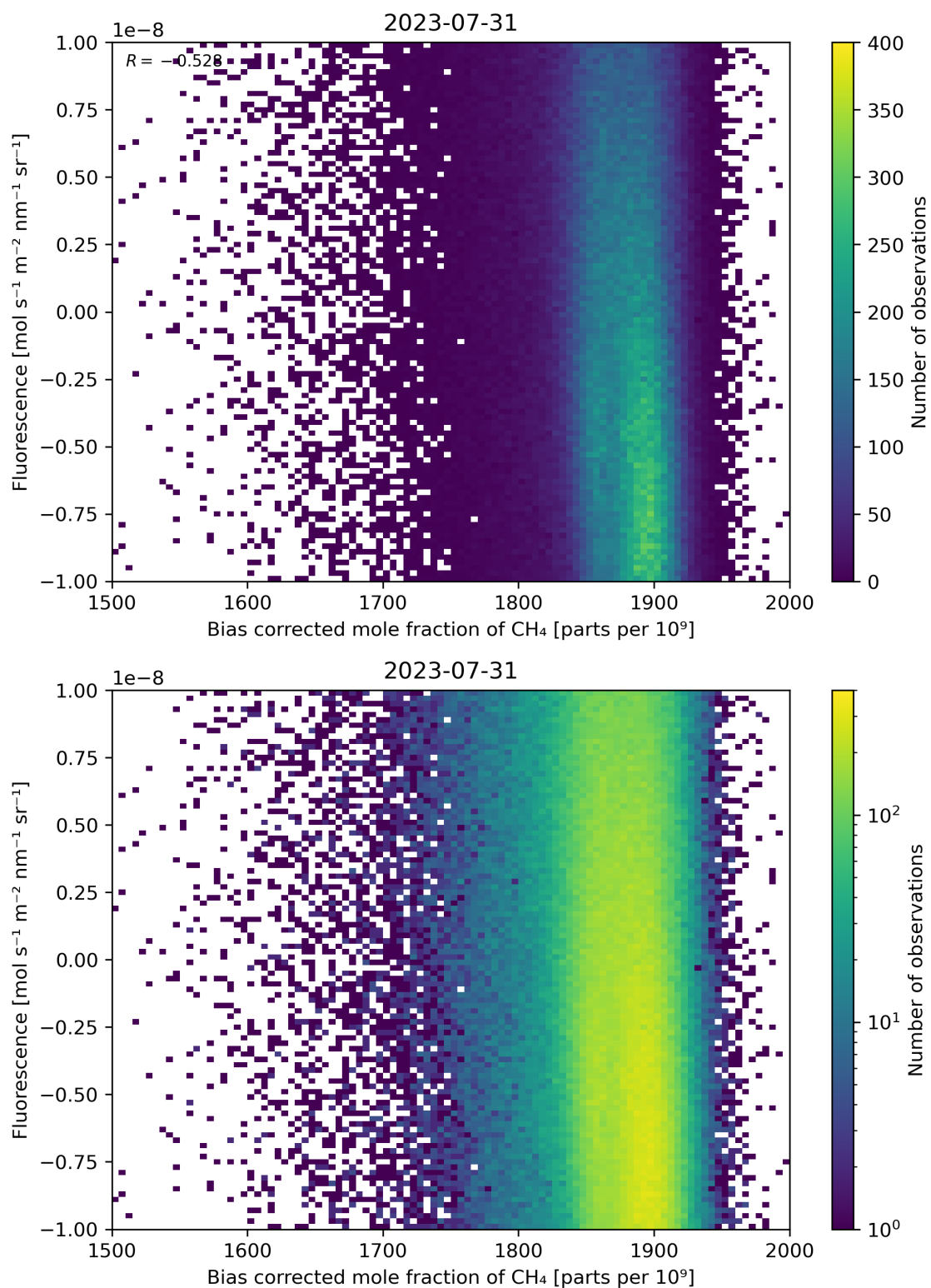
Figure 66: Scatter density plot of “Bias corrected mole fraction of \text{CH}_4 ” against “Fluorescence” for 2023-07-30 to 2023-08-01.
