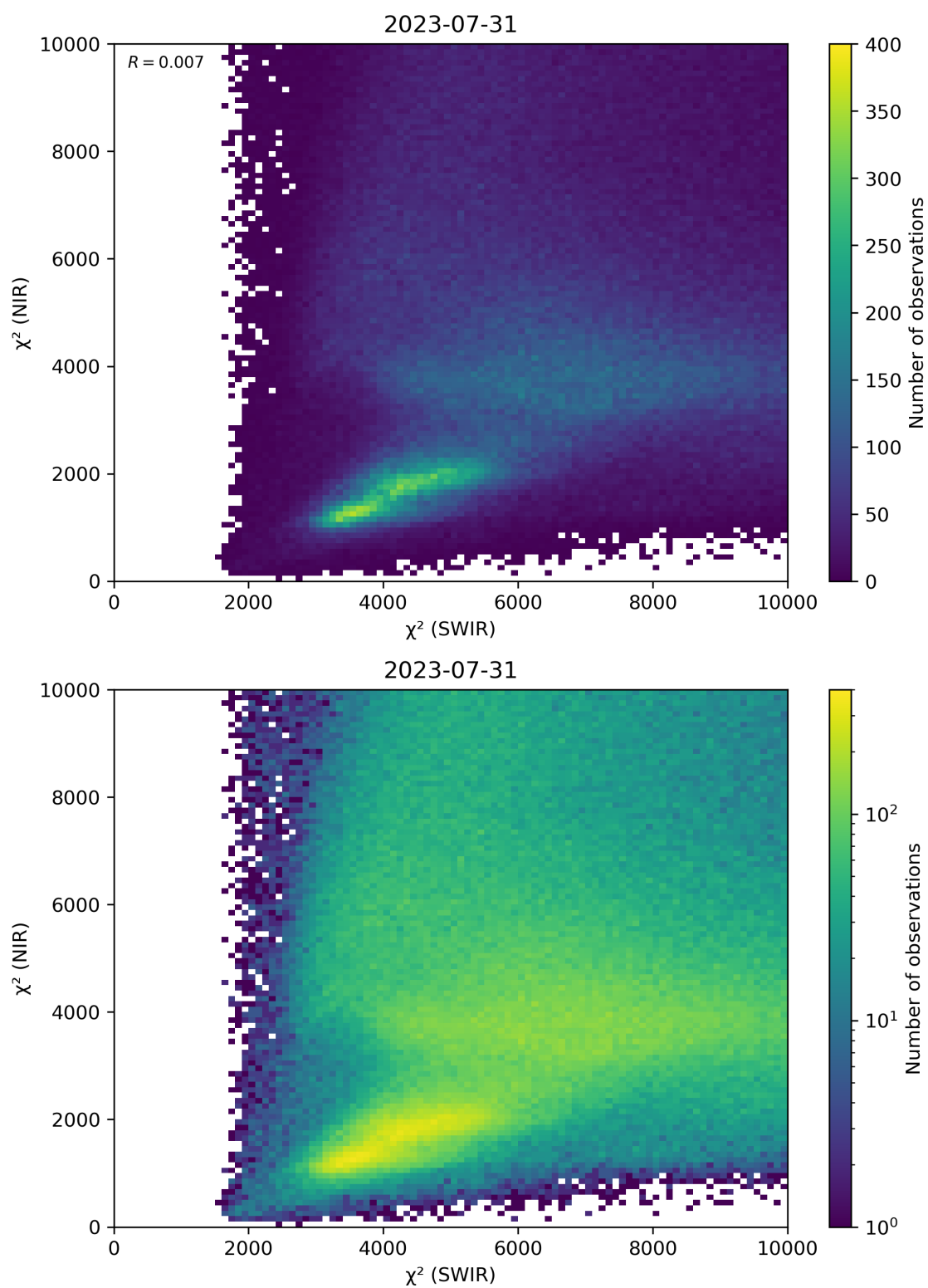
Figure 47: Scatter density plot of “ \chi^2 (SWIR)” against “ \chi^2 (NIR)” for 2023-07-30 to 2023-08-01.
