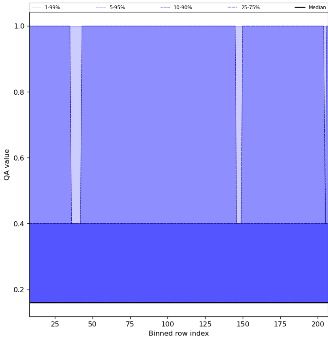
Figure 33: Along track statistics of “QA value” for 2023-07-30 to 2023-08-01
