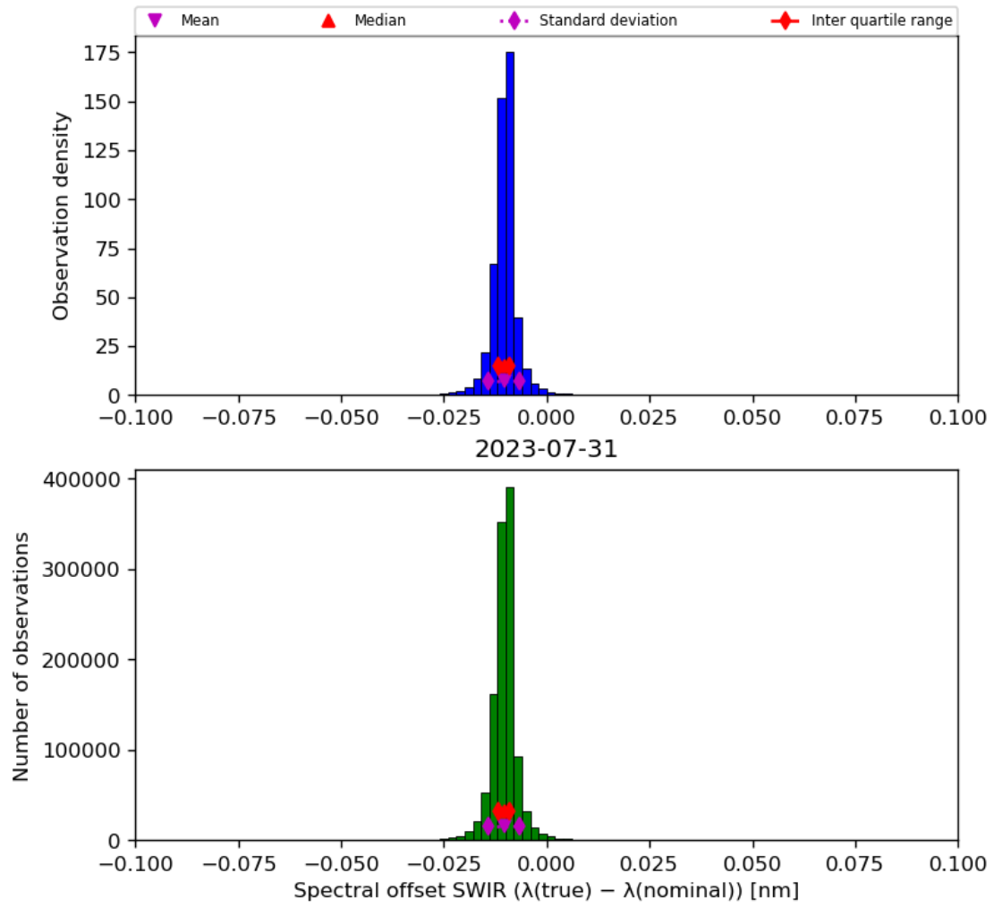
Figure 27: Histogram of “Spectral offset SWIR ( \lambda(\text{true}) - \lambda(\text{nominal}) )” for 2023-07-30 to 2023-08-01
