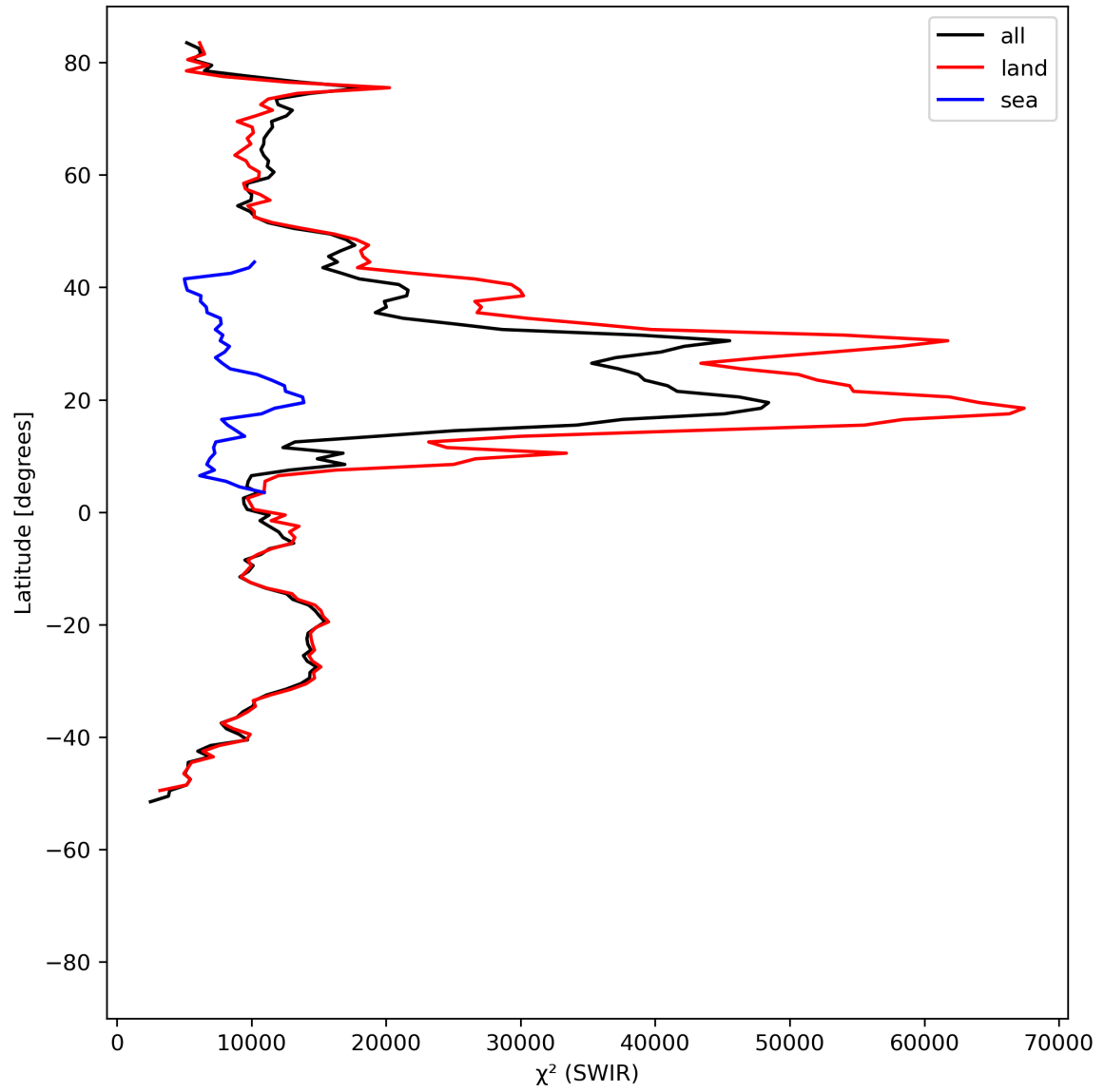
Figure 17: Zonal average of “ \chi^2 (SWIR)” for 2023-07-30 to 2023-08-01.
