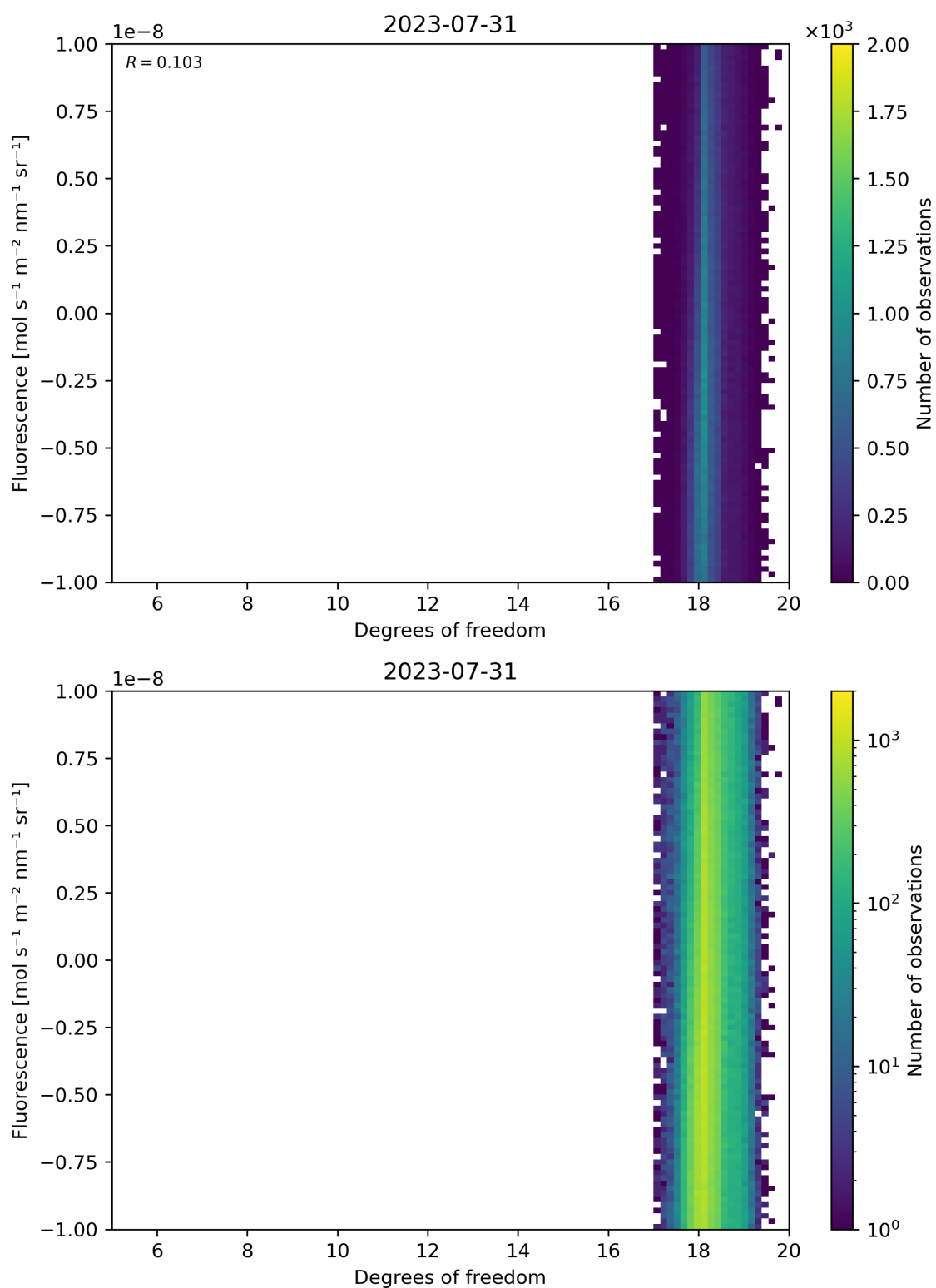
Figure 51: Scatter density plot of “Degrees of freedom” against “Fluorescence” for 2023-07-30 to 2023-08-01.
