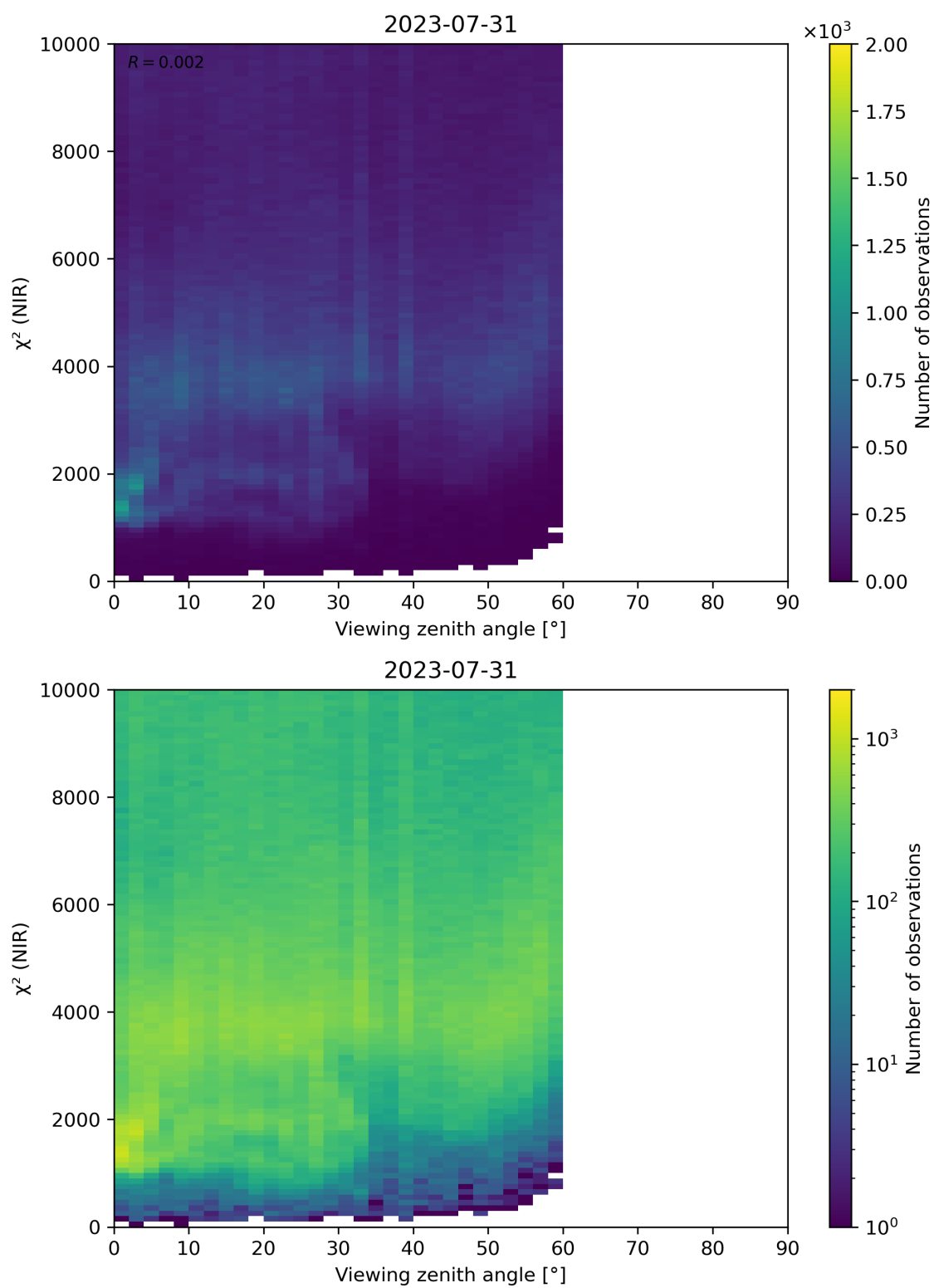
Figure 105: Scatter density plot of “Viewing zenith angle” against “ \chi^2 (NIR)” for 2023-07-30 to 2023-08-01.
