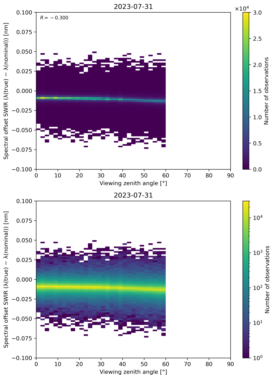
Figure 116: Scatter density plot of “Viewing zenith angle” against “Spectral offset SWIR ( \lambda(\text{true}) - \lambda(\text{nominal}) )” for 2023-07-30 to 2023-08-01.
