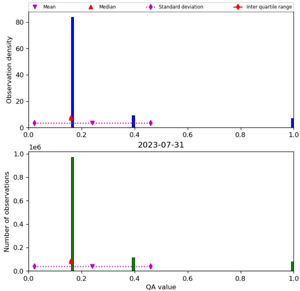
Figure 22: Histogram of “QA value” for 2023-07-30 to 2023-08-01
