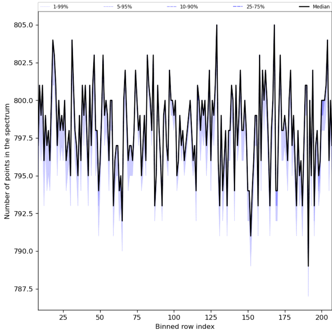
Figure 37: Along track statistics of “Number of points in the spectrum” for 2023-07-30 to 2023-08-01
