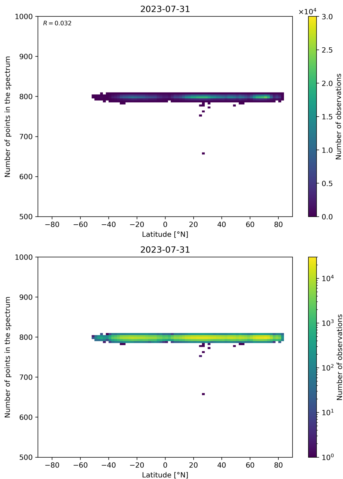
Figure 61: Scatter density plot of “Latitude” against “Number of points in the spectrum” for 2023-07-30 to 2023-08-01.
