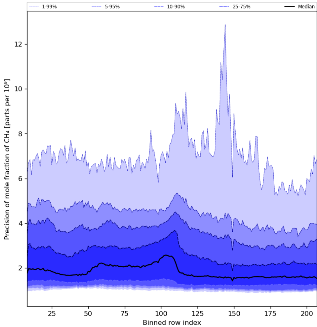
Figure 35: Along track statistics of “Precision of mole fraction of CH 4 ” for 2023-07-30 to 2023-08-01
