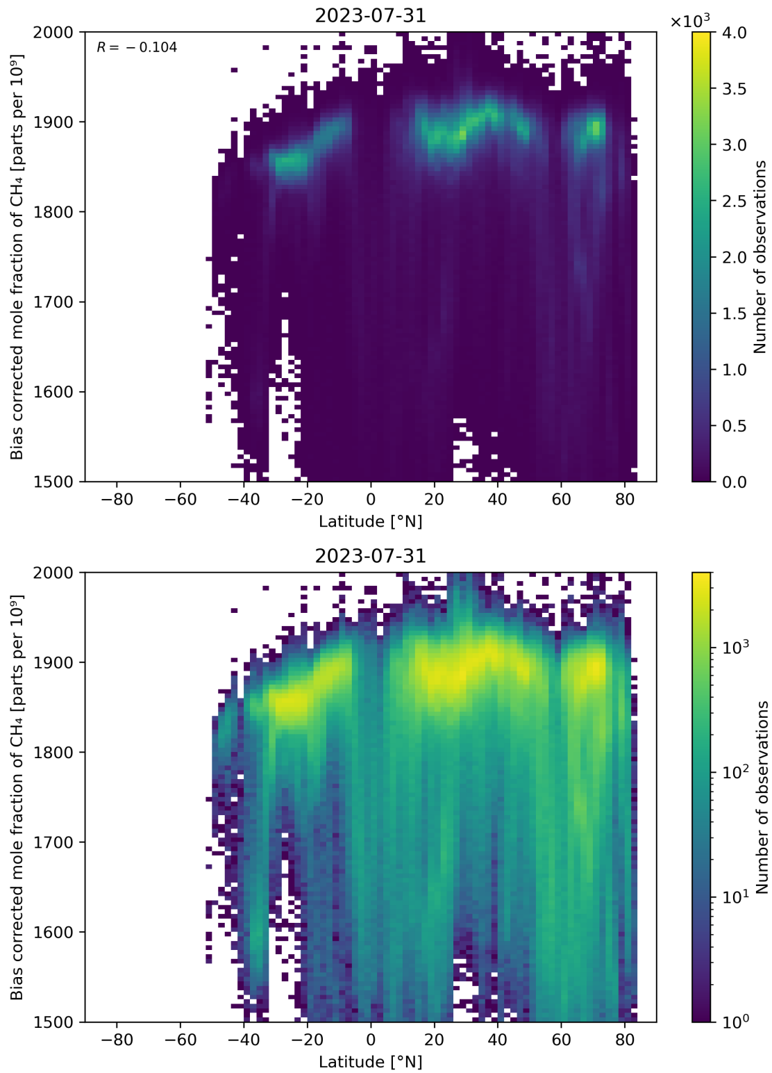
Figure 58: Scatter density plot of “Latitude” against “Bias corrected mole fraction of \text{CH}_4 ” for 2023-07-30 to 2023-08-01.
