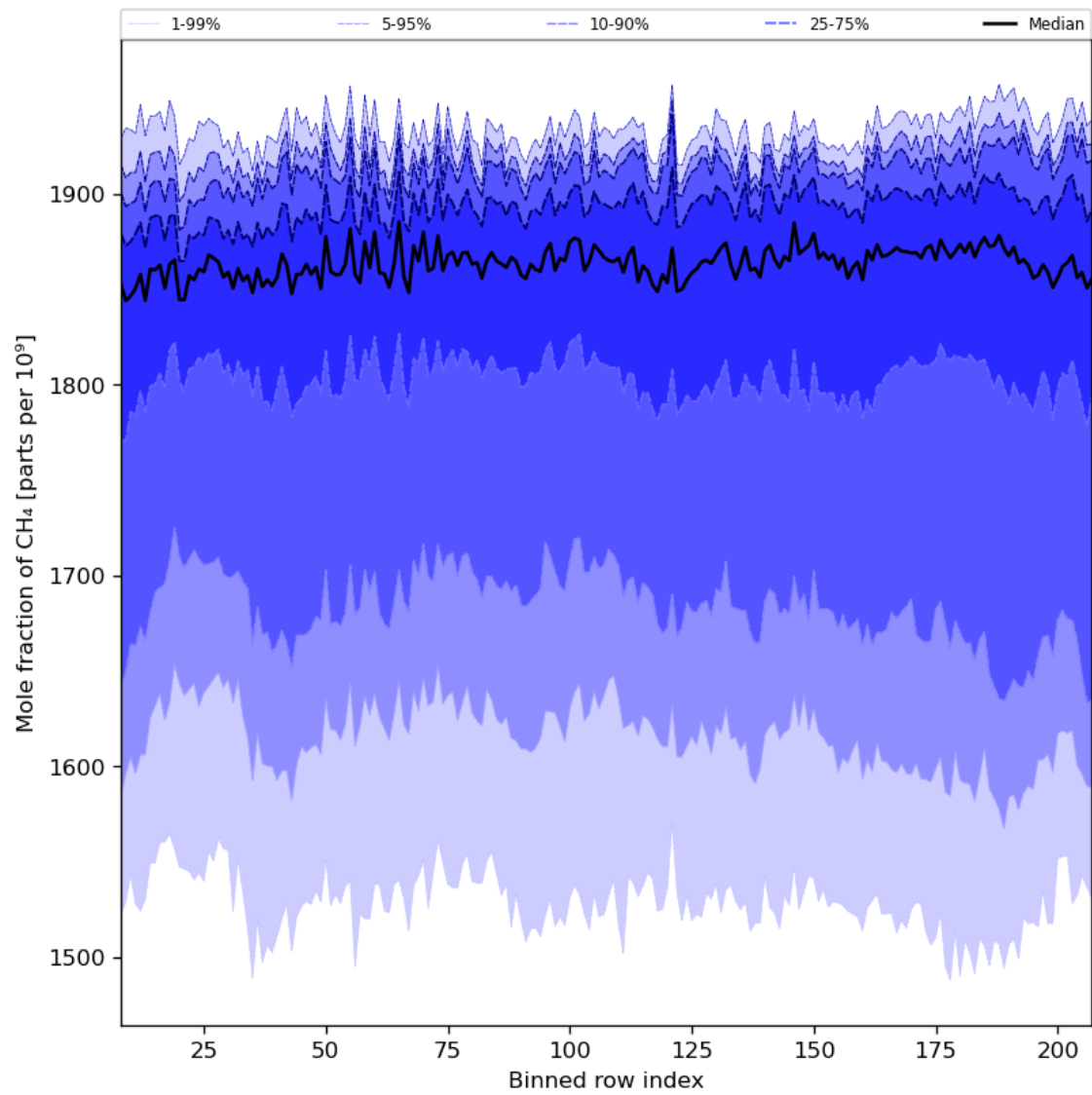
Figure 34: Along track statistics of “Mole fraction of CH 4 ” for 2023-07-30 to 2023-08-01
