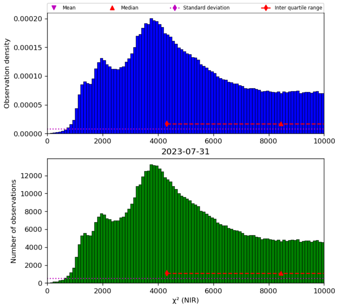
Figure 29: Histogram of “ \chi^2 (NIR)” for 2023-07-30 to 2023-08-01
