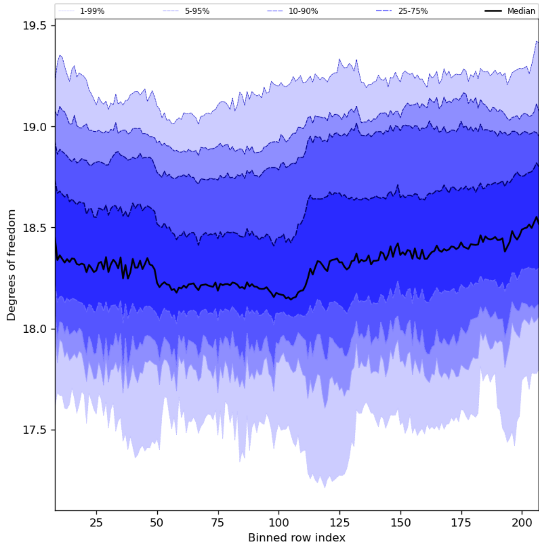
Figure 41: Along track statistics of “Degrees of freedom” for 2023-07-30 to 2023-08-01
