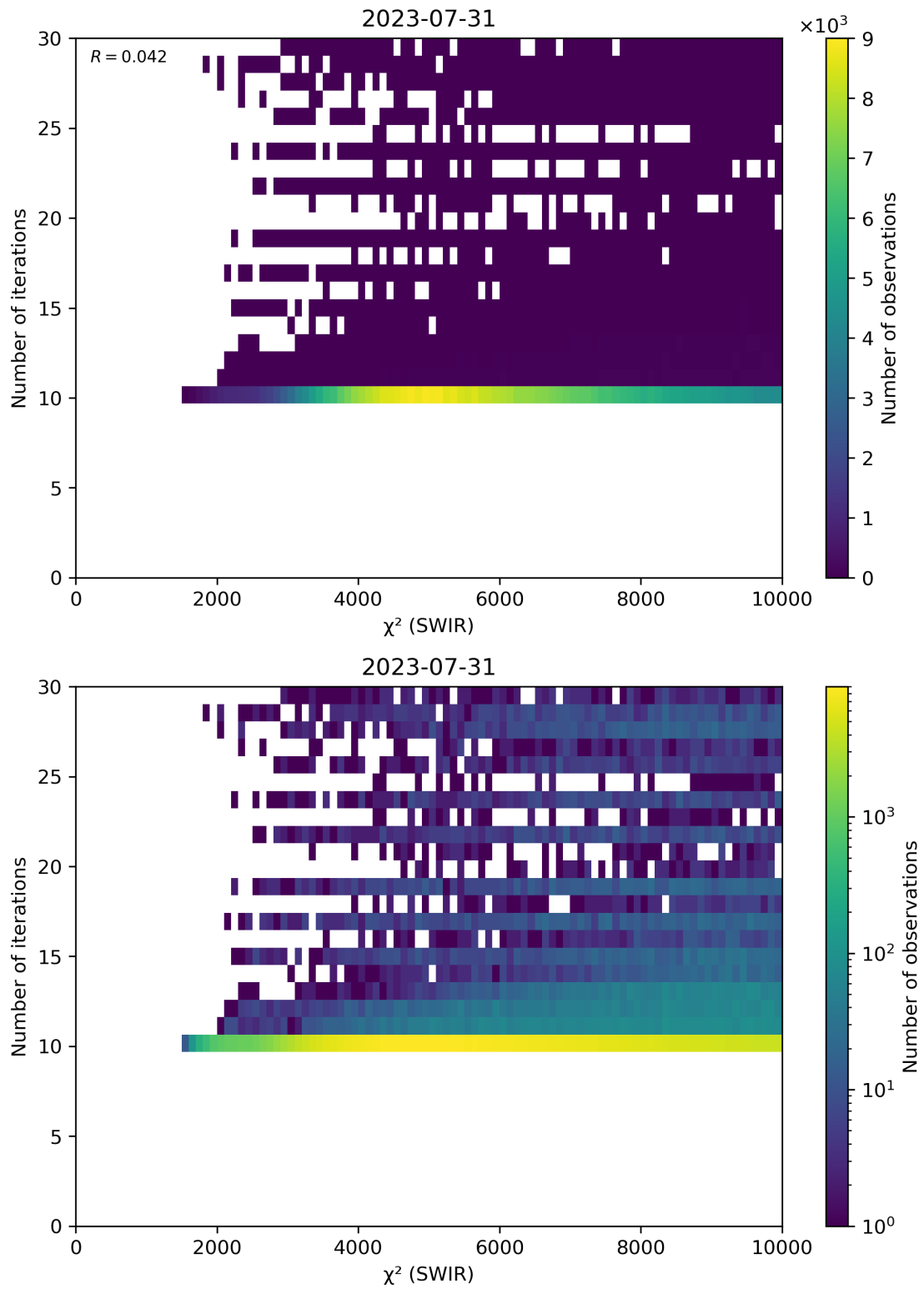
Figure 50: Scatter density plot of “ \chi^2 (SWIR)” against “Number of iterations” for 2023-07-30 to 2023-08-01.
