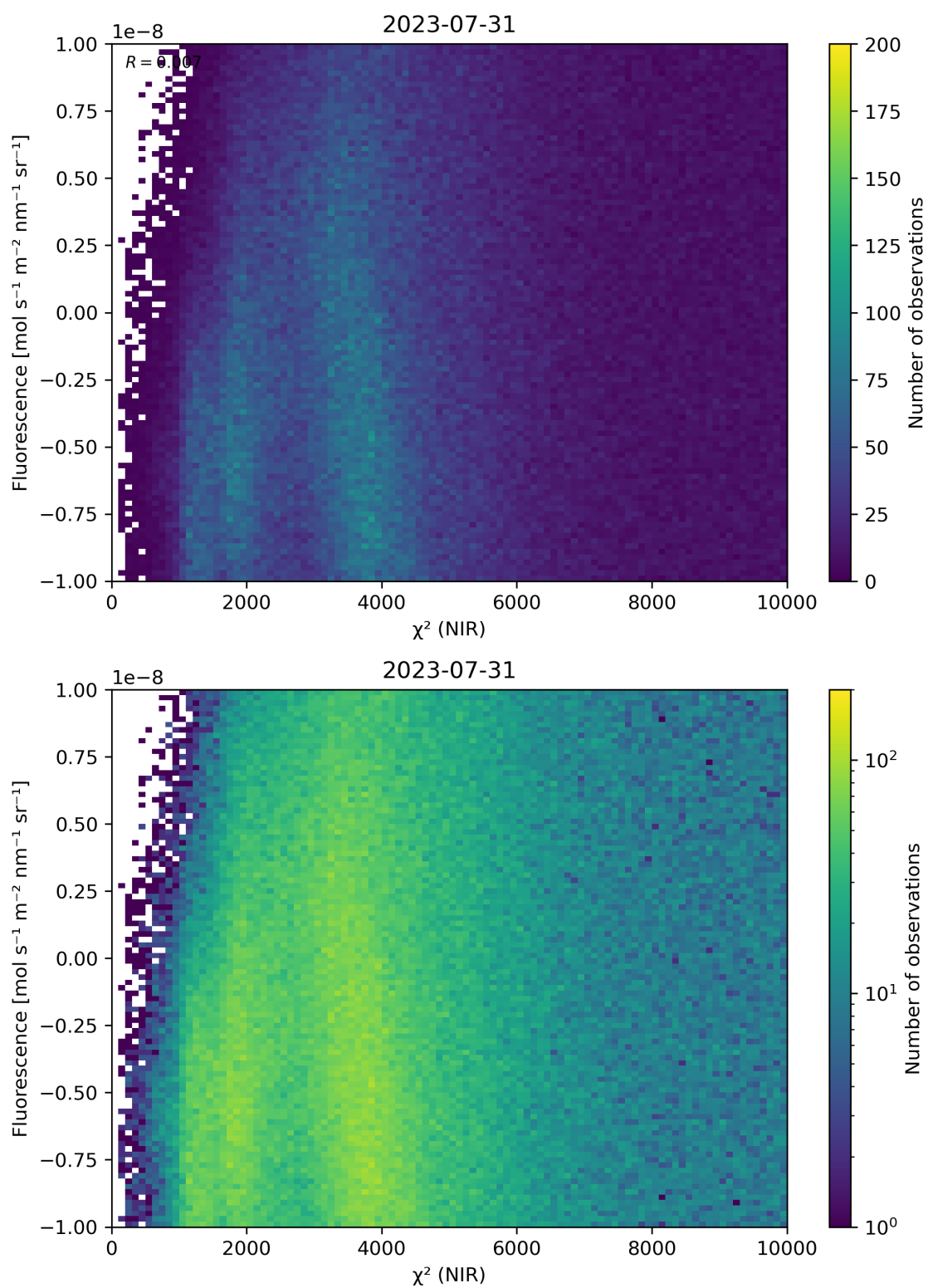
Figure 45: Scatter density plot of “ \chi^2 (NIR)” against “Fluorescence” for 2023-07-30 to 2023-08-01.
