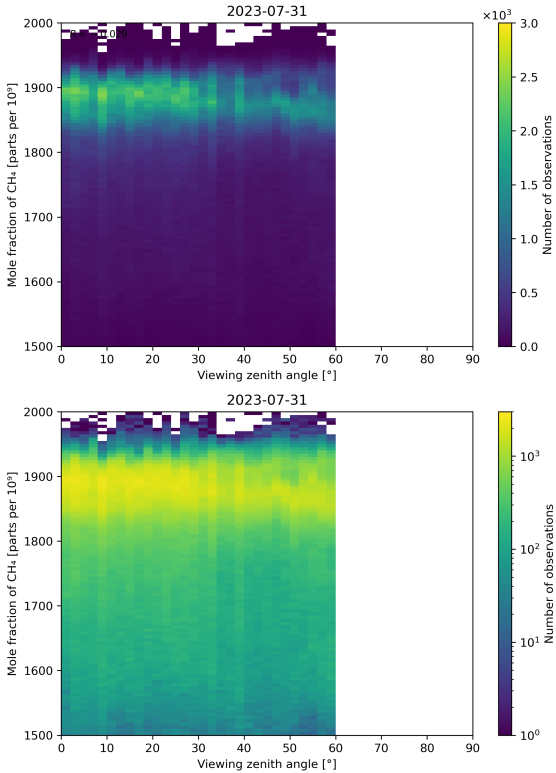
Figure 110: Scatter density plot of “Viewing zenith angle” against “Mole fraction of CH 4 ” for 2023-07-30 to 2023-08-01.
