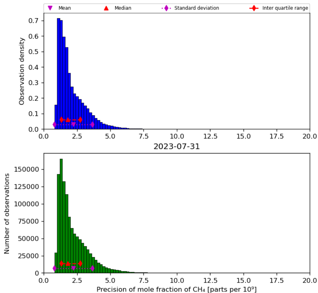
Figure 24: Histogram of “Precision of mole fraction of CH 4 ” for 2023-07-30 to 2023-08-01
