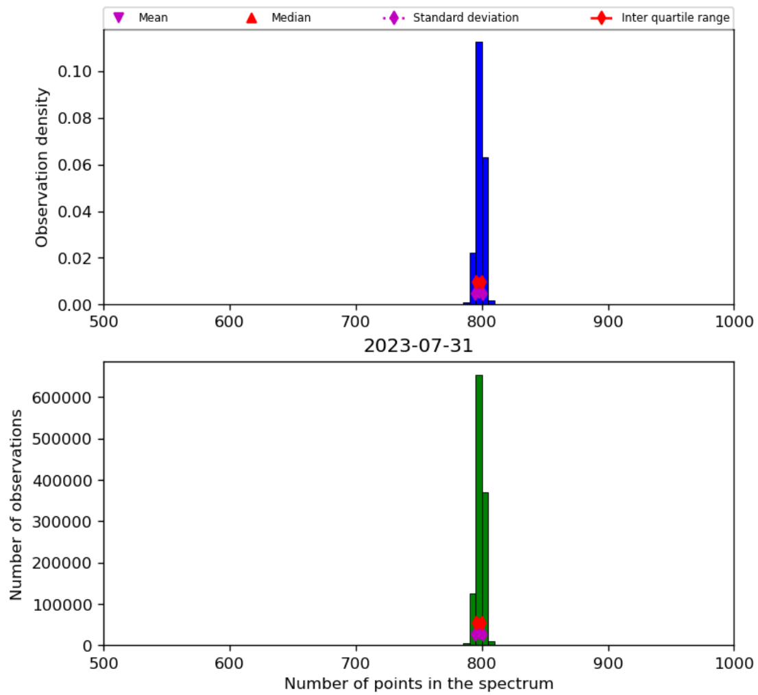
Figure 26: Histogram of “Number of points in the spectrum” for 2023-07-30 to 2023-08-01
