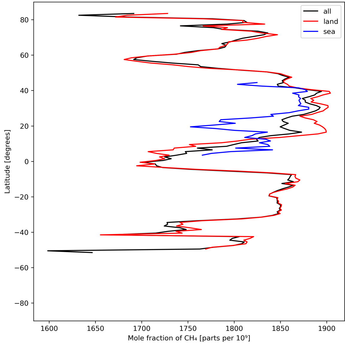
Figure 12: Zonal average of “Mole fraction of \text{CH}_4 ” for 2023-07-30 to 2023-08-01.
