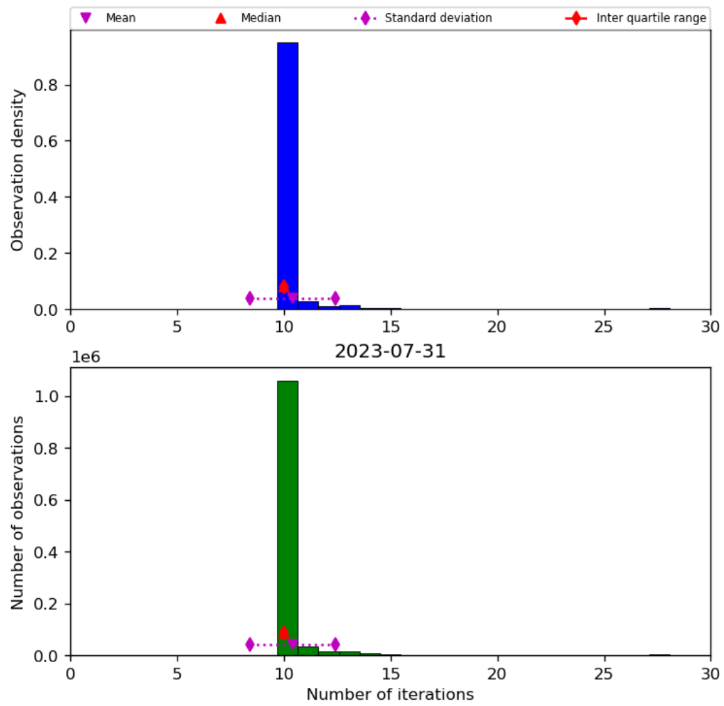
Figure 31: Histogram of “Number of iterations” for 2023-07-30 to 2023-08-01
