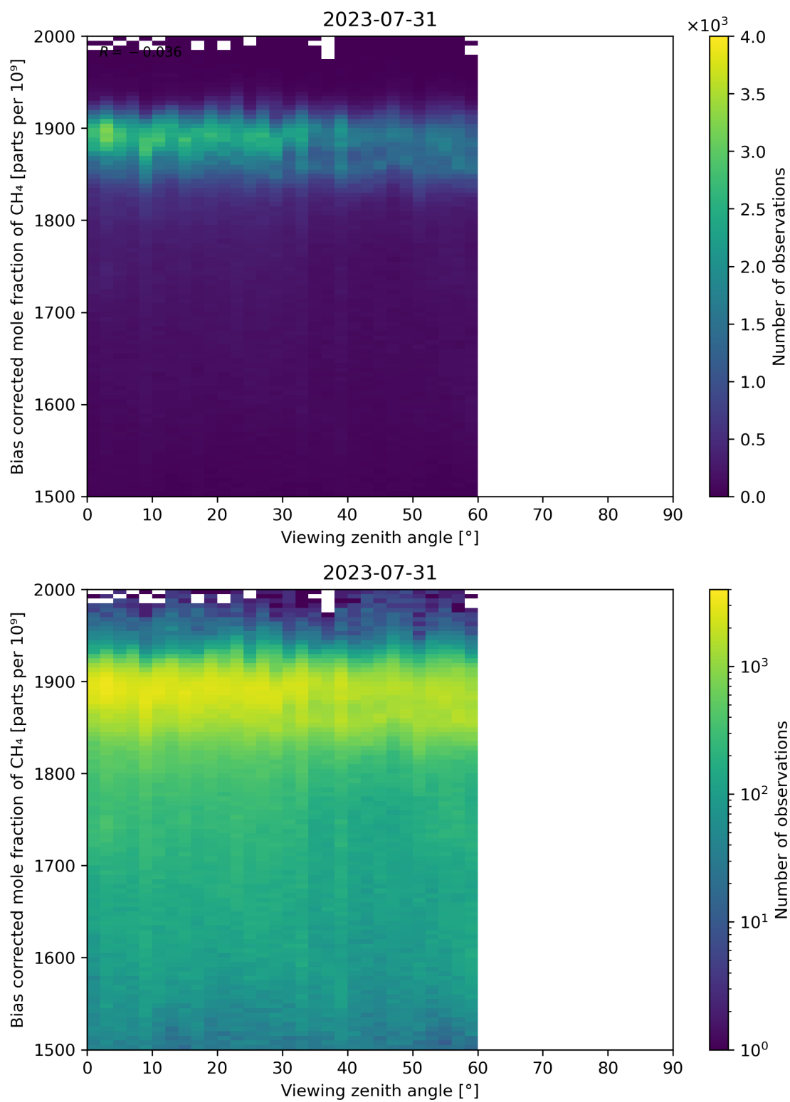
Figure 111: Scatter density plot of “Viewing zenith angle” against “Bias corrected mole fraction of CH 4 ” for 2023-07-30 to 2023-08-01.
