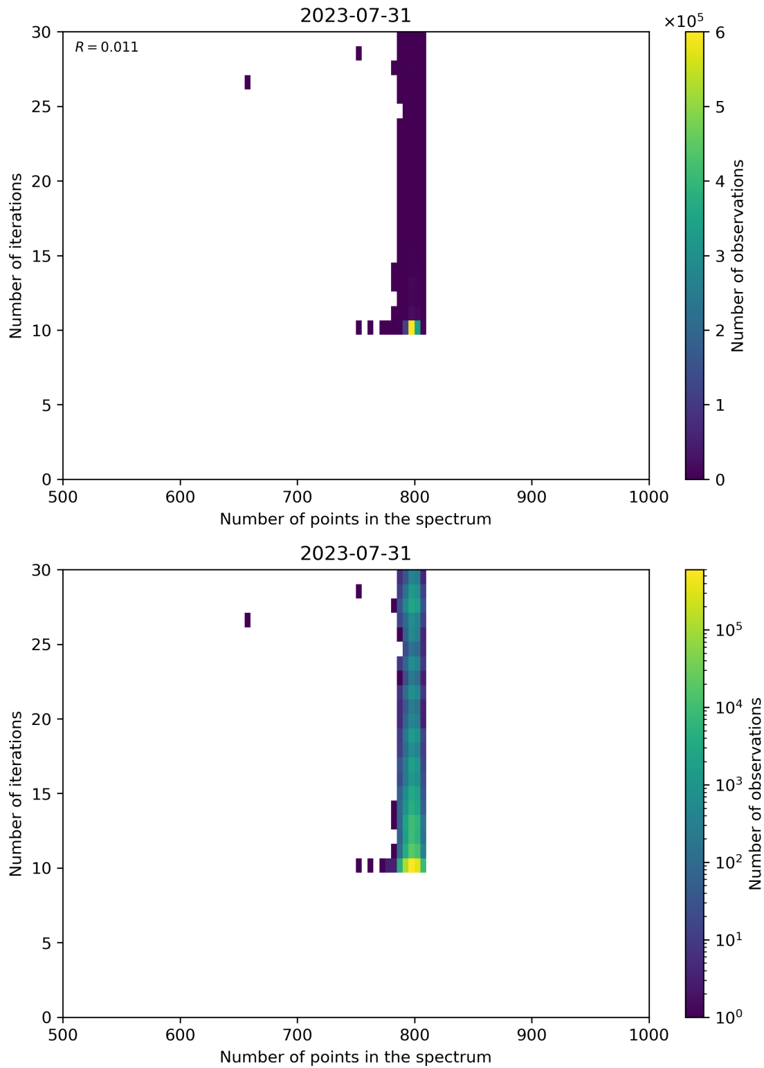
Figure 92: Scatter density plot of “Number of points in the spectrum” against “Number of iterations” for 2023-07-30 to 2023-08-01.
