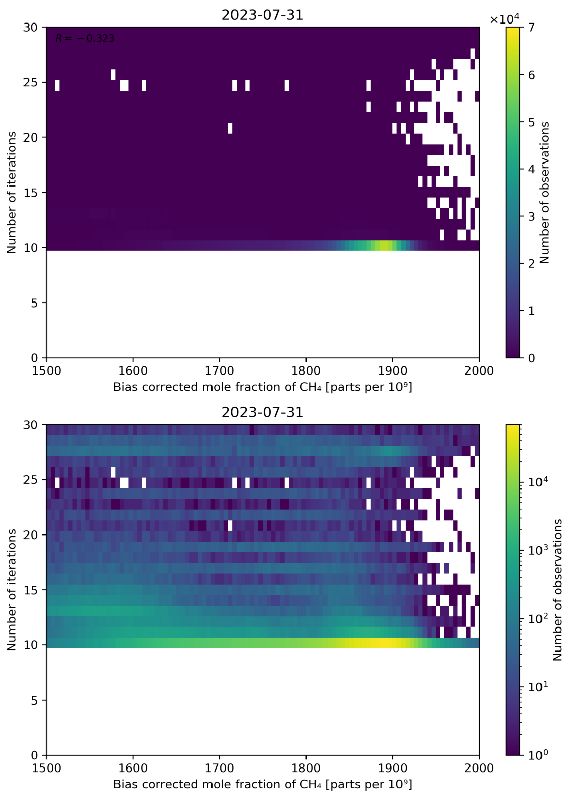
Figure 67: Scatter density plot of “Bias corrected mole fraction of CH 4 ” against “Number of iterations” for 2023-07-30 to 2023-08-01.
