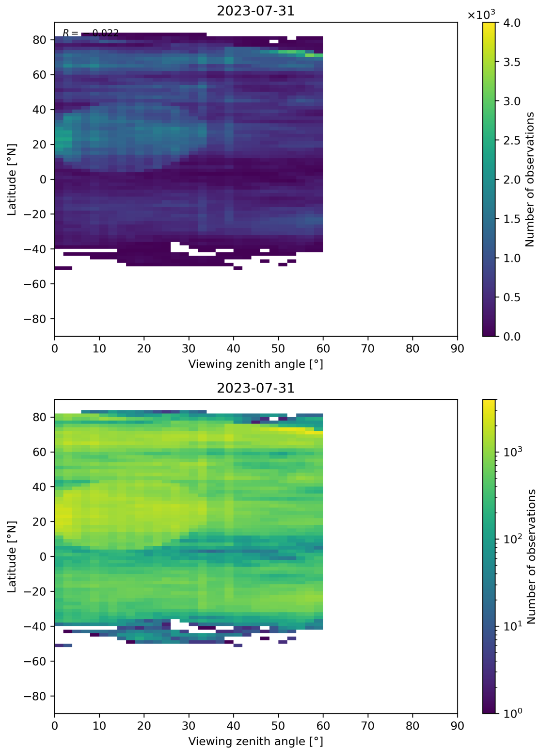
Figure 109: Scatter density plot of “Viewing zenith angle” against “Latitude” for 2023-07-30 to 2023-08-01.
