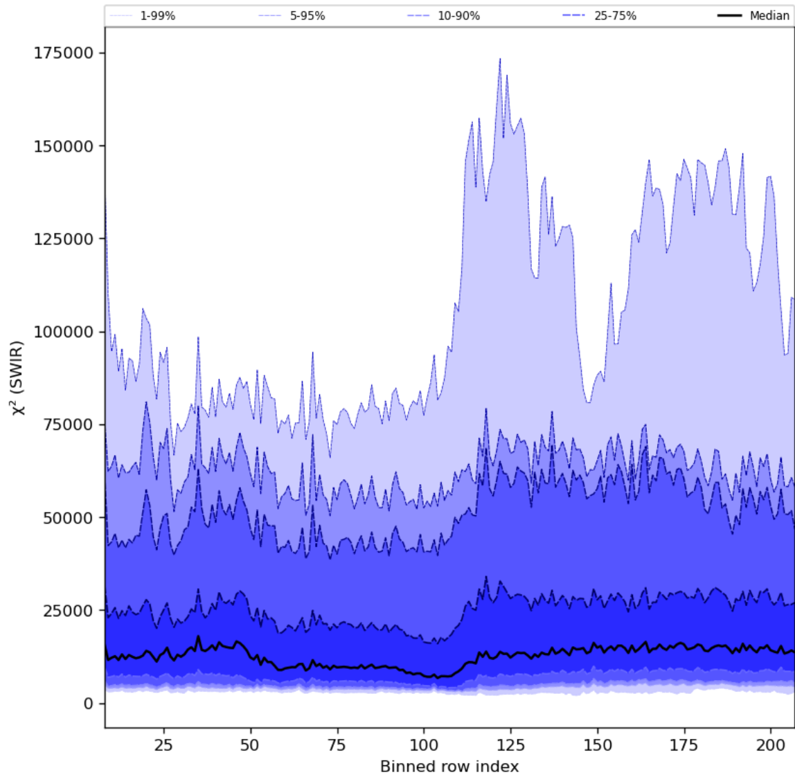
Figure 39: Along track statistics of " \chi^2 (SWIR)" for 2023-07-30 to 2023-08-01
