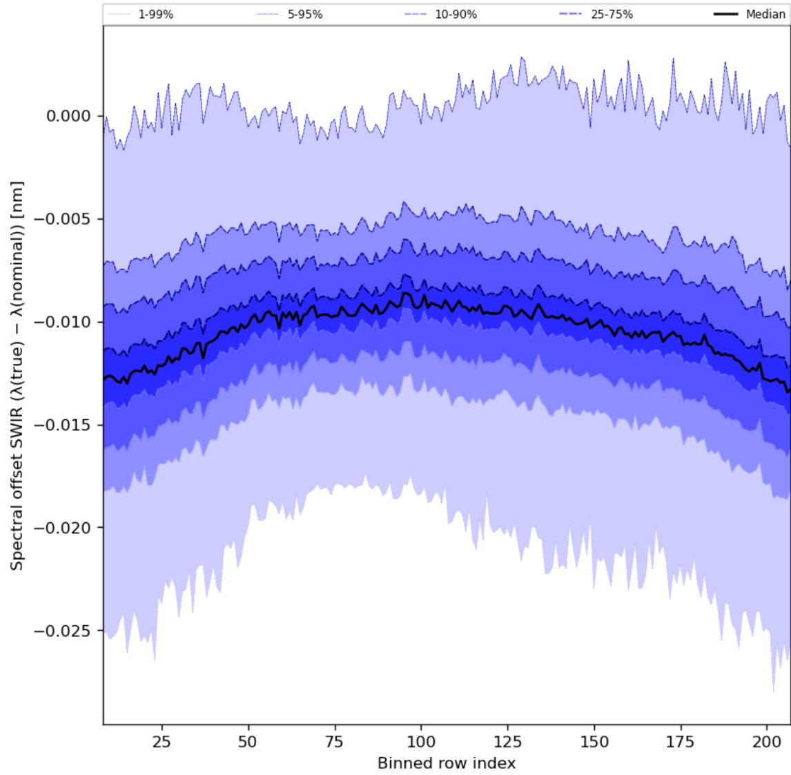
Figure 38: Along track statistics of “Spectral offset SWIR ( \lambda(\text{true}) - \lambda(\text{nominal}) )” for 2023-07-30 to 2023-08-01
