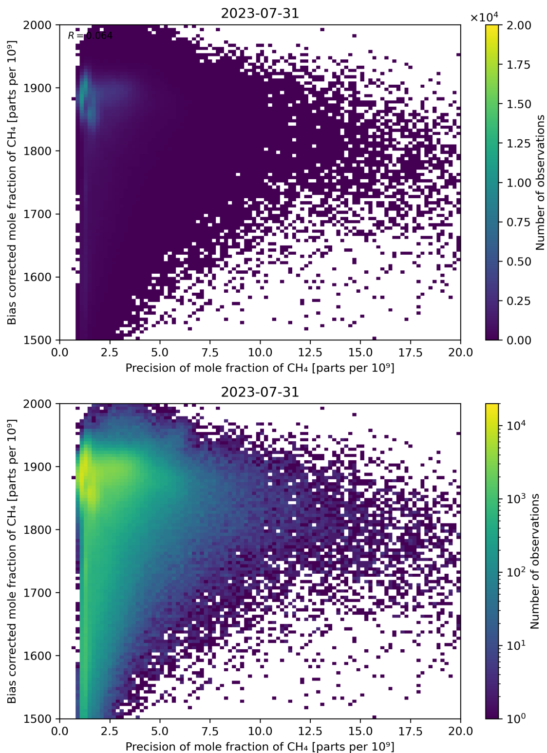
Figure 82: Scatter density plot of “Precision of mole fraction of CH 4 ” against “Bias corrected mole fraction of CH 4 ” for 2023-07-30 to 2023-08-01.
