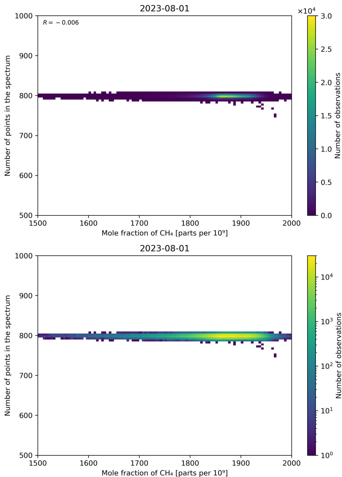
Figure 77: Scatter density plot of “Mole fraction of CH 4 ” against “Number of points in the spectrum” for 2023-07-31 to 2023-08-02.
