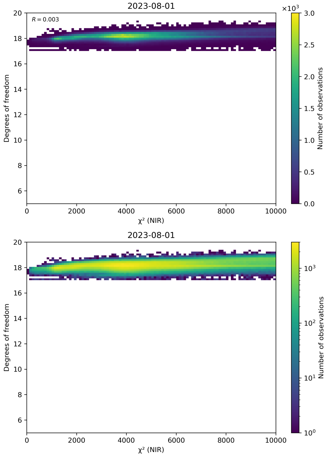
Figure 44: Scatter density plot of “ \chi^2 (NIR)” against “Degrees of freedom” for 2023-07-31 to 2023-08-02.
