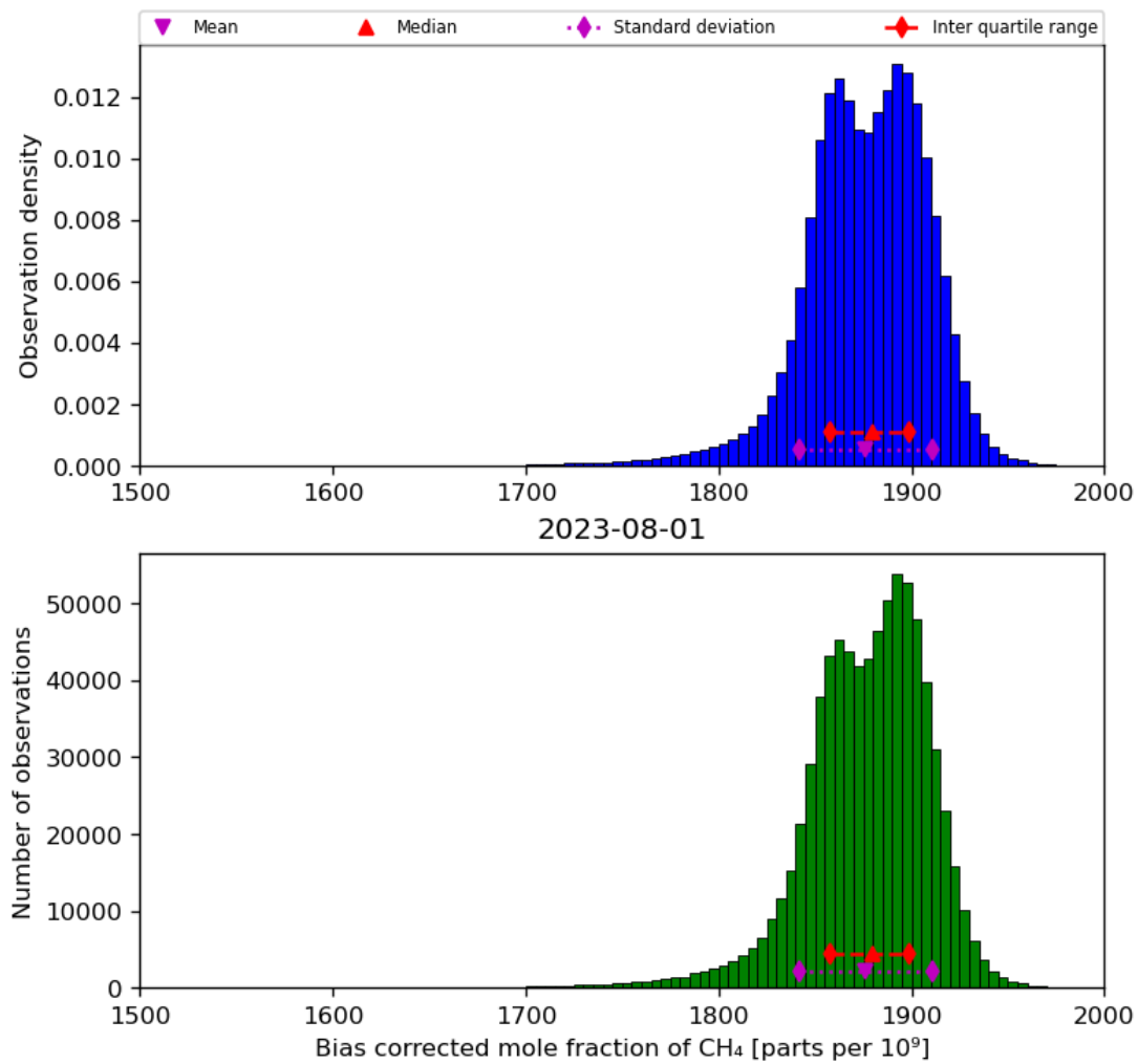
Figure 25: Histogram of “Bias corrected mole fraction of CH 4 ” for 2023-07-31 to 2023-08-02
