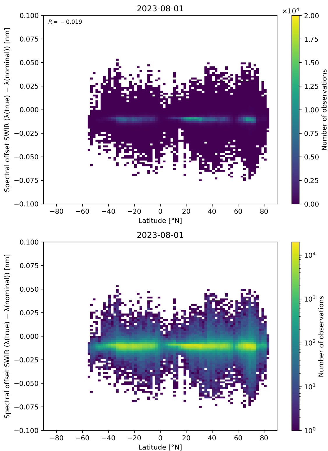
Figure 62: Scatter density plot of “Latitude” against “Spectral offset SWIR ( \lambda(\text{true}) - \lambda(\text{nominal}) )” for 2023-07-31 to 2023-08-02.
