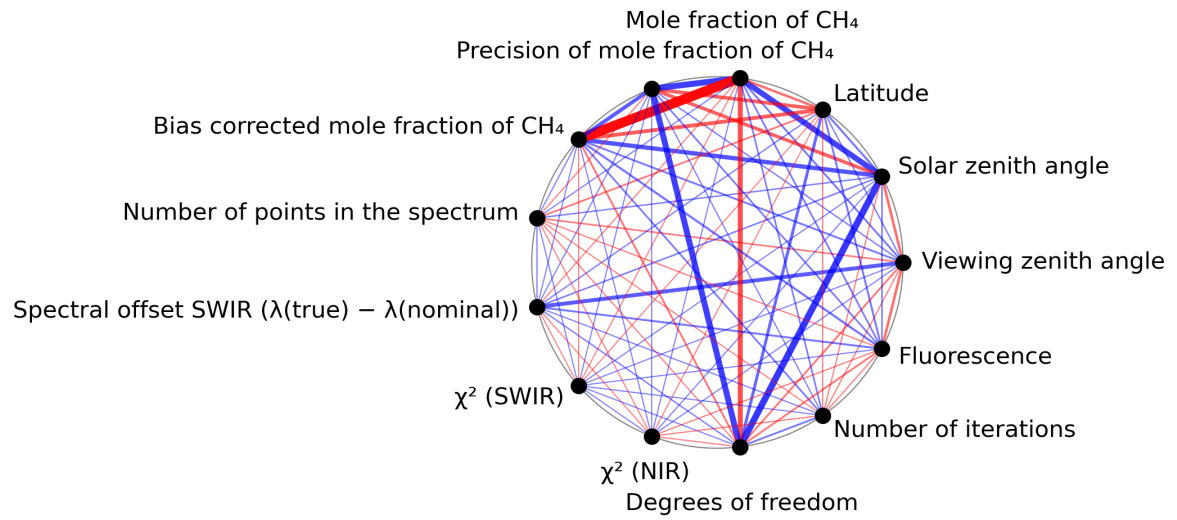
Figure 1: Map of correlation graph for 2023-07-31 to 2023-08-02.
