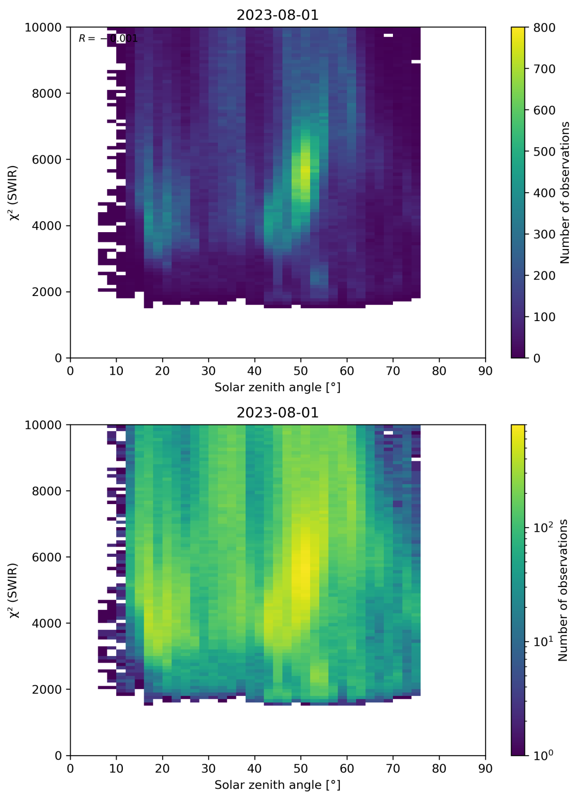
Figure 95: Scatter density plot of “Solar zenith angle” against “ \chi^2 (SWIR)” for 2023-07-31 to 2023-08-02.
