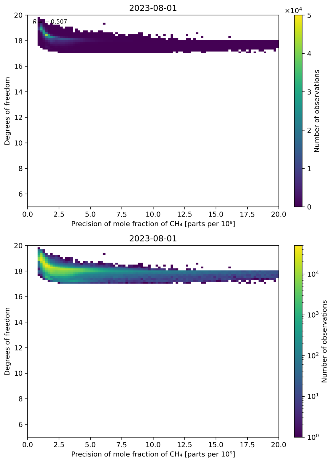
Figure 80: Scatter density plot of “Precision of mole fraction of CH 4 ” against “Degrees of freedom” for 2023-07-31 to 2023-08-02.
