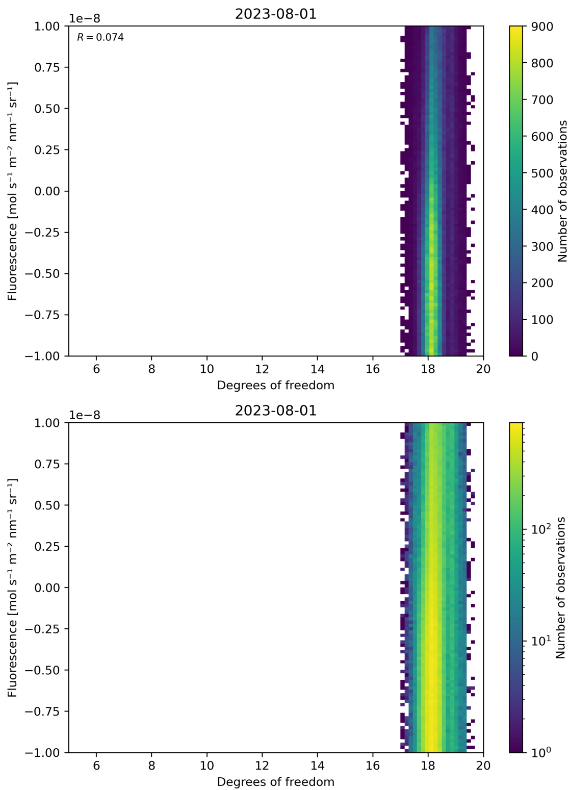
Figure 51: Scatter density plot of “Degrees of freedom” against “Fluorescence” for 2023-07-31 to 2023-08-02.
