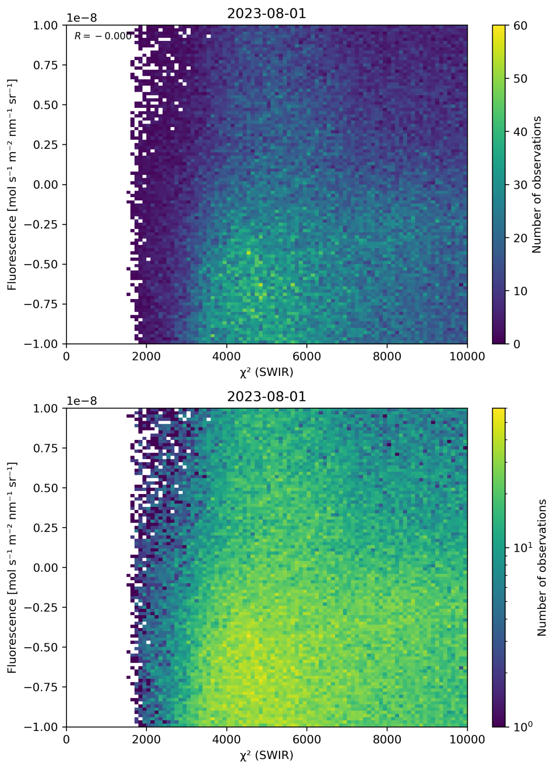
Figure 49: Scatter density plot of “ \chi^2 (SWIR)” against “Fluorescence” for 2023-07-31 to 2023-08-02.
