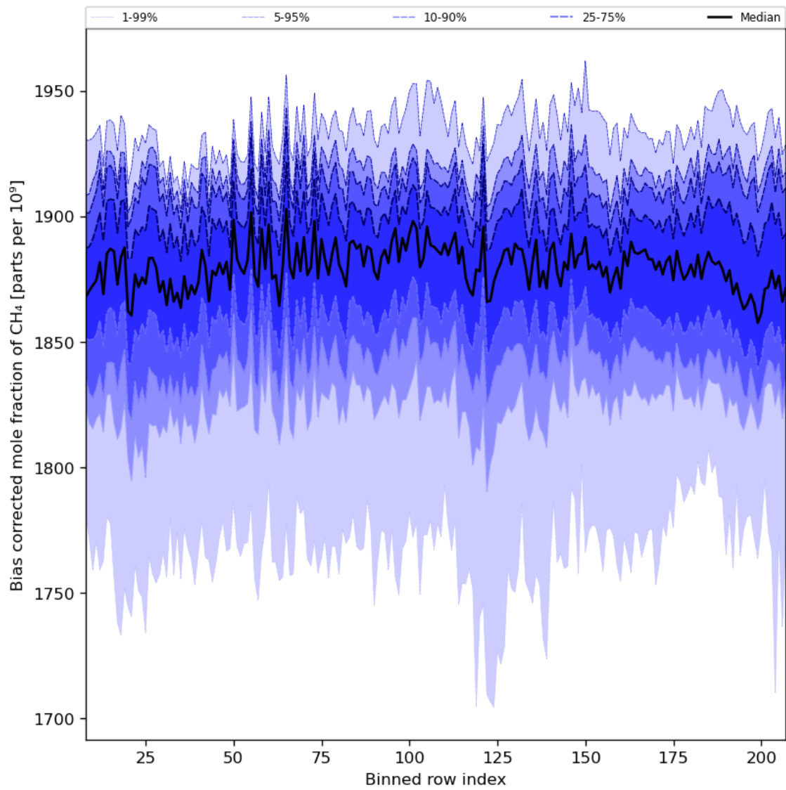
Figure 36: Along track statistics of “Bias corrected mole fraction of CH 4 ” for 2023-07-31 to 2023-08-02
