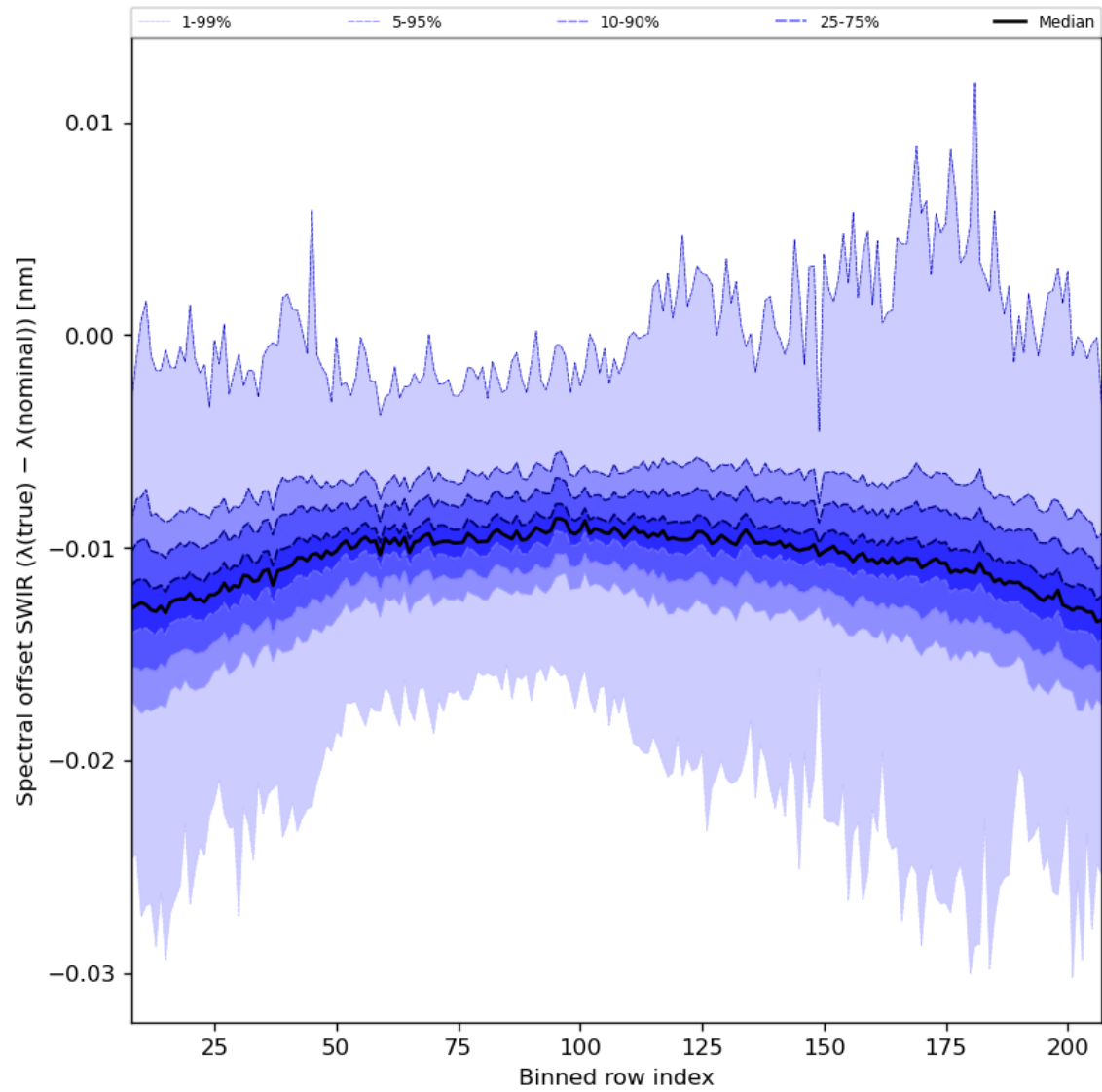
Figure 38: Along track statistics of “Spectral offset SWIR ( \lambda(\text{true}) - \lambda(\text{nominal}) )” for 2023-07-31 to 2023-08-02
