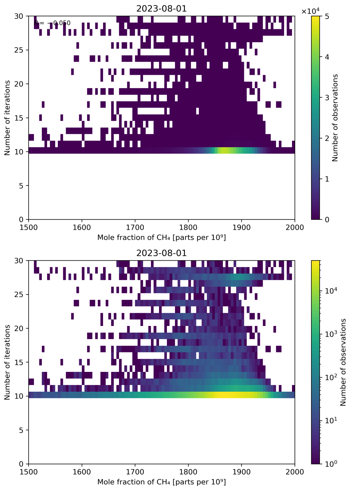
Figure 76: Scatter density plot of “Mole fraction of CH 4 ” against “Number of iterations” for 2023-07-31 to 2023-08-02.
