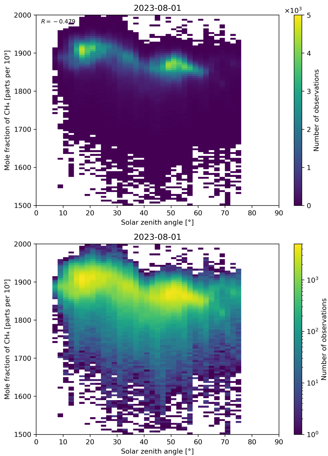
Figure 99: Scatter density plot of “Solar zenith angle” against “Mole fraction of CH 4 ” for 2023-07-31 to 2023-08-02.
