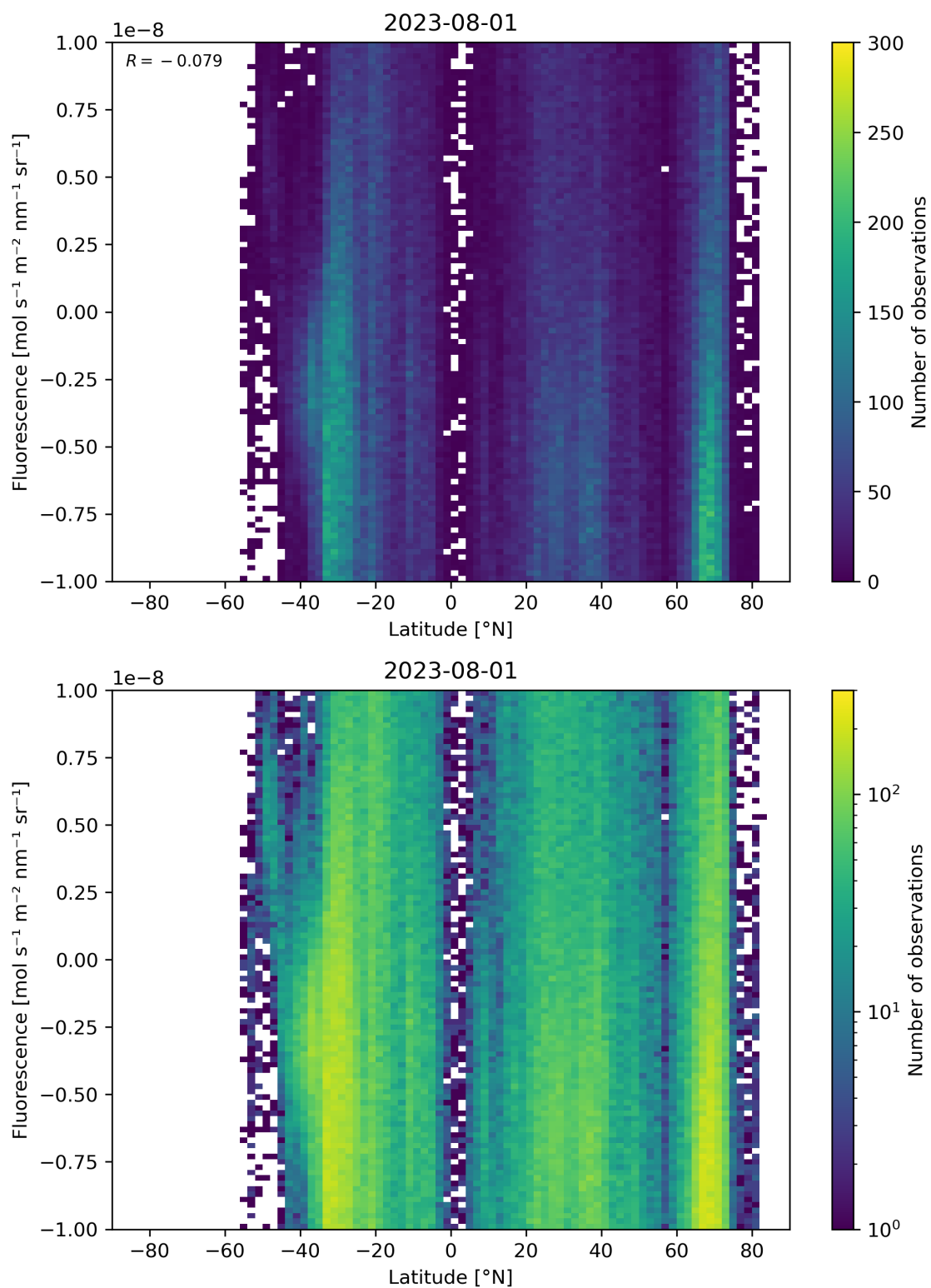
Figure 56: Scatter density plot of “Latitude” against “Fluorescence” for 2023-07-31 to 2023-08-02.
