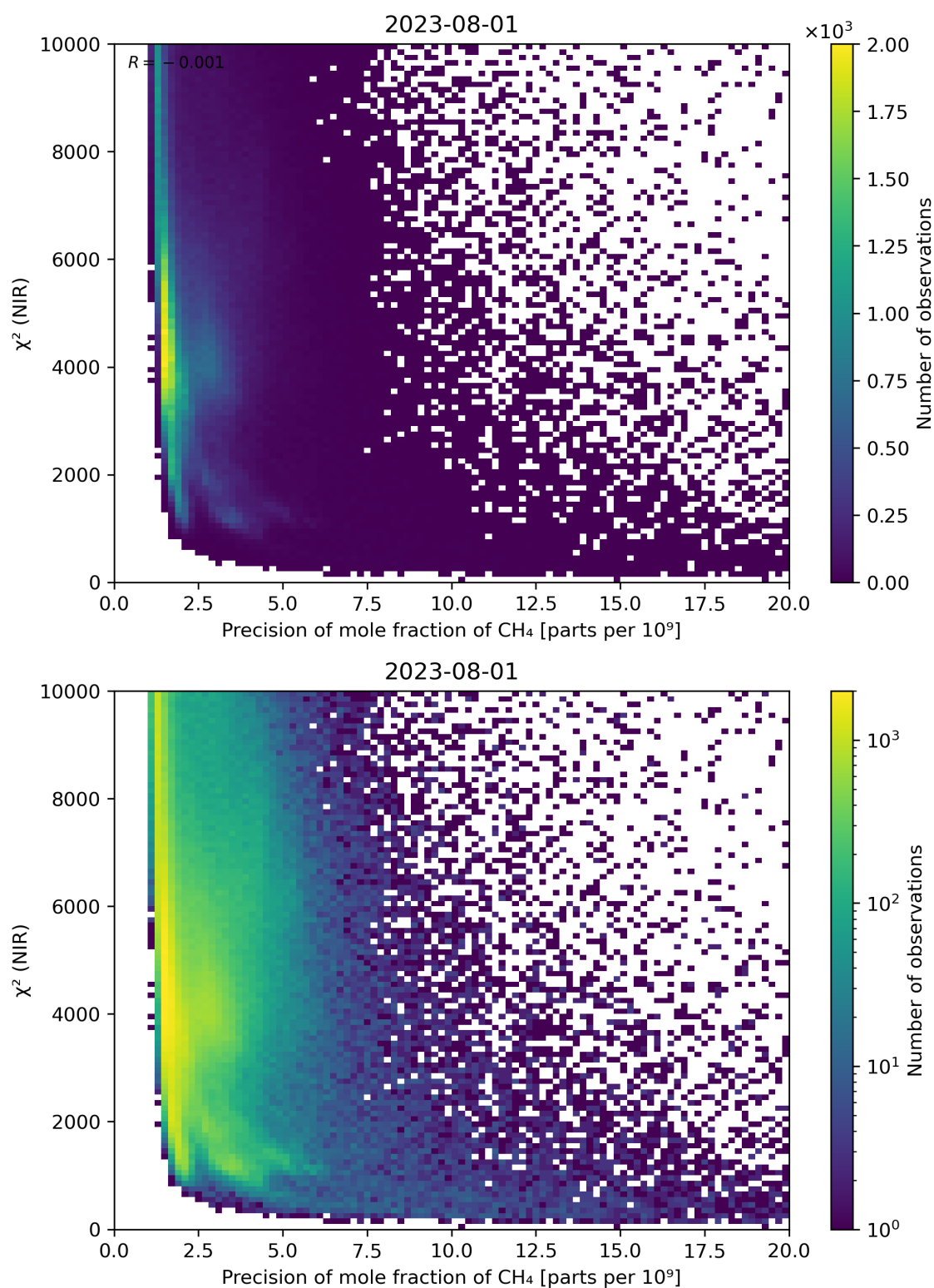
Figure 78: Scatter density plot of “Precision of mole fraction of CH 4 ” against “ \chi^2 (NIR)” for 2023-07-31 to 2023-08-02.
