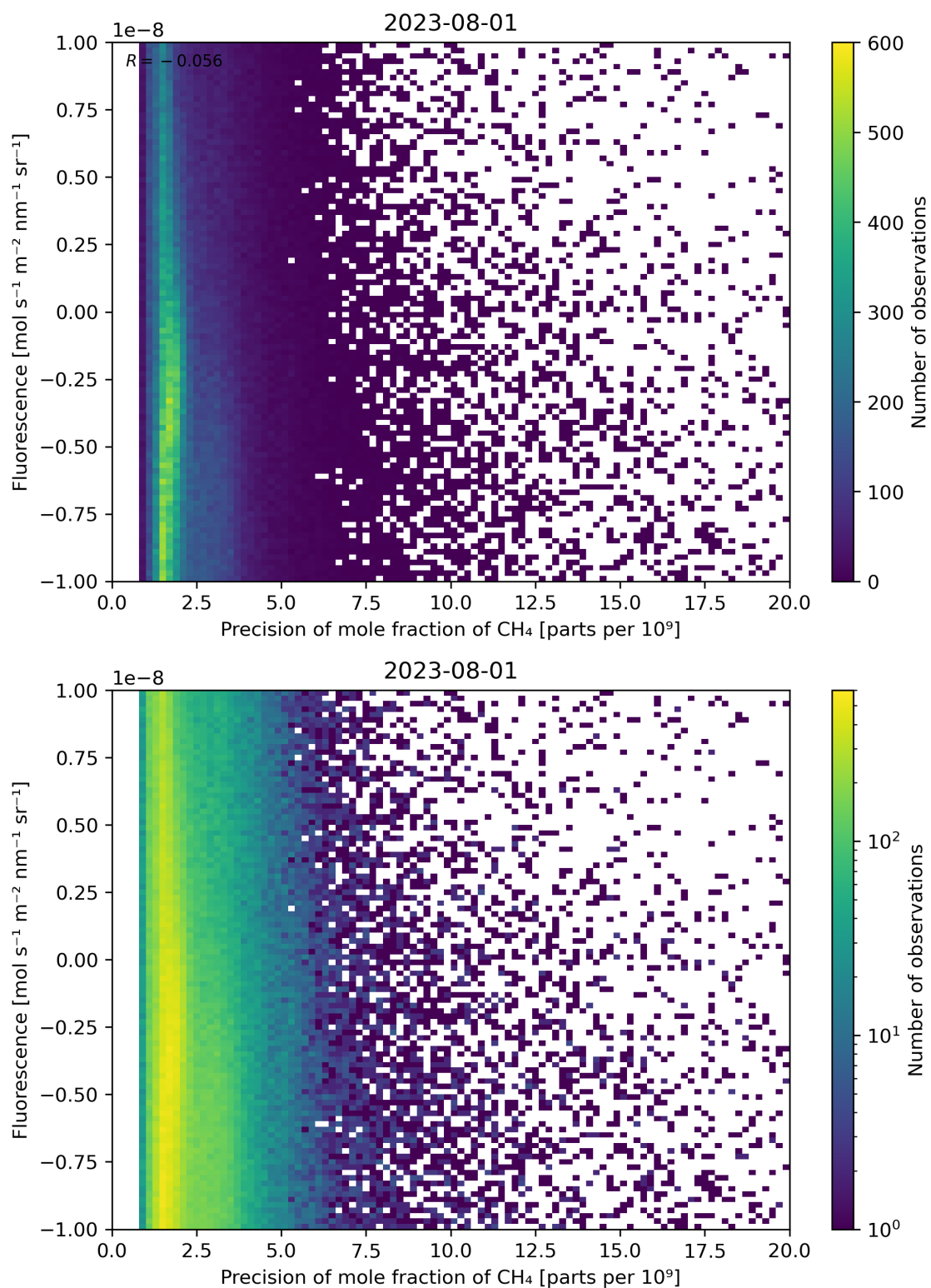
Figure 81: Scatter density plot of “Precision of mole fraction of \text{CH}_4 ” against “Fluorescence” for 2023-07-31 to 2023-08-02.
