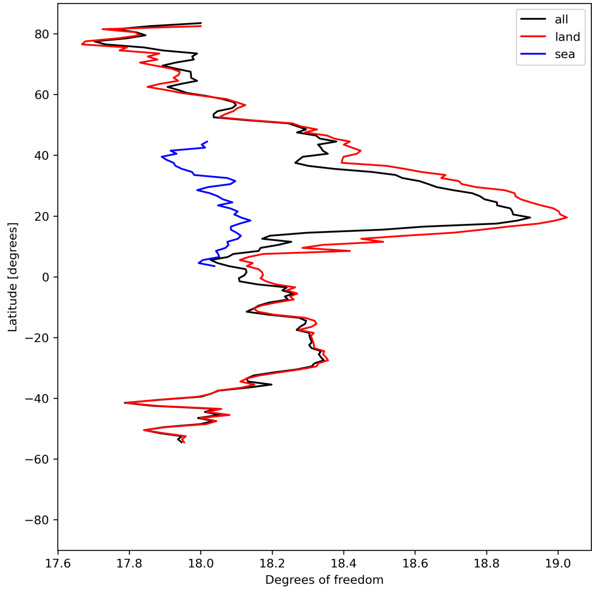
Figure 19: Zonal average of “Degrees of freedom” for 2023-07-31 to 2023-08-02.
