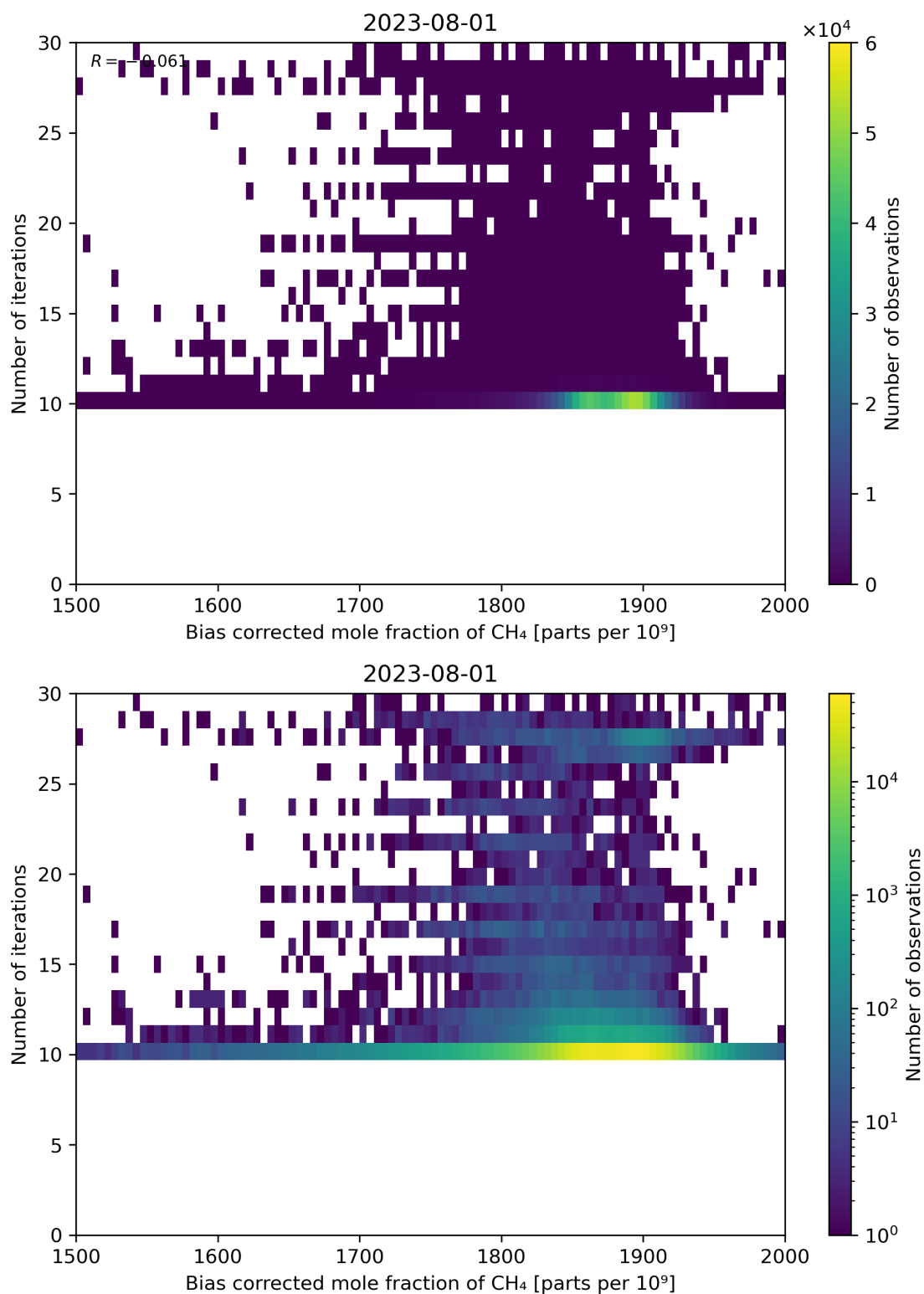
Figure 67: Scatter density plot of “Bias corrected mole fraction of CH 4 ” against “Number of iterations” for 2023-07-31 to 2023-08-02.
