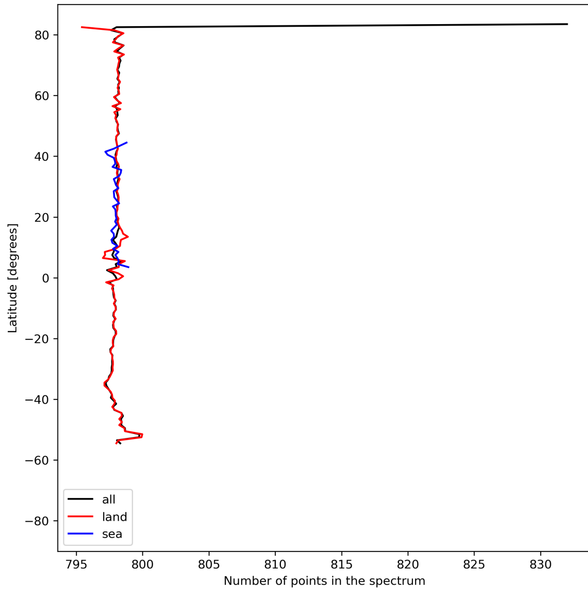
Figure 15: Zonal average of “Number of points in the spectrum” for 2023-07-31 to 2023-08-02.
