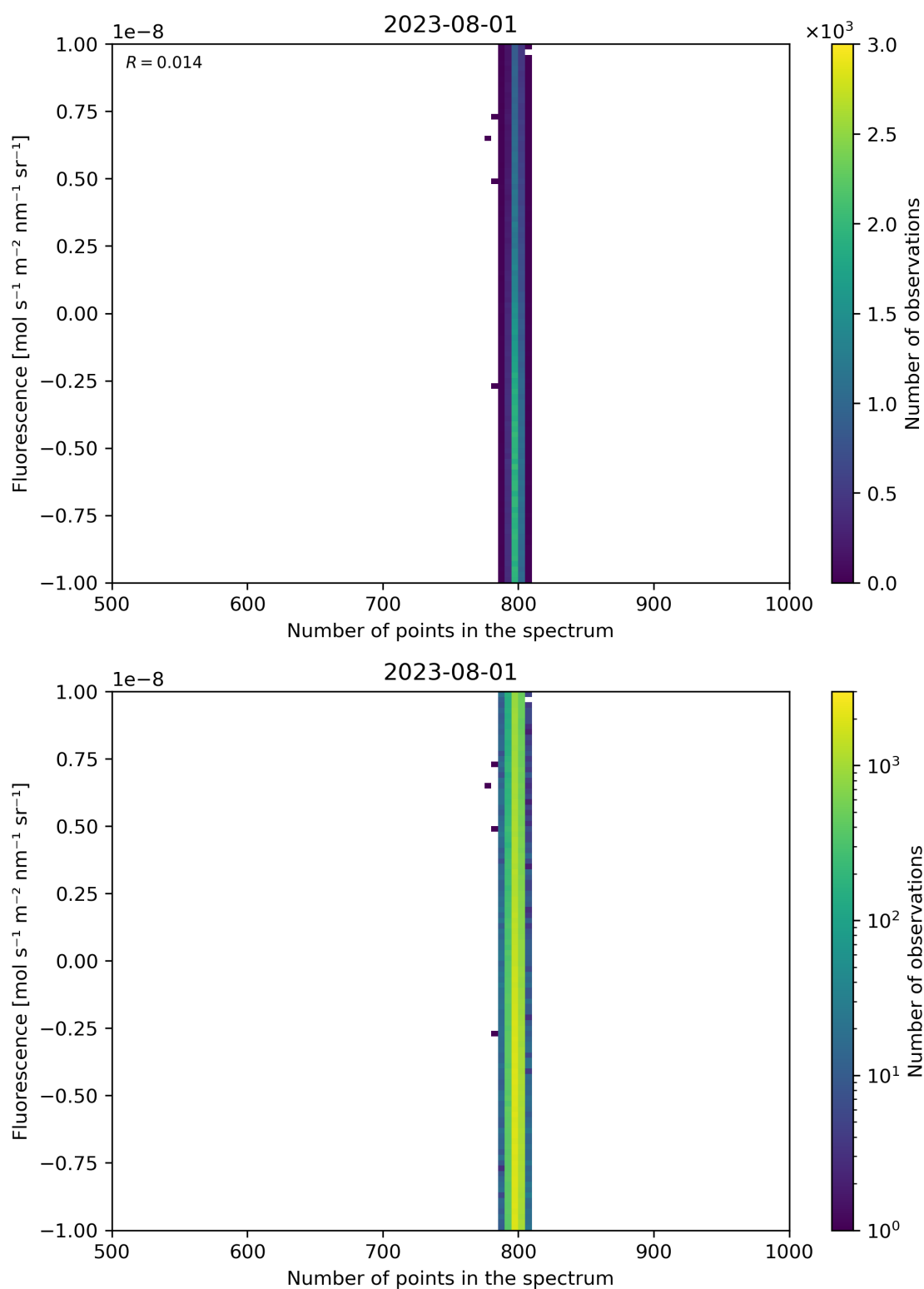
Figure 91: Scatter density plot of “Number of points in the spectrum” against “Fluorescence” for 2023-07-31 to 2023-08-02.
