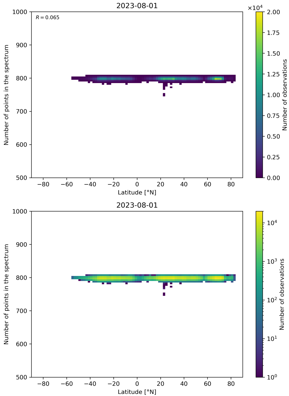
Figure 61: Scatter density plot of “Latitude” against “Number of points in the spectrum” for 2023-07-31 to 2023-08-02.
