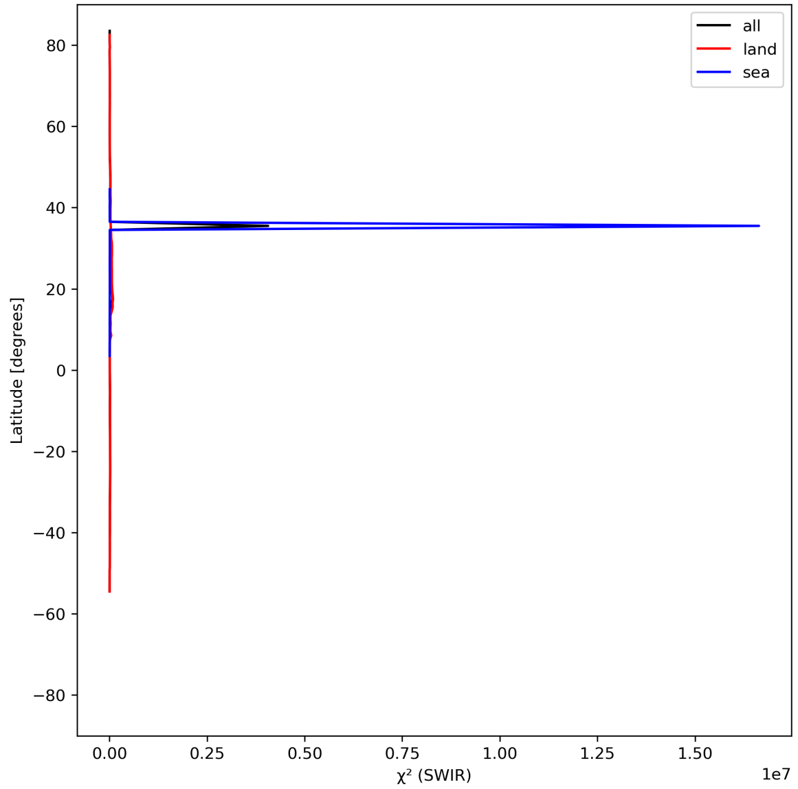
Figure 17: Zonal average of “ \chi^2 (SWIR)” for 2023-07-31 to 2023-08-02.
