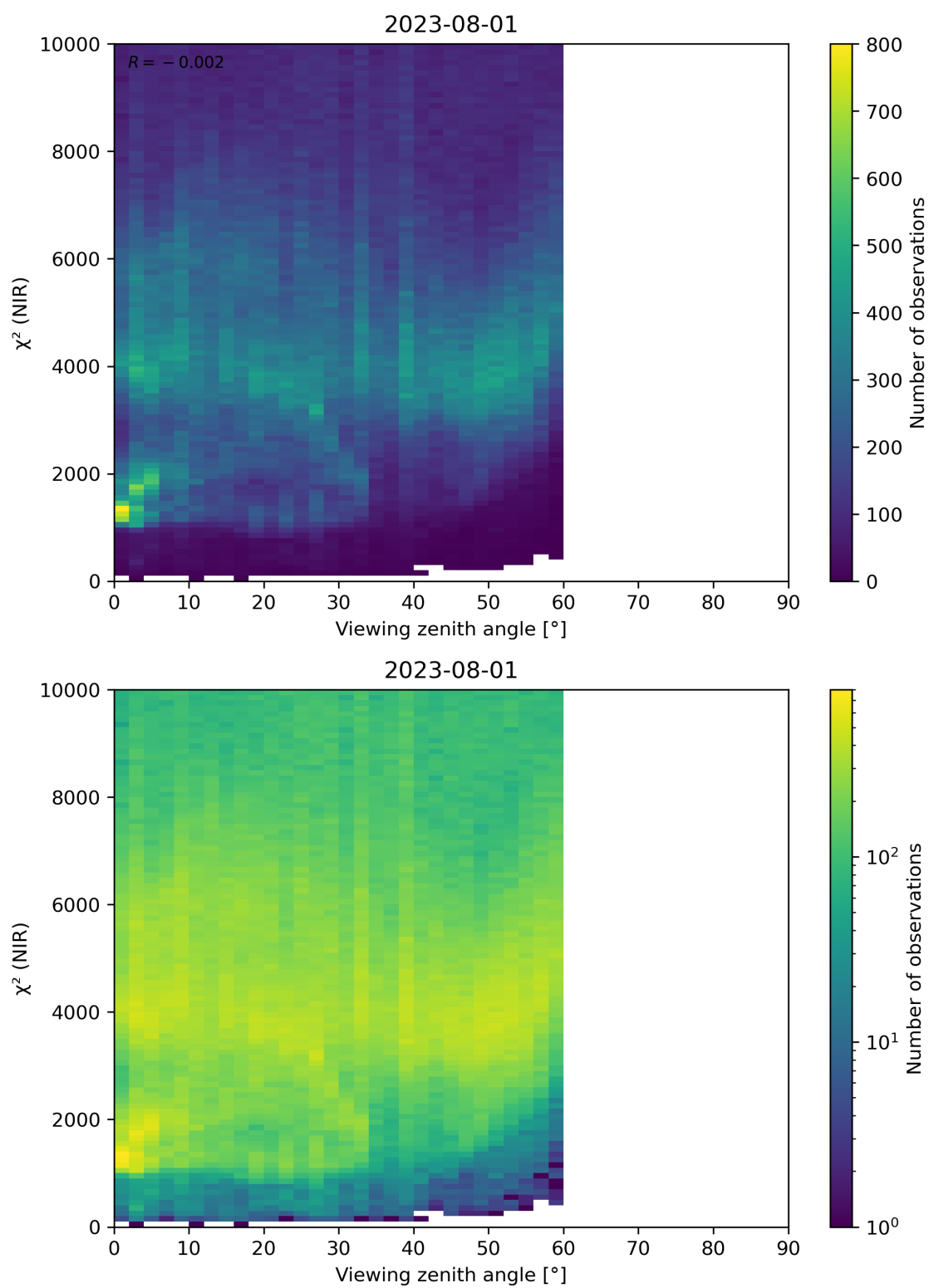
Figure 105: Scatter density plot of “Viewing zenith angle” against “ \chi^2 (NIR)” for 2023-07-31 to 2023-08-02.
