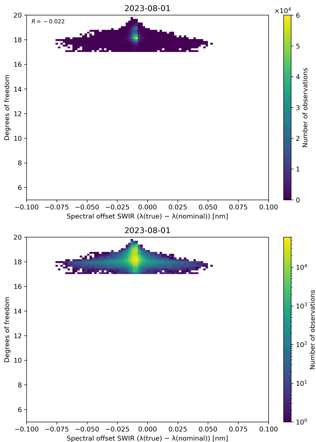
Figure 119: Scatter density plot of “Spectral offset SWIR ( \lambda(\text{true}) - \lambda(\text{nominal}) )” against “Degrees of freedom” for 2023-07-31 to 2023-08-02.
