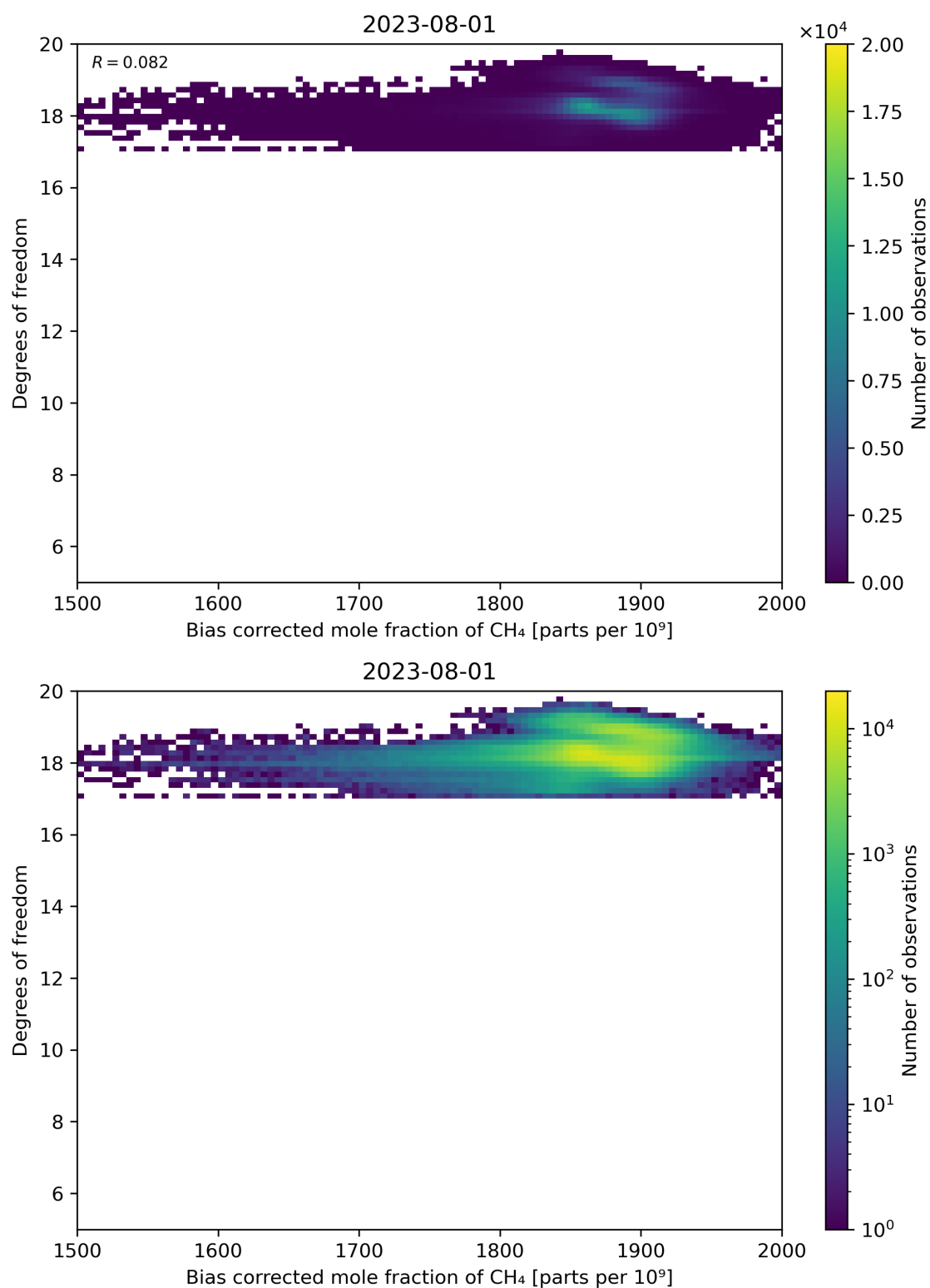
Figure 65: Scatter density plot of “Bias corrected mole fraction of CH 4 ” against “Degrees of freedom” for 2023-07-31 to 2023-08-02.
