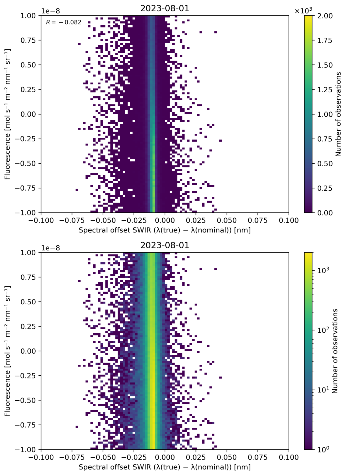
Figure 120: Scatter density plot of “Spectral offset SWIR ( \lambda(\text{true}) - \lambda(\text{nominal}) )” against “Fluorescence” for 2023-07-31 to 2023-08-02.
