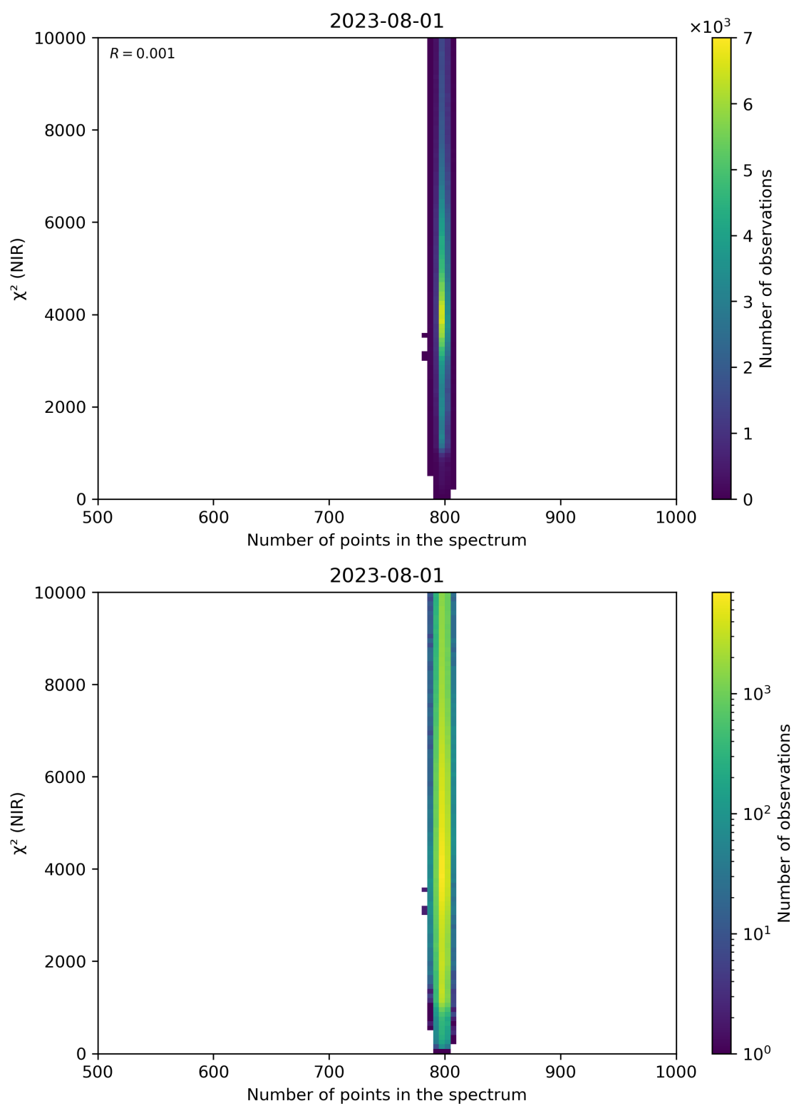
Figure 88: Scatter density plot of “Number of points in the spectrum” against “ \chi^2 (NIR)” for 2023-07-31 to 2023-08-02.
