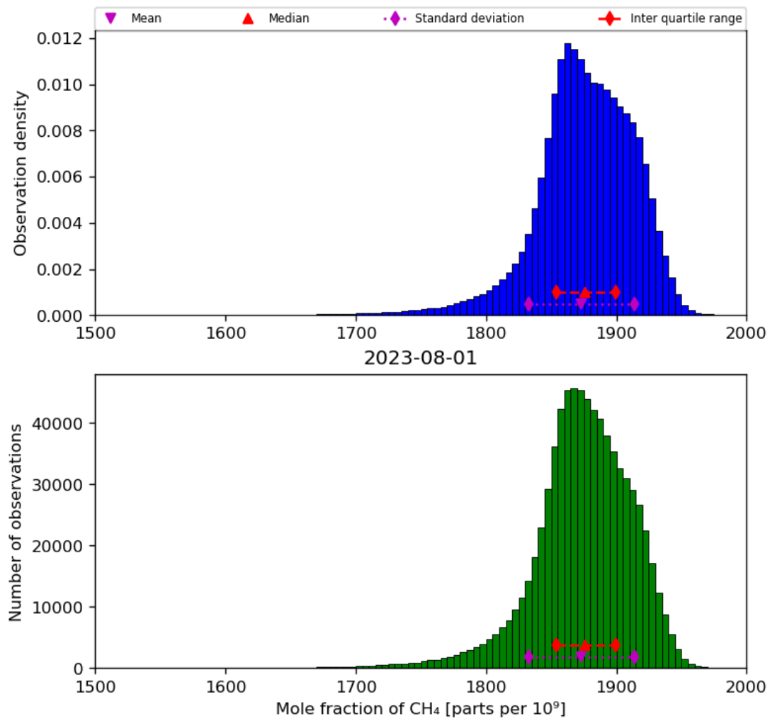
Figure 23: Histogram of “Mole fraction of CH 4 ” for 2023-07-31 to 2023-08-02
