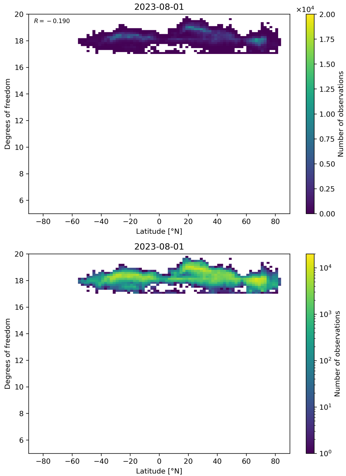
Figure 55: Scatter density plot of “Latitude” against “Degrees of freedom” for 2023-07-31 to 2023-08-02.
