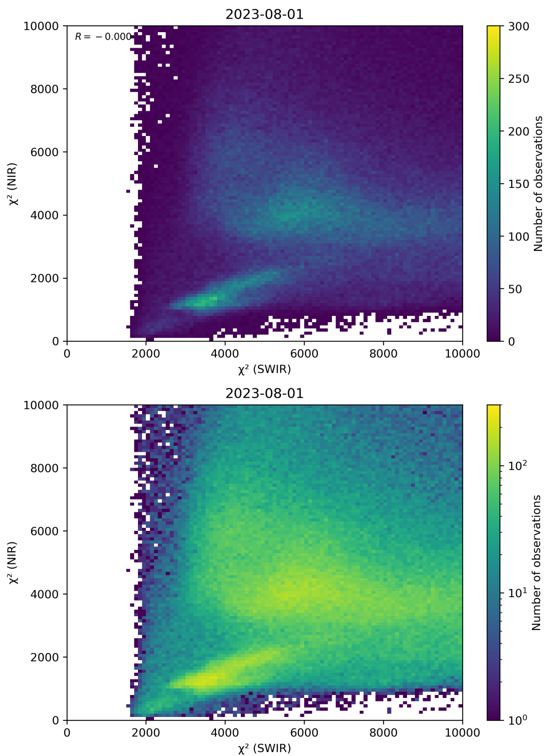
Figure 47: Scatter density plot of “ \chi^2 (SWIR)” against “ \chi^2 (NIR)” for 2023-07-31 to 2023-08-02.
