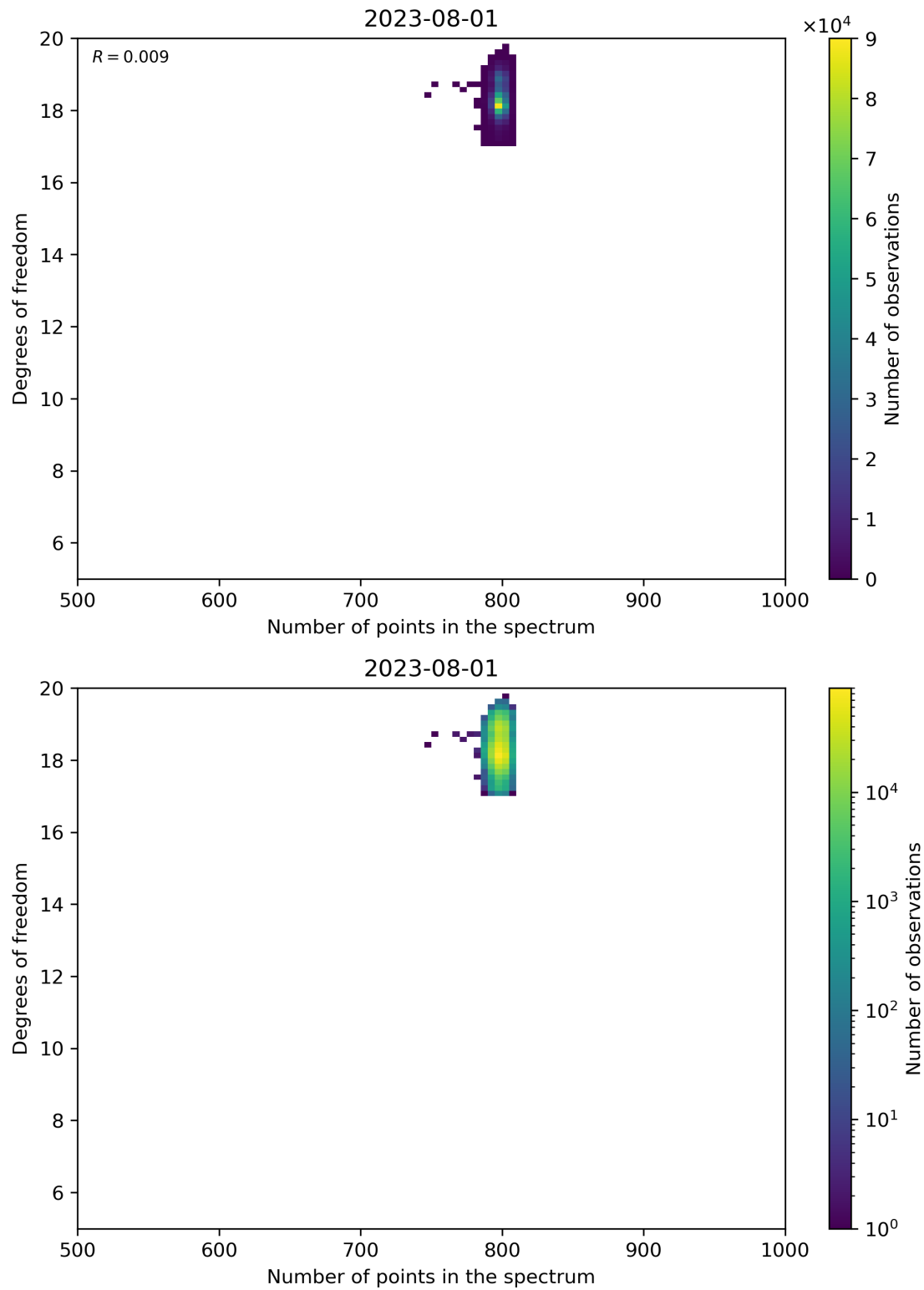
Figure 90: Scatter density plot of “Number of points in the spectrum” against “Degrees of freedom” for 2023-07-31 to 2023-08-02.
