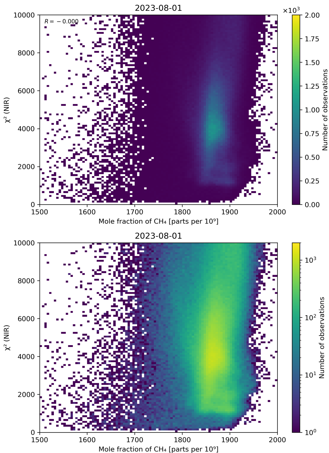
Figure 70: Scatter density plot of “Mole fraction of \text{CH}_4 ” against “ \chi^2 (NIR)” for 2023-07-31 to 2023-08-02.
