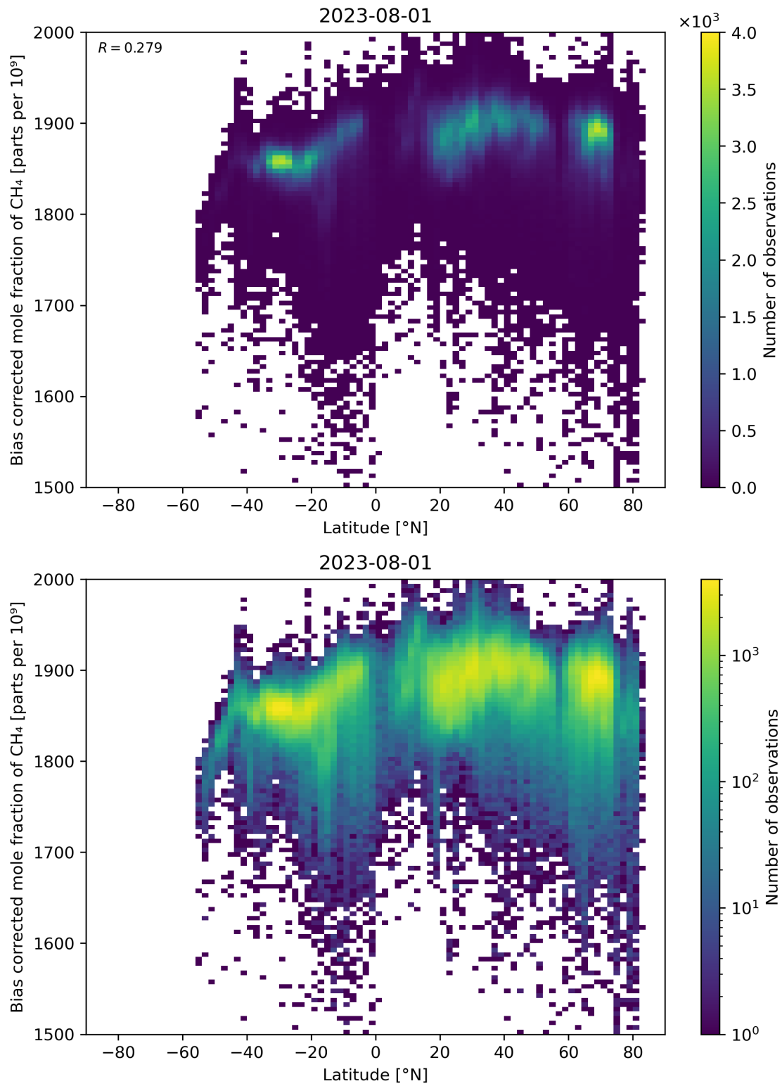
Figure 58: Scatter density plot of “Latitude” against “Bias corrected mole fraction of CH 4 ” for 2023-07-31 to 2023-08-02.
