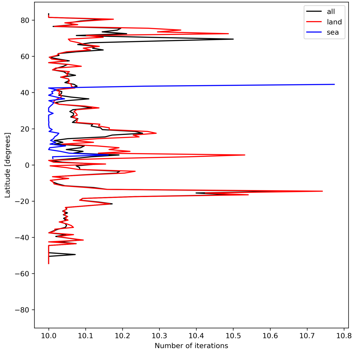
Figure 20: Zonal average of “Number of iterations” for 2023-07-31 to 2023-08-02.
