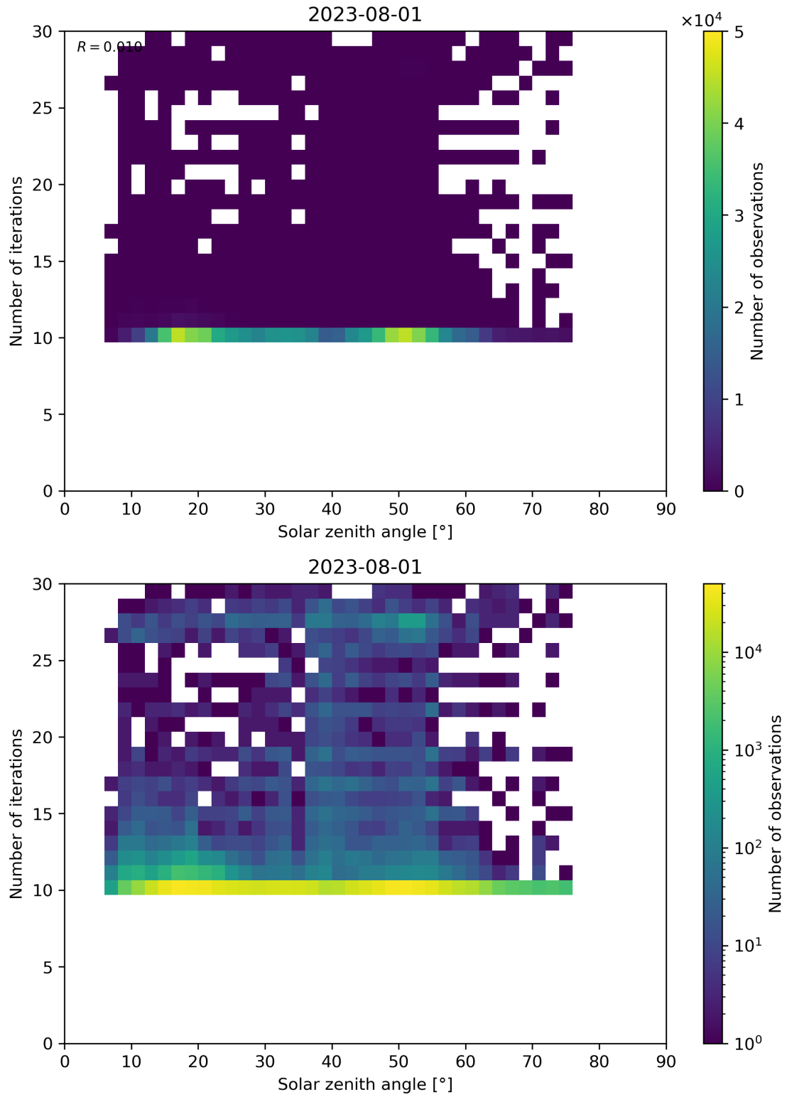
Figure 102: Scatter density plot of “Solar zenith angle” against “Number of iterations” for 2023-07-31 to 2023-08-02.
