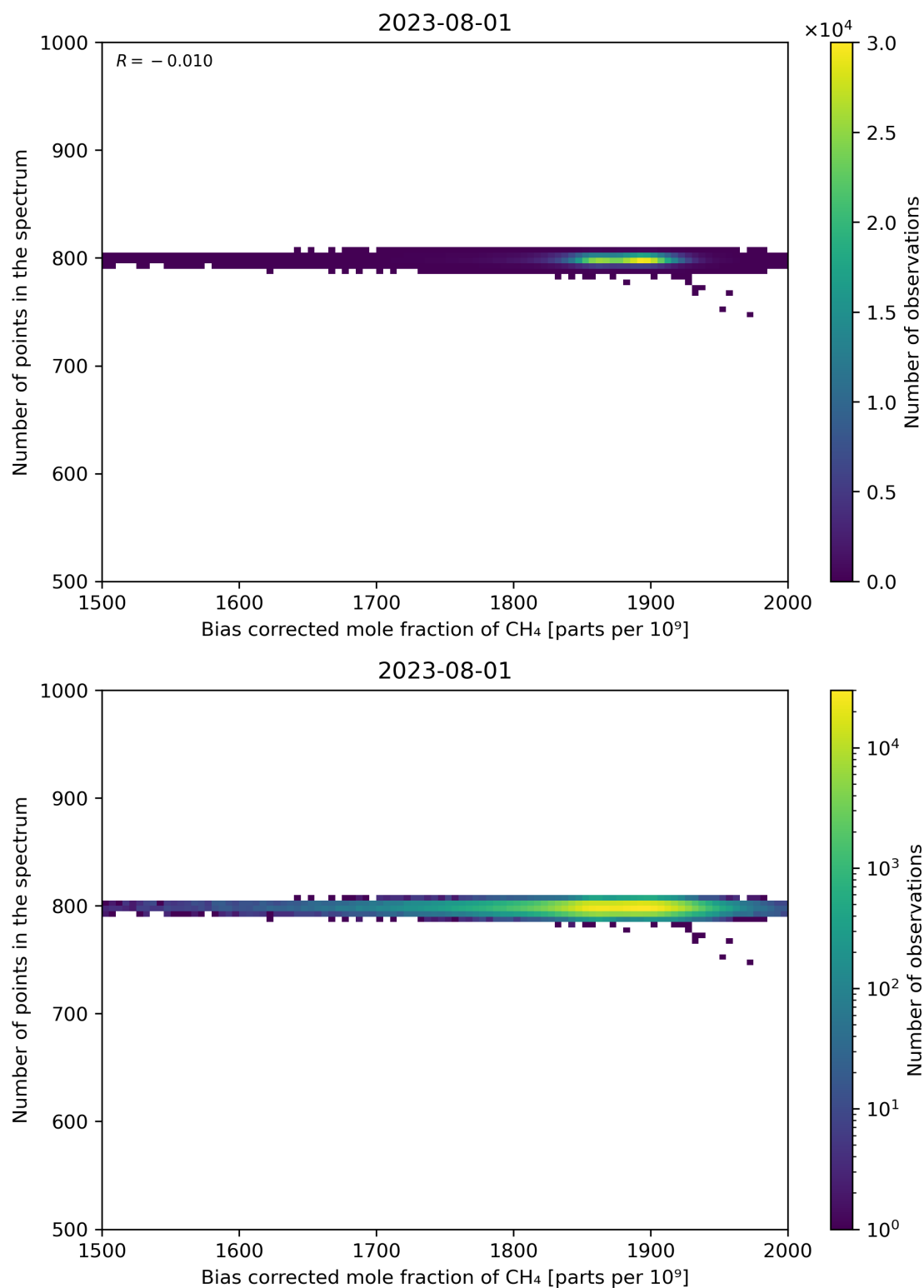
Figure 68: Scatter density plot of “Bias corrected mole fraction of CH 4 ” against “Number of points in the spectrum” for 2023-07-31 to 2023-08-02.
