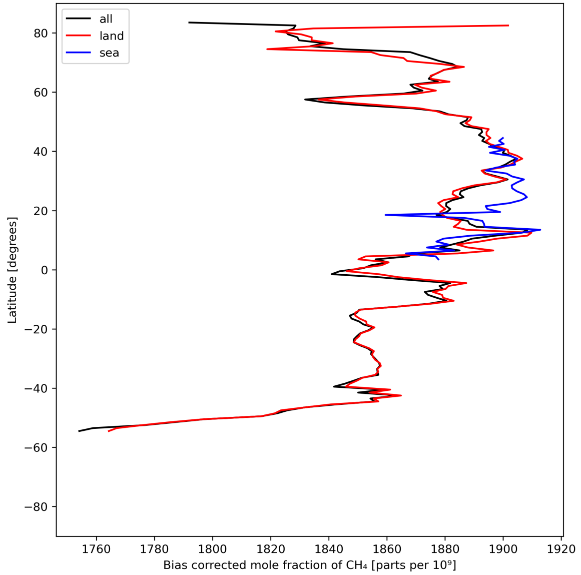
Figure 14: Zonal average of “Bias corrected mole fraction of CH 4 ” for 2023-07-31 to 2023-08-02.
