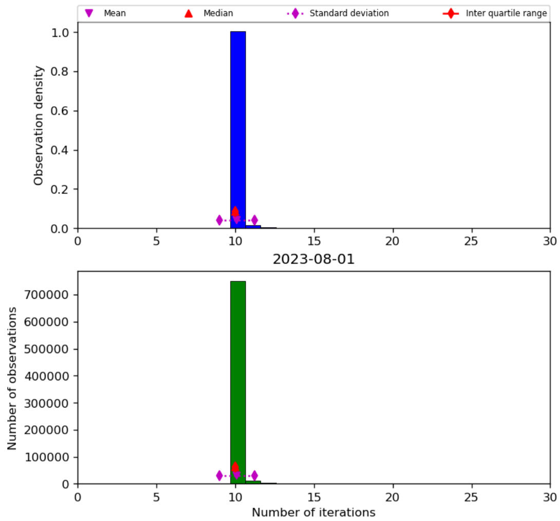
Figure 31: Histogram of “Number of iterations” for 2023-07-31 to 2023-08-02
