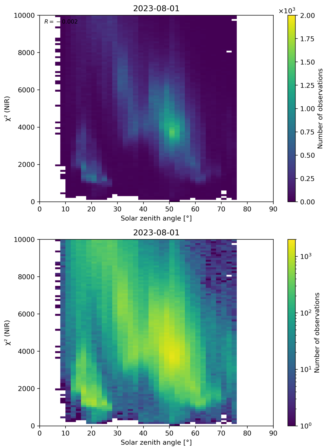
Figure 94: Scatter density plot of “Solar zenith angle” against “ \chi^2 (NIR)” for 2023-07-31 to 2023-08-02.
