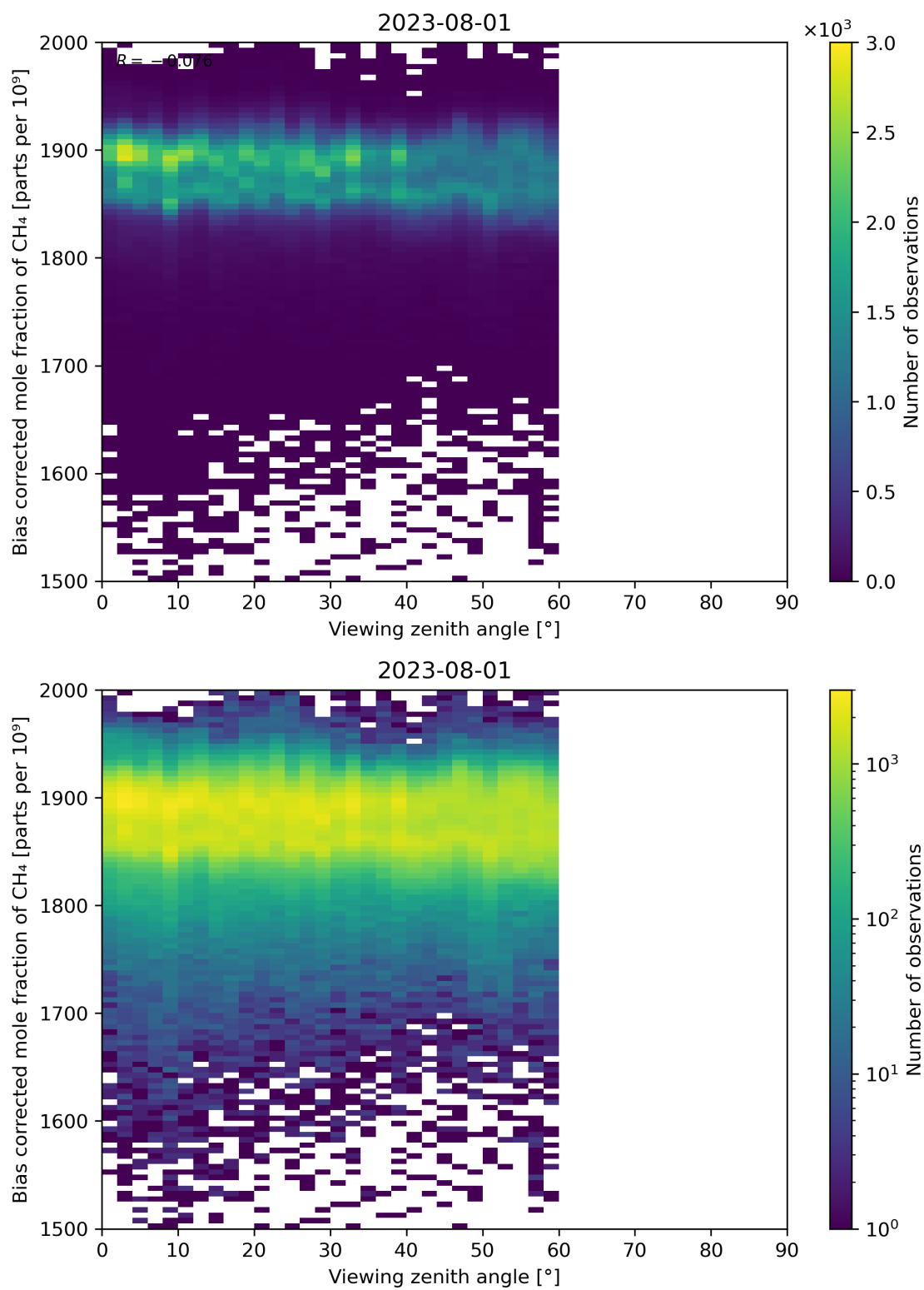
Figure 111: Scatter density plot of “Viewing zenith angle” against “Bias corrected mole fraction of CH 4 ” for 2023-07-31 to 2023-08-02.
