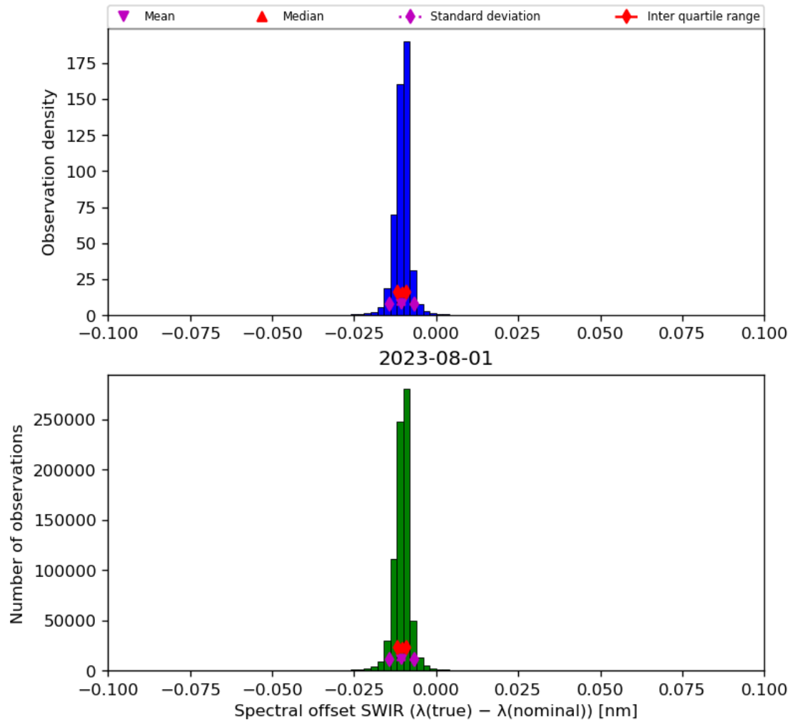
Figure 27: Histogram of “Spectral offset SWIR ( \lambda(\text{true}) - \lambda(\text{nominal}) )” for 2023-07-31 to 2023-08-02
