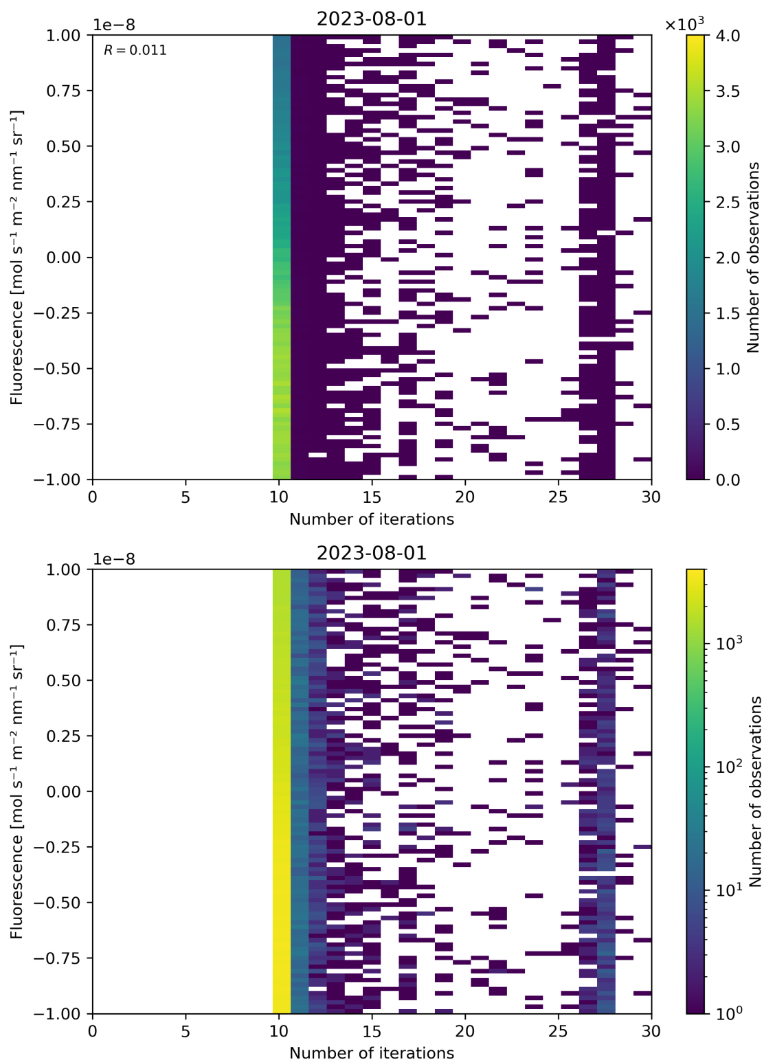
Figure 87: Scatter density plot of “Number of iterations” against “Fluorescence” for 2023-07-31 to 2023-08-02.
