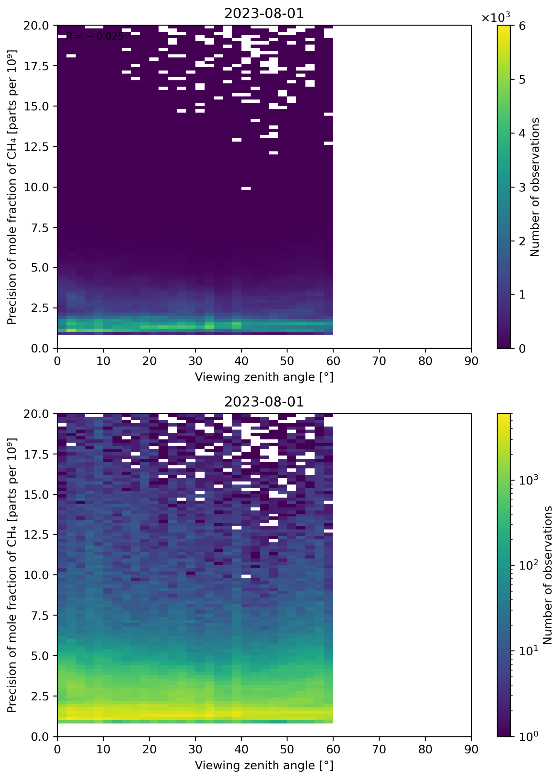
Figure 112: Scatter density plot of “Viewing zenith angle” against “Precision of mole fraction of CH 4 ” for 2023-07-31 to 2023-08-02.
