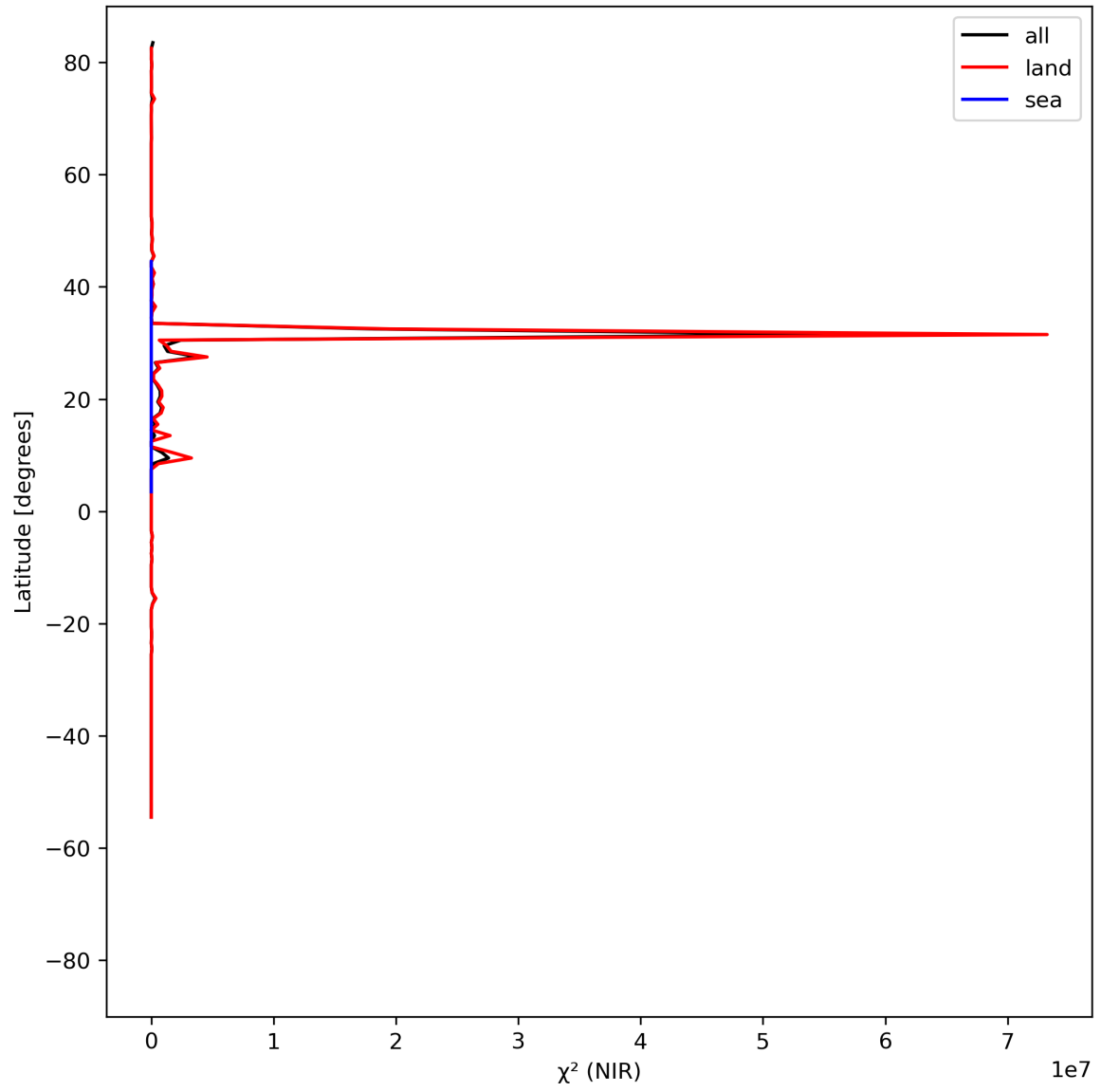
Figure 18: Zonal average of “ \chi^2 (NIR)” for 2023-07-31 to 2023-08-02.
