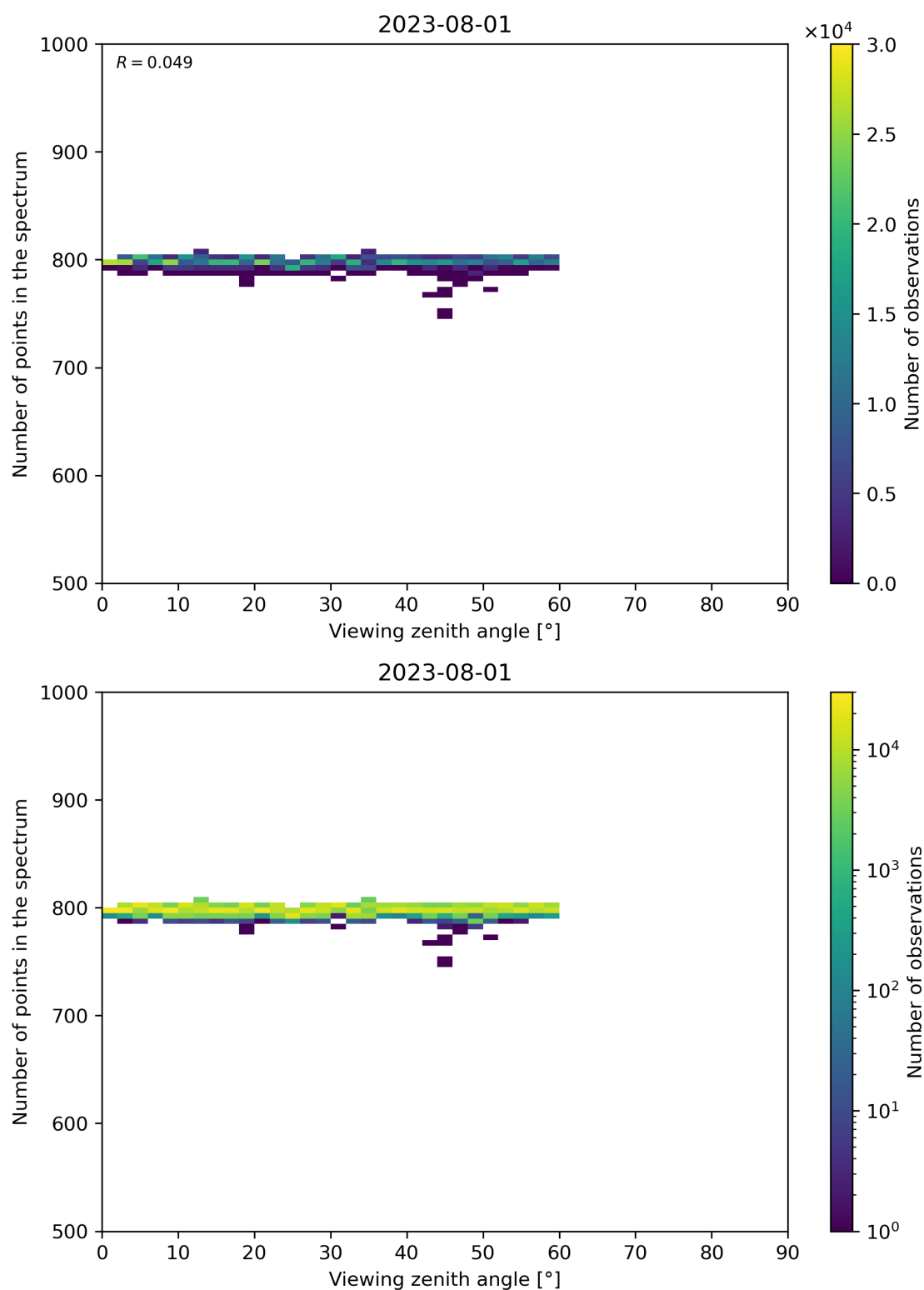
Figure 114: Scatter density plot of “Viewing zenith angle” against “Number of points in the spectrum” for 2023-07-31 to 2023-08-02.
