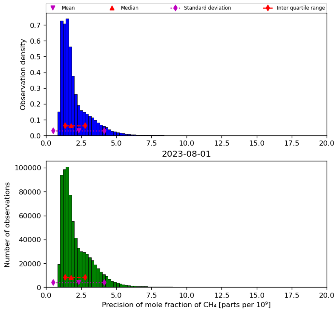
Figure 24: Histogram of “Precision of mole fraction of CH 4 ” for 2023-07-31 to 2023-08-02
