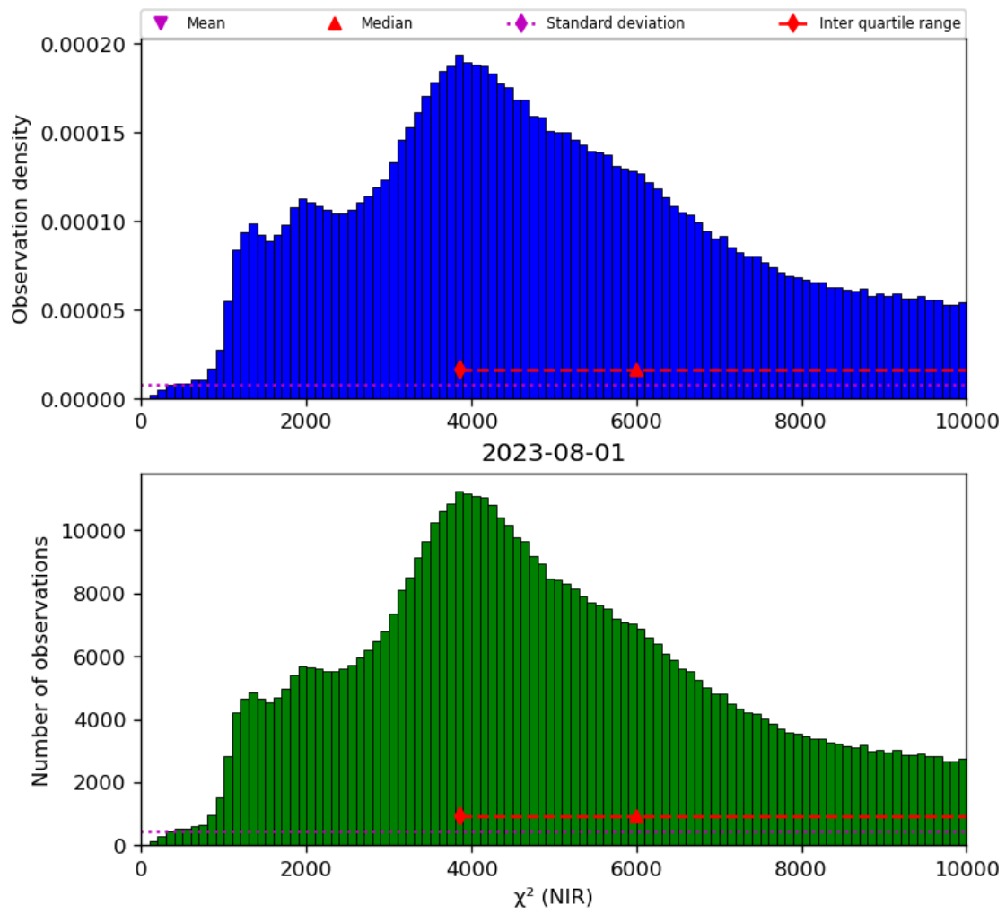
Figure 29: Histogram of " \chi^2 (NIR)" for 2023-07-31 to 2023-08-02
