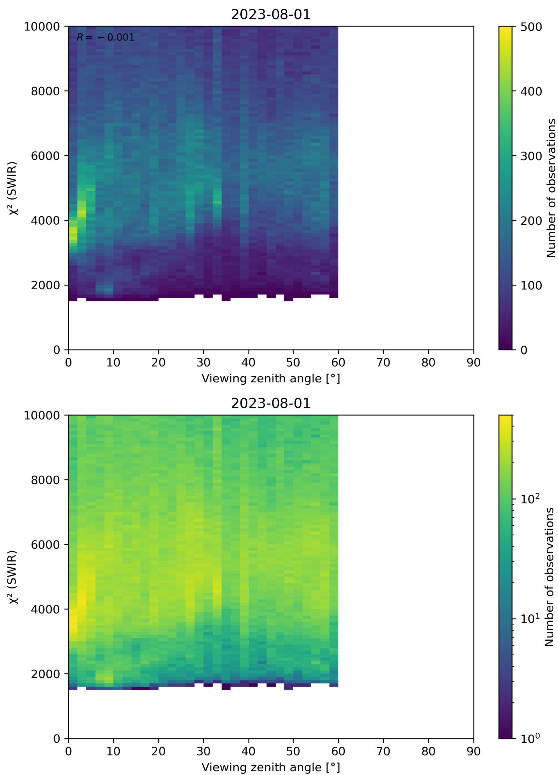
Figure 106: Scatter density plot of “Viewing zenith angle” against “ \chi^2 (SWIR)” for 2023-07-31 to 2023-08-02.
