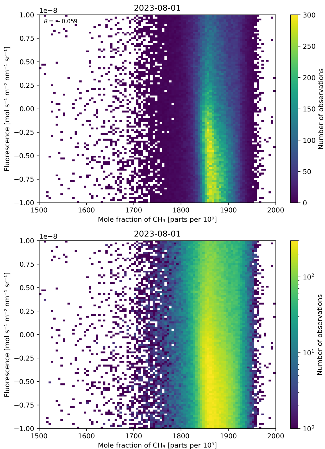
Figure 73: Scatter density plot of “Mole fraction of \text{CH}_4 ” against “Fluorescence” for 2023-07-31 to 2023-08-02.
