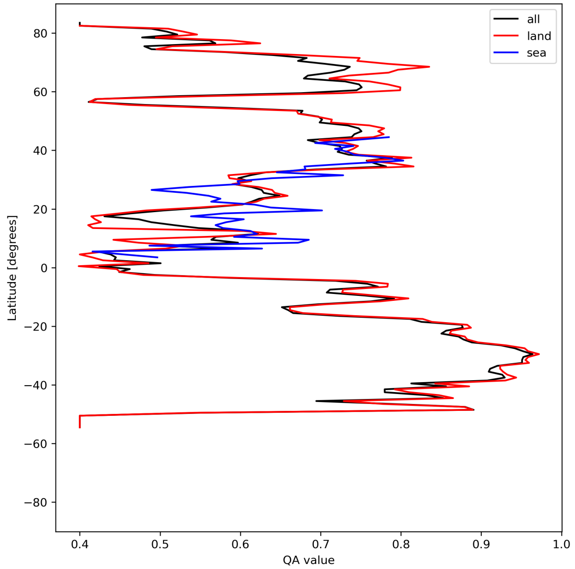
Figure 11: Zonal average of “QA value” for 2023-07-31 to 2023-08-02.
