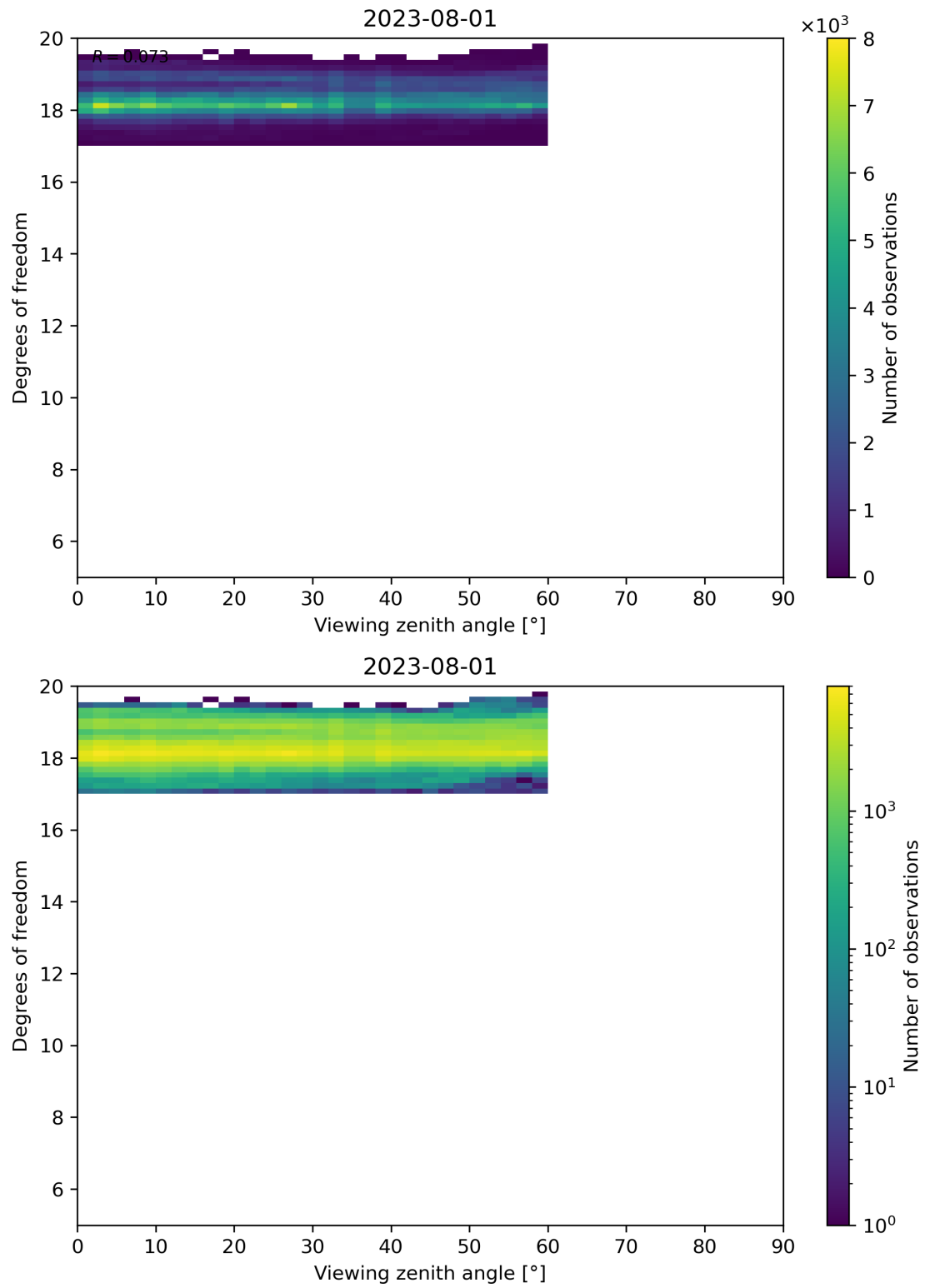
Figure 107: Scatter density plot of “Viewing zenith angle” against “Degrees of freedom” for 2023-07-31 to 2023-08-02.
