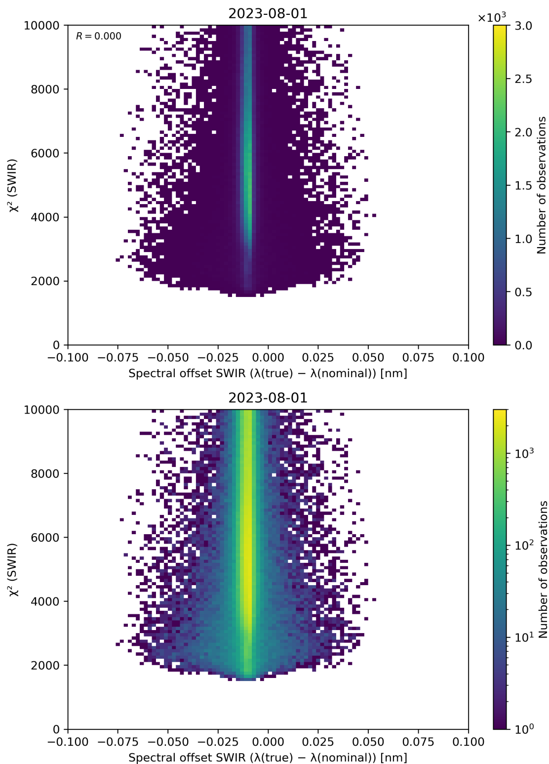
Figure 118: Scatter density plot of “Spectral offset SWIR ( \lambda(\text{true}) - \lambda(\text{nominal}) )” against “ \chi^2 (SWIR)” for 2023-07-31 to 2023-08-02.
