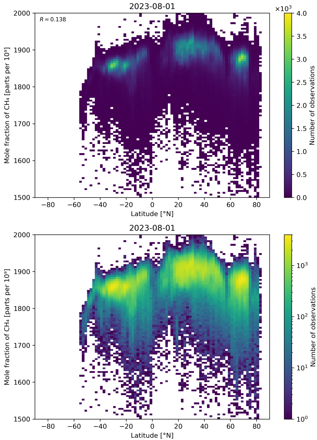
Figure 57: Scatter density plot of “Latitude” against “Mole fraction of \text{CH}_4 ” for 2023-07-31 to 2023-08-02.
