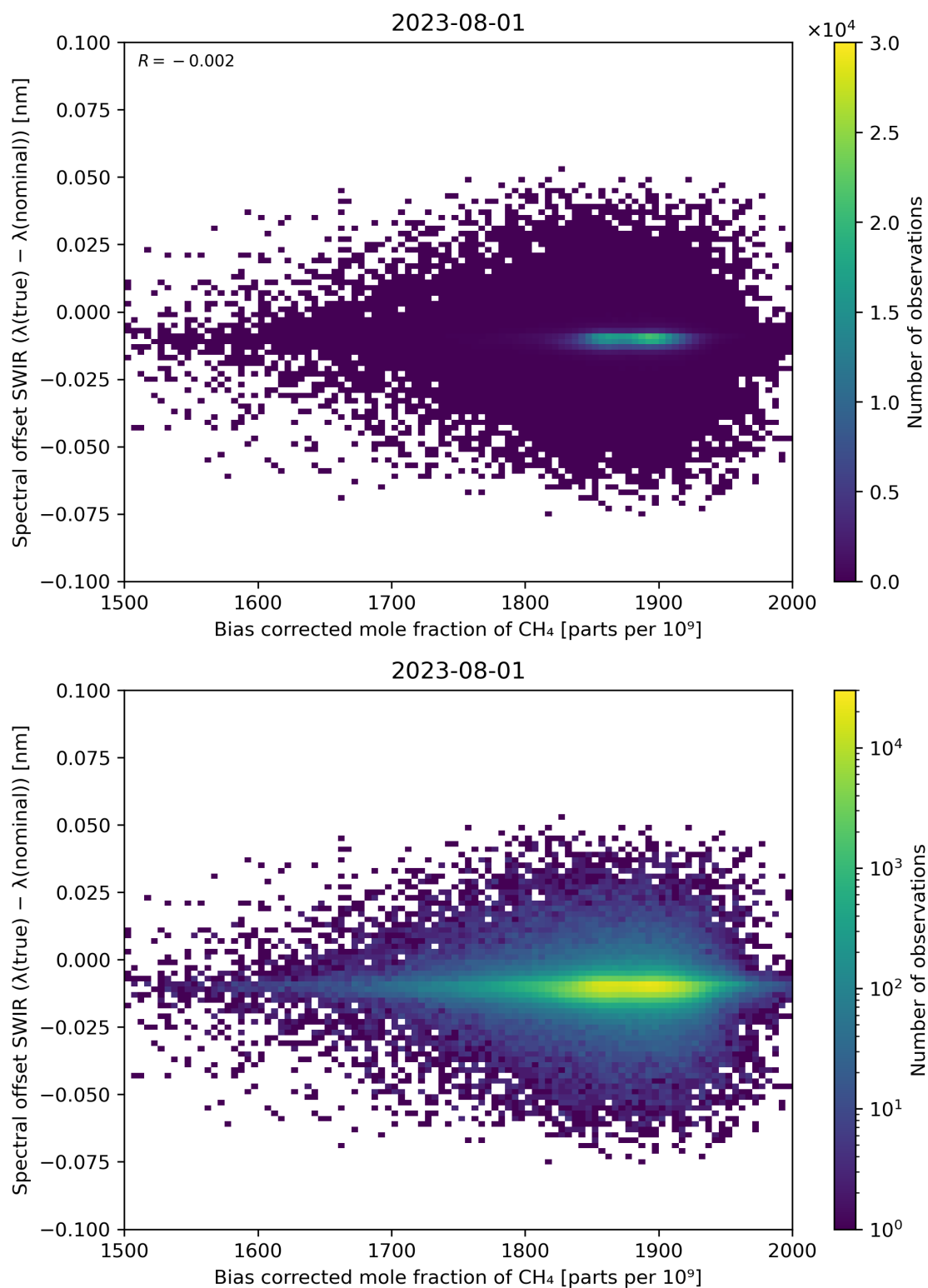
Figure 69: Scatter density plot of “Bias corrected mole fraction of \text{CH}_4 ” against “Spectral offset SWIR ( \lambda(\text{true}) - \lambda(\text{nominal}) )” for 2023-07-31 to 2023-08-02.
