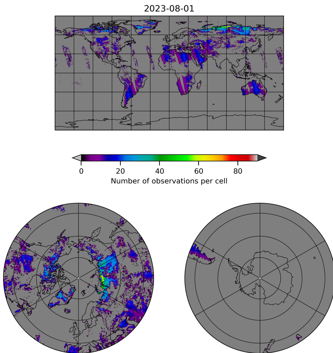
Figure 10: Map of the number of observations for 2023-07-31 to 2023-08-02
