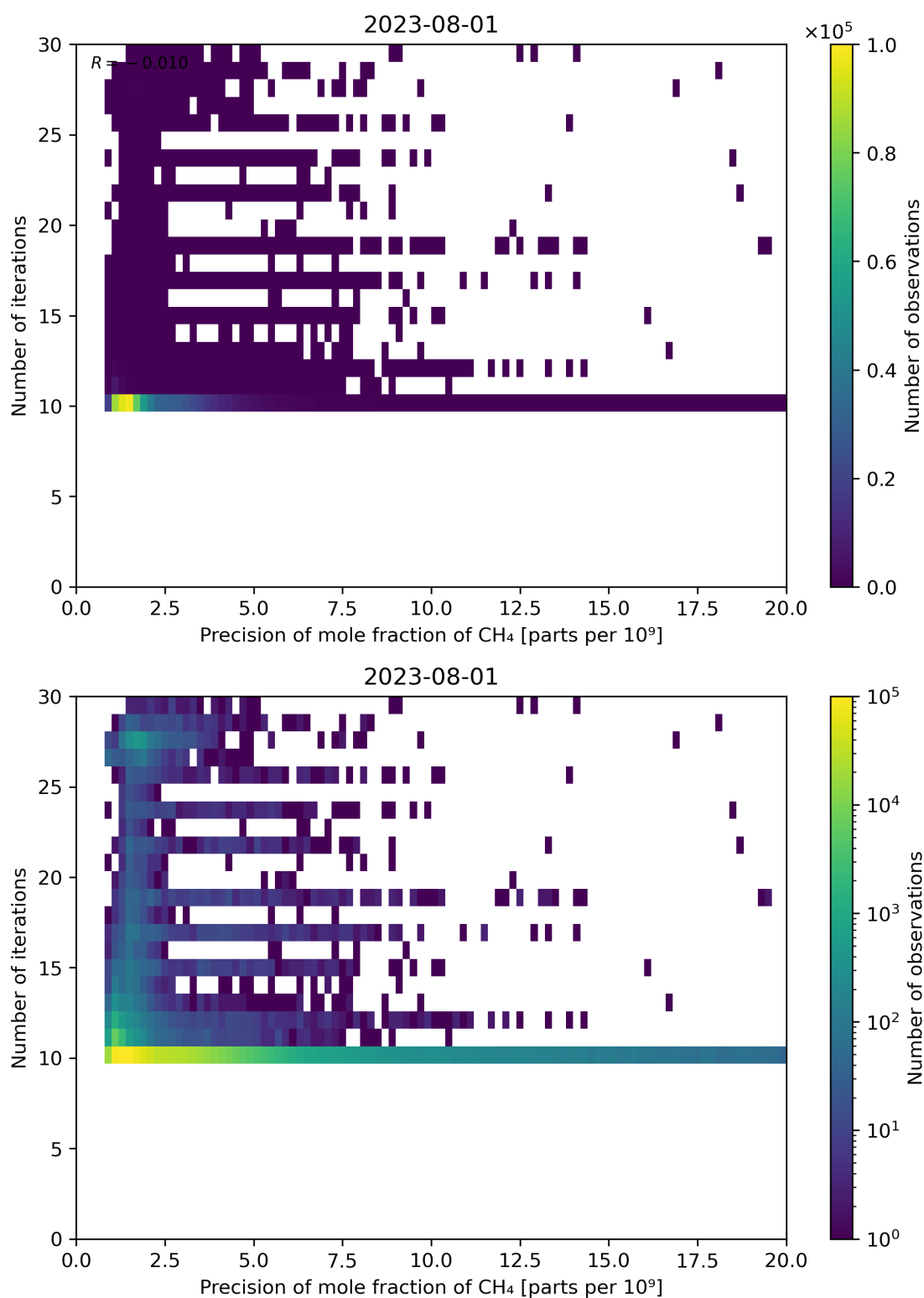
Figure 83: Scatter density plot of “Precision of mole fraction of CH 4 ” against “Number of iterations” for 2023-07-31 to 2023-08-02.
