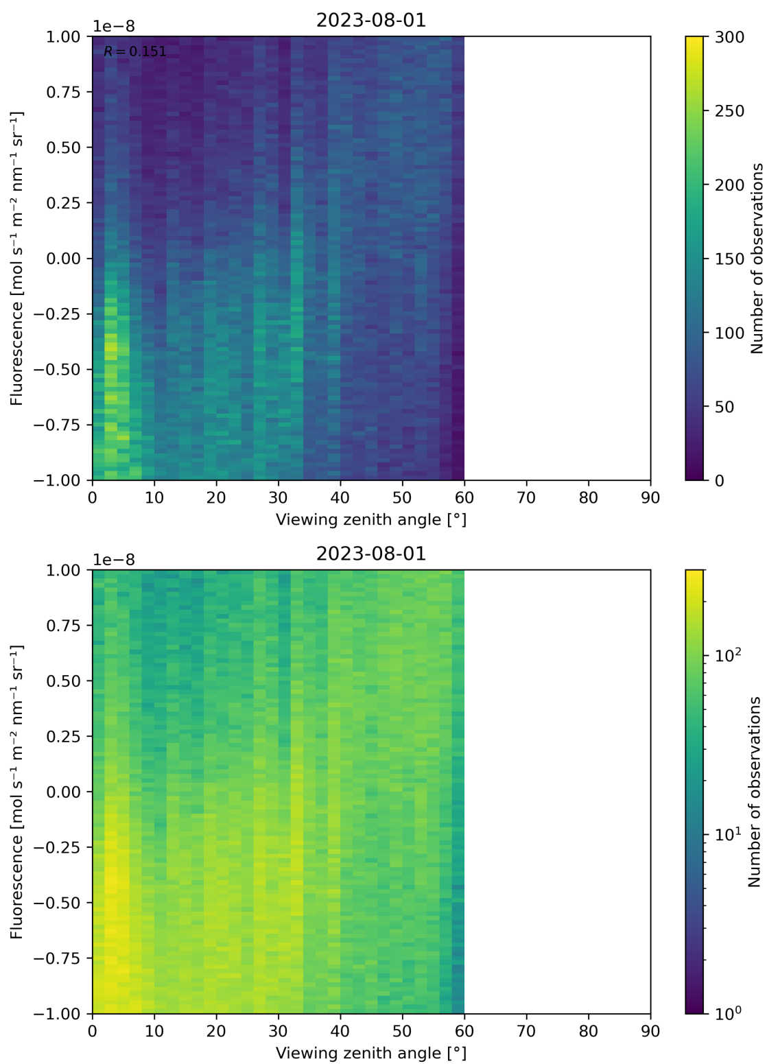
Figure 108: Scatter density plot of “Viewing zenith angle” against “Fluorescence” for 2023-07-31 to 2023-08-02.
