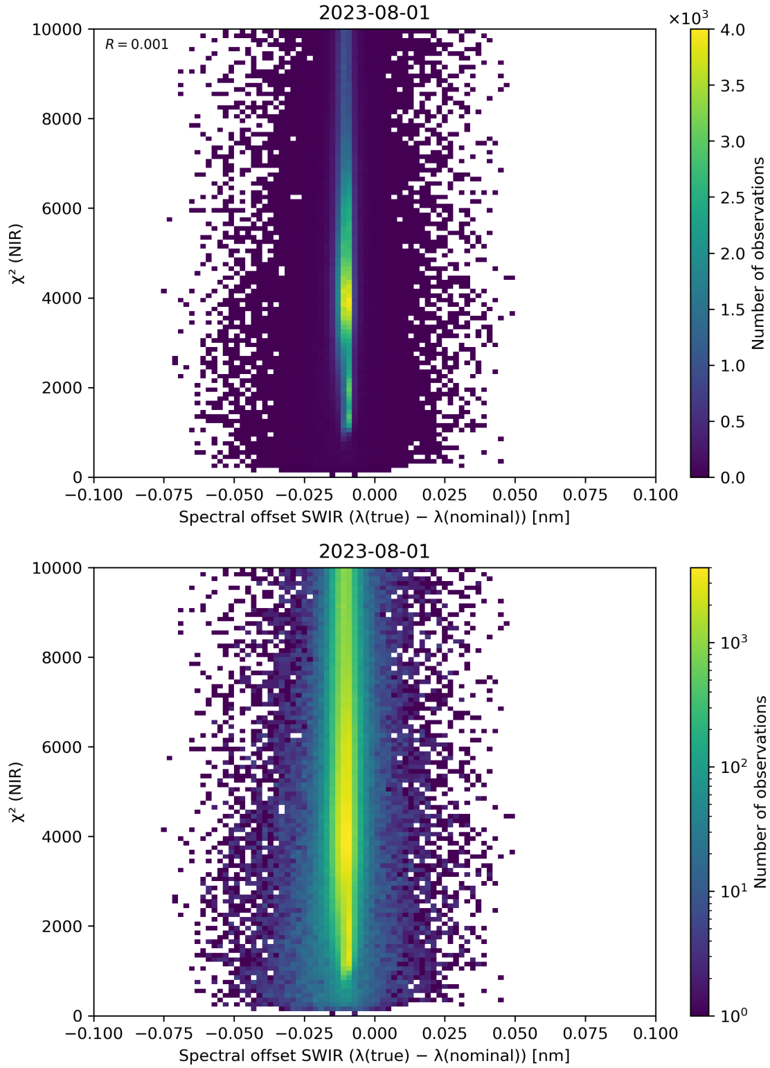
Figure 117: Scatter density plot of “Spectral offset SWIR ( \lambda(\text{true}) - \lambda(\text{nominal}) )” against “ \chi^2 (NIR)” for 2023-07-31 to 2023-08-02.
