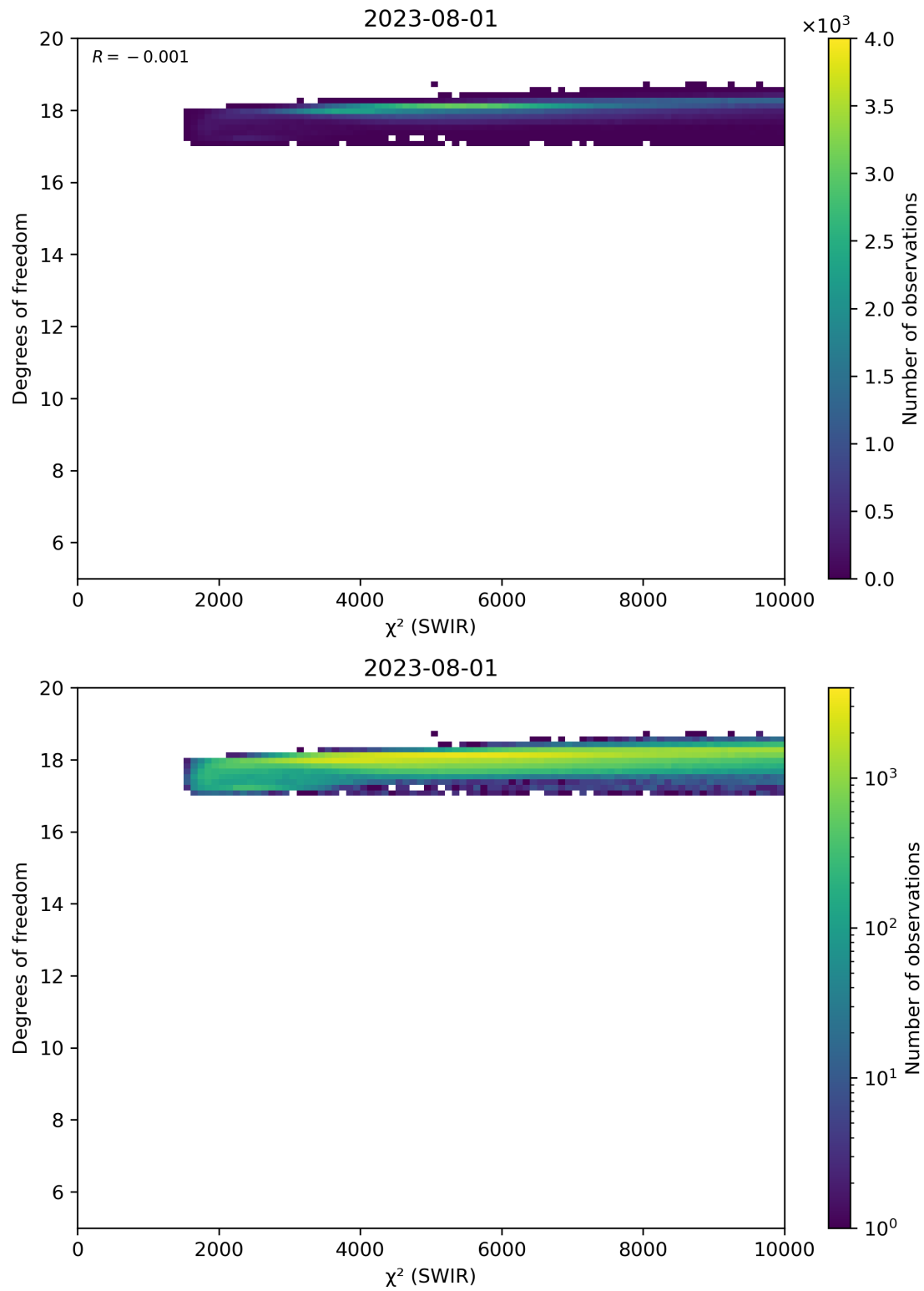
Figure 48: Scatter density plot of “ \chi^2 (SWIR)” against “Degrees of freedom” for 2023-07-31 to 2023-08-02.
