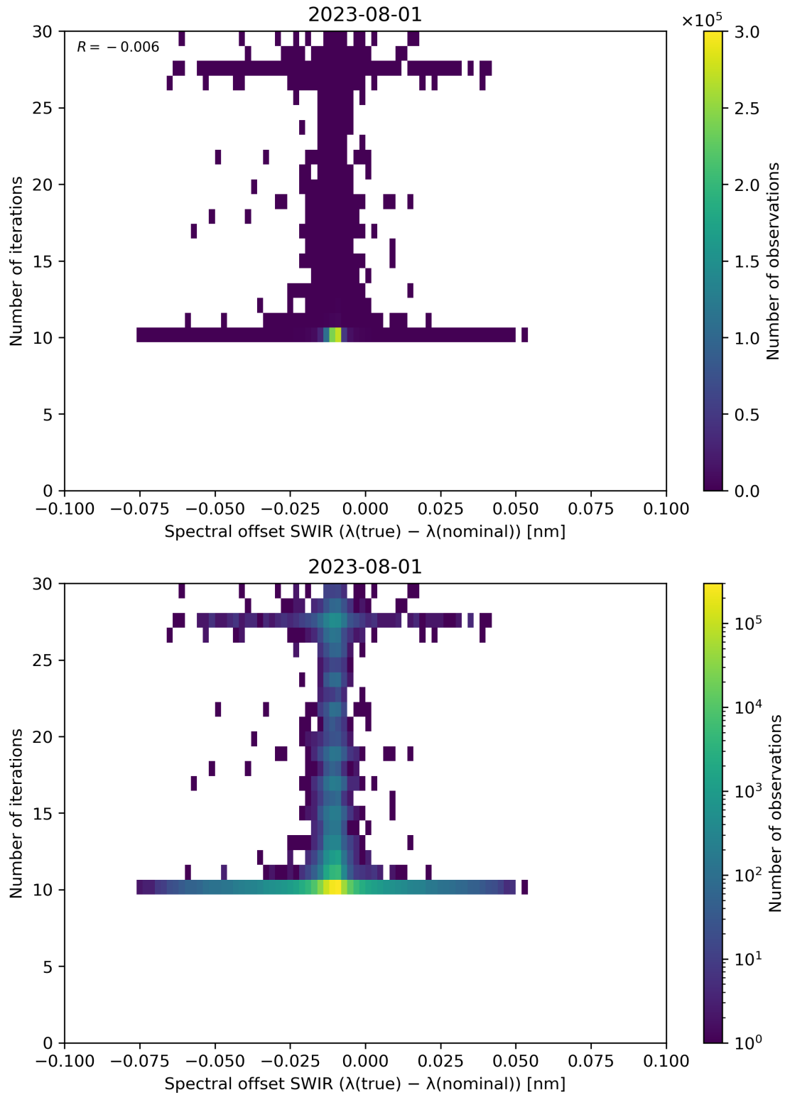
Figure 121: Scatter density plot of “Spectral offset SWIR ( \lambda(\text{true}) - \lambda(\text{nominal}) )” against “Number of iterations” for 2023-07-31 to 2023-08-02.
