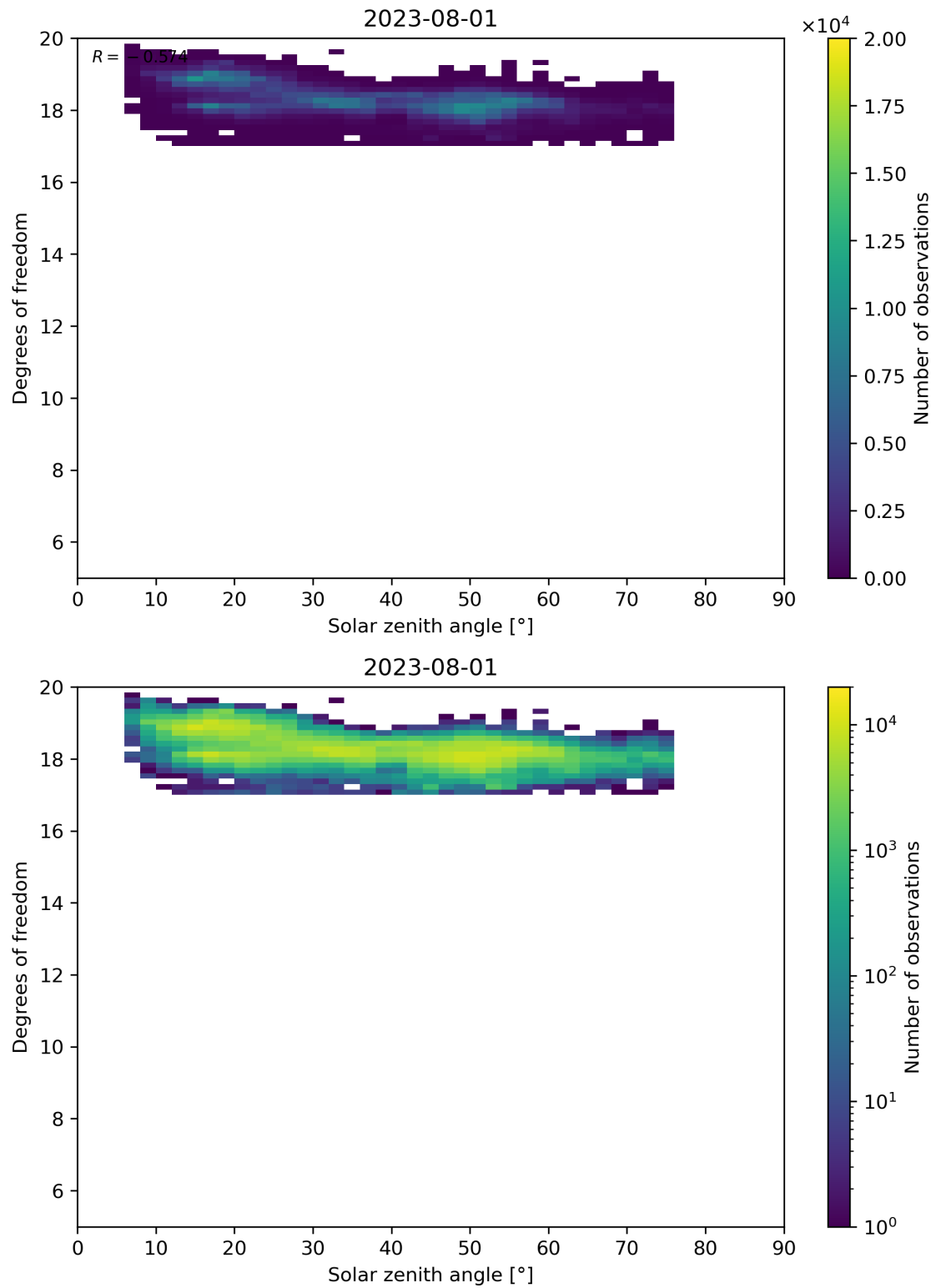
Figure 96: Scatter density plot of “Solar zenith angle” against “Degrees of freedom” for 2023-07-31 to 2023-08-02.
