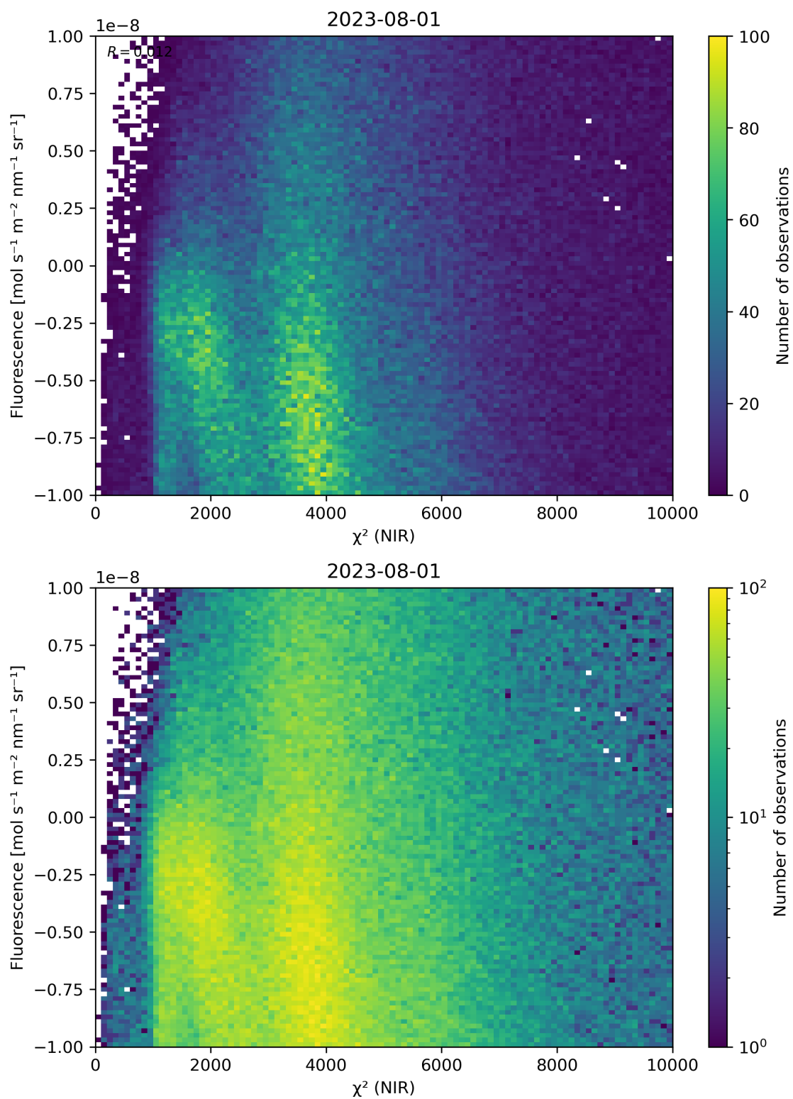
Figure 45: Scatter density plot of “ \chi^2 (NIR)” against “Fluorescence” for 2023-07-31 to 2023-08-02.
