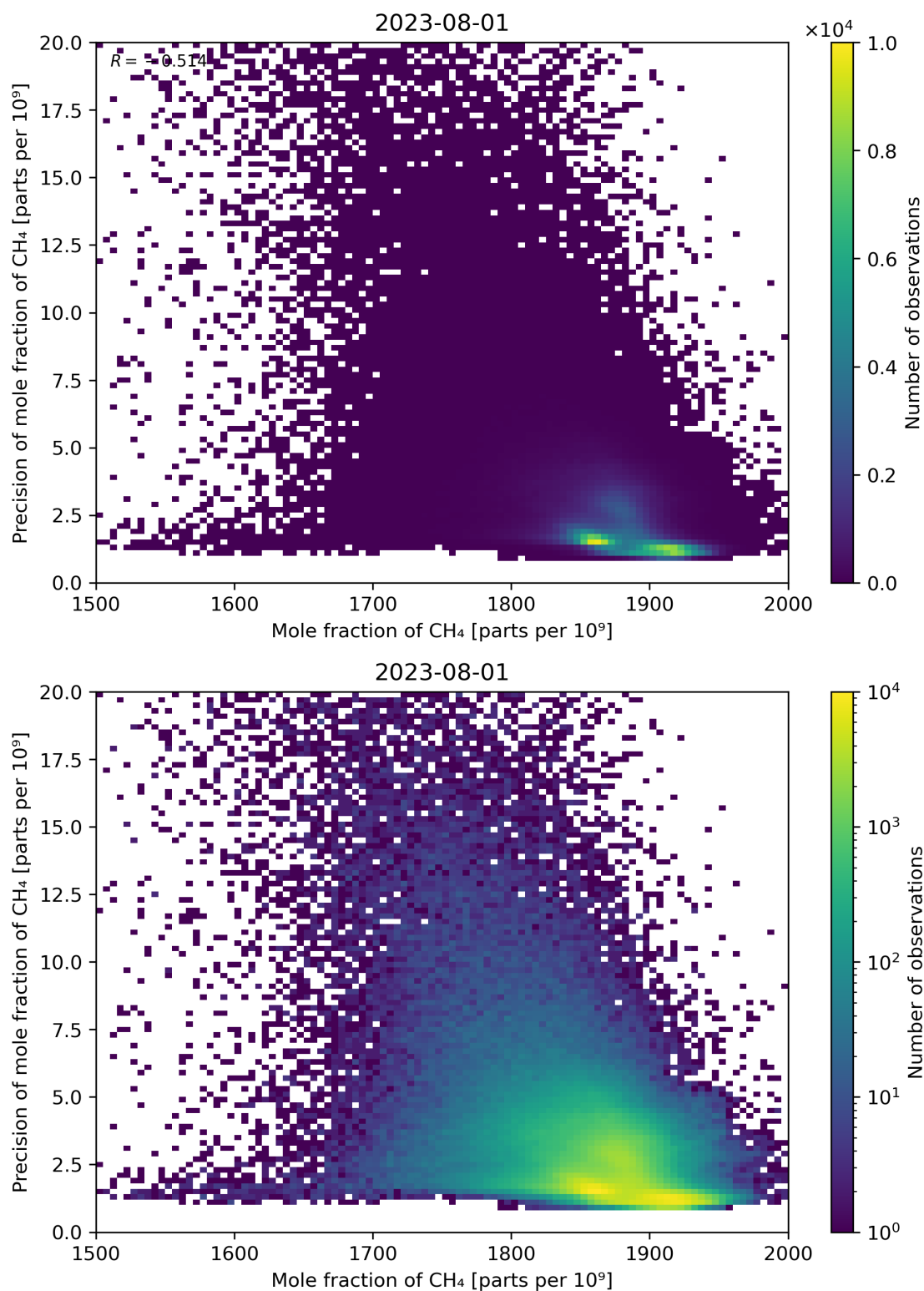
Figure 75: Scatter density plot of “Mole fraction of CH 4 ” against “Precision of mole fraction of CH 4 ” for 2023-07-31 to 2023-08-02.
