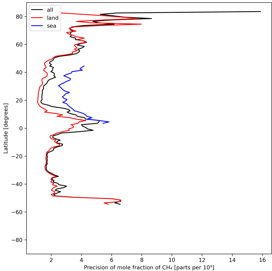
Figure 13: Zonal average of “Precision of mole fraction of CH 4 ” for 2023-07-31 to 2023-08-02.
