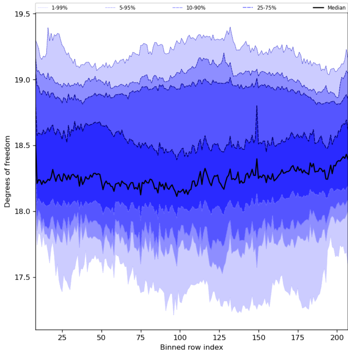
Figure 41: Along track statistics of “Degrees of freedom” for 2023-07-31 to 2023-08-02
