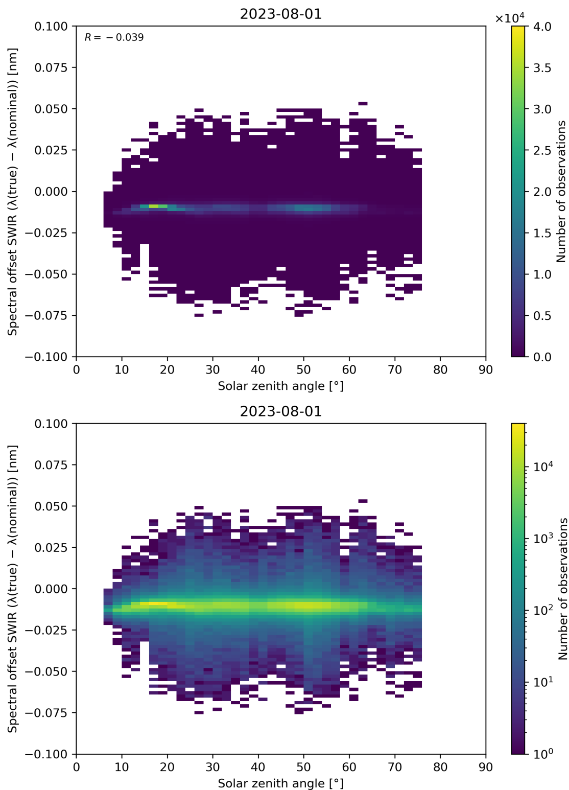
Figure 104: Scatter density plot of “Solar zenith angle” against “Spectral offset SWIR ( \lambda(\text{true}) - \lambda(\text{nominal}) )” for 2023-07-31 to 2023-08-02.
