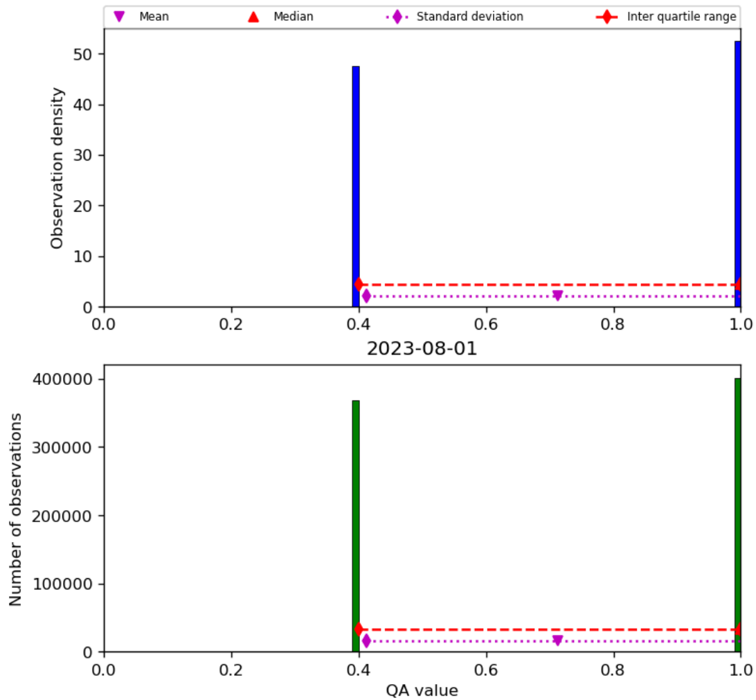
Figure 22: Histogram of “QA value” for 2023-07-31 to 2023-08-02
