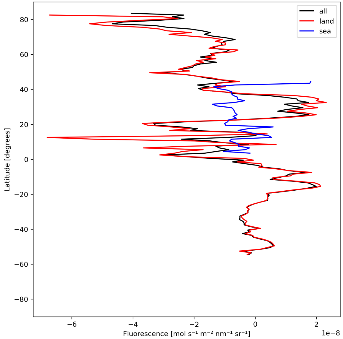
Figure 21: Zonal average of “Fluorescence” for 2023-07-31 to 2023-08-02.
