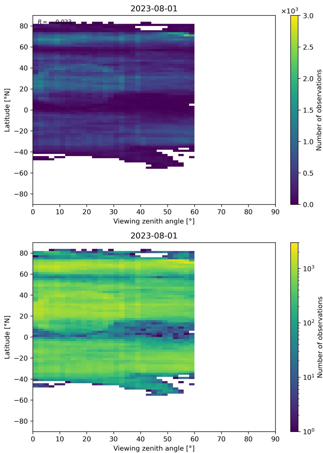
Figure 109: Scatter density plot of “Viewing zenith angle” against “Latitude” for 2023-07-31 to 2023-08-02.
