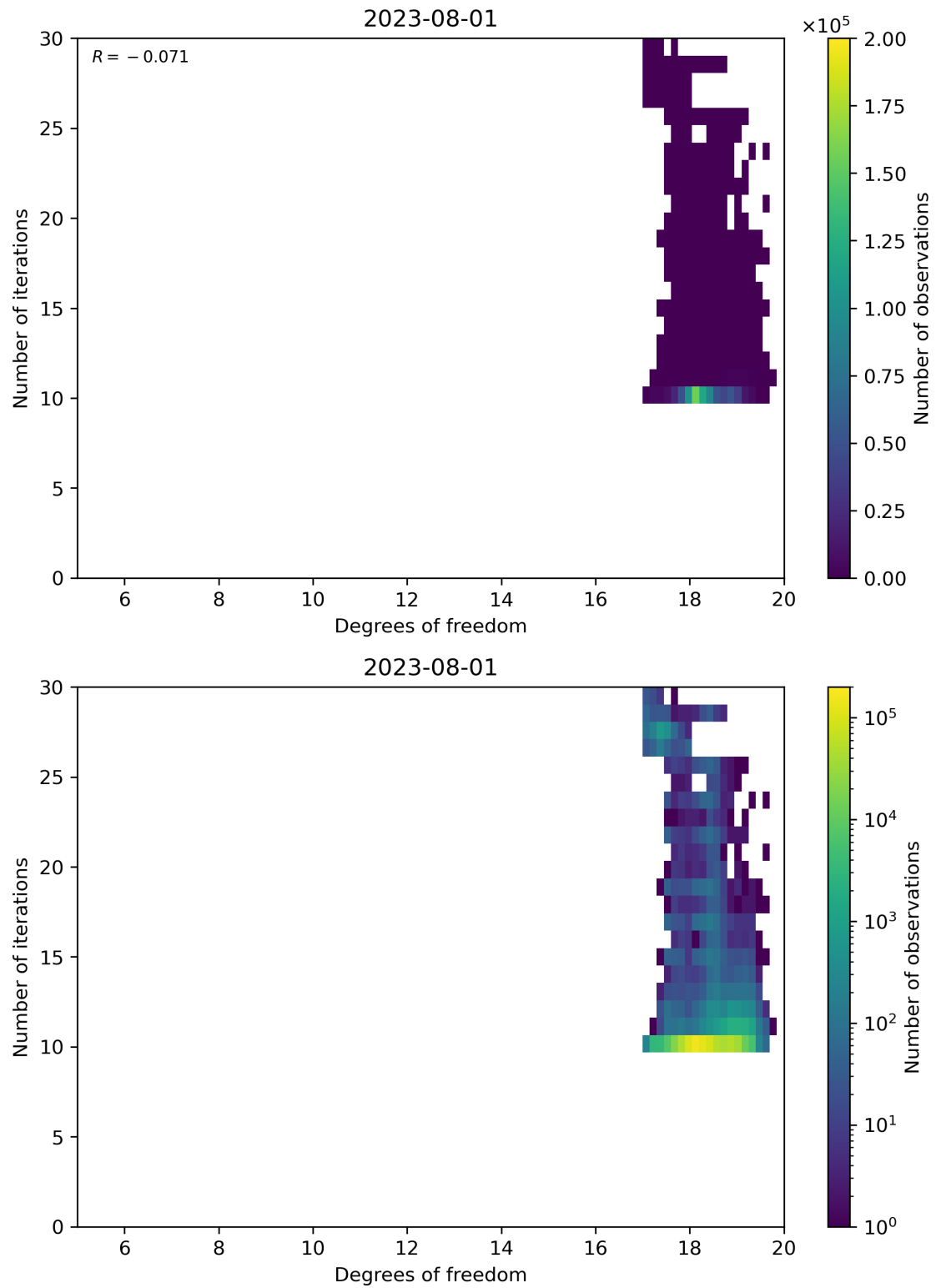
Figure 52: Scatter density plot of “Degrees of freedom” against “Number of iterations” for 2023-07-31 to 2023-08-02.
