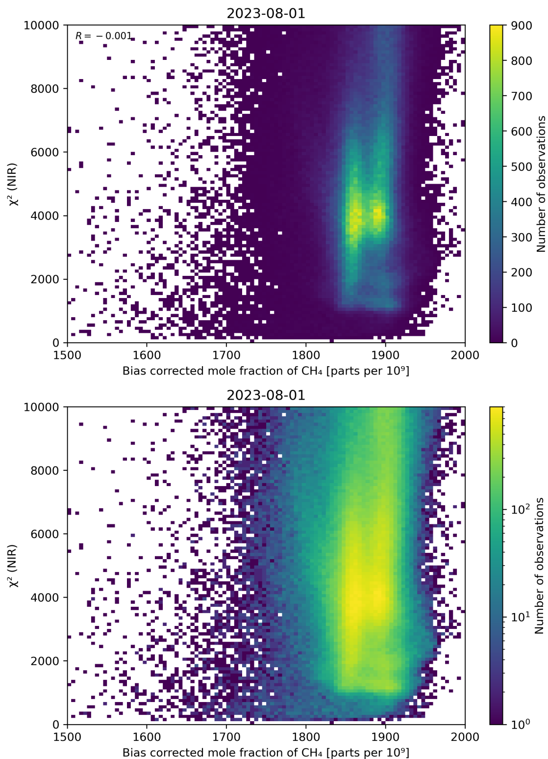
Figure 63: Scatter density plot of “Bias corrected mole fraction of CH 4 ” against “ \chi^2 (NIR)” for 2023-07-31 to 2023-08-02.
