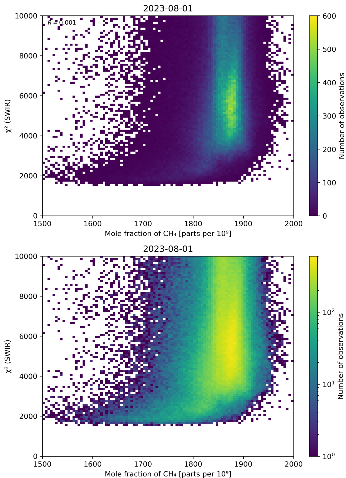
Figure 71: Scatter density plot of “Mole fraction of CH 4 ” against “ \chi^2 (SWIR)” for 2023-07-31 to 2023-08-02.
