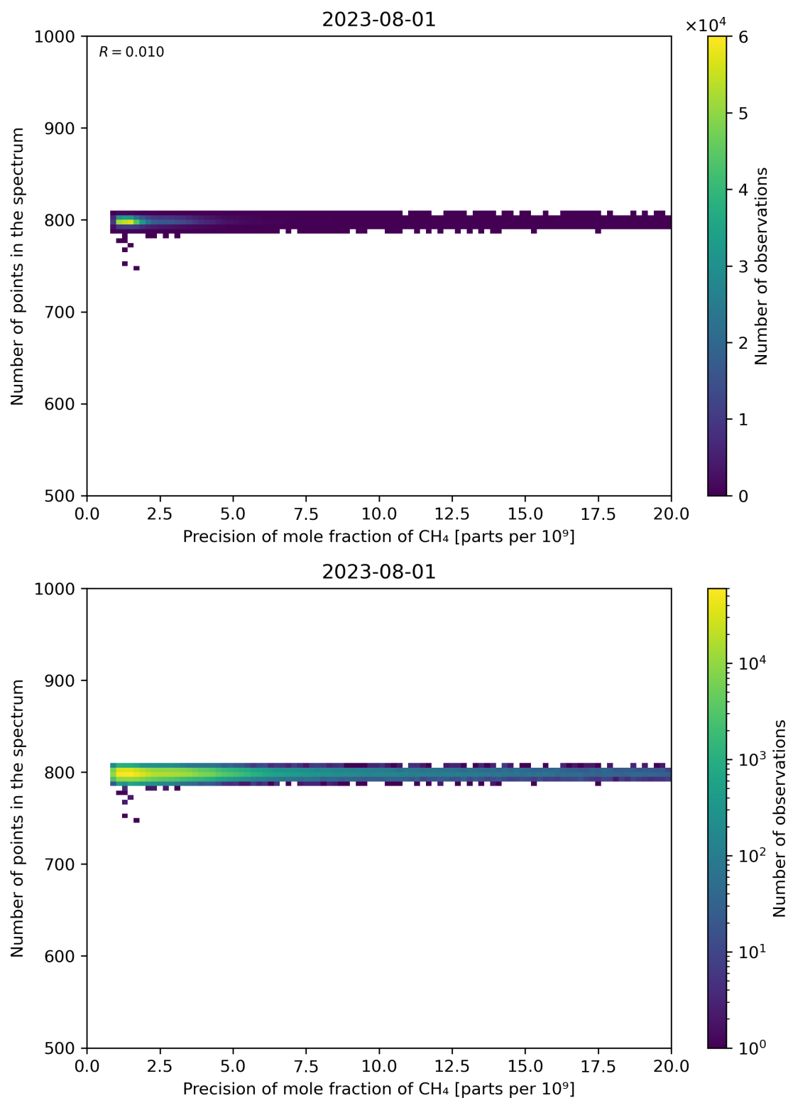
Figure 84: Scatter density plot of “Precision of mole fraction of CH 4 ” against “Number of points in the spectrum” for 2023-07-31 to 2023-08-02.
