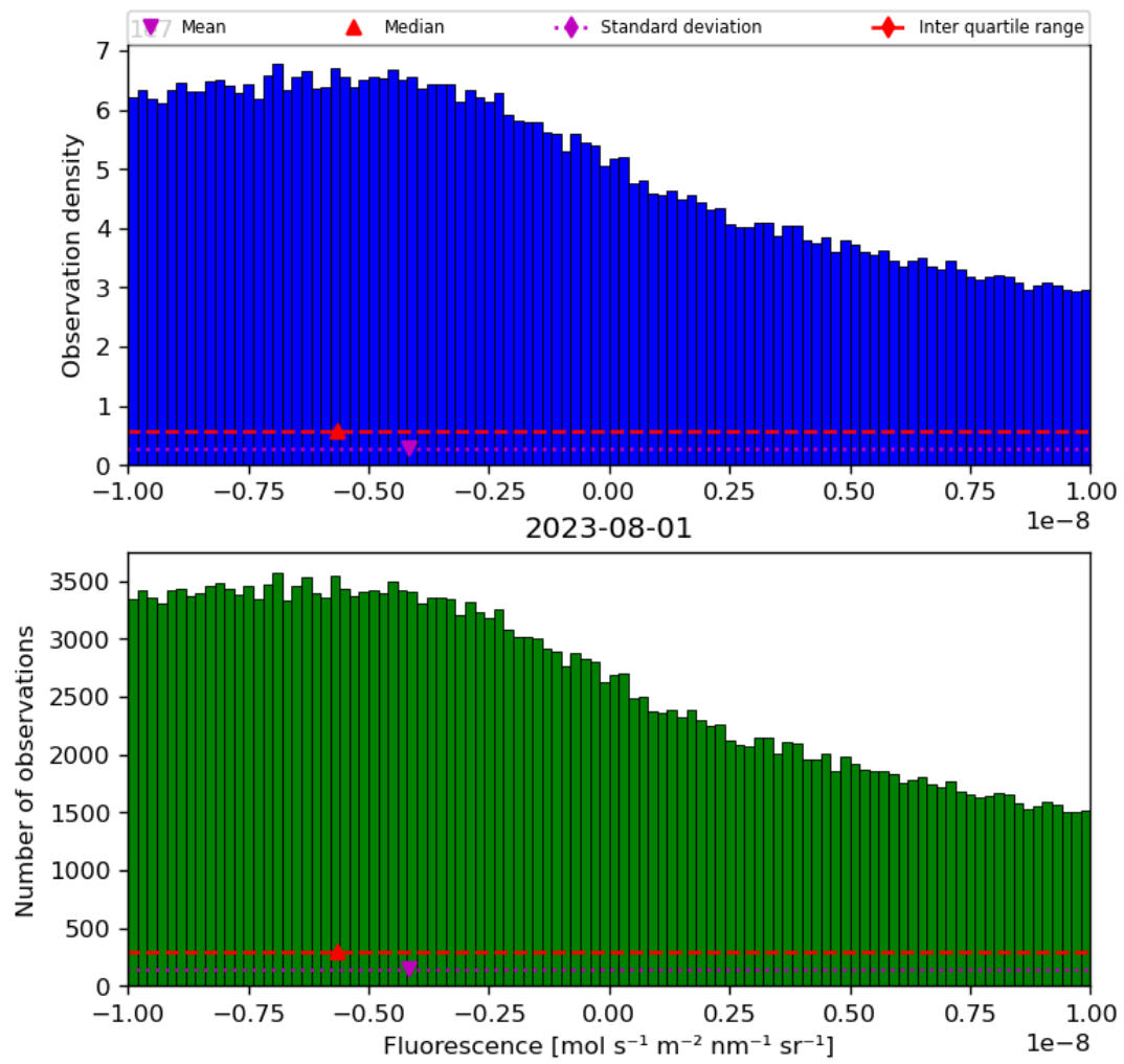
Figure 32: Histogram of “Fluorescence” for 2023-07-31 to 2023-08-02
