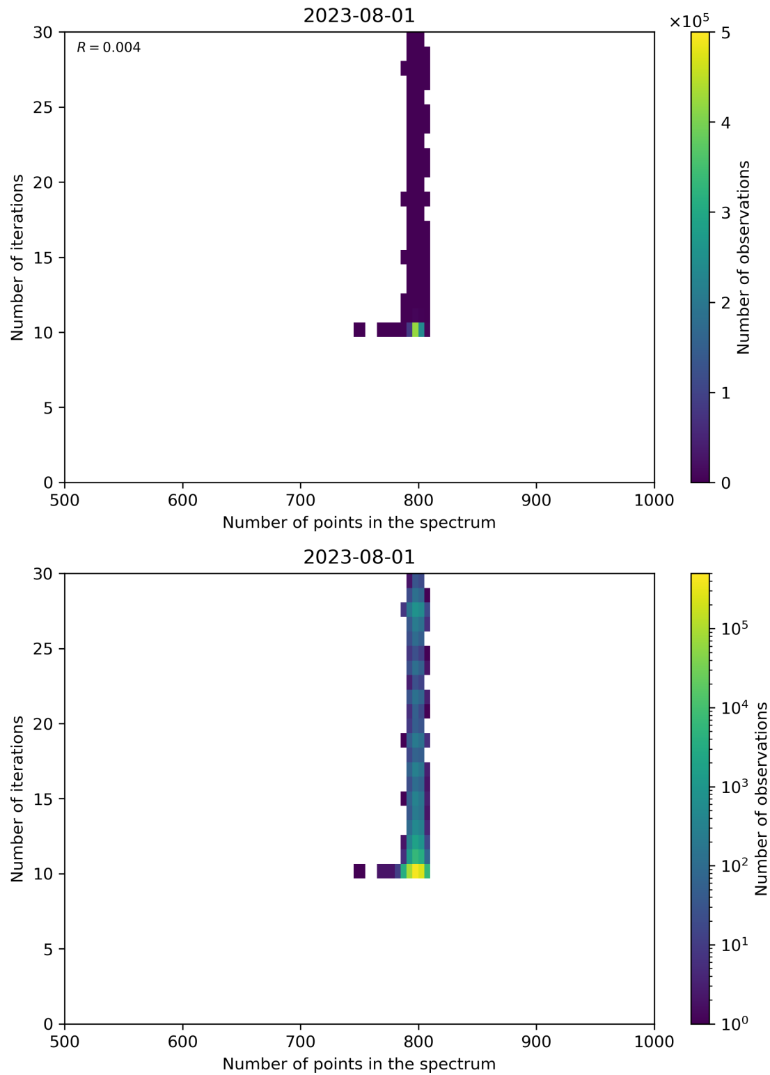
Figure 92: Scatter density plot of “Number of points in the spectrum” against “Number of iterations” for 2023-07-31 to 2023-08-02.
