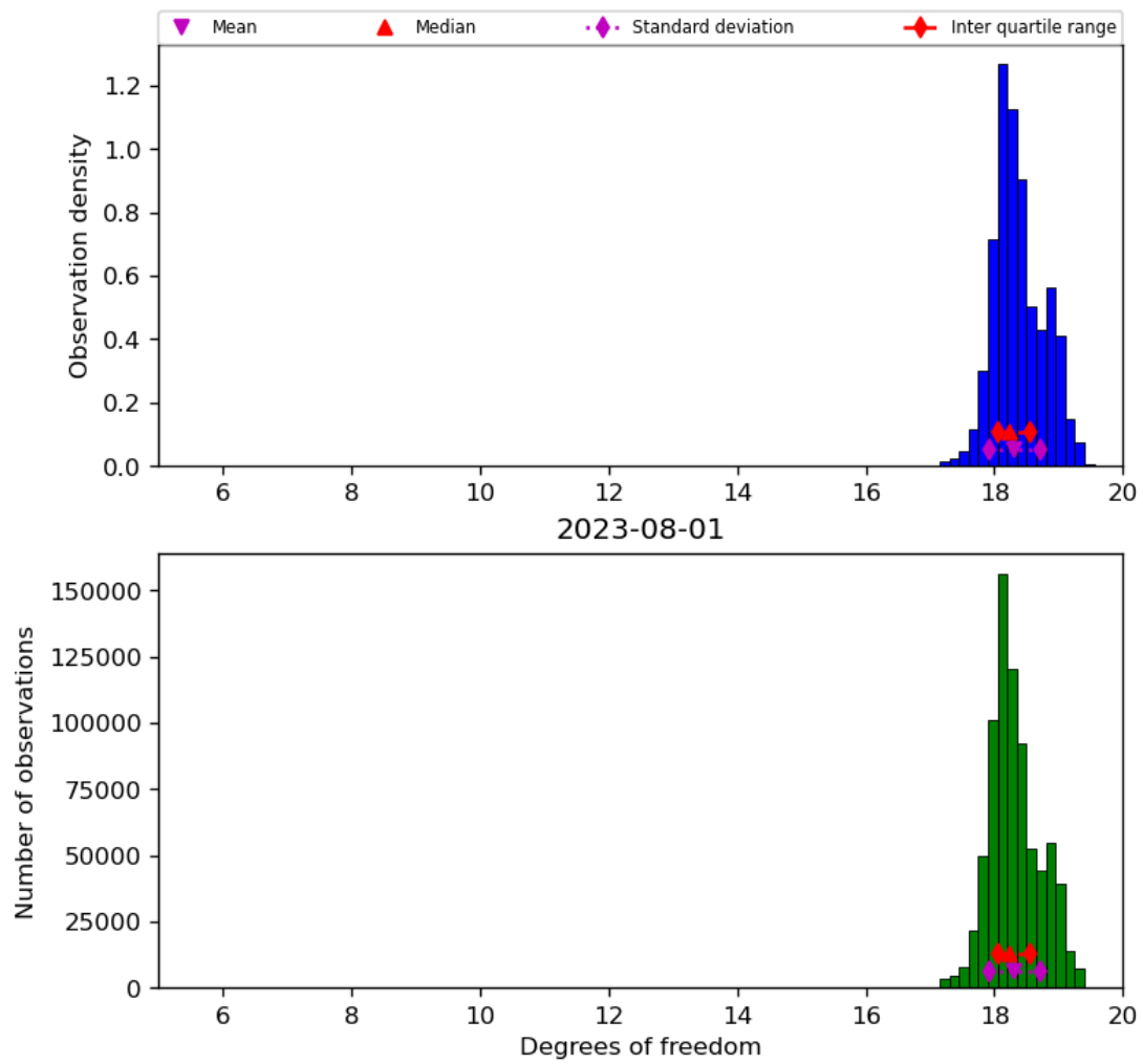
Figure 30: Histogram of “Degrees of freedom” for 2023-07-31 to 2023-08-02
