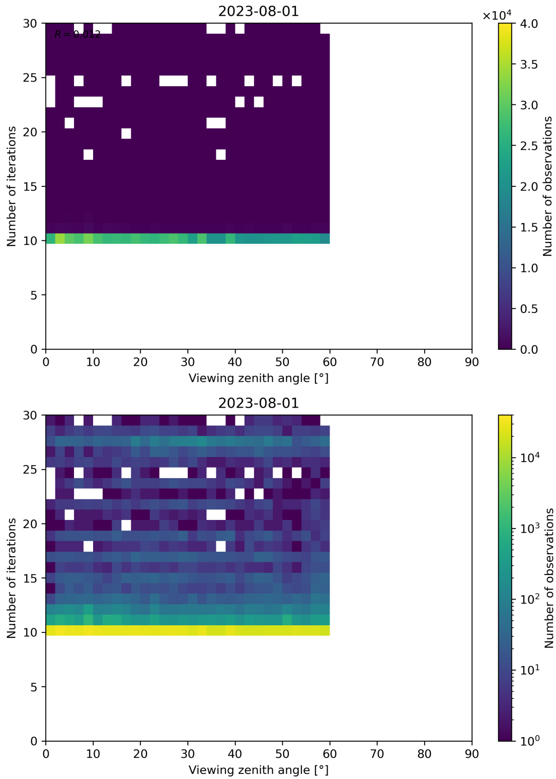
Figure 113: Scatter density plot of “Viewing zenith angle” against “Number of iterations” for 2023-07-31 to 2023-08-02.
