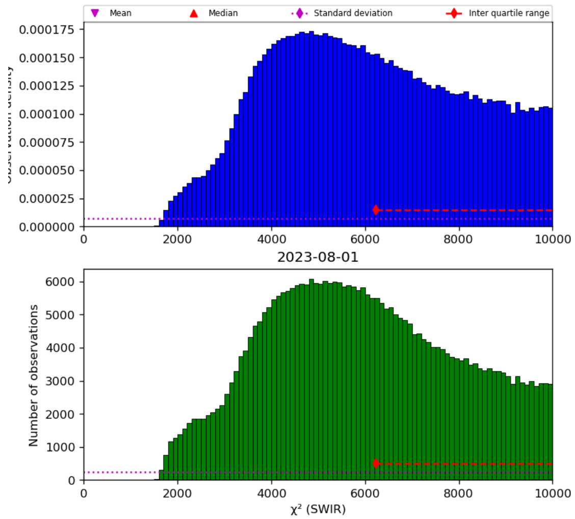
Figure 28: Histogram of “ \chi^2 (SWIR)” for 2023-07-31 to 2023-08-02
