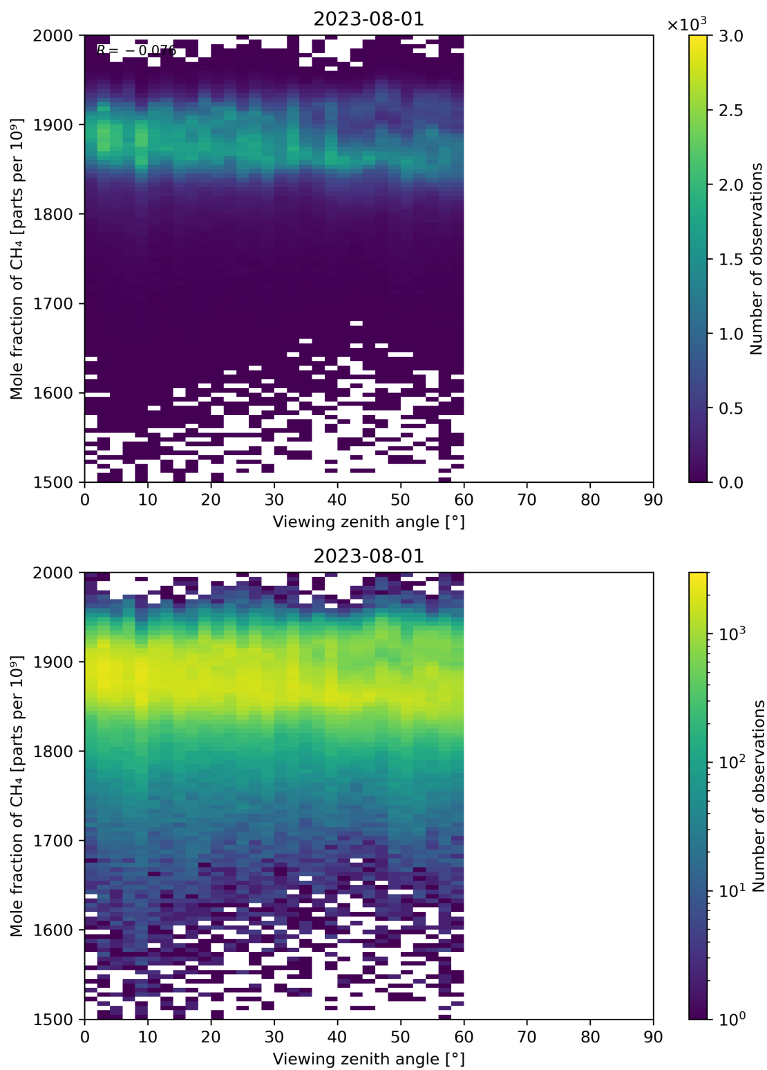
Figure 110: Scatter density plot of “Viewing zenith angle” against “Mole fraction of CH 4 ” for 2023-07-31 to 2023-08-02.
