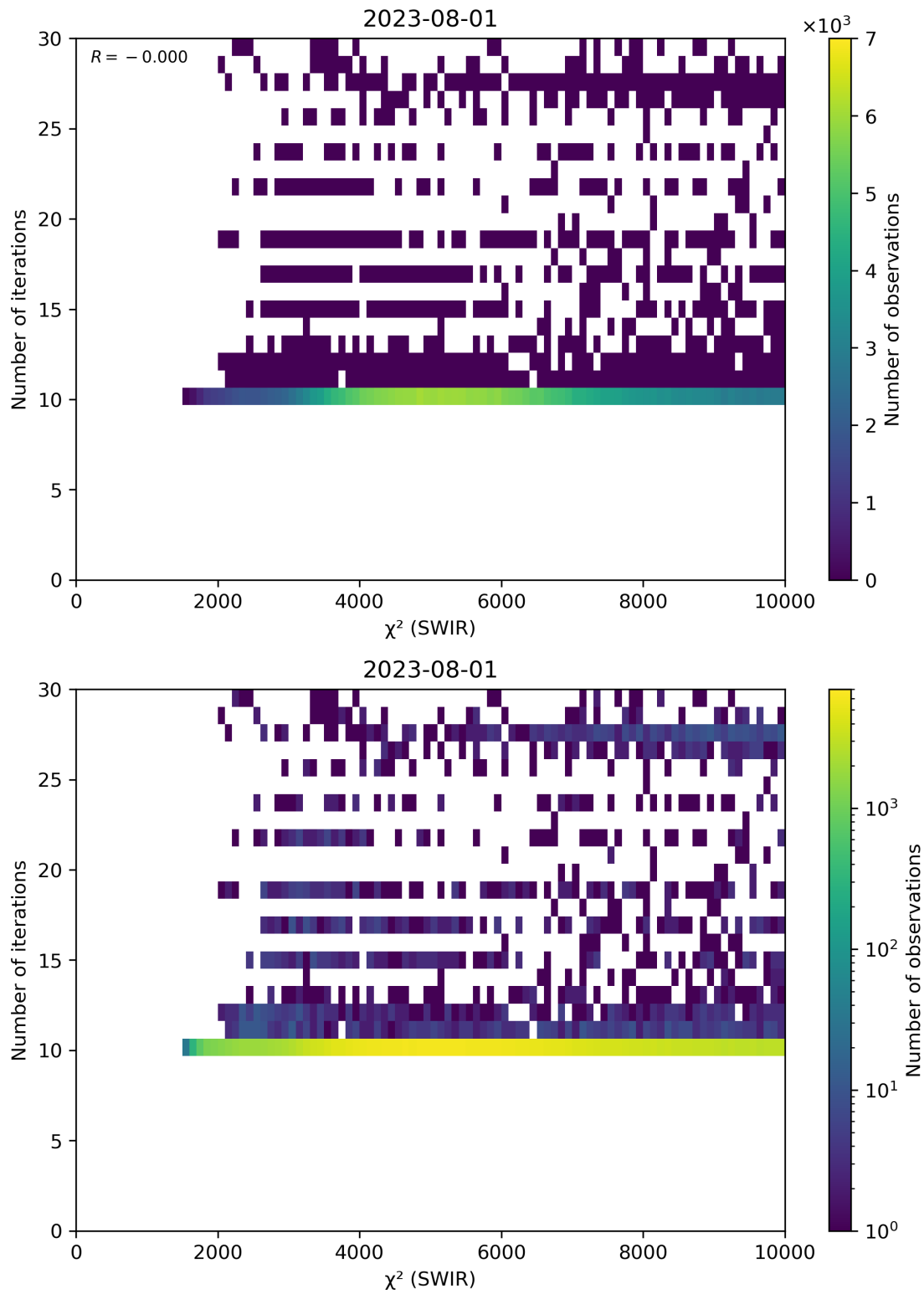
Figure 50: Scatter density plot of “ \chi^2 (SWIR)” against “Number of iterations” for 2023-07-31 to 2023-08-02.
