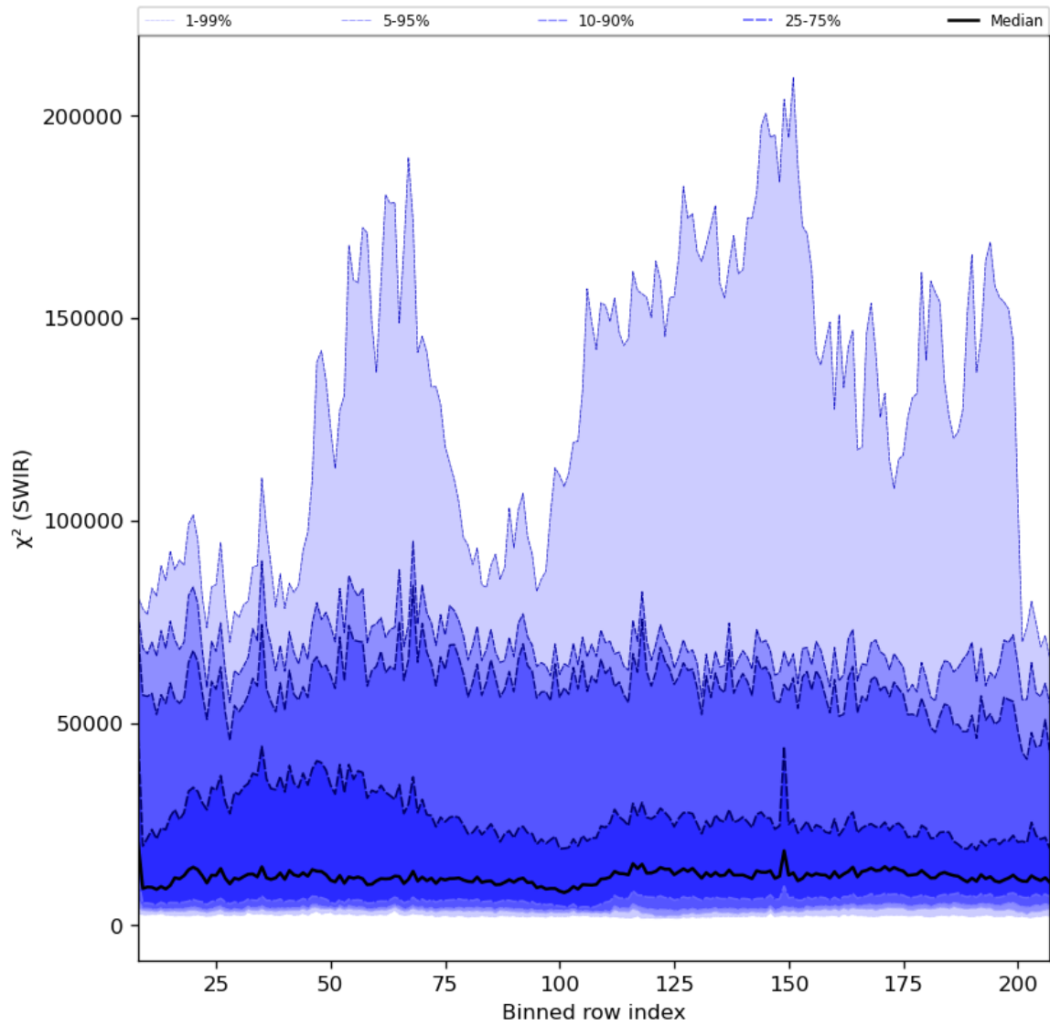
Figure 39: Along track statistics of “ \chi^2 (SWIR)” for 2023-07-31 to 2023-08-02
