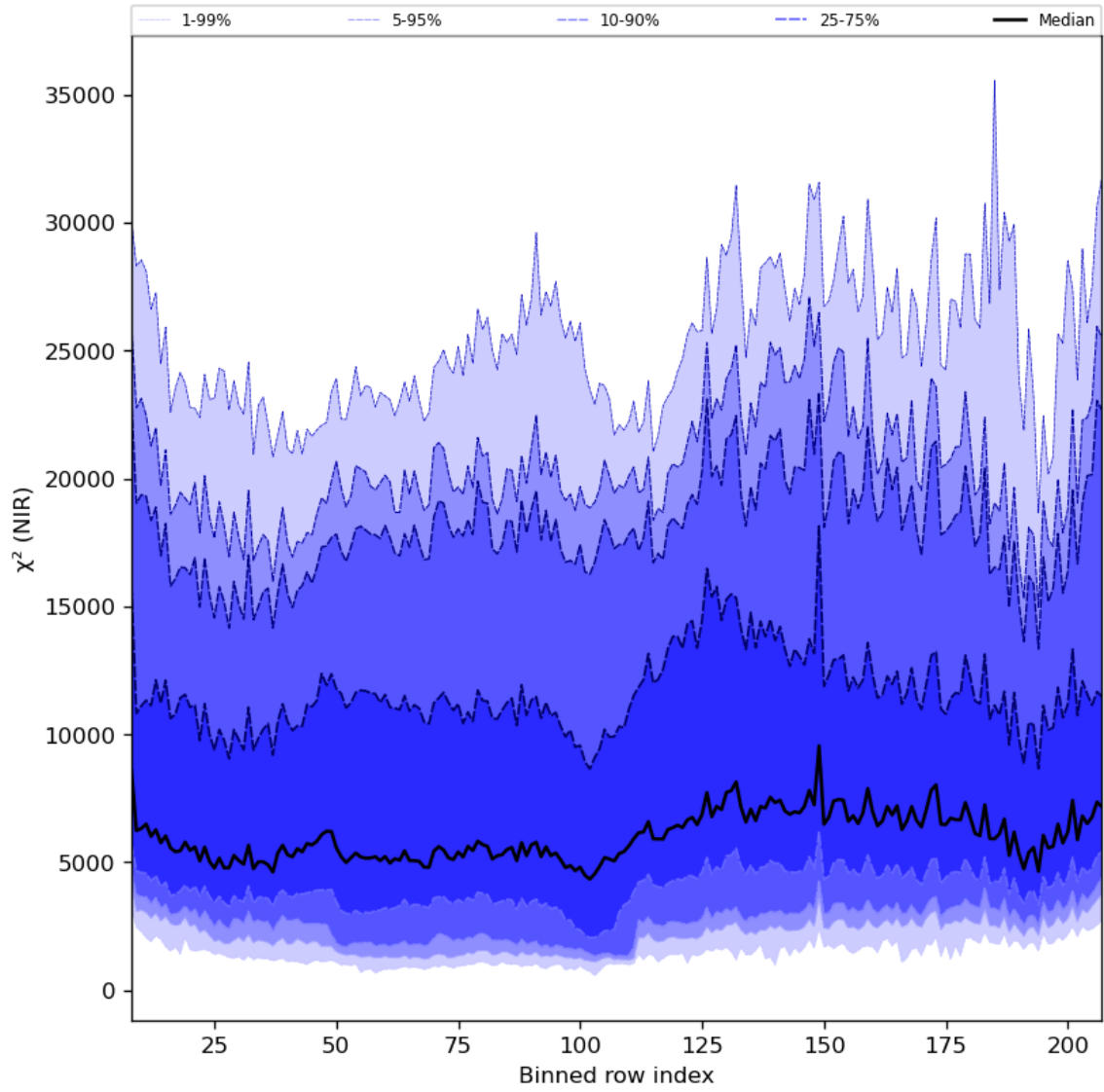
Figure 40: Along track statistics of “ \chi^2 (NIR)” for 2023-07-31 to 2023-08-02
