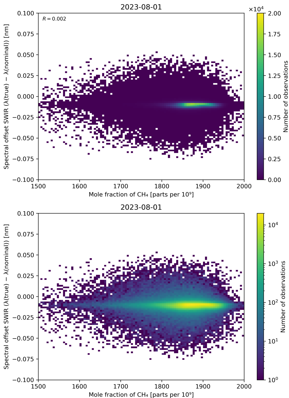
Figure 86: Scatter density plot of “Mole fraction of CH 4 ” against “Spectral offset SWIR ( \lambda(\text{true}) - \lambda(\text{nominal}) )” for 2023-07-31 to 2023-08-02.
