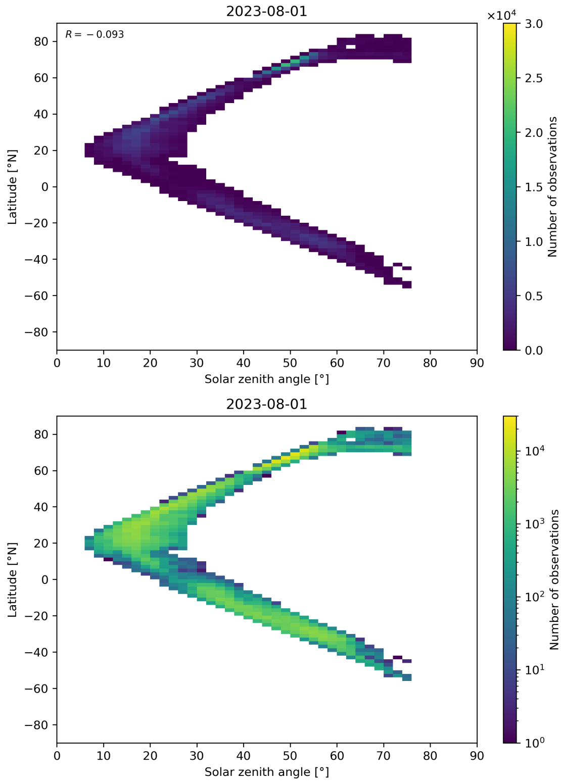
Figure 98: Scatter density plot of “Solar zenith angle” against “Latitude” for 2023-07-31 to 2023-08-02.
