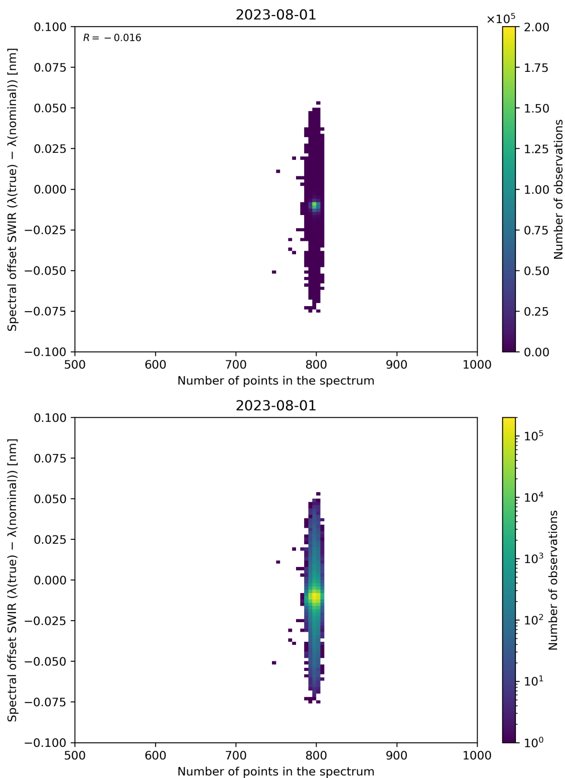
Figure 93: Scatter density plot of “Number of points in the spectrum” against “Spectral offset SWIR ( \lambda(\text{true}) - \lambda(\text{nominal}) )” for 2023-07-31 to 2023-08-02.
