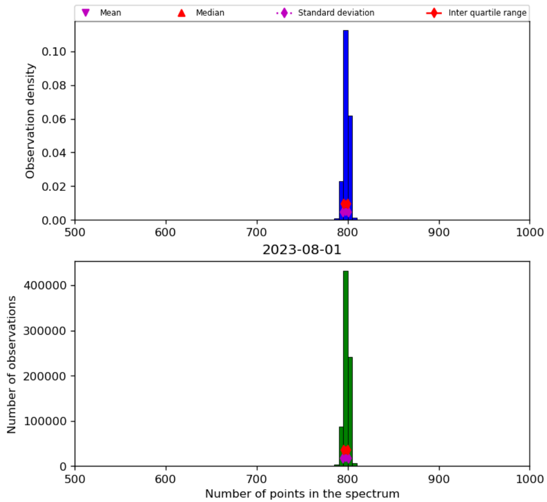
Figure 26: Histogram of “Number of points in the spectrum” for 2023-07-31 to 2023-08-02
