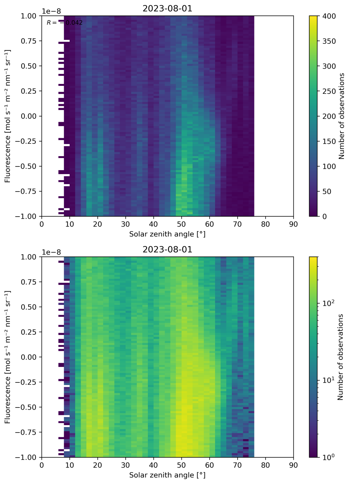
Figure 97: Scatter density plot of “Solar zenith angle” against “Fluorescence” for 2023-07-31 to 2023-08-02.
