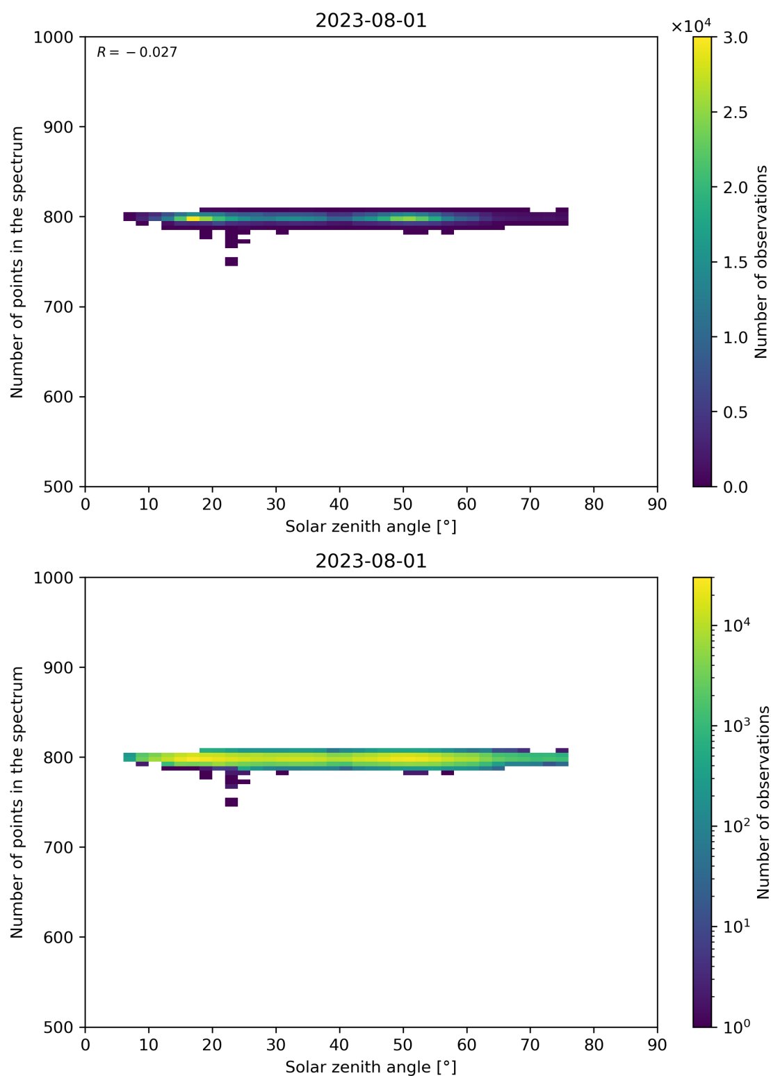
Figure 103: Scatter density plot of “Solar zenith angle” against “Number of points in the spectrum” for 2023-07-31 to 2023-08-02.
