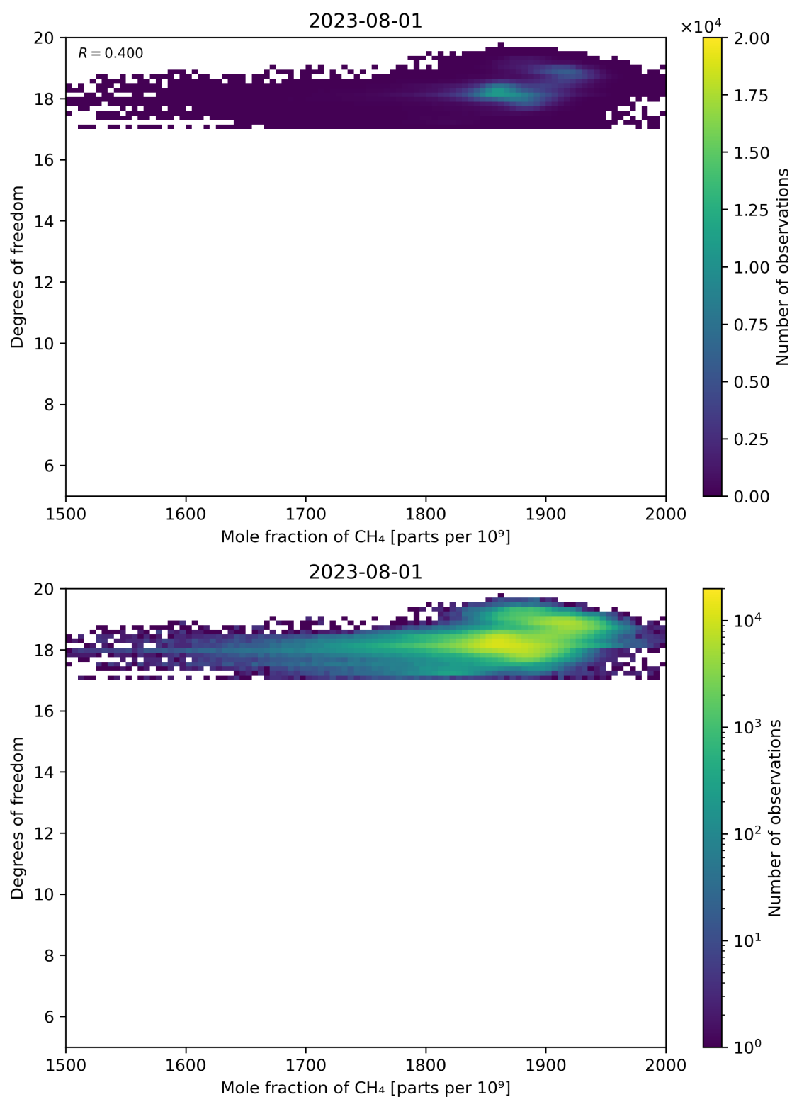
Figure 72: Scatter density plot of “Mole fraction of CH 4 ” against “Degrees of freedom” for 2023-07-31 to 2023-08-02.
