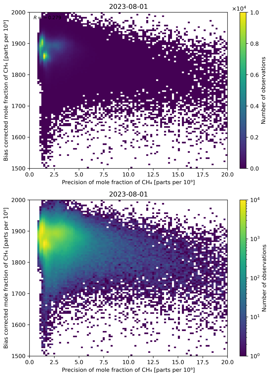
Figure 82: Scatter density plot of “Precision of mole fraction of CH 4 ” against “Bias corrected mole fraction of CH 4 ” for 2023-07-31 to 2023-08-02.
