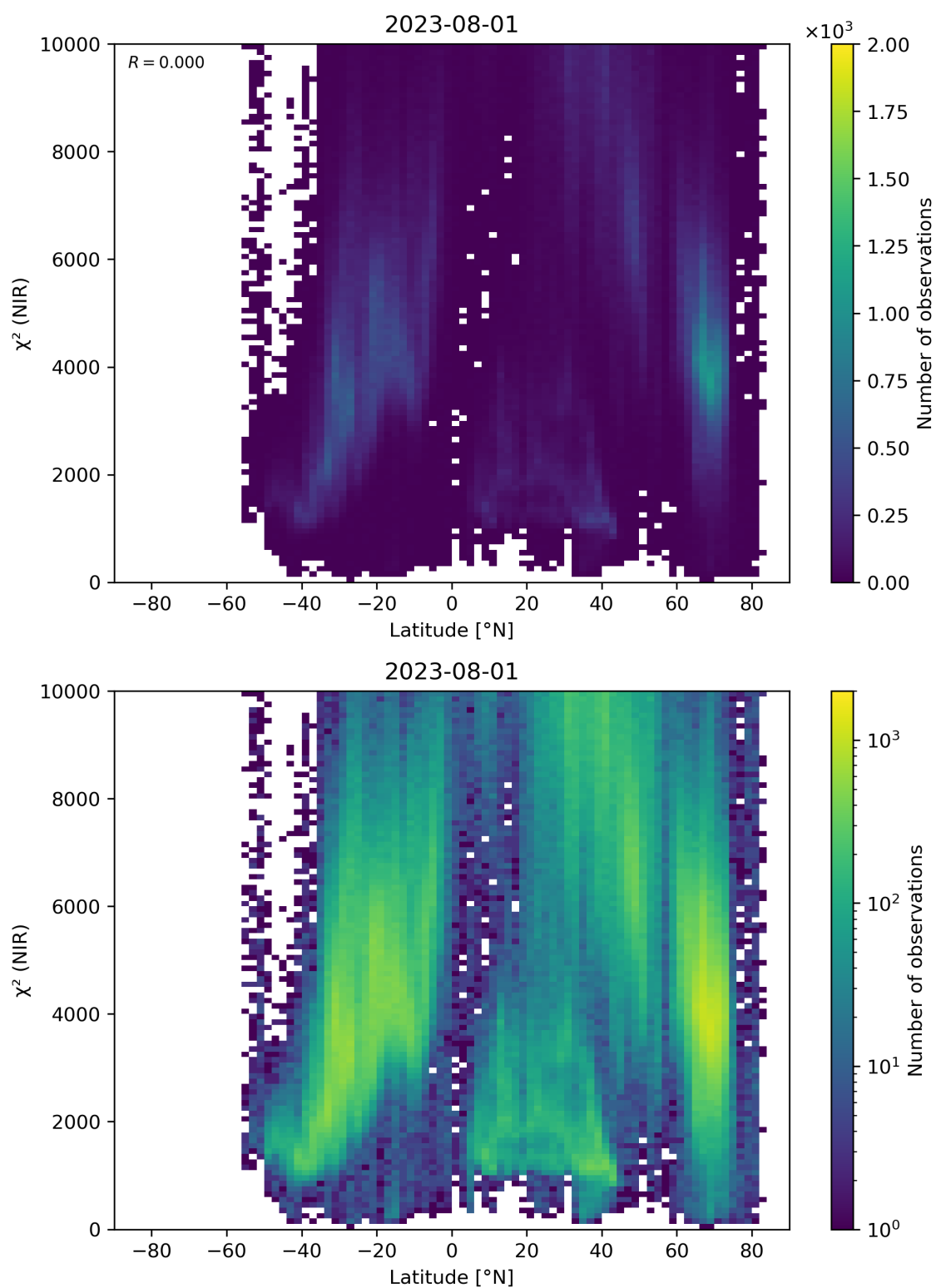
Figure 53: Scatter density plot of “Latitude” against “ \chi^2 (NIR)” for 2023-07-31 to 2023-08-02.
