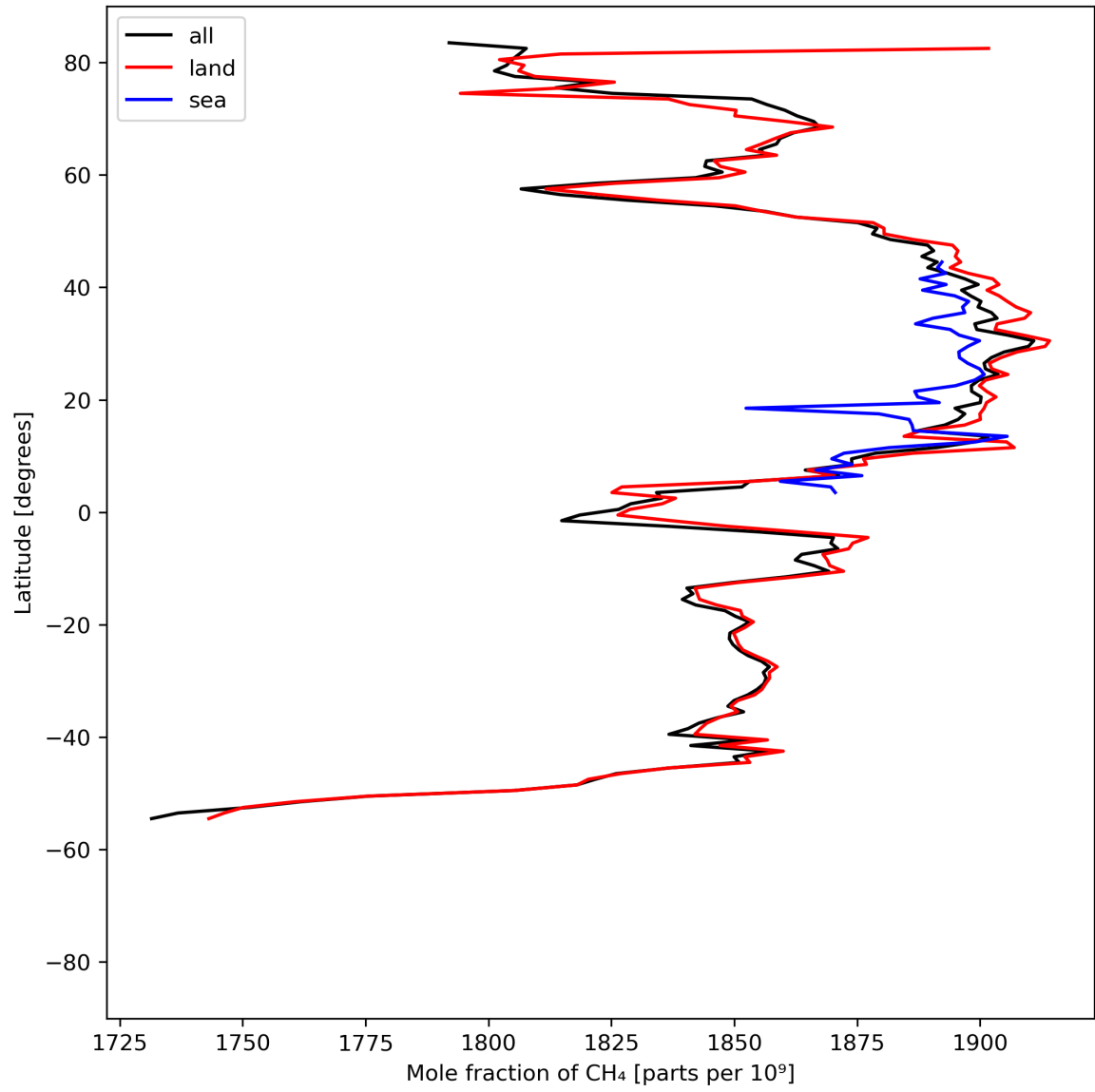
Figure 12: Zonal average of “Mole fraction of CH 4 ” for 2023-07-31 to 2023-08-02.
