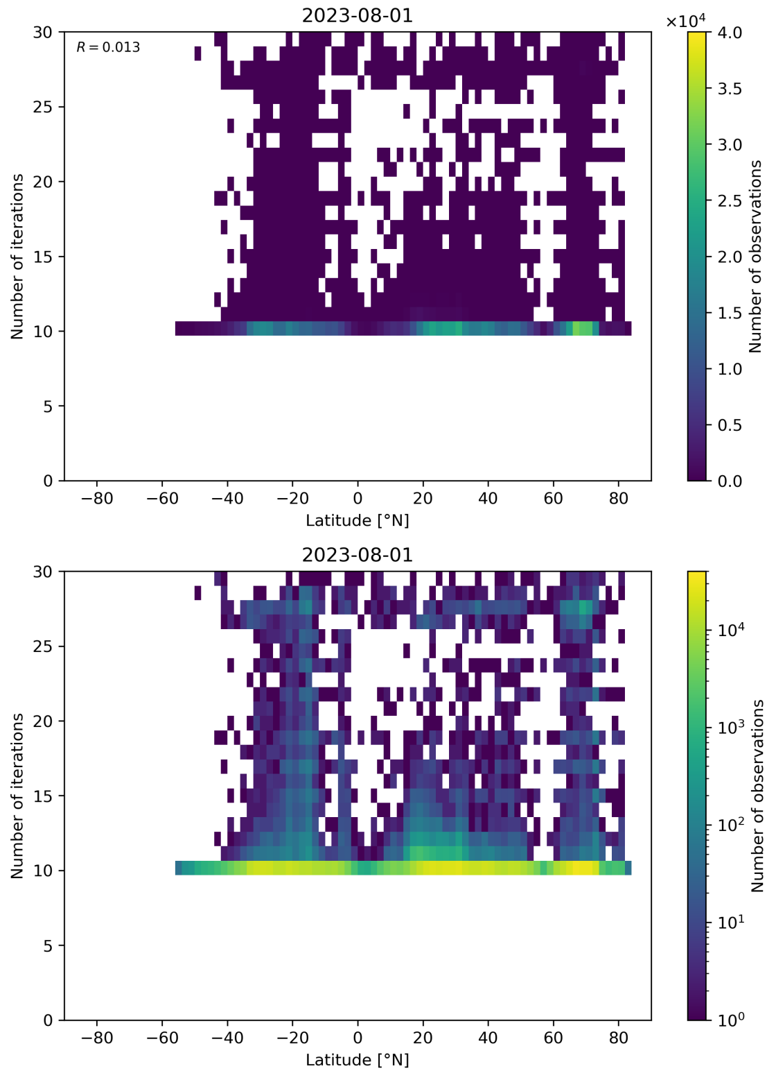
Figure 60: Scatter density plot of “Latitude” against “Number of iterations” for 2023-07-31 to 2023-08-02.
