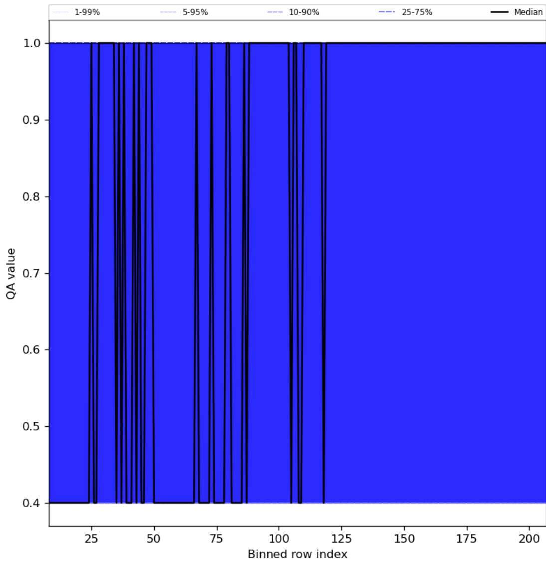
Figure 33: Along track statistics of “QA value” for 2023-07-31 to 2023-08-02
