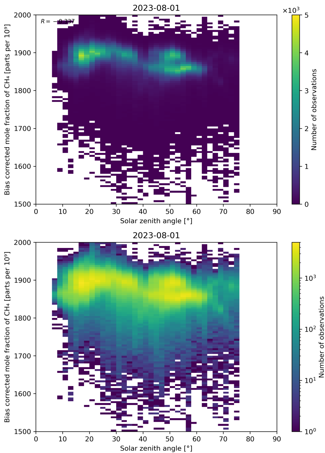
Figure 100: Scatter density plot of “Solar zenith angle” against “Bias corrected mole fraction of \text{CH}_4 ” for 2023-07-31 to 2023-08-02.
