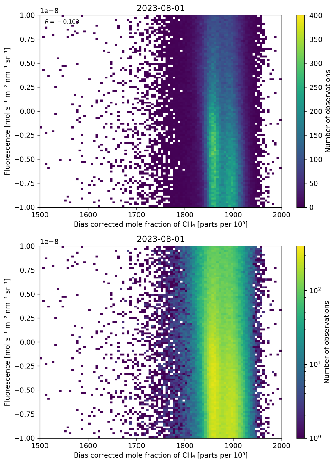
Figure 66: Scatter density plot of “Bias corrected mole fraction of \text{CH}_4 ” against “Fluorescence” for 2023-07-31 to 2023-08-02.
