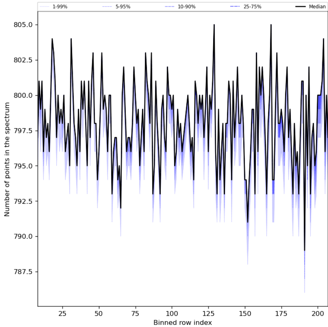
Figure 37: Along track statistics of “Number of points in the spectrum” for 2023-07-31 to 2023-08-02
