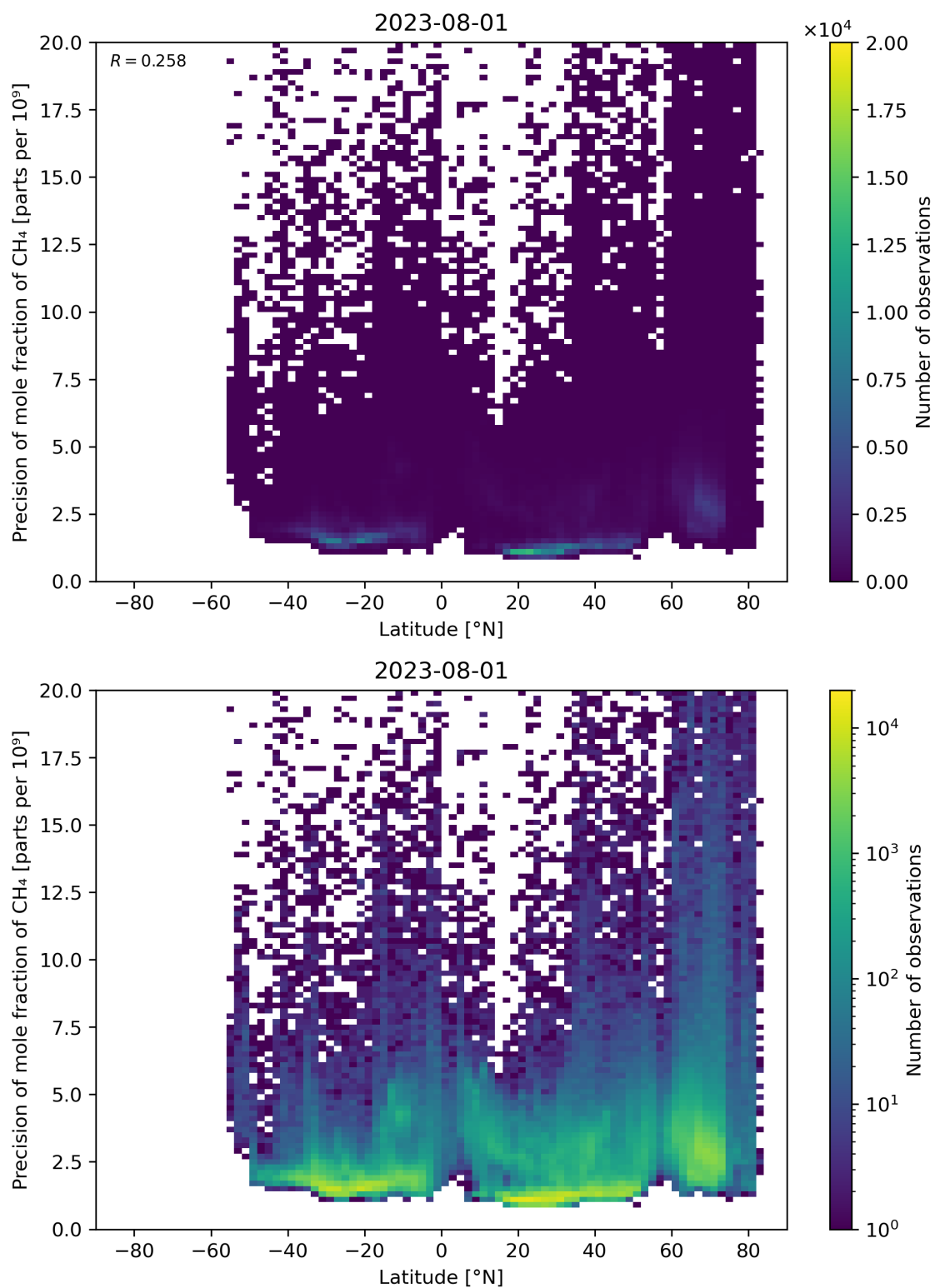
Figure 59: Scatter density plot of “Latitude” against “Precision of mole fraction of \text{CH}_4 ” for 2023-07-31 to 2023-08-02.
