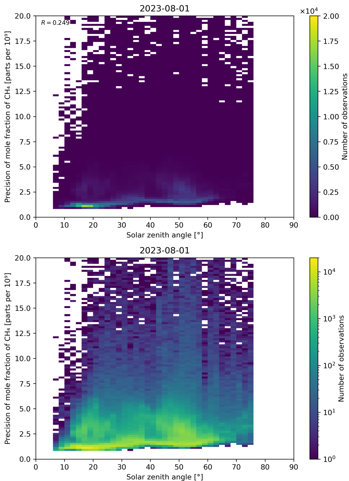
Figure 101: Scatter density plot of “Solar zenith angle” against “Precision of mole fraction of CH 4 ” for 2023-07-31 to 2023-08-02.
