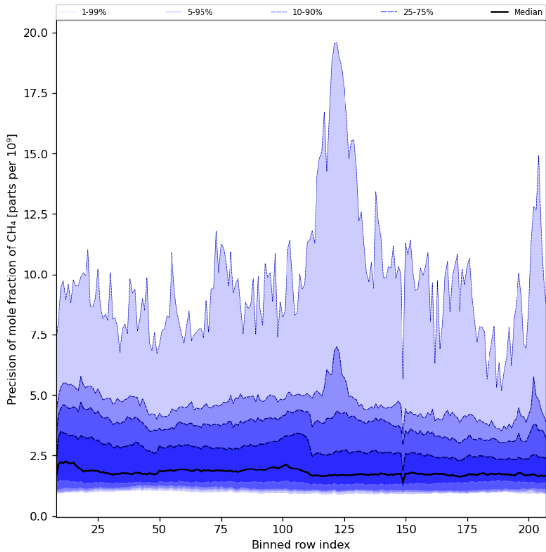
Figure 35: Along track statistics of “Precision of mole fraction of CH 4 ” for 2023-07-31 to 2023-08-02
