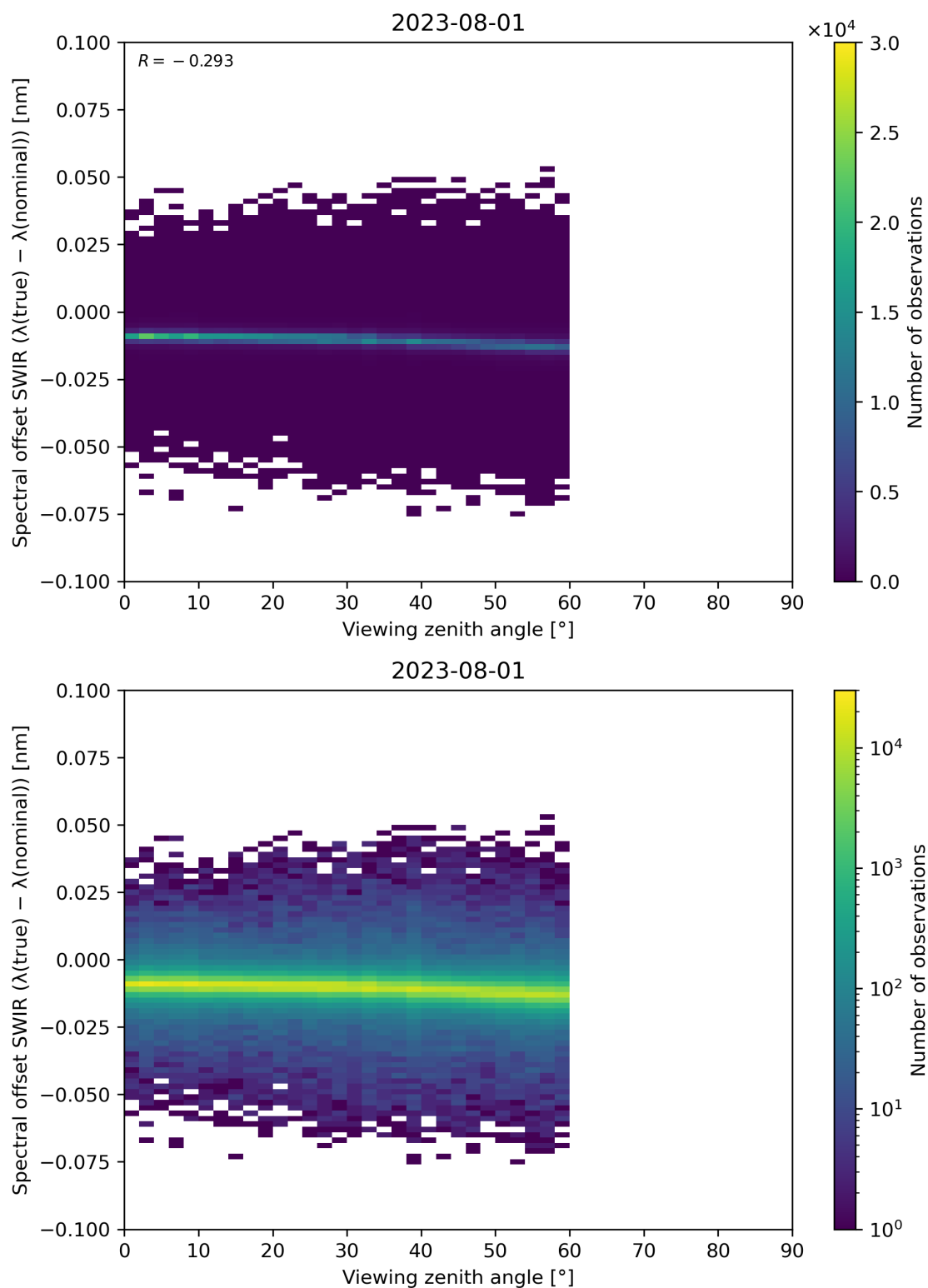
Figure 116: Scatter density plot of “Viewing zenith angle” against “Spectral offset SWIR ( \lambda(\text{true}) - \lambda(\text{nominal}) )” for 2023-07-31 to 2023-08-02.
