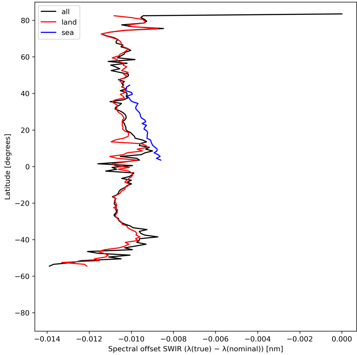
Figure 16: Zonal average of “Spectral offset SWIR ( \lambda(\text{true}) - \lambda(\text{nominal}) )” for 2023-07-31 to 2023-08-02.
