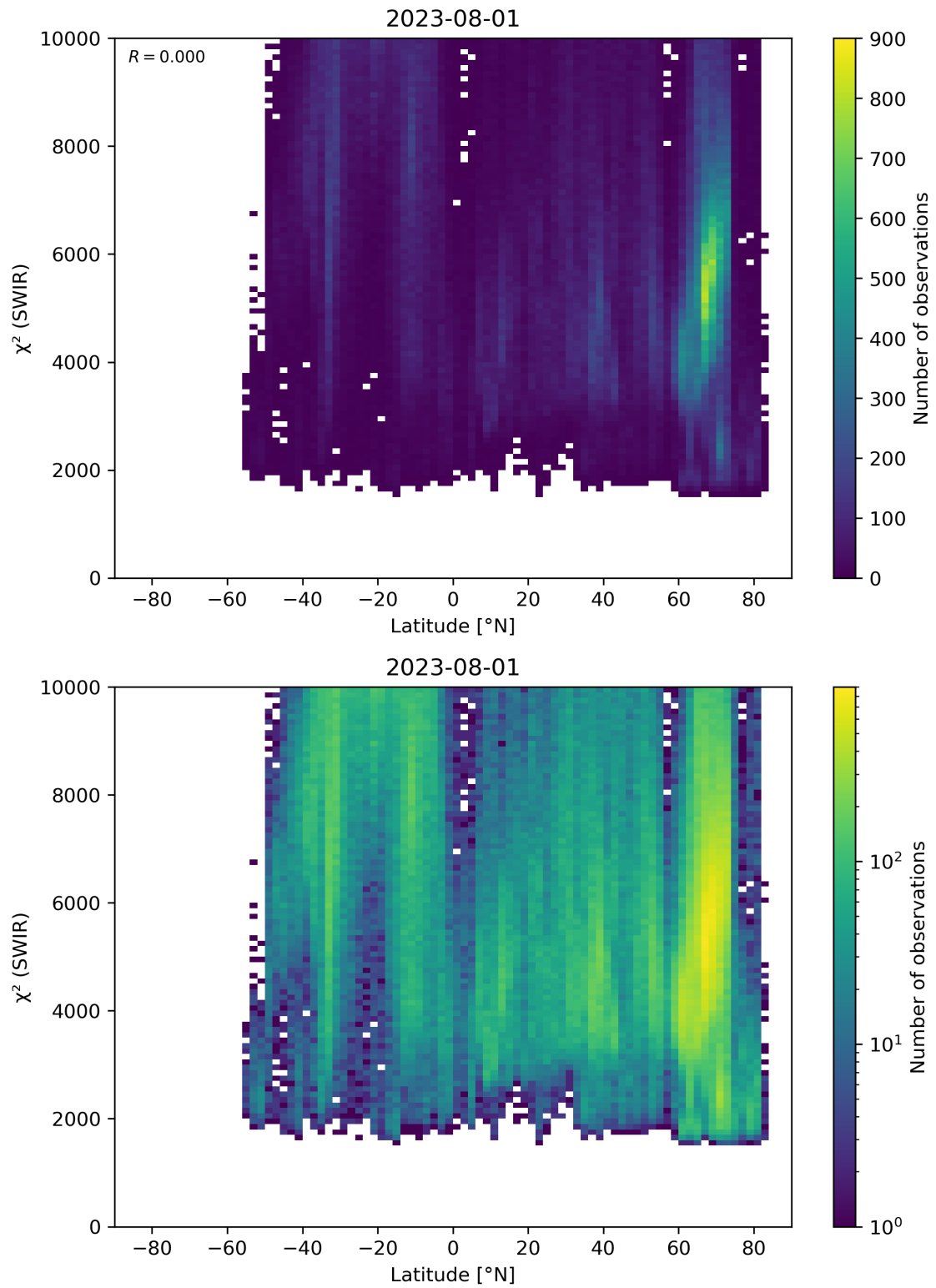
Figure 54: Scatter density plot of “Latitude” against “ \chi^2 (SWIR)” for 2023-07-31 to 2023-08-02.
