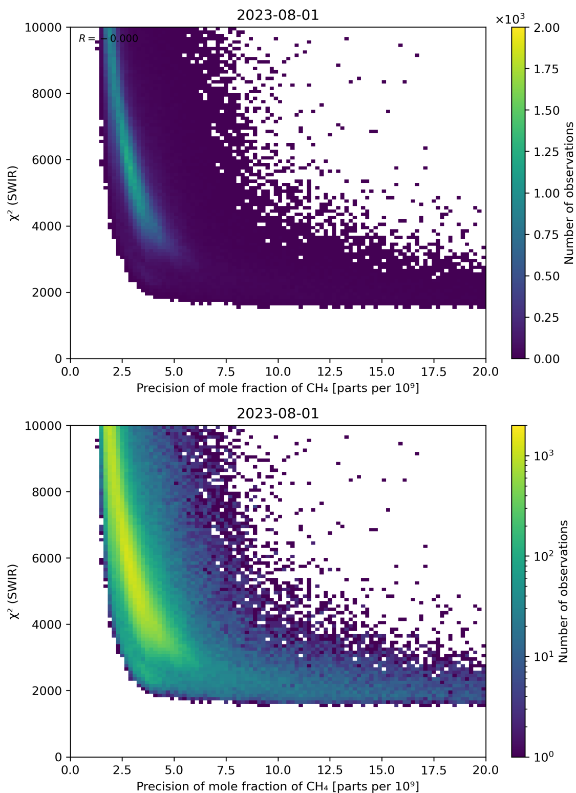
Figure 79: Scatter density plot of “Precision of mole fraction of CH 4 ” against “ \chi^2 (SWIR)” for 2023-07-31 to 2023-08-02.
