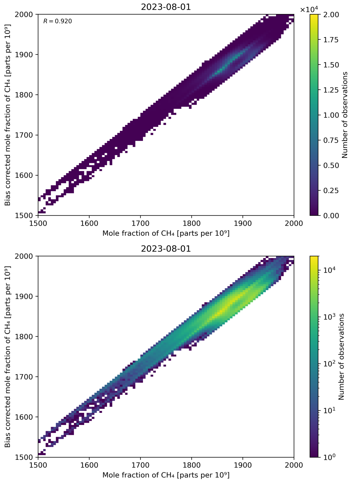
Figure 74: Scatter density plot of “Mole fraction of CH 4 ” against “Bias corrected mole fraction of CH 4 ” for 2023-07-31 to 2023-08-02.
