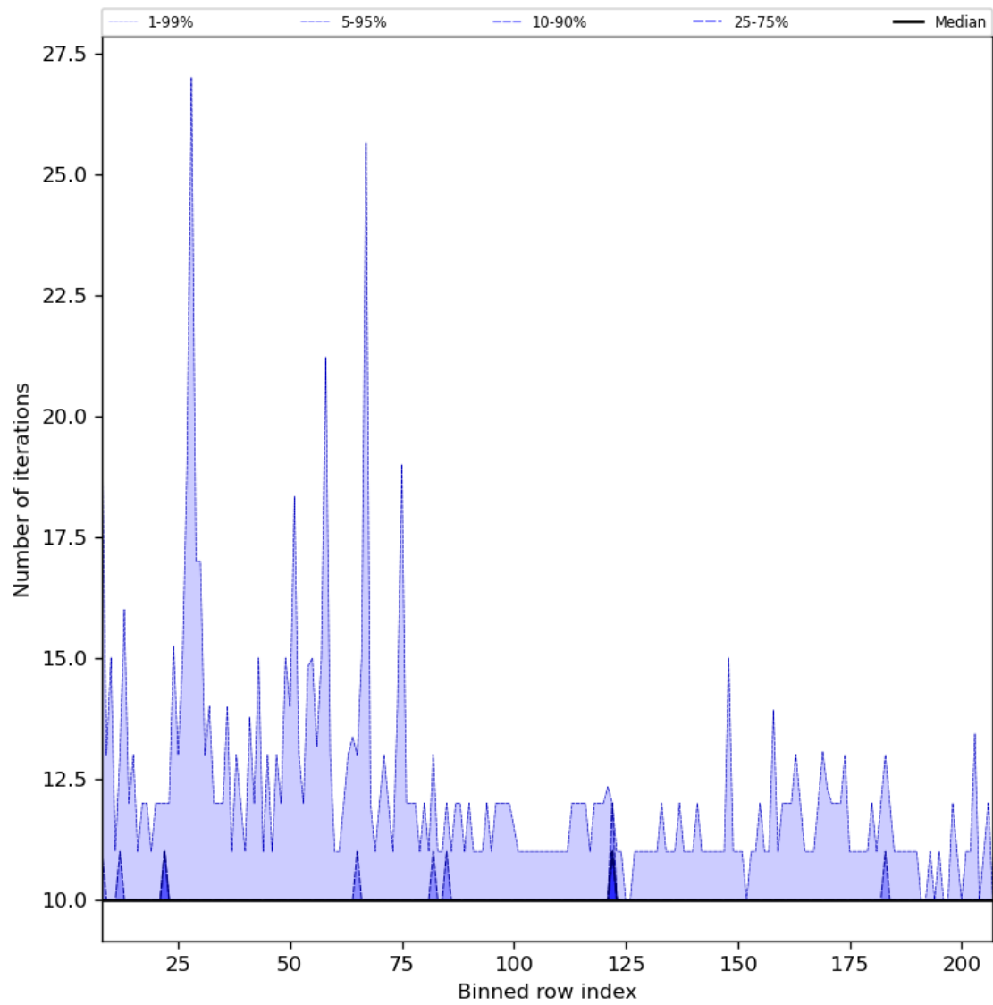
Figure 42: Along track statistics of “Number of iterations” for 2023-07-31 to 2023-08-02
