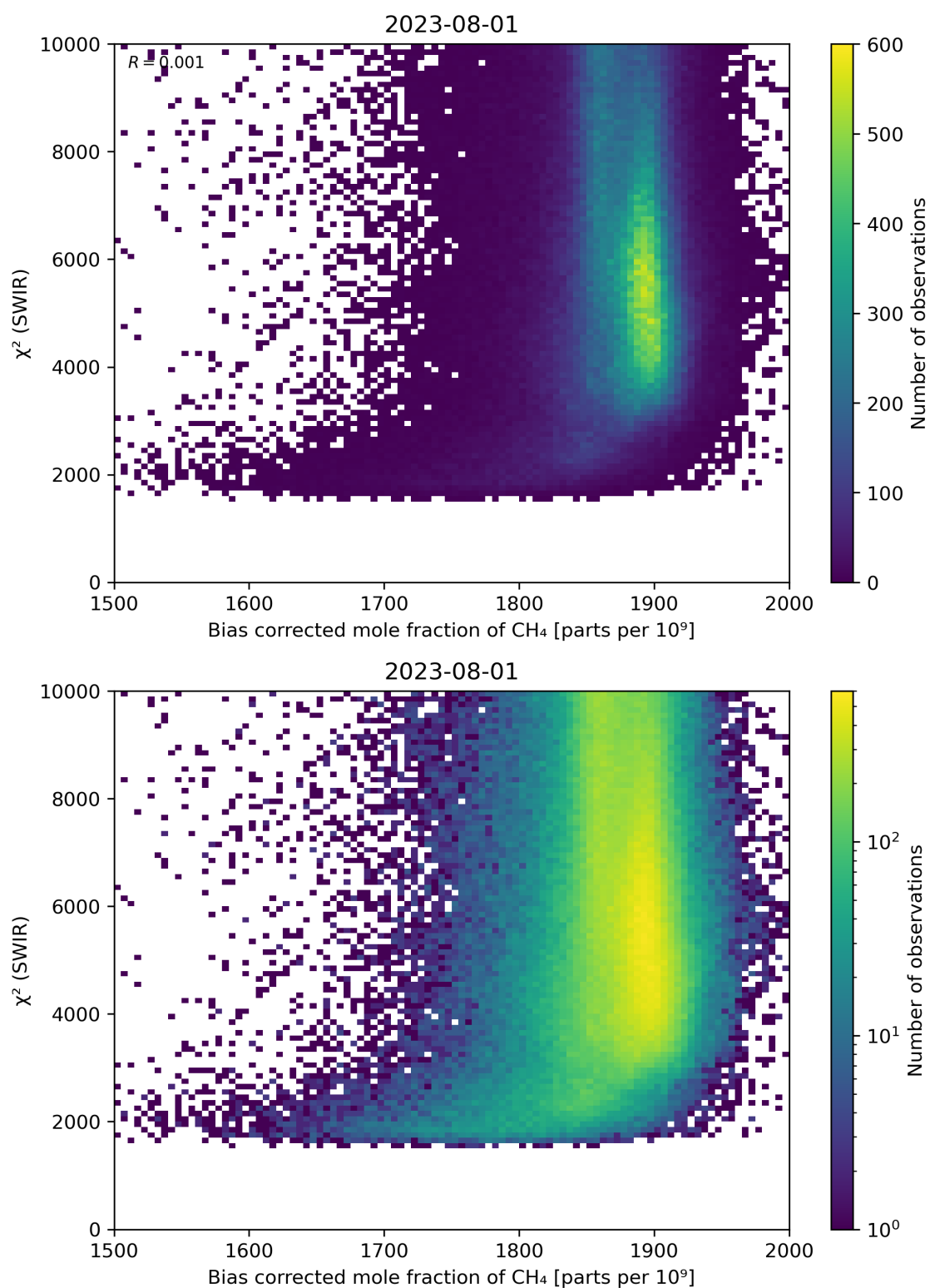
Figure 64: Scatter density plot of “Bias corrected mole fraction of CH 4 ” against “ \chi^2 (SWIR)” for 2023-07-31 to 2023-08-02.
