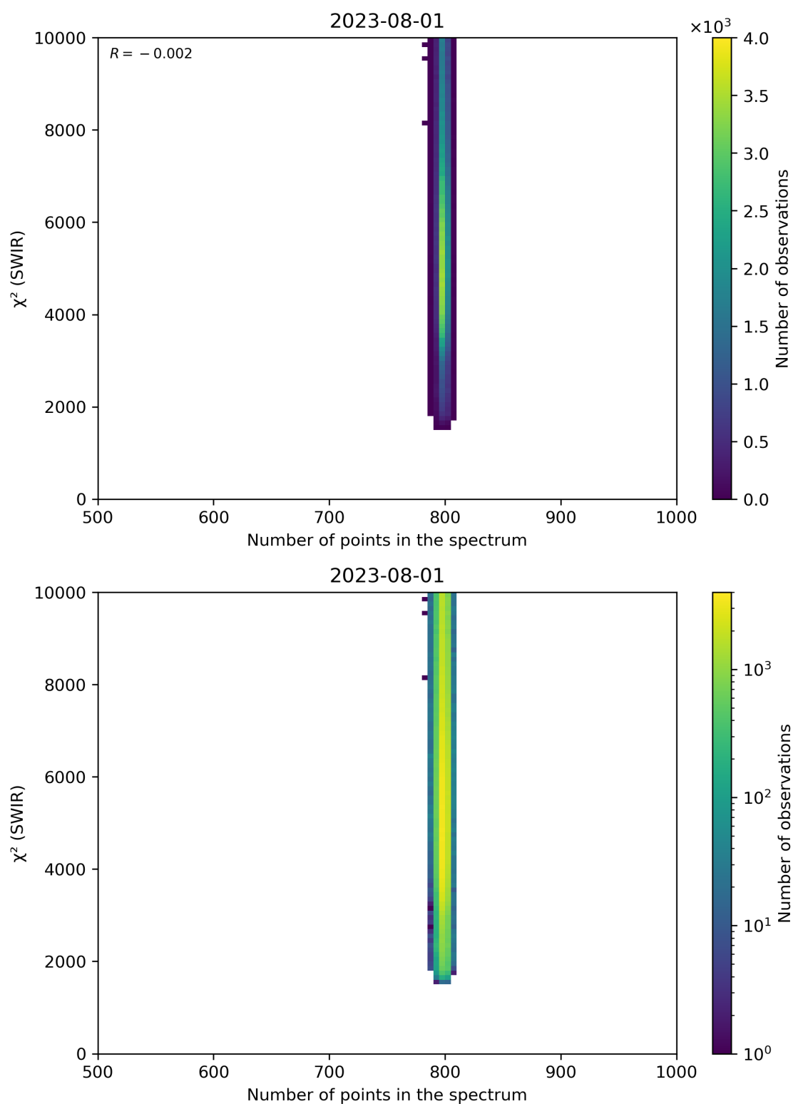
Figure 89: Scatter density plot of “Number of points in the spectrum” against “ \chi^2 (SWIR)” for 2023-07-31 to 2023-08-02.
