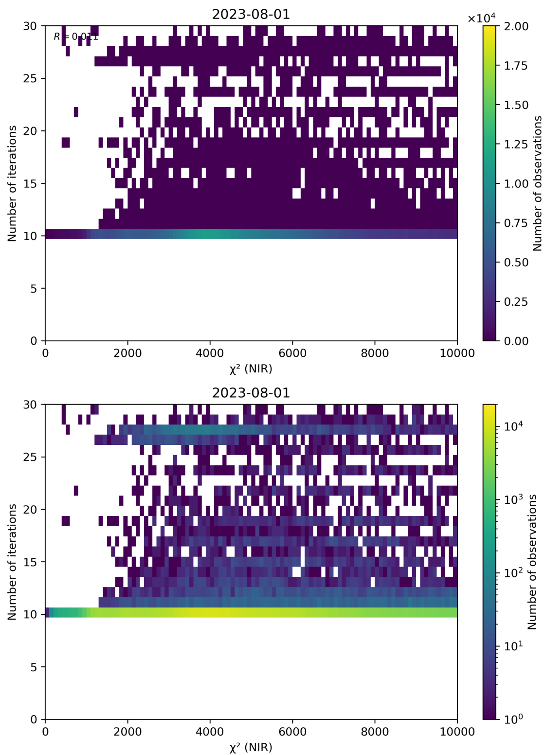
Figure 46: Scatter density plot of " \chi^2 (NIR)" against "Number of iterations" for 2023-07-31 to 2023-08-02.
