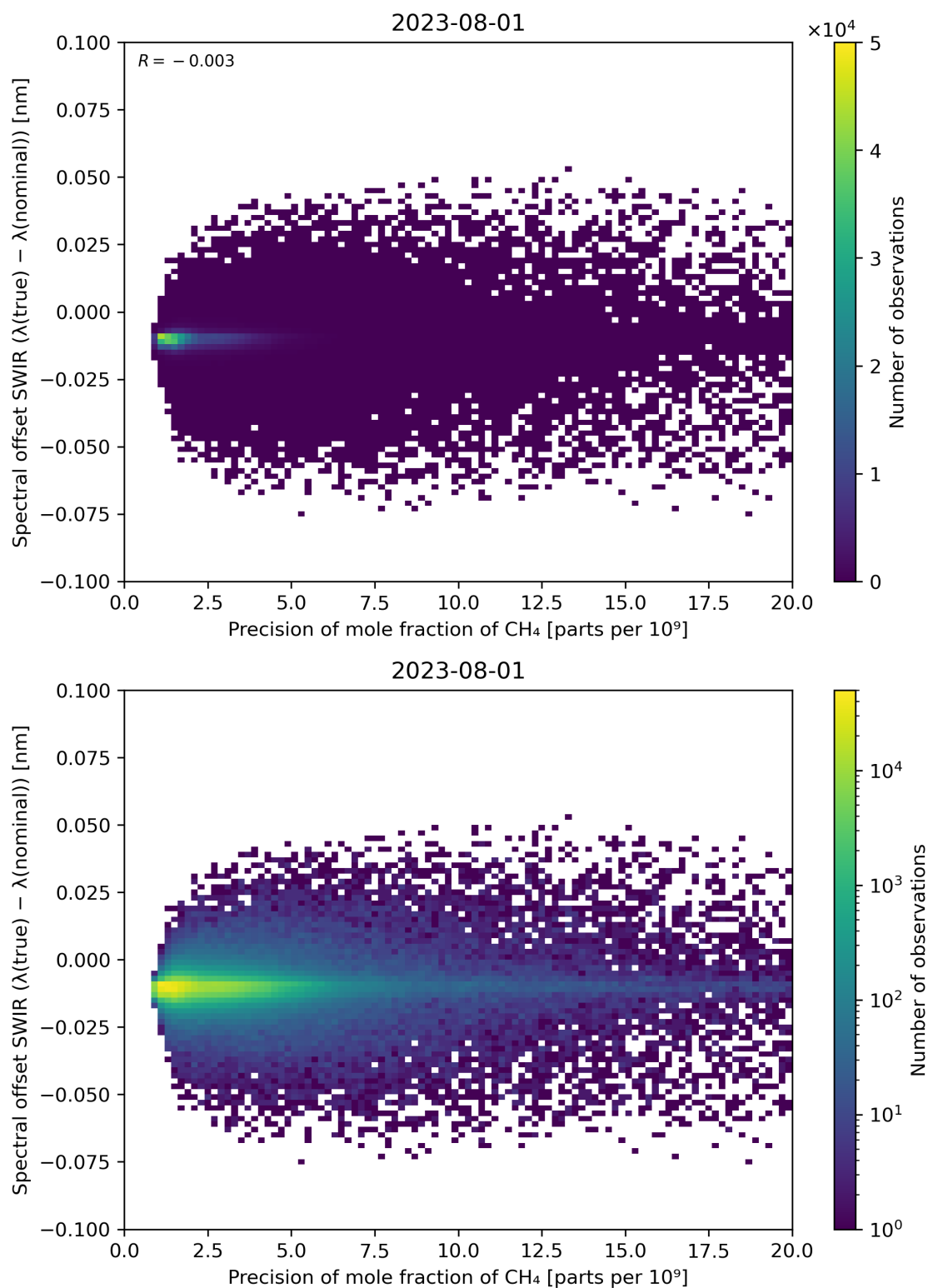
Figure 85: Scatter density plot of “Precision of mole fraction of \text{CH}_4 ” against “Spectral offset SWIR ( \lambda(\text{true}) - \lambda(\text{nominal}) )” for 2023-07-31 to 2023-08-02.
