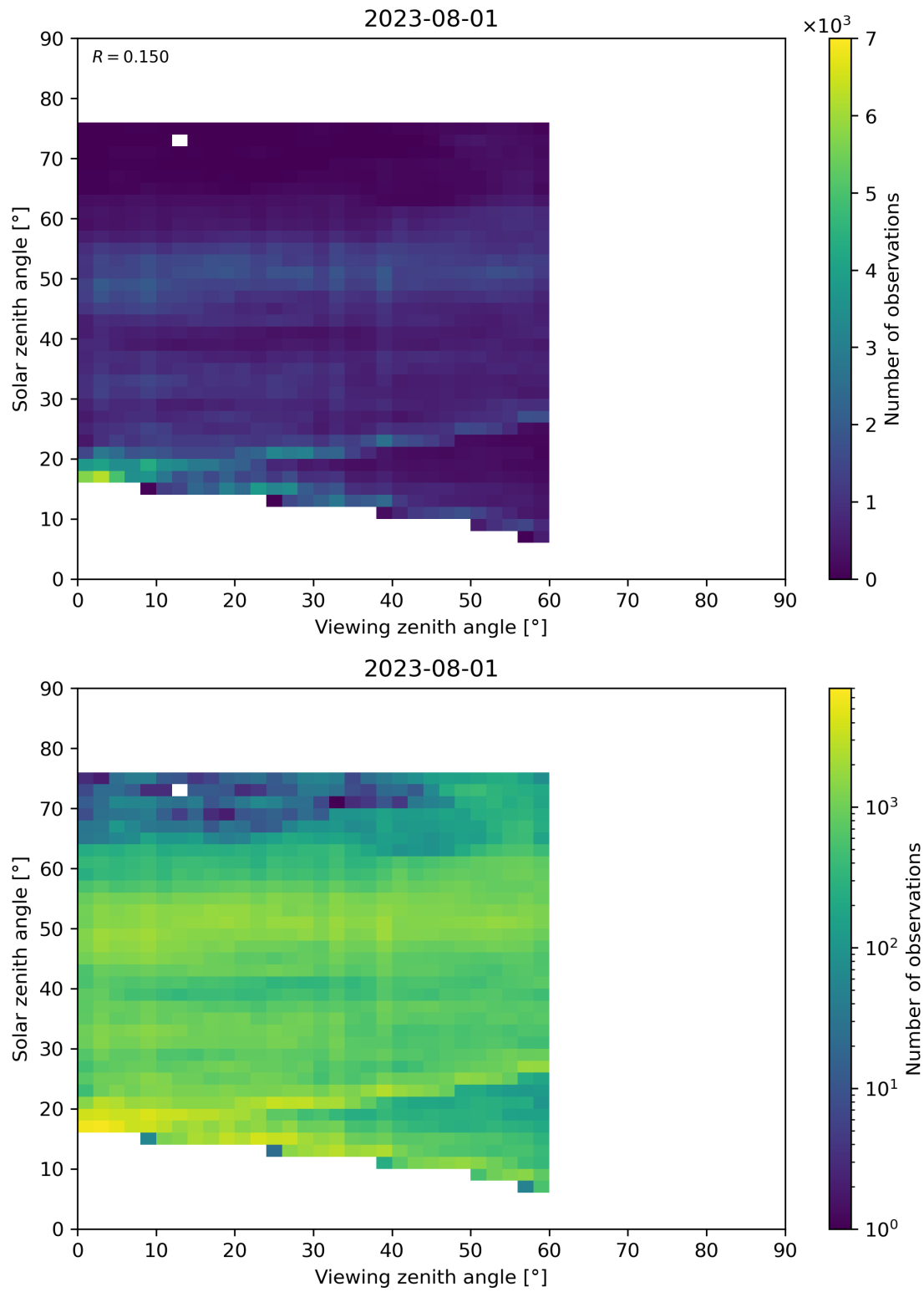
Figure 115: Scatter density plot of “Viewing zenith angle” against “Solar zenith angle” for 2023-07-31 to 2023-08-02.
