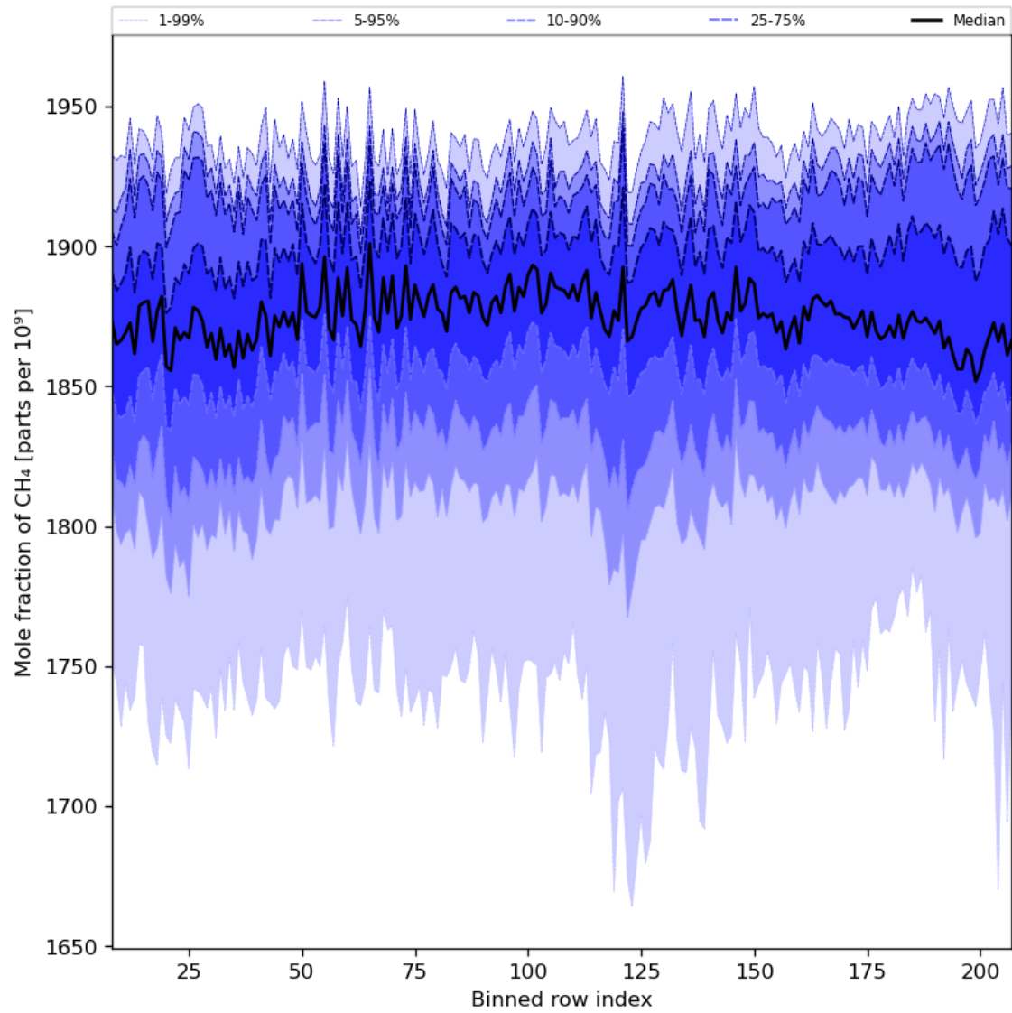
Figure 34: Along track statistics of “Mole fraction of CH 4 ” for 2023-07-31 to 2023-08-02
