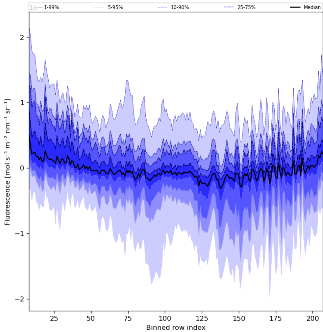
Figure 43: Along track statistics of “Fluorescence” for 2023-07-31 to 2023-08-02
