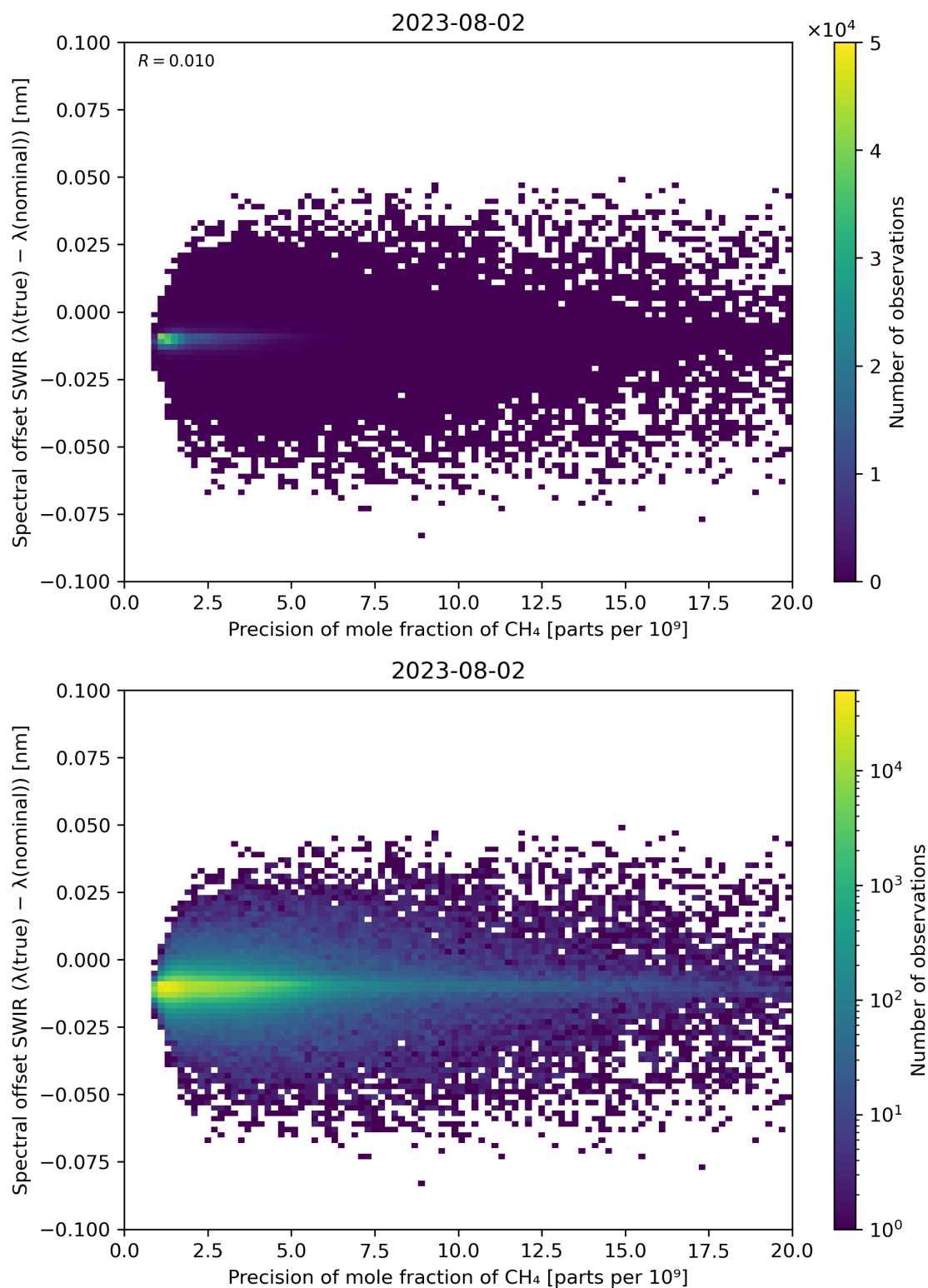
Figure 85: Scatter density plot of “Precision of mole fraction of CH 4 ” against “Spectral offset SWIR ( \lambda(\text{true}) - \lambda(\text{nominal}) )” for 2023-08-01 to 2023-08-03.
