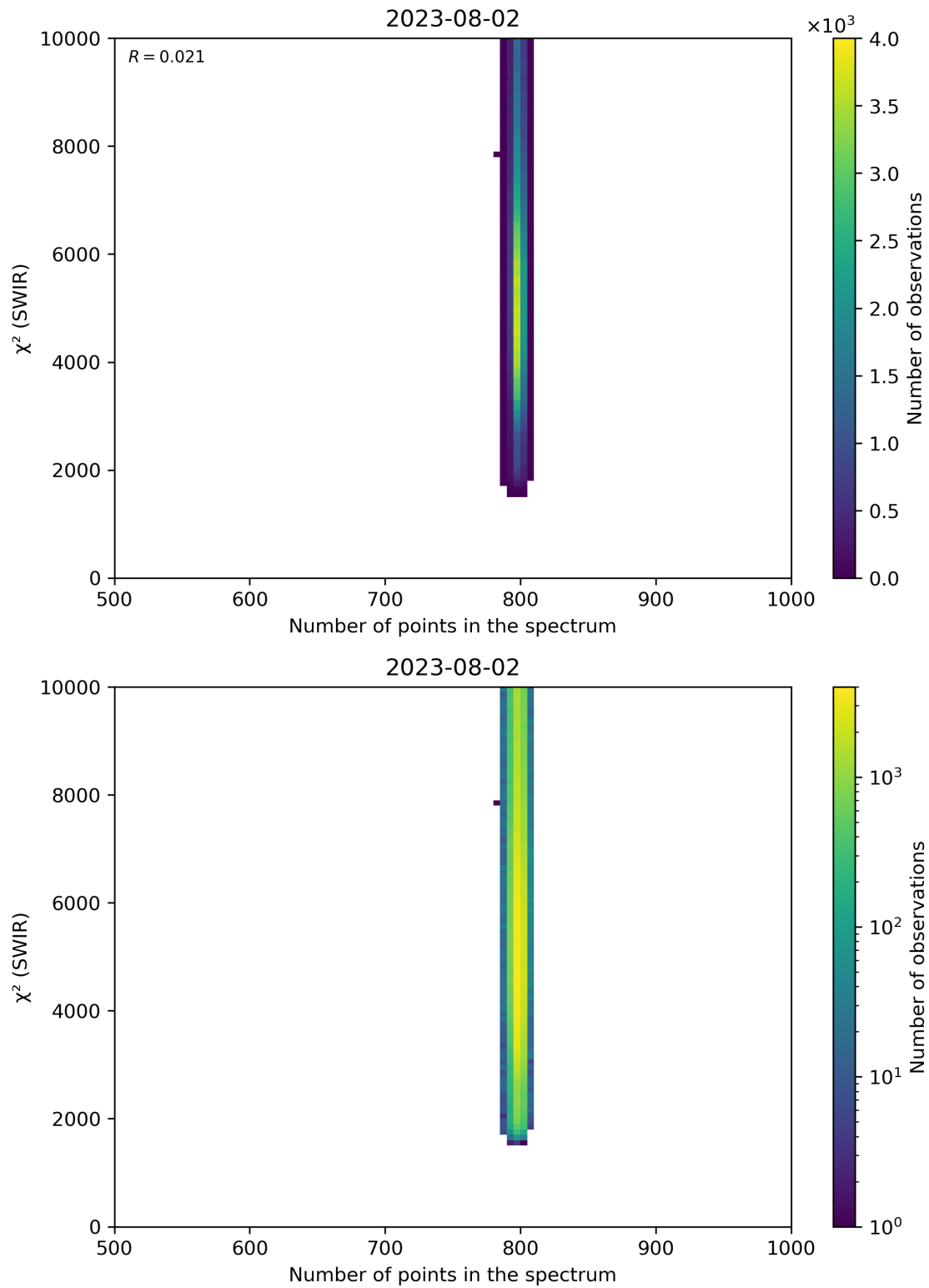
Figure 89: Scatter density plot of “Number of points in the spectrum” against “ \chi^2 (SWIR)” for 2023-08-01 to 2023-08-03.
