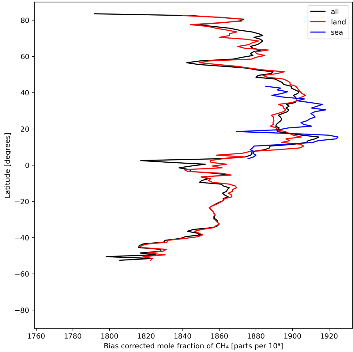
Figure 14: Zonal average of “Bias corrected mole fraction of CH 4 ” for 2023-08-01 to 2023-08-03.
