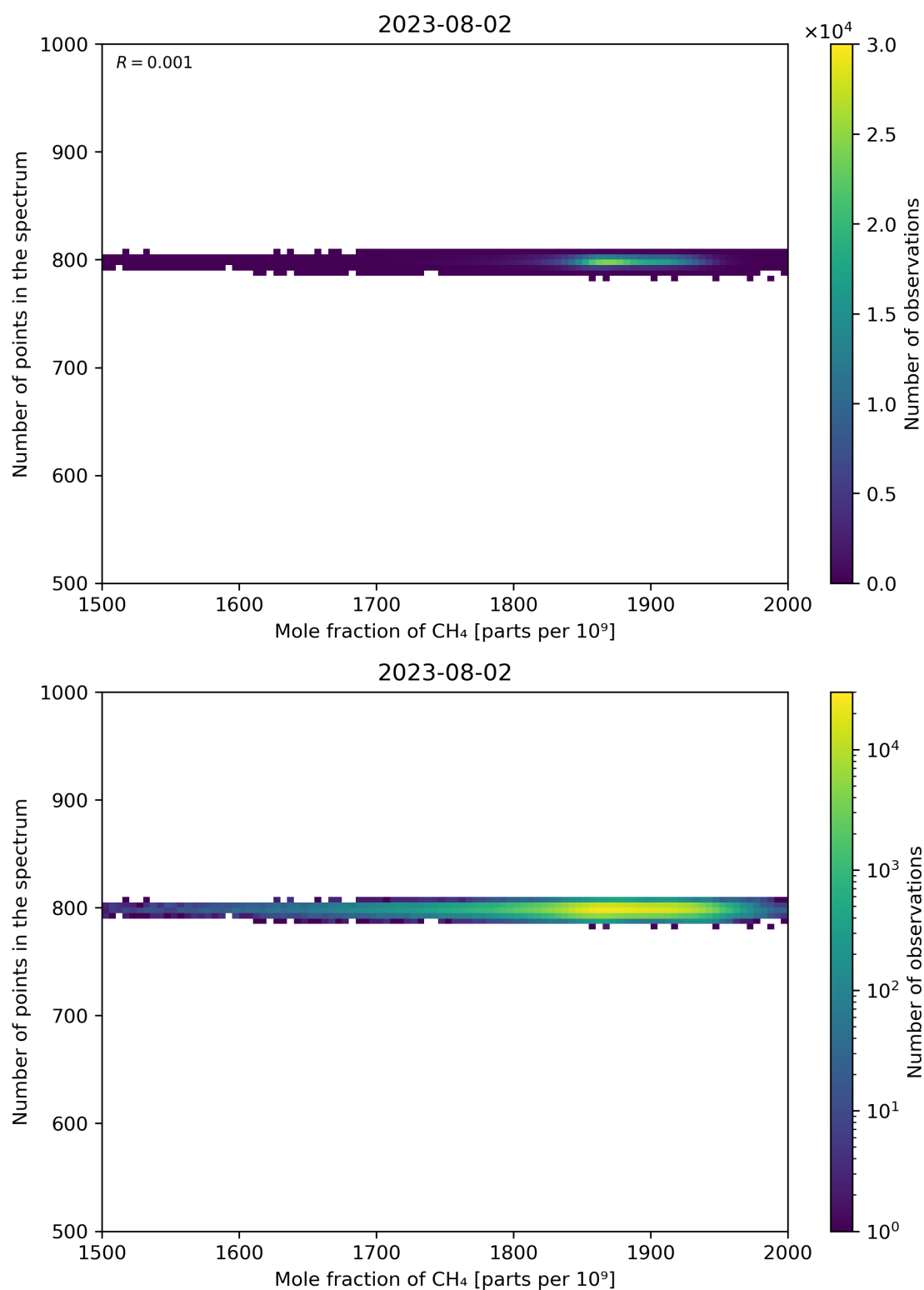
Figure 77: Scatter density plot of “Mole fraction of CH 4 ” against “Number of points in the spectrum” for 2023-08-01 to 2023-08-03.
