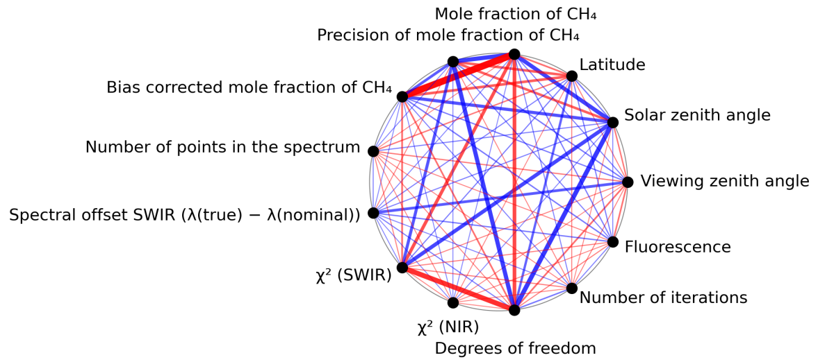
Figure 1: Map of correlation graph for 2023-08-01 to 2023-08-03.
