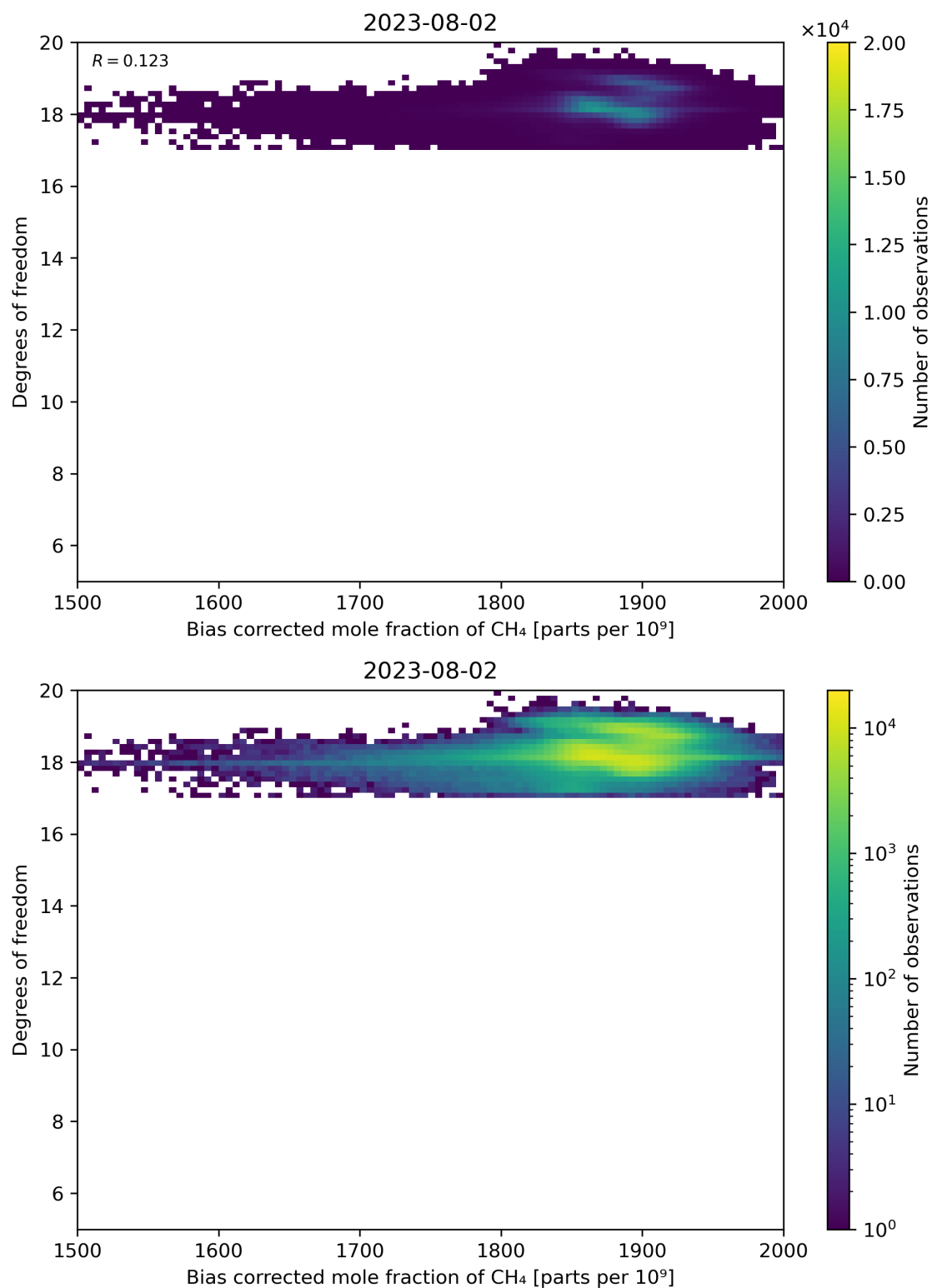
Figure 65: Scatter density plot of “Bias corrected mole fraction of CH 4 ” against “Degrees of freedom” for 2023-08-01 to 2023-08-03.
