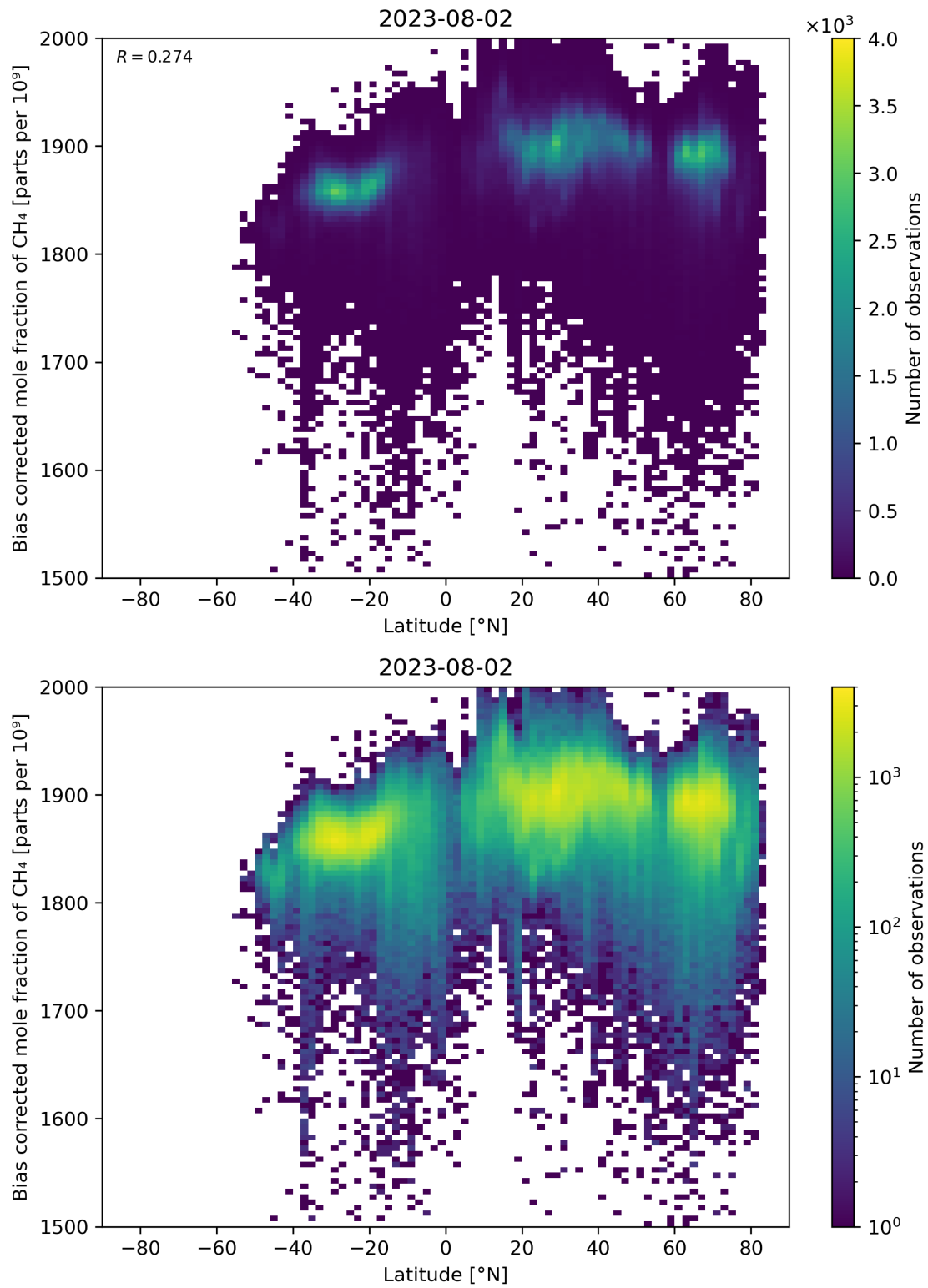
Figure 58: Scatter density plot of “Latitude” against “Bias corrected mole fraction of CH 4 ” for 2023-08-01 to 2023-08-03.
