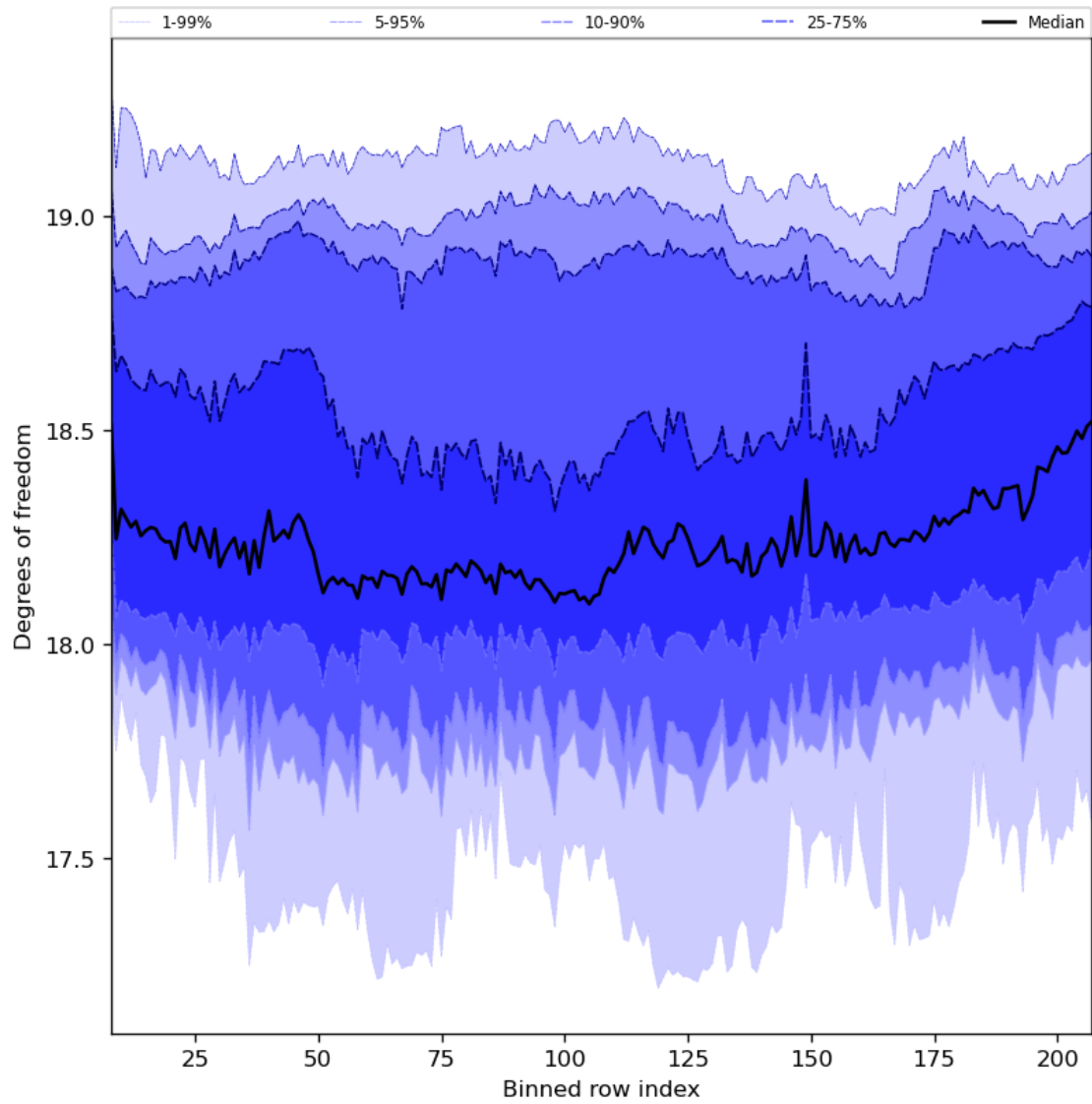
Figure 41: Along track statistics of “Degrees of freedom” for 2023-08-01 to 2023-08-03
