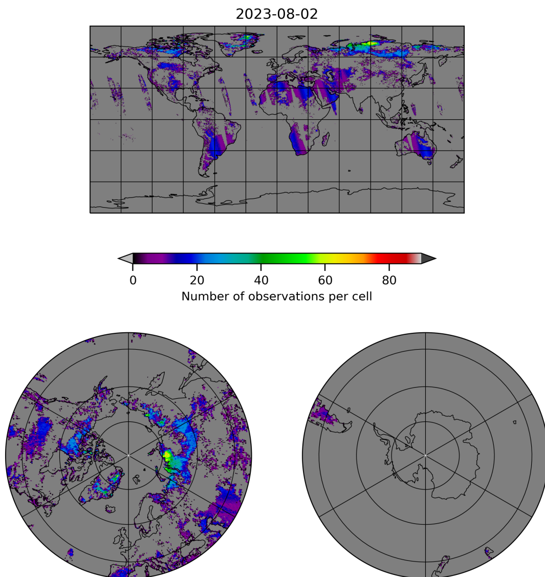
Figure 10: Map of the number of observations for 2023-08-01 to 2023-08-03
