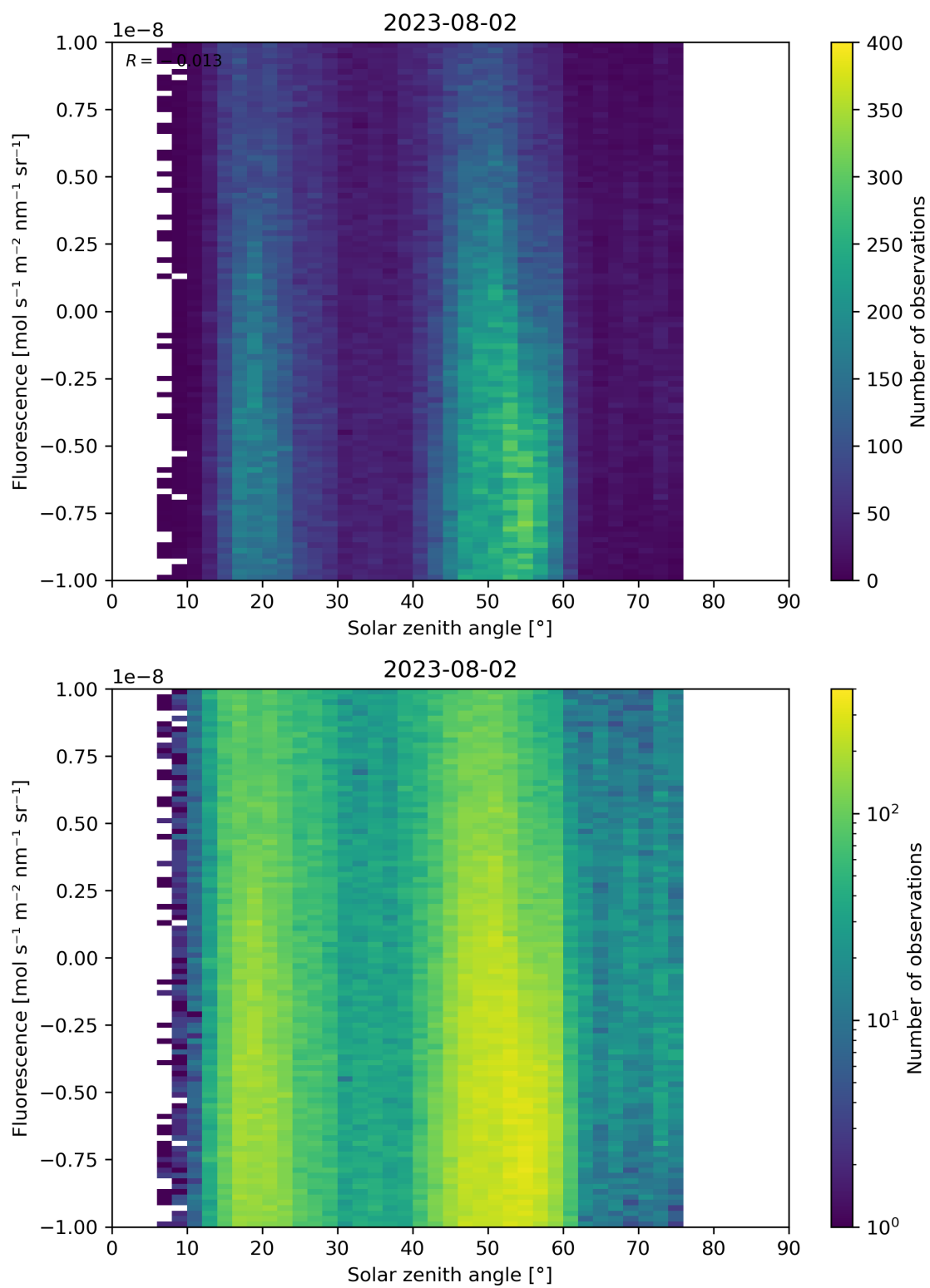
Figure 97: Scatter density plot of “Solar zenith angle” against “Fluorescence” for 2023-08-01 to 2023-08-03.
