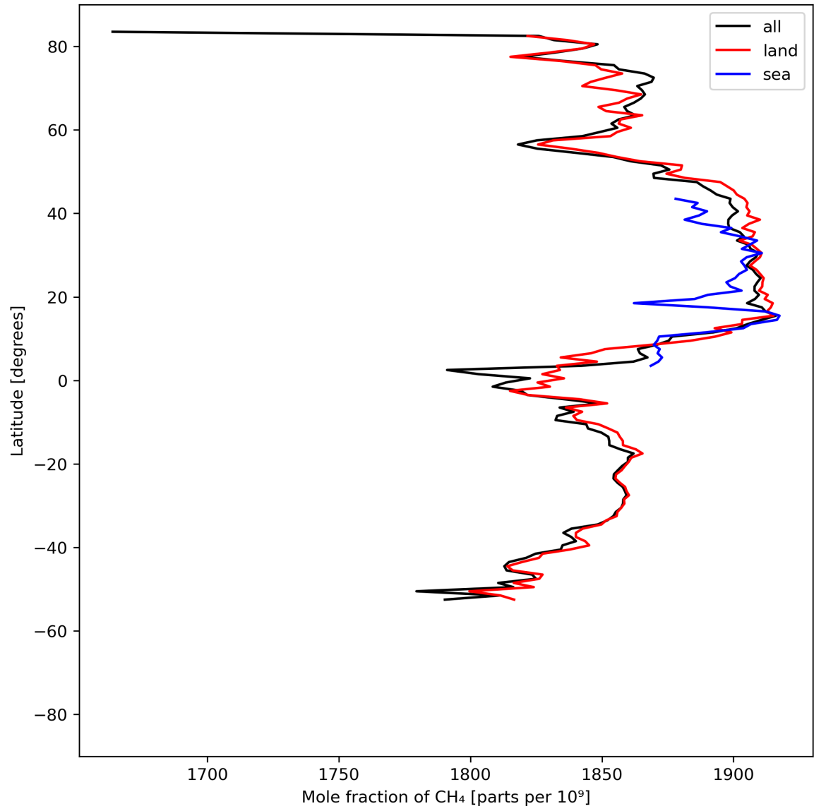
Figure 12: Zonal average of “Mole fraction of CH 4 ” for 2023-08-01 to 2023-08-03.
