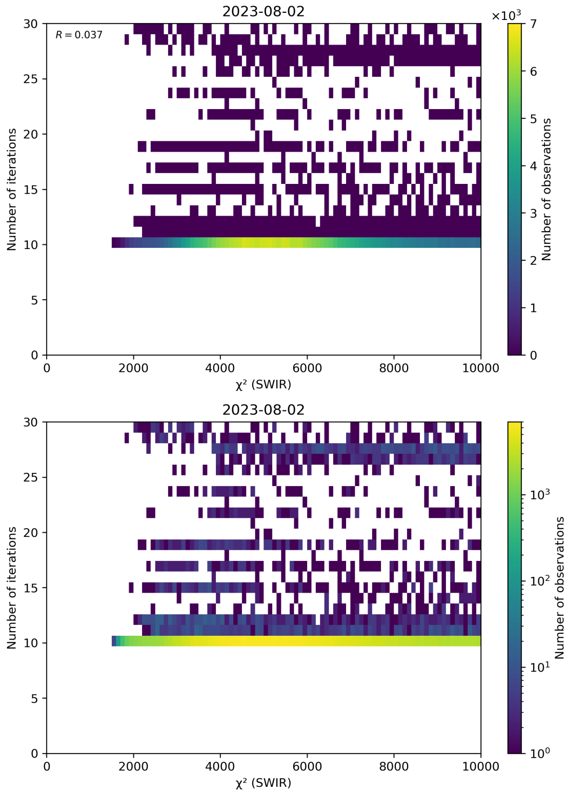
Figure 50: Scatter density plot of “ \chi^2 (SWIR)” against “Number of iterations” for 2023-08-01 to 2023-08-03.
