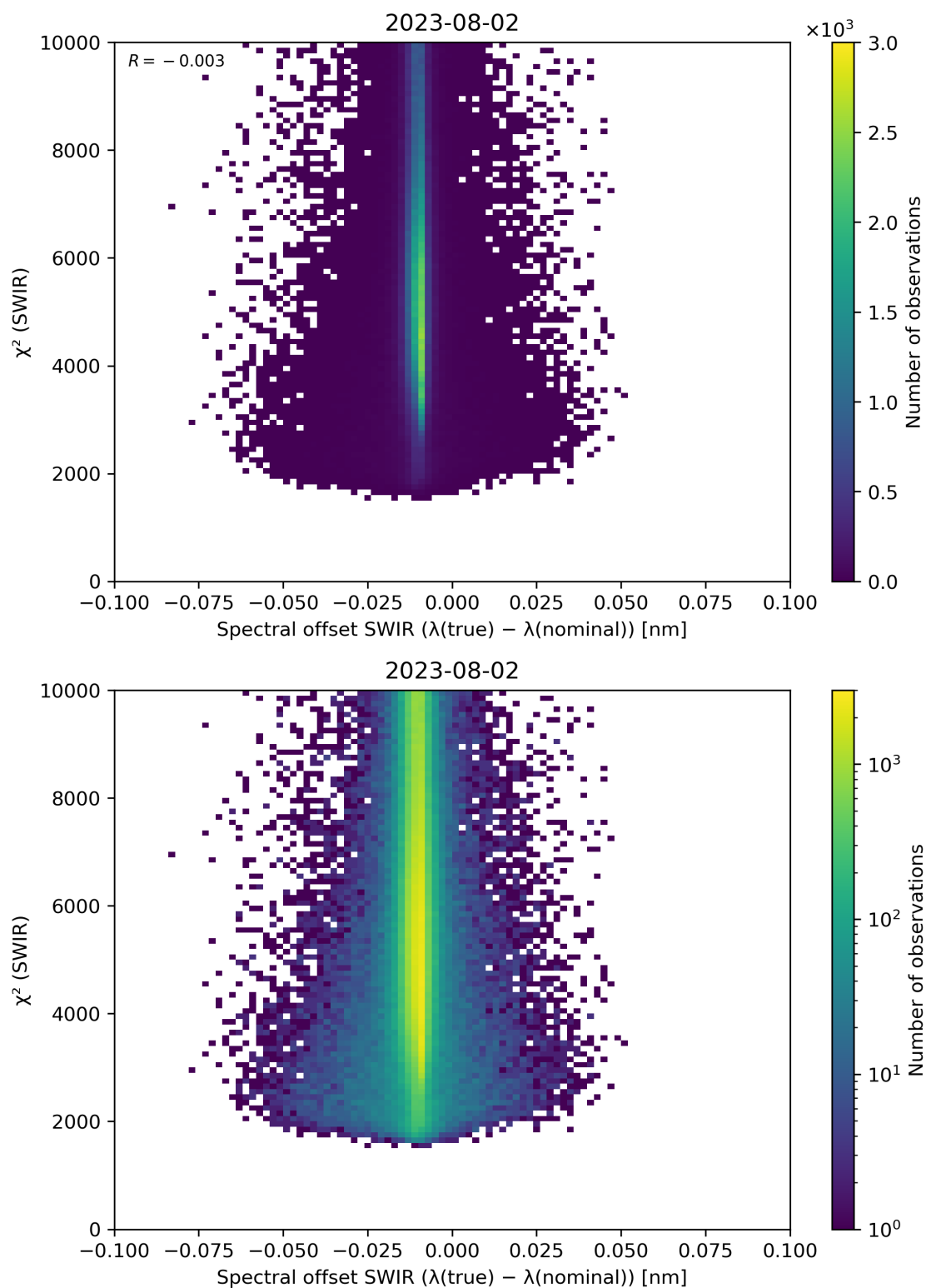
Figure 118: Scatter density plot of “Spectral offset SWIR ( \lambda(\text{true}) - \lambda(\text{nominal}) )” against “ \chi^2 (SWIR)” for 2023-08-01 to 2023-08-03.
