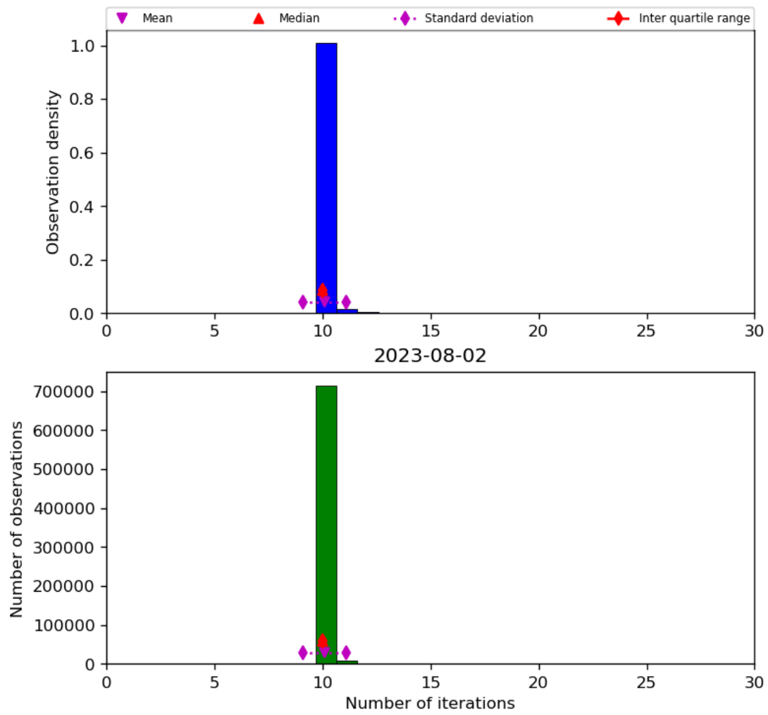
Figure 31: Histogram of “Number of iterations” for 2023-08-01 to 2023-08-03
