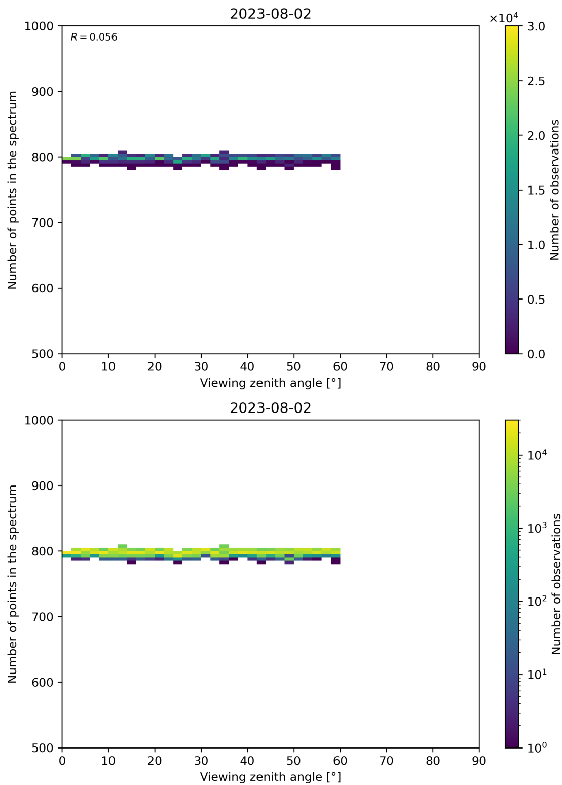
Figure 114: Scatter density plot of “Viewing zenith angle” against “Number of points in the spectrum” for 2023-08-01 to 2023-08-03.
