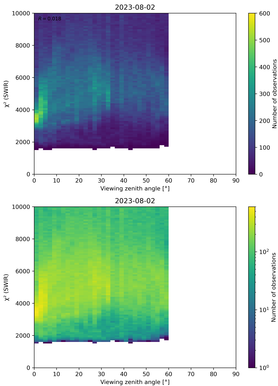
Figure 106: Scatter density plot of “Viewing zenith angle” against “ \chi^2 (SWIR)” for 2023-08-01 to 2023-08-03.
