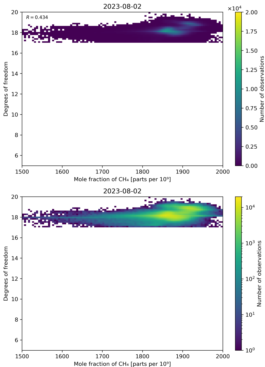
Figure 72: Scatter density plot of “Mole fraction of CH 4 ” against “Degrees of freedom” for 2023-08-01 to 2023-08-03.
