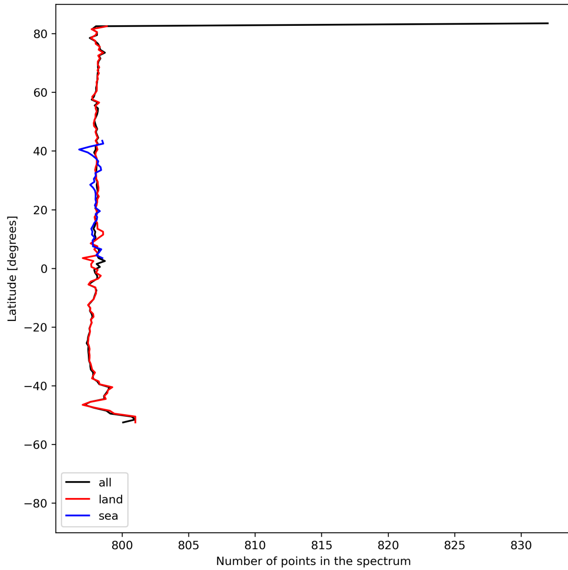
Figure 15: Zonal average of “Number of points in the spectrum” for 2023-08-01 to 2023-08-03.
