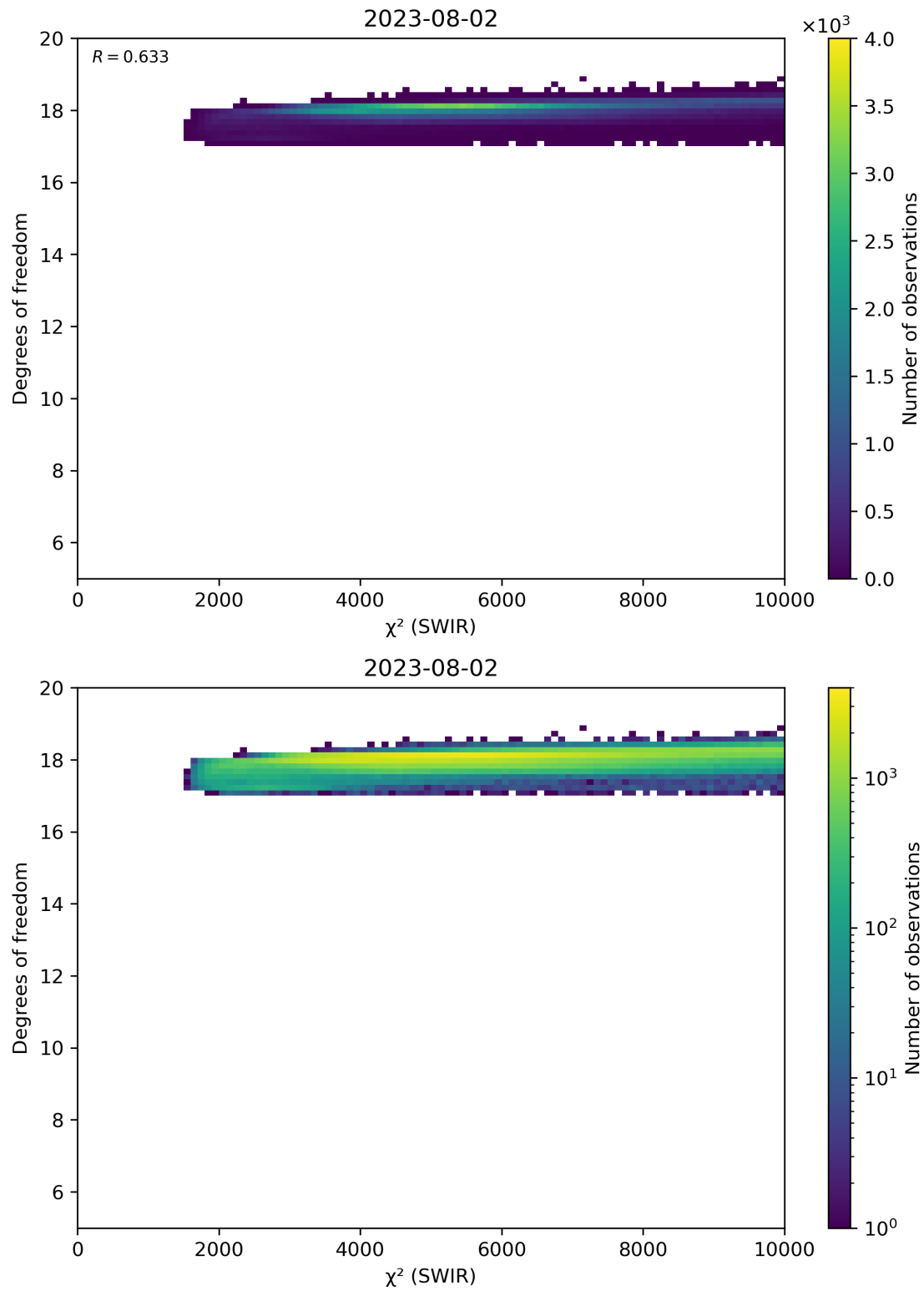
Figure 48: Scatter density plot of “ \chi^2 (SWIR)” against “Degrees of freedom” for 2023-08-01 to 2023-08-03.
