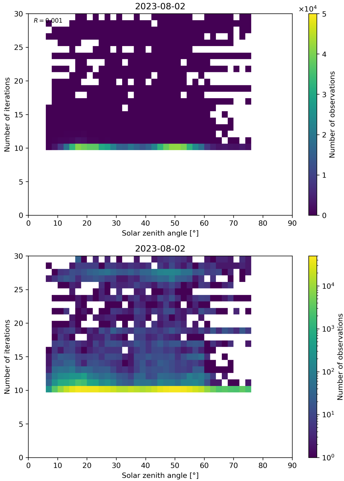
Figure 102: Scatter density plot of “Solar zenith angle” against “Number of iterations” for 2023-08-01 to 2023-08-03.
