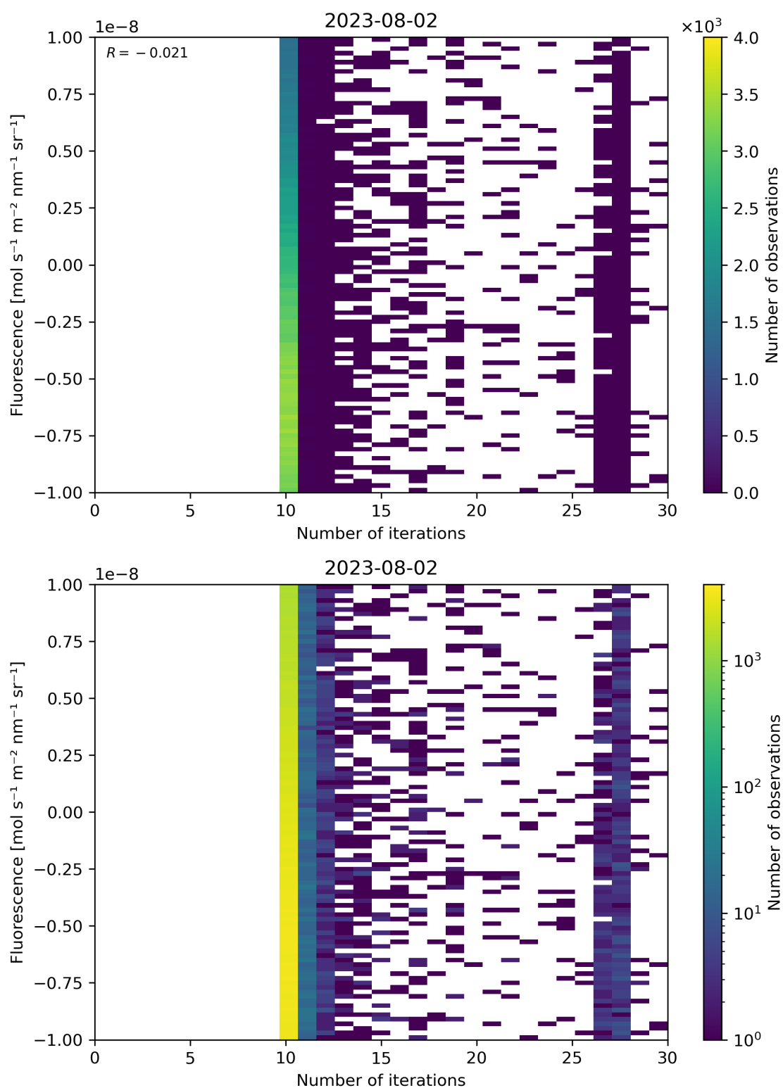
Figure 87: Scatter density plot of “Number of iterations” against “Fluorescence” for 2023-08-01 to 2023-08-03.
