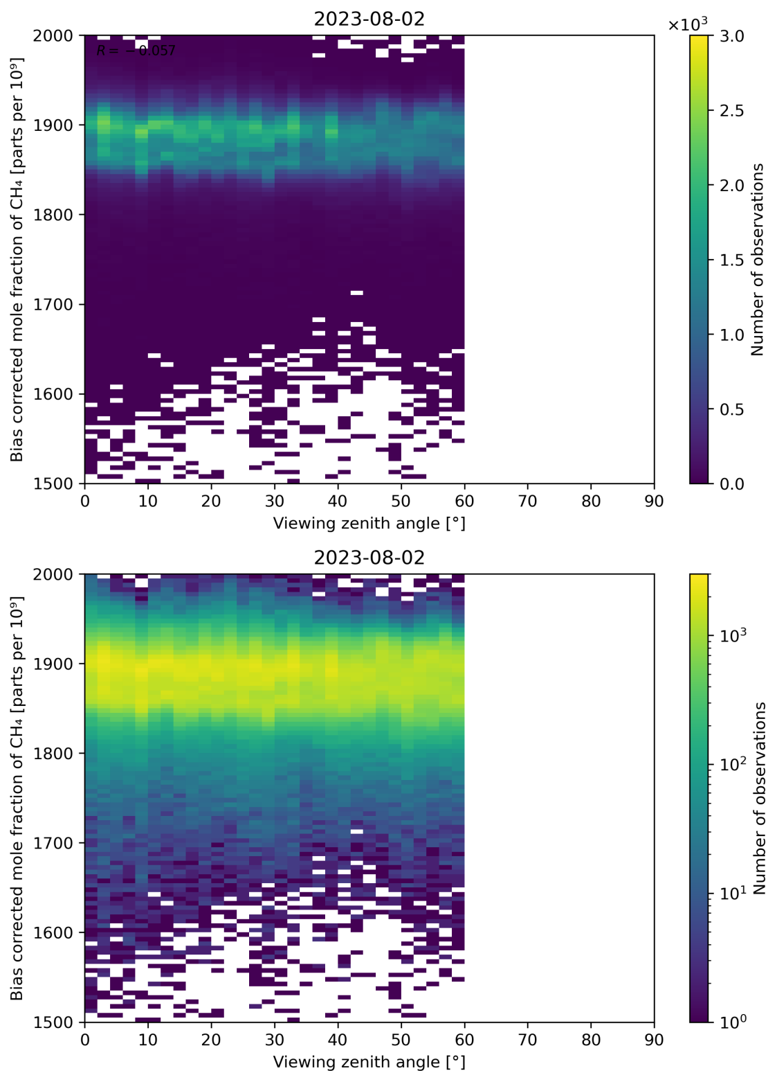
Figure 111: Scatter density plot of “Viewing zenith angle” against “Bias corrected mole fraction of CH 4 ” for 2023-08-01 to 2023-08-03.
