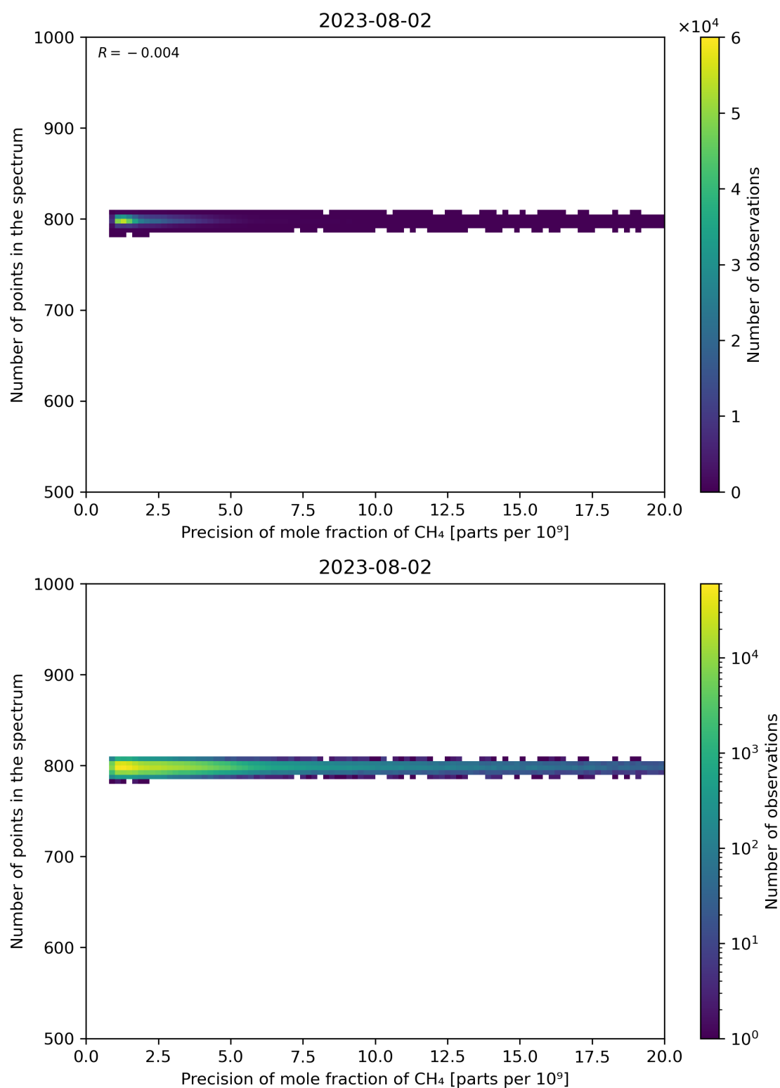
Figure 84: Scatter density plot of “Precision of mole fraction of CH 4 ” against “Number of points in the spectrum” for 2023-08-01 to 2023-08-03.
