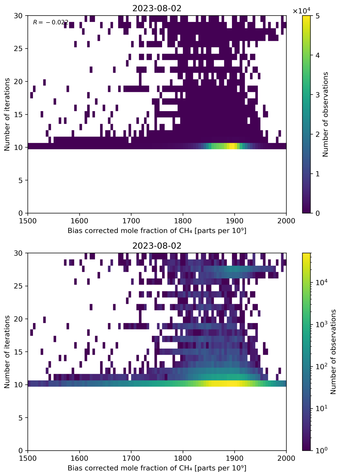
Figure 67: Scatter density plot of “Bias corrected mole fraction of CH 4 ” against “Number of iterations” for 2023-08-01 to 2023-08-03.
