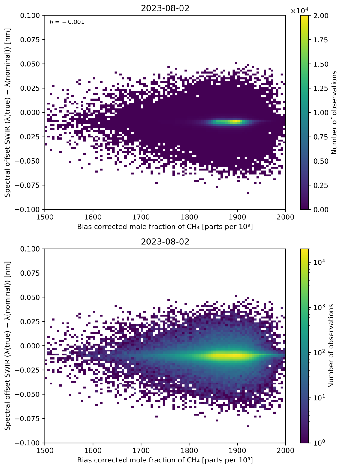
Figure 69: Scatter density plot of “Bias corrected mole fraction of \text{CH}_4 ” against “Spectral offset SWIR ( \lambda(\text{true}) - \lambda(\text{nominal}) )” for 2023-08-01 to 2023-08-03.
