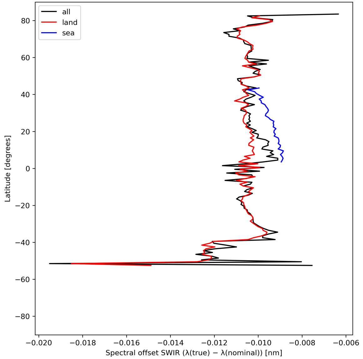
Figure 16: Zonal average of “Spectral offset SWIR ( \lambda(\text{true}) - \lambda(\text{nominal}) )” for 2023-08-01 to 2023-08-03.
