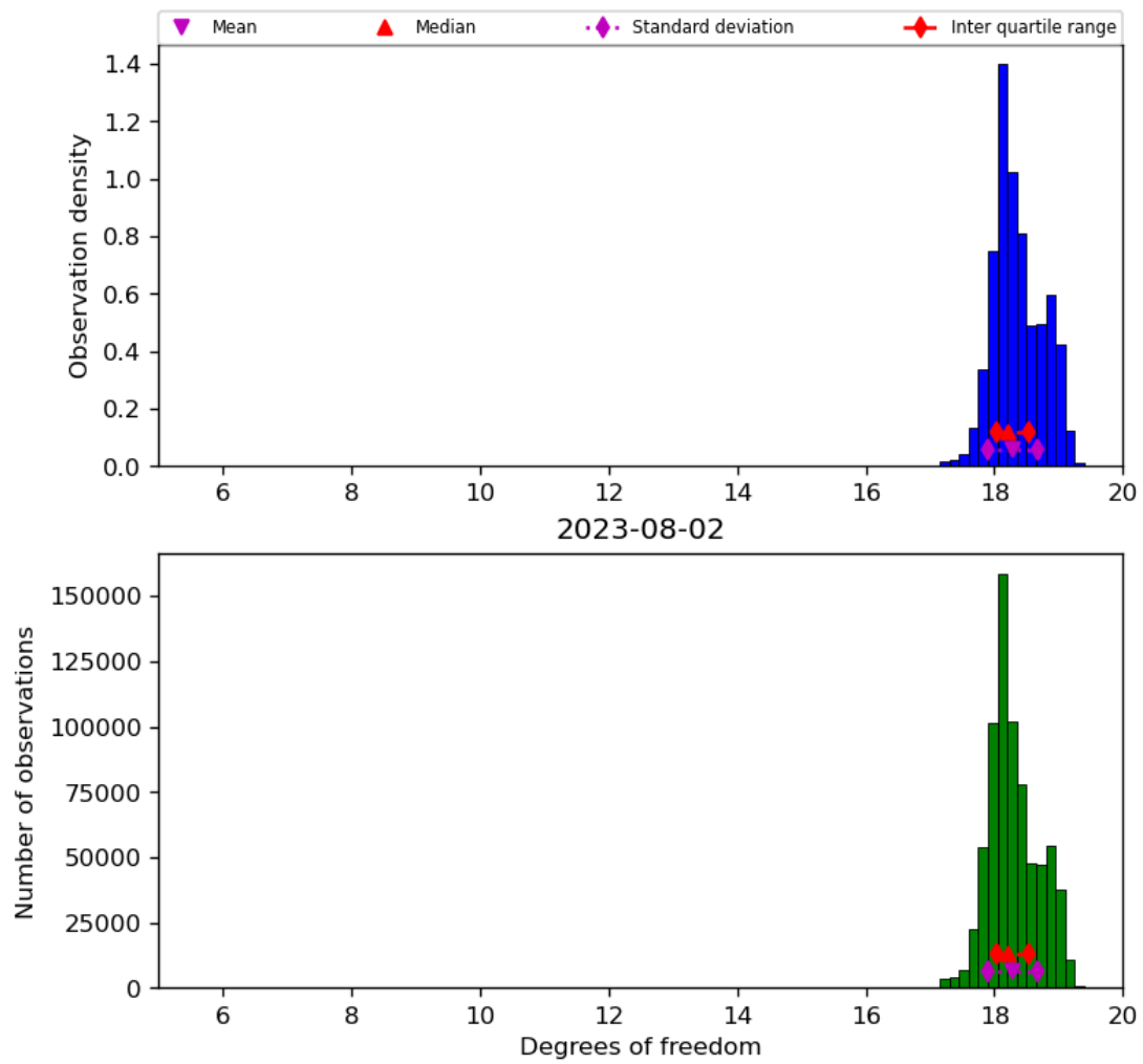
Figure 30: Histogram of “Degrees of freedom” for 2023-08-01 to 2023-08-03
