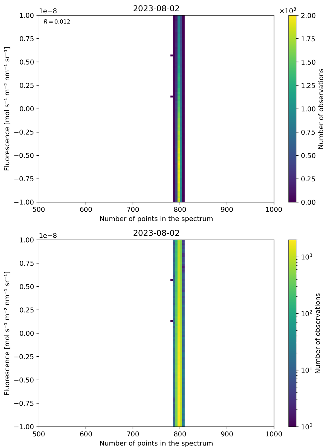
Figure 91: Scatter density plot of “Number of points in the spectrum” against “Fluorescence” for 2023-08-01 to 2023-08-03.
