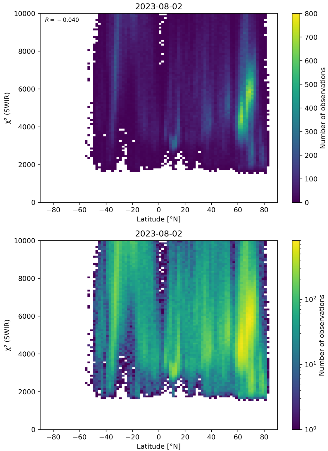
Figure 54: Scatter density plot of “Latitude” against “ \chi^2 (SWIR)” for 2023-08-01 to 2023-08-03.
