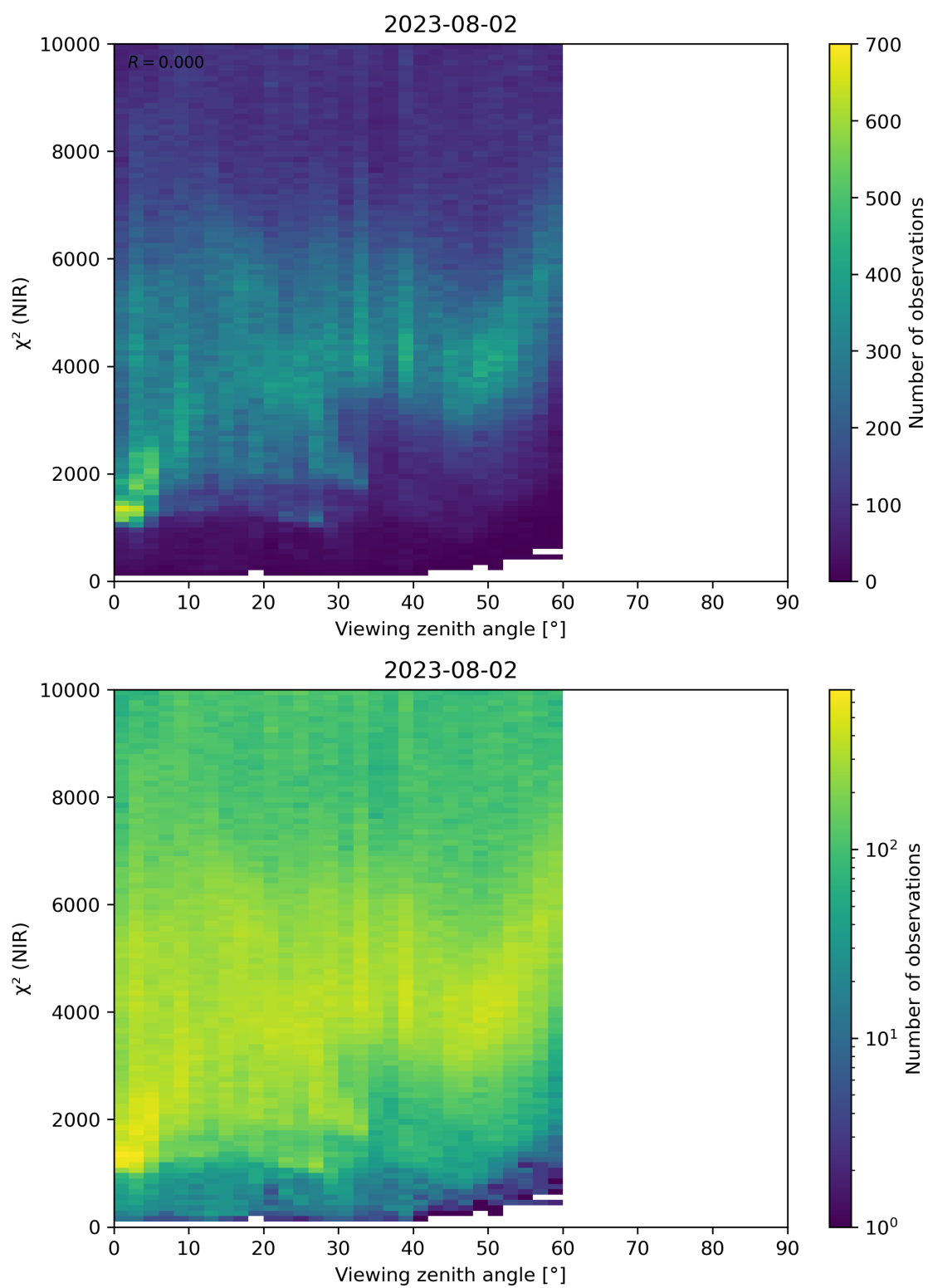
Figure 105: Scatter density plot of “Viewing zenith angle” against “ \chi^2 (NIR)” for 2023-08-01 to 2023-08-03.
