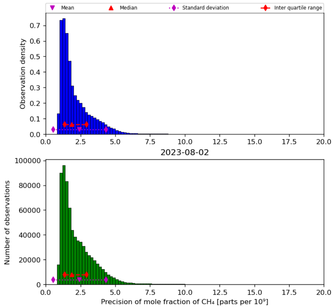
Figure 24: Histogram of “Precision of mole fraction of CH 4 ” for 2023-08-01 to 2023-08-03
