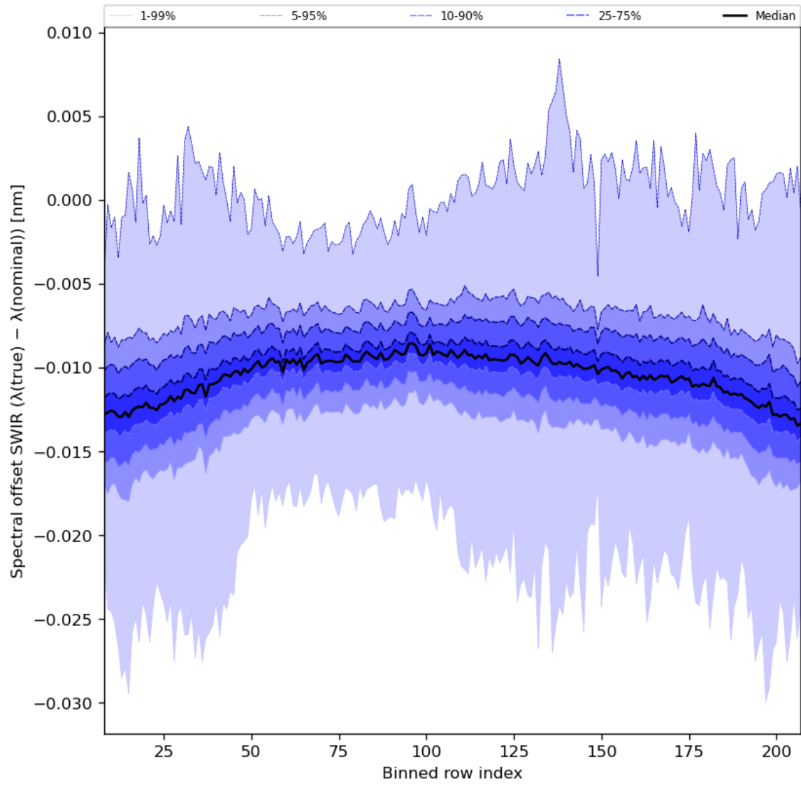
Figure 38: Along track statistics of “Spectral offset SWIR ( \lambda(\text{true}) - \lambda(\text{nominal}) )” for 2023-08-01 to 2023-08-03
