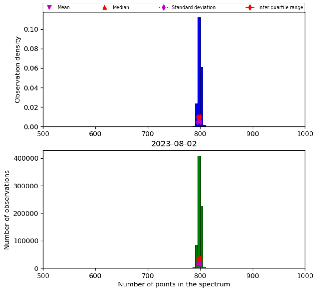
Figure 26: Histogram of “Number of points in the spectrum” for 2023-08-01 to 2023-08-03
