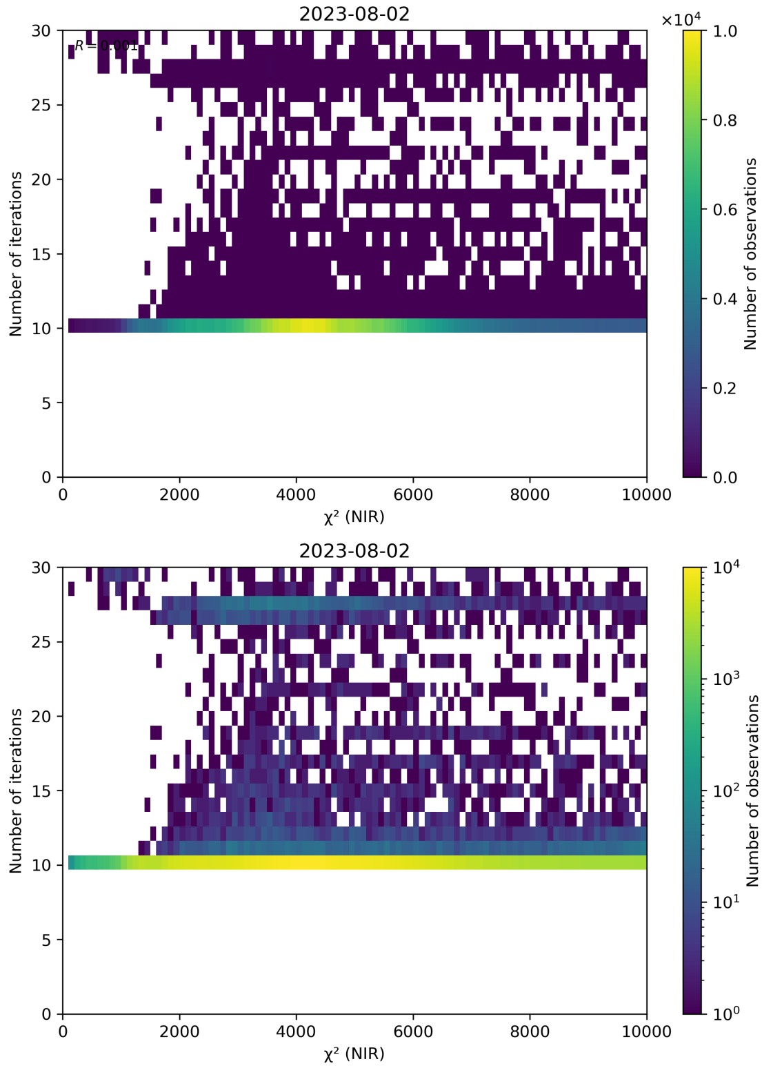
Figure 46: Scatter density plot of “ \chi^2 (NIR)” against “Number of iterations” for 2023-08-01 to 2023-08-03.
