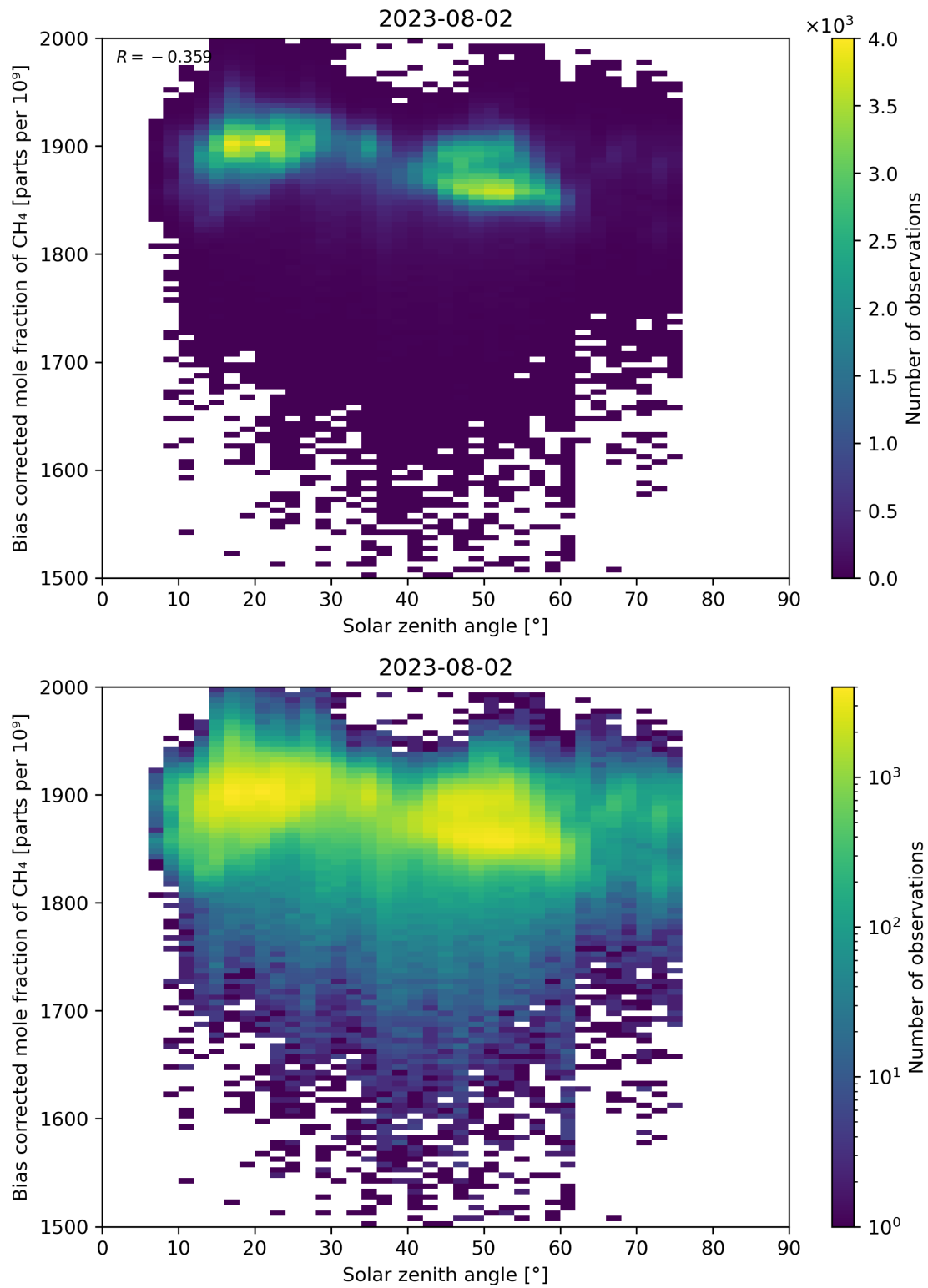
Figure 100: Scatter density plot of “Solar zenith angle” against “Bias corrected mole fraction of \text{CH}_4 ” for 2023-08-01 to 2023-08-03.
