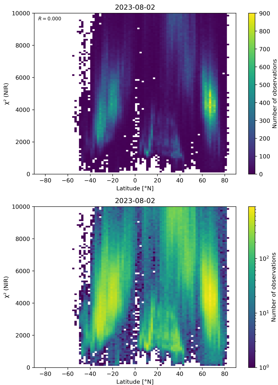
Figure 53: Scatter density plot of “Latitude” against “ \chi^2 (NIR)” for 2023-08-01 to 2023-08-03.
