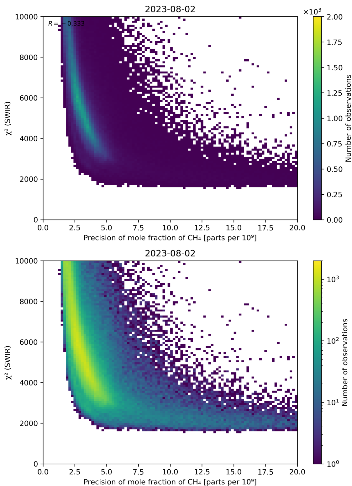
Figure 79: Scatter density plot of “Precision of mole fraction of CH 4 ” against “ \chi^2 (SWIR)” for 2023-08-01 to 2023-08-03.
