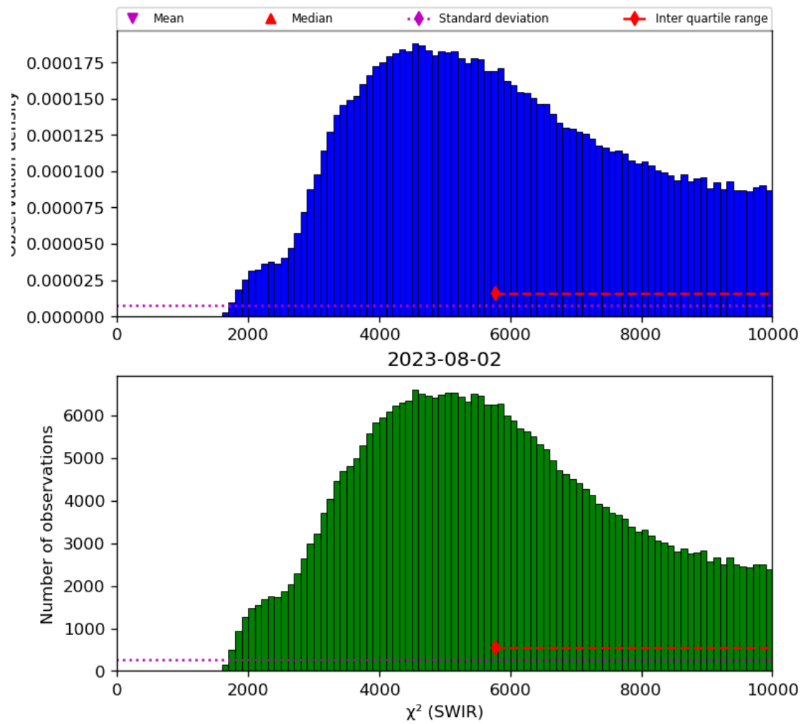
Figure 28: Histogram of “ \chi^2 (SWIR)” for 2023-08-01 to 2023-08-03
