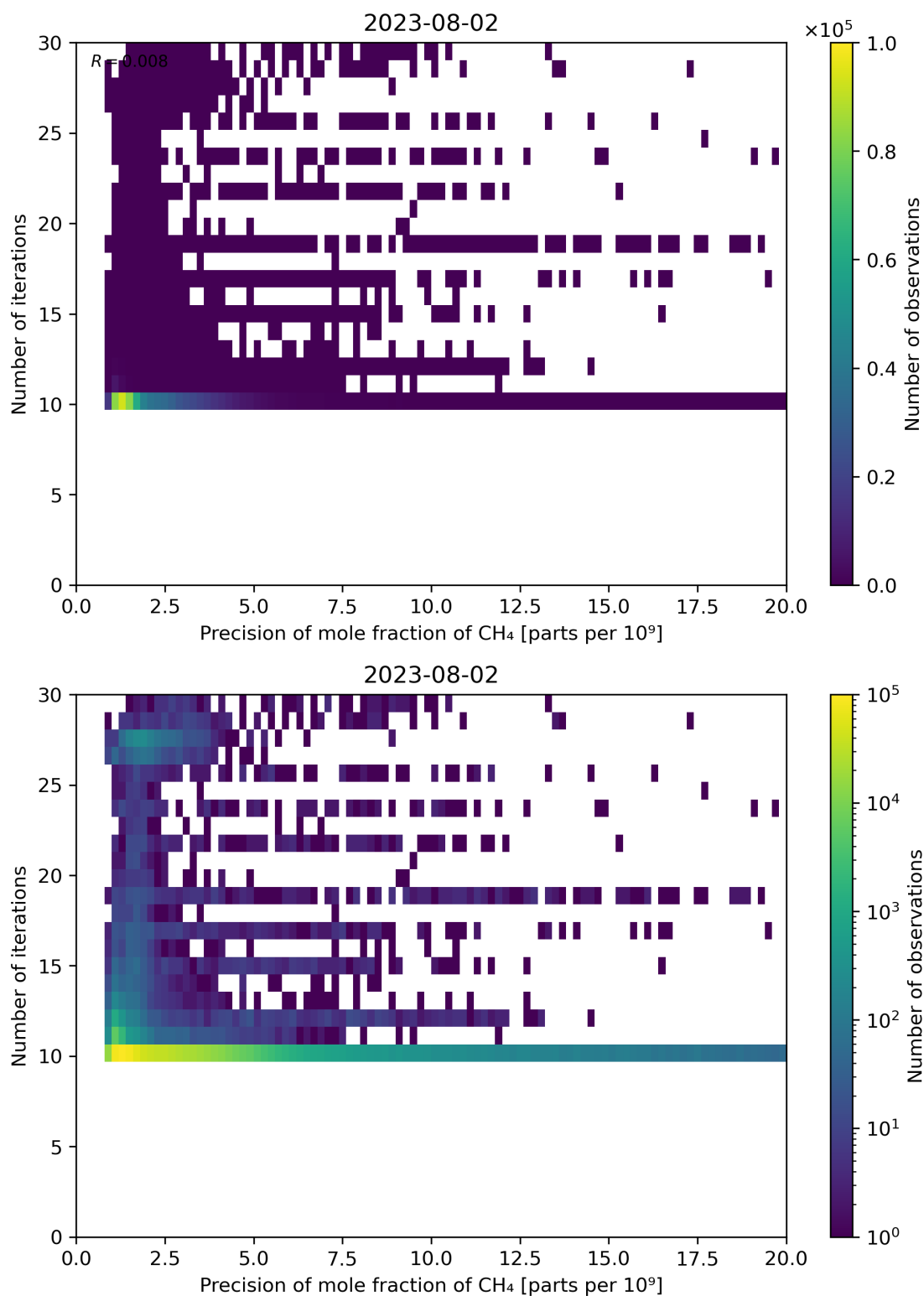
Figure 83: Scatter density plot of “Precision of mole fraction of CH 4 ” against “Number of iterations” for 2023-08-01 to 2023-08-03.
