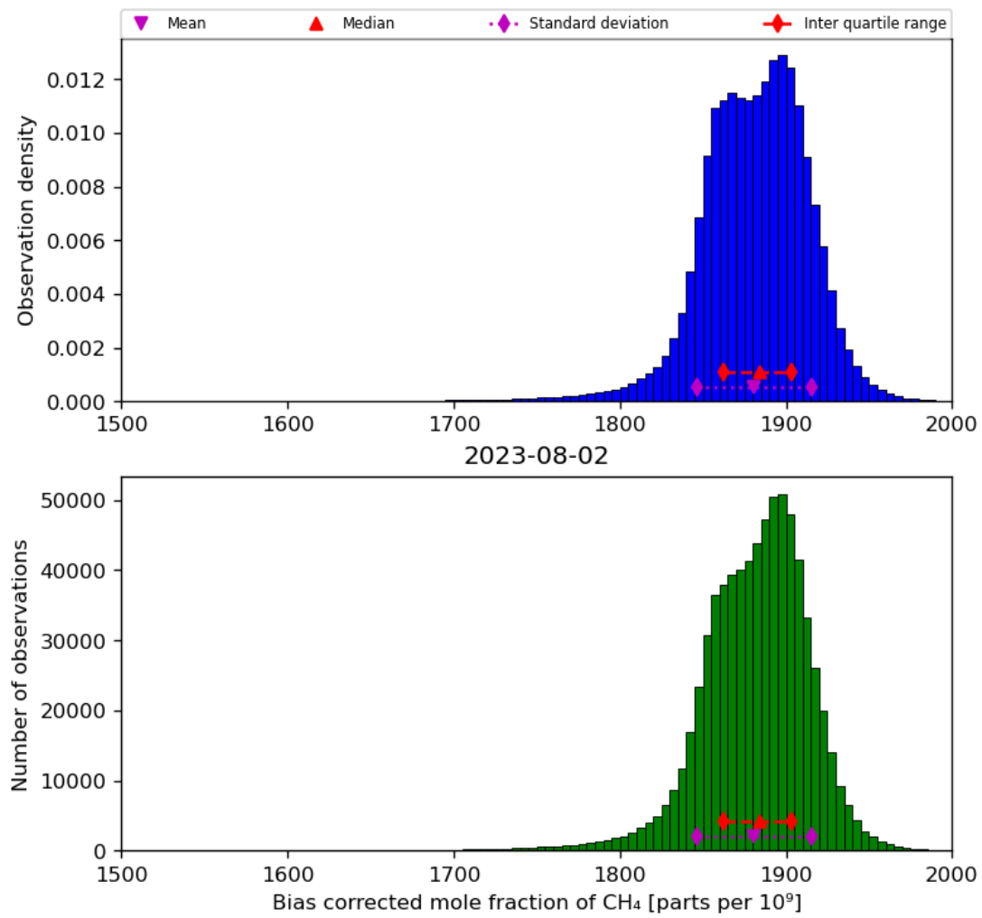
Figure 25: Histogram of “Bias corrected mole fraction of CH 4 ” for 2023-08-01 to 2023-08-03
