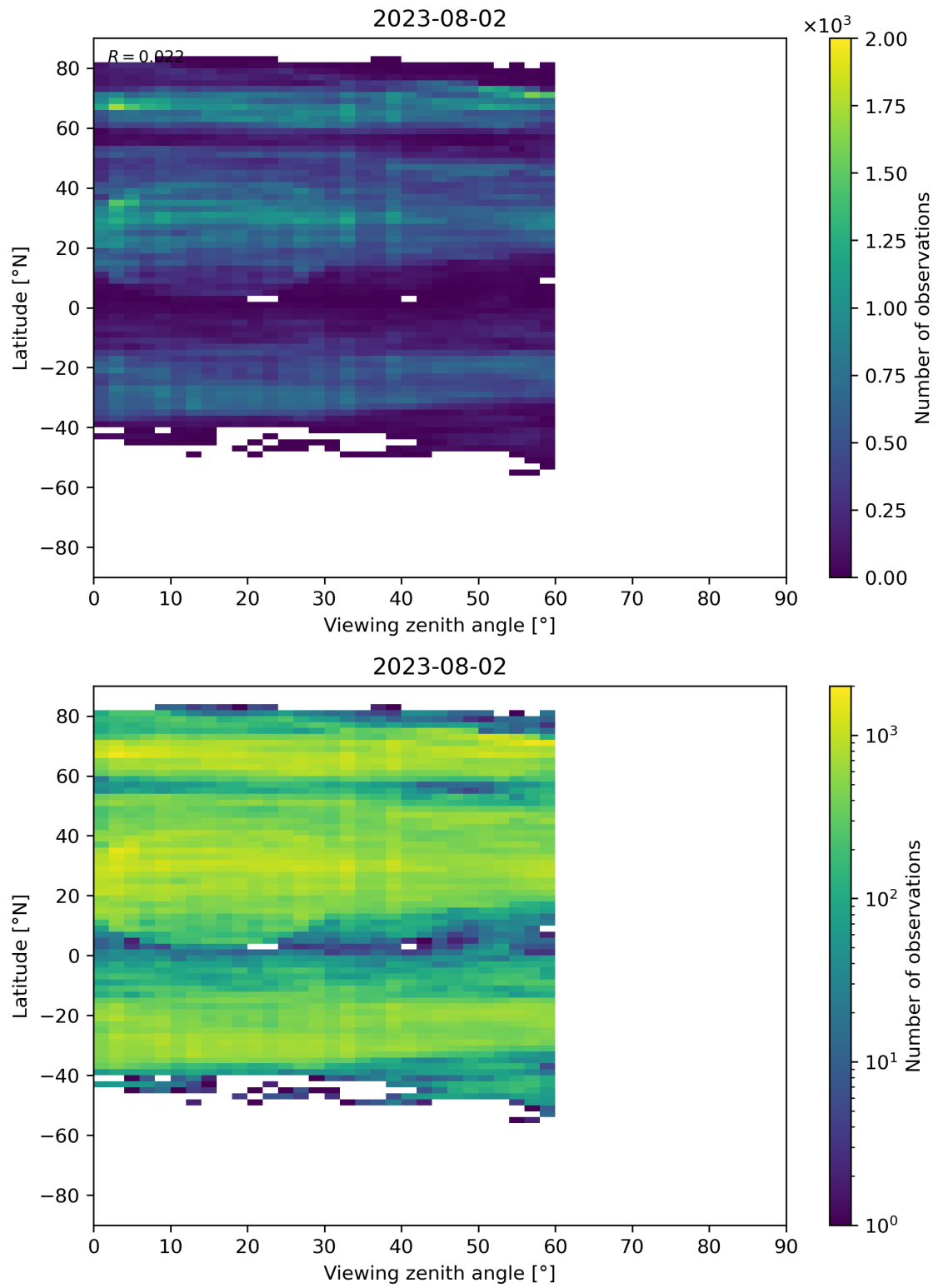
Figure 109: Scatter density plot of “Viewing zenith angle” against “Latitude” for 2023-08-01 to 2023-08-03.
