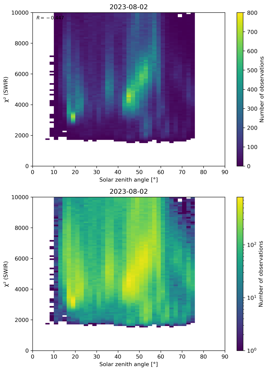
Figure 95: Scatter density plot of “Solar zenith angle” against “ \chi^2 (SWIR)” for 2023-08-01 to 2023-08-03.
