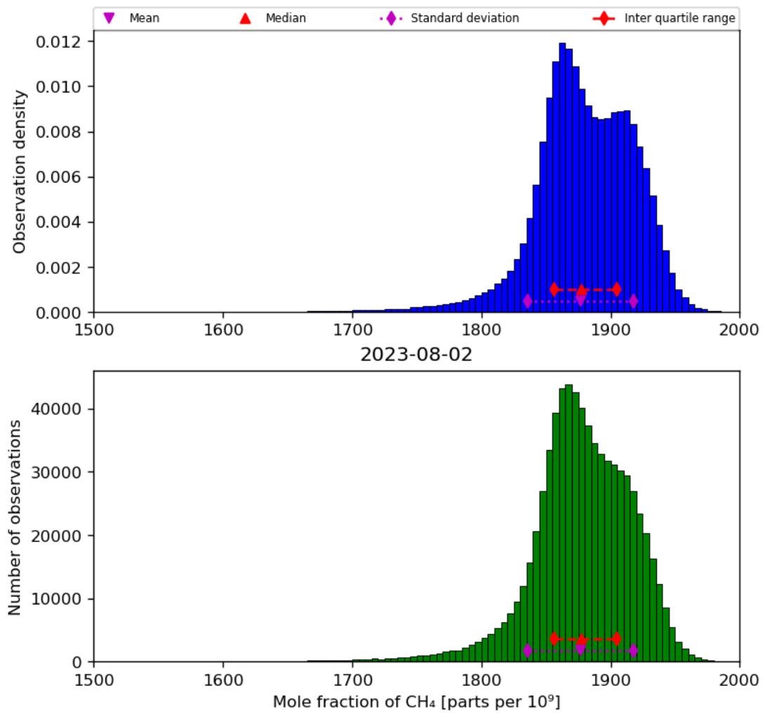
Figure 23: Histogram of “Mole fraction of CH 4 ” for 2023-08-01 to 2023-08-03
