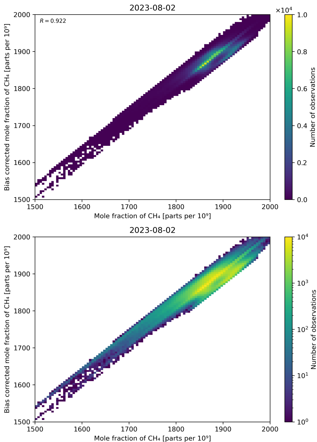
Figure 74: Scatter density plot of “Mole fraction of CH 4 ” against “Bias corrected mole fraction of CH 4 ” for 2023-08-01 to 2023-08-03.
