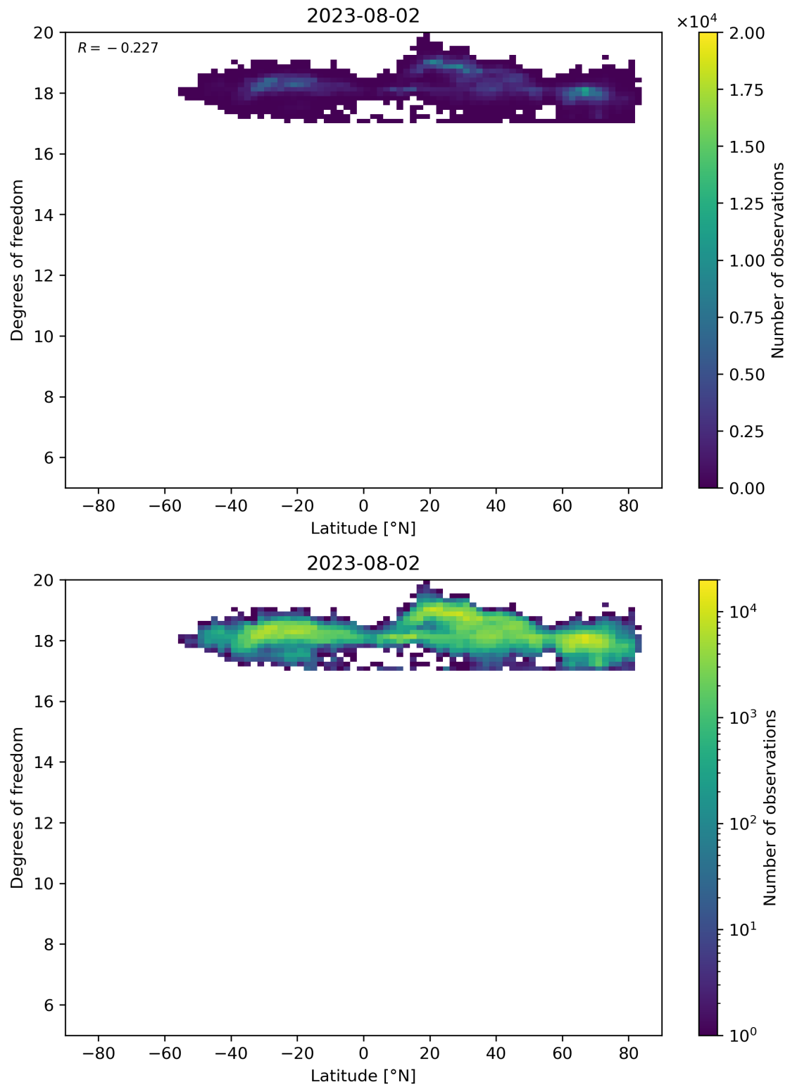
Figure 55: Scatter density plot of “Latitude” against “Degrees of freedom” for 2023-08-01 to 2023-08-03.
