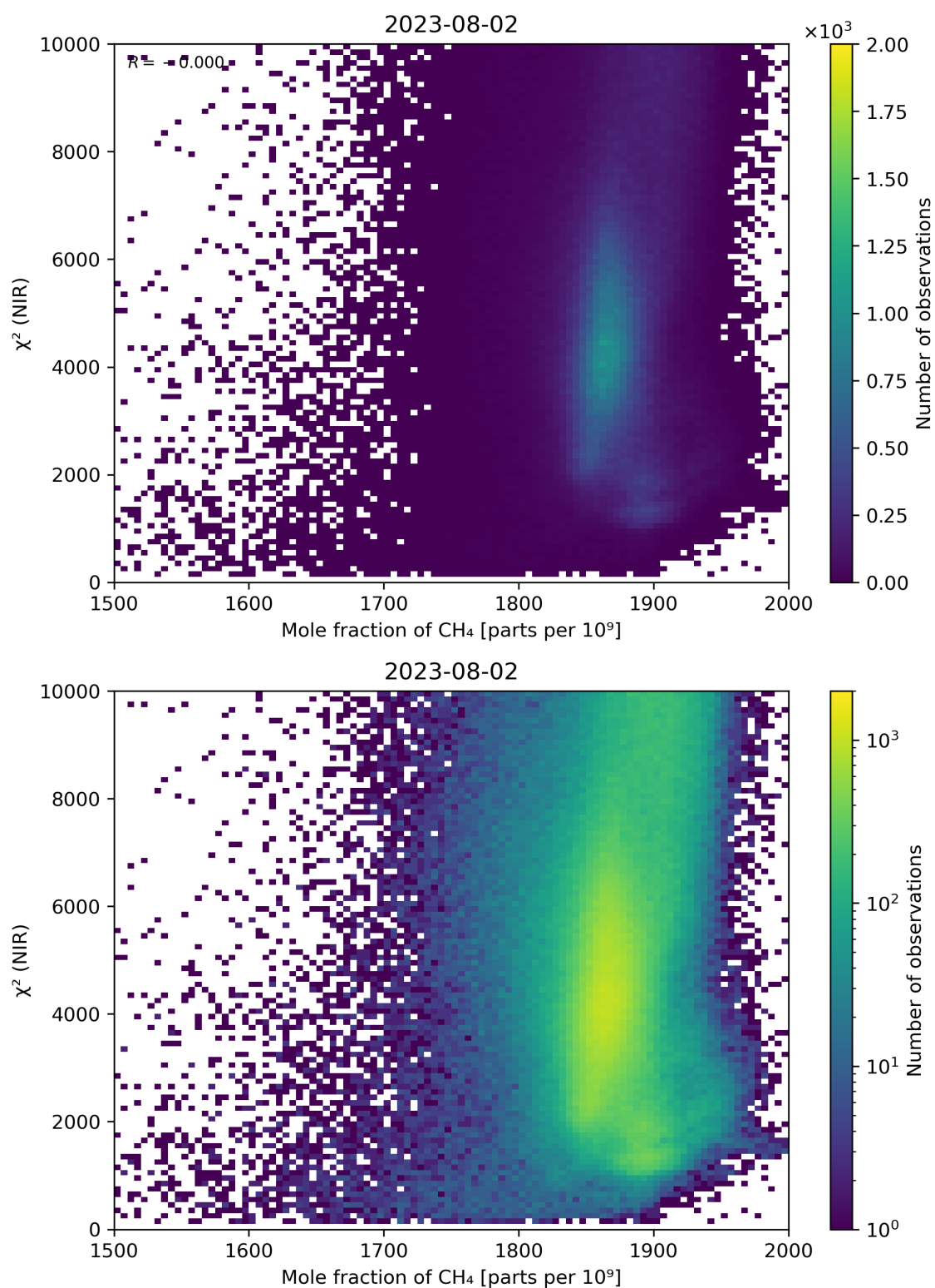
Figure 70: Scatter density plot of “Mole fraction of \text{CH}_4 ” against “ \chi^2 (NIR)” for 2023-08-01 to 2023-08-03.
