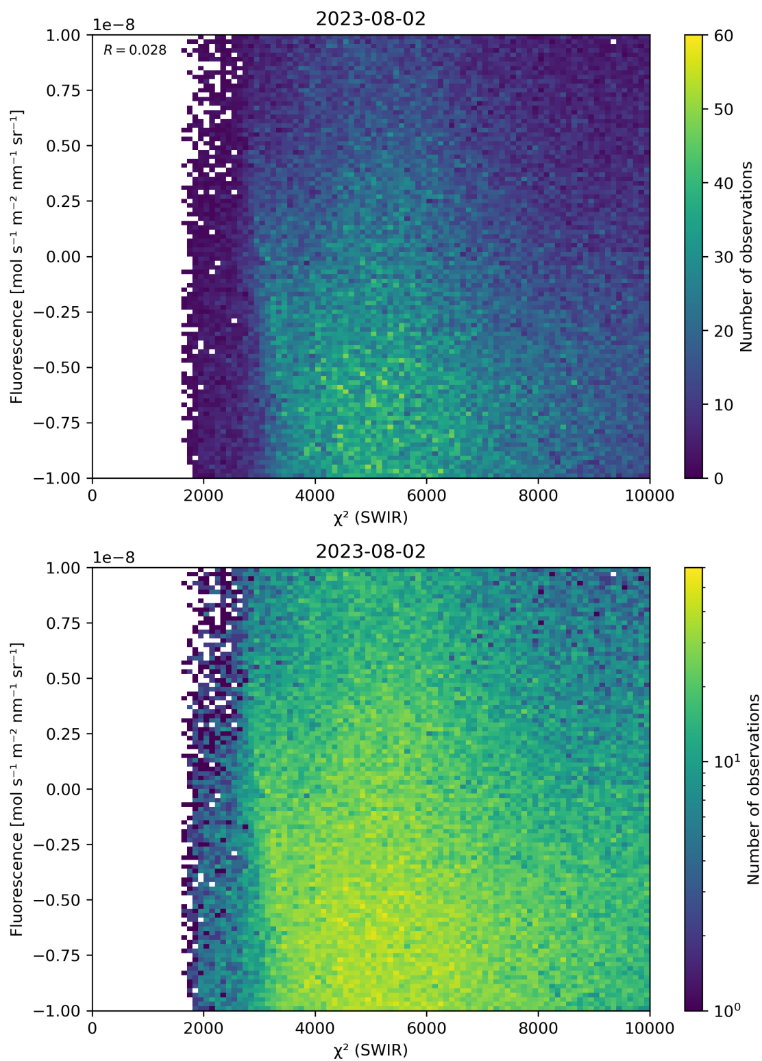
Figure 49: Scatter density plot of “ \chi^2 (SWIR)” against “Fluorescence” for 2023-08-01 to 2023-08-03.
