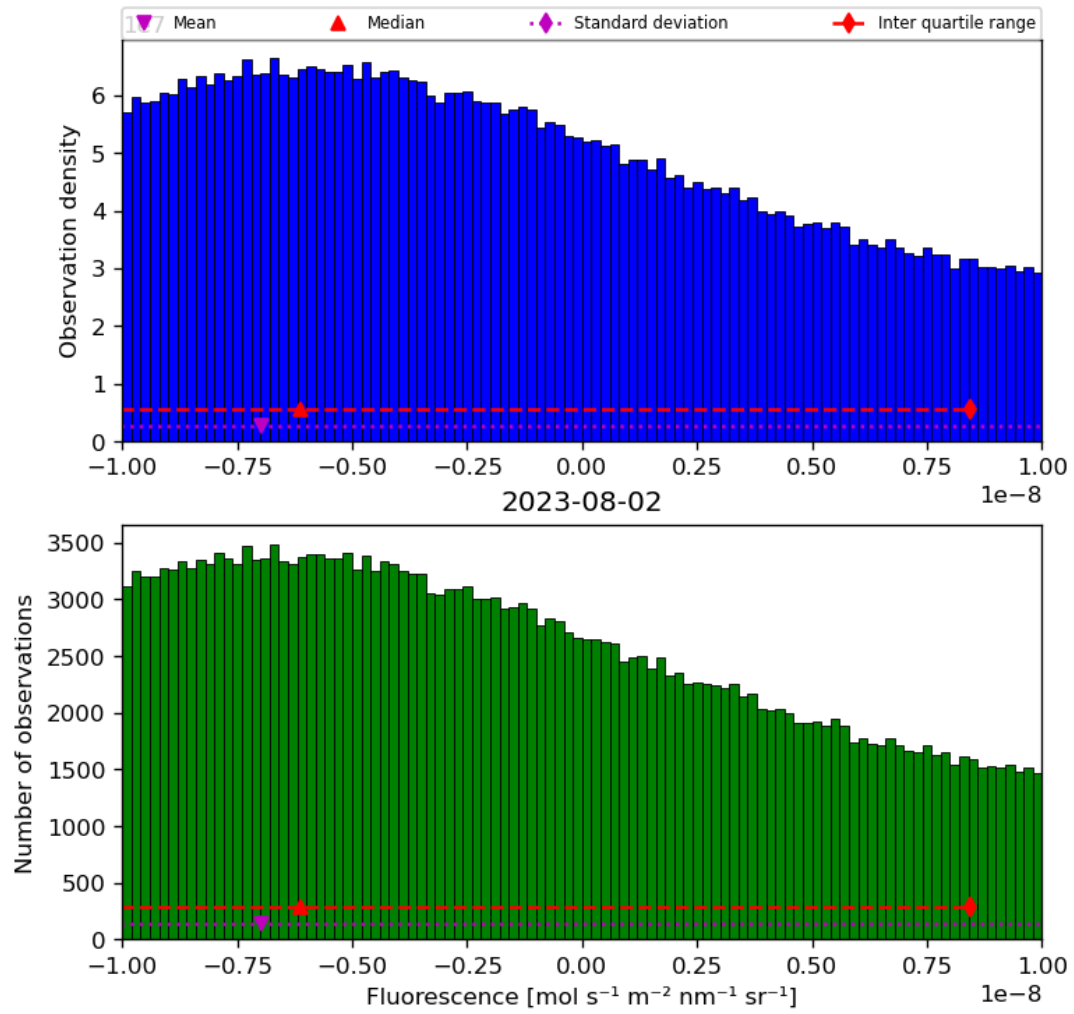
Figure 32: Histogram of “Fluorescence” for 2023-08-01 to 2023-08-03
