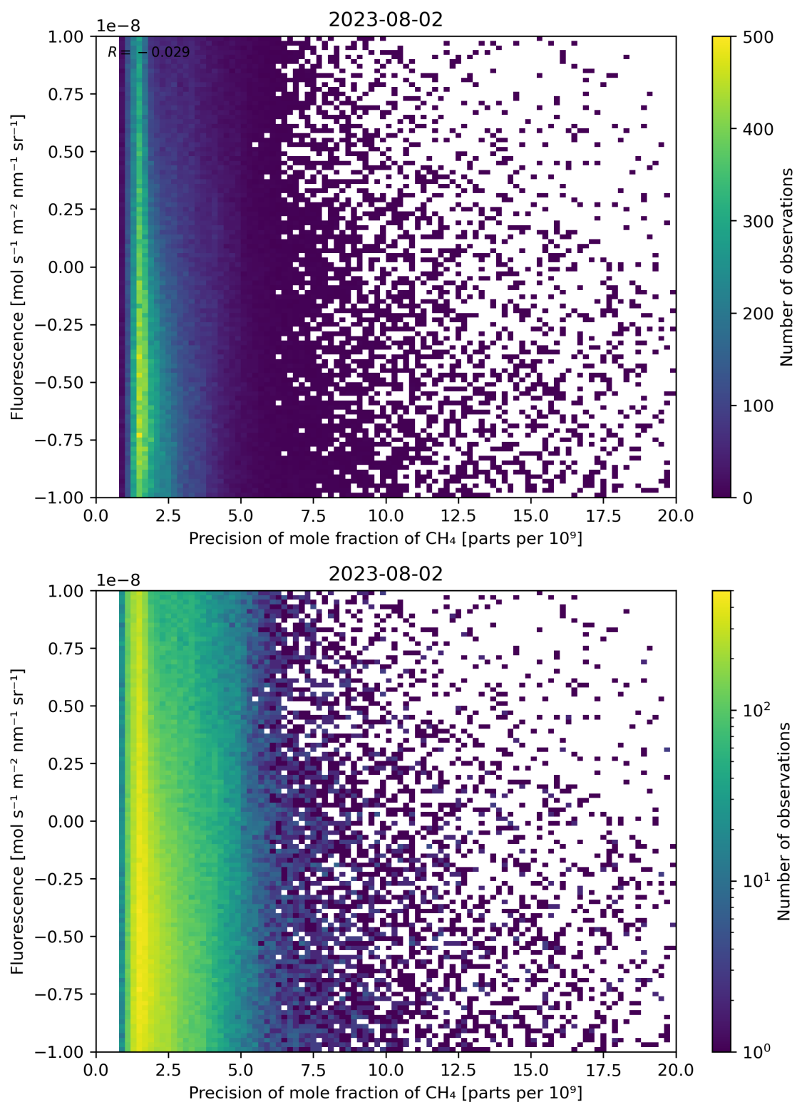
Figure 81: Scatter density plot of “Precision of mole fraction of \text{CH}_4 ” against “Fluorescence” for 2023-08-01 to 2023-08-03.
