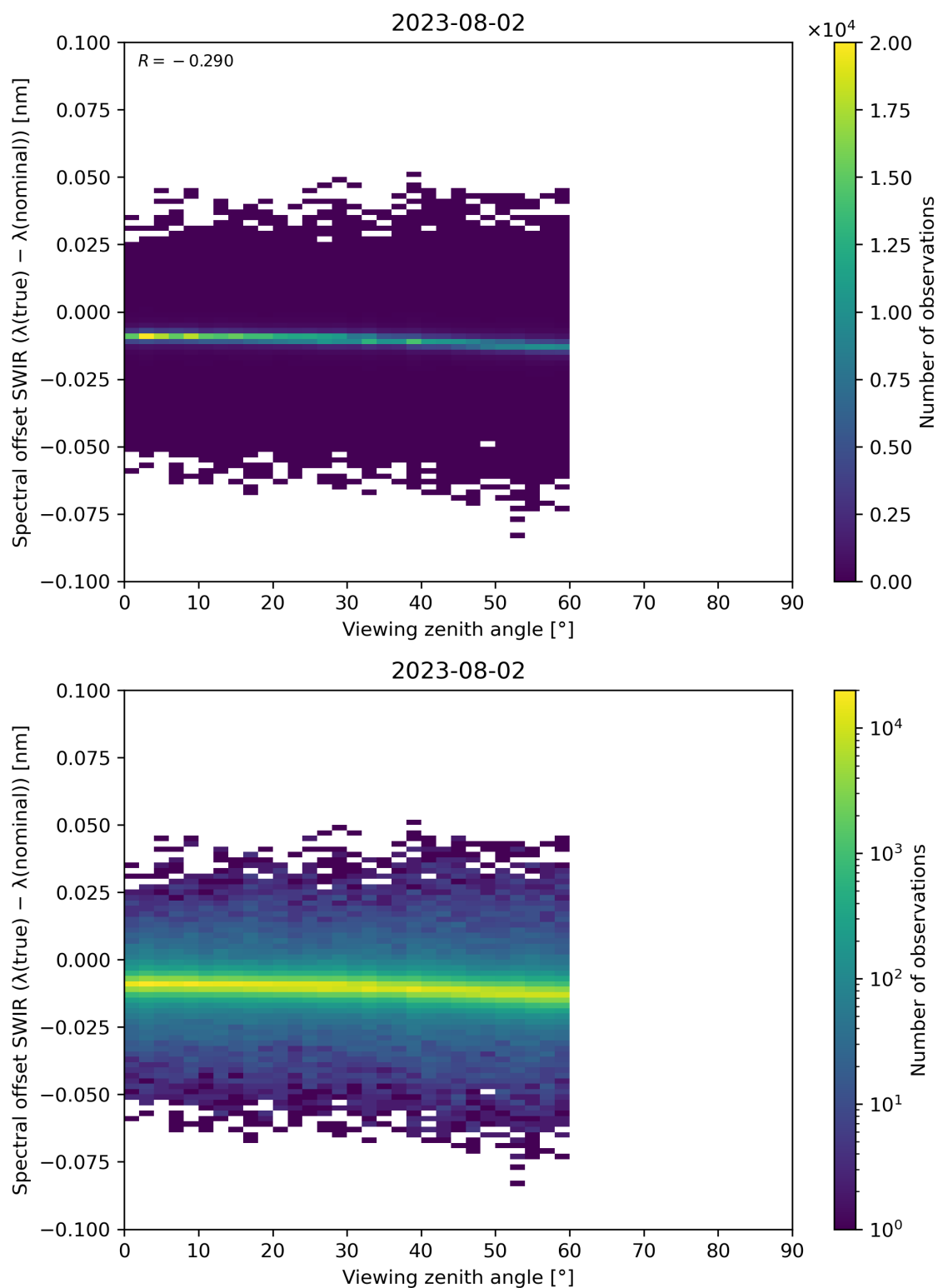
Figure 116: Scatter density plot of “Viewing zenith angle” against “Spectral offset SWIR ( \lambda(\text{true}) - \lambda(\text{nominal}) )” for 2023-08-01 to 2023-08-03.
