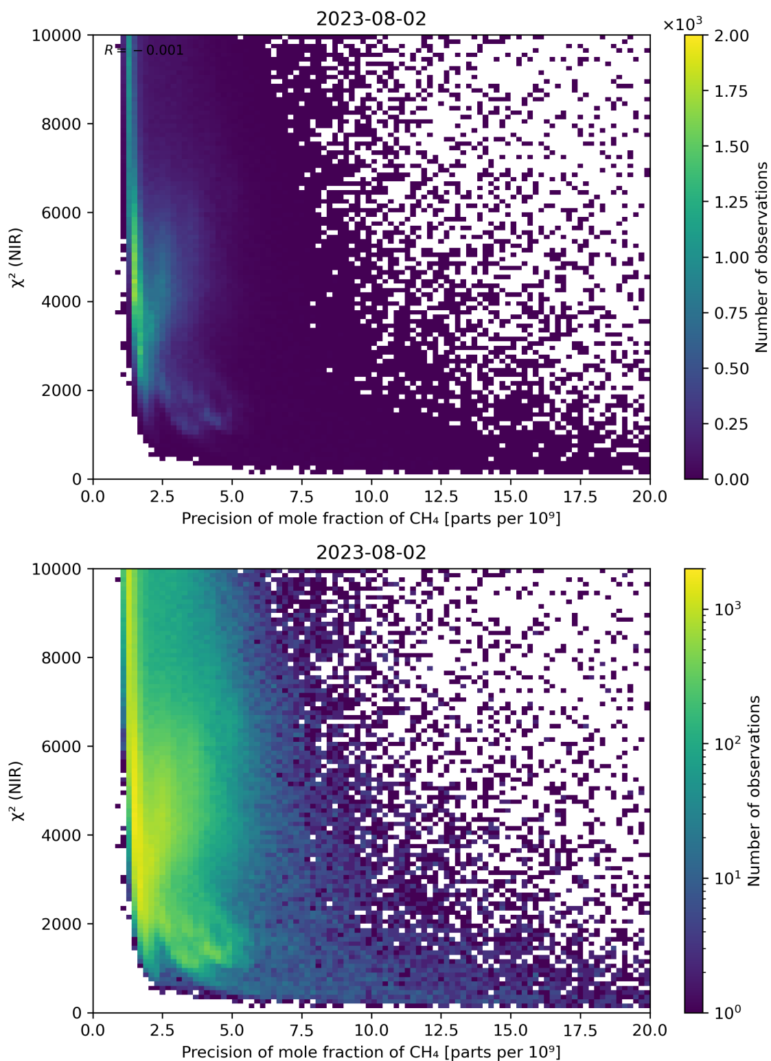
Figure 78: Scatter density plot of “Precision of mole fraction of \text{CH}_4 ” against “ \chi^2 (NIR)” for 2023-08-01 to 2023-08-03.
