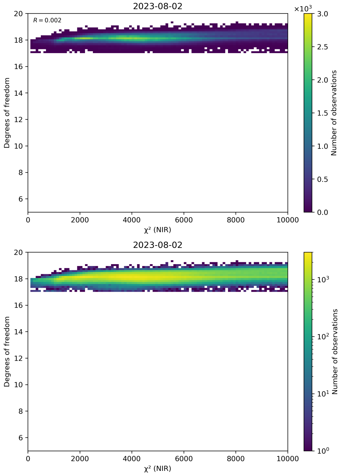
Figure 44: Scatter density plot of “ \chi^2 (NIR)” against “Degrees of freedom” for 2023-08-01 to 2023-08-03.
