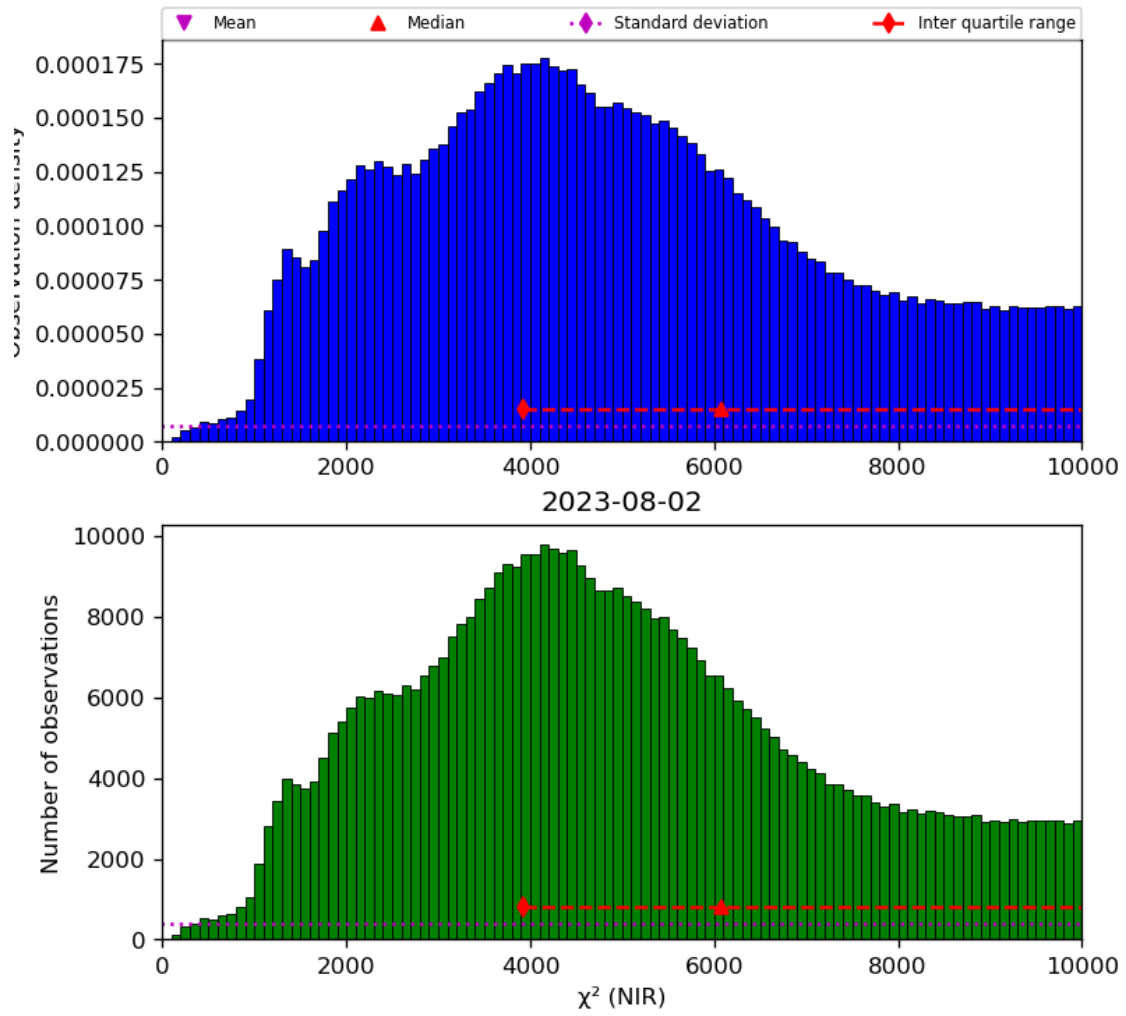
Figure 29: Histogram of “ \chi^2 (NIR)” for 2023-08-01 to 2023-08-03
