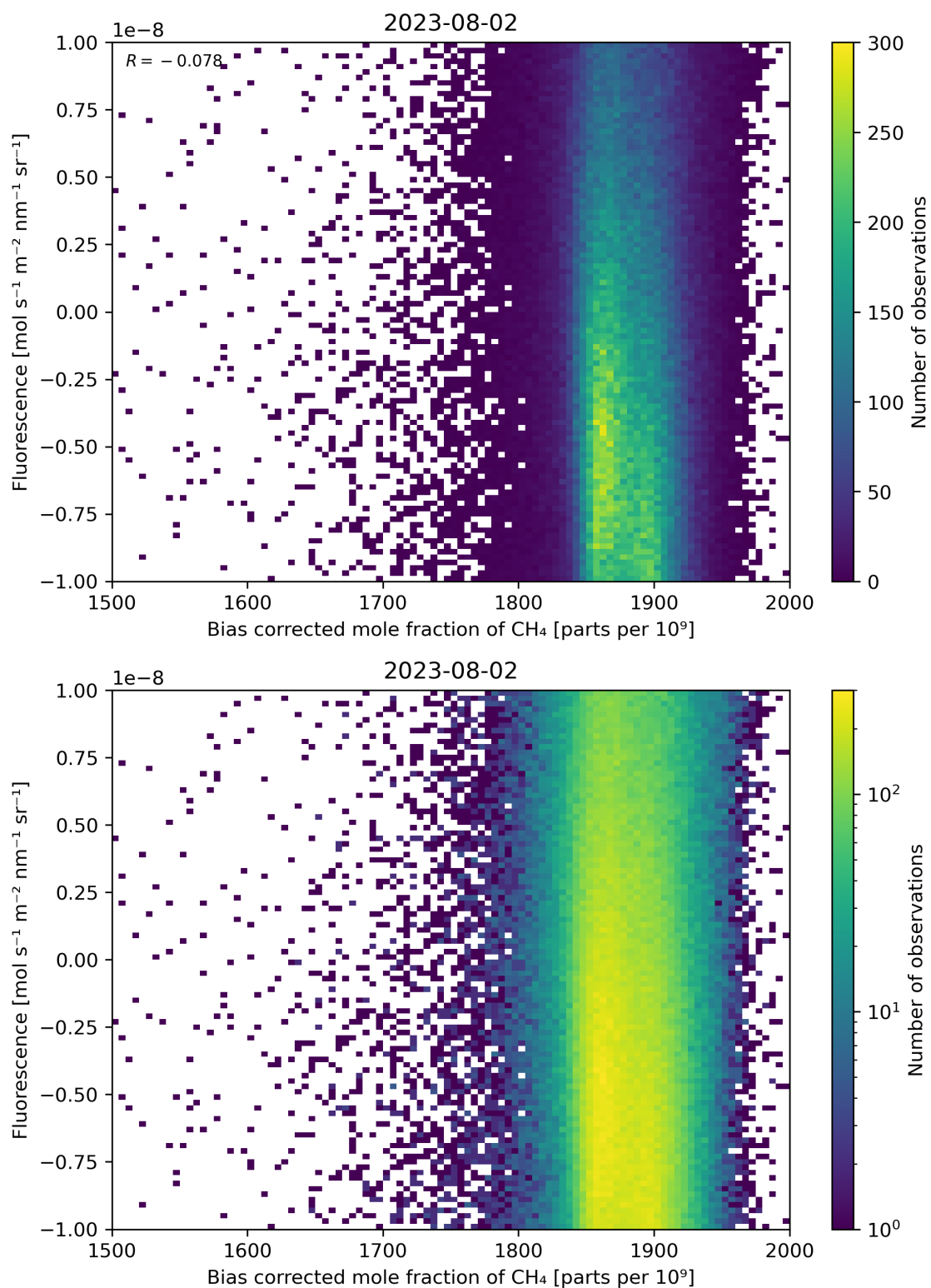
Figure 66: Scatter density plot of “Bias corrected mole fraction of \text{CH}_4 ” against “Fluorescence” for 2023-08-01 to 2023-08-03.
