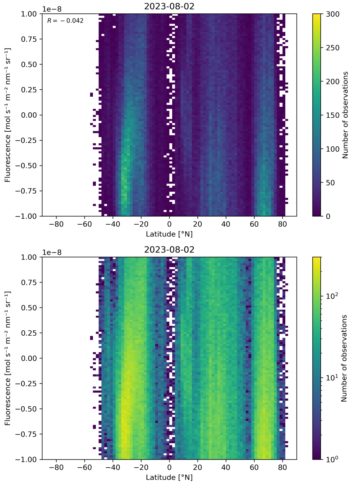
Figure 56: Scatter density plot of “Latitude” against “Fluorescence” for 2023-08-01 to 2023-08-03.
