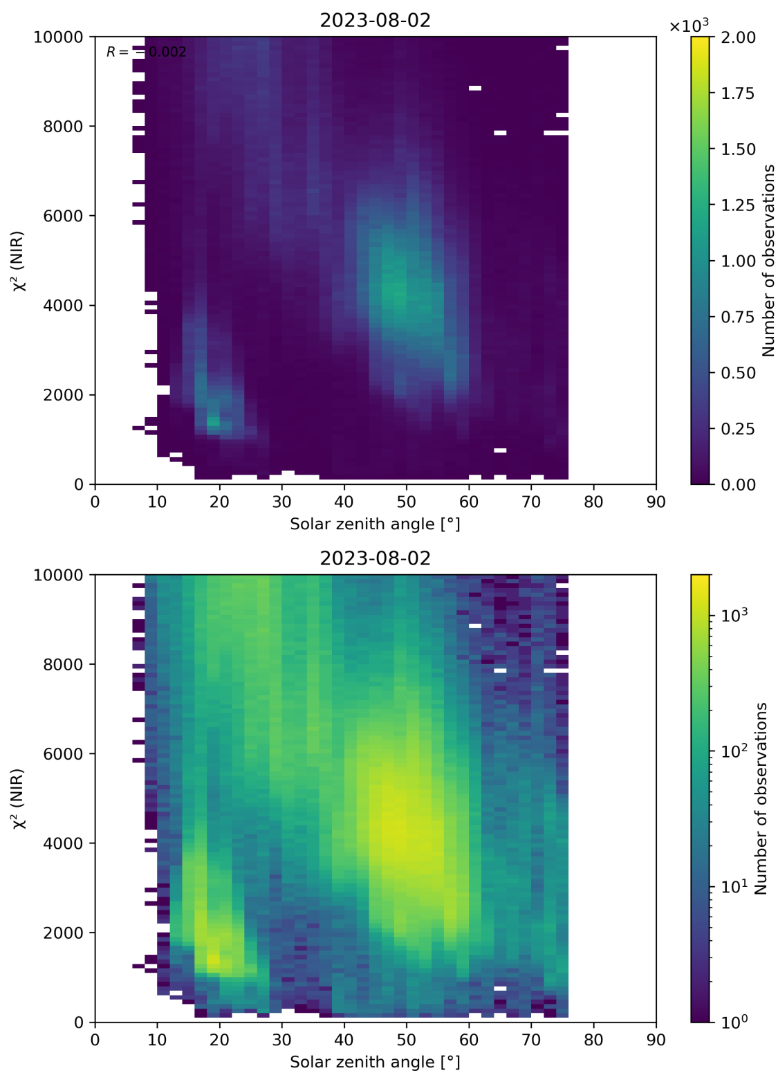
Figure 94: Scatter density plot of “Solar zenith angle” against “ \chi^2 (NIR)” for 2023-08-01 to 2023-08-03.
