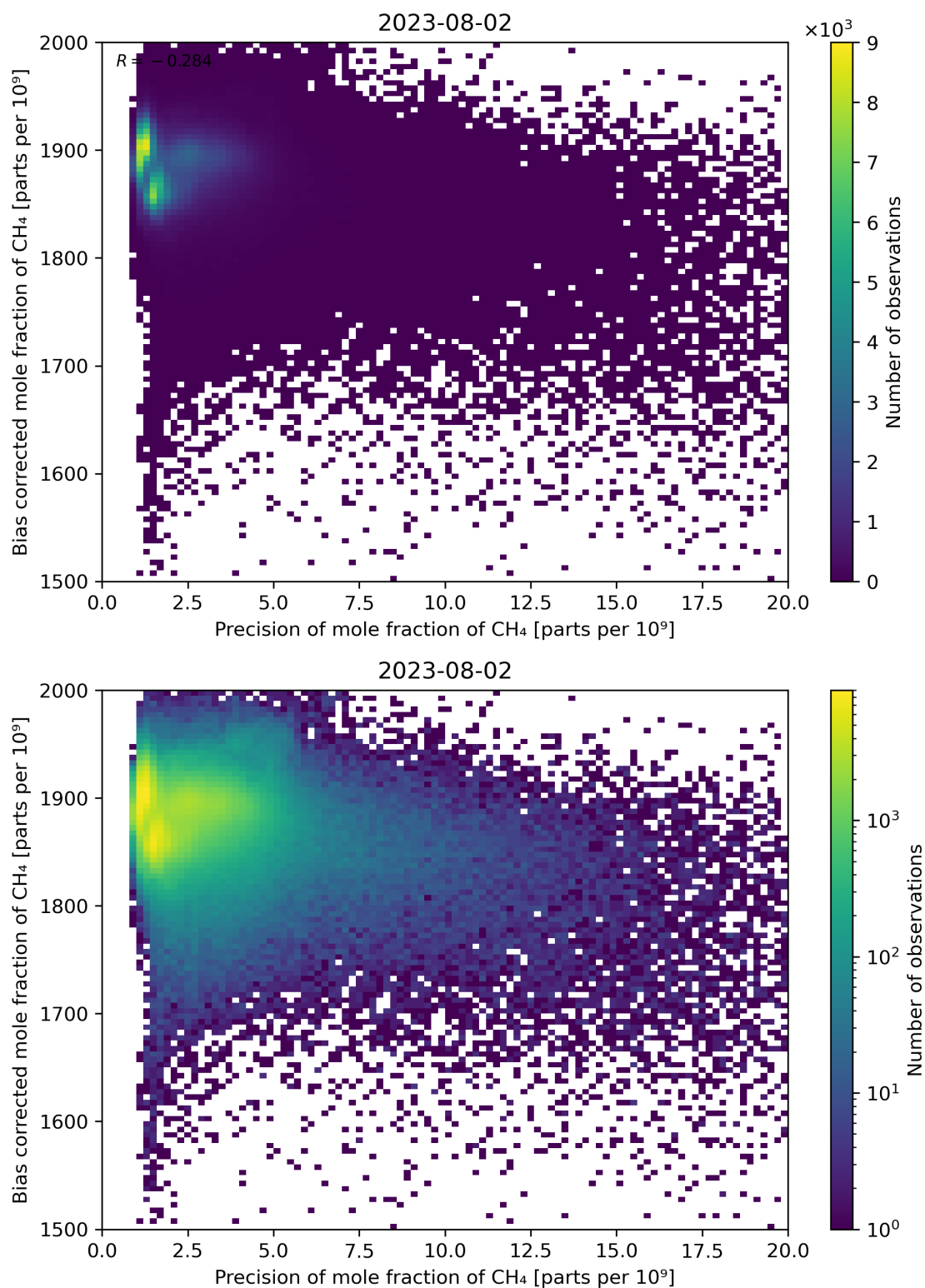
Figure 82: Scatter density plot of “Precision of mole fraction of CH 4 ” against “Bias corrected mole fraction of CH 4 ” for 2023-08-01 to 2023-08-03.
