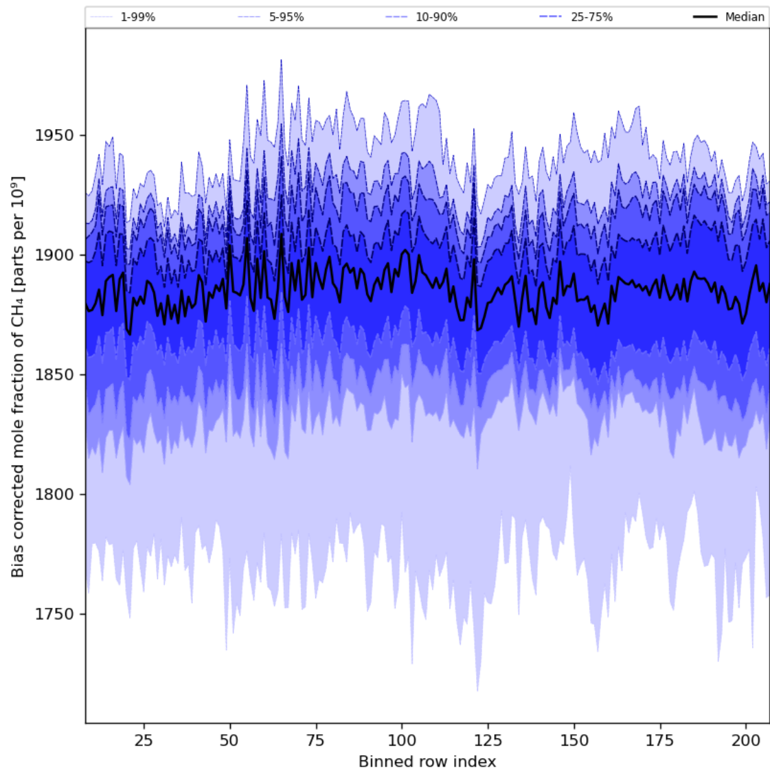
Figure 36: Along track statistics of “Bias corrected mole fraction of \text{CH}_4 ” for 2023-08-01 to 2023-08-03
