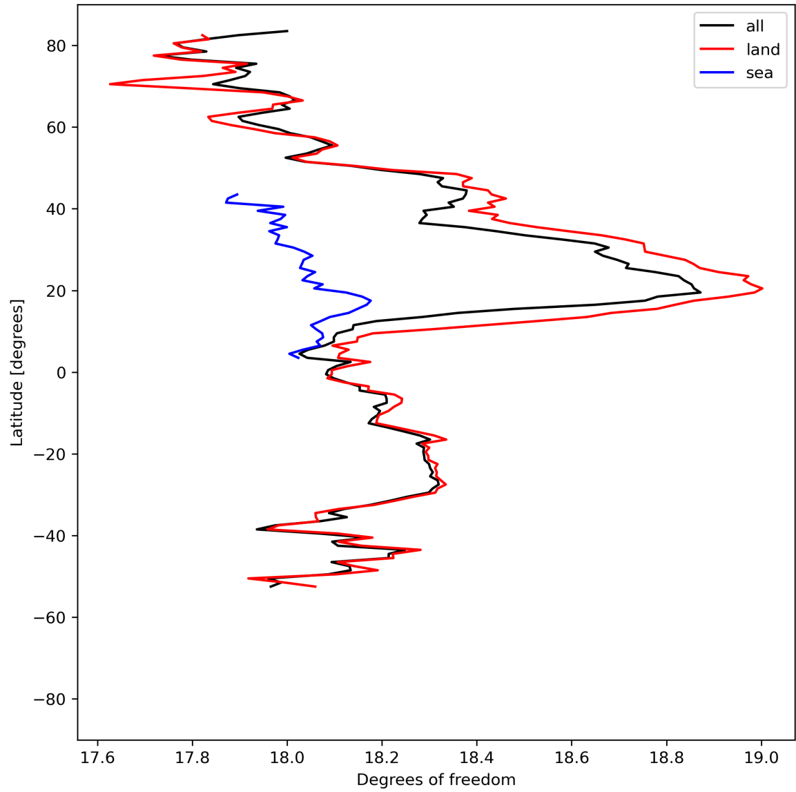
Figure 19: Zonal average of “Degrees of freedom” for 2023-08-01 to 2023-08-03.
