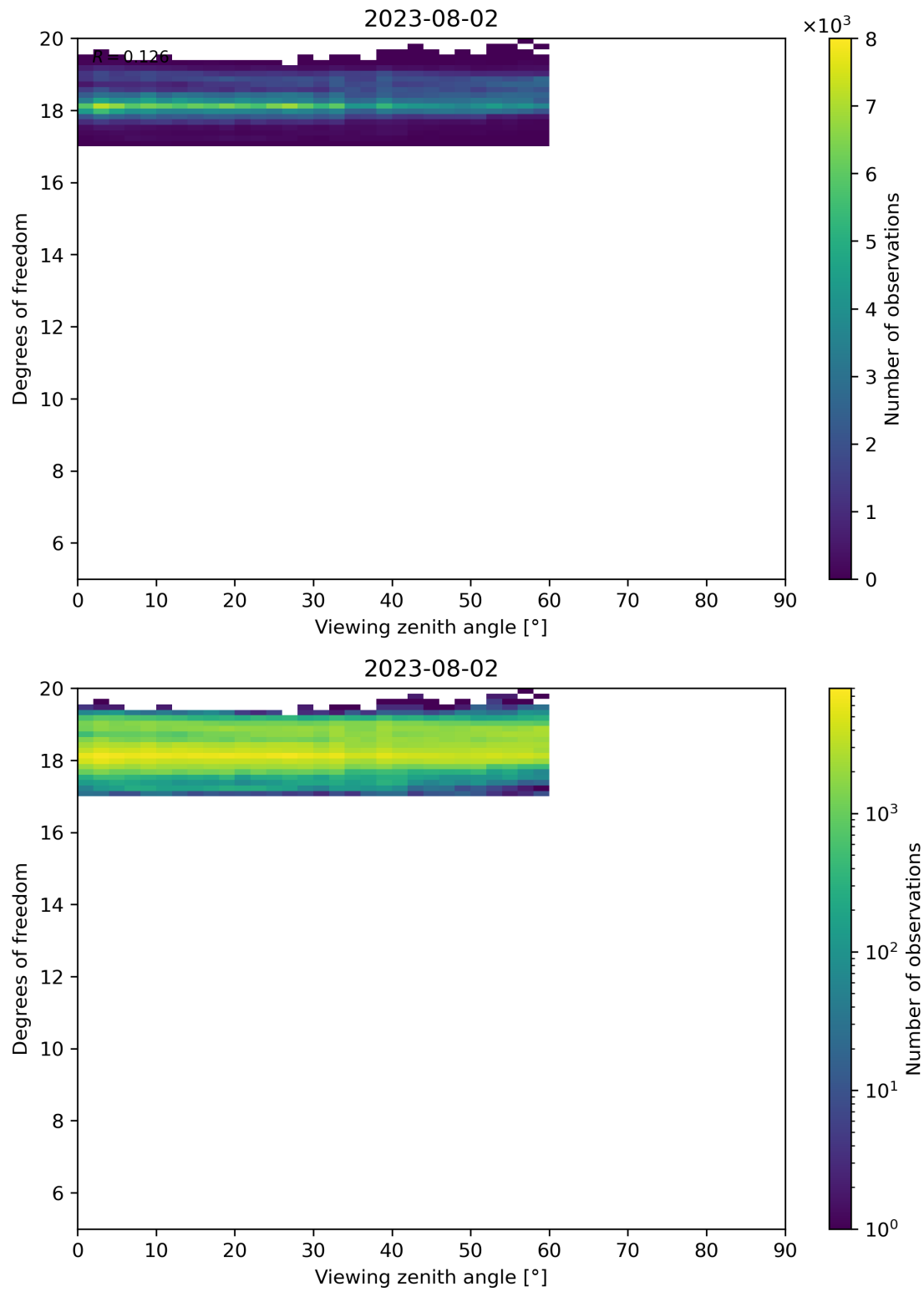
Figure 107: Scatter density plot of “Viewing zenith angle” against “Degrees of freedom” for 2023-08-01 to 2023-08-03.
