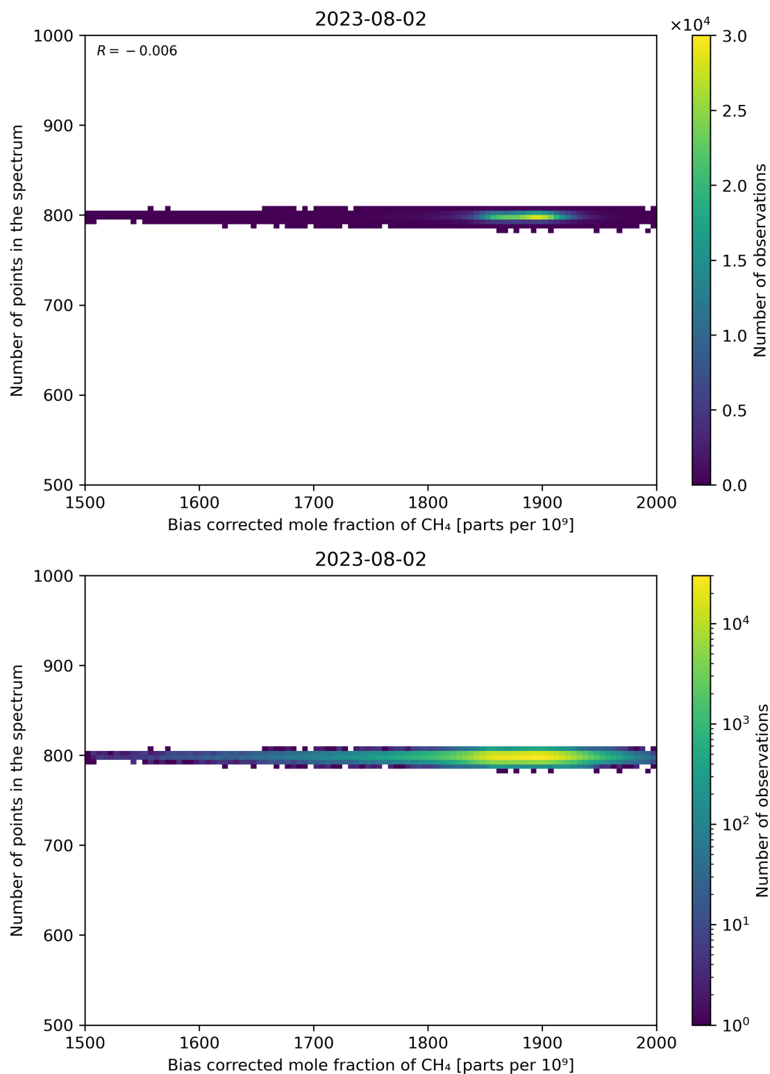
Figure 68: Scatter density plot of “Bias corrected mole fraction of CH 4 ” against “Number of points in the spectrum” for 2023-08-01 to 2023-08-03.
