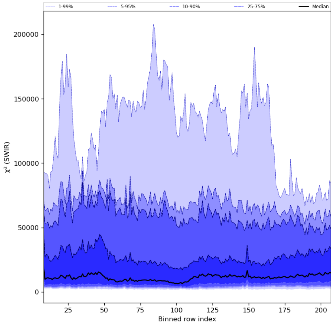
Figure 39: Along track statistics of “ \chi^2 (SWIR)” for 2023-08-01 to 2023-08-03
