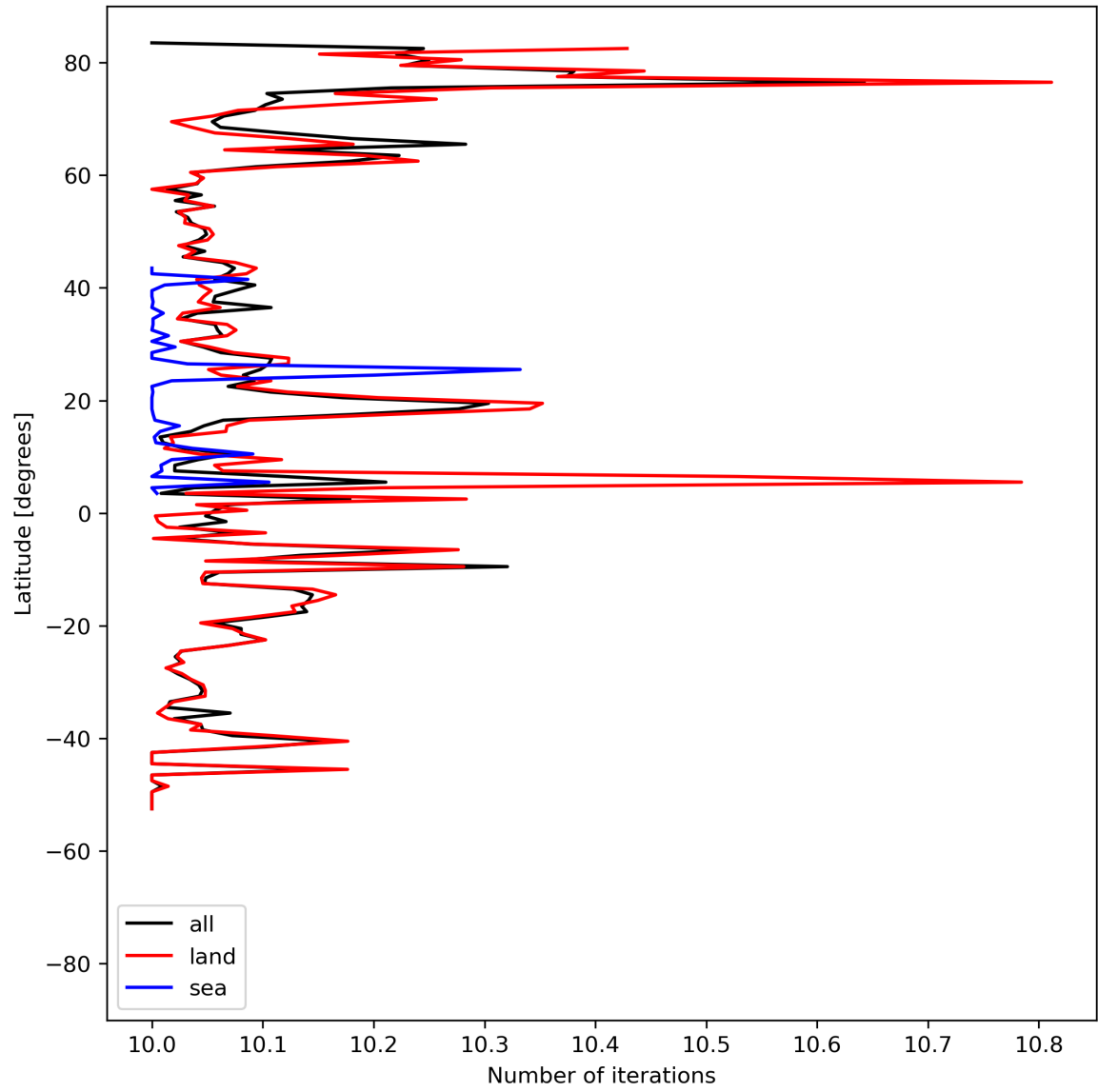
Figure 20: Zonal average of “Number of iterations” for 2023-08-01 to 2023-08-03.
