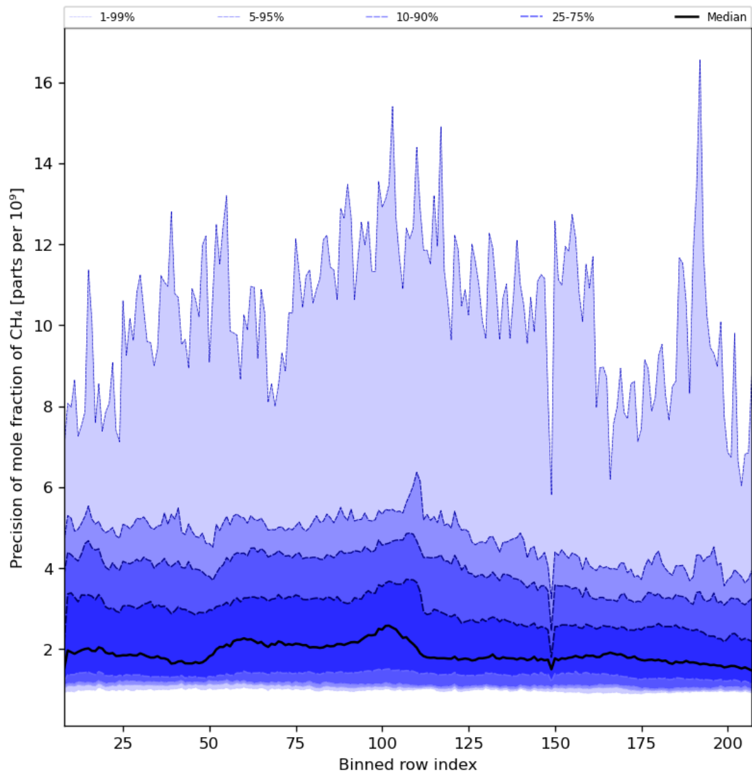
Figure 35: Along track statistics of “Precision of mole fraction of CH 4 ” for 2023-08-01 to 2023-08-03
