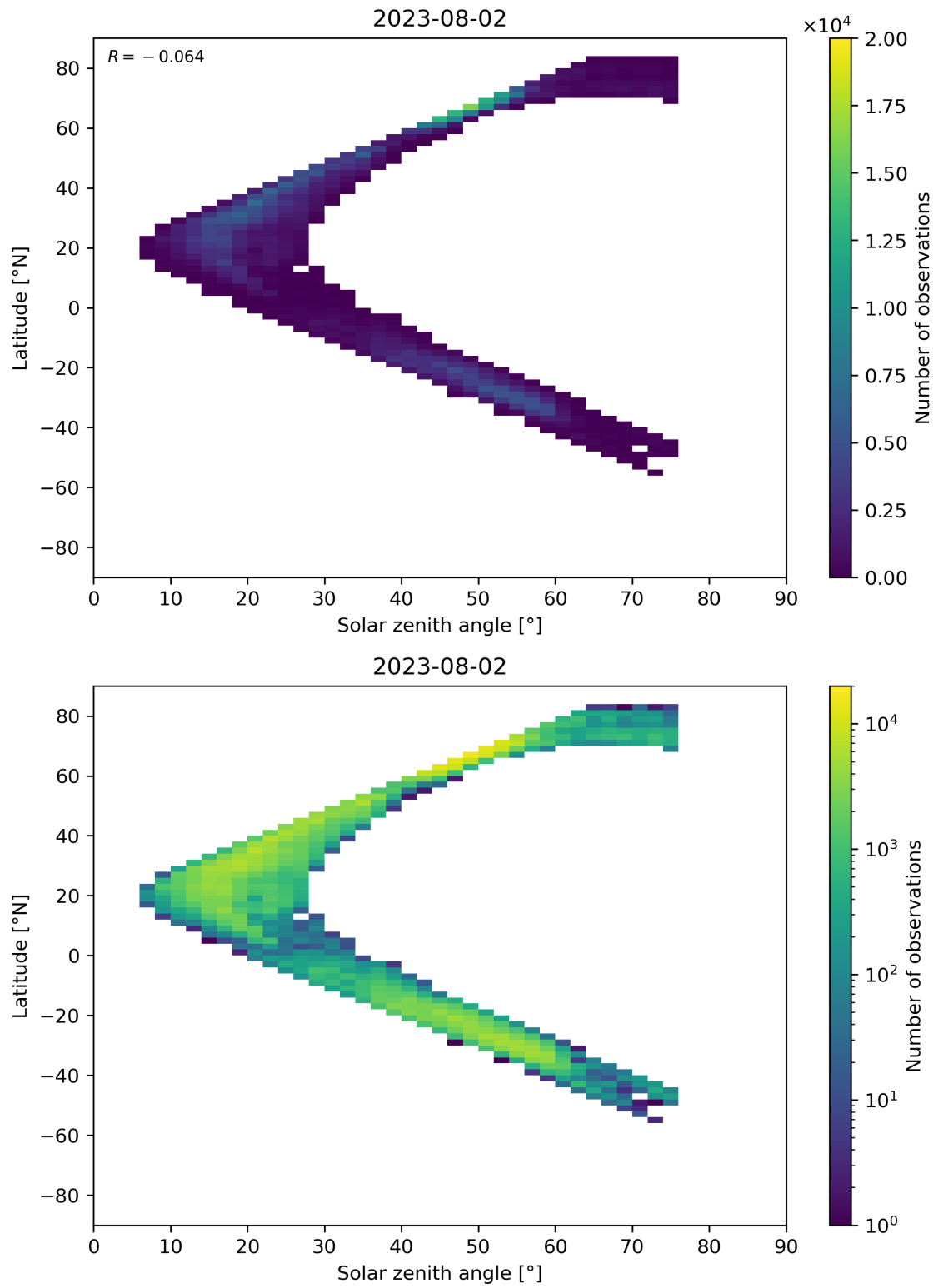
Figure 98: Scatter density plot of “Solar zenith angle” against “Latitude” for 2023-08-01 to 2023-08-03.
