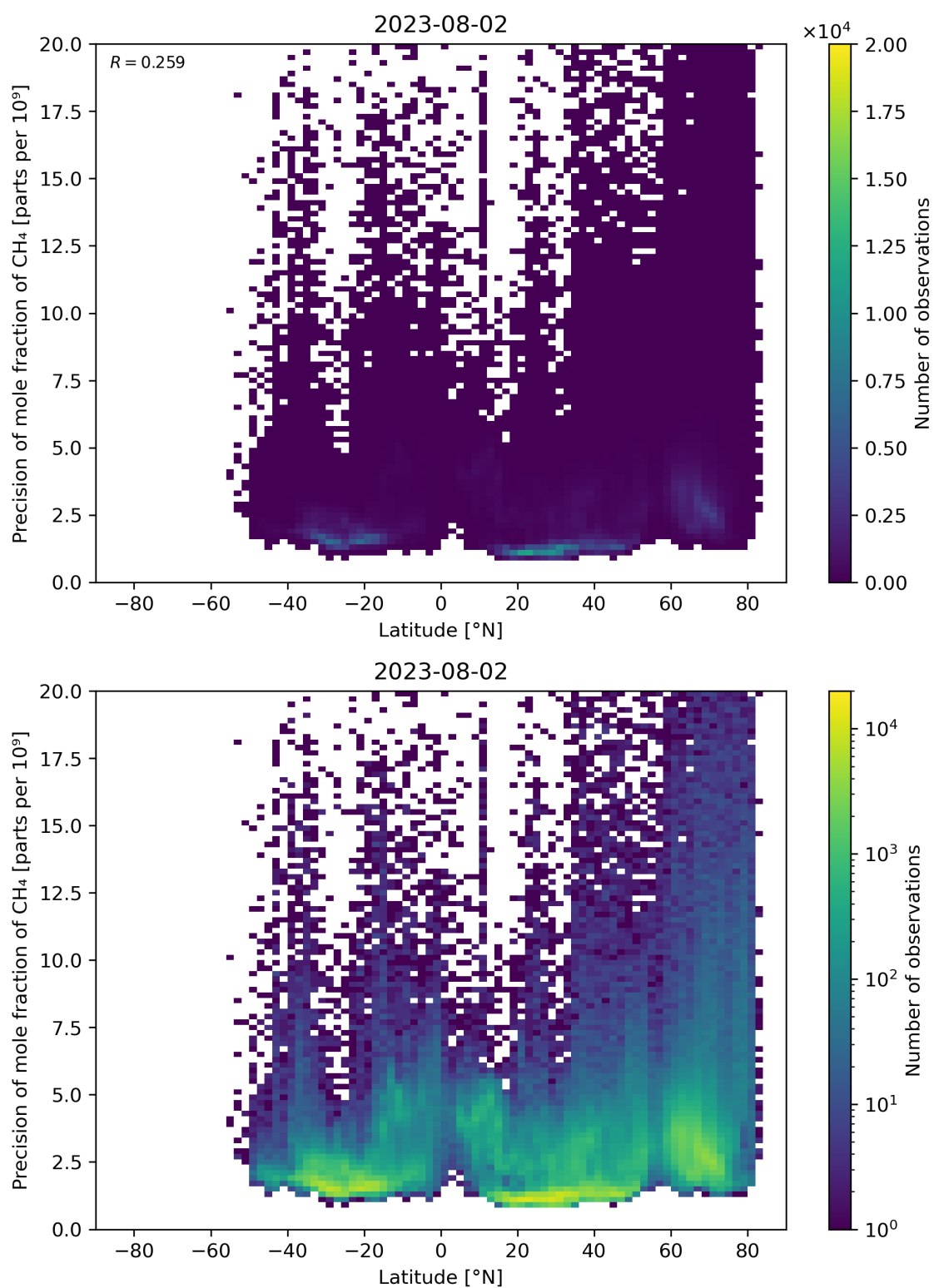
Figure 59: Scatter density plot of “Latitude” against “Precision of mole fraction of CH 4 ” for 2023-08-01 to 2023-08-03.
