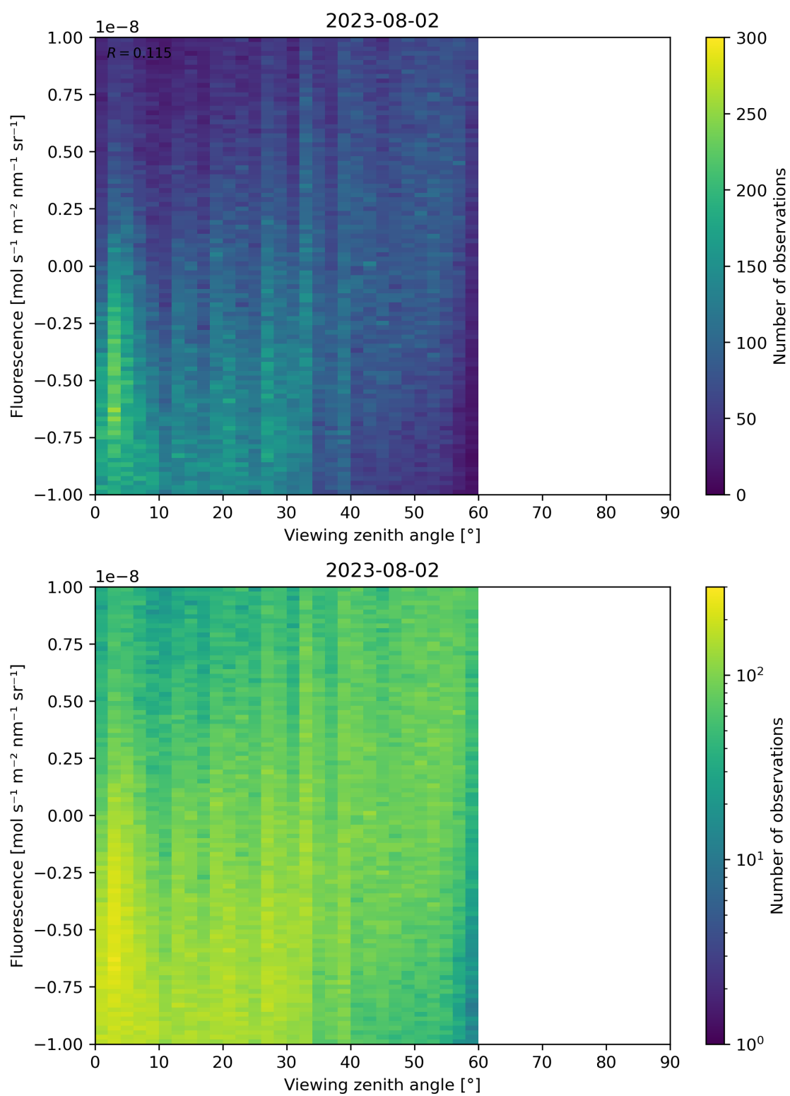
Figure 108: Scatter density plot of “Viewing zenith angle” against “Fluorescence” for 2023-08-01 to 2023-08-03.
