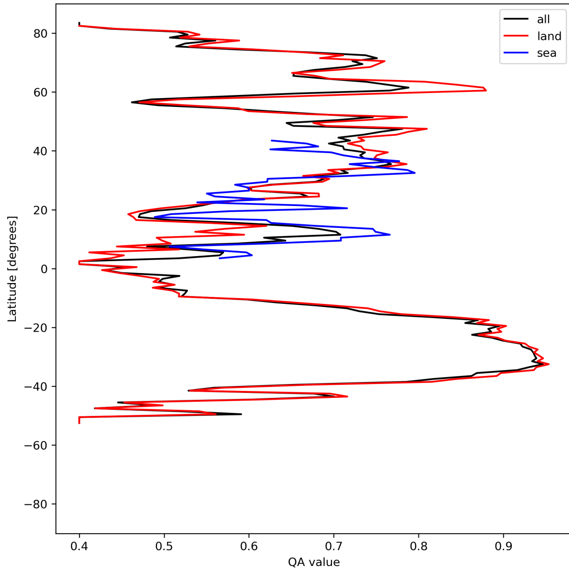
Figure 11: Zonal average of “QA value” for 2023-08-01 to 2023-08-03.
