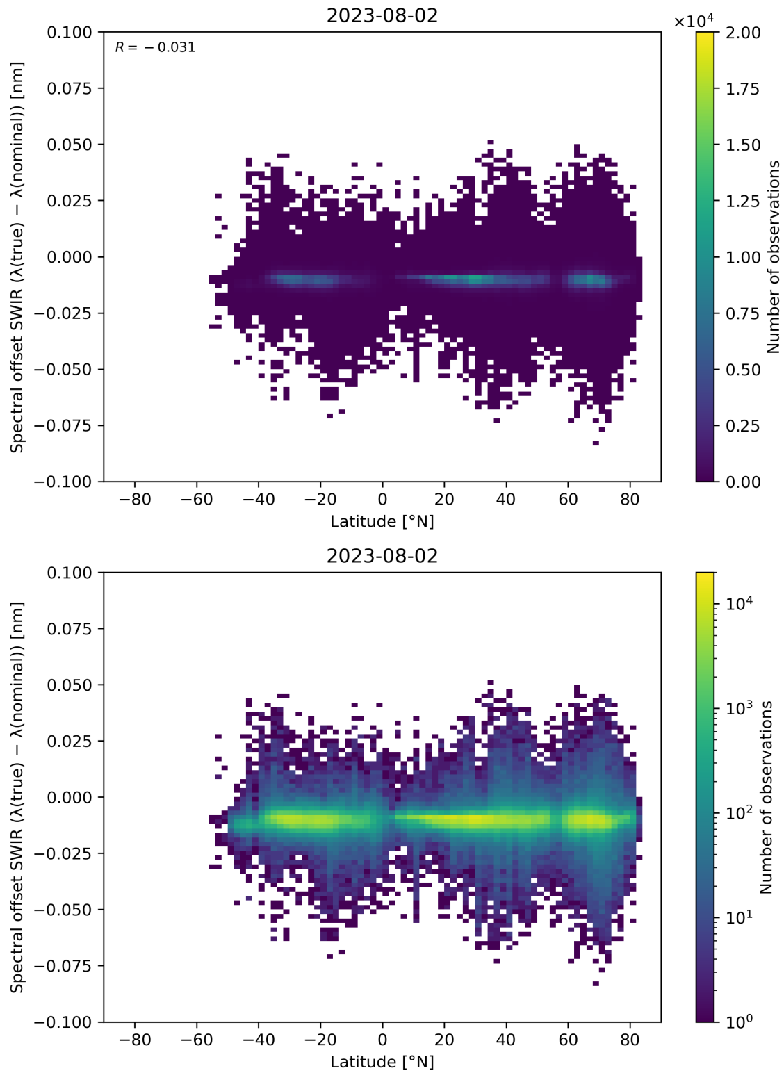
Figure 62: Scatter density plot of “Latitude” against “Spectral offset SWIR ( \lambda(\text{true}) - \lambda(\text{nominal}) )” for 2023-08-01 to 2023-08-03.
