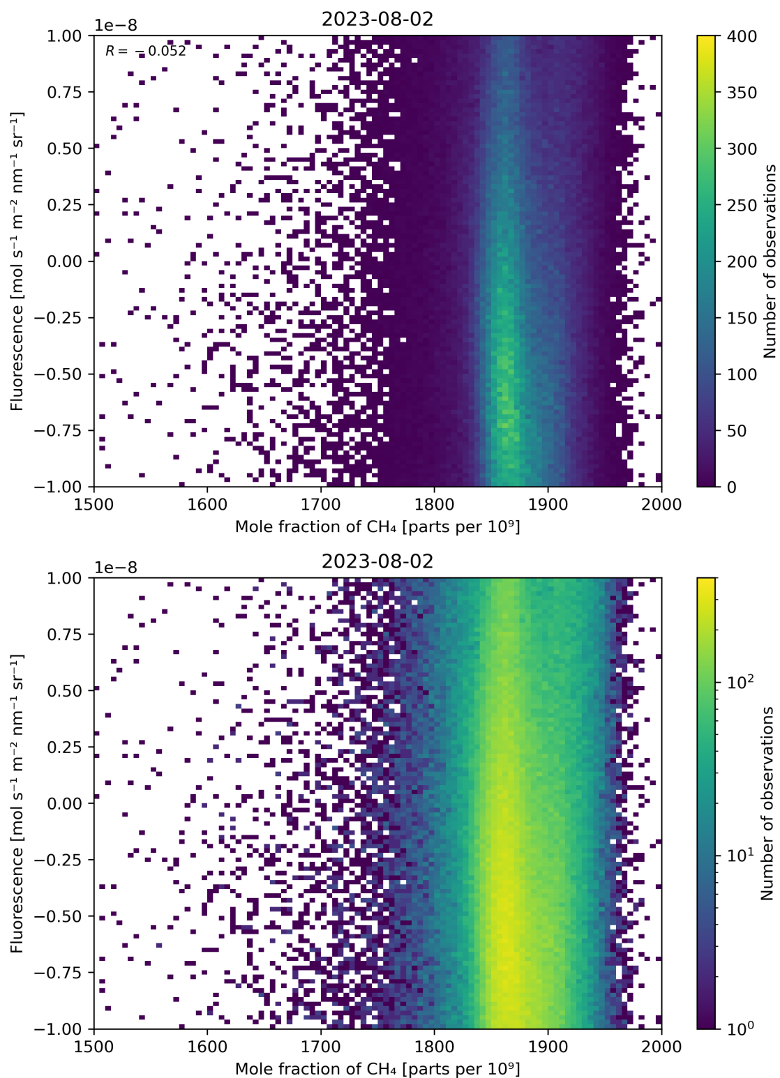
Figure 73: Scatter density plot of “Mole fraction of \text{CH}_4 ” against “Fluorescence” for 2023-08-01 to 2023-08-03.
