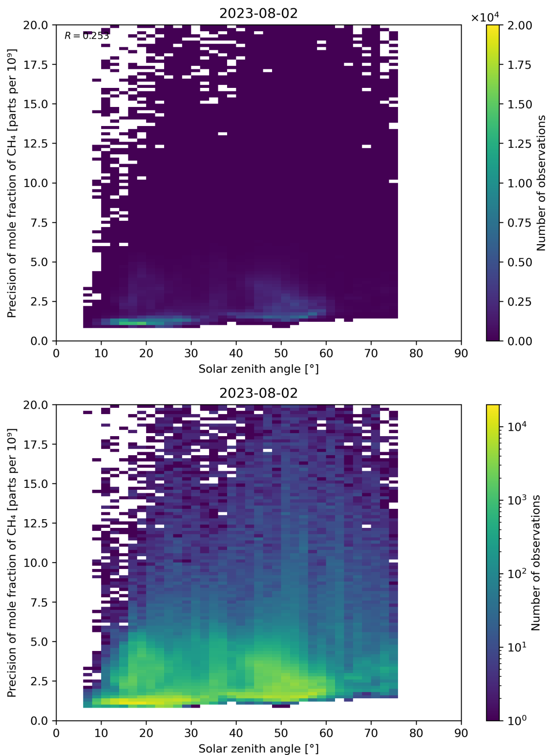
Figure 101: Scatter density plot of “Solar zenith angle” against “Precision of mole fraction of CH 4 ” for 2023-08-01 to 2023-08-03.
