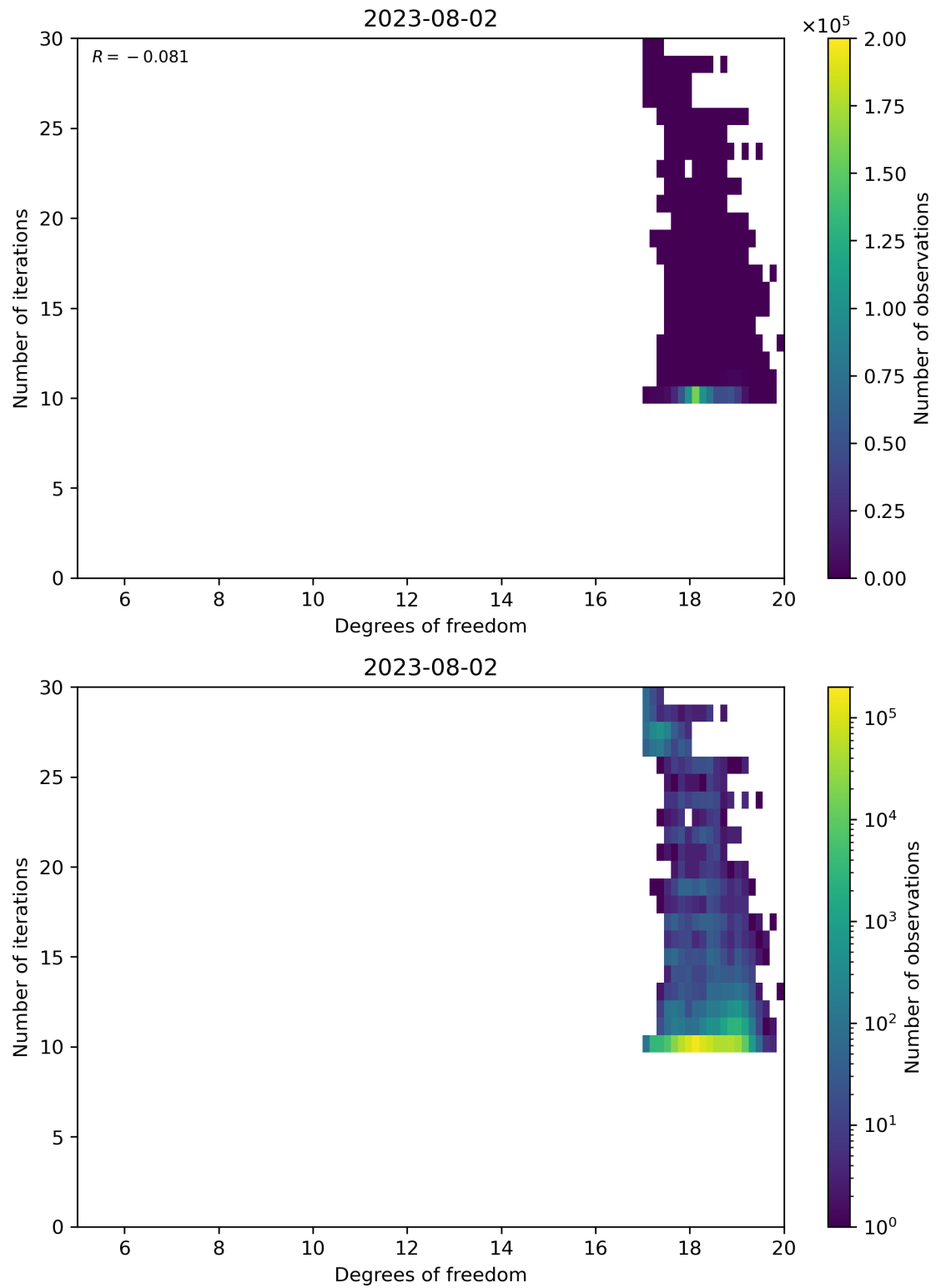
Figure 52: Scatter density plot of “Degrees of freedom” against “Number of iterations” for 2023-08-01 to 2023-08-03.
