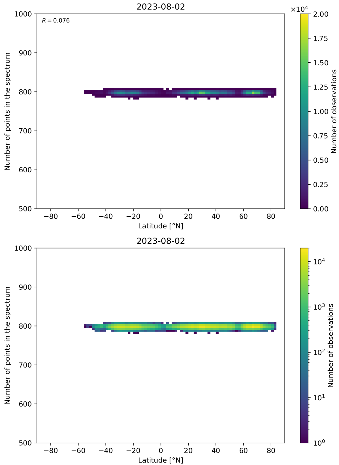
Figure 61: Scatter density plot of “Latitude” against “Number of points in the spectrum” for 2023-08-01 to 2023-08-03.
