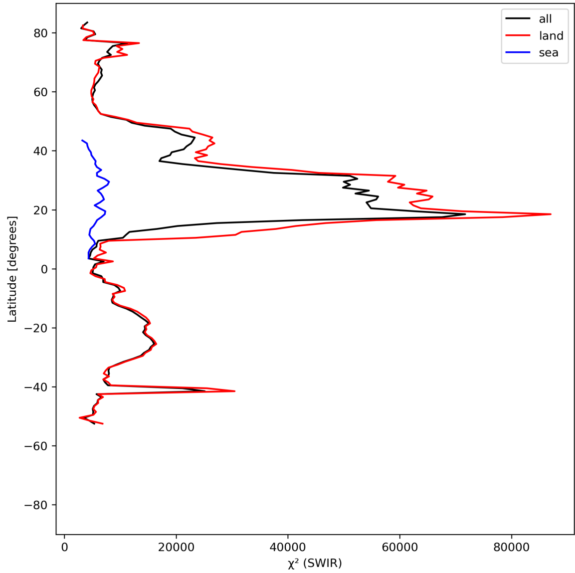
Figure 17: Zonal average of “ \chi^2 (SWIR)” for 2023-08-01 to 2023-08-03.
