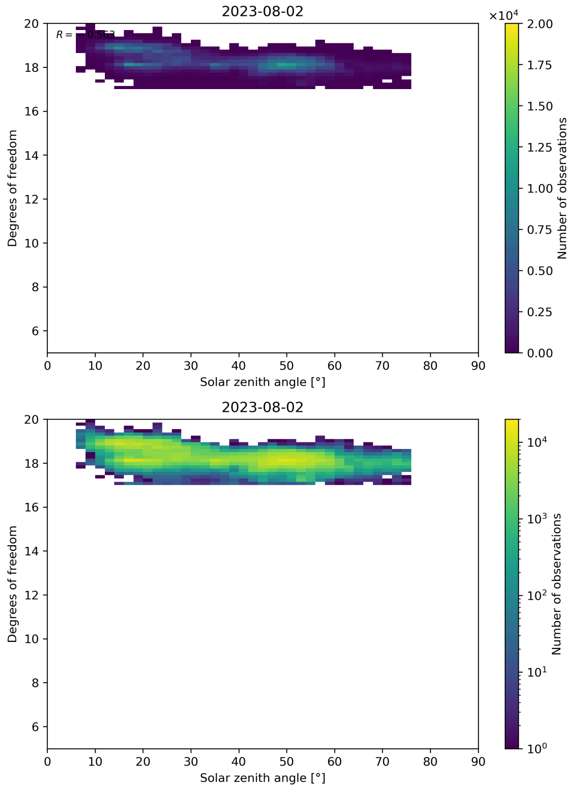
Figure 96: Scatter density plot of “Solar zenith angle” against “Degrees of freedom” for 2023-08-01 to 2023-08-03.
