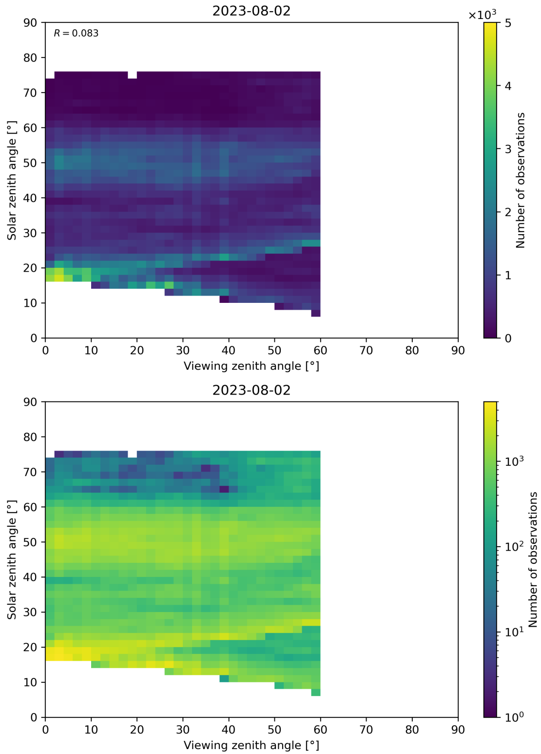
Figure 115: Scatter density plot of “Viewing zenith angle” against “Solar zenith angle” for 2023-08-01 to 2023-08-03.
