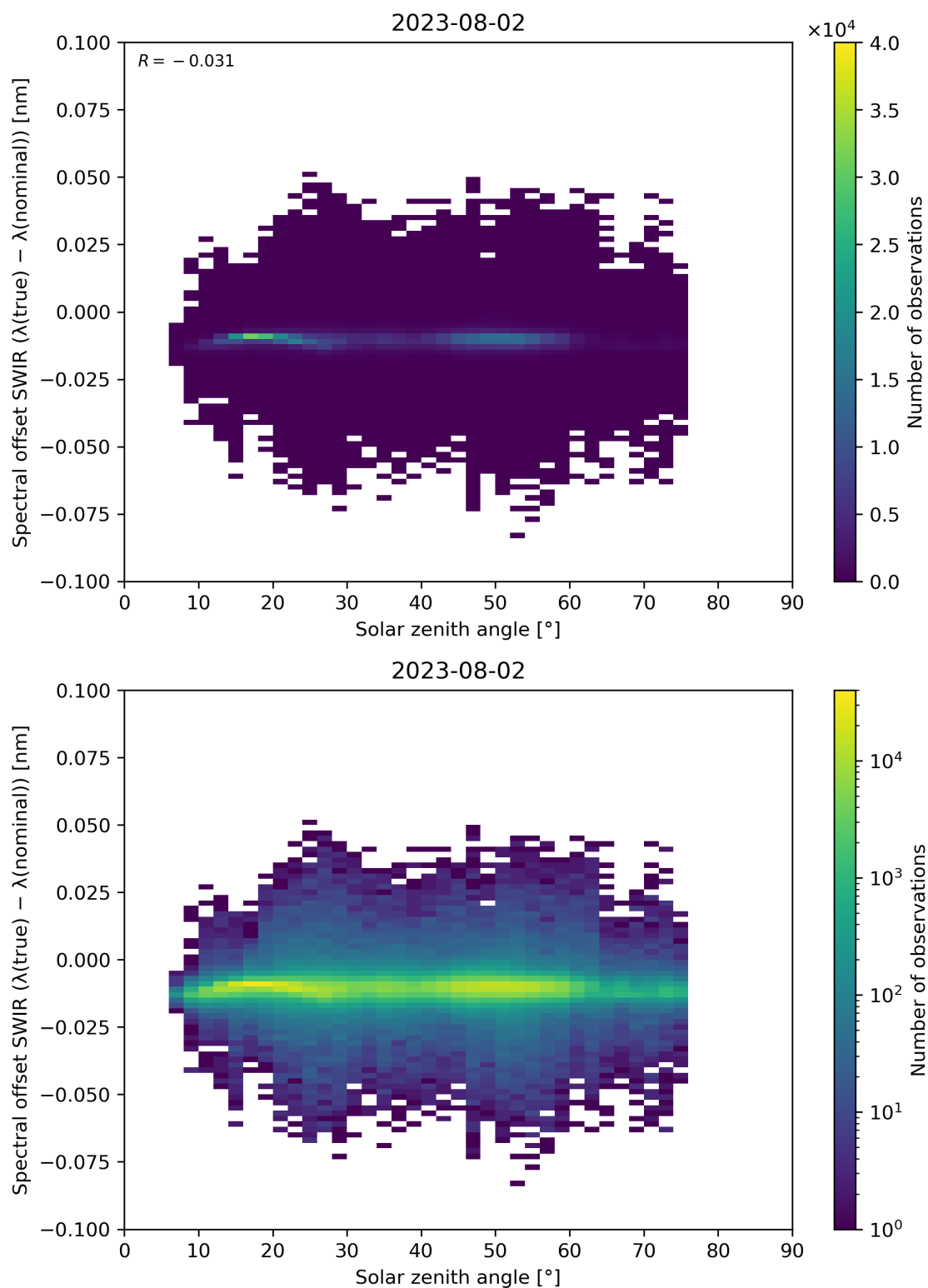
Figure 104: Scatter density plot of “Solar zenith angle” against “Spectral offset SWIR ( \lambda(\text{true}) - \lambda(\text{nominal}) )” for 2023-08-01 to 2023-08-03.
