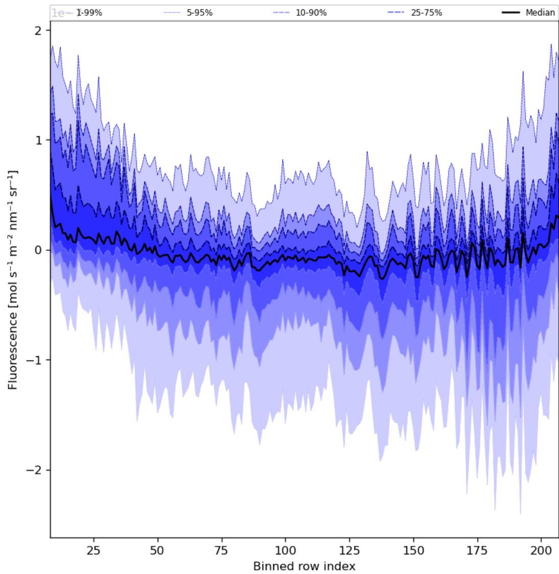
Figure 43: Along track statistics of “Fluorescence” for 2023-08-01 to 2023-08-03
