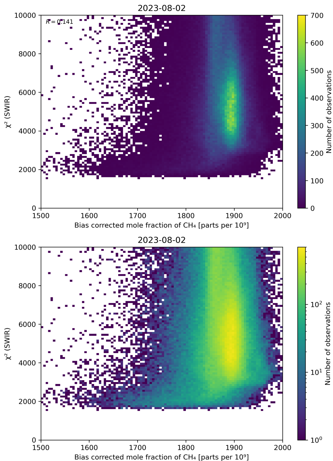
Figure 64: Scatter density plot of “Bias corrected mole fraction of CH 4 ” against “ \chi^2 (SWIR)” for 2023-08-01 to 2023-08-03.
