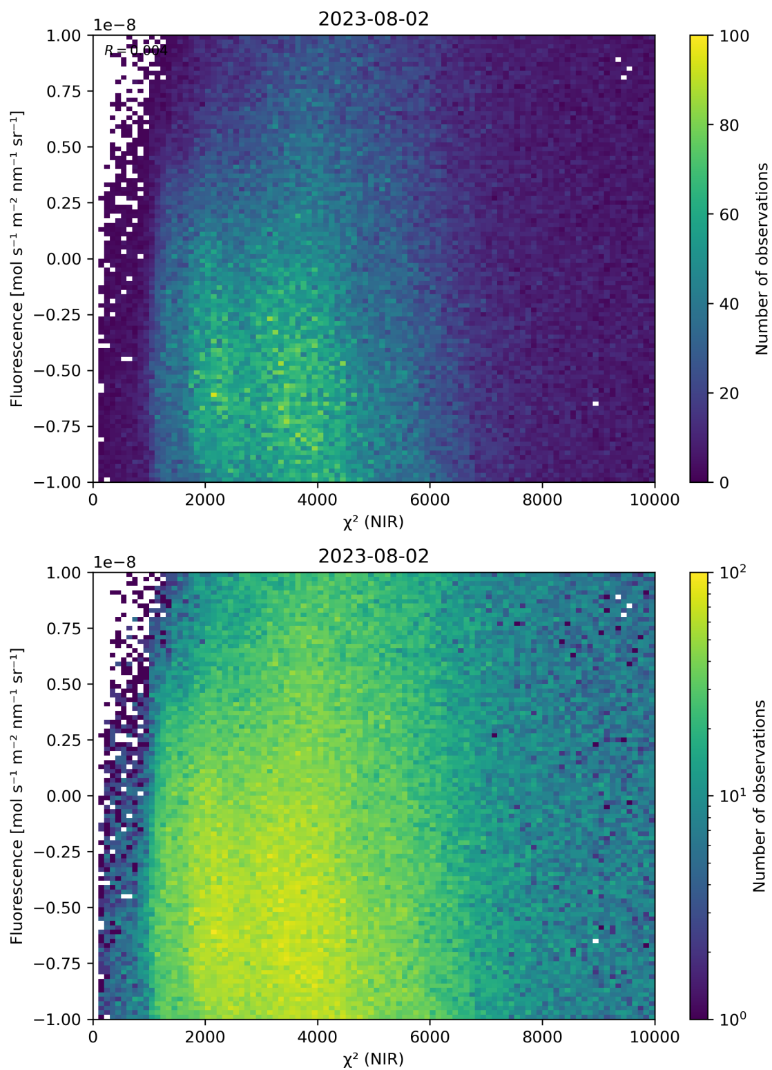
Figure 45: Scatter density plot of “ \chi^2 (NIR)” against “Fluorescence” for 2023-08-01 to 2023-08-03.
