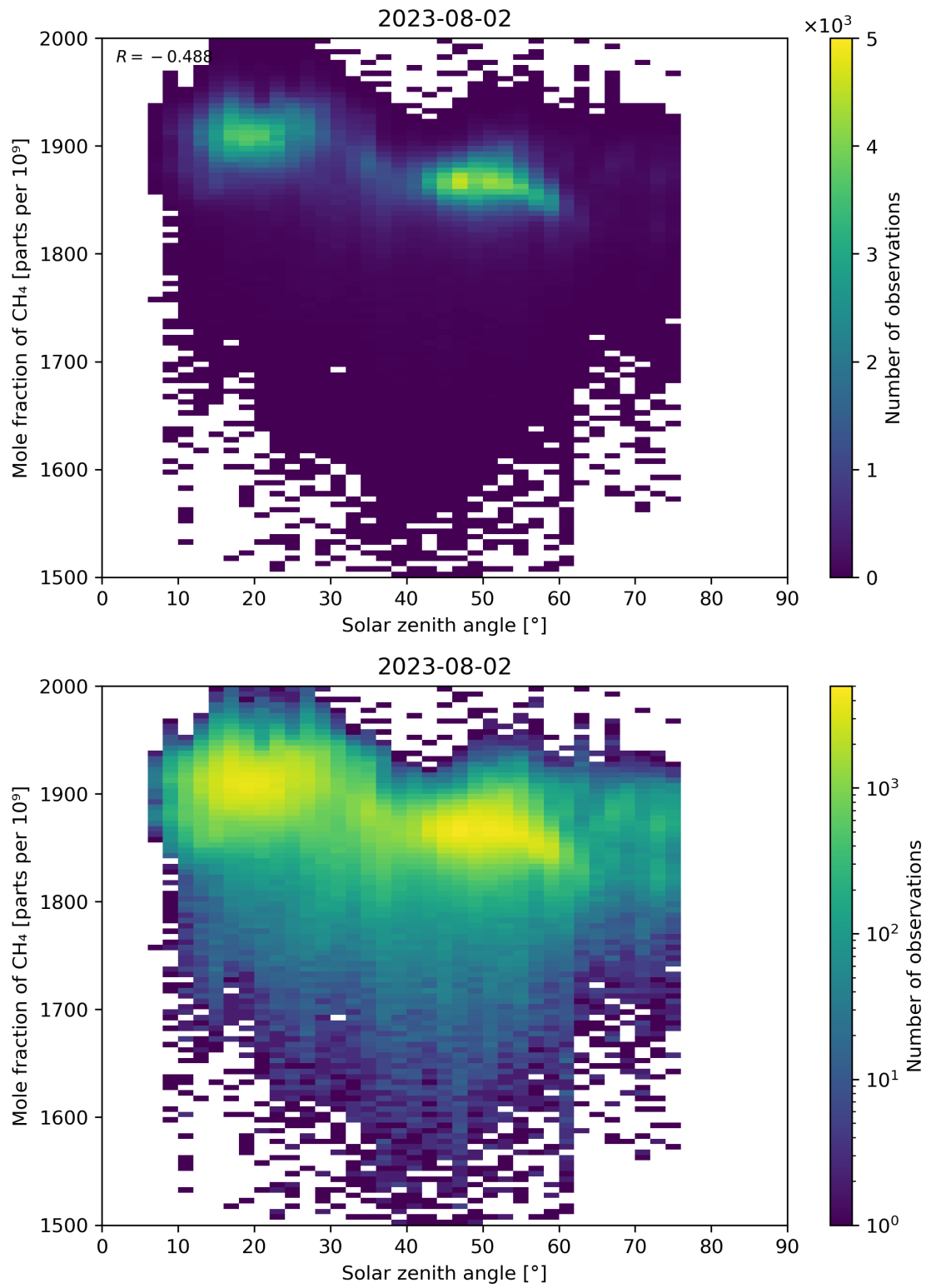
Figure 99: Scatter density plot of “Solar zenith angle” against “Mole fraction of CH 4 ” for 2023-08-01 to 2023-08-03.
