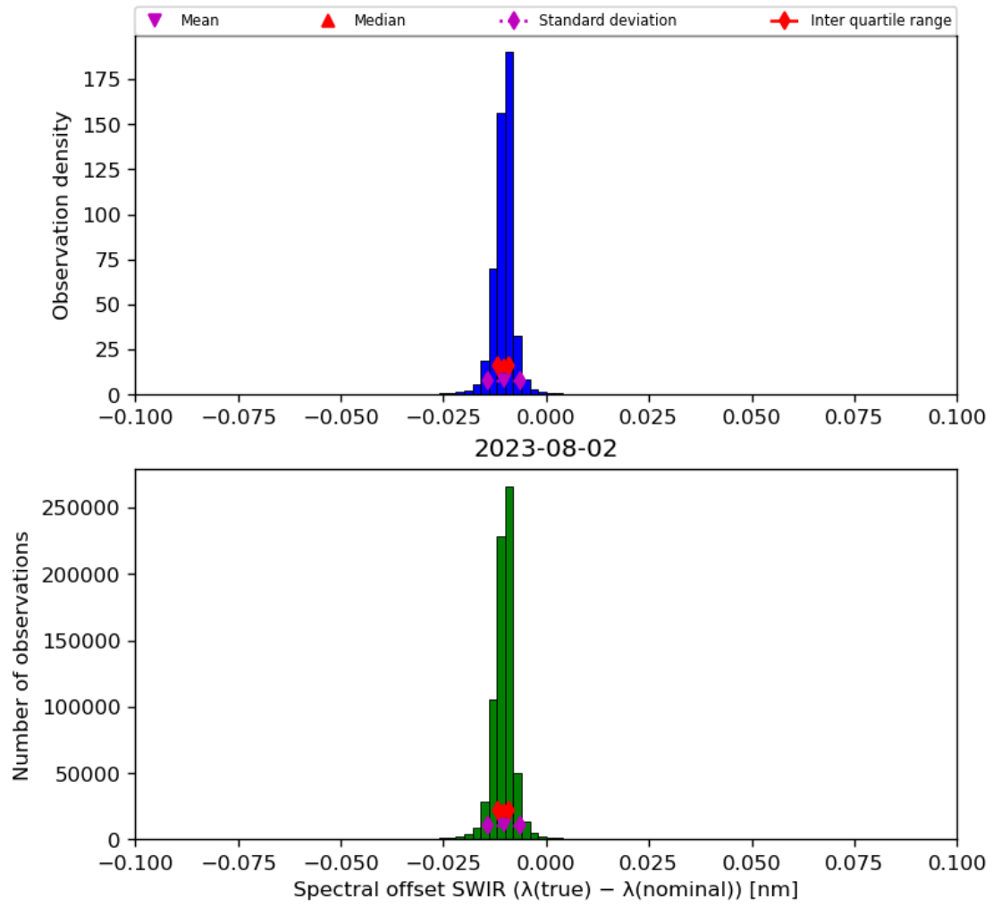
Figure 27: Histogram of “Spectral offset SWIR ( \lambda(\text{true}) - \lambda(\text{nominal}) )” for 2023-08-01 to 2023-08-03
