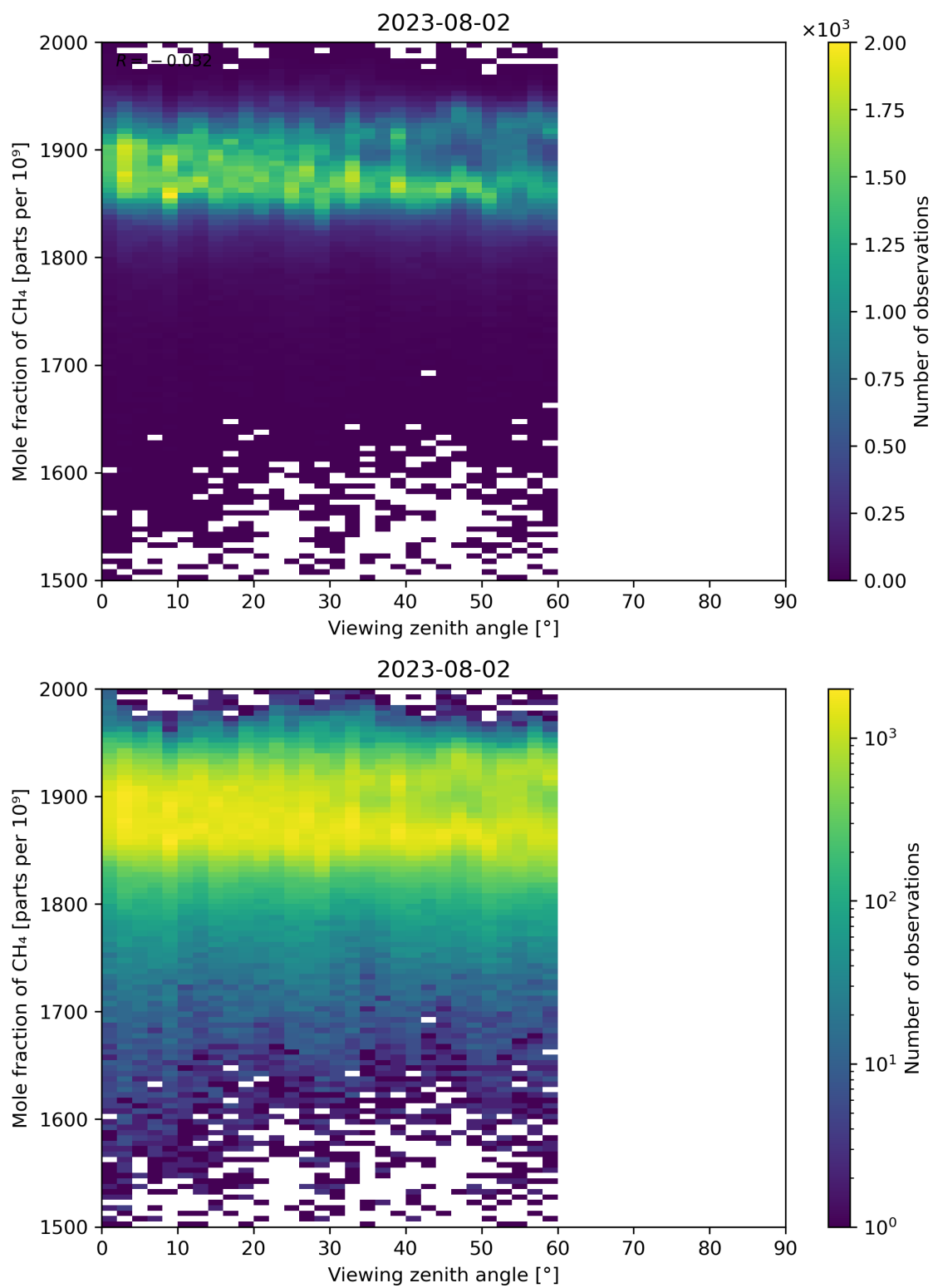
Figure 110: Scatter density plot of “Viewing zenith angle” against “Mole fraction of CH 4 ” for 2023-08-01 to 2023-08-03.
