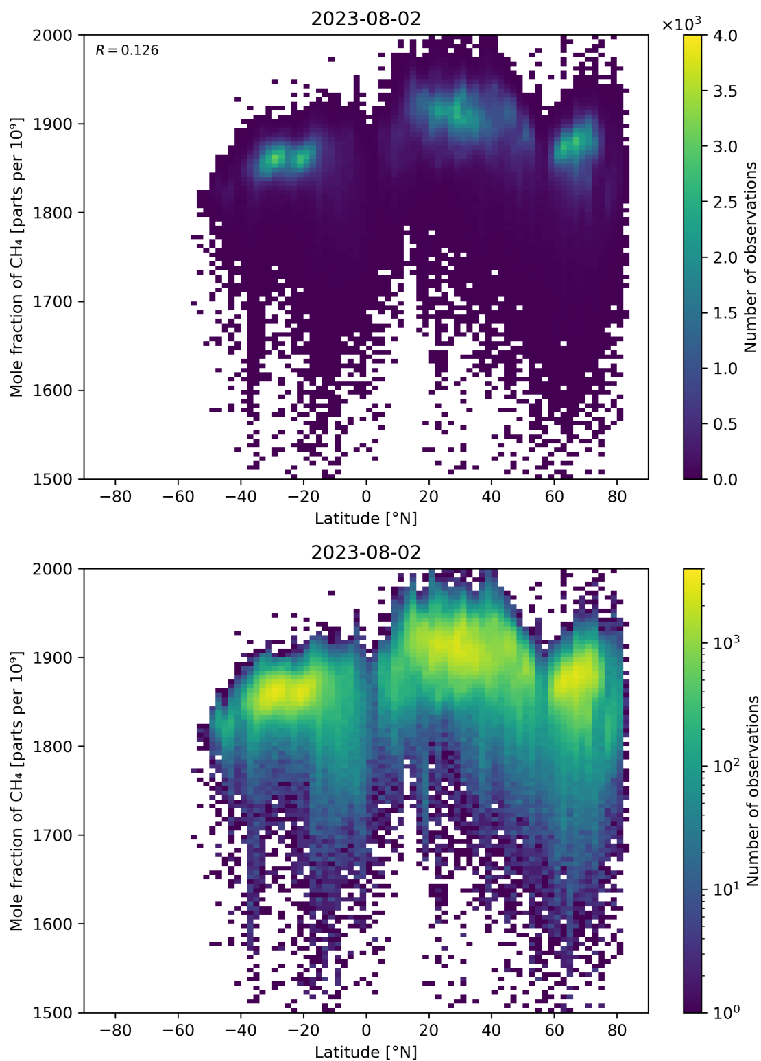
Figure 57: Scatter density plot of “Latitude” against “Mole fraction of CH 4 ” for 2023-08-01 to 2023-08-03.
