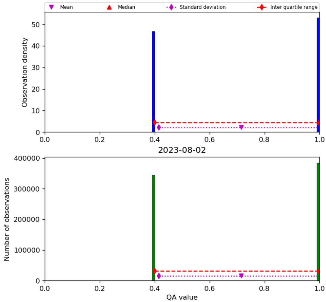
Figure 22: Histogram of “QA value” for 2023-08-01 to 2023-08-03
