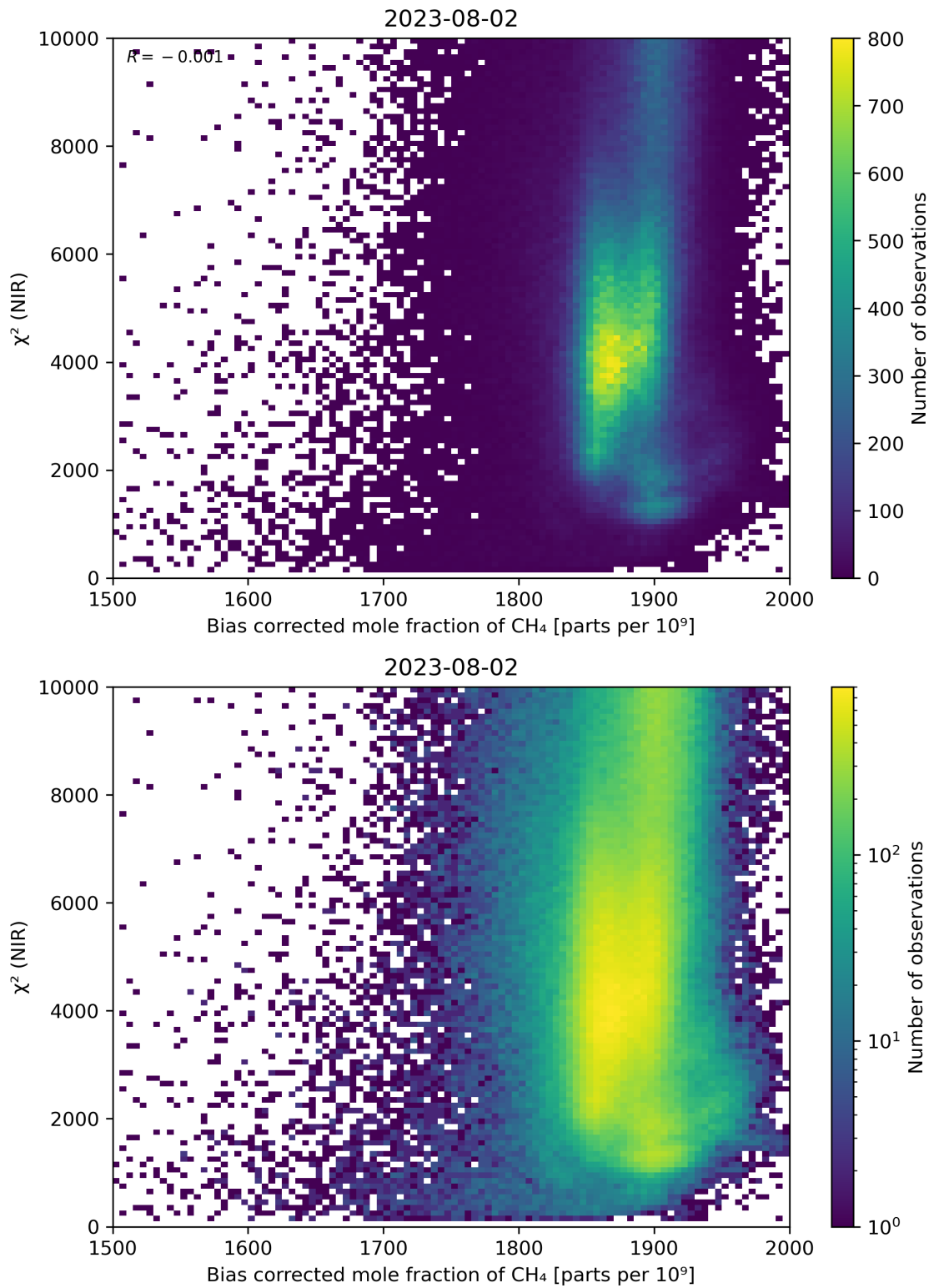
Figure 63: Scatter density plot of “Bias corrected mole fraction of CH 4 ” against “ \chi^2 (NIR)” for 2023-08-01 to 2023-08-03.
