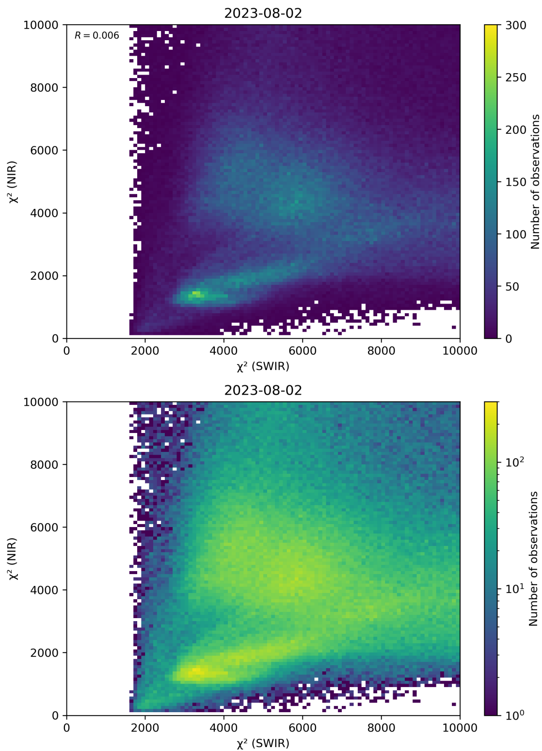
Figure 47: Scatter density plot of “ \chi^2 (SWIR)” against “ \chi^2 (NIR)” for 2023-08-01 to 2023-08-03.
