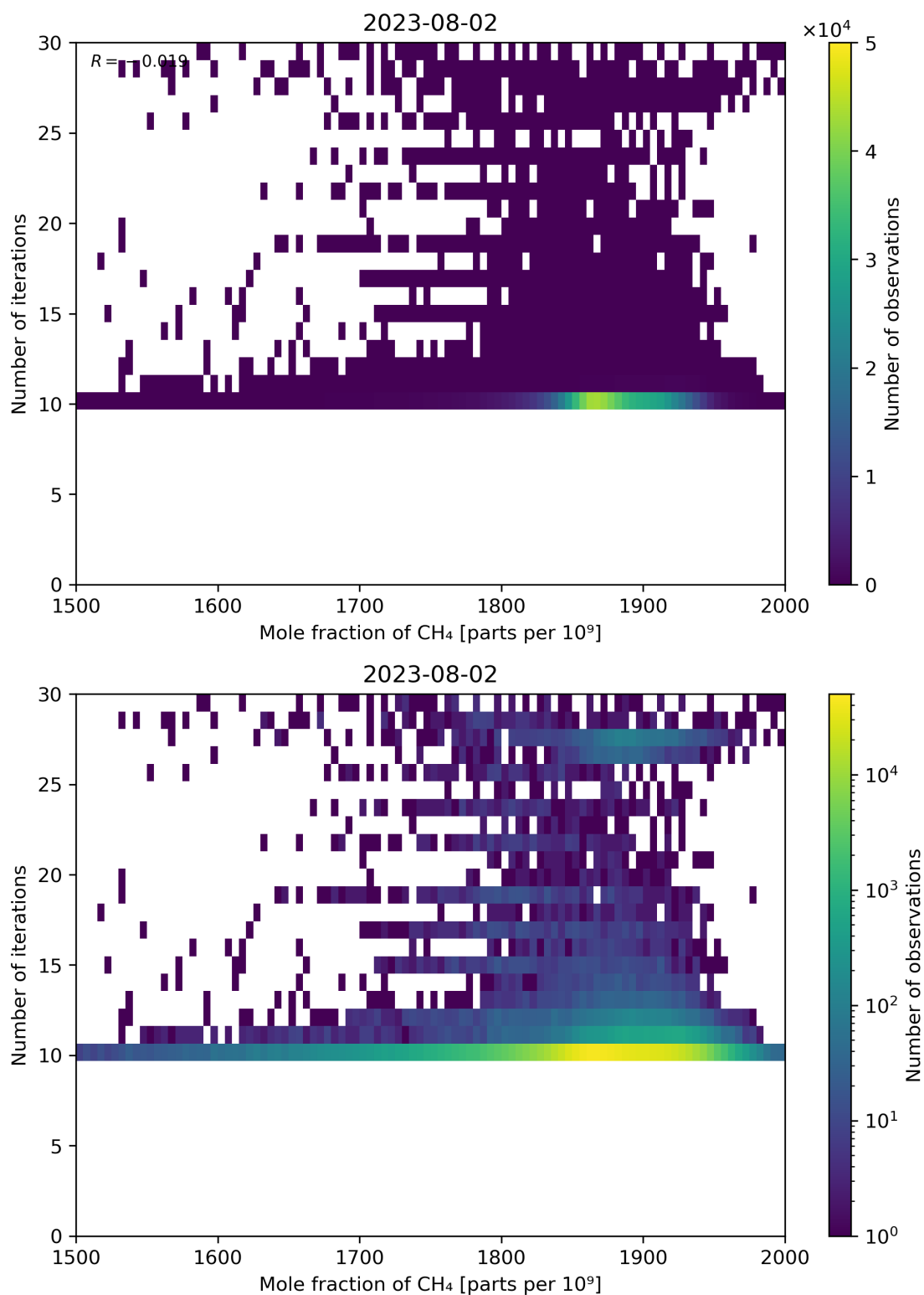
Figure 76: Scatter density plot of “Mole fraction of CH 4 ” against “Number of iterations” for 2023-08-01 to 2023-08-03.
