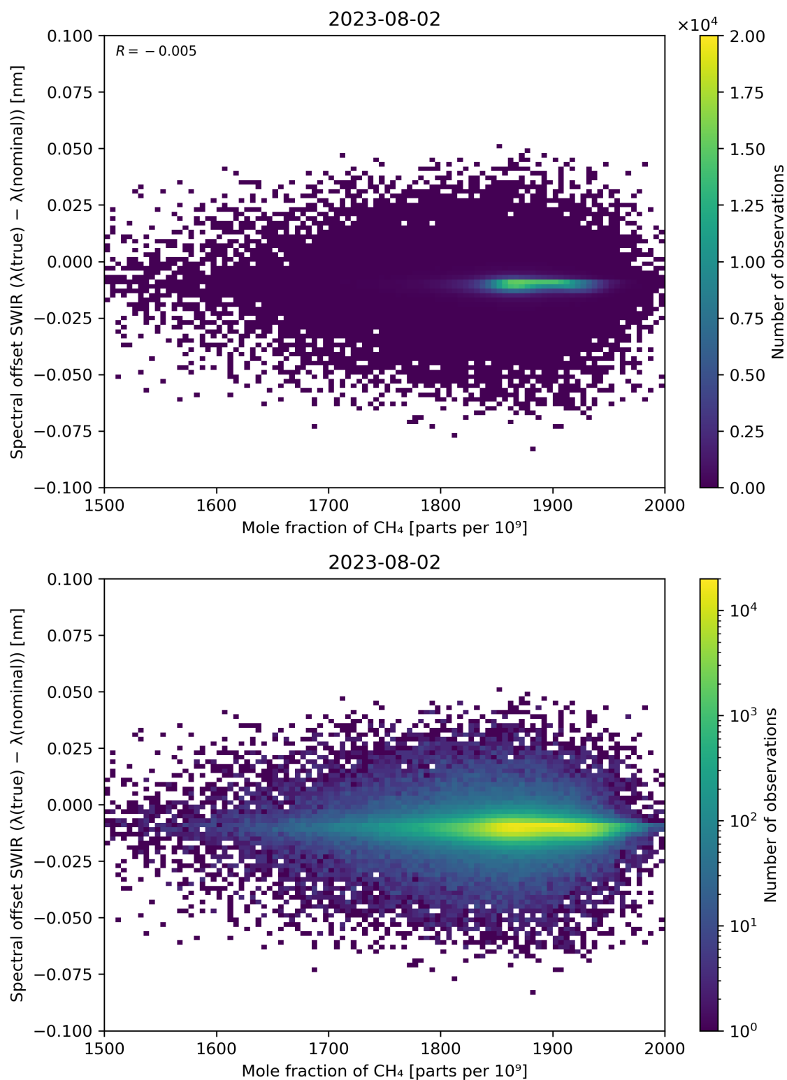
Figure 86: Scatter density plot of “Mole fraction of CH 4 ” against “Spectral offset SWIR ( \lambda(\text{true}) - \lambda(\text{nominal}) )” for 2023-08-01 to 2023-08-03.
