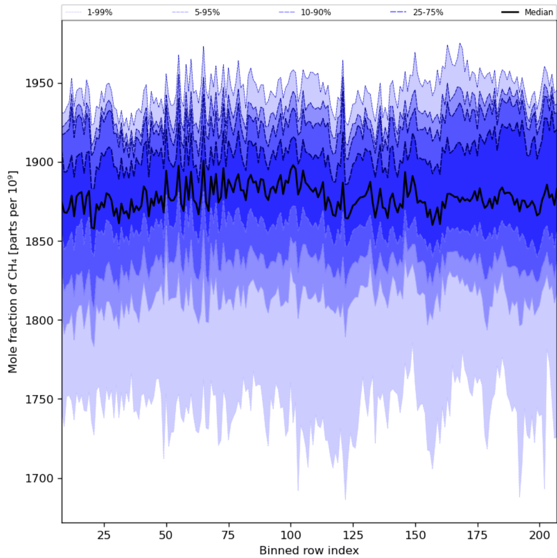
Figure 34: Along track statistics of “Mole fraction of CH 4 ” for 2023-08-01 to 2023-08-03
