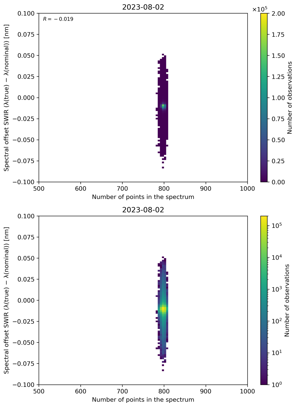
Figure 93: Scatter density plot of “Number of points in the spectrum” against “Spectral offset SWIR ( \lambda(\text{true}) - \lambda(\text{nominal}) )” for 2023-08-01 to 2023-08-03.
