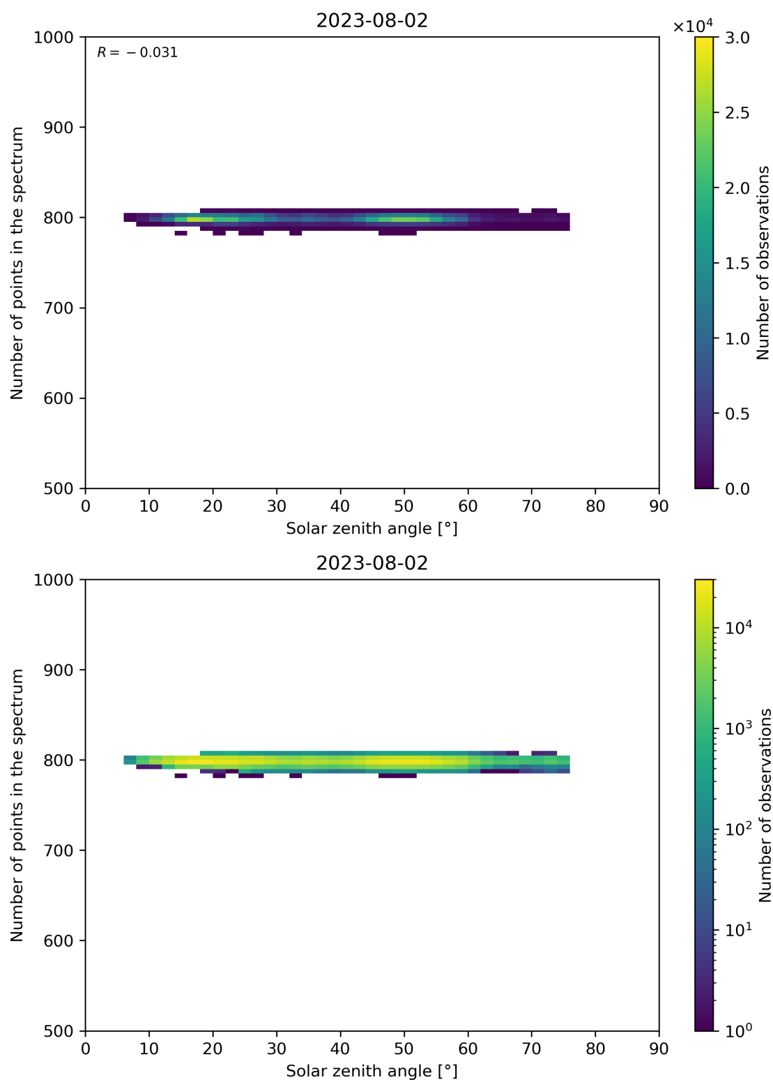
Figure 103: Scatter density plot of “Solar zenith angle” against “Number of points in the spectrum” for 2023-08-01 to 2023-08-03.
