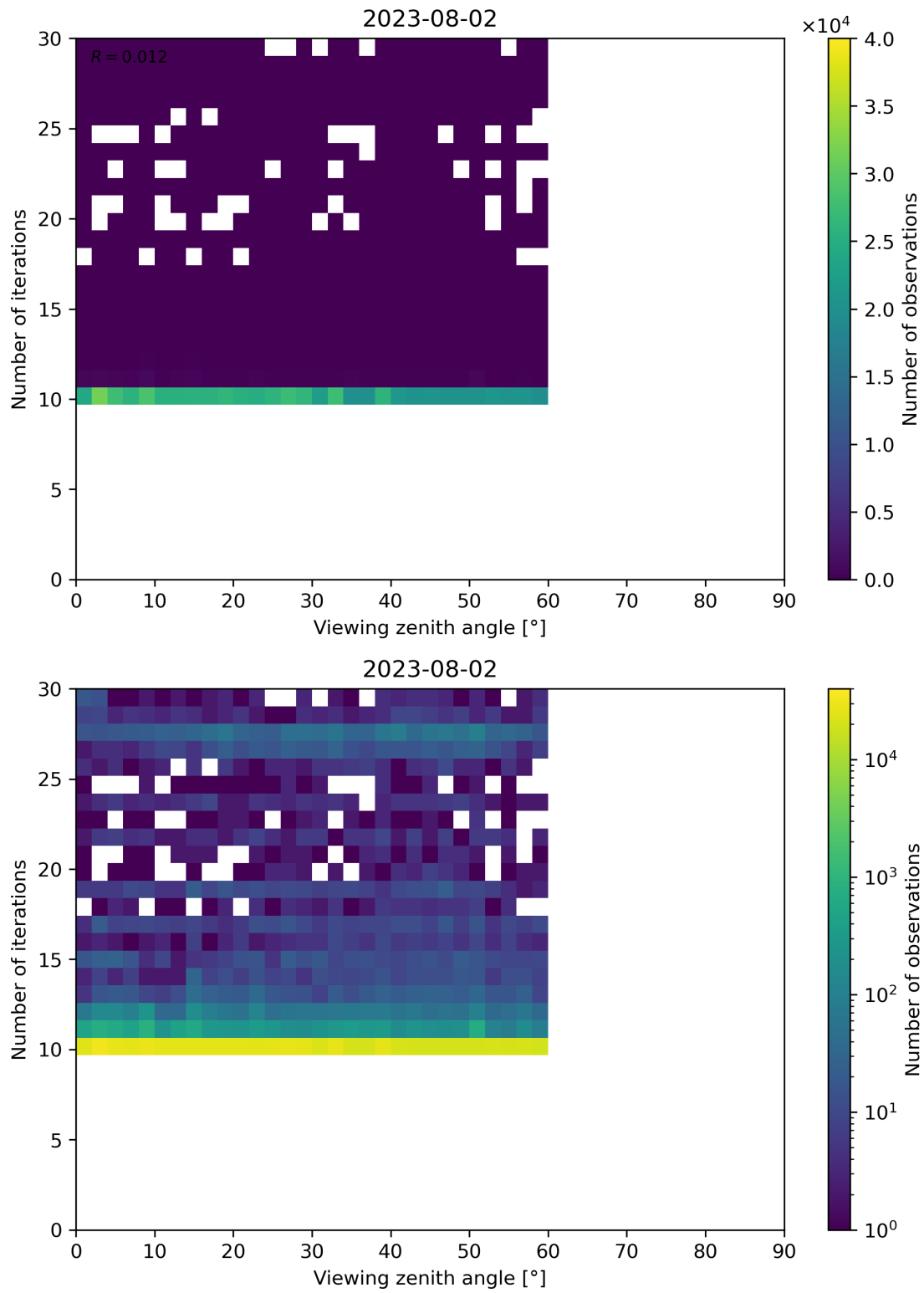
Figure 113: Scatter density plot of “Viewing zenith angle” against “Number of iterations” for 2023-08-01 to 2023-08-03.
