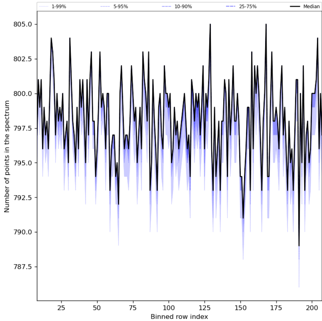
Figure 37: Along track statistics of “Number of points in the spectrum” for 2023-08-01 to 2023-08-03
