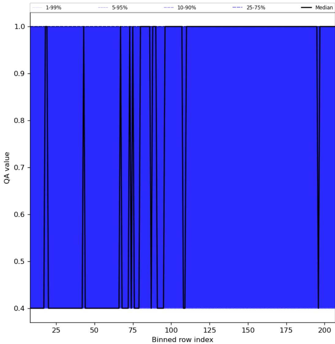
Figure 33: Along track statistics of “QA value” for 2023-08-01 to 2023-08-03
