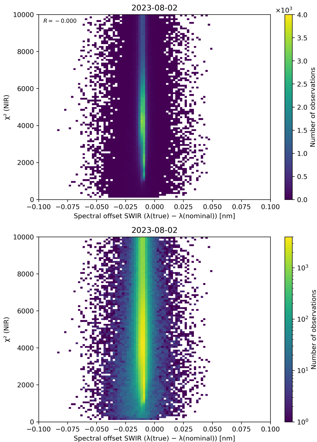
Figure 117: Scatter density plot of “Spectral offset SWIR ( \lambda(\text{true}) - \lambda(\text{nominal}) )” against “ \chi^2 (NIR)” for 2023-08-01 to 2023-08-03.
