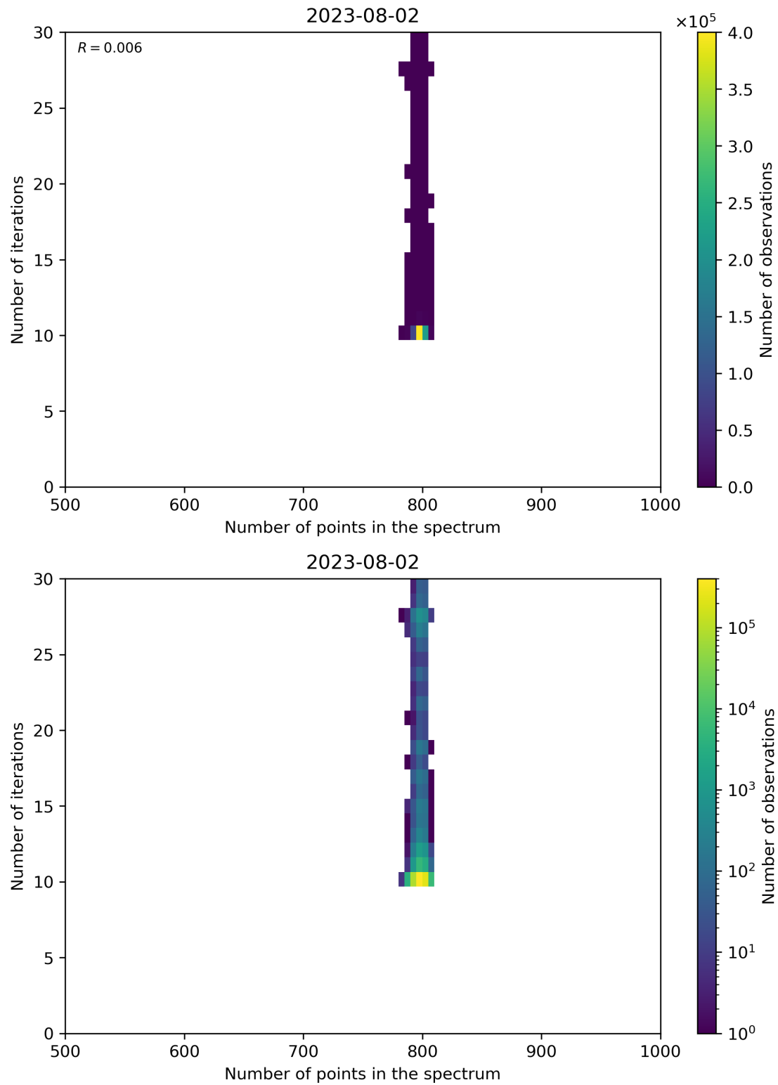
Figure 92: Scatter density plot of “Number of points in the spectrum” against “Number of iterations” for 2023-08-01 to 2023-08-03.
