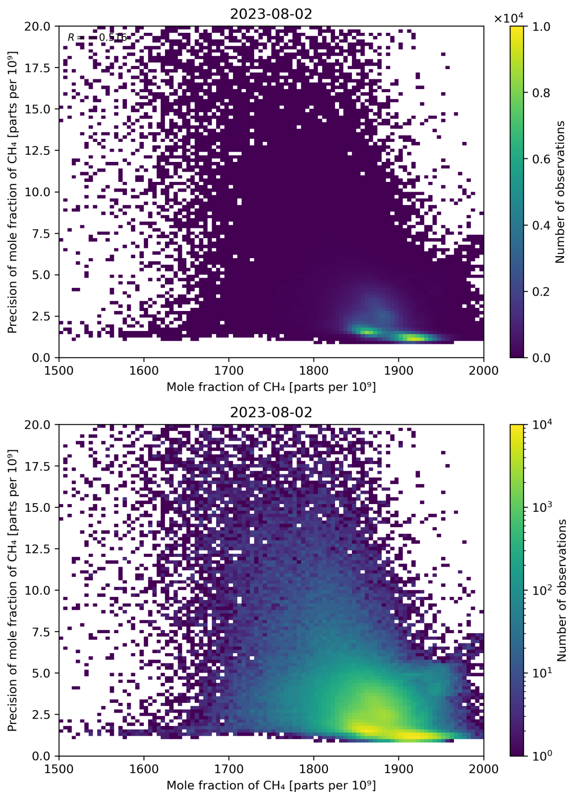
Figure 75: Scatter density plot of “Mole fraction of CH 4 ” against “Precision of mole fraction of CH 4 ” for 2023-08-01 to 2023-08-03.
