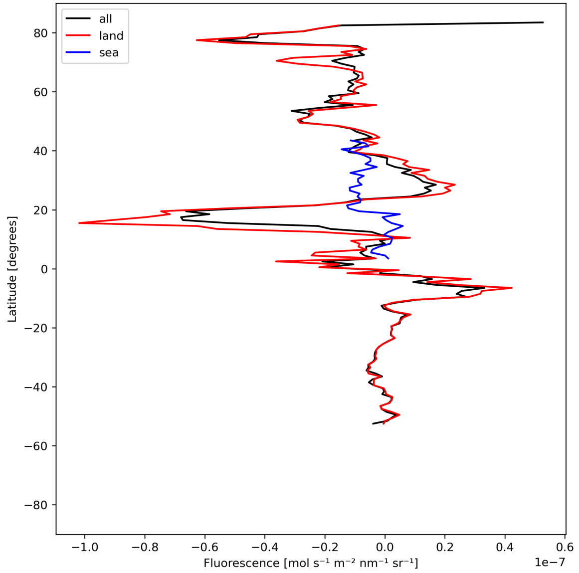
Figure 21: Zonal average of “Fluorescence” for 2023-08-01 to 2023-08-03.
