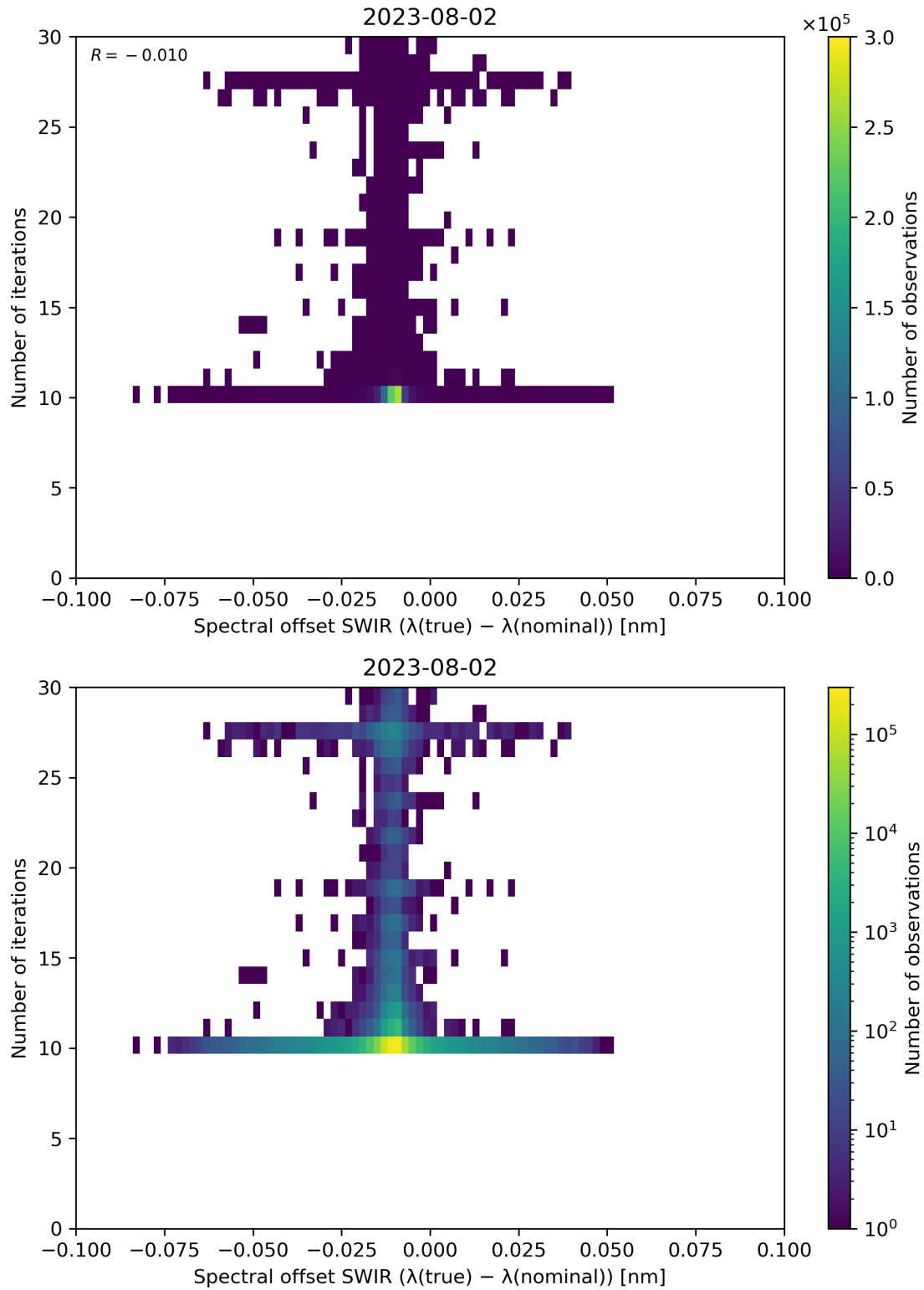
Figure 121: Scatter density plot of “Spectral offset SWIR ( \lambda(\text{true}) - \lambda(\text{nominal}) )” against “Number of iterations” for 2023-08-01 to 2023-08-03.
