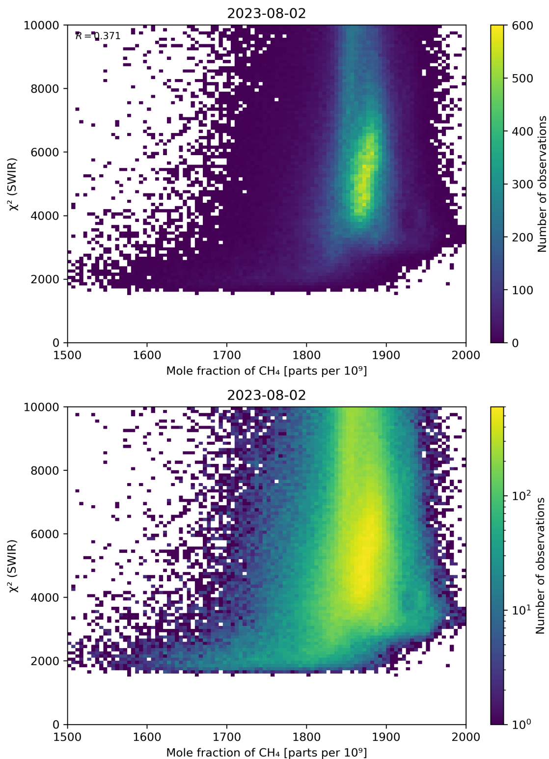
Figure 71: Scatter density plot of “Mole fraction of \text{CH}_4 ” against “ \chi^2 (SWIR)” for 2023-08-01 to 2023-08-03.
