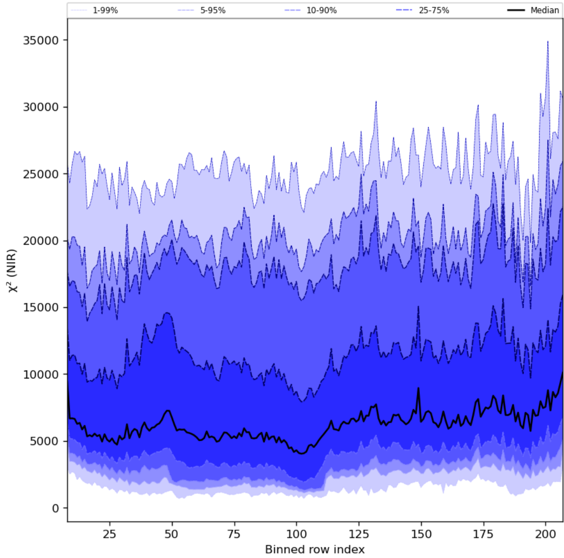
Figure 40: Along track statistics of “ \chi^2 (NIR)” for 2023-08-01 to 2023-08-03
