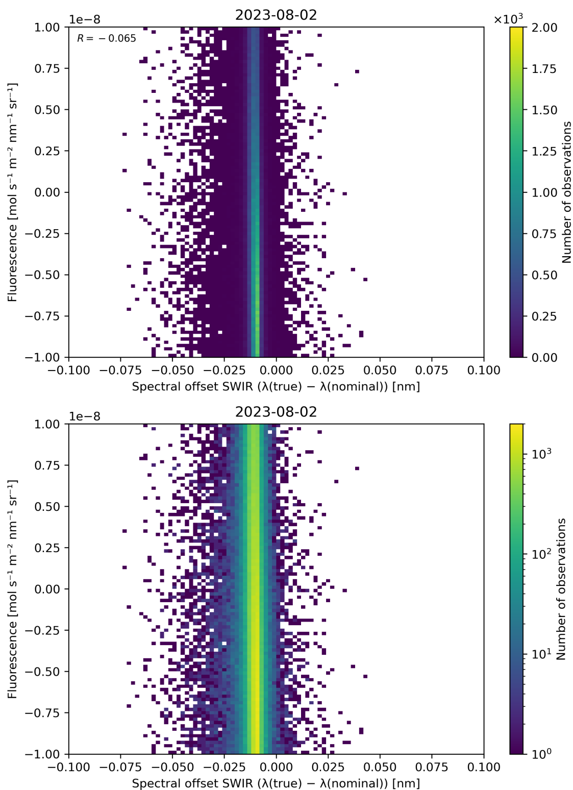
Figure 120: Scatter density plot of “Spectral offset SWIR ( \lambda(\text{true}) - \lambda(\text{nominal}) )” against “Fluorescence” for 2023-08-01 to 2023-08-03.
