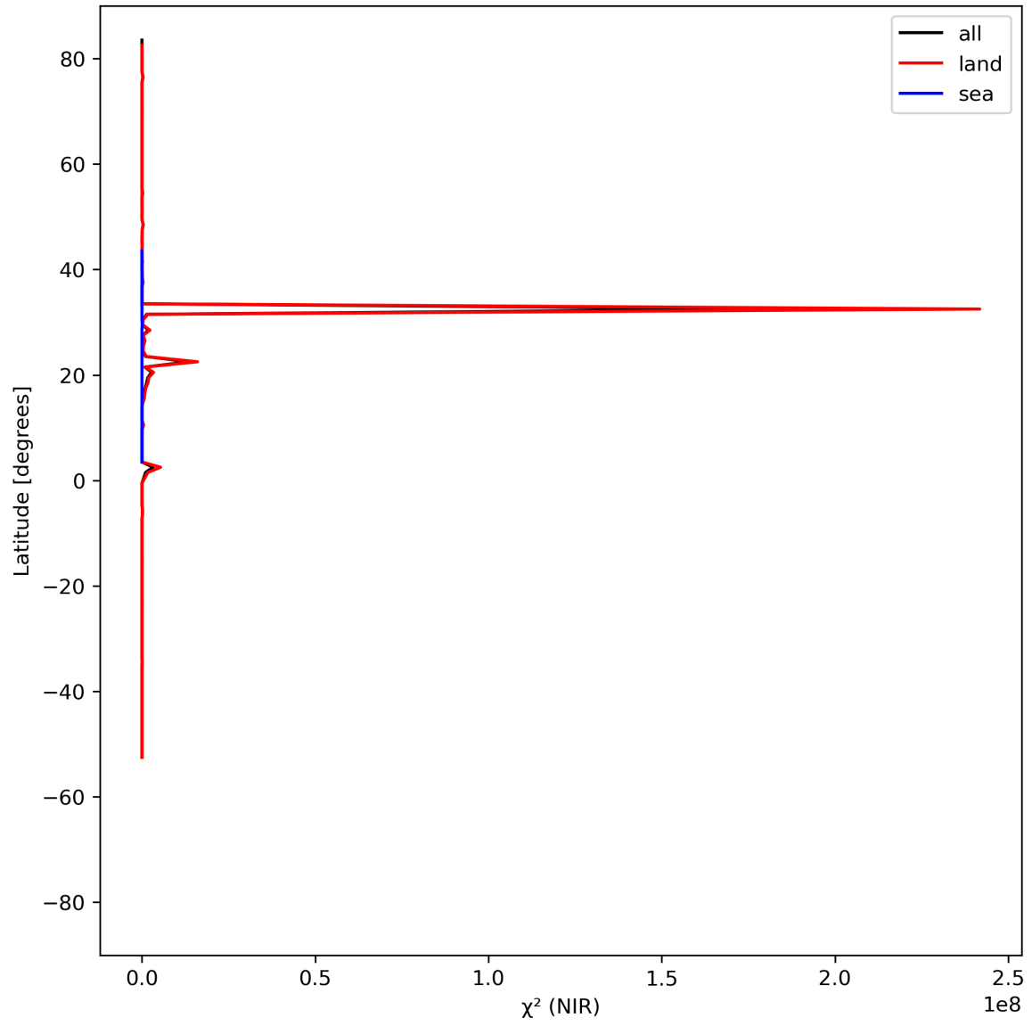
Figure 18: Zonal average of “ \chi^2 (NIR)” for 2023-08-01 to 2023-08-03.
