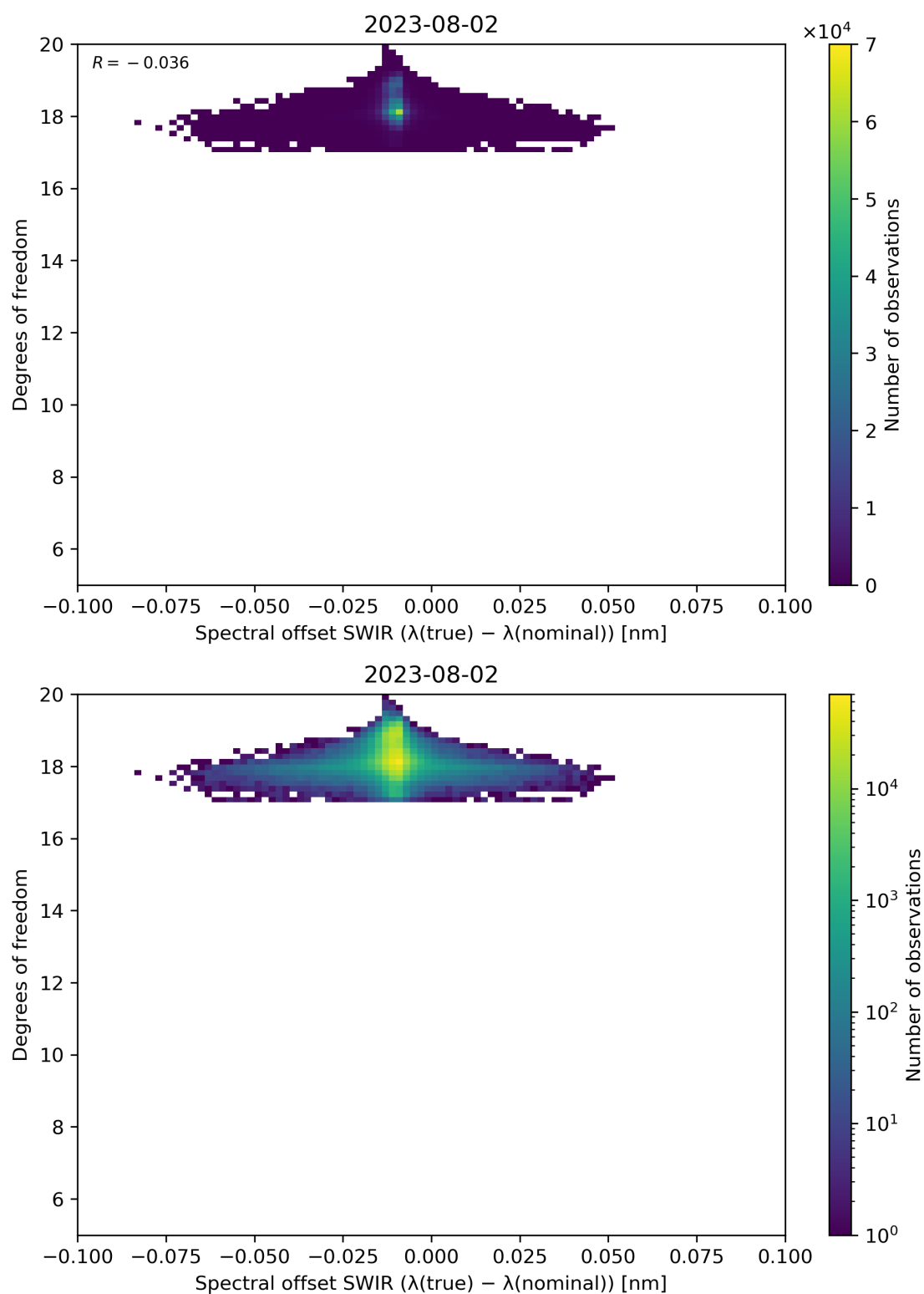
Figure 119: Scatter density plot of “Spectral offset SWIR ( \lambda(\text{true}) - \lambda(\text{nominal}) )” against “Degrees of freedom” for 2023-08-01 to 2023-08-03.
