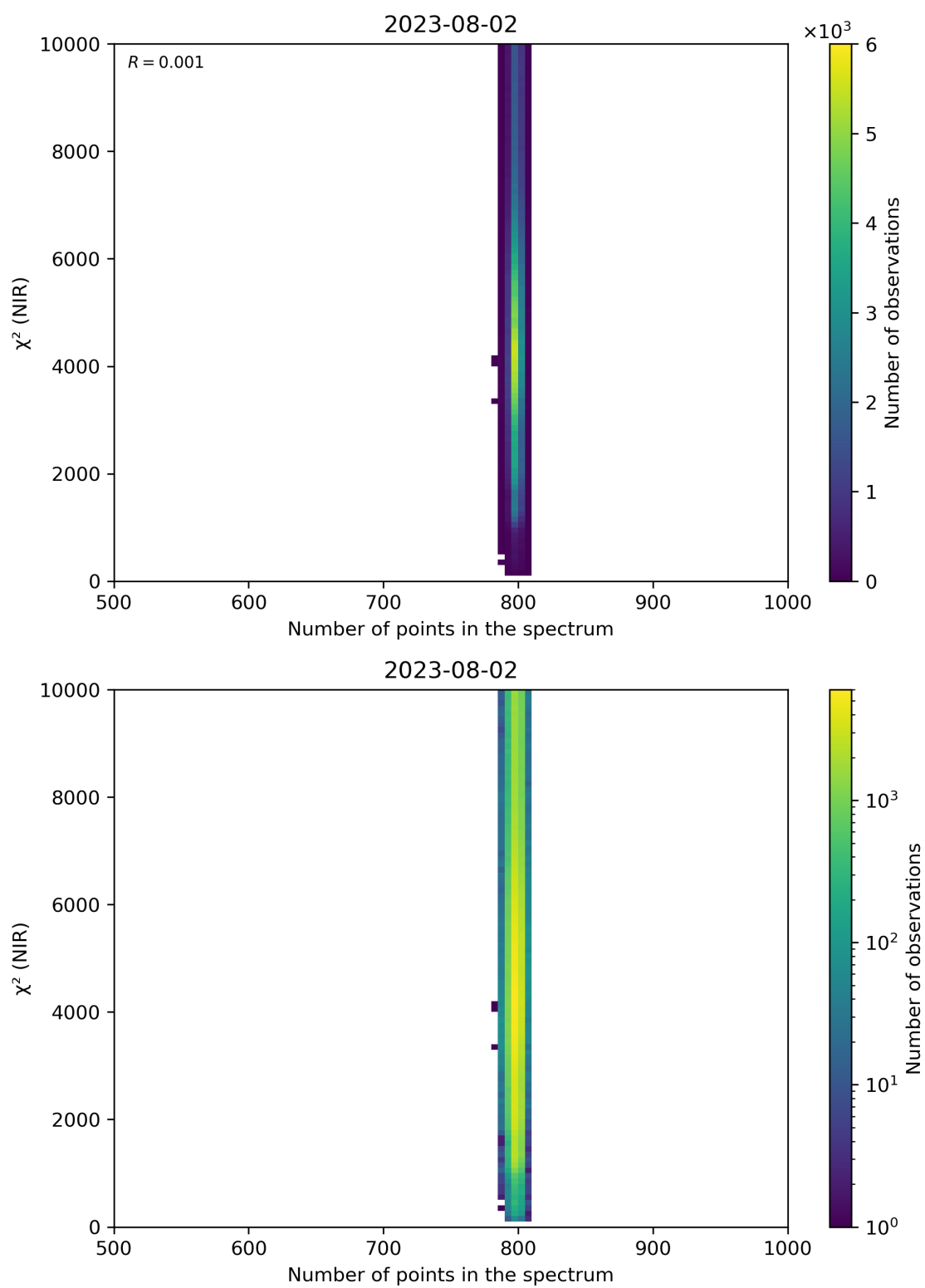
Figure 88: Scatter density plot of “Number of points in the spectrum” against “ \chi^2 (NIR)” for 2023-08-01 to 2023-08-03.
