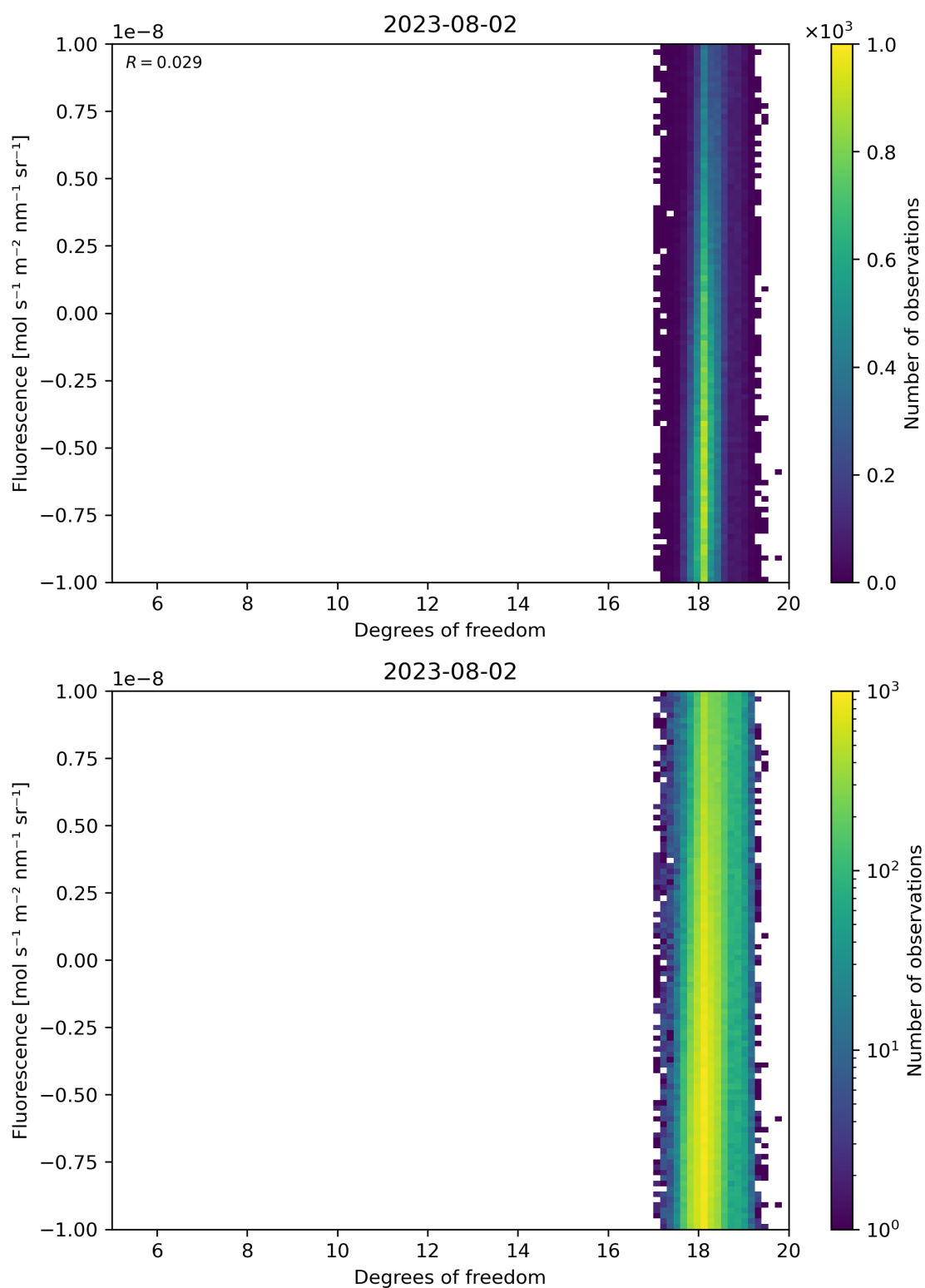
Figure 51: Scatter density plot of “Degrees of freedom” against “Fluorescence” for 2023-08-01 to 2023-08-03.
