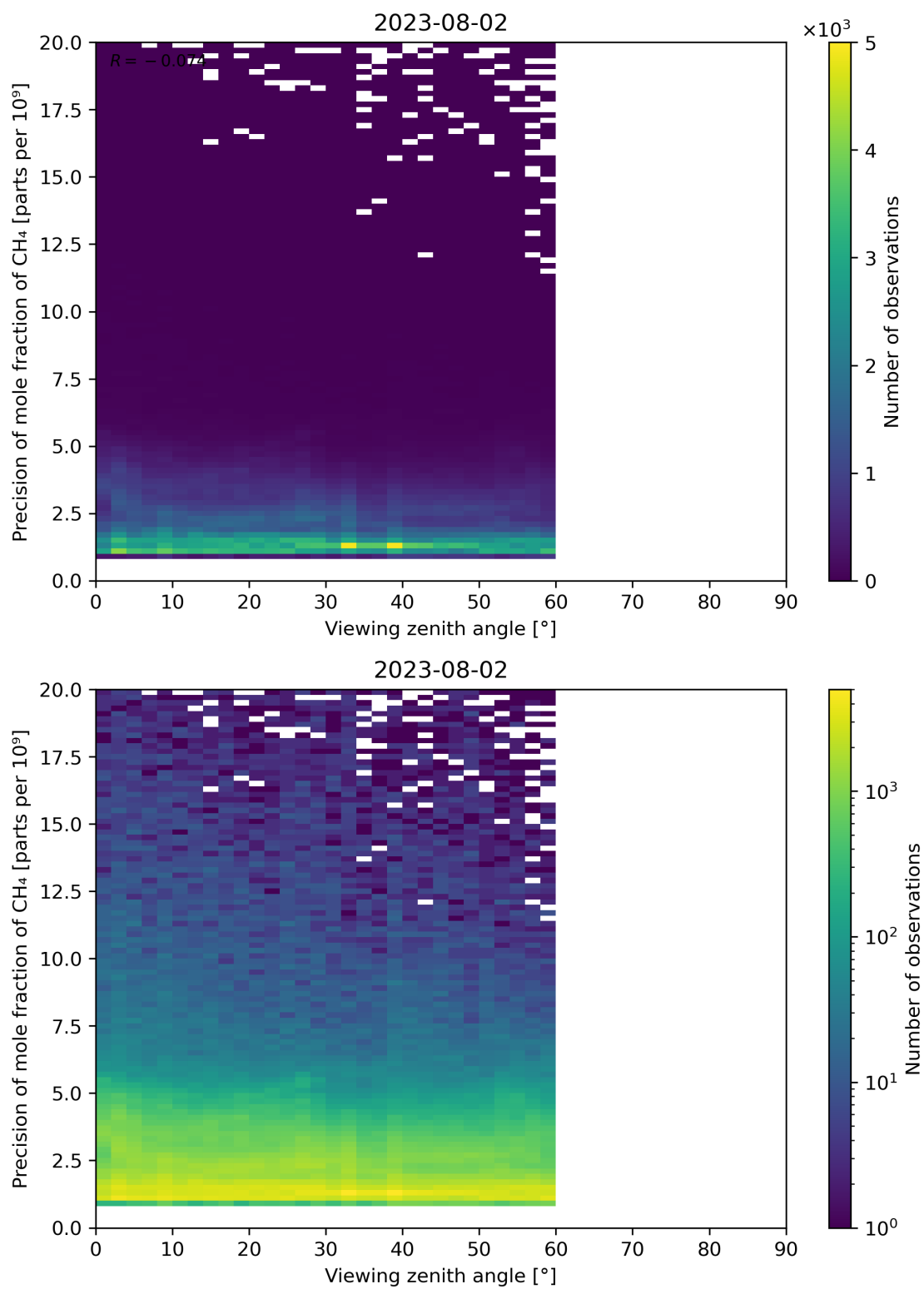
Figure 112: Scatter density plot of “Viewing zenith angle” against “Precision of mole fraction of CH 4 ” for 2023-08-01 to 2023-08-03.
