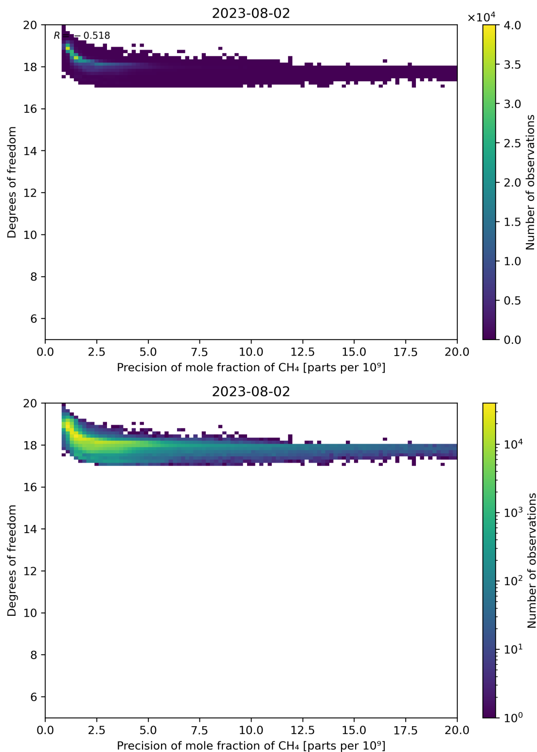
Figure 80: Scatter density plot of “Precision of mole fraction of CH 4 ” against “Degrees of freedom” for 2023-08-01 to 2023-08-03.
