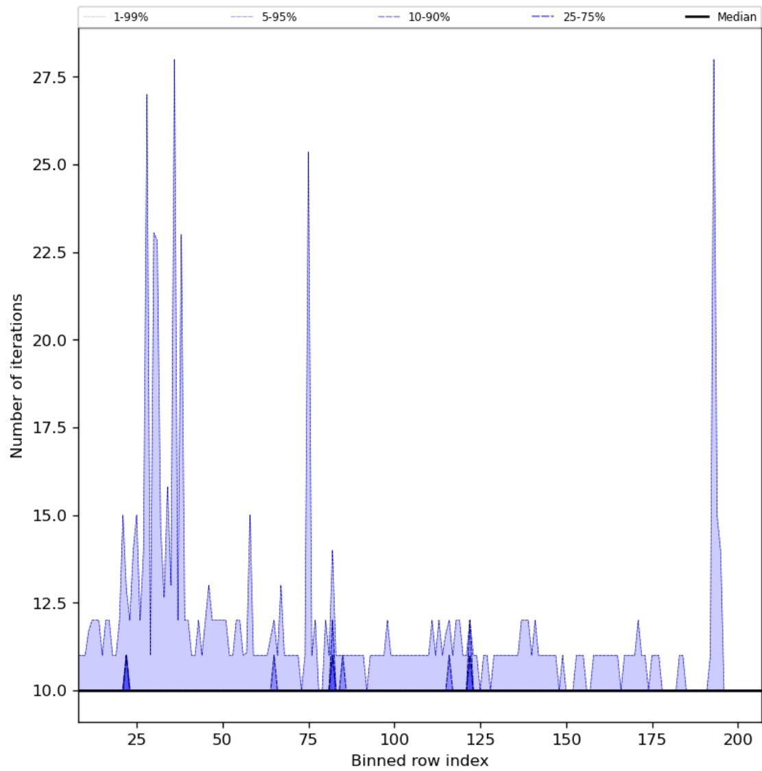
Figure 42: Along track statistics of “Number of iterations” for 2023-08-01 to 2023-08-03
