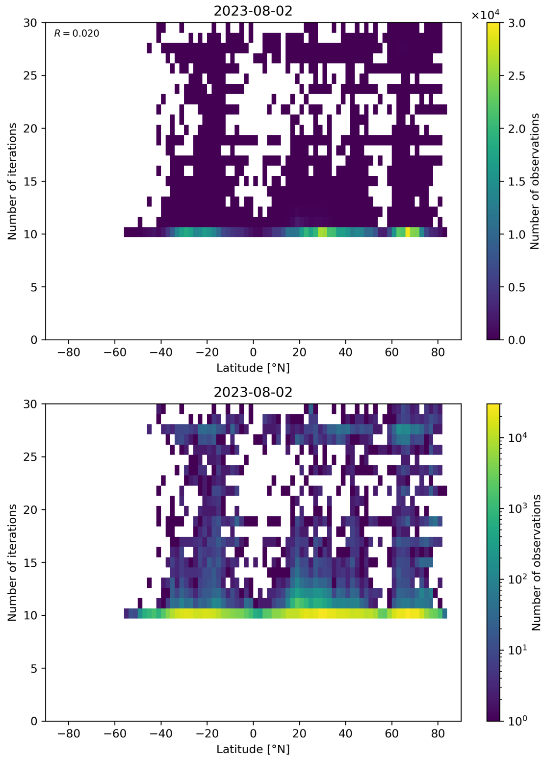
Figure 60: Scatter density plot of “Latitude” against “Number of iterations” for 2023-08-01 to 2023-08-03.
