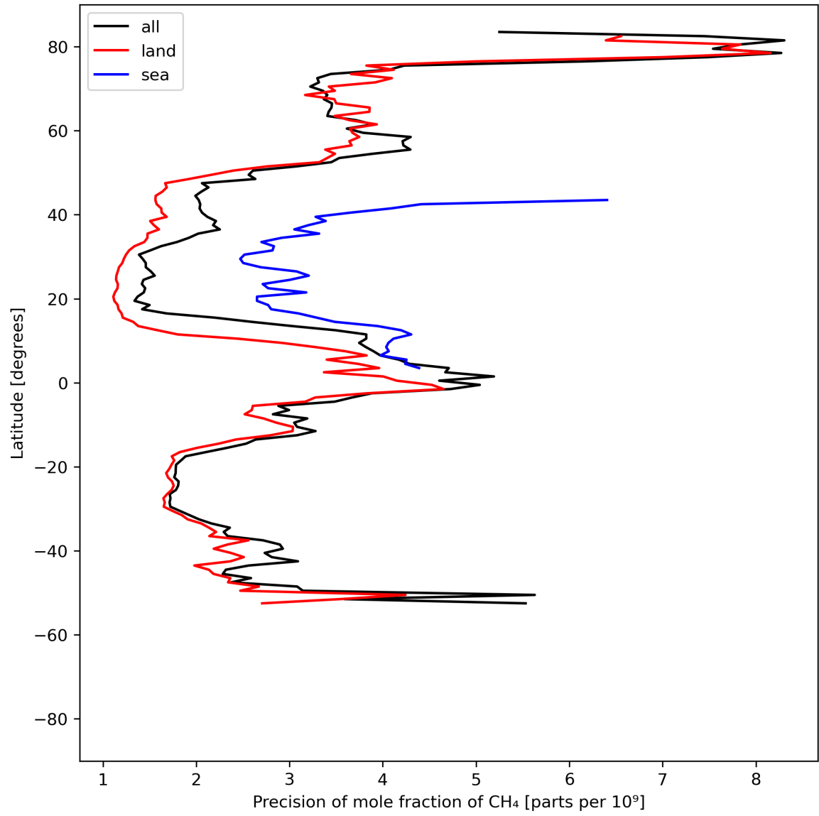
Figure 13: Zonal average of “Precision of mole fraction of CH 4 ” for 2023-08-01 to 2023-08-03.
