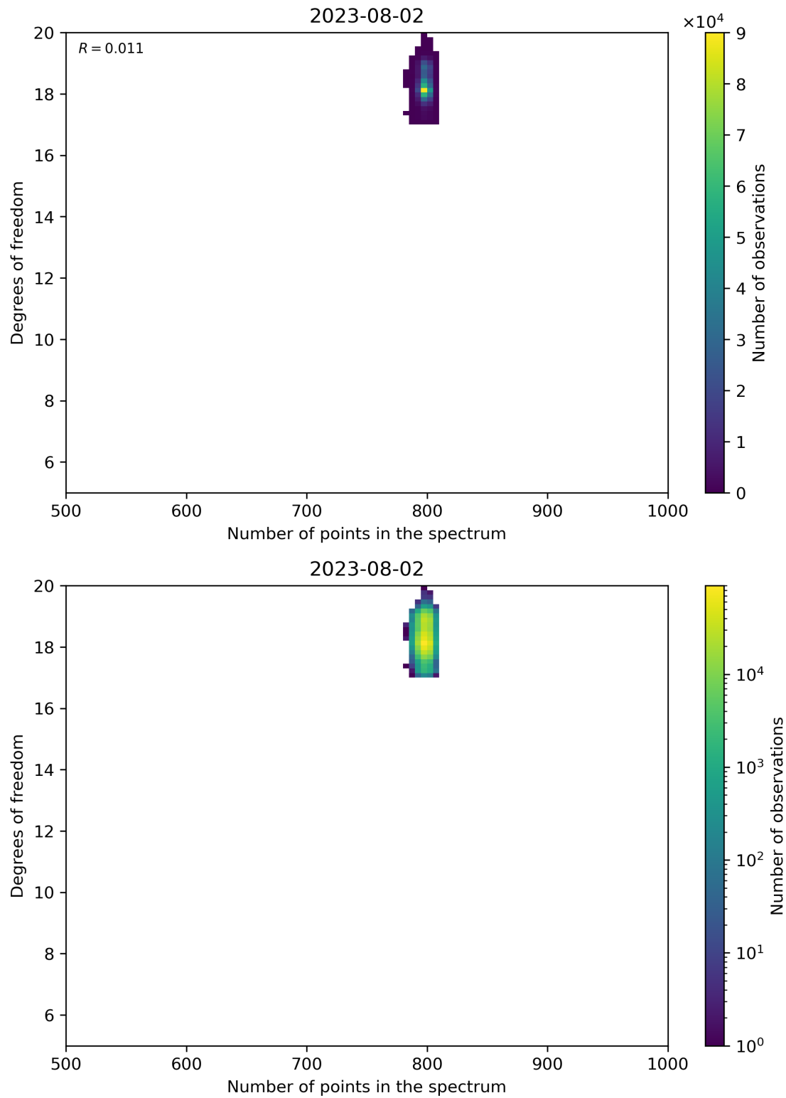
Figure 90: Scatter density plot of “Number of points in the spectrum” against “Degrees of freedom” for 2023-08-01 to 2023-08-03.
