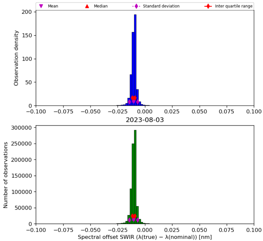
Figure 27: Histogram of “Spectral offset SWIR ( \lambda(\text{true}) - \lambda(\text{nominal}) )” for 2023-08-02 to 2023-08-04
