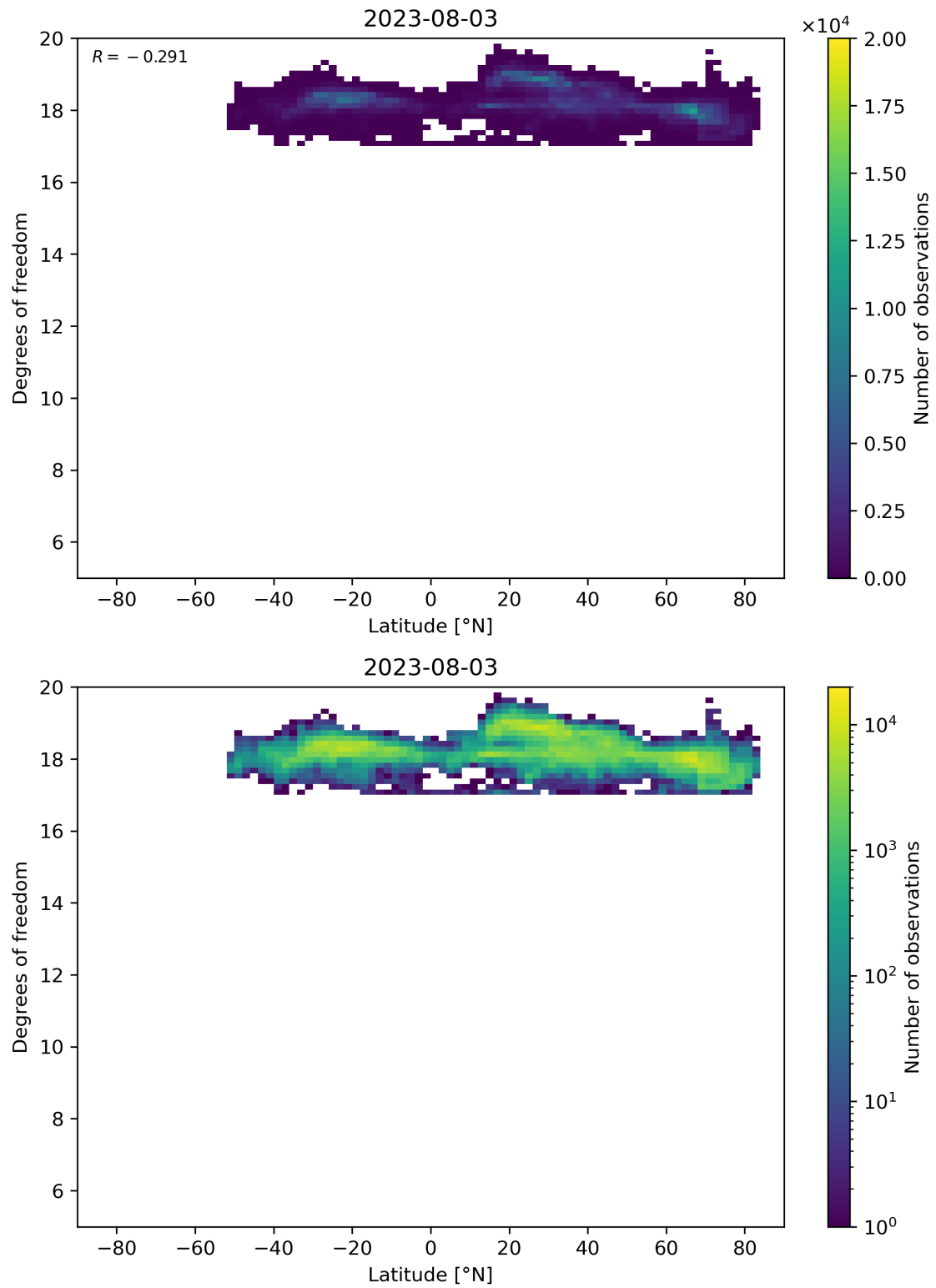
Figure 55: Scatter density plot of “Latitude” against “Degrees of freedom” for 2023-08-02 to 2023-08-04.
