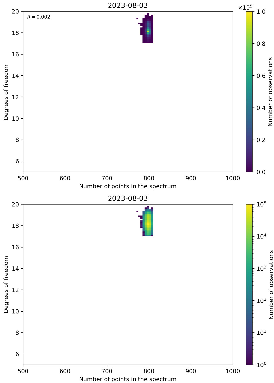
Figure 90: Scatter density plot of “Number of points in the spectrum” against “Degrees of freedom” for 2023-08-02 to 2023-08-04.
