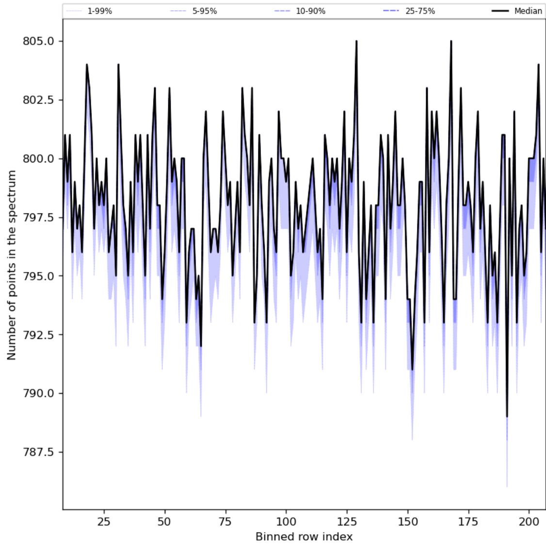
Figure 37: Along track statistics of “Number of points in the spectrum” for 2023-08-02 to 2023-08-04
