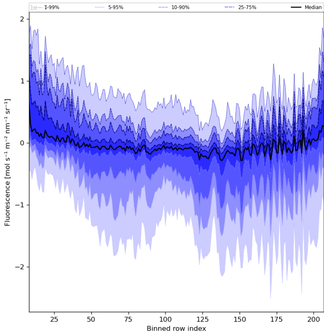
Figure 43: Along track statistics of “Fluorescence” for 2023-08-02 to 2023-08-04
