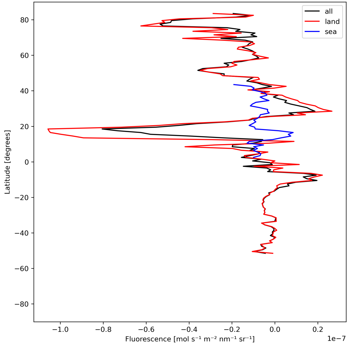
Figure 21: Zonal average of “Fluorescence” for 2023-08-02 to 2023-08-04.
