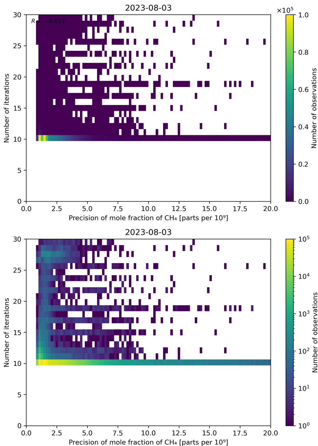
Figure 83: Scatter density plot of “Precision of mole fraction of CH 4 ” against “Number of iterations” for 2023-08-02 to 2023-08-04.
