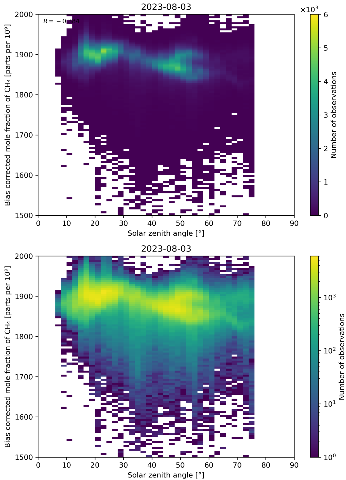
Figure 100: Scatter density plot of “Solar zenith angle” against “Bias corrected mole fraction of CH 4 ” for 2023-08-02 to 2023-08-04.
