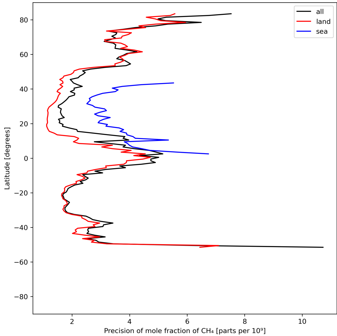
Figure 13: Zonal average of “Precision of mole fraction of CH 4 ” for 2023-08-02 to 2023-08-04.
