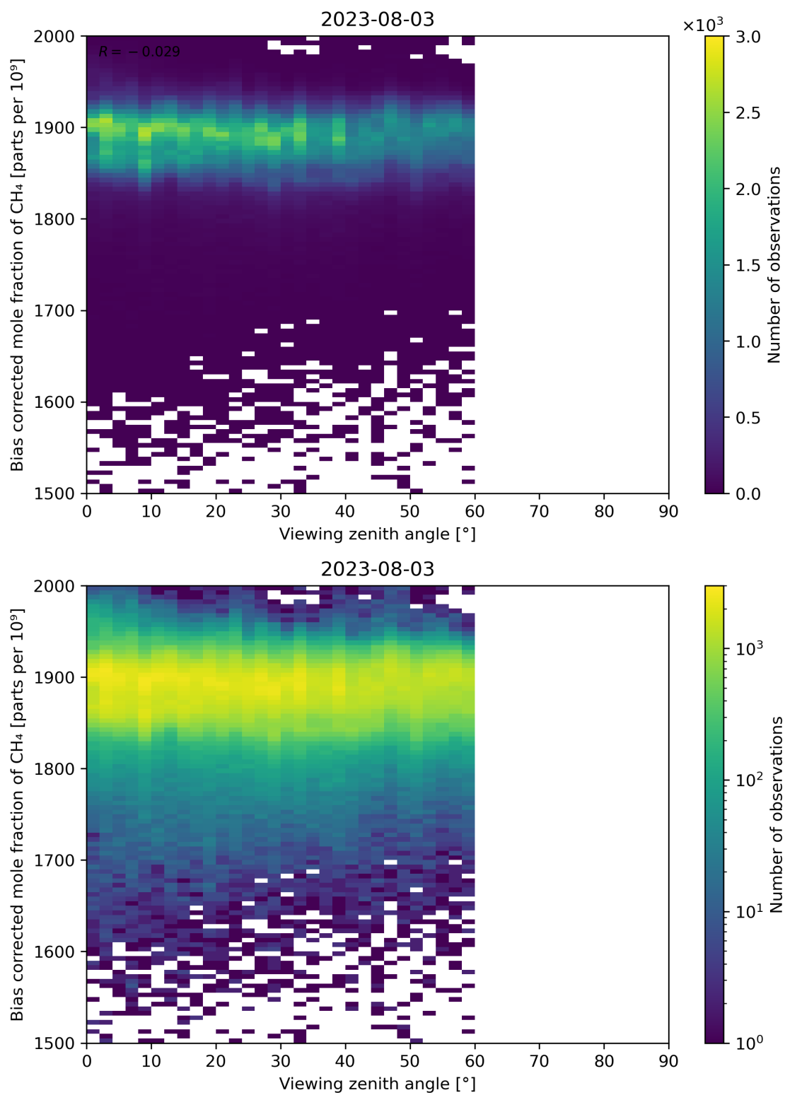
Figure 111: Scatter density plot of “Viewing zenith angle” against “Bias corrected mole fraction of CH 4 ” for 2023-08-02 to 2023-08-04.
