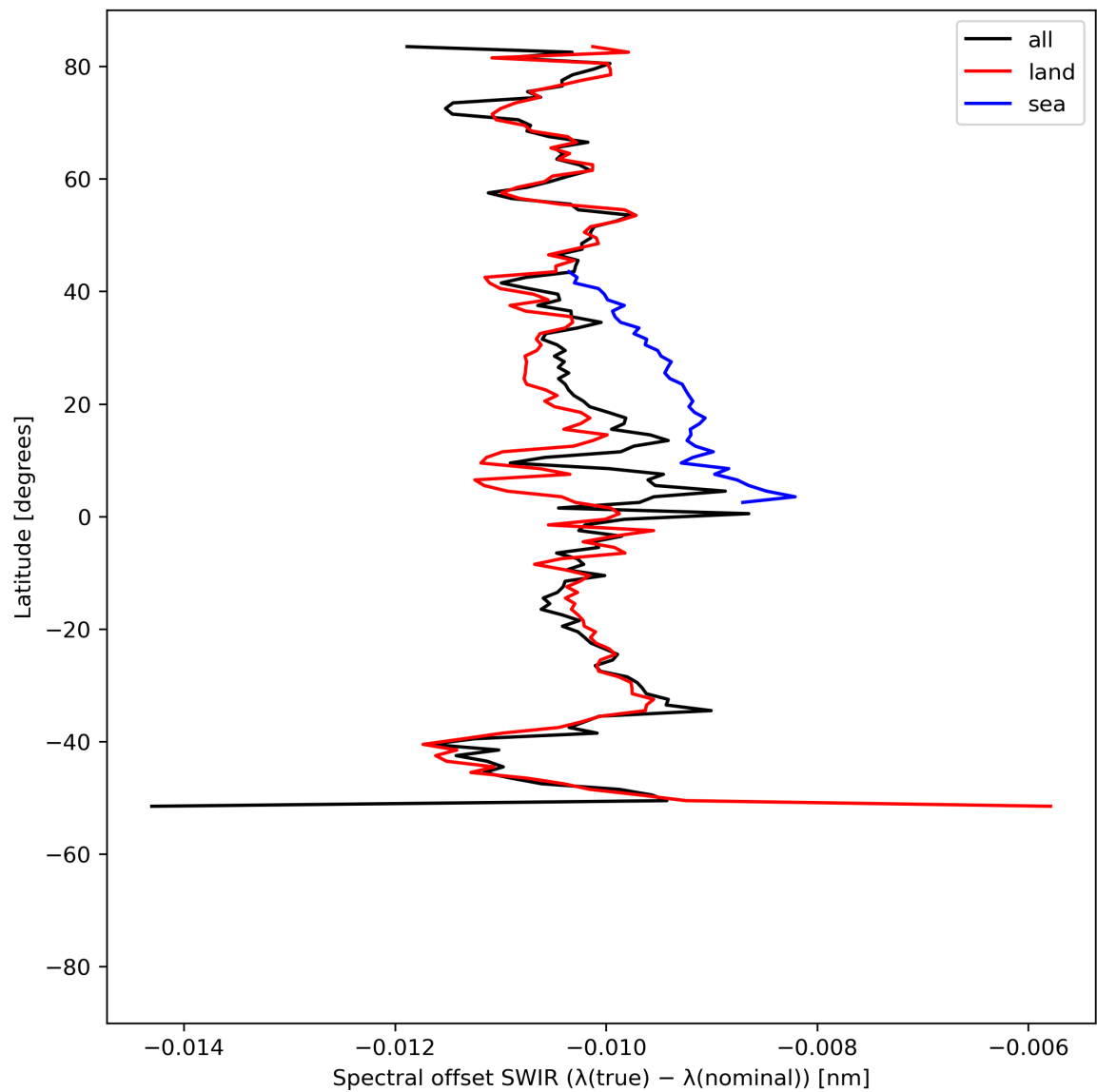
Figure 16: Zonal average of “Spectral offset SWIR ( \lambda(\text{true}) - \lambda(\text{nominal}) )” for 2023-08-02 to 2023-08-04.
