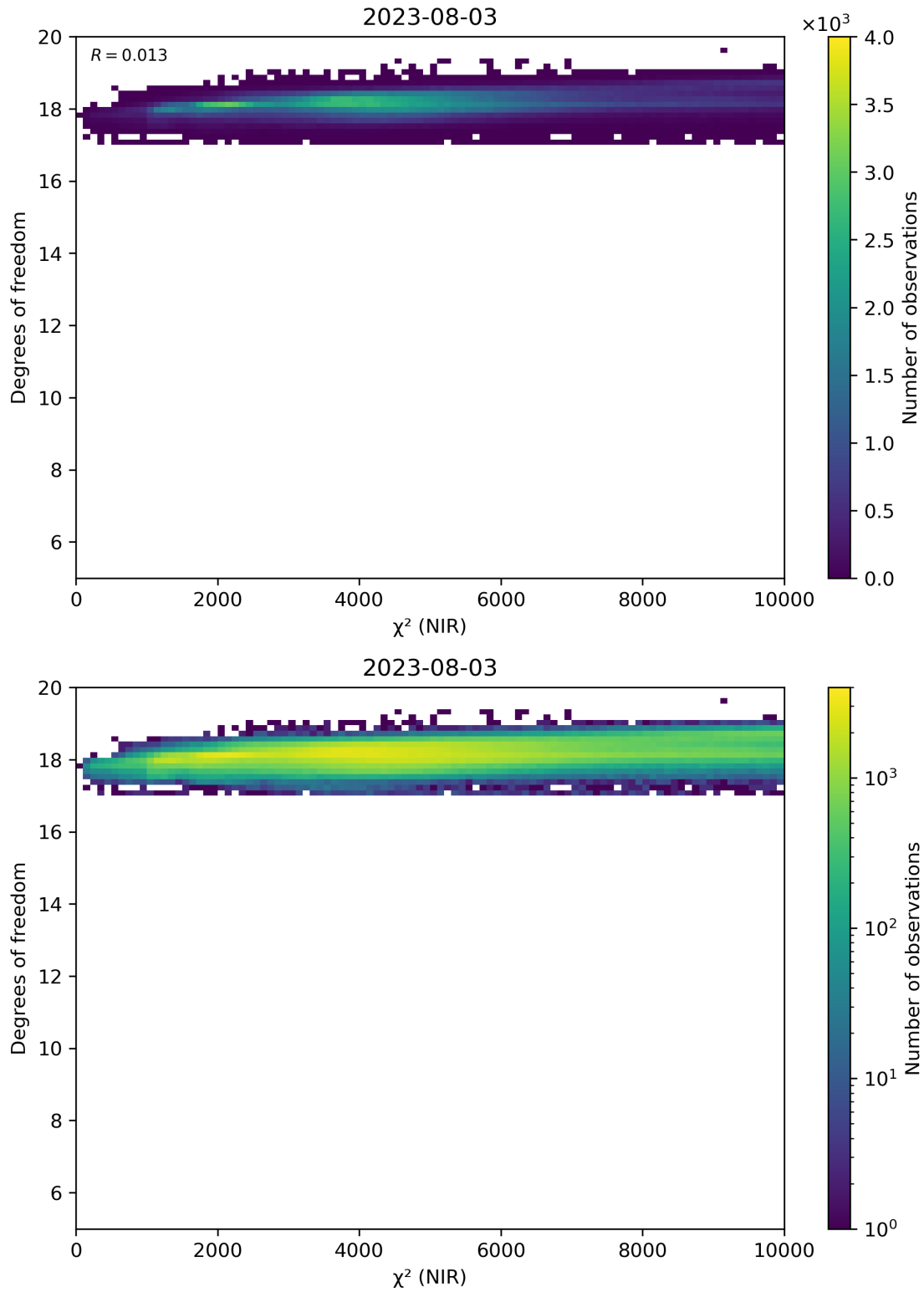
Figure 44: Scatter density plot of “ \chi^2 (NIR)” against “Degrees of freedom” for 2023-08-02 to 2023-08-04.
