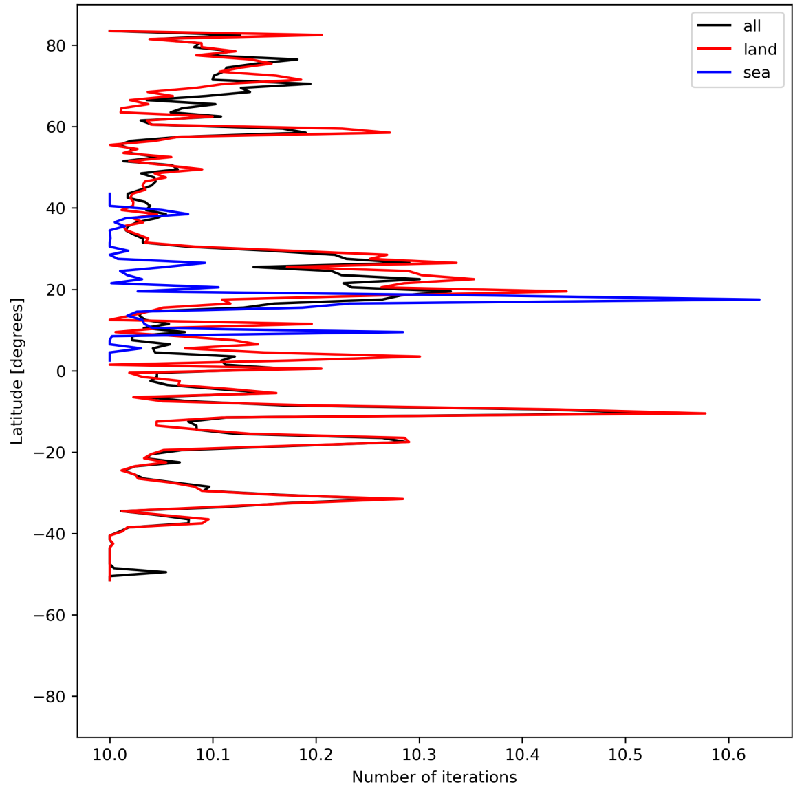
Figure 20: Zonal average of “Number of iterations” for 2023-08-02 to 2023-08-04.
