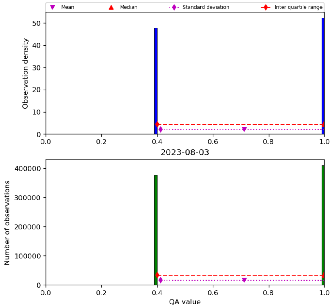
Figure 22: Histogram of “QA value” for 2023-08-02 to 2023-08-04
