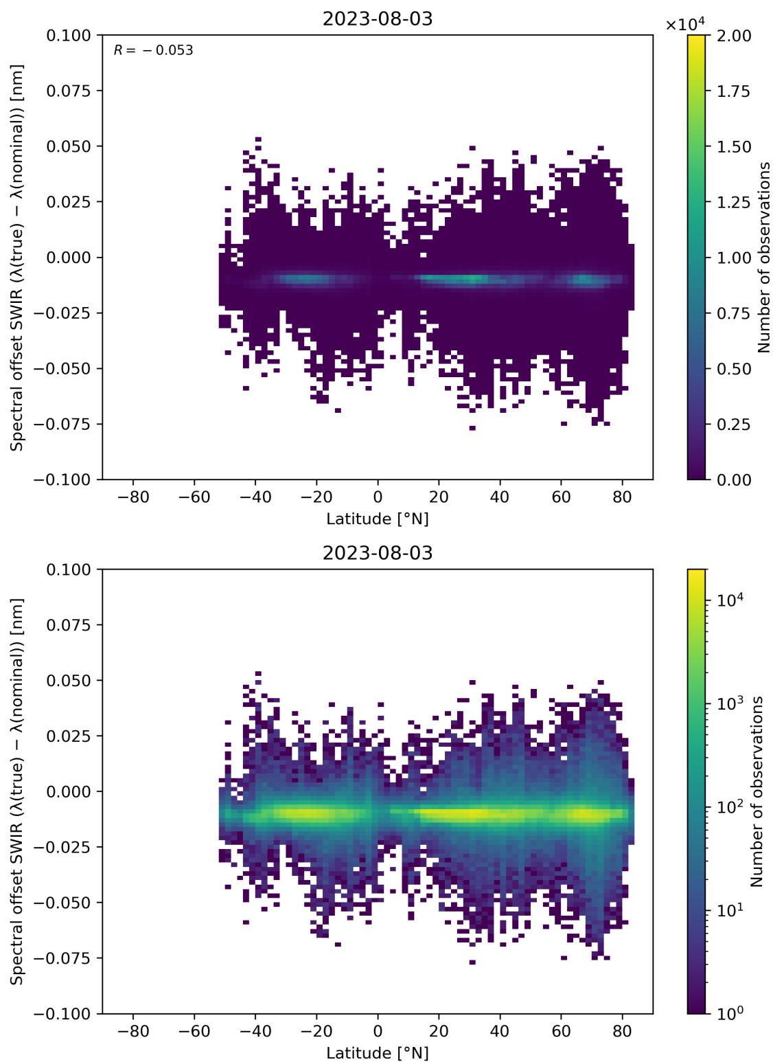
Figure 62: Scatter density plot of “Latitude” against “Spectral offset SWIR ( \lambda(\text{true}) - \lambda(\text{nominal}) )” for 2023-08-02 to 2023-08-04.
