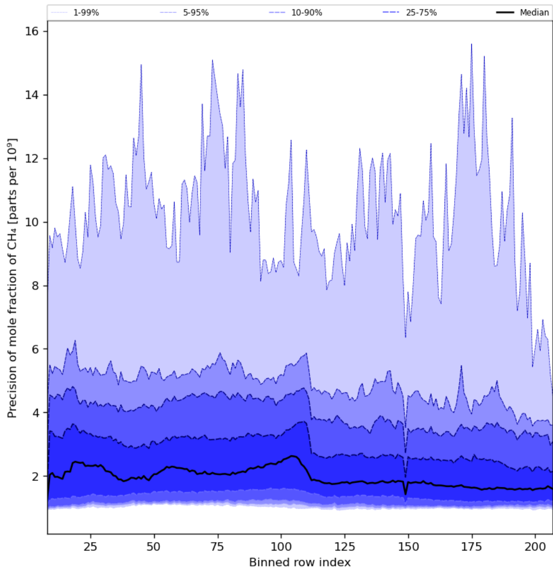
Figure 35: Along track statistics of "Precision of mole fraction of CH 4 " for 2023-08-02 to 2023-08-04
