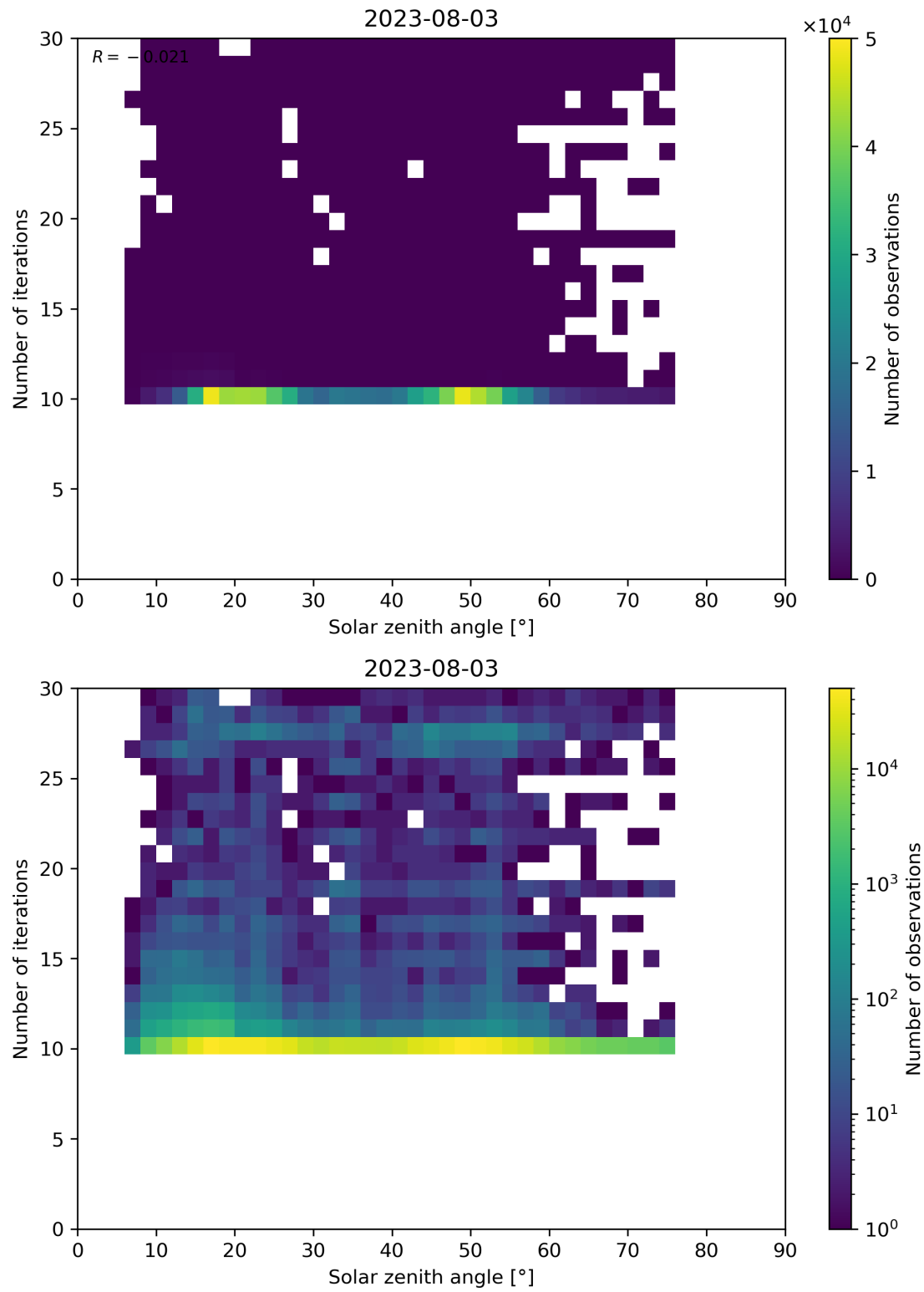
Figure 102: Scatter density plot of “Solar zenith angle” against “Number of iterations” for 2023-08-02 to 2023-08-04.
