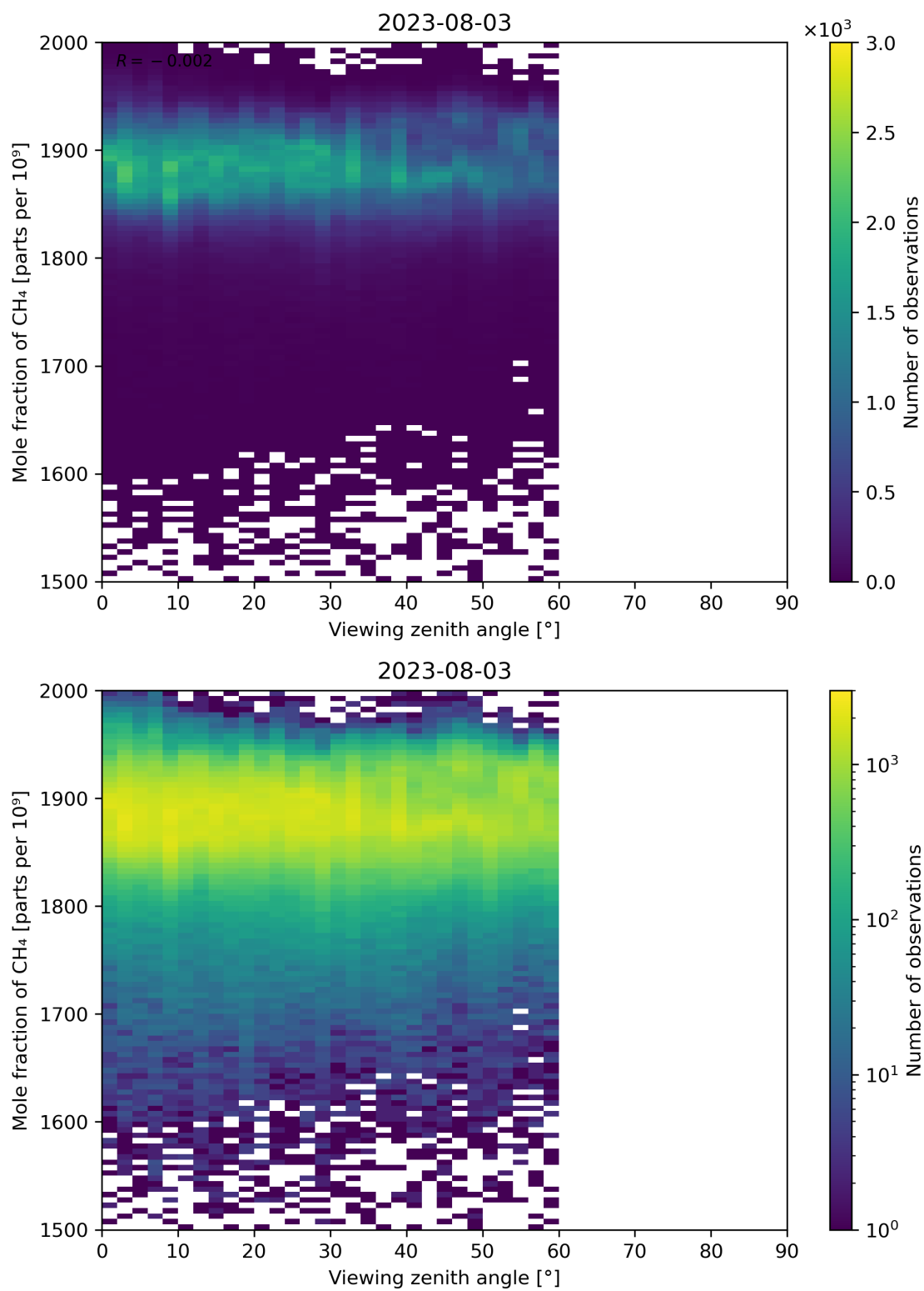
Figure 110: Scatter density plot of “Viewing zenith angle” against “Mole fraction of CH 4 ” for 2023-08-02 to 2023-08-04.
