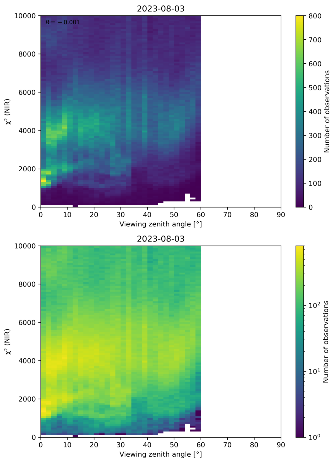
Figure 105: Scatter density plot of “Viewing zenith angle” against “ \chi^2 (NIR)” for 2023-08-02 to 2023-08-04.
