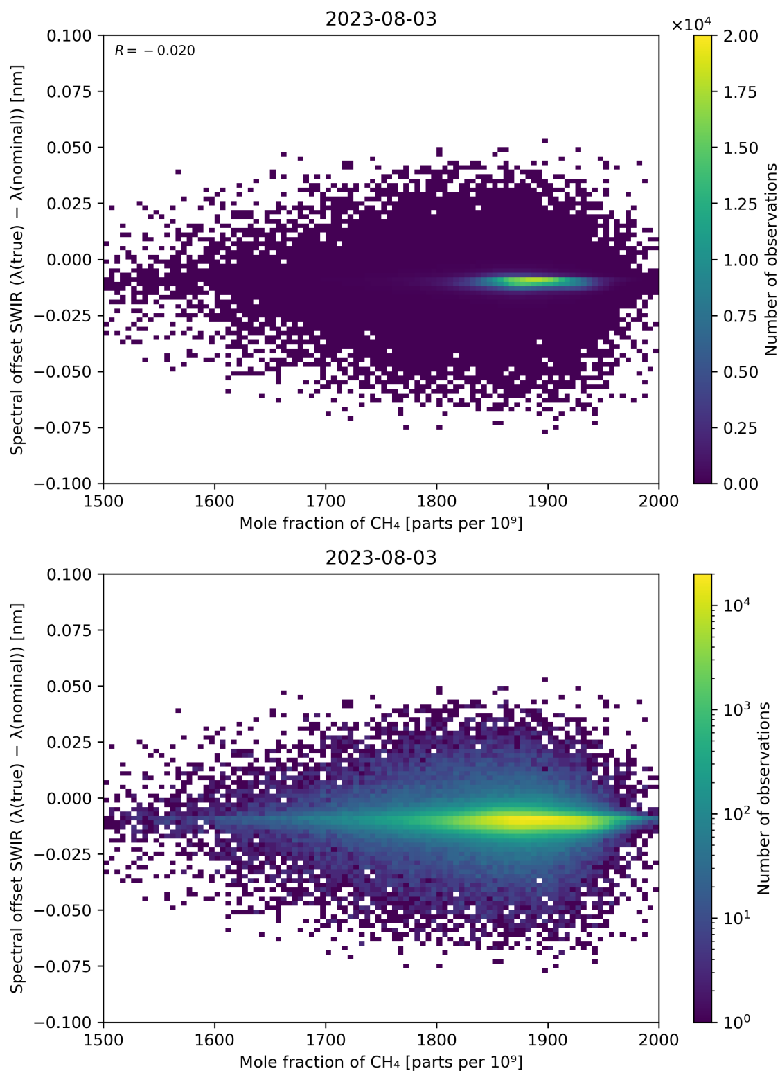
Figure 86: Scatter density plot of “Mole fraction of CH 4 ” against “Spectral offset SWIR ( \lambda(\text{true}) - \lambda(\text{nominal}) )” for 2023-08-02 to 2023-08-04.
