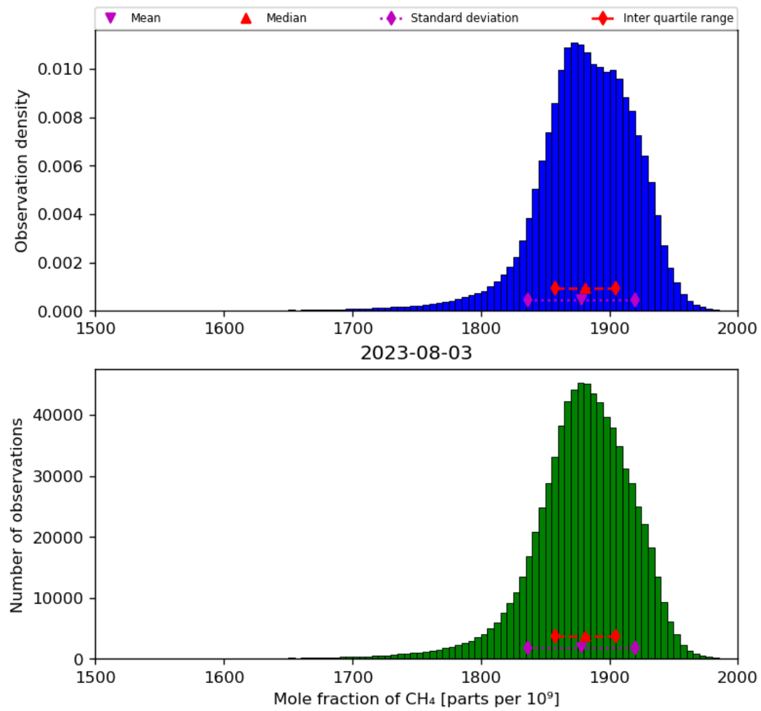
Figure 23: Histogram of “Mole fraction of CH 4 ” for 2023-08-02 to 2023-08-04
