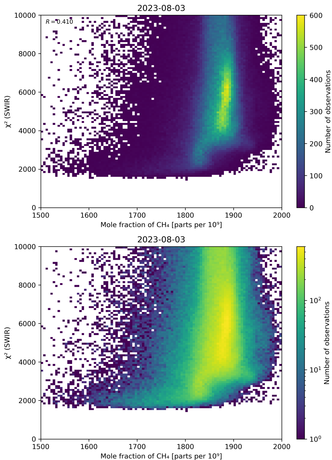
Figure 71: Scatter density plot of “Mole fraction of \text{CH}_4 ” against “ \chi^2 (SWIR)” for 2023-08-02 to 2023-08-04.
