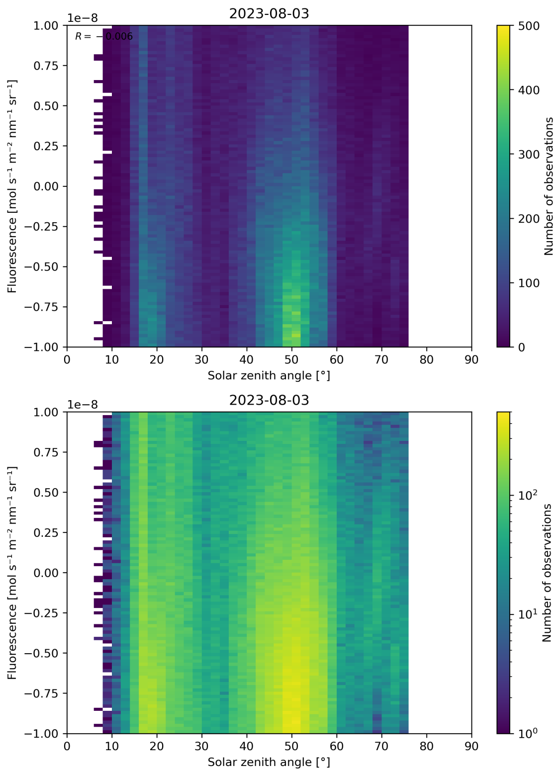
Figure 97: Scatter density plot of “Solar zenith angle” against “Fluorescence” for 2023-08-02 to 2023-08-04.
