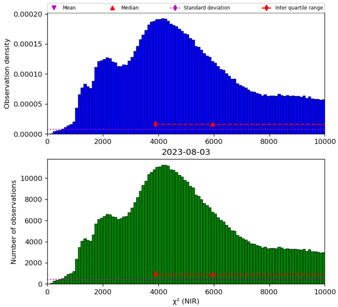
Figure 29: Histogram of “ \chi^2 (NIR)” for 2023-08-02 to 2023-08-04
