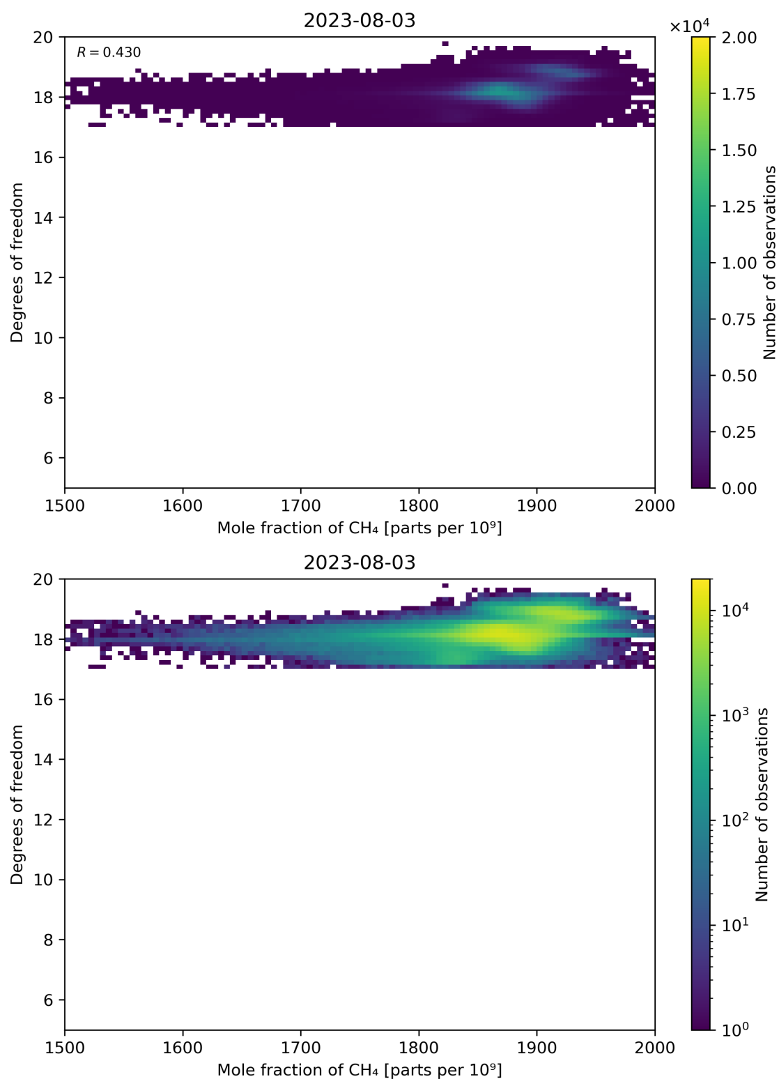
Figure 72: Scatter density plot of “Mole fraction of CH 4 ” against “Degrees of freedom” for 2023-08-02 to 2023-08-04.
