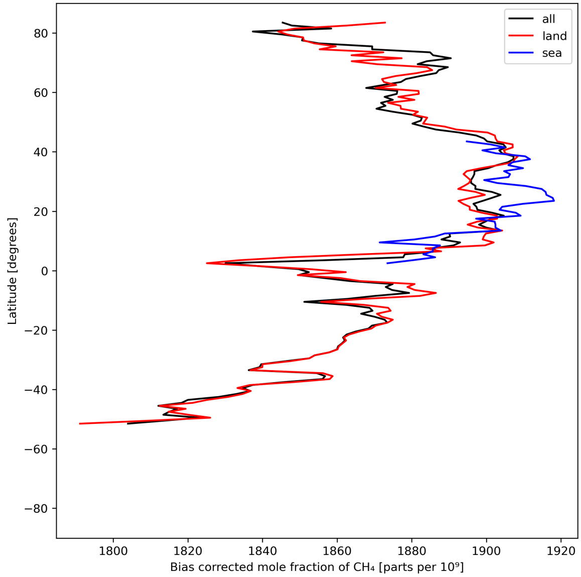
Figure 14: Zonal average of “Bias corrected mole fraction of CH 4 ” for 2023-08-02 to 2023-08-04.
