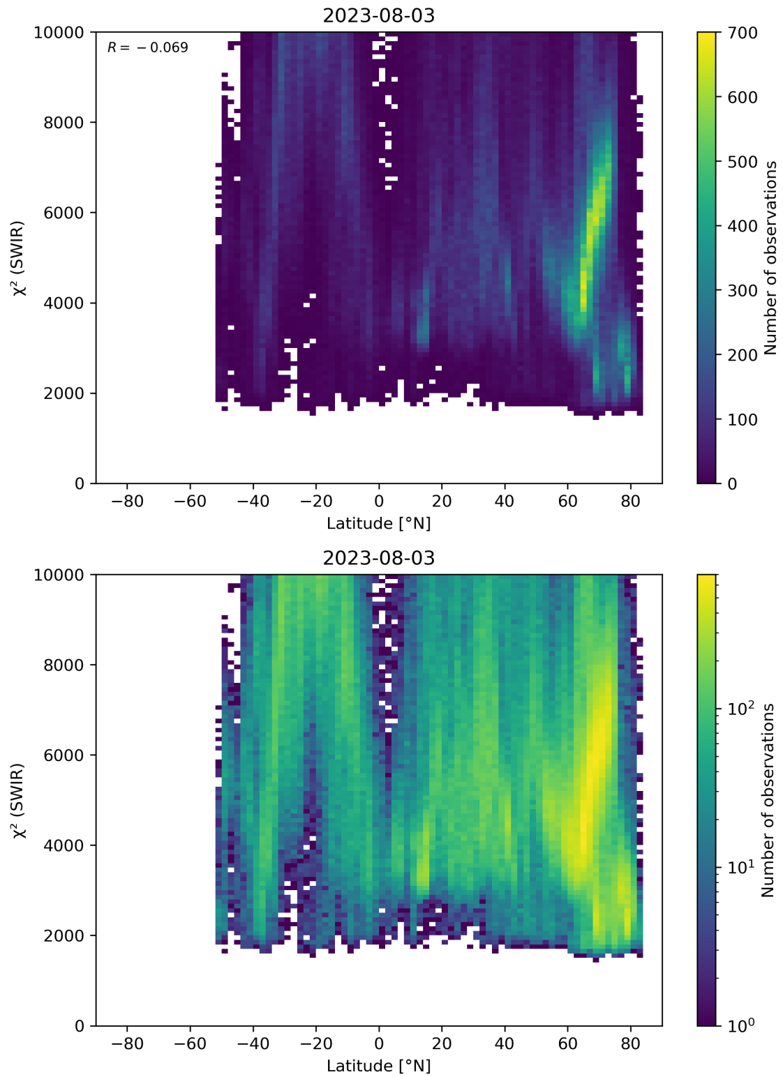
Figure 54: Scatter density plot of “Latitude” against “ \chi^2 (SWIR)” for 2023-08-02 to 2023-08-04.
