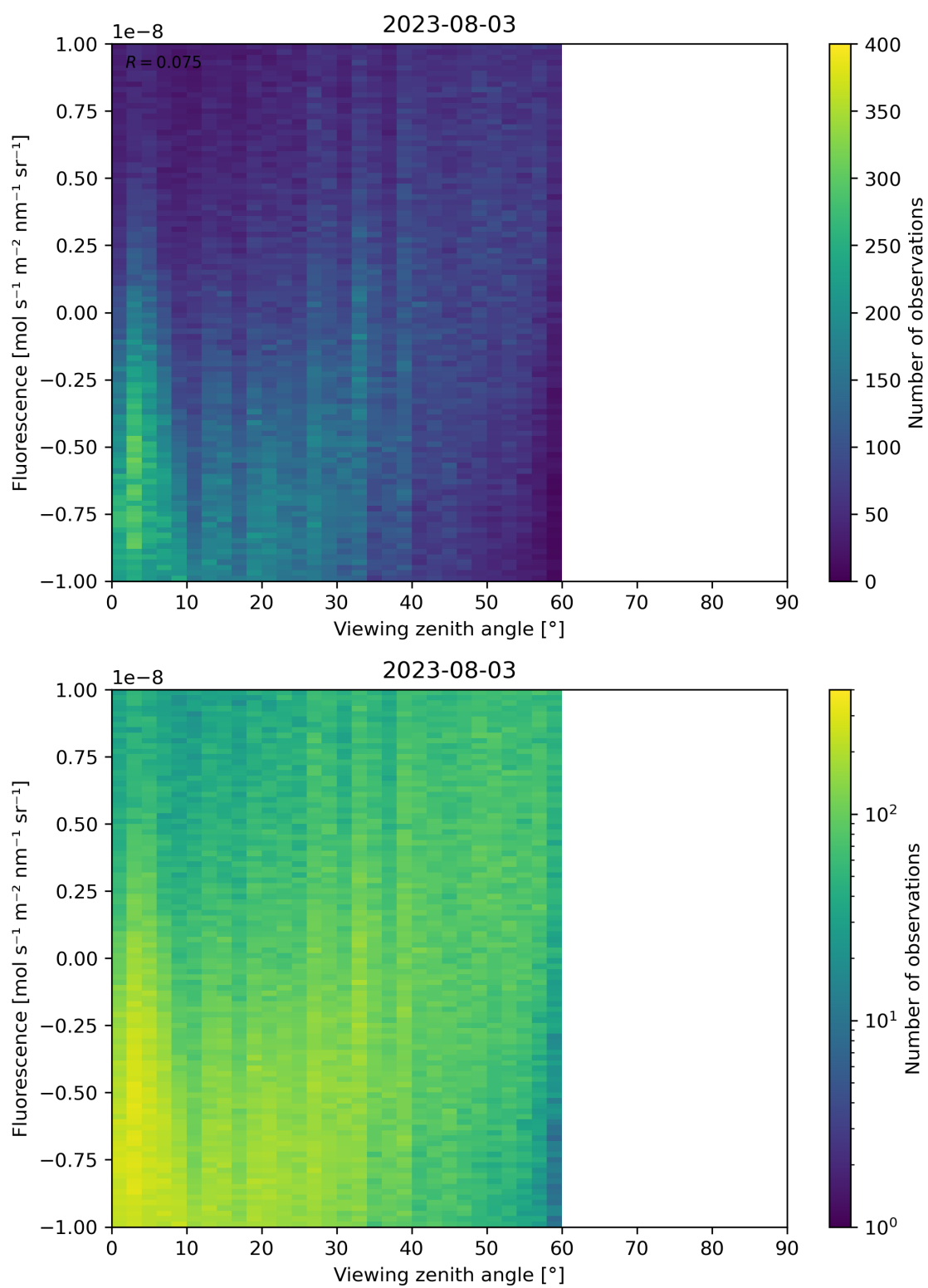
Figure 108: Scatter density plot of “Viewing zenith angle” against “Fluorescence” for 2023-08-02 to 2023-08-04.
