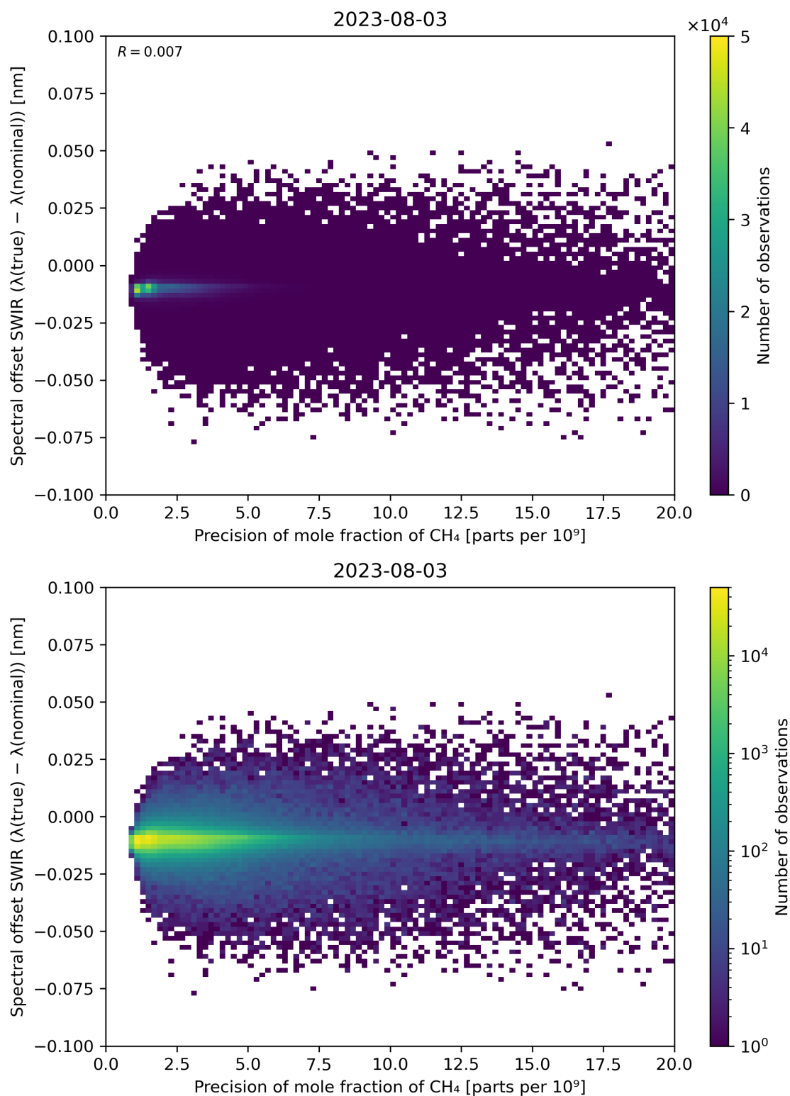
Figure 85: Scatter density plot of “Precision of mole fraction of CH 4 ” against “Spectral offset SWIR ( \lambda(\text{true}) - \lambda(\text{nominal}) )” for 2023-08-02 to 2023-08-04.
