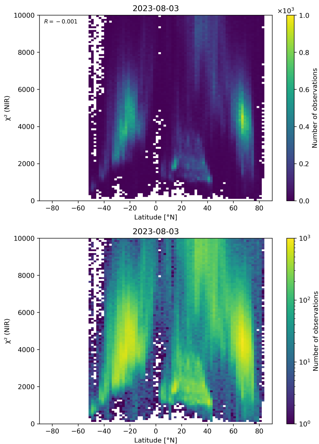
Figure 53: Scatter density plot of “Latitude” against “ \chi^2 (NIR)” for 2023-08-02 to 2023-08-04.
