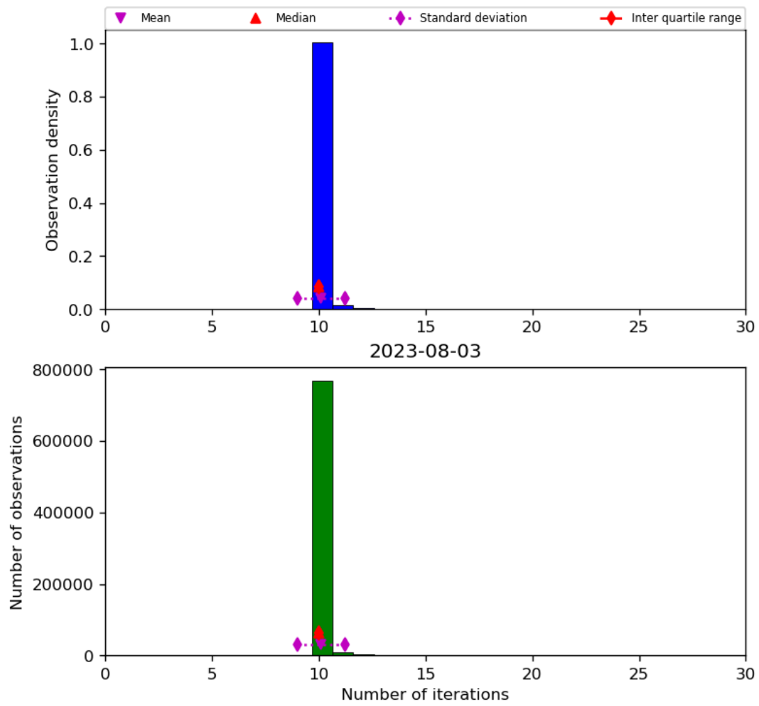
Figure 31: Histogram of “Number of iterations” for 2023-08-02 to 2023-08-04
