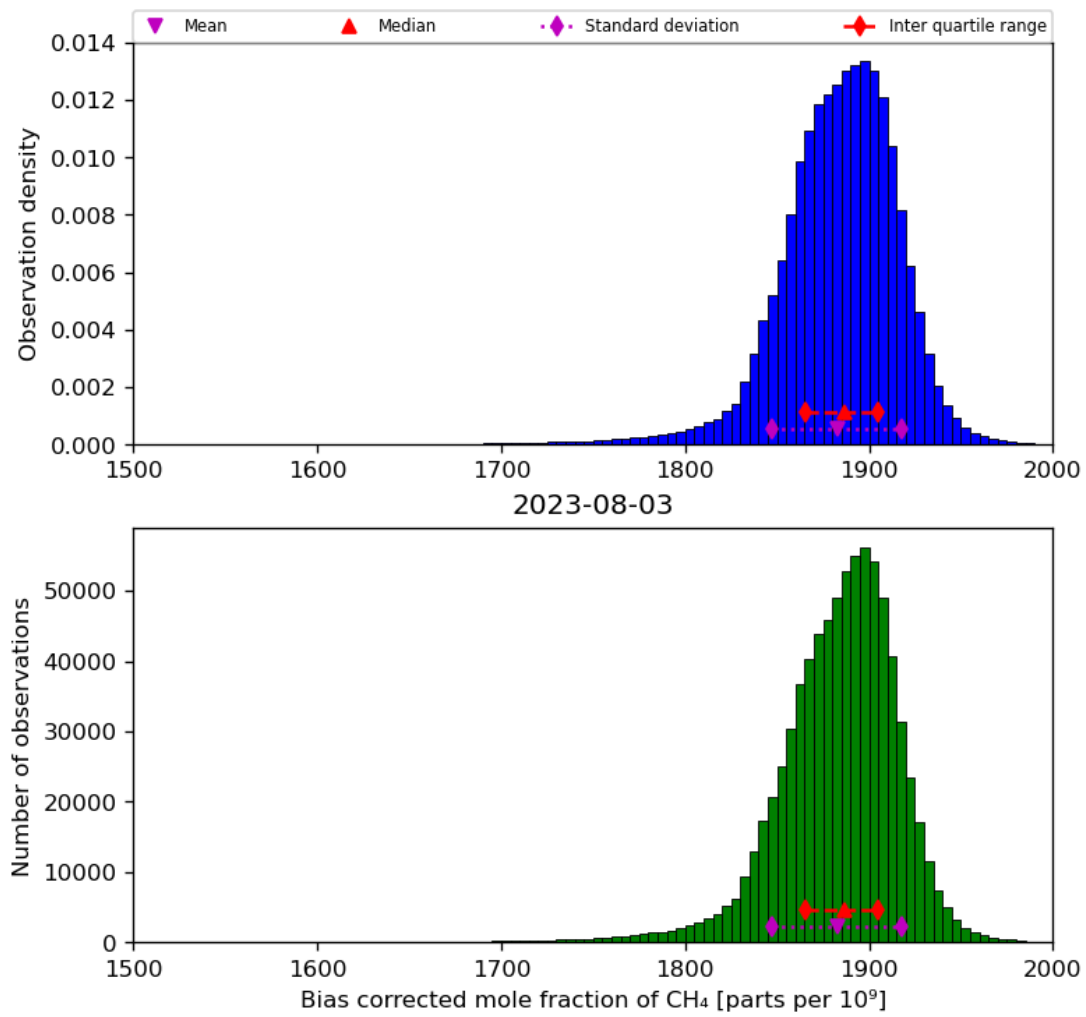
Figure 25: Histogram of “Bias corrected mole fraction of CH 4 ” for 2023-08-02 to 2023-08-04
