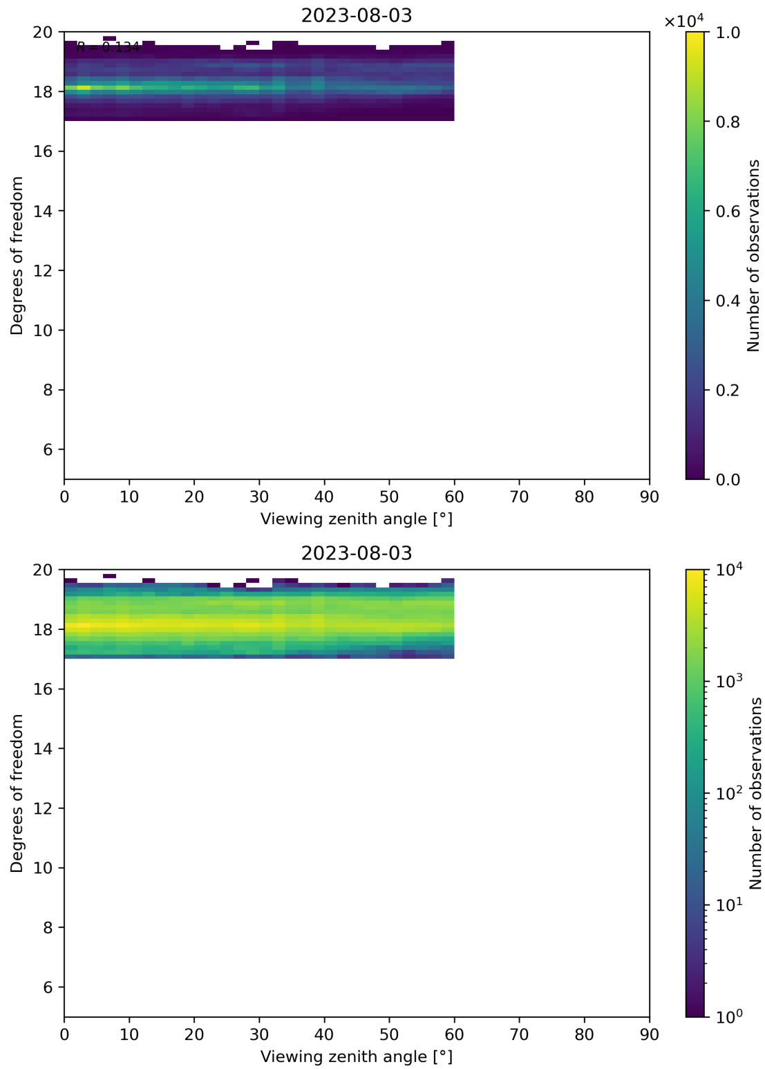
Figure 107: Scatter density plot of “Viewing zenith angle” against “Degrees of freedom” for 2023-08-02 to 2023-08-04.
