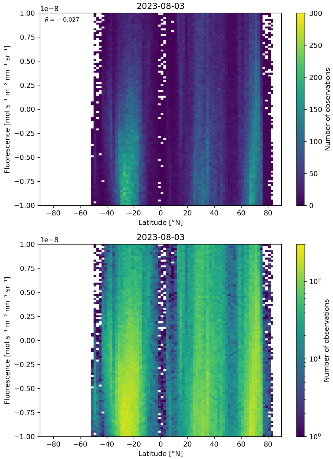
Figure 56: Scatter density plot of “Latitude” against “Fluorescence” for 2023-08-02 to 2023-08-04.
