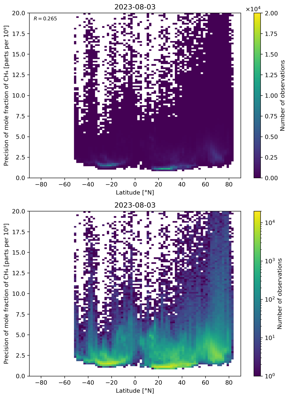
Figure 59: Scatter density plot of “Latitude” against “Precision of mole fraction of \text{CH}_4 ” for 2023-08-02 to 2023-08-04.
