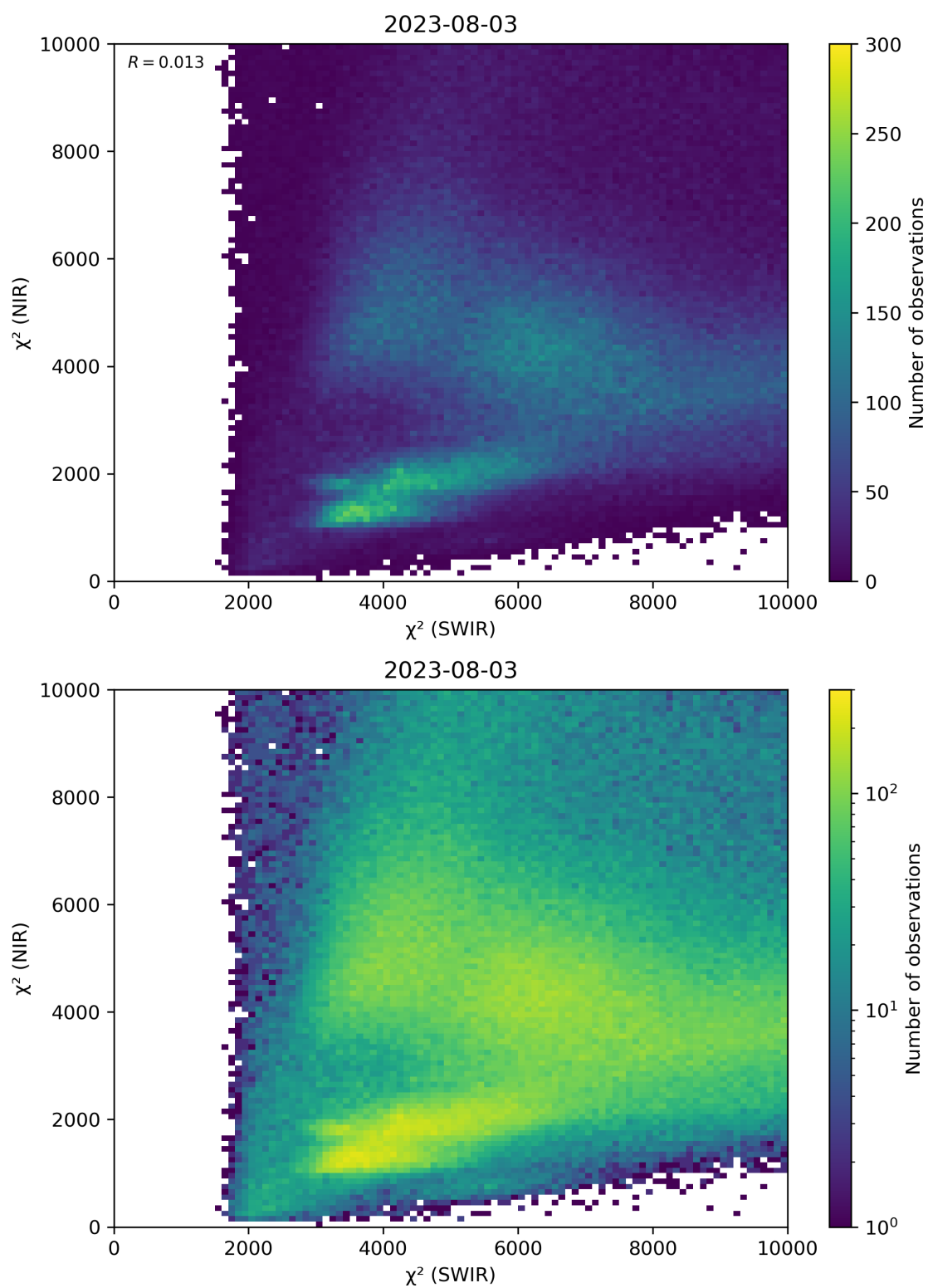
Figure 47: Scatter density plot of “ \chi^2 (SWIR)” against “ \chi^2 (NIR)” for 2023-08-02 to 2023-08-04.
