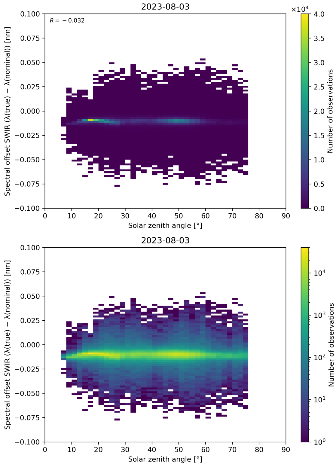
Figure 104: Scatter density plot of “Solar zenith angle” against “Spectral offset SWIR ( \lambda(\text{true}) - \lambda(\text{nominal}) )” for 2023-08-02 to 2023-08-04.
