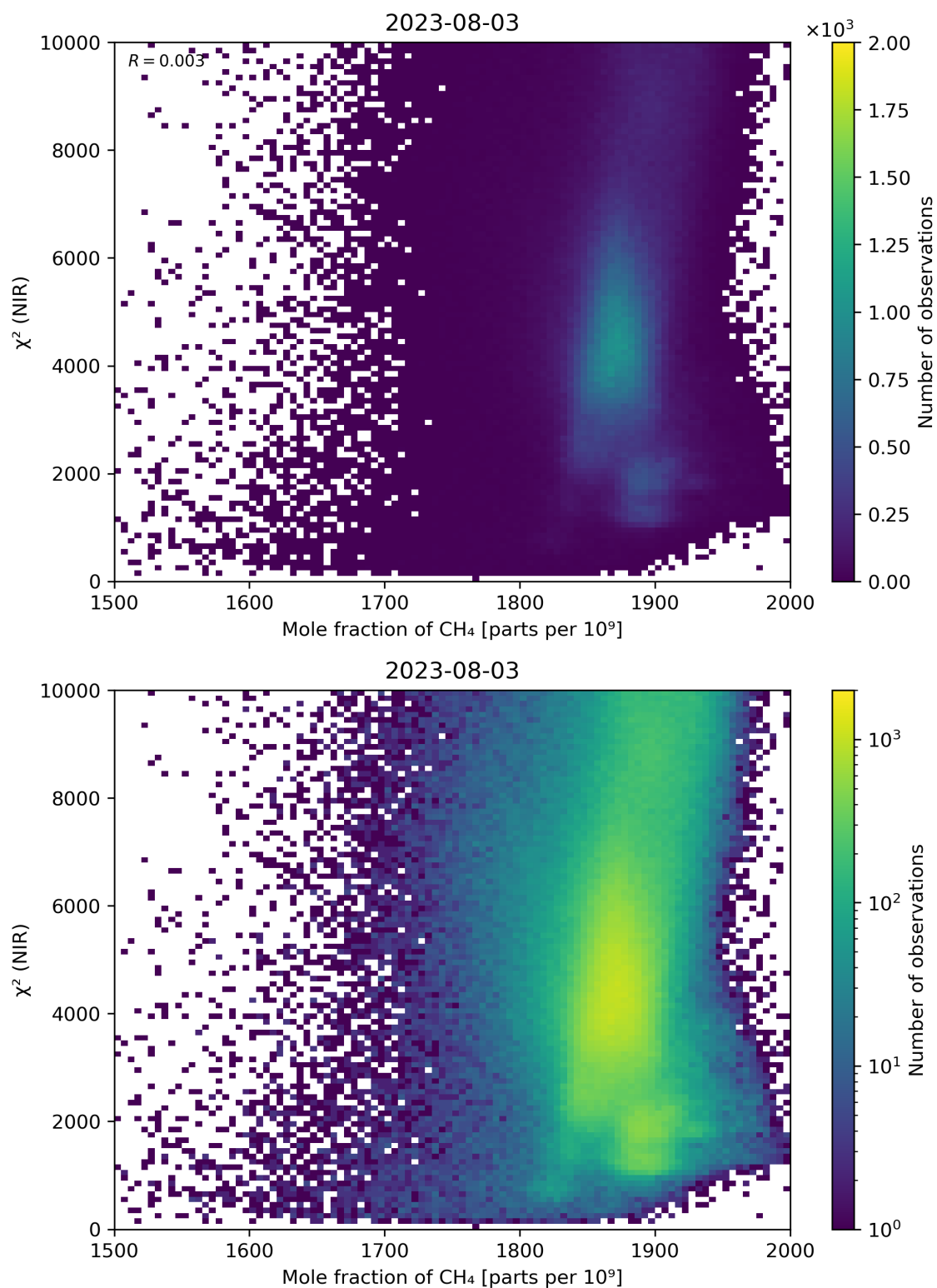
Figure 70: Scatter density plot of “Mole fraction of \text{CH}_4 ” against “ \chi^2 (NIR)” for 2023-08-02 to 2023-08-04.
