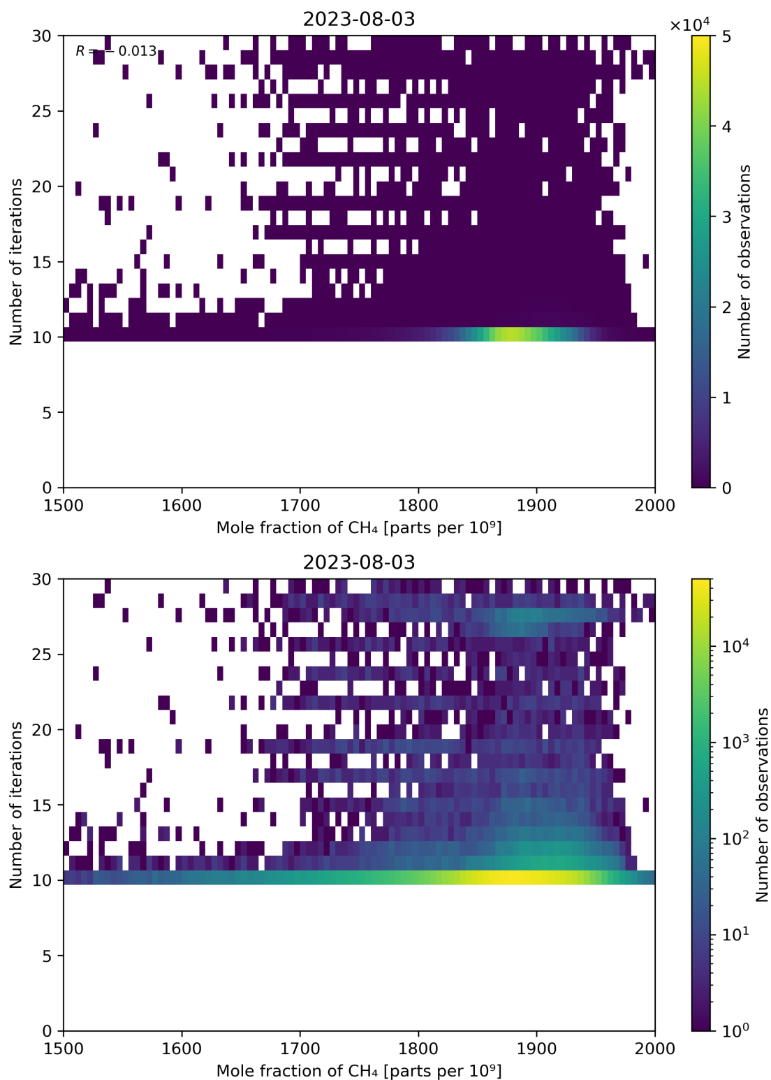
Figure 76: Scatter density plot of “Mole fraction of CH 4 ” against “Number of iterations” for 2023-08-02 to 2023-08-04.
