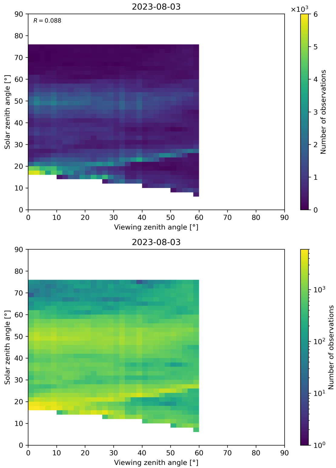
Figure 115: Scatter density plot of “Viewing zenith angle” against “Solar zenith angle” for 2023-08-02 to 2023-08-04.
