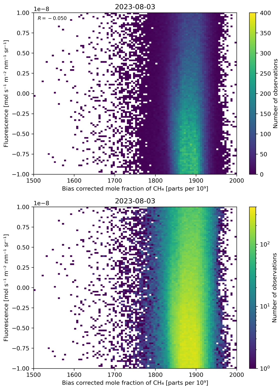
Figure 66: Scatter density plot of “Bias corrected mole fraction of \text{CH}_4 ” against “Fluorescence” for 2023-08-02 to 2023-08-04.
