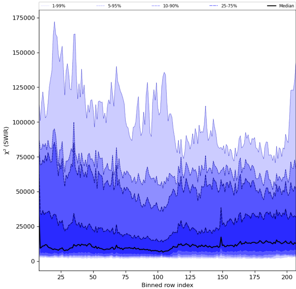
Figure 39: Along track statistics of “ \chi^2 (SWIR)” for 2023-08-02 to 2023-08-04
