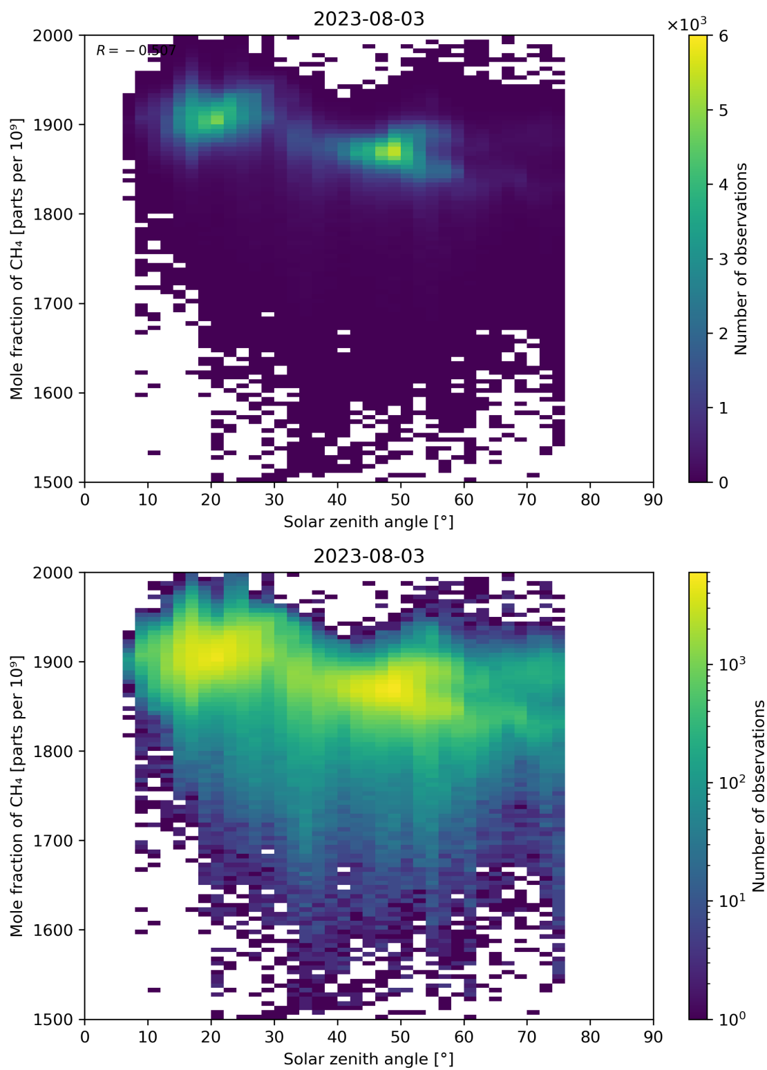
Figure 99: Scatter density plot of “Solar zenith angle” against “Mole fraction of CH 4 ” for 2023-08-02 to 2023-08-04.
