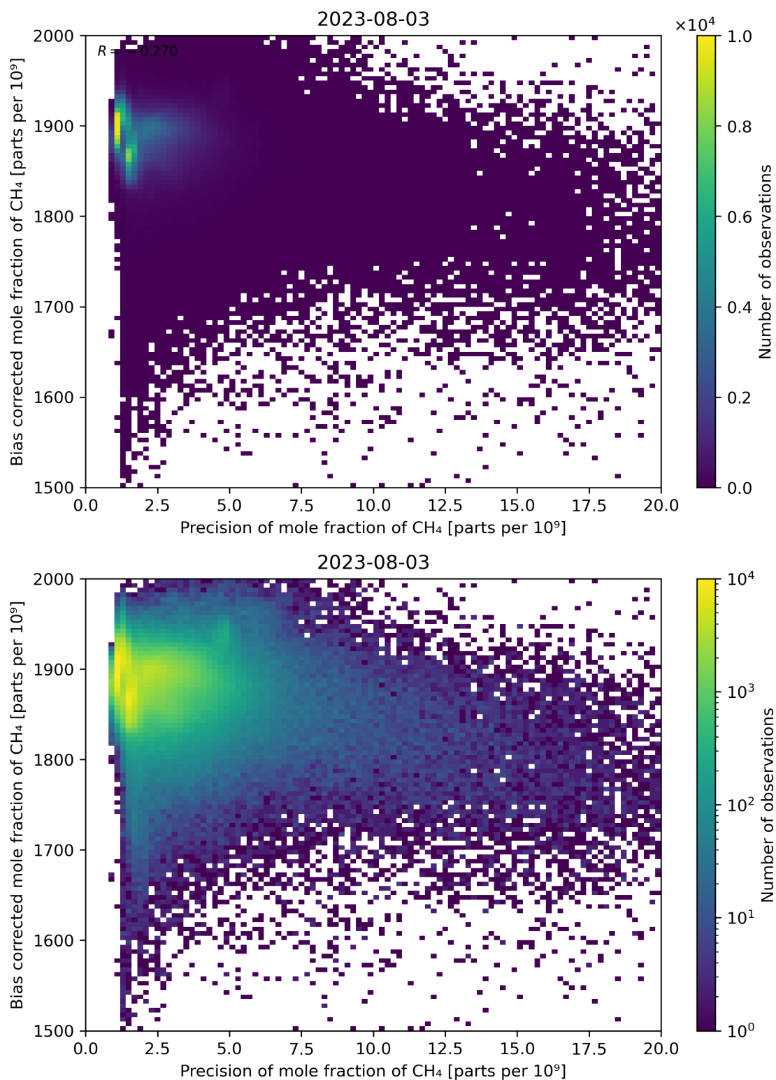
Figure 82: Scatter density plot of “Precision of mole fraction of CH 4 ” against “Bias corrected mole fraction of CH 4 ” for 2023-08-02 to 2023-08-04.
