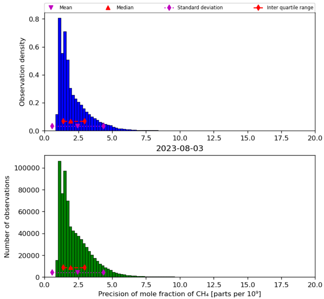
Figure 24: Histogram of “Precision of mole fraction of CH 4 ” for 2023-08-02 to 2023-08-04
