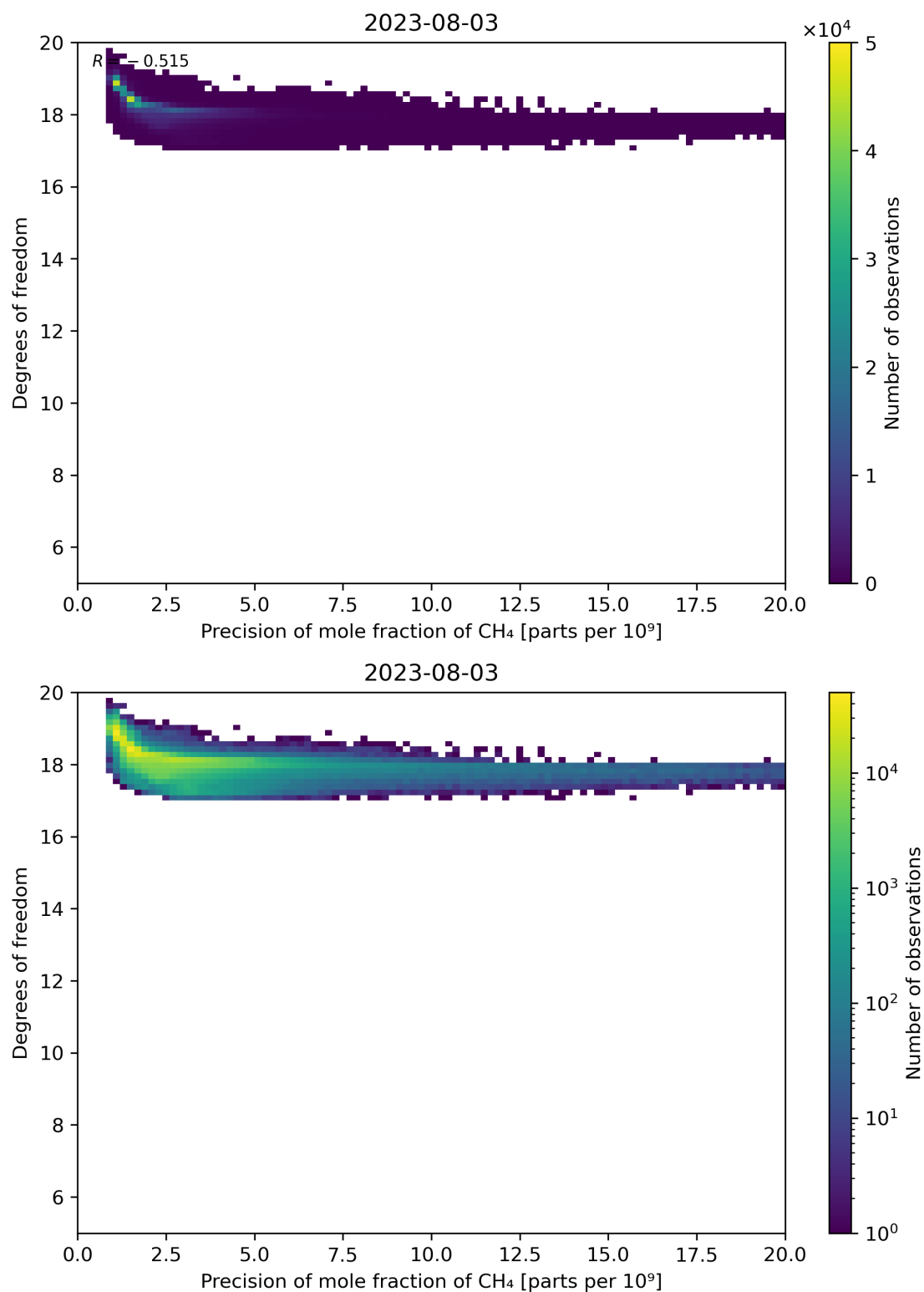
Figure 80: Scatter density plot of “Precision of mole fraction of CH 4 ” against “Degrees of freedom” for 2023-08-02 to 2023-08-04.
