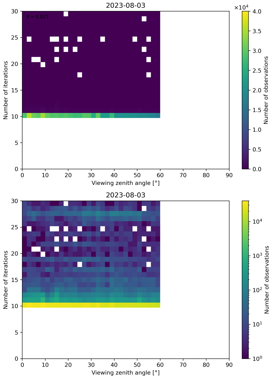
Figure 113: Scatter density plot of “Viewing zenith angle” against “Number of iterations” for 2023-08-02 to 2023-08-04.
