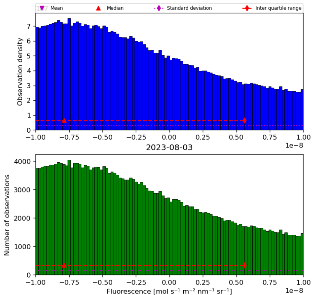
Figure 32: Histogram of “Fluorescence” for 2023-08-02 to 2023-08-04
