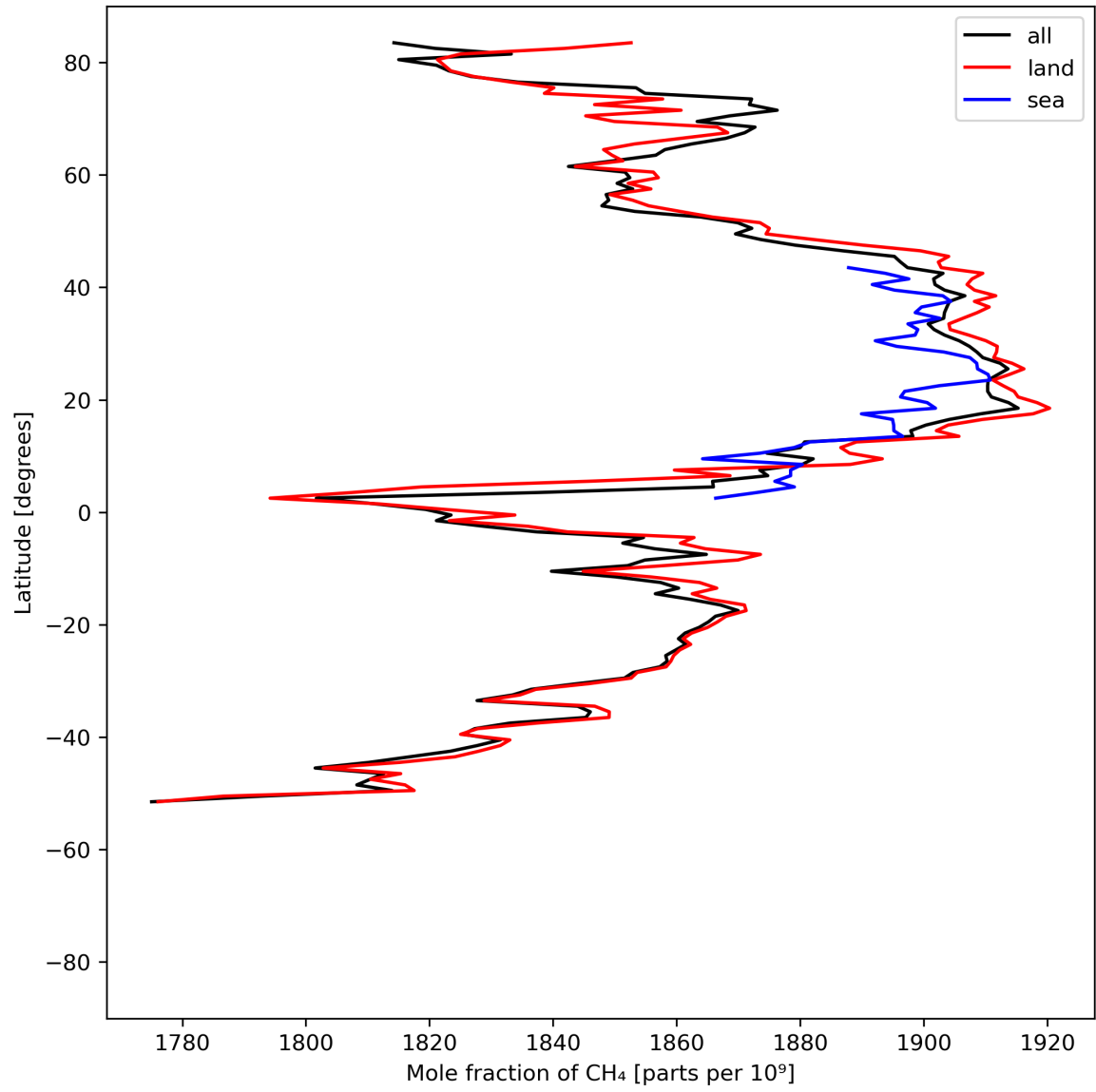
Figure 12: Zonal average of “Mole fraction of \text{CH}_4 ” for 2023-08-02 to 2023-08-04.
