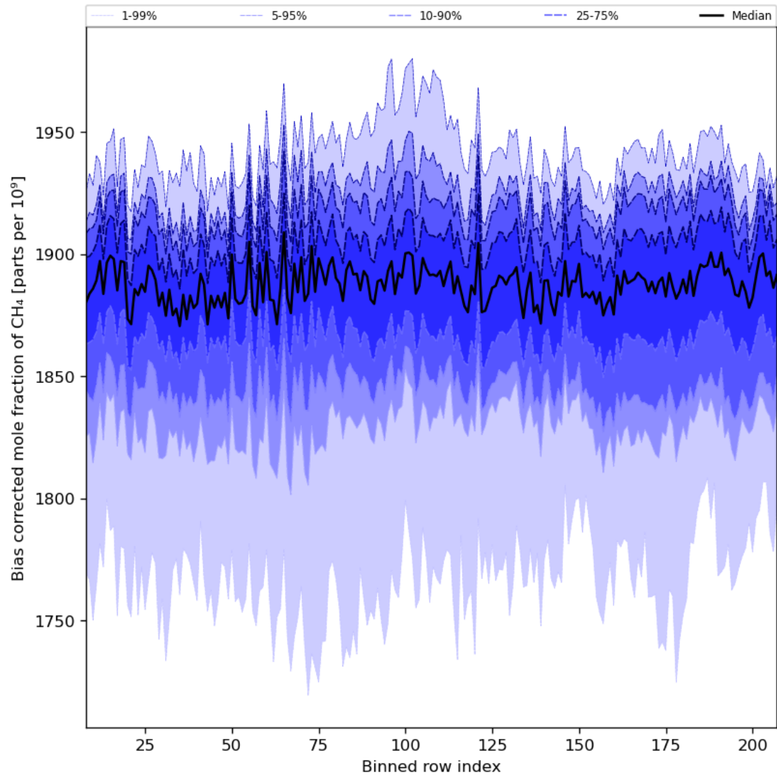
Figure 36: Along track statistics of “Bias corrected mole fraction of CH 4 ” for 2023-08-02 to 2023-08-04
