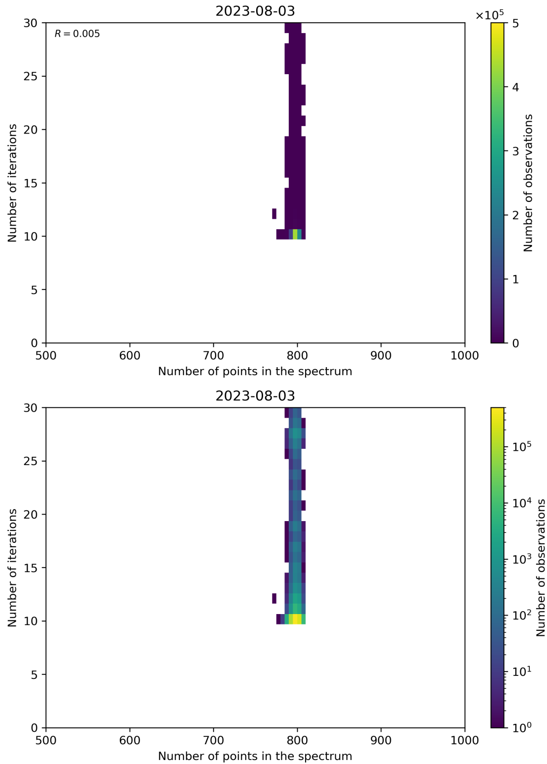
Figure 92: Scatter density plot of “Number of points in the spectrum” against “Number of iterations” for 2023-08-02 to 2023-08-04.
