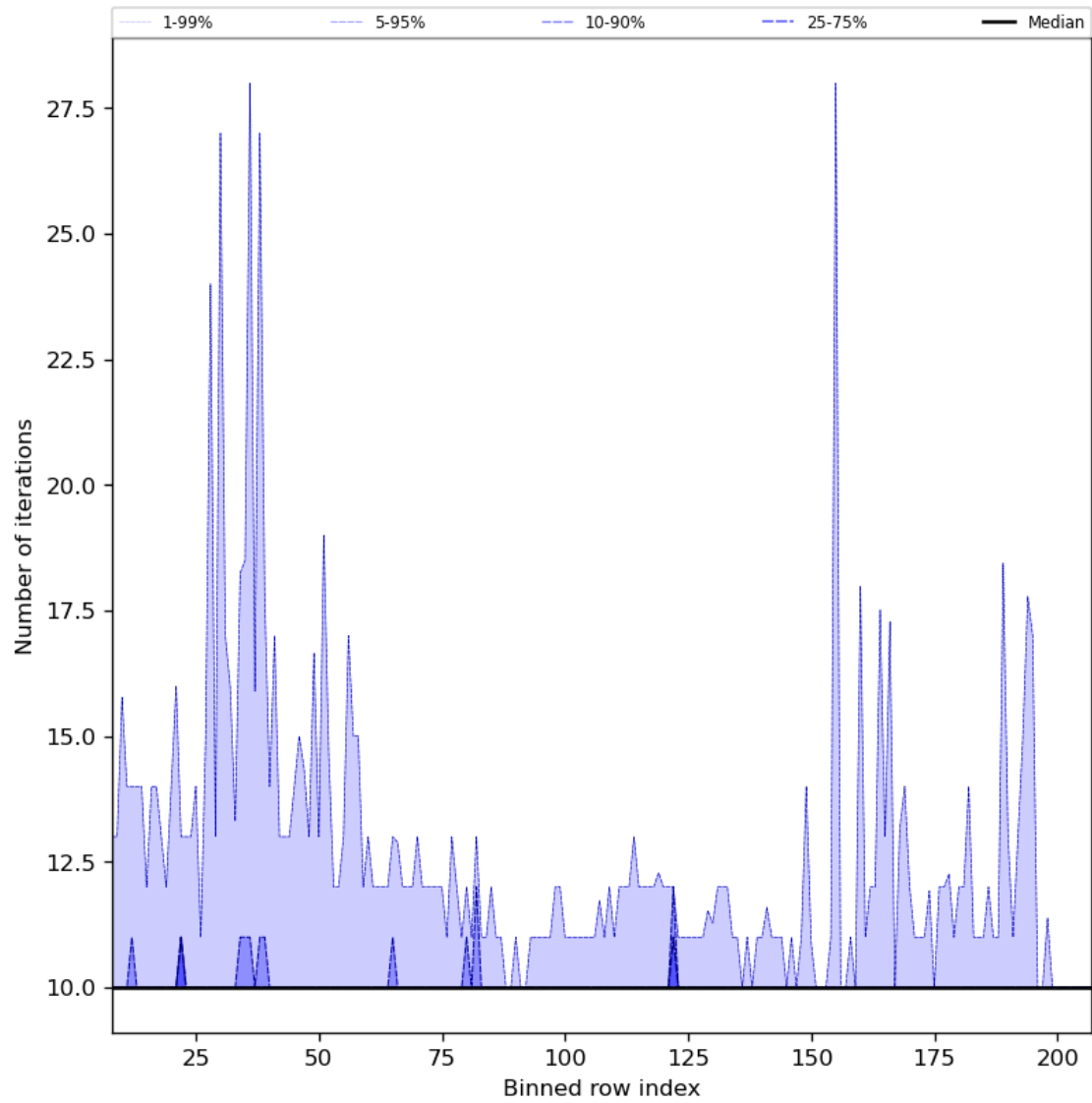
Figure 42: Along track statistics of “Number of iterations” for 2023-08-02 to 2023-08-04
