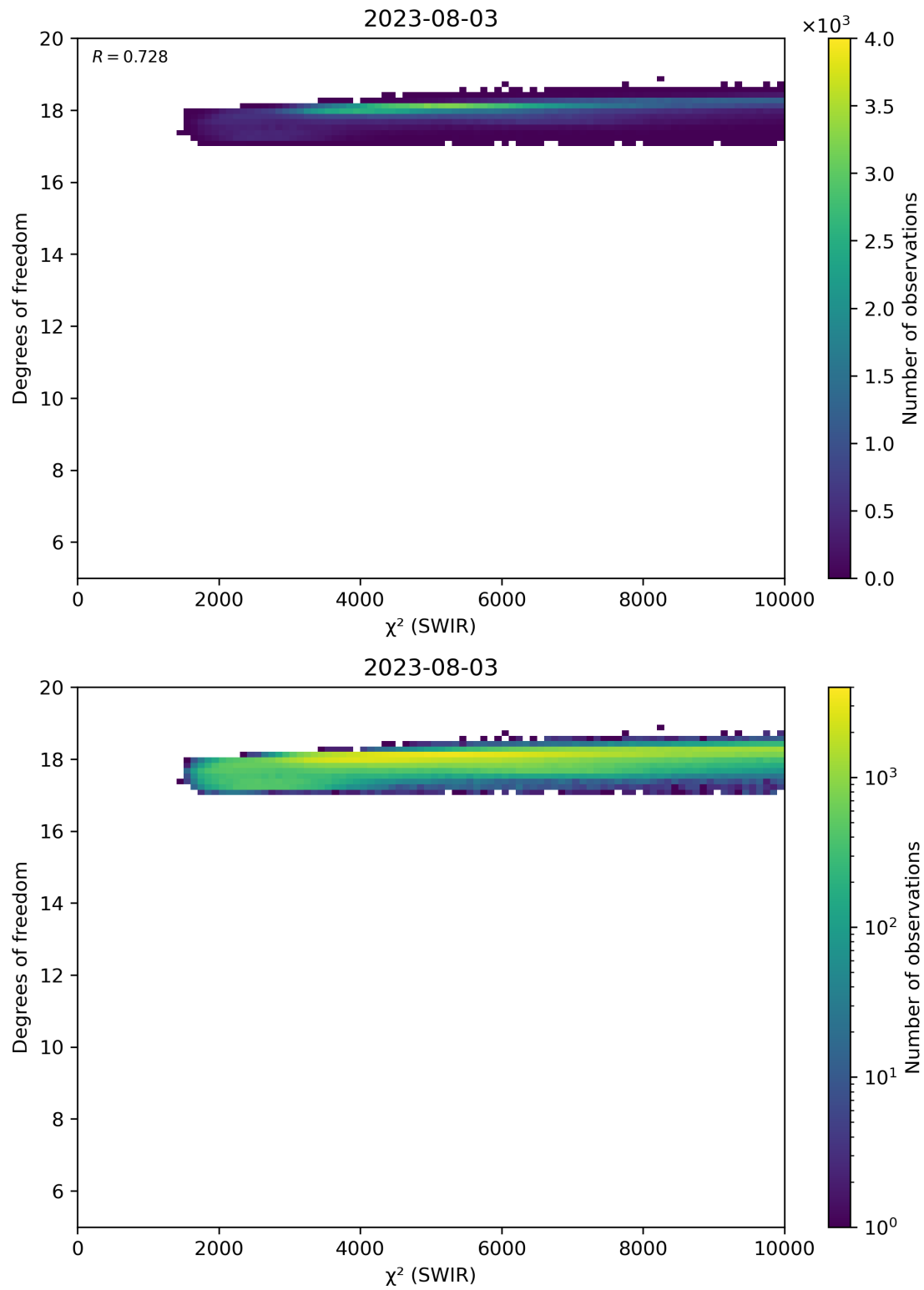
Figure 48: Scatter density plot of “ \chi^2 (SWIR)” against “Degrees of freedom” for 2023-08-02 to 2023-08-04.
