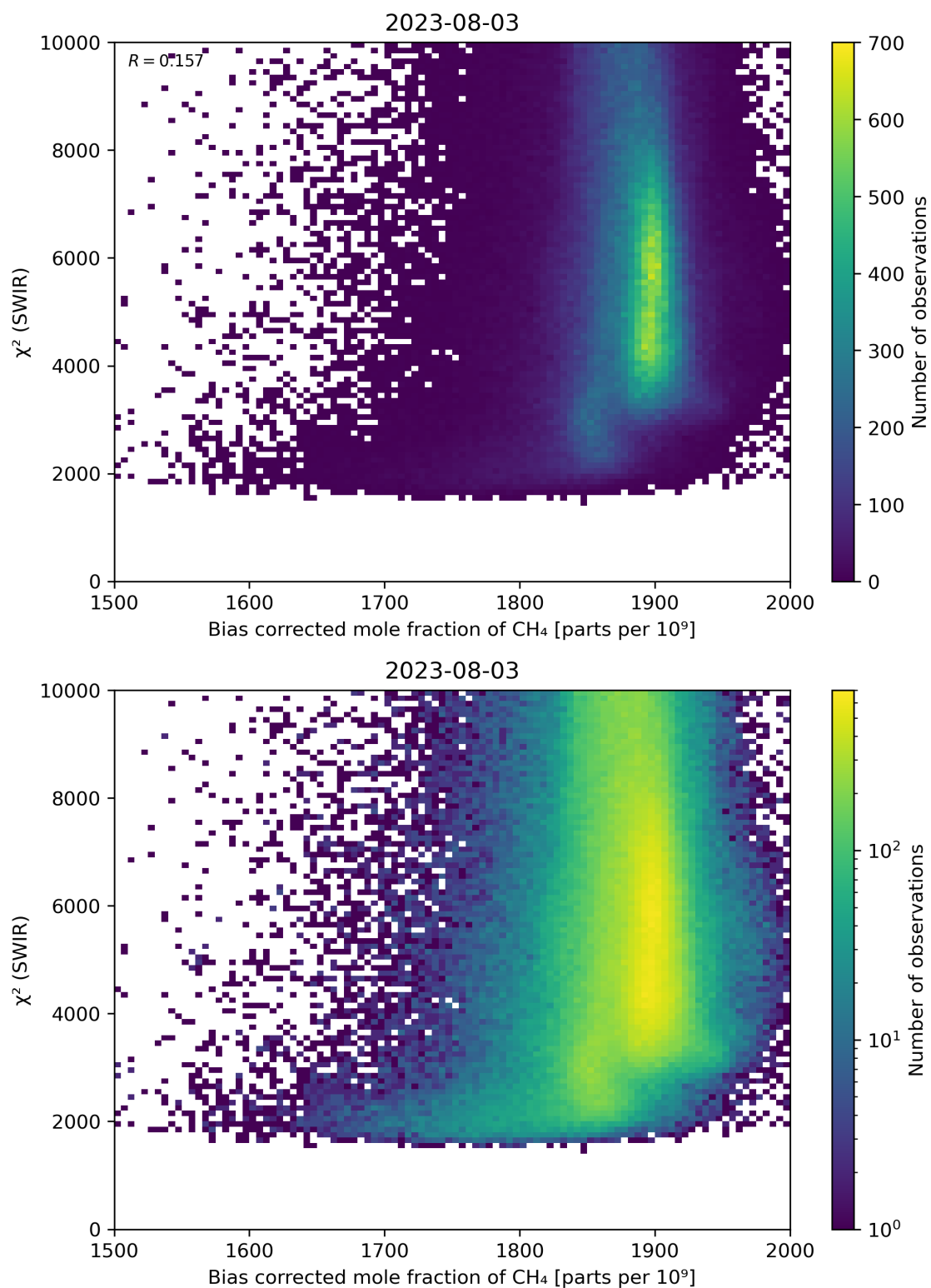
Figure 64: Scatter density plot of “Bias corrected mole fraction of CH 4 ” against “ \chi^2 (SWIR)” for 2023-08-02 to 2023-08-04.
