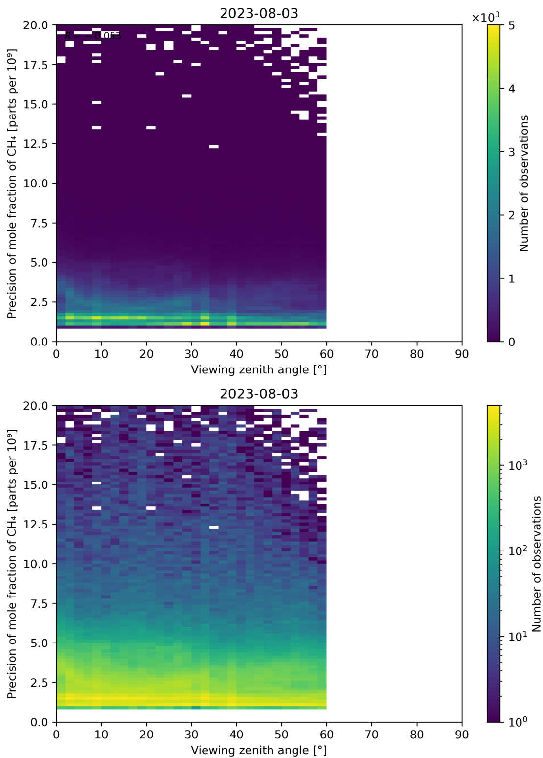
Figure 112: Scatter density plot of “Viewing zenith angle” against “Precision of mole fraction of CH 4 ” for 2023-08-02 to 2023-08-04.
