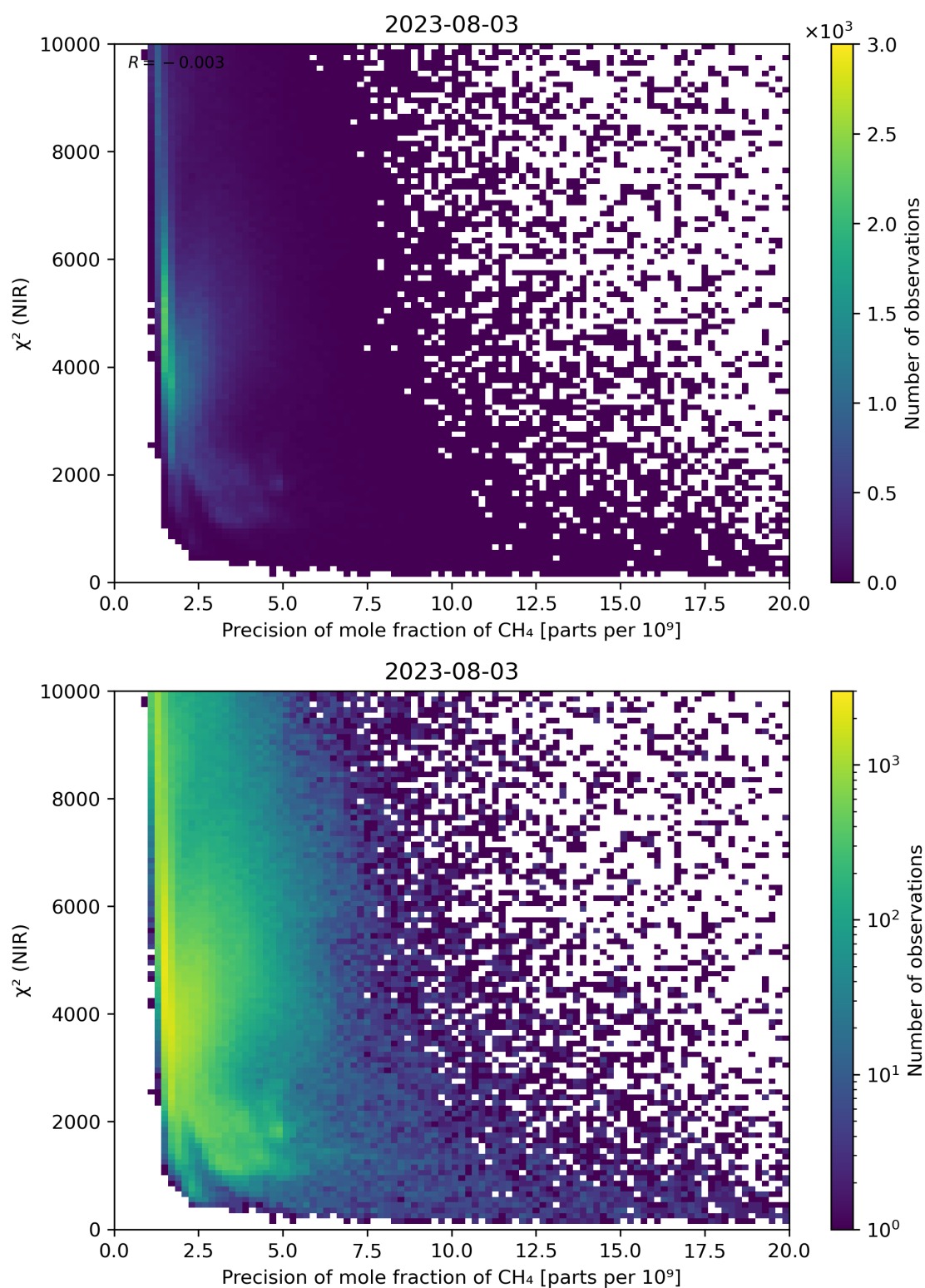
Figure 78: Scatter density plot of “Precision of mole fraction of CH 4 ” against “ \chi^2 (NIR)” for 2023-08-02 to 2023-08-04.
