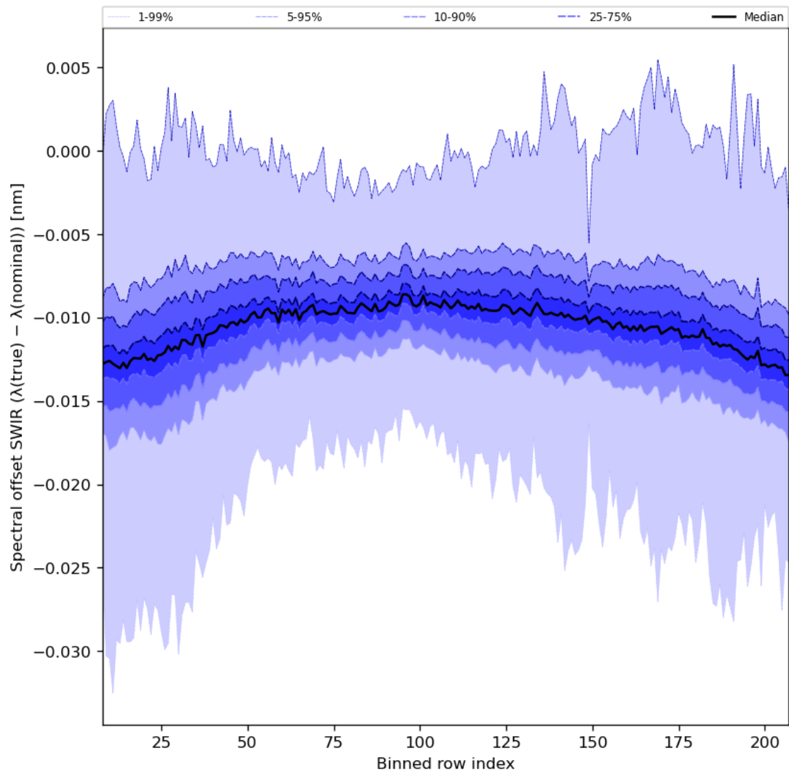
Figure 38: Along track statistics of “Spectral offset SWIR ( \lambda(\text{true}) - \lambda(\text{nominal}) )” for 2023-08-02 to 2023-08-04
