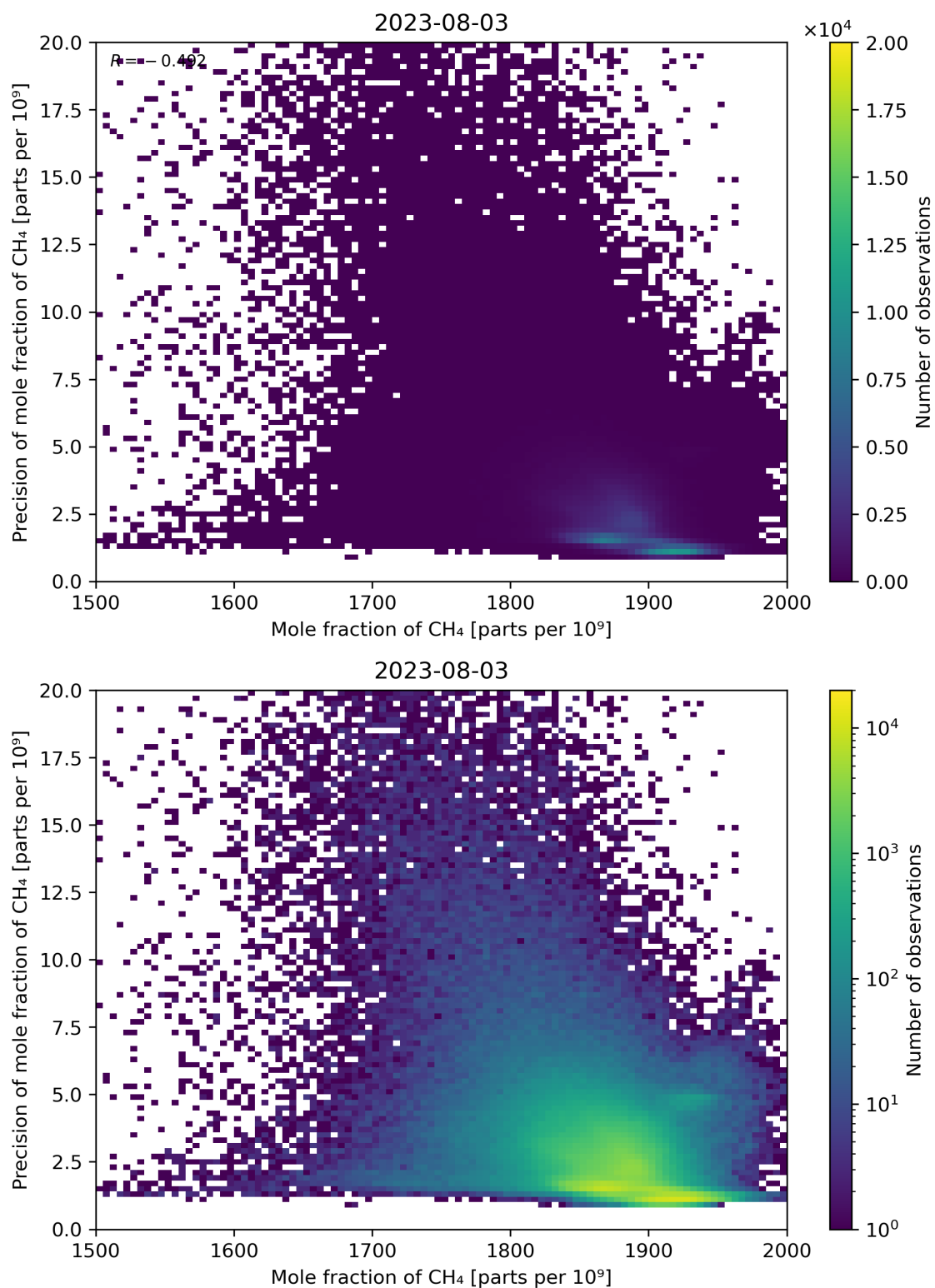
Figure 75: Scatter density plot of “Mole fraction of CH 4 ” against “Precision of mole fraction of CH 4 ” for 2023-08-02 to 2023-08-04.
