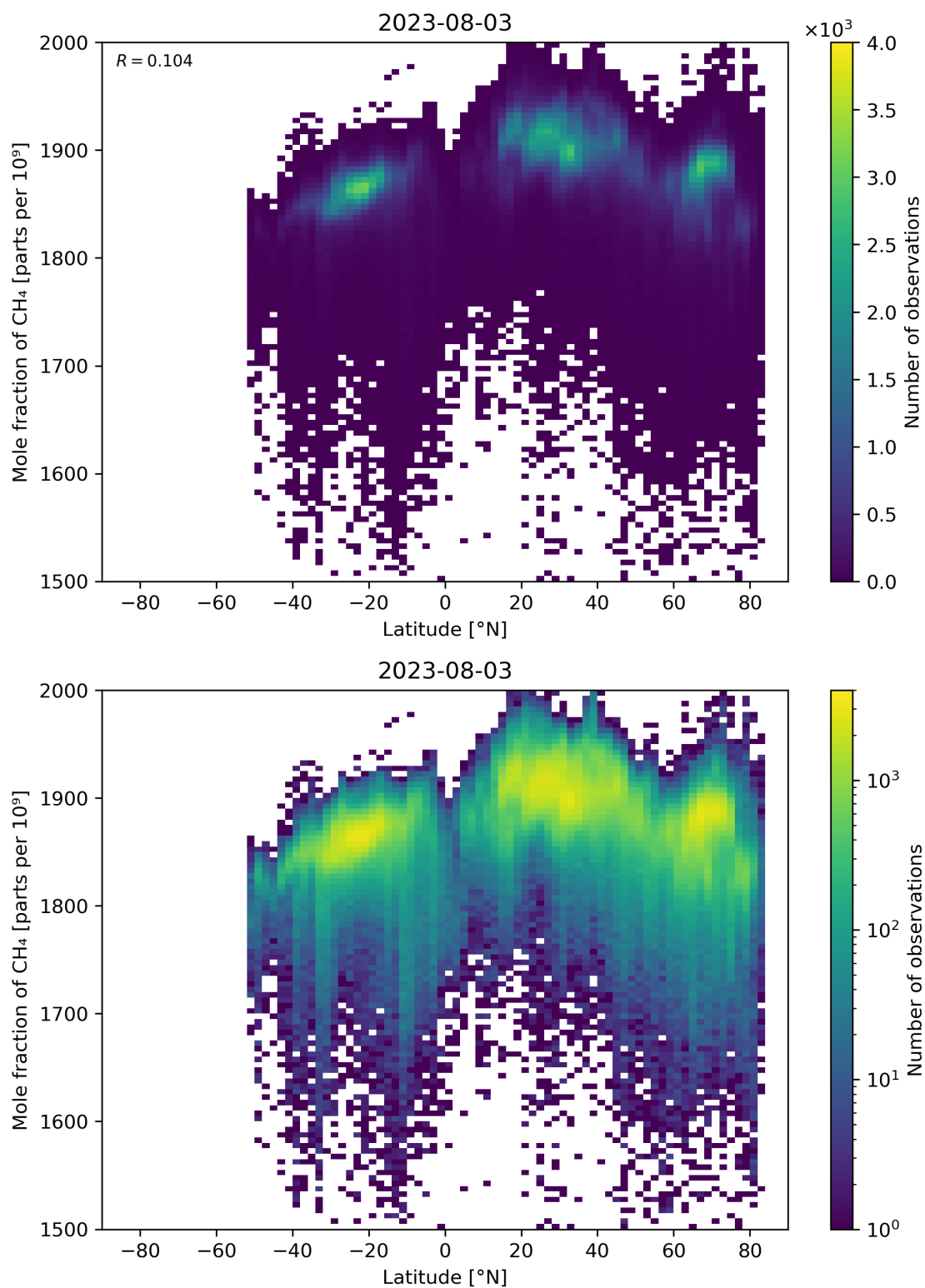
Figure 57: Scatter density plot of “Latitude” against “Mole fraction of CH 4 ” for 2023-08-02 to 2023-08-04.
