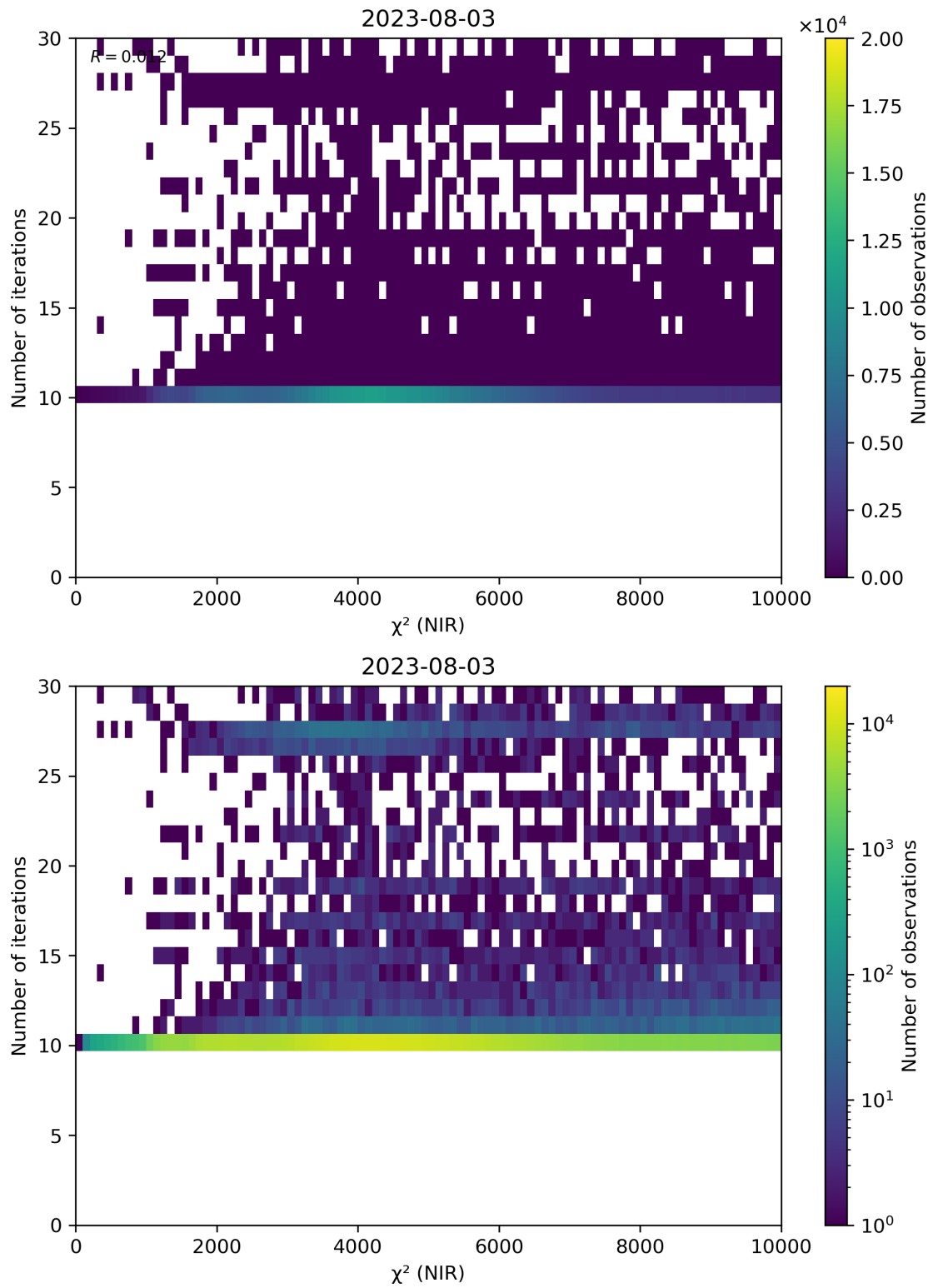
Figure 46: Scatter density plot of “ \chi^2 (NIR)” against “Number of iterations” for 2023-08-02 to 2023-08-04.
