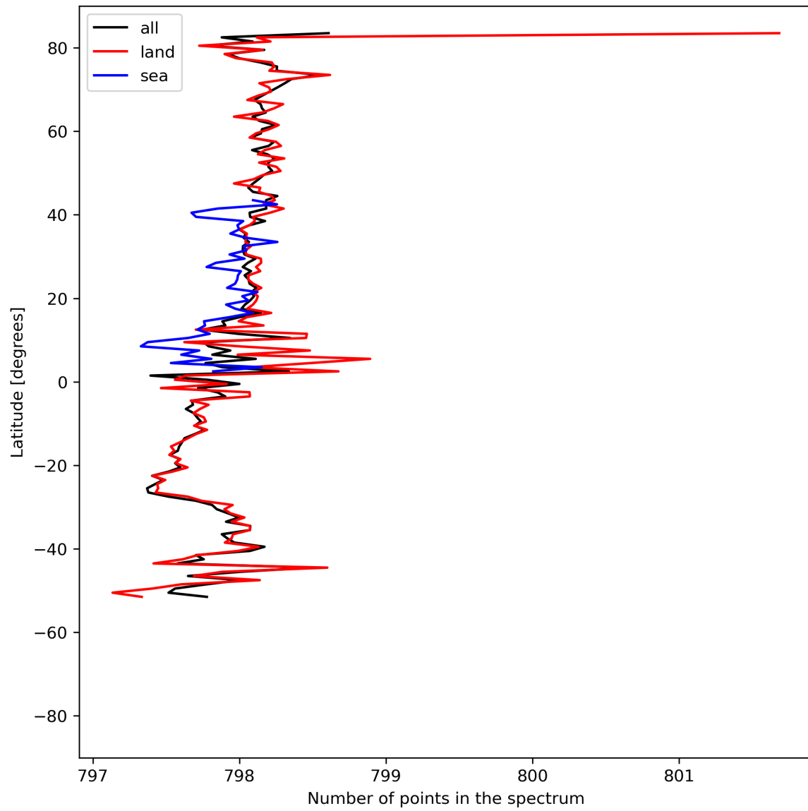
Figure 15: Zonal average of “Number of points in the spectrum” for 2023-08-02 to 2023-08-04.
