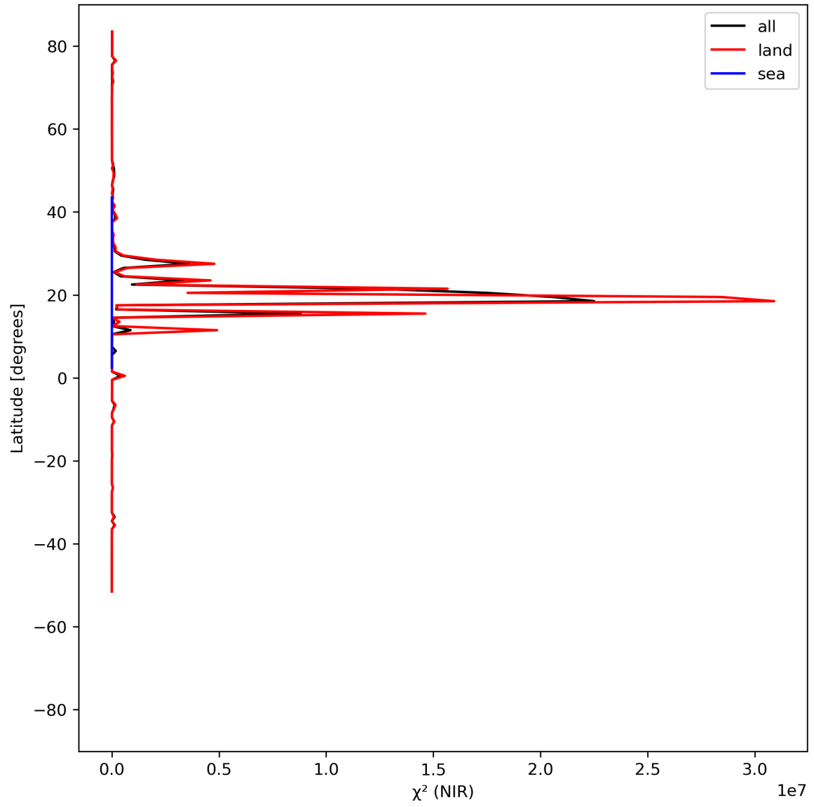
Figure 18: Zonal average of “ \chi^2 (NIR)” for 2023-08-02 to 2023-08-04.
