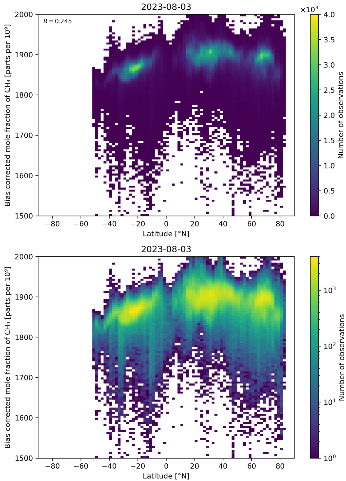
Figure 58: Scatter density plot of “Latitude” against “Bias corrected mole fraction of \text{CH}_4 ” for 2023-08-02 to 2023-08-04.
