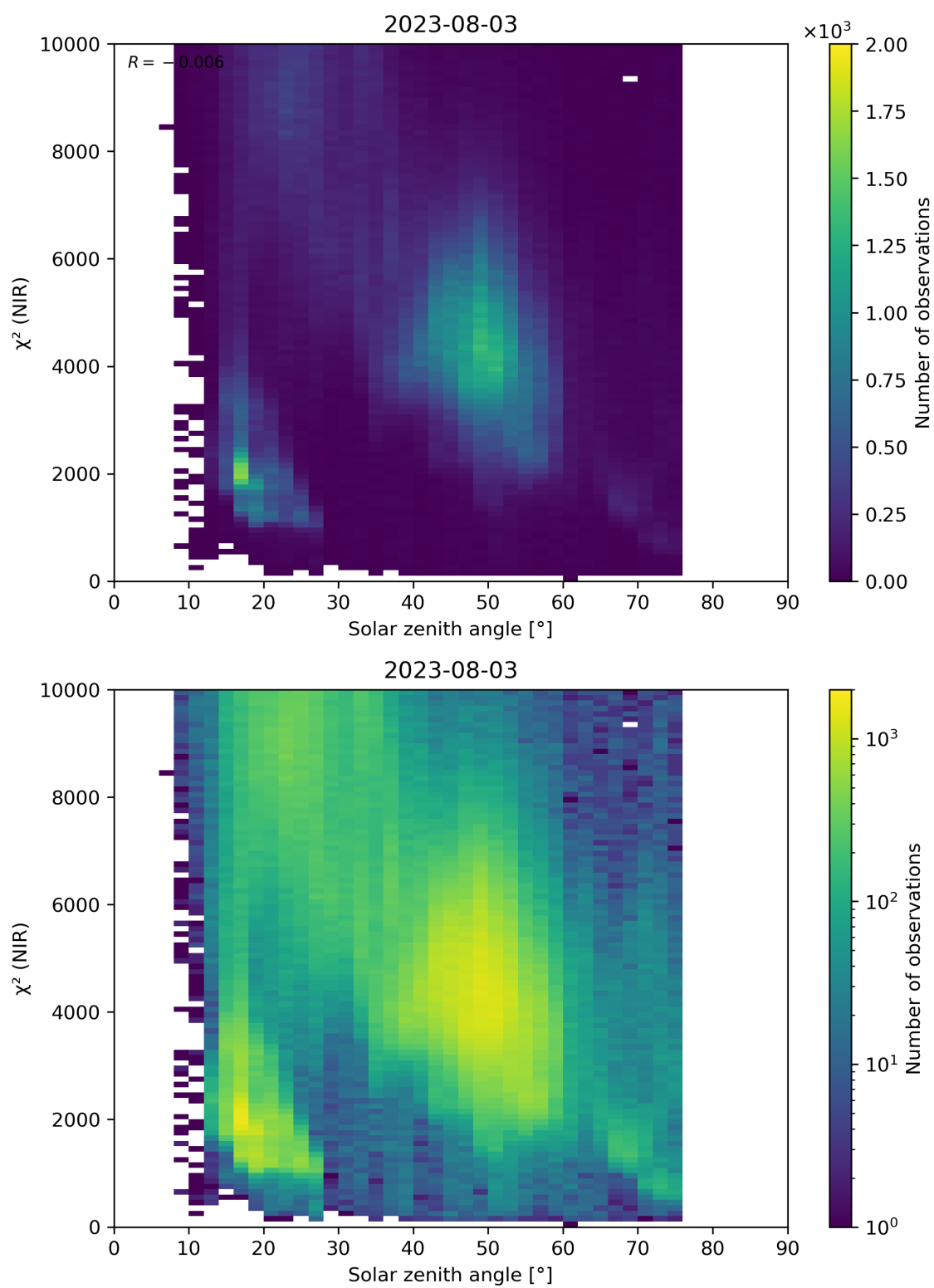
Figure 94: Scatter density plot of “Solar zenith angle” against “ \chi^2 (NIR)” for 2023-08-02 to 2023-08-04.
