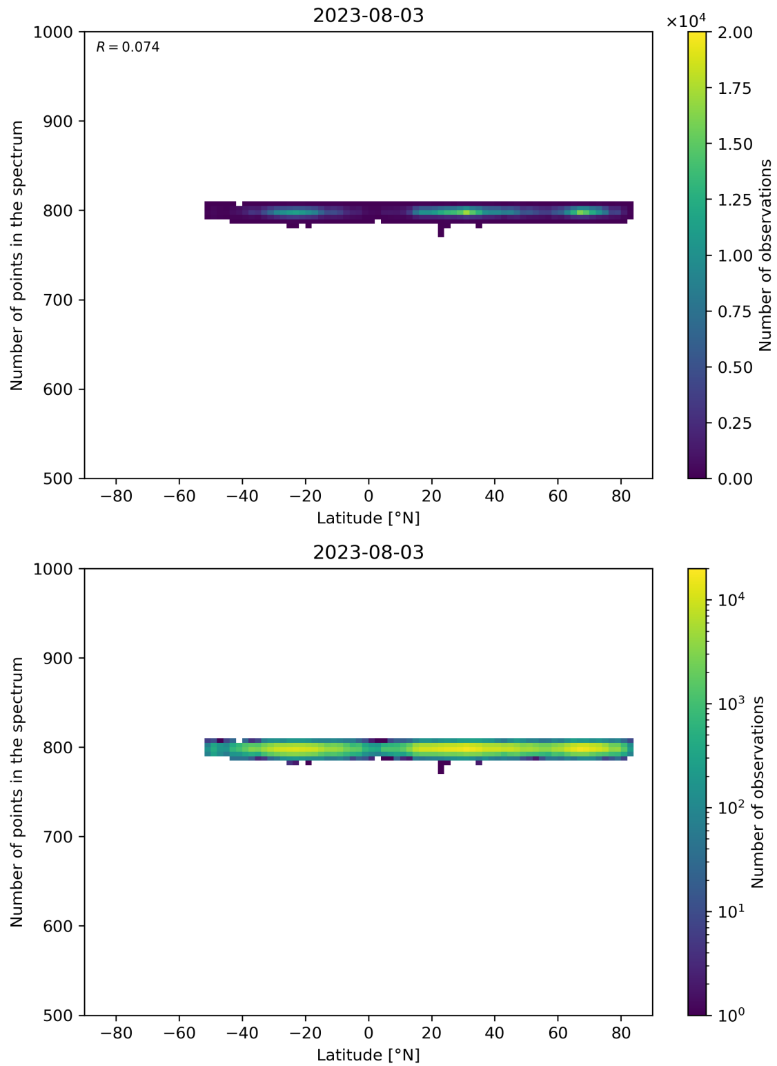
Figure 61: Scatter density plot of “Latitude” against “Number of points in the spectrum” for 2023-08-02 to 2023-08-04.
