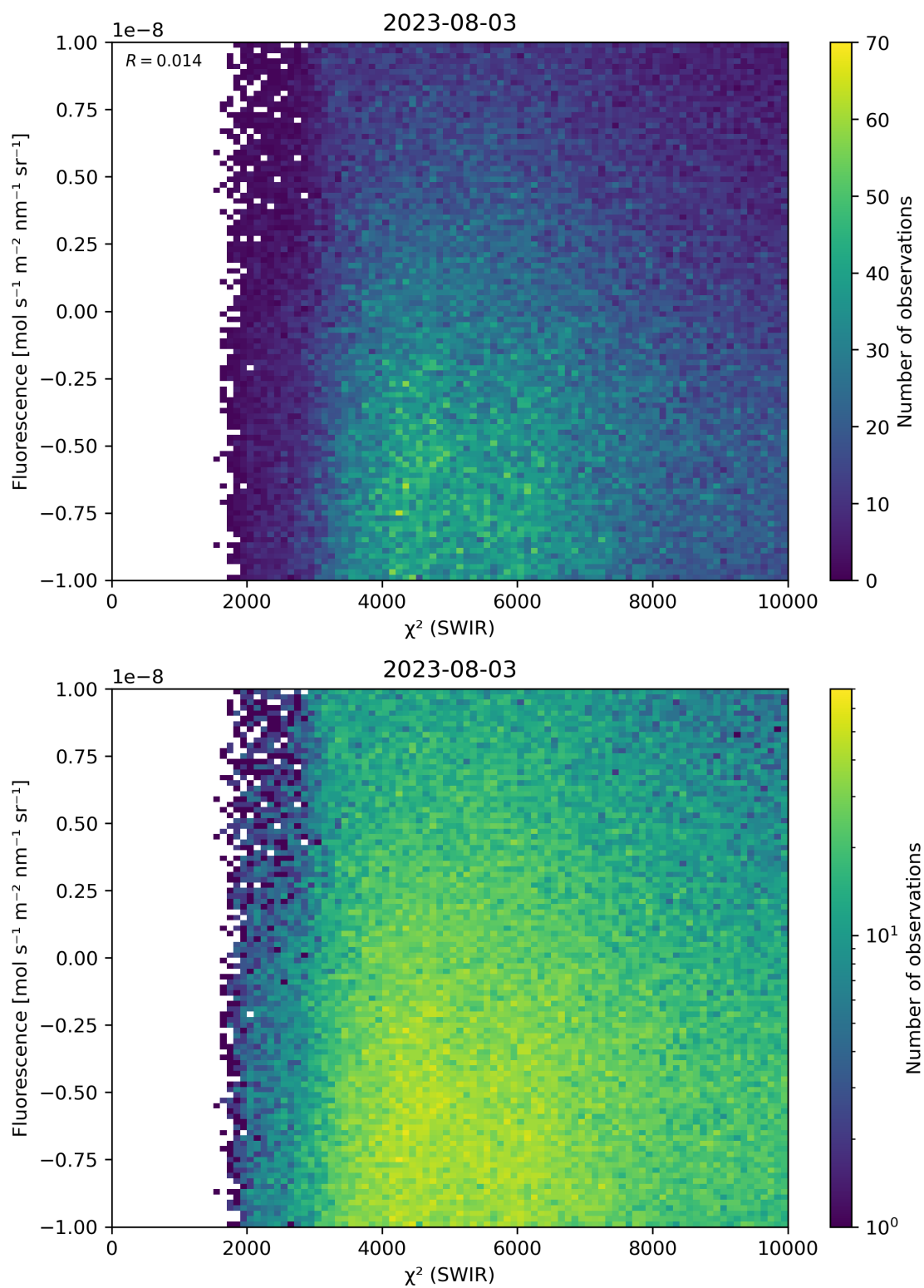
Figure 49: Scatter density plot of “ \chi^2 (SWIR)” against “Fluorescence” for 2023-08-02 to 2023-08-04.
