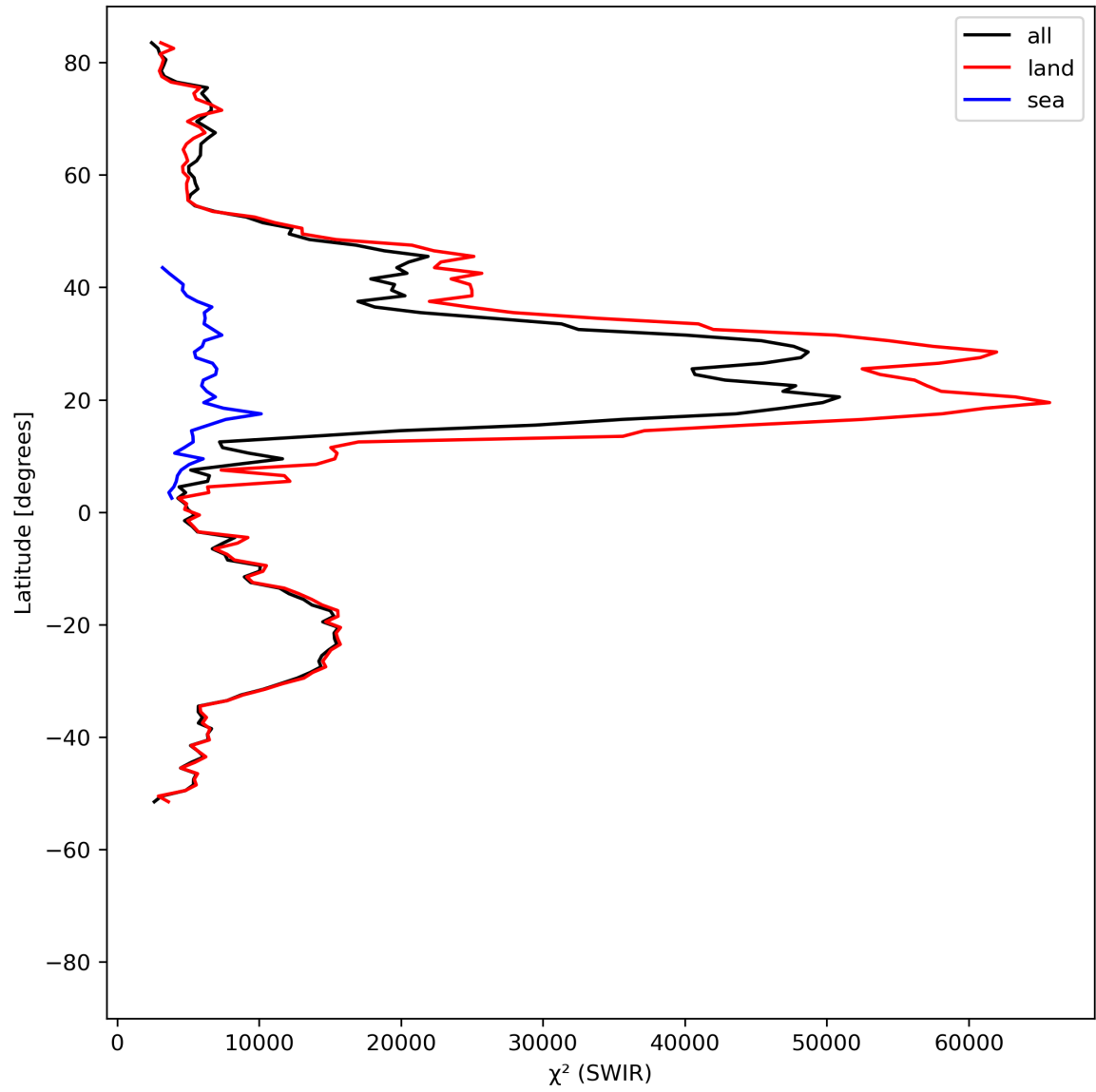
Figure 17: Zonal average of “ \chi^2 (SWIR)” for 2023-08-02 to 2023-08-04.
