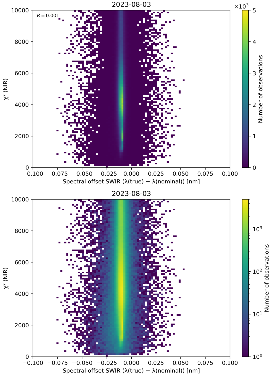
Figure 117: Scatter density plot of “Spectral offset SWIR ( \lambda(\text{true}) - \lambda(\text{nominal}) )” against “ \chi^2 (NIR)” for 2023-08-02 to 2023-08-04.
