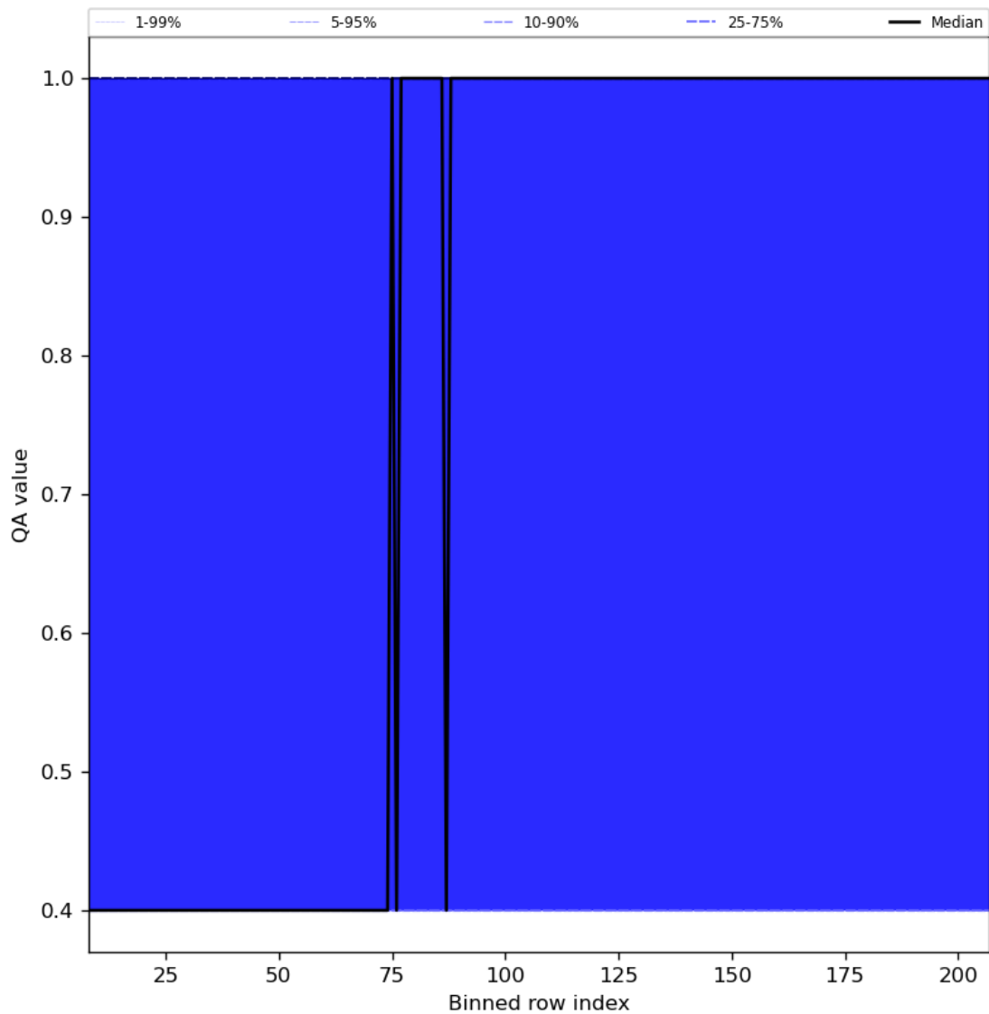
Figure 33: Along track statistics of “QA value” for 2023-08-02 to 2023-08-04
