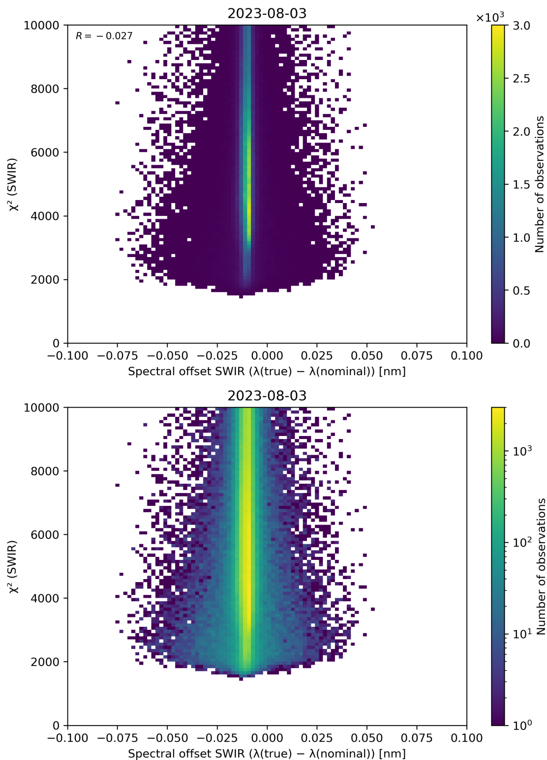
Figure 118: Scatter density plot of “Spectral offset SWIR ( \lambda(\text{true}) - \lambda(\text{nominal}) )” against “ \chi^2 (SWIR)” for 2023-08-02 to 2023-08-04.
