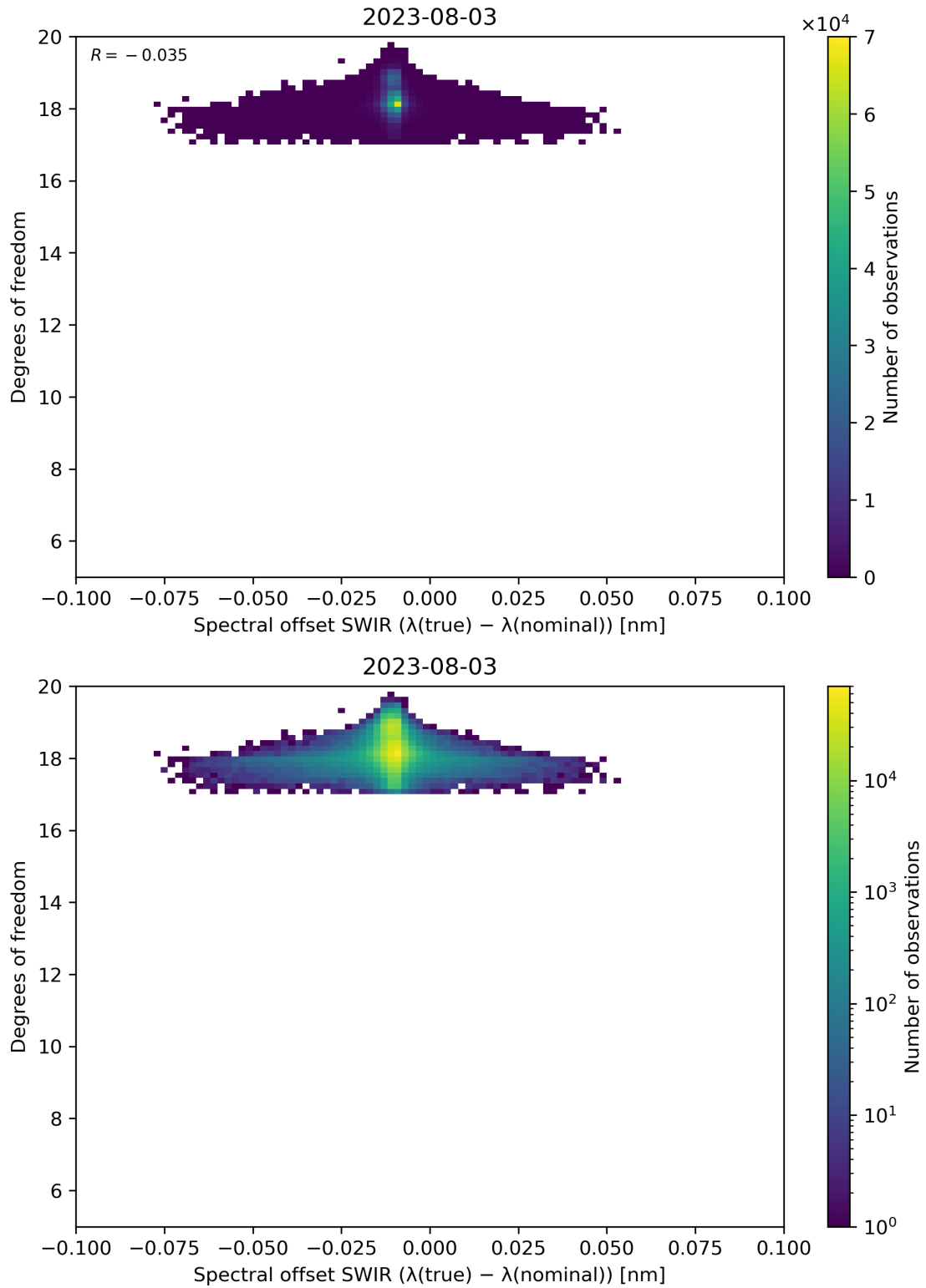
Figure 119: Scatter density plot of “Spectral offset SWIR ( \lambda(\text{true}) - \lambda(\text{nominal}) )” against “Degrees of freedom” for 2023-08-02 to 2023-08-04.
