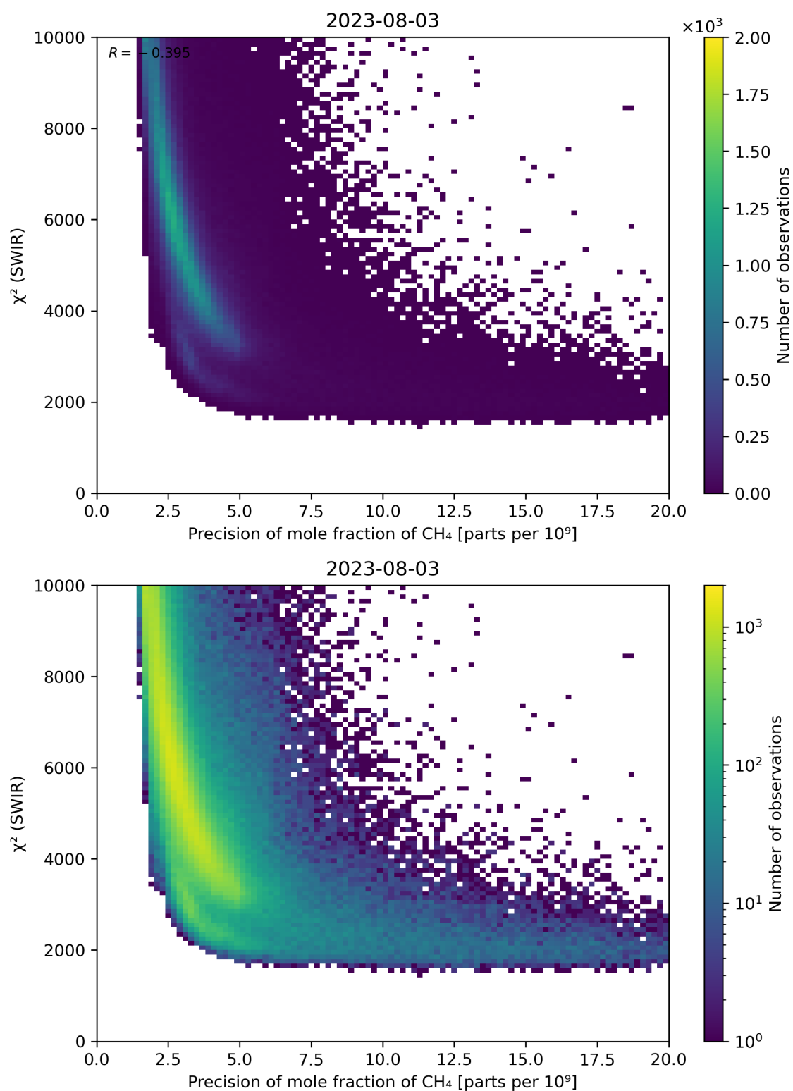
Figure 79: Scatter density plot of “Precision of mole fraction of \text{CH}_4 ” against “ \chi^2 (SWIR)” for 2023-08-02 to 2023-08-04.
