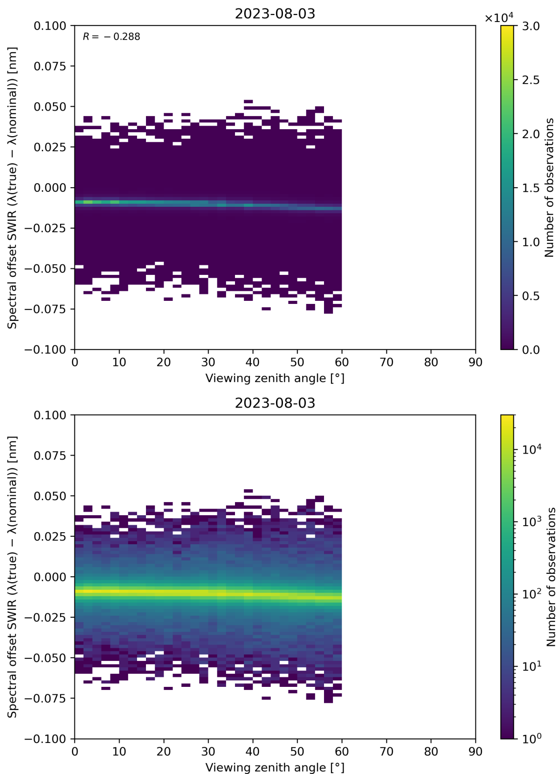
Figure 116: Scatter density plot of “Viewing zenith angle” against “Spectral offset SWIR ( \lambda(\text{true}) - \lambda(\text{nominal}) )” for 2023-08-02 to 2023-08-04.
