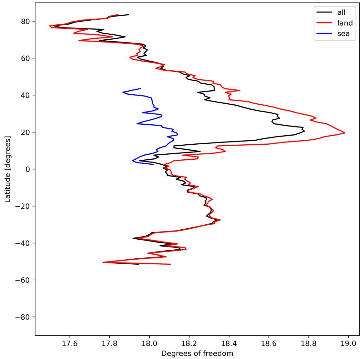
Figure 19: Zonal average of “Degrees of freedom” for 2023-08-02 to 2023-08-04.
