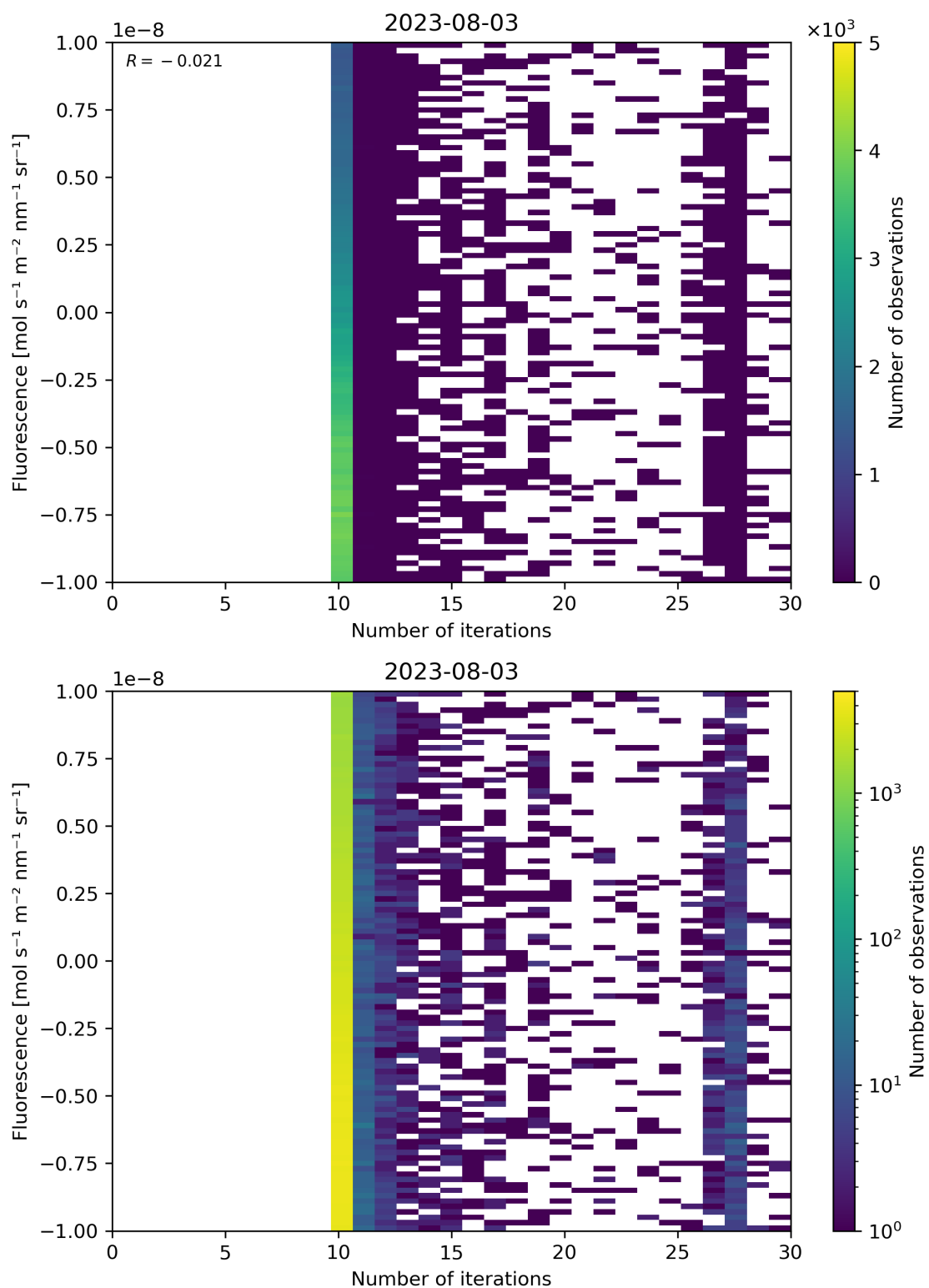
Figure 87: Scatter density plot of “Number of iterations” against “Fluorescence” for 2023-08-02 to 2023-08-04.
