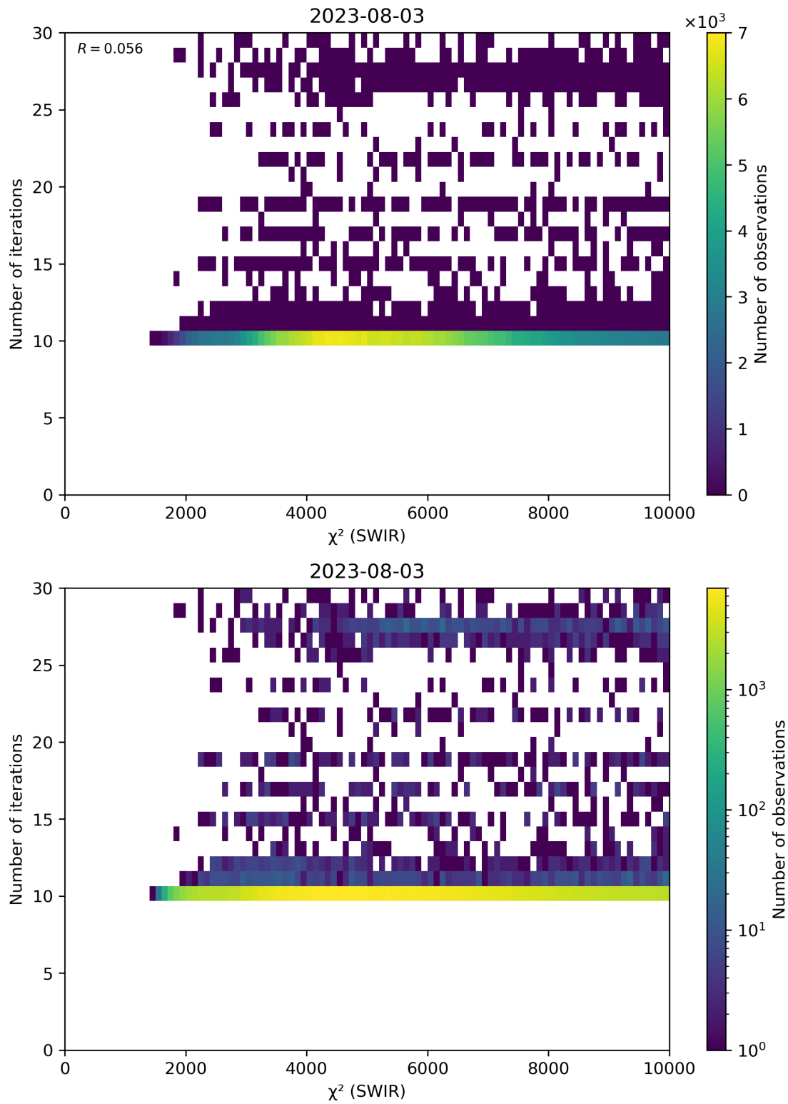
Figure 50: Scatter density plot of “ \chi^2 (SWIR)” against “Number of iterations” for 2023-08-02 to 2023-08-04.
