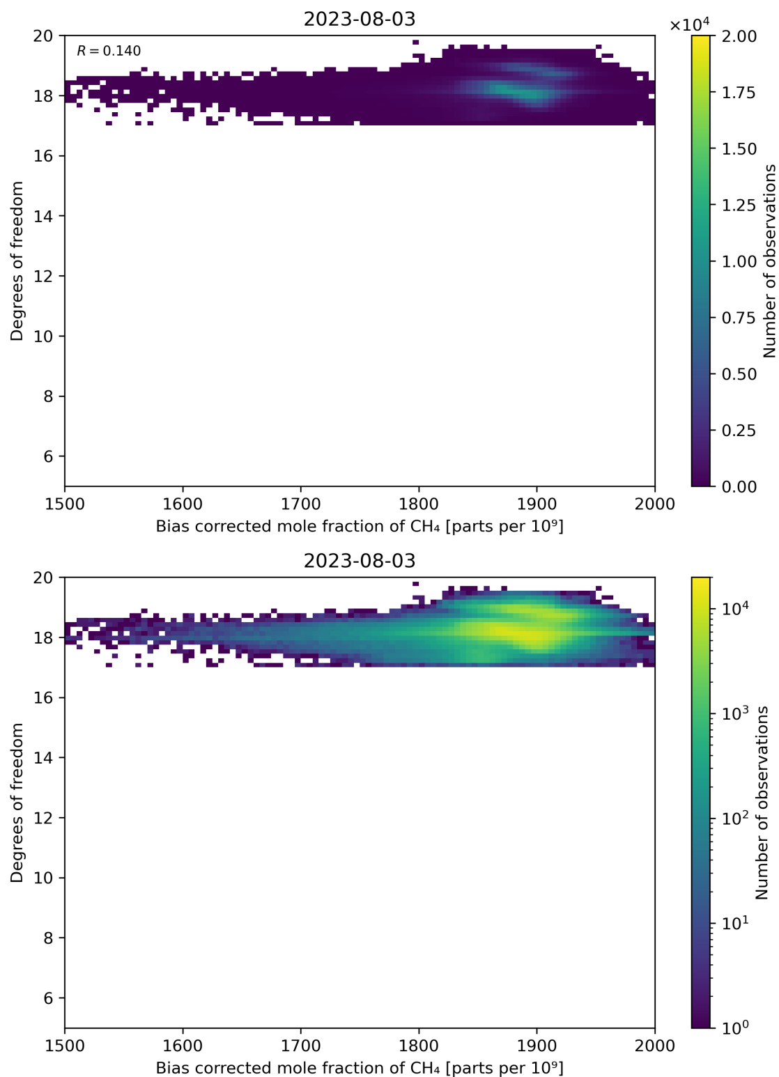
Figure 65: Scatter density plot of “Bias corrected mole fraction of CH 4 ” against “Degrees of freedom” for 2023-08-02 to 2023-08-04.
