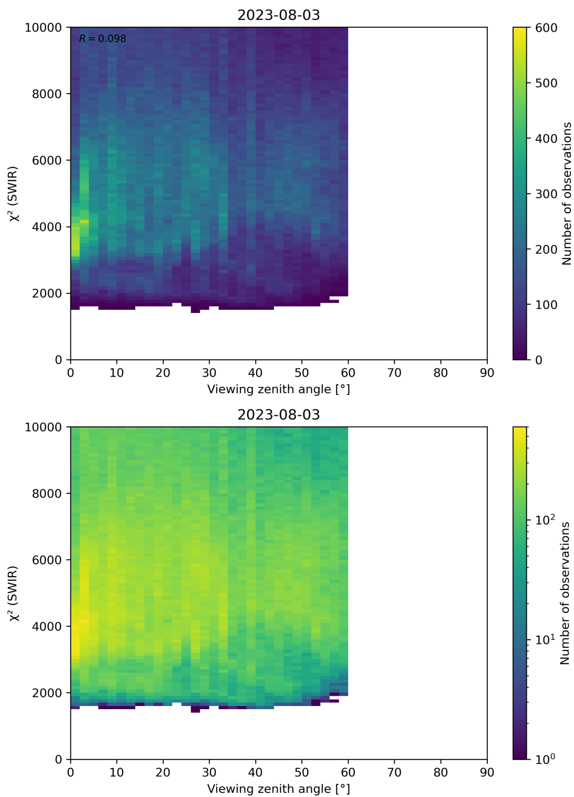
Figure 106: Scatter density plot of “Viewing zenith angle” against “ \chi^2 (SWIR)” for 2023-08-02 to 2023-08-04.
