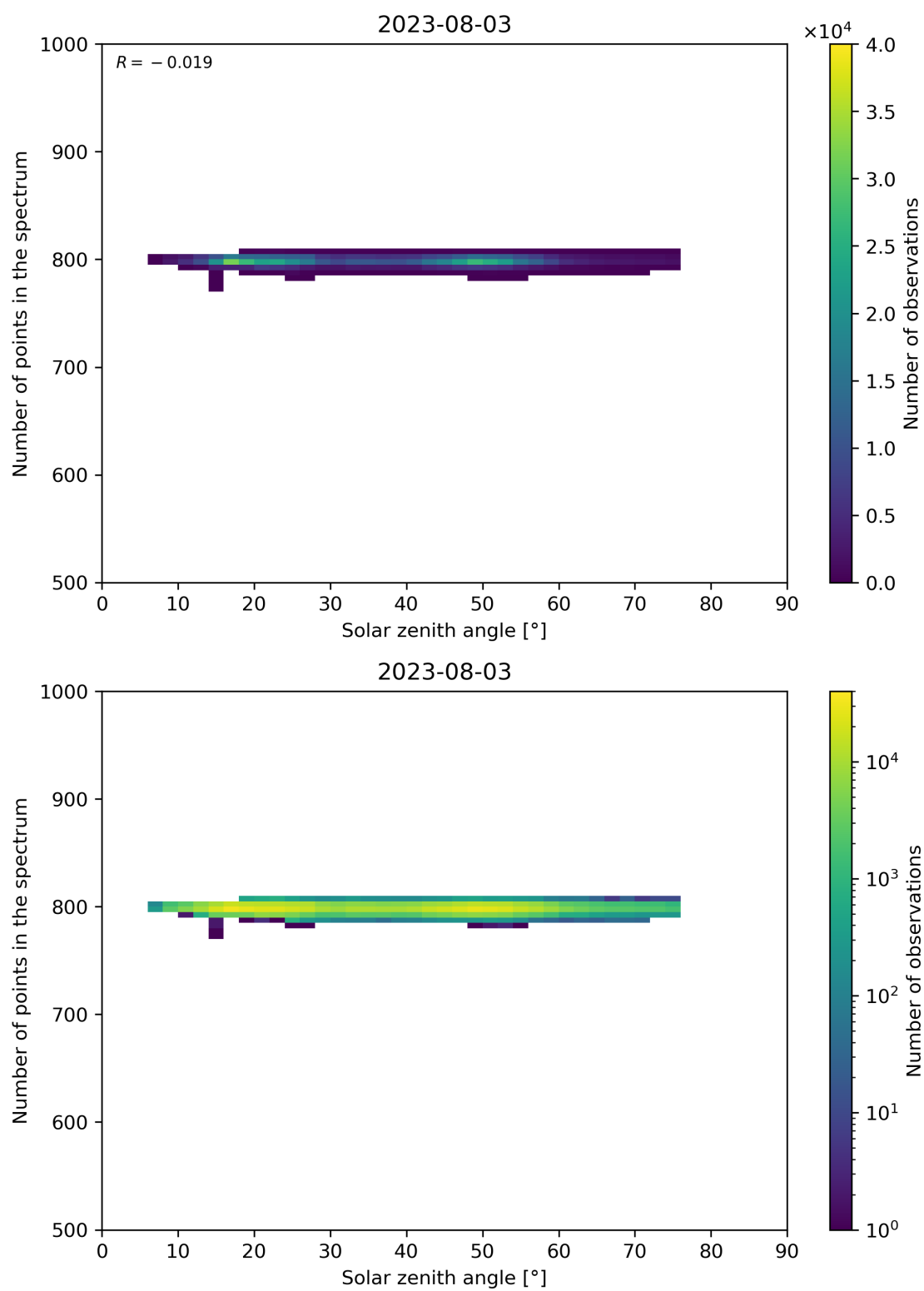
Figure 103: Scatter density plot of “Solar zenith angle” against “Number of points in the spectrum” for 2023-08-02 to 2023-08-04.
