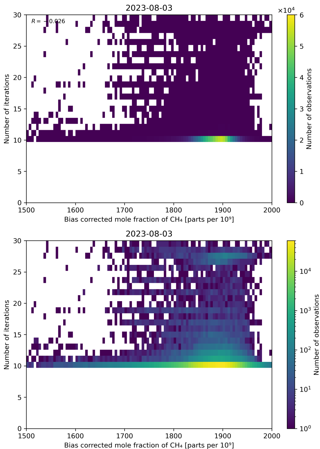
Figure 67: Scatter density plot of “Bias corrected mole fraction of CH 4 ” against “Number of iterations” for 2023-08-02 to 2023-08-04.
