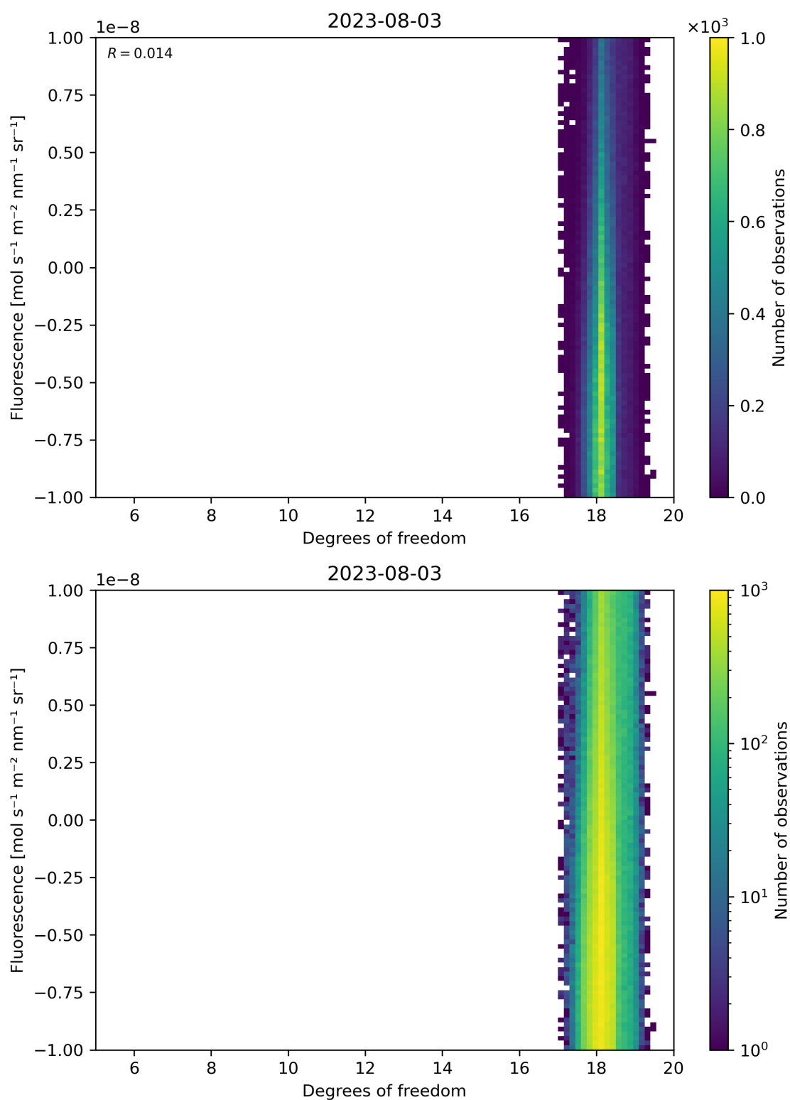
Figure 51: Scatter density plot of “Degrees of freedom” against “Fluorescence” for 2023-08-02 to 2023-08-04.
