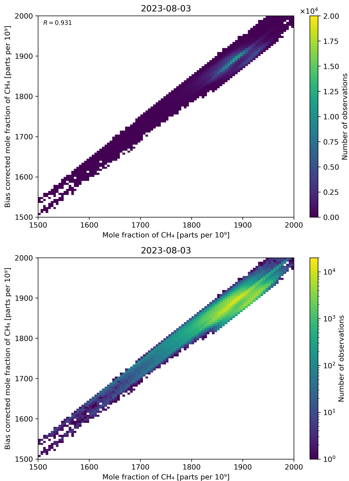
Figure 74: Scatter density plot of “Mole fraction of CH 4 ” against “Bias corrected mole fraction of CH 4 ” for 2023-08-02 to 2023-08-04.
