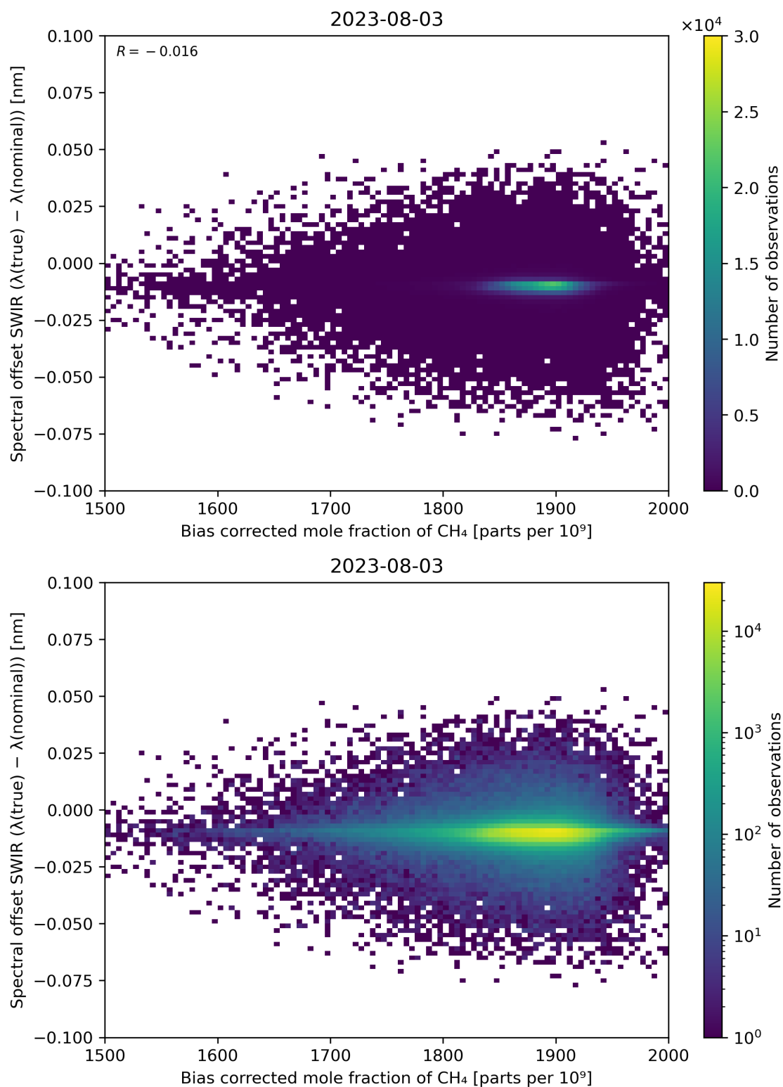
Figure 69: Scatter density plot of “Bias corrected mole fraction of \text{CH}_4 ” against “Spectral offset SWIR ( \lambda(\text{true}) - \lambda(\text{nominal}) )” for 2023-08-02 to 2023-08-04.
