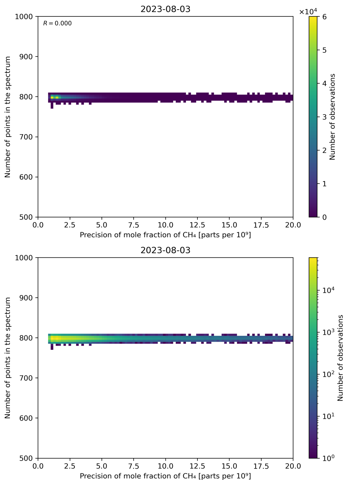
Figure 84: Scatter density plot of “Precision of mole fraction of CH 4 ” against “Number of points in the spectrum” for 2023-08-02 to 2023-08-04.
