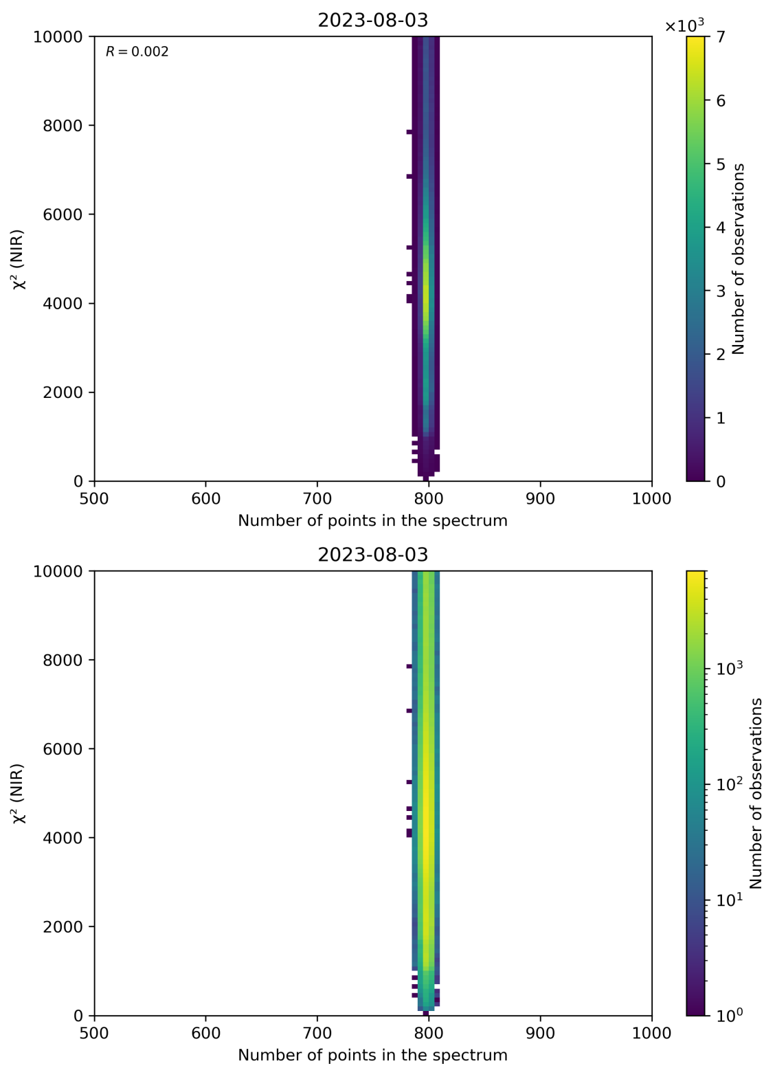
Figure 88: Scatter density plot of “Number of points in the spectrum” against “ \chi^2 (NIR)” for 2023-08-02 to 2023-08-04.
