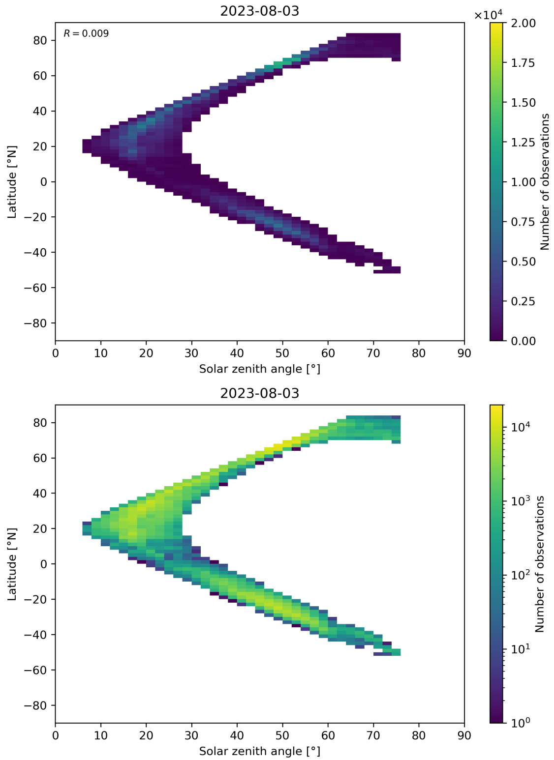
Figure 98: Scatter density plot of “Solar zenith angle” against “Latitude” for 2023-08-02 to 2023-08-04.
