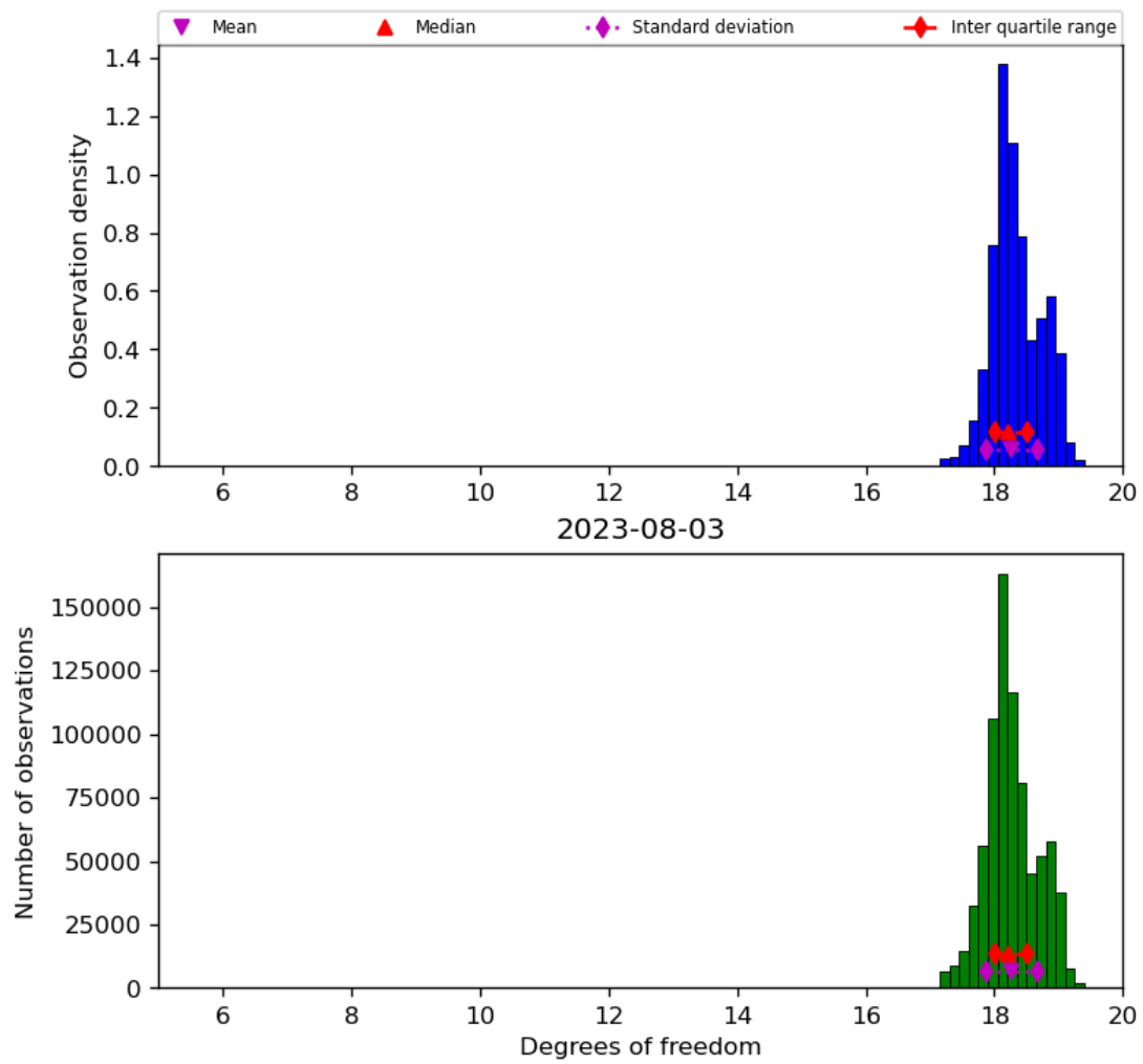
Figure 30: Histogram of “Degrees of freedom” for 2023-08-02 to 2023-08-04
