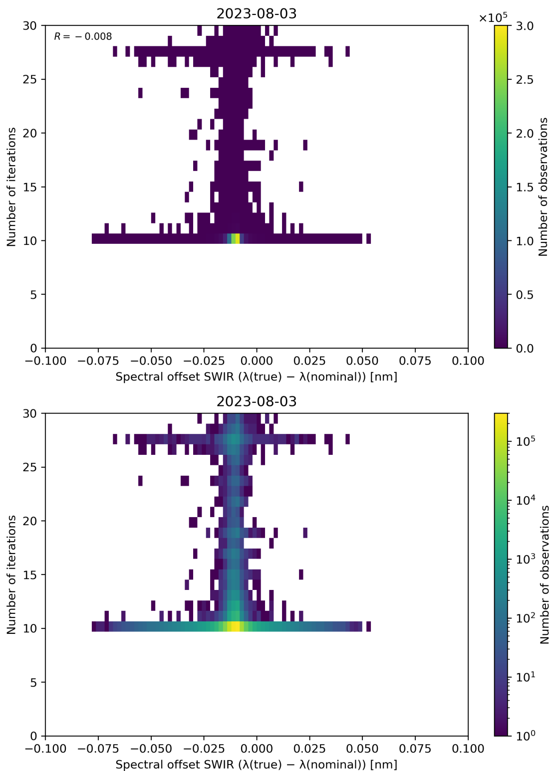
Figure 121: Scatter density plot of “Spectral offset SWIR ( \lambda(\text{true}) - \lambda(\text{nominal}) )” against “Number of iterations” for 2023-08-02 to 2023-08-04.
