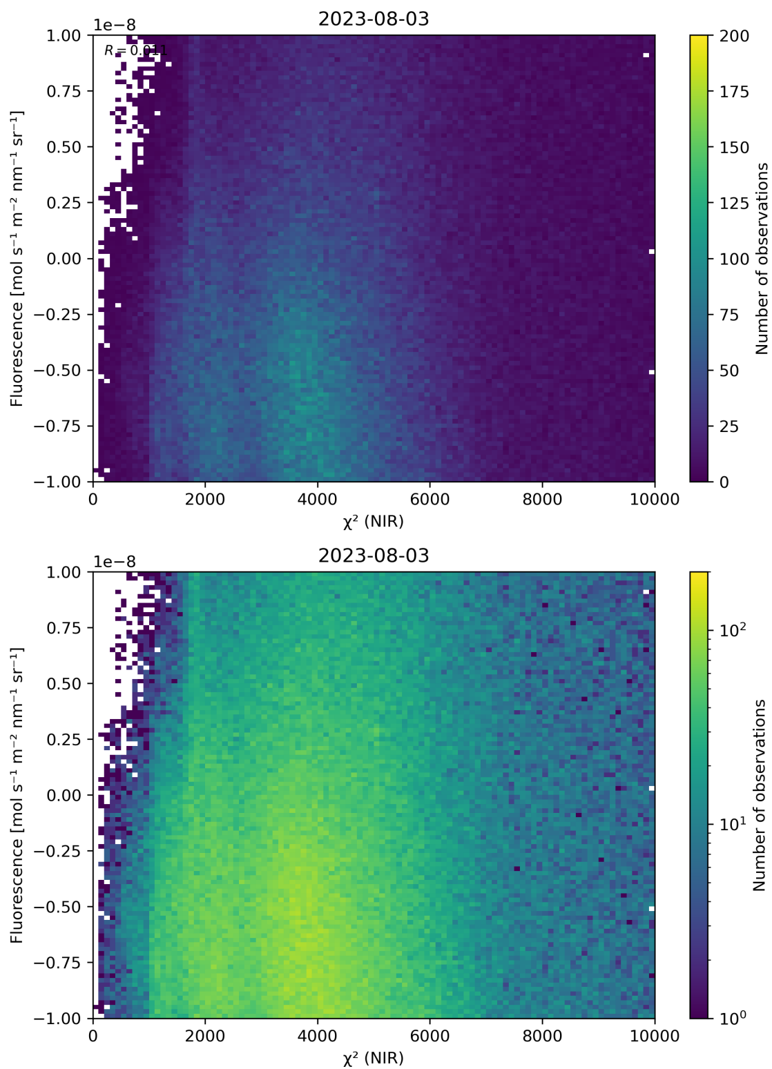
Figure 45: Scatter density plot of “ \chi^2 (NIR)” against “Fluorescence” for 2023-08-02 to 2023-08-04.
