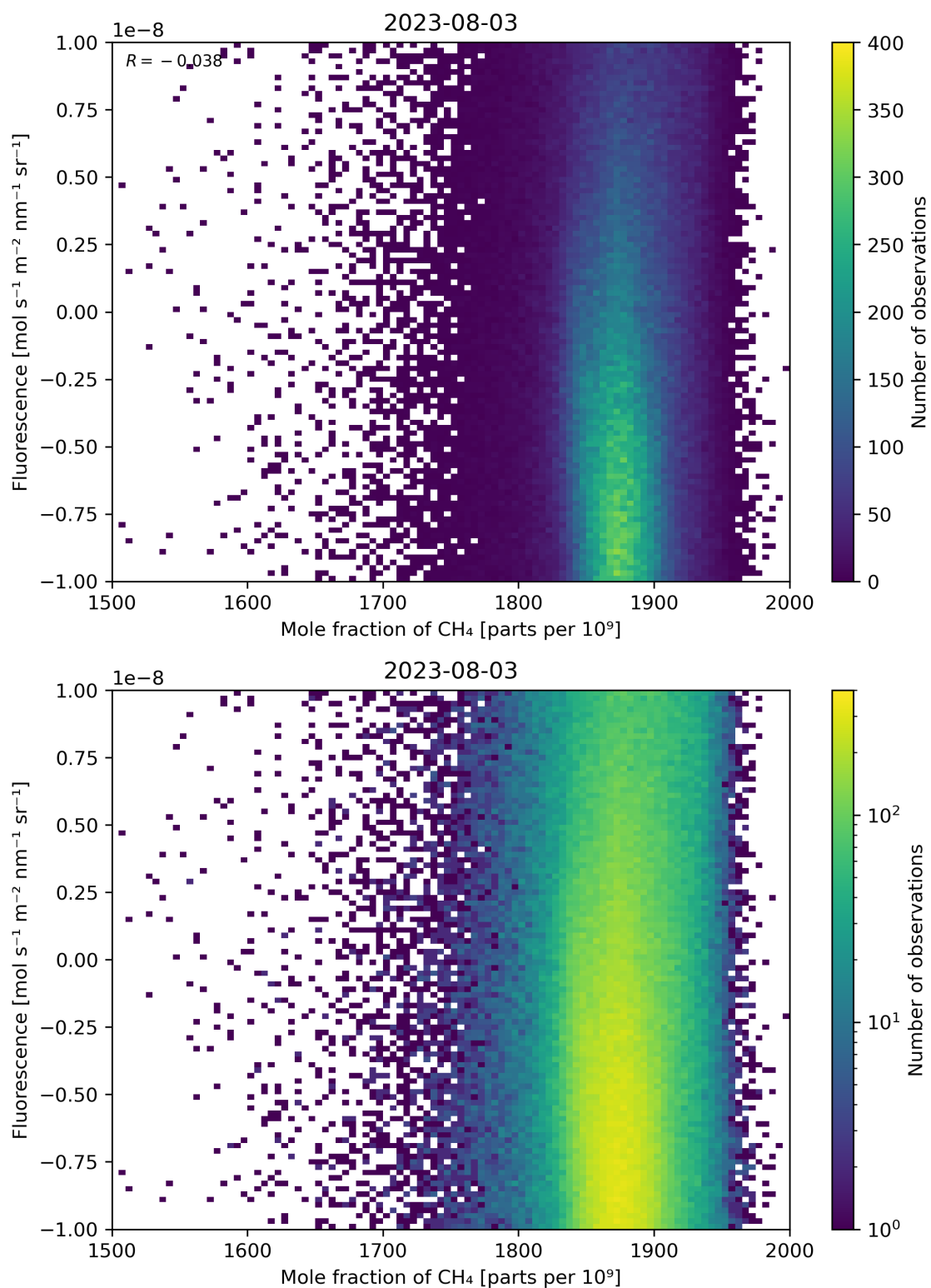
Figure 73: Scatter density plot of “Mole fraction of \text{CH}_4 ” against “Fluorescence” for 2023-08-02 to 2023-08-04.
