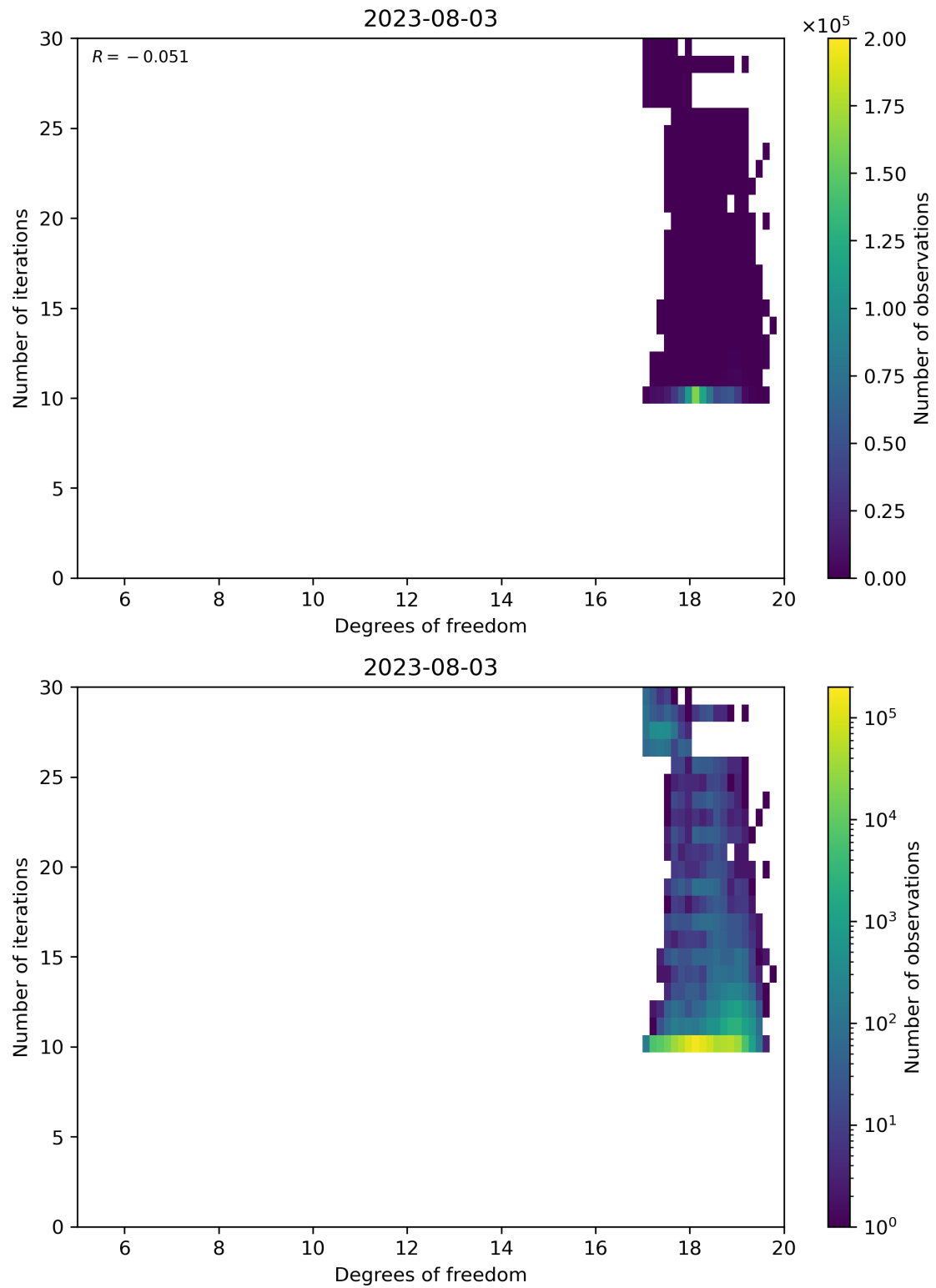
Figure 52: Scatter density plot of “Degrees of freedom” against “Number of iterations” for 2023-08-02 to 2023-08-04.
