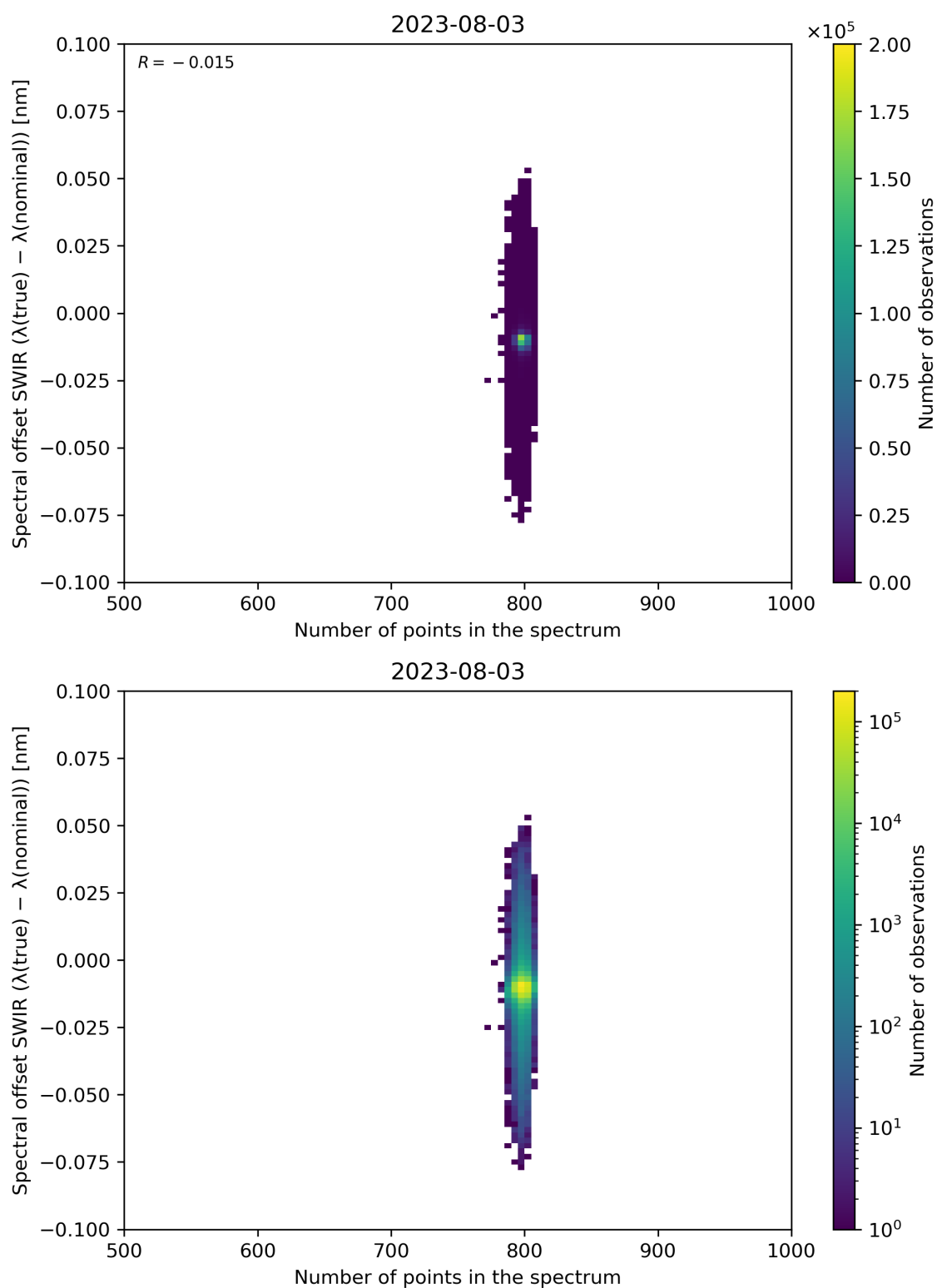
Figure 93: Scatter density plot of “Number of points in the spectrum” against “Spectral offset SWIR ( \lambda(\text{true}) - \lambda(\text{nominal}) )” for 2023-08-02 to 2023-08-04.
