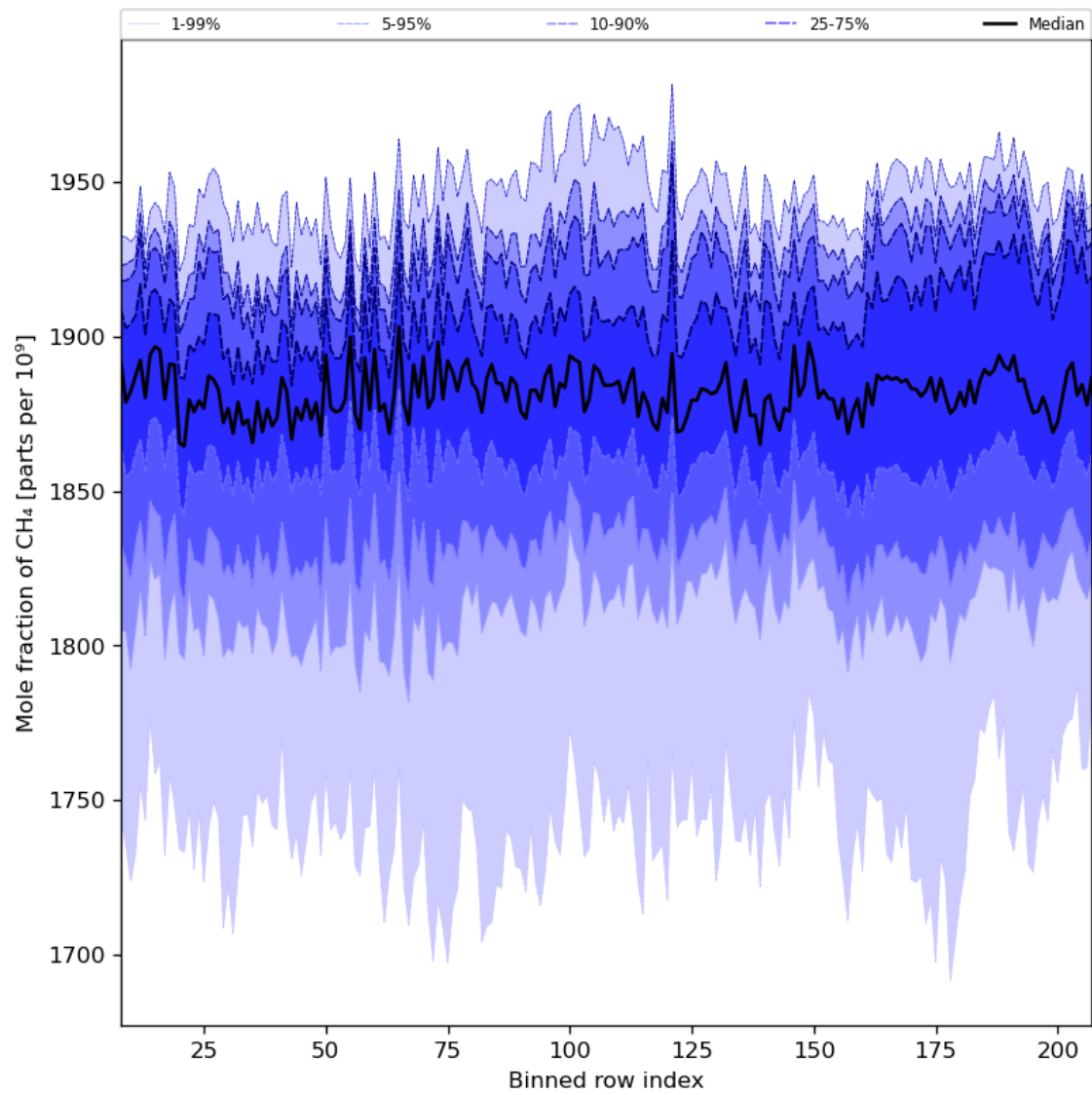
Figure 34: Along track statistics of “Mole fraction of CH 4 ” for 2023-08-02 to 2023-08-04
