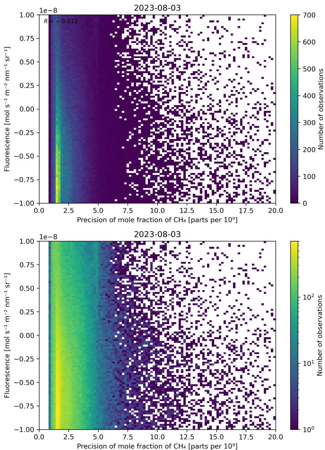
Figure 81: Scatter density plot of “Precision of mole fraction of \text{CH}_4 ” against “Fluorescence” for 2023-08-02 to 2023-08-04.
