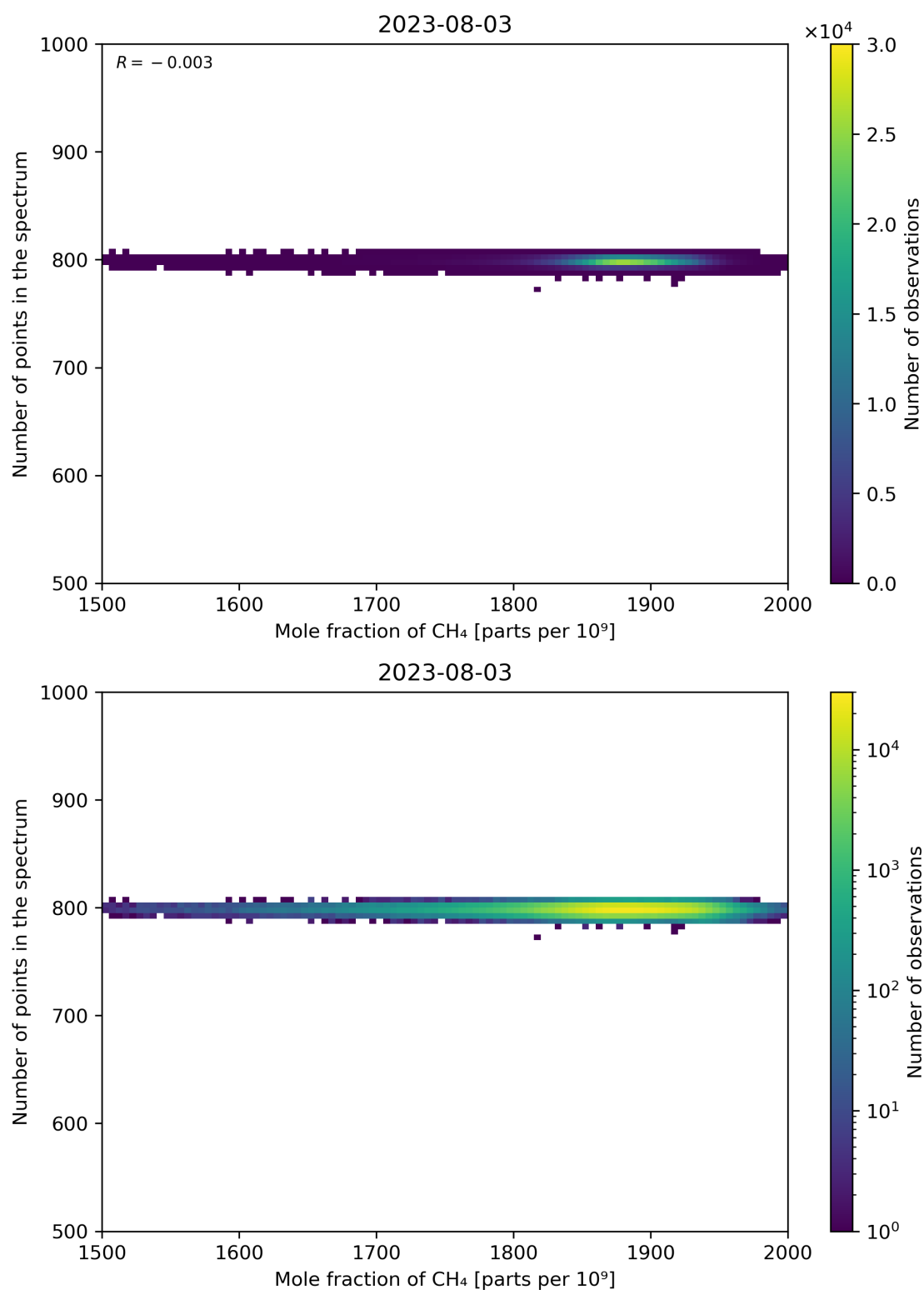
Figure 77: Scatter density plot of “Mole fraction of CH 4 ” against “Number of points in the spectrum” for 2023-08-02 to 2023-08-04.
