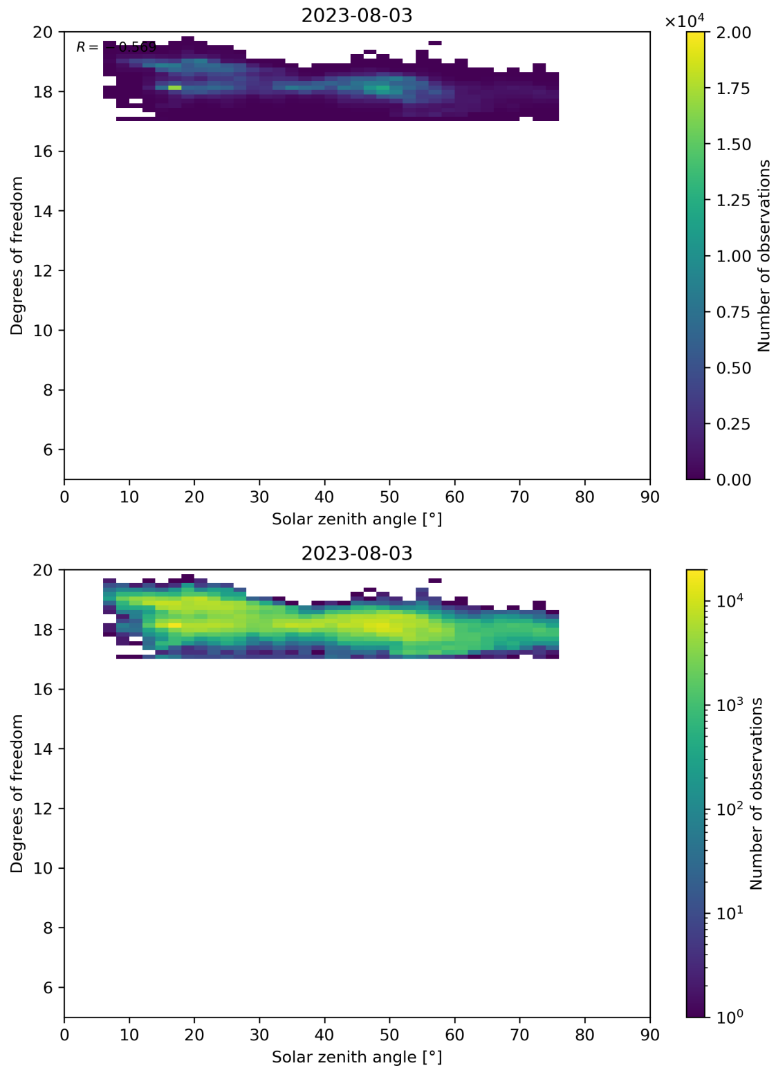
Figure 96: Scatter density plot of “Solar zenith angle” against “Degrees of freedom” for 2023-08-02 to 2023-08-04.
