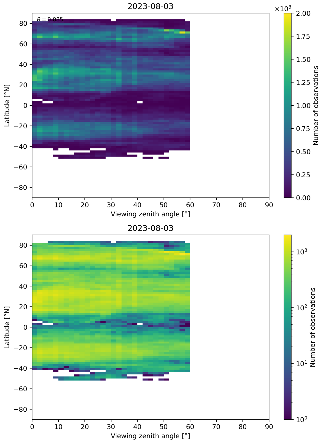
Figure 109: Scatter density plot of “Viewing zenith angle” against “Latitude” for 2023-08-02 to 2023-08-04.
