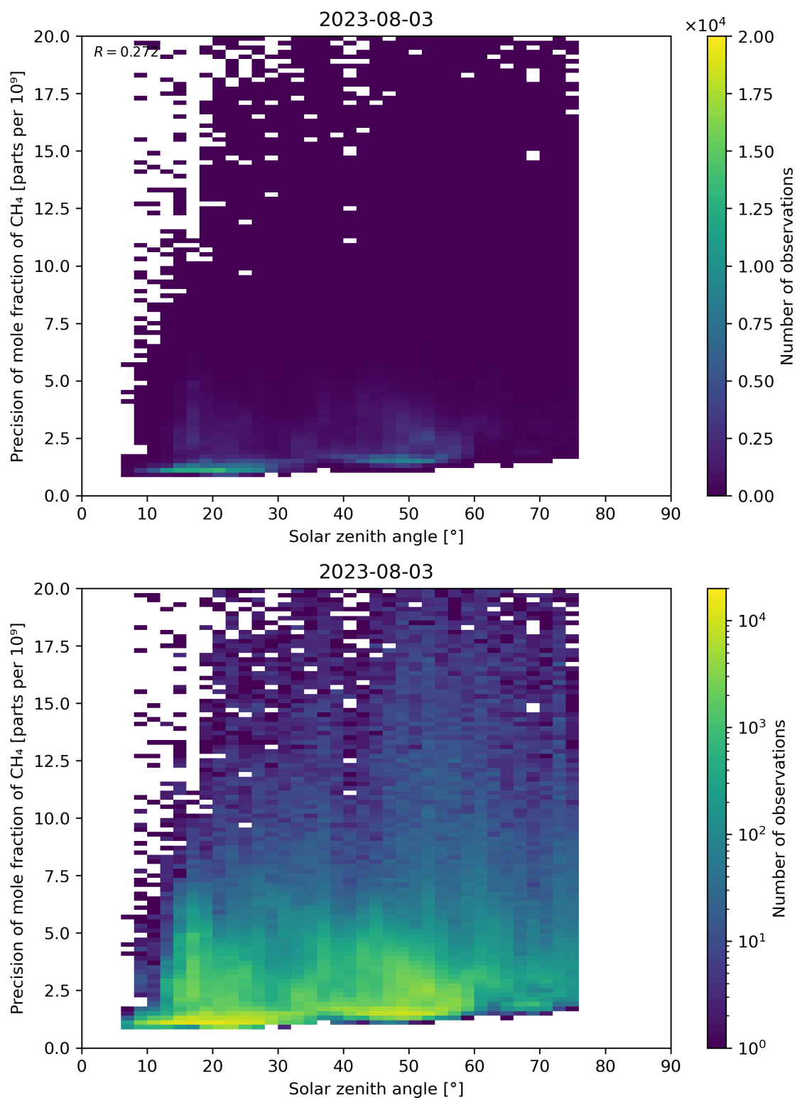
Figure 101: Scatter density plot of “Solar zenith angle” against “Precision of mole fraction of CH 4 ” for 2023-08-02 to 2023-08-04.
