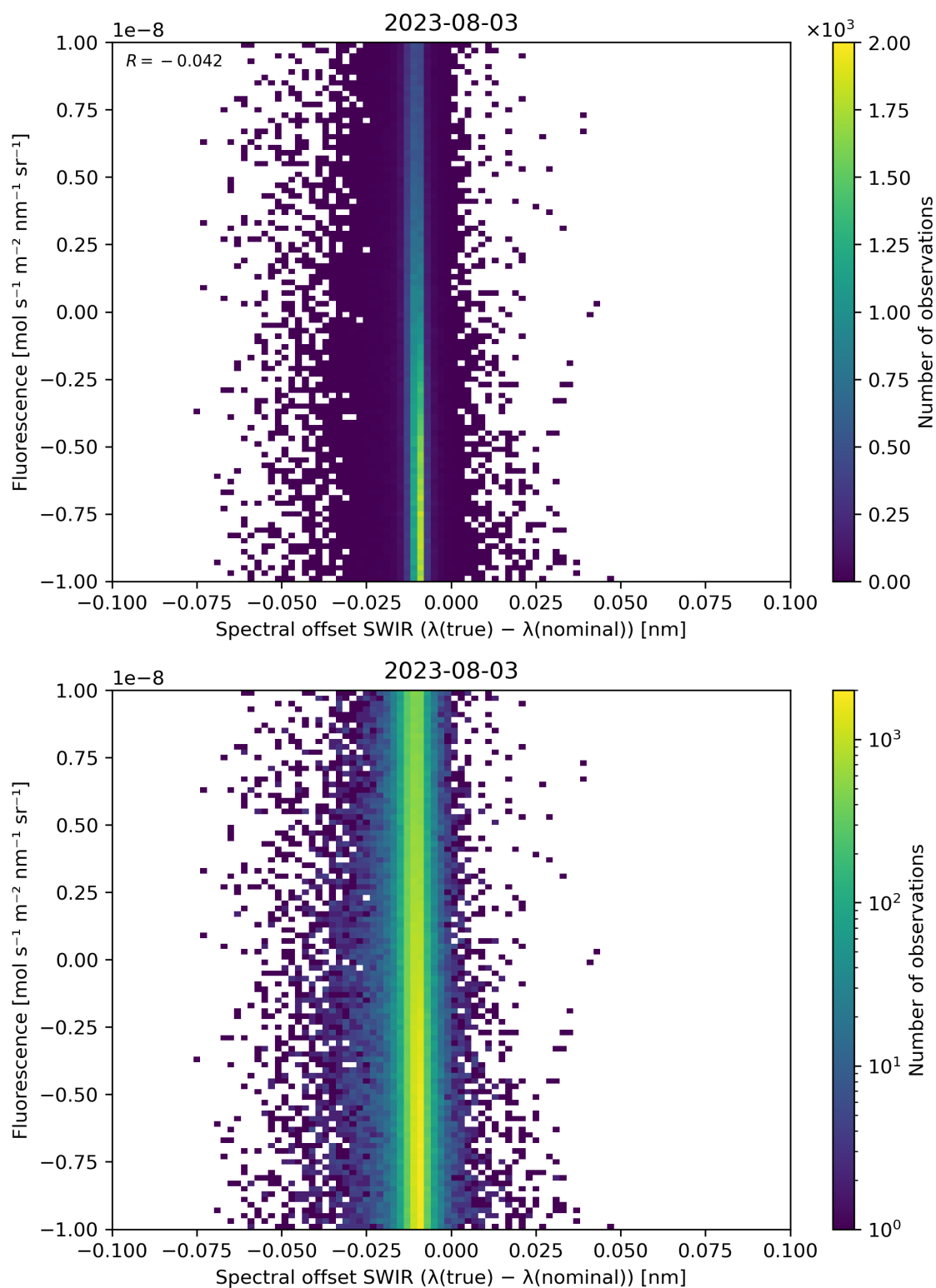
Figure 120: Scatter density plot of “Spectral offset SWIR ( \lambda(\text{true}) - \lambda(\text{nominal}) )” against “Fluorescence” for 2023-08-02 to 2023-08-04.
