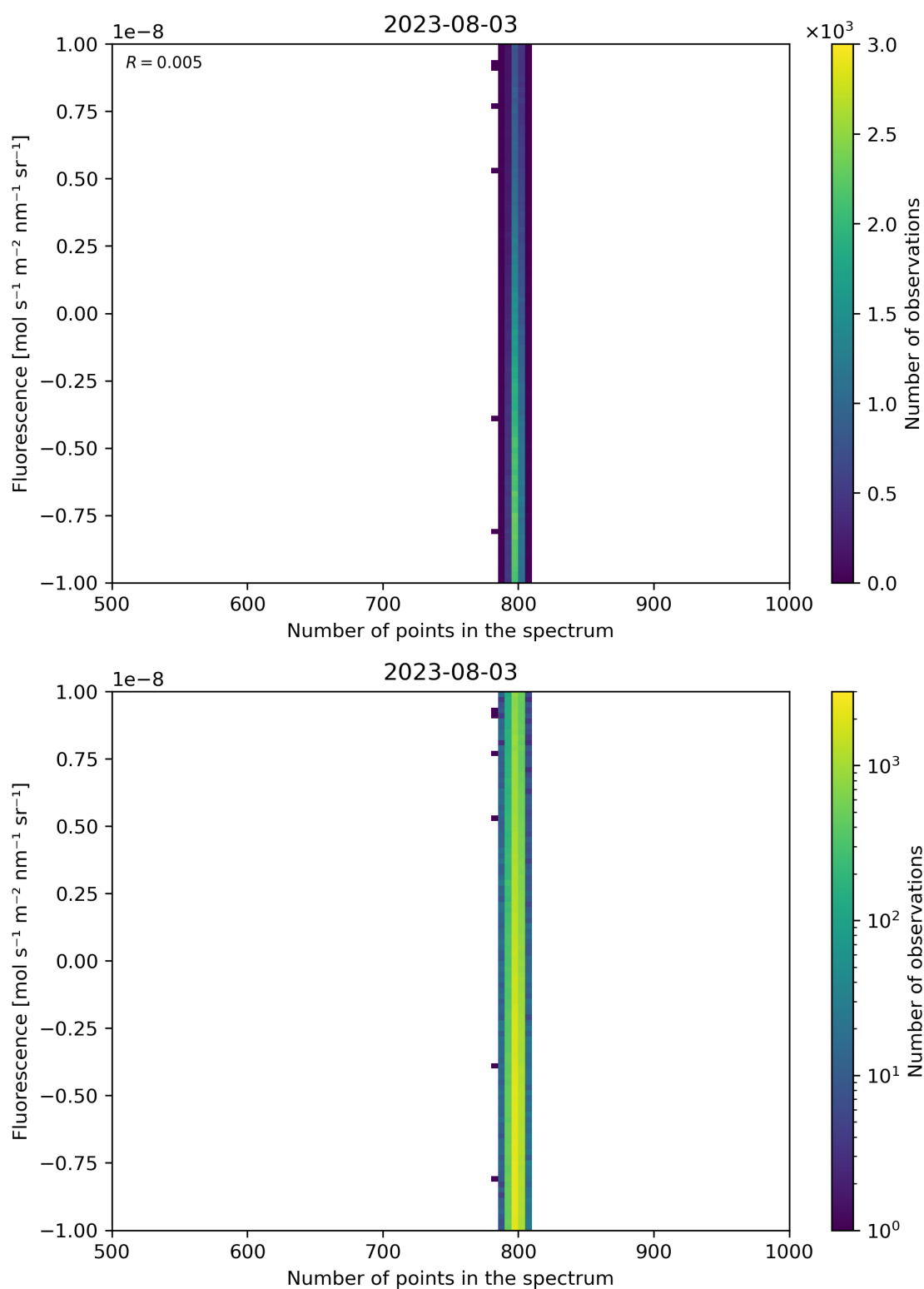
Figure 91: Scatter density plot of “Number of points in the spectrum” against “Fluorescence” for 2023-08-02 to 2023-08-04.
