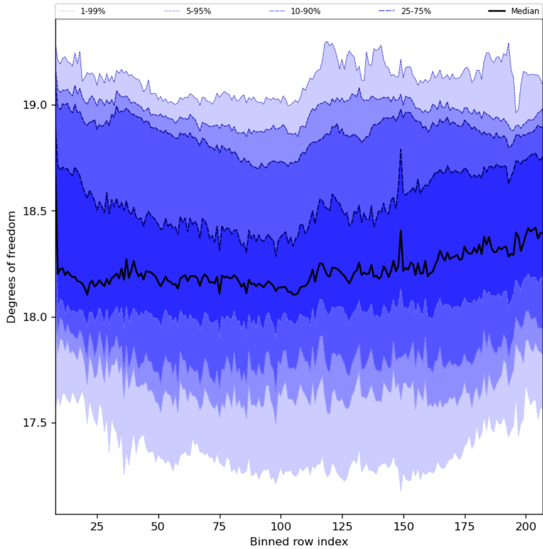
Figure 41: Along track statistics of “Degrees of freedom” for 2023-08-02 to 2023-08-04
