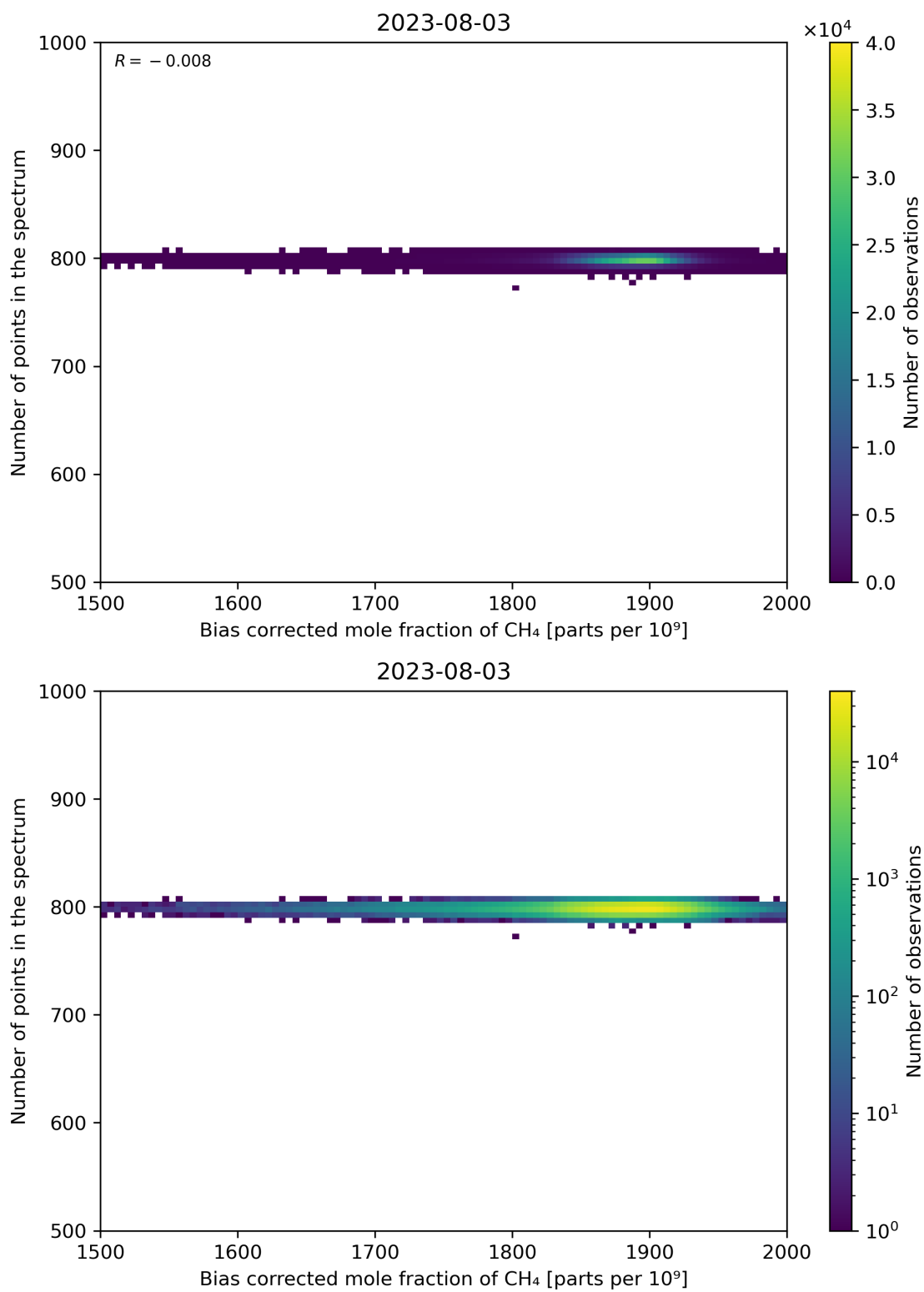
Figure 68: Scatter density plot of “Bias corrected mole fraction of CH 4 ” against “Number of points in the spectrum” for 2023-08-02 to 2023-08-04.
