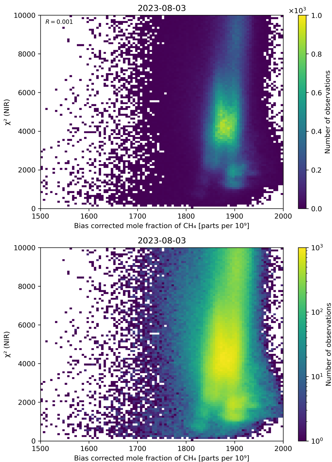
Figure 63: Scatter density plot of “Bias corrected mole fraction of CH 4 ” against “ \chi^2 (NIR)” for 2023-08-02 to 2023-08-04.
