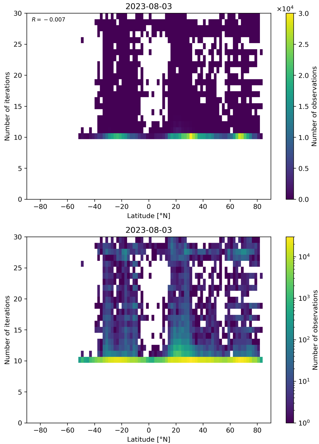
Figure 60: Scatter density plot of “Latitude” against “Number of iterations” for 2023-08-02 to 2023-08-04.
