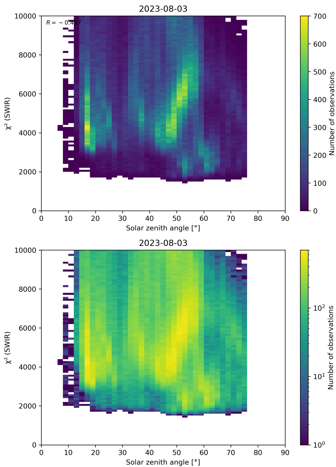
Figure 95: Scatter density plot of “Solar zenith angle” against “ \chi^2 (SWIR)” for 2023-08-02 to 2023-08-04.
