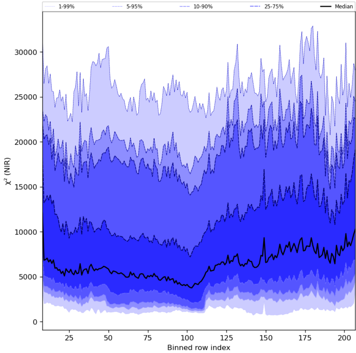
Figure 40: Along track statistics of “ \chi^2 (NIR)” for 2023-08-02 to 2023-08-04
