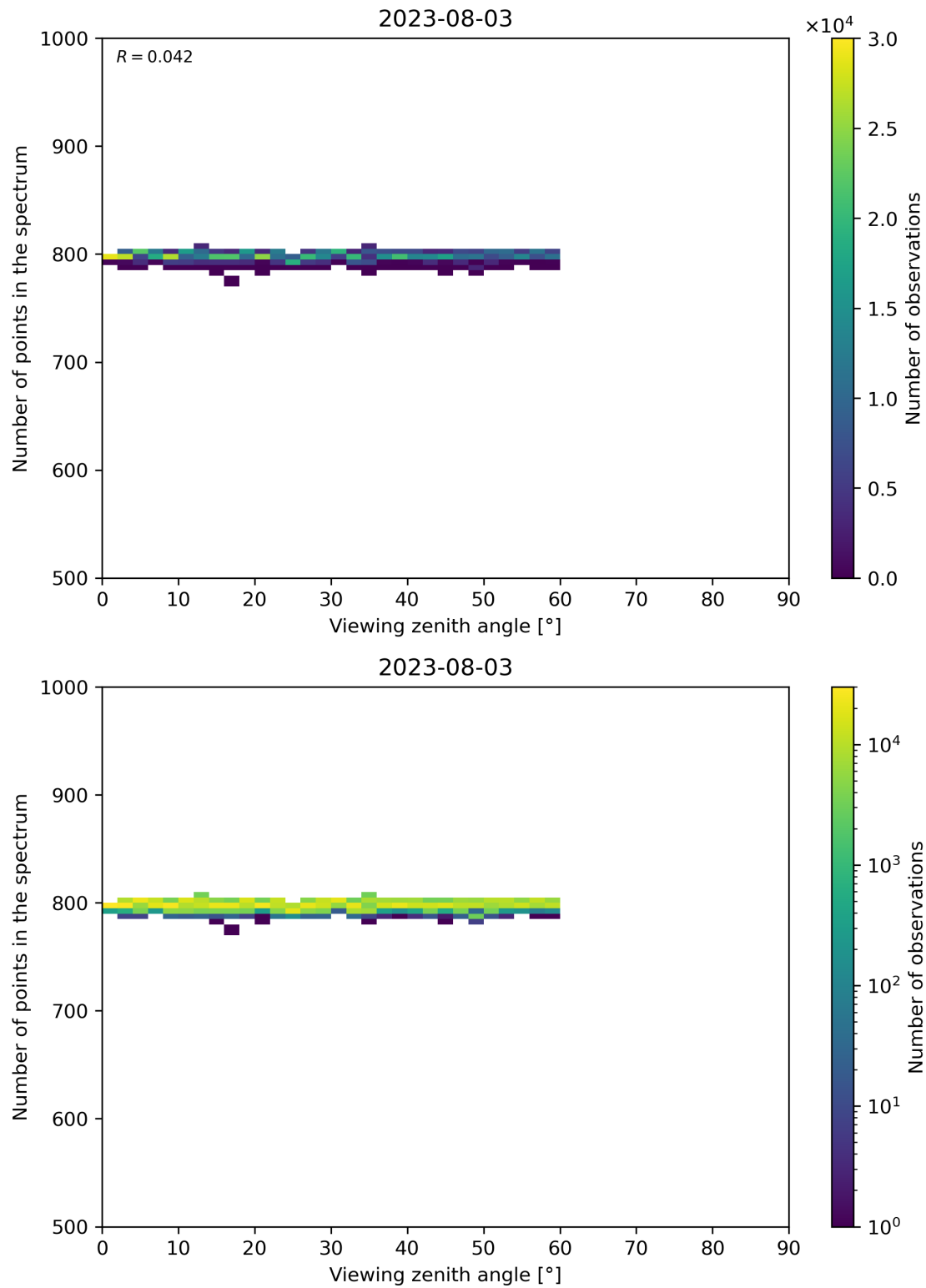
Figure 114: Scatter density plot of “Viewing zenith angle” against “Number of points in the spectrum” for 2023-08-02 to 2023-08-04.
