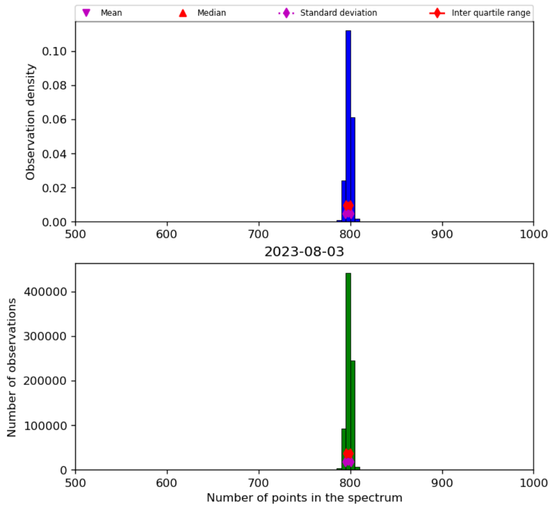
Figure 26: Histogram of “Number of points in the spectrum” for 2023-08-02 to 2023-08-04
