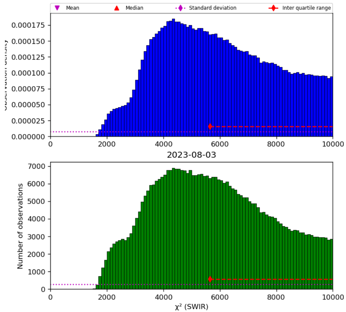
Figure 28: Histogram of “ \chi^2 (SWIR)” for 2023-08-02 to 2023-08-04
