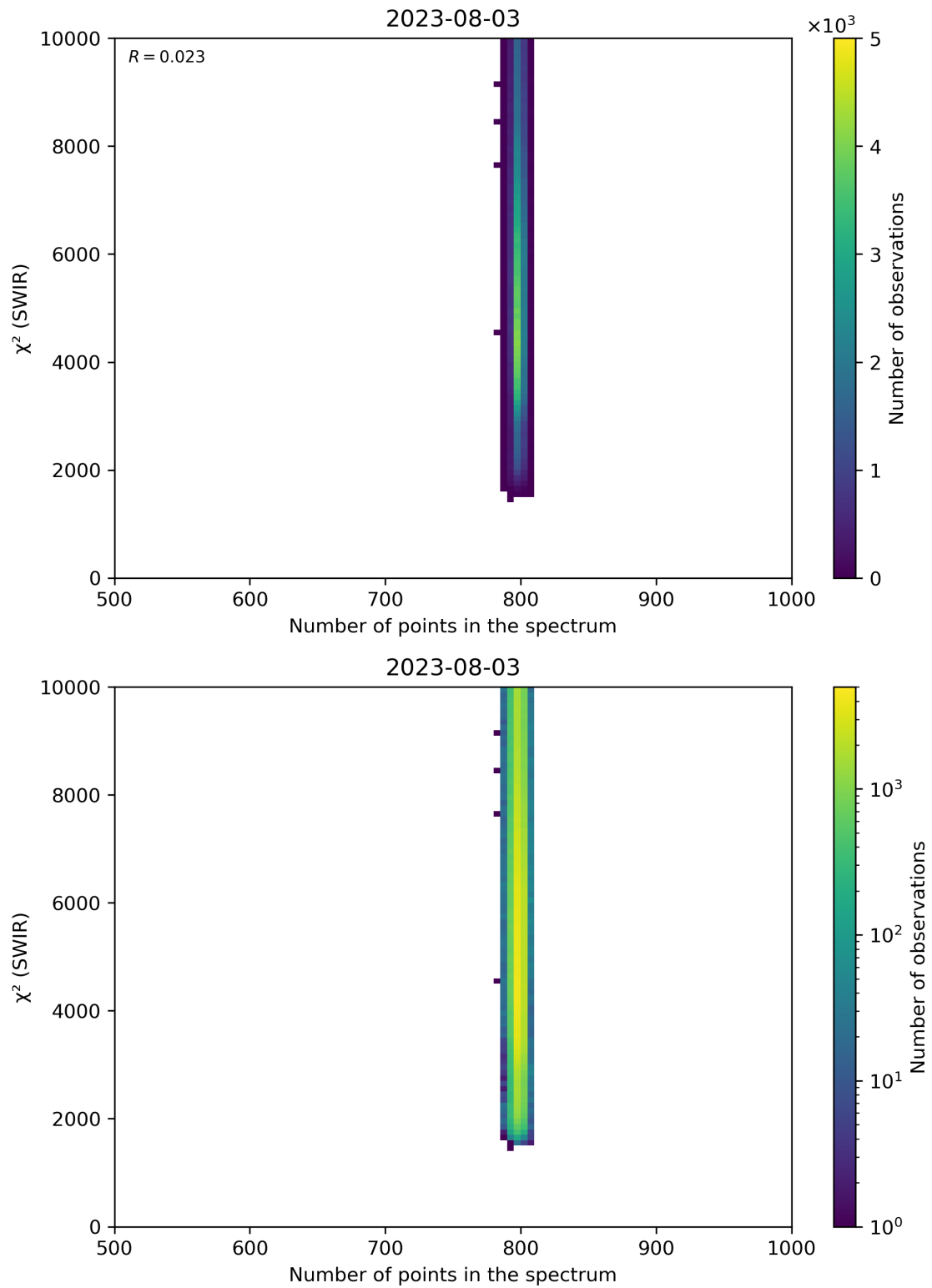
Figure 89: Scatter density plot of “Number of points in the spectrum” against “ \chi^2 (SWIR)” for 2023-08-02 to 2023-08-04.
