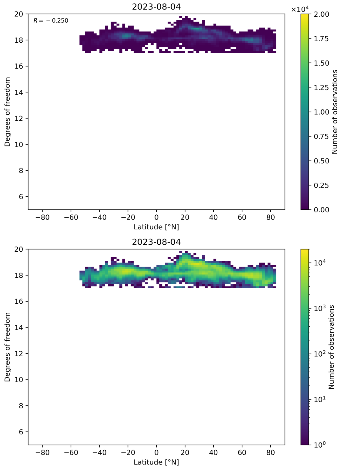
Figure 55: Scatter density plot of “Latitude” against “Degrees of freedom” for 2023-08-04 to 2023-08-05.
