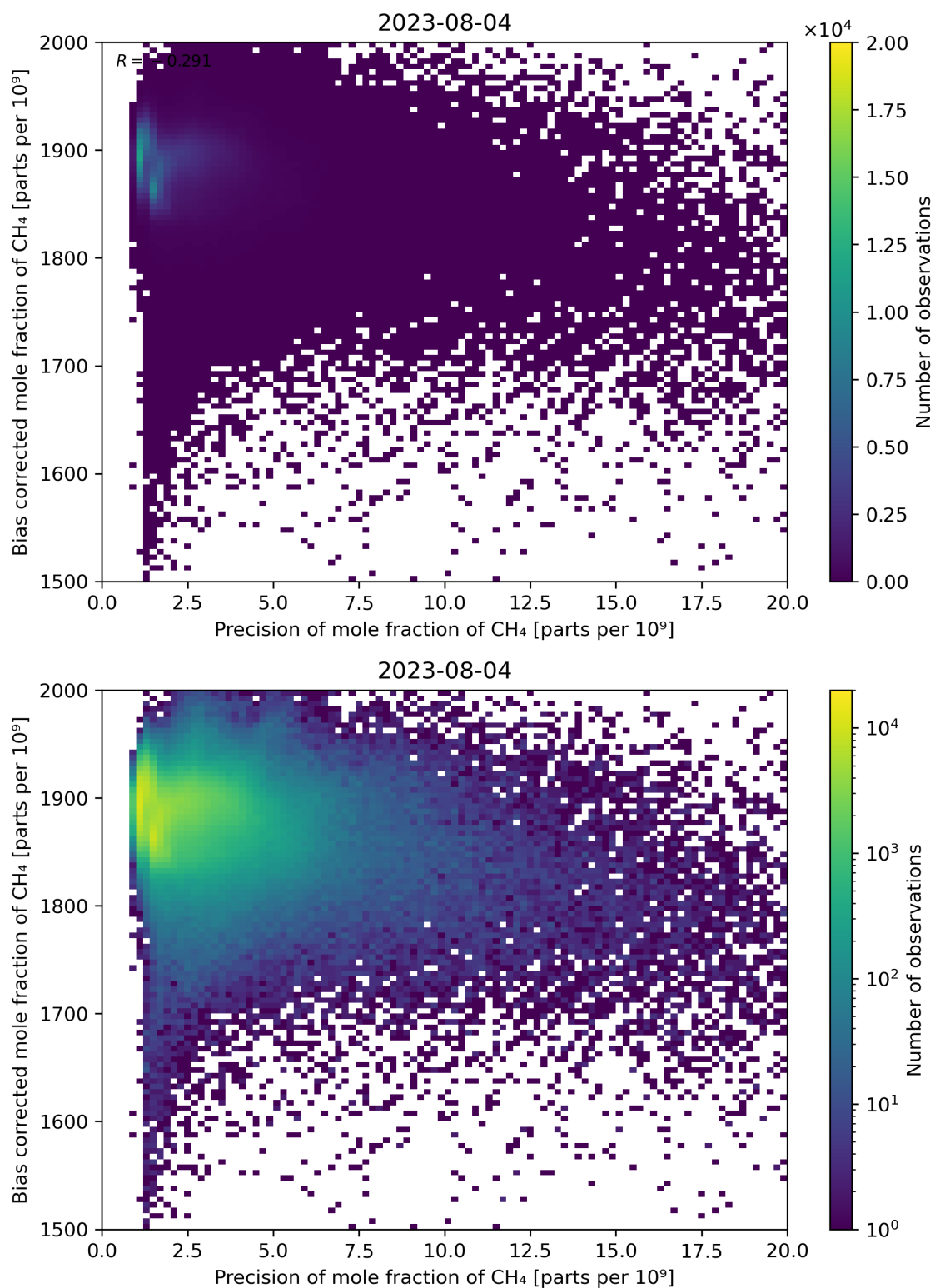
Figure 82: Scatter density plot of “Precision of mole fraction of CH 4 ” against “Bias corrected mole fraction of CH 4 ” for 2023-08-04 to 2023-08-05.
