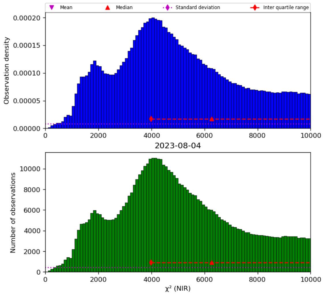
Figure 29: Histogram of " \chi^2 (NIR)" for 2023-08-04 to 2023-08-05
