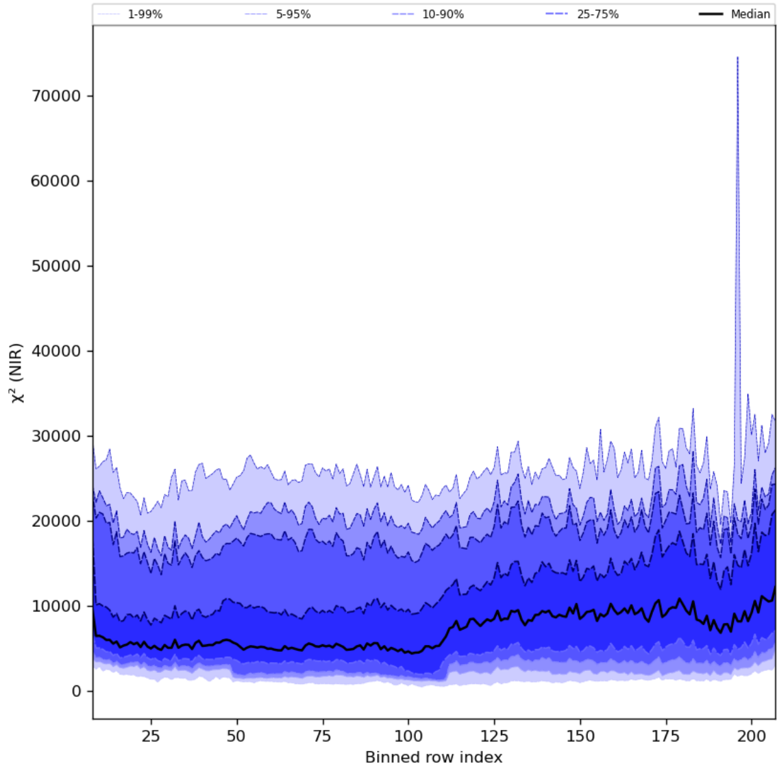
Figure 40: Along track statistics of “ \chi^2 (NIR)” for 2023-08-04 to 2023-08-05
