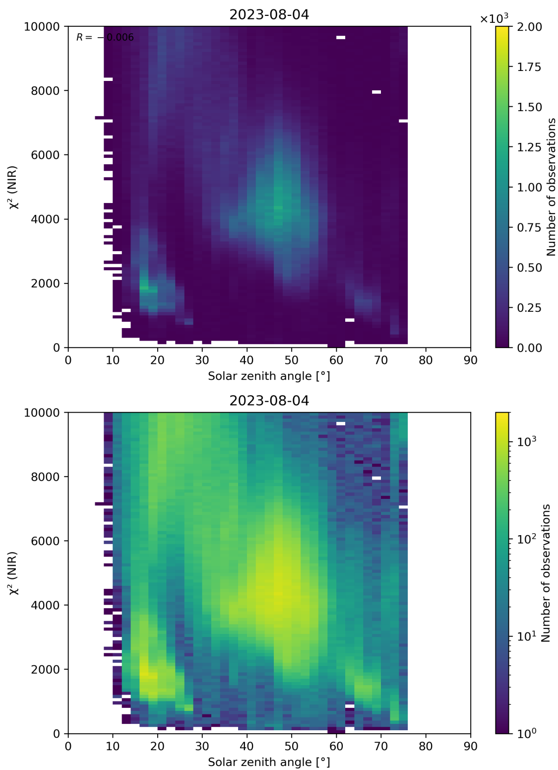
Figure 94: Scatter density plot of “Solar zenith angle” against “ \chi^2 (NIR)” for 2023-08-04 to 2023-08-05.
