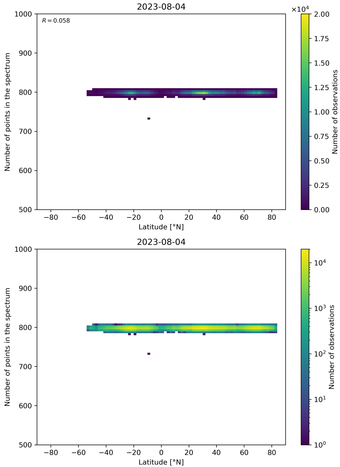
Figure 61: Scatter density plot of “Latitude” against “Number of points in the spectrum” for 2023-08-04 to 2023-08-05.
