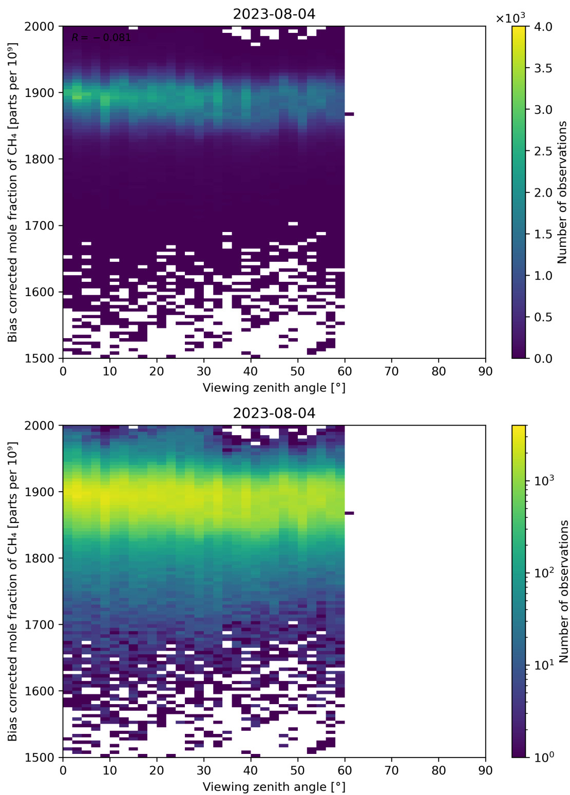
Figure 111: Scatter density plot of “Viewing zenith angle” against “Bias corrected mole fraction of CH 4 ” for 2023-08-04 to 2023-08-05.
