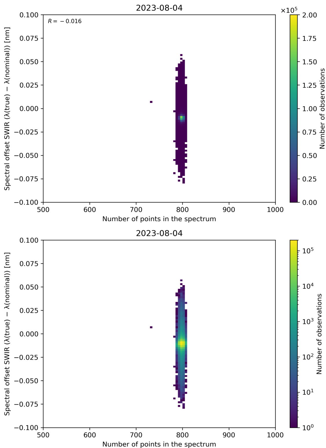
Figure 93: Scatter density plot of “Number of points in the spectrum” against “Spectral offset SWIR ( \lambda(\text{true}) - \lambda(\text{nominal}) )” for 2023-08-04 to 2023-08-05.
