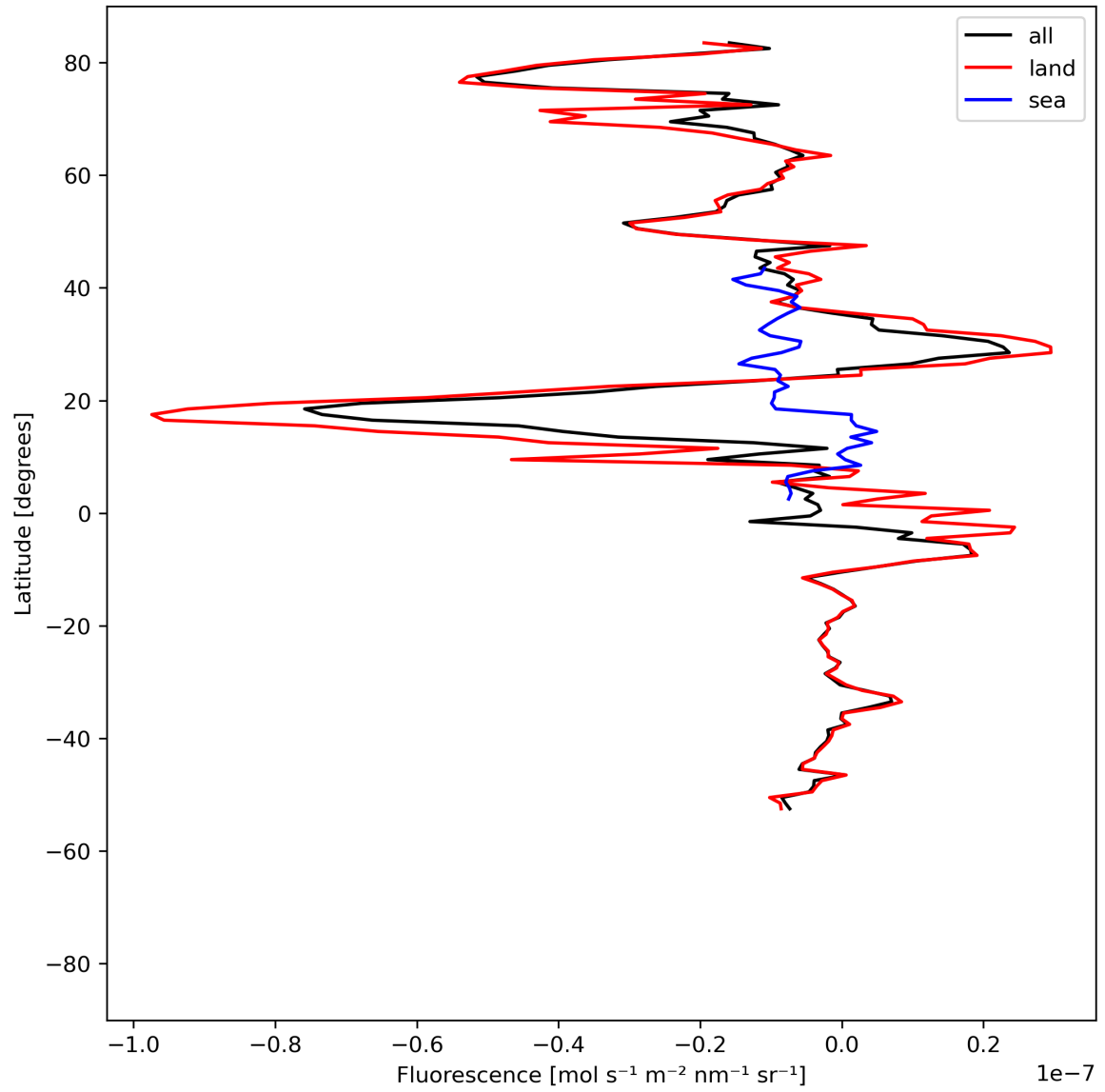
Figure 21: Zonal average of “Fluorescence” for 2023-08-04 to 2023-08-05.
