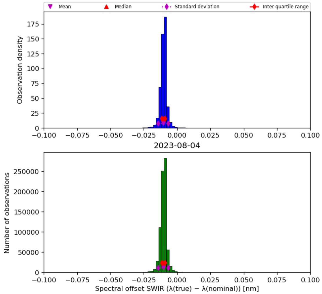
Figure 27: Histogram of “Spectral offset SWIR ( \lambda(\text{true}) - \lambda(\text{nominal}) )” for 2023-08-04 to 2023-08-05
