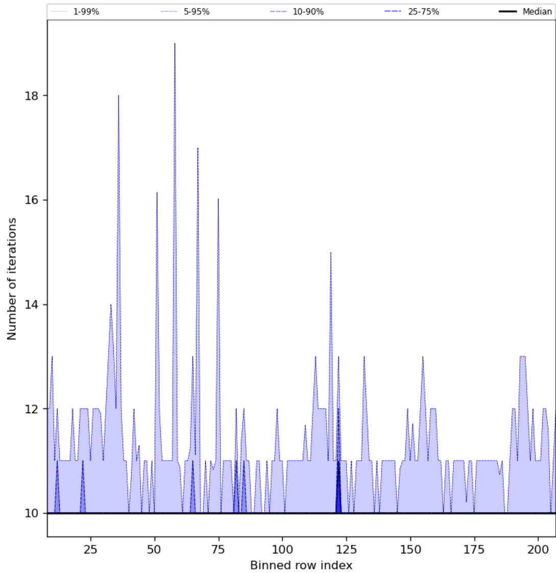
Figure 42: Along track statistics of “Number of iterations” for 2023-08-04 to 2023-08-05
