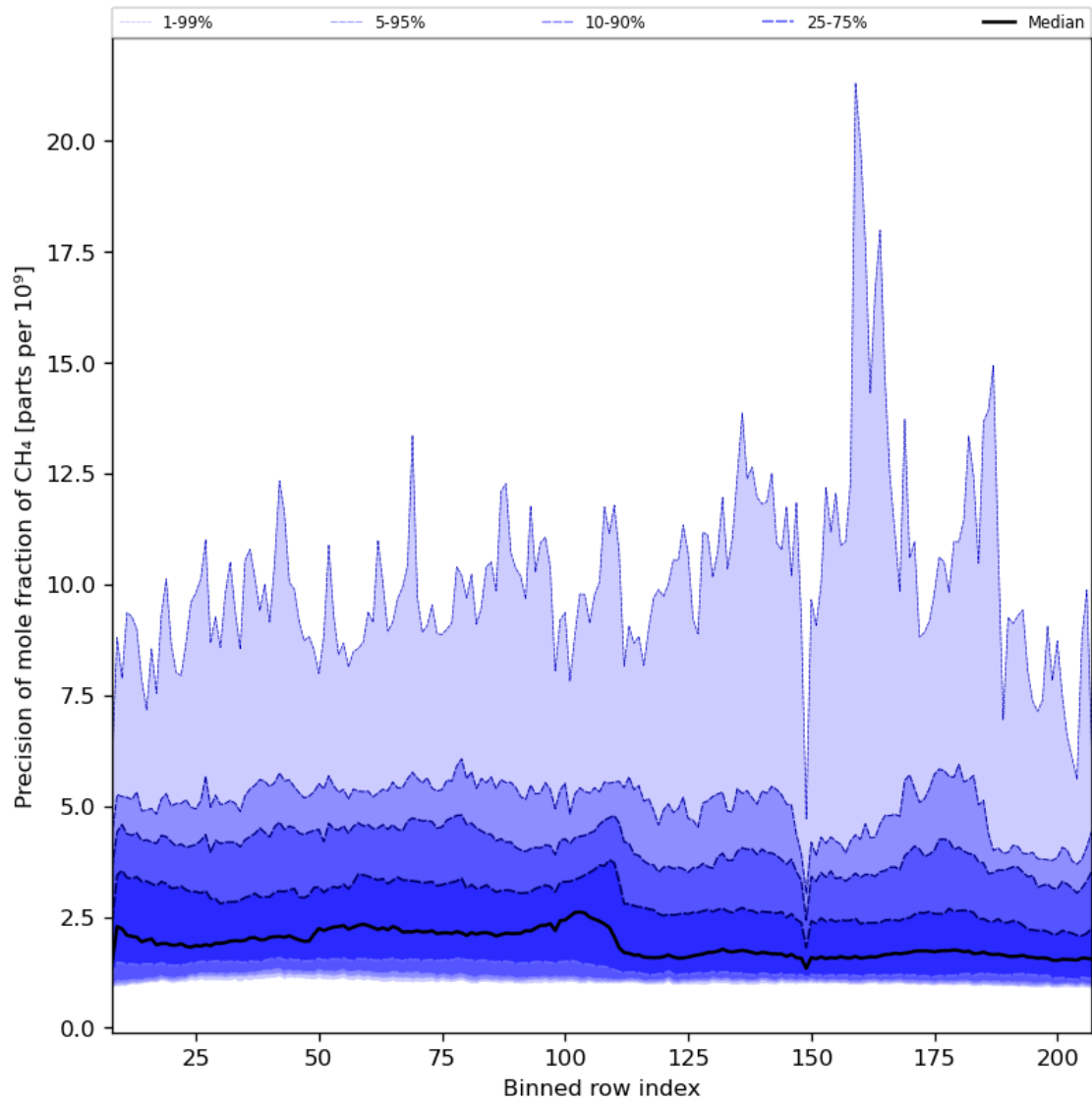
Figure 35: Along track statistics of “Precision of mole fraction of CH 4 ” for 2023-08-04 to 2023-08-05
