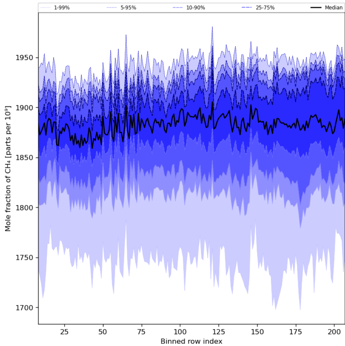
Figure 34: Along track statistics of “Mole fraction of CH 4 ” for 2023-08-04 to 2023-08-05
