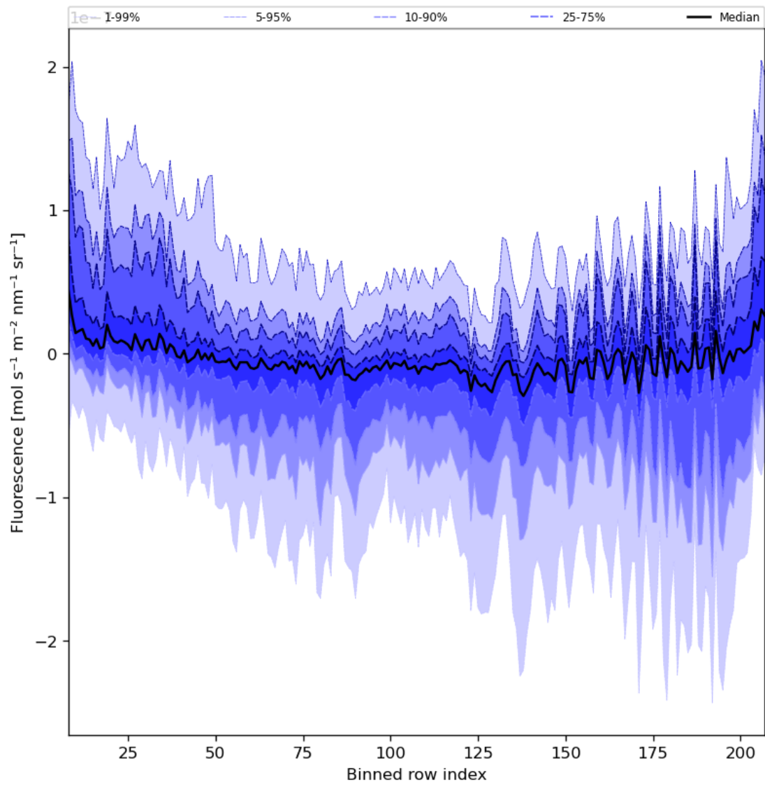
Figure 43: Along track statistics of “Fluorescence” for 2023-08-04 to 2023-08-05
