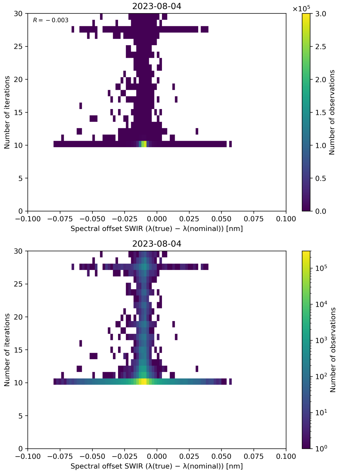
Figure 121: Scatter density plot of “Spectral offset SWIR ( \lambda(\text{true}) - \lambda(\text{nominal}) )” against “Number of iterations” for 2023-08-04 to 2023-08-05.
