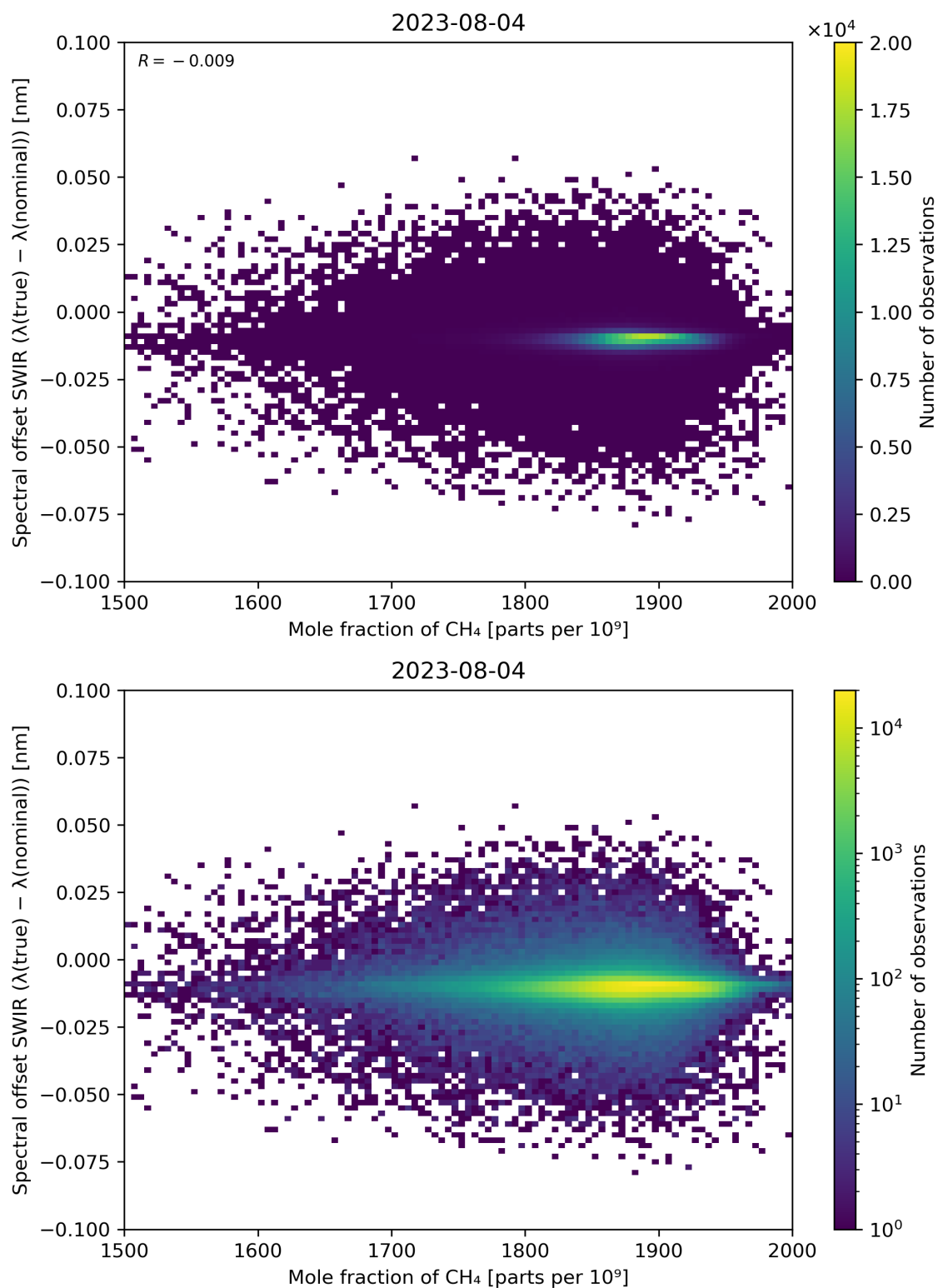
Figure 86: Scatter density plot of “Mole fraction of CH 4 ” against “Spectral offset SWIR ( \lambda(\text{true}) - \lambda(\text{nominal}) )” for 2023-08-04 to 2023-08-05.
