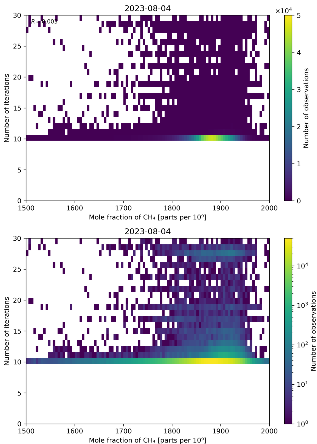
Figure 76: Scatter density plot of “Mole fraction of CH 4 ” against “Number of iterations” for 2023-08-04 to 2023-08-05.
