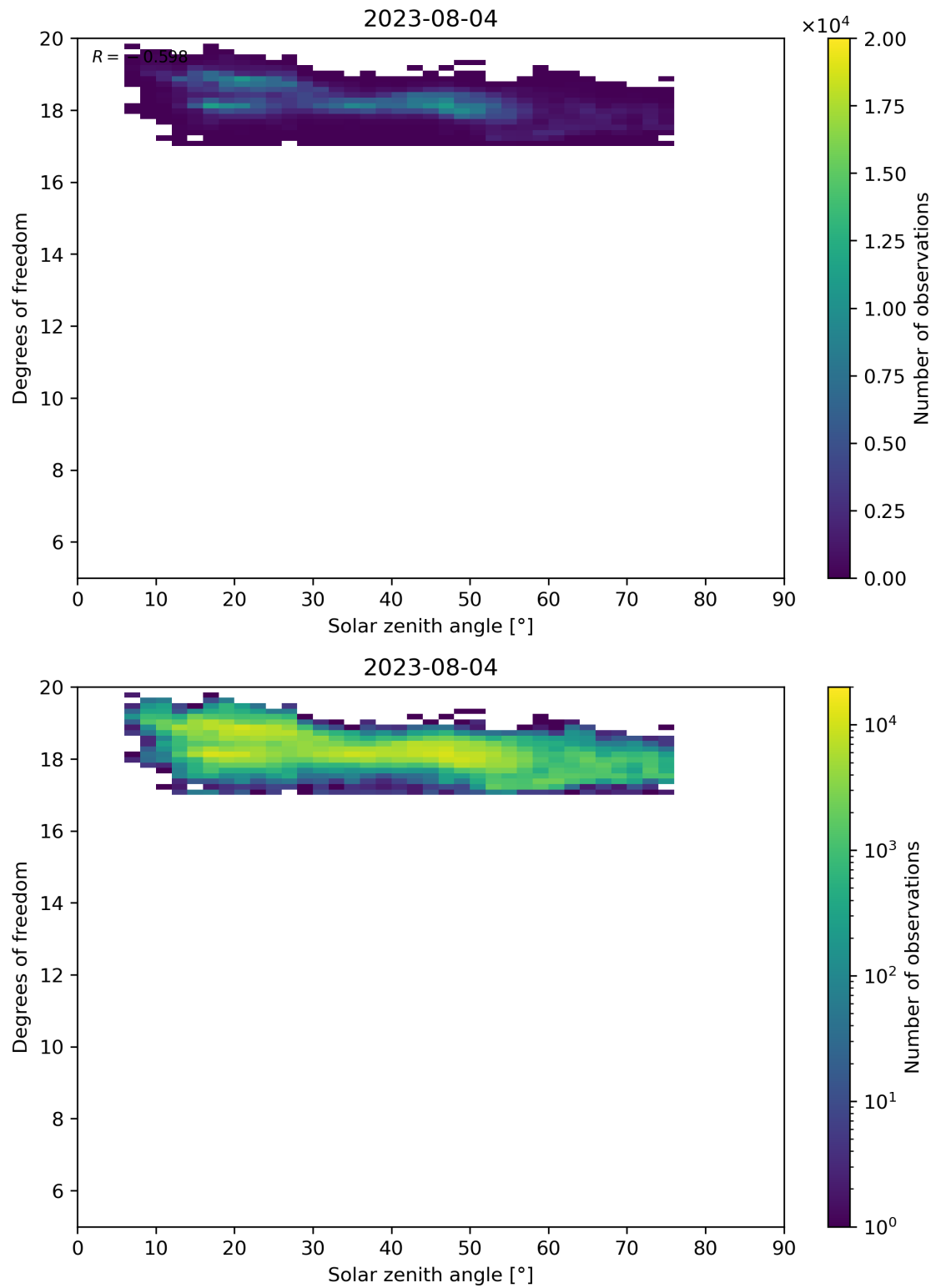
Figure 96: Scatter density plot of “Solar zenith angle” against “Degrees of freedom” for 2023-08-04 to 2023-08-05.
