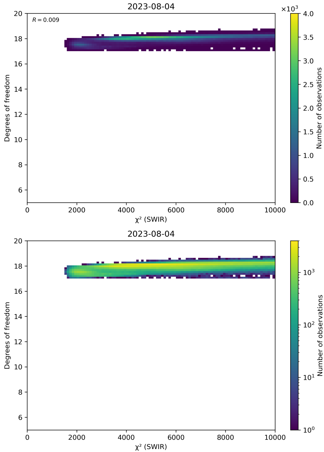
Figure 48: Scatter density plot of “ \chi^2 (SWIR)” against “Degrees of freedom” for 2023-08-04 to 2023-08-05.
