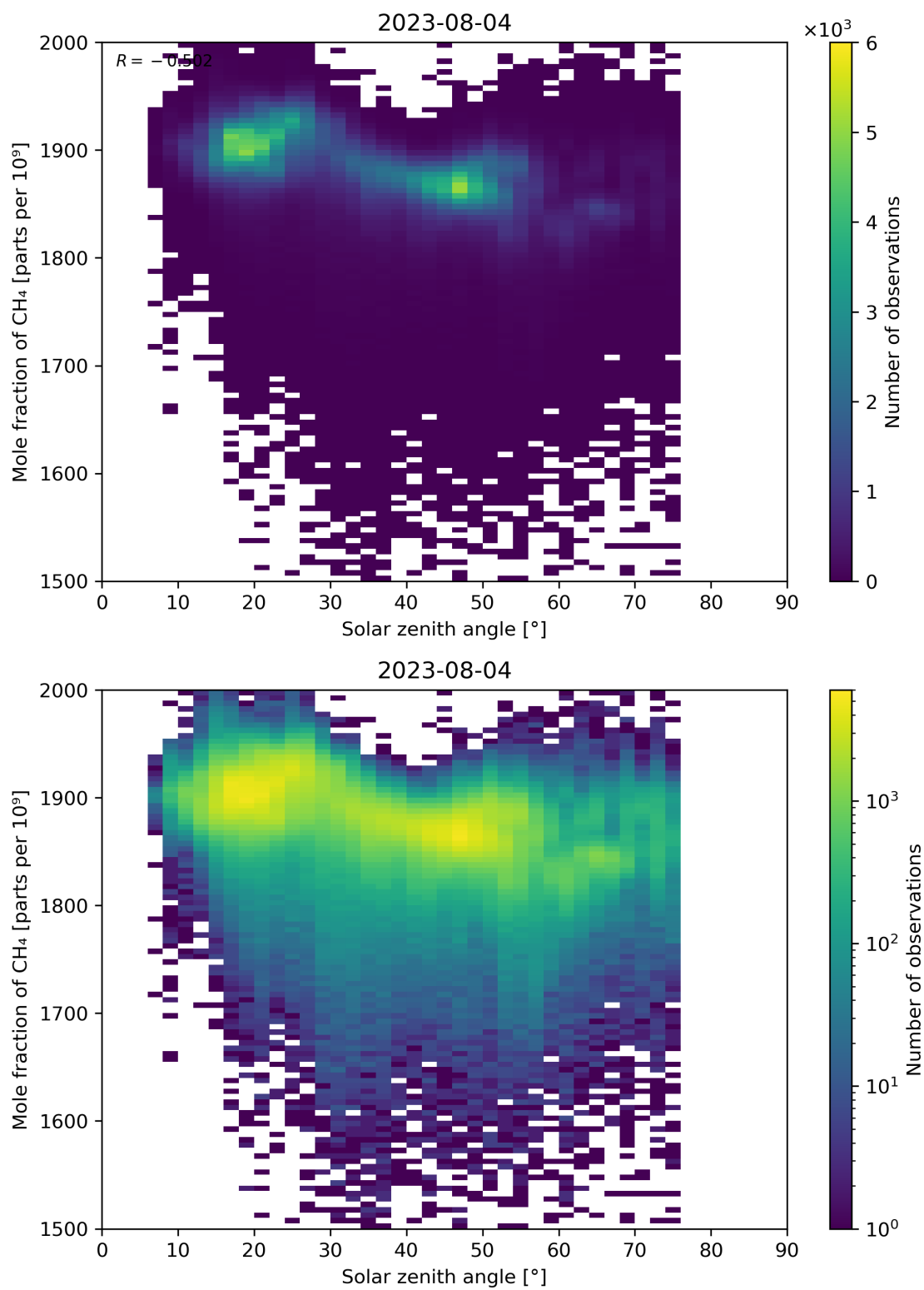
Figure 99: Scatter density plot of “Solar zenith angle” against “Mole fraction of \text{CH}_4 ” for 2023-08-04 to 2023-08-05.
