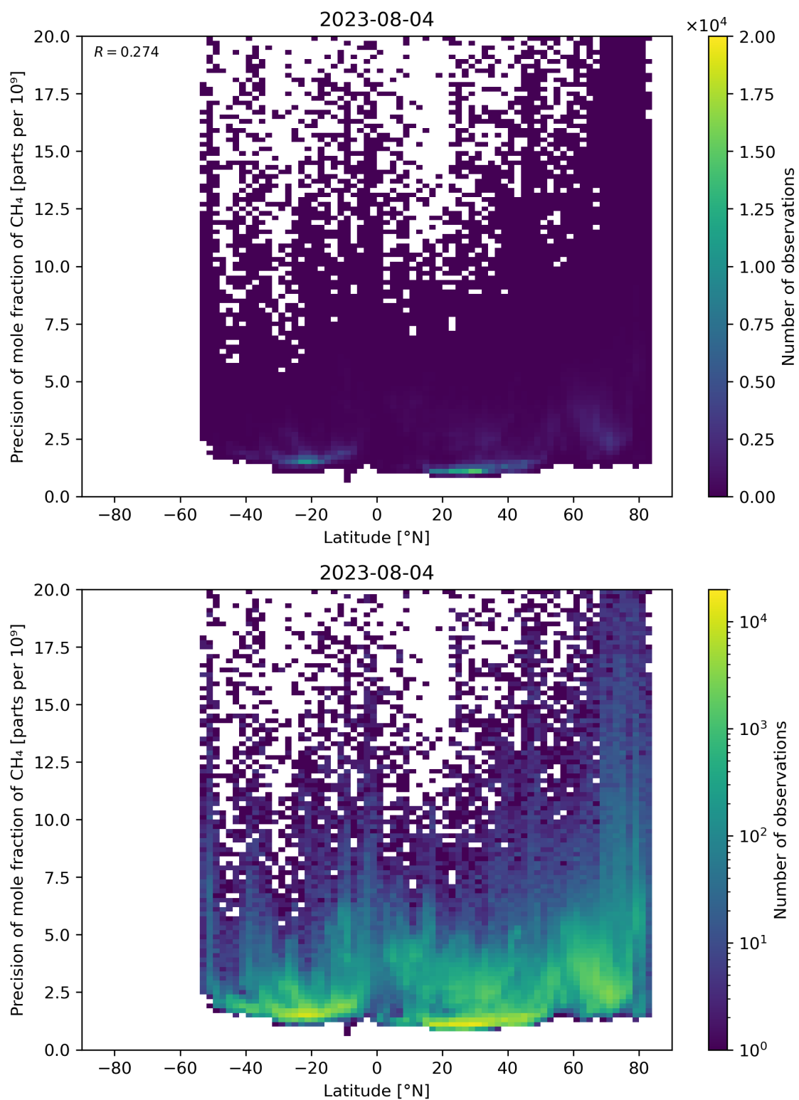
Figure 59: Scatter density plot of “Latitude” against “Precision of mole fraction of \text{CH}_4 ” for 2023-08-04 to 2023-08-05.
