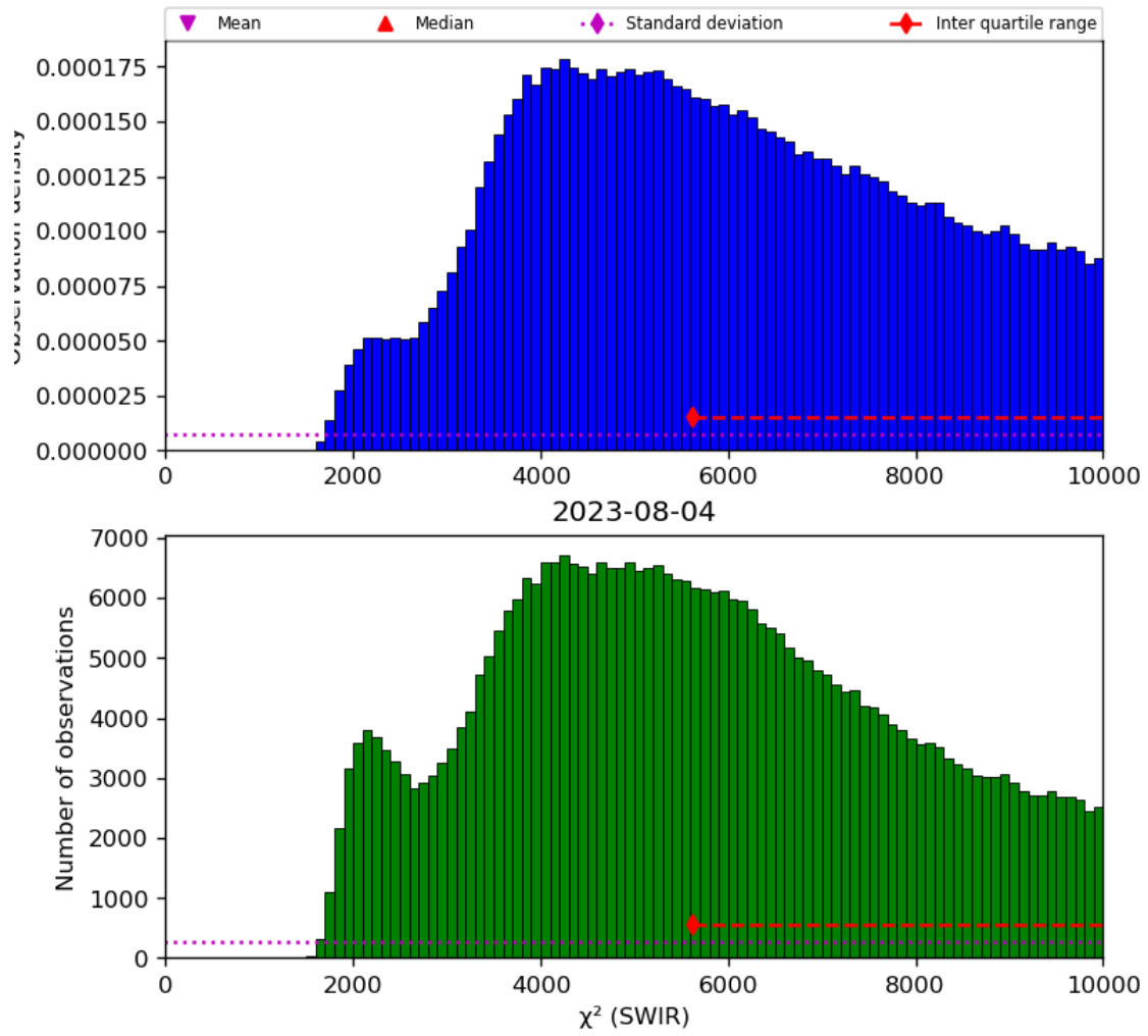
Figure 28: Histogram of “ \chi^2 (SWIR)” for 2023-08-04 to 2023-08-05
