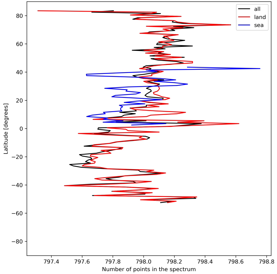
Figure 15: Zonal average of “Number of points in the spectrum” for 2023-08-04 to 2023-08-05.
