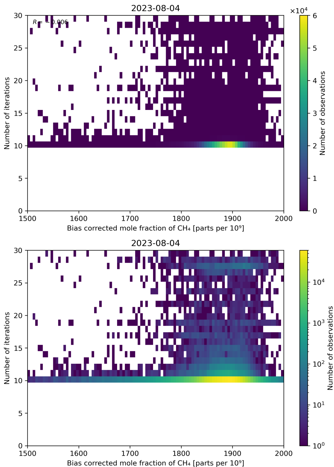
Figure 67: Scatter density plot of “Bias corrected mole fraction of CH 4 ” against “Number of iterations” for 2023-08-04 to 2023-08-05.
