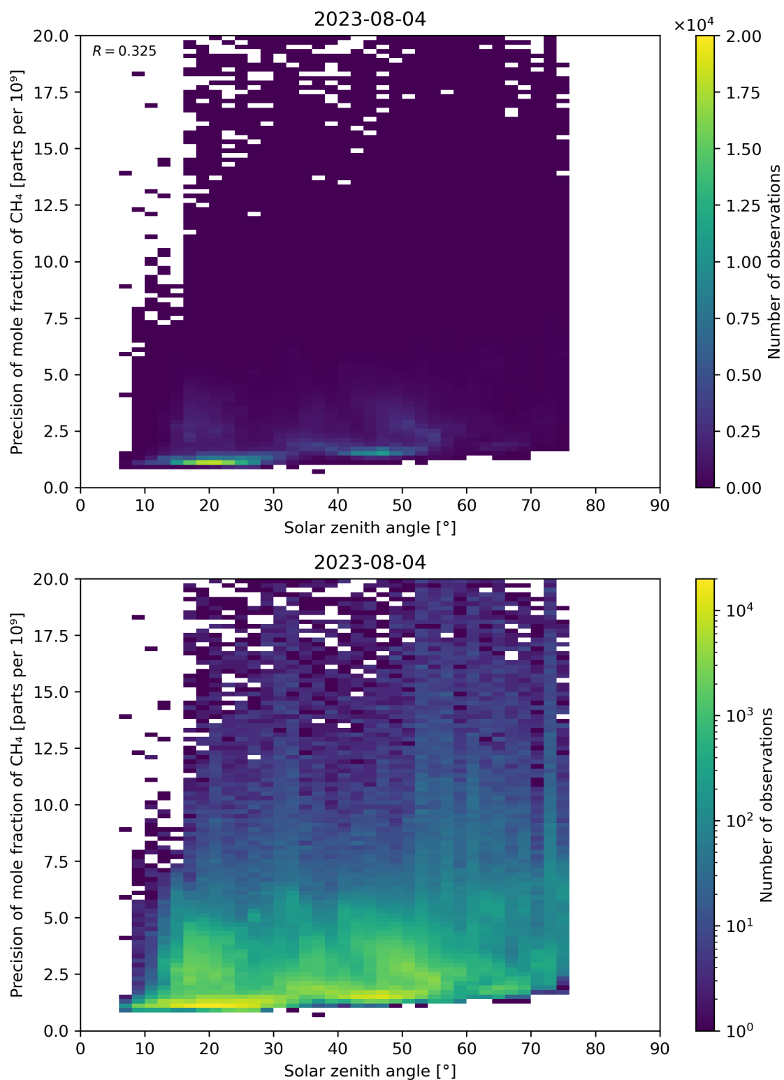
Figure 101: Scatter density plot of “Solar zenith angle” against “Precision of mole fraction of CH 4 ” for 2023-08-04 to 2023-08-05.
