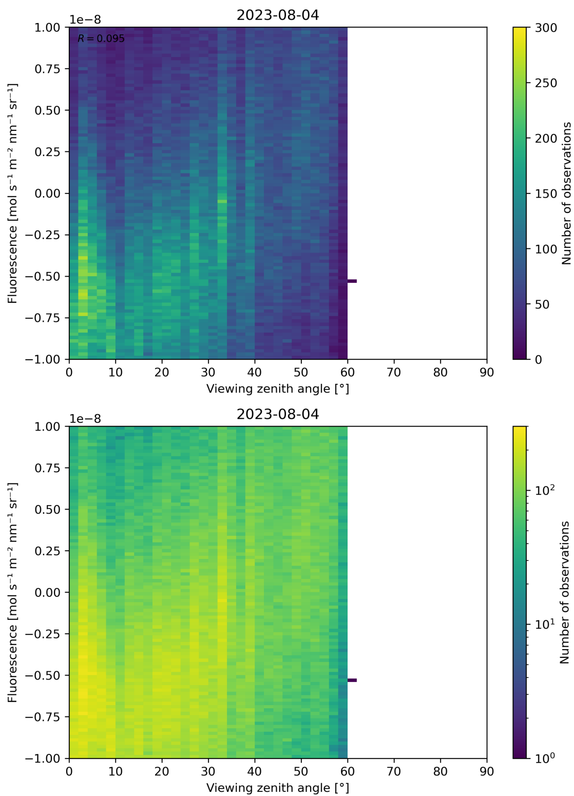
Figure 108: Scatter density plot of “Viewing zenith angle” against “Fluorescence” for 2023-08-04 to 2023-08-05.
