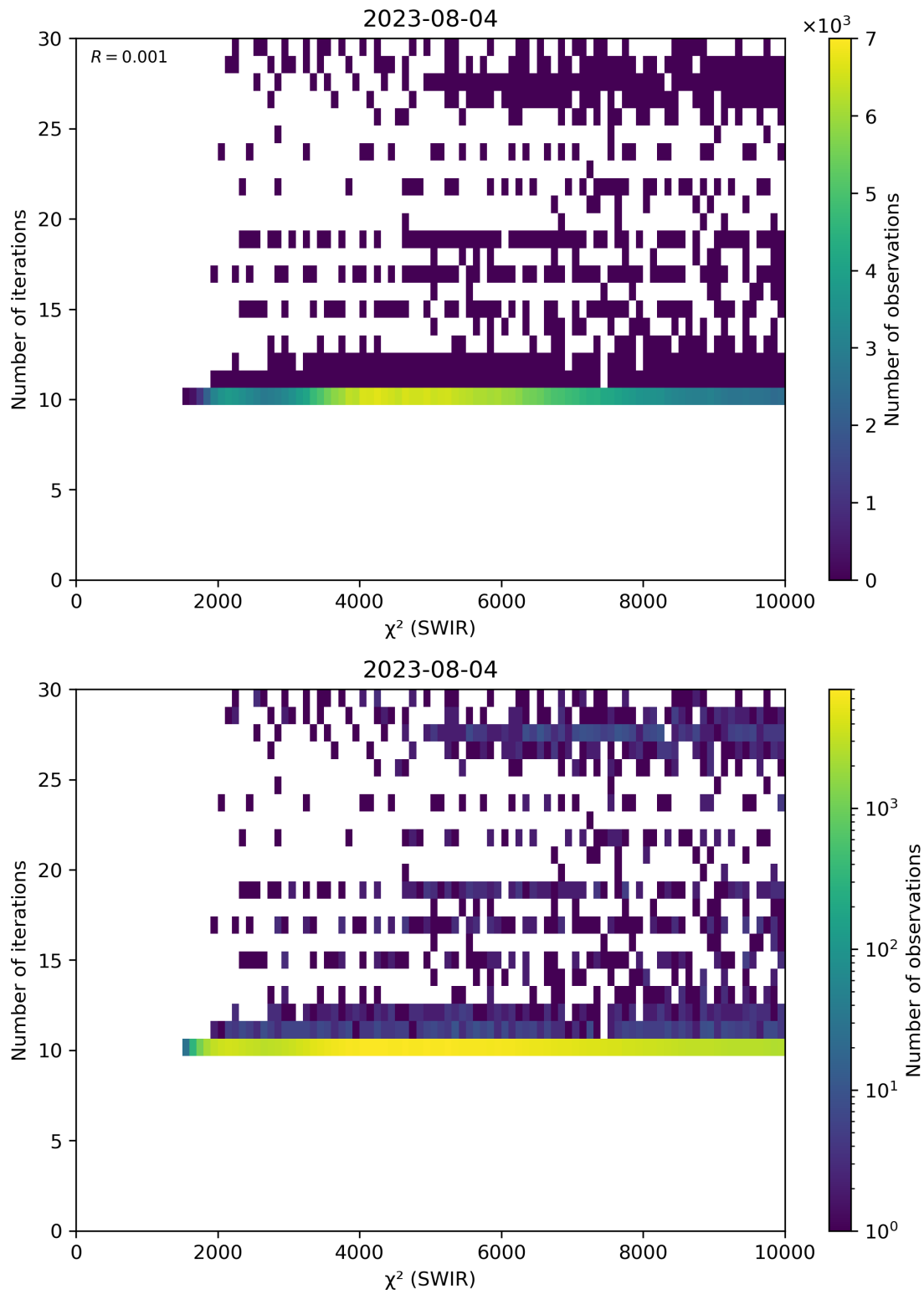
Figure 50: Scatter density plot of “ \chi^2 (SWIR)” against “Number of iterations” for 2023-08-04 to 2023-08-05.
