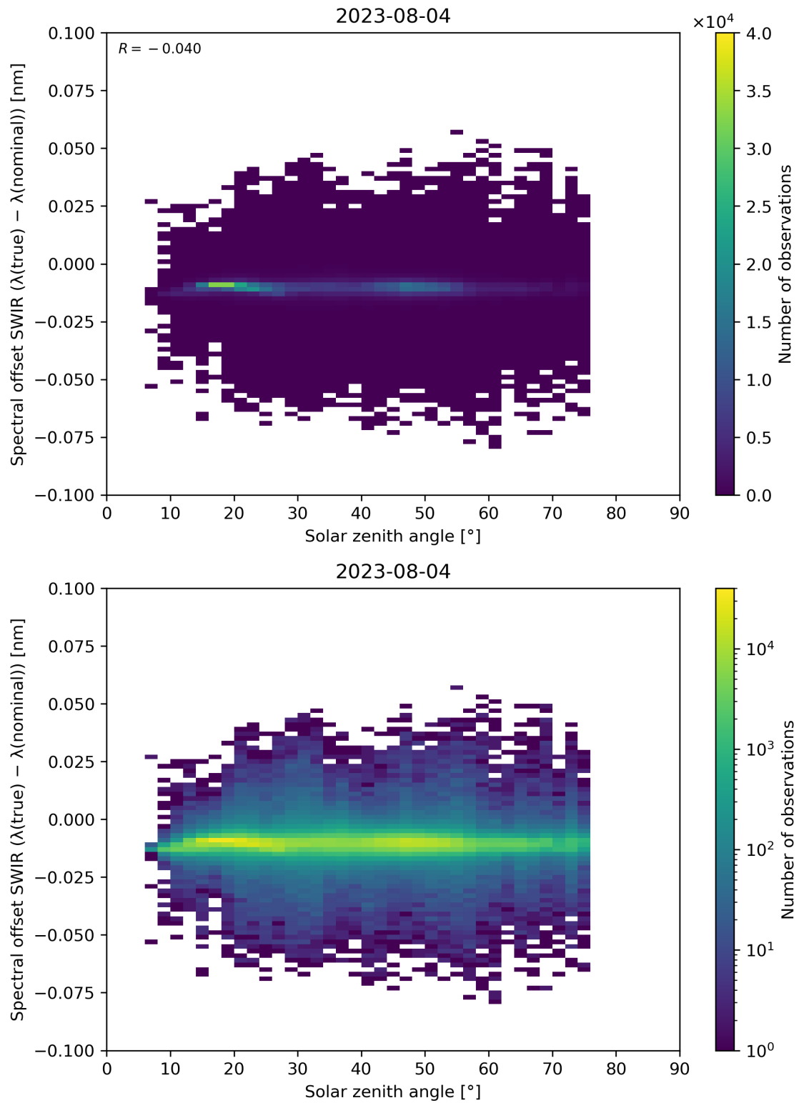
Figure 104: Scatter density plot of “Solar zenith angle” against “Spectral offset SWIR ( \lambda(\text{true}) - \lambda(\text{nominal}) )” for 2023-08-04 to 2023-08-05.
