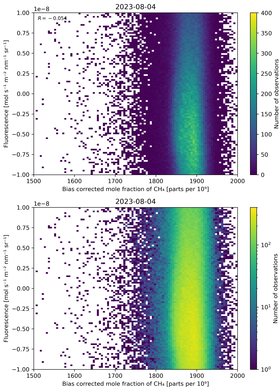
Figure 66: Scatter density plot of “Bias corrected mole fraction of \text{CH}_4 ” against “Fluorescence” for 2023-08-04 to 2023-08-05.
