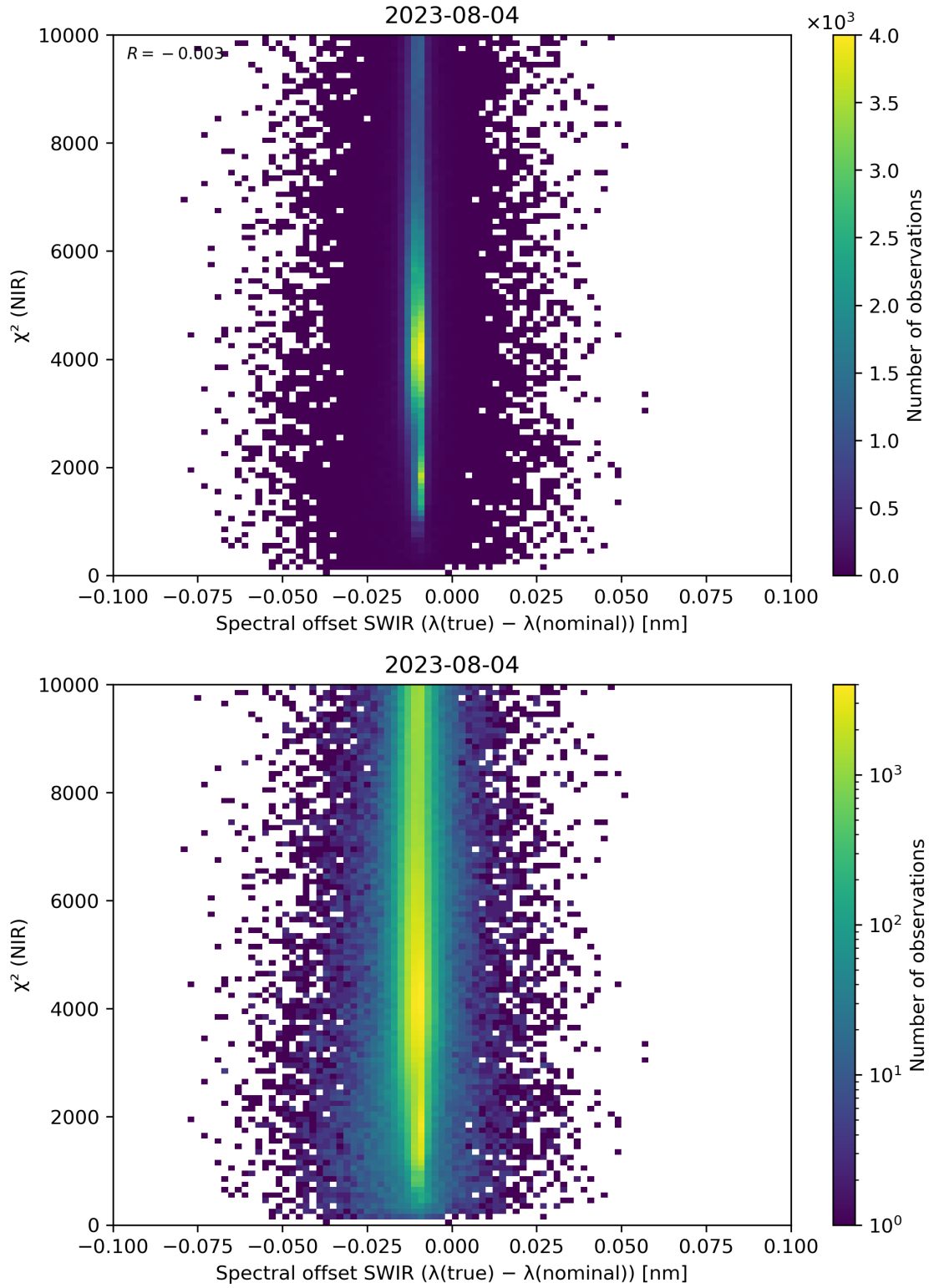
Figure 117: Scatter density plot of “Spectral offset SWIR ( \lambda(\text{true}) - \lambda(\text{nominal}) )” against “ \chi^2 (NIR)” for 2023-08-04 to 2023-08-05.
