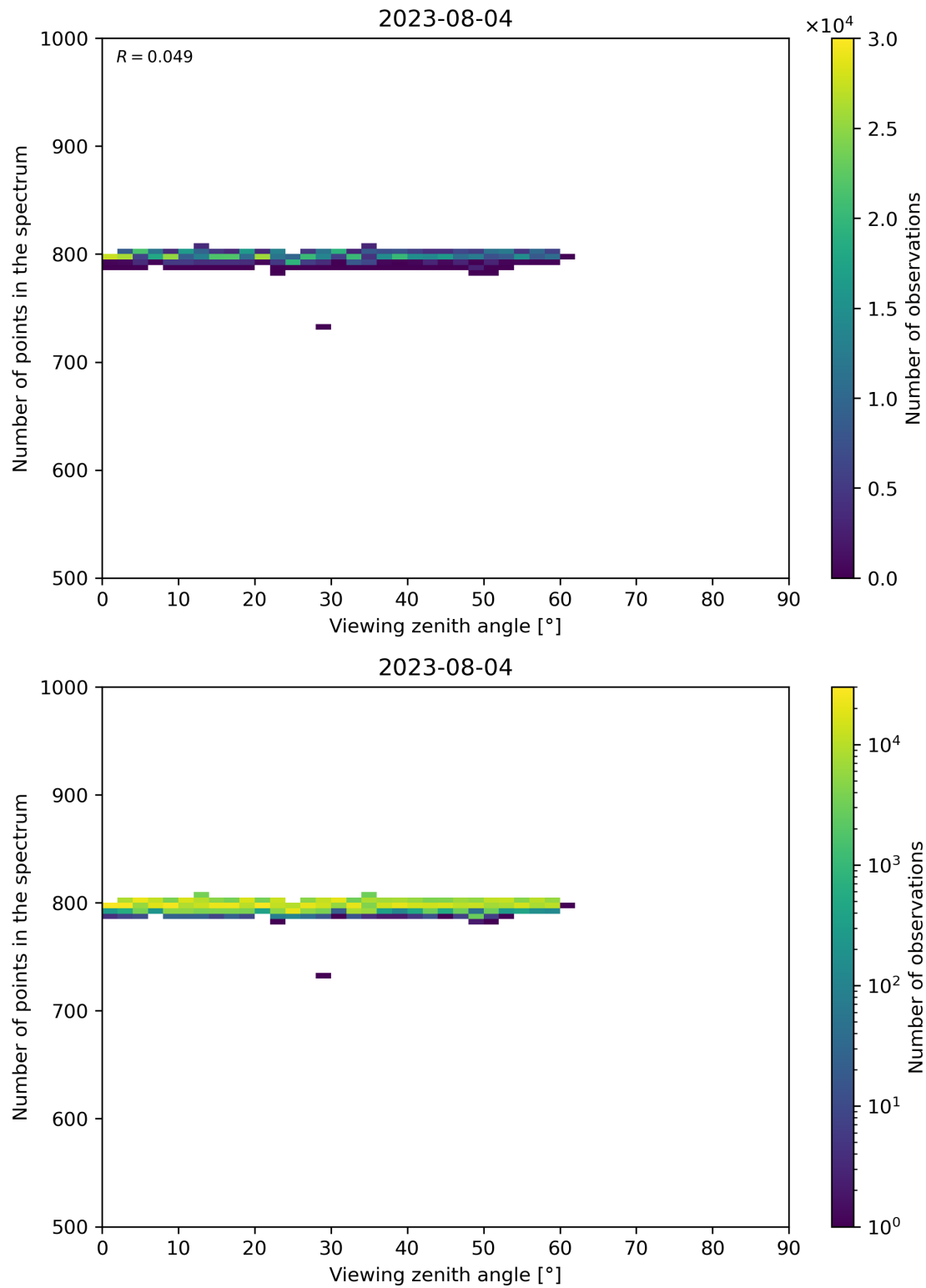
Figure 114: Scatter density plot of “Viewing zenith angle” against “Number of points in the spectrum” for 2023-08-04 to 2023-08-05.
