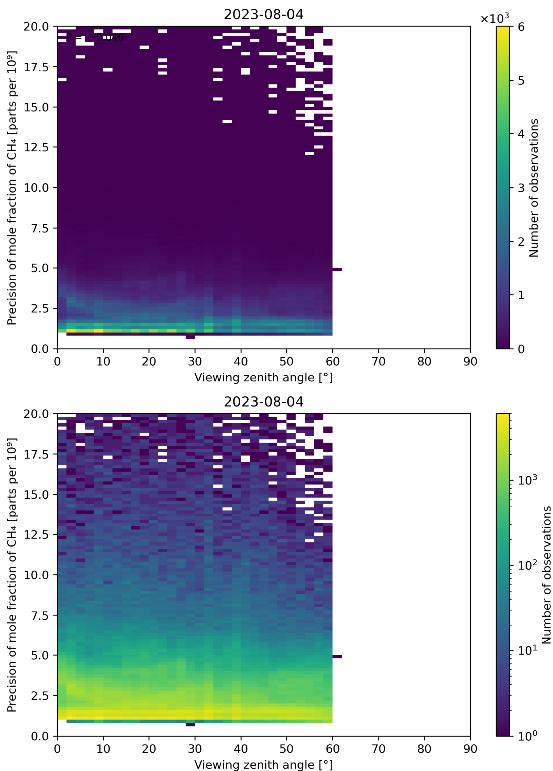
Figure 112: Scatter density plot of “Viewing zenith angle” against “Precision of mole fraction of CH 4 ” for 2023-08-04 to 2023-08-05.
