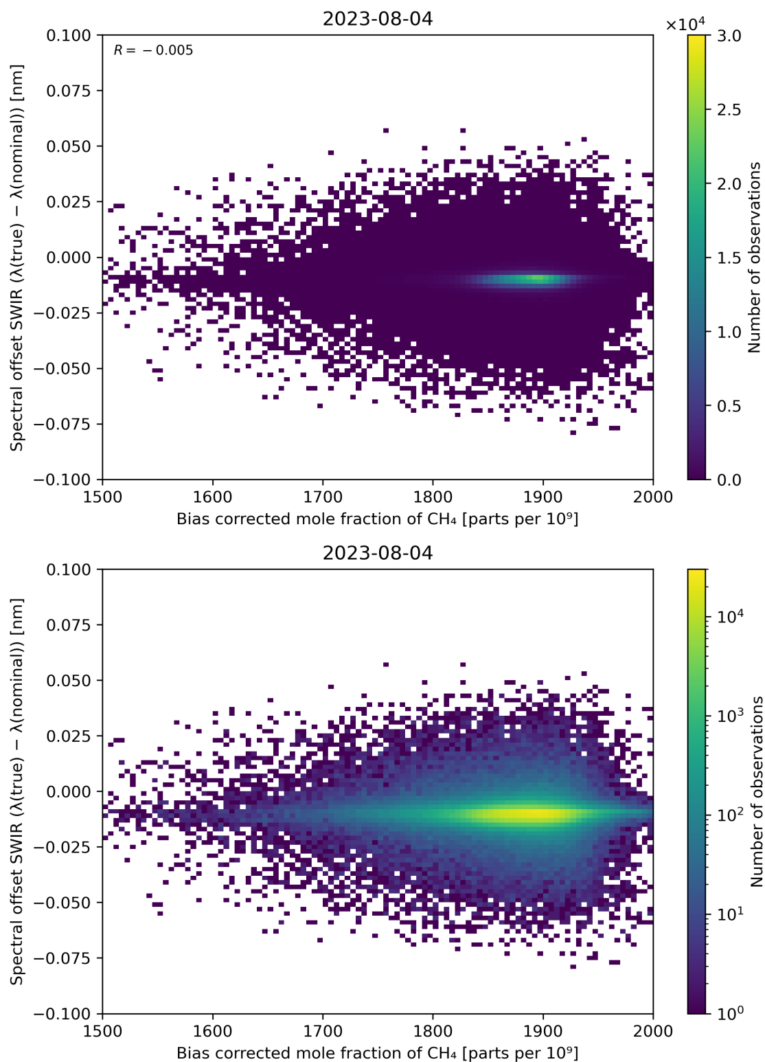
Figure 69: Scatter density plot of “Bias corrected mole fraction of \text{CH}_4 ” against “Spectral offset SWIR ( \lambda(\text{true}) - \lambda(\text{nominal}) )” for 2023-08-04 to 2023-08-05.
