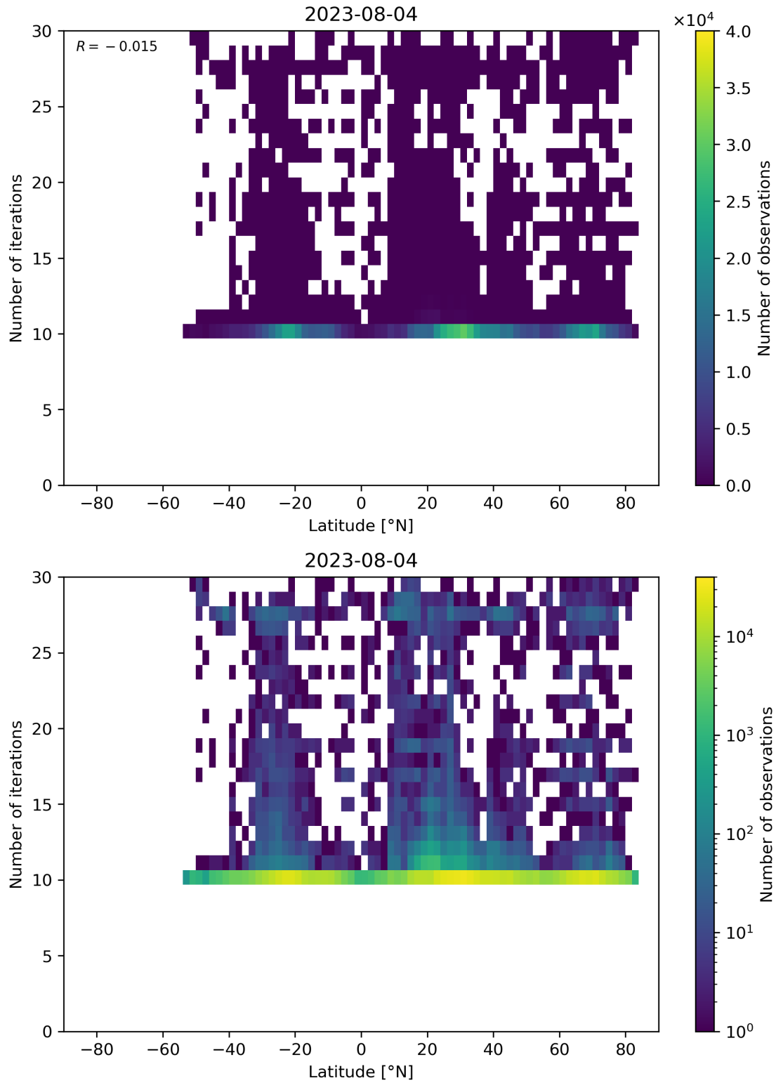
Figure 60: Scatter density plot of “Latitude” against “Number of iterations” for 2023-08-04 to 2023-08-05.
