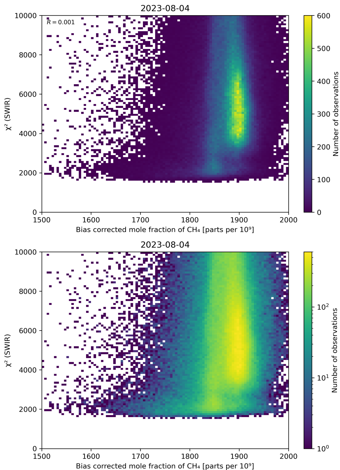
Figure 64: Scatter density plot of “Bias corrected mole fraction of CH 4 ” against “ \chi^2 (SWIR)” for 2023-08-04 to 2023-08-05.
