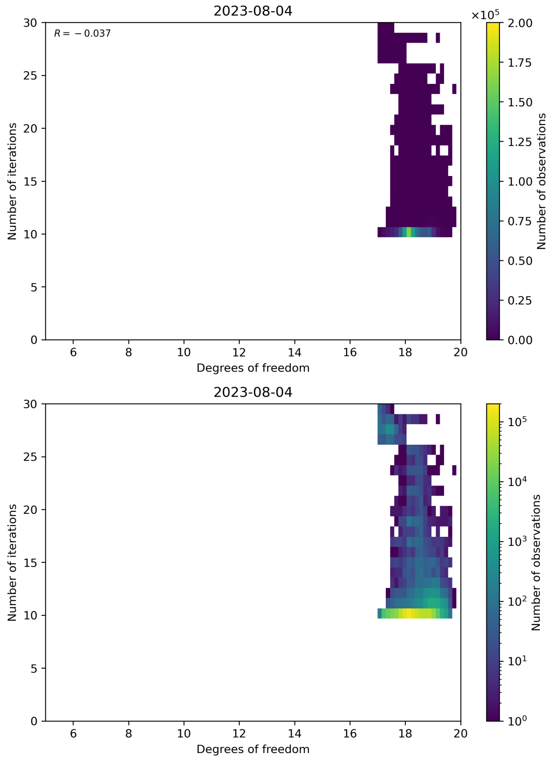
Figure 52: Scatter density plot of “Degrees of freedom” against “Number of iterations” for 2023-08-04 to 2023-08-05.
