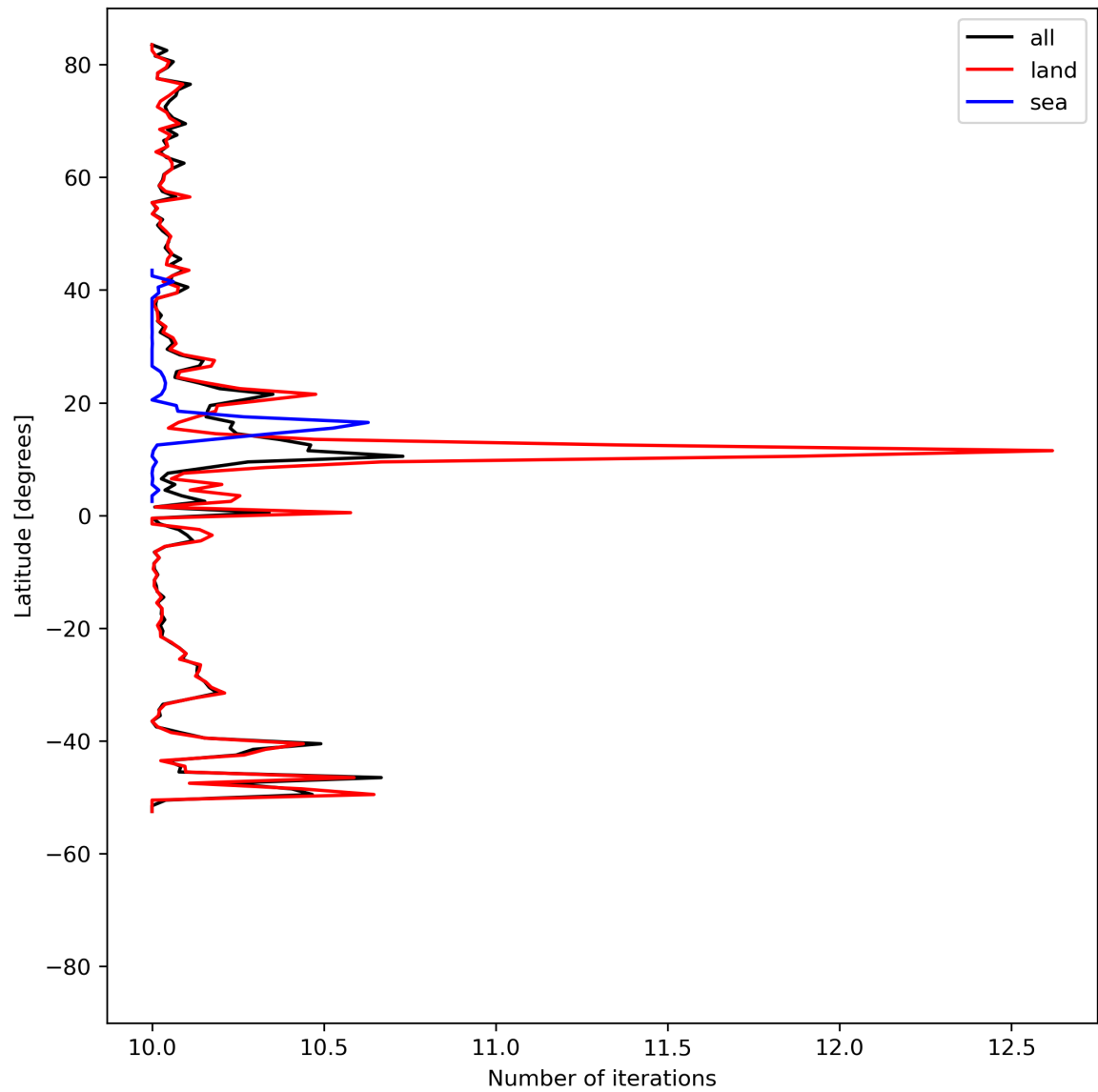
Figure 20: Zonal average of “Number of iterations” for 2023-08-04 to 2023-08-05.
