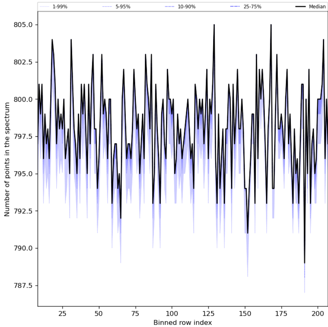
Figure 37: Along track statistics of “Number of points in the spectrum” for 2023-08-04 to 2023-08-05
