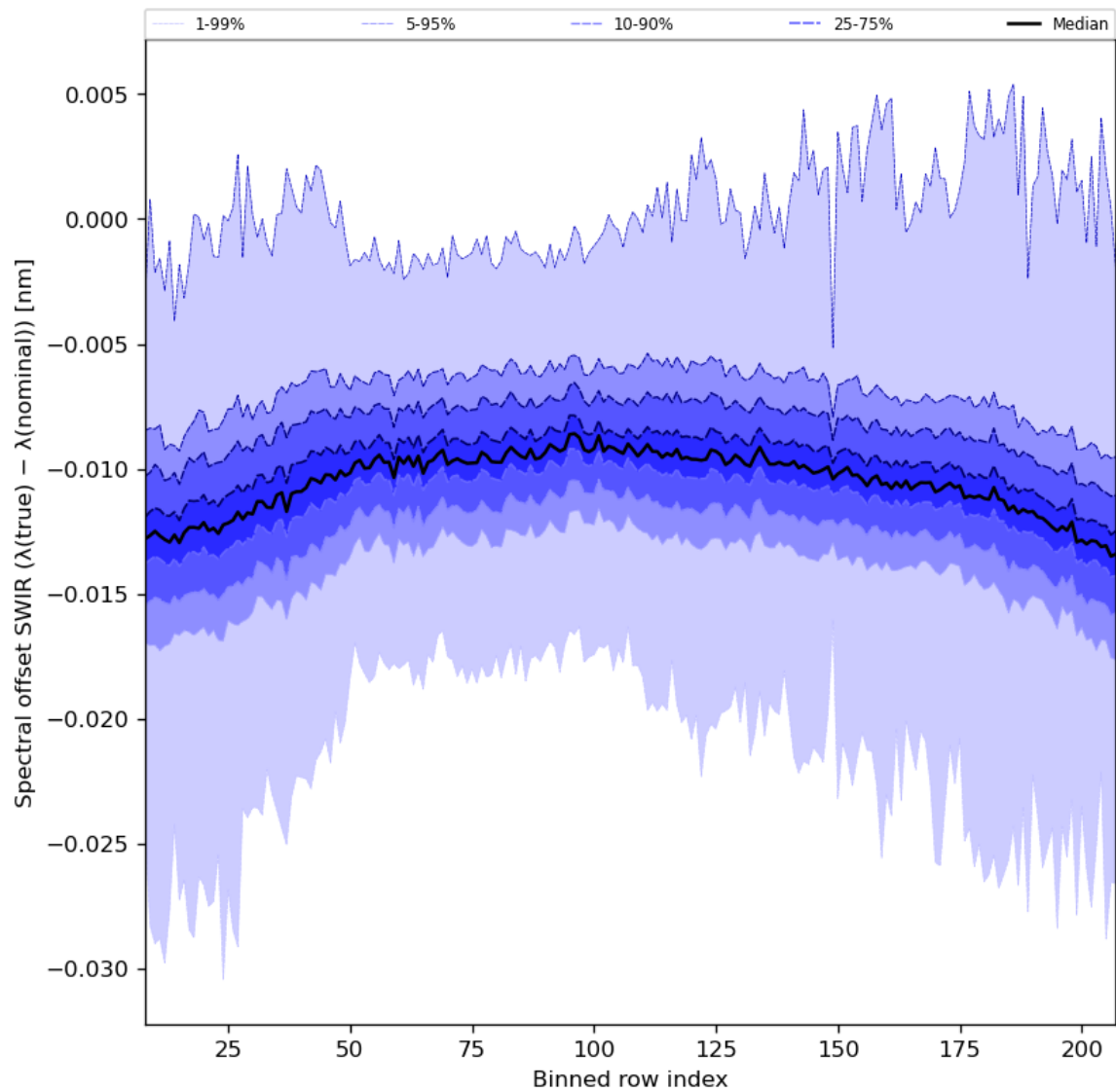
Figure 38: Along track statistics of “Spectral offset SWIR ( \lambda(\text{true}) - \lambda(\text{nominal}) )” for 2023-08-04 to 2023-08-05
