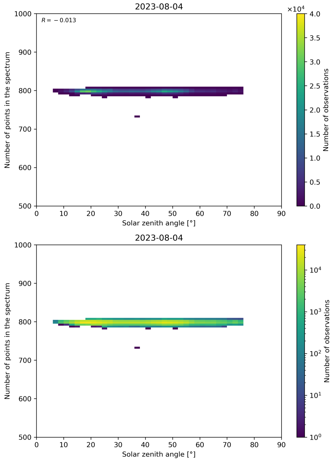
Figure 103: Scatter density plot of “Solar zenith angle” against “Number of points in the spectrum” for 2023-08-04 to 2023-08-05.
