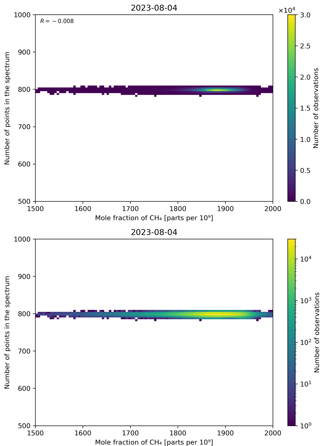
Figure 77: Scatter density plot of “Mole fraction of CH 4 ” against “Number of points in the spectrum” for 2023-08-04 to 2023-08-05.
