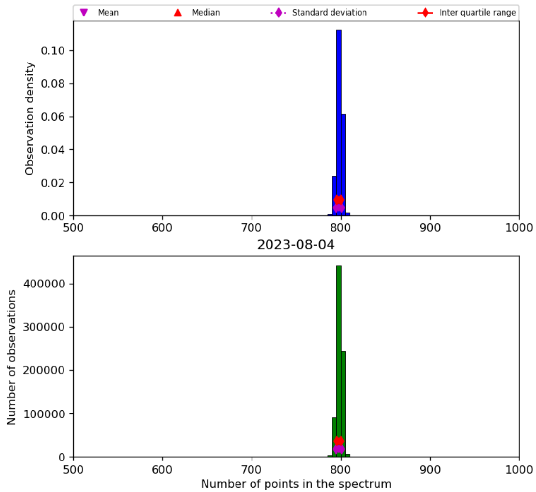
Figure 26: Histogram of “Number of points in the spectrum” for 2023-08-04 to 2023-08-05
