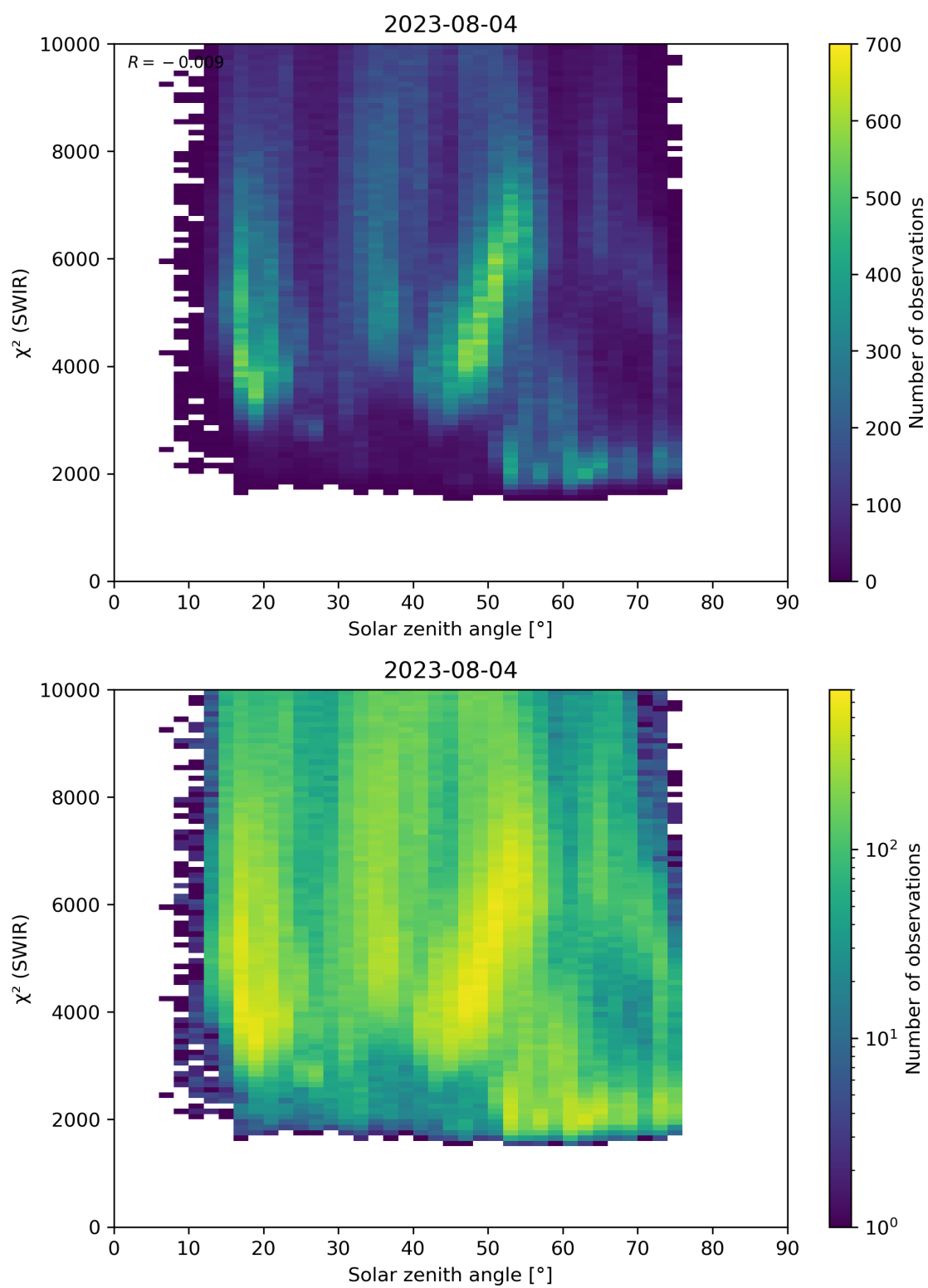
Figure 95: Scatter density plot of “Solar zenith angle” against “ \chi^2 (SWIR)” for 2023-08-04 to 2023-08-05.
