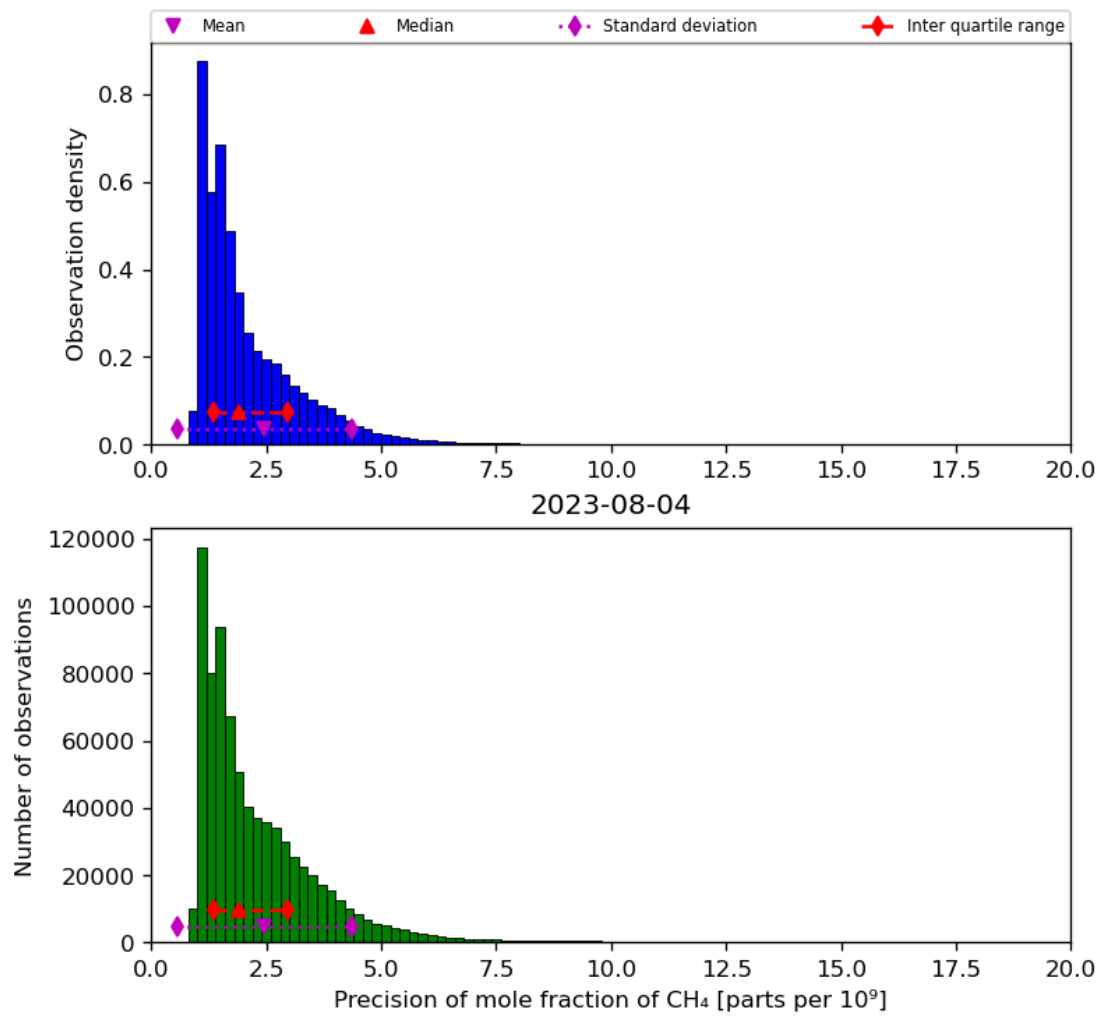
Figure 24: Histogram of “Precision of mole fraction of CH 4 ” for 2023-08-04 to 2023-08-05
