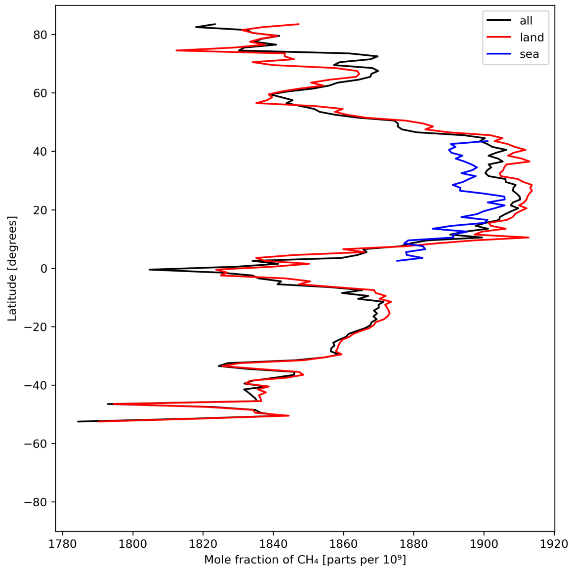
Figure 12: Zonal average of “Mole fraction of \text{CH}_4 ” for 2023-08-04 to 2023-08-05.
