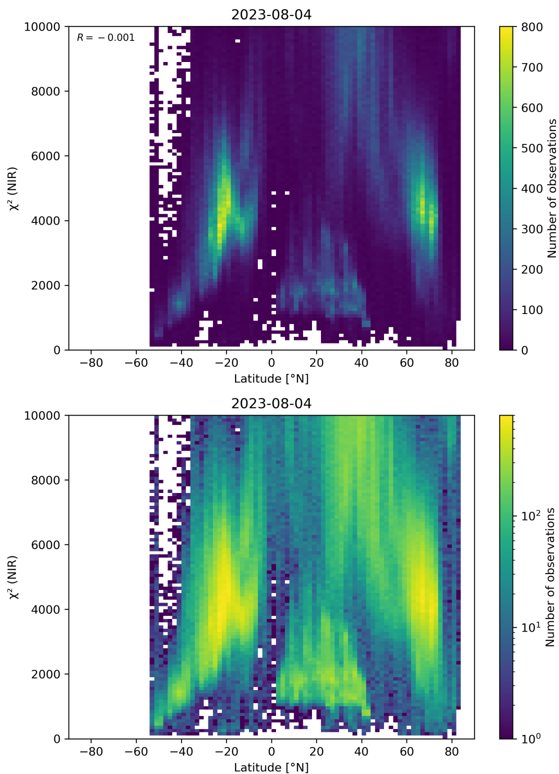
Figure 53: Scatter density plot of “Latitude” against “ \chi^2 (NIR)” for 2023-08-04 to 2023-08-05.
