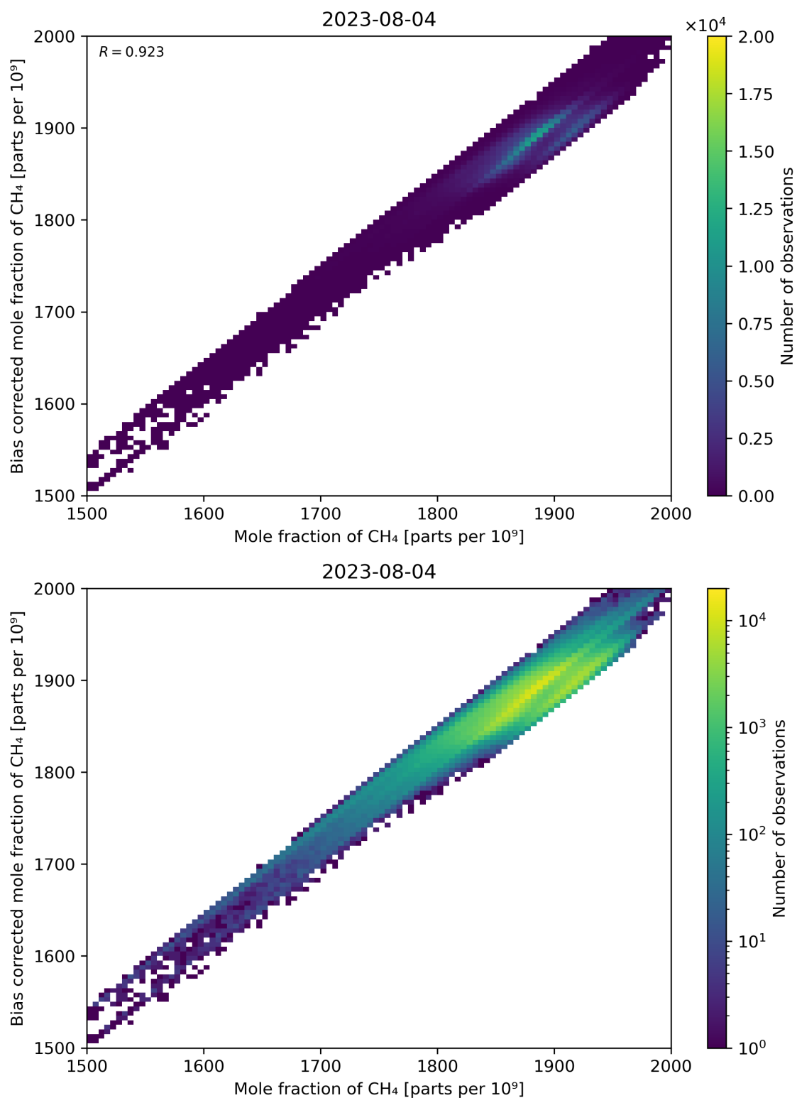
Figure 74: Scatter density plot of “Mole fraction of CH 4 ” against “Bias corrected mole fraction of CH 4 ” for 2023-08-04 to 2023-08-05.
