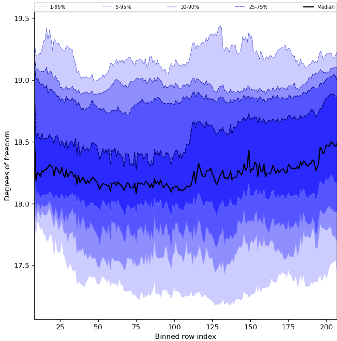
Figure 41: Along track statistics of “Degrees of freedom” for 2023-08-04 to 2023-08-05
