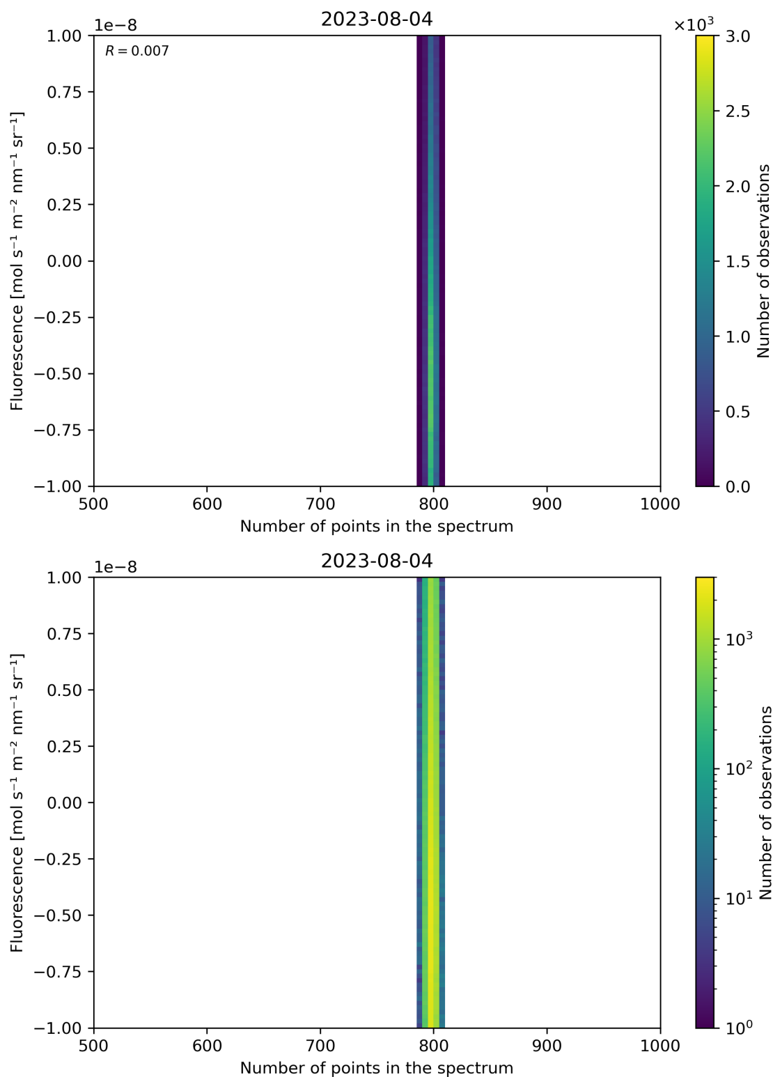
Figure 91: Scatter density plot of “Number of points in the spectrum” against “Fluorescence” for 2023-08-04 to 2023-08-05.
