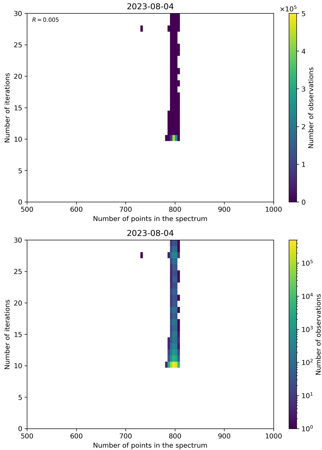
Figure 92: Scatter density plot of “Number of points in the spectrum” against “Number of iterations” for 2023-08-04 to 2023-08-05.
