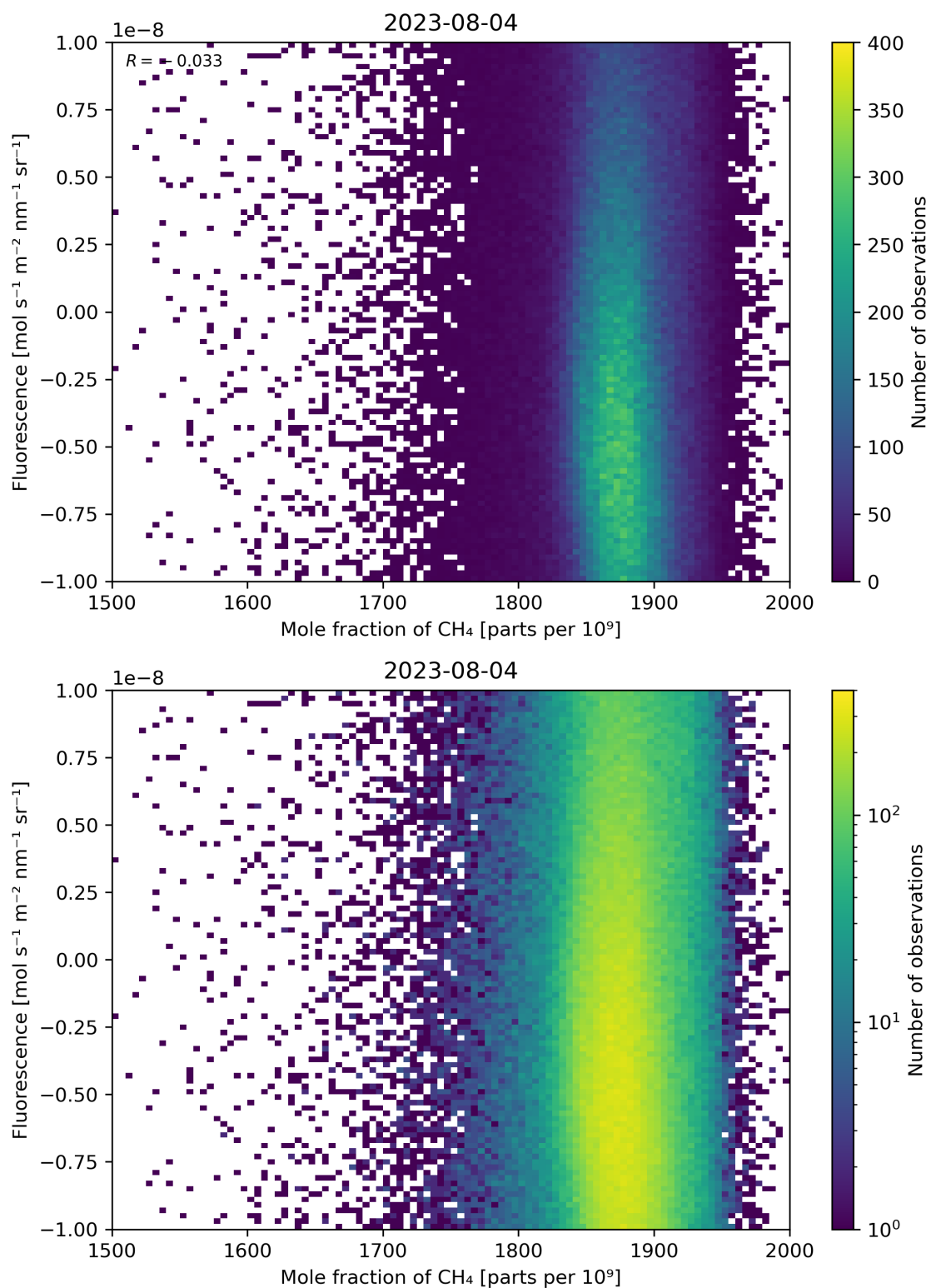
Figure 73: Scatter density plot of “Mole fraction of \text{CH}_4 ” against “Fluorescence” for 2023-08-04 to 2023-08-05.
