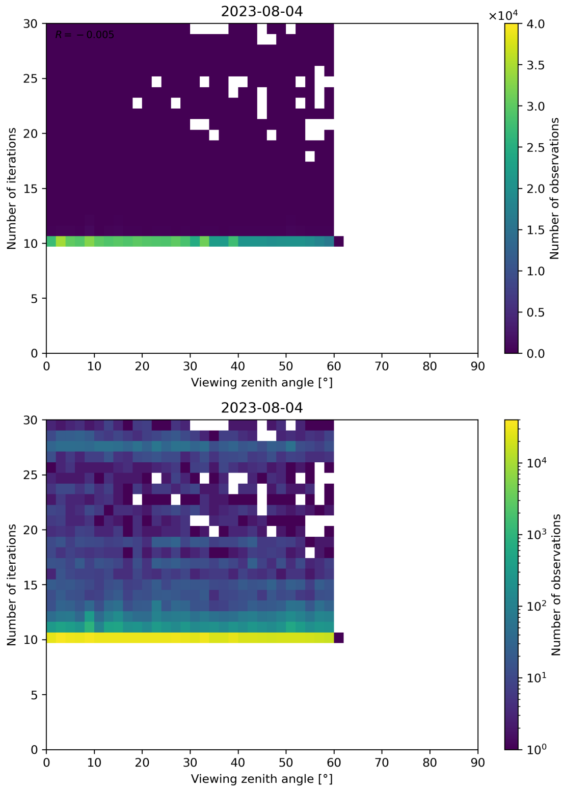
Figure 113: Scatter density plot of “Viewing zenith angle” against “Number of iterations” for 2023-08-04 to 2023-08-05.
