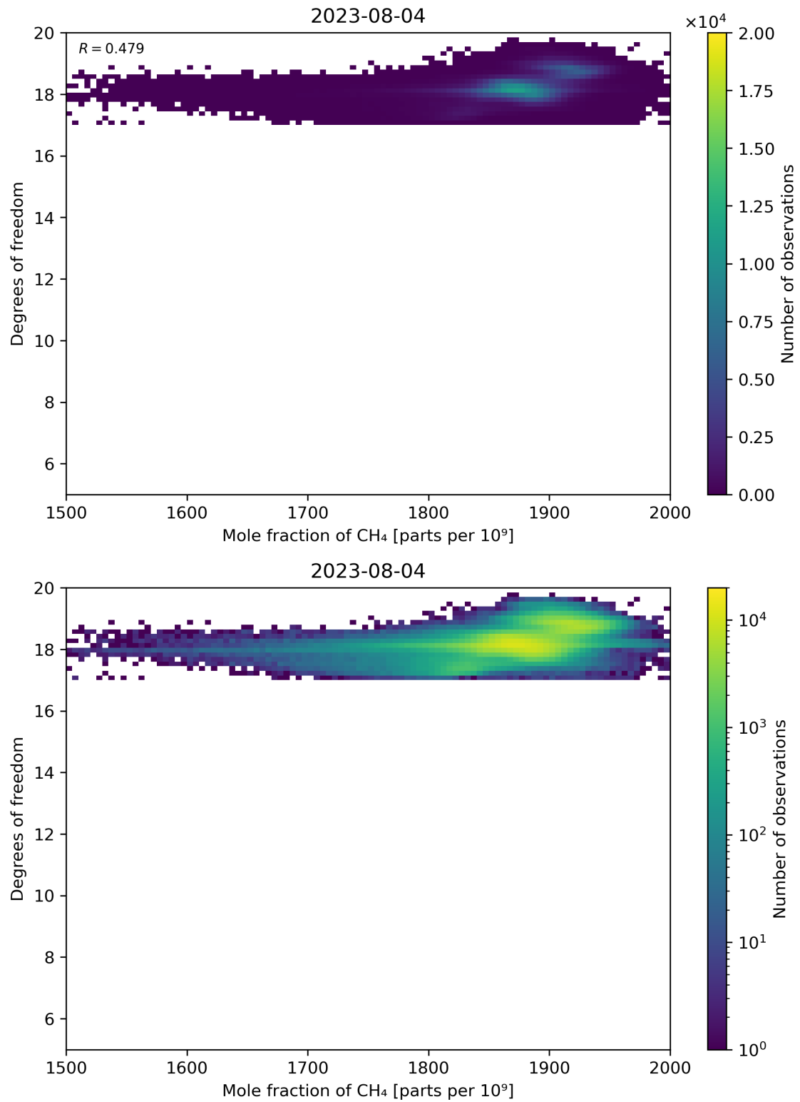
Figure 72: Scatter density plot of “Mole fraction of CH 4 ” against “Degrees of freedom” for 2023-08-04 to 2023-08-05.
