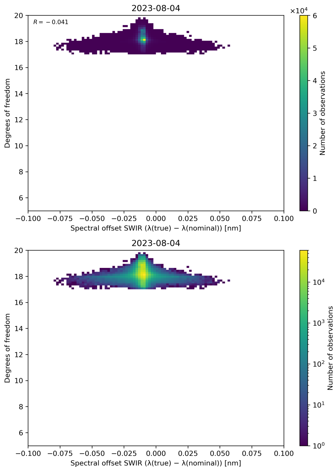
Figure 119: Scatter density plot of “Spectral offset SWIR ( \lambda(\text{true}) - \lambda(\text{nominal}) )” against “Degrees of freedom” for 2023-08-04 to 2023-08-05.
