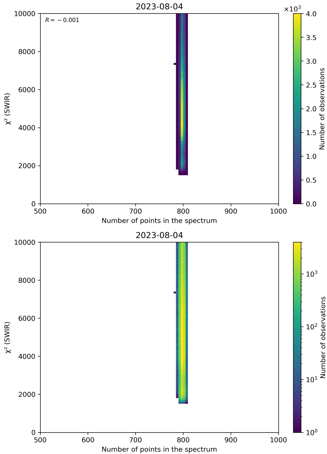
Figure 89: Scatter density plot of “Number of points in the spectrum” against “ \chi^2 (SWIR)” for 2023-08-04 to 2023-08-05.
