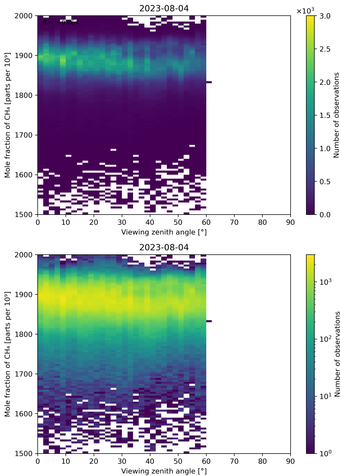
Figure 110: Scatter density plot of “Viewing zenith angle” against “Mole fraction of CH 4 ” for 2023-08-04 to 2023-08-05.
