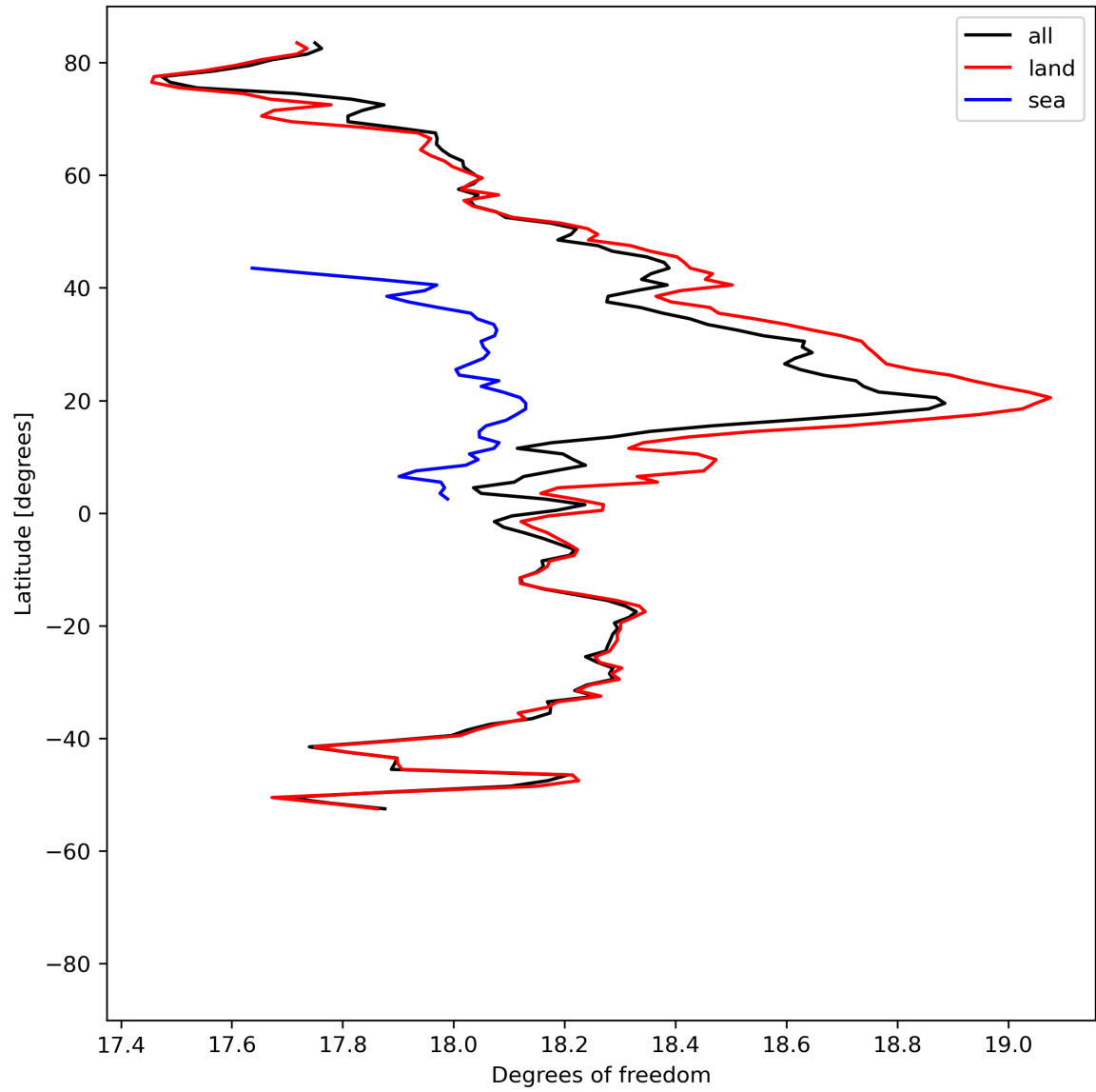
Figure 19: Zonal average of “Degrees of freedom” for 2023-08-04 to 2023-08-05.
