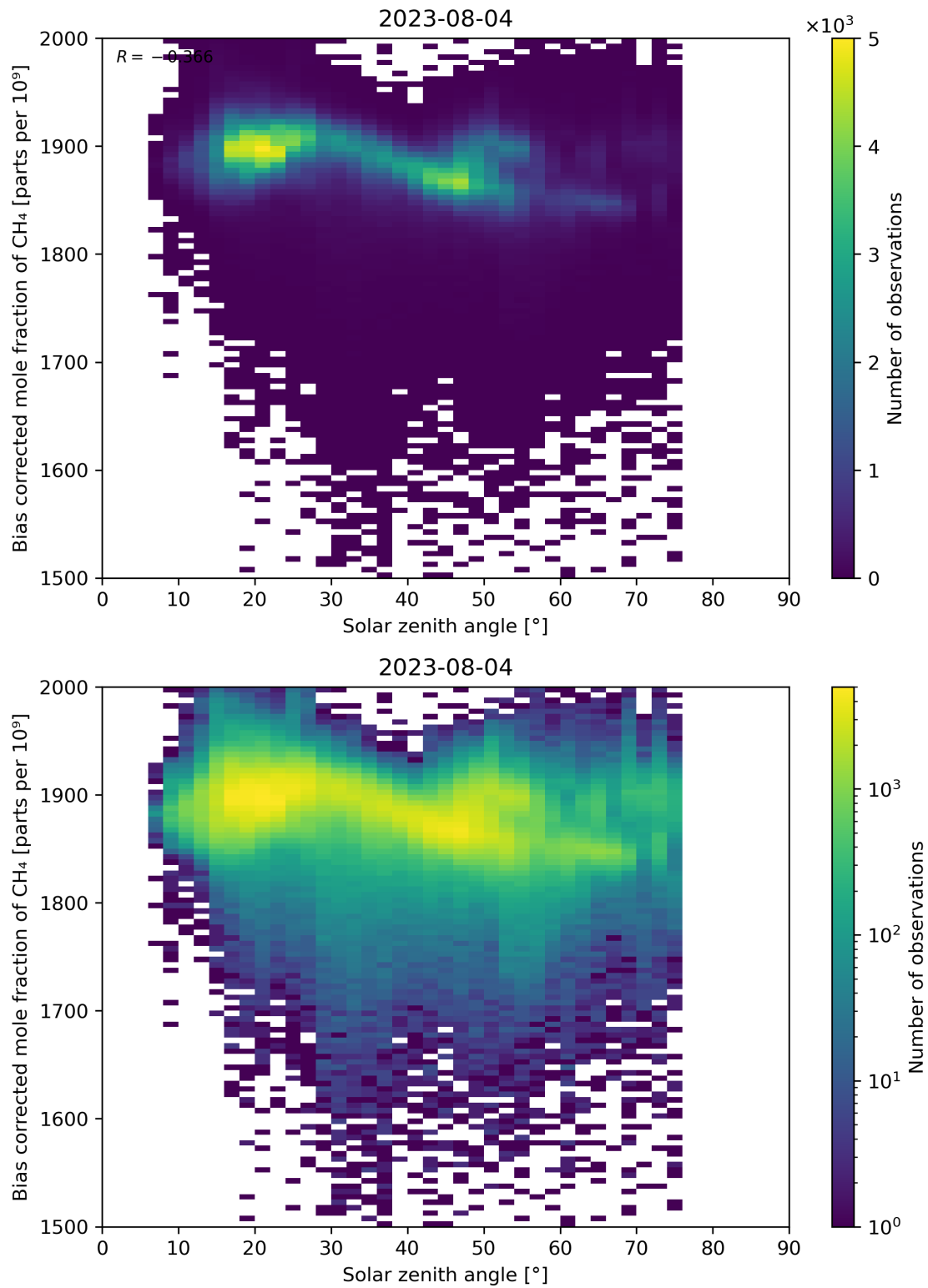
Figure 100: Scatter density plot of “Solar zenith angle” against “Bias corrected mole fraction of CH 4 ” for 2023-08-04 to 2023-08-05.
