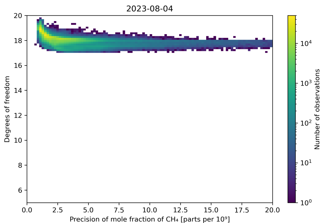
Figure 80: Scatter density plot of “Precision of mole fraction of CH 4 ” against “Degrees of freedom” for 2023-08-04 to 2023-08-05.
