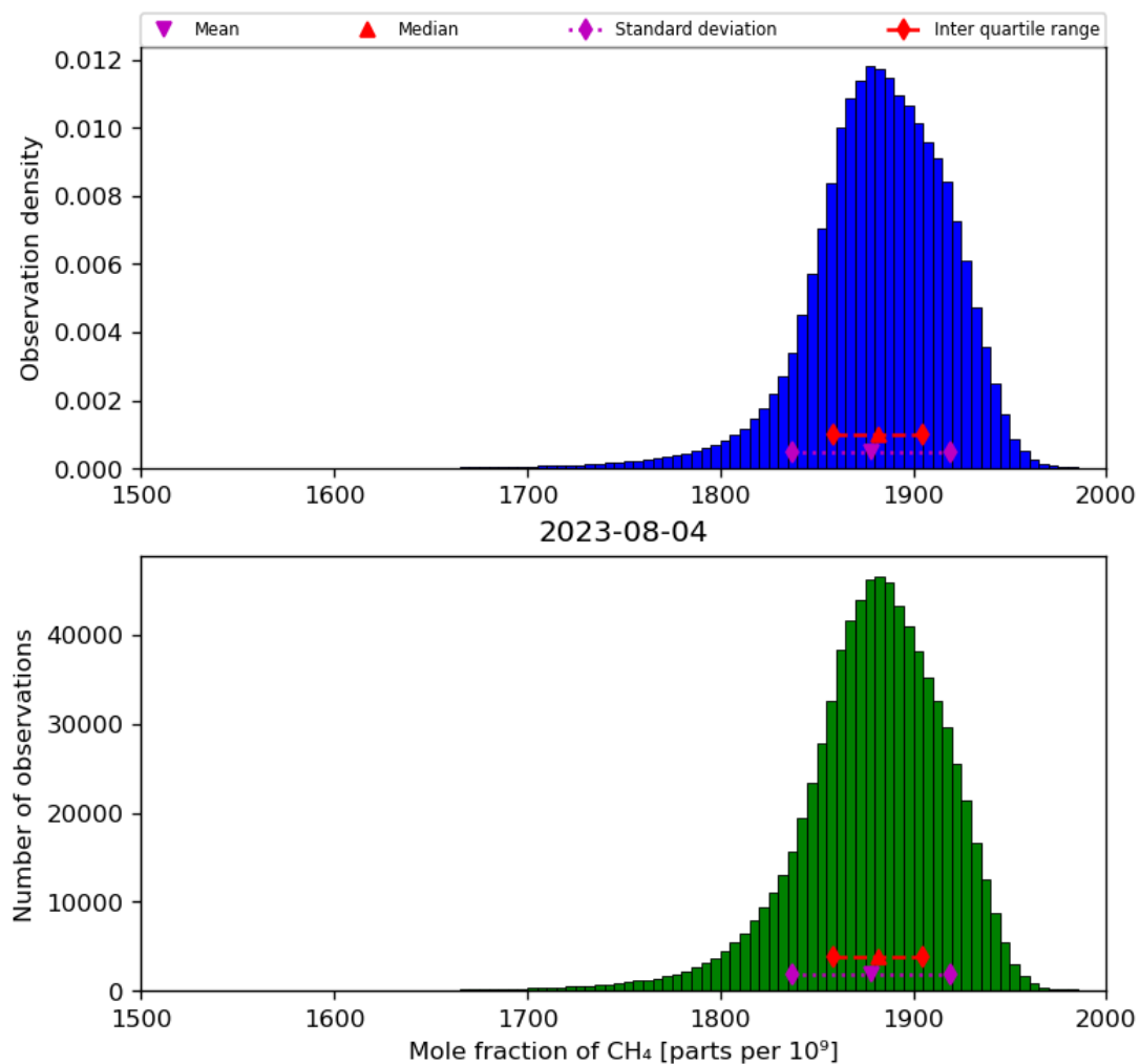
Figure 23: Histogram of “Mole fraction of CH 4 ” for 2023-08-04 to 2023-08-05
