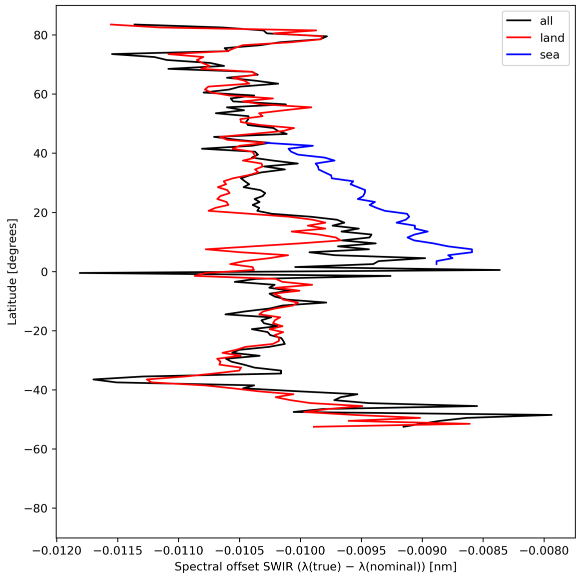
Figure 16: Zonal average of “Spectral offset SWIR ( \lambda(\text{true}) - \lambda(\text{nominal}) )” for 2023-08-04 to 2023-08-05.
