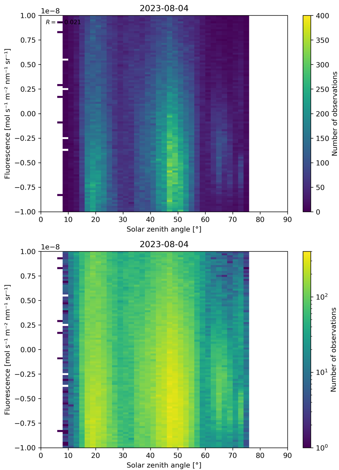
Figure 97: Scatter density plot of “Solar zenith angle” against “Fluorescence” for 2023-08-04 to 2023-08-05.
