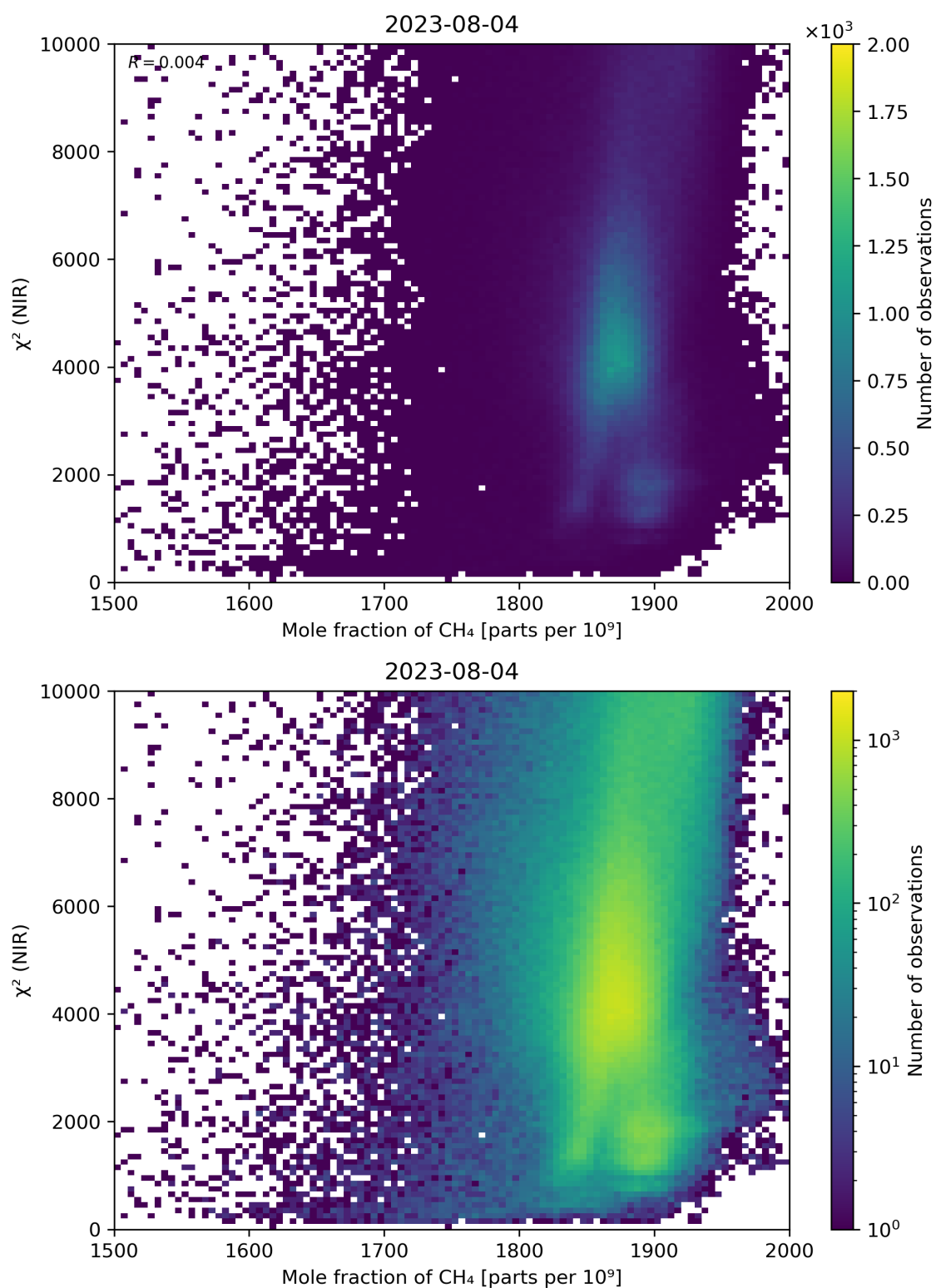
Figure 70: Scatter density plot of “Mole fraction of \text{CH}_4 ” against “ \chi^2 (NIR)” for 2023-08-04 to 2023-08-05.
