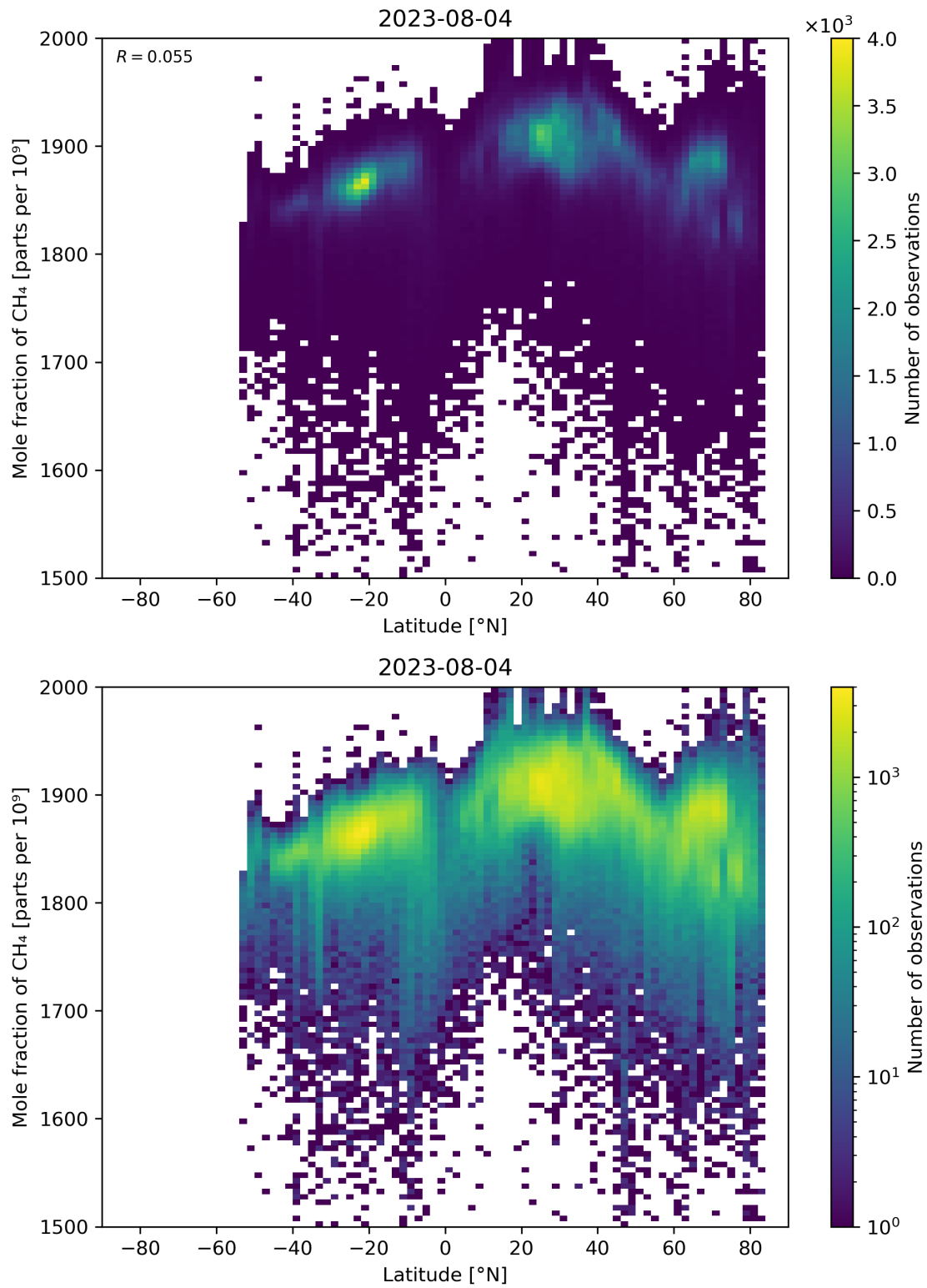
Figure 57: Scatter density plot of “Latitude” against “Mole fraction of CH 4 ” for 2023-08-04 to 2023-08-05.
