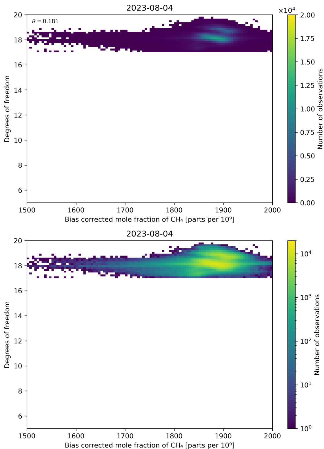
Figure 65: Scatter density plot of “Bias corrected mole fraction of \text{CH}_4 ” against “Degrees of freedom” for 2023-08-04 to 2023-08-05.
