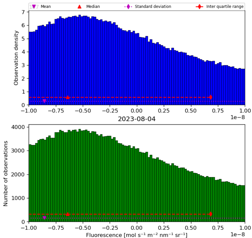
Figure 32: Histogram of “Fluorescence” for 2023-08-04 to 2023-08-05
