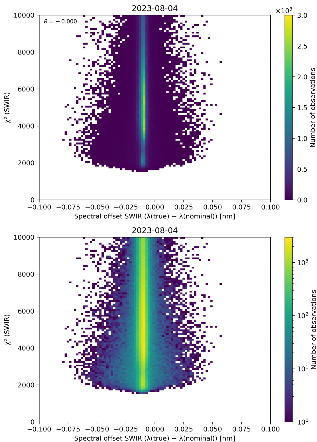
Figure 118: Scatter density plot of “Spectral offset SWIR ( \lambda(\text{true}) - \lambda(\text{nominal}) )” against “ \chi^2 (SWIR)” for 2023-08-04 to 2023-08-05.
