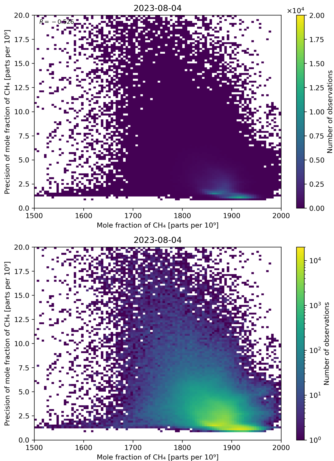
Figure 75: Scatter density plot of “Mole fraction of CH 4 ” against “Precision of mole fraction of CH 4 ” for 2023-08-04 to 2023-08-05.
