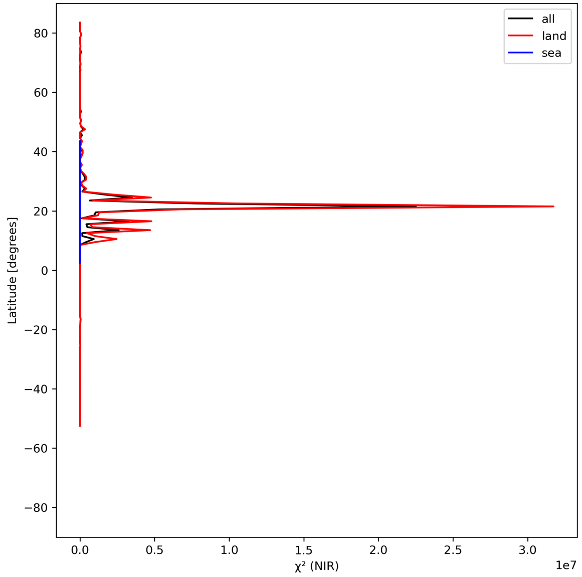
Figure 18: Zonal average of “ \chi^2 (NIR)” for 2023-08-04 to 2023-08-05.
