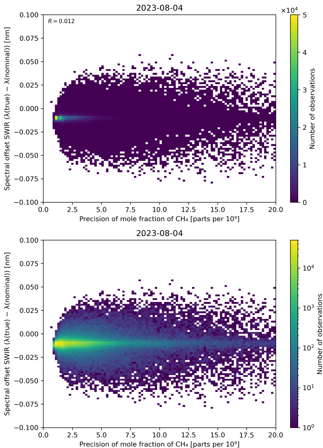
Figure 85: Scatter density plot of “Precision of mole fraction of CH 4 ” against “Spectral offset SWIR ( \lambda(\text{true}) - \lambda(\text{nominal}) )” for 2023-08-04 to 2023-08-05.
