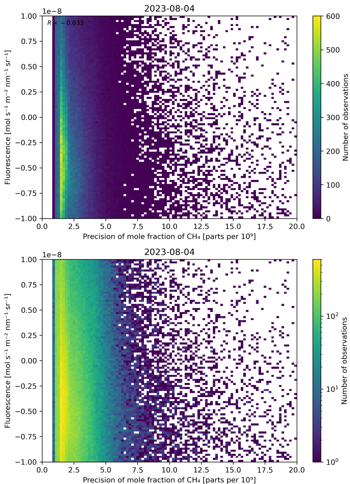
Figure 81: Scatter density plot of “Precision of mole fraction of \text{CH}_4 ” against “Fluorescence” for 2023-08-04 to 2023-08-05.
