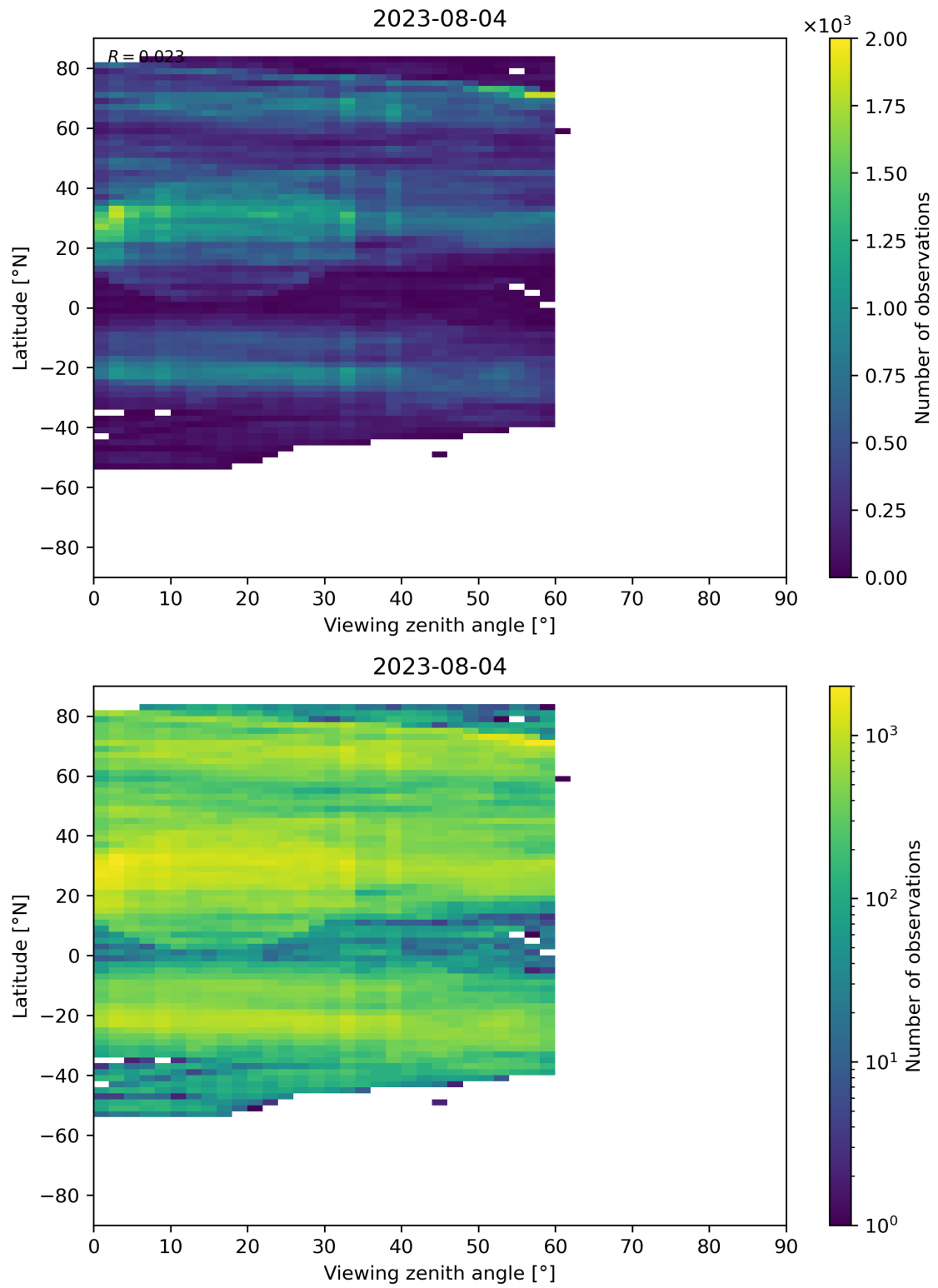
Figure 109: Scatter density plot of “Viewing zenith angle” against “Latitude” for 2023-08-04 to 2023-08-05.
