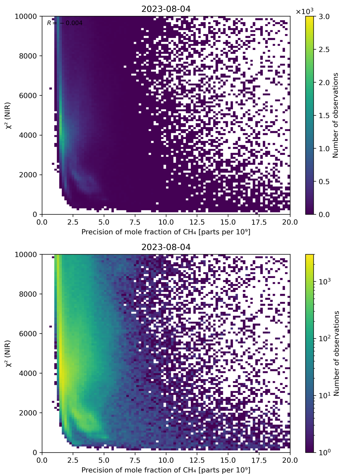
Figure 78: Scatter density plot of “Precision of mole fraction of \text{CH}_4 ” against “ \chi^2 (NIR)” for 2023-08-04 to 2023-08-05.
