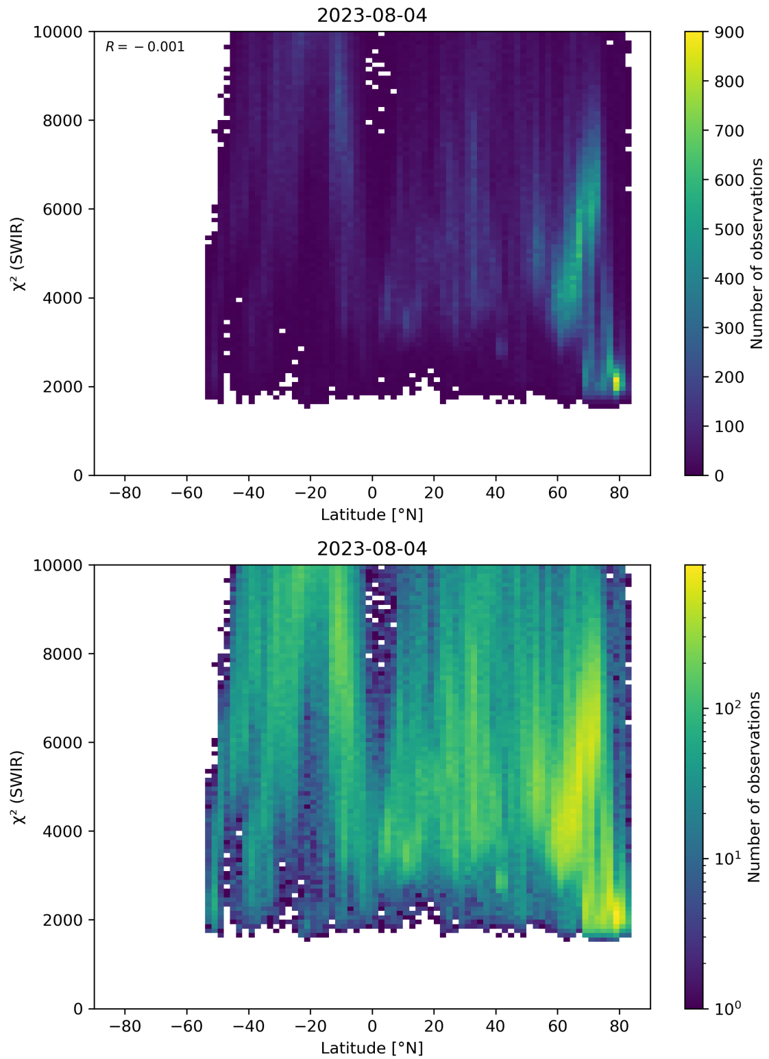
Figure 54: Scatter density plot of “Latitude” against “ \chi^2 (SWIR)” for 2023-08-04 to 2023-08-05.
