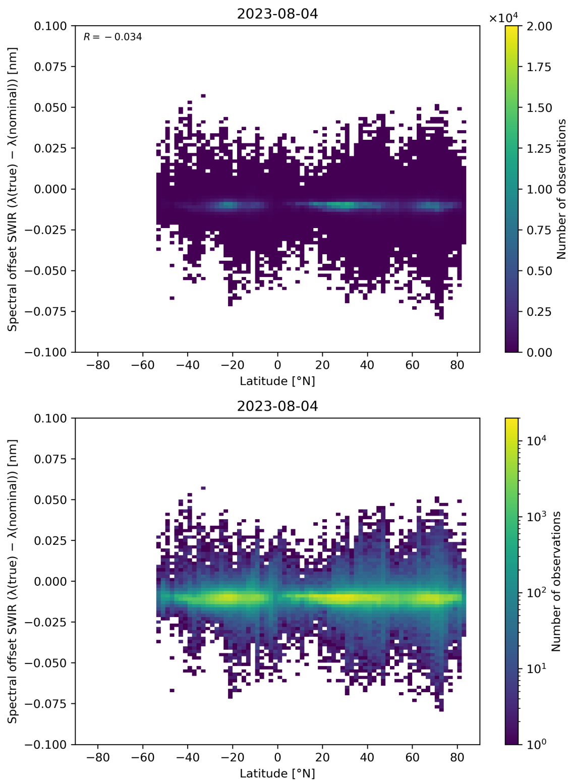
Figure 62: Scatter density plot of “Latitude” against “Spectral offset SWIR ( \lambda(\text{true}) - \lambda(\text{nominal}) )” for 2023-08-04 to 2023-08-05.
