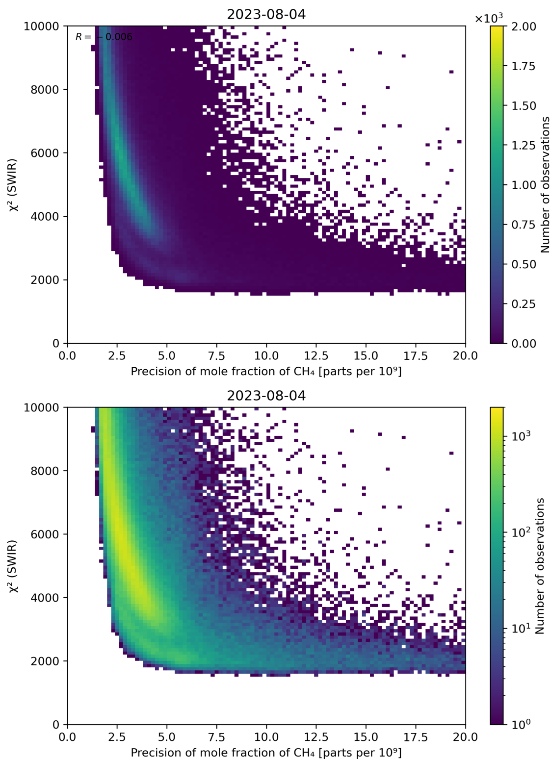
Figure 79: Scatter density plot of “Precision of mole fraction of \text{CH}_4 ” against “ \chi^2 (SWIR)” for 2023-08-04 to 2023-08-05.
