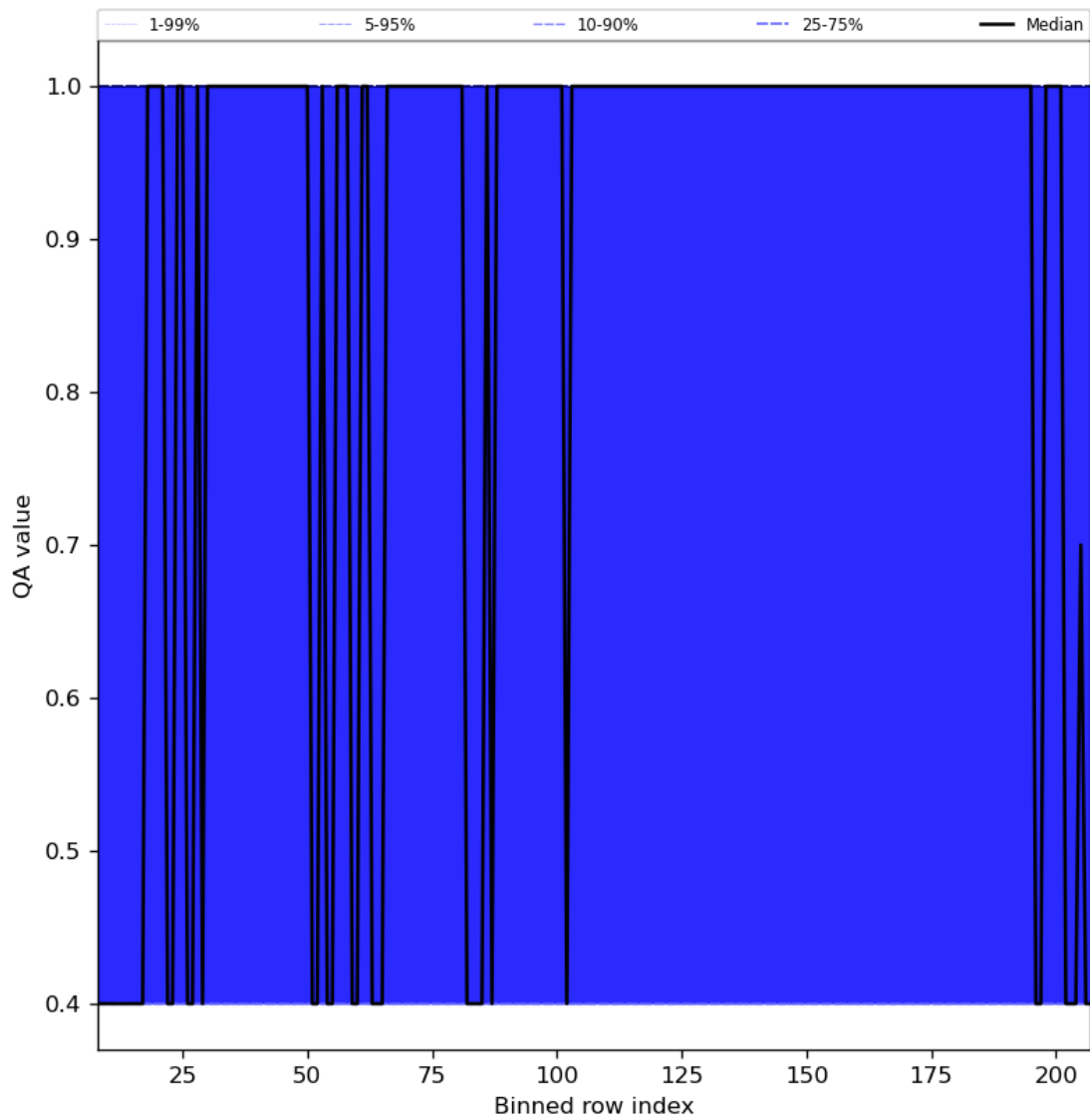
Figure 33: Along track statistics of “QA value” for 2023-08-04 to 2023-08-05
