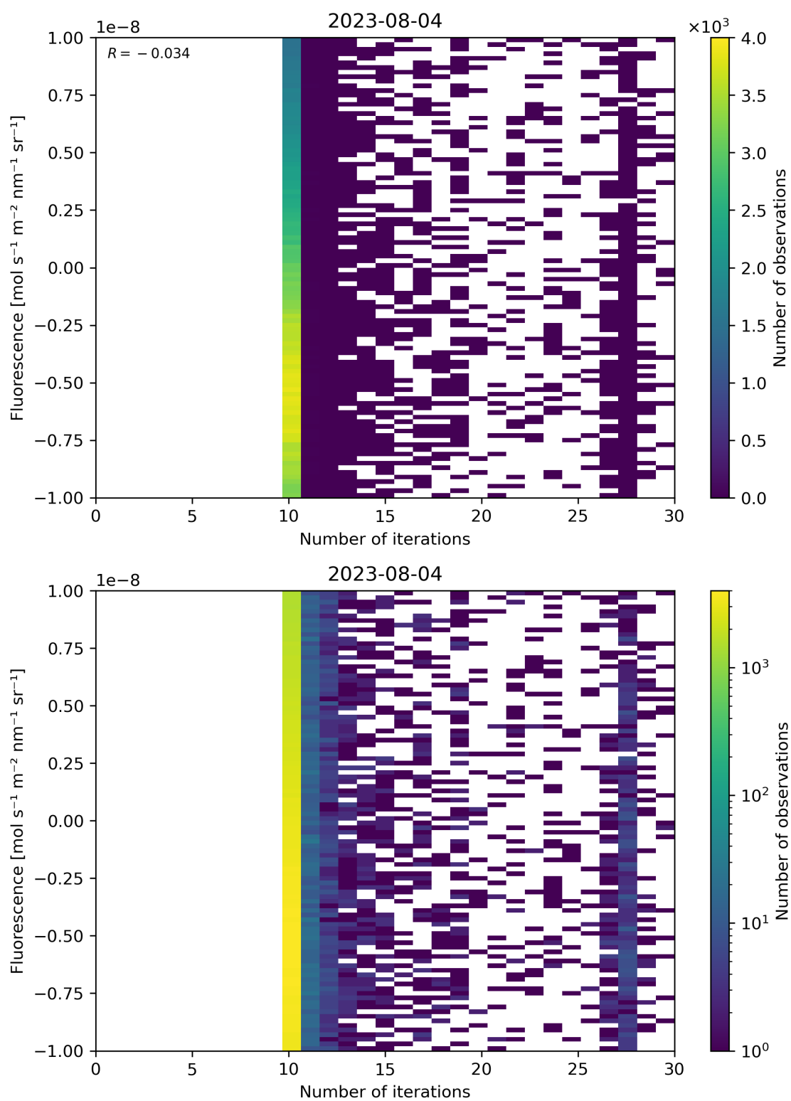
Figure 87: Scatter density plot of “Number of iterations” against “Fluorescence” for 2023-08-04 to 2023-08-05.
