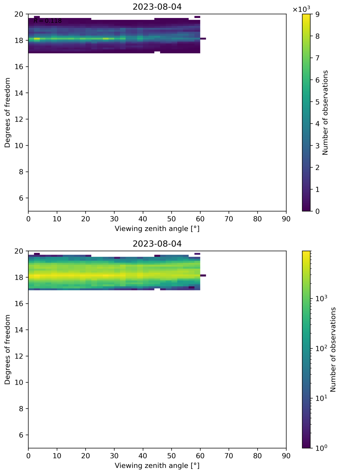
Figure 107: Scatter density plot of “Viewing zenith angle” against “Degrees of freedom” for 2023-08-04 to 2023-08-05.
