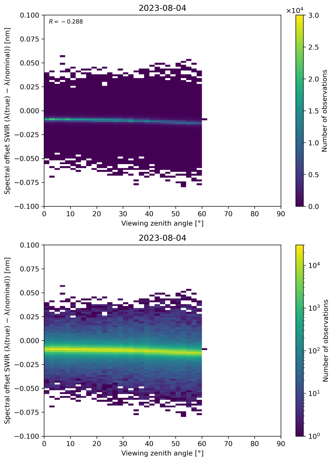
Figure 116: Scatter density plot of “Viewing zenith angle” against “Spectral offset SWIR ( \lambda(\text{true}) - \lambda(\text{nominal}) )” for 2023-08-04 to 2023-08-05.
