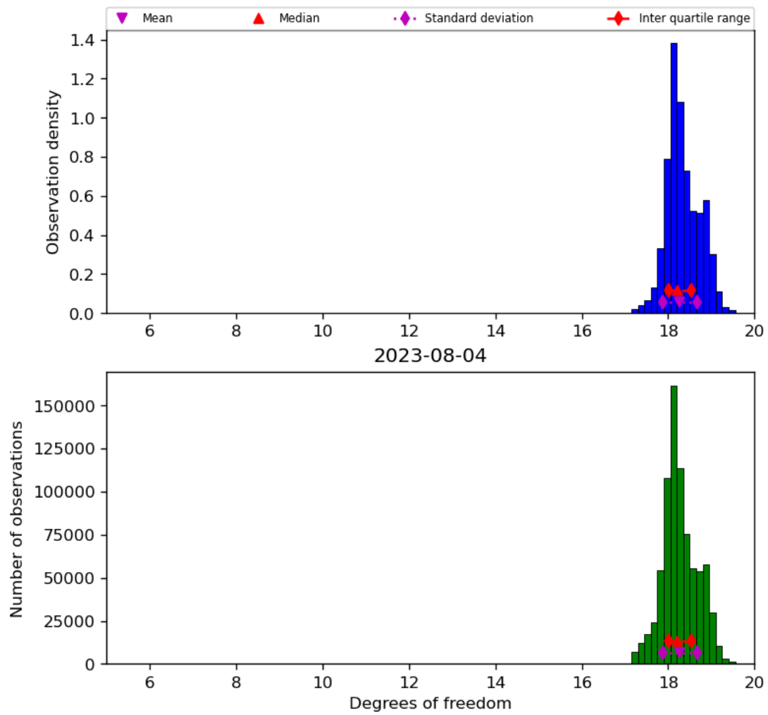
Figure 30: Histogram of “Degrees of freedom” for 2023-08-04 to 2023-08-05
