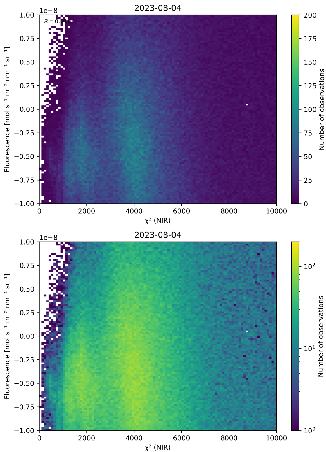
Figure 45: Scatter density plot of “ \chi^2 (NIR)” against “Fluorescence” for 2023-08-04 to 2023-08-05.
