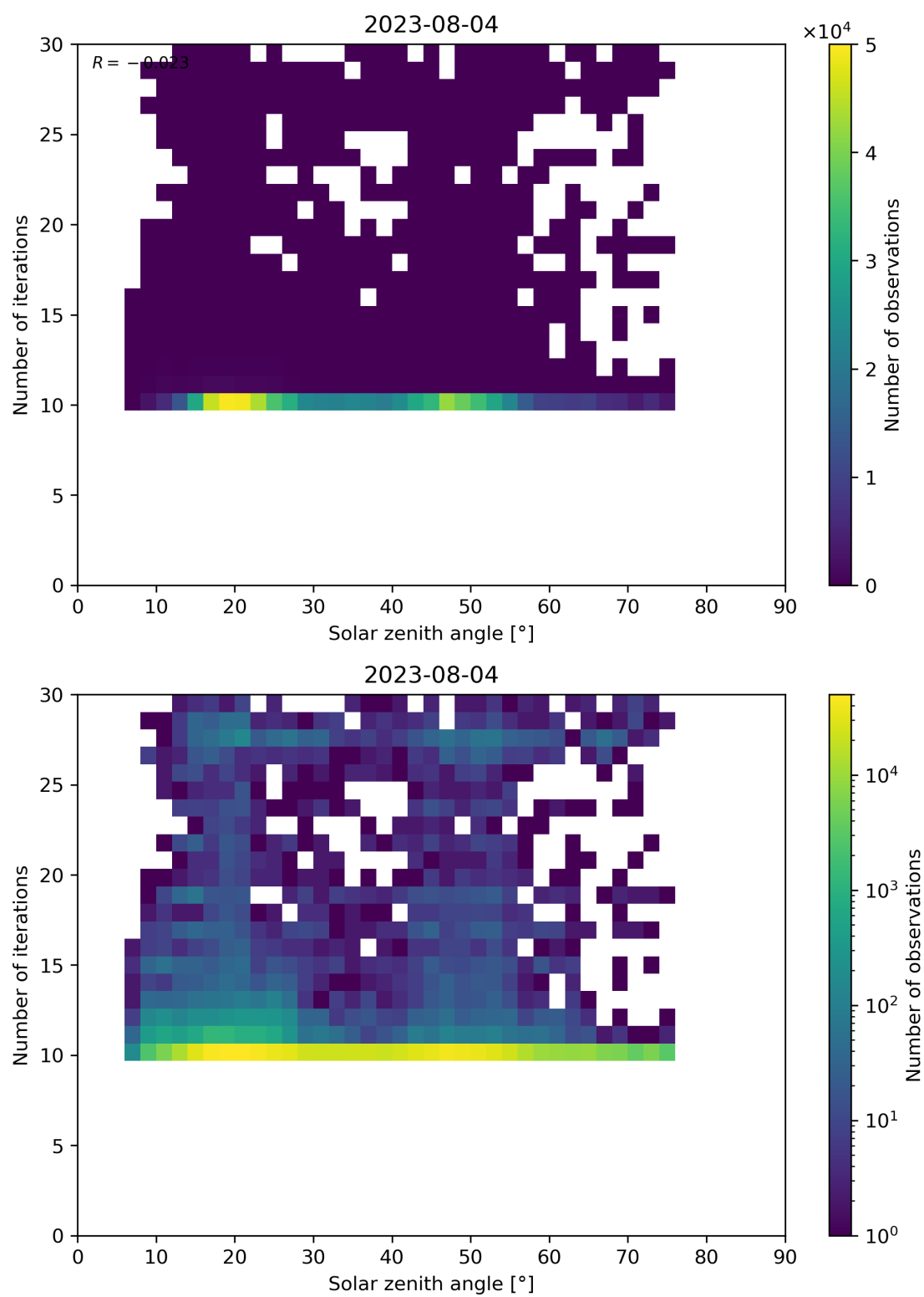
Figure 102: Scatter density plot of “Solar zenith angle” against “Number of iterations” for 2023-08-04 to 2023-08-05.
