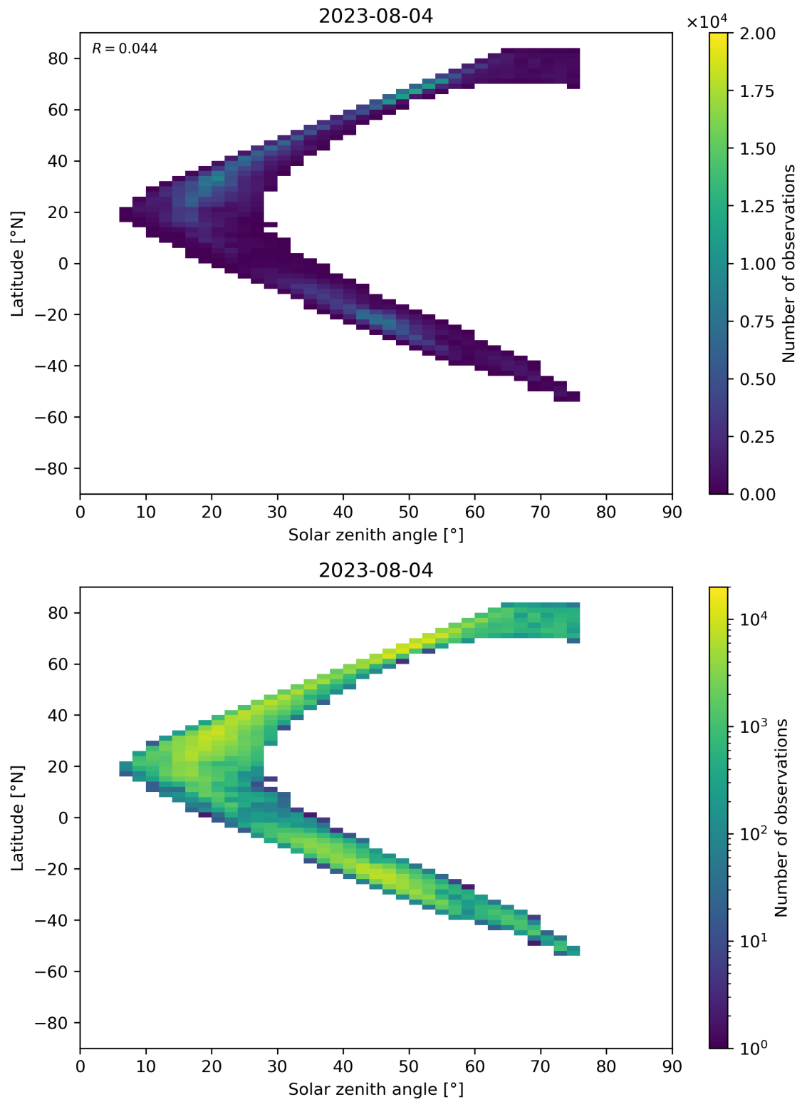
Figure 98: Scatter density plot of “Solar zenith angle” against “Latitude” for 2023-08-04 to 2023-08-05.
