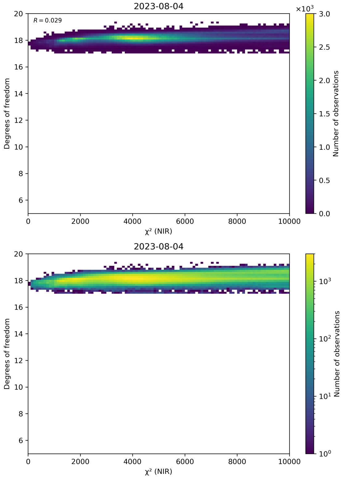
Figure 44: Scatter density plot of “ \chi^2 (NIR)” against “Degrees of freedom” for 2023-08-04 to 2023-08-05.
