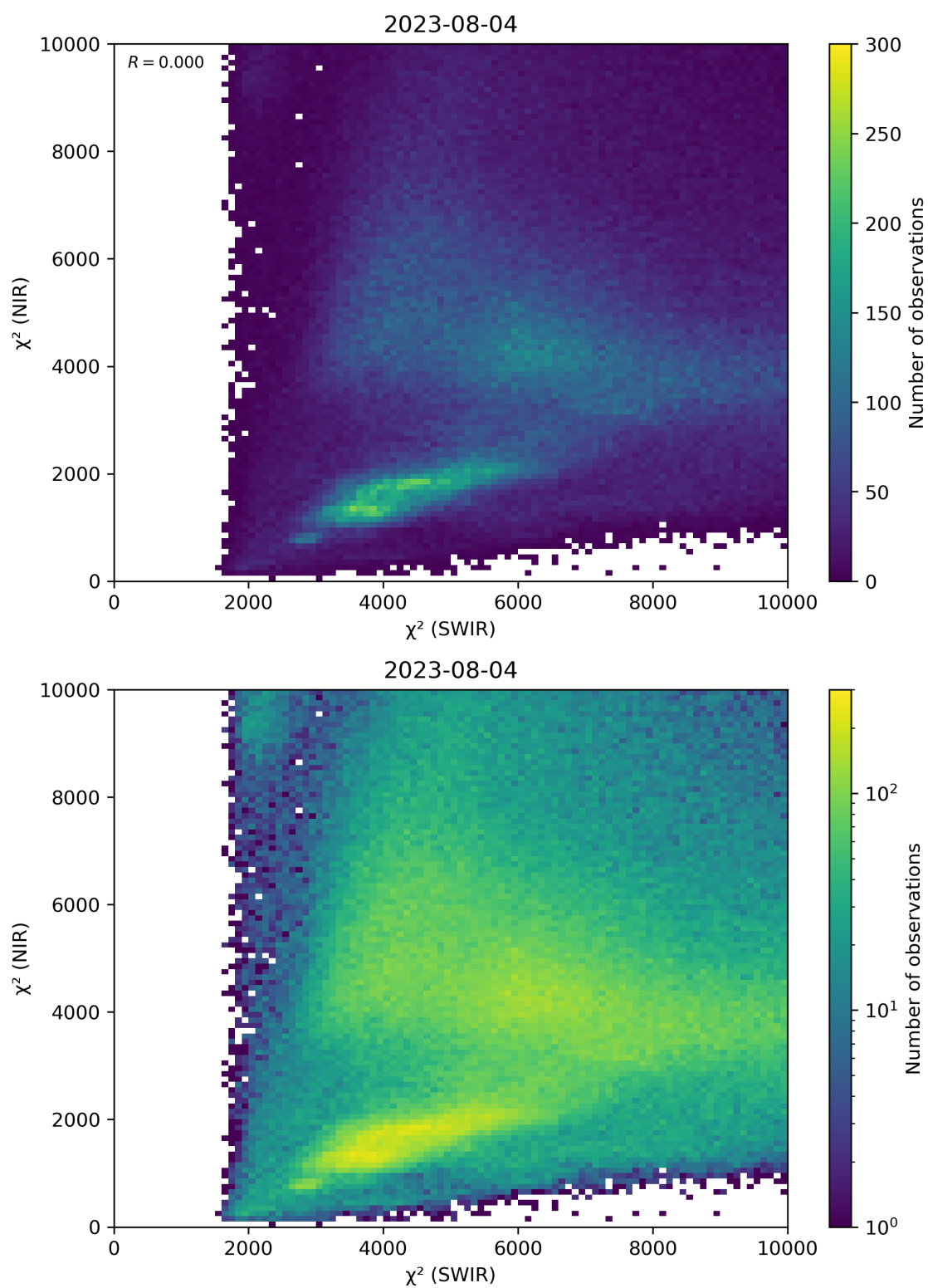
Figure 47: Scatter density plot of “ \chi^2 (SWIR)” against “ \chi^2 (NIR)” for 2023-08-04 to 2023-08-05.
