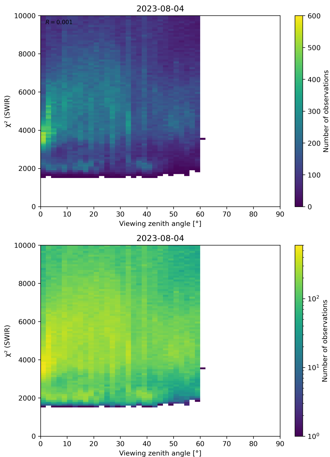
Figure 106: Scatter density plot of “Viewing zenith angle” against “ \chi^2 (SWIR)” for 2023-08-04 to 2023-08-05.
