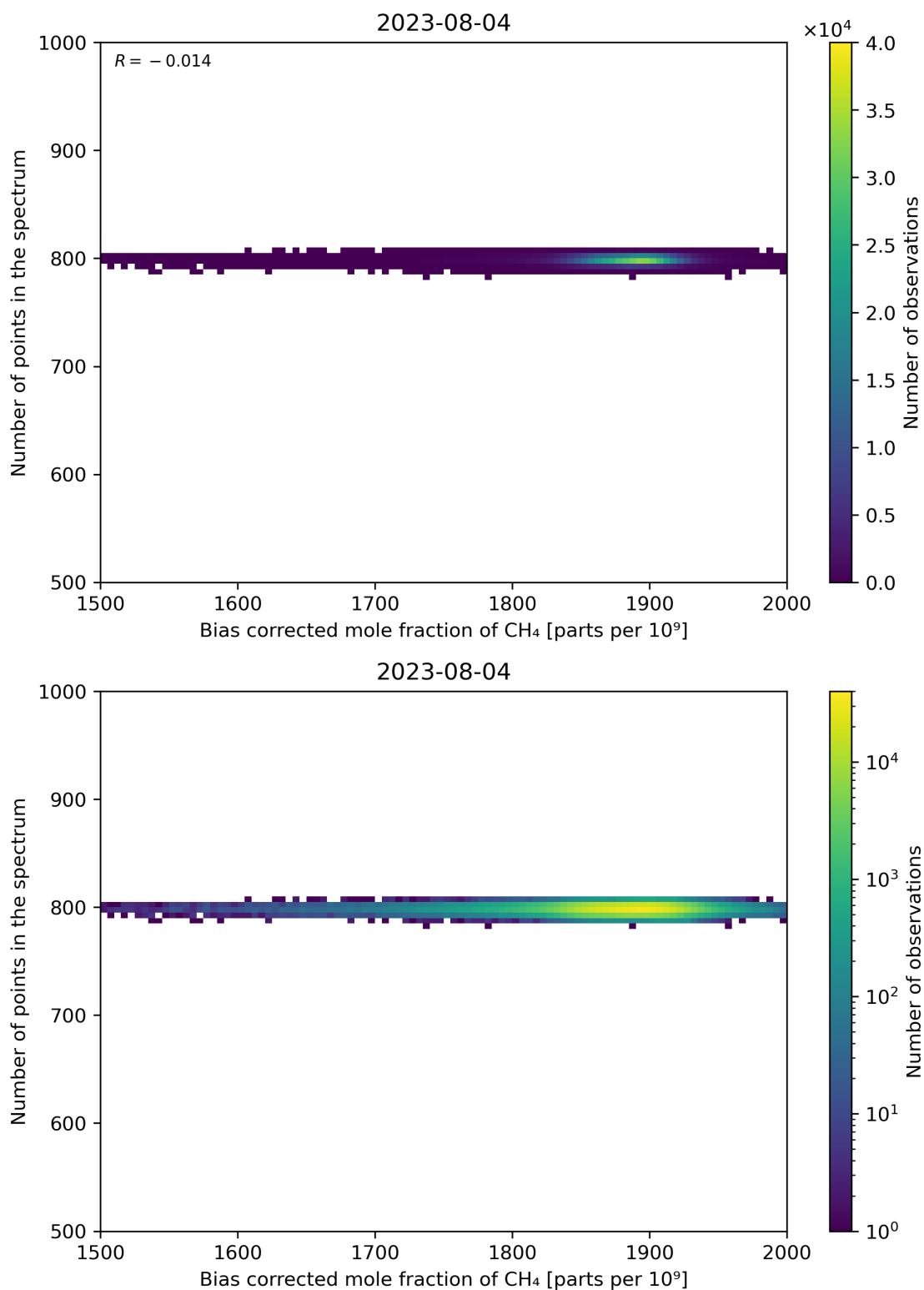
Figure 68: Scatter density plot of “Bias corrected mole fraction of CH 4 ” against “Number of points in the spectrum” for 2023-08-04 to 2023-08-05.
