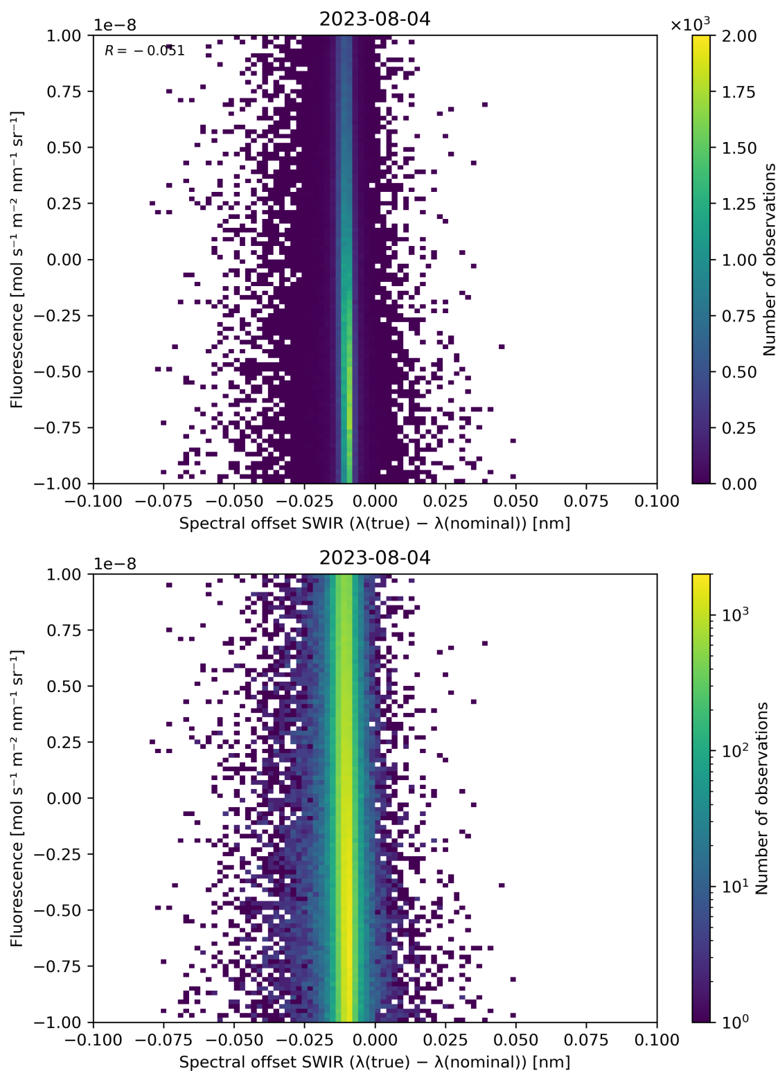
Figure 120: Scatter density plot of “Spectral offset SWIR ( \lambda(\text{true}) - \lambda(\text{nominal}) )” against “Fluorescence” for 2023-08-04 to 2023-08-05.
