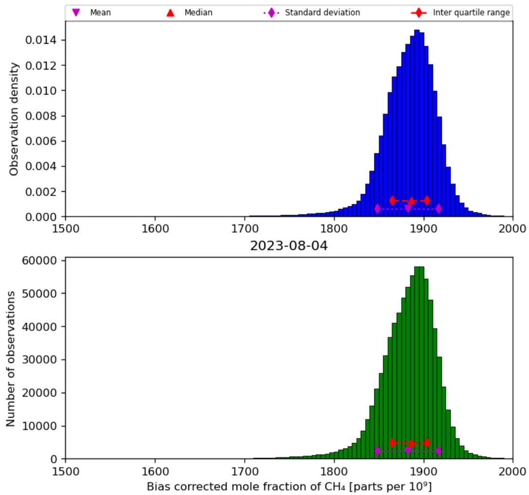
Figure 25: Histogram of “Bias corrected mole fraction of CH 4 ” for 2023-08-04 to 2023-08-05
