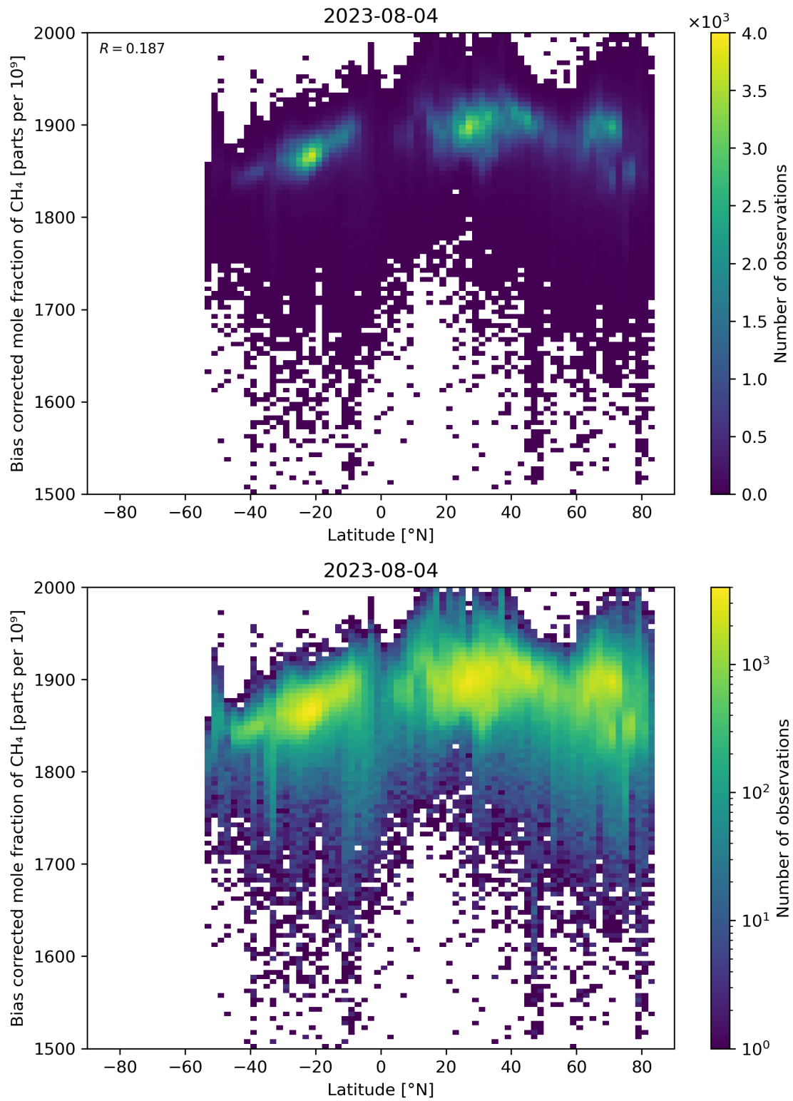
Figure 58: Scatter density plot of “Latitude” against “Bias corrected mole fraction of \text{CH}_4 ” for 2023-08-04 to 2023-08-05.
