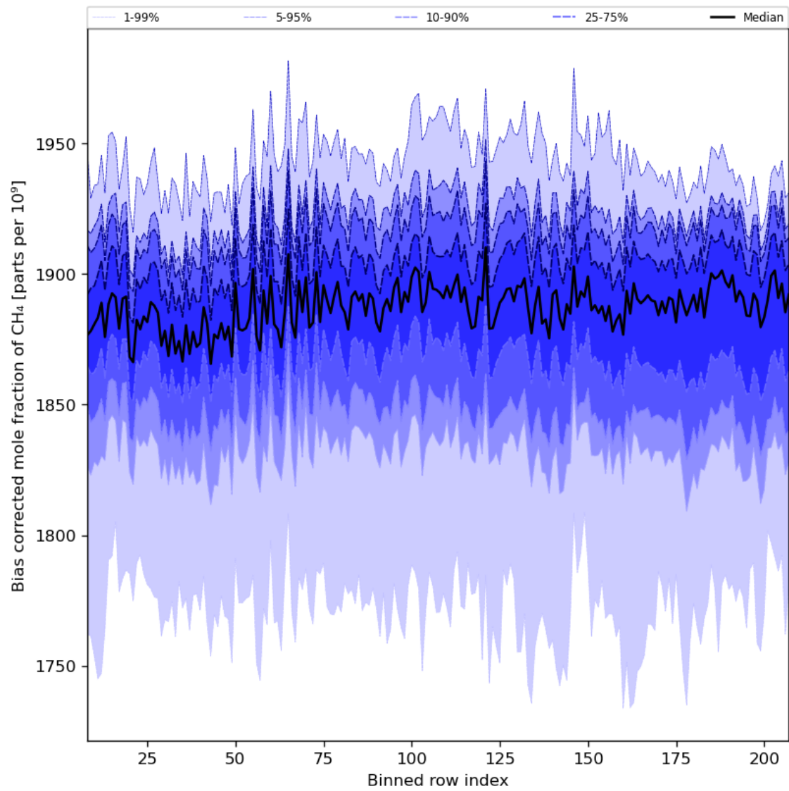
Figure 36: Along track statistics of “Bias corrected mole fraction of \text{CH}_4 ” for 2023-08-04 to 2023-08-05
