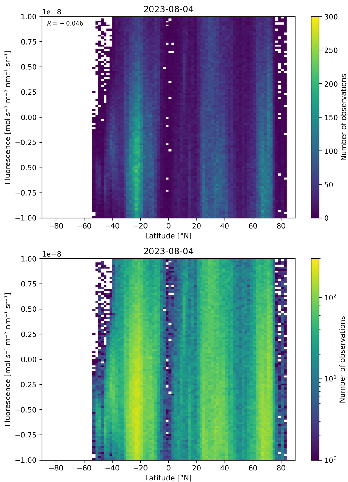
Figure 56: Scatter density plot of “Latitude” against “Fluorescence” for 2023-08-04 to 2023-08-05.
