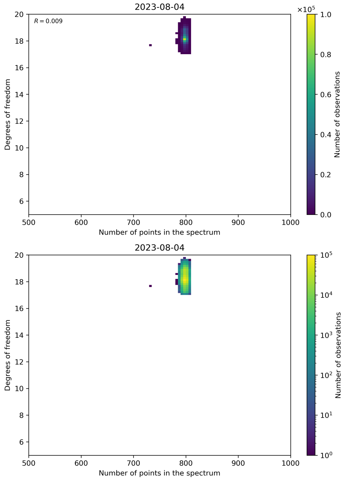
Figure 90: Scatter density plot of “Number of points in the spectrum” against “Degrees of freedom” for 2023-08-04 to 2023-08-05.
