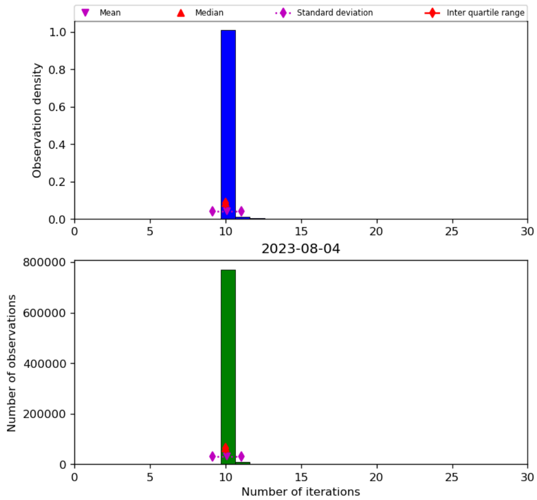
Figure 31: Histogram of “Number of iterations” for 2023-08-04 to 2023-08-05
