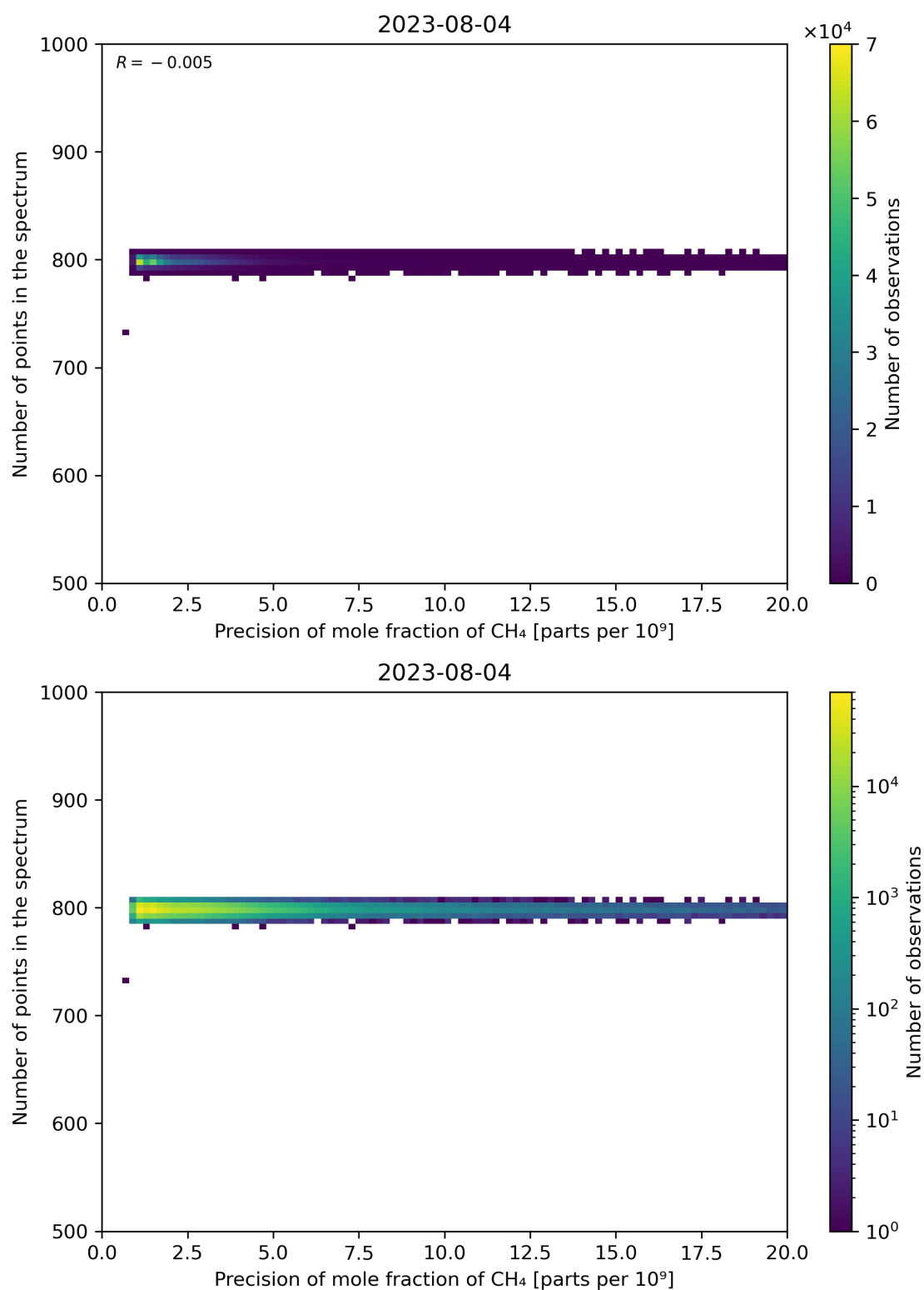
Figure 84: Scatter density plot of “Precision of mole fraction of CH 4 ” against “Number of points in the spectrum” for 2023-08-04 to 2023-08-05.
