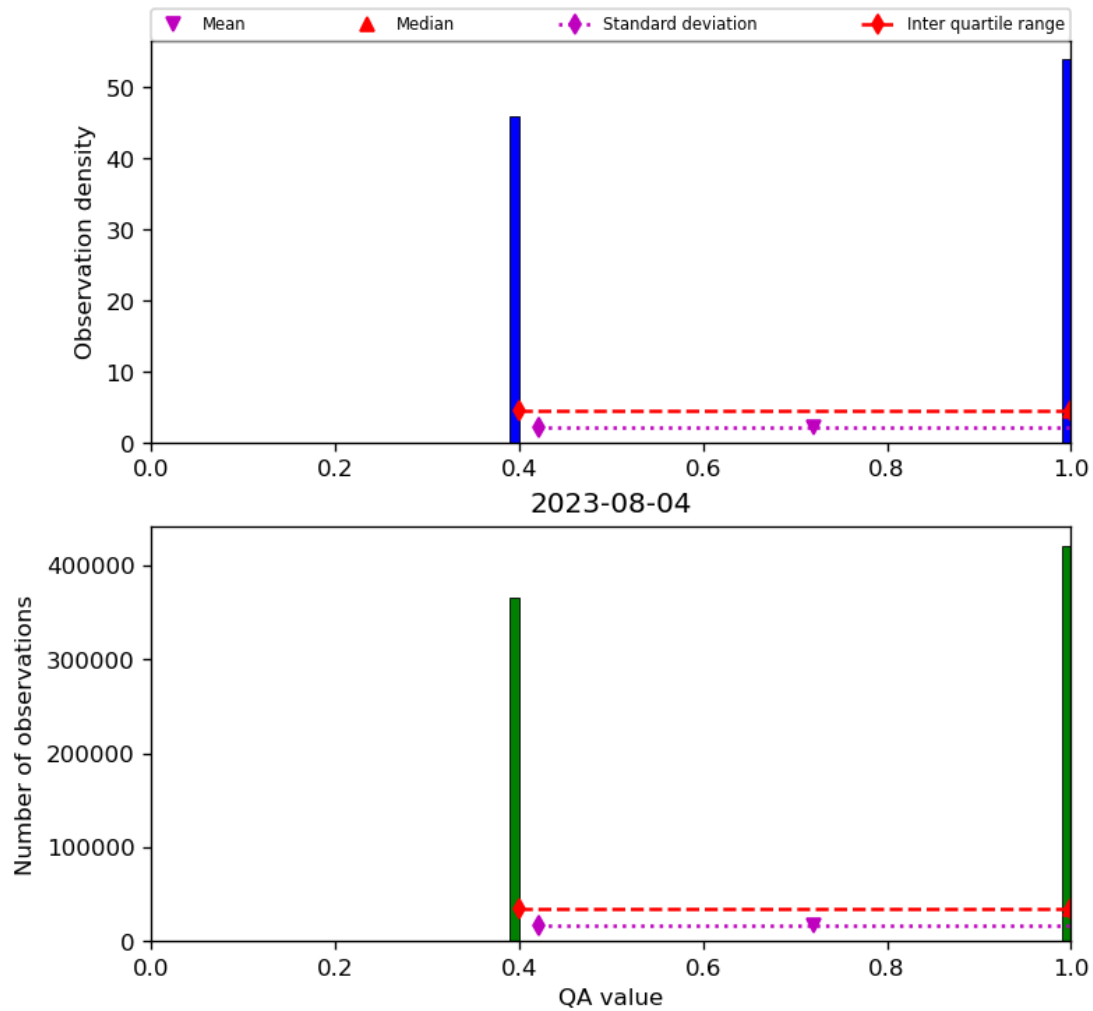
Figure 22: Histogram of “QA value” for 2023-08-04 to 2023-08-05
