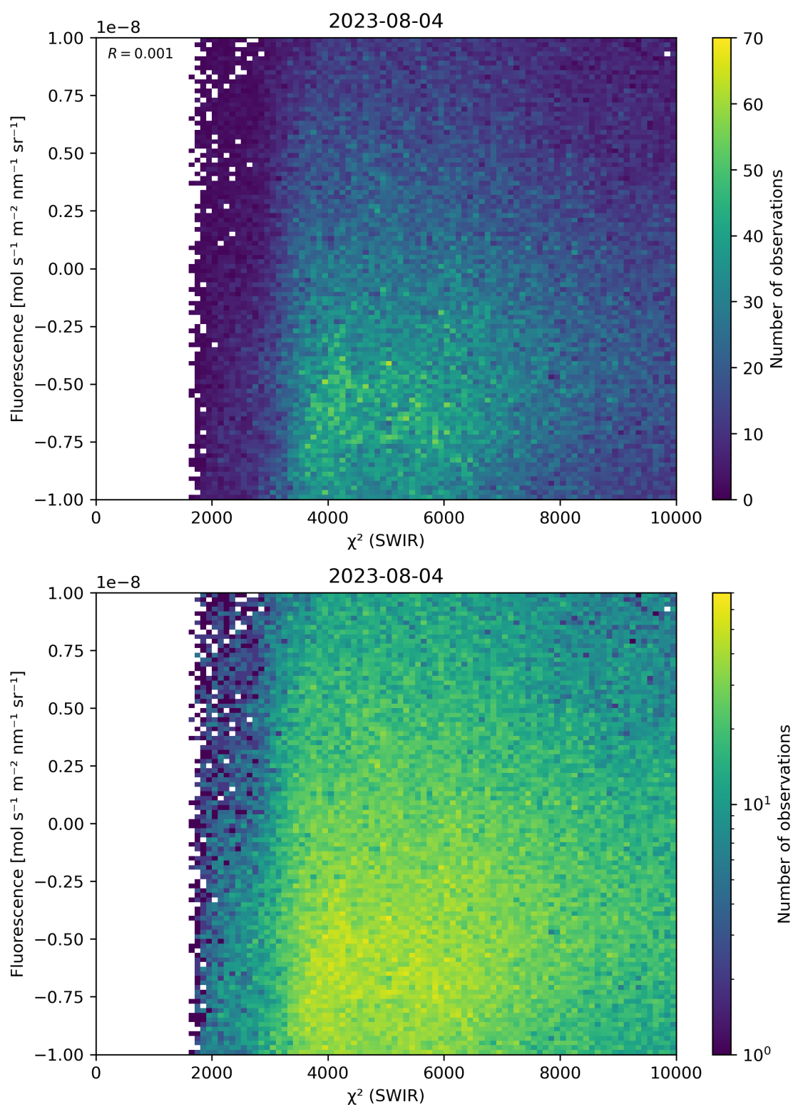
Figure 49: Scatter density plot of “ \chi^2 (SWIR)” against “Fluorescence” for 2023-08-04 to 2023-08-05.
