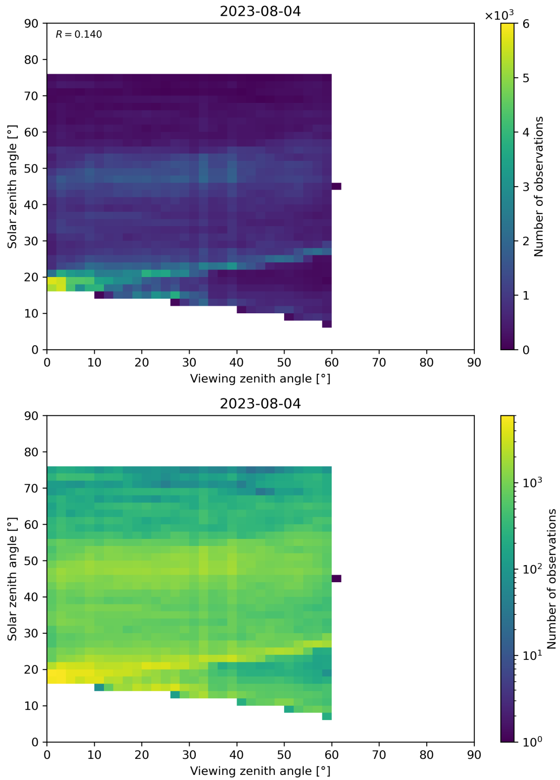
Figure 115: Scatter density plot of “Viewing zenith angle” against “Solar zenith angle” for 2023-08-04 to 2023-08-05.
