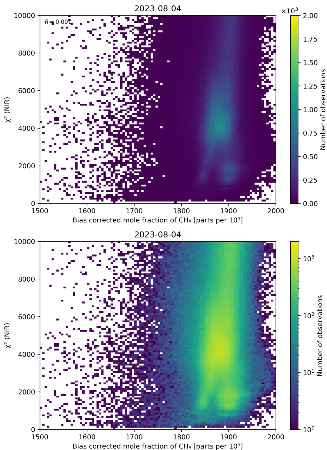
Figure 63: Scatter density plot of “Bias corrected mole fraction of CH 4 ” against “ \chi^2 (NIR)” for 2023-08-04 to 2023-08-05.
