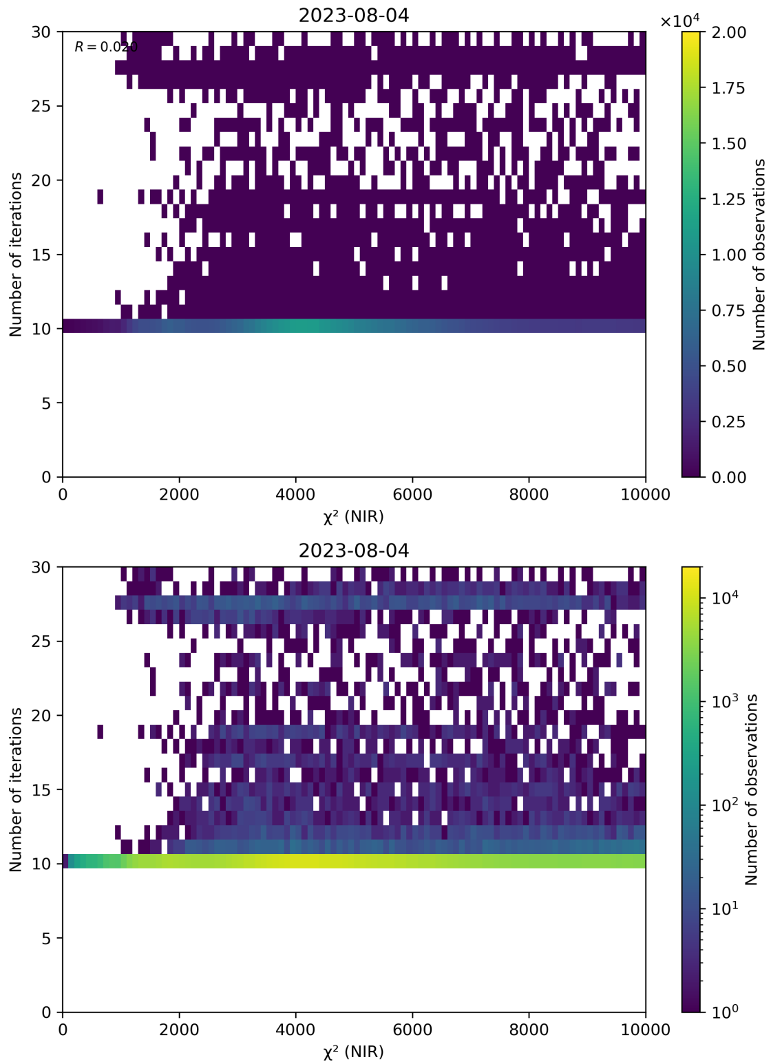
Figure 46: Scatter density plot of “ \chi^2 (NIR)” against “Number of iterations” for 2023-08-04 to 2023-08-05.
