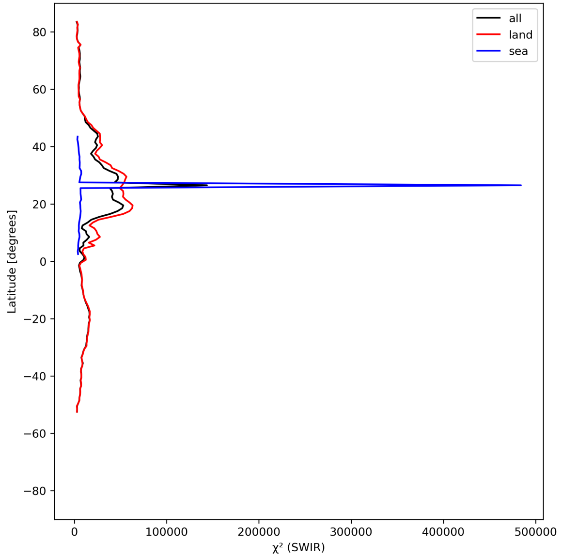
Figure 17: Zonal average of “ \chi^2 (SWIR)” for 2023-08-04 to 2023-08-05.
