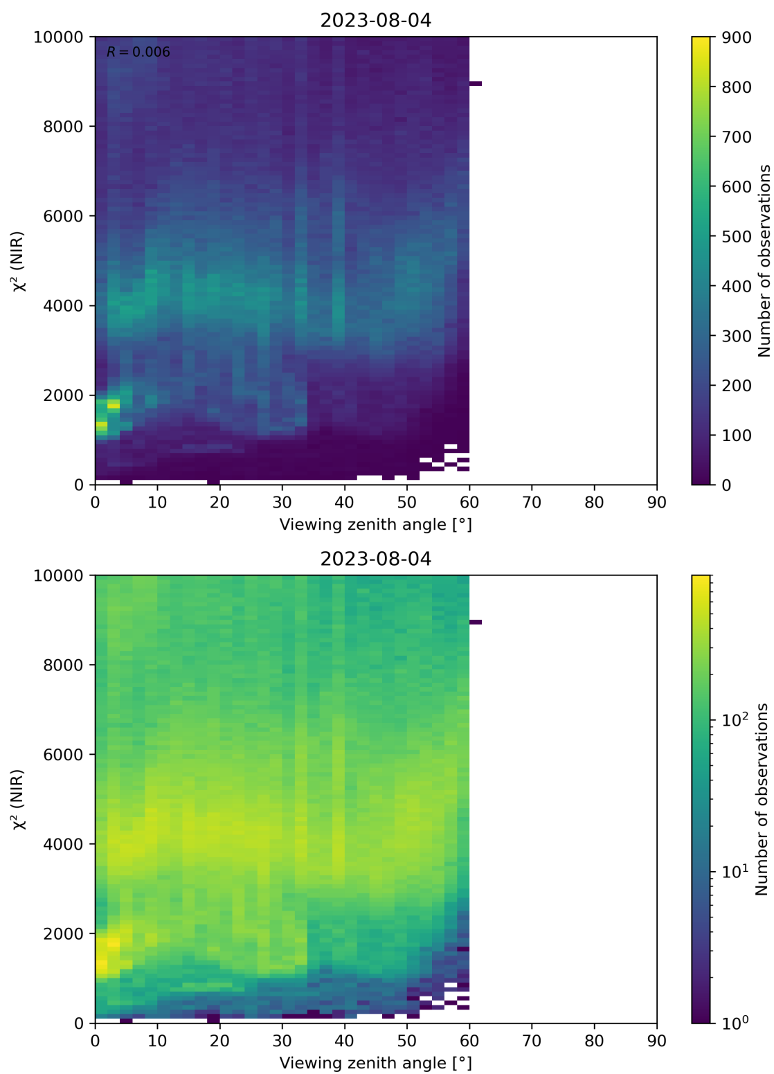
Figure 105: Scatter density plot of “Viewing zenith angle” against “ \chi^2 (NIR)” for 2023-08-04 to 2023-08-05.
