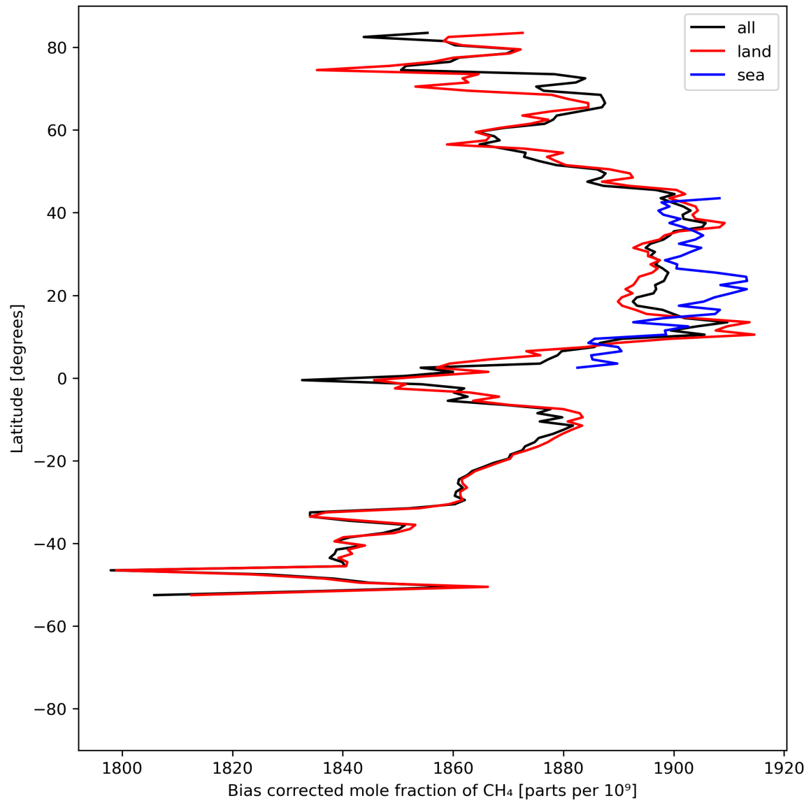
Figure 14: Zonal average of “Bias corrected mole fraction of \text{CH}_4 ” for 2023-08-04 to 2023-08-05.
