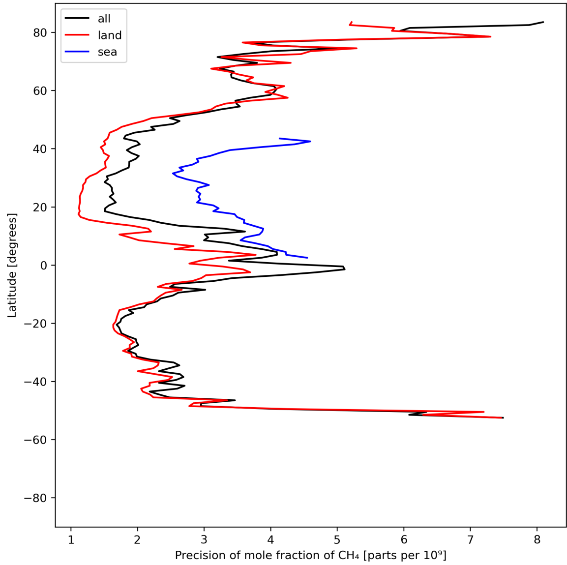
Figure 13: Zonal average of “Precision of mole fraction of CH 4 ” for 2023-08-04 to 2023-08-05.
