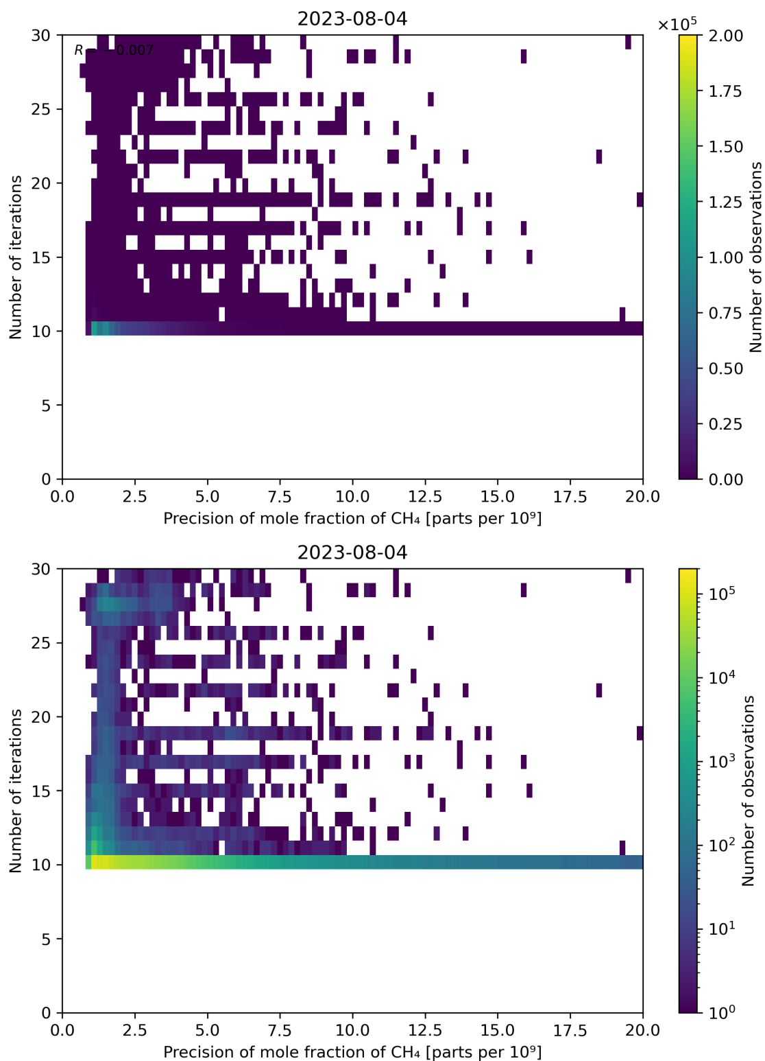
Figure 83: Scatter density plot of “Precision of mole fraction of CH 4 ” against “Number of iterations” for 2023-08-04 to 2023-08-05.
