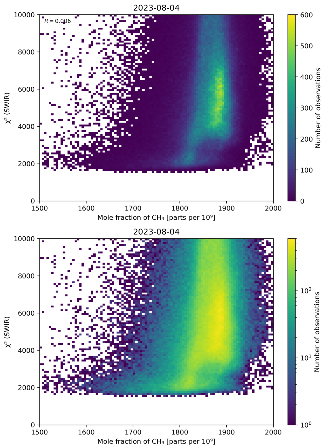
Figure 71: Scatter density plot of “Mole fraction of \text{CH}_4 ” against “ \chi^2 (SWIR)” for 2023-08-04 to 2023-08-05.
