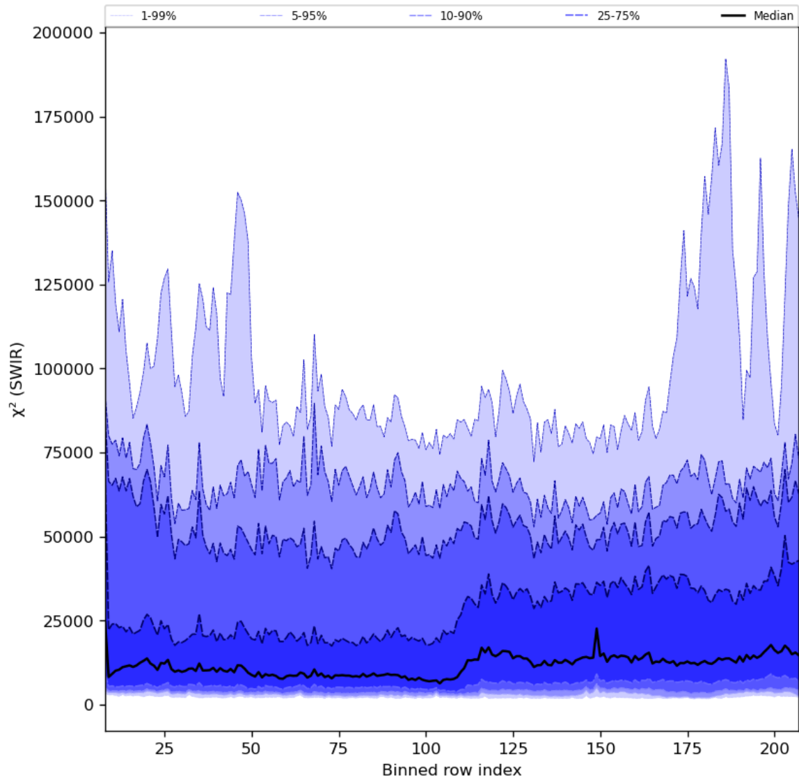
Figure 39: Along track statistics of " \chi^2 (SWIR)" for 2023-08-04 to 2023-08-05
