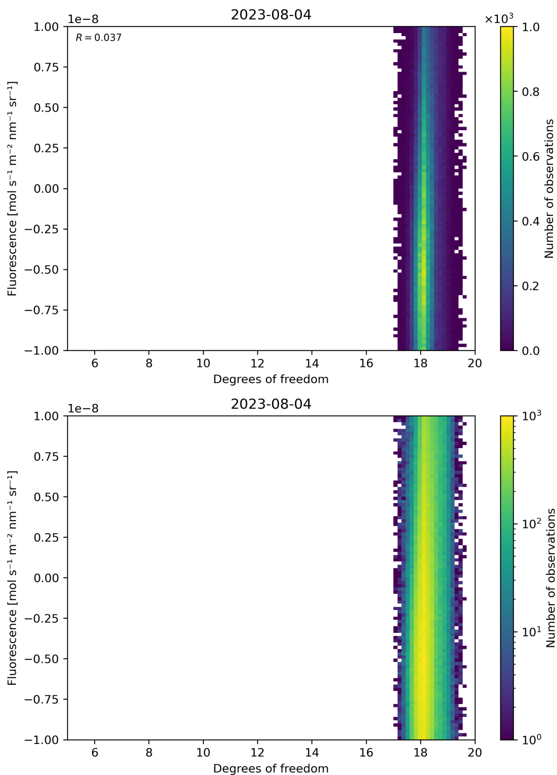
Figure 51: Scatter density plot of “Degrees of freedom” against “Fluorescence” for 2023-08-04 to 2023-08-05.
