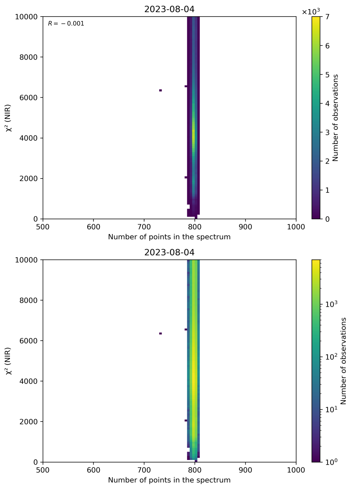
Figure 88: Scatter density plot of “Number of points in the spectrum” against “ \chi^2 (NIR)” for 2023-08-04 to 2023-08-05.
