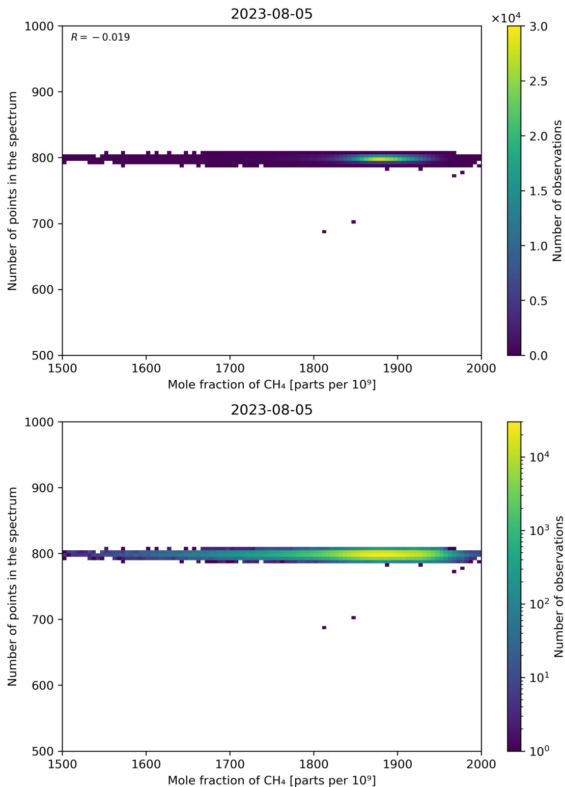
Figure 77: Scatter density plot of “Mole fraction of CH 4 ” against “Number of points in the spectrum” for 2023-08-04 to 2023-08-06.
