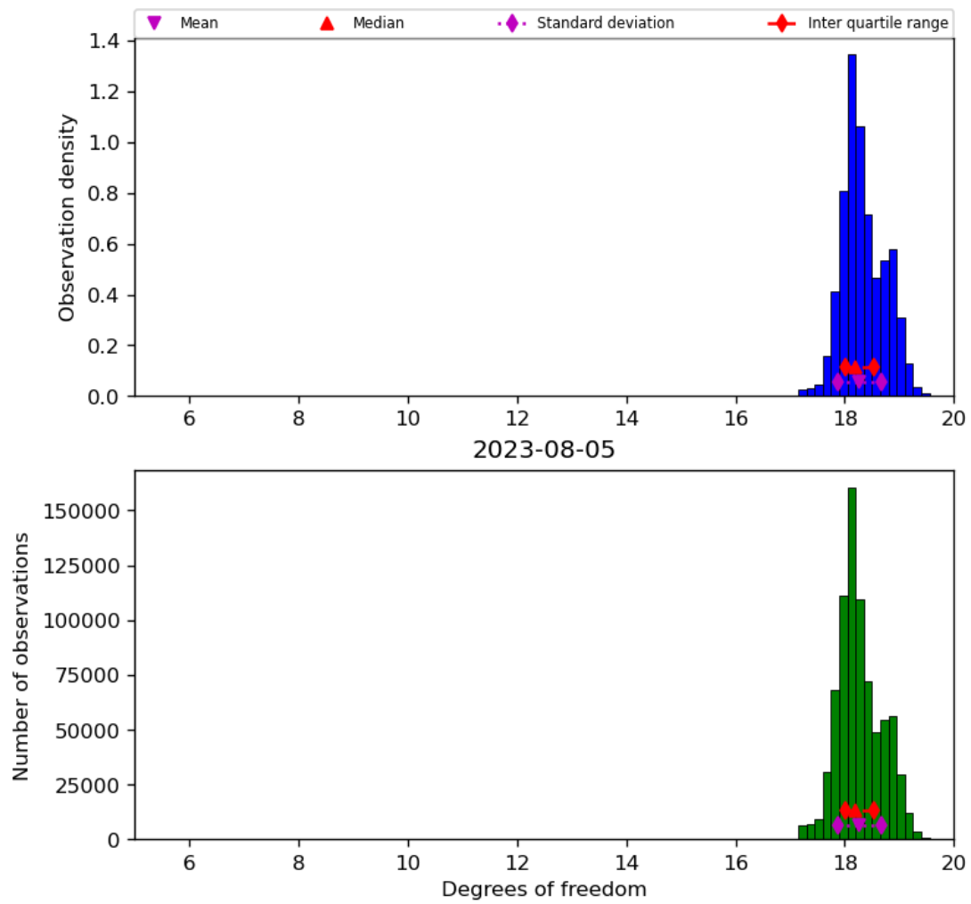
Figure 30: Histogram of “Degrees of freedom” for 2023-08-04 to 2023-08-06
