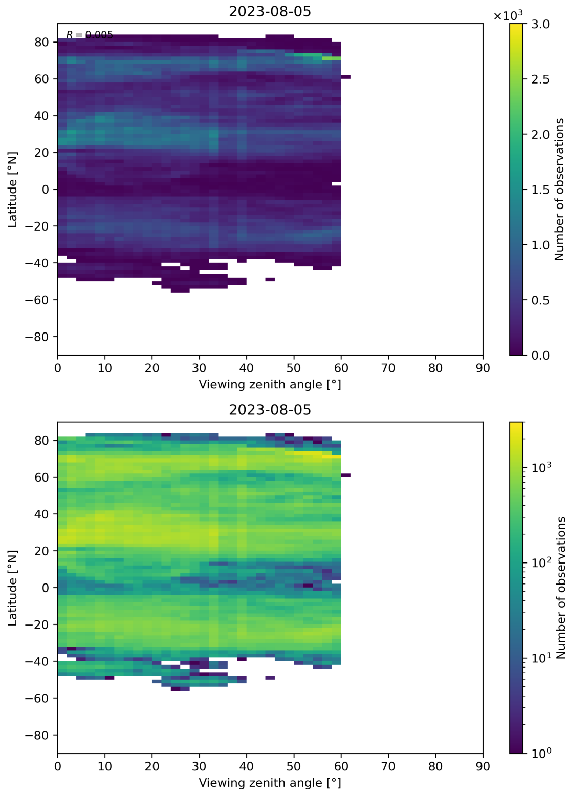
Figure 109: Scatter density plot of “Viewing zenith angle” against “Latitude” for 2023-08-04 to 2023-08-06.
