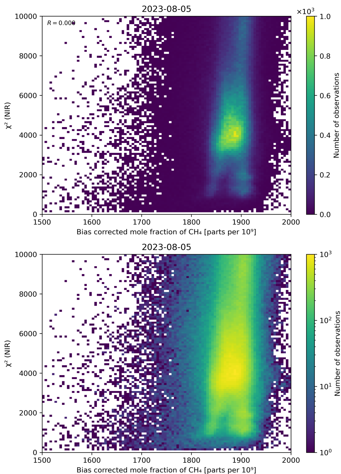
Figure 63: Scatter density plot of “Bias corrected mole fraction of CH 4 ” against “ \chi^2 (NIR)” for 2023-08-04 to 2023-08-06.
