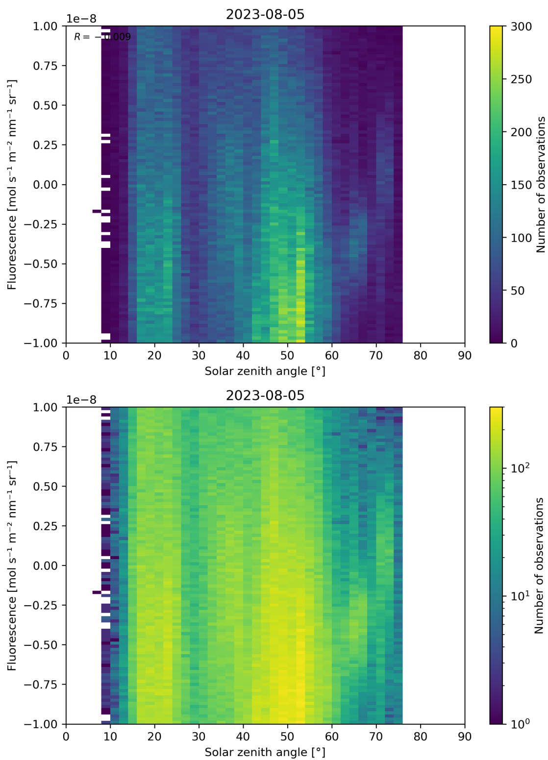
Figure 97: Scatter density plot of “Solar zenith angle” against “Fluorescence” for 2023-08-04 to 2023-08-06.
