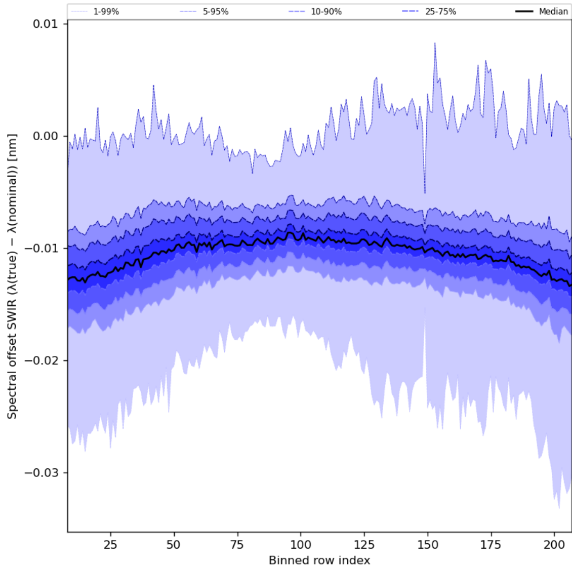
Figure 38: Along track statistics of "Spectral offset SWIR ( \lambda(\text{true}) - \lambda(\text{nominal}) )" for 2023-08-04 to 2023-08-06
