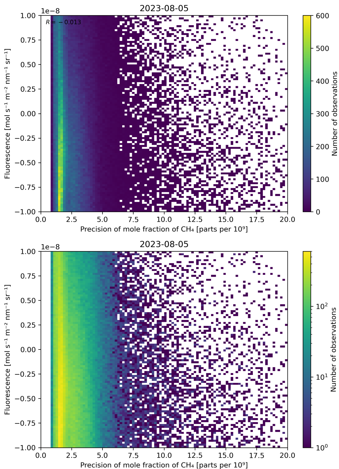
Figure 81: Scatter density plot of “Precision of mole fraction of \text{CH}_4 ” against “Fluorescence” for 2023-08-04 to 2023-08-06.
