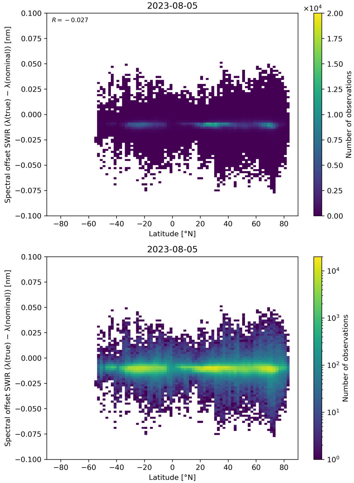
Figure 62: Scatter density plot of “Latitude” against “Spectral offset SWIR ( \lambda(\text{true}) - \lambda(\text{nominal}) )” for 2023-08-04 to 2023-08-06.
