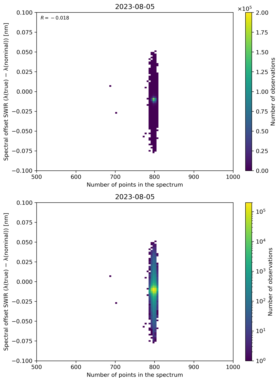
Figure 93: Scatter density plot of “Number of points in the spectrum” against “Spectral offset SWIR ( \lambda(\text{true}) - \lambda(\text{nominal}) )” for 2023-08-04 to 2023-08-06.
