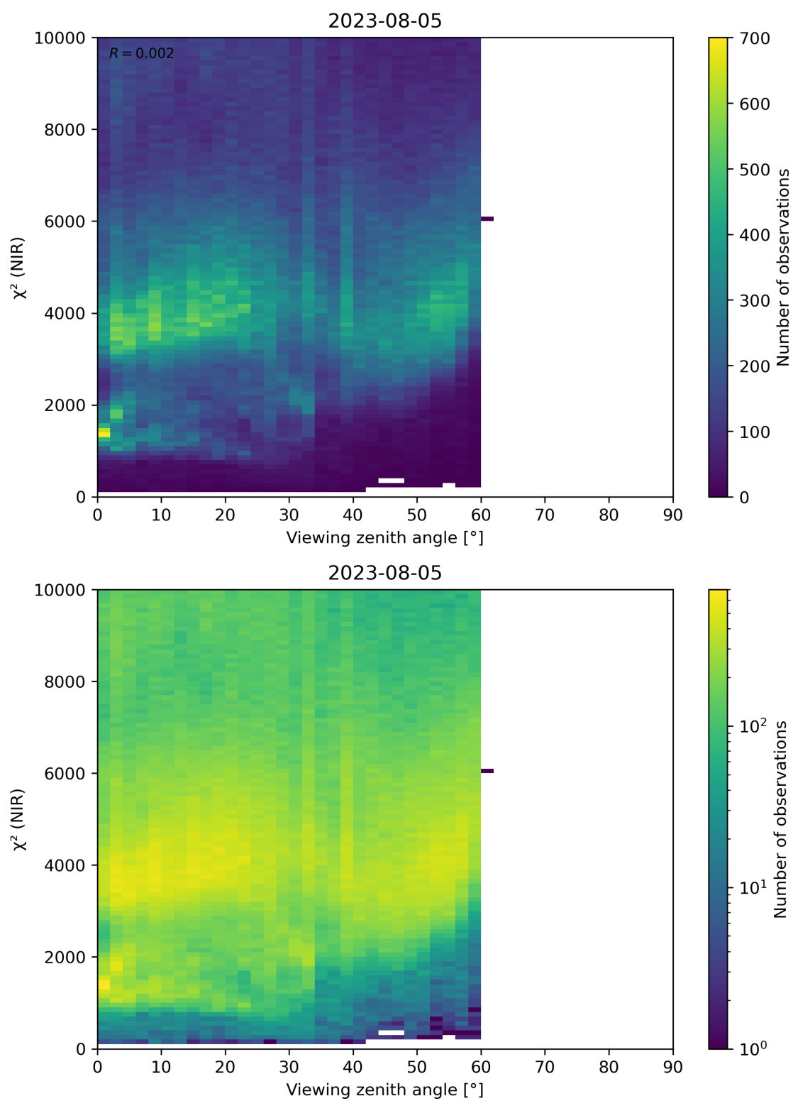
Figure 105: Scatter density plot of “Viewing zenith angle” against “ \chi^2 (NIR)” for 2023-08-04 to 2023-08-06.
