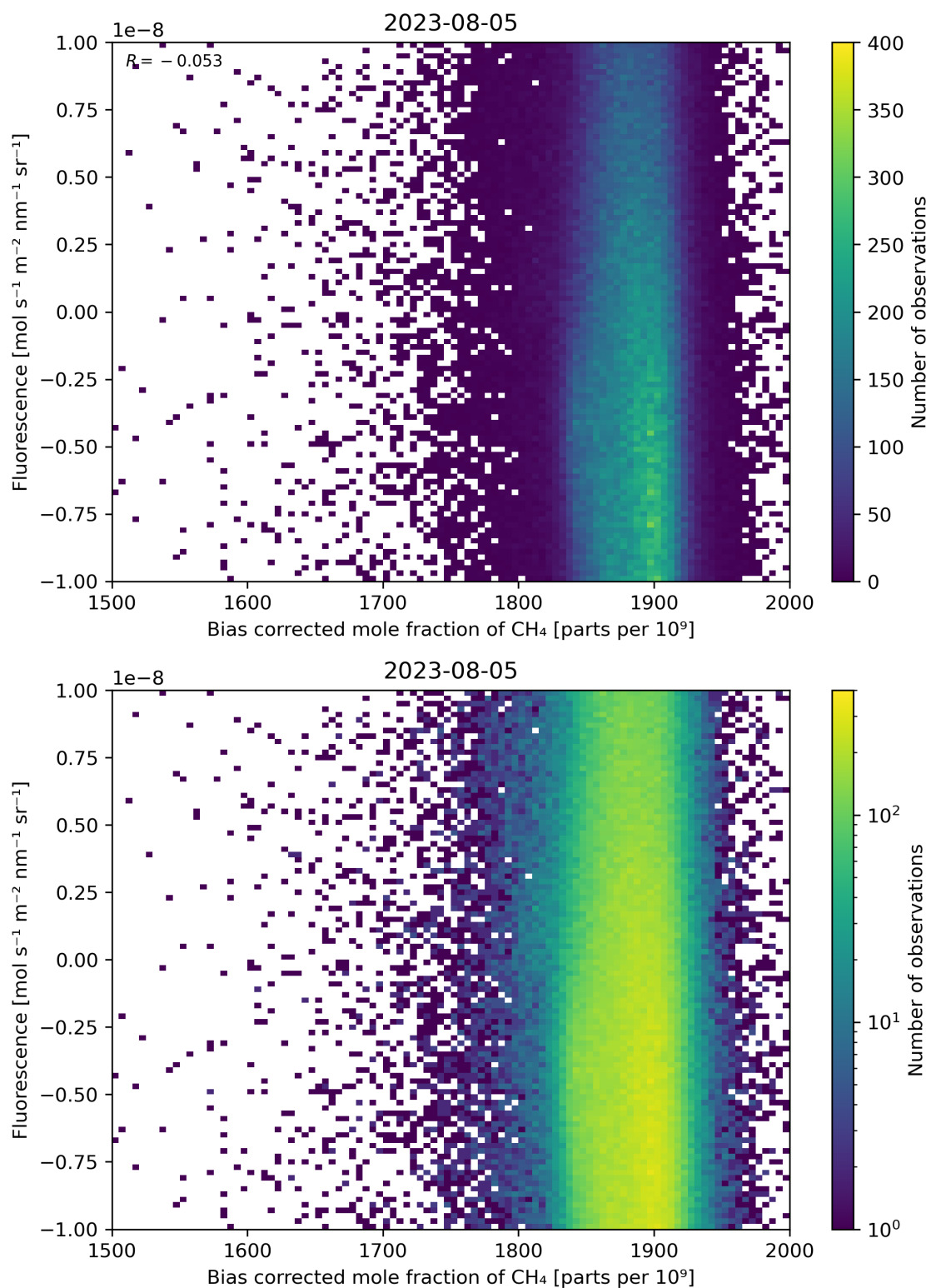
Figure 66: Scatter density plot of “Bias corrected mole fraction of \text{CH}_4 ” against “Fluorescence” for 2023-08-04 to 2023-08-06.
