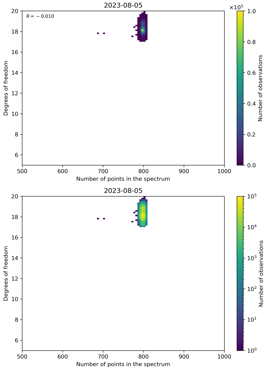
Figure 90: Scatter density plot of “Number of points in the spectrum” against “Degrees of freedom” for 2023-08-04 to 2023-08-06.
