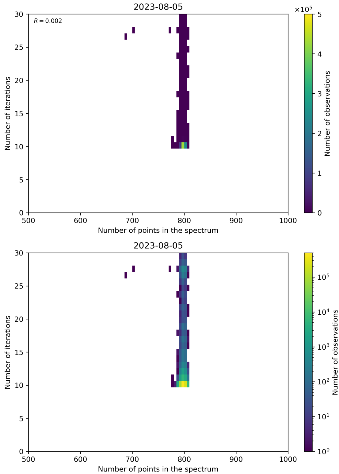
Figure 92: Scatter density plot of “Number of points in the spectrum” against “Number of iterations” for 2023-08-04 to 2023-08-06.
