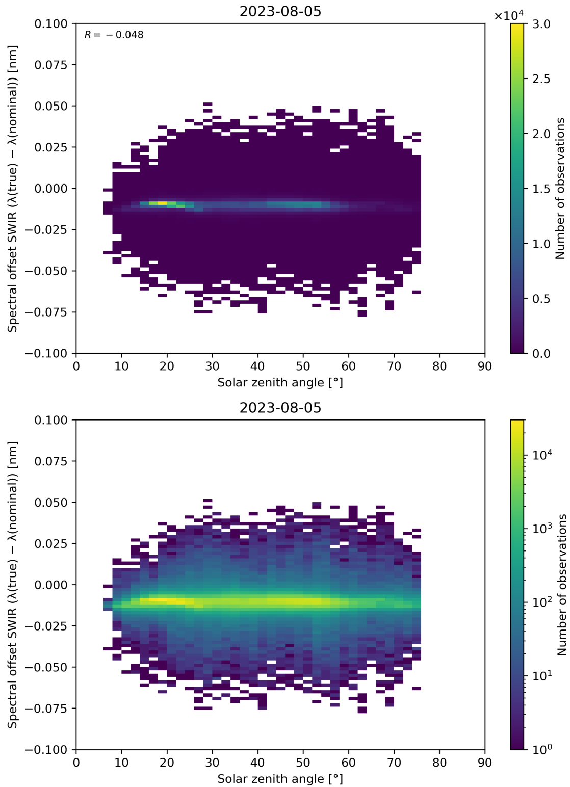
Figure 104: Scatter density plot of “Solar zenith angle” against “Spectral offset SWIR ( \lambda(\text{true}) - \lambda(\text{nominal}) )” for 2023-08-04 to 2023-08-06.
