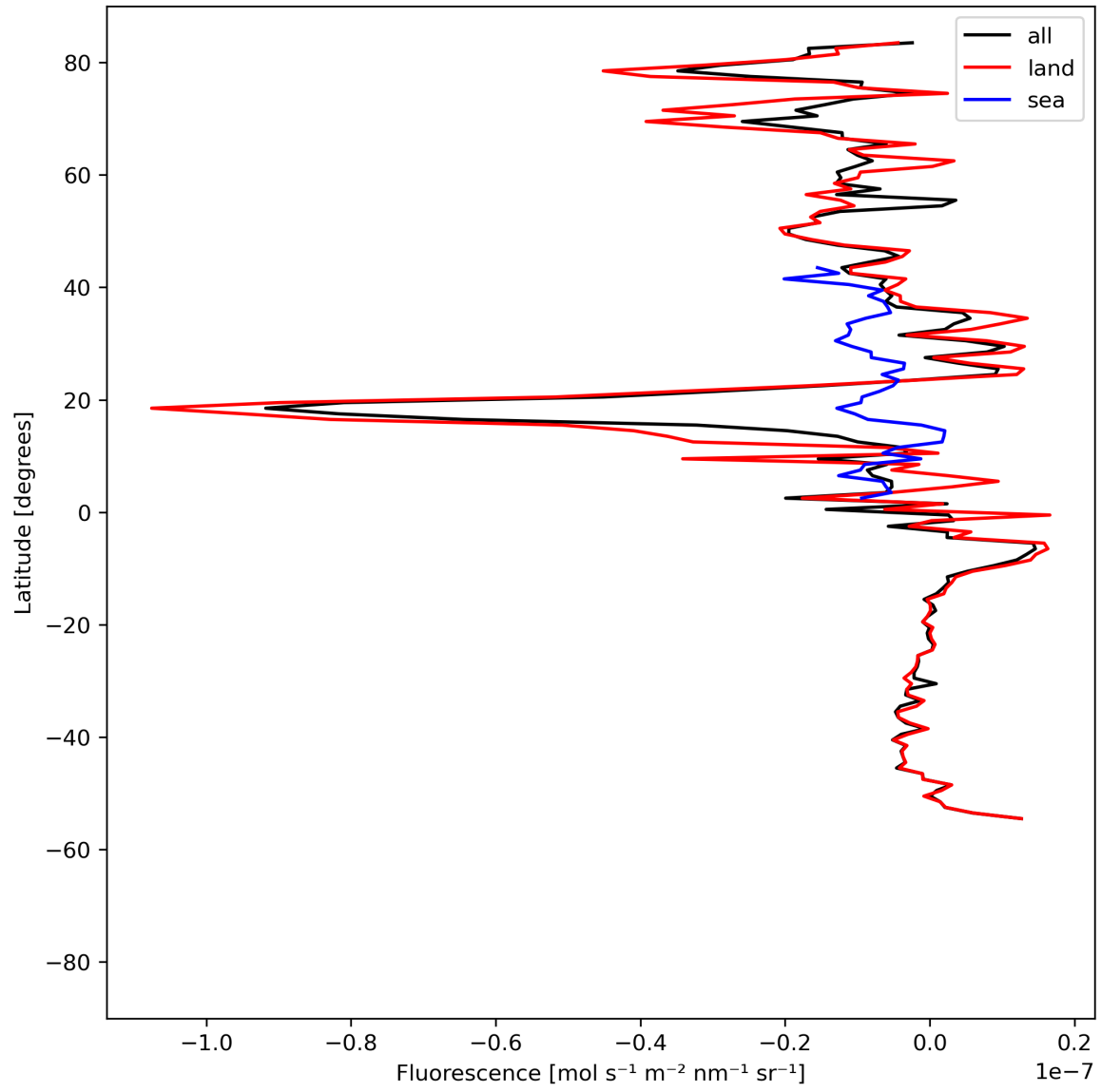
Figure 21: Zonal average of “Fluorescence” for 2023-08-04 to 2023-08-06.
