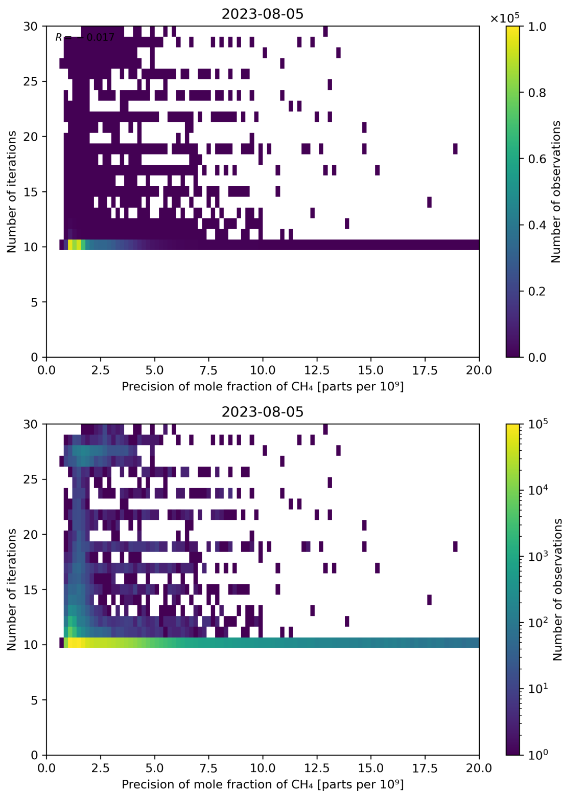
Figure 83: Scatter density plot of “Precision of mole fraction of CH 4 ” against “Number of iterations” for 2023-08-04 to 2023-08-06.
