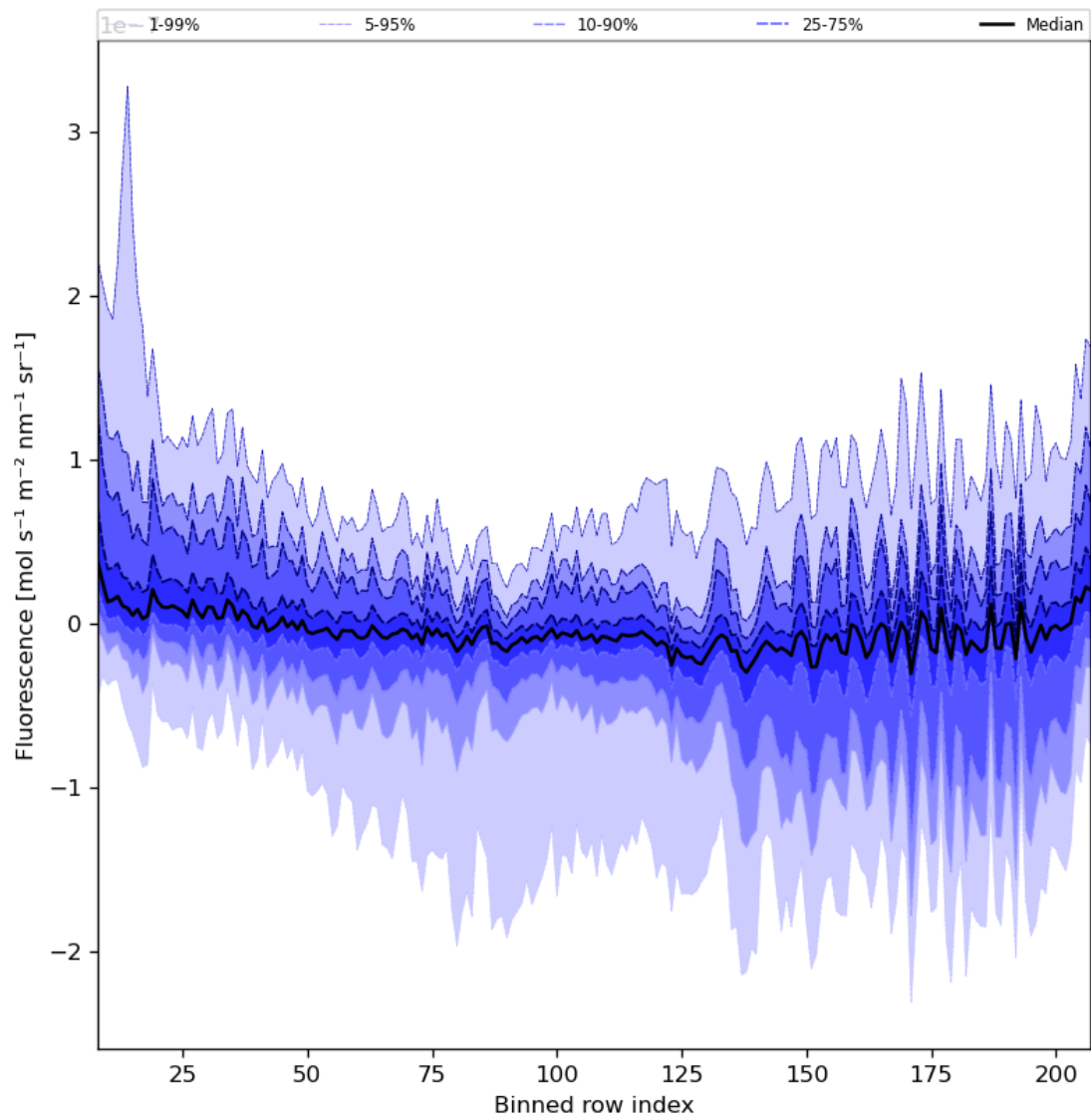
Figure 43: Along track statistics of “Fluorescence” for 2023-08-04 to 2023-08-06
