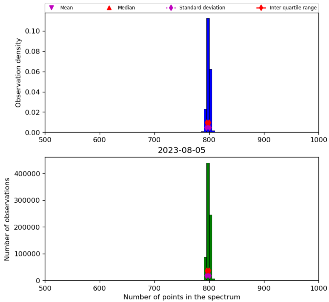
Figure 26: Histogram of “Number of points in the spectrum” for 2023-08-04 to 2023-08-06
