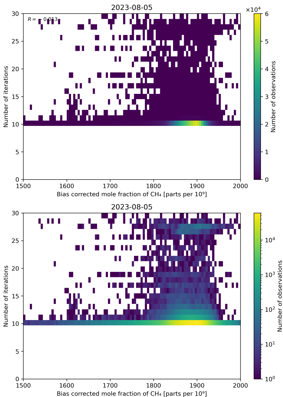
Figure 67: Scatter density plot of “Bias corrected mole fraction of CH 4 ” against “Number of iterations” for 2023-08-04 to 2023-08-06.
