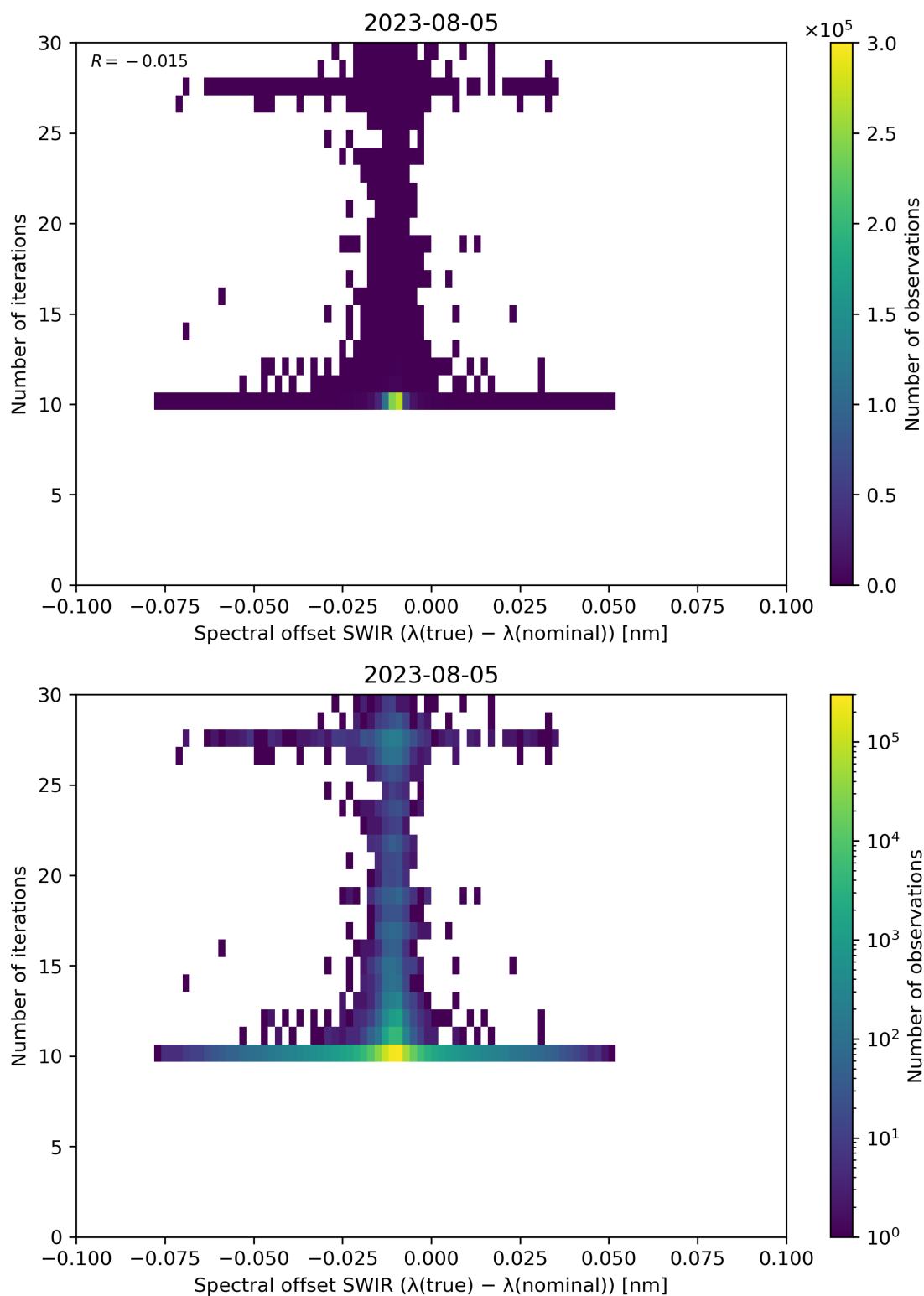
Figure 121: Scatter density plot of “Spectral offset SWIR ( \lambda(\text{true}) - \lambda(\text{nominal}) )” against “Number of iterations” for 2023-08-04 to 2023-08-06.
