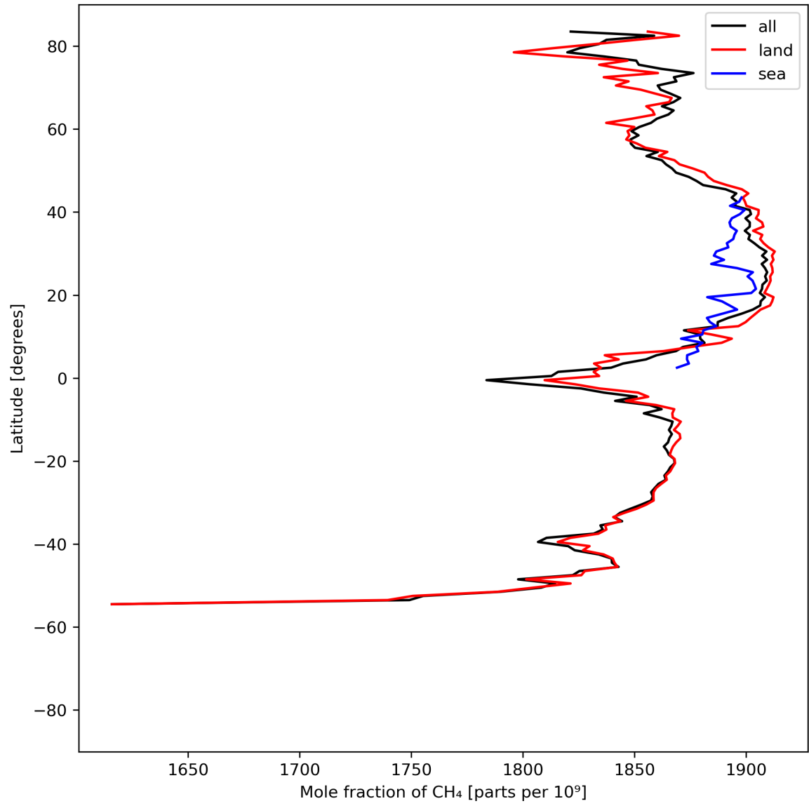
Figure 12: Zonal average of “Mole fraction of \text{CH}_4 ” for 2023-08-04 to 2023-08-06.
