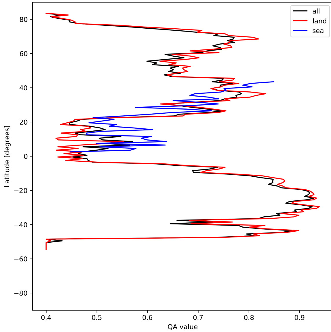
Figure 11: Zonal average of “QA value” for 2023-08-04 to 2023-08-06.
