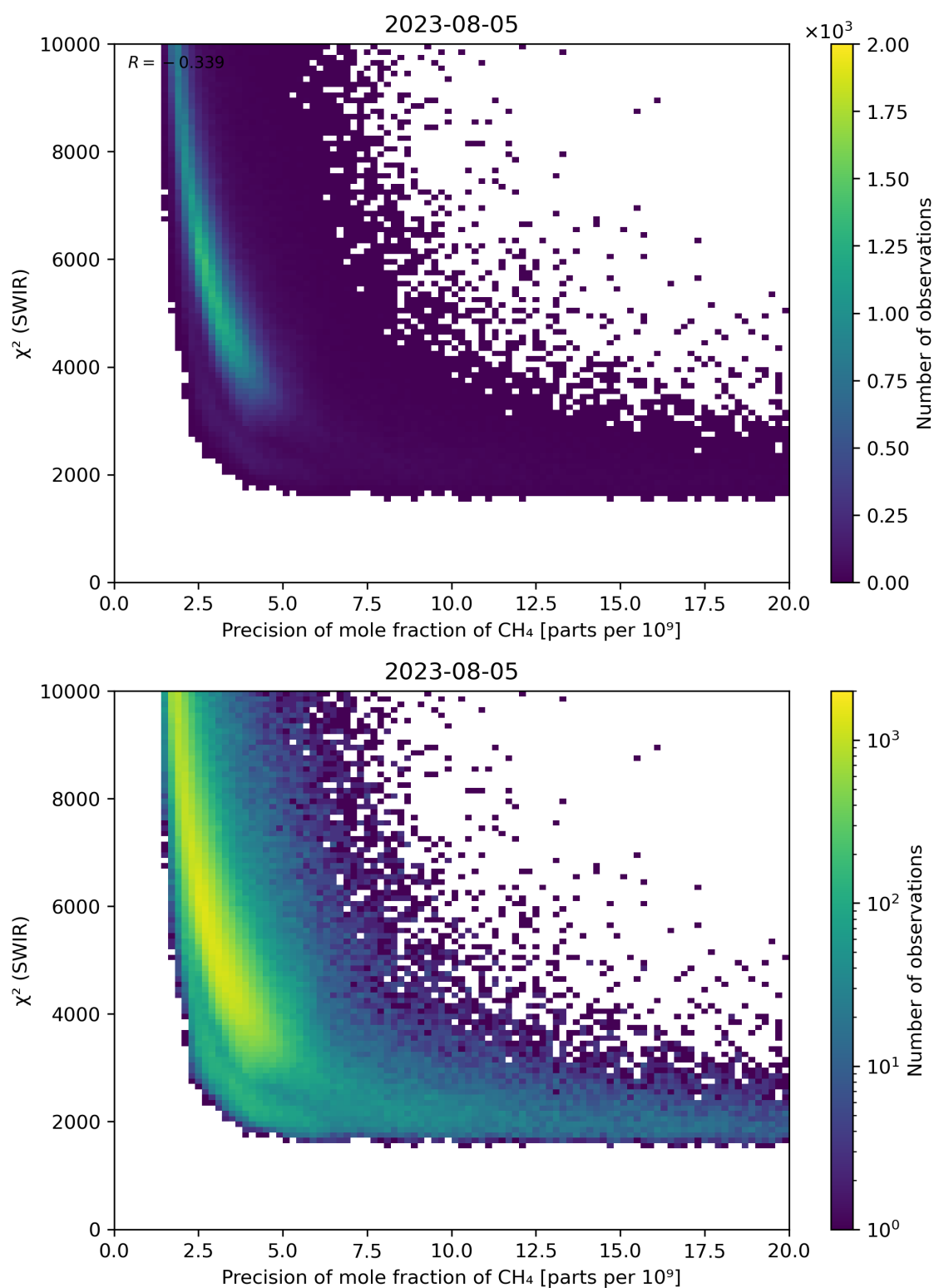
Figure 79: Scatter density plot of “Precision of mole fraction of \text{CH}_4 ” against “ \chi^2 (SWIR)” for 2023-08-04 to 2023-08-06.
