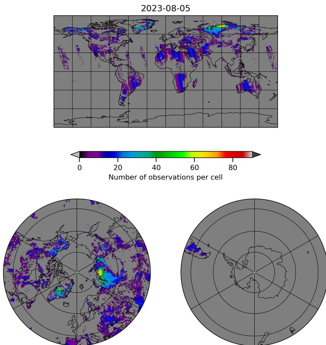
Figure 10: Map of the number of observations for 2023-08-04 to 2023-08-06
