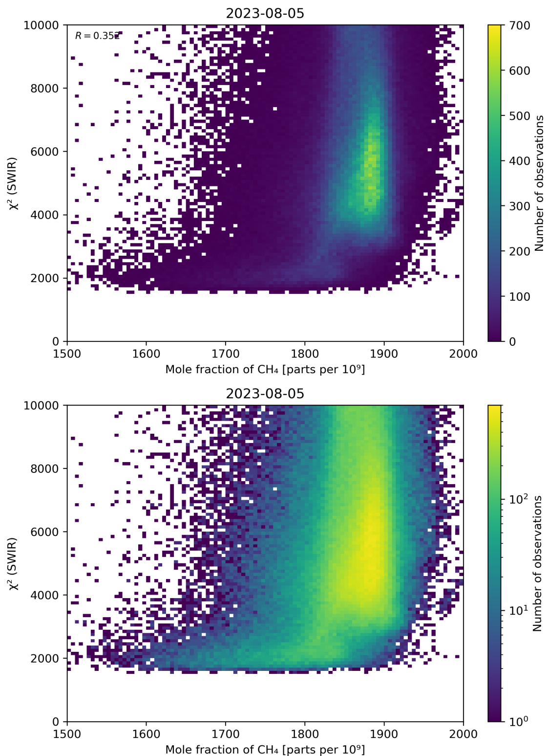
Figure 71: Scatter density plot of “Mole fraction of \text{CH}_4 ” against “ \chi^2 (SWIR)” for 2023-08-04 to 2023-08-06.
