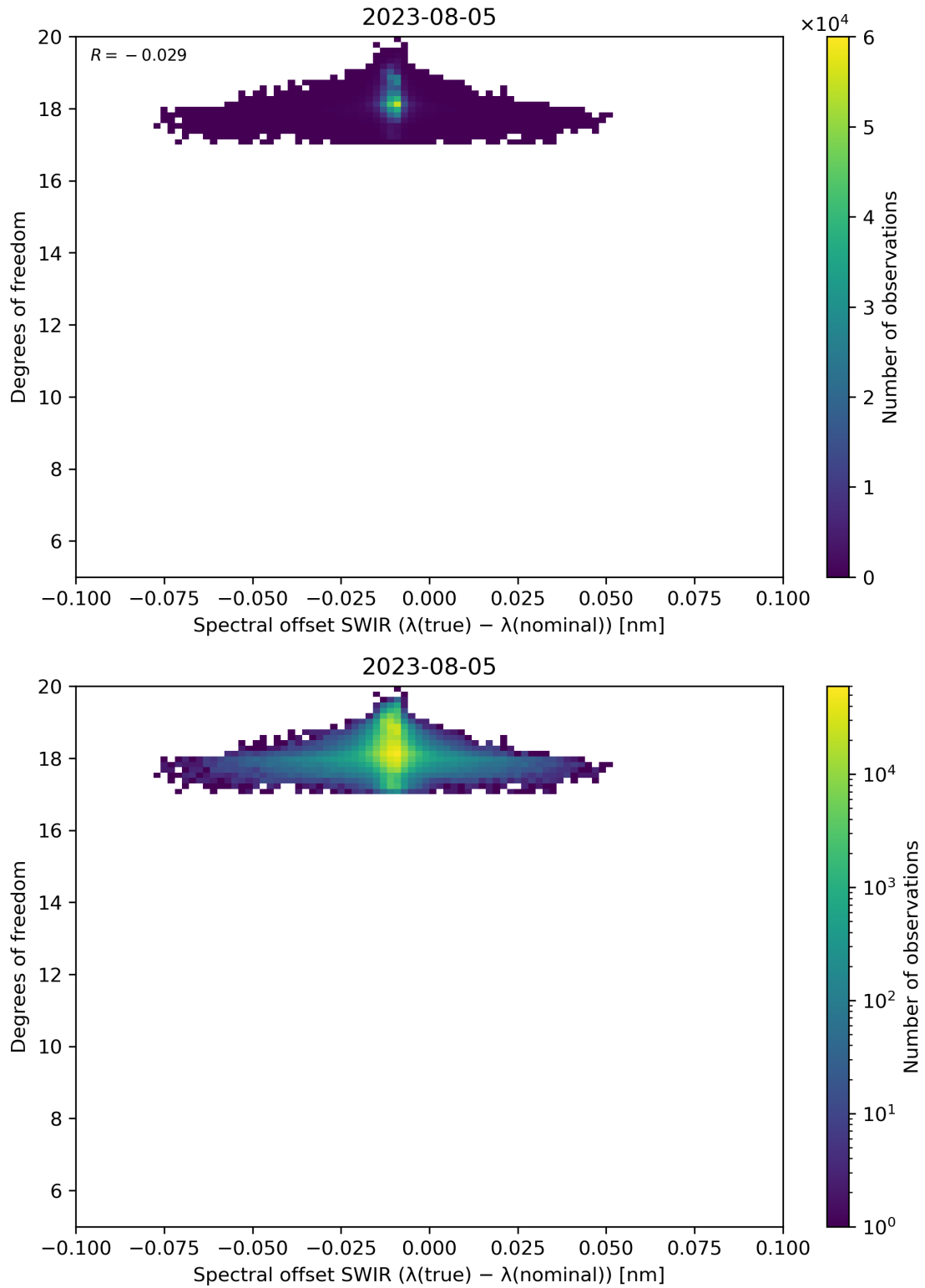
Figure 119: Scatter density plot of “Spectral offset SWIR ( \lambda(\text{true}) - \lambda(\text{nominal}) )” against “Degrees of freedom” for 2023-08-04 to 2023-08-06.
