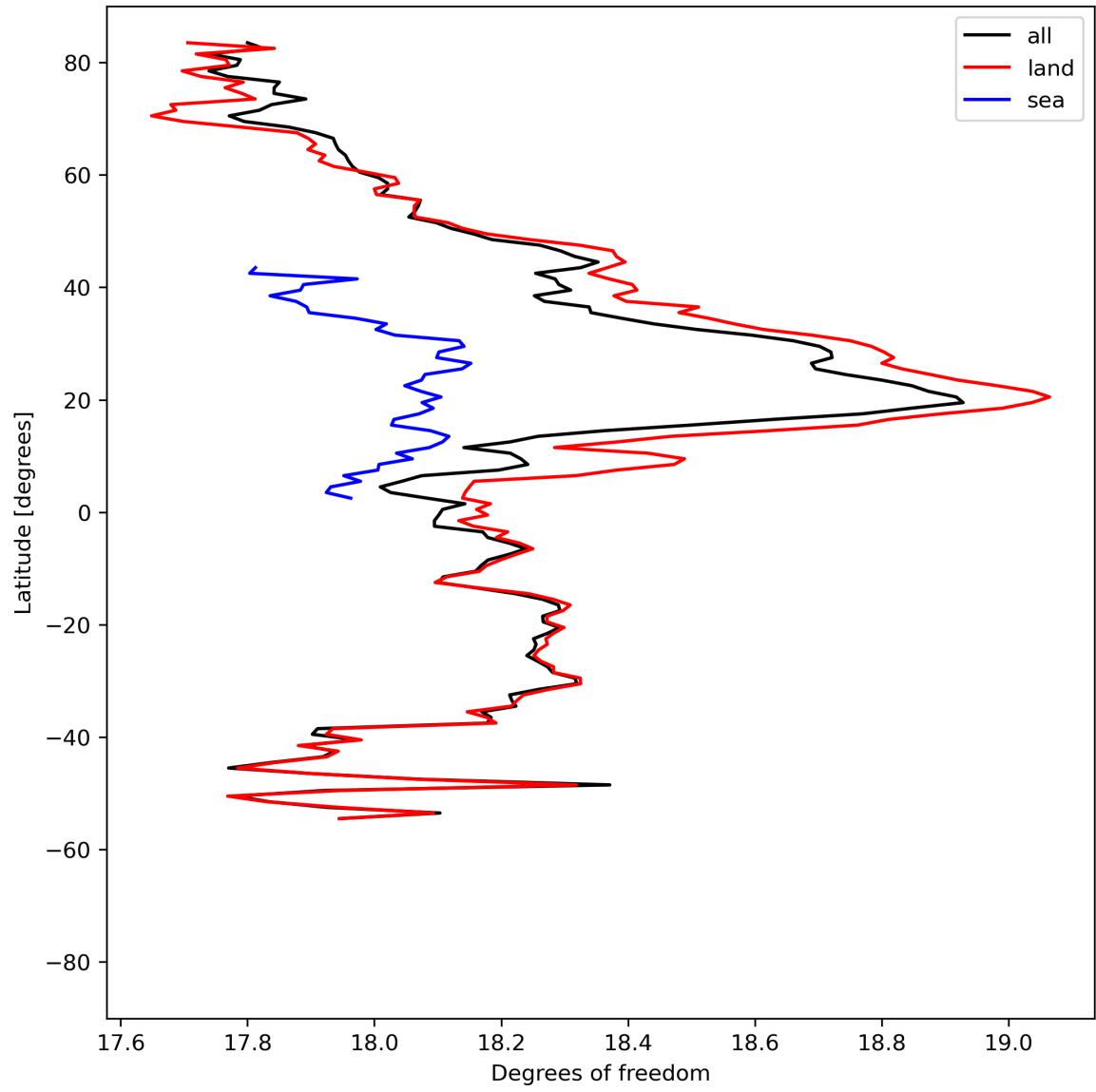
Figure 19: Zonal average of “Degrees of freedom” for 2023-08-04 to 2023-08-06.
