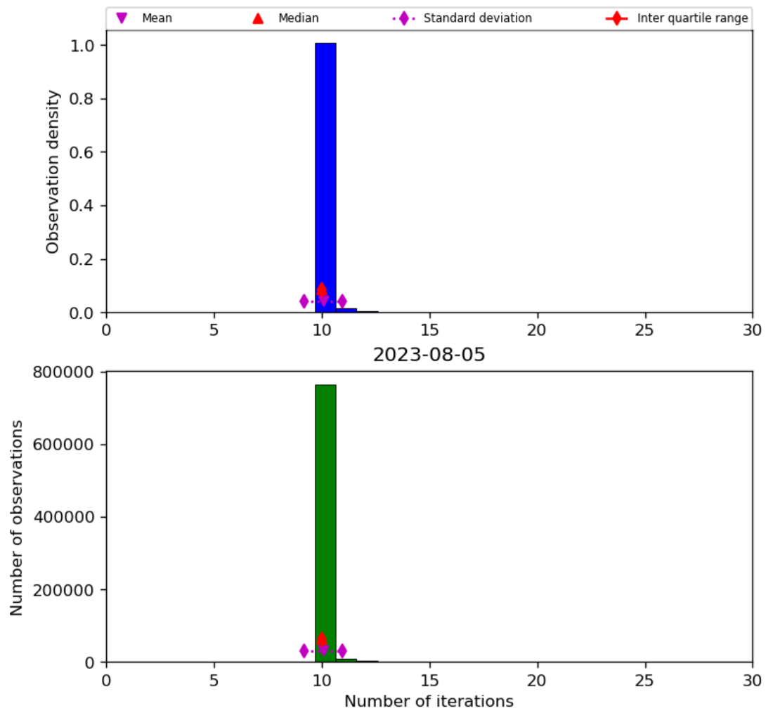
Figure 31: Histogram of “Number of iterations” for 2023-08-04 to 2023-08-06
