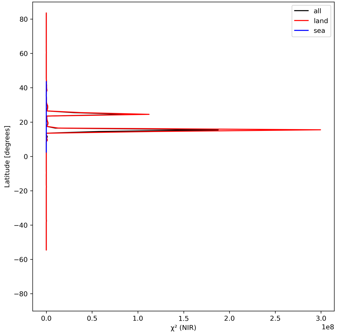
Figure 18: Zonal average of “ \chi^2 (NIR)” for 2023-08-04 to 2023-08-06.
