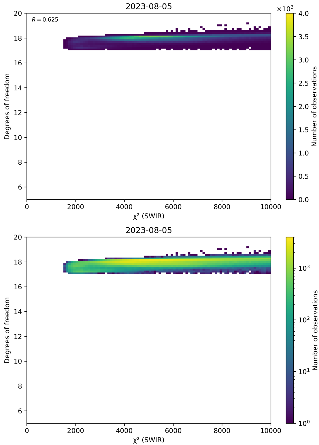
Figure 48: Scatter density plot of “ \chi^2 (SWIR)” against “Degrees of freedom” for 2023-08-04 to 2023-08-06.
