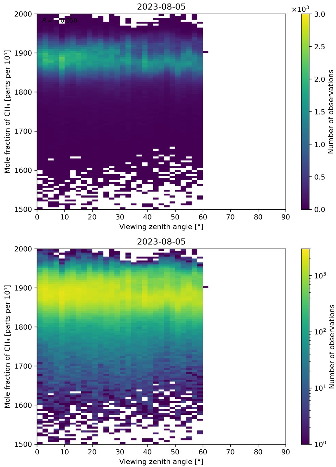
Figure 110: Scatter density plot of “Viewing zenith angle” against “Mole fraction of CH 4 ” for 2023-08-04 to 2023-08-06.
