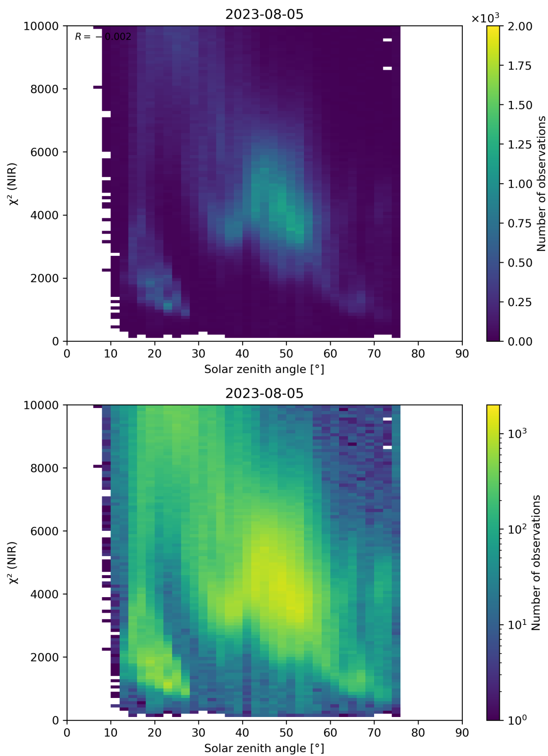
Figure 94: Scatter density plot of “Solar zenith angle” against “ \chi^2 (NIR)” for 2023-08-04 to 2023-08-06.
