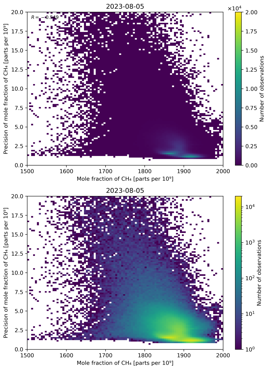
Figure 75: Scatter density plot of “Mole fraction of CH 4 ” against “Precision of mole fraction of CH 4 ” for 2023-08-04 to 2023-08-06.
