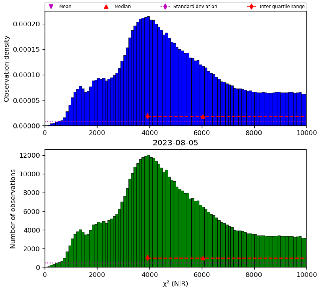
Figure 29: Histogram of " \chi^2 (NIR)" for 2023-08-04 to 2023-08-06
