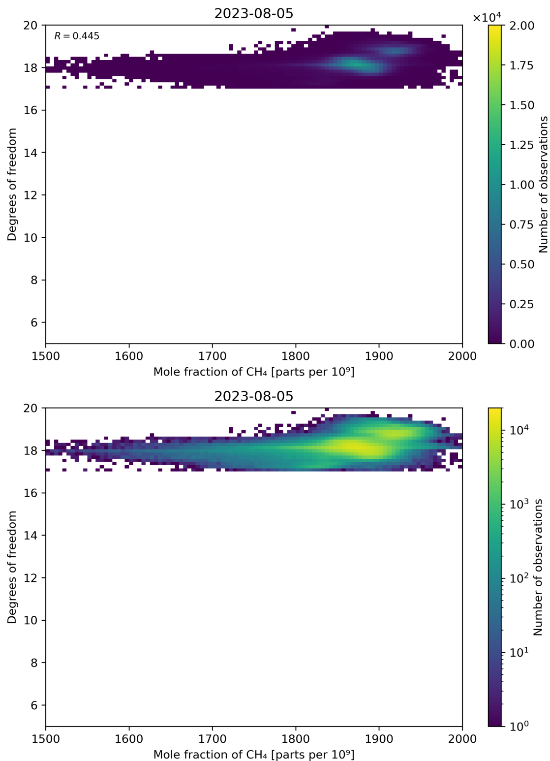
Figure 72: Scatter density plot of “Mole fraction of CH 4 ” against “Degrees of freedom” for 2023-08-04 to 2023-08-06.
