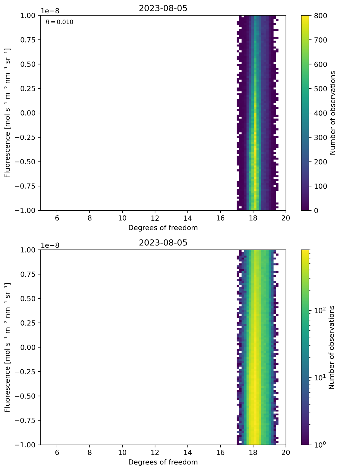
Figure 51: Scatter density plot of “Degrees of freedom” against “Fluorescence” for 2023-08-04 to 2023-08-06.
