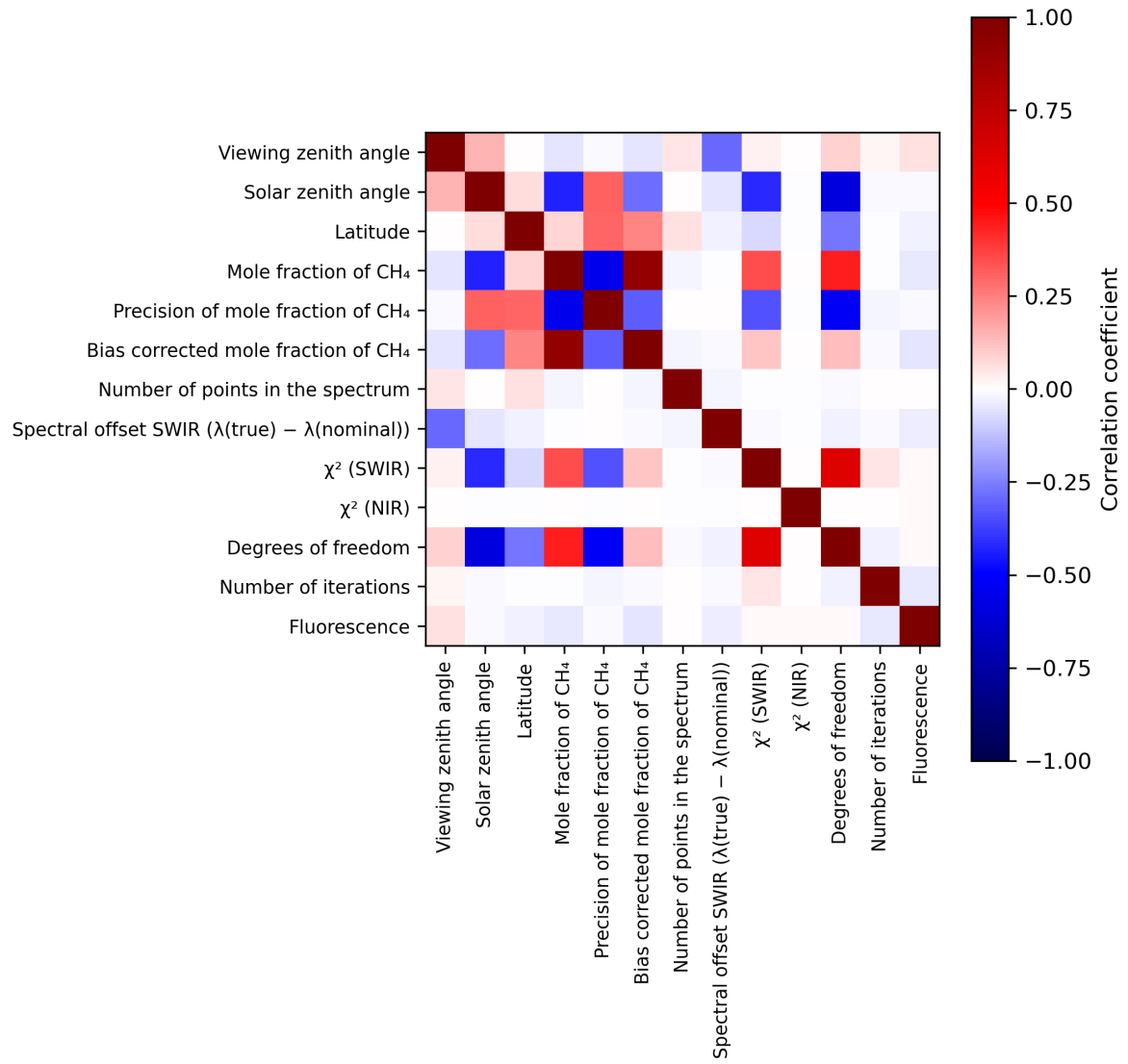
Figure 2: Map of correlation matrix for 2023-08-04 to 2023-08-06.
