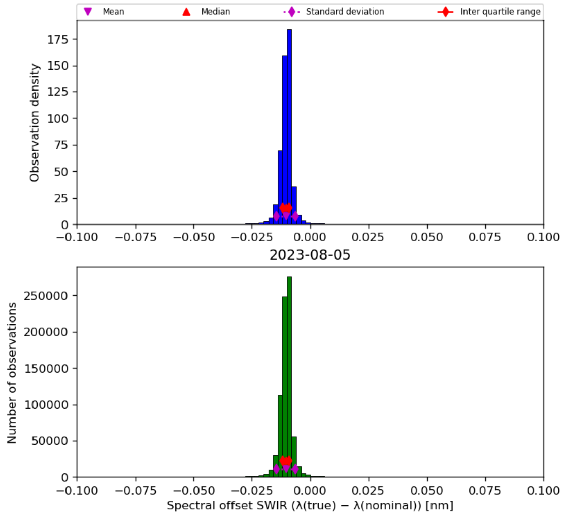
Figure 27: Histogram of “Spectral offset SWIR ( \lambda(\text{true}) - \lambda(\text{nominal}) )” for 2023-08-04 to 2023-08-06
