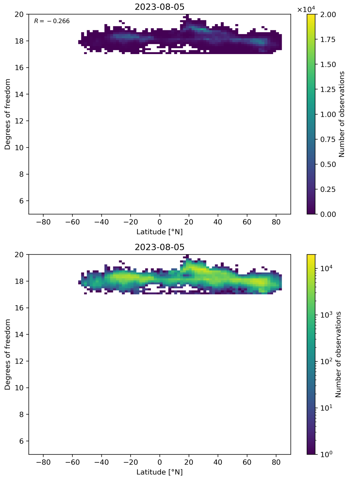
Figure 55: Scatter density plot of “Latitude” against “Degrees of freedom” for 2023-08-04 to 2023-08-06.
