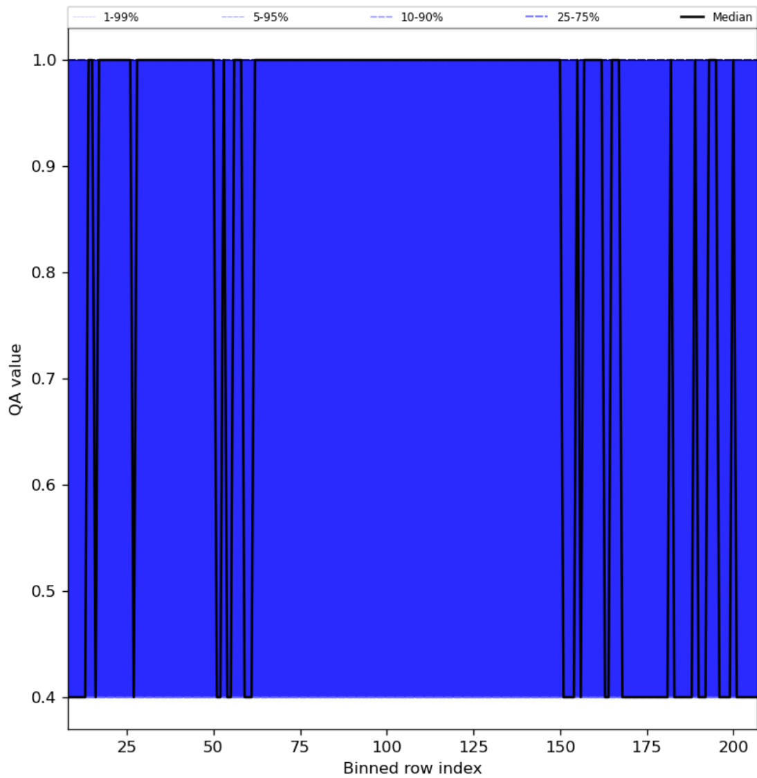
Figure 33: Along track statistics of “QA value” for 2023-08-04 to 2023-08-06
