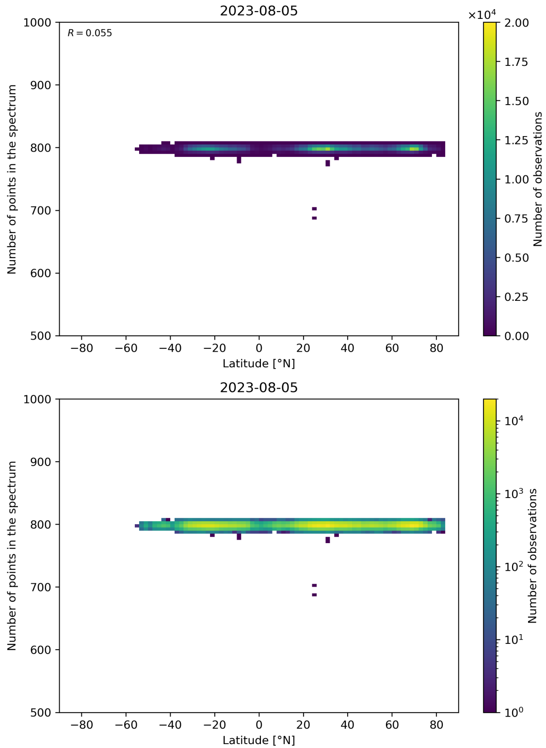
Figure 61: Scatter density plot of “Latitude” against “Number of points in the spectrum” for 2023-08-04 to 2023-08-06.
