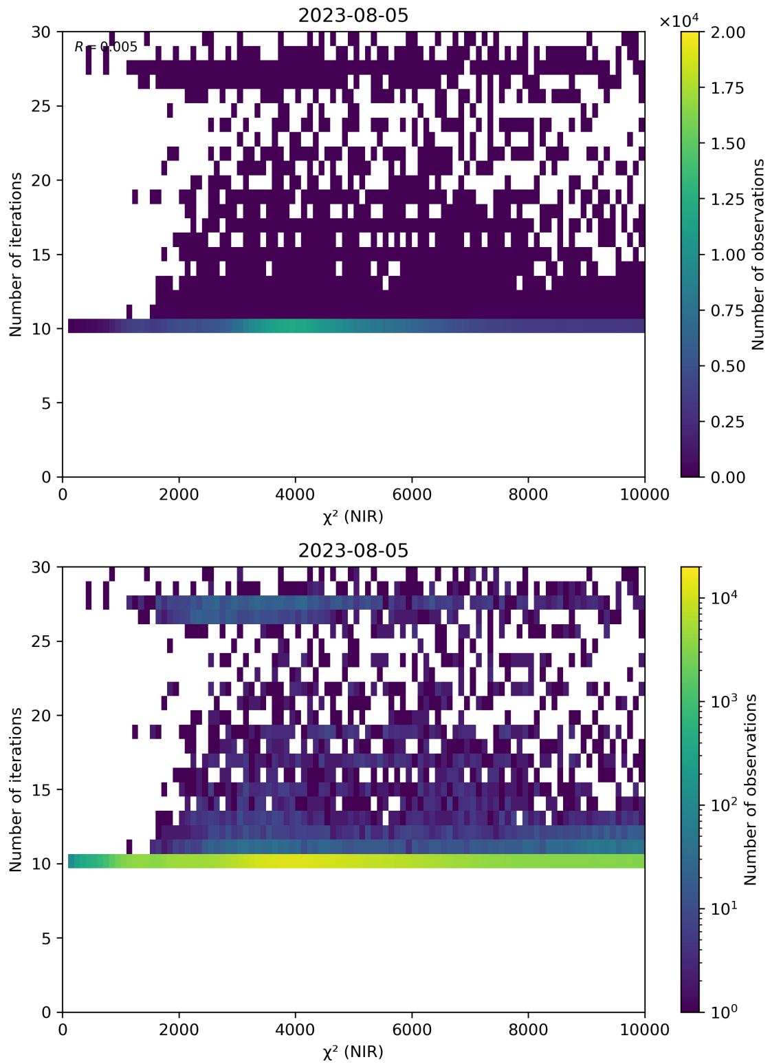
Figure 46: Scatter density plot of “ \chi^2 (NIR)” against “Number of iterations” for 2023-08-04 to 2023-08-06.
