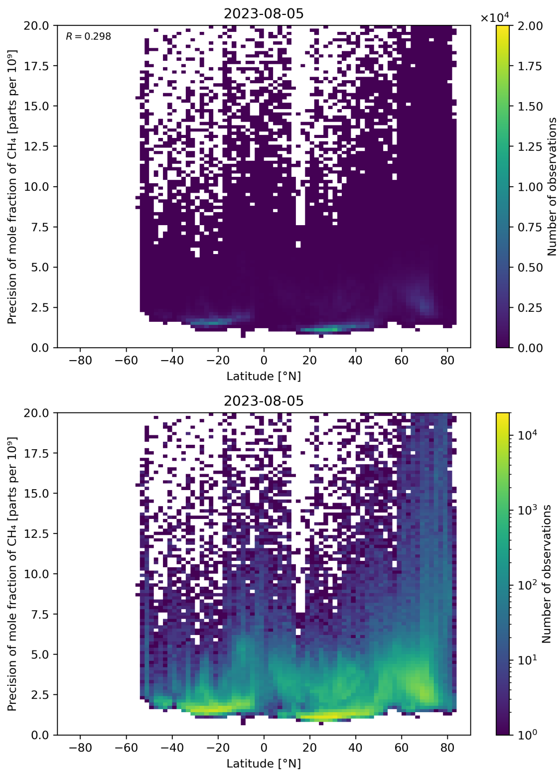
Figure 59: Scatter density plot of “Latitude” against “Precision of mole fraction of CH 4 ” for 2023-08-04 to 2023-08-06.
