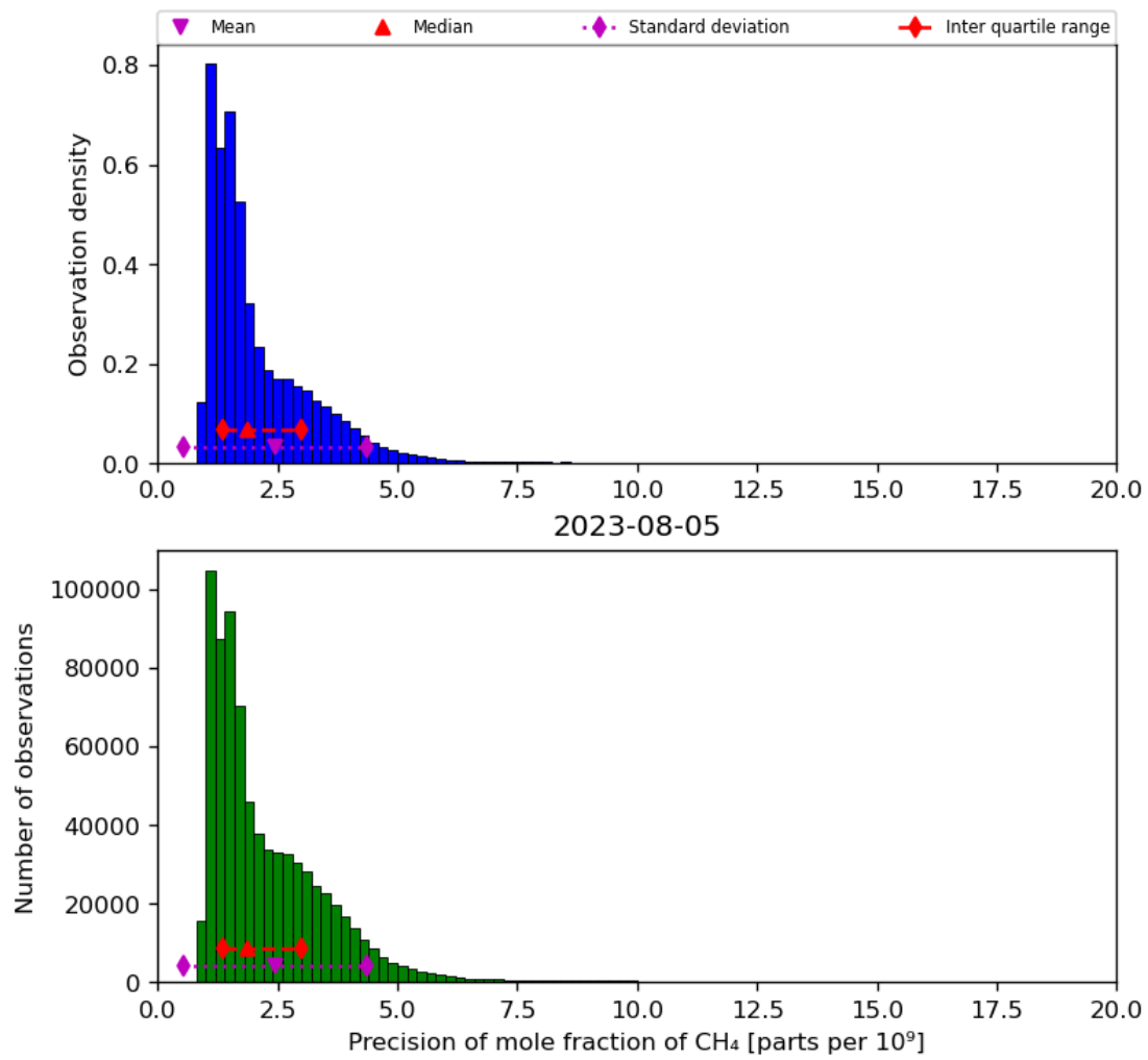
Figure 24: Histogram of “Precision of mole fraction of CH 4 ” for 2023-08-04 to 2023-08-06
