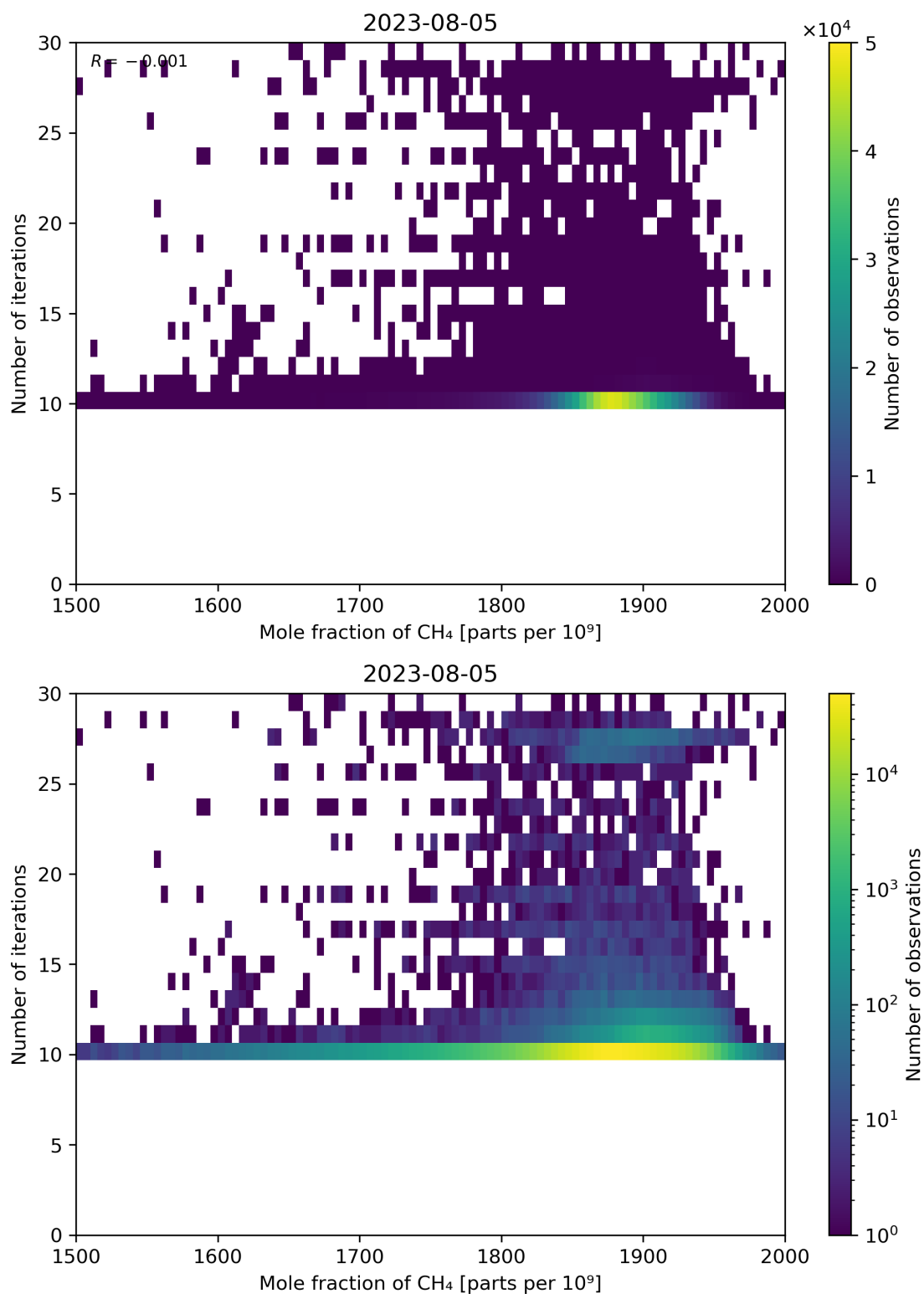
Figure 76: Scatter density plot of “Mole fraction of CH 4 ” against “Number of iterations” for 2023-08-04 to 2023-08-06.
