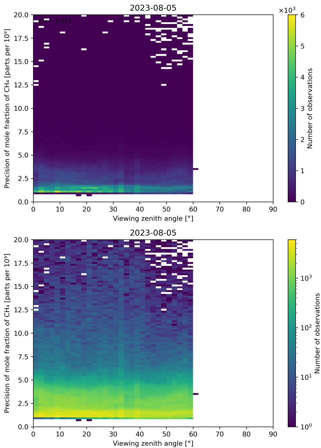
Figure 112: Scatter density plot of “Viewing zenith angle” against “Precision of mole fraction of CH 4 ” for 2023-08-04 to 2023-08-06.
