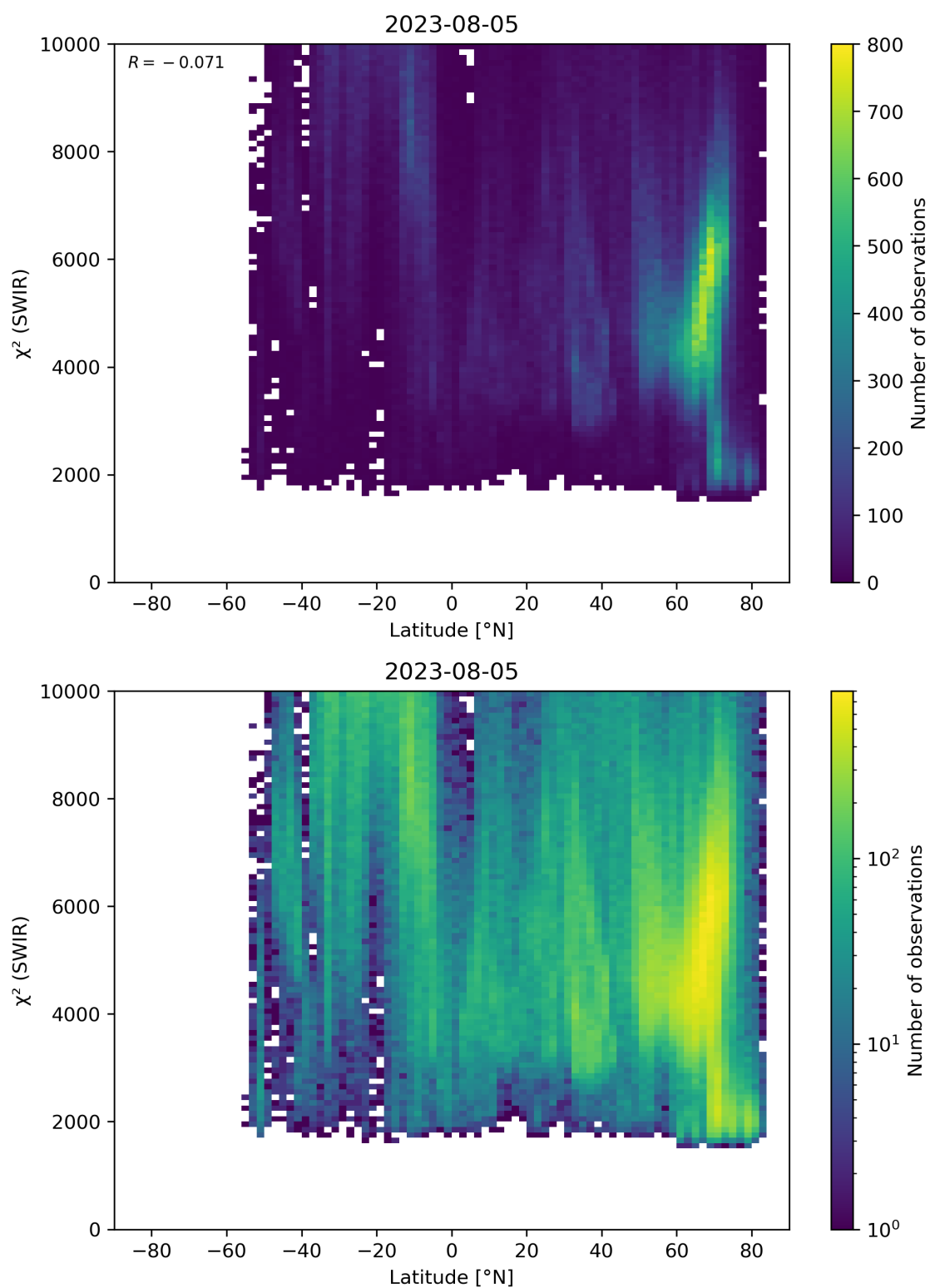
Figure 54: Scatter density plot of “Latitude” against “ \chi^2 (SWIR)” for 2023-08-04 to 2023-08-06.
