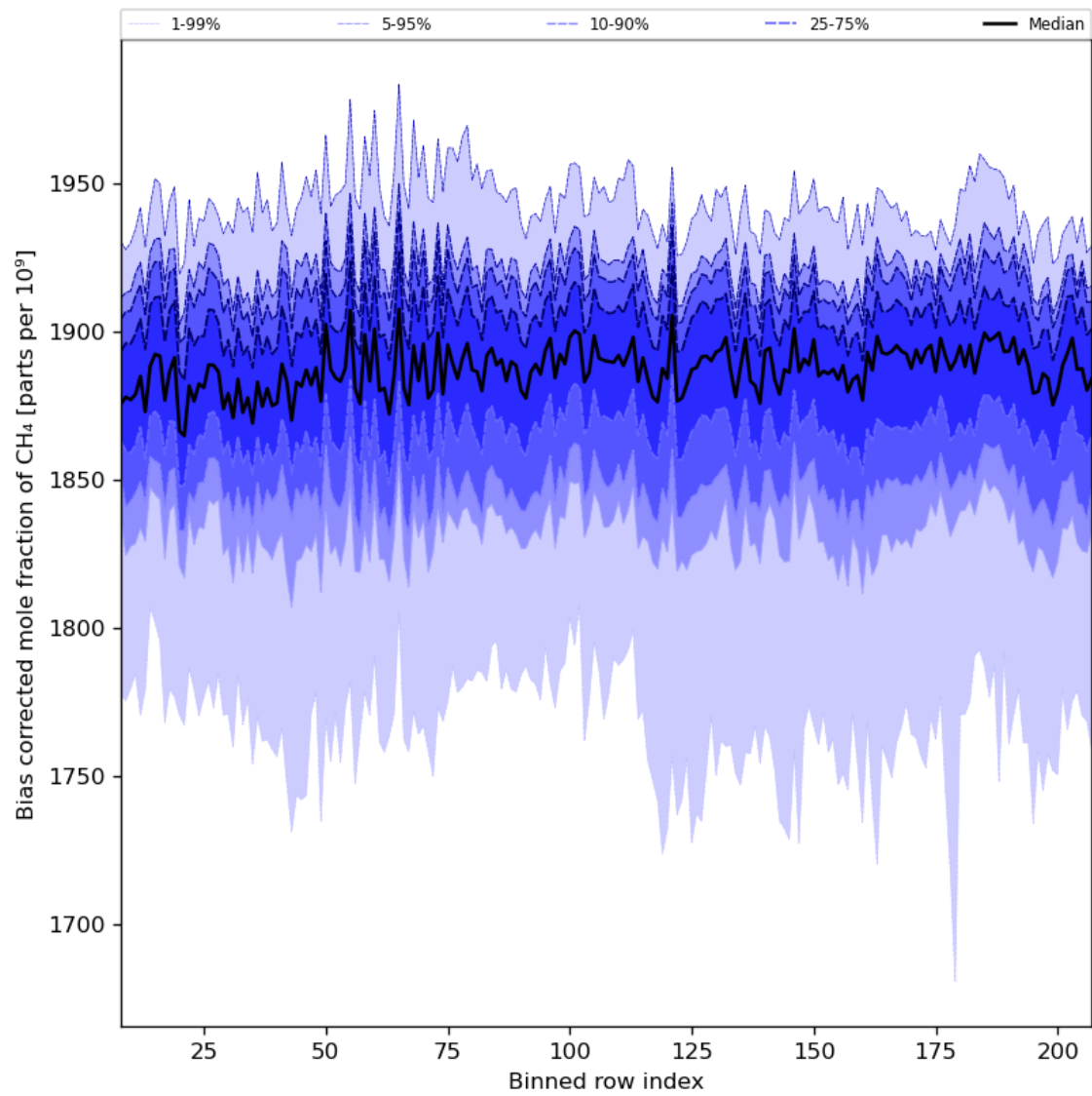
Figure 36: Along track statistics of “Bias corrected mole fraction of CH 4 ” for 2023-08-04 to 2023-08-06
