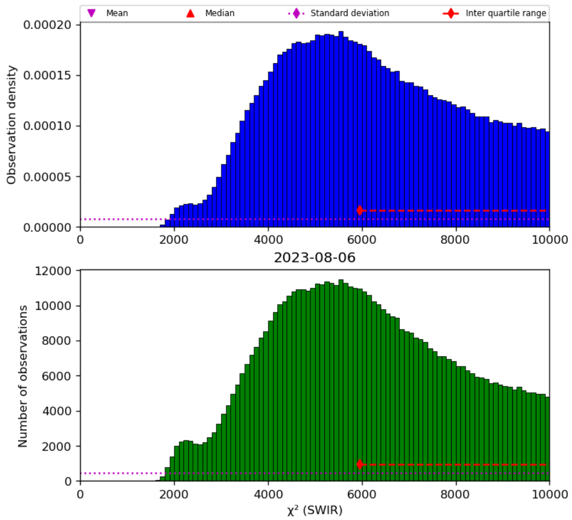
Figure 28: Histogram of “ \chi^2 (SWIR)” for 2023-08-05 to 2023-08-07
