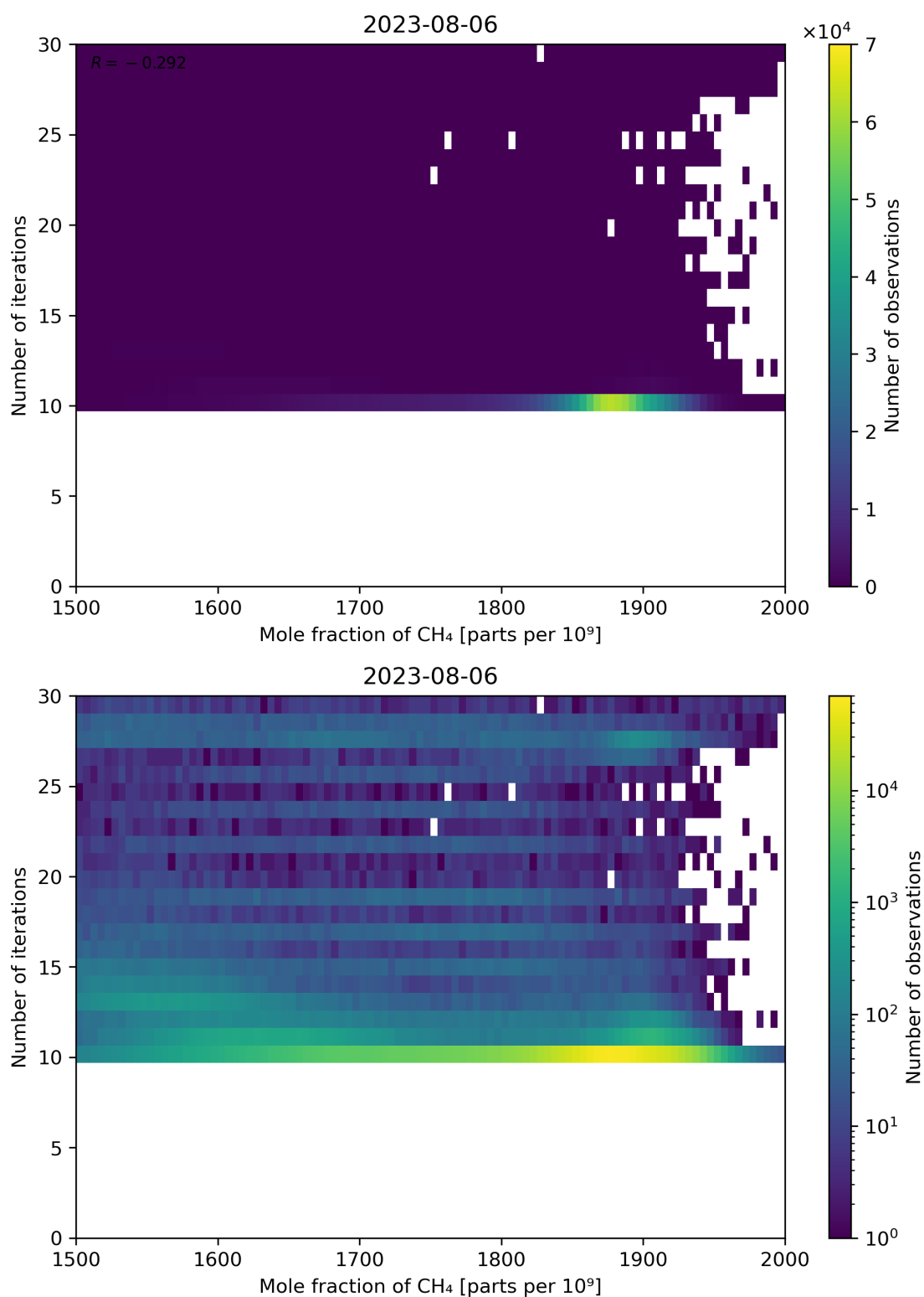
Figure 76: Scatter density plot of “Mole fraction of CH 4 ” against “Number of iterations” for 2023-08-05 to 2023-08-07.
