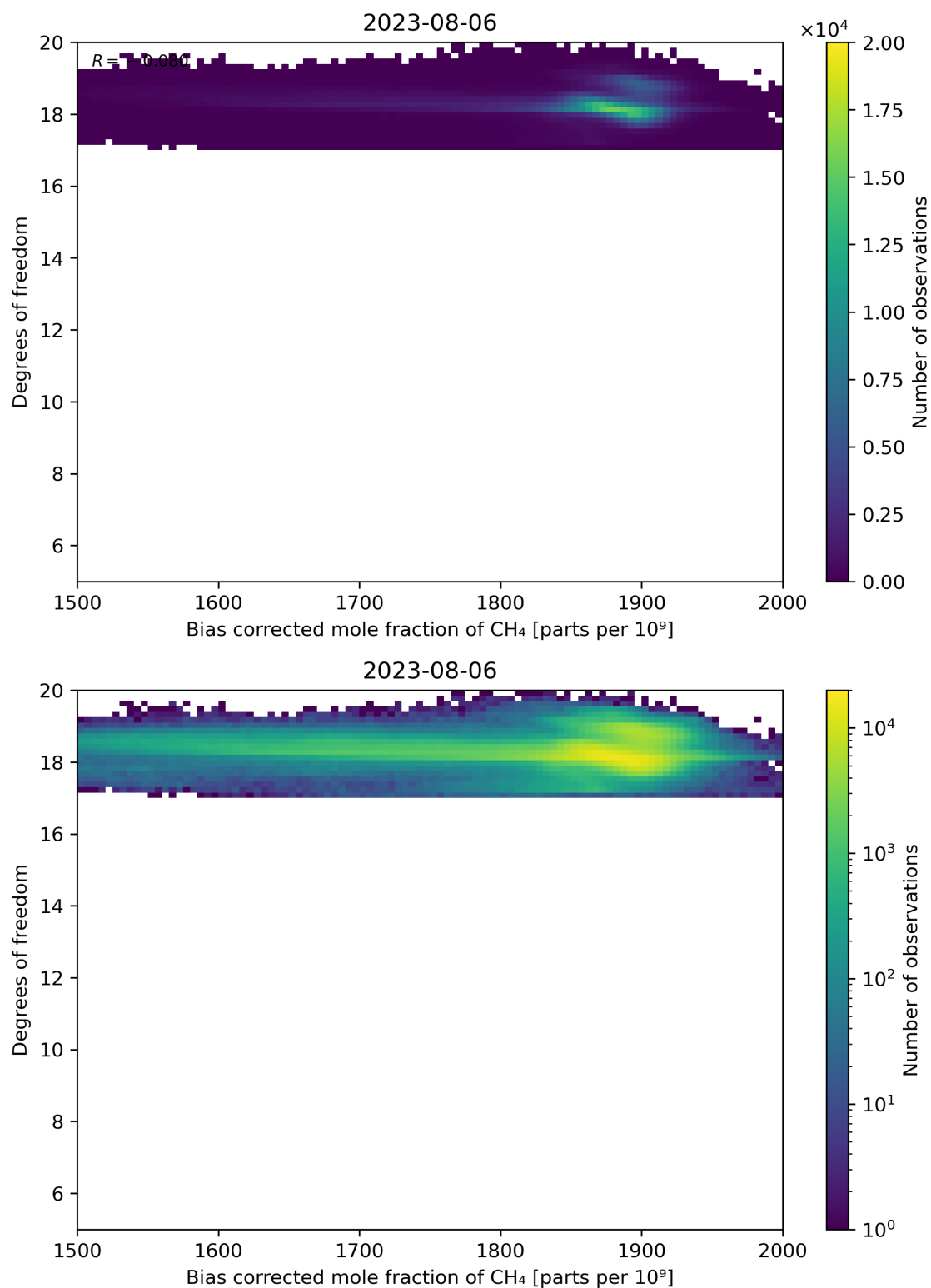
Figure 65: Scatter density plot of “Bias corrected mole fraction of CH 4 ” against “Degrees of freedom” for 2023-08-05 to 2023-08-07.
