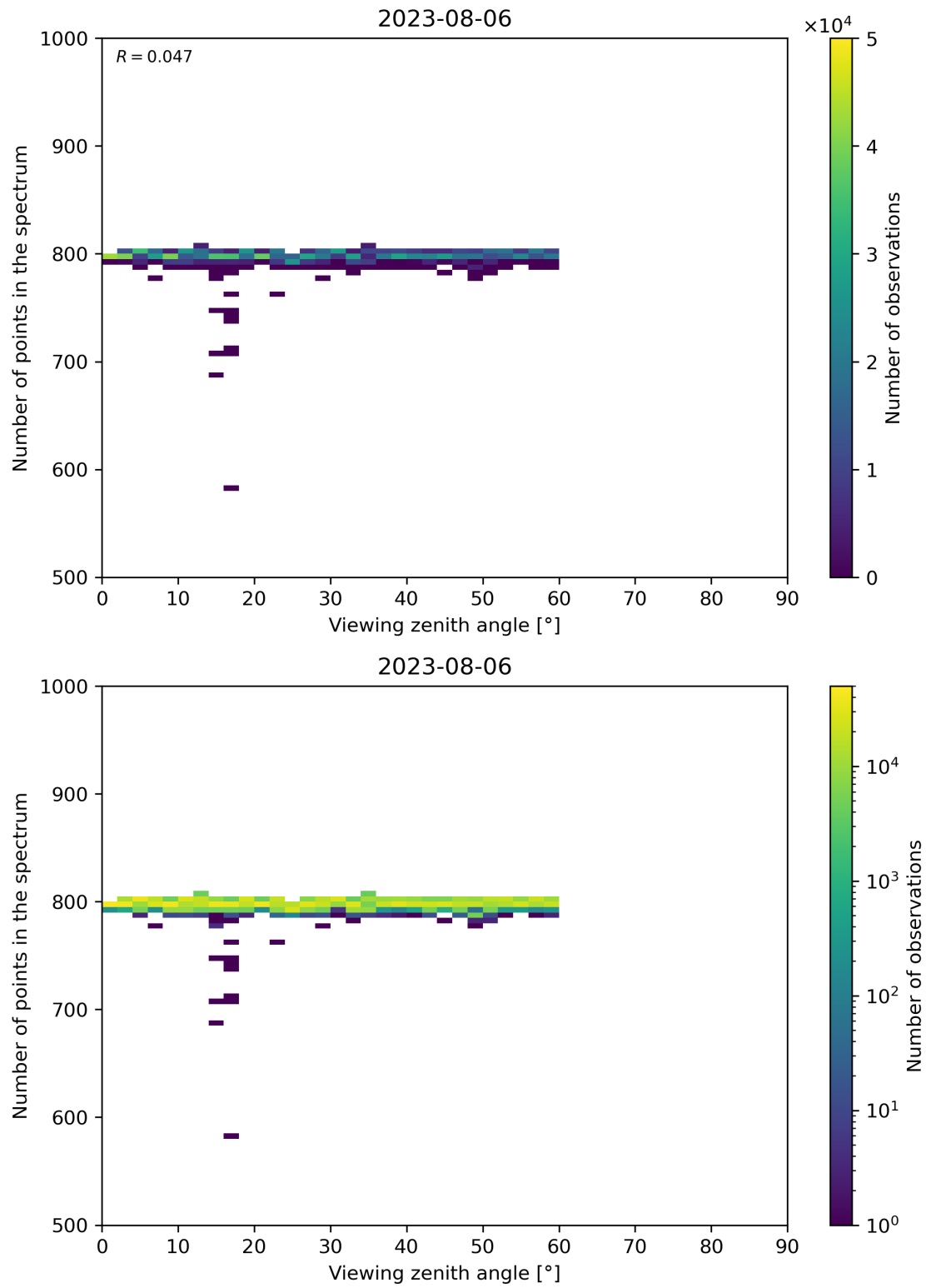
Figure 114: Scatter density plot of “Viewing zenith angle” against “Number of points in the spectrum” for 2023-08-05 to 2023-08-07.
