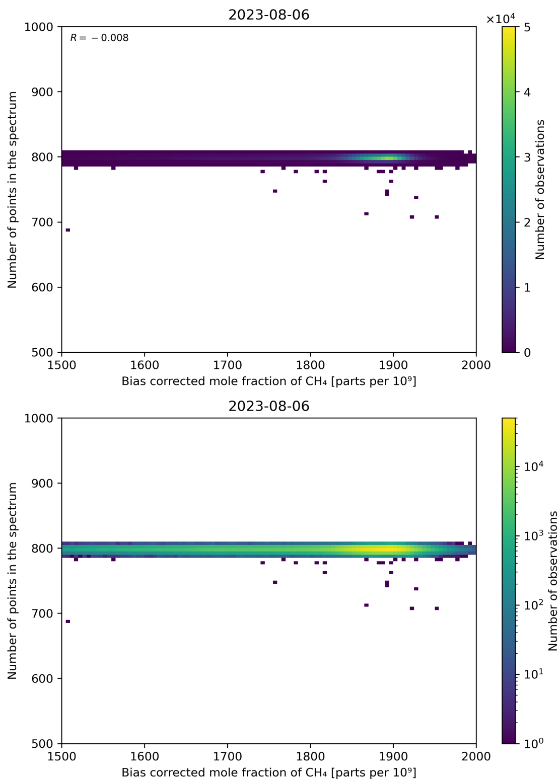
Figure 68: Scatter density plot of “Bias corrected mole fraction of CH 4 ” against “Number of points in the spectrum” for 2023-08-05 to 2023-08-07.
