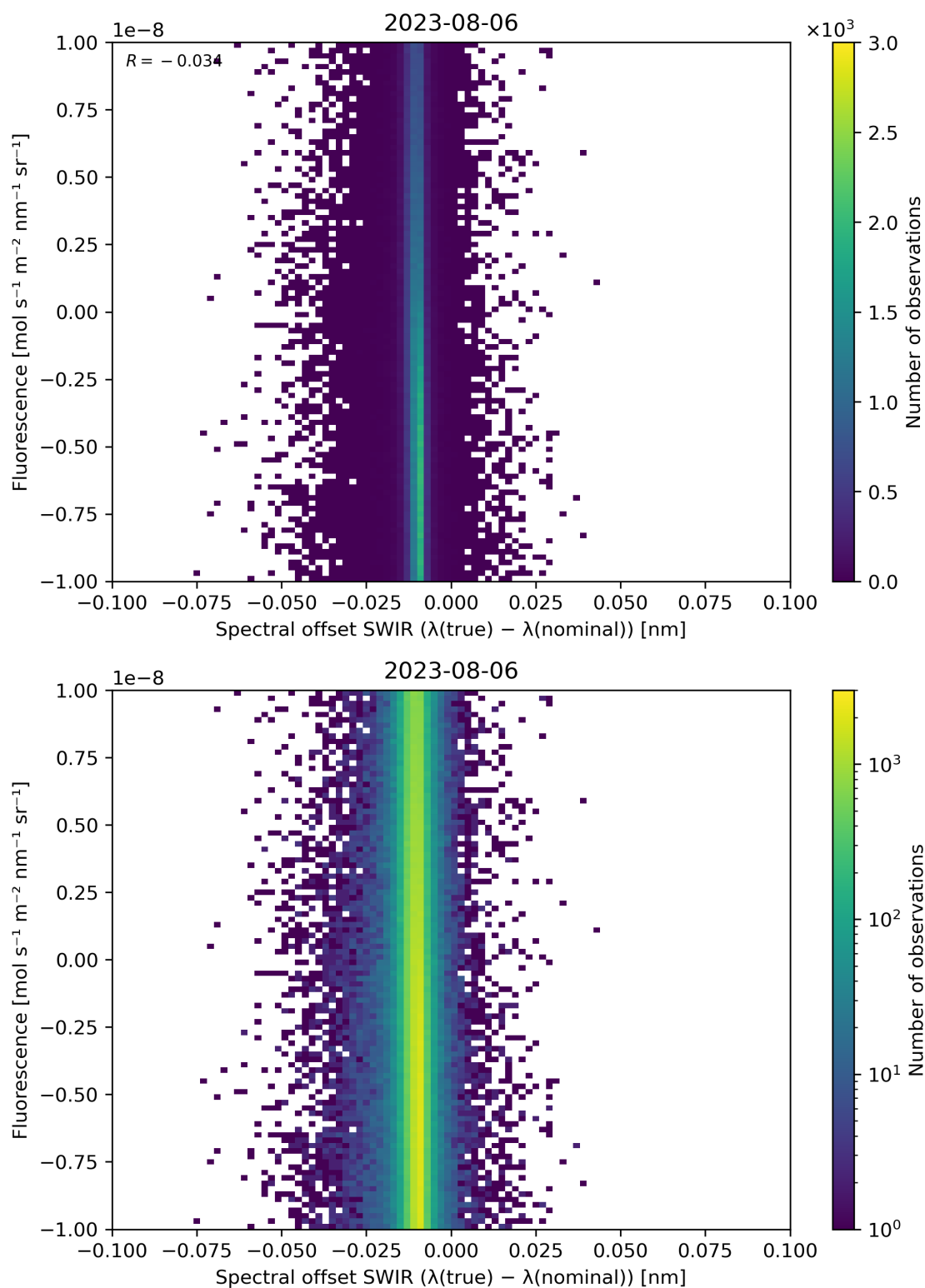
Figure 120: Scatter density plot of “Spectral offset SWIR ( \lambda(\text{true}) - \lambda(\text{nominal}) )” against “Fluorescence” for 2023-08-05 to 2023-08-07.
