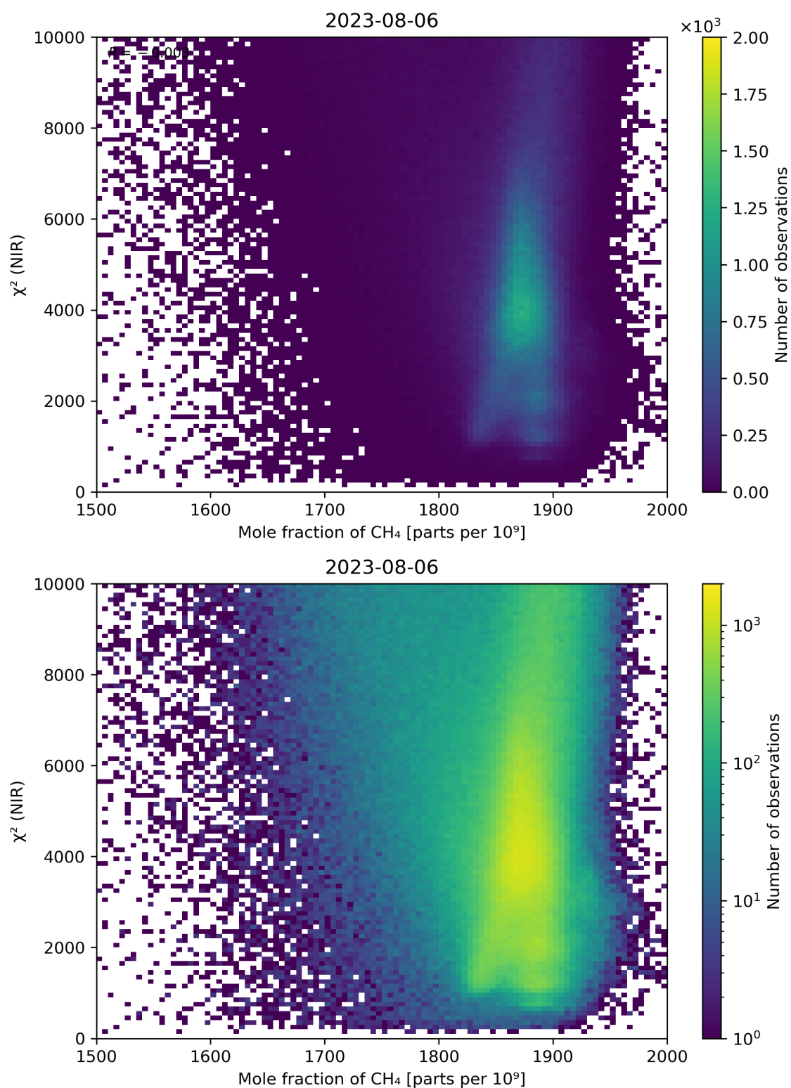
Figure 70: Scatter density plot of “Mole fraction of CH 4 ” against “ \chi^2 (NIR)” for 2023-08-05 to 2023-08-07.
