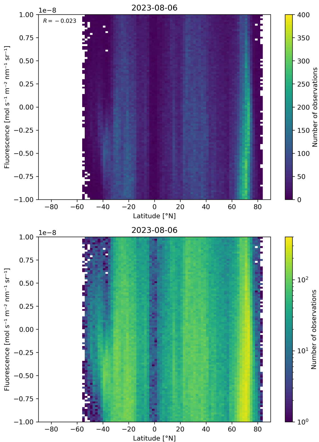
Figure 56: Scatter density plot of “Latitude” against “Fluorescence” for 2023-08-05 to 2023-08-07.
