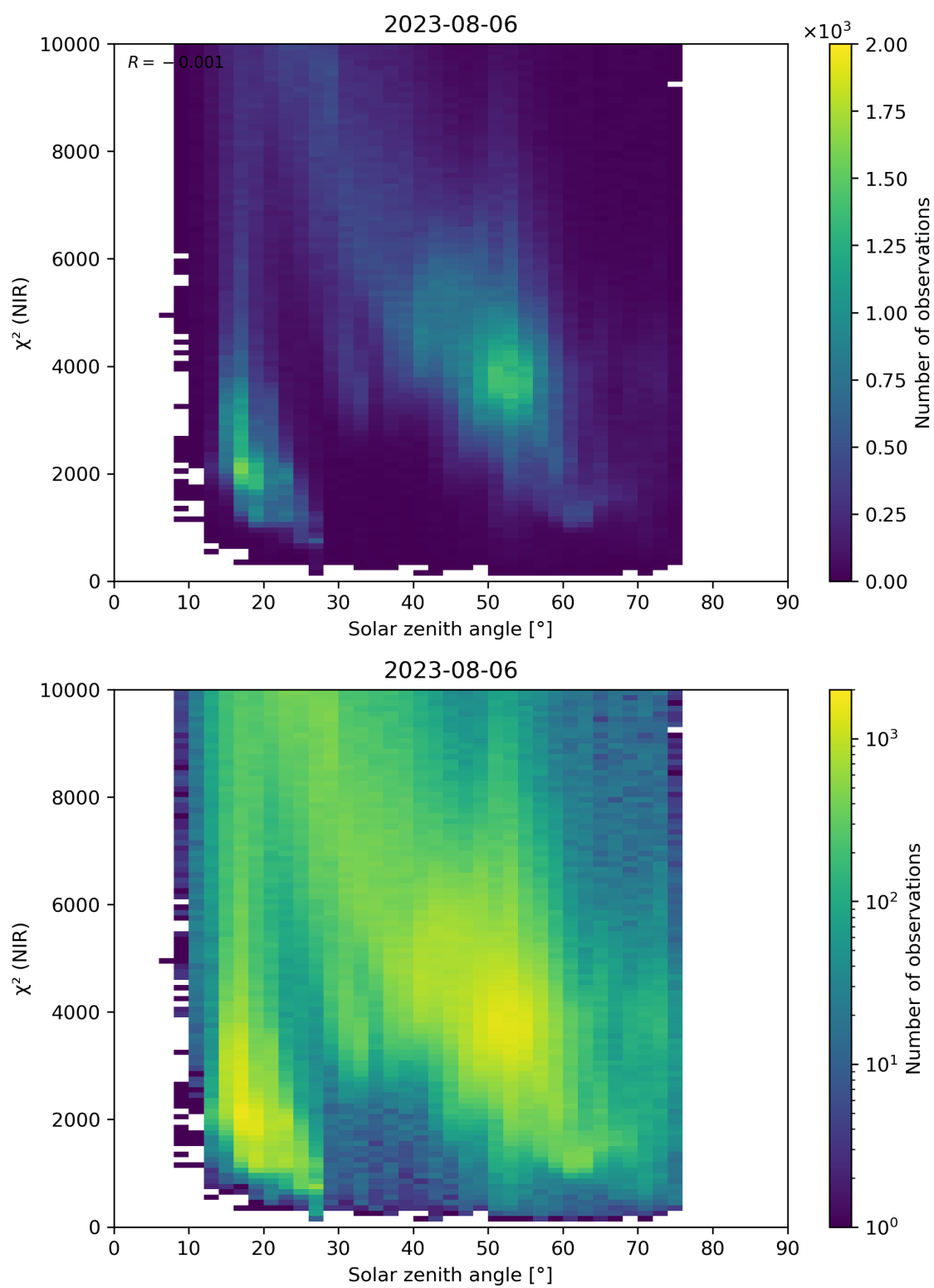
Figure 94: Scatter density plot of “Solar zenith angle” against “ \chi^2 (NIR)” for 2023-08-05 to 2023-08-07.
