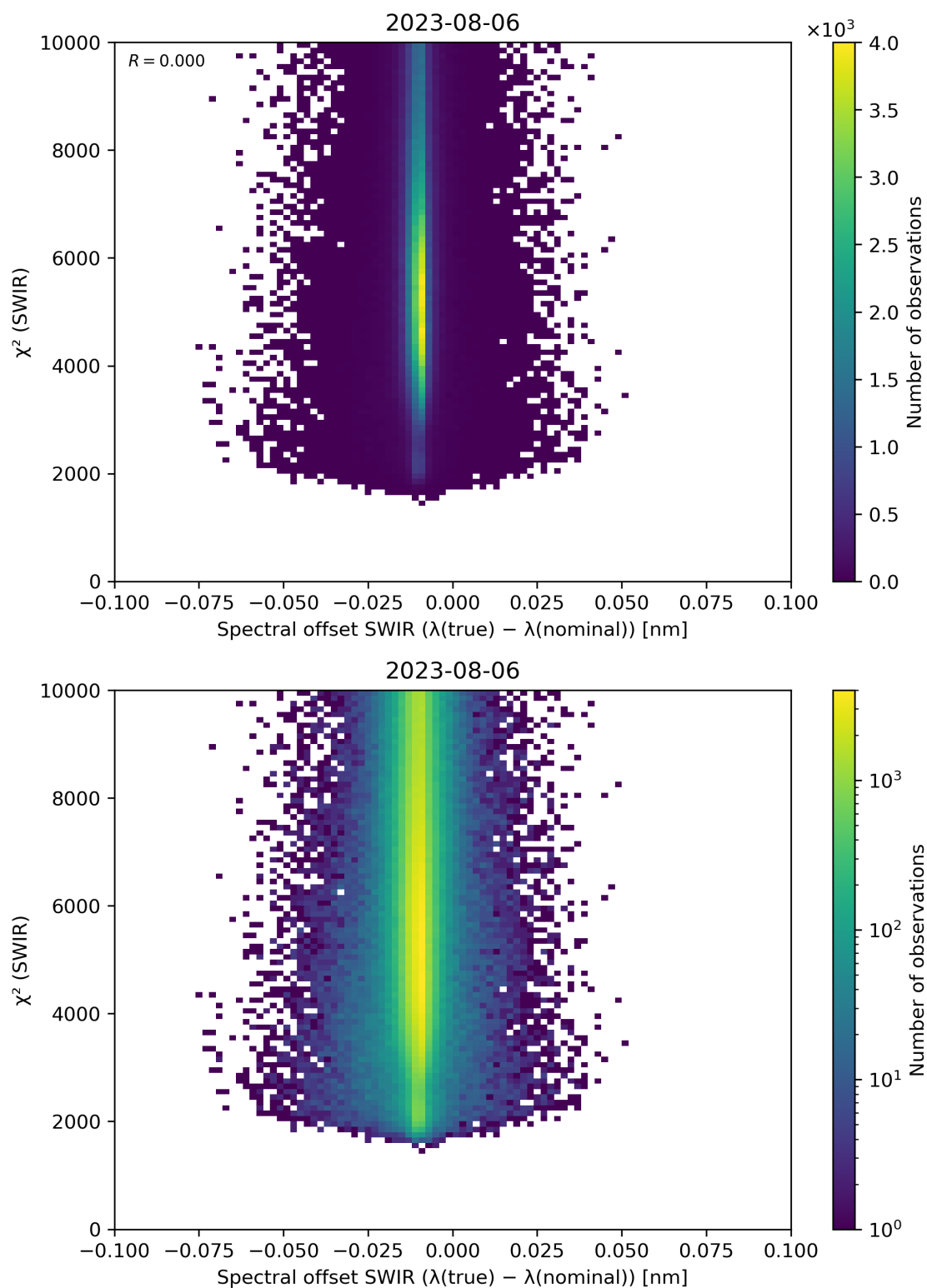
Figure 118: Scatter density plot of “Spectral offset SWIR ( \lambda(\text{true}) - \lambda(\text{nominal}) )” against “ \chi^2 (SWIR)” for 2023-08-05 to 2023-08-07.
