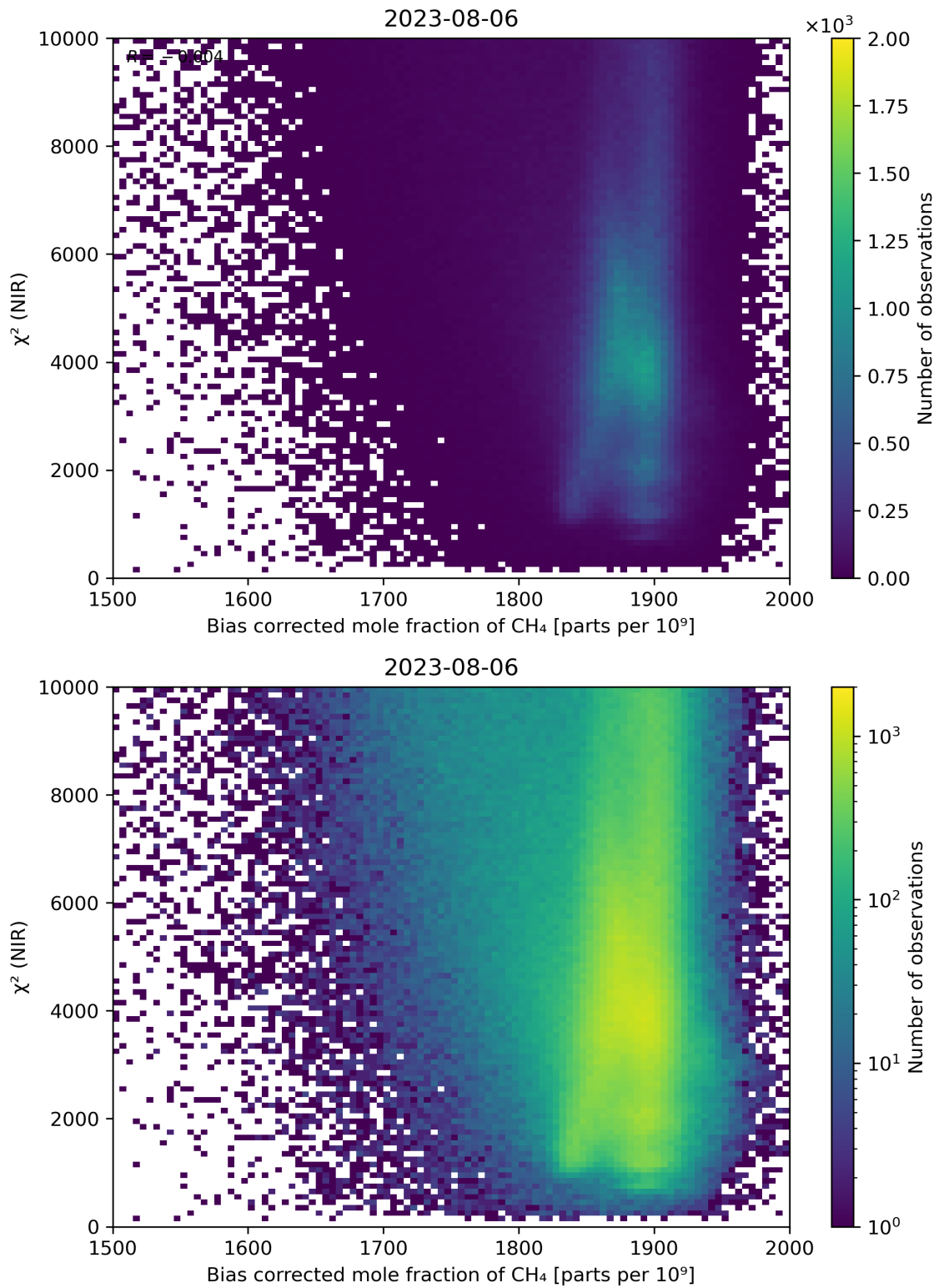
Figure 63: Scatter density plot of “Bias corrected mole fraction of CH 4 ” against “ \chi^2 (NIR)” for 2023-08-05 to 2023-08-07.
