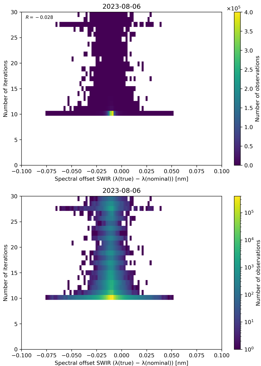
Figure 121: Scatter density plot of “Spectral offset SWIR ( \lambda(\text{true}) - \lambda(\text{nominal}) )” against “Number of iterations” for 2023-08-05 to 2023-08-07.
