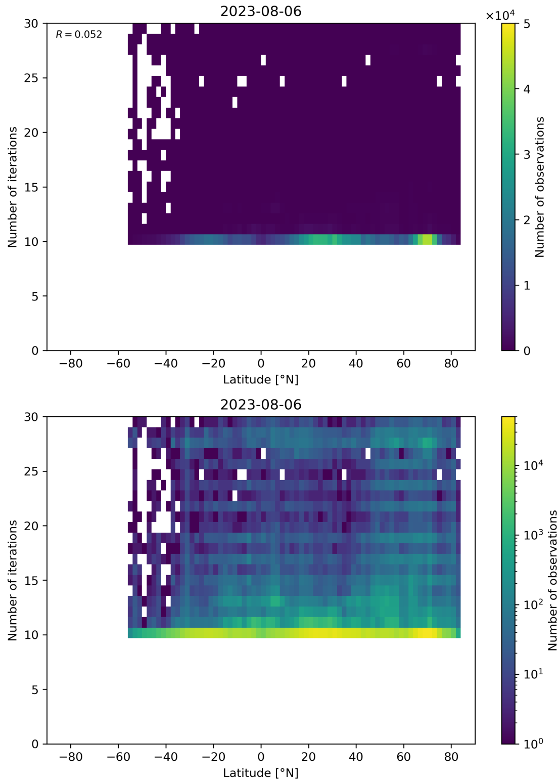
Figure 60: Scatter density plot of “Latitude” against “Number of iterations” for 2023-08-05 to 2023-08-07.
