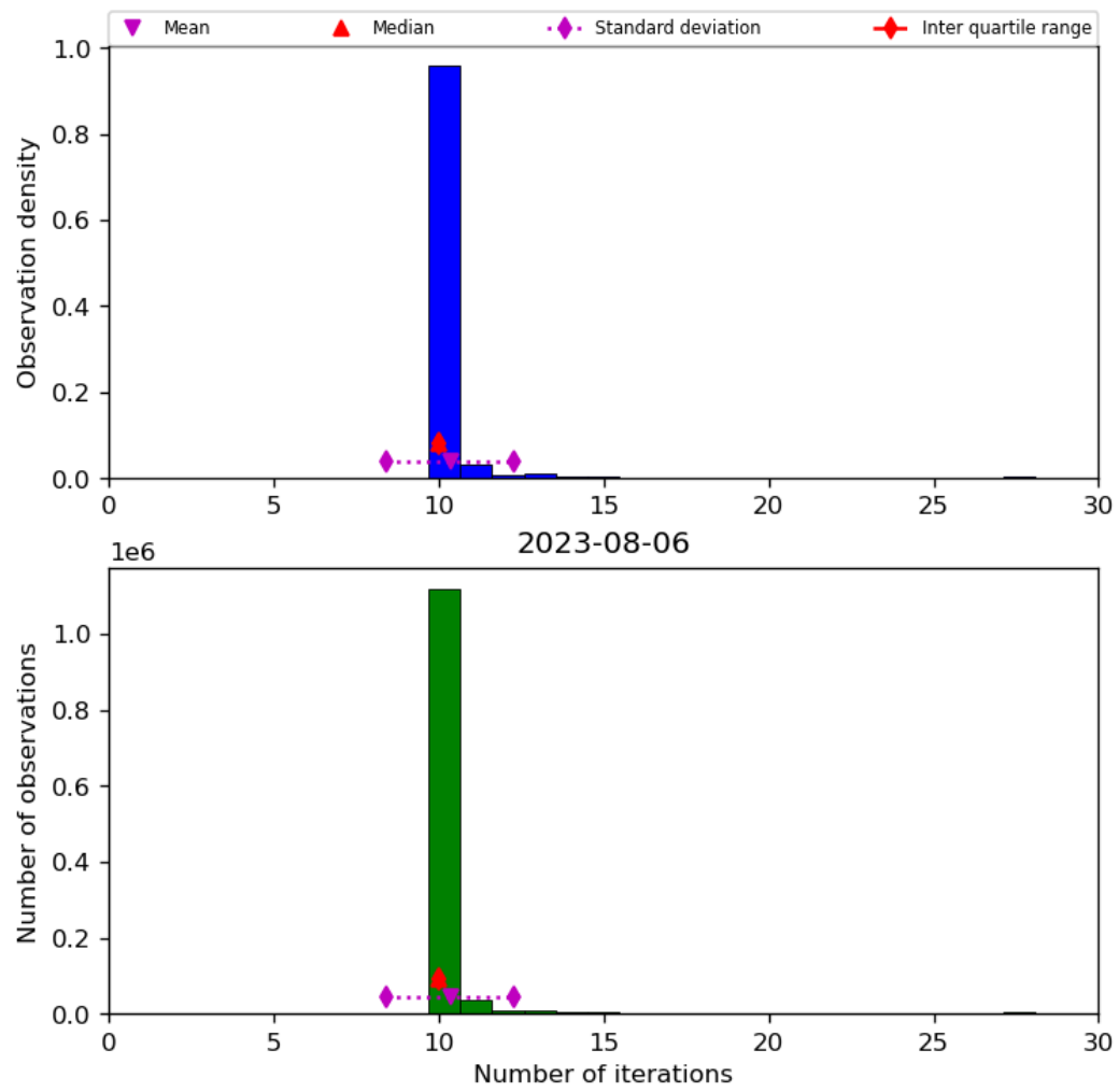
Figure 31: Histogram of “Number of iterations” for 2023-08-05 to 2023-08-07
