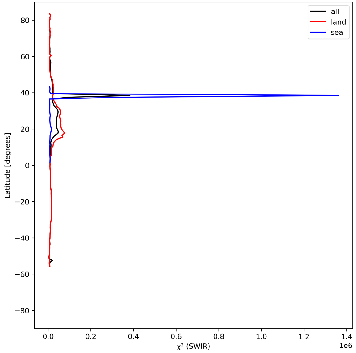
Figure 17: Zonal average of “ \chi^2 (SWIR)” for 2023-08-05 to 2023-08-07.
