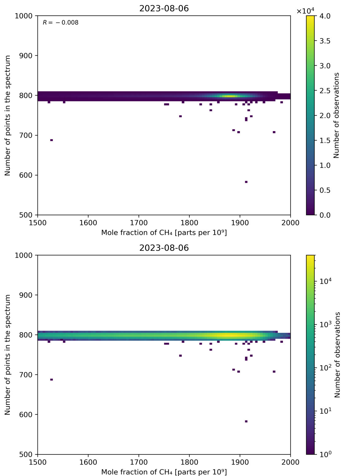
Figure 77: Scatter density plot of “Mole fraction of CH 4 ” against “Number of points in the spectrum” for 2023-08-05 to 2023-08-07.
