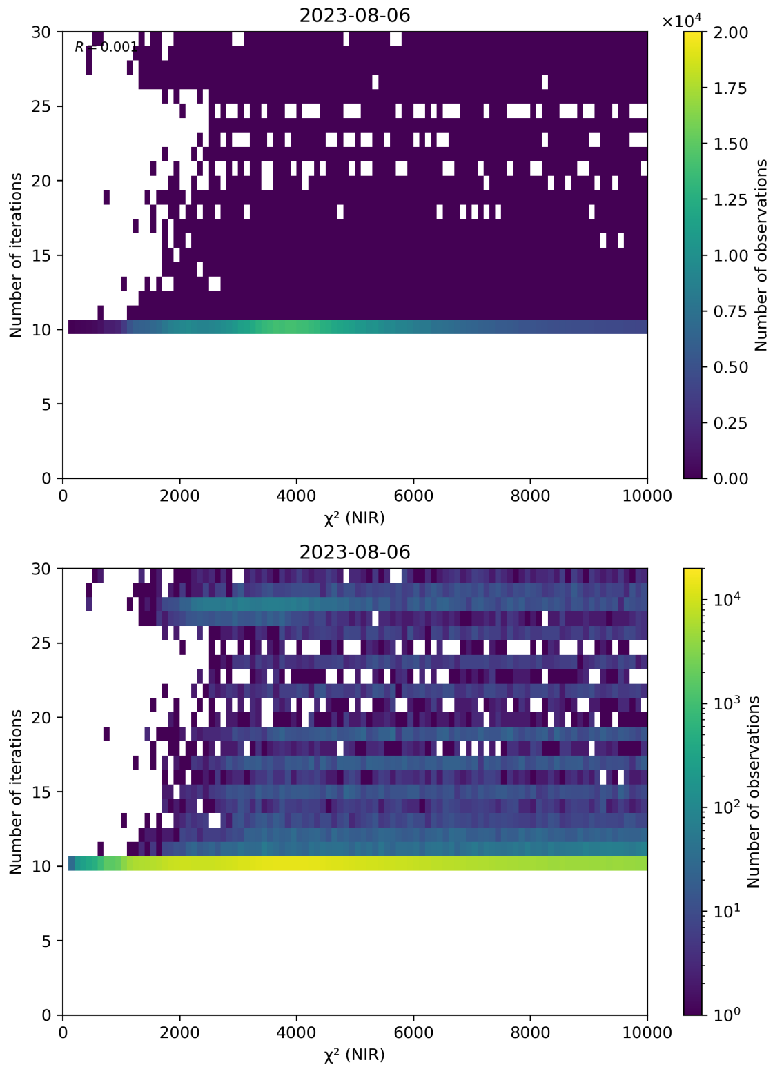
Figure 46: Scatter density plot of “ \chi^2 (NIR)” against “Number of iterations” for 2023-08-05 to 2023-08-07.
