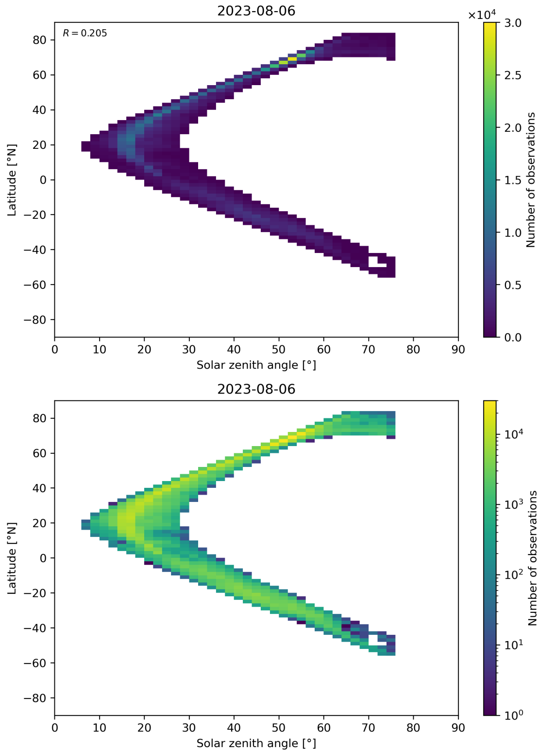
Figure 98: Scatter density plot of “Solar zenith angle” against “Latitude” for 2023-08-05 to 2023-08-07.
