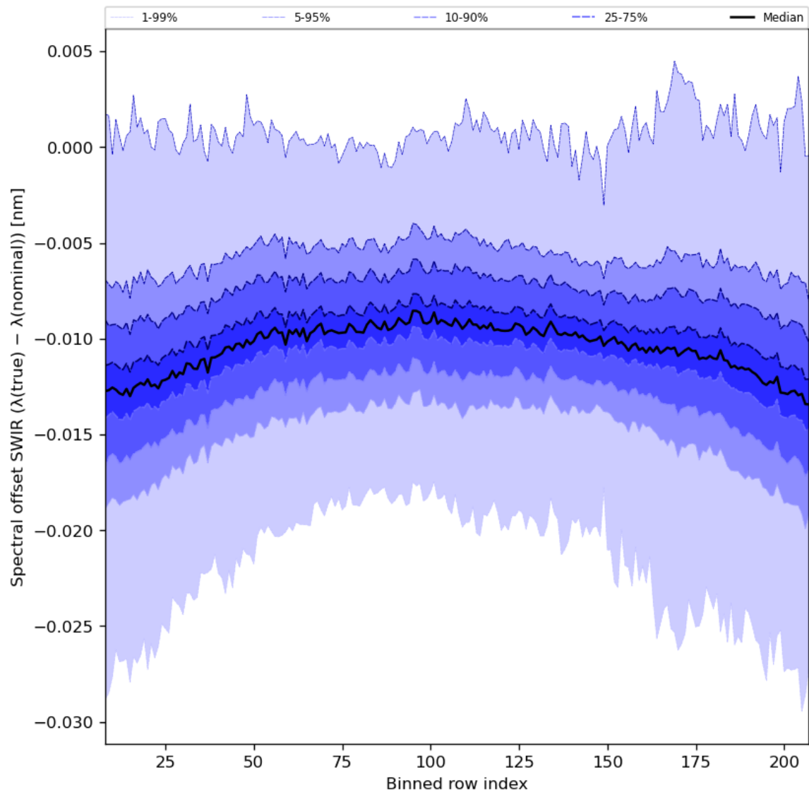
Figure 38: Along track statistics of "Spectral offset SWIR ( \lambda(\text{true}) - \lambda(\text{nominal}) )" for 2023-08-05 to 2023-08-07
