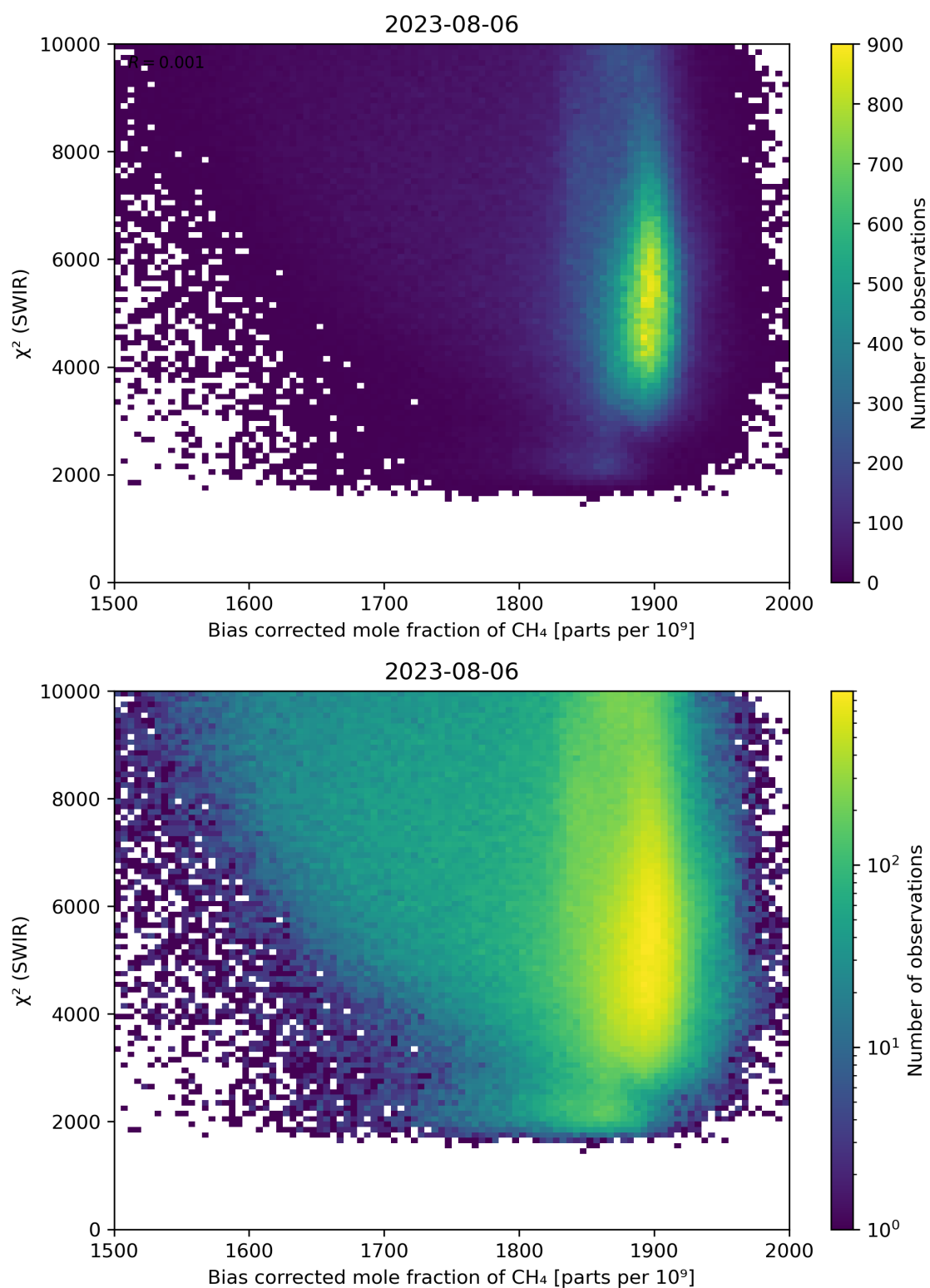
Figure 64: Scatter density plot of “Bias corrected mole fraction of CH 4 ” against “ \chi^2 (SWIR)” for 2023-08-05 to 2023-08-07.
