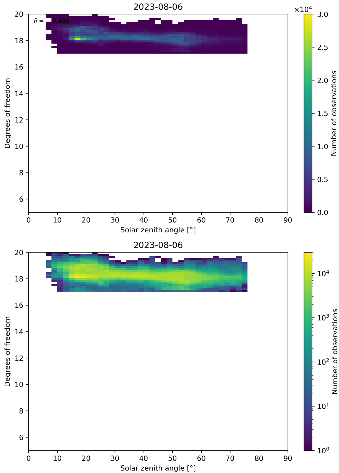
Figure 96: Scatter density plot of “Solar zenith angle” against “Degrees of freedom” for 2023-08-05 to 2023-08-07.
