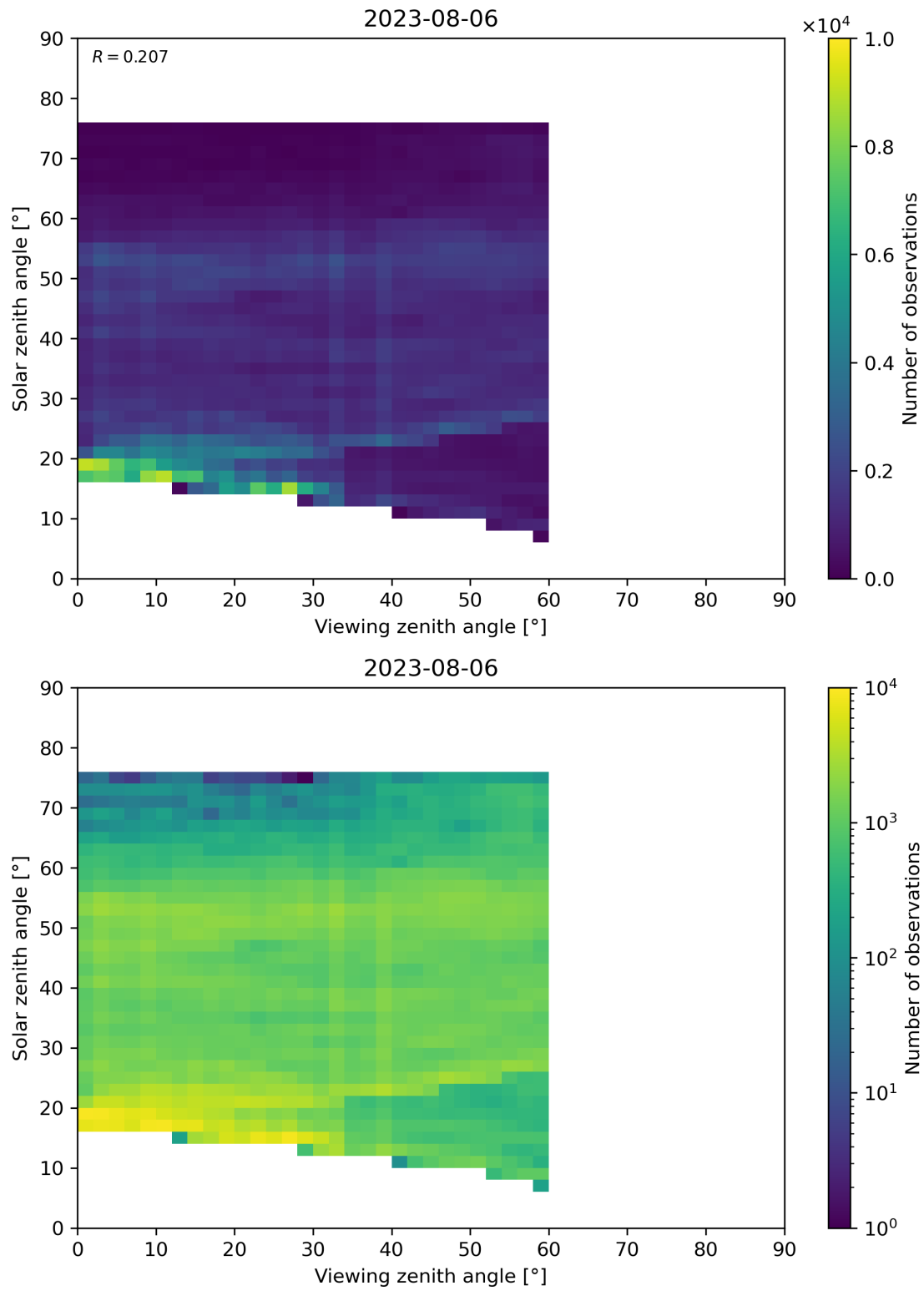
Figure 115: Scatter density plot of “Viewing zenith angle” against “Solar zenith angle” for 2023-08-05 to 2023-08-07.
