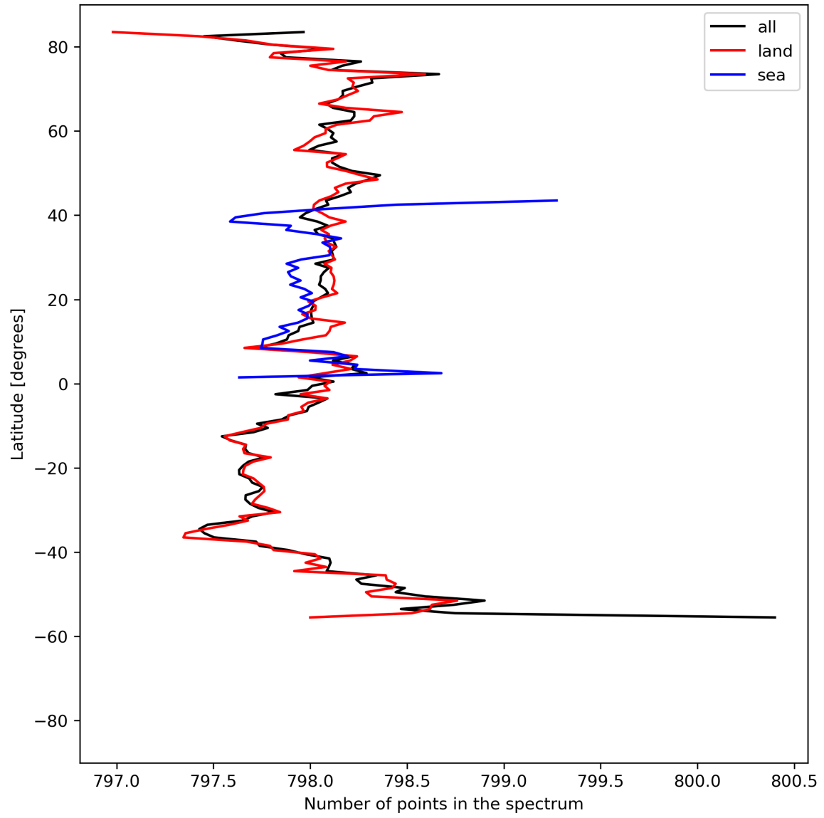
Figure 15: Zonal average of “Number of points in the spectrum” for 2023-08-05 to 2023-08-07.
