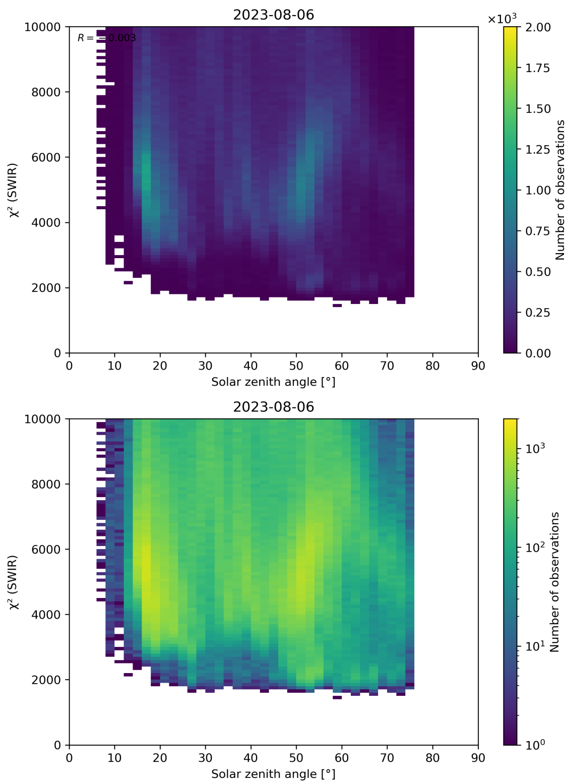
Figure 95: Scatter density plot of “Solar zenith angle” against “ \chi^2 (SWIR)” for 2023-08-05 to 2023-08-07.
