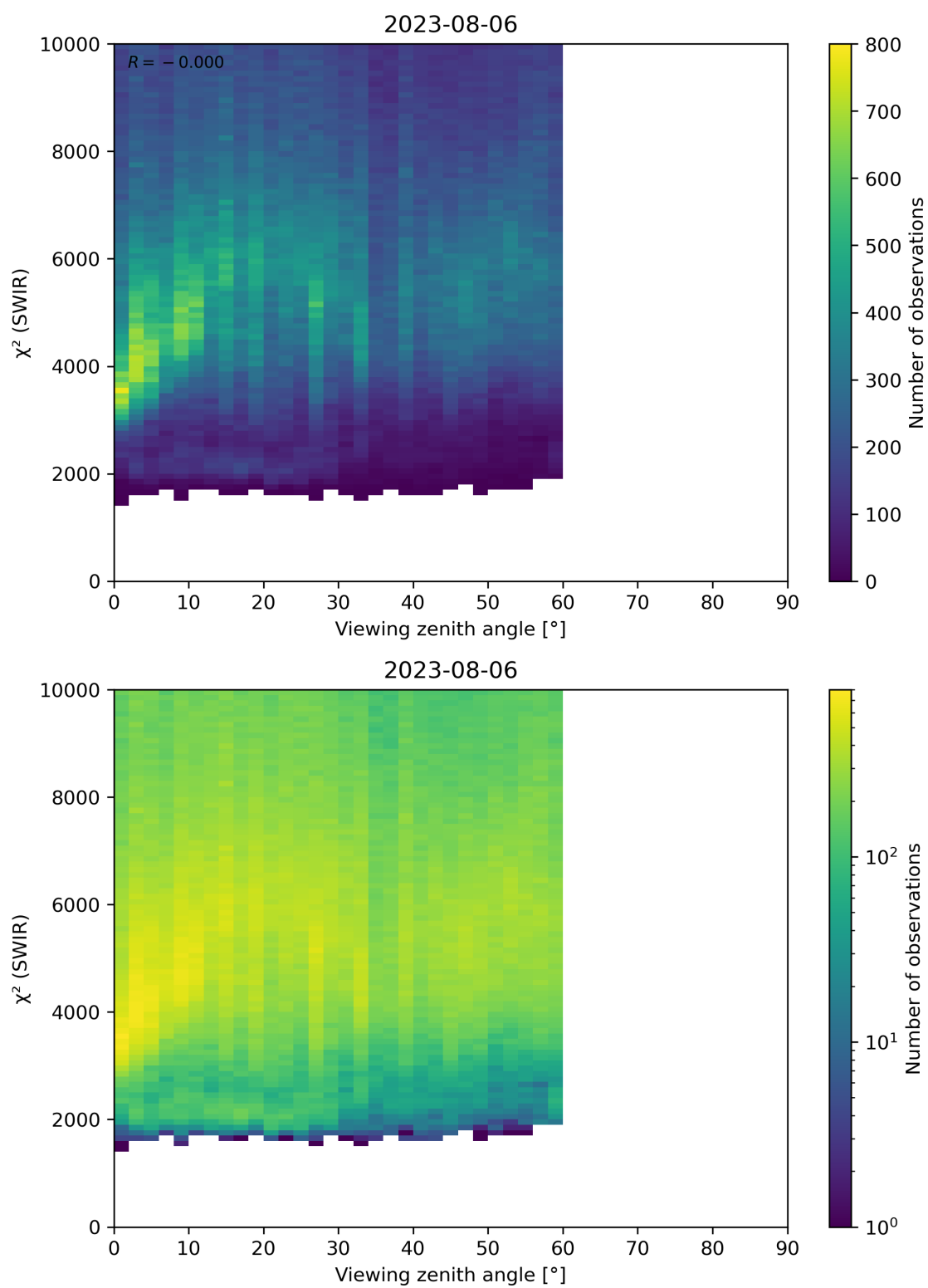
Figure 106: Scatter density plot of “Viewing zenith angle” against “ \chi^2 (SWIR)” for 2023-08-05 to 2023-08-07.
