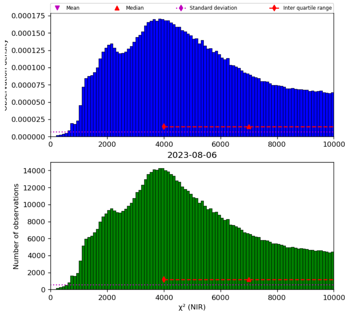
Figure 29: Histogram of “ \chi^2 (NIR)” for 2023-08-05 to 2023-08-07
