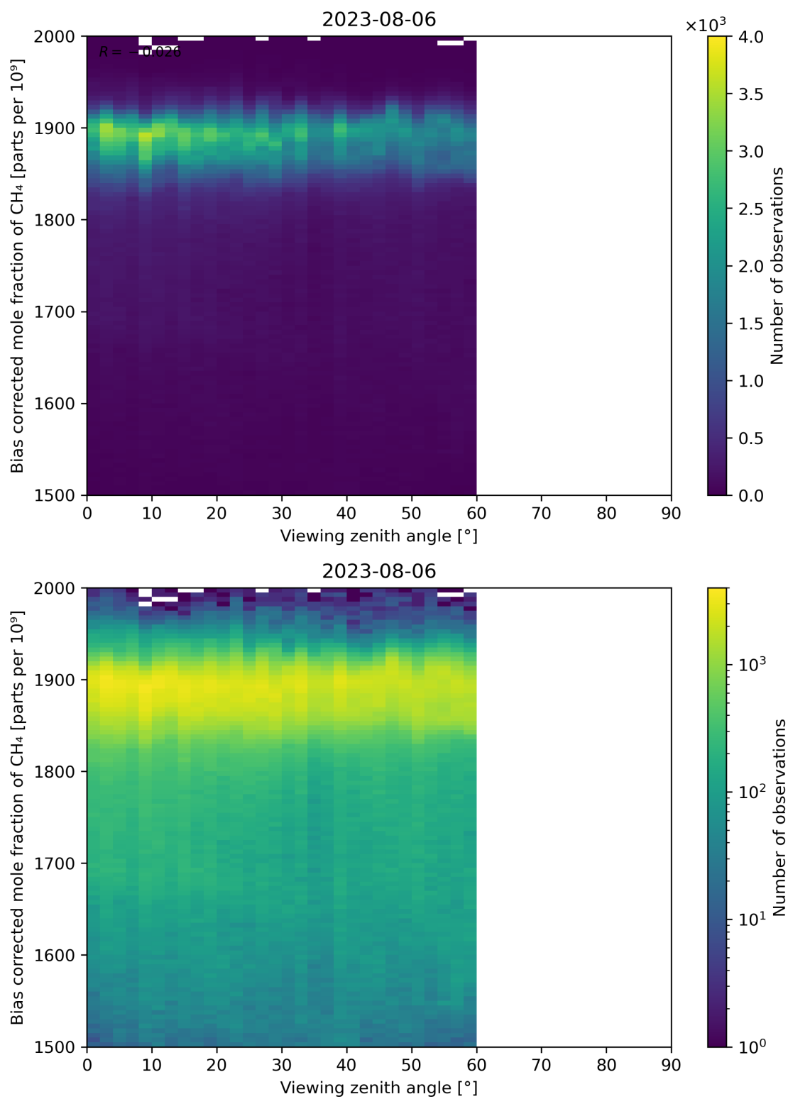
Figure 111: Scatter density plot of “Viewing zenith angle” against “Bias corrected mole fraction of CH 4 ” for 2023-08-05 to 2023-08-07.
