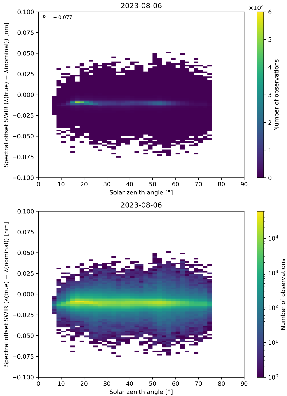
Figure 104: Scatter density plot of “Solar zenith angle” against “Spectral offset SWIR ( \lambda(\text{true}) - \lambda(\text{nominal}) )” for 2023-08-05 to 2023-08-07.
