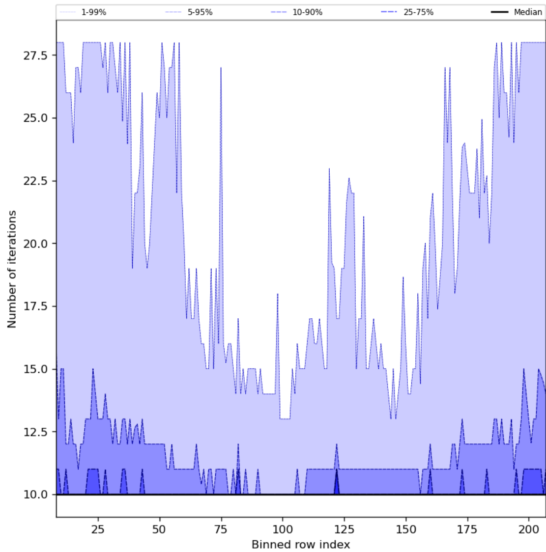
Figure 42: Along track statistics of “Number of iterations” for 2023-08-05 to 2023-08-07
