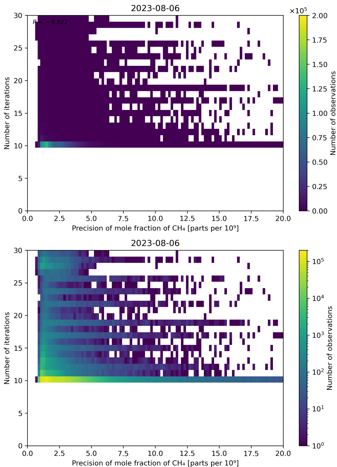
Figure 83: Scatter density plot of “Precision of mole fraction of CH 4 ” against “Number of iterations” for 2023-08-05 to 2023-08-07.
