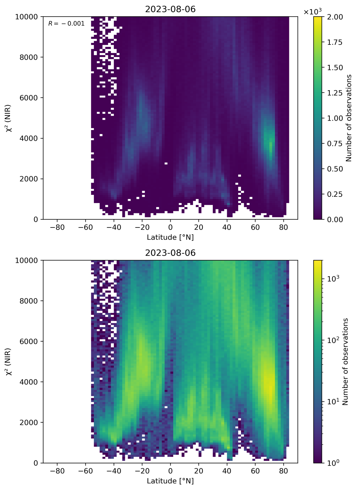
Figure 53: Scatter density plot of “Latitude” against “ \chi^2 (NIR)” for 2023-08-05 to 2023-08-07.
