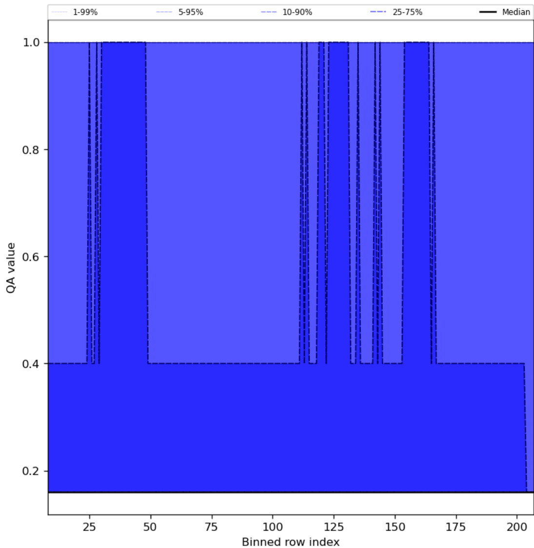
Figure 33: Along track statistics of “QA value” for 2023-08-05 to 2023-08-07
