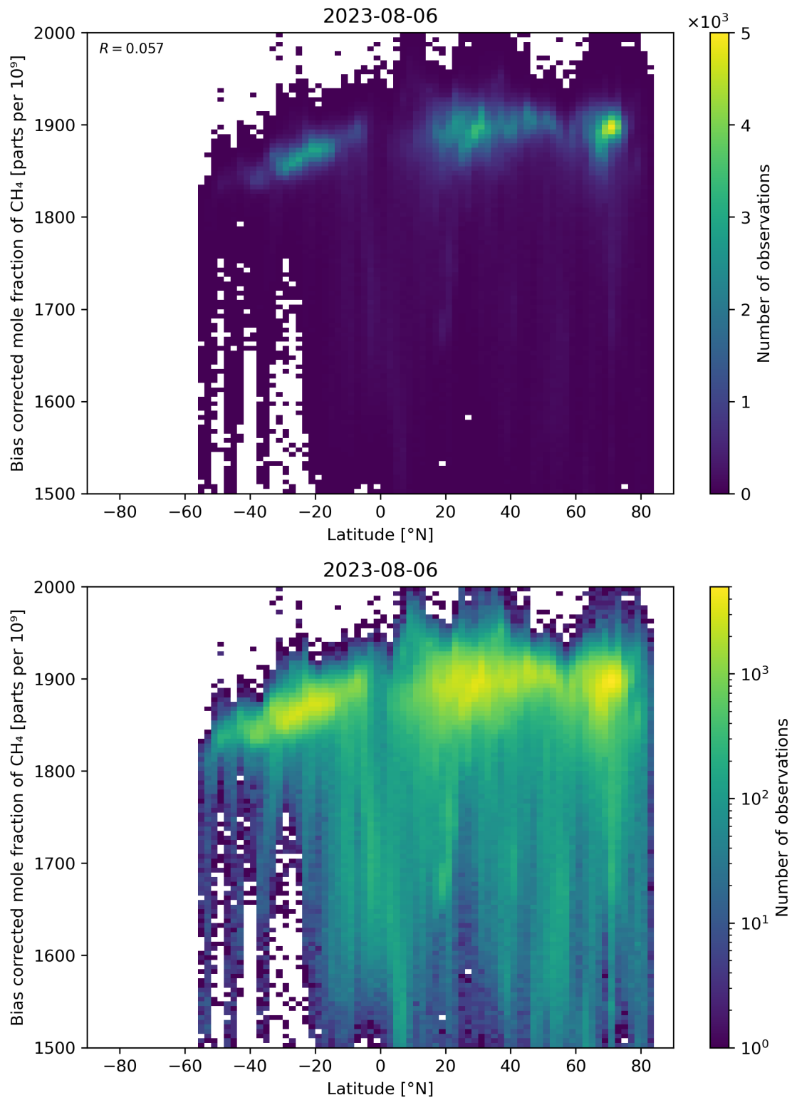
Figure 58: Scatter density plot of “Latitude” against “Bias corrected mole fraction of \text{CH}_4 ” for 2023-08-05 to 2023-08-07.
