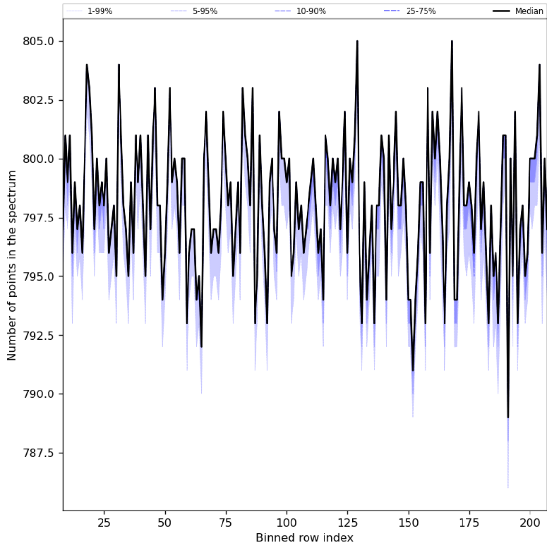
Figure 37: Along track statistics of “Number of points in the spectrum” for 2023-08-05 to 2023-08-07
