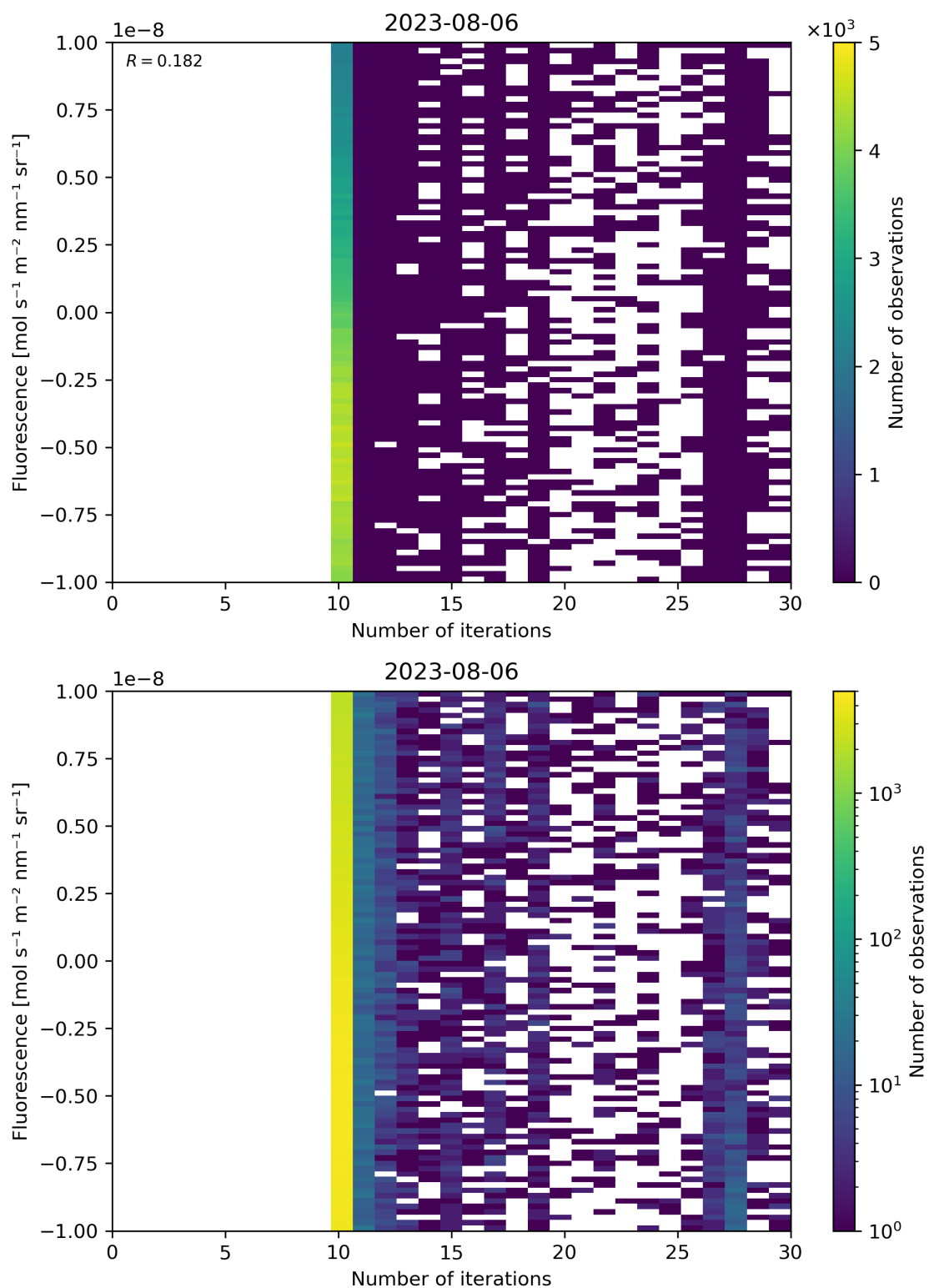
Figure 87: Scatter density plot of “Number of iterations” against “Fluorescence” for 2023-08-05 to 2023-08-07.
