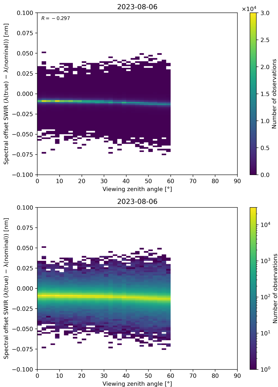
Figure 116: Scatter density plot of “Viewing zenith angle” against “Spectral offset SWIR ( \lambda(\text{true}) - \lambda(\text{nominal}) )” for 2023-08-05 to 2023-08-07.
