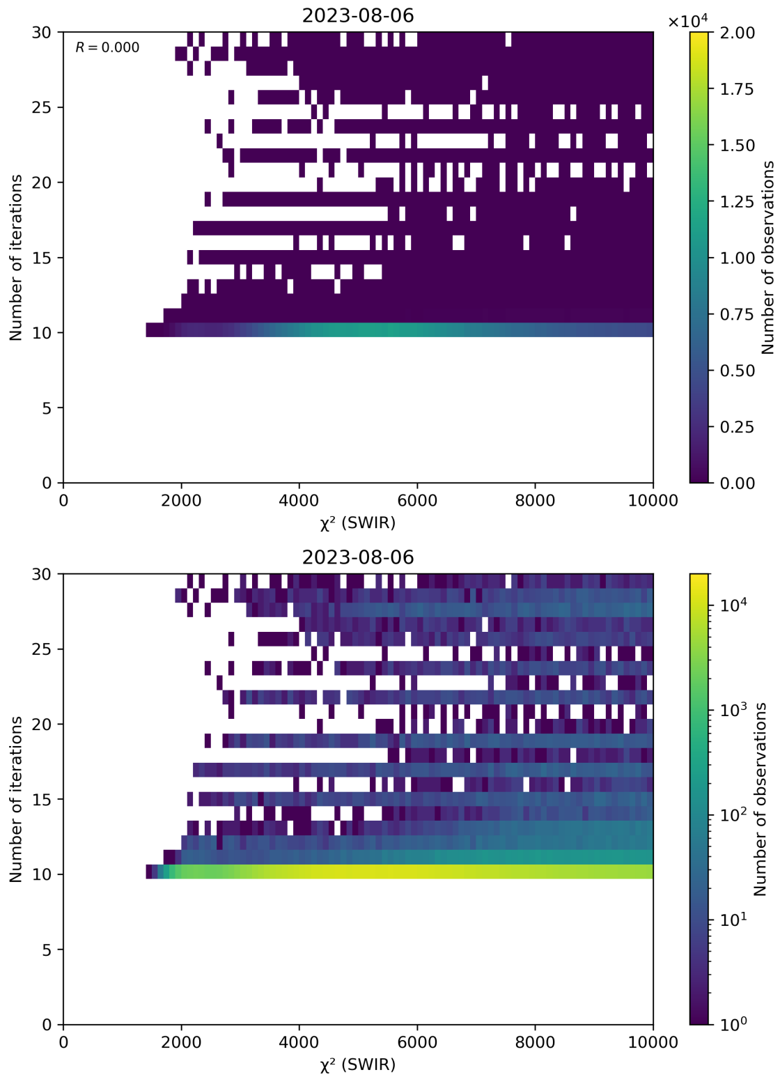
Figure 50: Scatter density plot of “ \chi^2 (SWIR)” against “Number of iterations” for 2023-08-05 to 2023-08-07.
