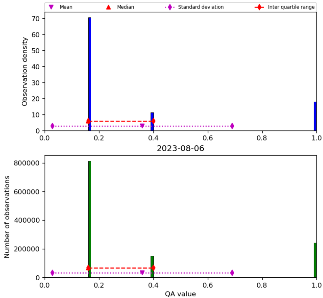
Figure 22: Histogram of “QA value” for 2023-08-05 to 2023-08-07
