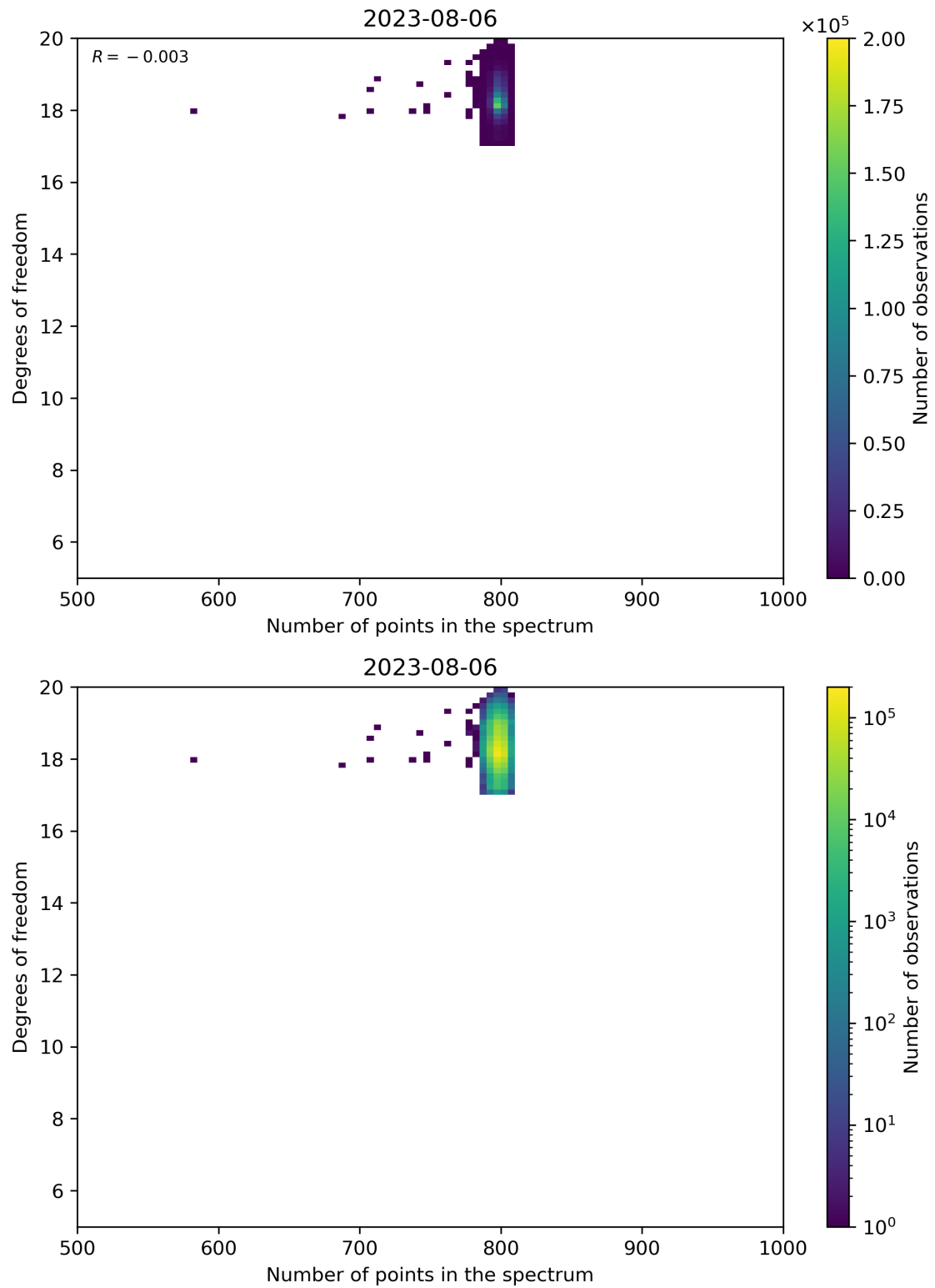
Figure 90: Scatter density plot of “Number of points in the spectrum” against “Degrees of freedom” for 2023-08-05 to 2023-08-07.
