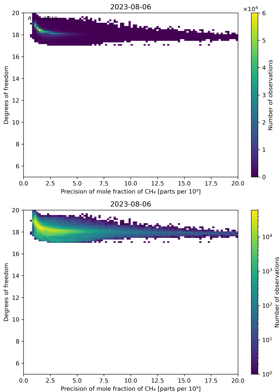
Figure 80: Scatter density plot of “Precision of mole fraction of CH 4 ” against “Degrees of freedom” for 2023-08-05 to 2023-08-07.
