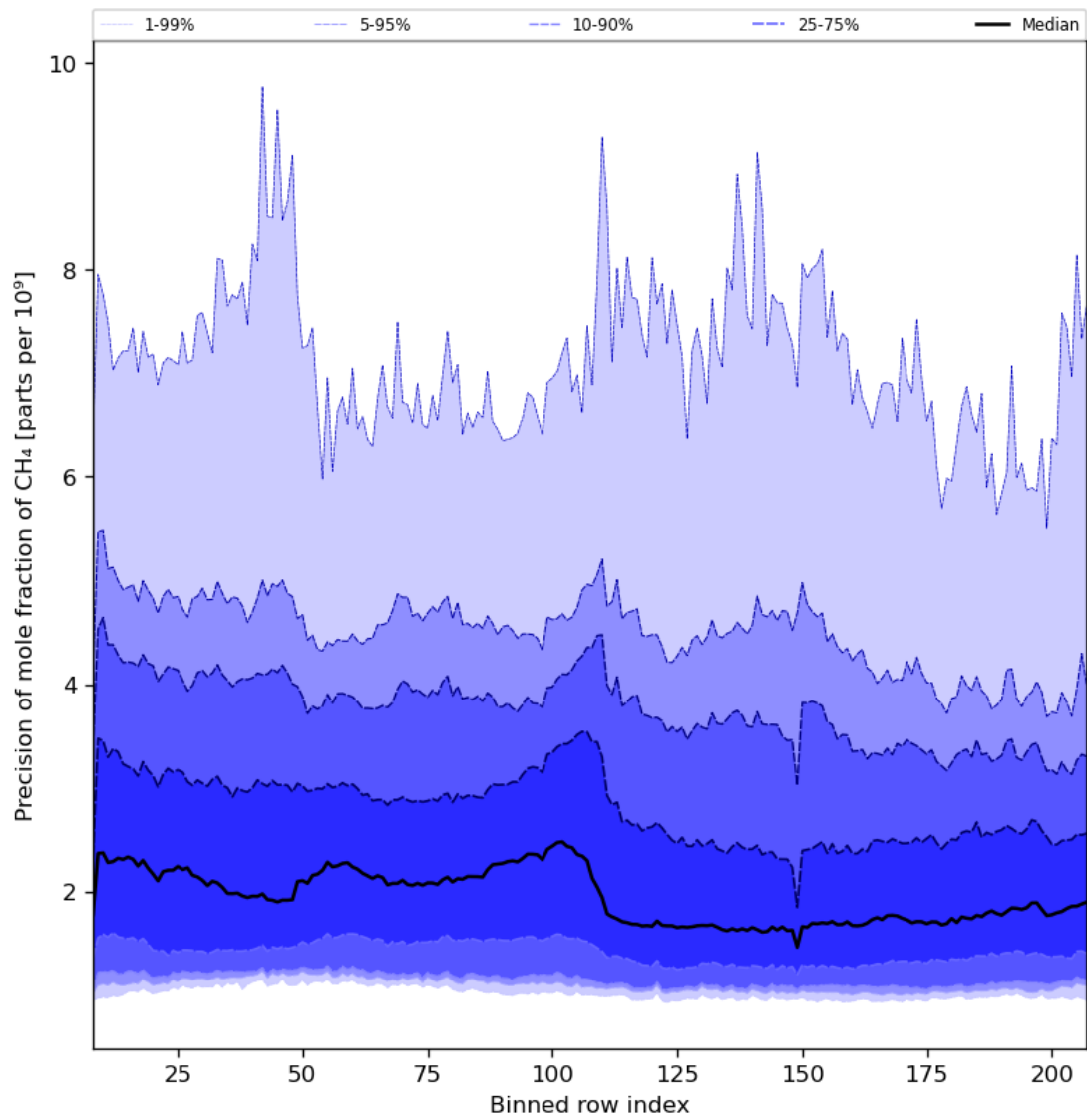
Figure 35: Along track statistics of “Precision of mole fraction of CH 4 ” for 2023-08-05 to 2023-08-07
