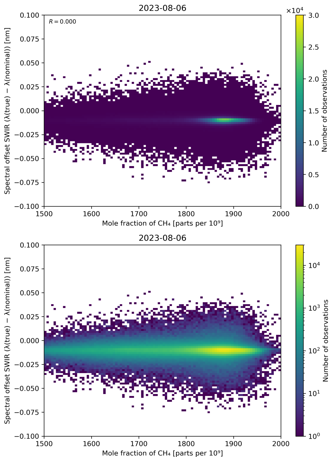
Figure 86: Scatter density plot of “Mole fraction of CH 4 ” against “Spectral offset SWIR ( \lambda(\text{true}) - \lambda(\text{nominal}) )” for 2023-08-05 to 2023-08-07.
