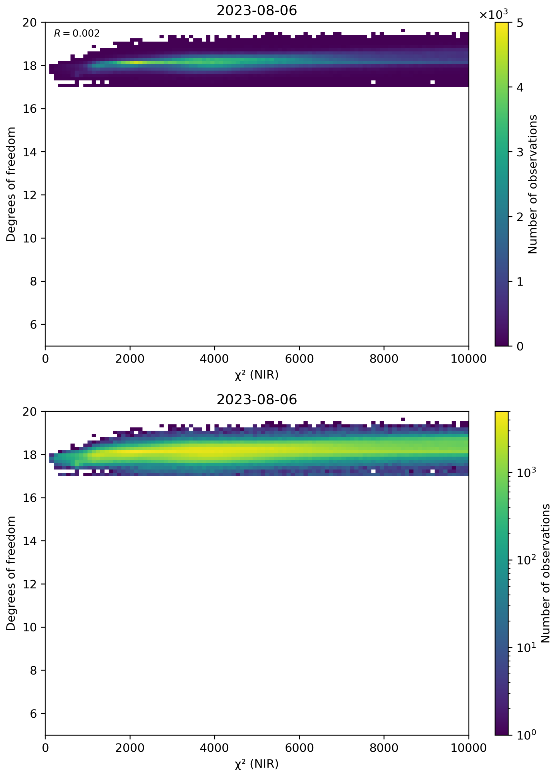
Figure 44: Scatter density plot of “ \chi^2 (NIR)” against “Degrees of freedom” for 2023-08-05 to 2023-08-07.
