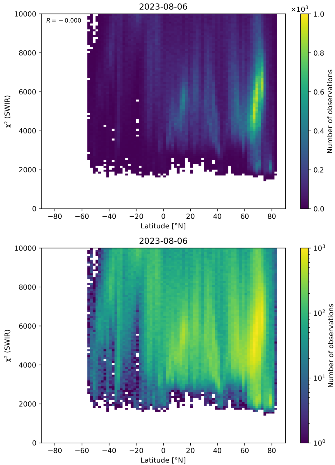
Figure 54: Scatter density plot of “Latitude” against “ \chi^2 (SWIR)” for 2023-08-05 to 2023-08-07.
