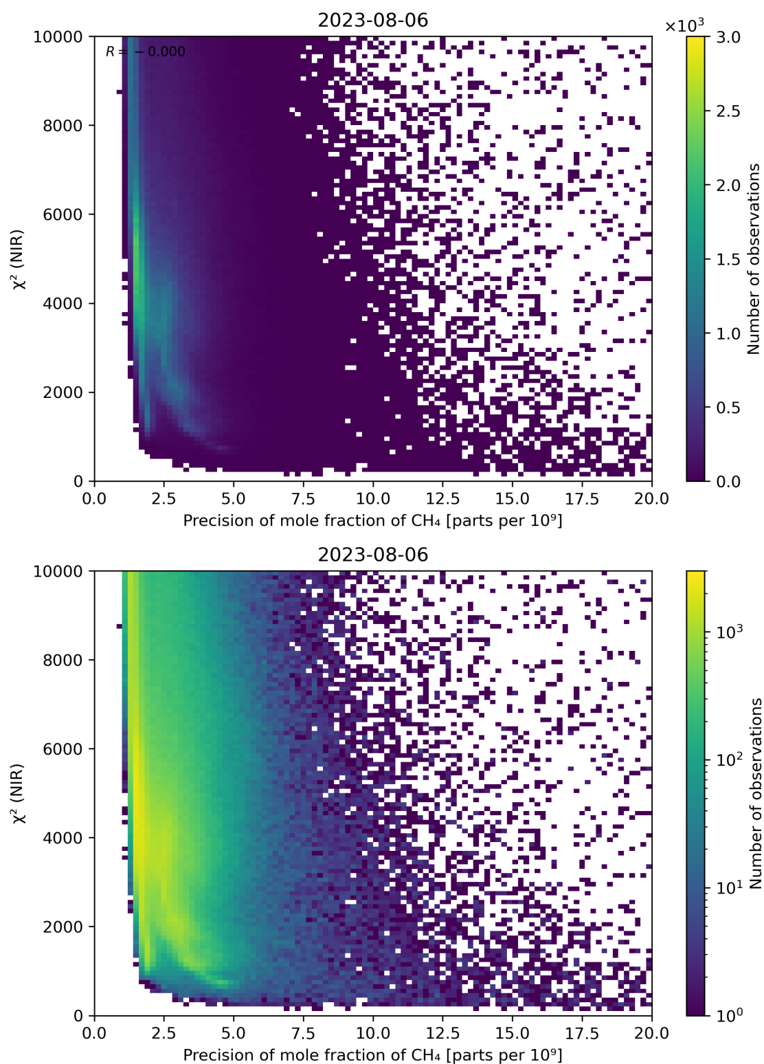
Figure 78: Scatter density plot of “Precision of mole fraction of CH 4 ” against “ \chi^2 (NIR)” for 2023-08-05 to 2023-08-07.
