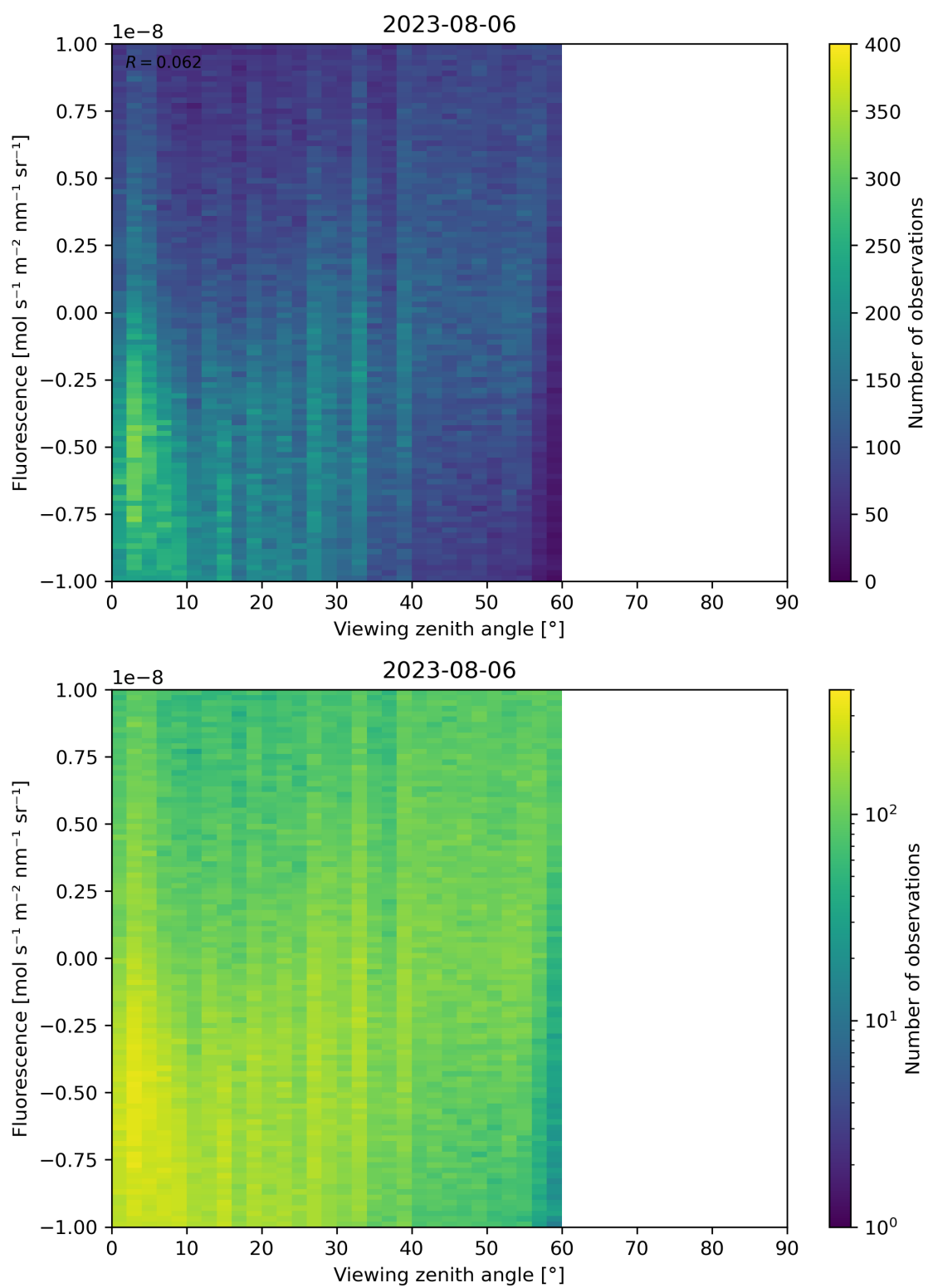
Figure 108: Scatter density plot of “Viewing zenith angle” against “Fluorescence” for 2023-08-05 to 2023-08-07.
