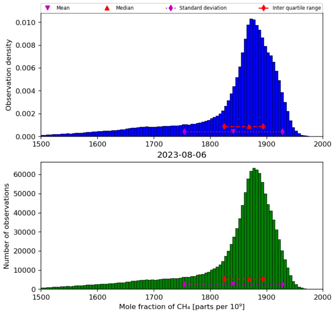
Figure 23: Histogram of “Mole fraction of CH 4 ” for 2023-08-05 to 2023-08-07
