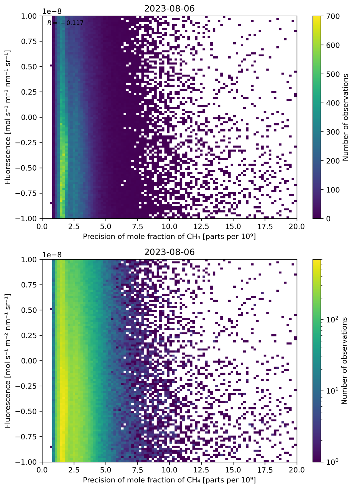
Figure 81: Scatter density plot of “Precision of mole fraction of \text{CH}_4 ” against “Fluorescence” for 2023-08-05 to 2023-08-07.
