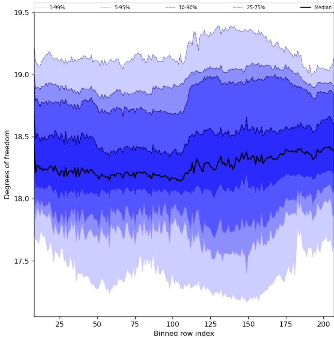
Figure 41: Along track statistics of “Degrees of freedom” for 2023-08-05 to 2023-08-07
