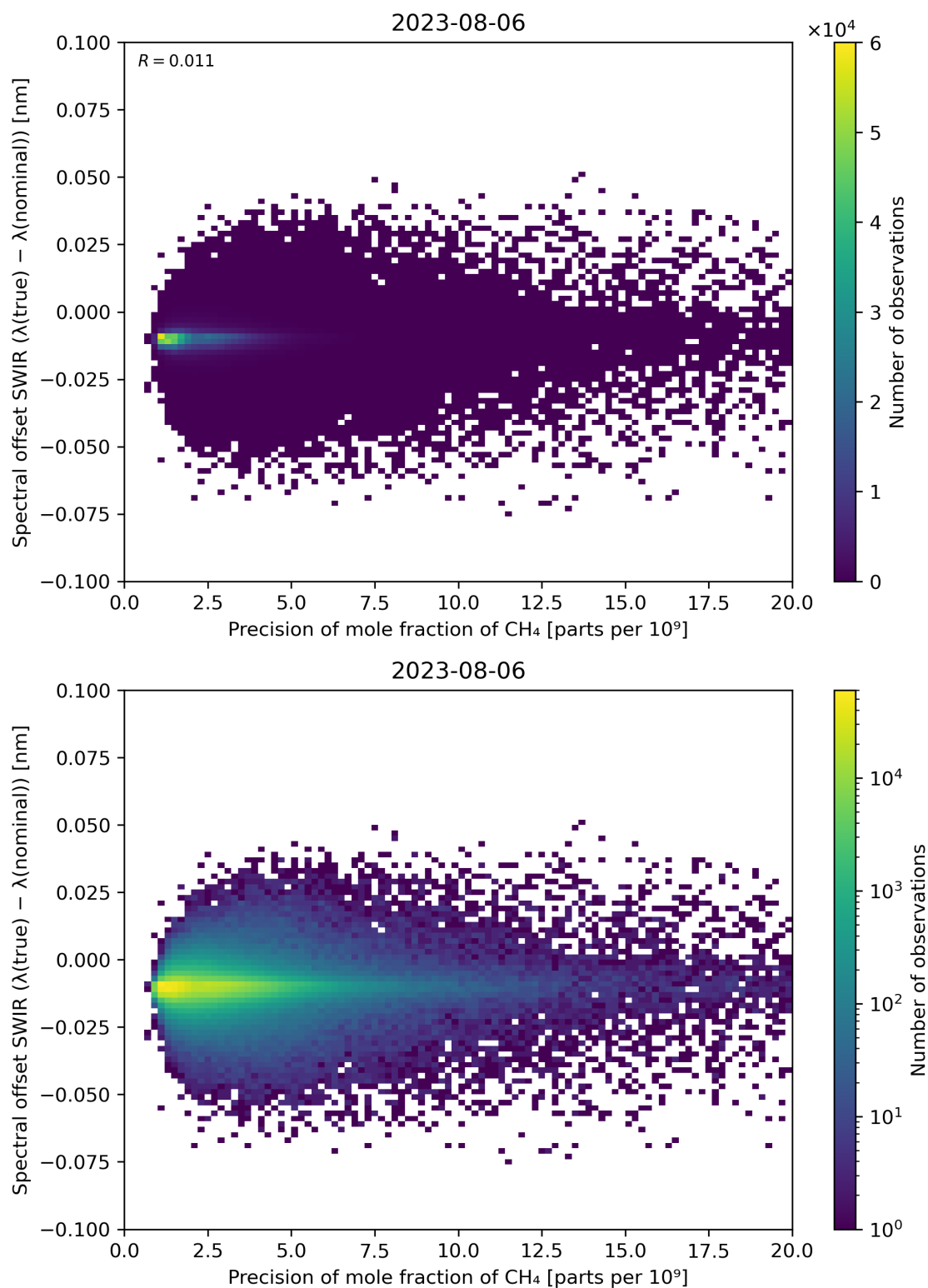
Figure 85: Scatter density plot of “Precision of mole fraction of \text{CH}_4 ” against “Spectral offset SWIR ( \lambda(\text{true}) - \lambda(\text{nominal}) )” for 2023-08-05 to 2023-08-07.
