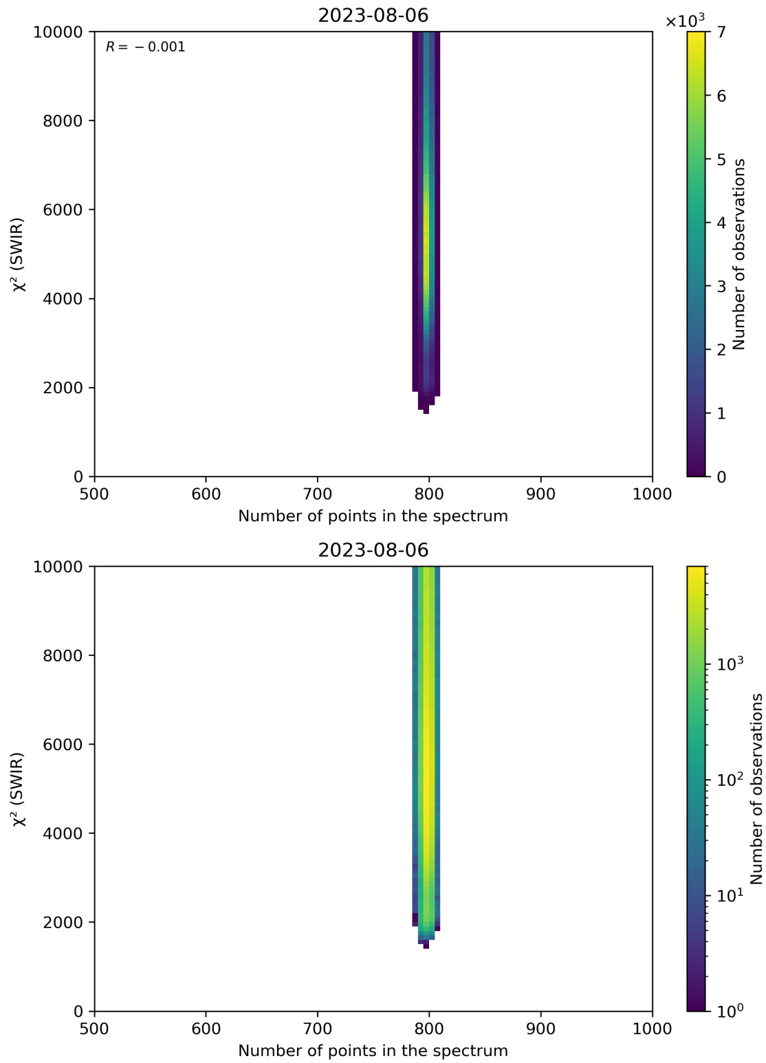
Figure 89: Scatter density plot of “Number of points in the spectrum” against “ \chi^2 (SWIR)” for 2023-08-05 to 2023-08-07.
