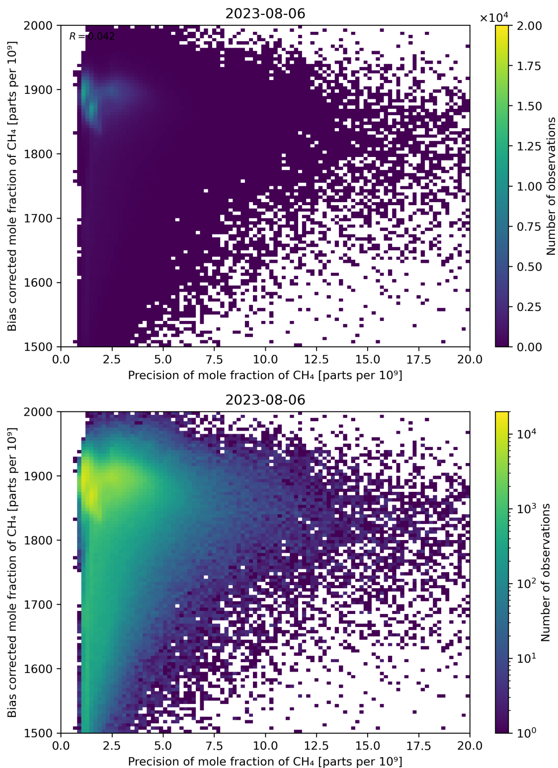
Figure 82: Scatter density plot of “Precision of mole fraction of CH 4 ” against “Bias corrected mole fraction of CH 4 ” for 2023-08-05 to 2023-08-07.
