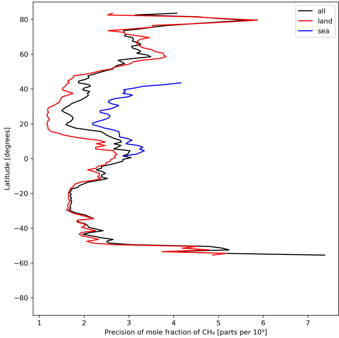
Figure 13: Zonal average of “Precision of mole fraction of CH 4 ” for 2023-08-05 to 2023-08-07.
