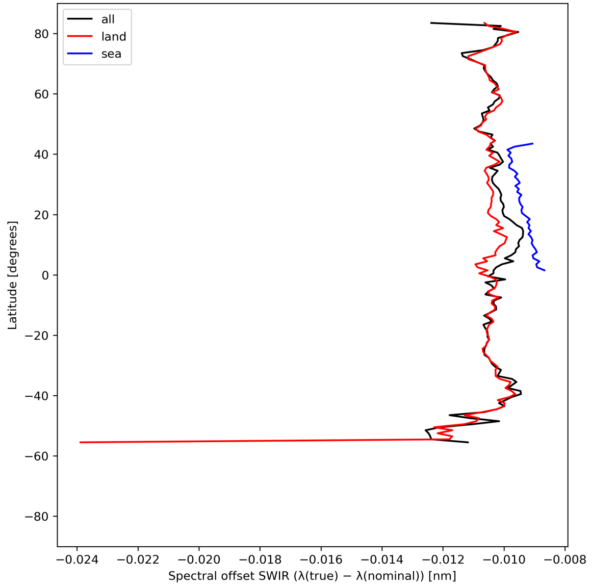
Figure 16: Zonal average of “Spectral offset SWIR ( \lambda(\text{true}) - \lambda(\text{nominal}) )” for 2023-08-05 to 2023-08-07.
