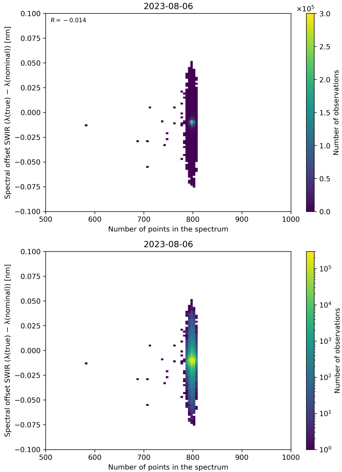
Figure 93: Scatter density plot of “Number of points in the spectrum” against “Spectral offset SWIR ( \lambda(\text{true}) - \lambda(\text{nominal}) )” for 2023-08-05 to 2023-08-07.
