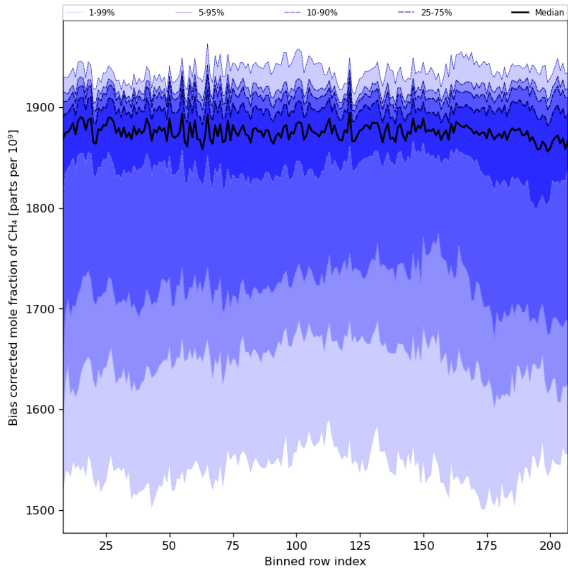
Figure 36: Along track statistics of “Bias corrected mole fraction of CH 4 ” for 2023-08-05 to 2023-08-07
