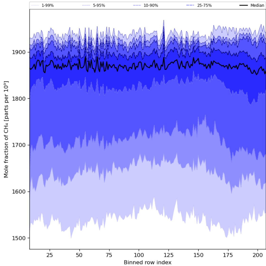
Figure 34: Along track statistics of “Mole fraction of CH 4 ” for 2023-08-05 to 2023-08-07
