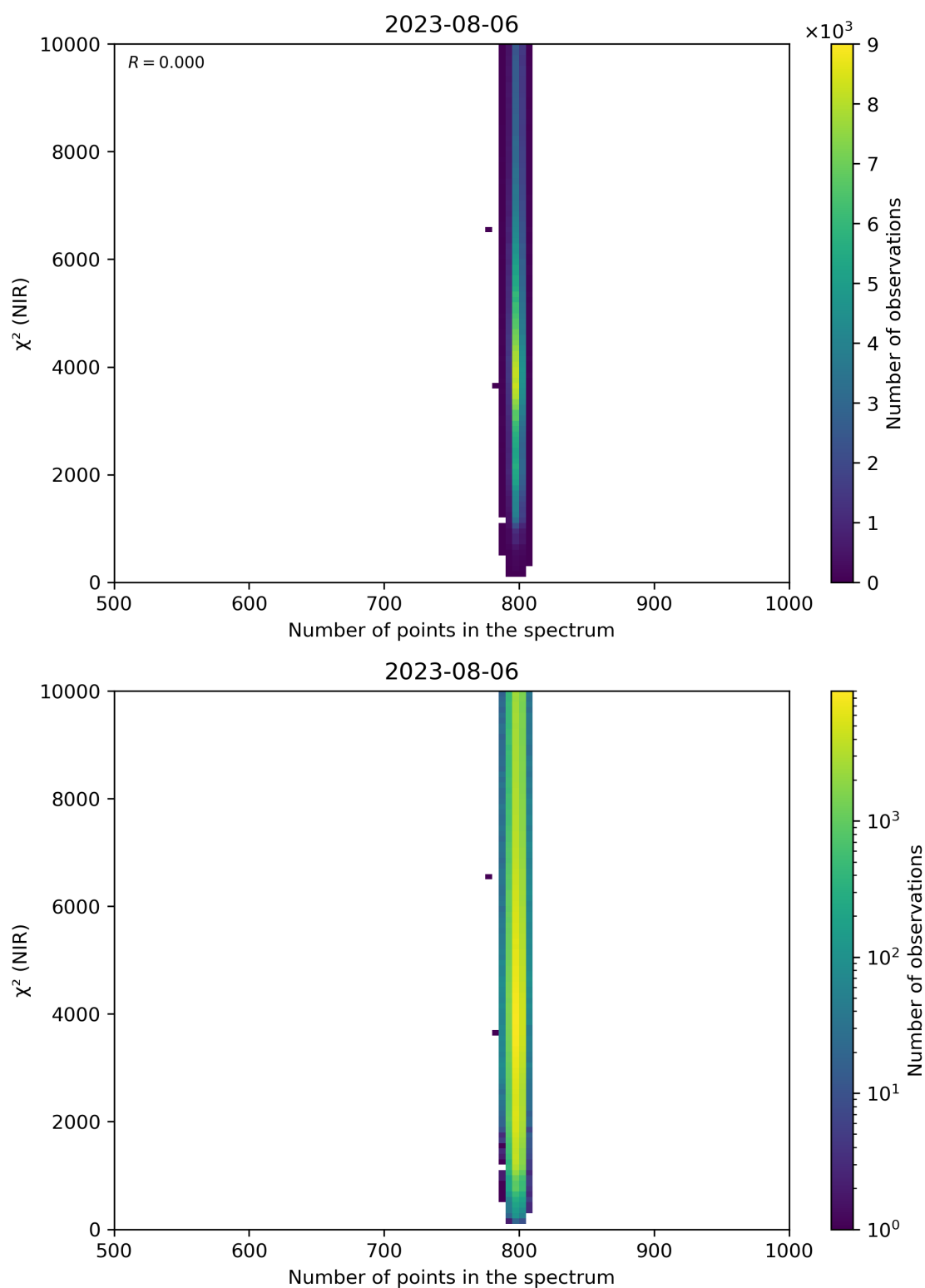
Figure 88: Scatter density plot of “Number of points in the spectrum” against “ \chi^2 (NIR)” for 2023-08-05 to 2023-08-07.
