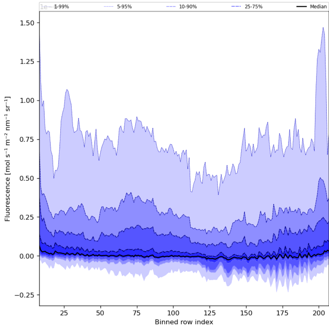
Figure 43: Along track statistics of “Fluorescence” for 2023-08-05 to 2023-08-07
