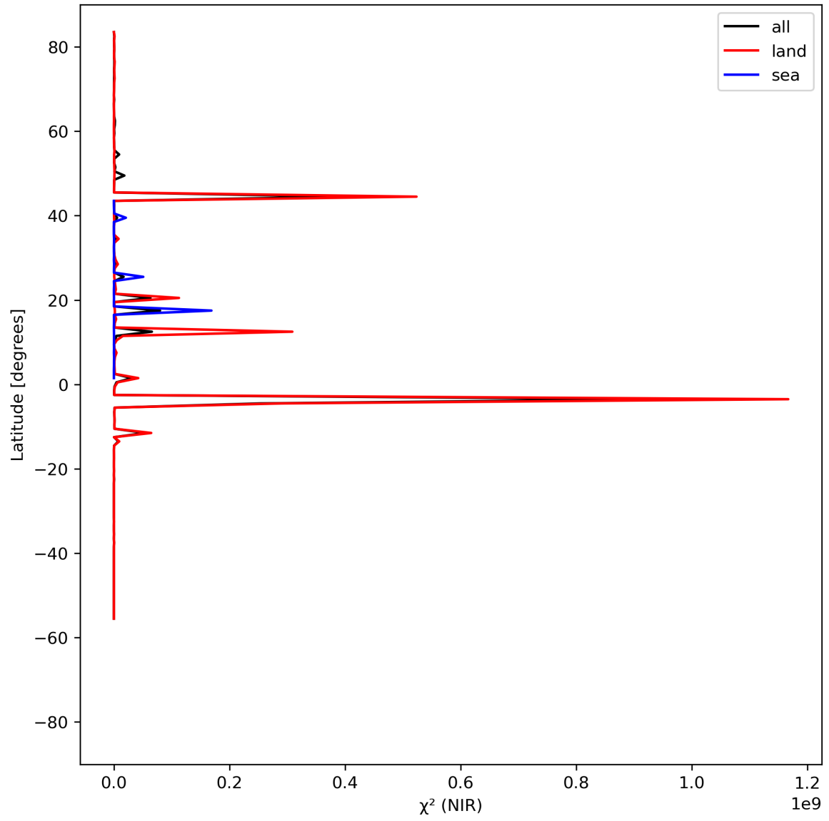
Figure 18: Zonal average of “ \chi^2 (NIR)” for 2023-08-05 to 2023-08-07.
