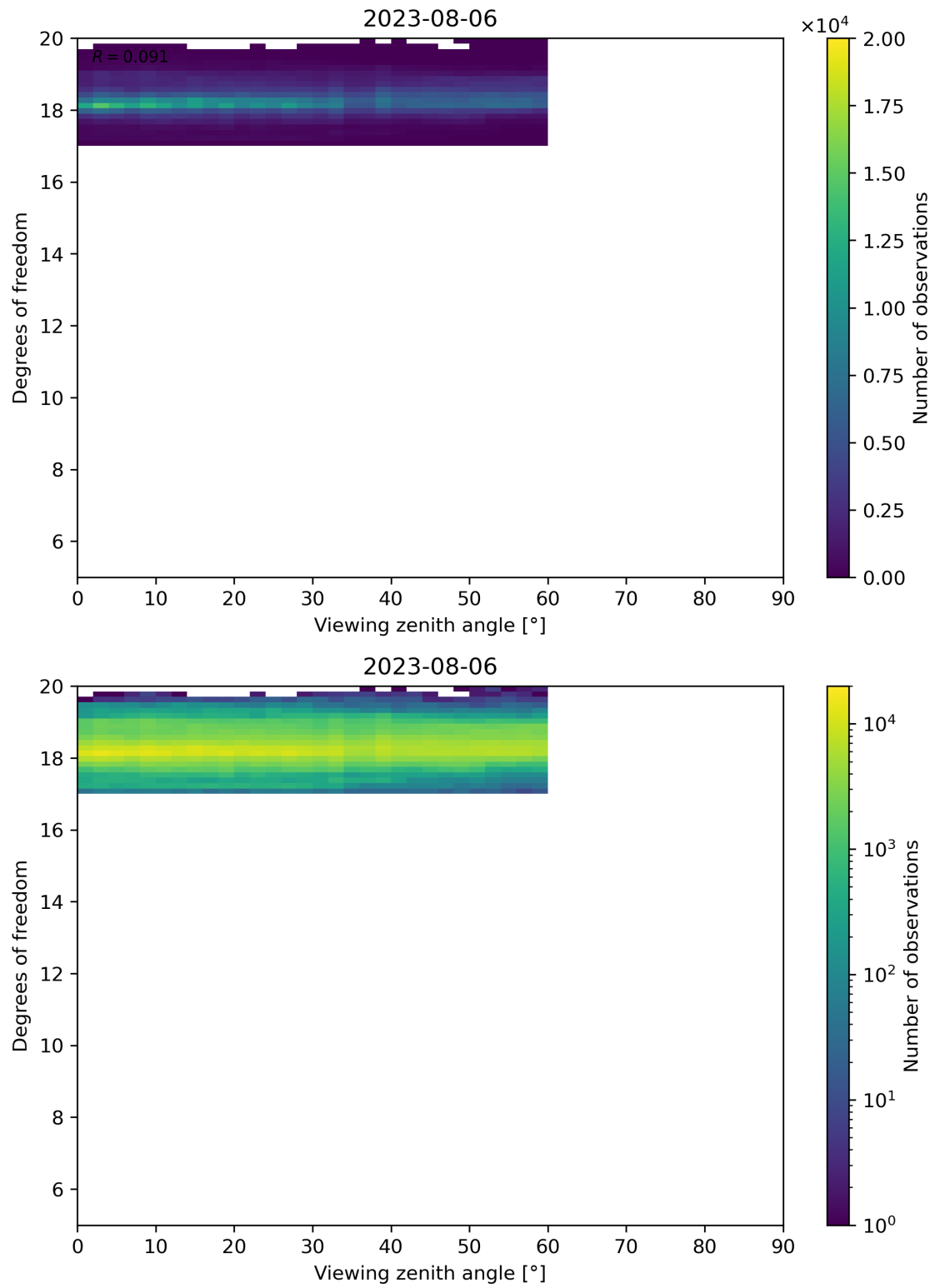
Figure 107: Scatter density plot of “Viewing zenith angle” against “Degrees of freedom” for 2023-08-05 to 2023-08-07.
