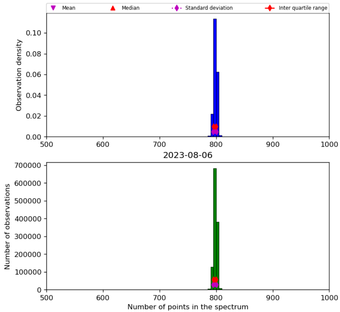
Figure 26: Histogram of “Number of points in the spectrum” for 2023-08-05 to 2023-08-07
