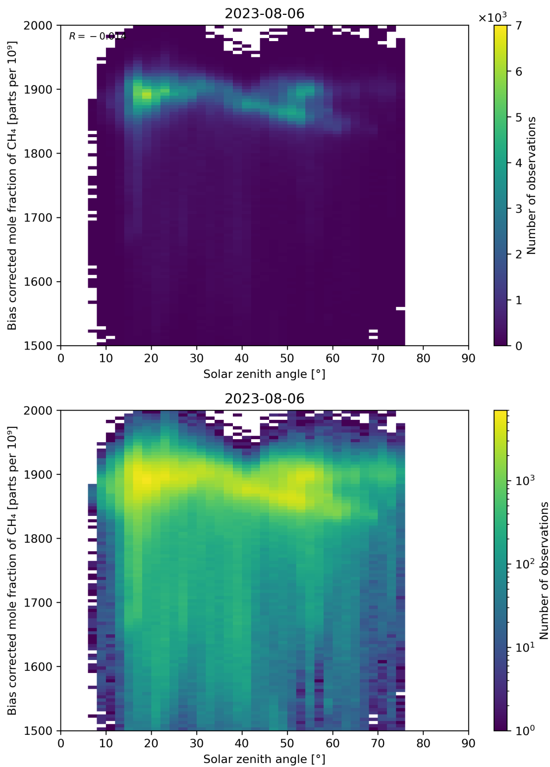
Figure 100: Scatter density plot of “Solar zenith angle” against “Bias corrected mole fraction of CH 4 ” for 2023-08-05 to 2023-08-07.
