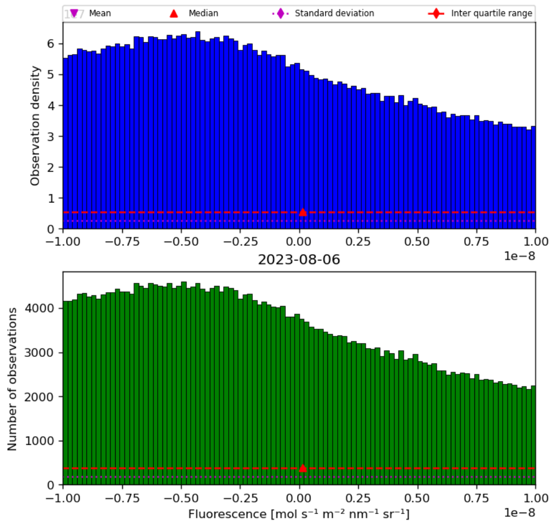
Figure 32: Histogram of “Fluorescence” for 2023-08-05 to 2023-08-07
