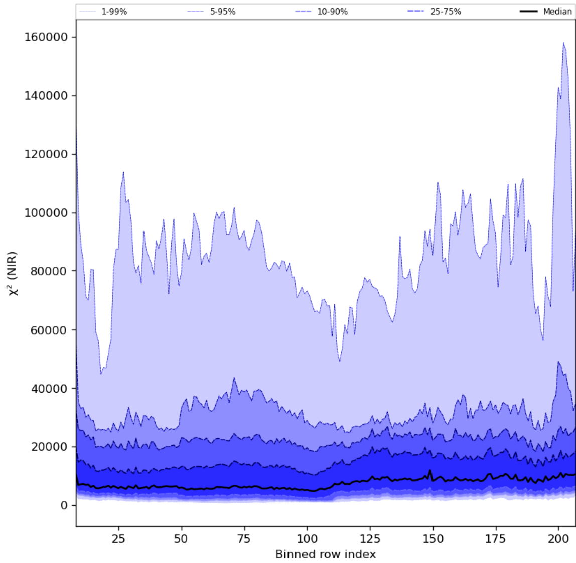
Figure 40: Along track statistics of “ \chi^2 (NIR)” for 2023-08-05 to 2023-08-07
