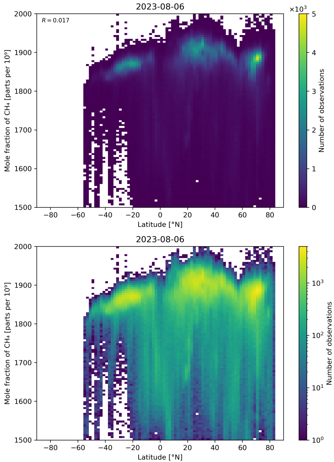
Figure 57: Scatter density plot of “Latitude” against “Mole fraction of CH 4 ” for 2023-08-05 to 2023-08-07.
