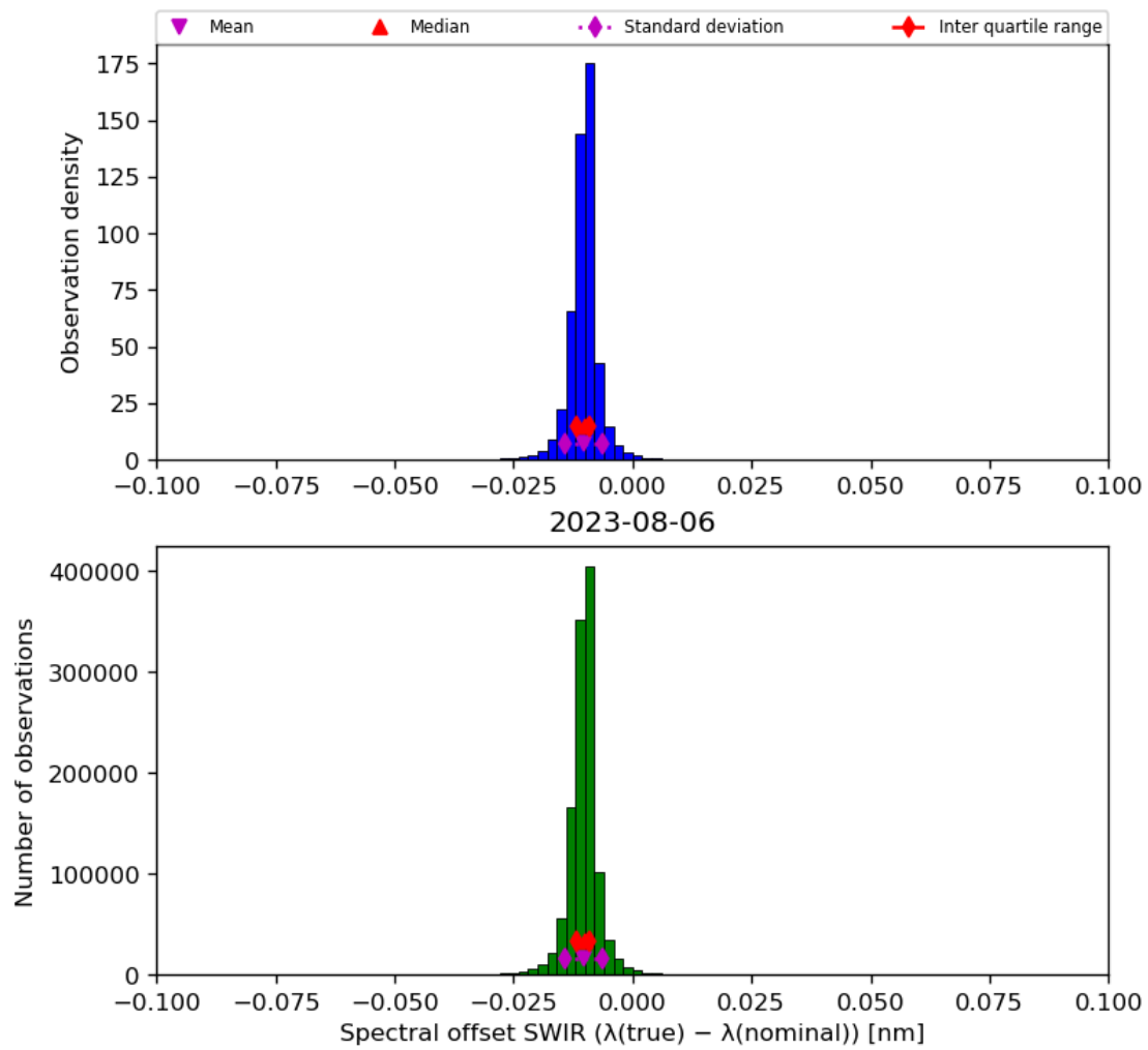
Figure 27: Histogram of “Spectral offset SWIR ( \lambda(\text{true}) - \lambda(\text{nominal}) )” for 2023-08-05 to 2023-08-07
