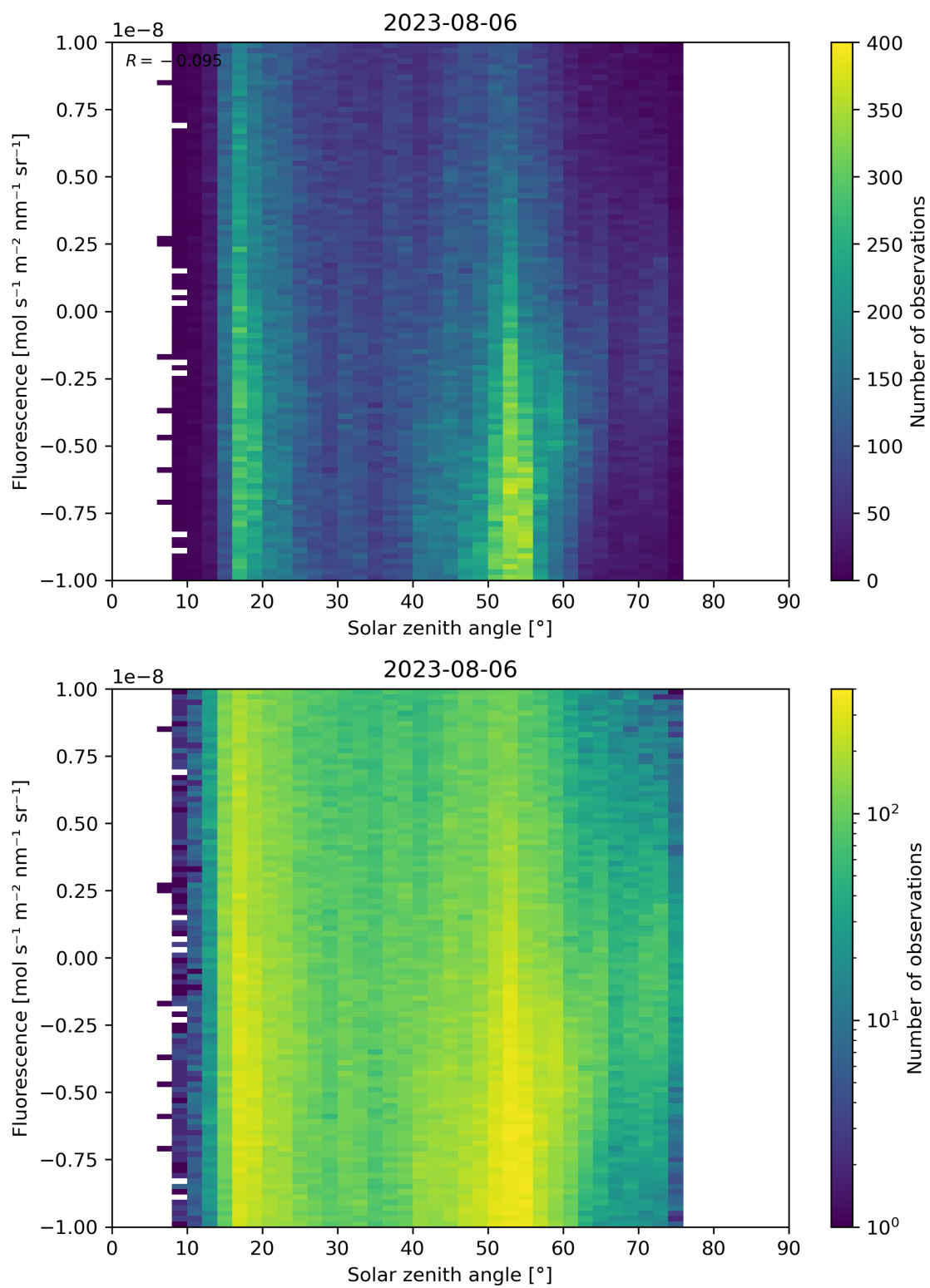
Figure 97: Scatter density plot of “Solar zenith angle” against “Fluorescence” for 2023-08-05 to 2023-08-07.
