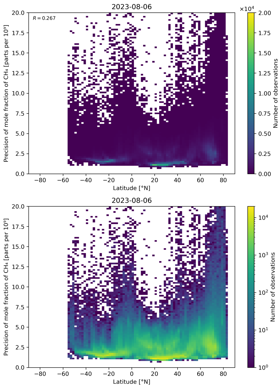
Figure 59: Scatter density plot of “Latitude” against “Precision of mole fraction of CH 4 ” for 2023-08-05 to 2023-08-07.
