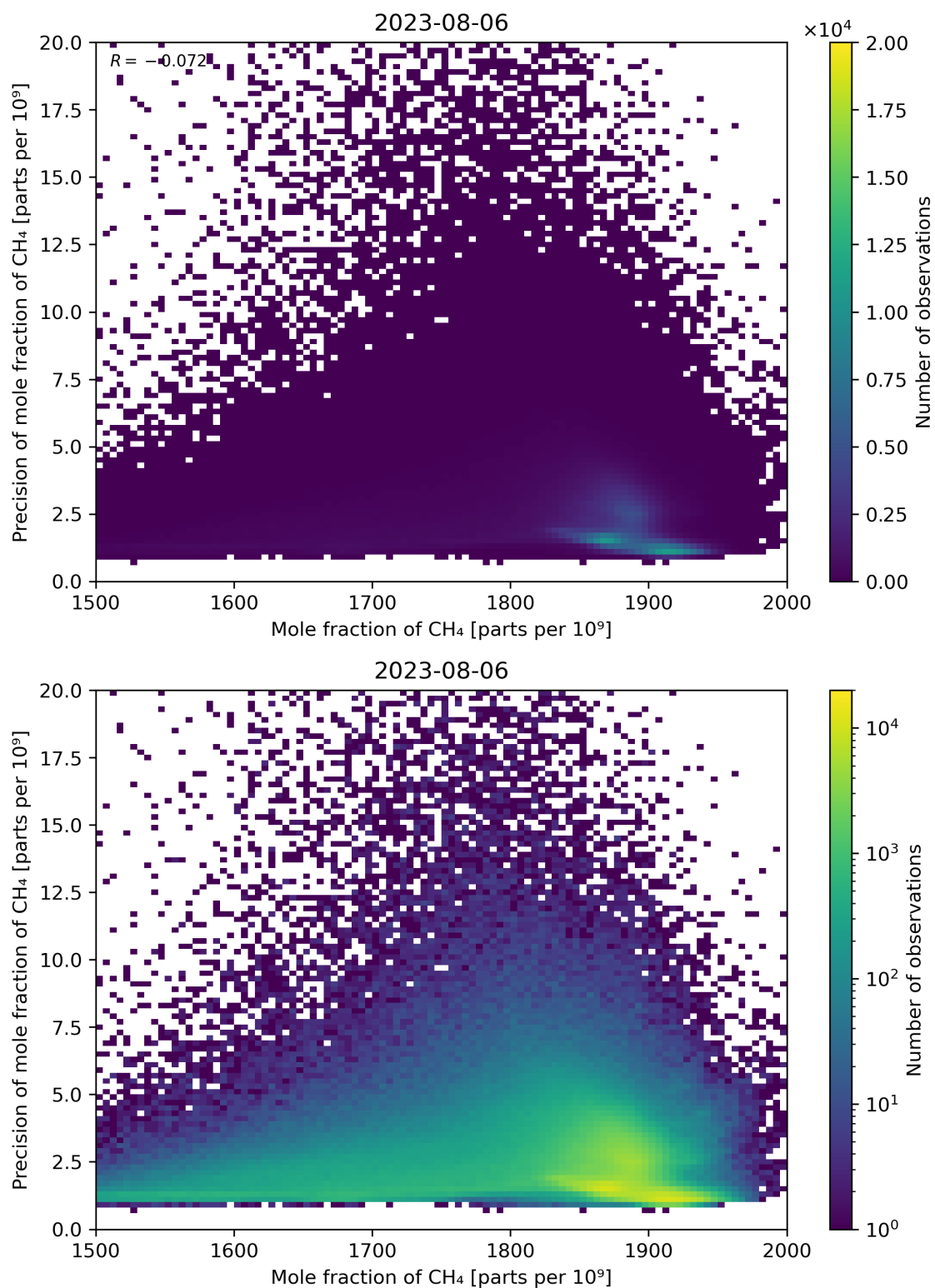
Figure 75: Scatter density plot of “Mole fraction of CH 4 ” against “Precision of mole fraction of CH 4 ” for 2023-08-05 to 2023-08-07.
