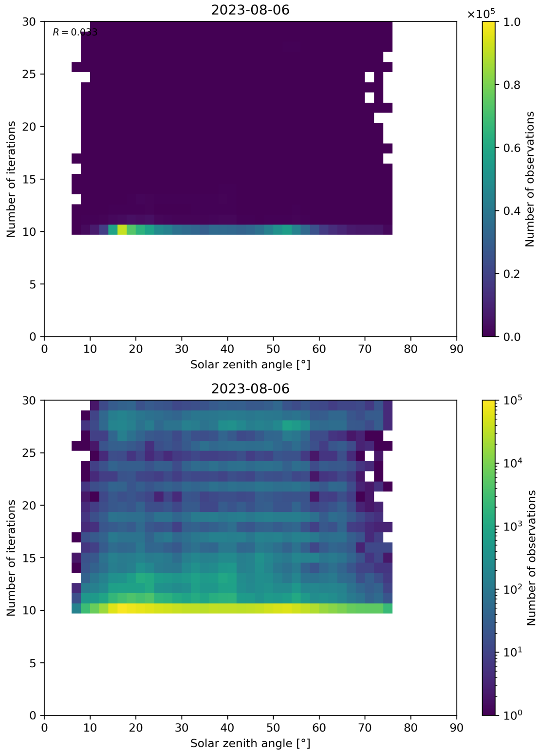
Figure 102: Scatter density plot of “Solar zenith angle” against “Number of iterations” for 2023-08-05 to 2023-08-07.
