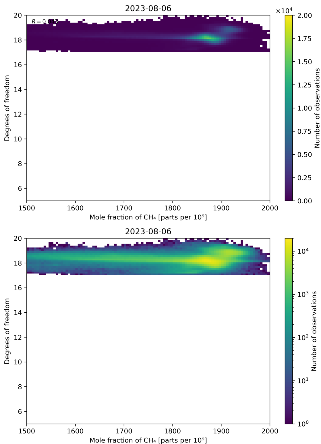
Figure 72: Scatter density plot of “Mole fraction of CH 4 ” against “Degrees of freedom” for 2023-08-05 to 2023-08-07.
