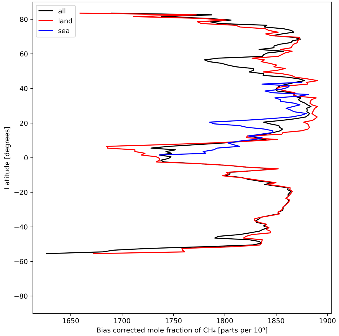
Figure 14: Zonal average of “Bias corrected mole fraction of \text{CH}_4 ” for 2023-08-05 to 2023-08-07.
