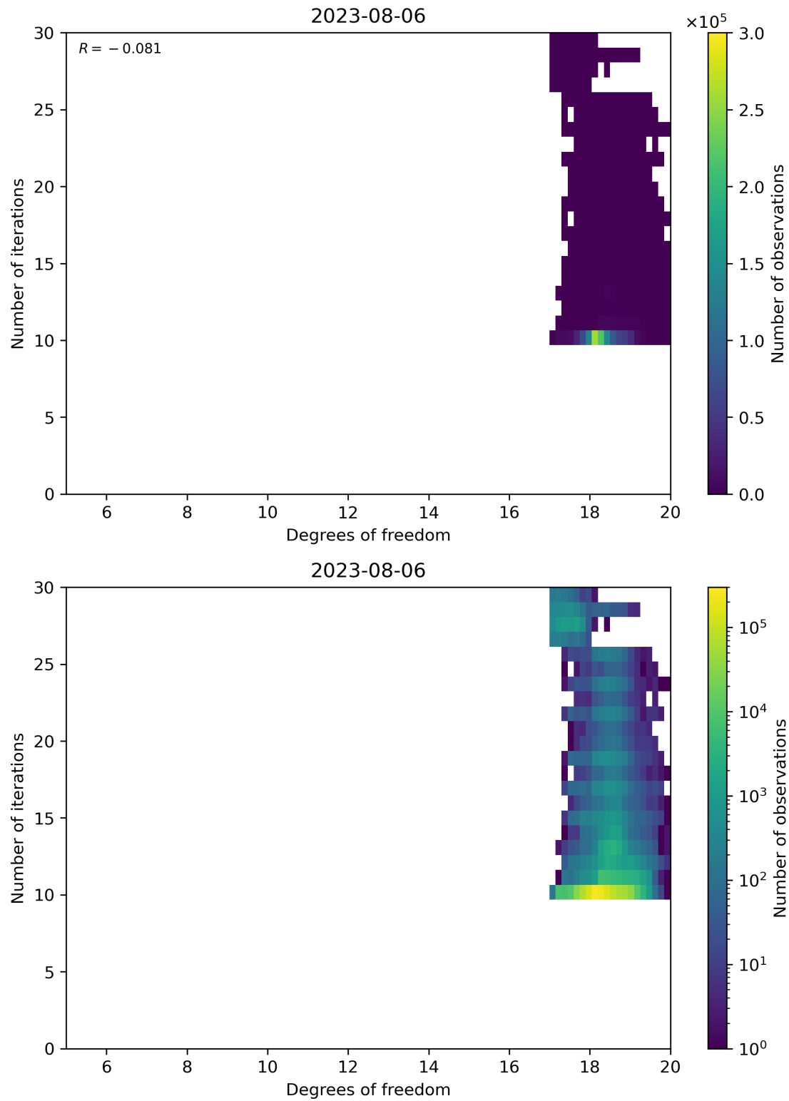
Figure 52: Scatter density plot of “Degrees of freedom” against “Number of iterations” for 2023-08-05 to 2023-08-07.
