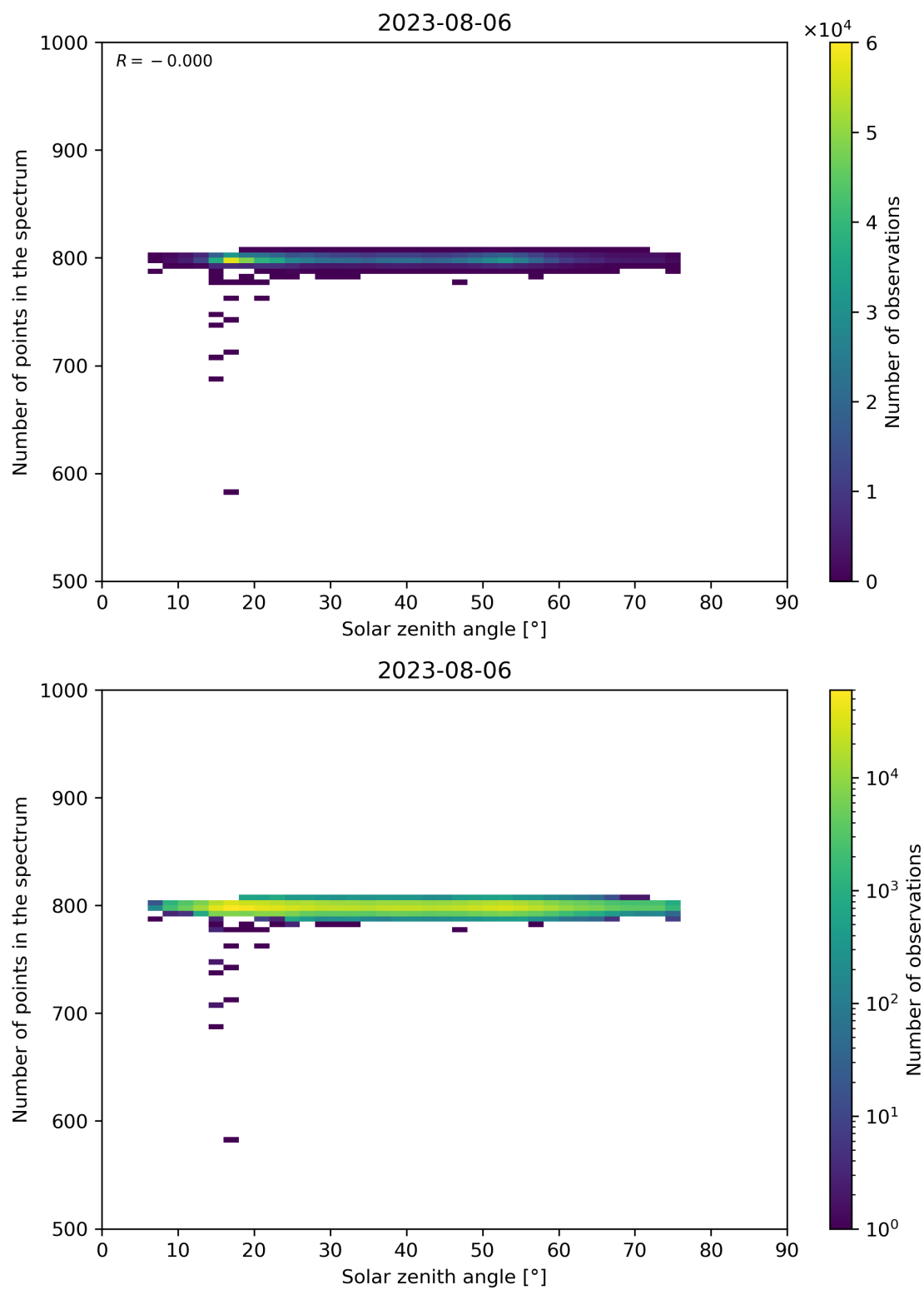
Figure 103: Scatter density plot of “Solar zenith angle” against “Number of points in the spectrum” for 2023-08-05 to 2023-08-07.
