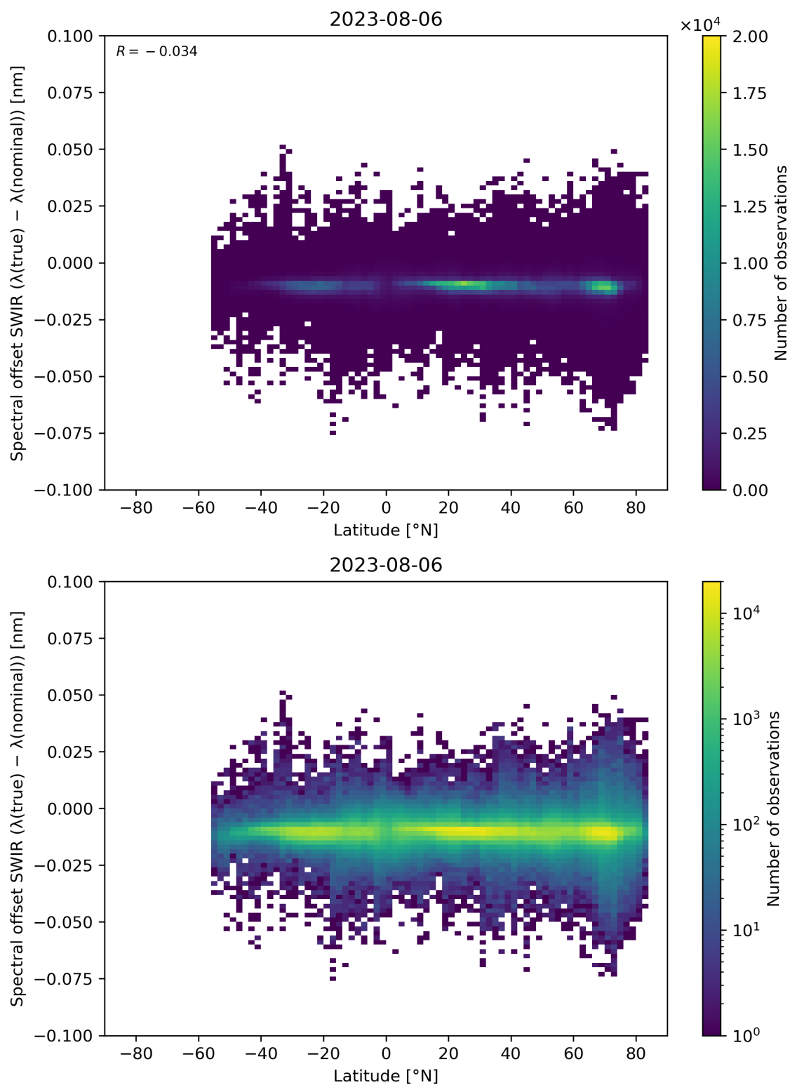
Figure 62: Scatter density plot of “Latitude” against “Spectral offset SWIR ( \lambda(\text{true}) - \lambda(\text{nominal}) )” for 2023-08-05 to 2023-08-07.
