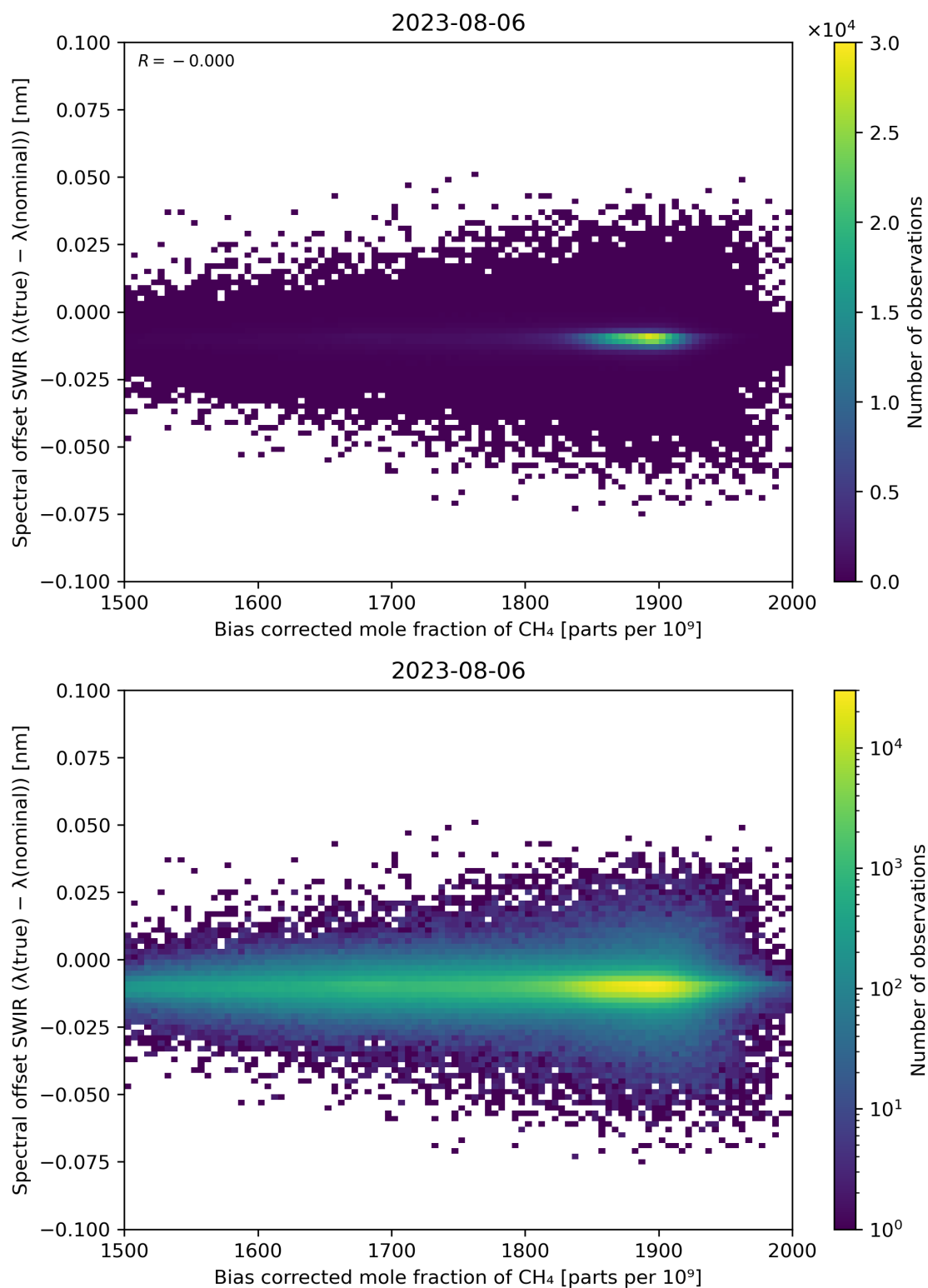
Figure 69: Scatter density plot of “Bias corrected mole fraction of \text{CH}_4 ” against “Spectral offset SWIR ( \lambda(\text{true}) - \lambda(\text{nominal}) )” for 2023-08-05 to 2023-08-07.
