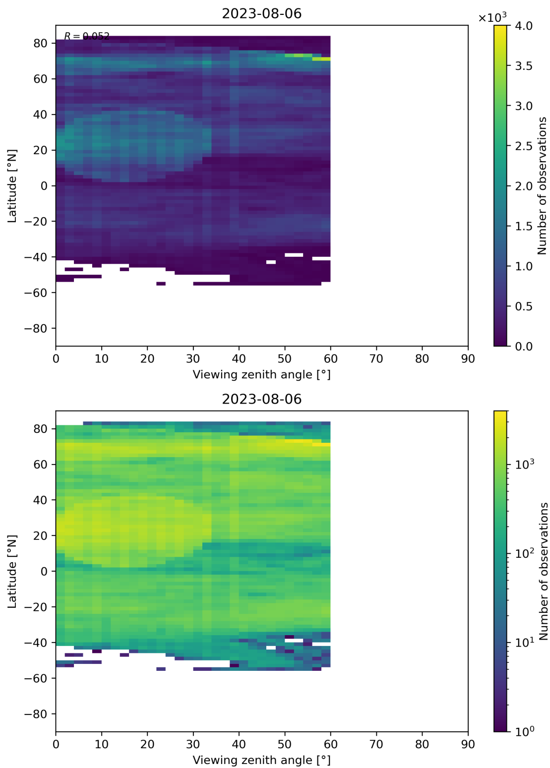
Figure 109: Scatter density plot of “Viewing zenith angle” against “Latitude” for 2023-08-05 to 2023-08-07.
