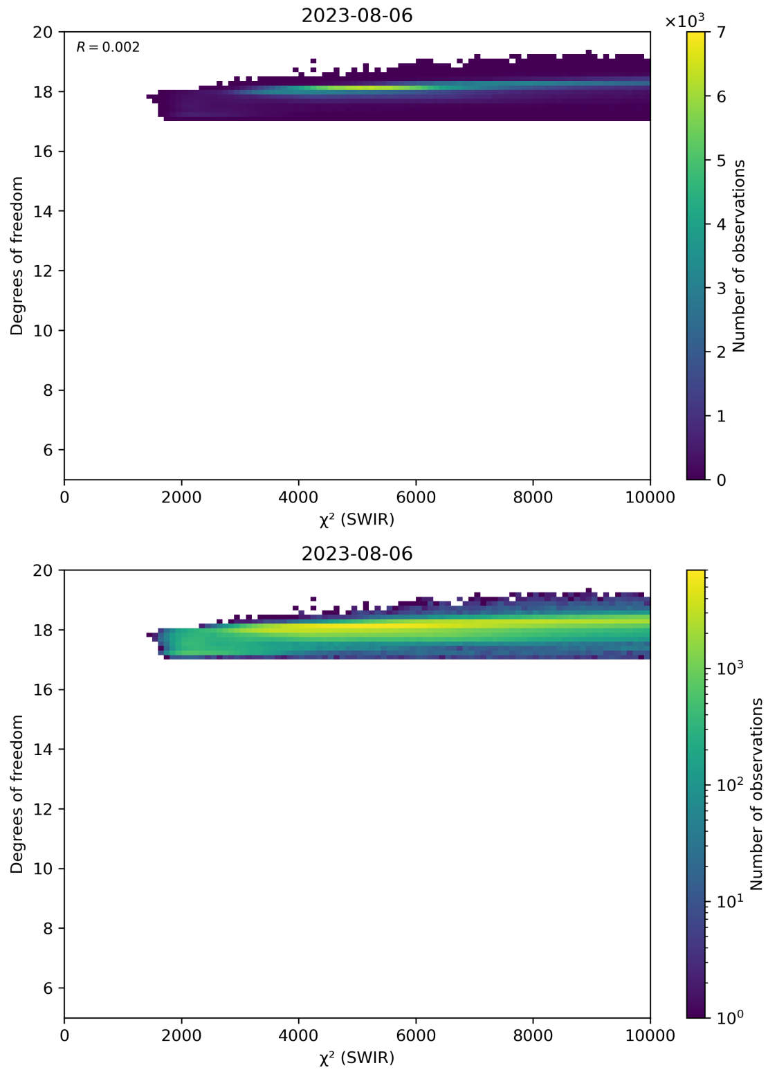
Figure 48: Scatter density plot of “ \chi^2 (SWIR)” against “Degrees of freedom” for 2023-08-05 to 2023-08-07.
