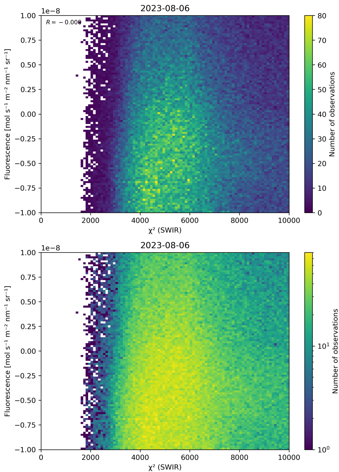
Figure 49: Scatter density plot of “ \chi^2 (SWIR)” against “Fluorescence” for 2023-08-05 to 2023-08-07.
