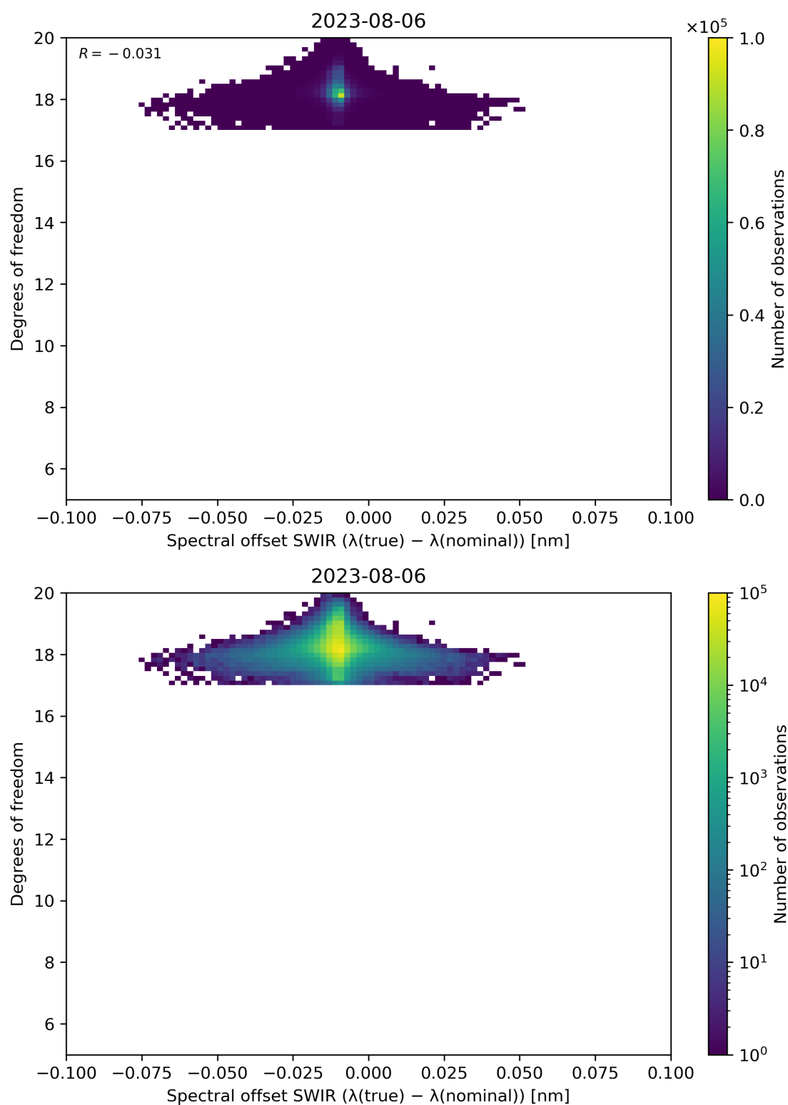
Figure 119: Scatter density plot of “Spectral offset SWIR ( \lambda(\text{true}) - \lambda(\text{nominal}) )” against “Degrees of freedom” for 2023-08-05 to 2023-08-07.
