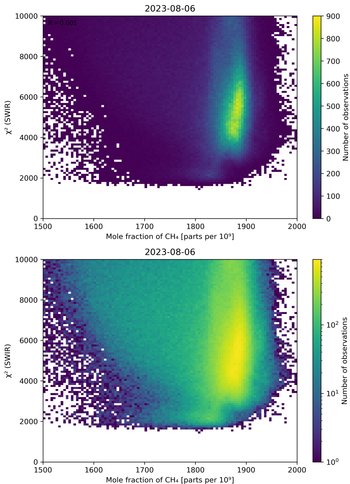
Figure 71: Scatter density plot of “Mole fraction of \text{CH}_4 ” against “ \chi^2 (SWIR)” for 2023-08-05 to 2023-08-07.
