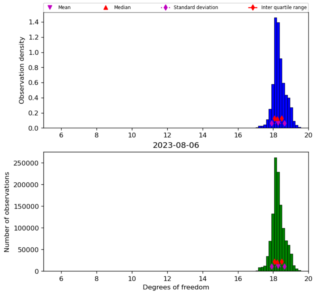
Figure 30: Histogram of “Degrees of freedom” for 2023-08-05 to 2023-08-07
