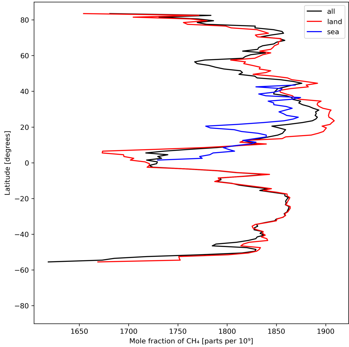
Figure 12: Zonal average of “Mole fraction of \text{CH}_4 ” for 2023-08-05 to 2023-08-07.
