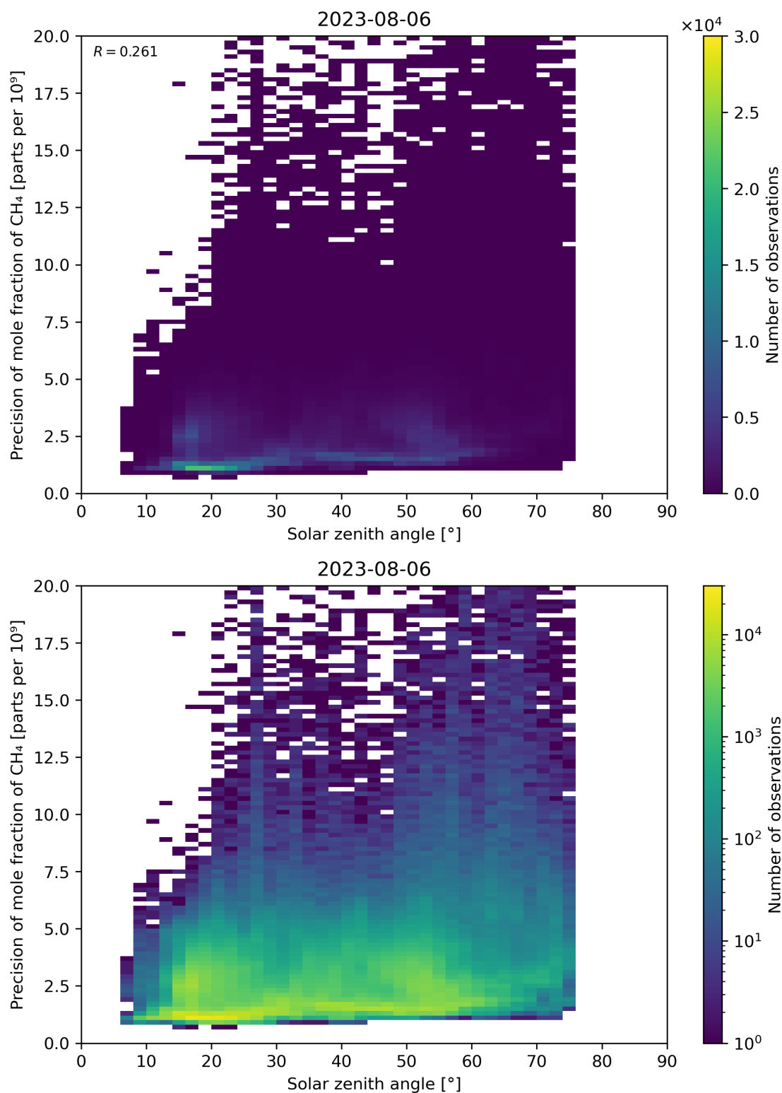
Figure 101: Scatter density plot of “Solar zenith angle” against “Precision of mole fraction of CH 4 ” for 2023-08-05 to 2023-08-07.
