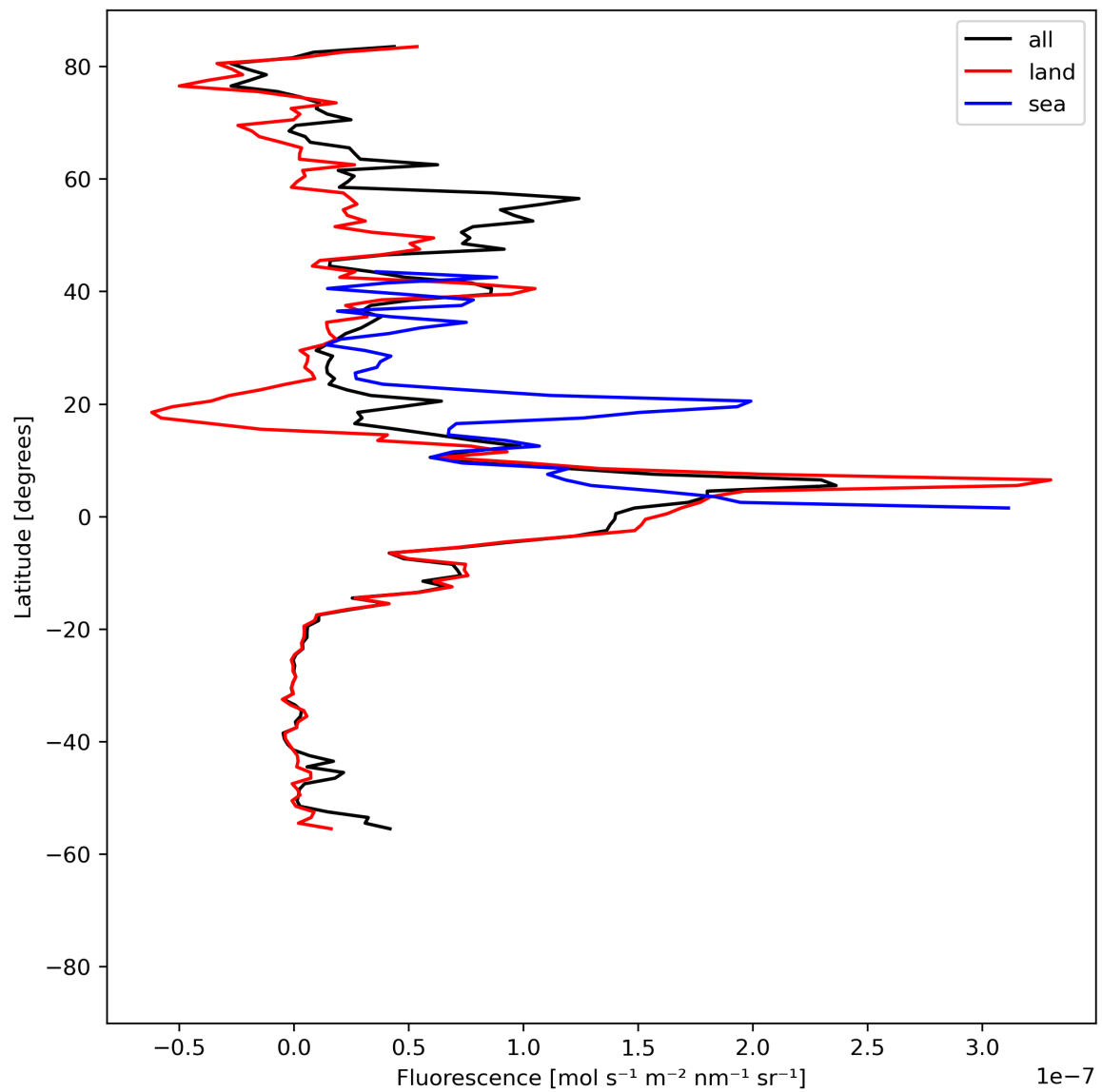
Figure 21: Zonal average of “Fluorescence” for 2023-08-05 to 2023-08-07.
