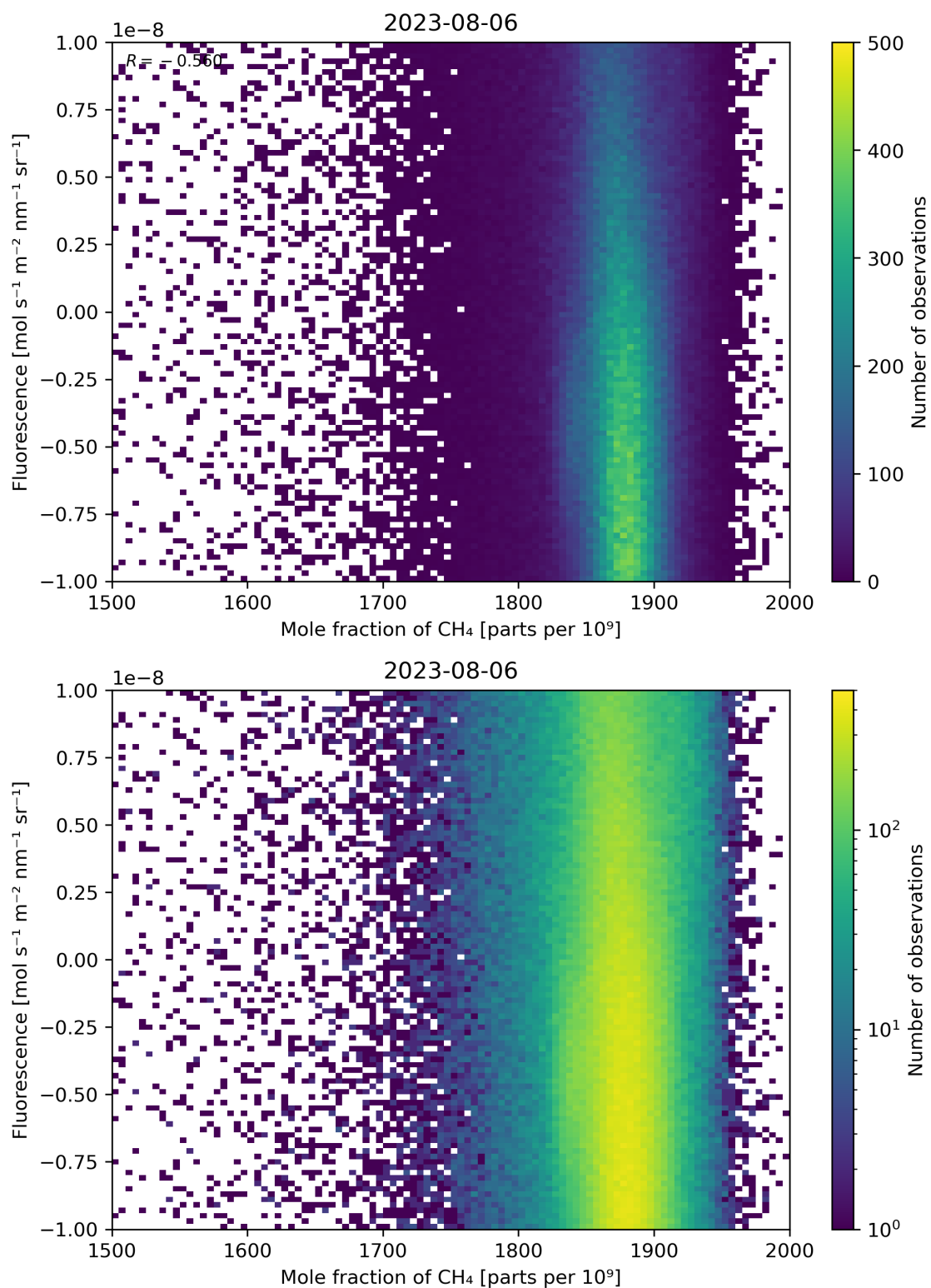
Figure 73: Scatter density plot of “Mole fraction of \text{CH}_4 ” against “Fluorescence” for 2023-08-05 to 2023-08-07.
