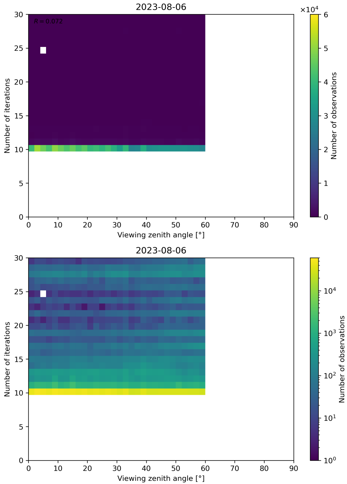
Figure 113: Scatter density plot of “Viewing zenith angle” against “Number of iterations” for 2023-08-05 to 2023-08-07.
