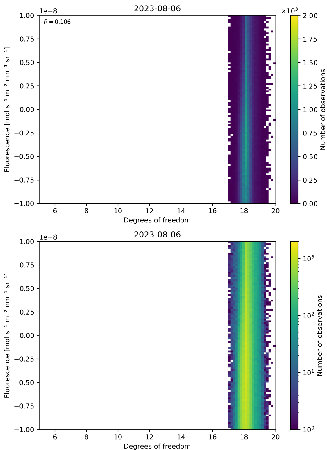
Figure 51: Scatter density plot of “Degrees of freedom” against “Fluorescence” for 2023-08-05 to 2023-08-07.
