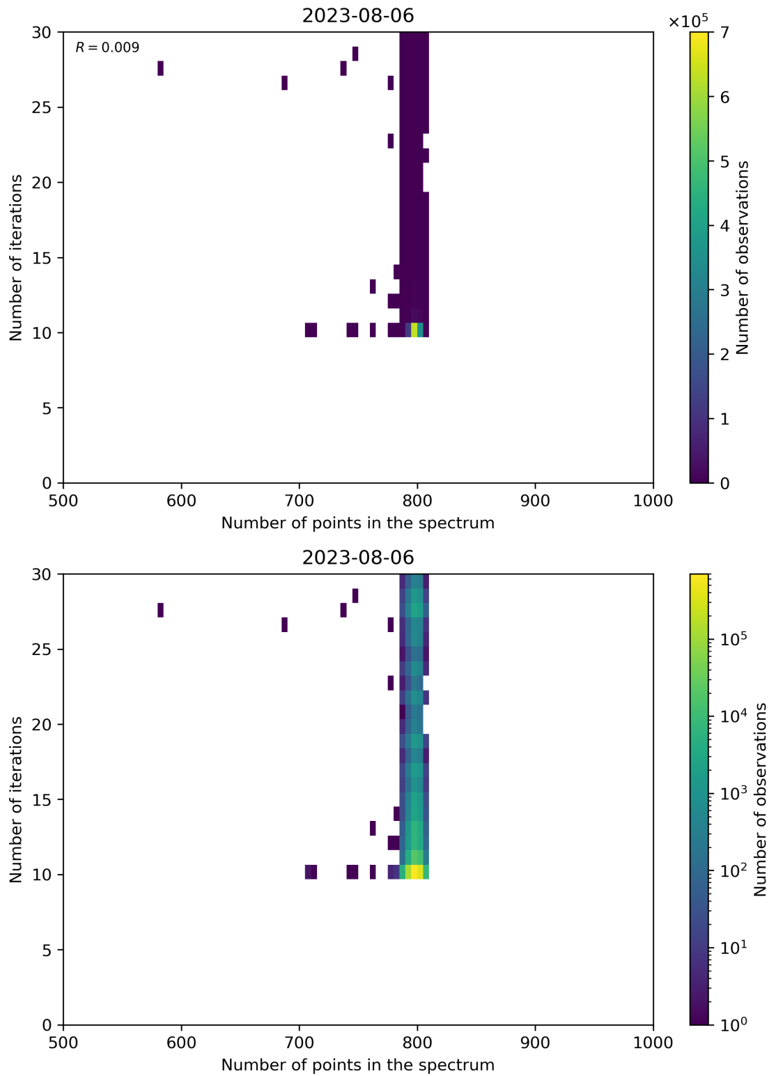
Figure 92: Scatter density plot of “Number of points in the spectrum” against “Number of iterations” for 2023-08-05 to 2023-08-07.
