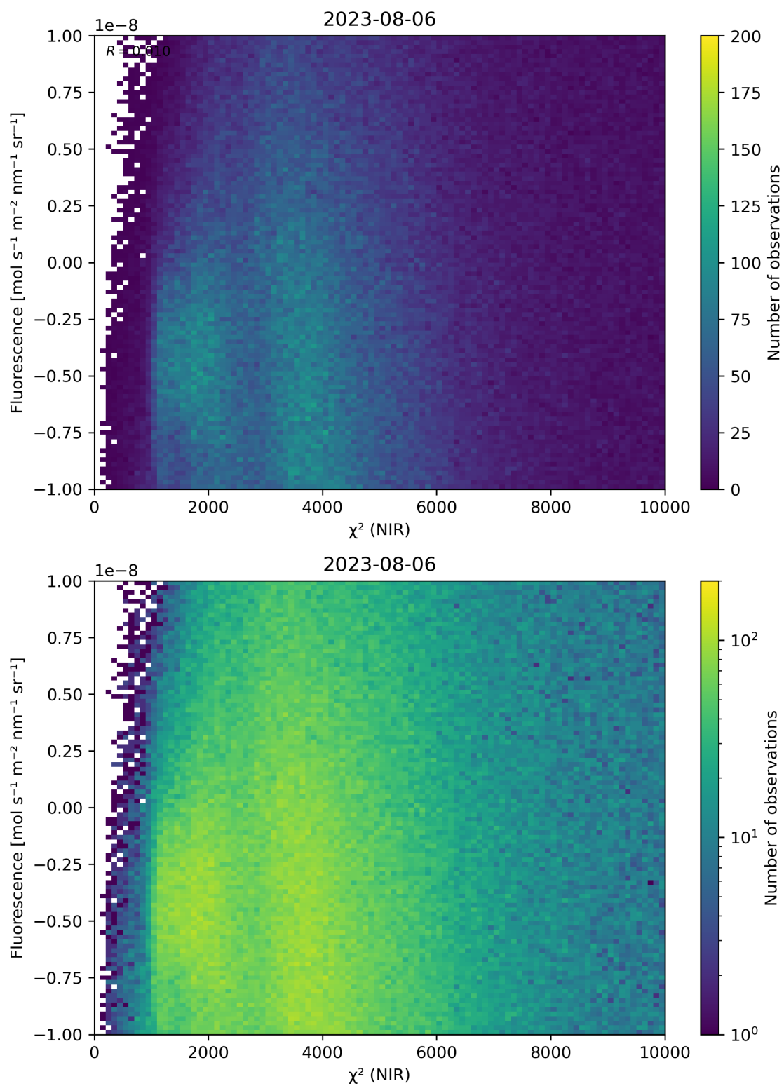
Figure 45: Scatter density plot of “ \chi^2 (NIR)” against “Fluorescence” for 2023-08-05 to 2023-08-07.
