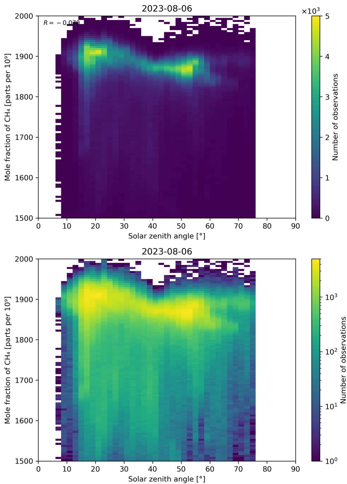
Figure 99: Scatter density plot of “Solar zenith angle” against “Mole fraction of CH 4 ” for 2023-08-05 to 2023-08-07.
