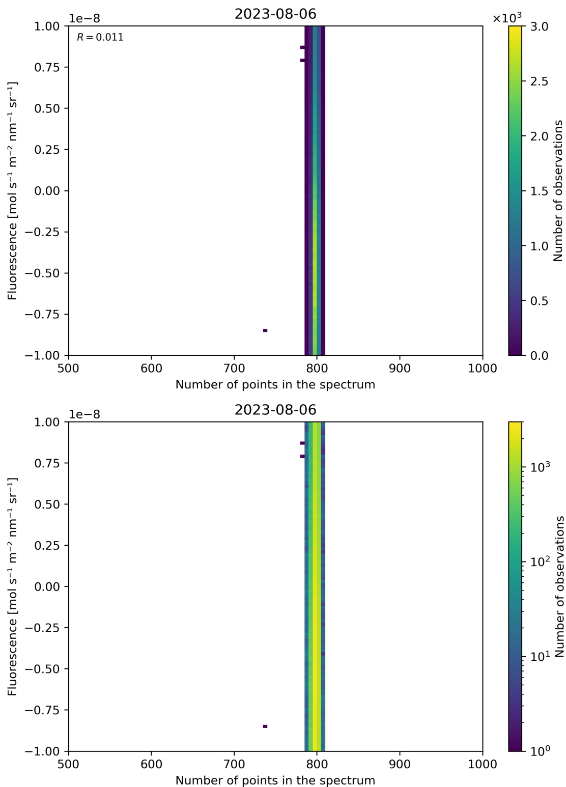
Figure 91: Scatter density plot of “Number of points in the spectrum” against “Fluorescence” for 2023-08-05 to 2023-08-07.
