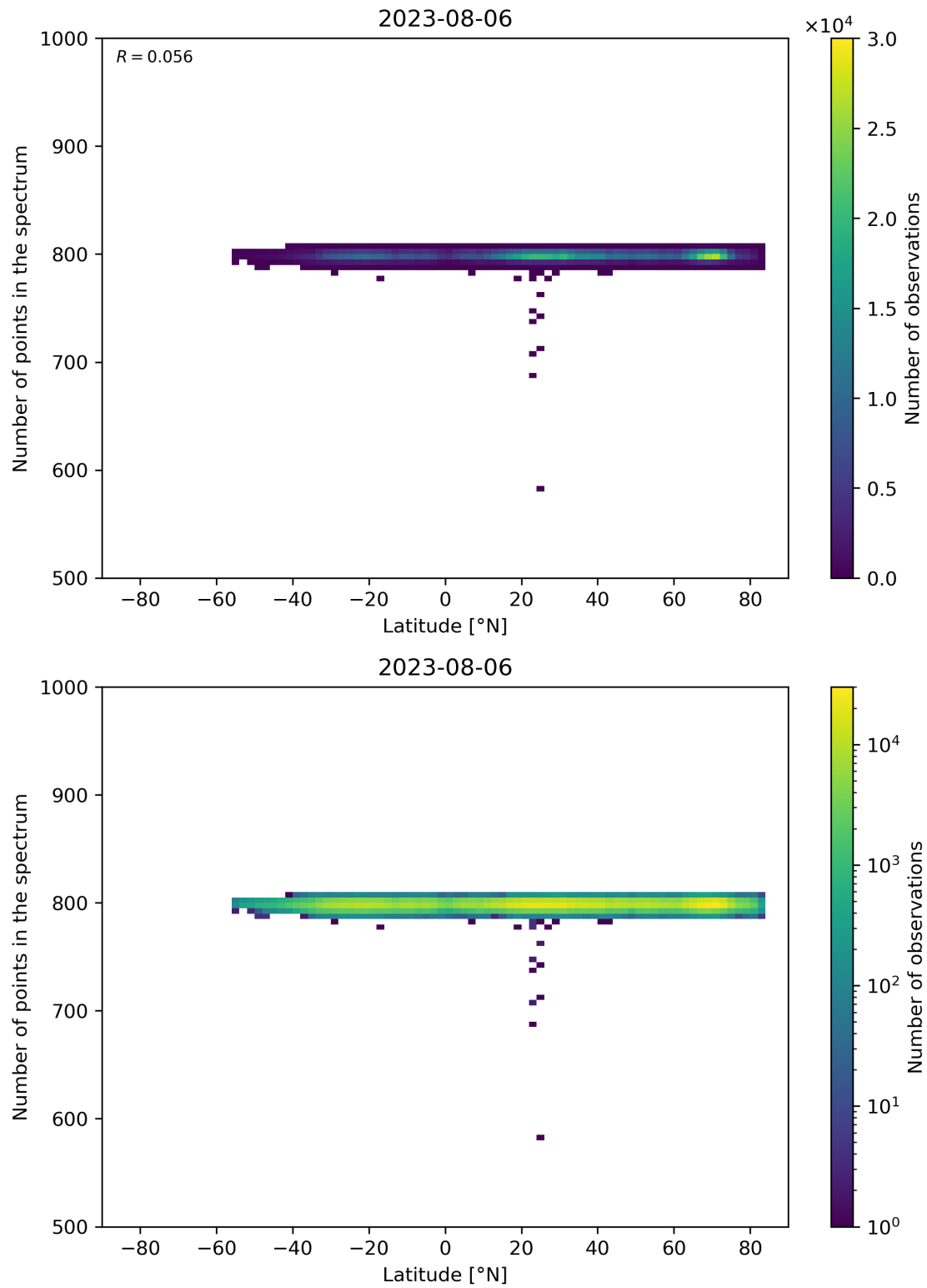
Figure 61: Scatter density plot of “Latitude” against “Number of points in the spectrum” for 2023-08-05 to 2023-08-07.
