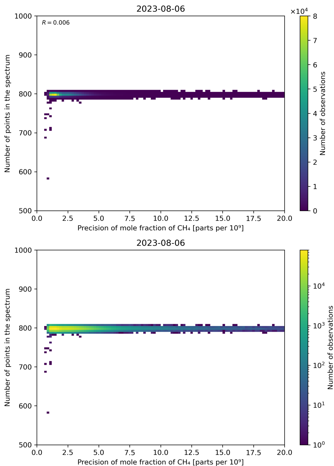
Figure 84: Scatter density plot of “Precision of mole fraction of CH 4 ” against “Number of points in the spectrum” for 2023-08-05 to 2023-08-07.
