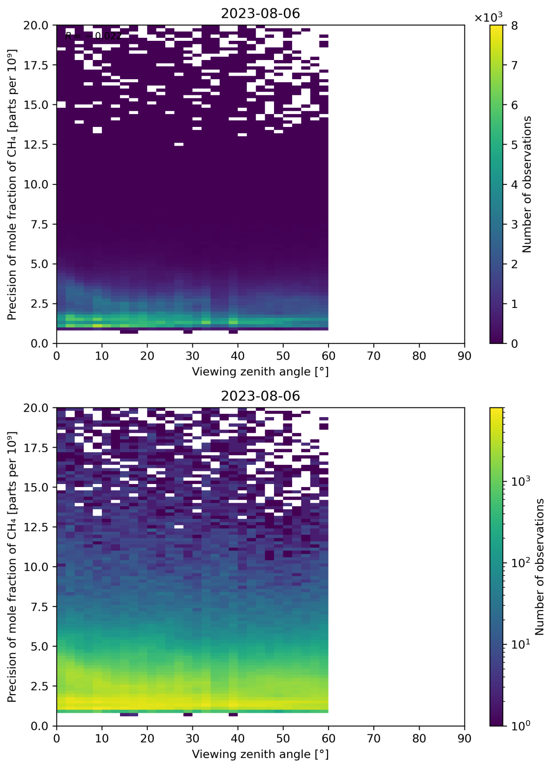
Figure 112: Scatter density plot of “Viewing zenith angle” against “Precision of mole fraction of CH 4 ” for 2023-08-05 to 2023-08-07.
