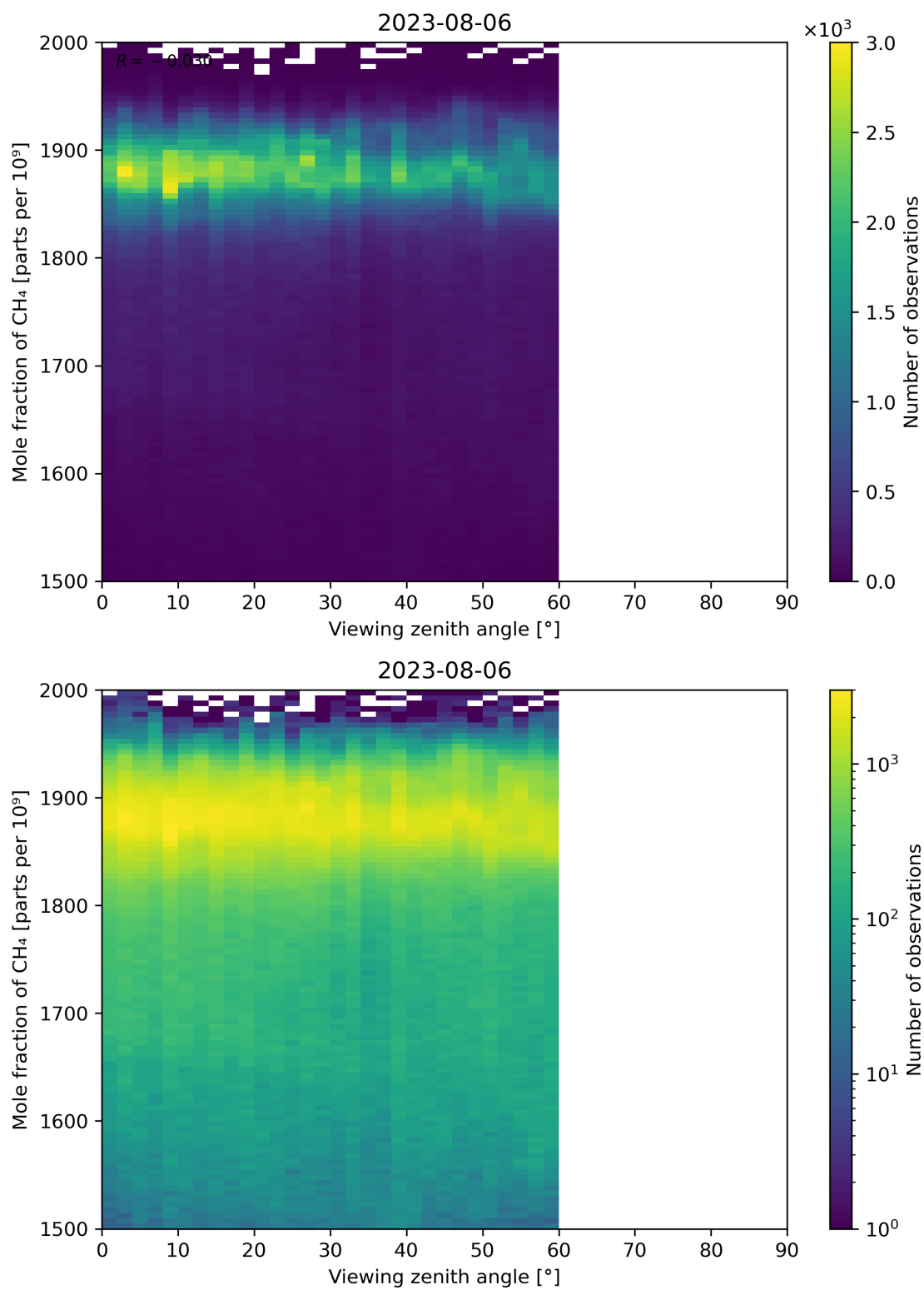
Figure 110: Scatter density plot of “Viewing zenith angle” against “Mole fraction of CH 4 ” for 2023-08-05 to 2023-08-07.
