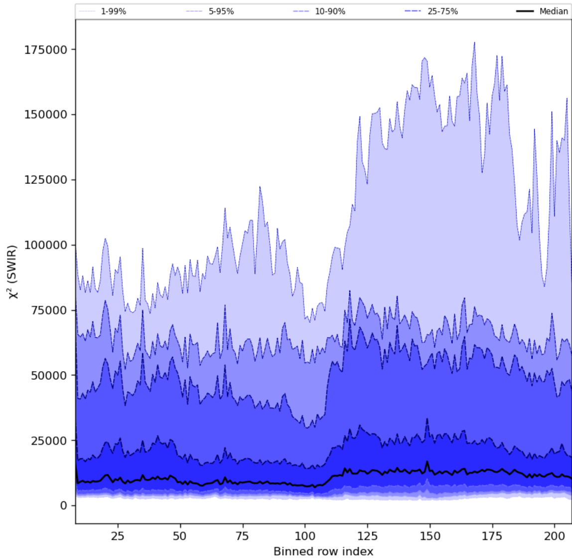
Figure 39: Along track statistics of “ \chi^2 (SWIR)” for 2023-08-05 to 2023-08-07
