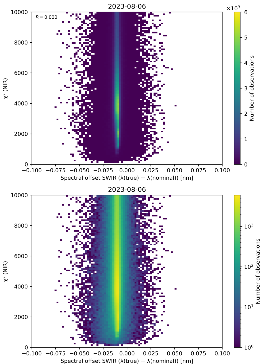
Figure 117: Scatter density plot of “Spectral offset SWIR ( \lambda(\text{true}) - \lambda(\text{nominal}) )” against “ \chi^2 (NIR)” for 2023-08-05 to 2023-08-07.
