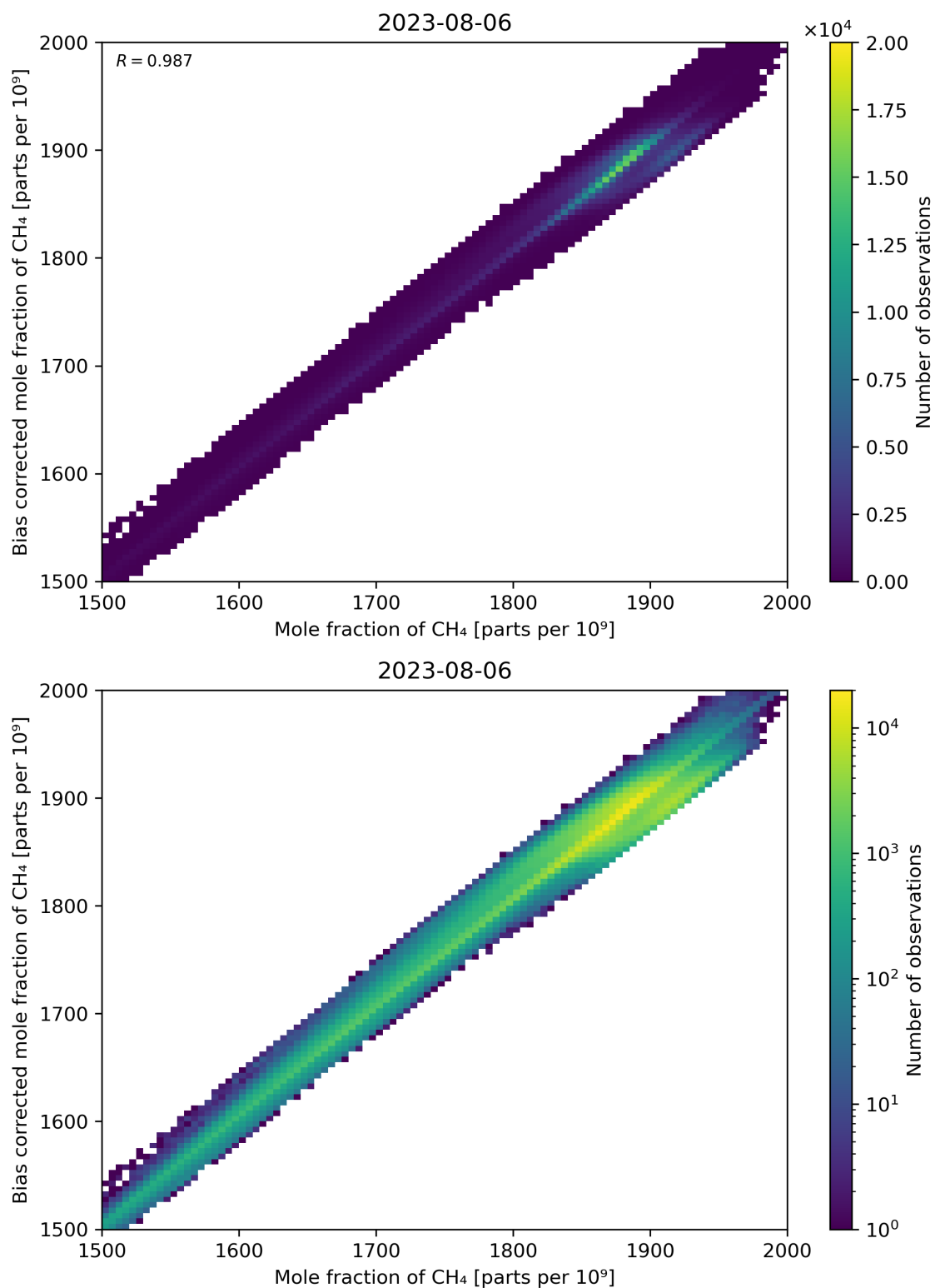
Figure 74: Scatter density plot of “Mole fraction of CH 4 ” against “Bias corrected mole fraction of CH 4 ” for 2023-08-05 to 2023-08-07.
