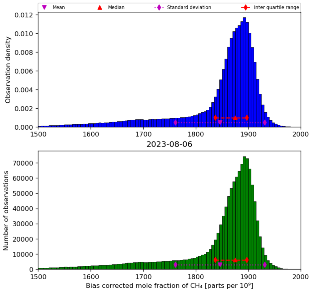
Figure 25: Histogram of “Bias corrected mole fraction of CH 4 ” for 2023-08-05 to 2023-08-07
