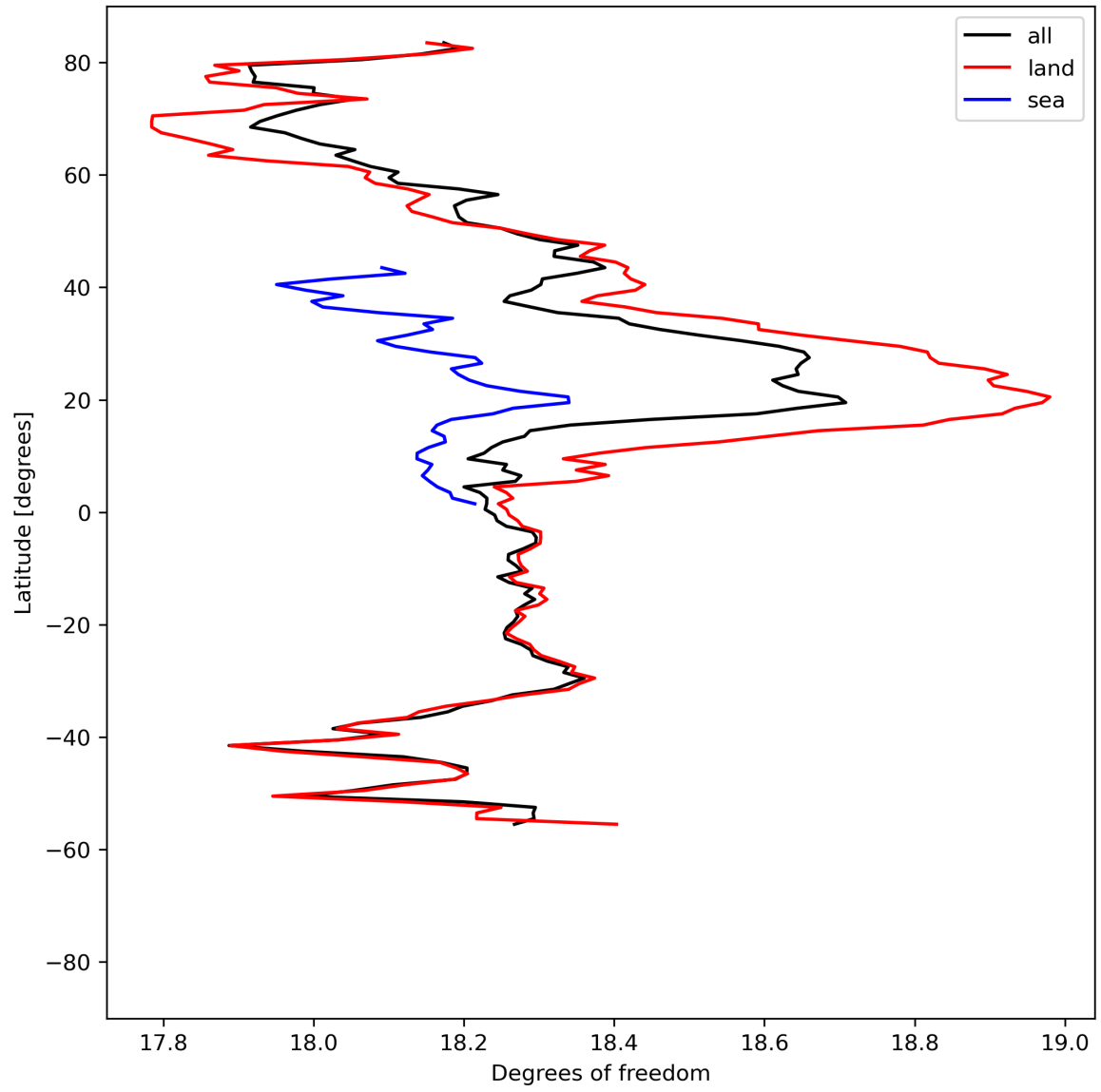
Figure 19: Zonal average of “Degrees of freedom” for 2023-08-05 to 2023-08-07.
