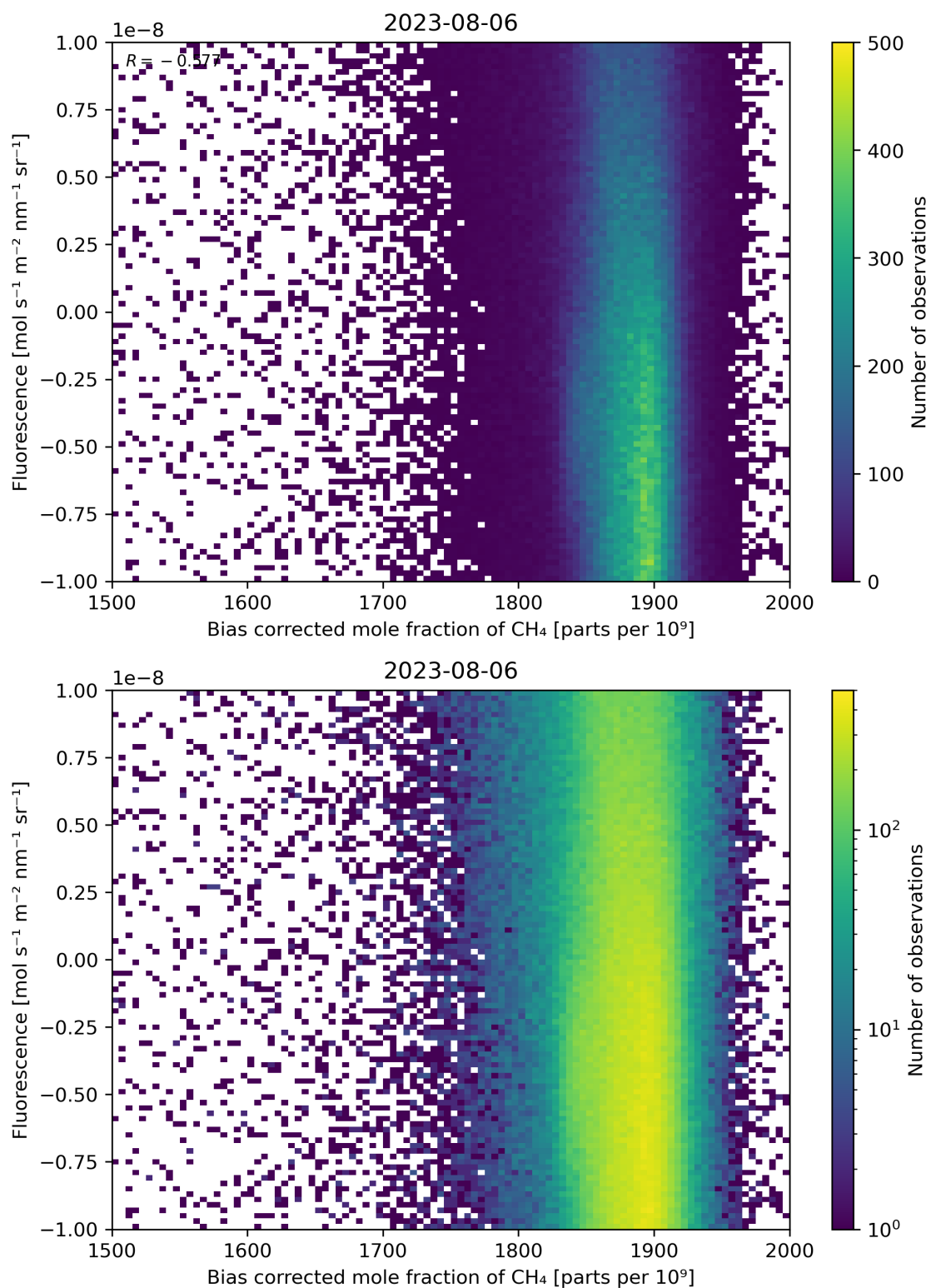
Figure 66: Scatter density plot of “Bias corrected mole fraction of \text{CH}_4 ” against “Fluorescence” for 2023-08-05 to 2023-08-07.
