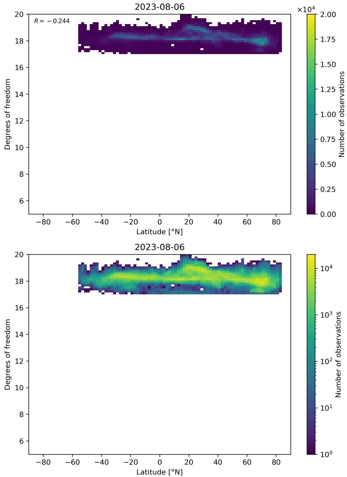
Figure 55: Scatter density plot of “Latitude” against “Degrees of freedom” for 2023-08-05 to 2023-08-07.
