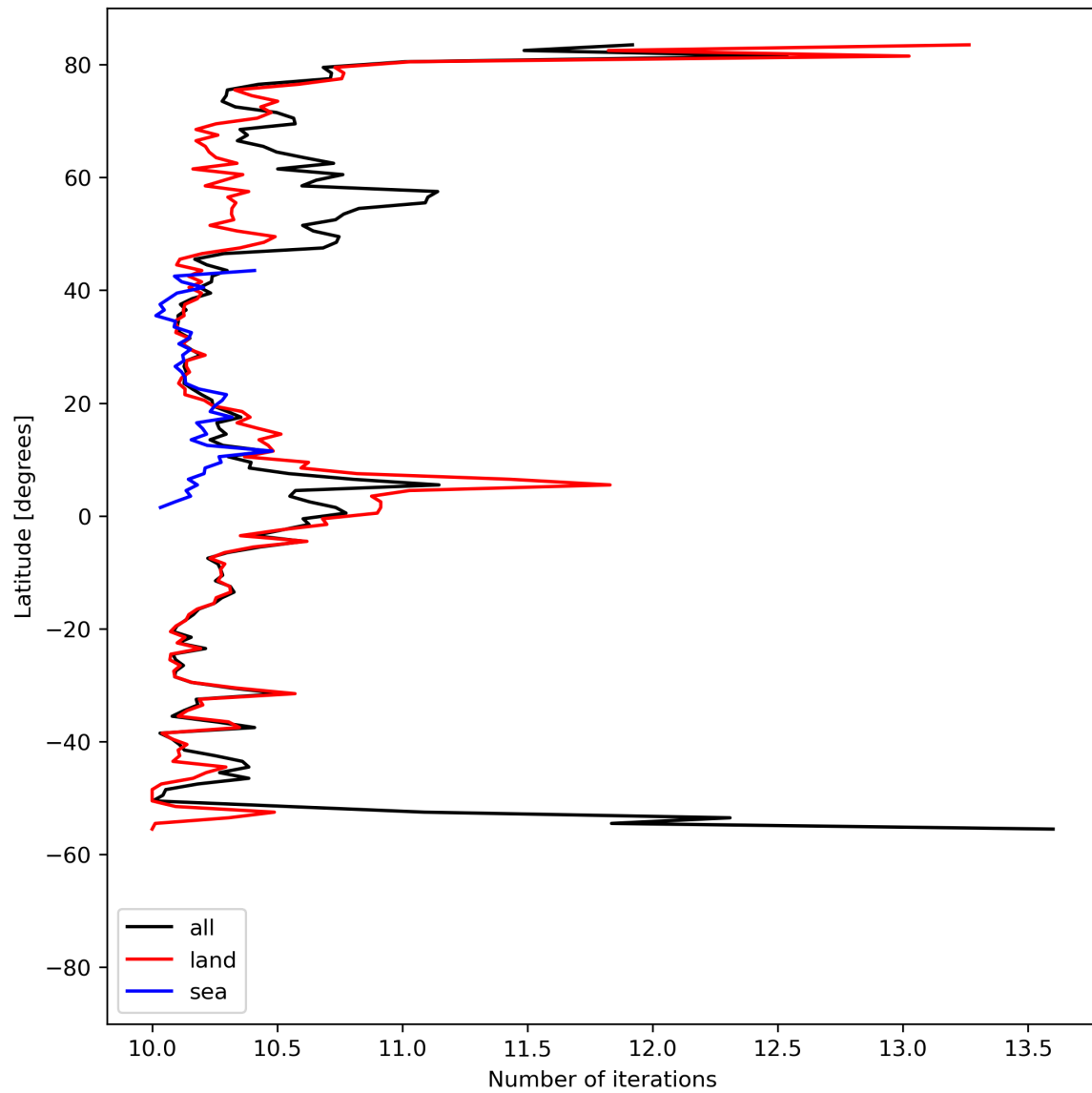
Figure 20: Zonal average of “Number of iterations” for 2023-08-05 to 2023-08-07.
