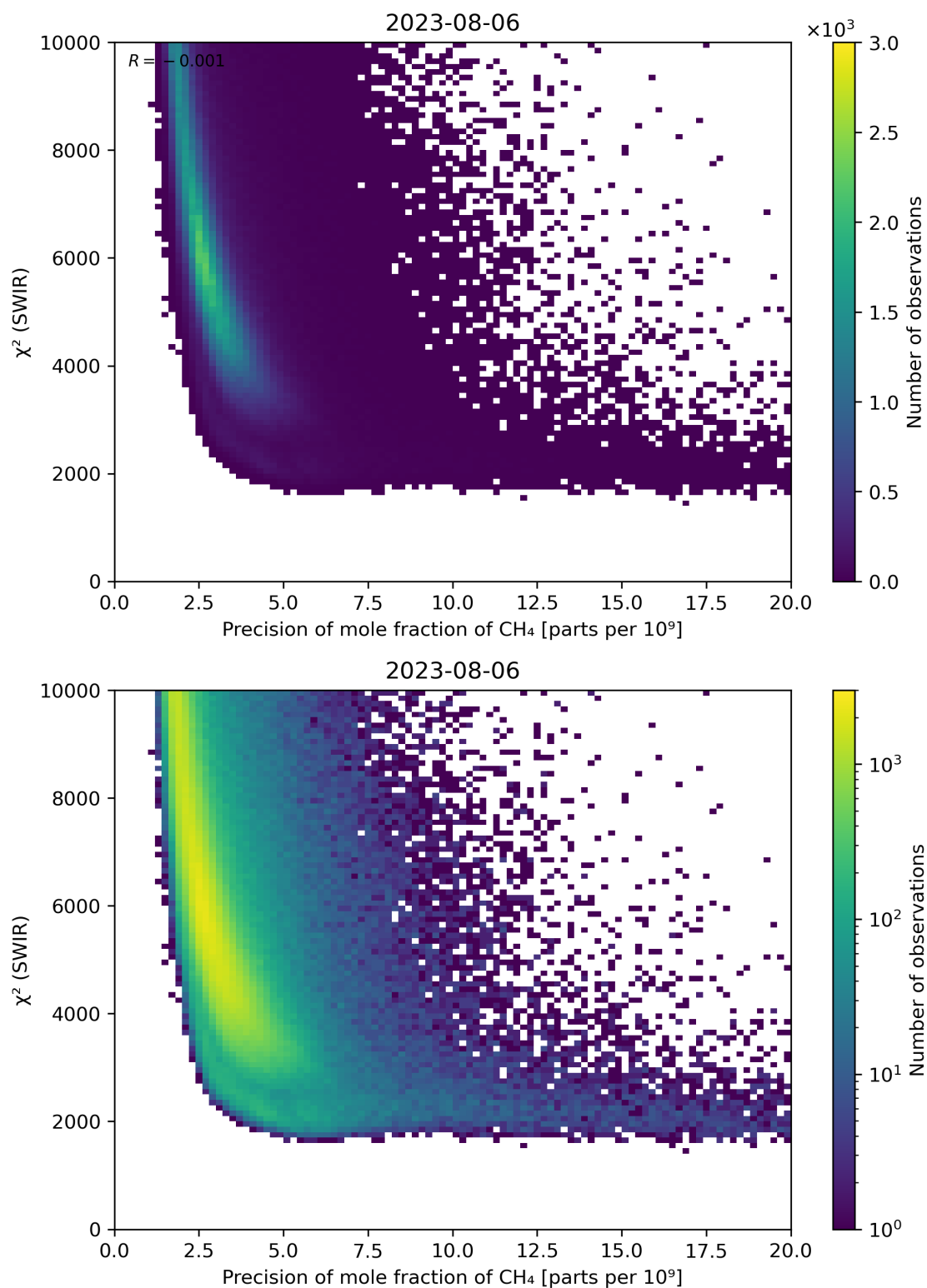
Figure 79: Scatter density plot of “Precision of mole fraction of CH 4 ” against “ \chi^2 (SWIR)” for 2023-08-05 to 2023-08-07.
