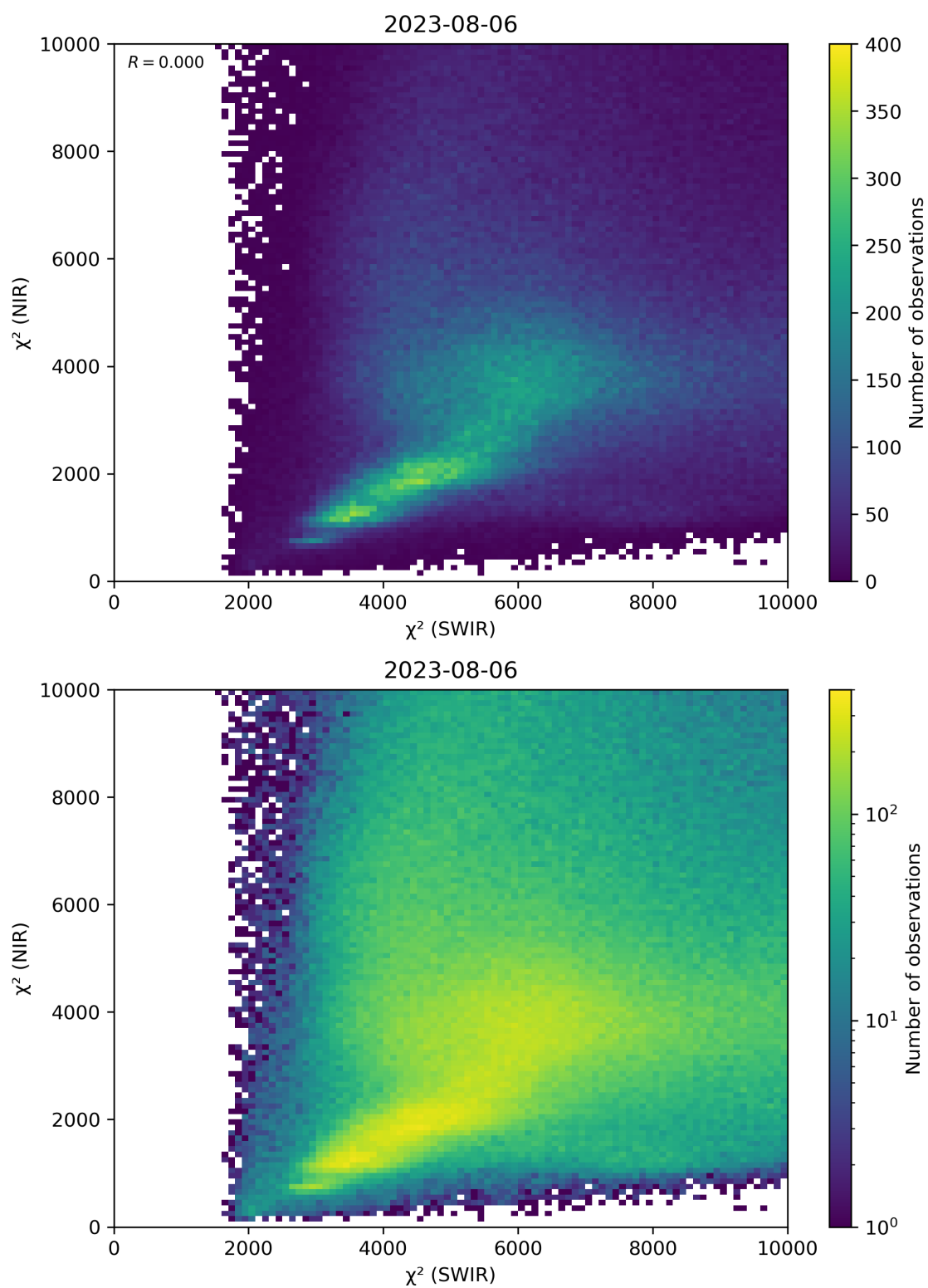
Figure 47: Scatter density plot of “ \chi^2 (SWIR)” against “ \chi^2 (NIR)” for 2023-08-05 to 2023-08-07.
