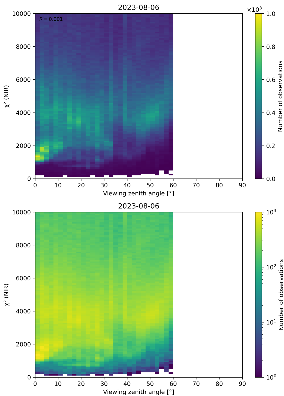
Figure 105: Scatter density plot of “Viewing zenith angle” against “ \chi^2 (NIR)” for 2023-08-05 to 2023-08-07.
