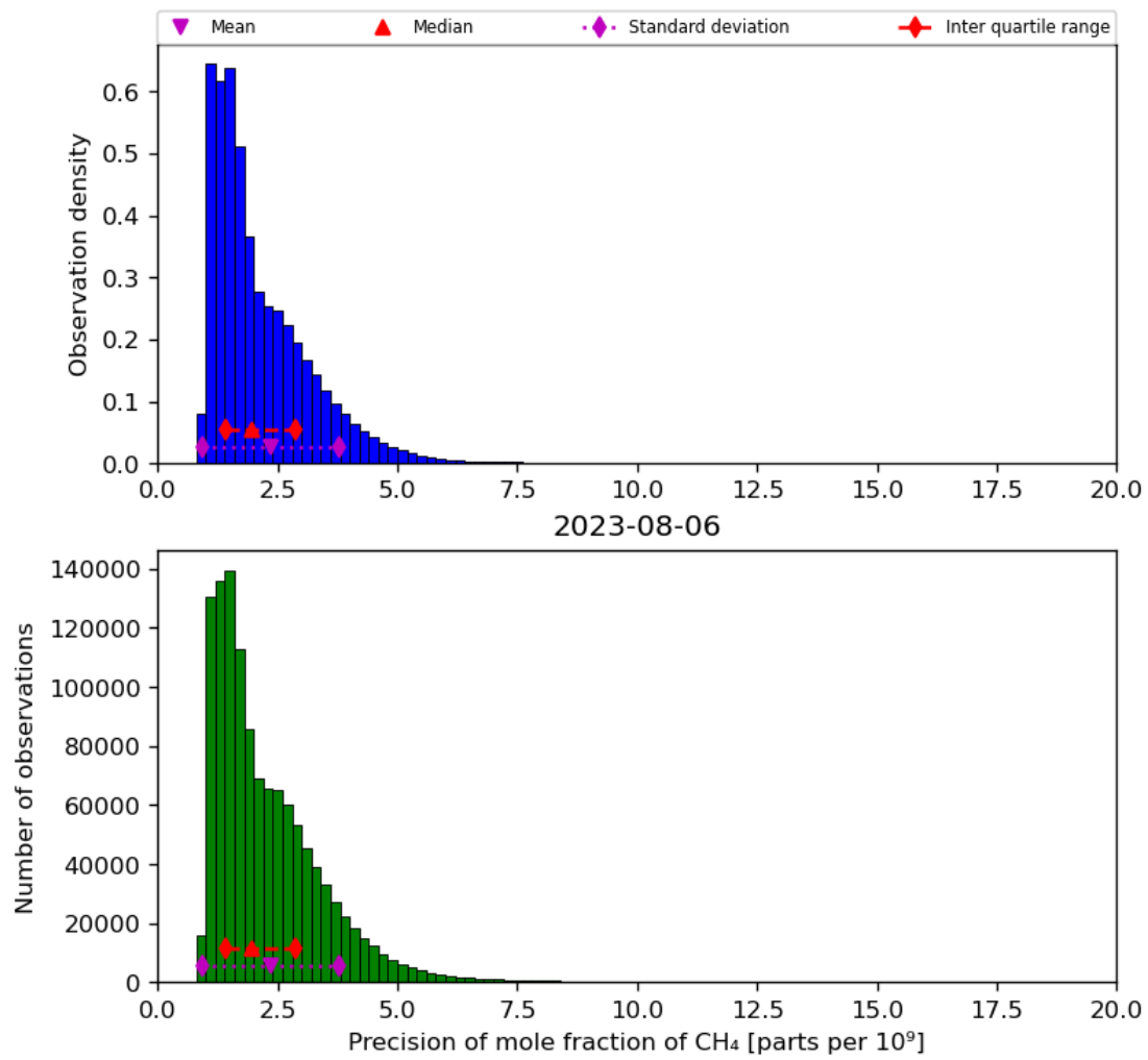
Figure 24: Histogram of “Precision of mole fraction of CH 4 ” for 2023-08-05 to 2023-08-07
