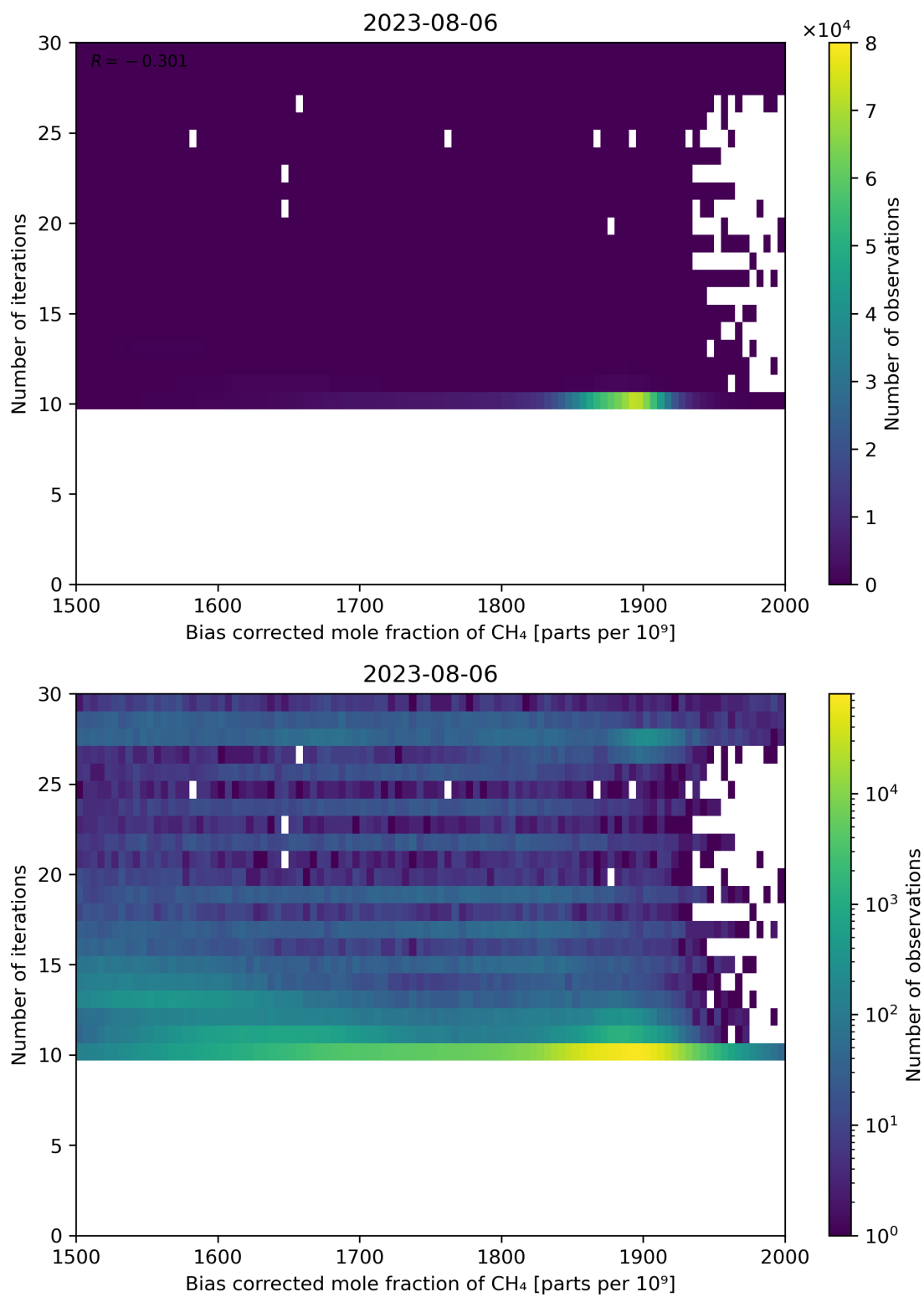
Figure 67: Scatter density plot of “Bias corrected mole fraction of CH 4 ” against “Number of iterations” for 2023-08-05 to 2023-08-07.
