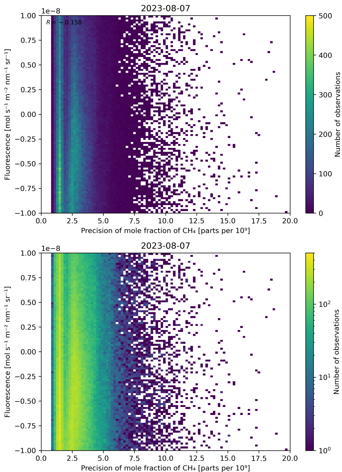
Figure 81: Scatter density plot of “Precision of mole fraction of \text{CH}_4 ” against “Fluorescence” for 2023-08-06 to 2023-08-08.
