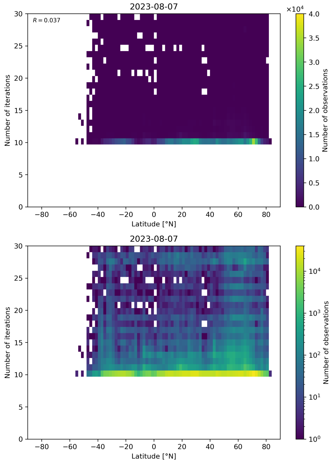
Figure 60: Scatter density plot of “Latitude” against “Number of iterations” for 2023-08-06 to 2023-08-08.
