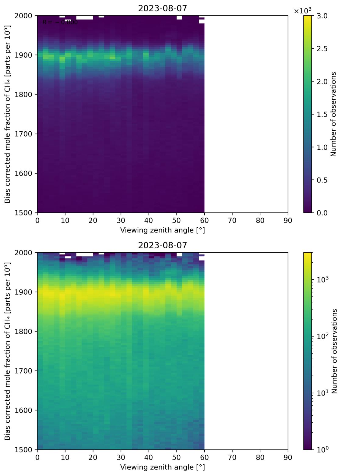
Figure 111: Scatter density plot of “Viewing zenith angle” against “Bias corrected mole fraction of CH 4 ” for 2023-08-06 to 2023-08-08.
