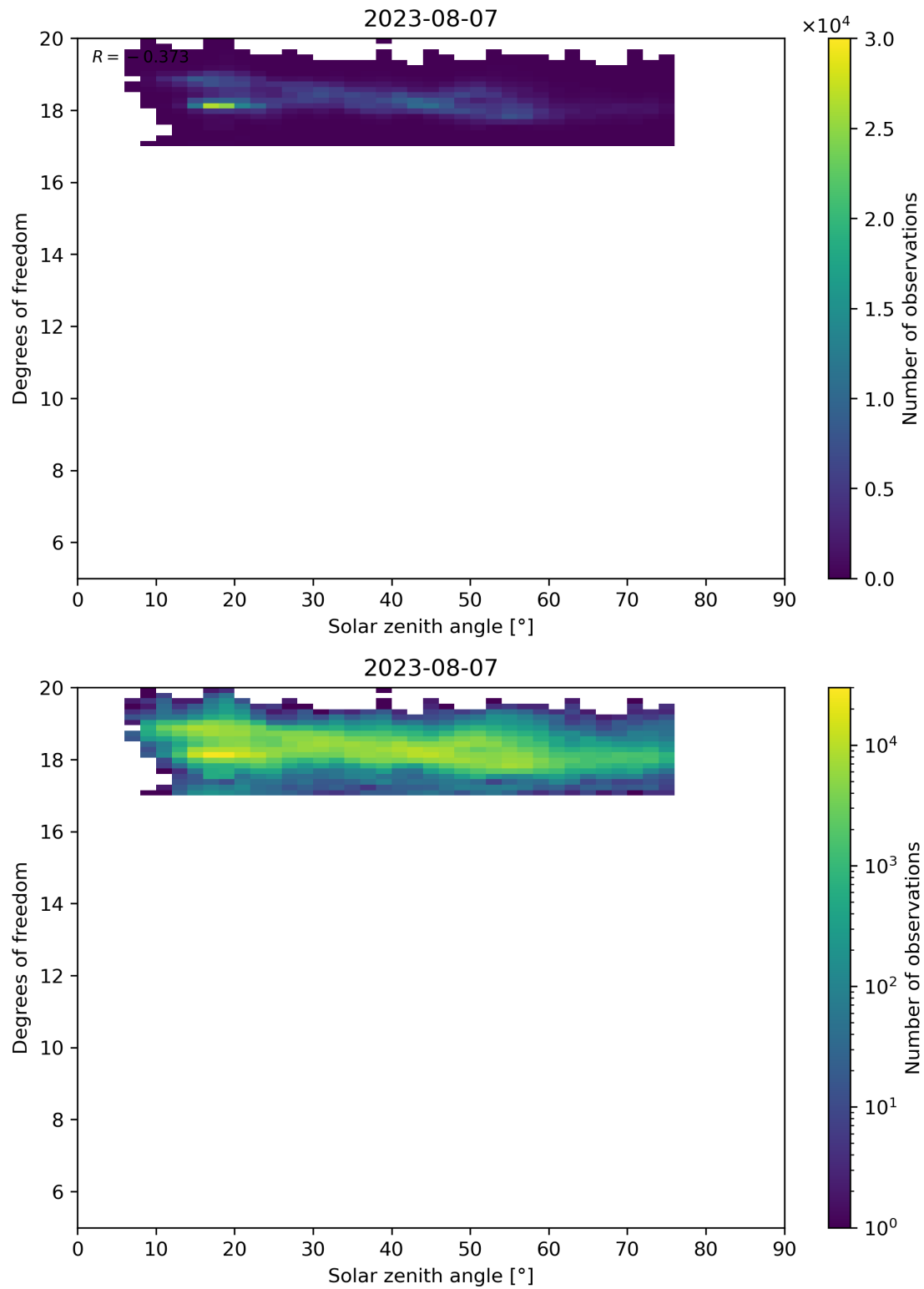
Figure 96: Scatter density plot of “Solar zenith angle” against “Degrees of freedom” for 2023-08-06 to 2023-08-08.
