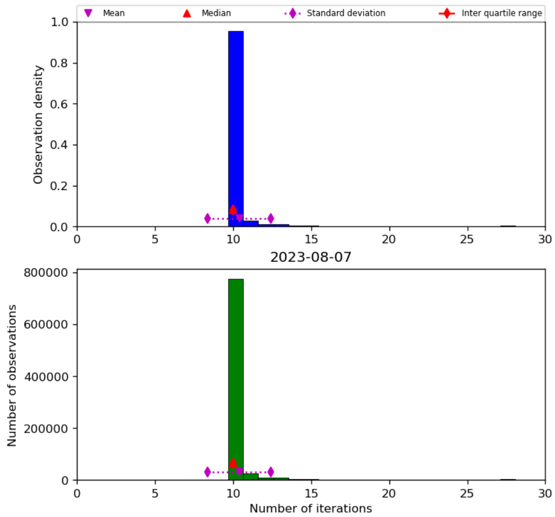
Figure 31: Histogram of “Number of iterations” for 2023-08-06 to 2023-08-08
