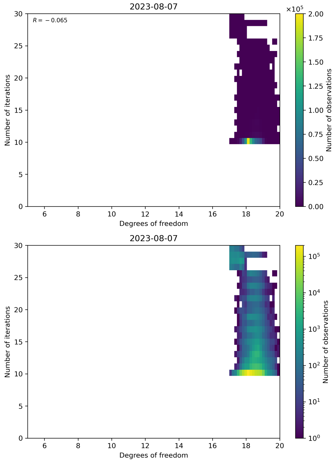
Figure 52: Scatter density plot of “Degrees of freedom” against “Number of iterations” for 2023-08-06 to 2023-08-08.
