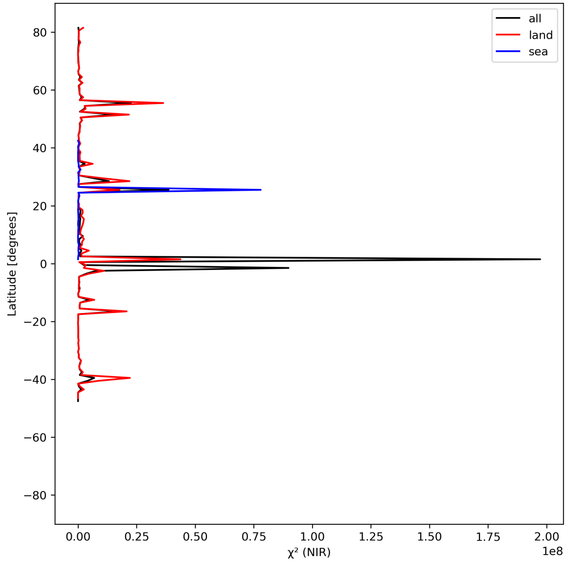
Figure 18: Zonal average of “ \chi^2 (NIR)” for 2023-08-06 to 2023-08-08.
