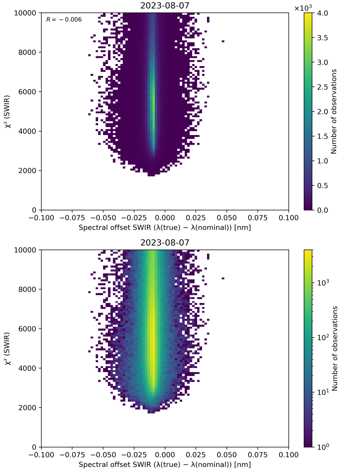
Figure 118: Scatter density plot of “Spectral offset SWIR ( \lambda(\text{true}) - \lambda(\text{nominal}) )” against “ \chi^2 (SWIR)” for 2023-08-06 to 2023-08-08.
