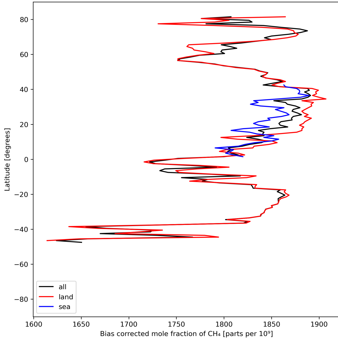
Figure 14: Zonal average of “Bias corrected mole fraction of CH 4 ” for 2023-08-06 to 2023-08-08.
