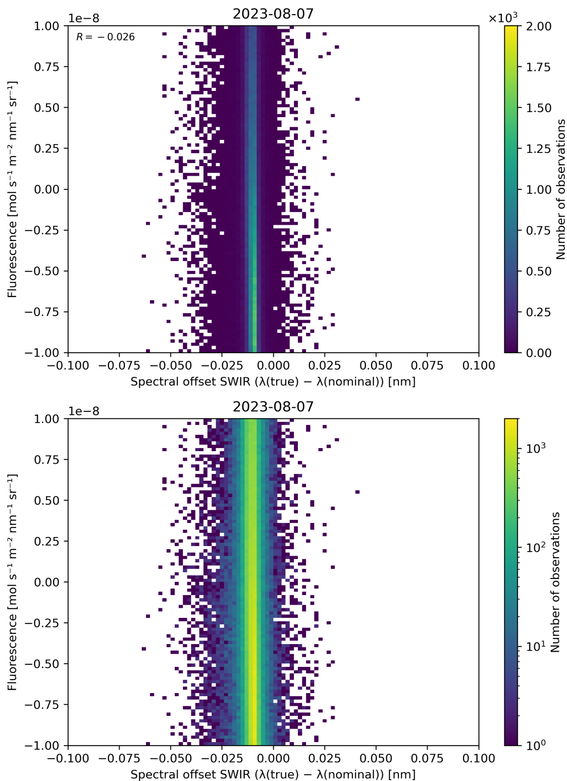
Figure 120: Scatter density plot of “Spectral offset SWIR ( \lambda(\text{true}) - \lambda(\text{nominal}) )” against “Fluorescence” for 2023-08-06 to 2023-08-08.
