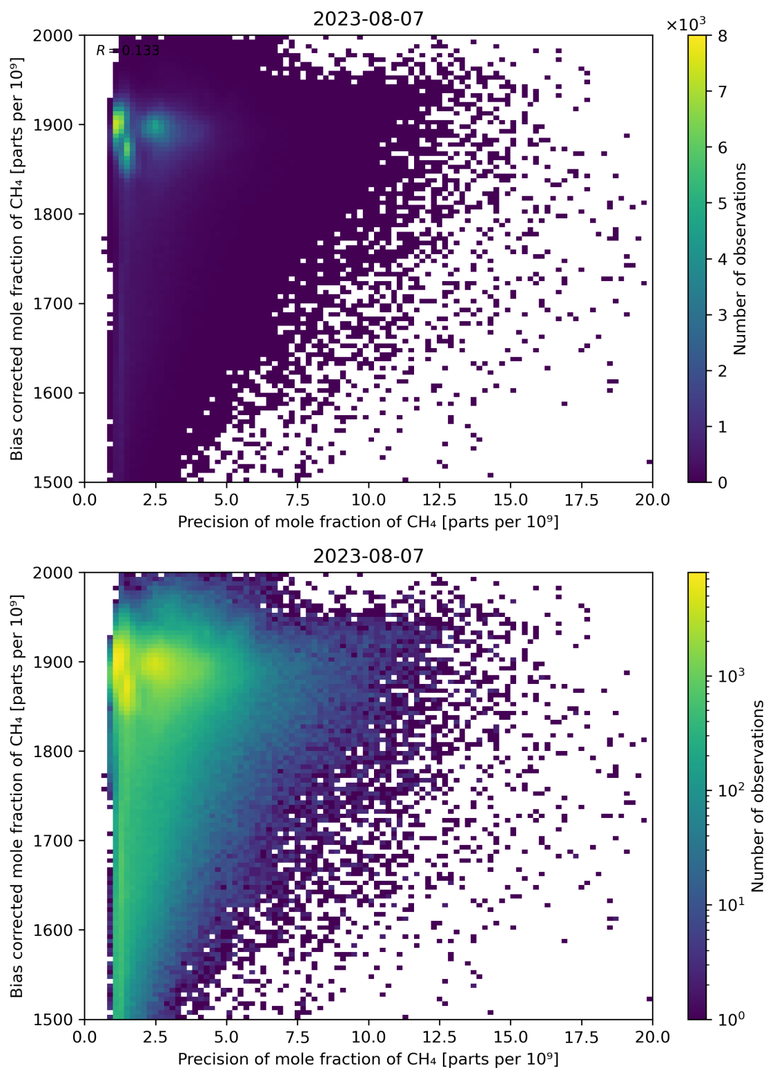
Figure 82: Scatter density plot of “Precision of mole fraction of CH 4 ” against “Bias corrected mole fraction of CH 4 ” for 2023-08-06 to 2023-08-08.
