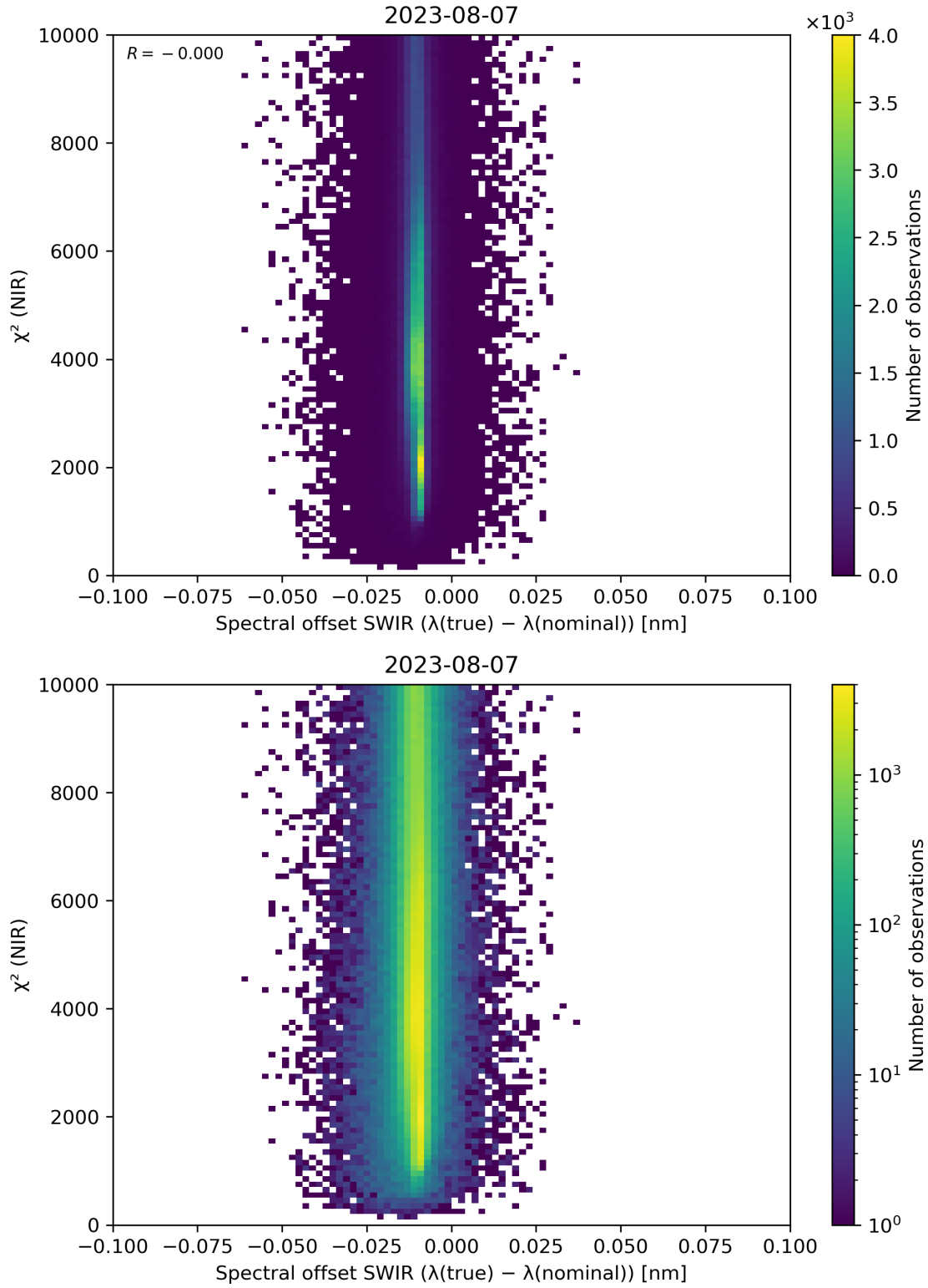
Figure 117: Scatter density plot of “Spectral offset SWIR ( \lambda(\text{true}) - \lambda(\text{nominal}) )” against “ \chi^2 (NIR)” for 2023-08-06 to 2023-08-08.
