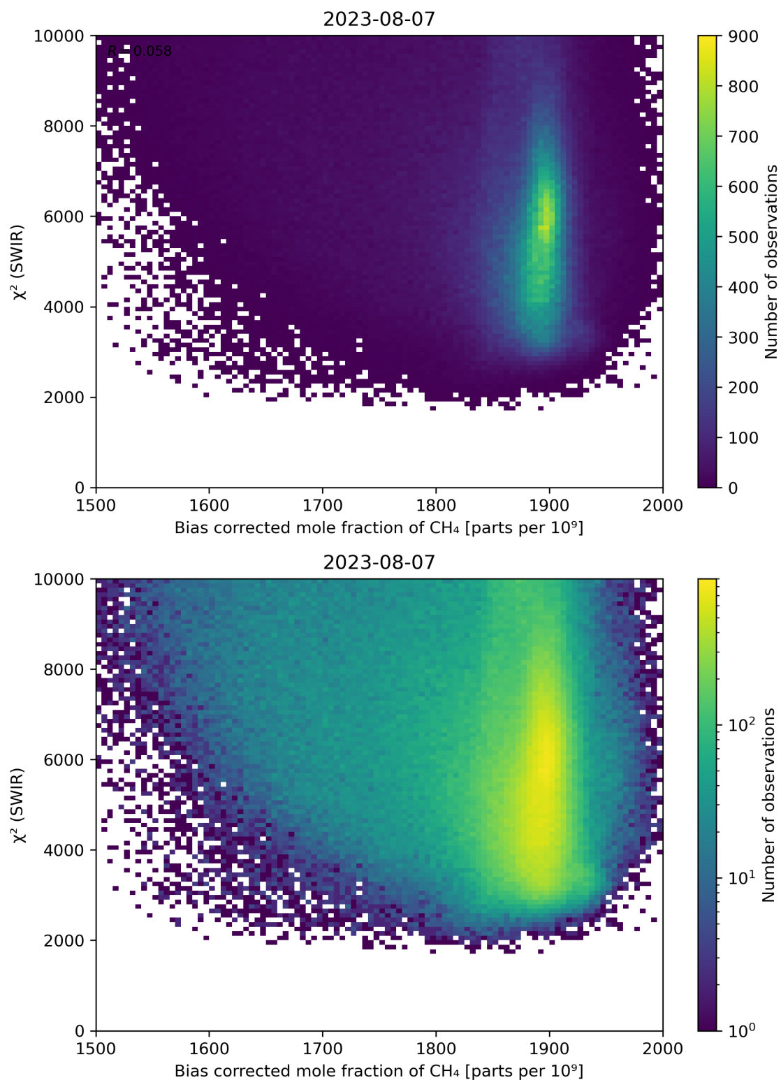
Figure 64: Scatter density plot of “Bias corrected mole fraction of \text{CH}_4 ” against “ \chi^2 (SWIR)” for 2023-08-06 to 2023-08-08.
