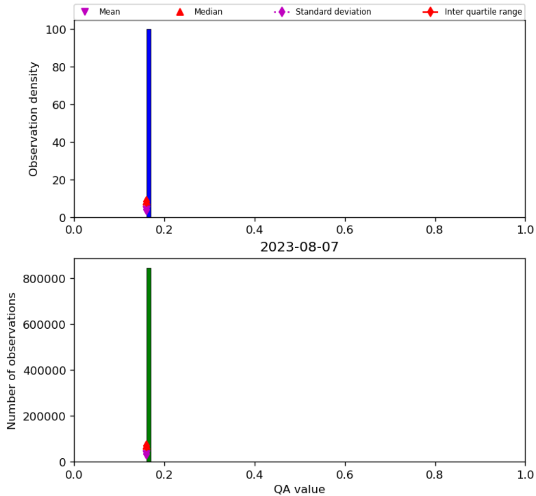
Figure 22: Histogram of “QA value” for 2023-08-06 to 2023-08-08
