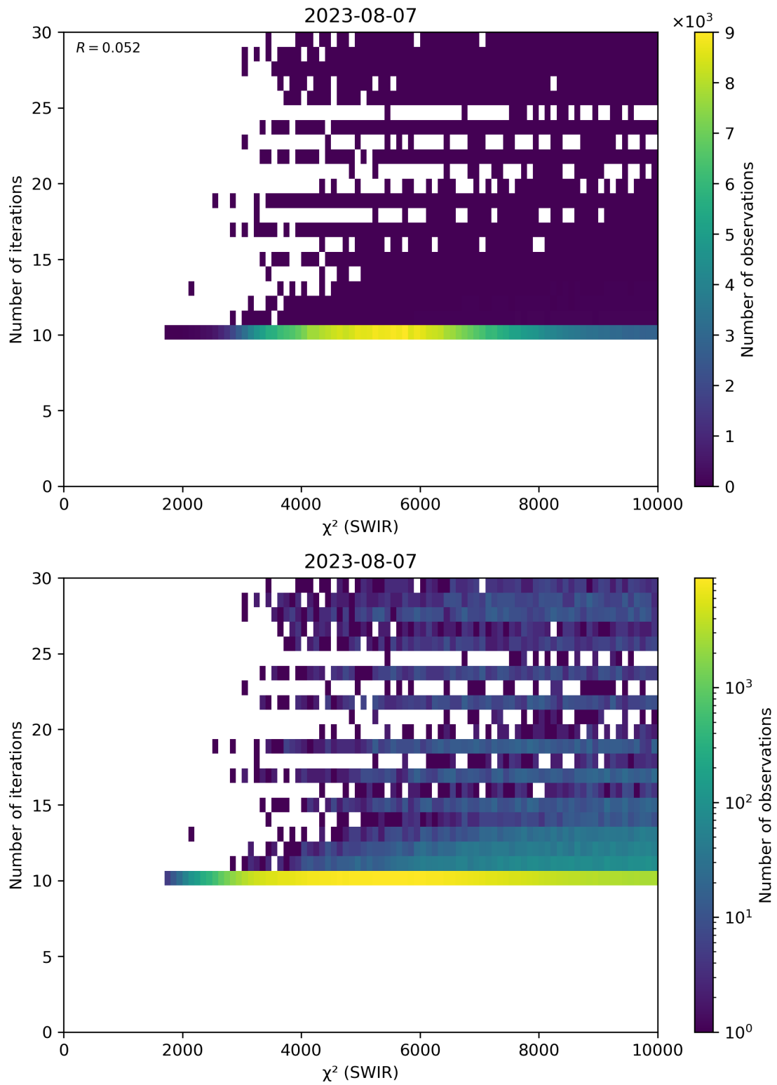
Figure 50: Scatter density plot of “ \chi^2 (SWIR)” against “Number of iterations” for 2023-08-06 to 2023-08-08.
