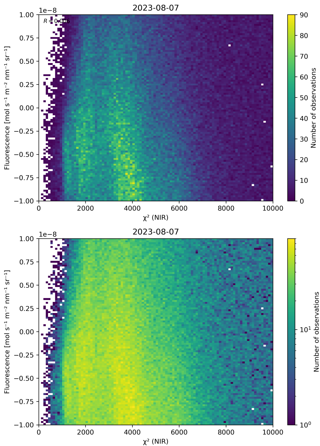
Figure 45: Scatter density plot of “ \chi^2 (NIR)” against “Fluorescence” for 2023-08-06 to 2023-08-08.
