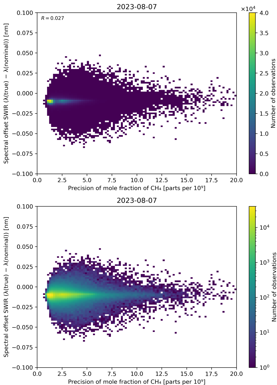
Figure 85: Scatter density plot of “Precision of mole fraction of CH 4 ” against “Spectral offset SWIR ( \lambda(\text{true}) - \lambda(\text{nominal}) )” for 2023-08-06 to 2023-08-08.
