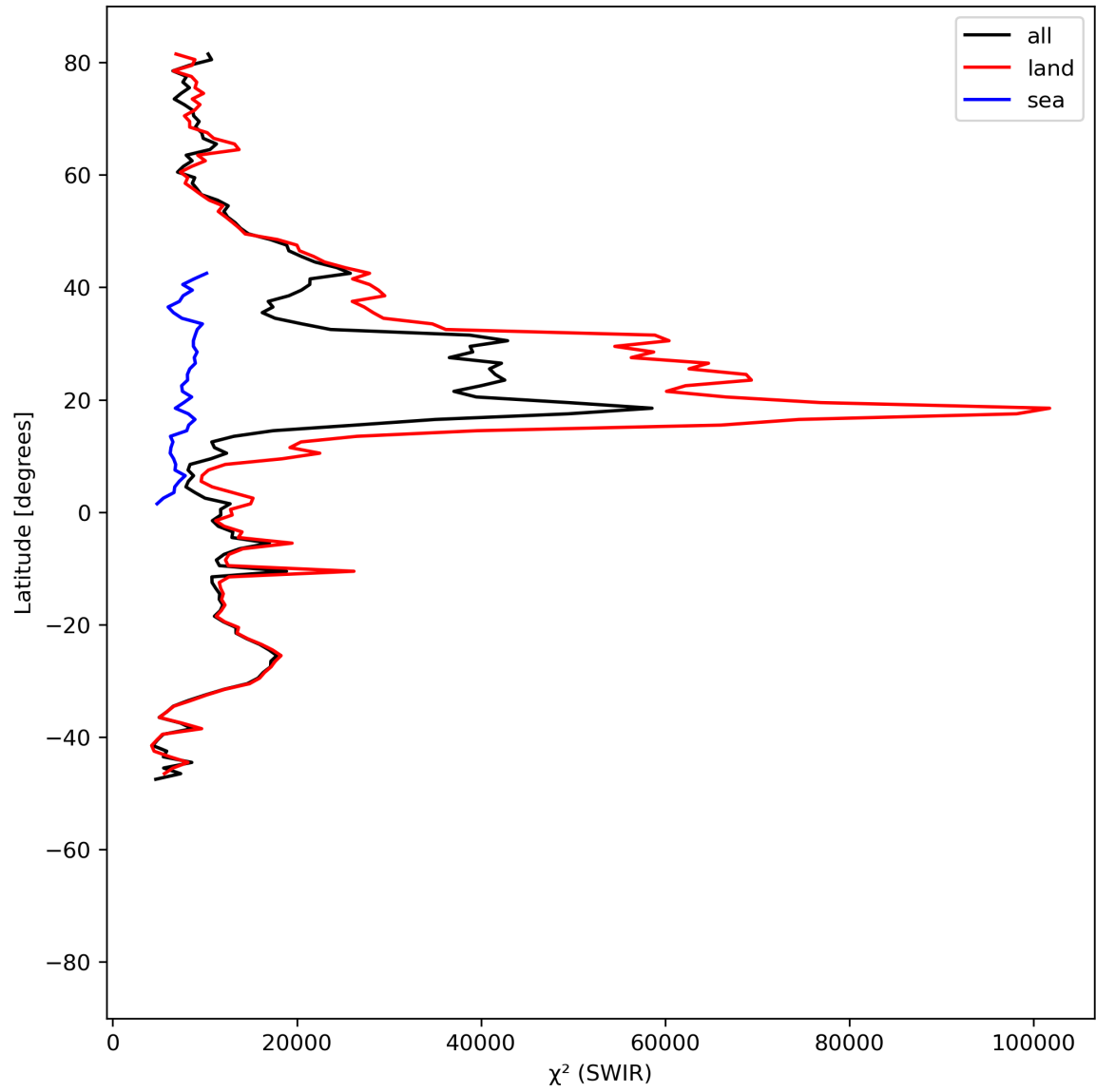
Figure 17: Zonal average of “ \chi^2 (SWIR)” for 2023-08-06 to 2023-08-08.
