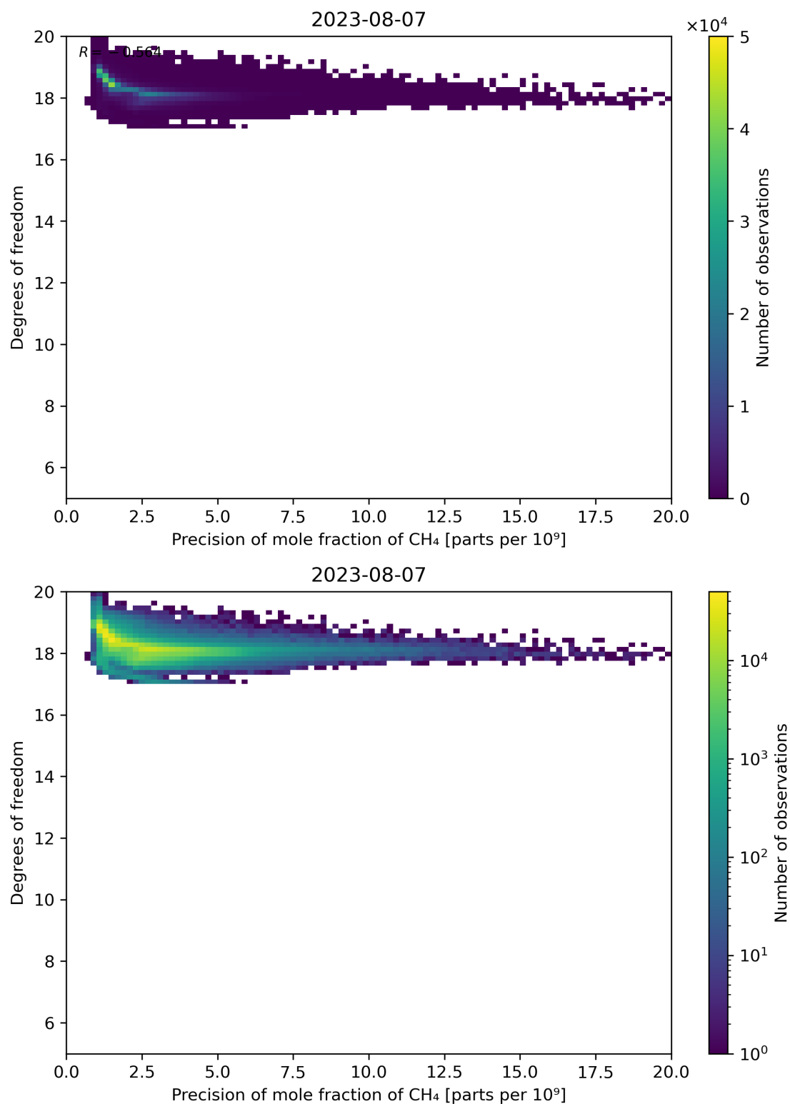
Figure 80: Scatter density plot of “Precision of mole fraction of CH 4 ” against “Degrees of freedom” for 2023-08-06 to 2023-08-08.
