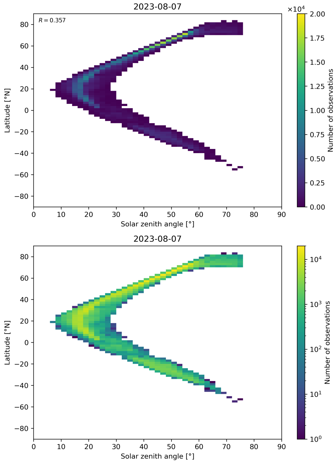
Figure 98: Scatter density plot of “Solar zenith angle” against “Latitude” for 2023-08-06 to 2023-08-08.
