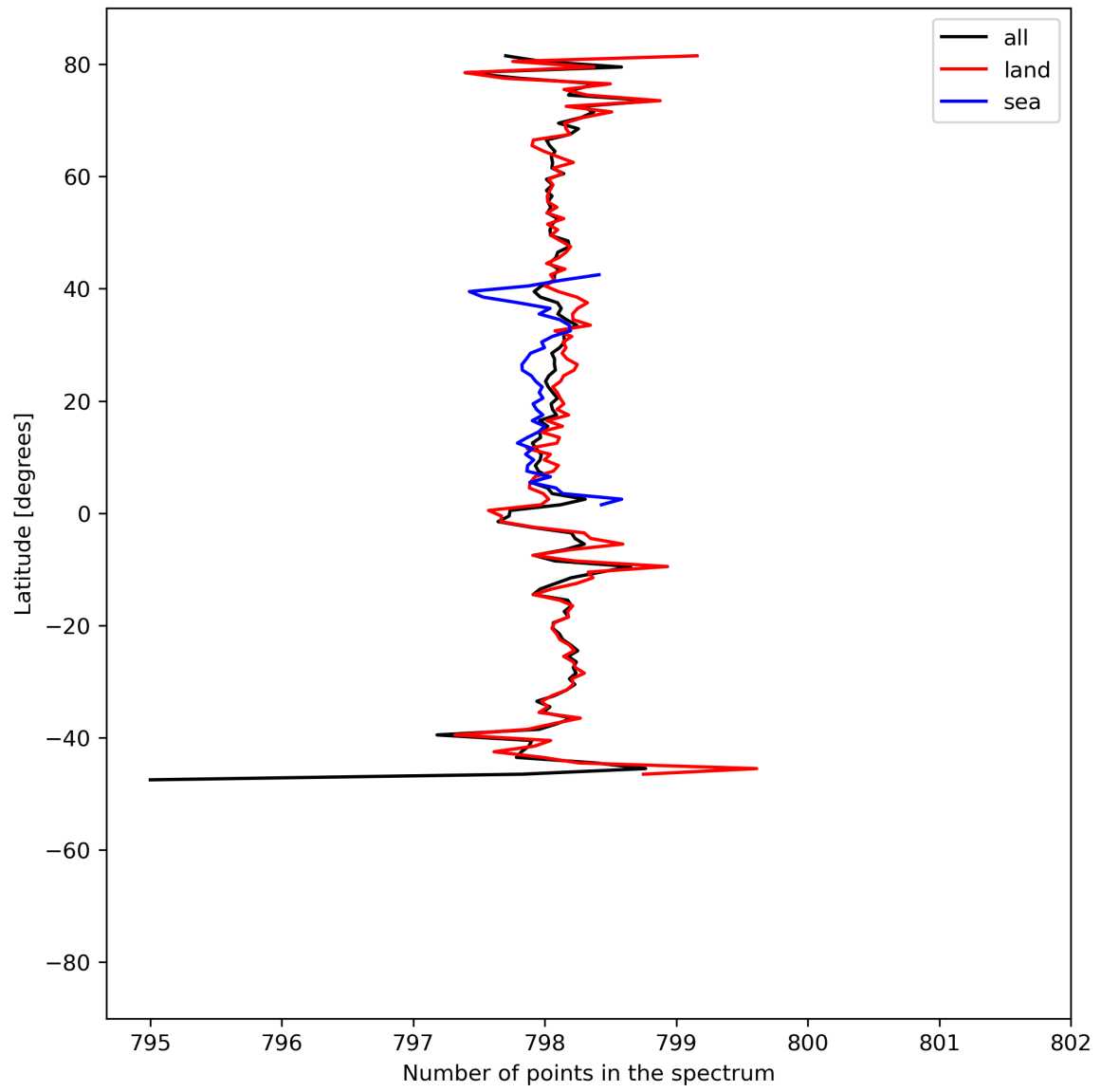
Figure 15: Zonal average of “Number of points in the spectrum” for 2023-08-06 to 2023-08-08.
