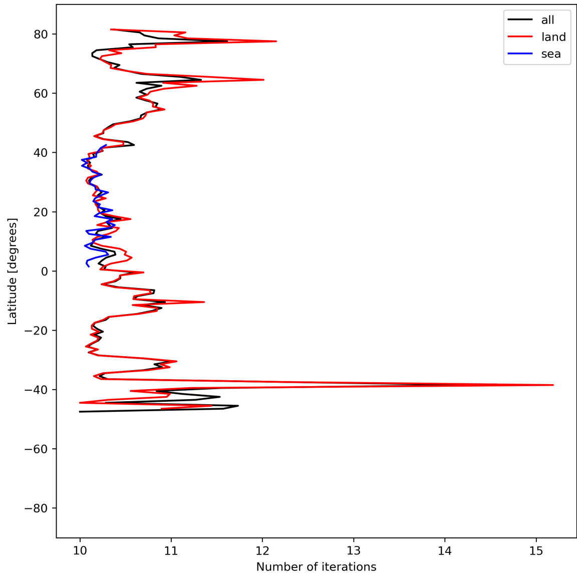
Figure 20: Zonal average of “Number of iterations” for 2023-08-06 to 2023-08-08.
