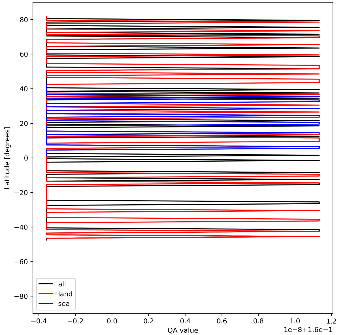
Figure 11: Zonal average of “QA value” for 2023-08-06 to 2023-08-08.
