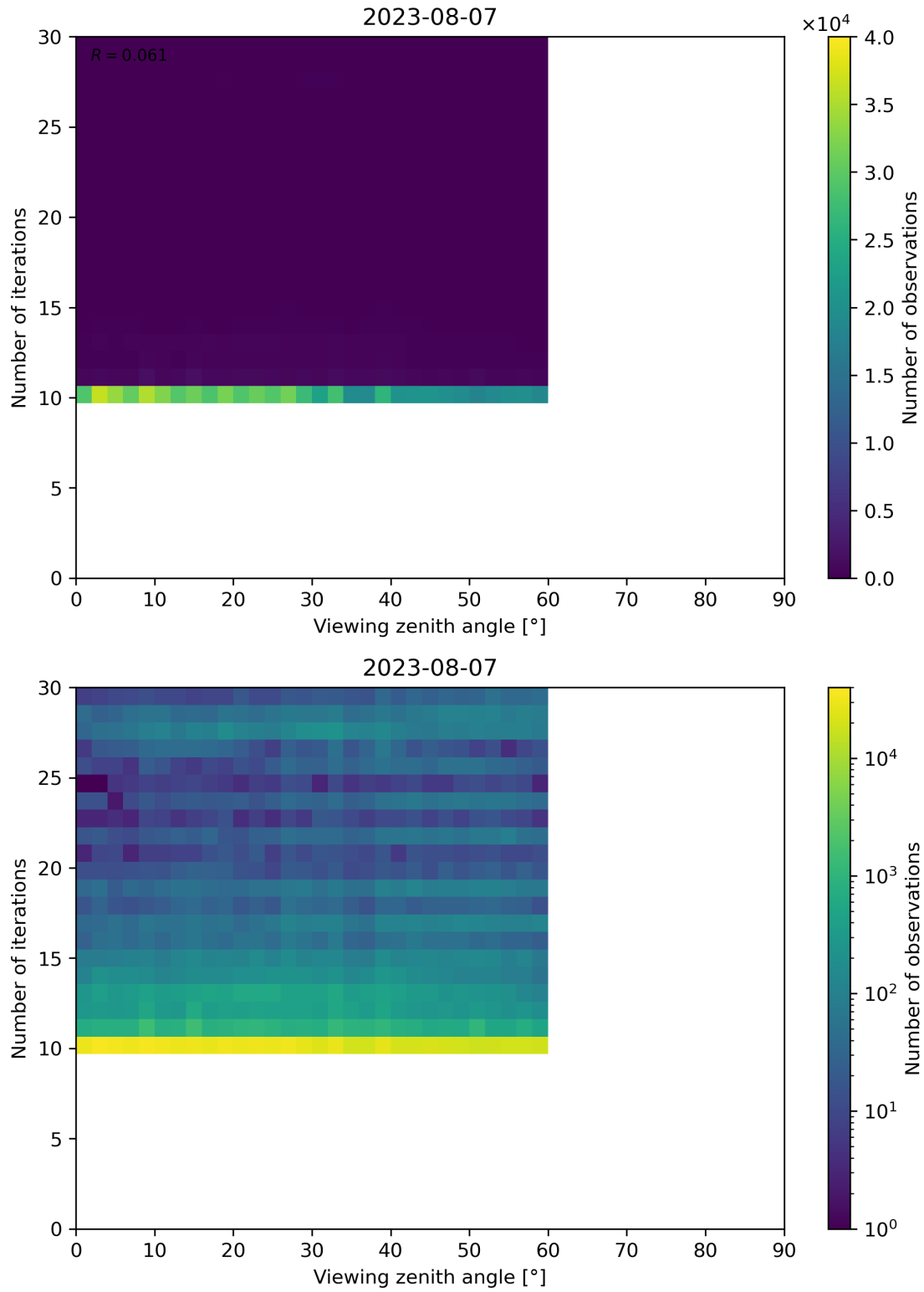
Figure 113: Scatter density plot of “Viewing zenith angle” against “Number of iterations” for 2023-08-06 to 2023-08-08.
