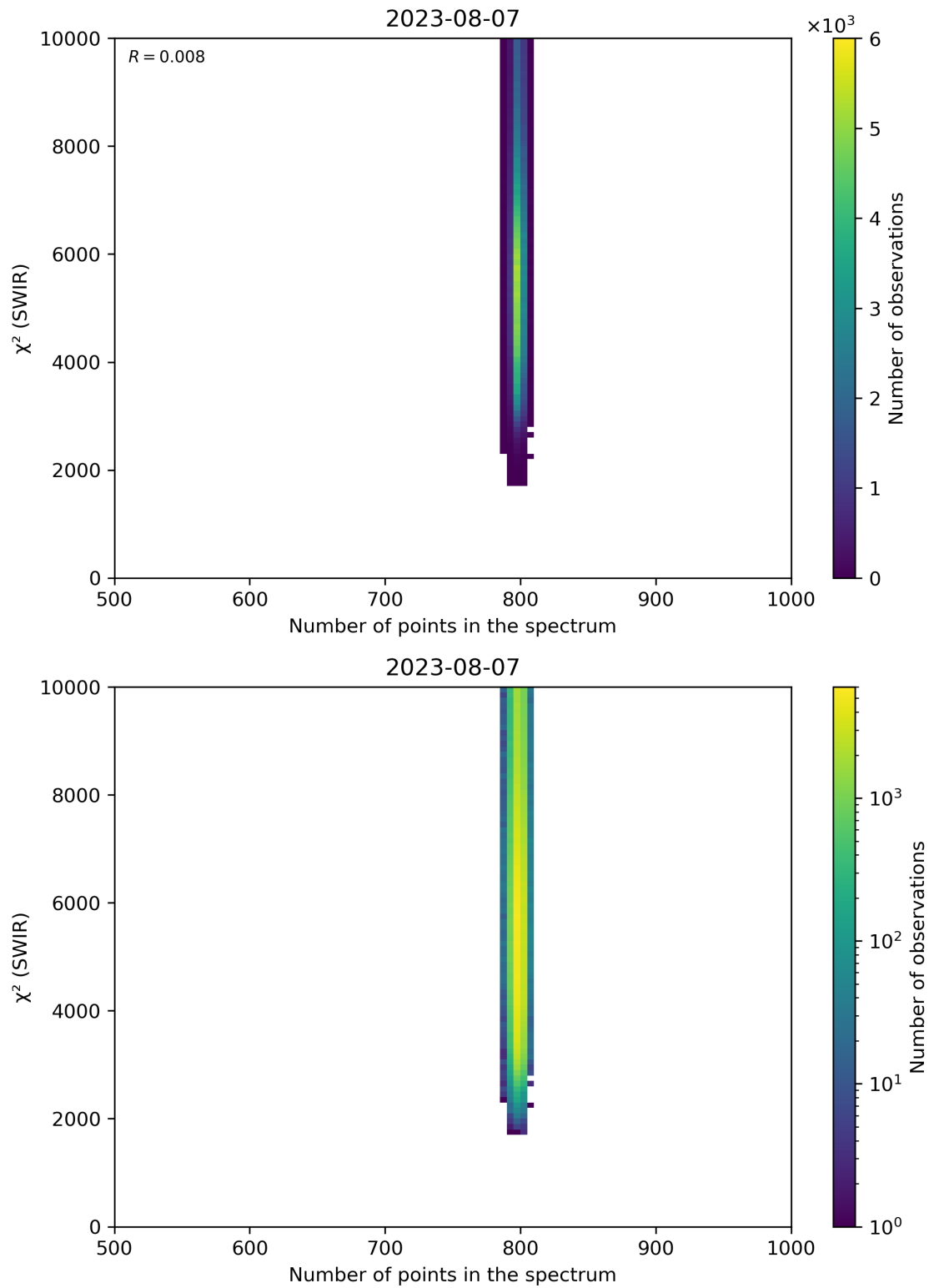
Figure 89: Scatter density plot of “Number of points in the spectrum” against “ \chi^2 (SWIR)” for 2023-08-06 to 2023-08-08.
