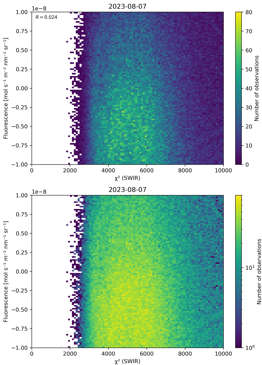
Figure 49: Scatter density plot of “ \chi^2 (SWIR)” against “Fluorescence” for 2023-08-06 to 2023-08-08.
