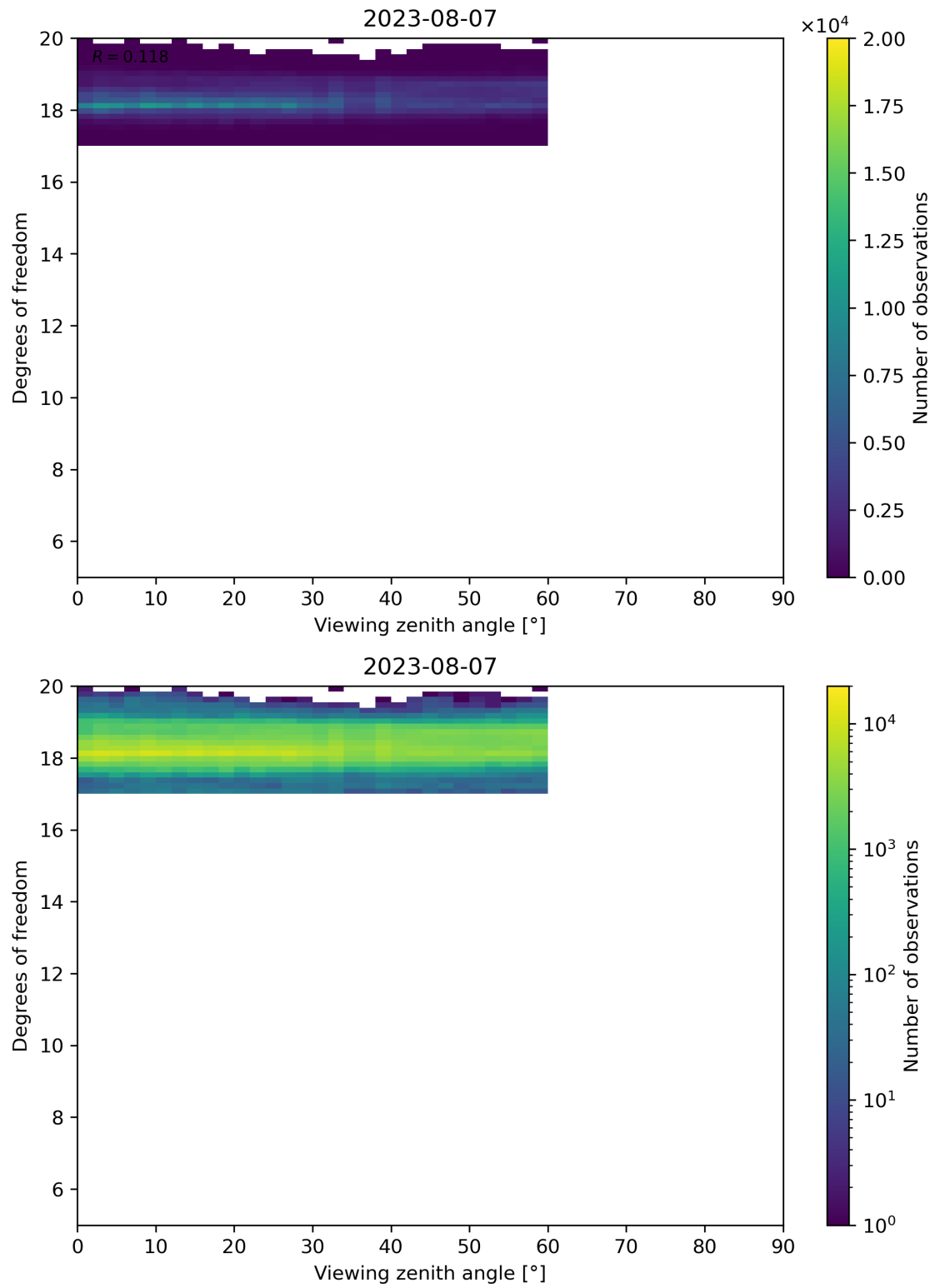
Figure 107: Scatter density plot of “Viewing zenith angle” against “Degrees of freedom” for 2023-08-06 to 2023-08-08.
