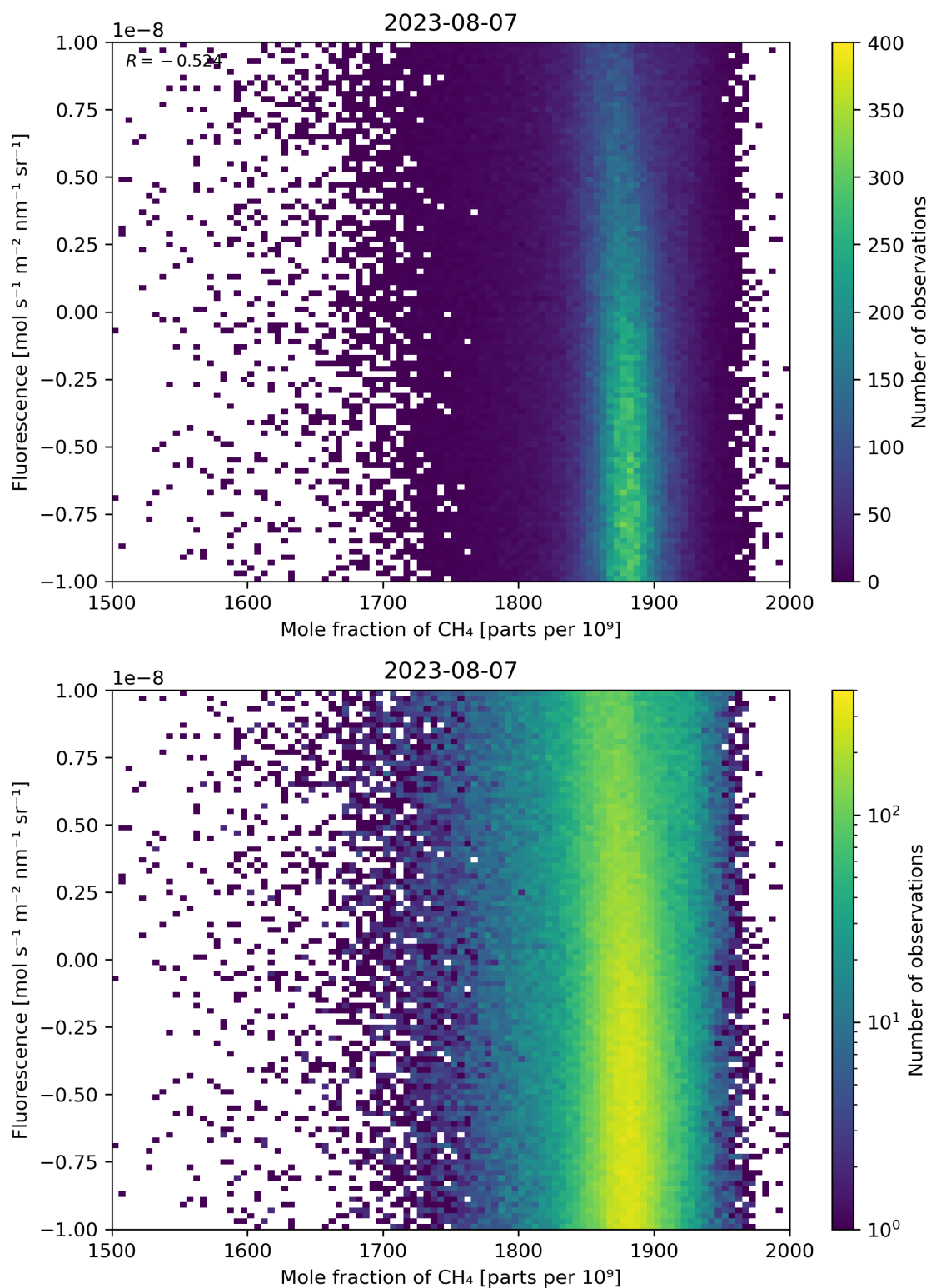
Figure 73: Scatter density plot of “Mole fraction of \text{CH}_4 ” against “Fluorescence” for 2023-08-06 to 2023-08-08.
