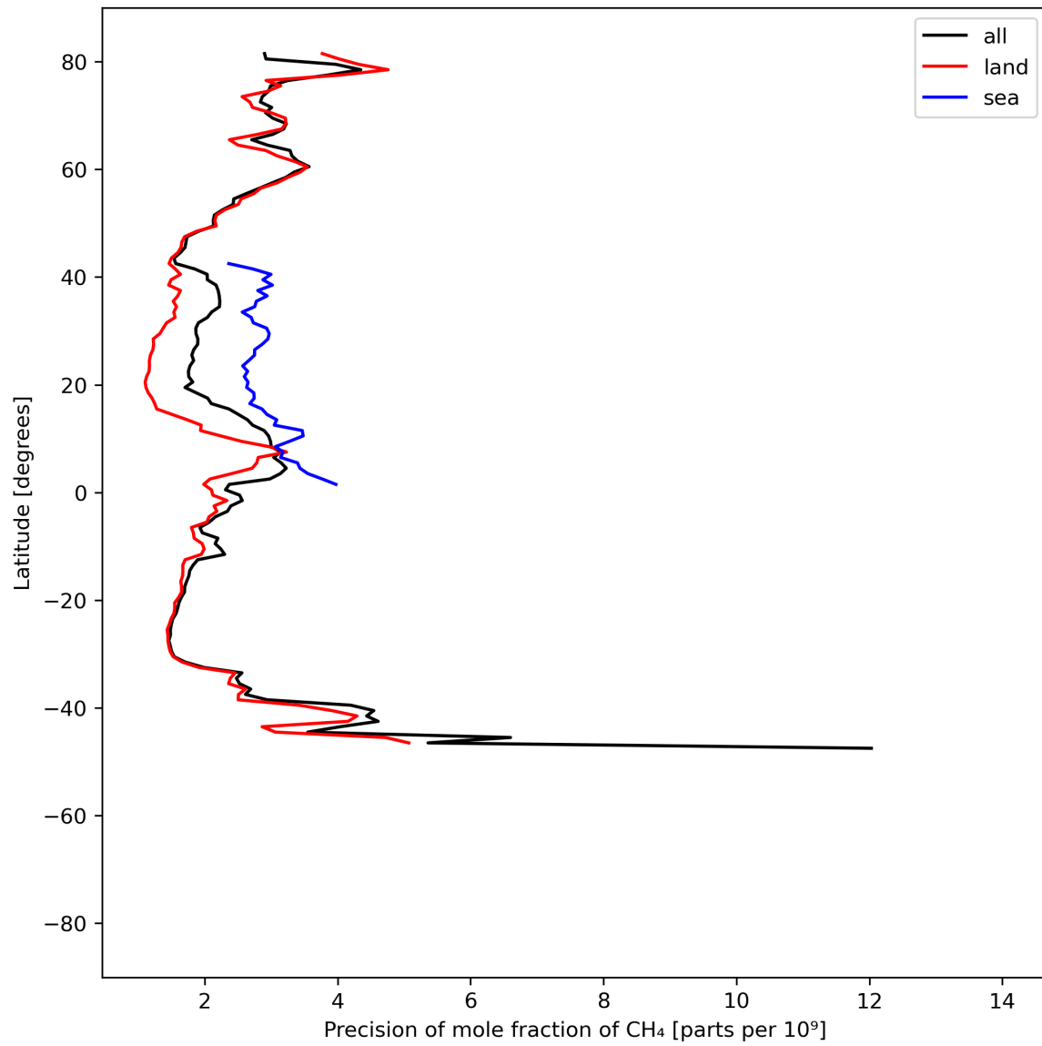
Figure 13: Zonal average of “Precision of mole fraction of CH 4 ” for 2023-08-06 to 2023-08-08.
