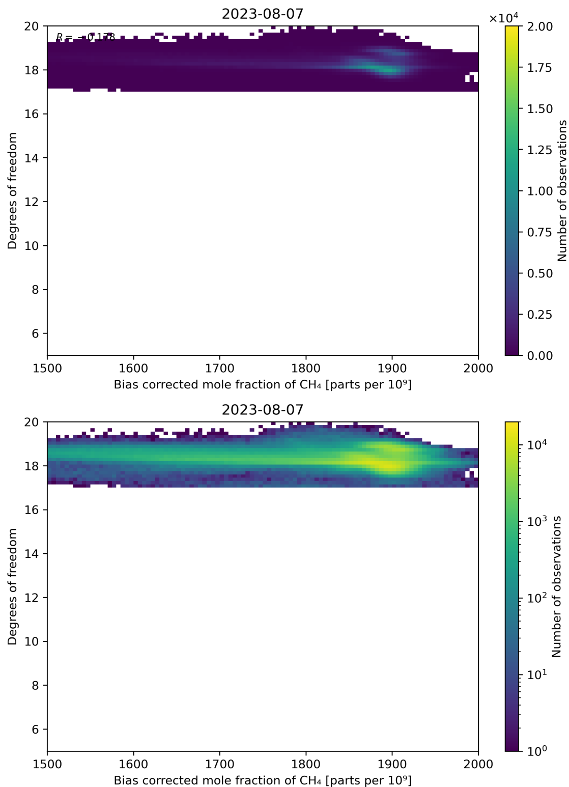
Figure 65: Scatter density plot of “Bias corrected mole fraction of CH 4 ” against “Degrees of freedom” for 2023-08-06 to 2023-08-08.
