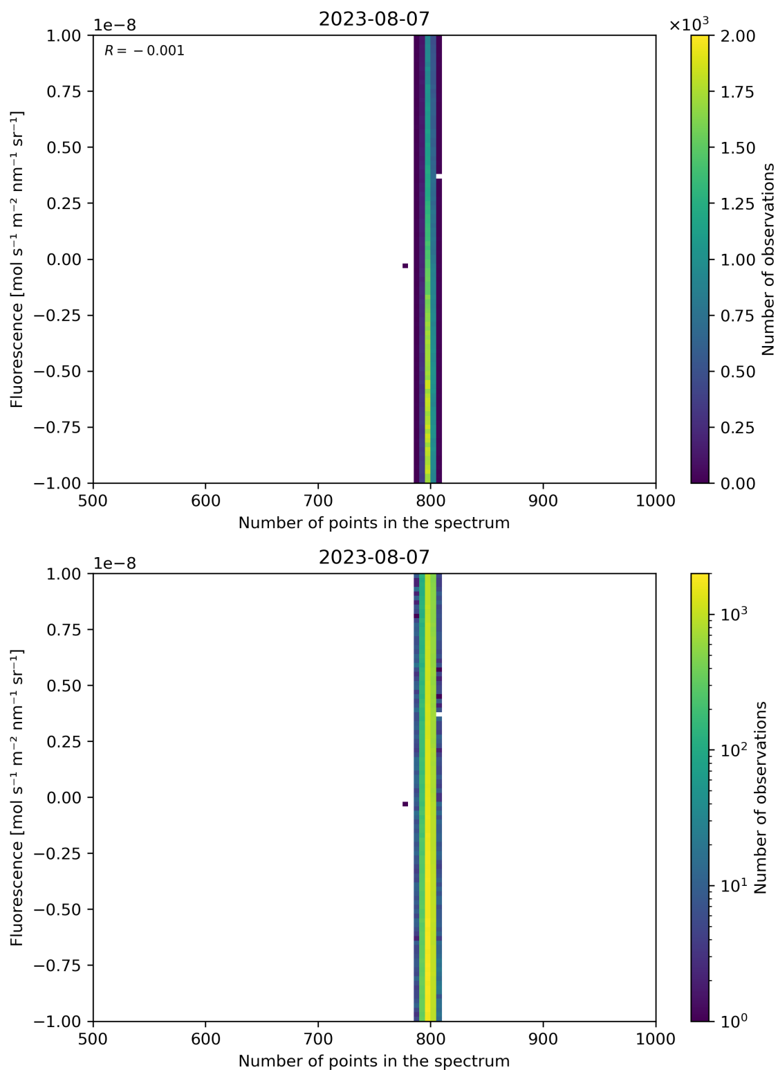
Figure 91: Scatter density plot of “Number of points in the spectrum” against “Fluorescence” for 2023-08-06 to 2023-08-08.
