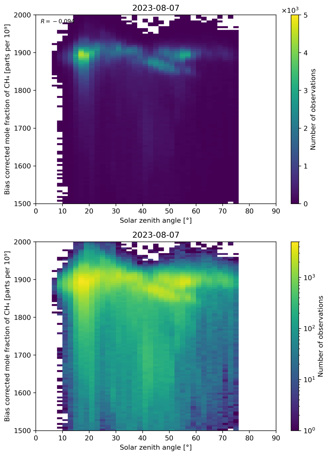
Figure 100: Scatter density plot of “Solar zenith angle” against “Bias corrected mole fraction of CH 4 ” for 2023-08-06 to 2023-08-08.
