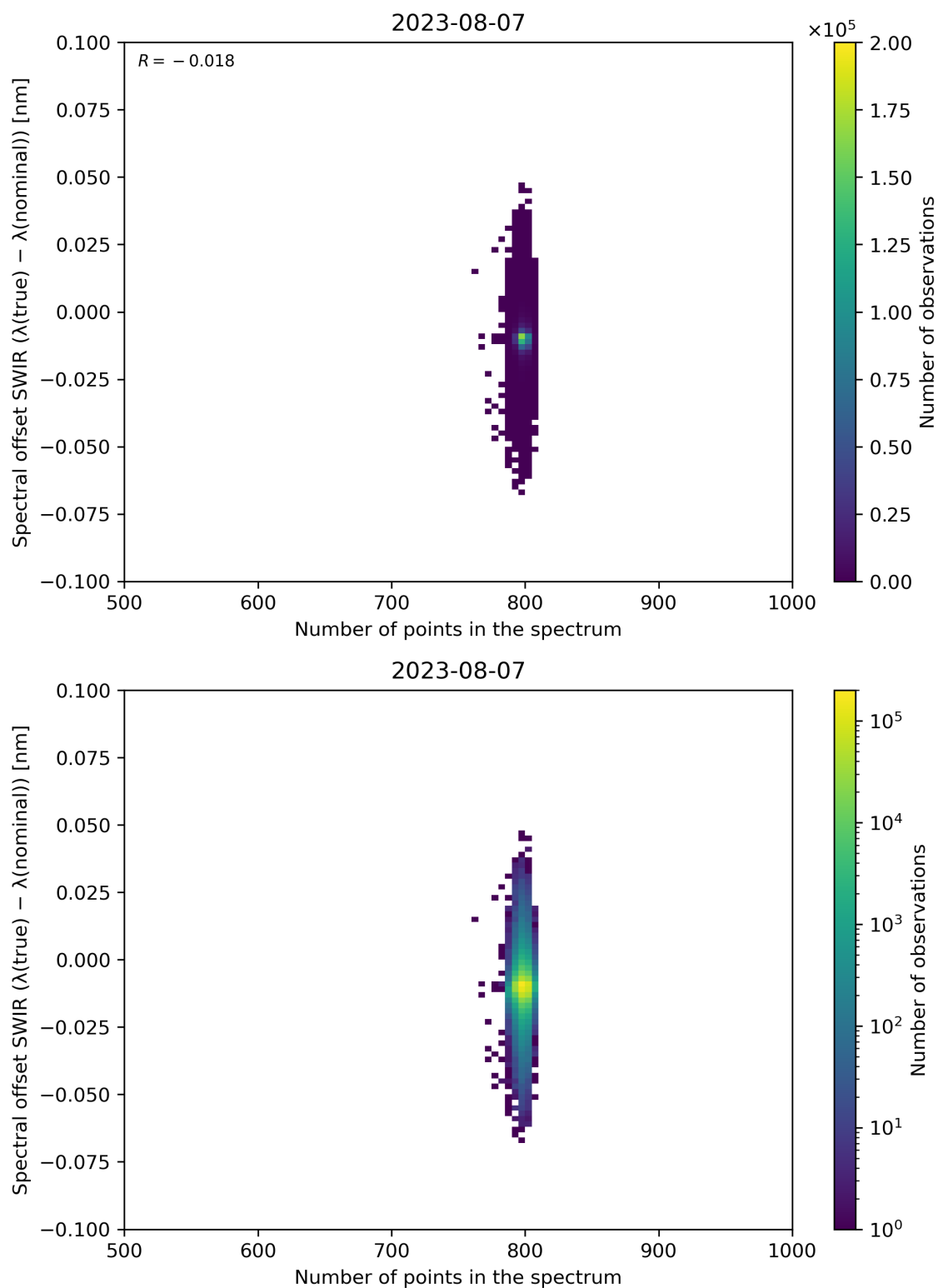
Figure 93: Scatter density plot of “Number of points in the spectrum” against “Spectral offset SWIR ( \lambda(\text{true}) - \lambda(\text{nominal}) )” for 2023-08-06 to 2023-08-08.
