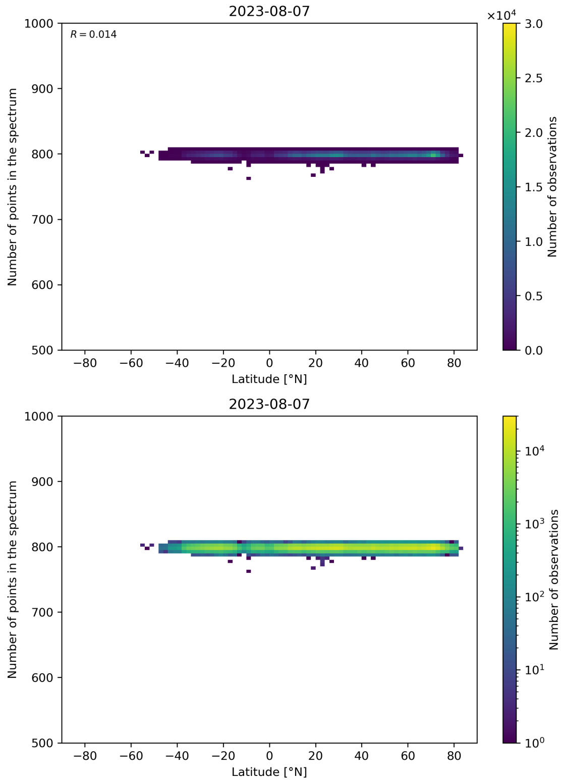
Figure 61: Scatter density plot of “Latitude” against “Number of points in the spectrum” for 2023-08-06 to 2023-08-08.
