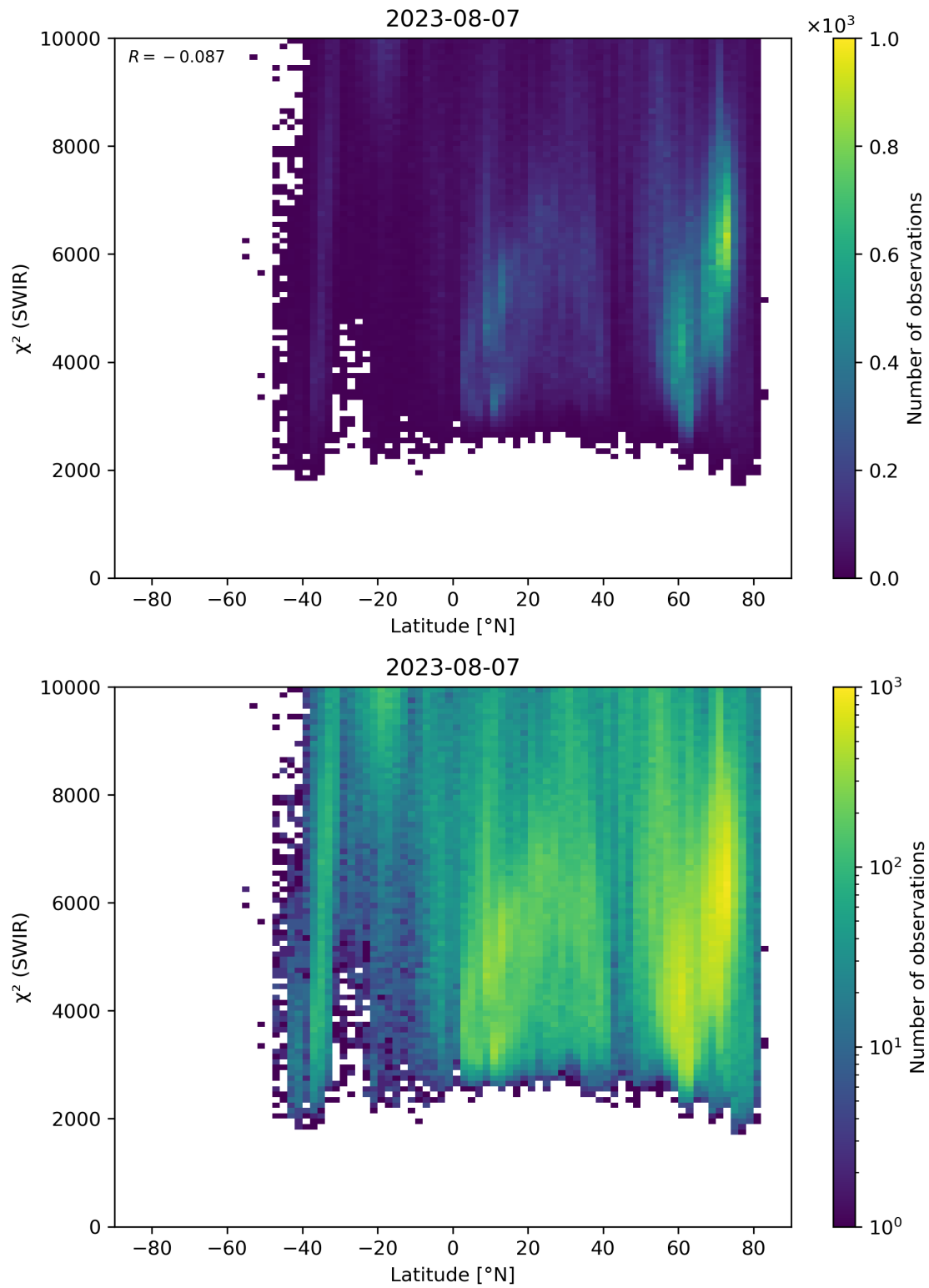
Figure 54: Scatter density plot of “Latitude” against “ \chi^2 (SWIR)” for 2023-08-06 to 2023-08-08.
