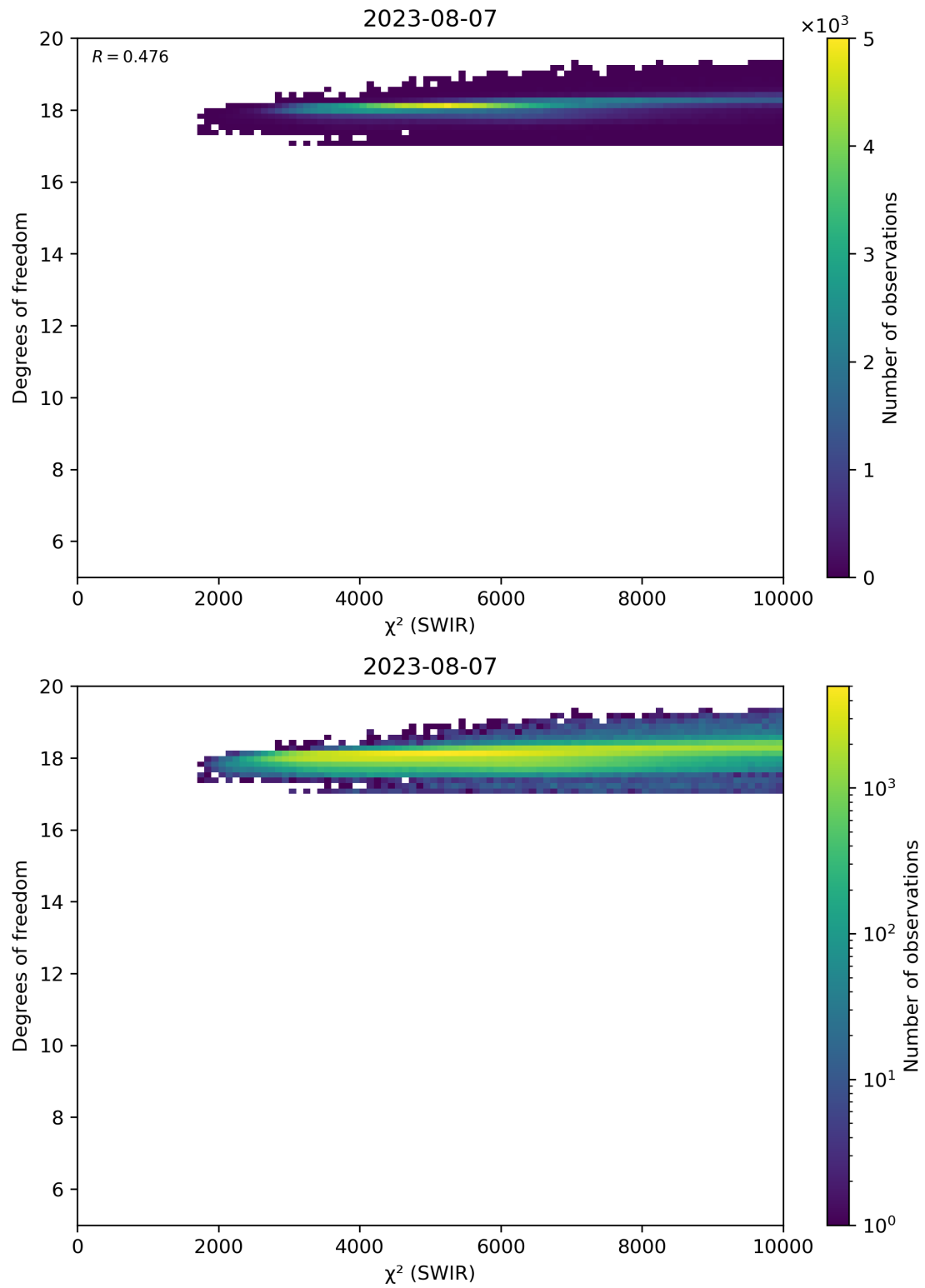
Figure 48: Scatter density plot of “ \chi^2 (SWIR)” against “Degrees of freedom” for 2023-08-06 to 2023-08-08.
