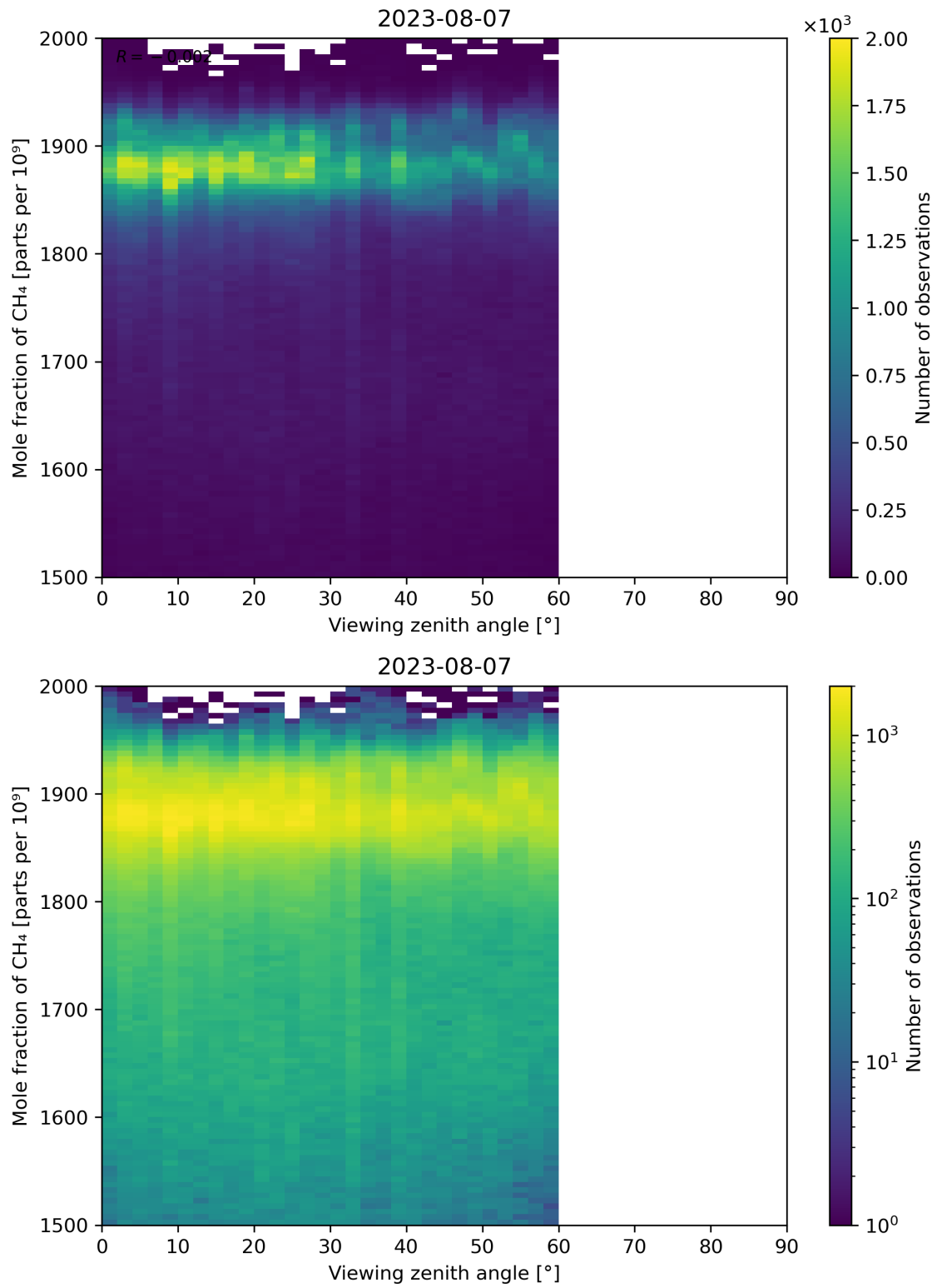
Figure 110: Scatter density plot of “Viewing zenith angle” against “Mole fraction of CH 4 ” for 2023-08-06 to 2023-08-08.
