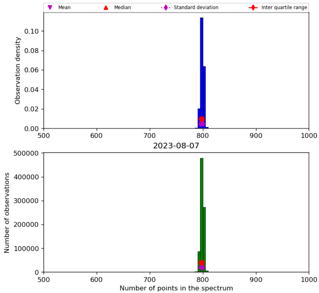
Figure 26: Histogram of “Number of points in the spectrum” for 2023-08-06 to 2023-08-08
