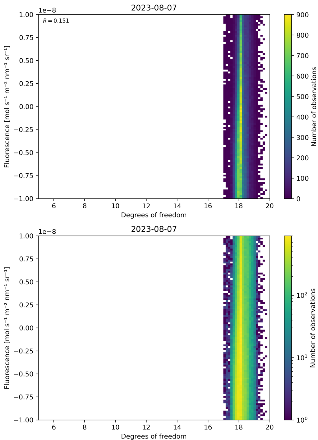
Figure 51: Scatter density plot of “Degrees of freedom” against “Fluorescence” for 2023-08-06 to 2023-08-08.
