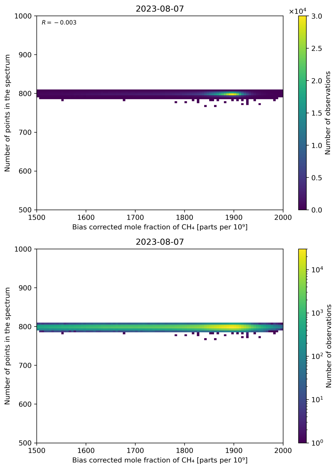
Figure 68: Scatter density plot of “Bias corrected mole fraction of CH 4 ” against “Number of points in the spectrum” for 2023-08-06 to 2023-08-08.
