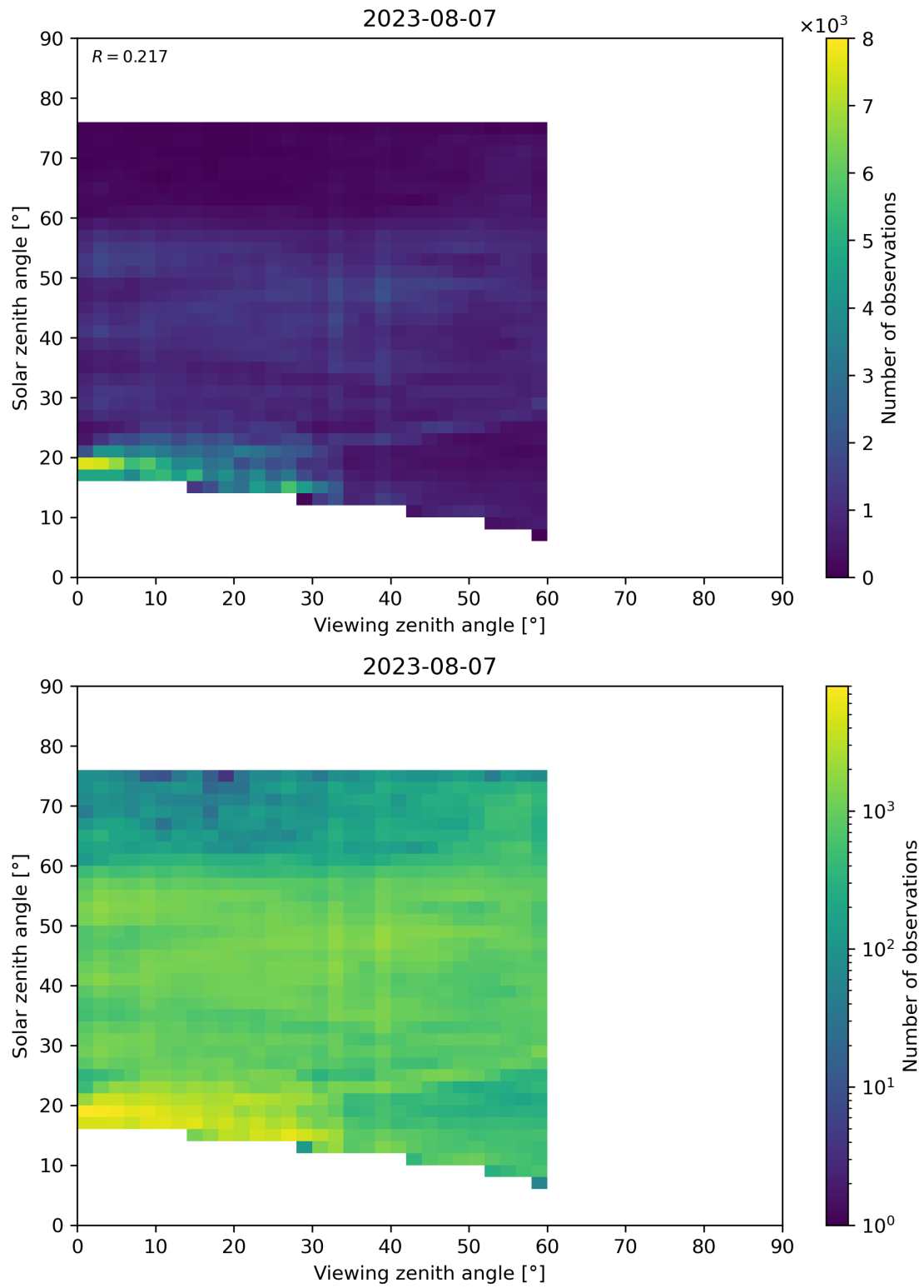
Figure 115: Scatter density plot of “Viewing zenith angle” against “Solar zenith angle” for 2023-08-06 to 2023-08-08.
