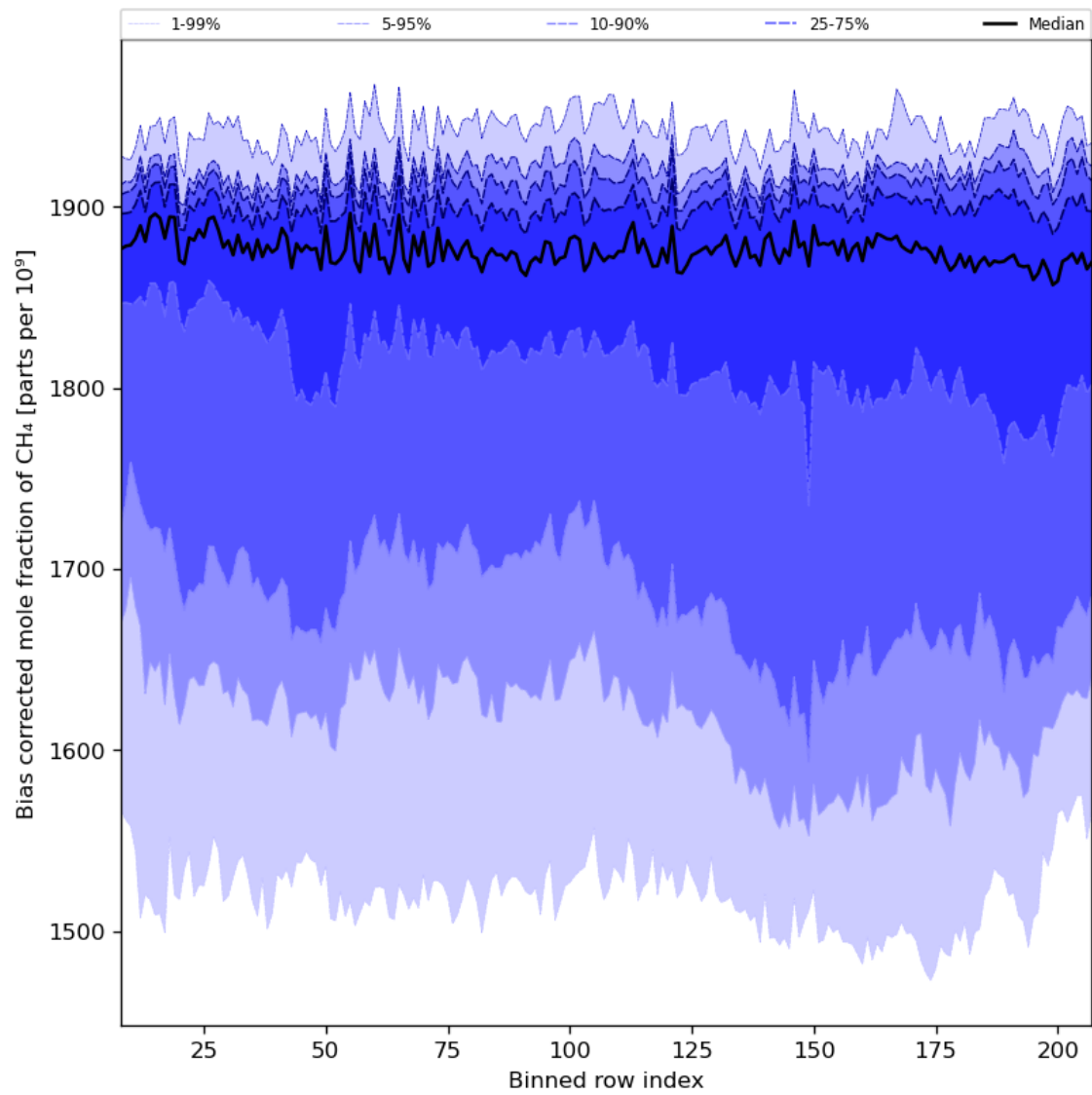
Figure 36: Along track statistics of “Bias corrected mole fraction of CH 4 ” for 2023-08-06 to 2023-08-08
