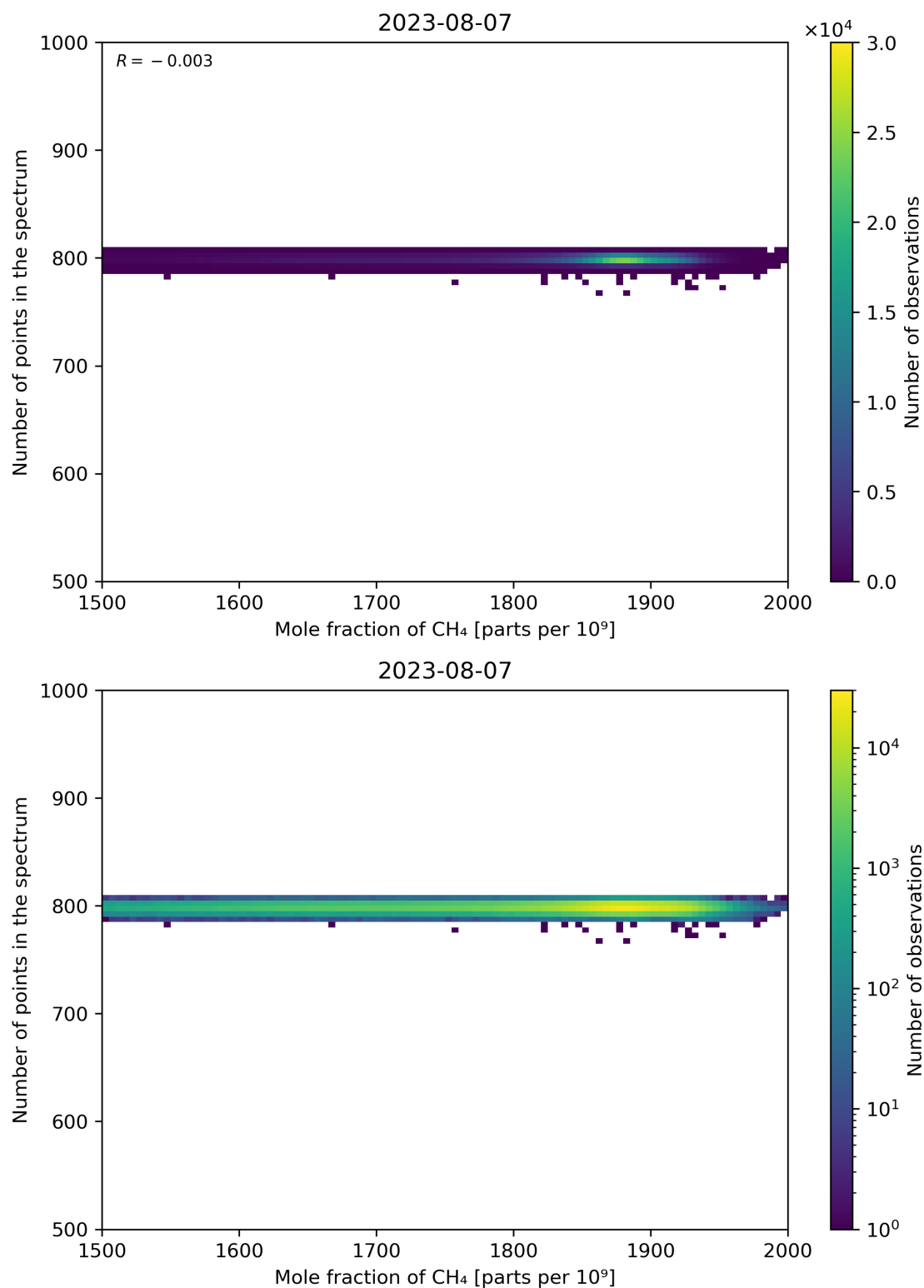
Figure 77: Scatter density plot of “Mole fraction of CH 4 ” against “Number of points in the spectrum” for 2023-08-06 to 2023-08-08.
