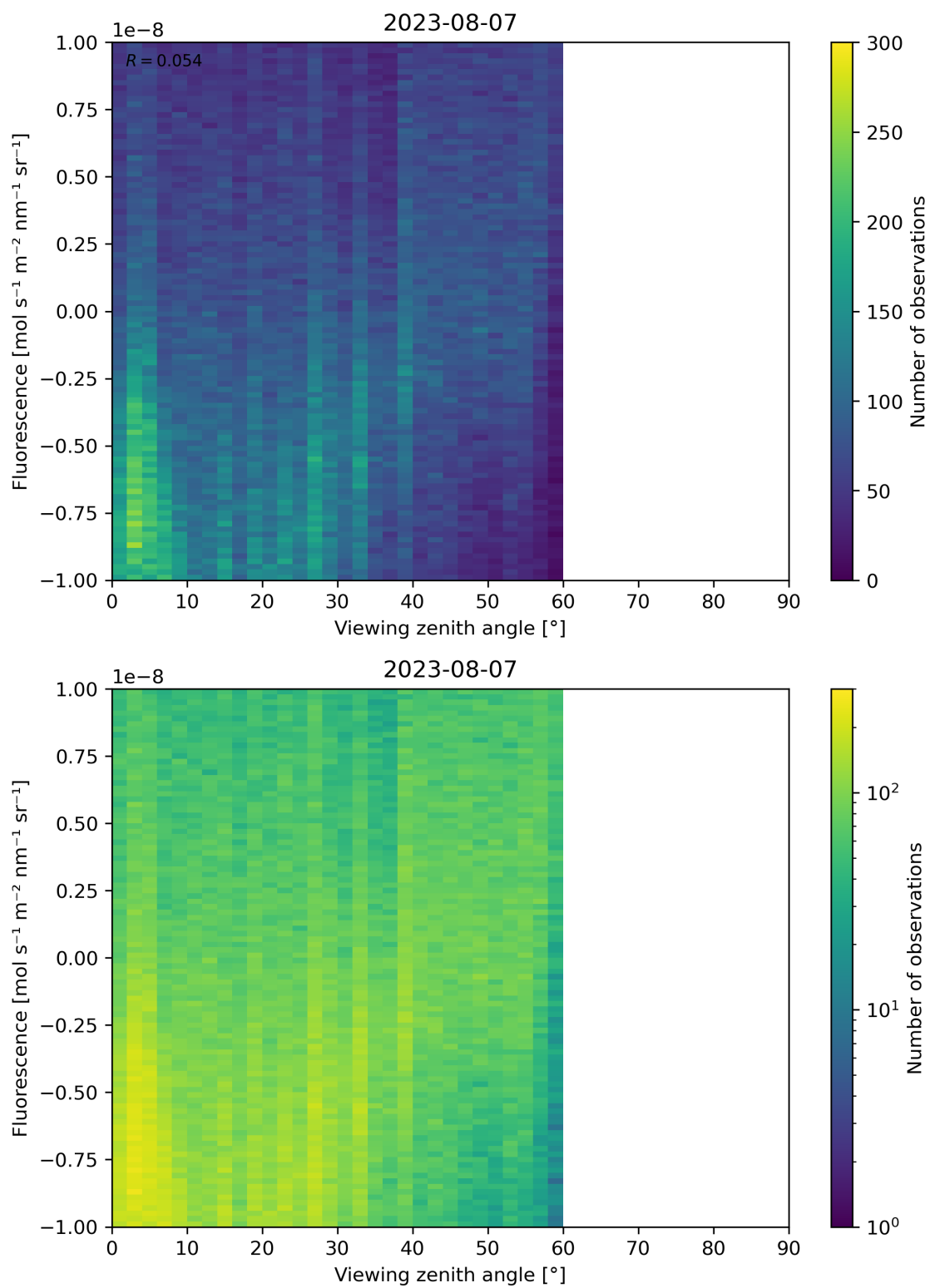
Figure 108: Scatter density plot of “Viewing zenith angle” against “Fluorescence” for 2023-08-06 to 2023-08-08.
