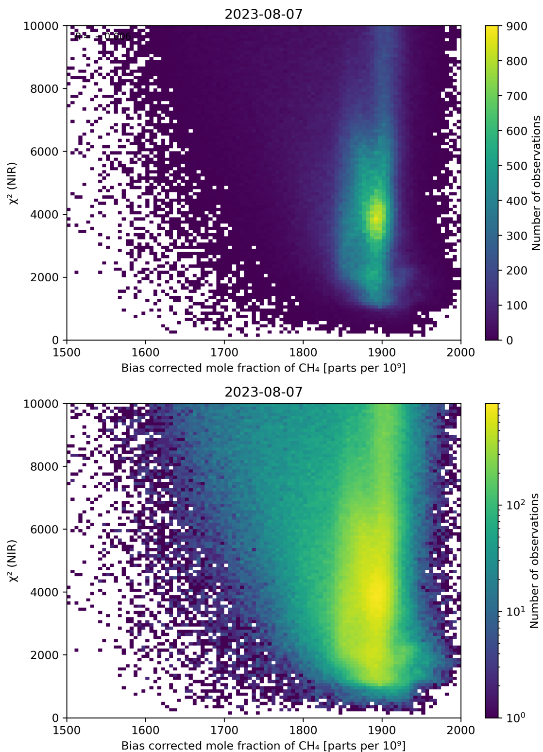
Figure 63: Scatter density plot of “Bias corrected mole fraction of CH 4 ” against “ \chi^2 (NIR)” for 2023-08-06 to 2023-08-08.
