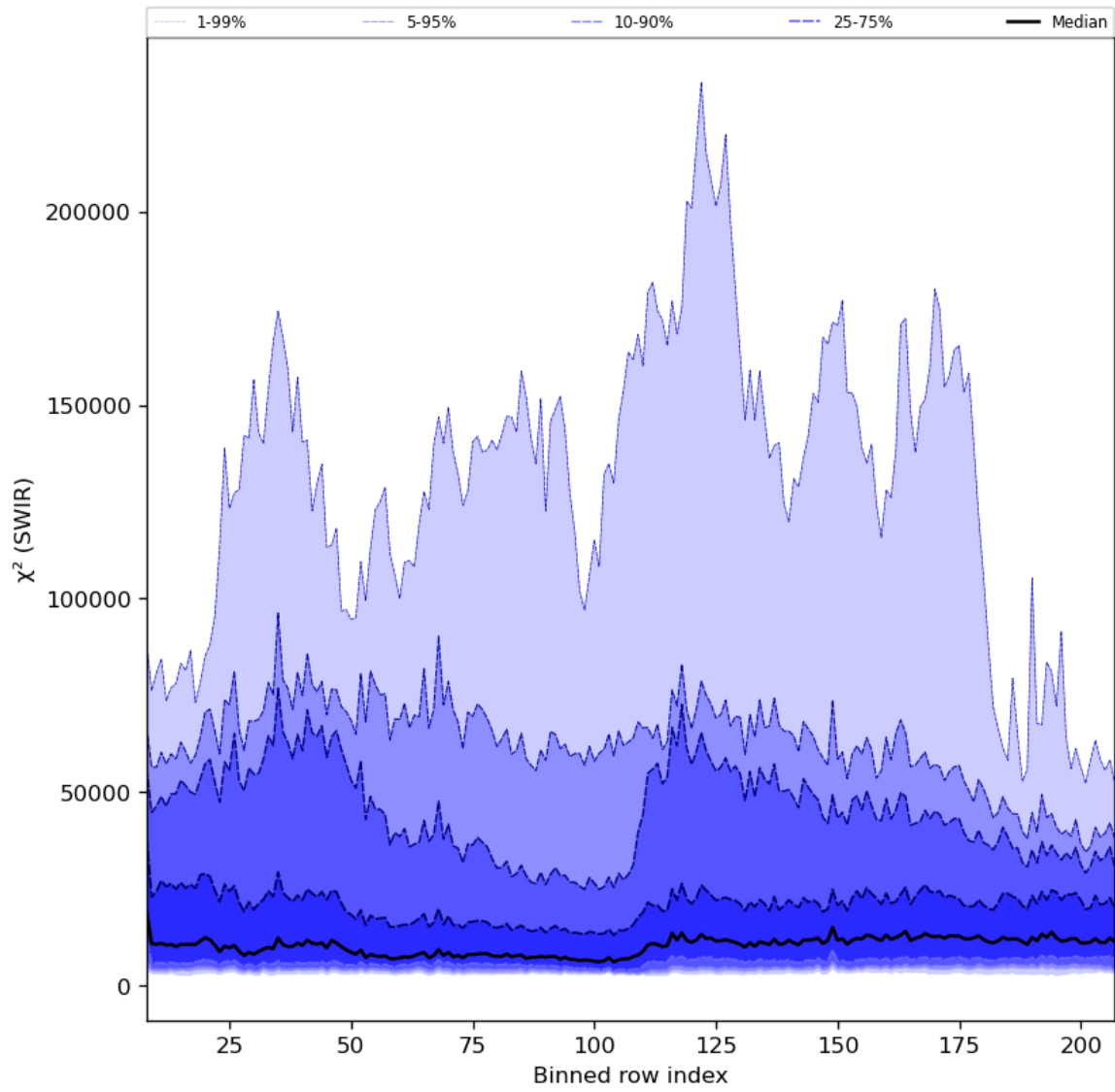
Figure 39: Along track statistics of " \chi^2 (SWIR)" for 2023-08-06 to 2023-08-08
