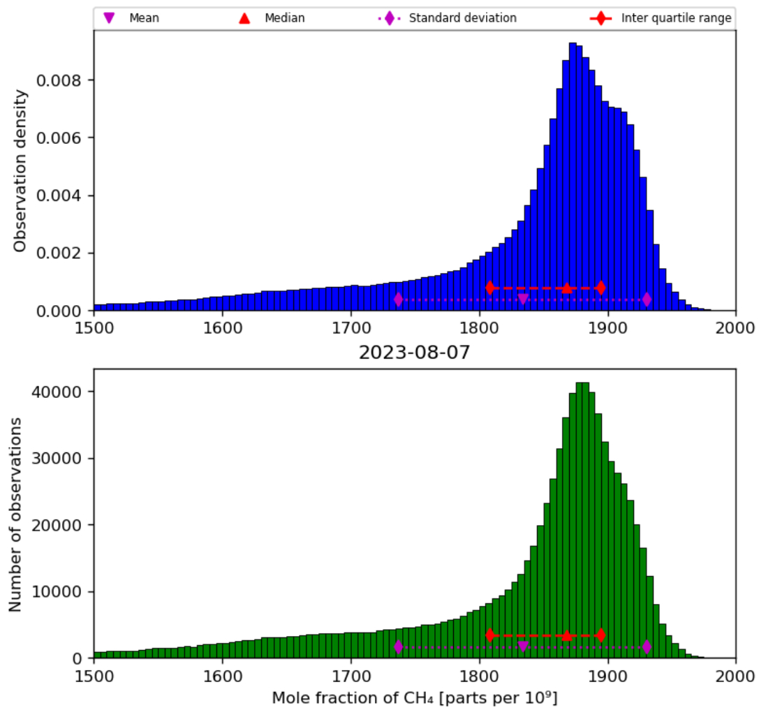
Figure 23: Histogram of “Mole fraction of CH 4 ” for 2023-08-06 to 2023-08-08
