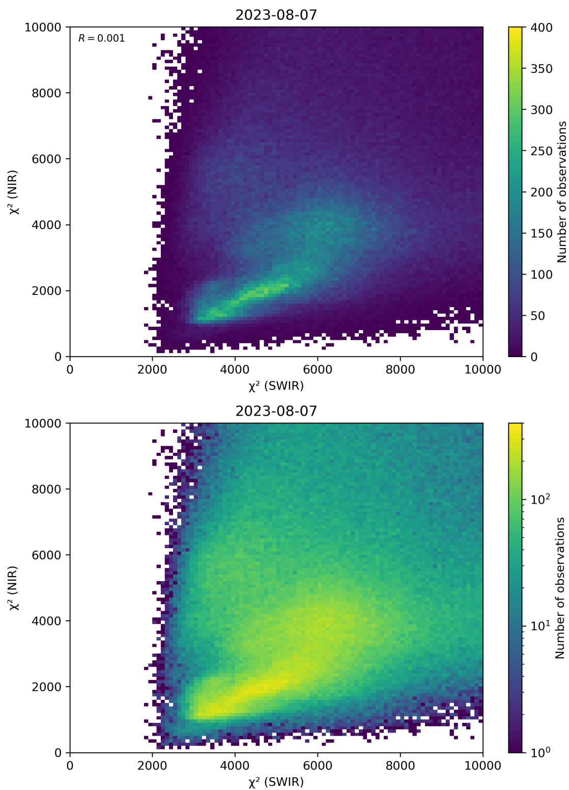
Figure 47: Scatter density plot of “ \chi^2 (SWIR)” against “ \chi^2 (NIR)” for 2023-08-06 to 2023-08-08.
