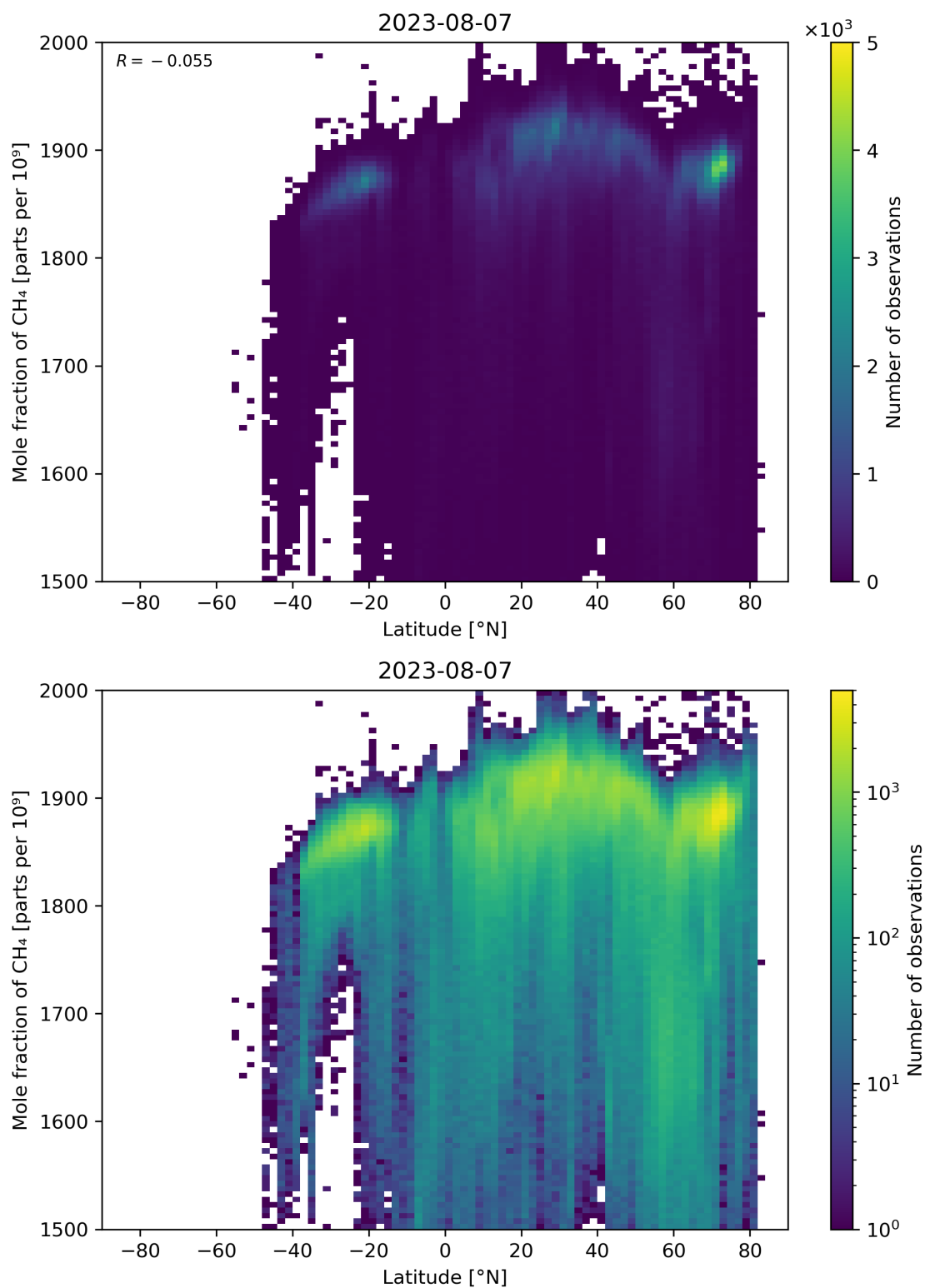
Figure 57: Scatter density plot of “Latitude” against “Mole fraction of \text{CH}_4 ” for 2023-08-06 to 2023-08-08.
