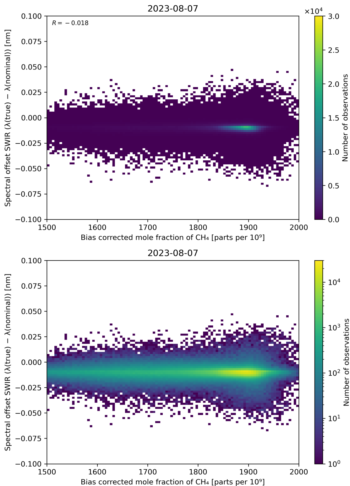
Figure 69: Scatter density plot of “Bias corrected mole fraction of \text{CH}_4 ” against “Spectral offset SWIR ( \lambda(\text{true}) - \lambda(\text{nominal}) )” for 2023-08-06 to 2023-08-08.
