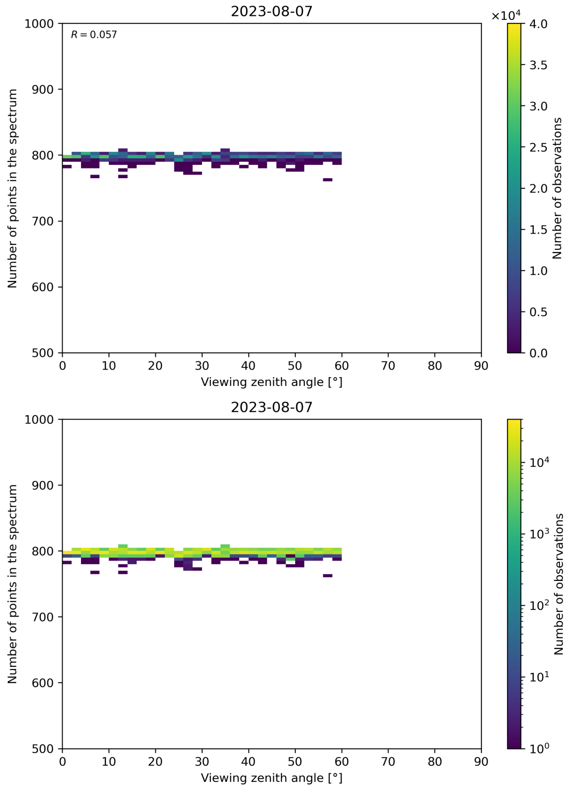
Figure 114: Scatter density plot of “Viewing zenith angle” against “Number of points in the spectrum” for 2023-08-06 to 2023-08-08.
