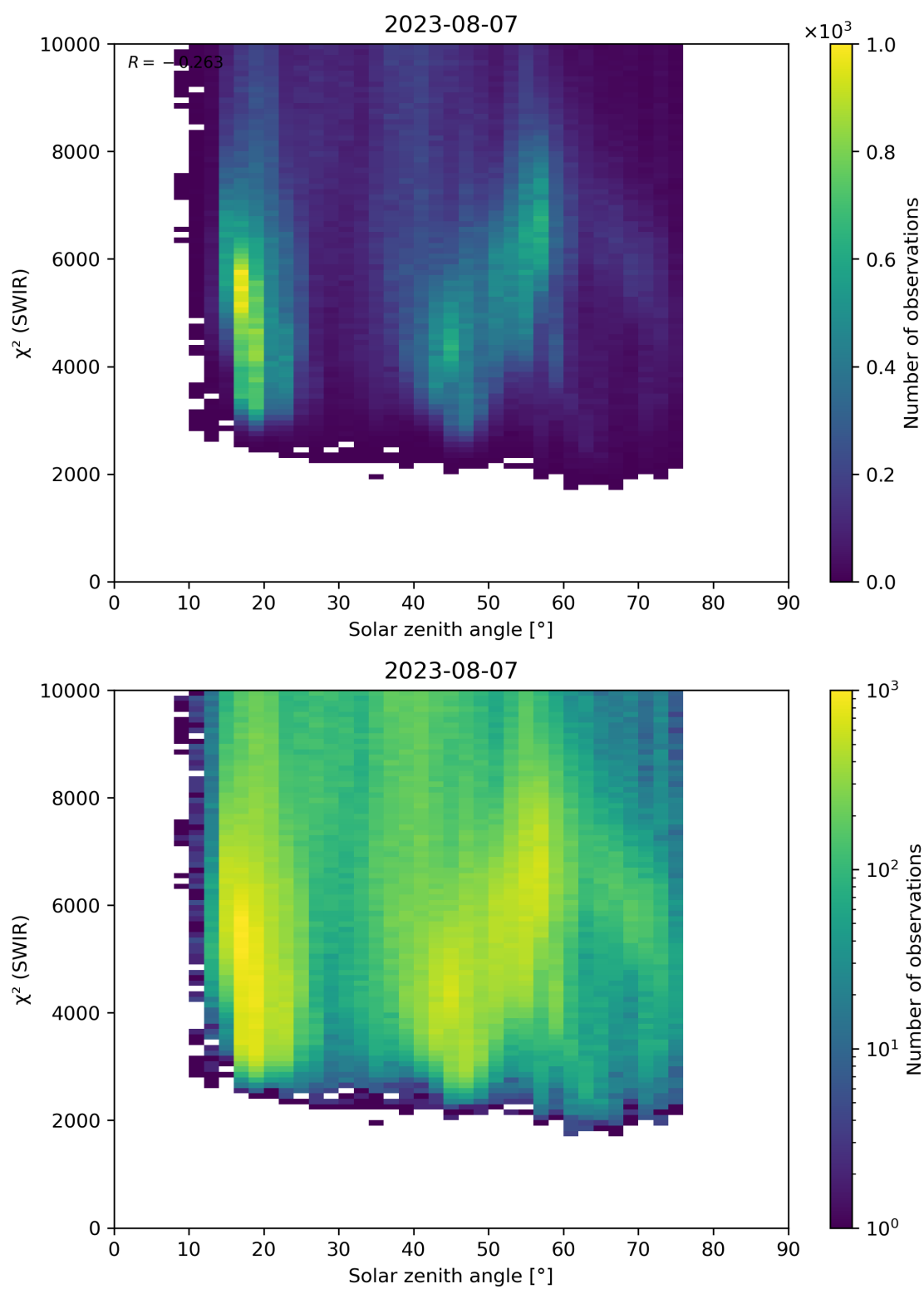
Figure 95: Scatter density plot of “Solar zenith angle” against “ \chi^2 (SWIR)” for 2023-08-06 to 2023-08-08.
