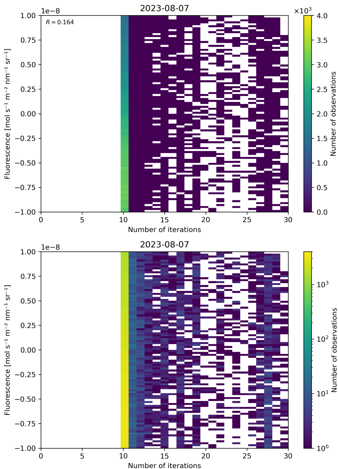
Figure 87: Scatter density plot of “Number of iterations” against “Fluorescence” for 2023-08-06 to 2023-08-08.
