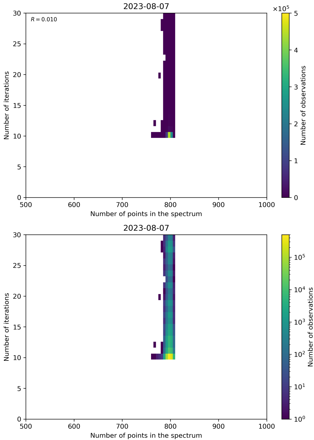
Figure 92: Scatter density plot of “Number of points in the spectrum” against “Number of iterations” for 2023-08-06 to 2023-08-08.
