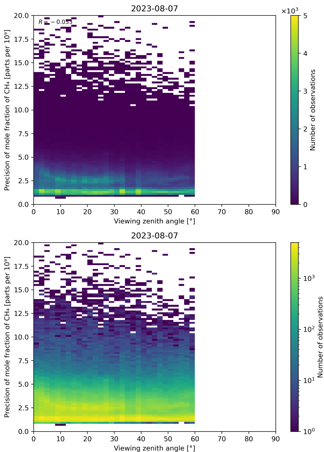
Figure 112: Scatter density plot of “Viewing zenith angle” against “Precision of mole fraction of CH 4 ” for 2023-08-06 to 2023-08-08.
