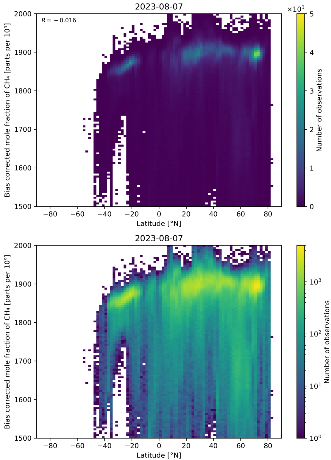
Figure 58: Scatter density plot of “Latitude” against “Bias corrected mole fraction of CH 4 ” for 2023-08-06 to 2023-08-08.
