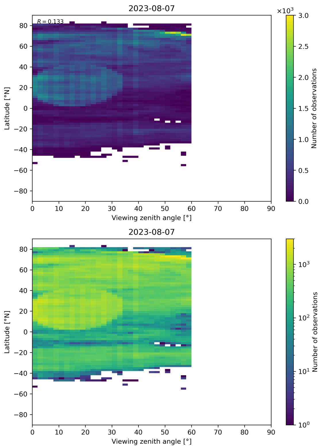
Figure 109: Scatter density plot of “Viewing zenith angle” against “Latitude” for 2023-08-06 to 2023-08-08.
