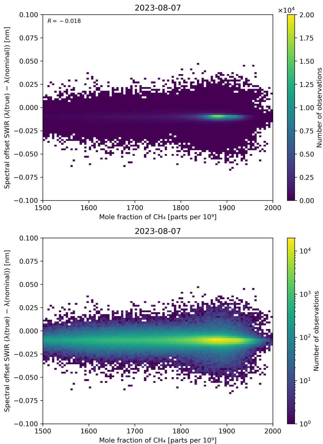
Figure 86: Scatter density plot of “Mole fraction of CH 4 ” against “Spectral offset SWIR ( \lambda(\text{true}) - \lambda(\text{nominal}) )” for 2023-08-06 to 2023-08-08.
