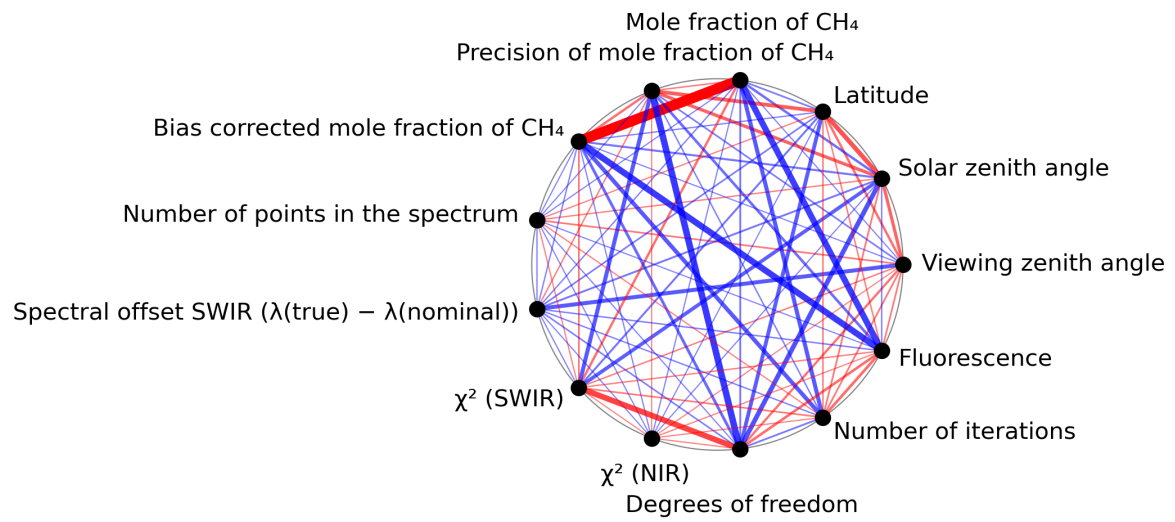
Figure 1: Map of correlation graph for 2023-08-06 to 2023-08-08.
