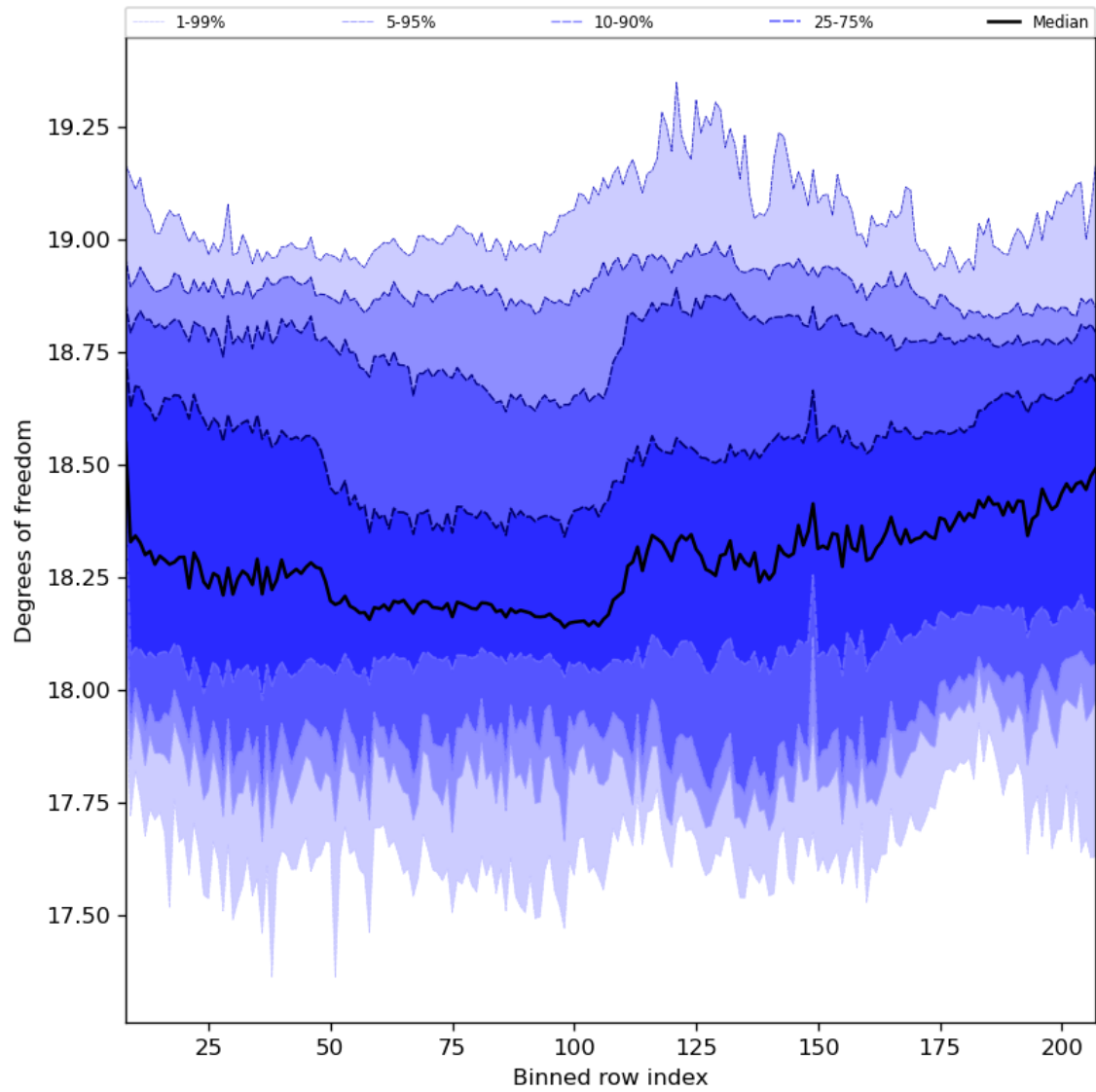
Figure 41: Along track statistics of “Degrees of freedom” for 2023-08-06 to 2023-08-08
