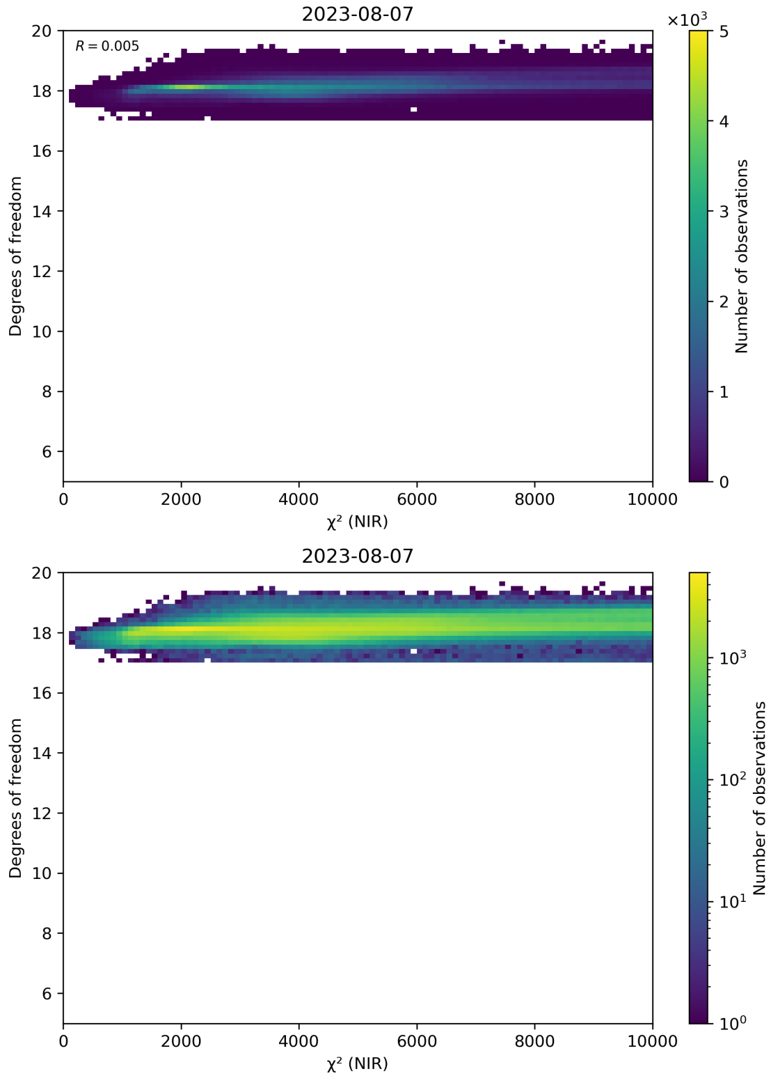
Figure 44: Scatter density plot of “ \chi^2 (NIR)” against “Degrees of freedom” for 2023-08-06 to 2023-08-08.
