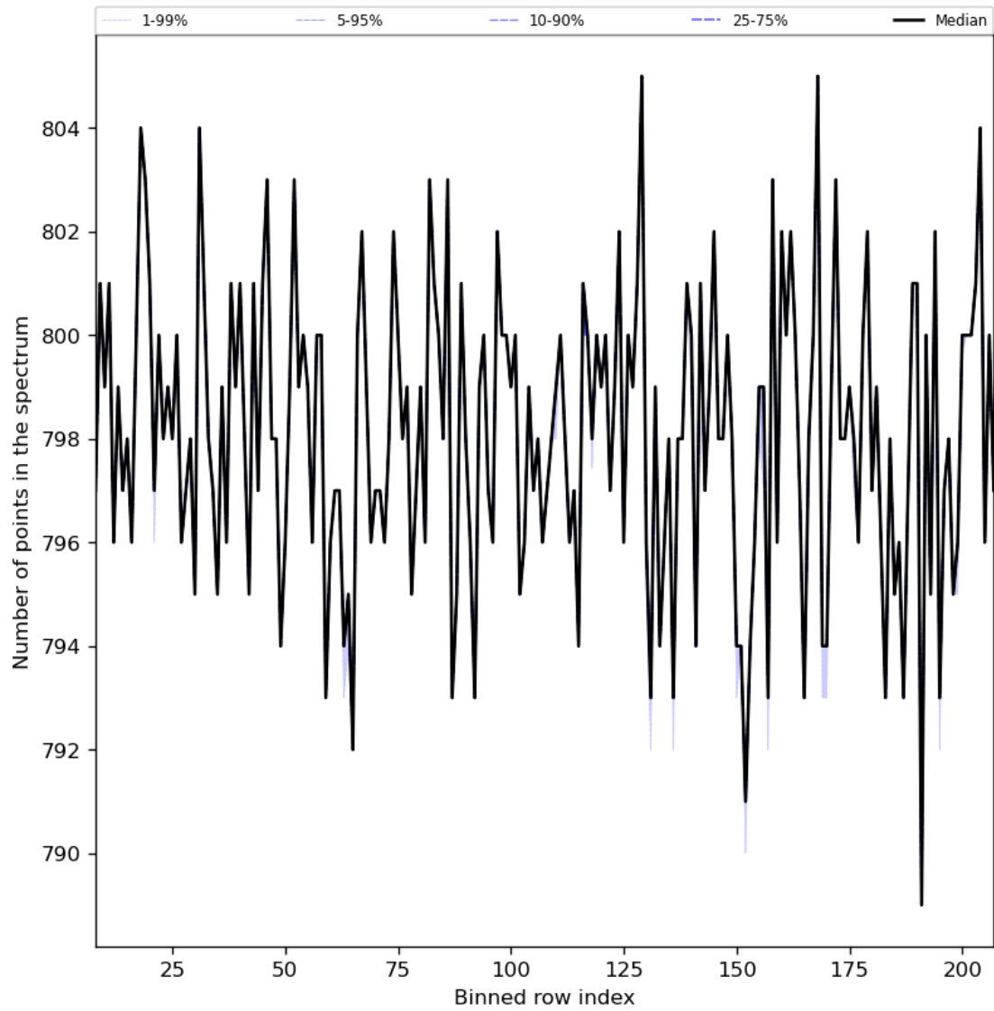
Figure 37: Along track statistics of “Number of points in the spectrum” for 2023-08-06 to 2023-08-08
