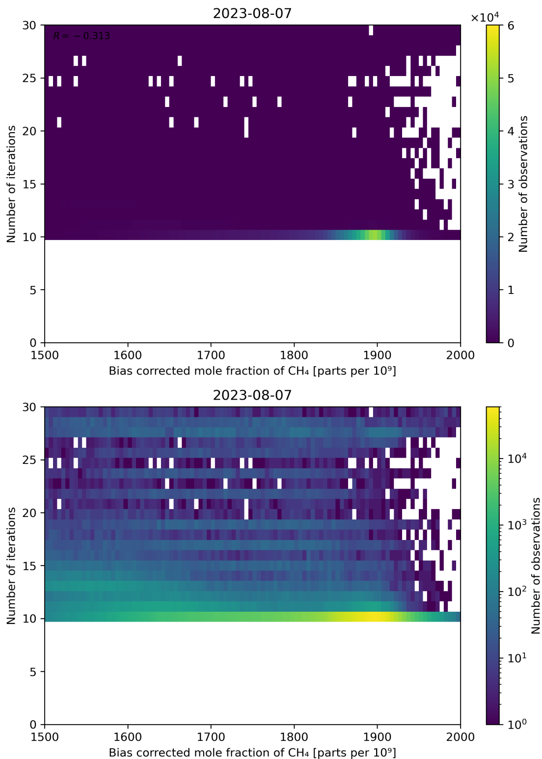
Figure 67: Scatter density plot of “Bias corrected mole fraction of CH 4 ” against “Number of iterations” for 2023-08-06 to 2023-08-08.
