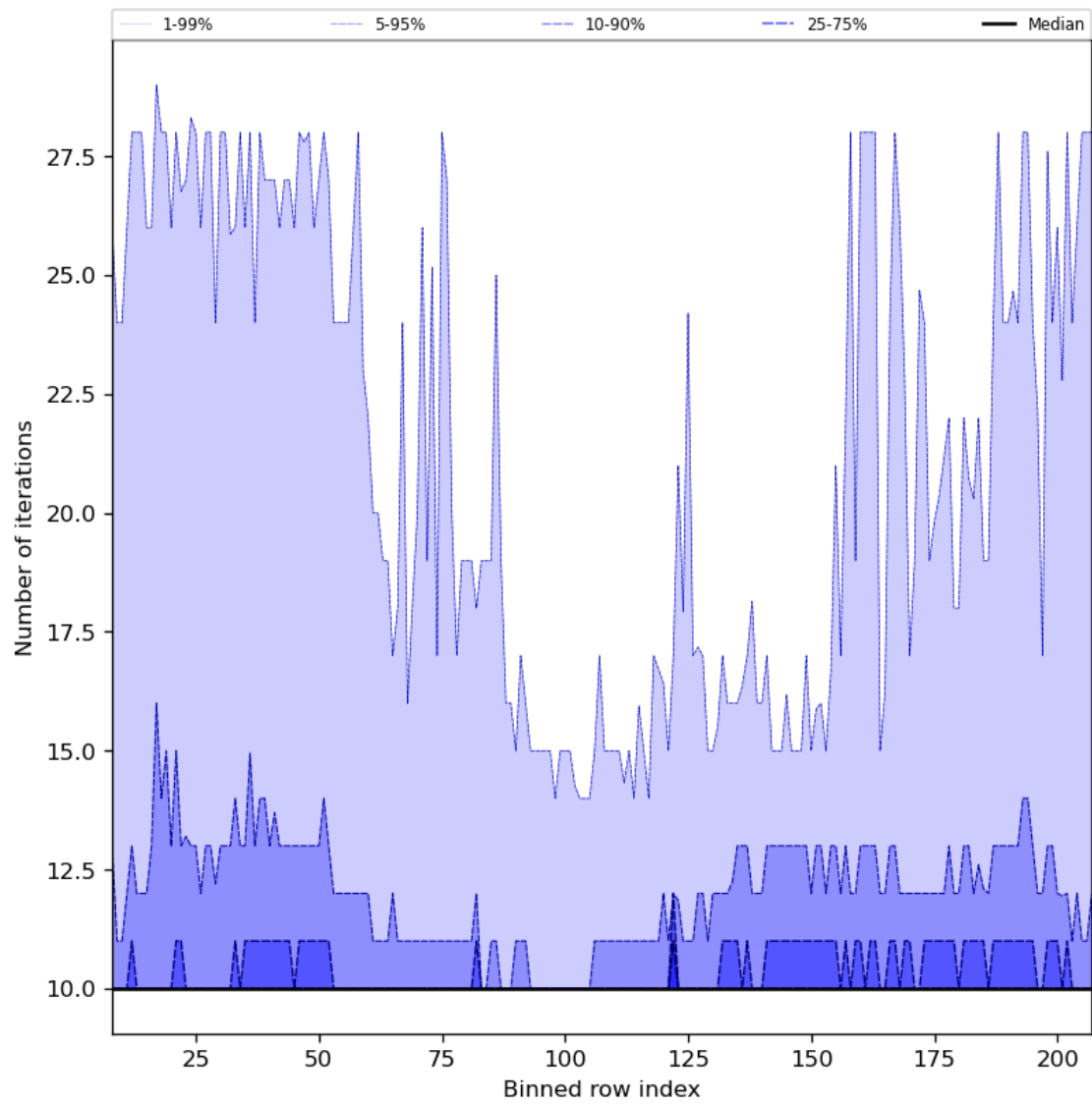
Figure 42: Along track statistics of “Number of iterations” for 2023-08-06 to 2023-08-08
