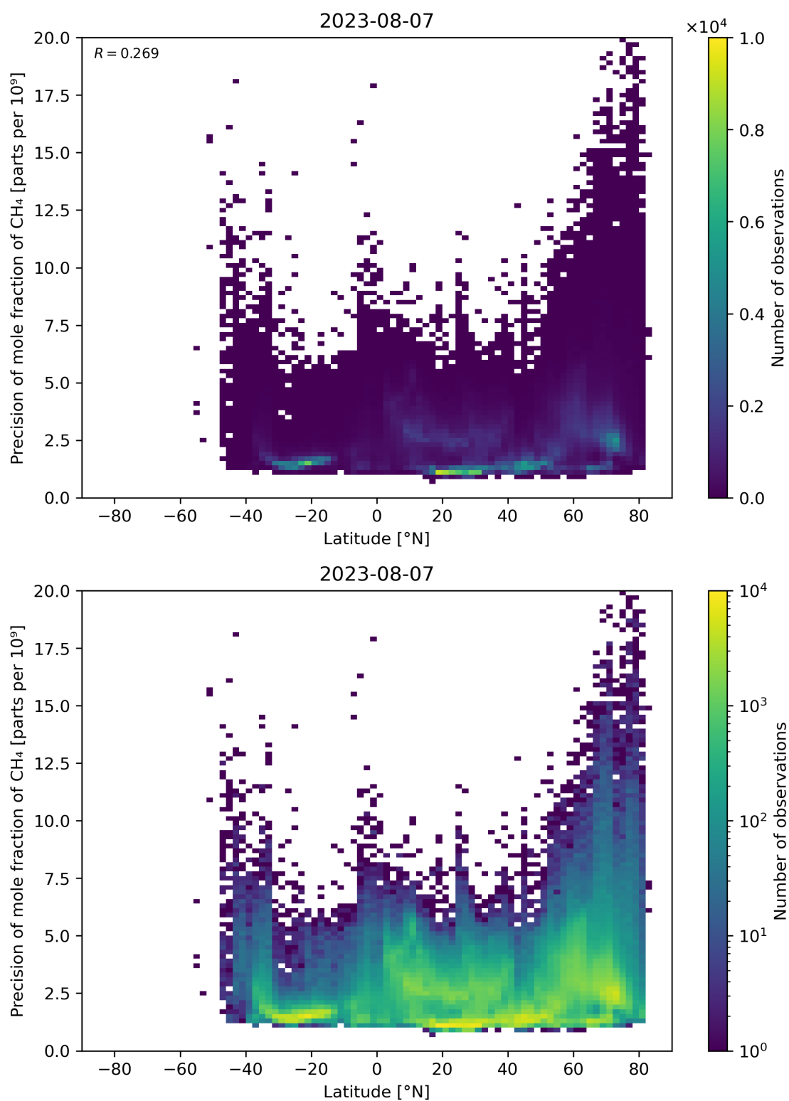
Figure 59: Scatter density plot of “Latitude” against “Precision of mole fraction of \text{CH}_4 ” for 2023-08-06 to 2023-08-08.
