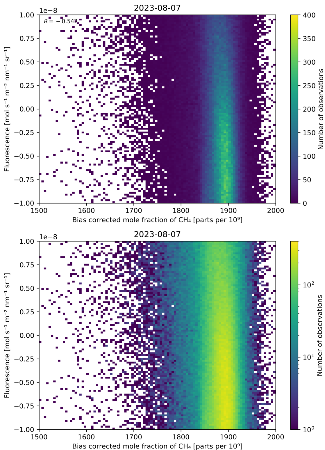
Figure 66: Scatter density plot of “Bias corrected mole fraction of \text{CH}_4 ” against “Fluorescence” for 2023-08-06 to 2023-08-08.
