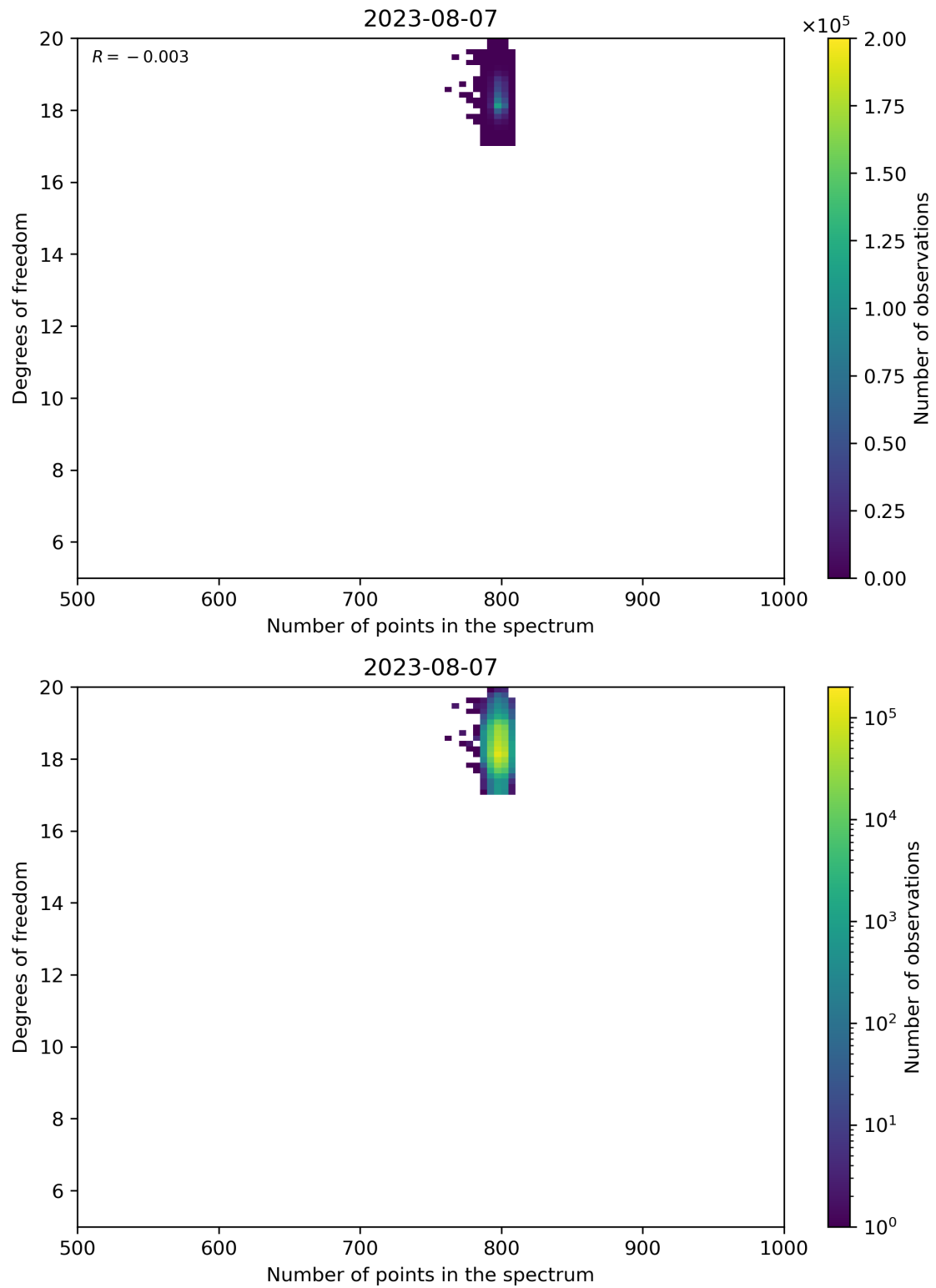
Figure 90: Scatter density plot of “Number of points in the spectrum” against “Degrees of freedom” for 2023-08-06 to 2023-08-08.
