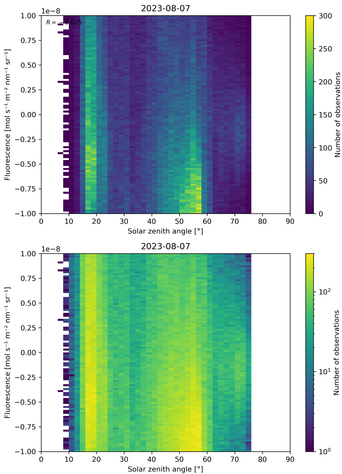
Figure 97: Scatter density plot of “Solar zenith angle” against “Fluorescence” for 2023-08-06 to 2023-08-08.
