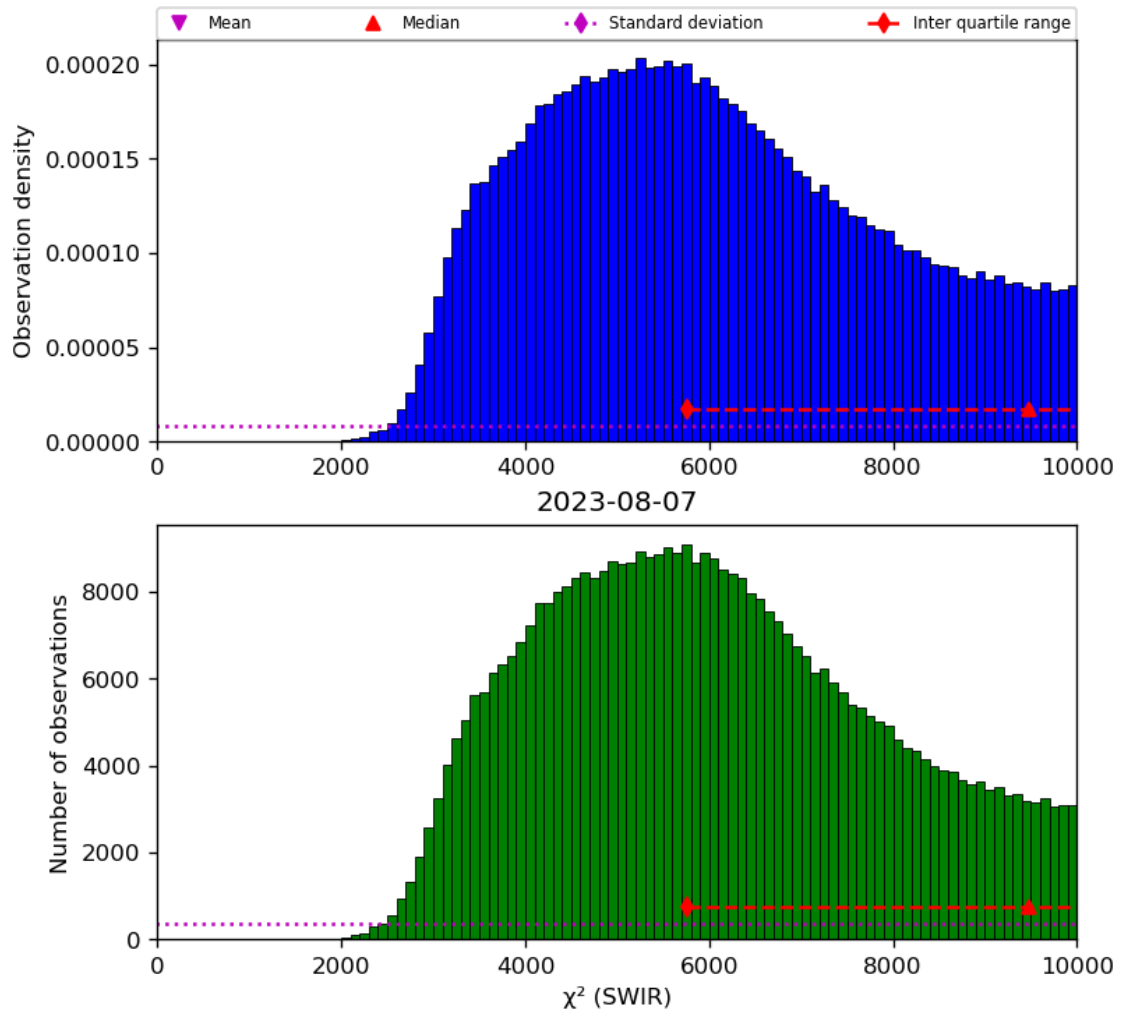
Figure 28: Histogram of “ \chi^2 (SWIR)” for 2023-08-06 to 2023-08-08
