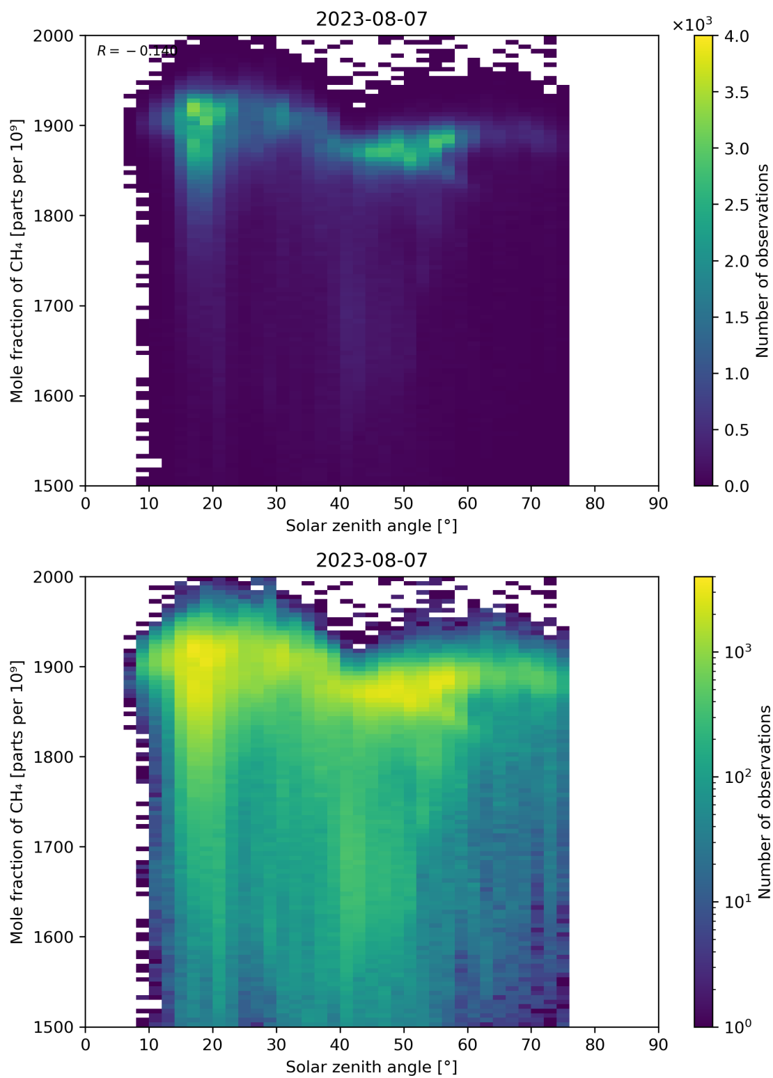
Figure 99: Scatter density plot of “Solar zenith angle” against “Mole fraction of CH 4 ” for 2023-08-06 to 2023-08-08.
