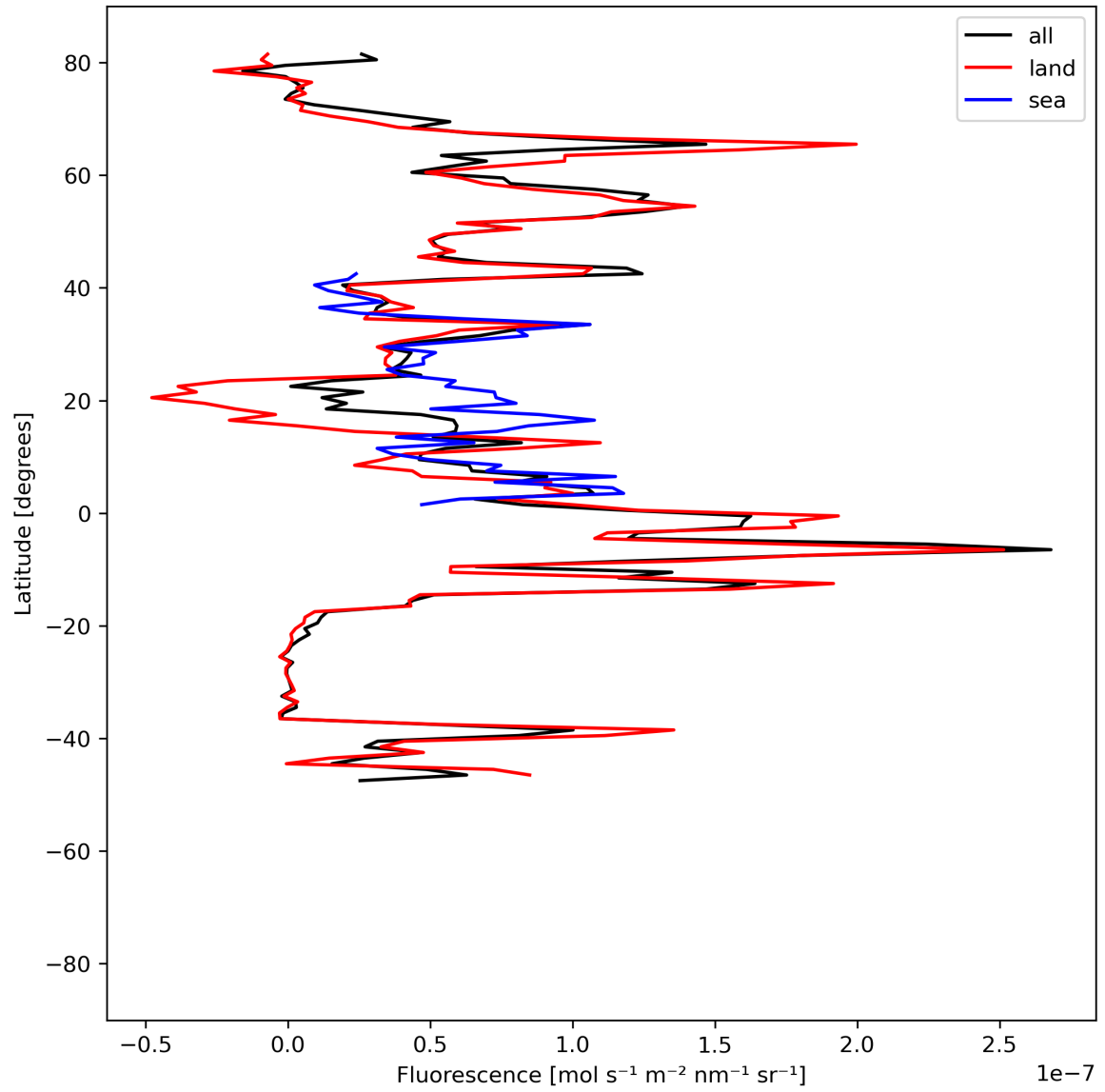
Figure 21: Zonal average of “Fluorescence” for 2023-08-06 to 2023-08-08.
