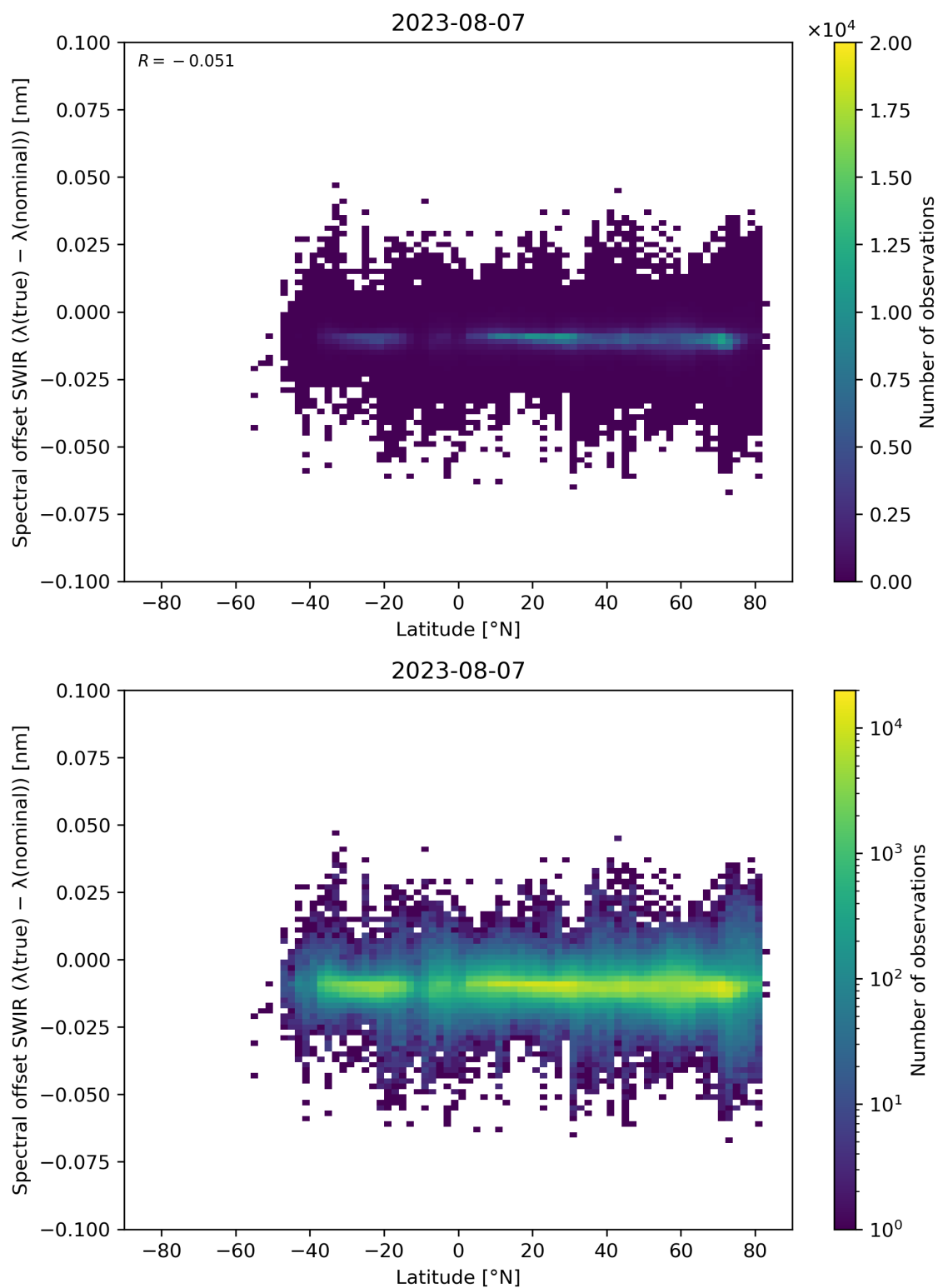
Figure 62: Scatter density plot of “Latitude” against “Spectral offset SWIR ( \lambda(\text{true}) - \lambda(\text{nominal}) )” for 2023-08-06 to 2023-08-08.
