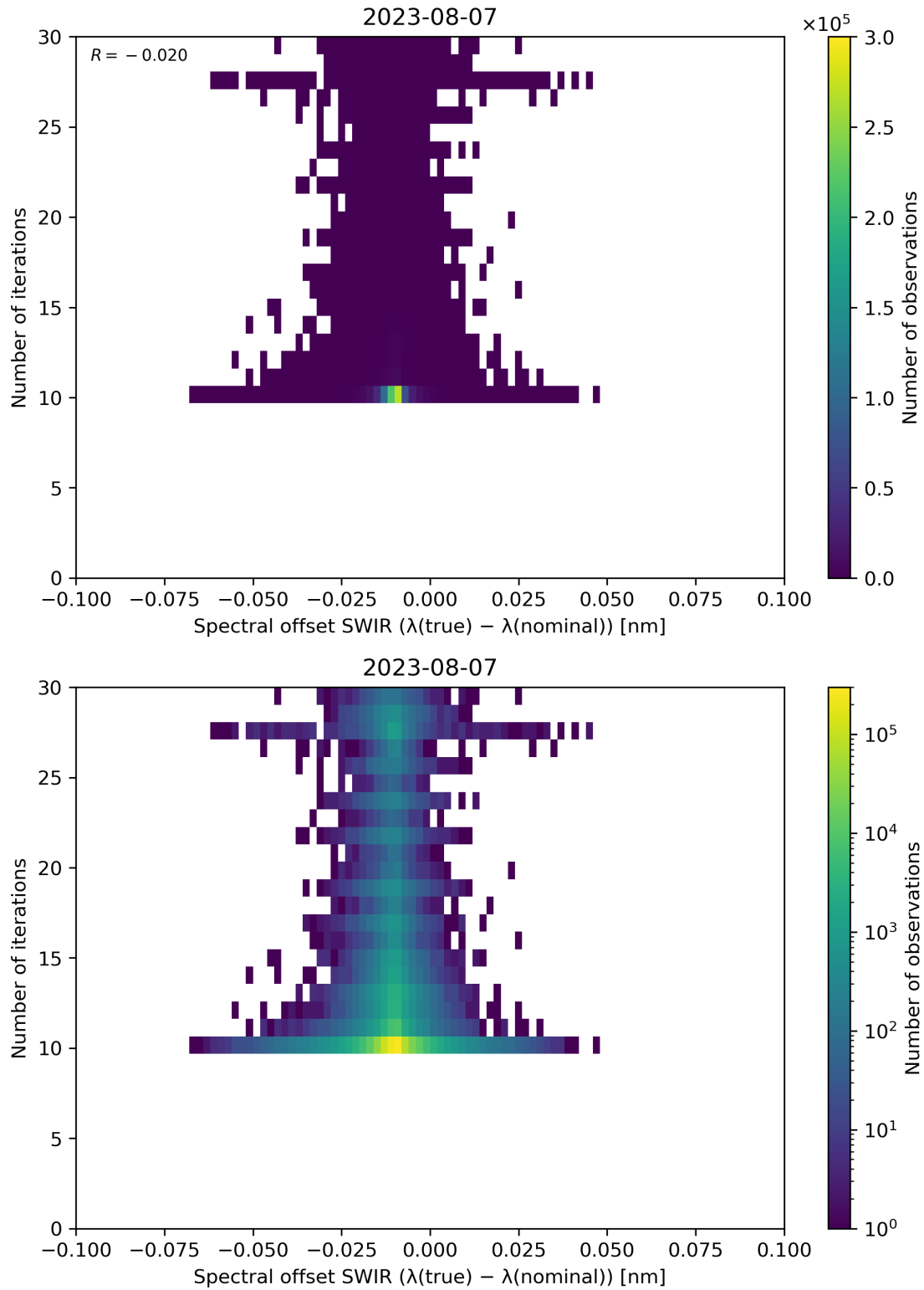
Figure 121: Scatter density plot of “Spectral offset SWIR ( \lambda(\text{true}) - \lambda(\text{nominal}) )” against “Number of iterations” for 2023-08-06 to 2023-08-08.
