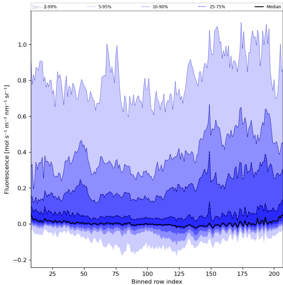
Figure 43: Along track statistics of “Fluorescence” for 2023-08-06 to 2023-08-08
