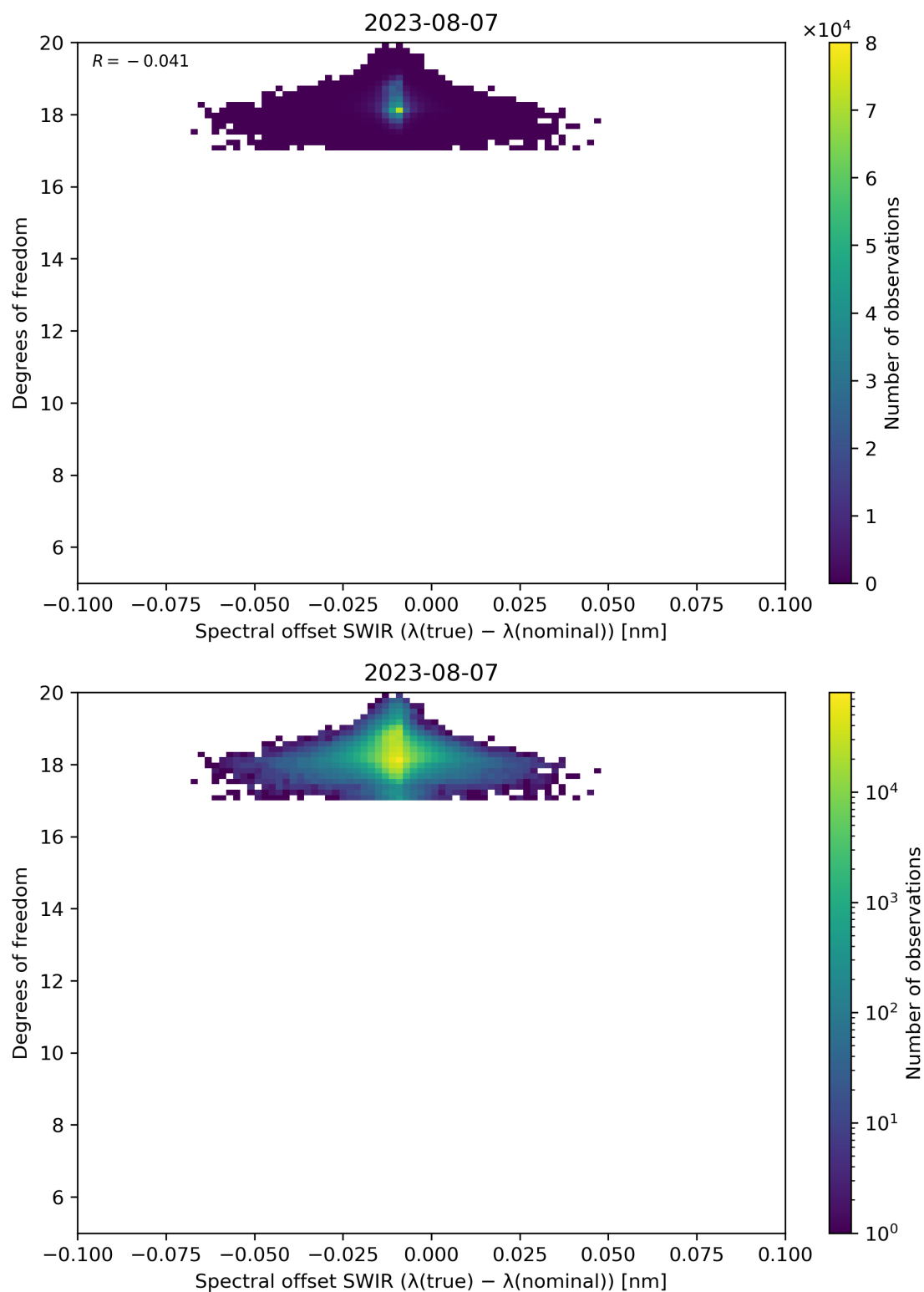
Figure 119: Scatter density plot of “Spectral offset SWIR ( \lambda(\text{true}) - \lambda(\text{nominal}) )” against “Degrees of freedom” for 2023-08-06 to 2023-08-08.
