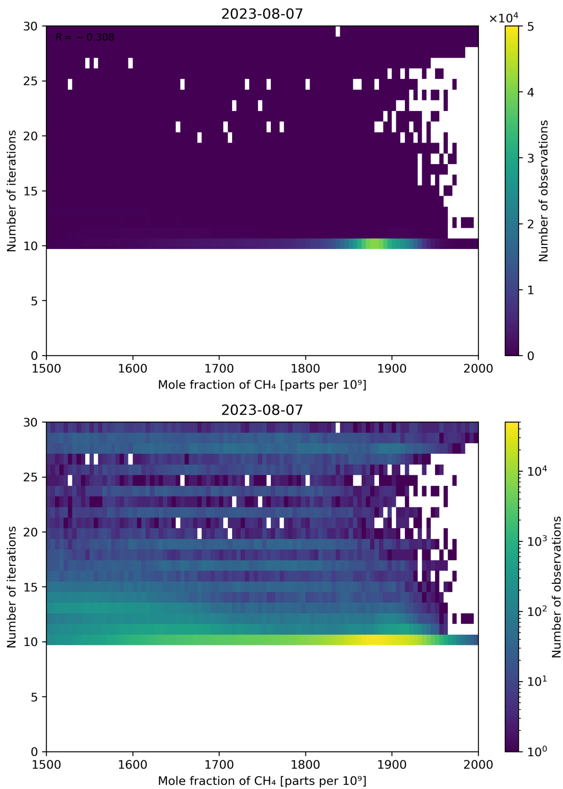
Figure 76: Scatter density plot of “Mole fraction of CH 4 ” against “Number of iterations” for 2023-08-06 to 2023-08-08.
