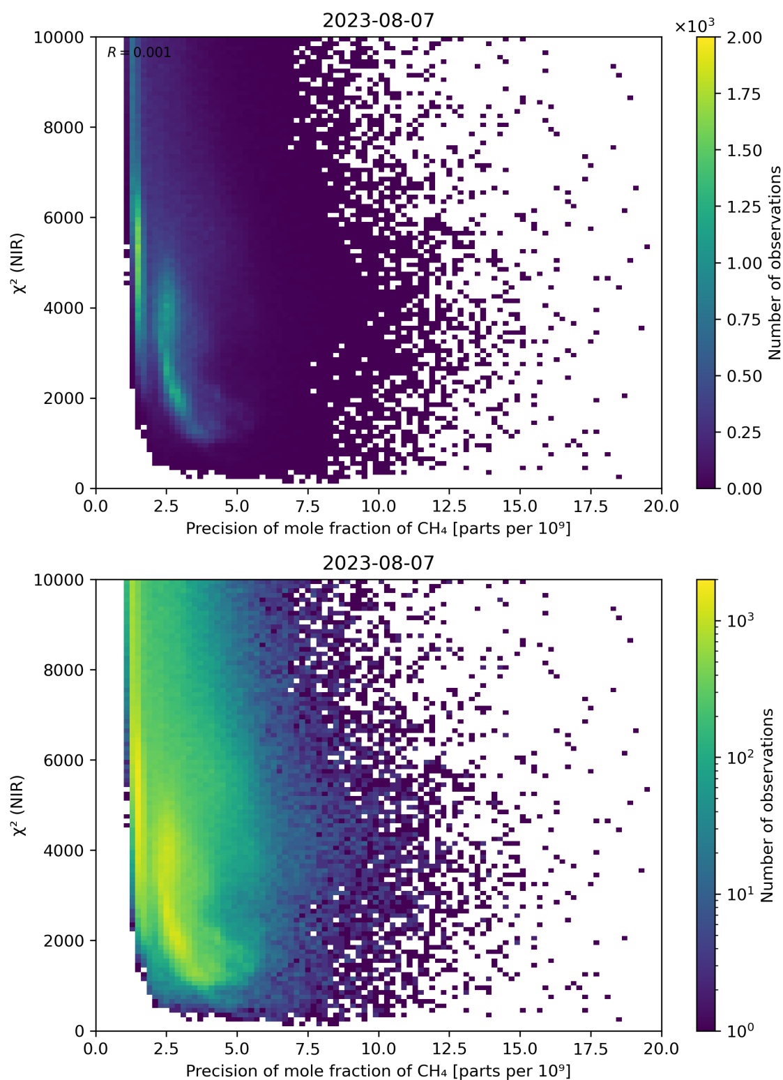
Figure 78: Scatter density plot of “Precision of mole fraction of \text{CH}_4 ” against “ \chi^2 (NIR)” for 2023-08-06 to 2023-08-08.
