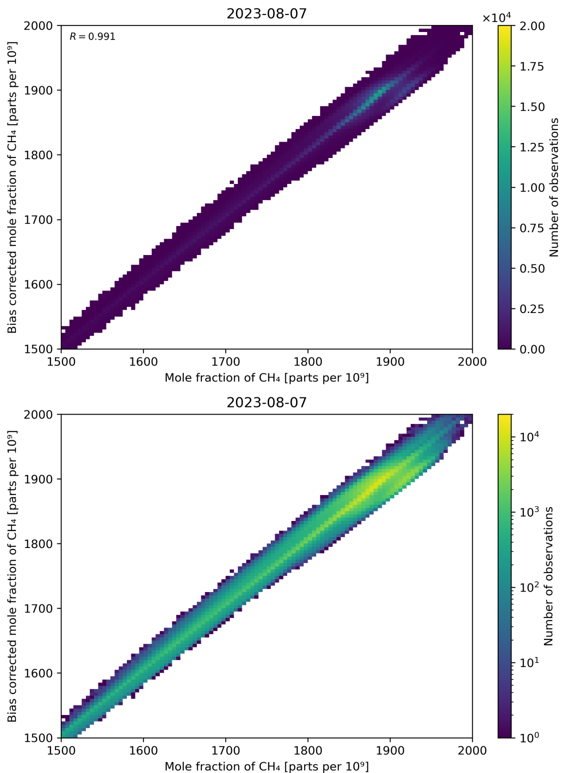
Figure 74: Scatter density plot of “Mole fraction of CH 4 ” against “Bias corrected mole fraction of CH 4 ” for 2023-08-06 to 2023-08-08.
