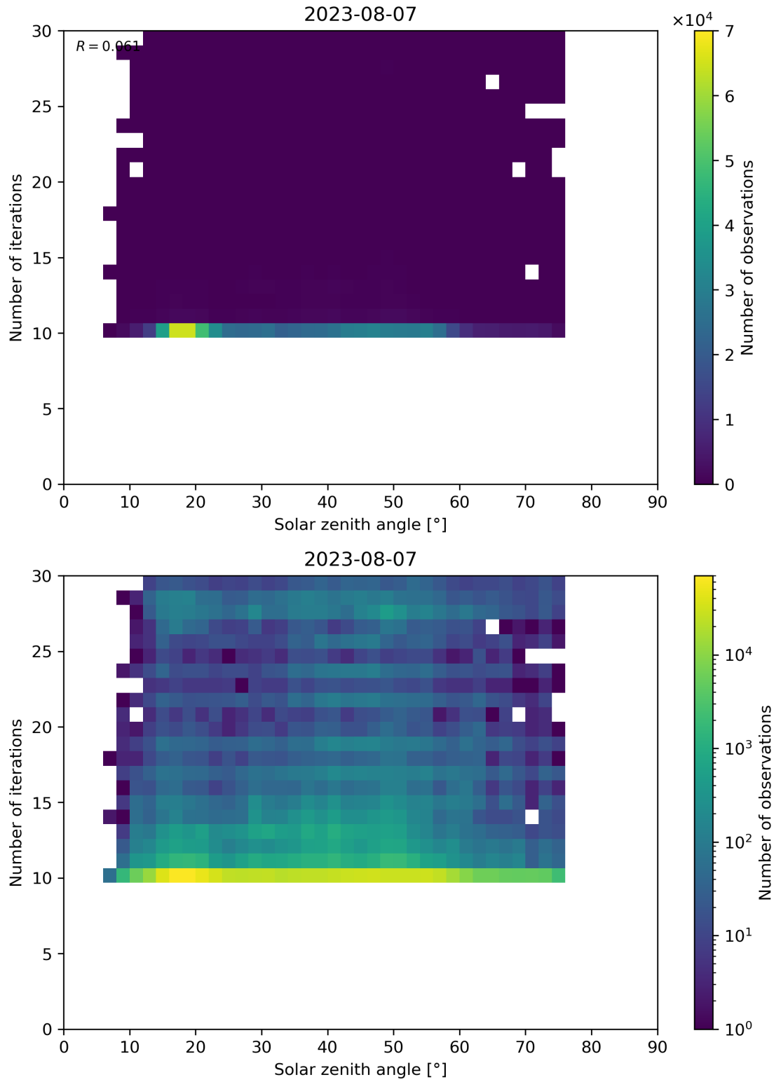
Figure 102: Scatter density plot of “Solar zenith angle” against “Number of iterations” for 2023-08-06 to 2023-08-08.
