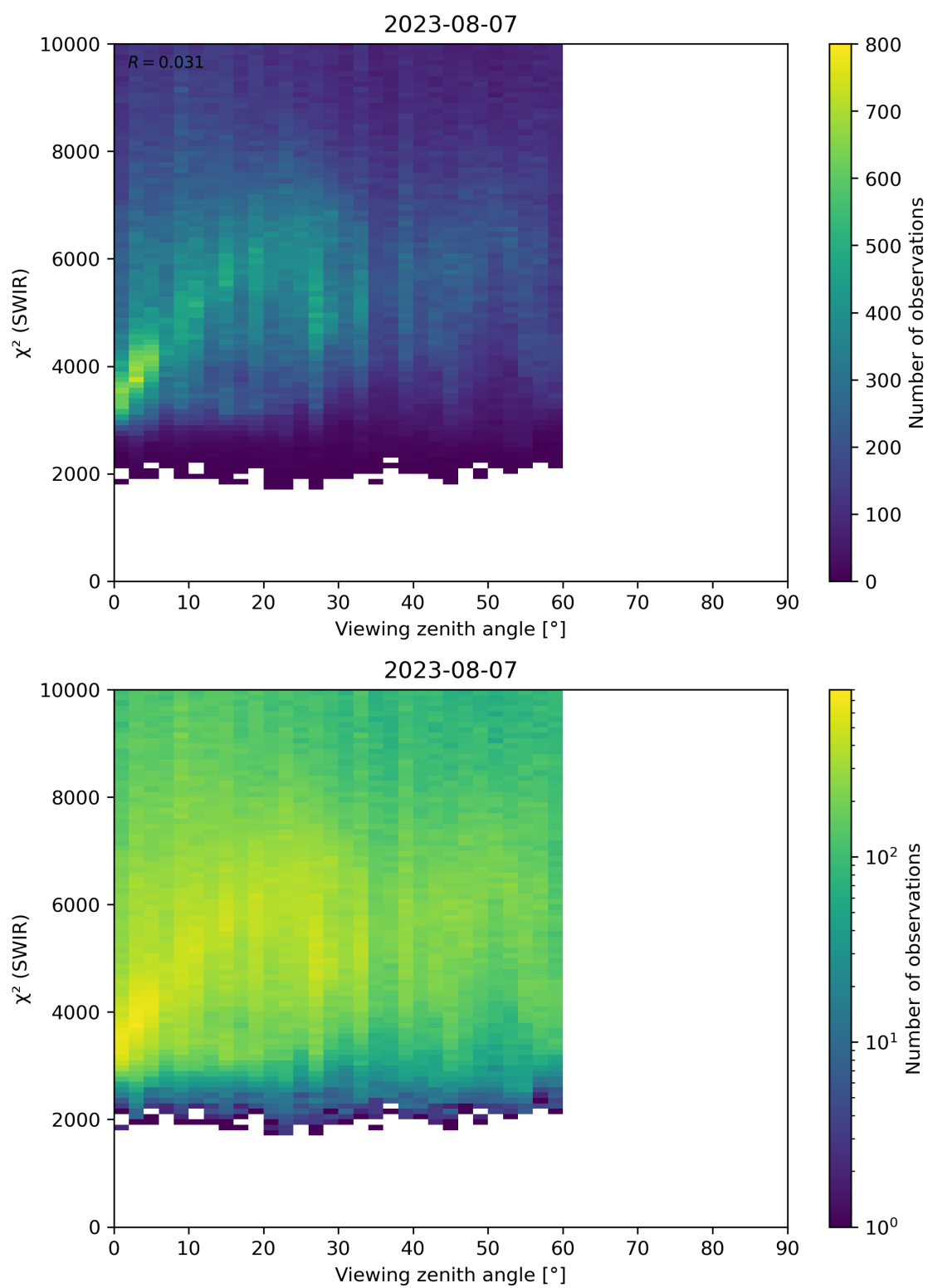
Figure 106: Scatter density plot of “Viewing zenith angle” against “ \chi^2 (SWIR)” for 2023-08-06 to 2023-08-08.
