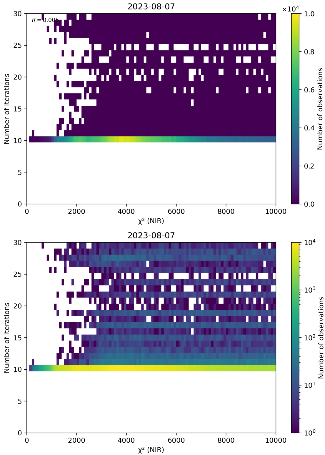
Figure 46: Scatter density plot of “ \chi^2 (NIR)” against “Number of iterations” for 2023-08-06 to 2023-08-08.
