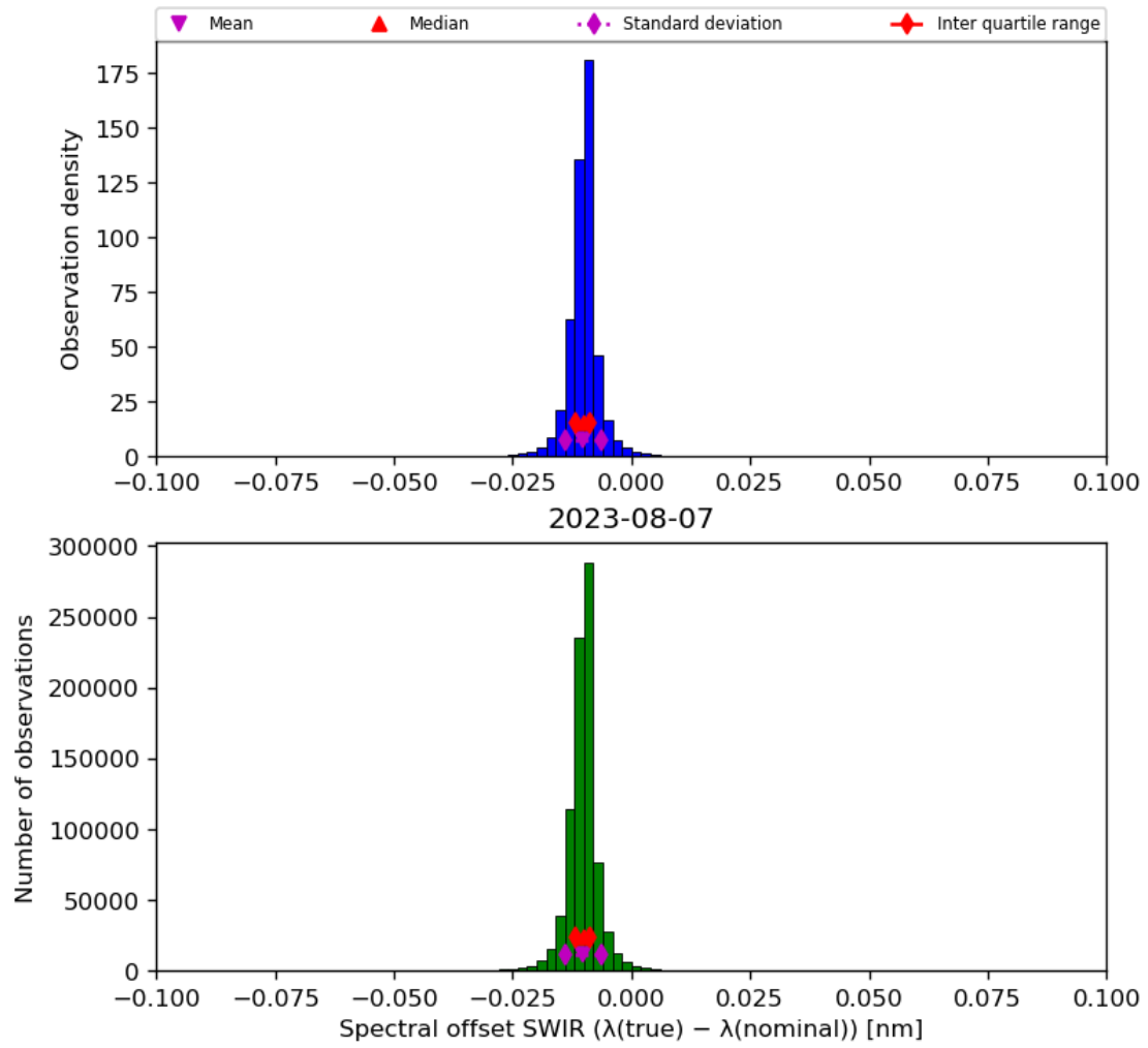
Figure 27: Histogram of “Spectral offset SWIR ( \lambda(\text{true}) - \lambda(\text{nominal}) )” for 2023-08-06 to 2023-08-08
