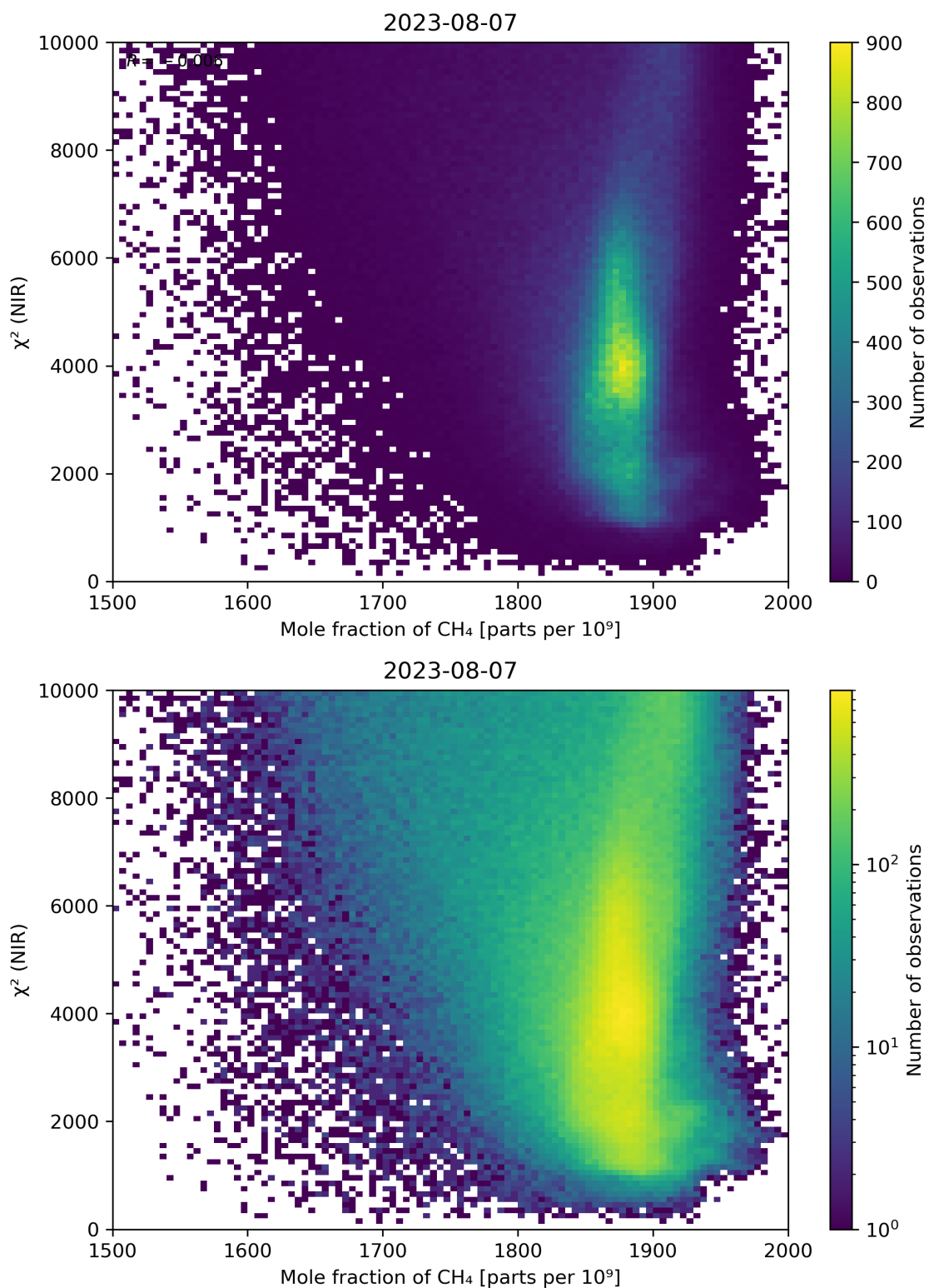
Figure 70: Scatter density plot of “Mole fraction of CH 4 ” against “ \chi^2 (NIR)” for 2023-08-06 to 2023-08-08.
