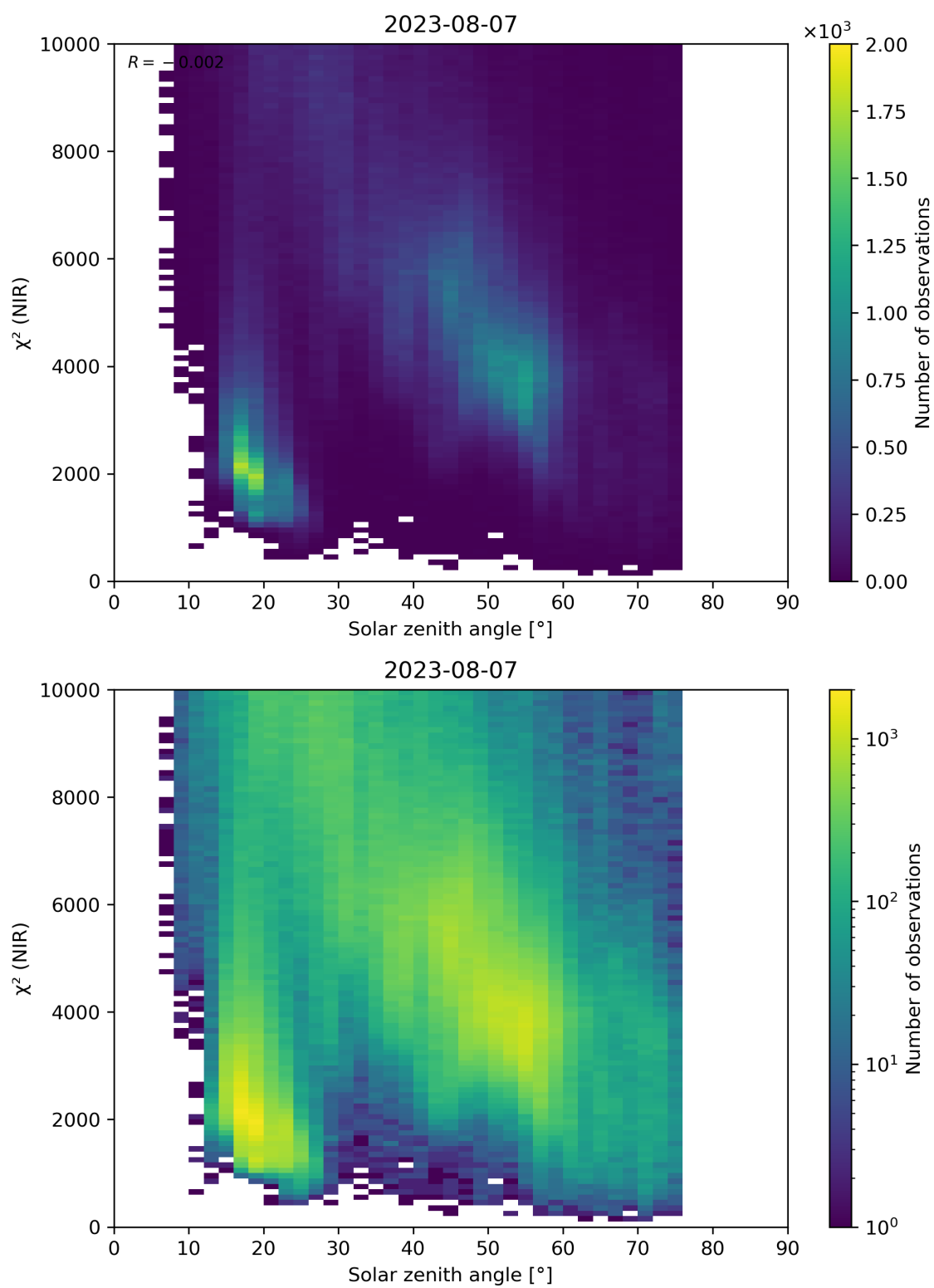
Figure 94: Scatter density plot of “Solar zenith angle” against “ \chi^2 (NIR)” for 2023-08-06 to 2023-08-08.
