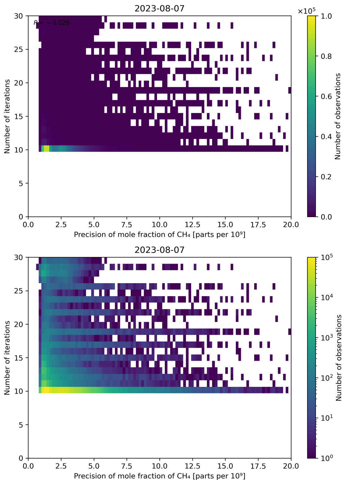
Figure 83: Scatter density plot of “Precision of mole fraction of CH 4 ” against “Number of iterations” for 2023-08-06 to 2023-08-08.
