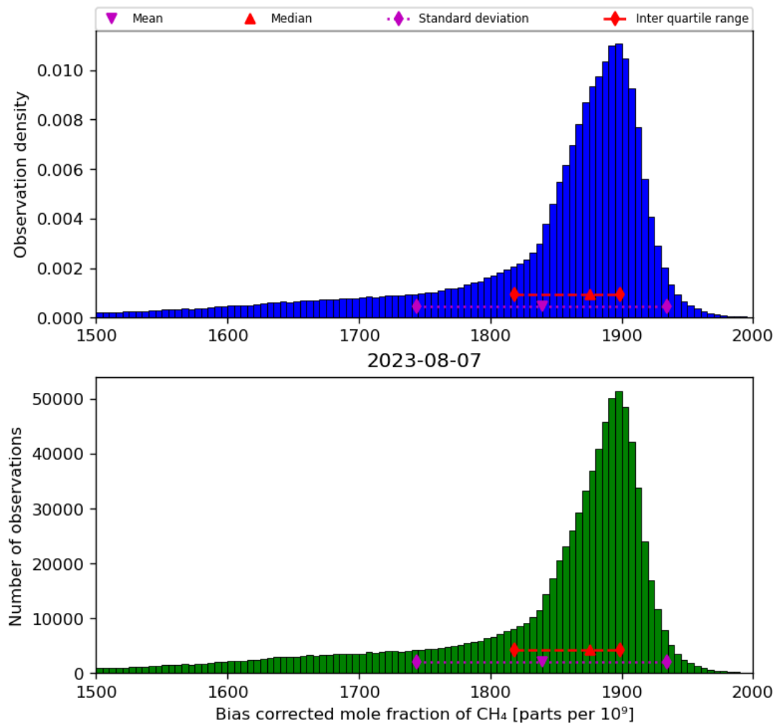
Figure 25: Histogram of “Bias corrected mole fraction of CH 4 ” for 2023-08-06 to 2023-08-08
