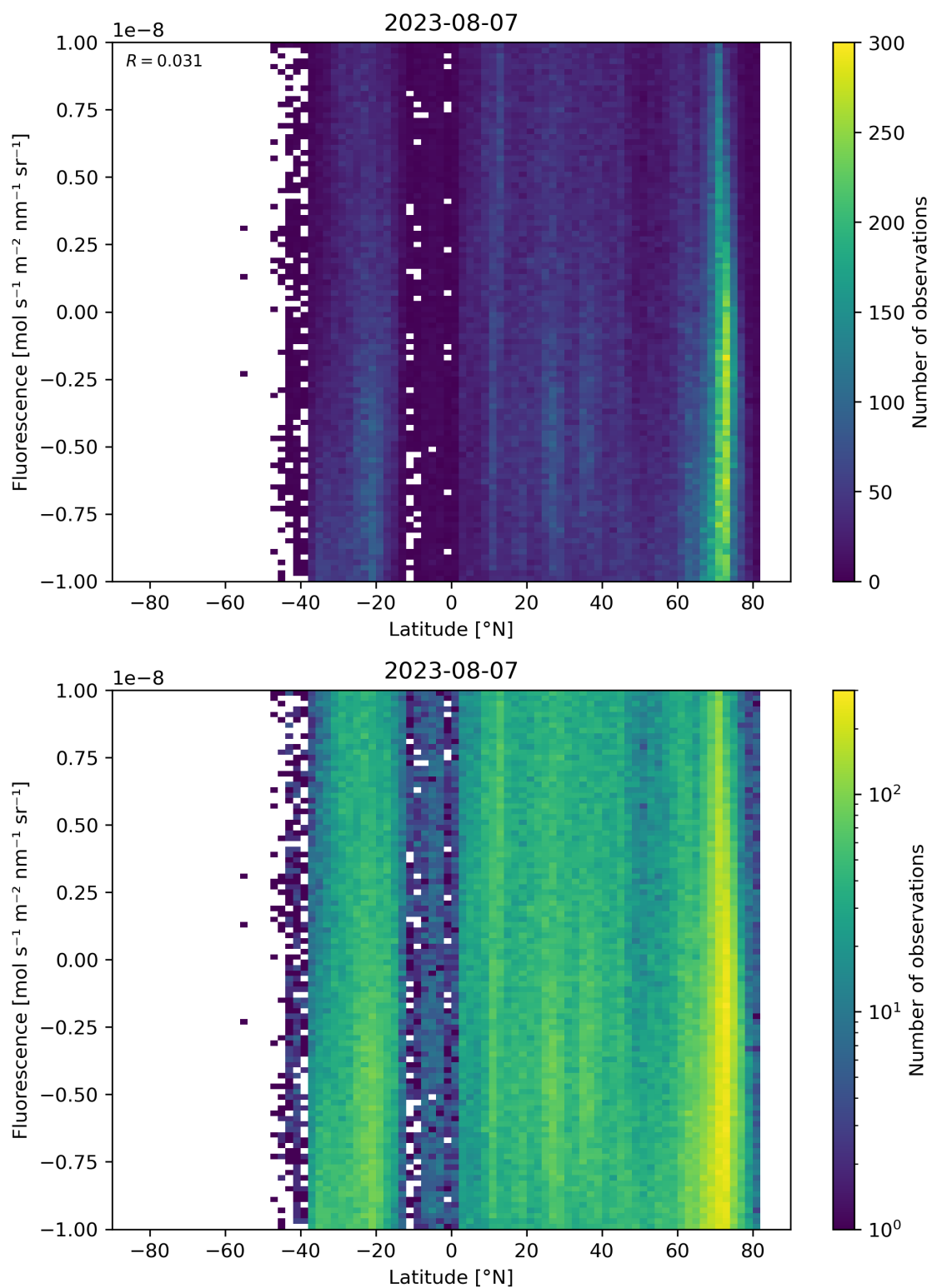
Figure 56: Scatter density plot of “Latitude” against “Fluorescence” for 2023-08-06 to 2023-08-08.
