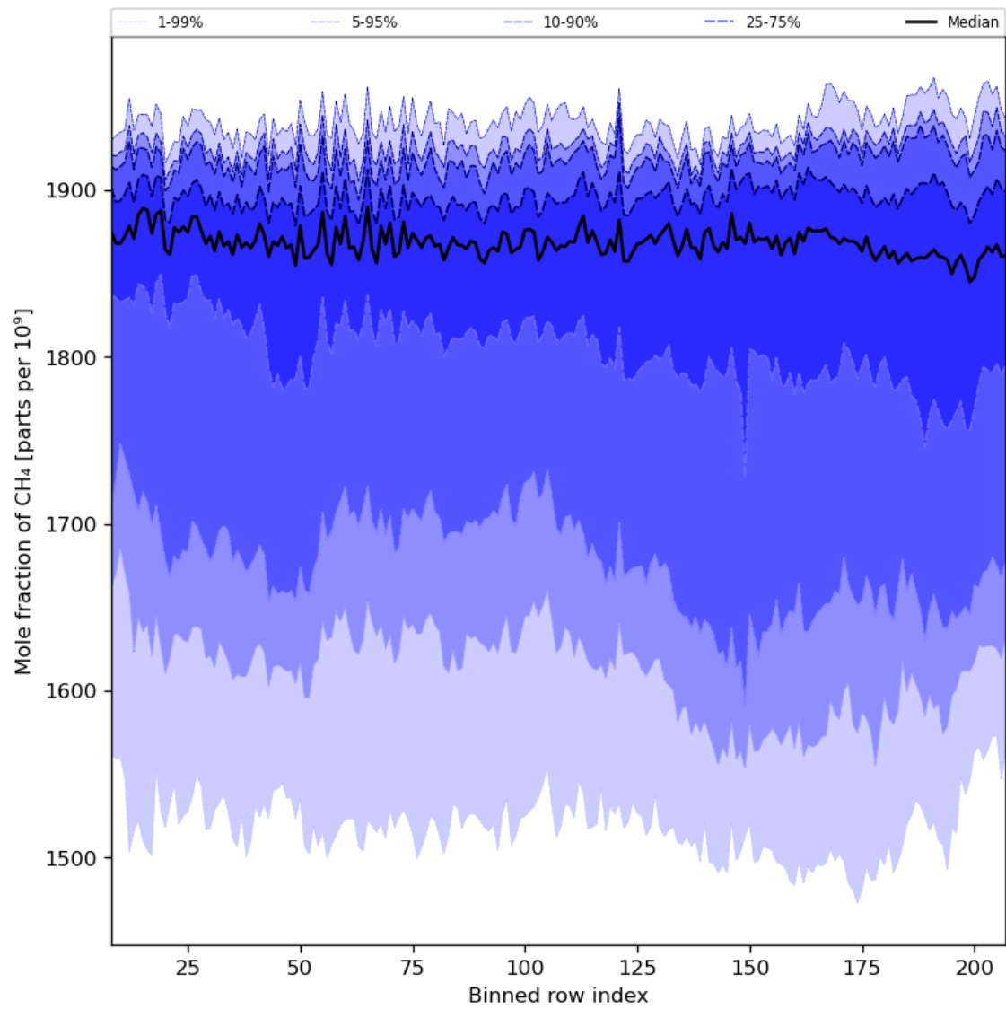
Figure 34: Along track statistics of “Mole fraction of CH 4 ” for 2023-08-06 to 2023-08-08
