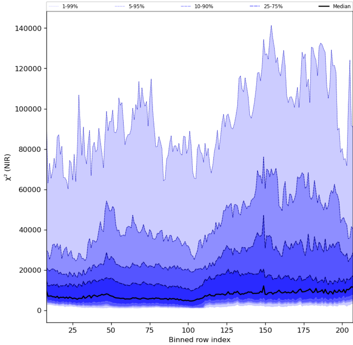
Figure 40: Along track statistics of " \chi^2 (NIR)" for 2023-08-06 to 2023-08-08
