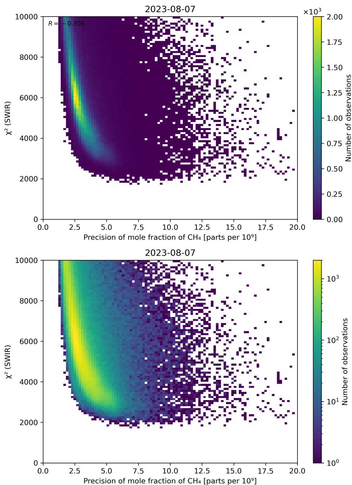
Figure 79: Scatter density plot of “Precision of mole fraction of CH 4 ” against “ \chi^2 (SWIR)” for 2023-08-06 to 2023-08-08.
