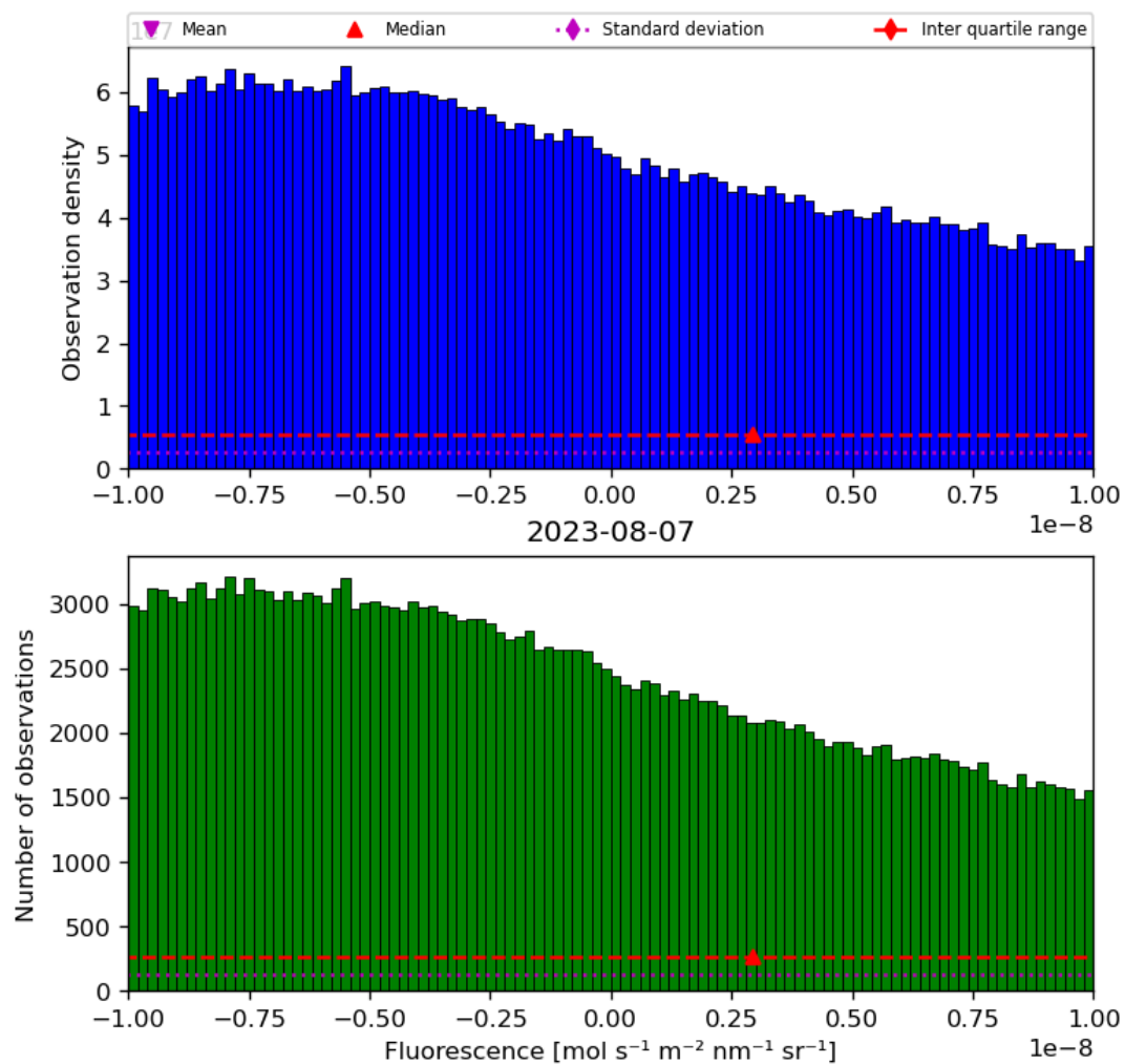
Figure 32: Histogram of “Fluorescence” for 2023-08-06 to 2023-08-08
