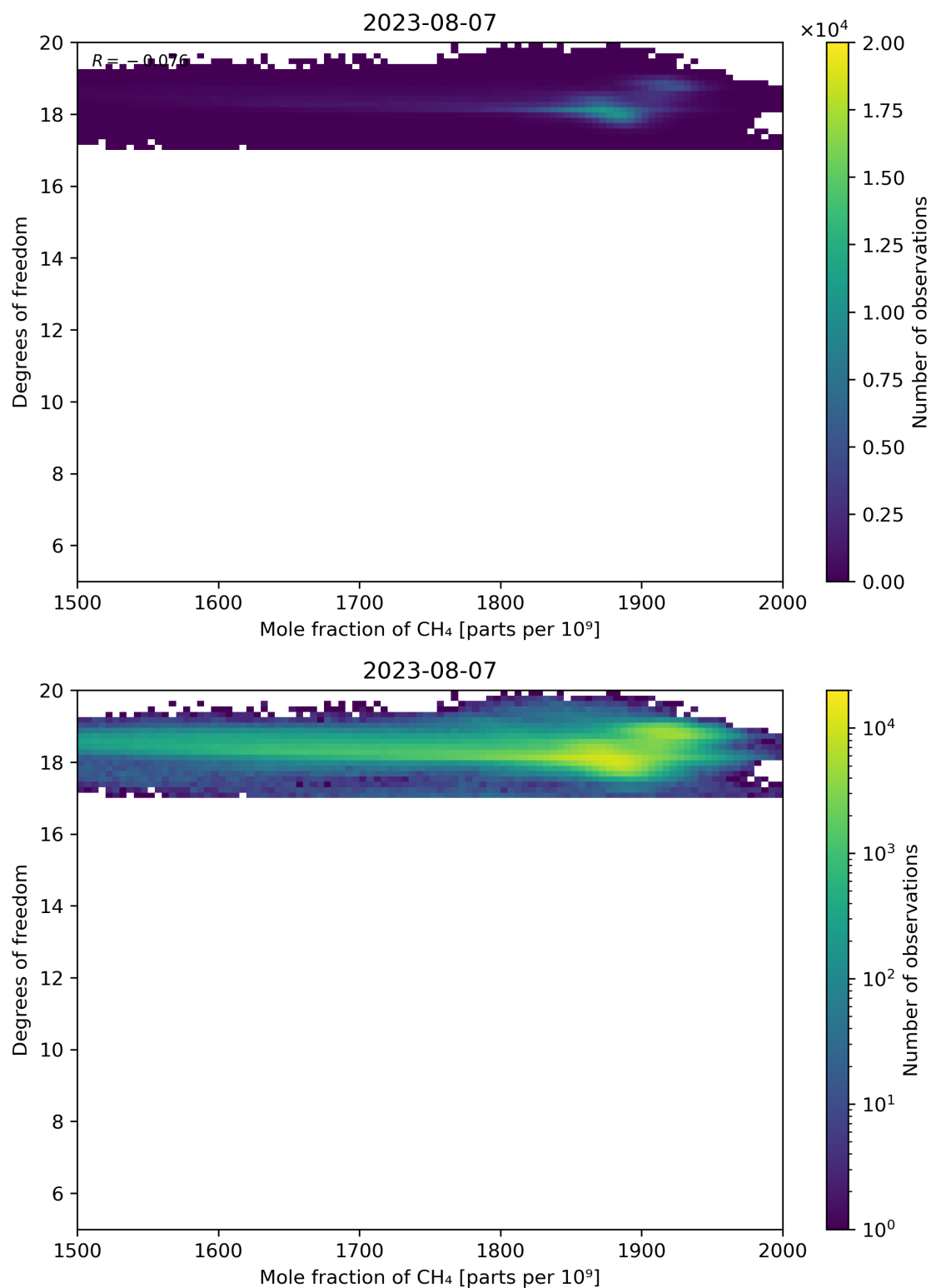
Figure 72: Scatter density plot of “Mole fraction of CH 4 ” against “Degrees of freedom” for 2023-08-06 to 2023-08-08.
