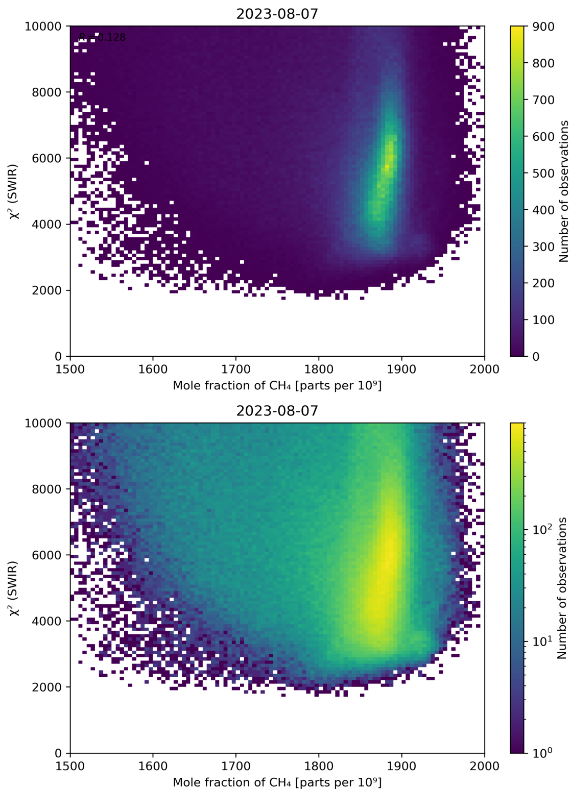
Figure 71: Scatter density plot of “Mole fraction of CH 4 ” against “ \chi^2 (SWIR)” for 2023-08-06 to 2023-08-08.
