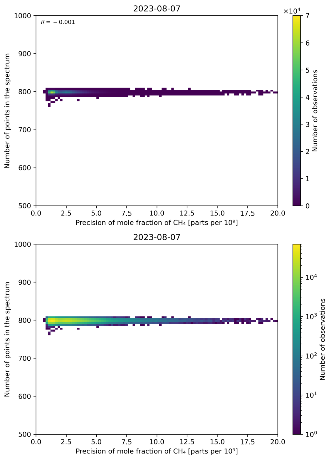
Figure 84: Scatter density plot of “Precision of mole fraction of CH 4 ” against “Number of points in the spectrum” for 2023-08-06 to 2023-08-08.
