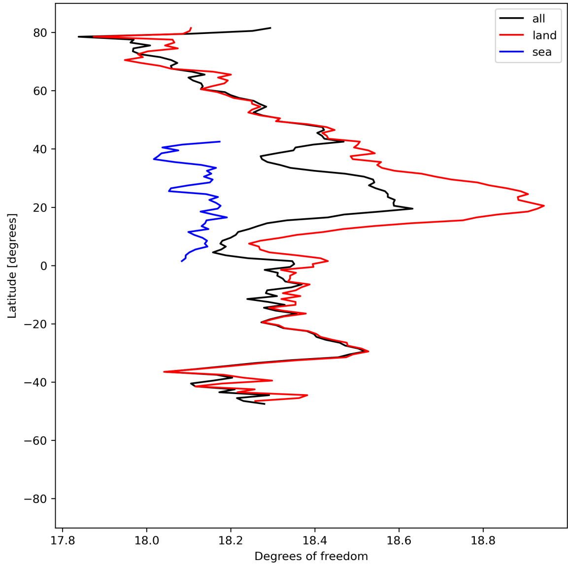
Figure 19: Zonal average of “Degrees of freedom” for 2023-08-06 to 2023-08-08.
