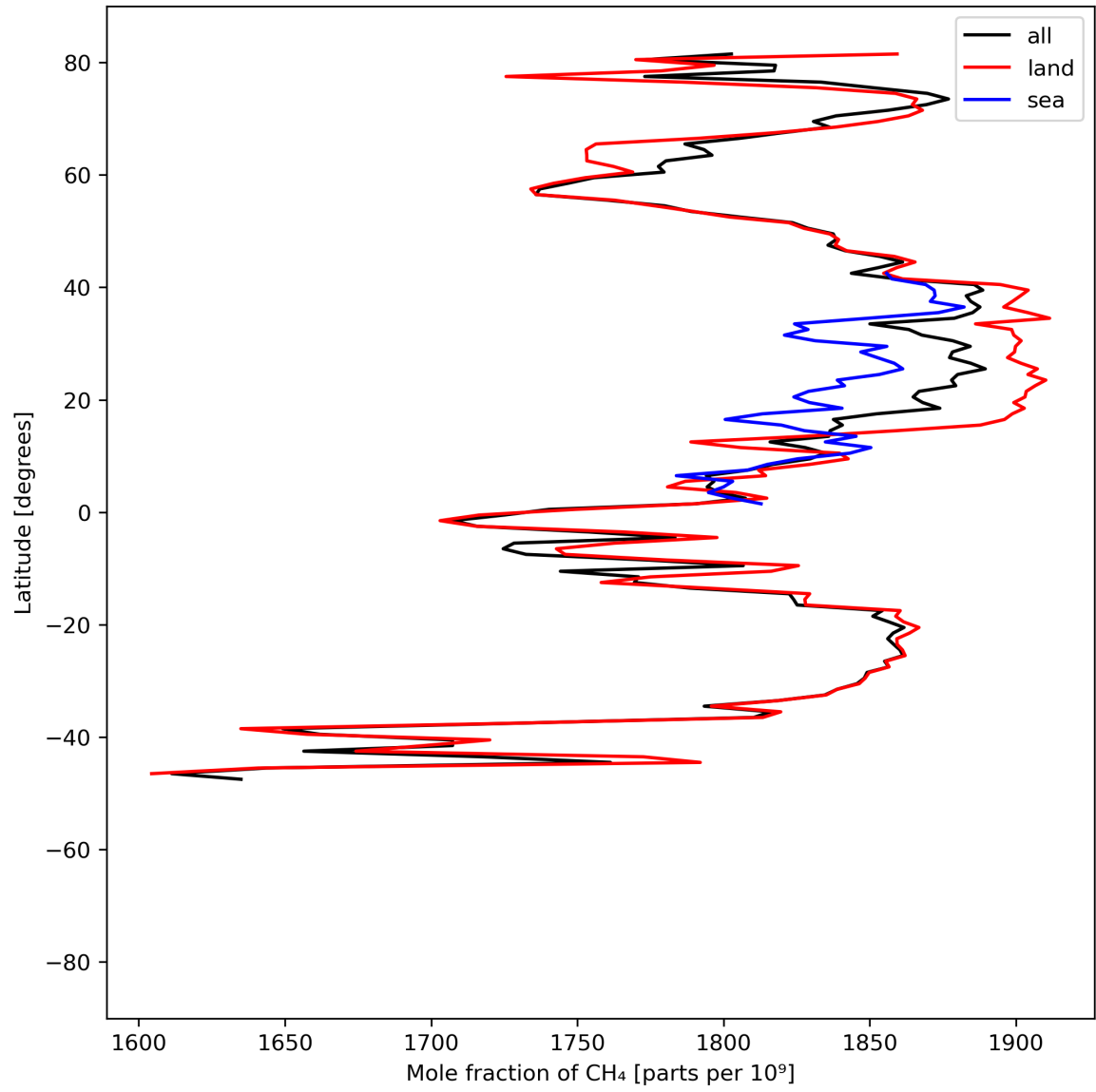
Figure 12: Zonal average of “Mole fraction of CH 4 ” for 2023-08-06 to 2023-08-08.
