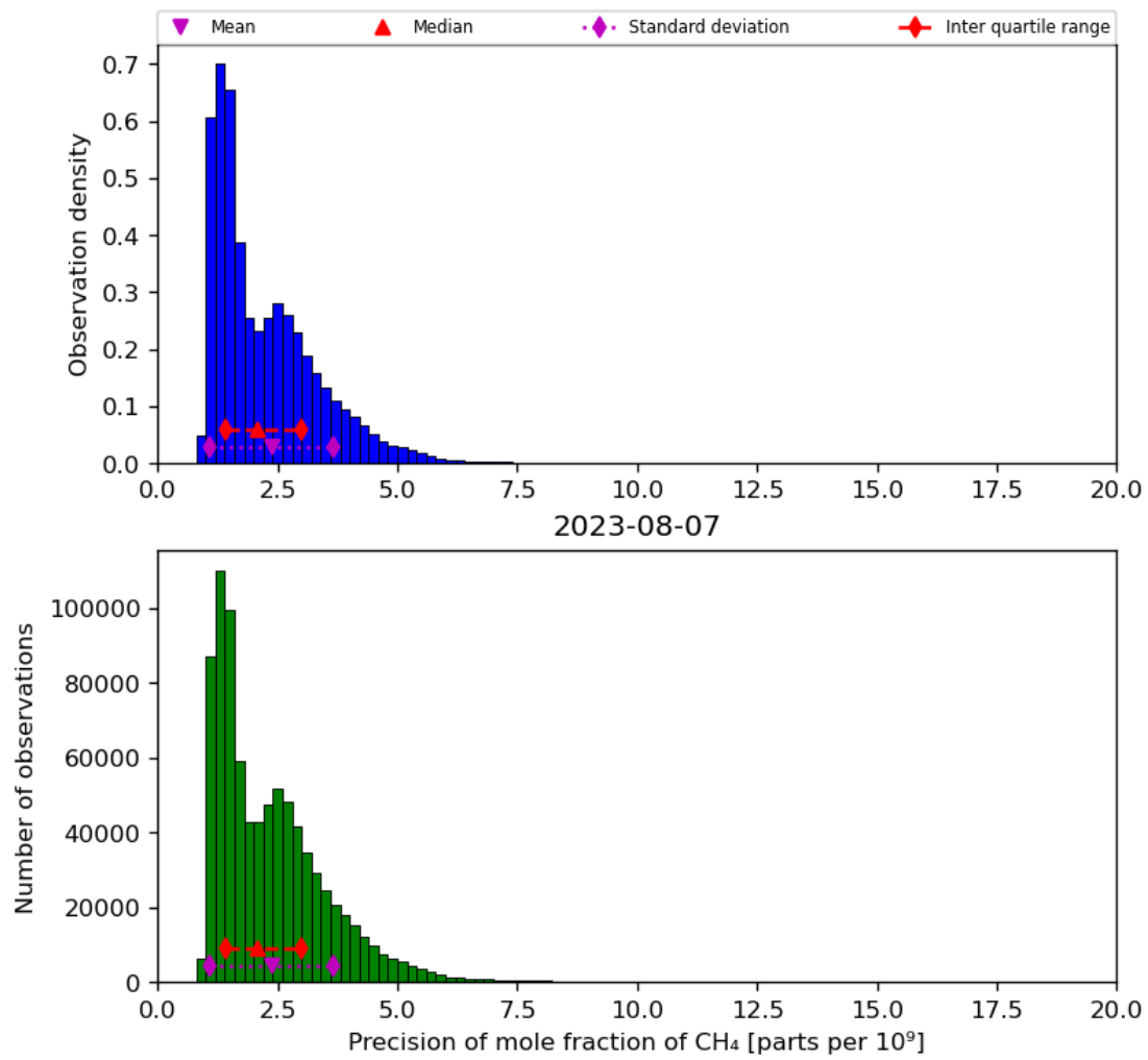
Figure 24: Histogram of “Precision of mole fraction of CH 4 ” for 2023-08-06 to 2023-08-08
