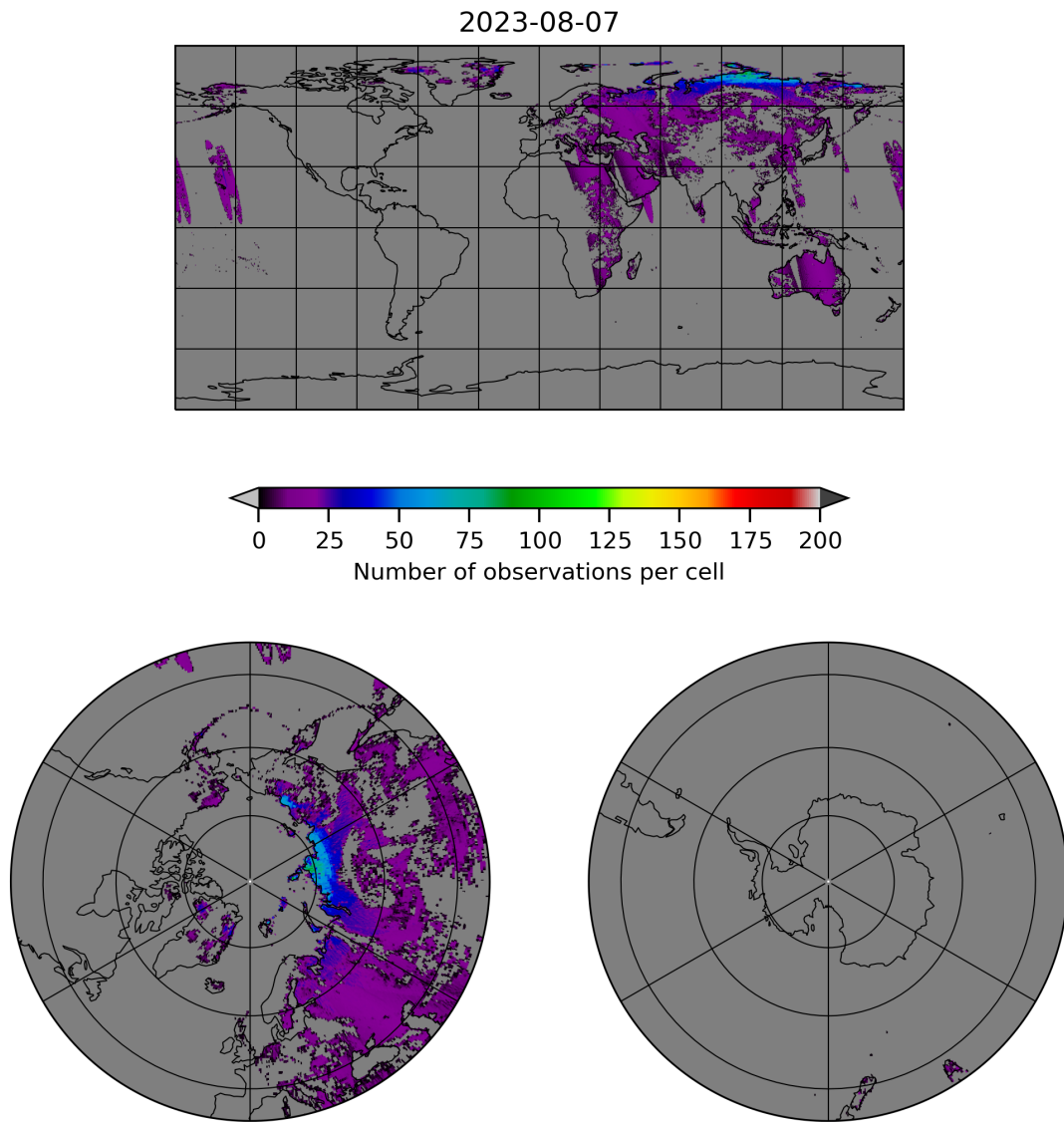
Figure 10: Map of the number of observations for 2023-08-06 to 2023-08-08
