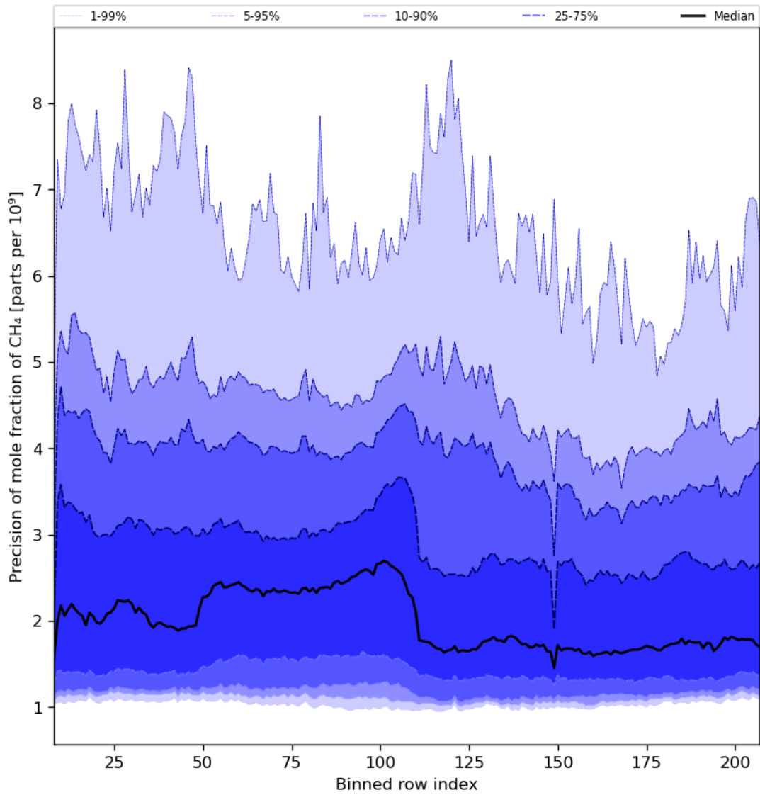
Figure 35: Along track statistics of “Precision of mole fraction of CH 4 ” for 2023-08-06 to 2023-08-08
