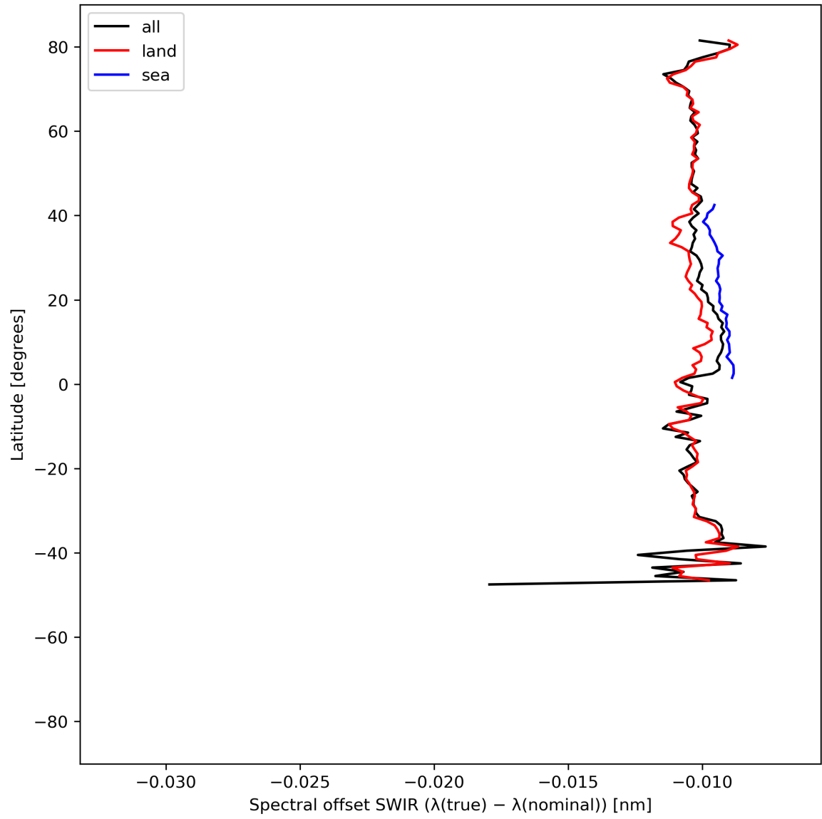
Figure 16: Zonal average of “Spectral offset SWIR ( \lambda(\text{true}) - \lambda(\text{nominal}) )” for 2023-08-06 to 2023-08-08.
