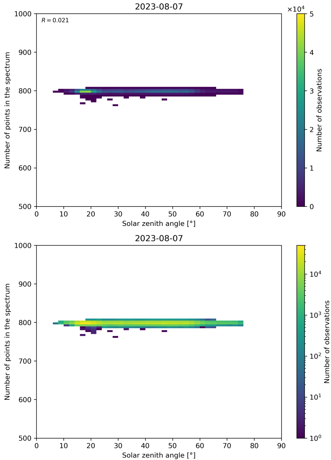
Figure 103: Scatter density plot of “Solar zenith angle” against “Number of points in the spectrum” for 2023-08-06 to 2023-08-08.
