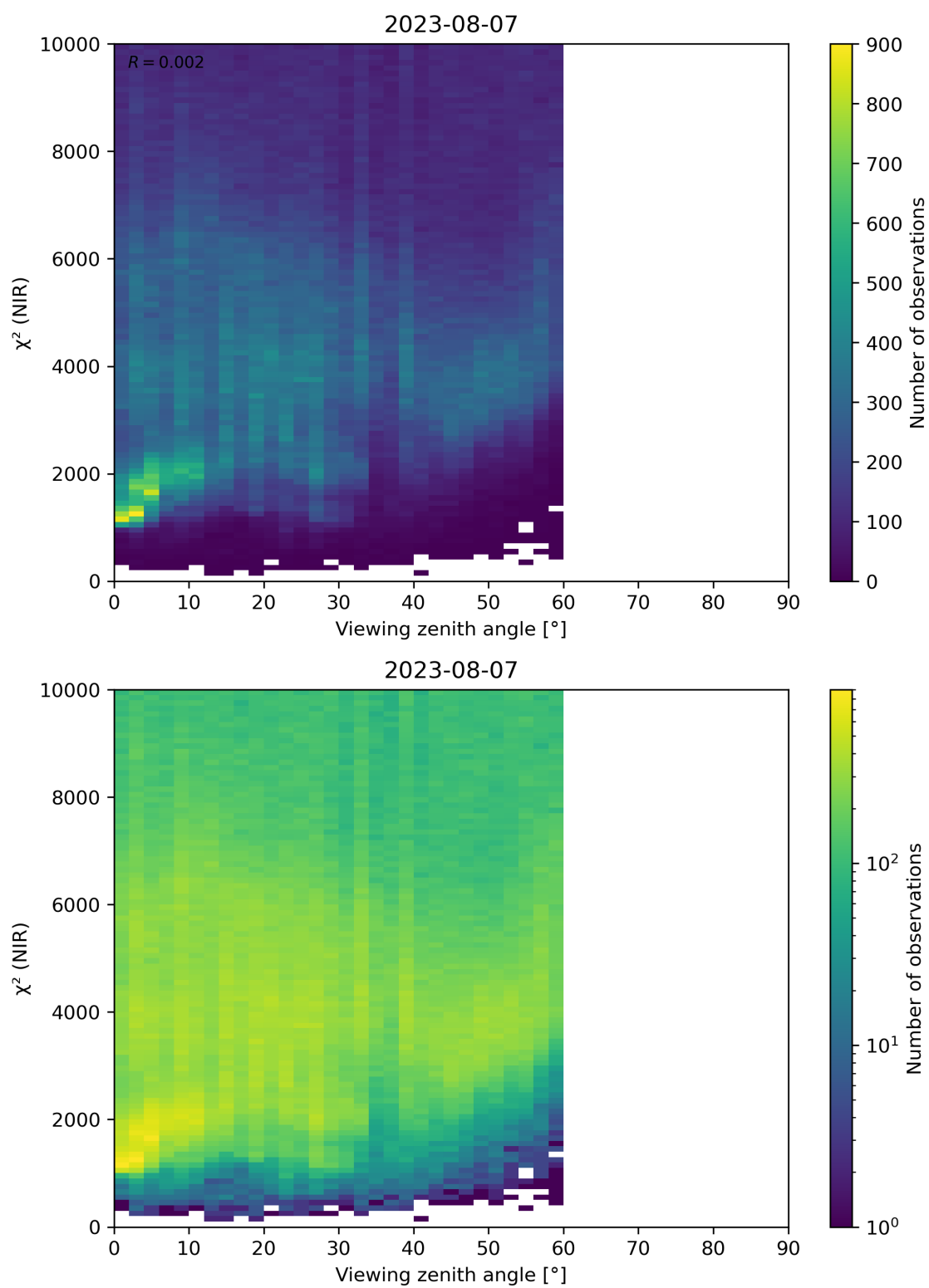
Figure 105: Scatter density plot of “Viewing zenith angle” against “ \chi^2 (NIR)” for 2023-08-06 to 2023-08-08.
