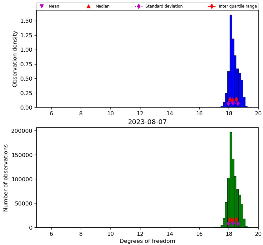
Figure 30: Histogram of “Degrees of freedom” for 2023-08-06 to 2023-08-08
