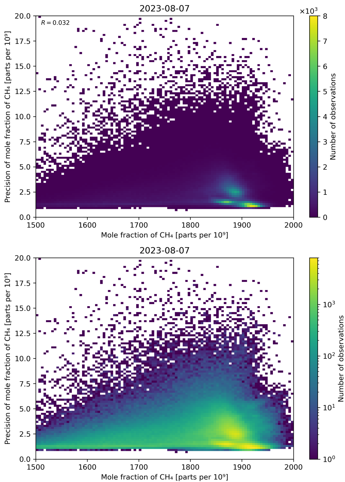
Figure 75: Scatter density plot of “Mole fraction of CH 4 ” against “Precision of mole fraction of CH 4 ” for 2023-08-06 to 2023-08-08.
