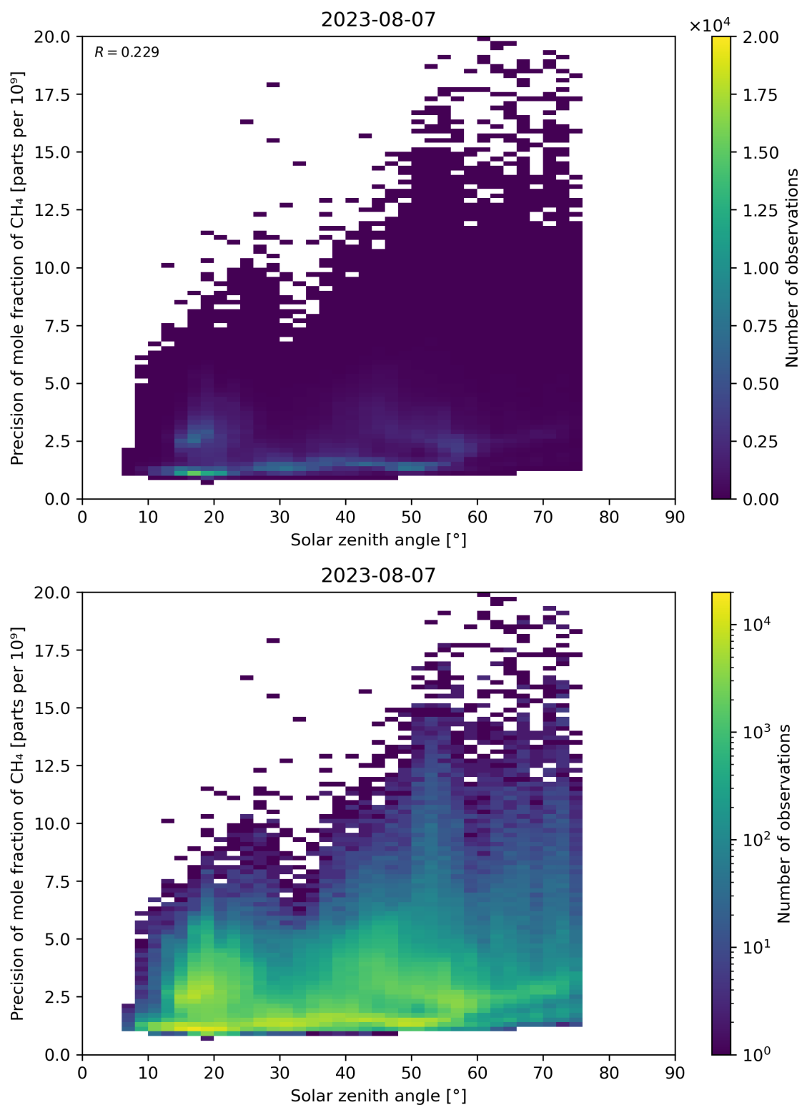
Figure 101: Scatter density plot of “Solar zenith angle” against “Precision of mole fraction of CH 4 ” for 2023-08-06 to 2023-08-08.
