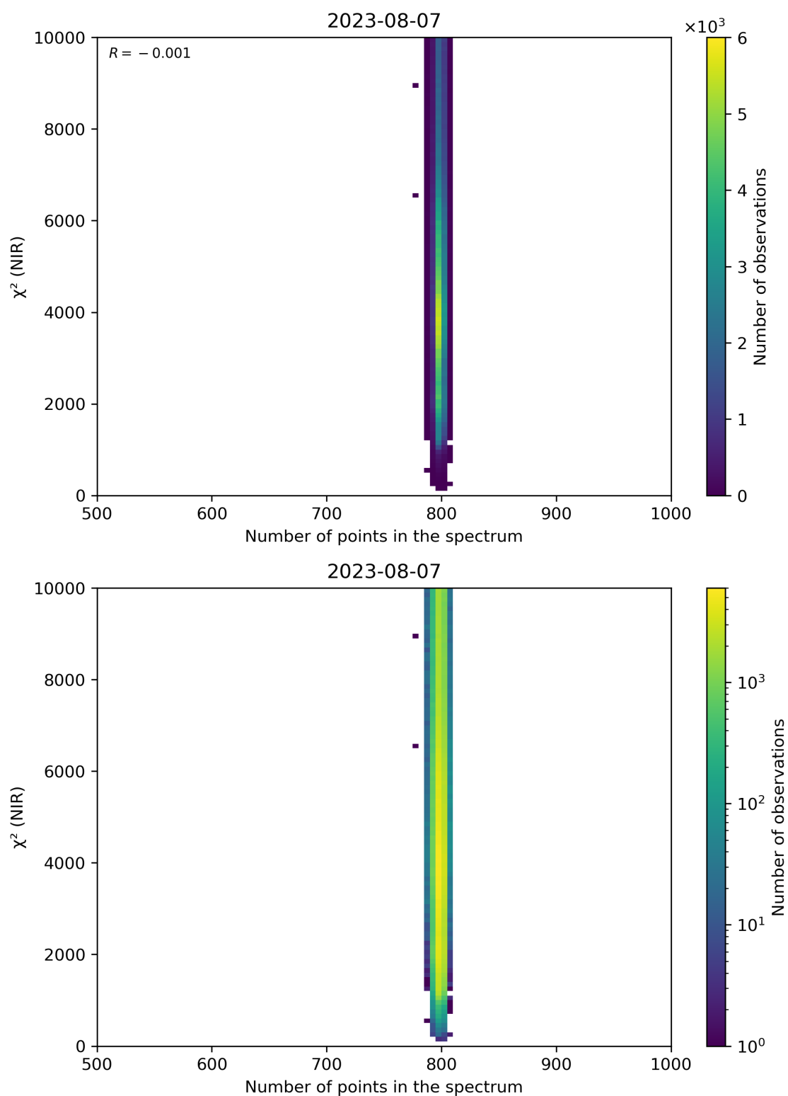
Figure 88: Scatter density plot of “Number of points in the spectrum” against “ \chi^2 (NIR)” for 2023-08-06 to 2023-08-08.
