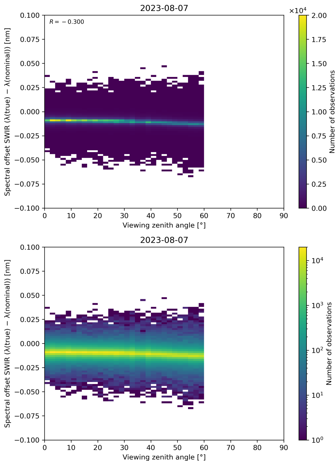
Figure 116: Scatter density plot of “Viewing zenith angle” against “Spectral offset SWIR ( \lambda(\text{true}) - \lambda(\text{nominal}) )” for 2023-08-06 to 2023-08-08.
