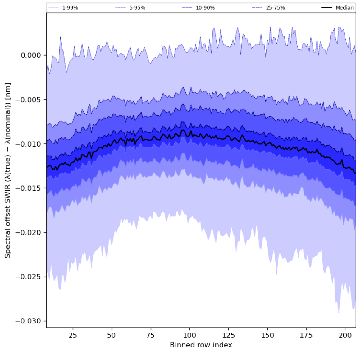
Figure 38: Along track statistics of “Spectral offset SWIR ( \lambda(\text{true}) - \lambda(\text{nominal}) )” for 2023-08-06 to 2023-08-08
