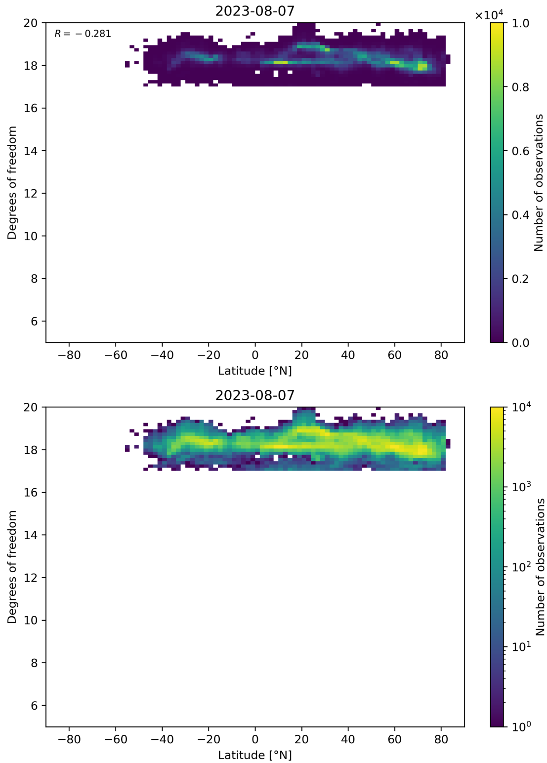
Figure 55: Scatter density plot of “Latitude” against “Degrees of freedom” for 2023-08-06 to 2023-08-08.
