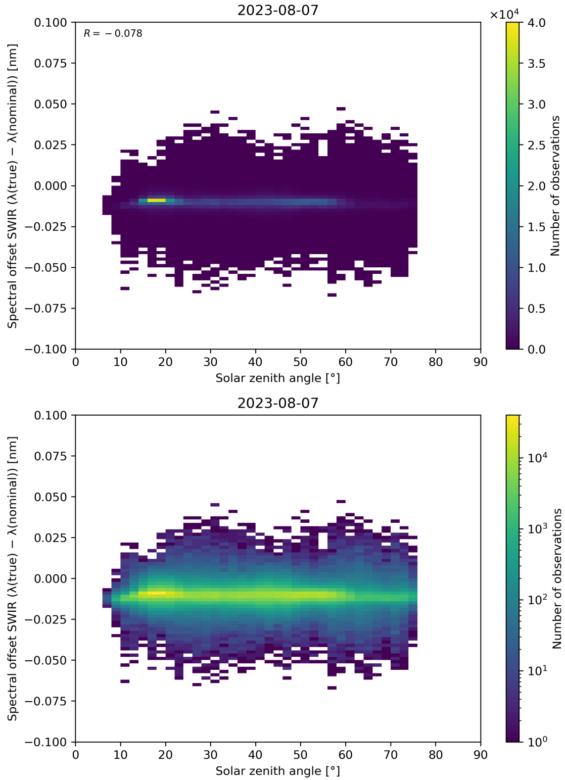
Figure 104: Scatter density plot of “Solar zenith angle” against “Spectral offset SWIR ( \lambda(\text{true}) - \lambda(\text{nominal}) )” for 2023-08-06 to 2023-08-08.
