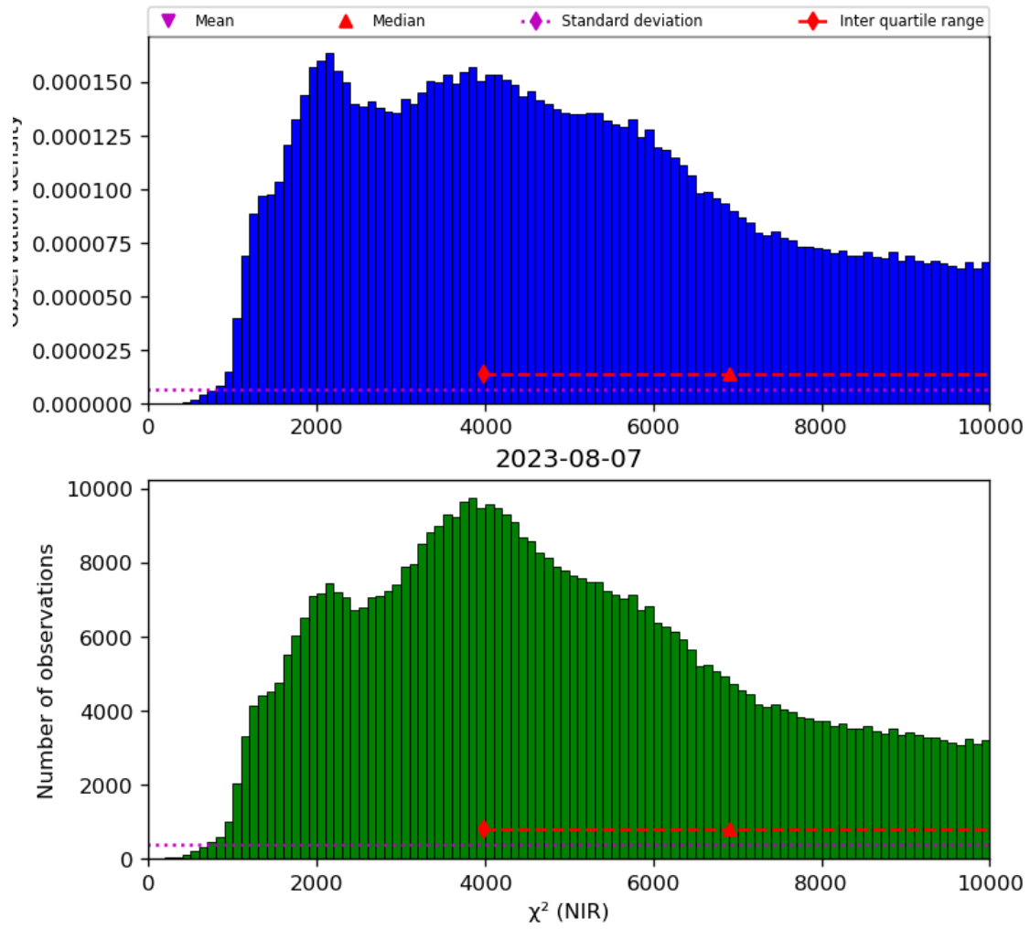
Figure 29: Histogram of “ \chi^2 (NIR)” for 2023-08-06 to 2023-08-08
