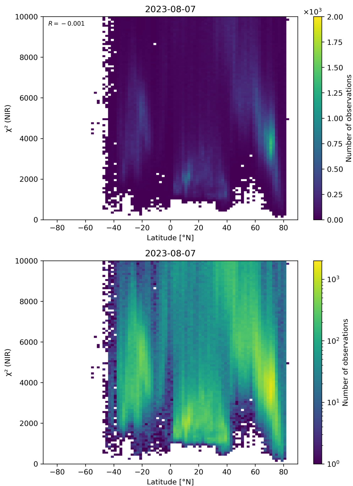
Figure 53: Scatter density plot of “Latitude” against “ \chi^2 (NIR)” for 2023-08-06 to 2023-08-08.
