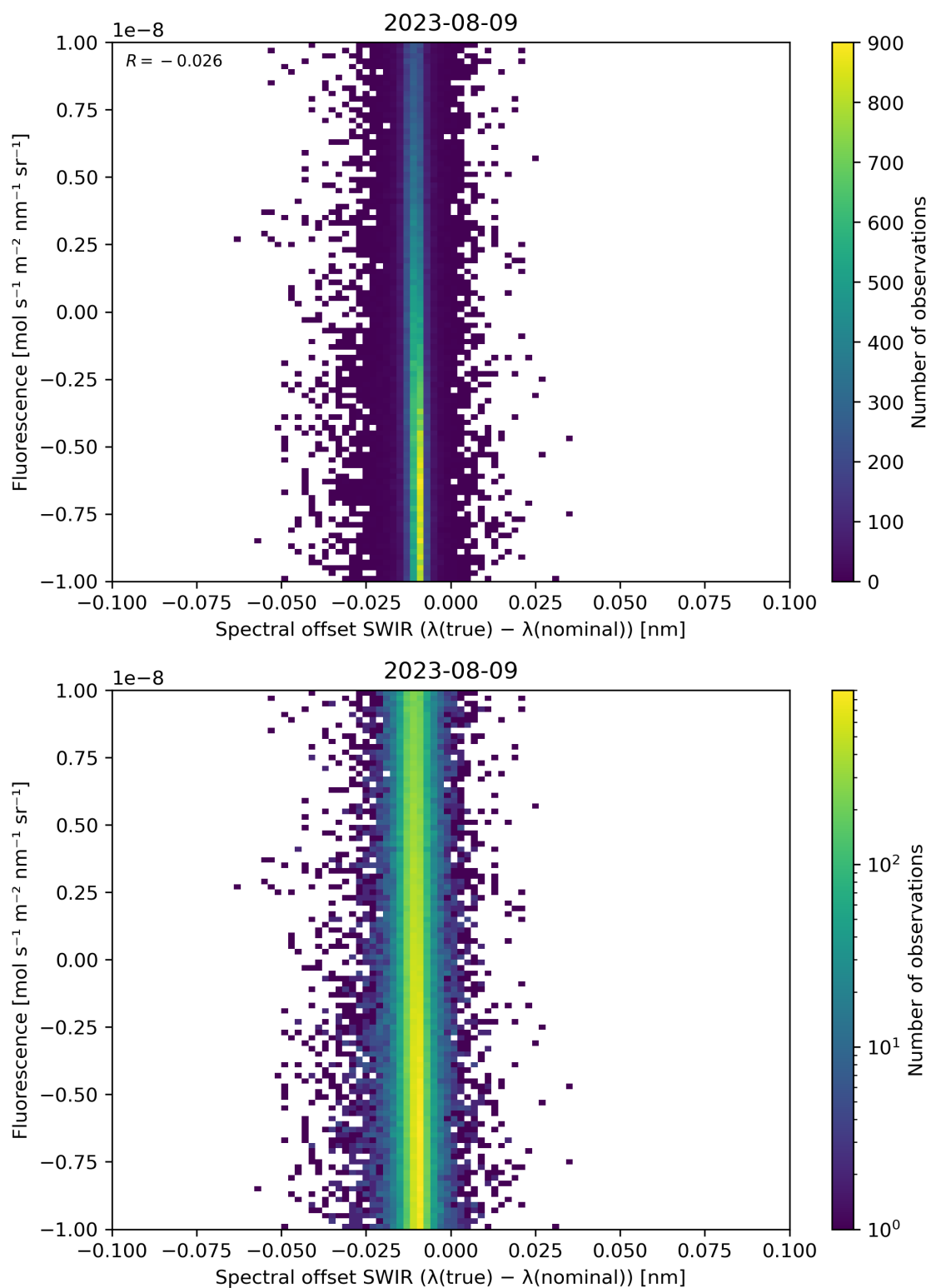
Figure 120: Scatter density plot of “Spectral offset SWIR ( \lambda(\text{true}) - \lambda(\text{nominal}) )” against “Fluorescence” for 2023-08-09 to 2023-08-10.
