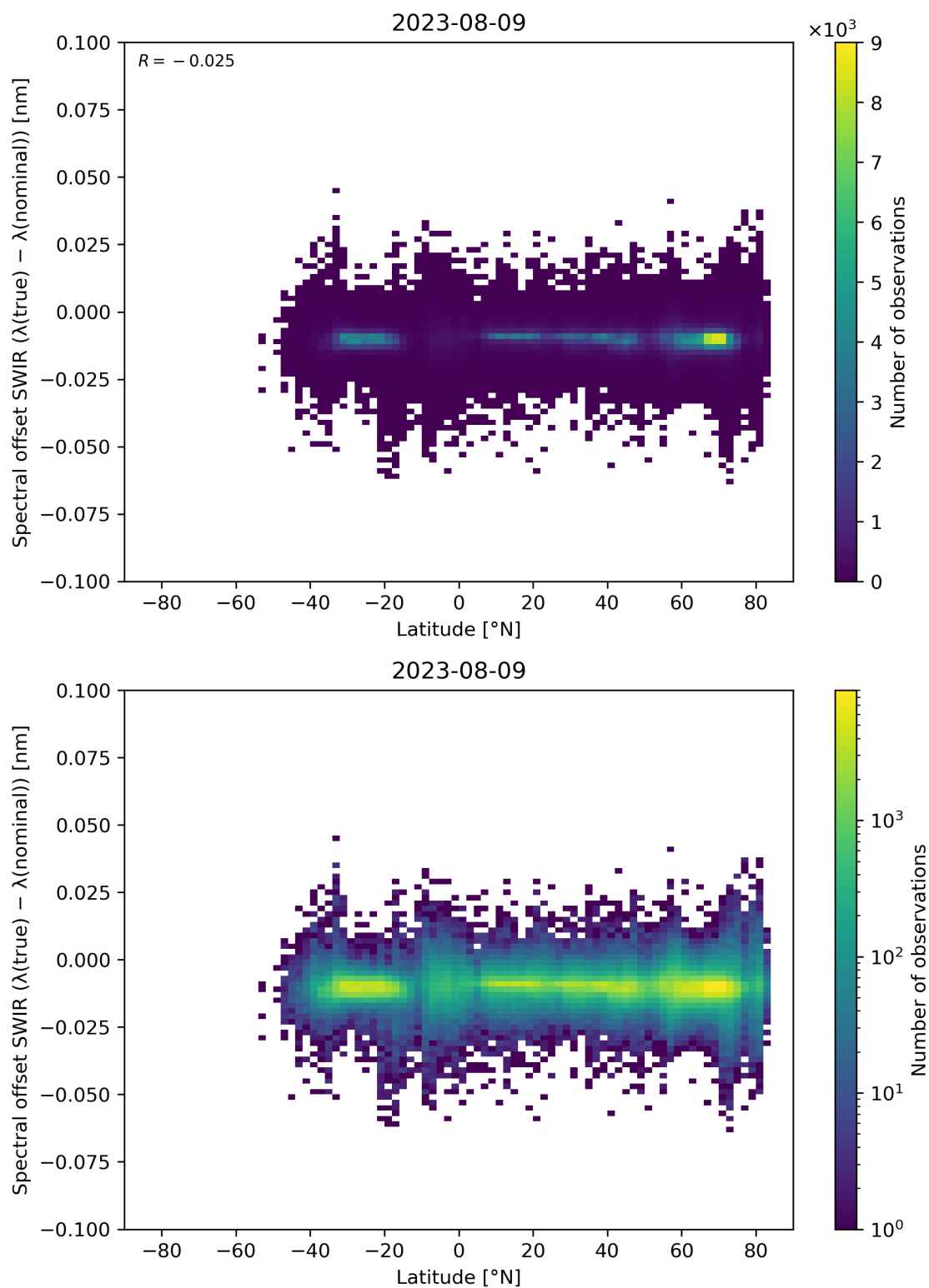
Figure 62: Scatter density plot of “Latitude” against “Spectral offset SWIR ( \lambda(\text{true}) - \lambda(\text{nominal}) )” for 2023-08-09 to 2023-08-10.
