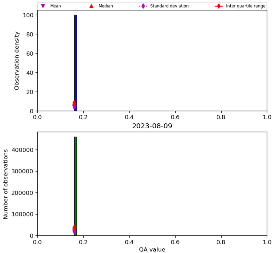
Figure 22: Histogram of “QA value” for 2023-08-09 to 2023-08-10
