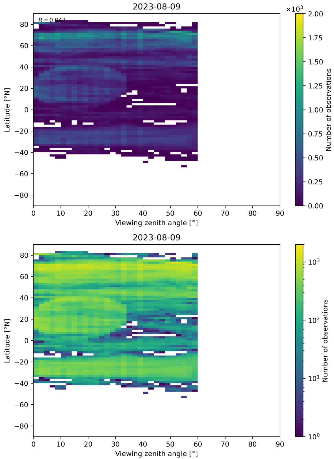
Figure 109: Scatter density plot of “Viewing zenith angle” against “Latitude” for 2023-08-09 to 2023-08-10.
