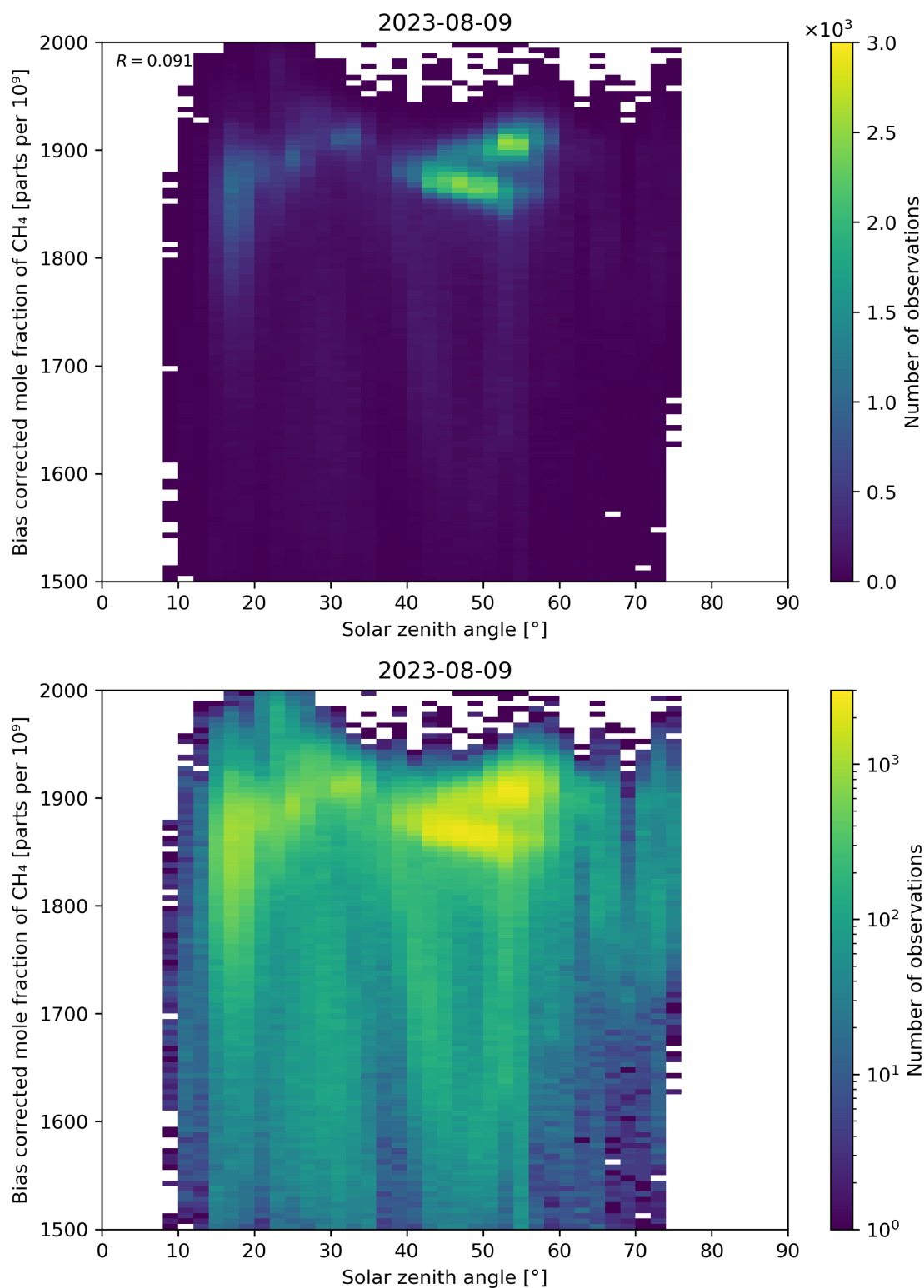
Figure 100: Scatter density plot of “Solar zenith angle” against “Bias corrected mole fraction of \text{CH}_4 ” for 2023-08-09 to 2023-08-10.
