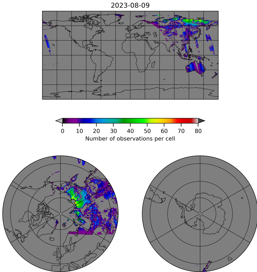
Figure 10: Map of the number of observations for 2023-08-09 to 2023-08-10
