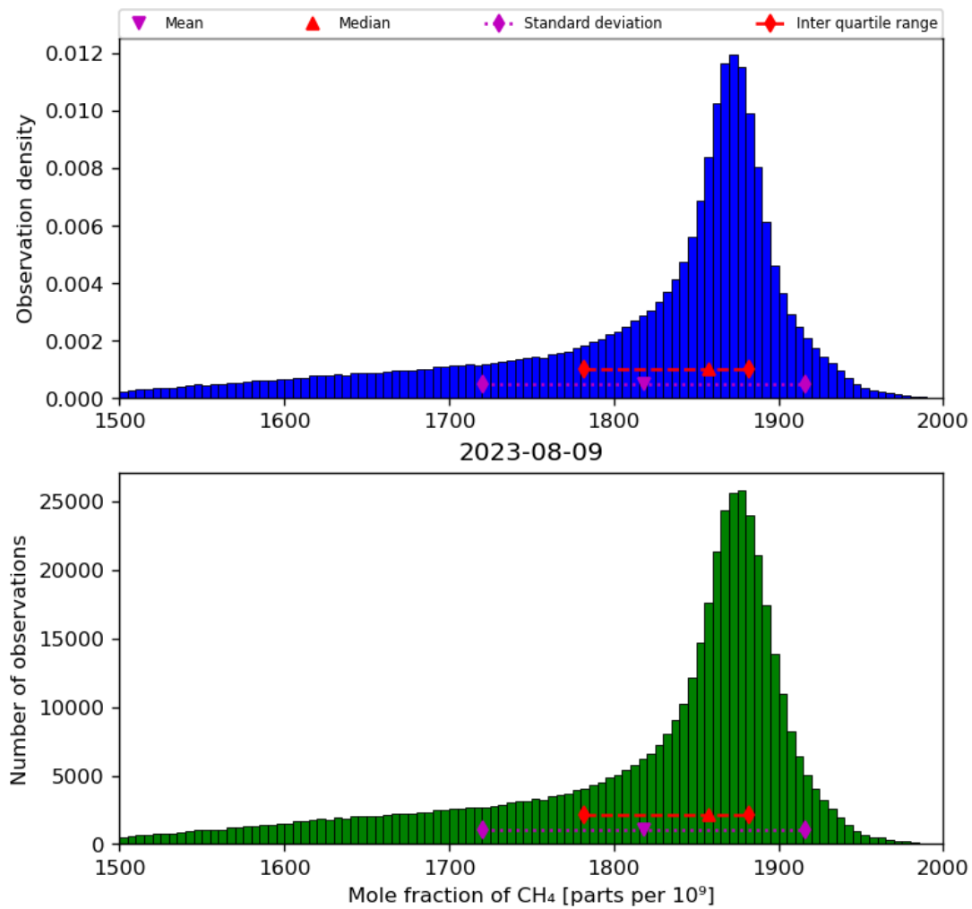
Figure 23: Histogram of “Mole fraction of CH 4 ” for 2023-08-09 to 2023-08-10
