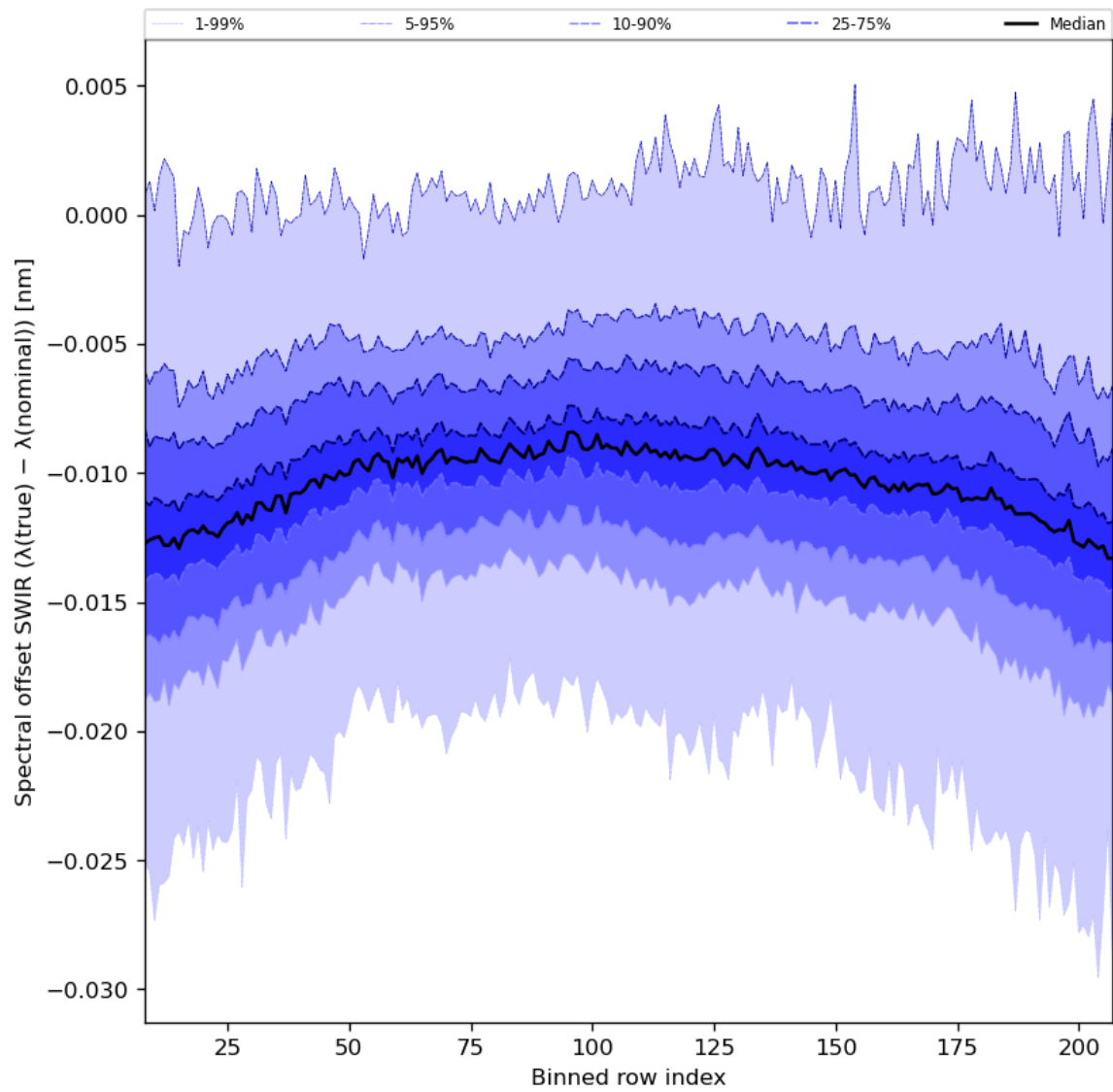
Figure 38: Along track statistics of “Spectral offset SWIR ( \lambda(\text{true}) - \lambda(\text{nominal}) )” for 2023-08-09 to 2023-08-10
