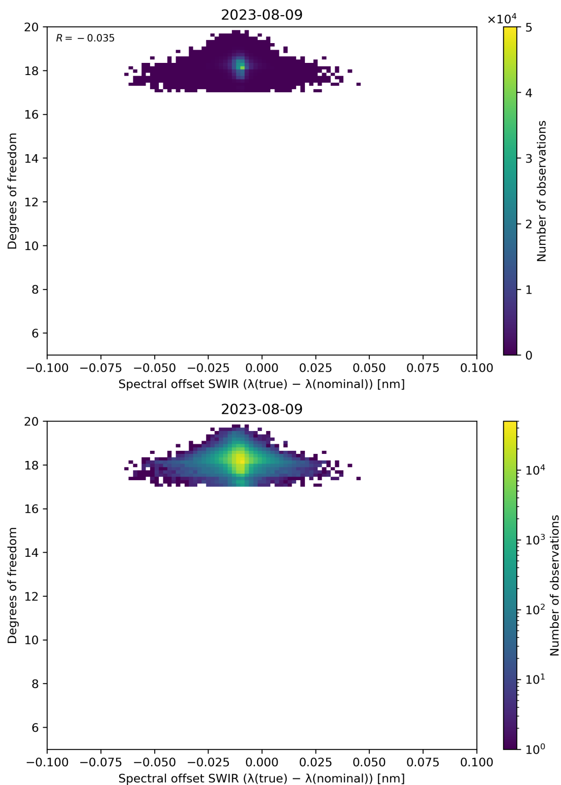
Figure 119: Scatter density plot of “Spectral offset SWIR ( \lambda(\text{true}) - \lambda(\text{nominal}) )” against “Degrees of freedom” for 2023-08-09 to 2023-08-10.
