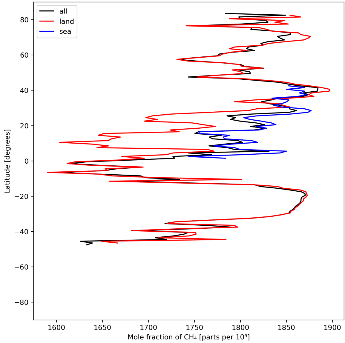
Figure 12: Zonal average of “Mole fraction of CH 4 ” for 2023-08-09 to 2023-08-10.
