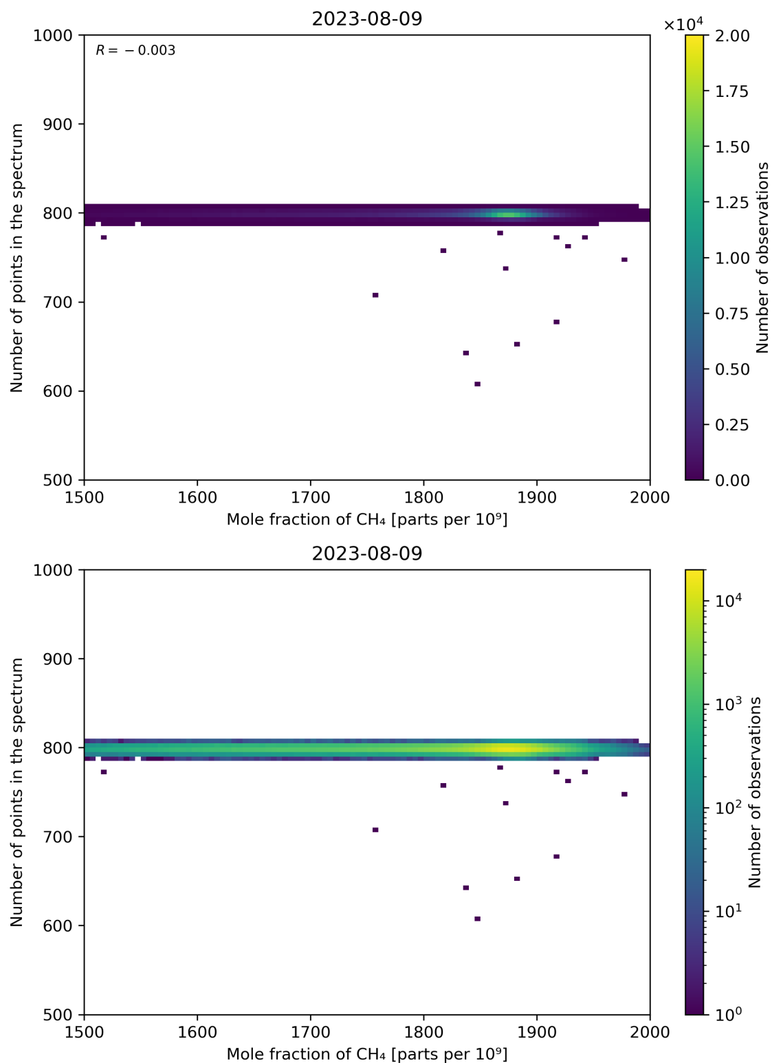
Figure 77: Scatter density plot of “Mole fraction of CH 4 ” against “Number of points in the spectrum” for 2023-08-09 to 2023-08-10.
