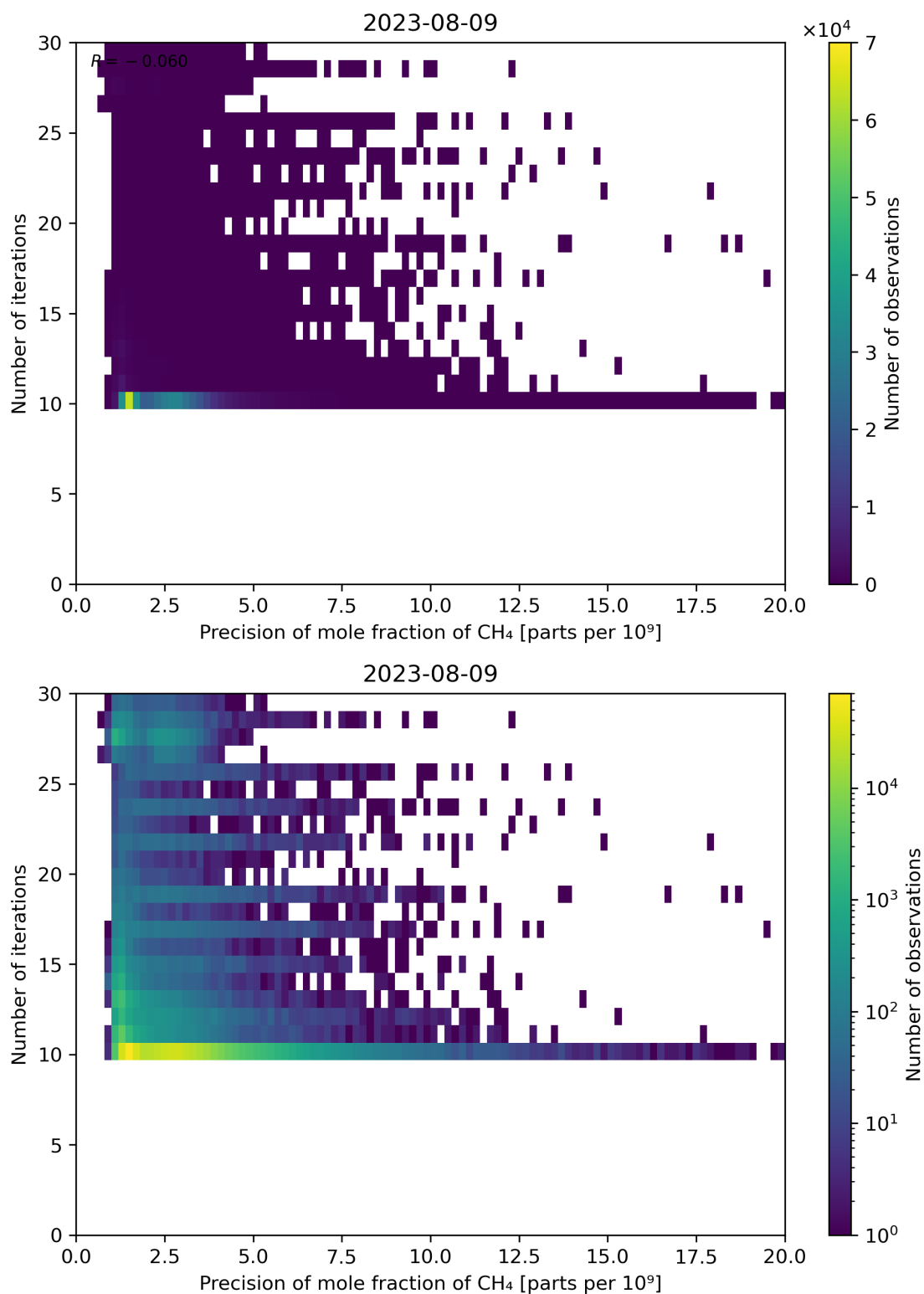
Figure 83: Scatter density plot of “Precision of mole fraction of CH 4 ” against “Number of iterations” for 2023-08-09 to 2023-08-10.
