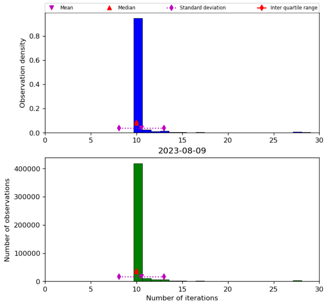
Figure 31: Histogram of “Number of iterations” for 2023-08-09 to 2023-08-10
