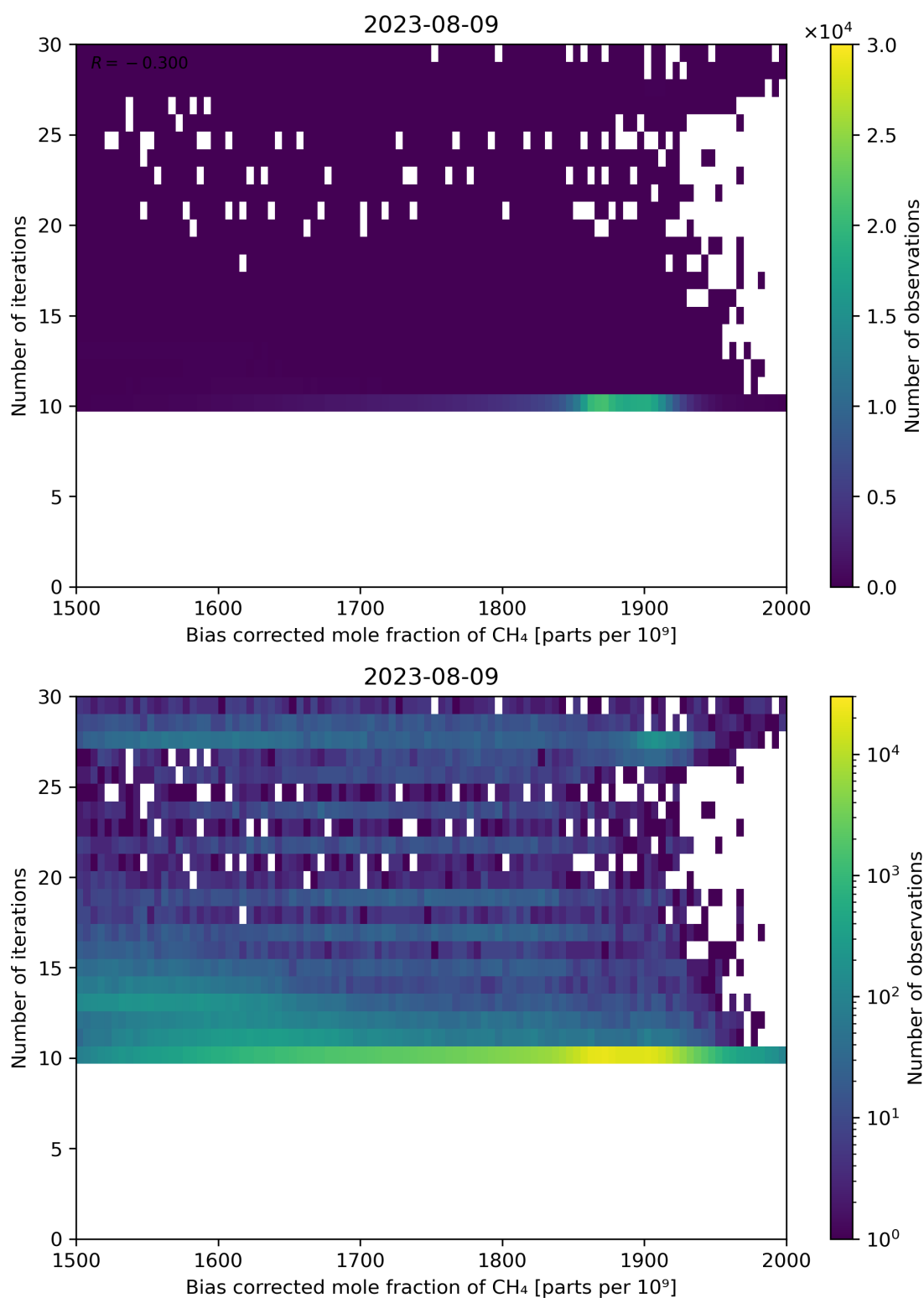
Figure 67: Scatter density plot of “Bias corrected mole fraction of \text{CH}_4 ” against “Number of iterations” for 2023-08-09 to 2023-08-10.
