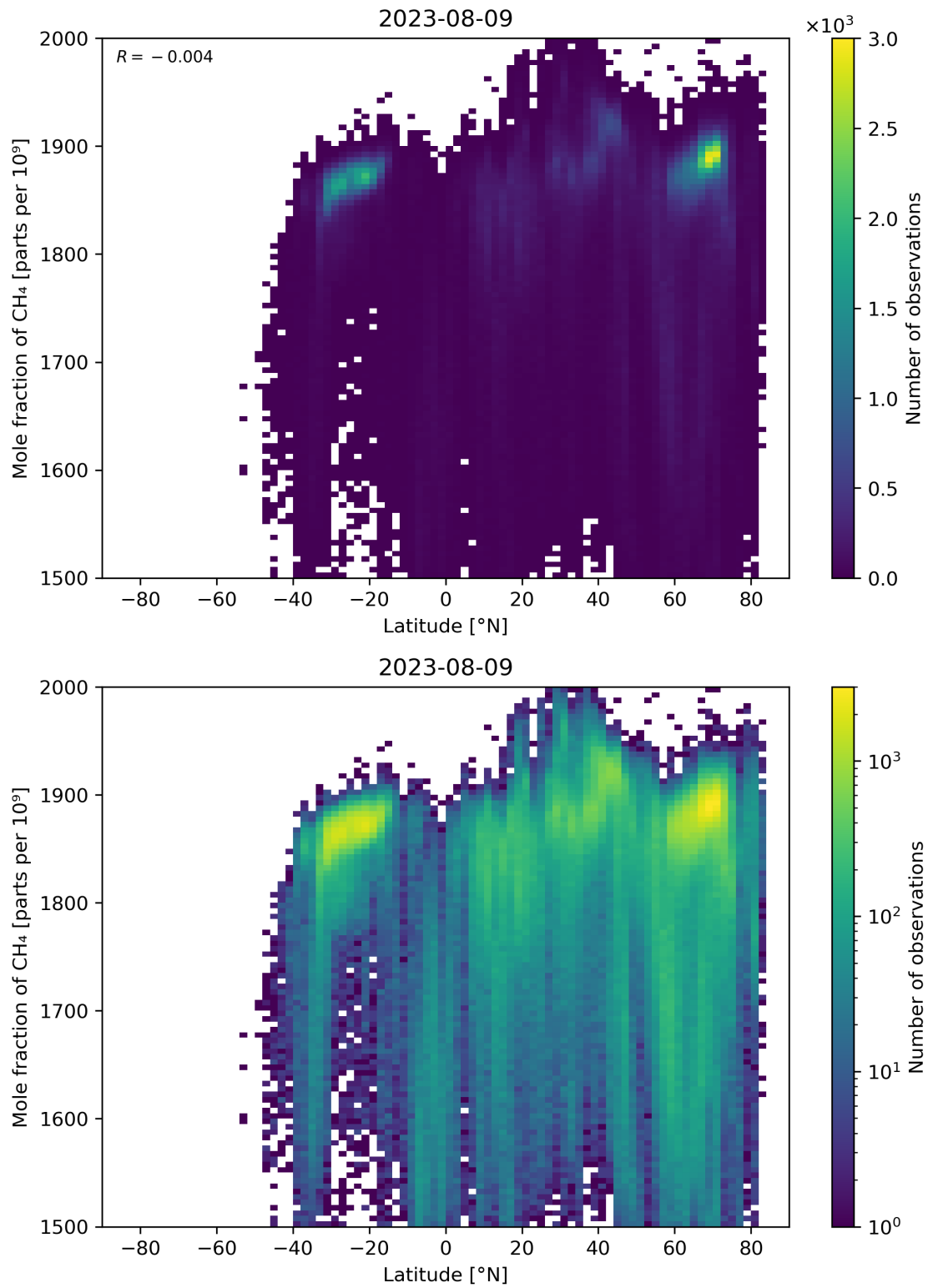
Figure 57: Scatter density plot of “Latitude” against “Mole fraction of CH 4 ” for 2023-08-09 to 2023-08-10.
