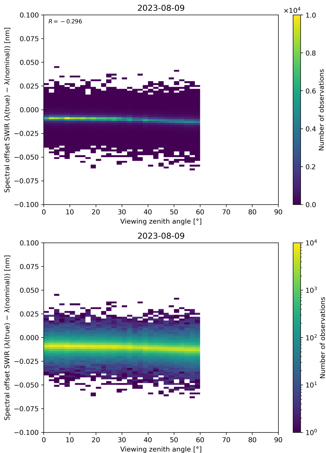
Figure 116: Scatter density plot of “Viewing zenith angle” against “Spectral offset SWIR ( \lambda(\text{true}) - \lambda(\text{nominal}) )” for 2023-08-09 to 2023-08-10.
