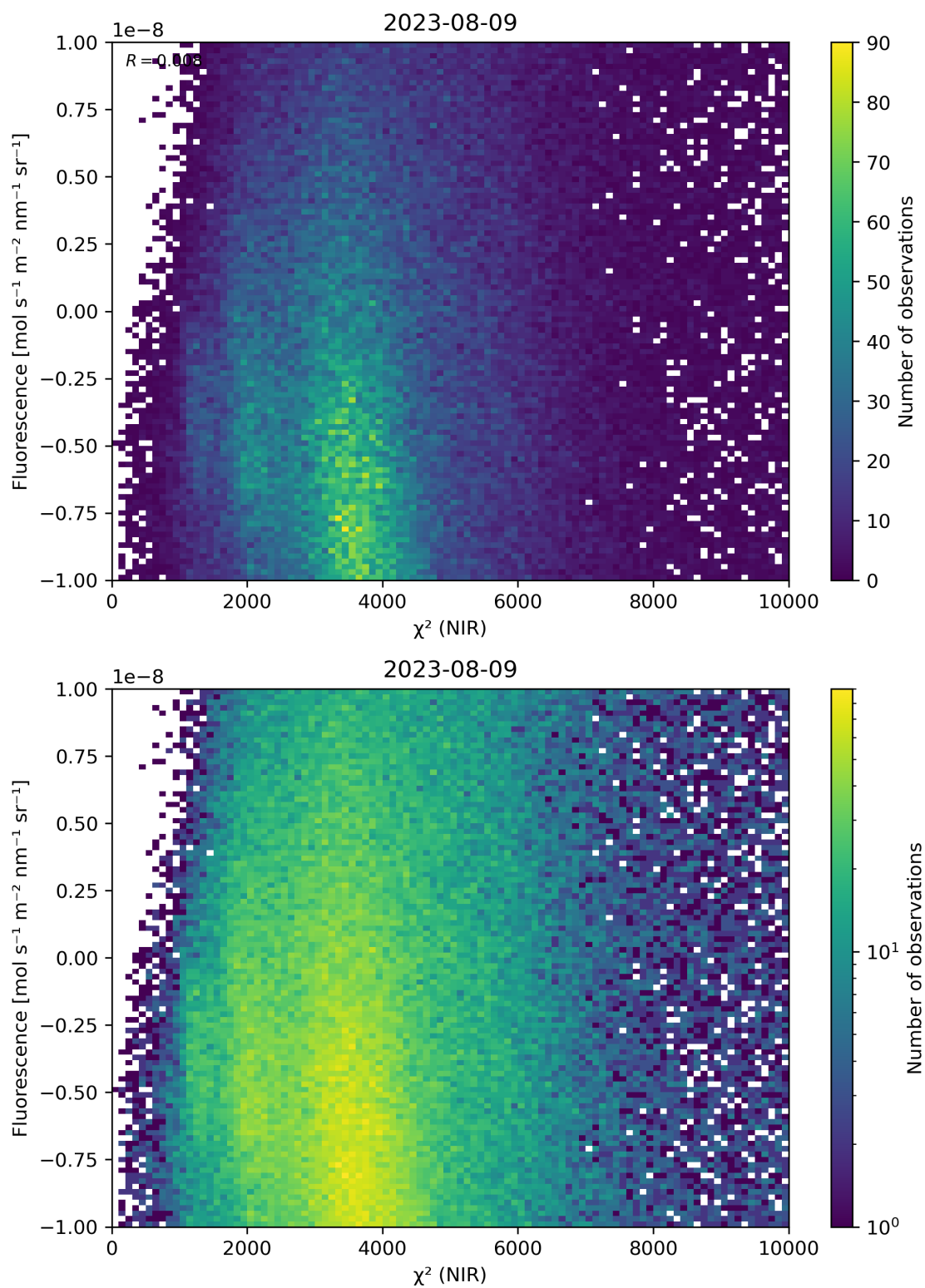
Figure 45: Scatter density plot of “ \chi^2 (NIR)” against “Fluorescence” for 2023-08-09 to 2023-08-10.
