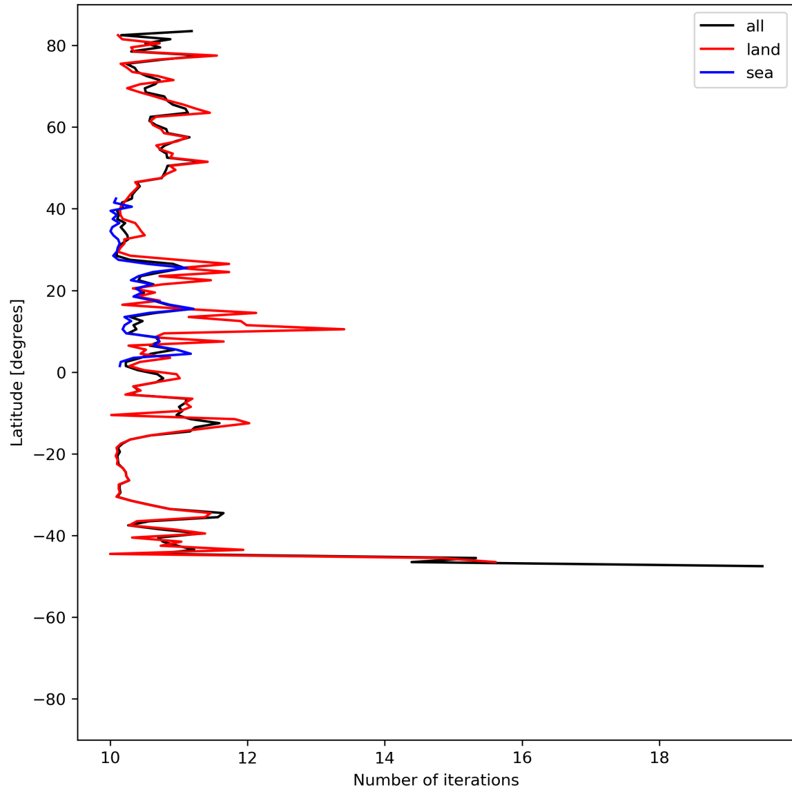
Figure 20: Zonal average of “Number of iterations” for 2023-08-09 to 2023-08-10.
