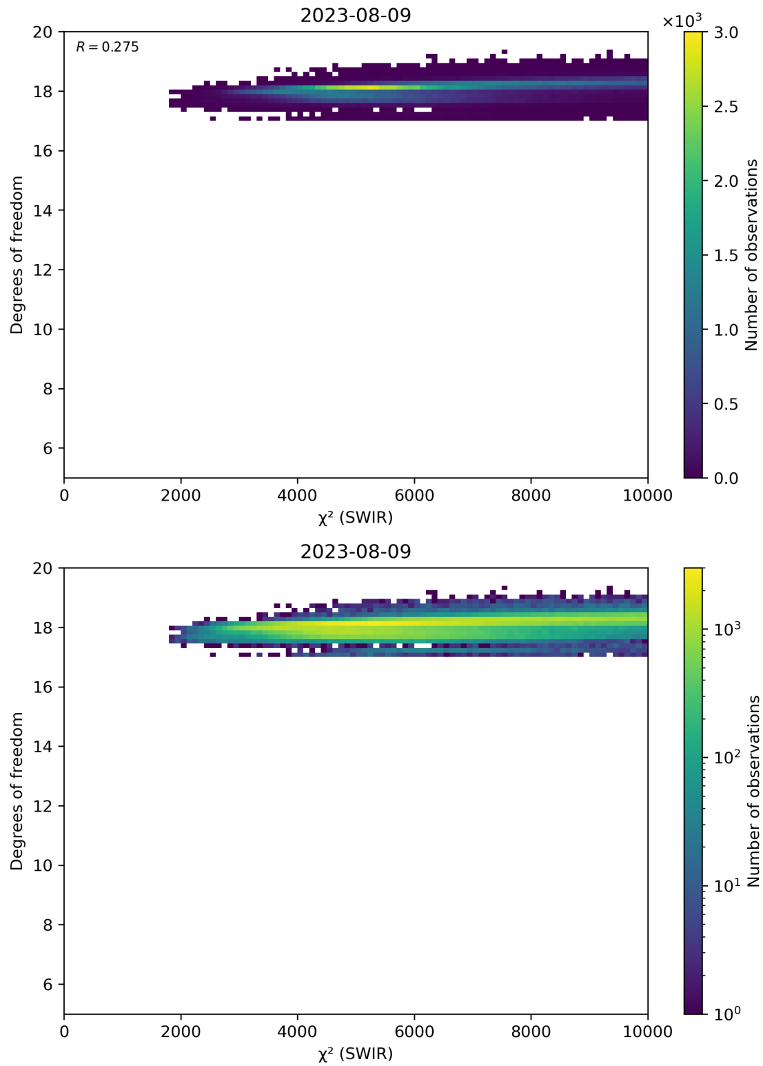
Figure 48: Scatter density plot of “ \chi^2 (SWIR)” against “Degrees of freedom” for 2023-08-09 to 2023-08-10.
