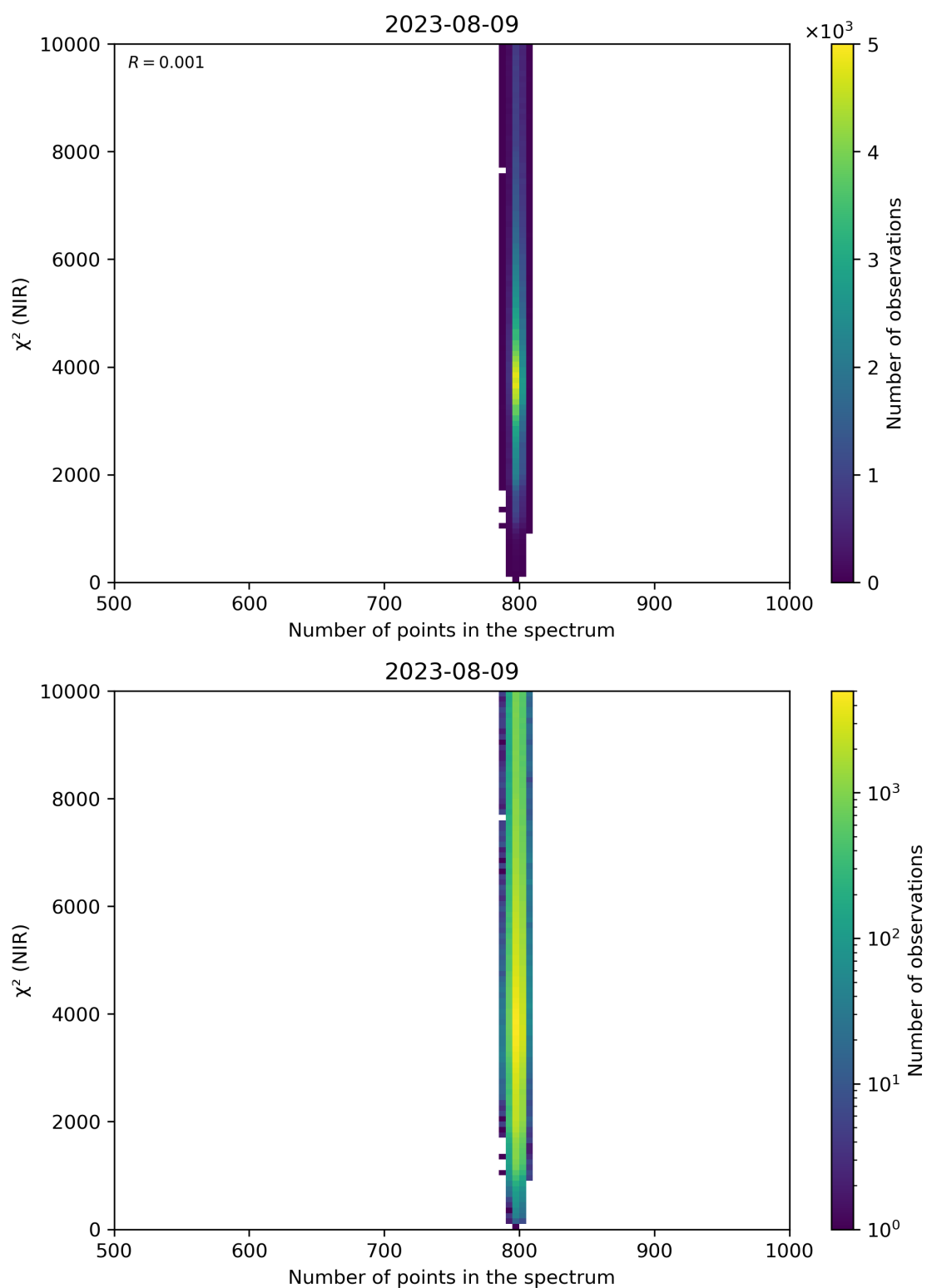
Figure 88: Scatter density plot of “Number of points in the spectrum” against “ \chi^2 (NIR)” for 2023-08-09 to 2023-08-10.
