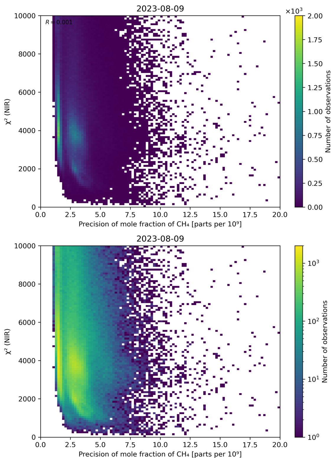
Figure 78: Scatter density plot of “Precision of mole fraction of \text{CH}_4 ” against “ \chi^2 (NIR)” for 2023-08-09 to 2023-08-10.
