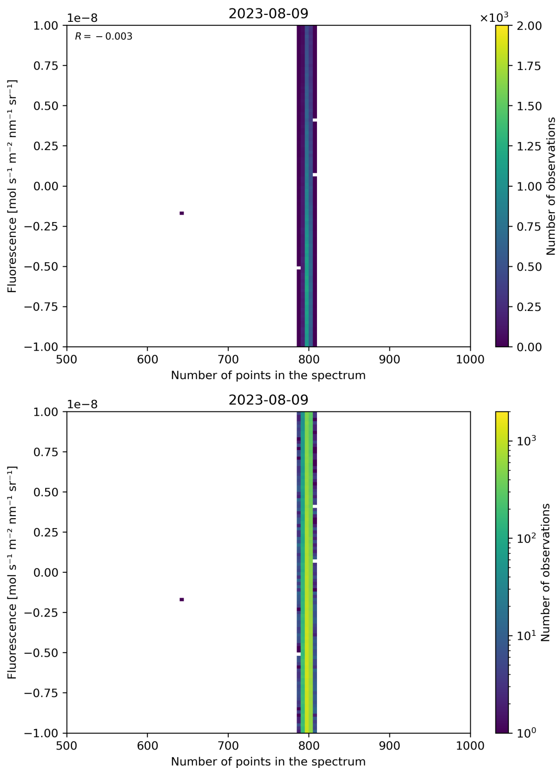
Figure 91: Scatter density plot of “Number of points in the spectrum” against “Fluorescence” for 2023-08-09 to 2023-08-10.
