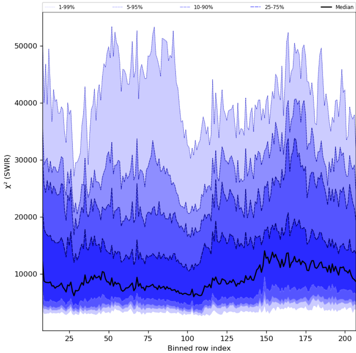
Figure 39: Along track statistics of “ \chi^2 (SWIR)” for 2023-08-09 to 2023-08-10
