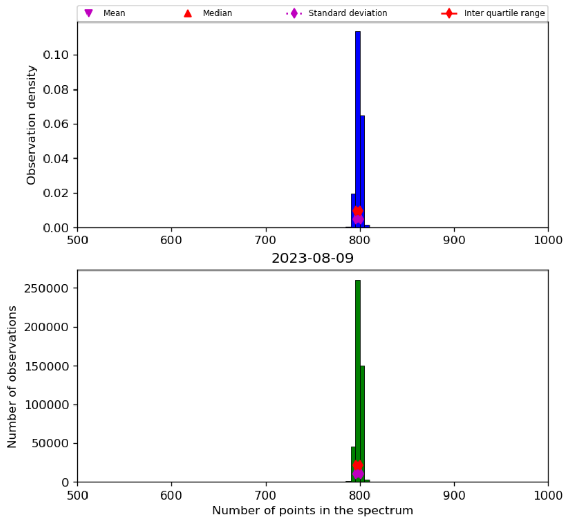
Figure 26: Histogram of “Number of points in the spectrum” for 2023-08-09 to 2023-08-10
