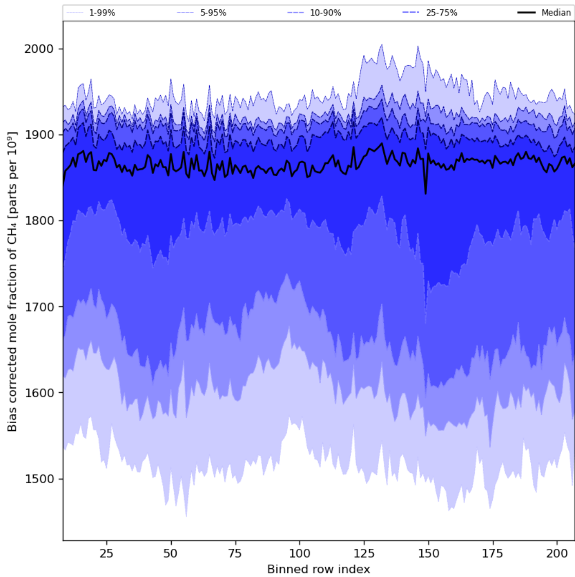
Figure 36: Along track statistics of “Bias corrected mole fraction of CH 4 ” for 2023-08-09 to 2023-08-10
