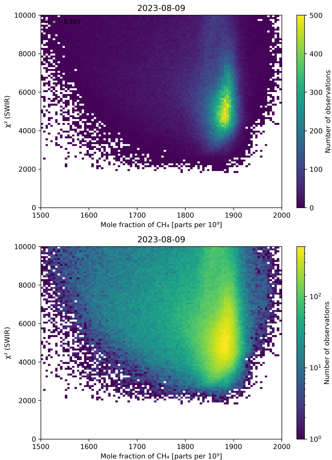
Figure 71: Scatter density plot of “Mole fraction of CH 4 ” against “ \chi^2 (SWIR)” for 2023-08-09 to 2023-08-10.
