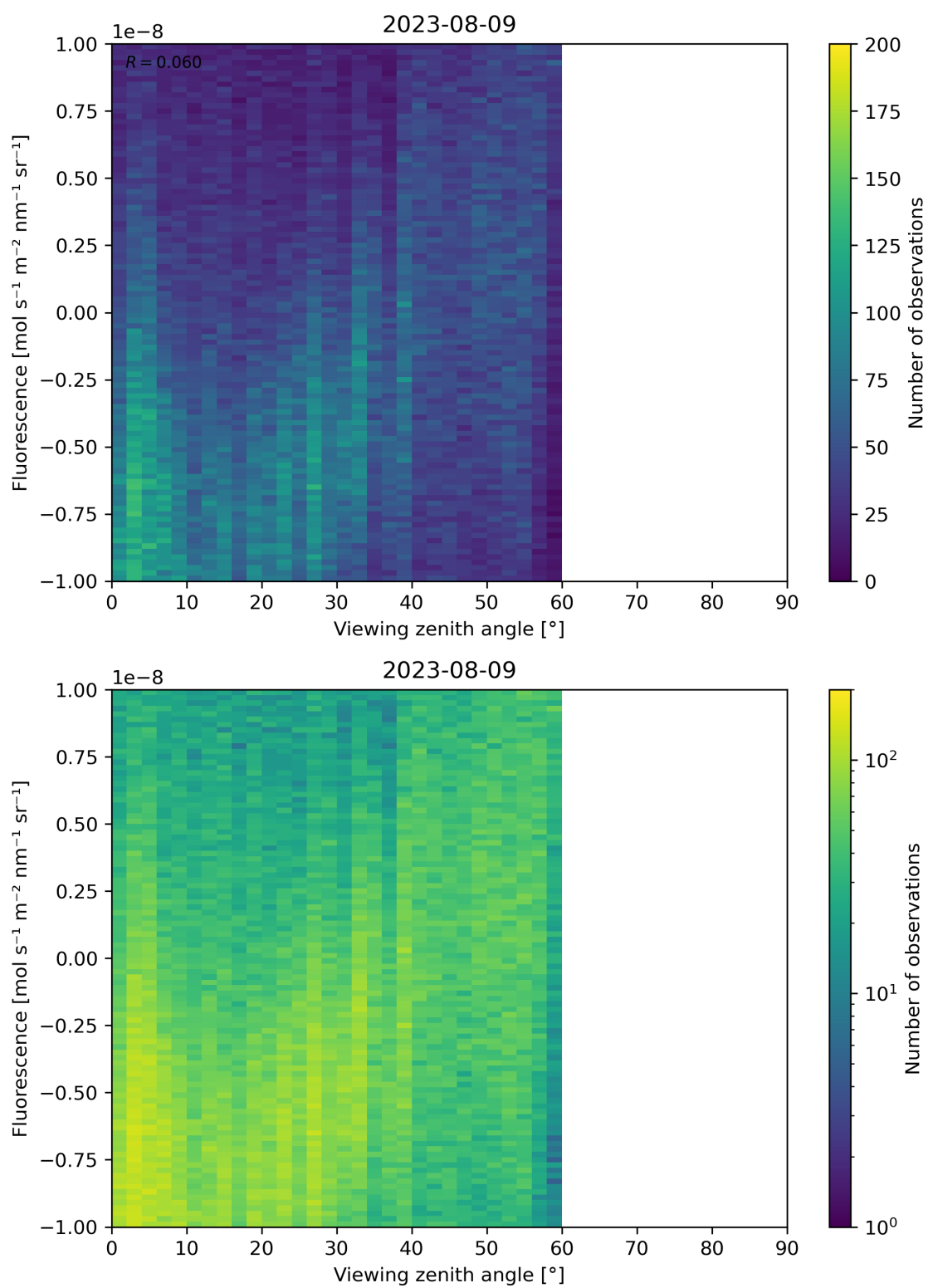
Figure 108: Scatter density plot of “Viewing zenith angle” against “Fluorescence” for 2023-08-09 to 2023-08-10.
