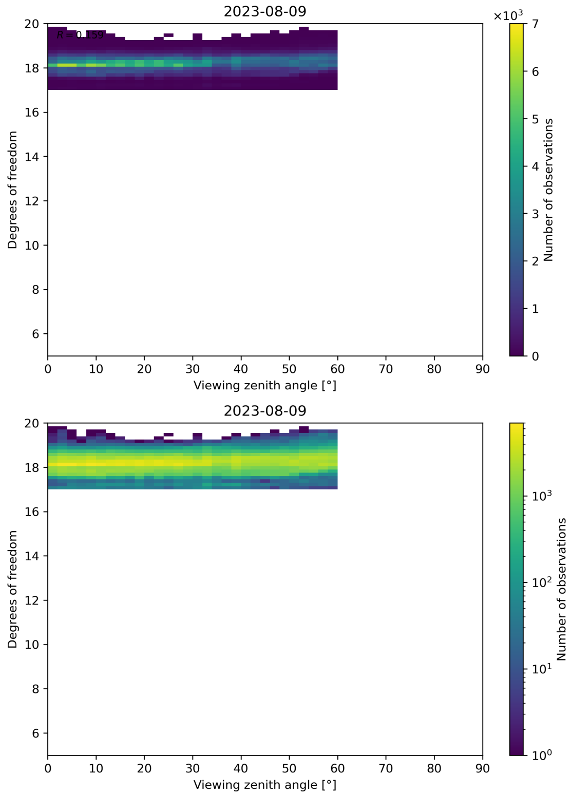
Figure 107: Scatter density plot of “Viewing zenith angle” against “Degrees of freedom” for 2023-08-09 to 2023-08-10.
