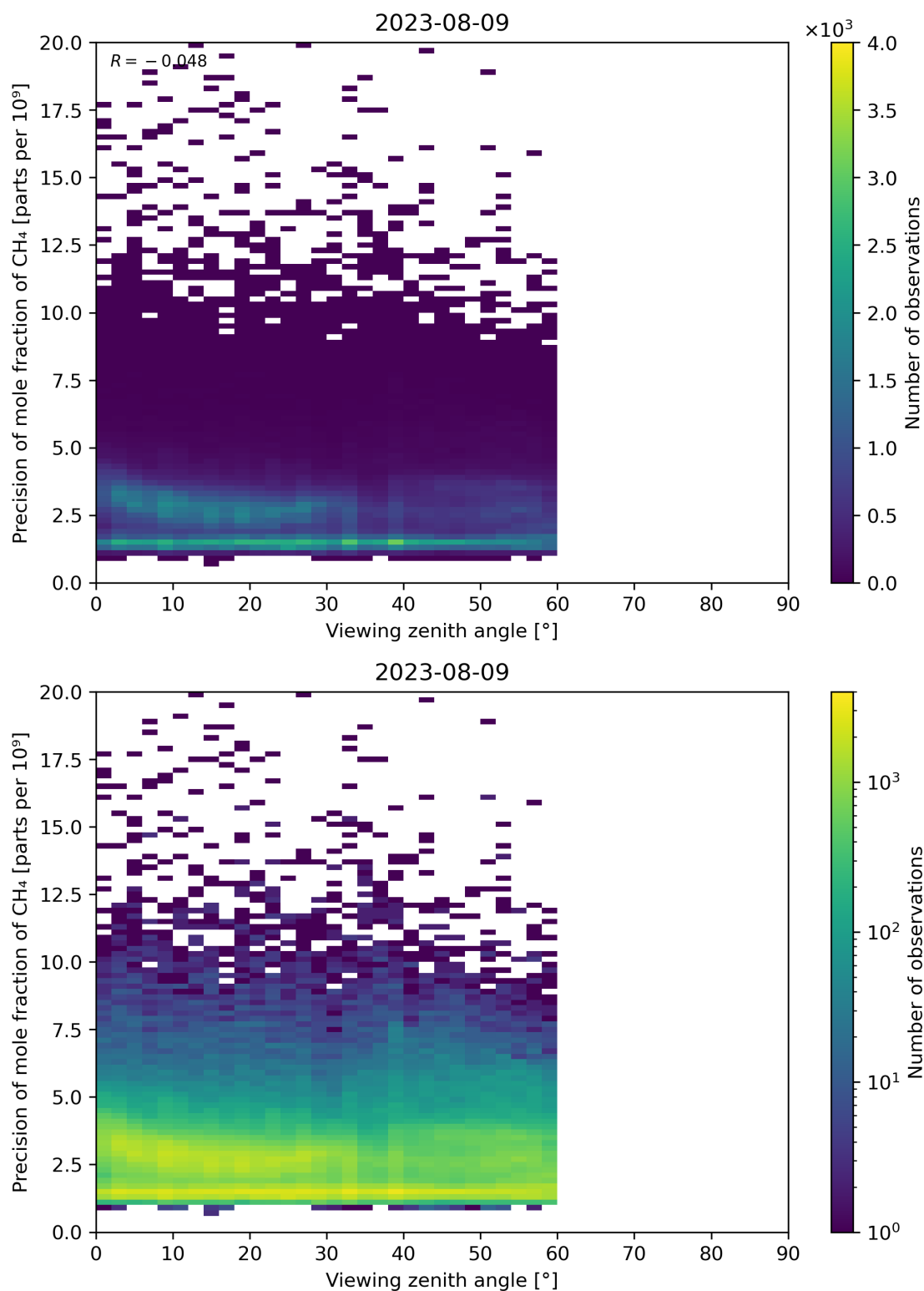
Figure 112: Scatter density plot of “Viewing zenith angle” against “Precision of mole fraction of CH 4 ” for 2023-08-09 to 2023-08-10.
