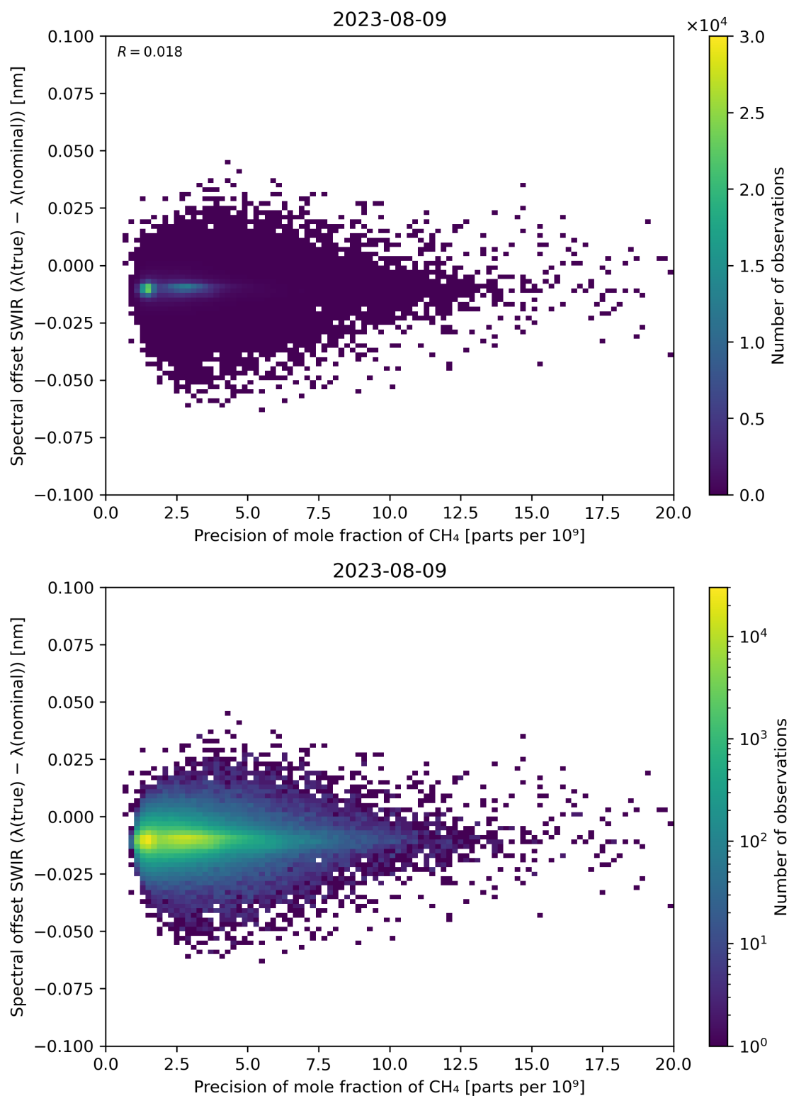
Figure 85: Scatter density plot of “Precision of mole fraction of CH 4 ” against “Spectral offset SWIR ( \lambda(\text{true}) - \lambda(\text{nominal}) )” for 2023-08-09 to 2023-08-10.
