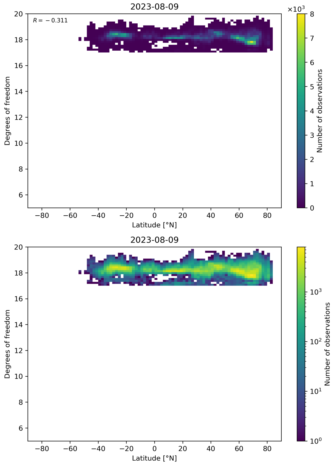
Figure 55: Scatter density plot of “Latitude” against “Degrees of freedom” for 2023-08-09 to 2023-08-10.
