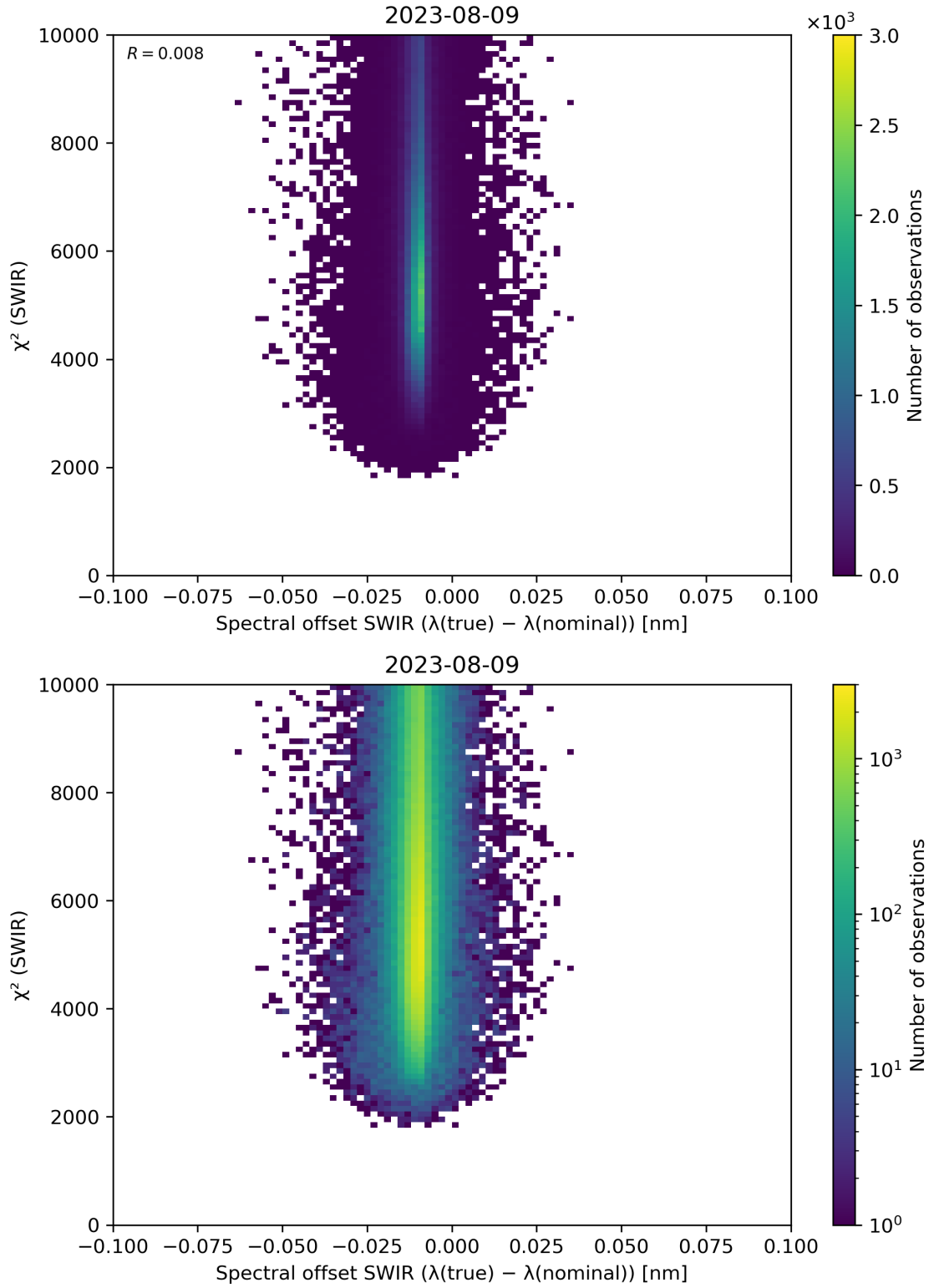
Figure 118: Scatter density plot of “Spectral offset SWIR ( \lambda(\text{true}) - \lambda(\text{nominal}) )” against “ \chi^2 (SWIR)” for 2023-08-09 to 2023-08-10.
