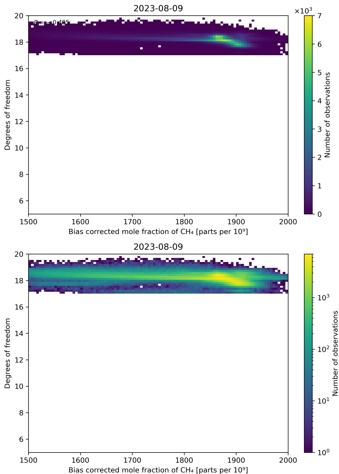
Figure 65: Scatter density plot of “Bias corrected mole fraction of CH 4 ” against “Degrees of freedom” for 2023-08-09 to 2023-08-10.
