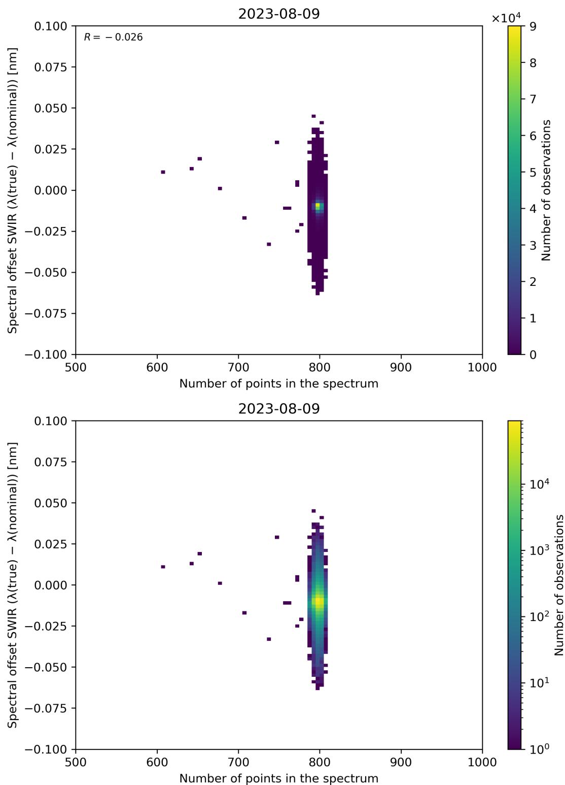
Figure 93: Scatter density plot of “Number of points in the spectrum” against “Spectral offset SWIR ( \lambda(\text{true}) - \lambda(\text{nominal}) )” for 2023-08-09 to 2023-08-10.
