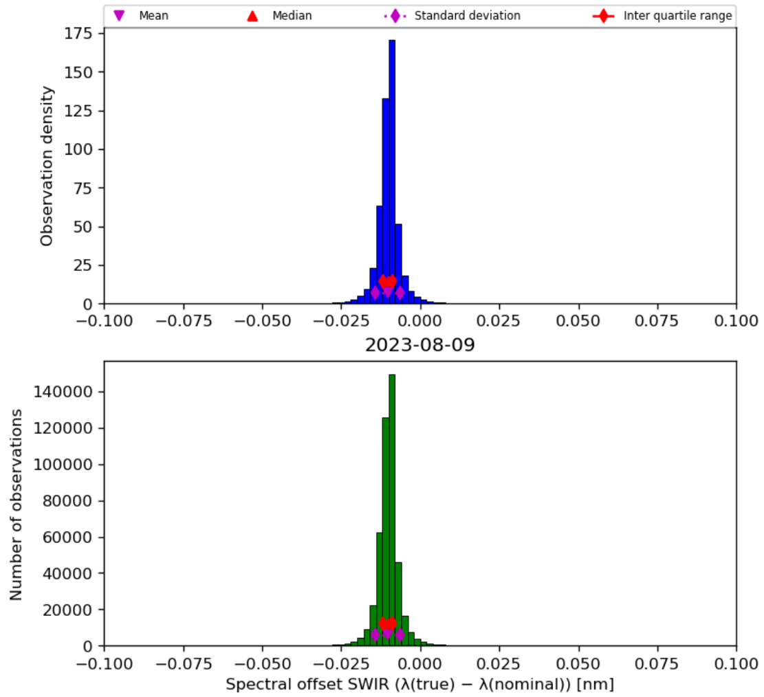
Figure 27: Histogram of “Spectral offset SWIR ( \lambda(\text{true}) - \lambda(\text{nominal}) )” for 2023-08-09 to 2023-08-10
