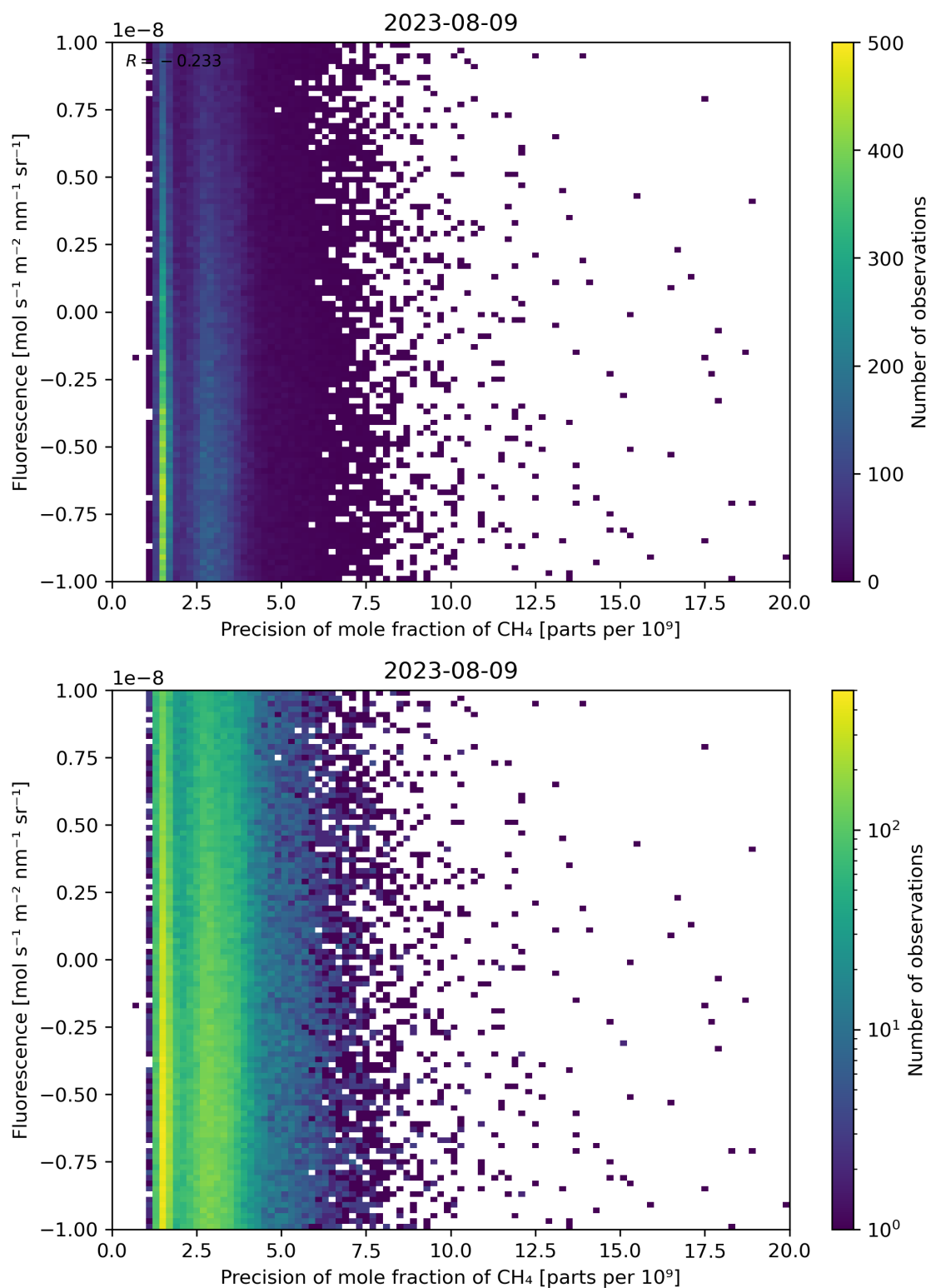
Figure 81: Scatter density plot of “Precision of mole fraction of CH 4 ” against “Fluorescence” for 2023-08-09 to 2023-08-10.
