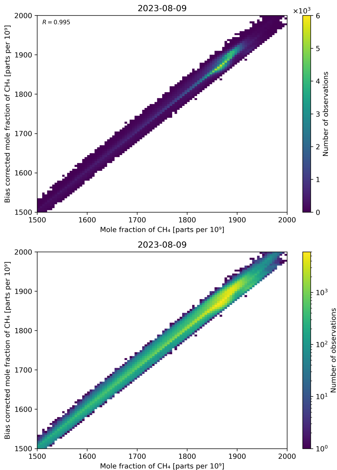
Figure 74: Scatter density plot of “Mole fraction of CH 4 ” against “Bias corrected mole fraction of CH 4 ” for 2023-08-09 to 2023-08-10.
