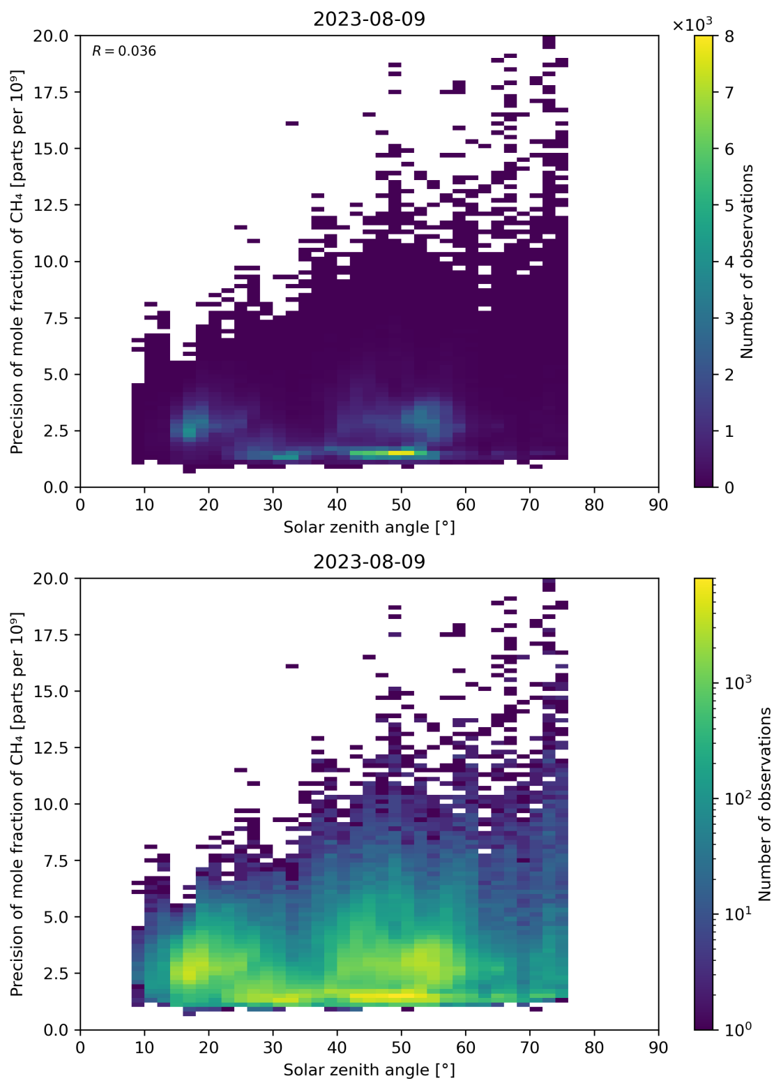
Figure 101: Scatter density plot of “Solar zenith angle” against “Precision of mole fraction of CH 4 ” for 2023-08-09 to 2023-08-10.
