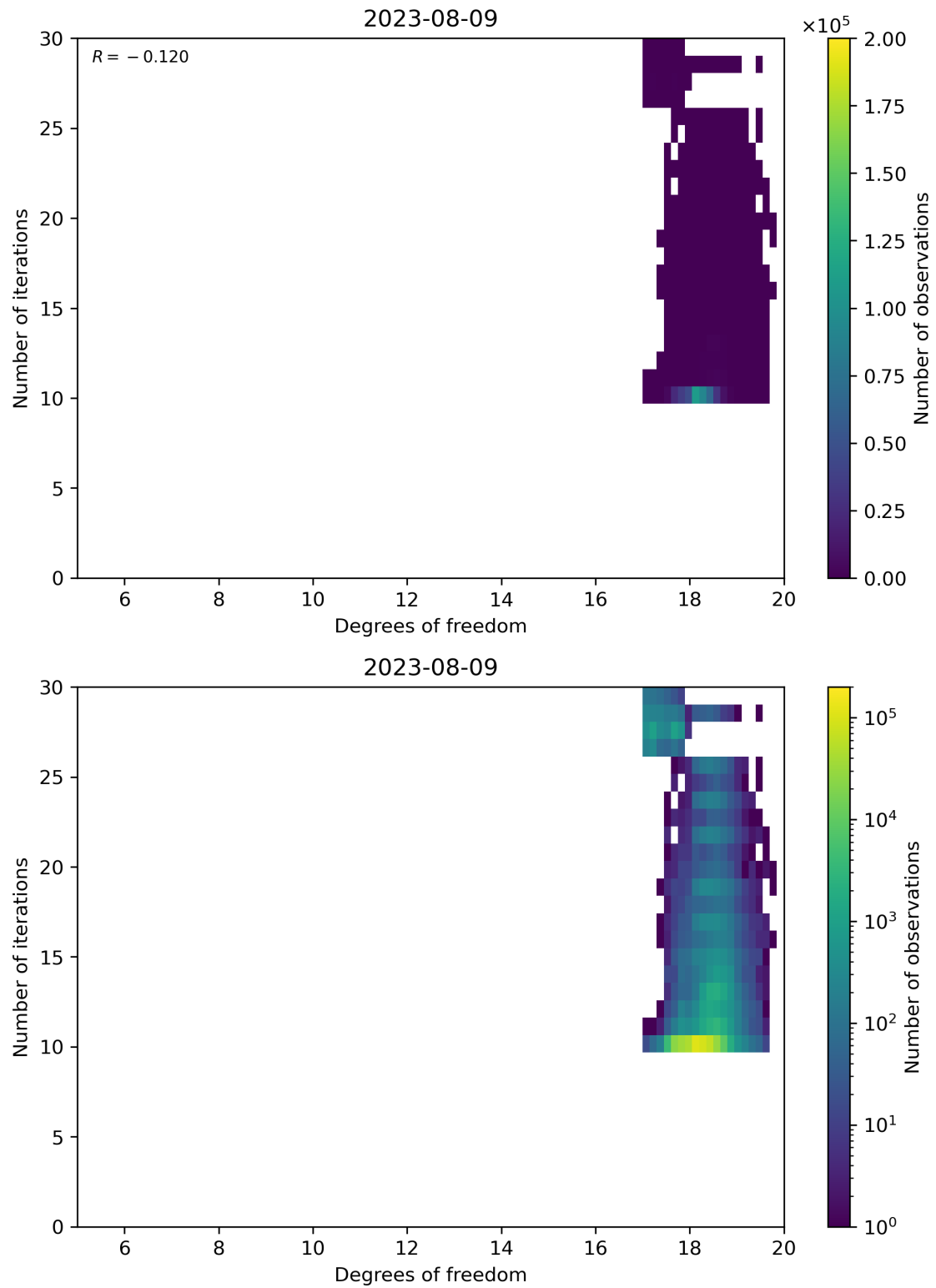
Figure 52: Scatter density plot of “Degrees of freedom” against “Number of iterations” for 2023-08-09 to 2023-08-10.
