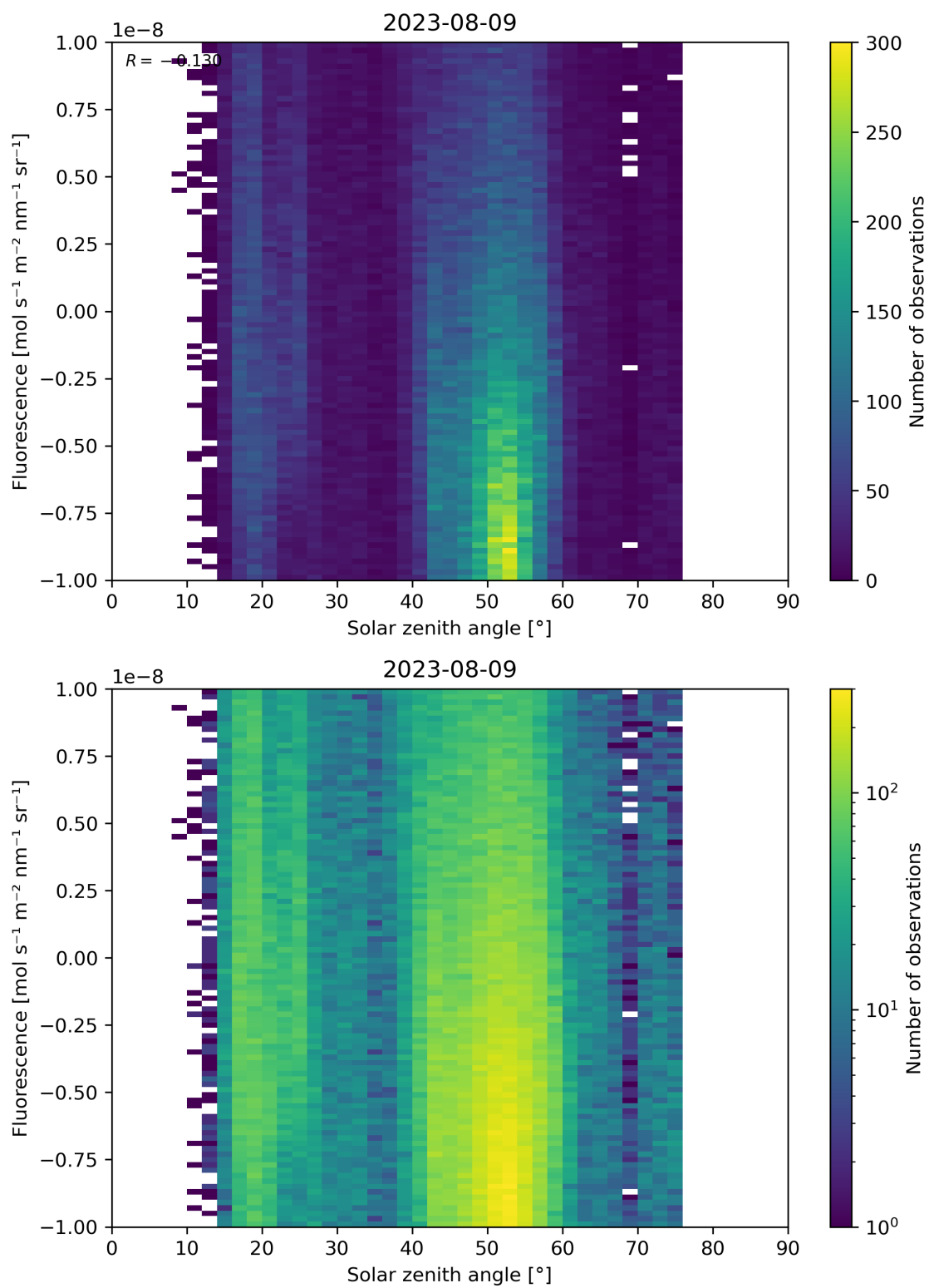
Figure 97: Scatter density plot of “Solar zenith angle” against “Fluorescence” for 2023-08-09 to 2023-08-10.
