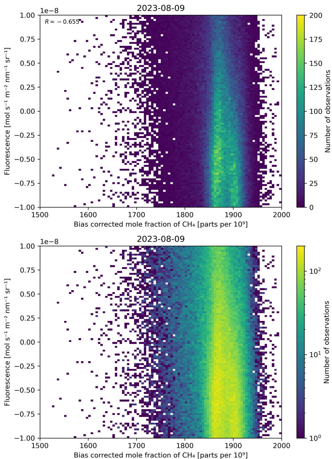
Figure 66: Scatter density plot of “Bias corrected mole fraction of \text{CH}_4 ” against “Fluorescence” for 2023-08-09 to 2023-08-10.
