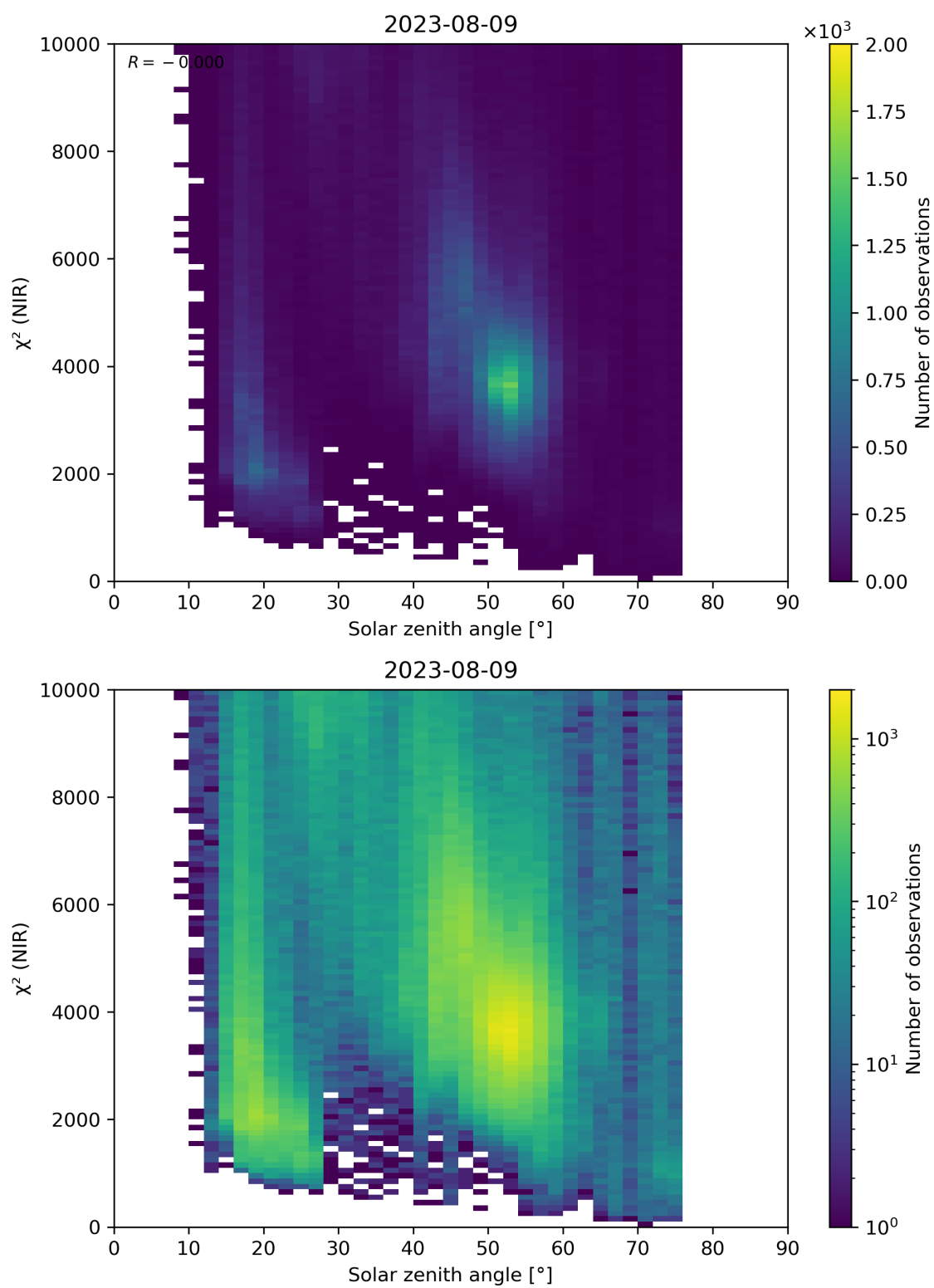
Figure 94: Scatter density plot of “Solar zenith angle” against “ \chi^2 (NIR)” for 2023-08-09 to 2023-08-10.
