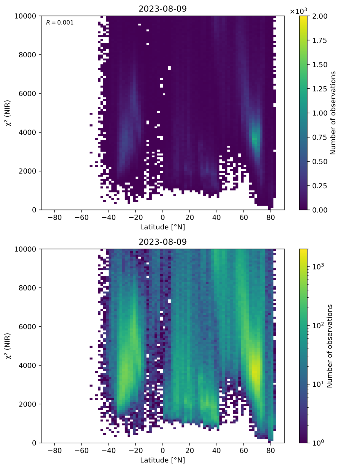
Figure 53: Scatter density plot of “Latitude” against “ \chi^2 (NIR)” for 2023-08-09 to 2023-08-10.
