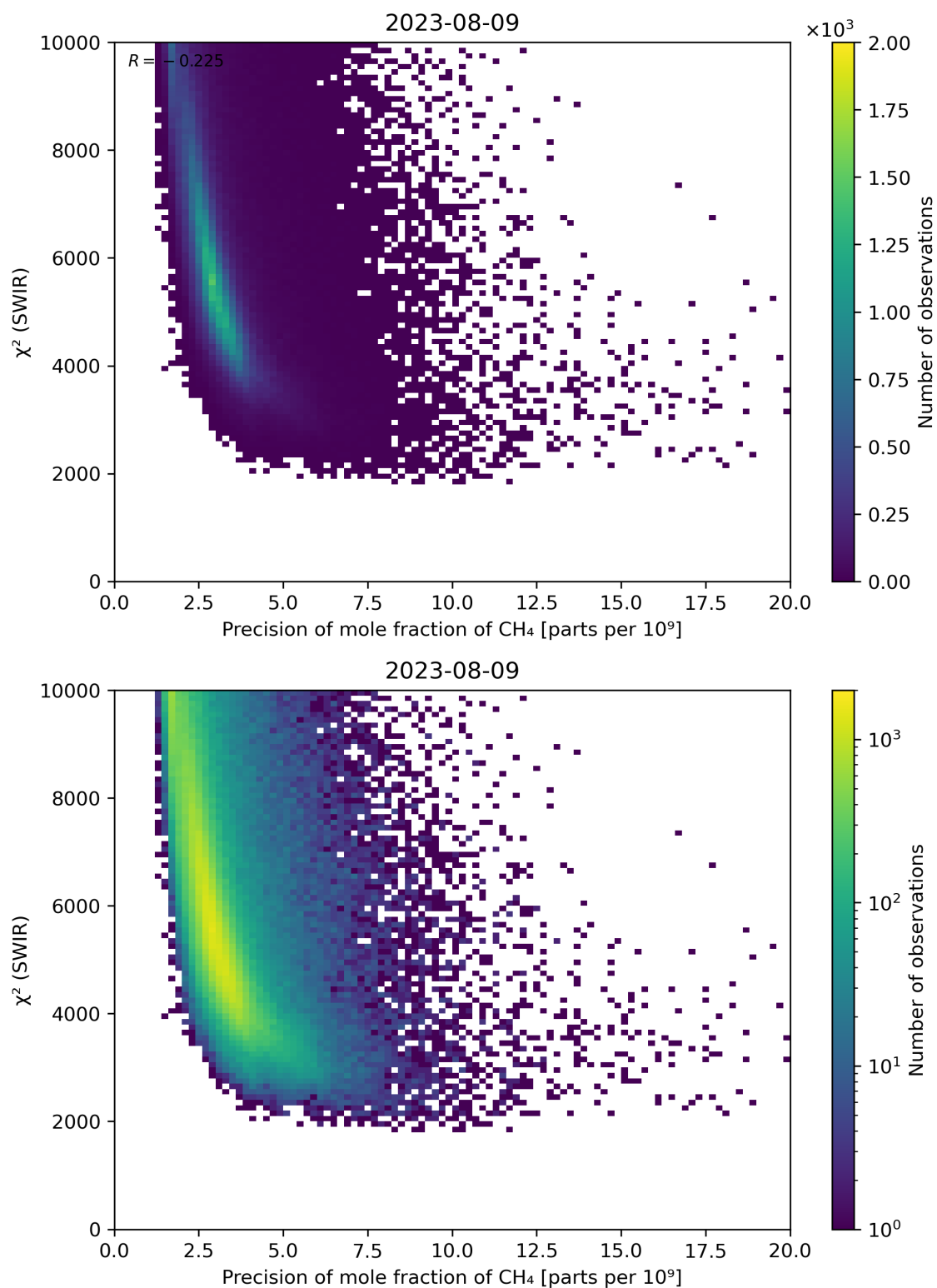
Figure 79: Scatter density plot of “Precision of mole fraction of \text{CH}_4 ” against “ \chi^2 (SWIR)” for 2023-08-09 to 2023-08-10.
