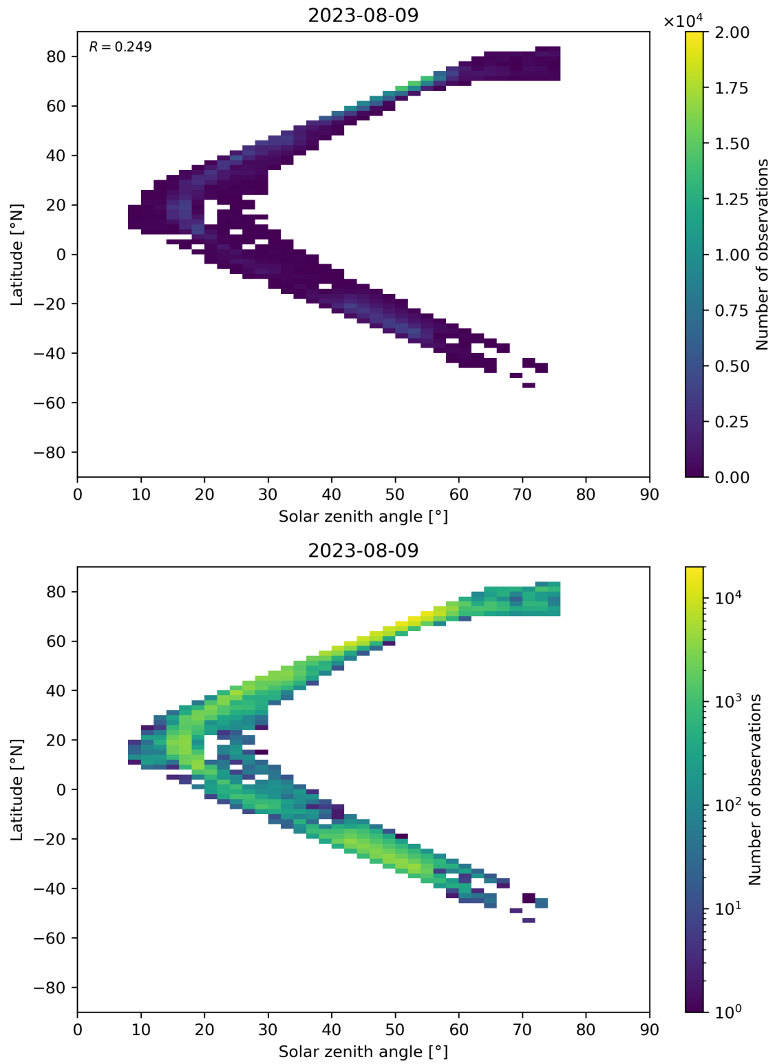
Figure 98: Scatter density plot of “Solar zenith angle” against “Latitude” for 2023-08-09 to 2023-08-10.
