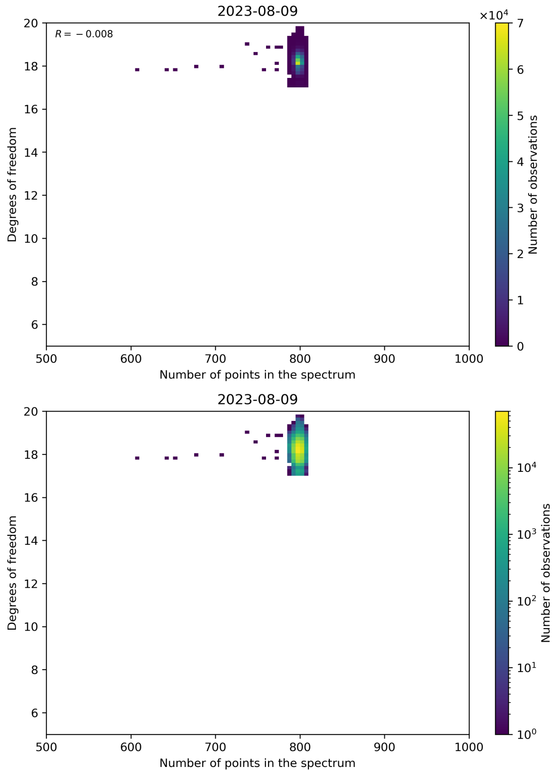
Figure 90: Scatter density plot of “Number of points in the spectrum” against “Degrees of freedom” for 2023-08-09 to 2023-08-10.
