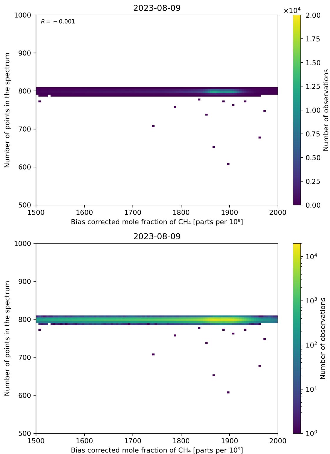
Figure 68: Scatter density plot of “Bias corrected mole fraction of CH 4 ” against “Number of points in the spectrum” for 2023-08-09 to 2023-08-10.
