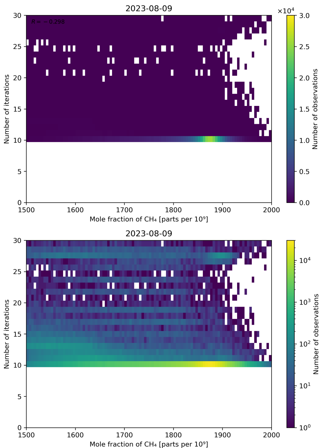
Figure 76: Scatter density plot of “Mole fraction of CH 4 ” against “Number of iterations” for 2023-08-09 to 2023-08-10.
