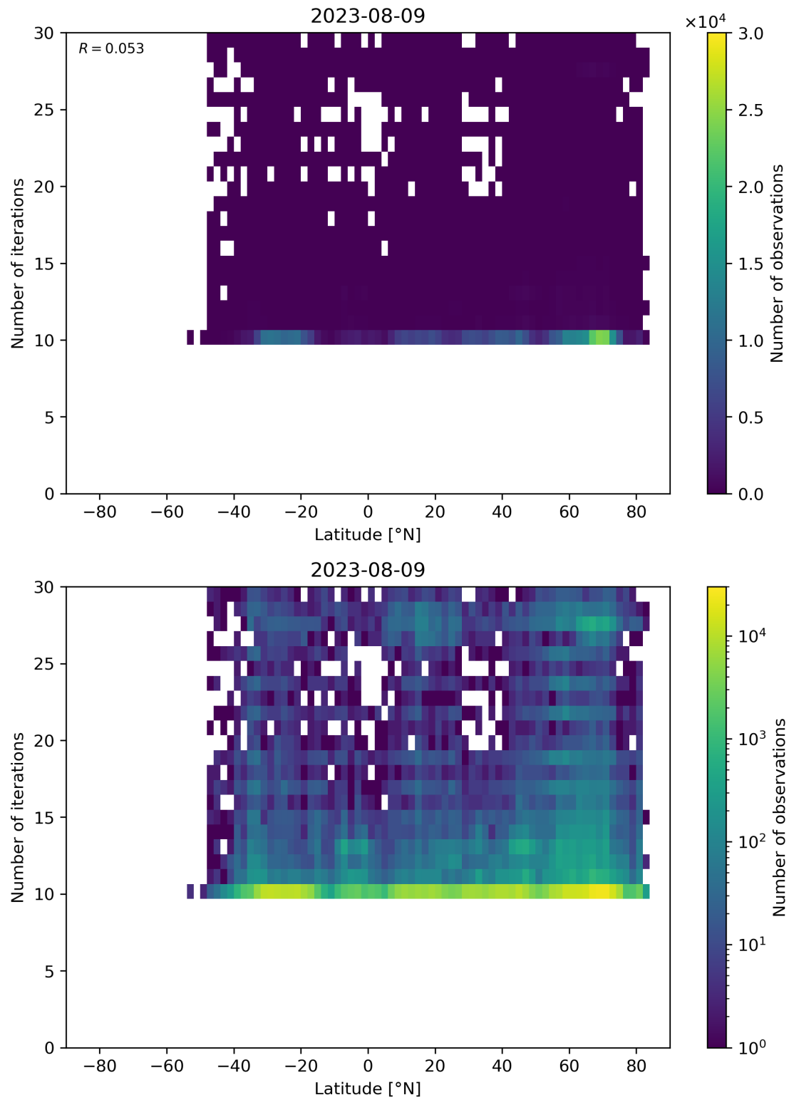
Figure 60: Scatter density plot of “Latitude” against “Number of iterations” for 2023-08-09 to 2023-08-10.
