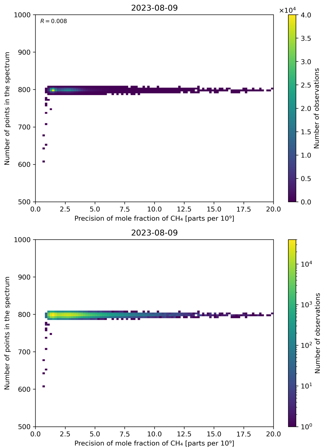
Figure 84: Scatter density plot of “Precision of mole fraction of CH 4 ” against “Number of points in the spectrum” for 2023-08-09 to 2023-08-10.
