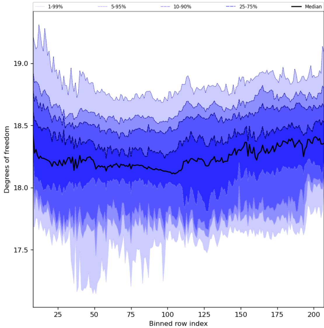
Figure 41: Along track statistics of “Degrees of freedom” for 2023-08-09 to 2023-08-10
