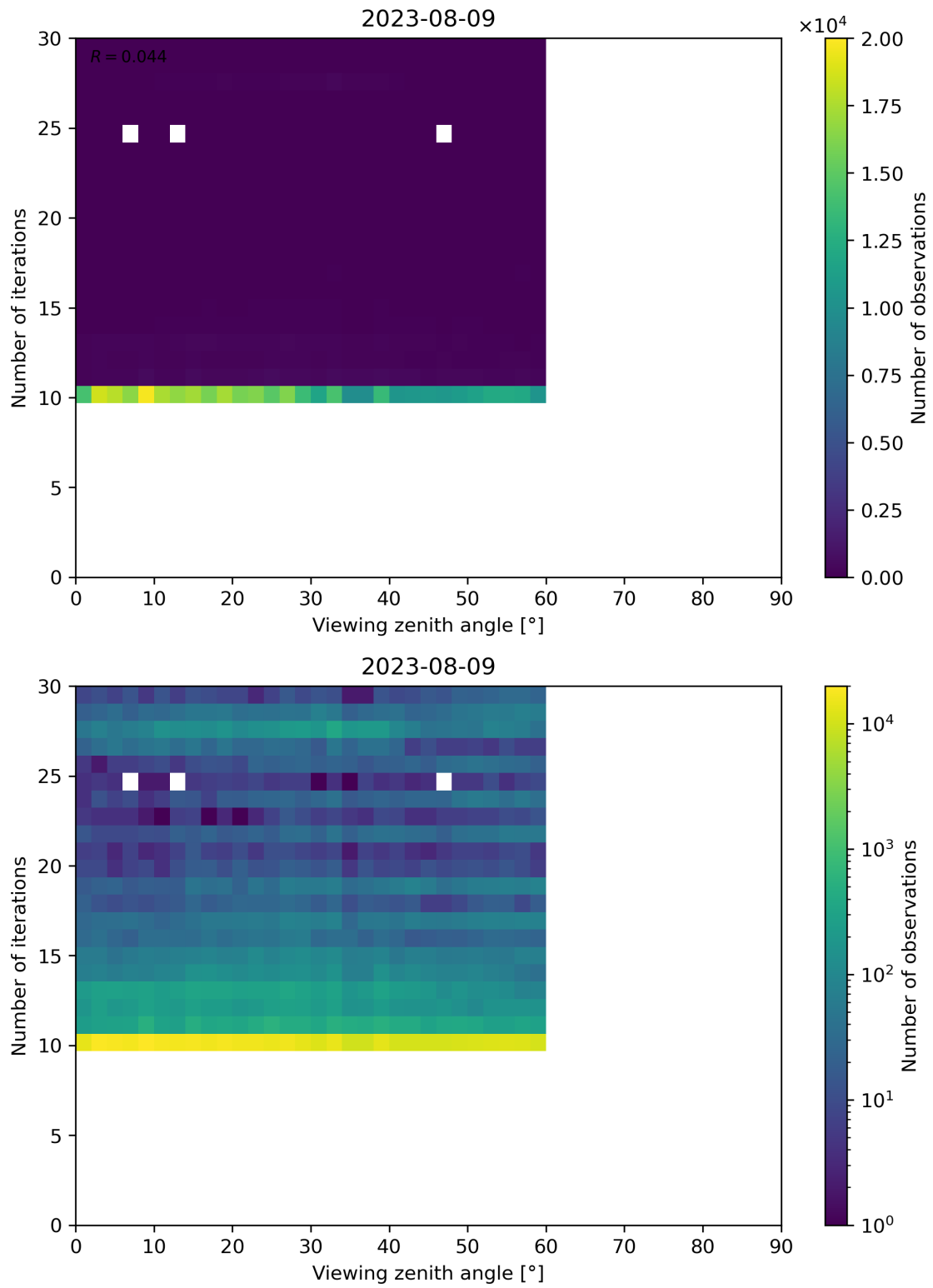
Figure 113: Scatter density plot of “Viewing zenith angle” against “Number of iterations” for 2023-08-09 to 2023-08-10.
