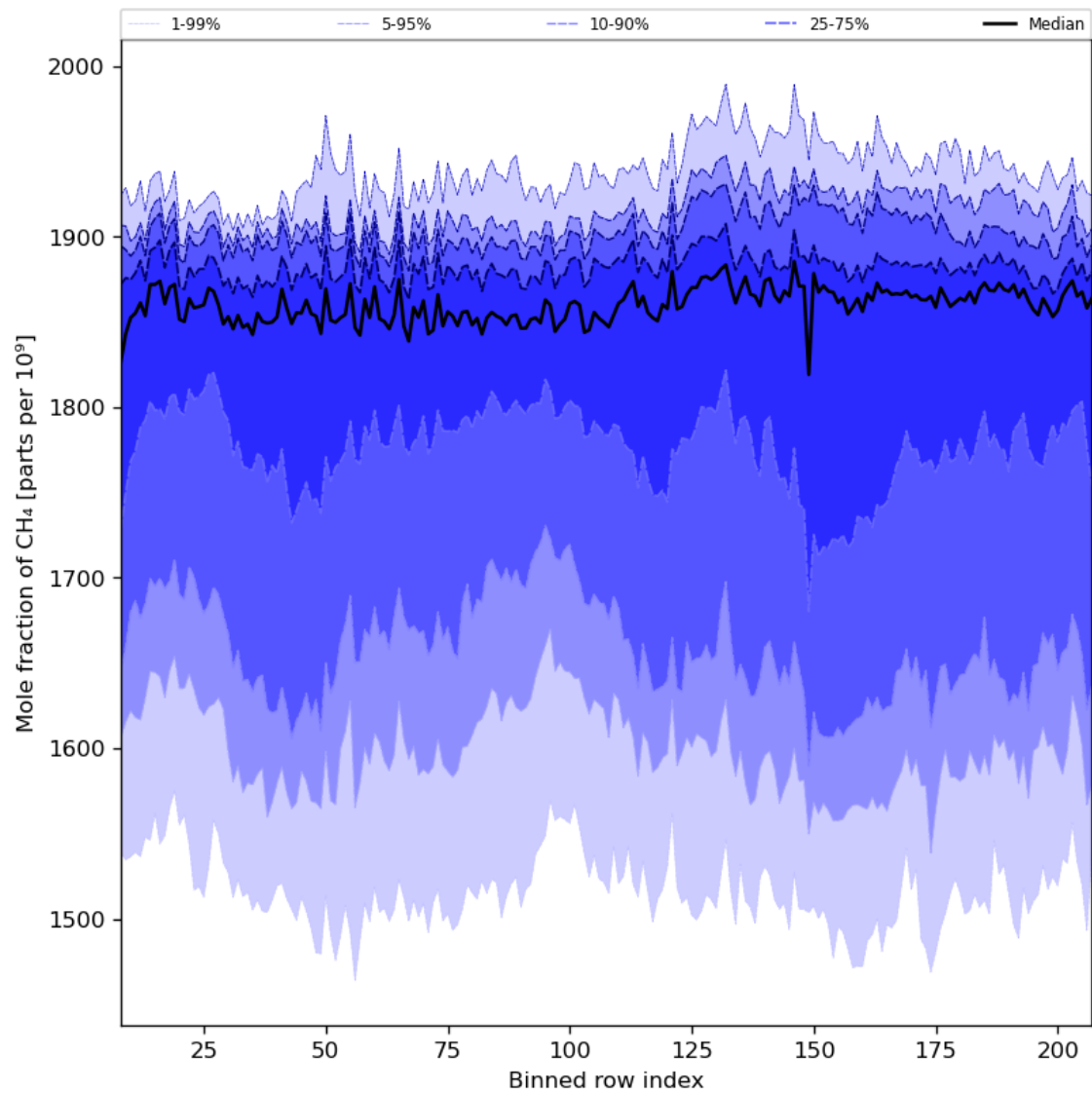
Figure 34: Along track statistics of “Mole fraction of CH 4 ” for 2023-08-09 to 2023-08-10
