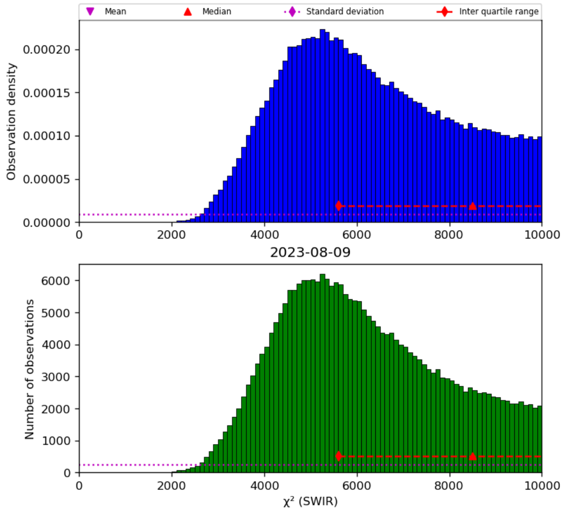
Figure 28: Histogram of “ \chi^2 (SWIR)” for 2023-08-09 to 2023-08-10
