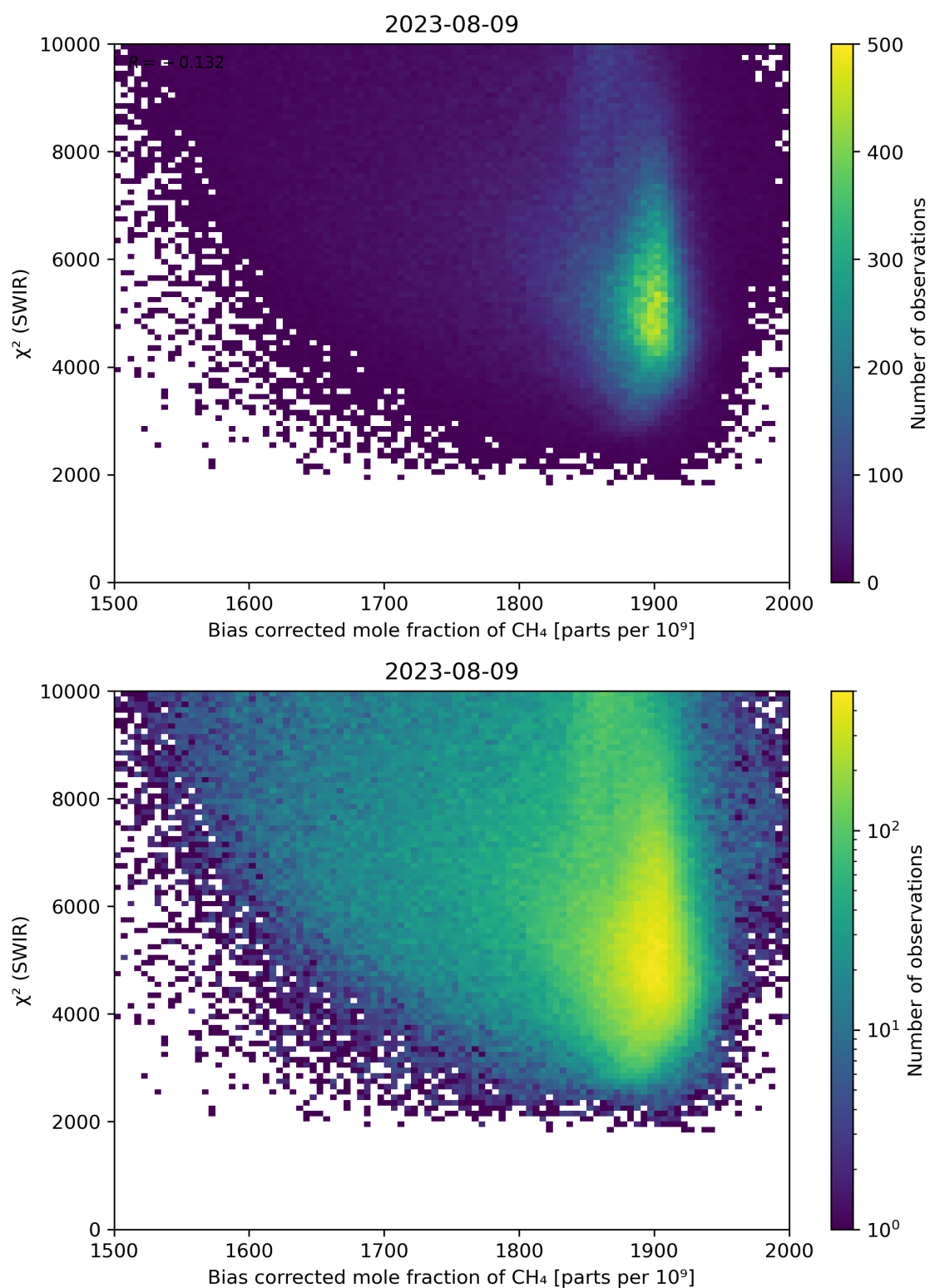
Figure 64: Scatter density plot of “Bias corrected mole fraction of CH 4 ” against “ \chi^2 (SWIR)” for 2023-08-09 to 2023-08-10.
