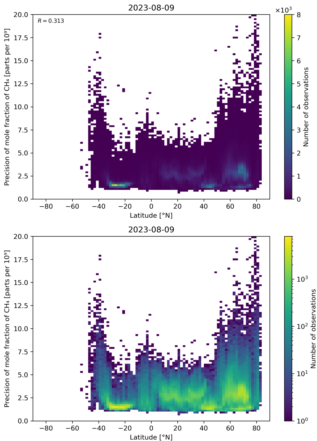
Figure 59: Scatter density plot of “Latitude” against “Precision of mole fraction of \text{CH}_4 ” for 2023-08-09 to 2023-08-10.
