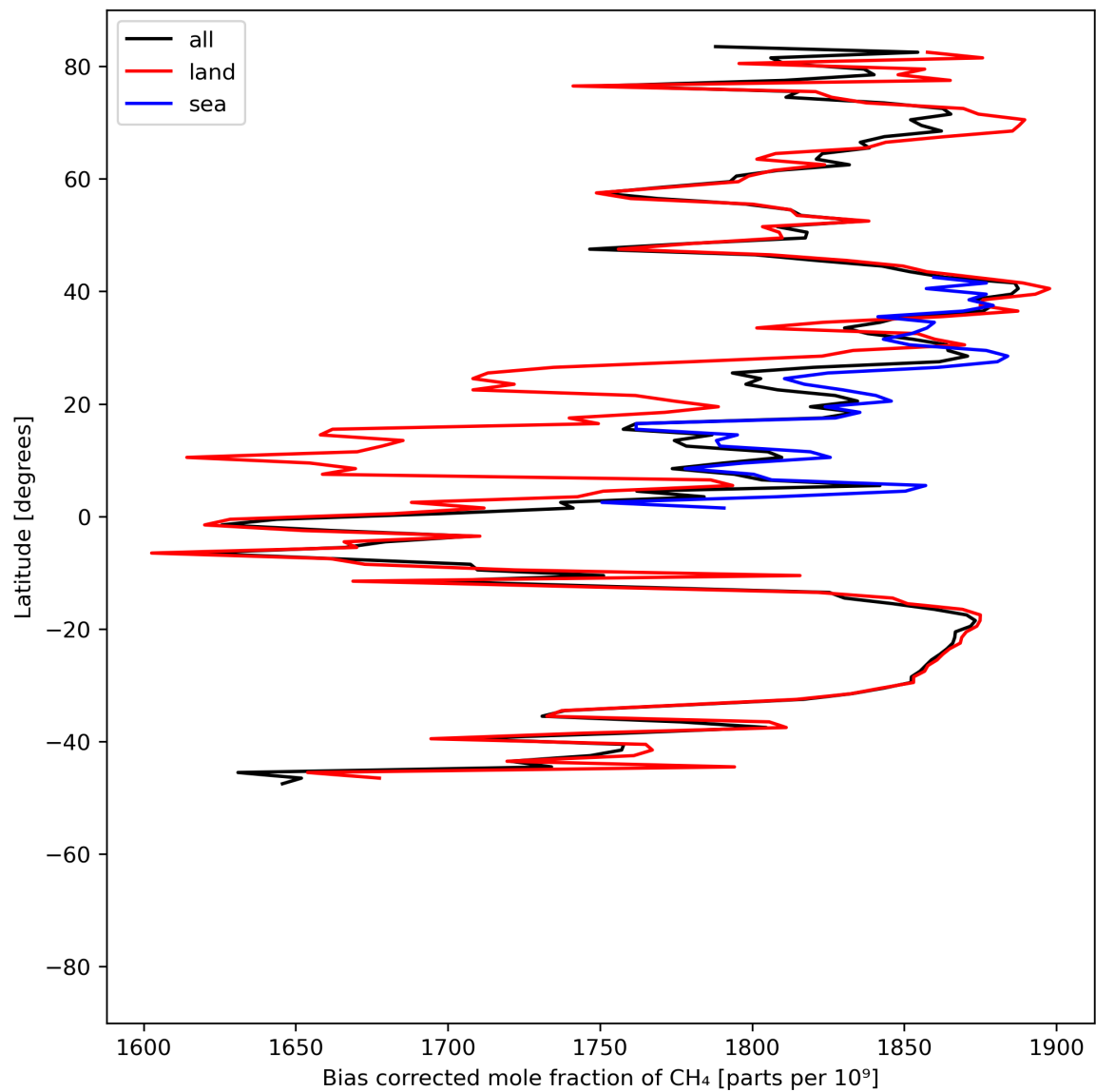
Figure 14: Zonal average of “Bias corrected mole fraction of CH 4 ” for 2023-08-09 to 2023-08-10.
