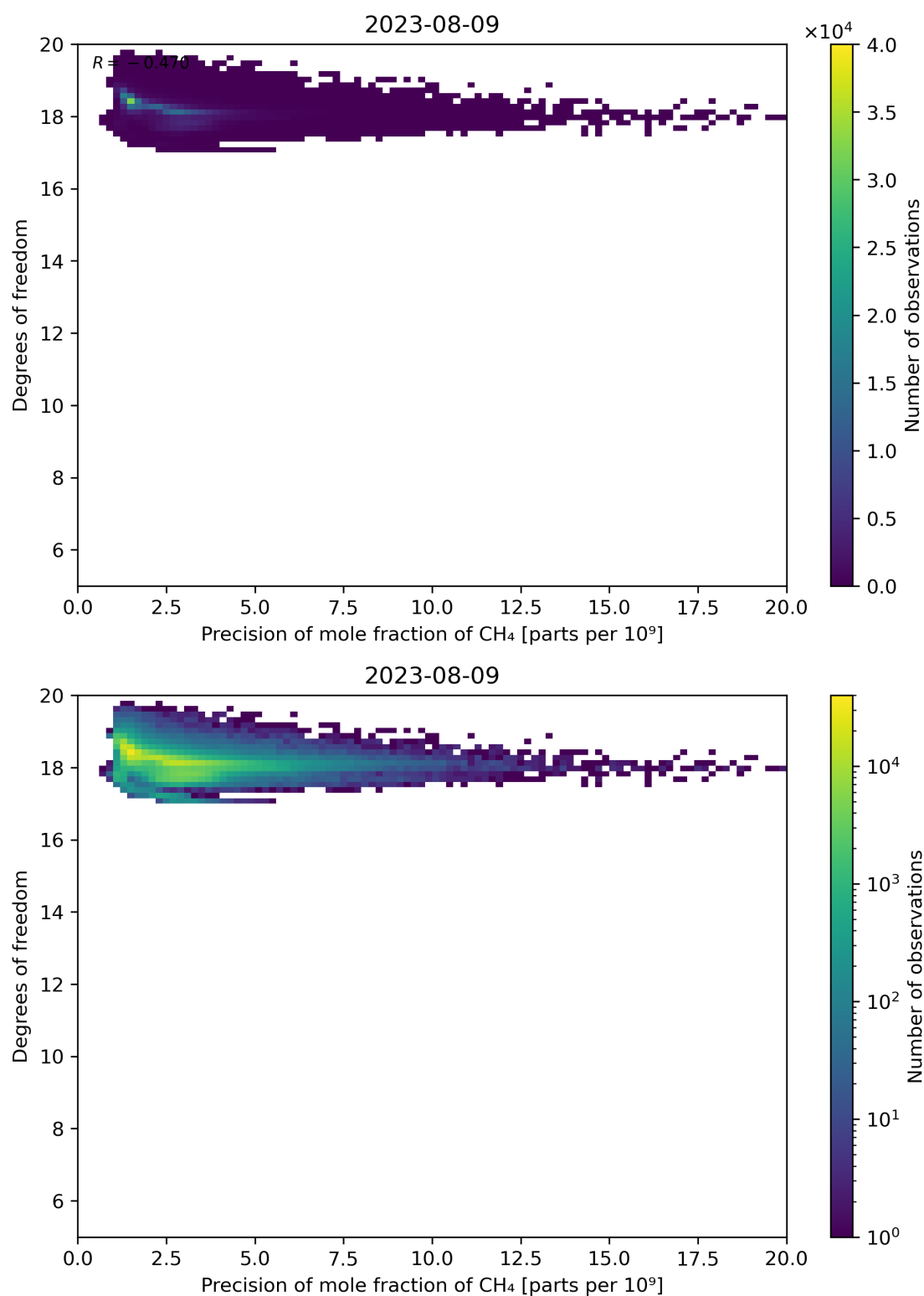
Figure 80: Scatter density plot of “Precision of mole fraction of CH 4 ” against “Degrees of freedom” for 2023-08-09 to 2023-08-10.
