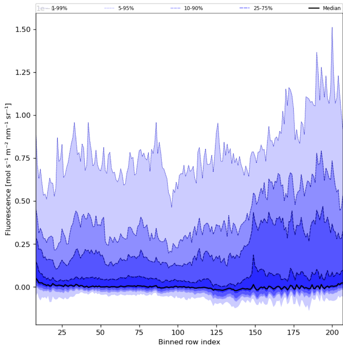
Figure 43: Along track statistics of “Fluorescence” for 2023-08-09 to 2023-08-10
