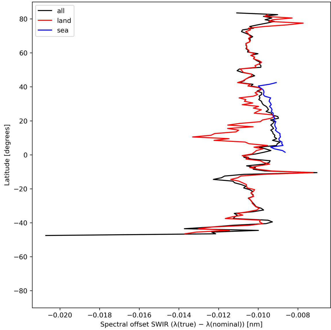
Figure 16: Zonal average of “Spectral offset SWIR ( \lambda(\text{true}) - \lambda(\text{nominal}) )” for 2023-08-09 to 2023-08-10.
