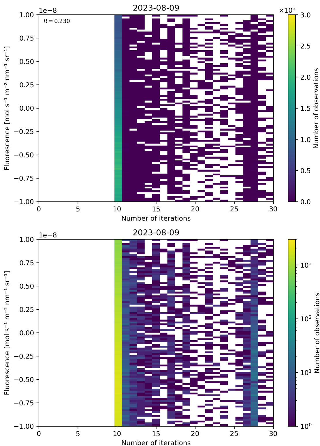
Figure 87: Scatter density plot of “Number of iterations” against “Fluorescence” for 2023-08-09 to 2023-08-10.
