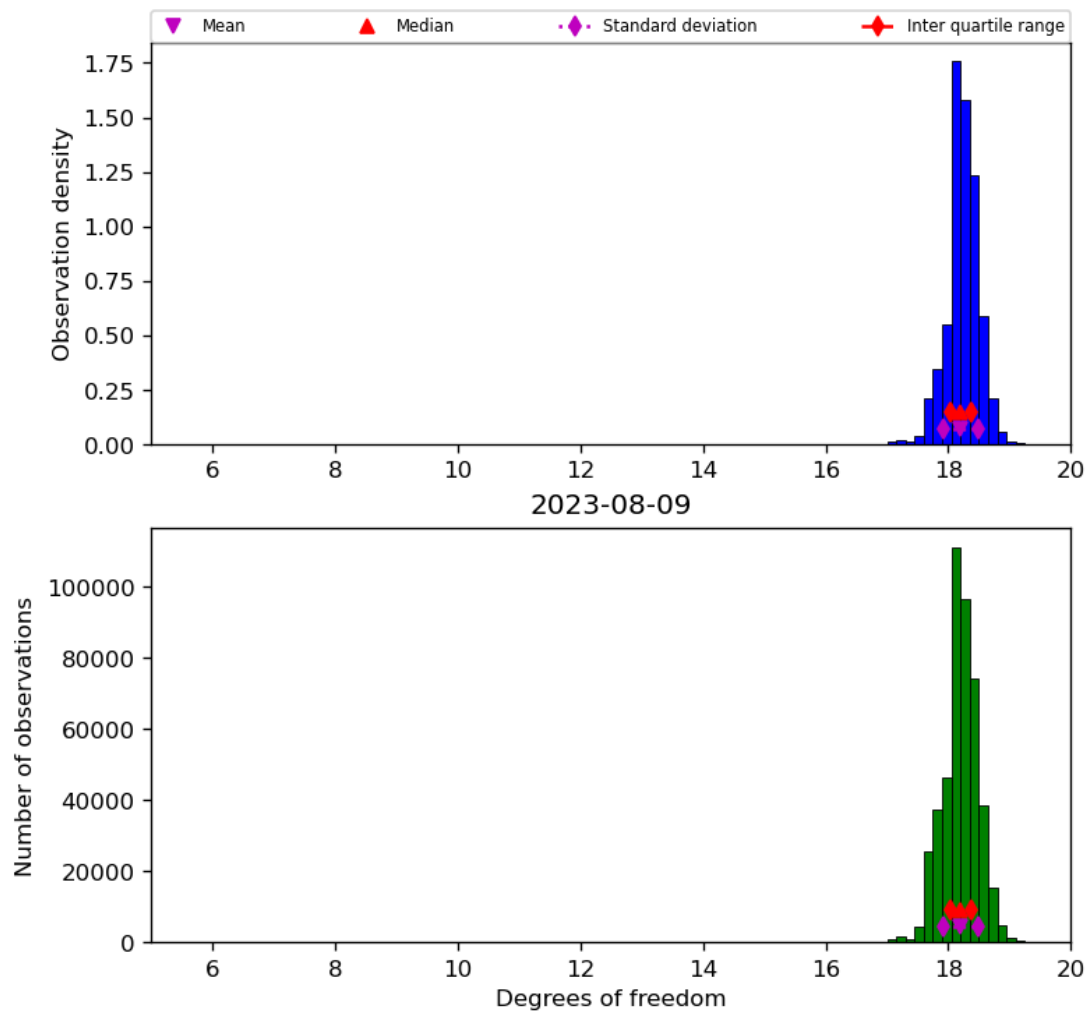
Figure 30: Histogram of “Degrees of freedom” for 2023-08-09 to 2023-08-10
