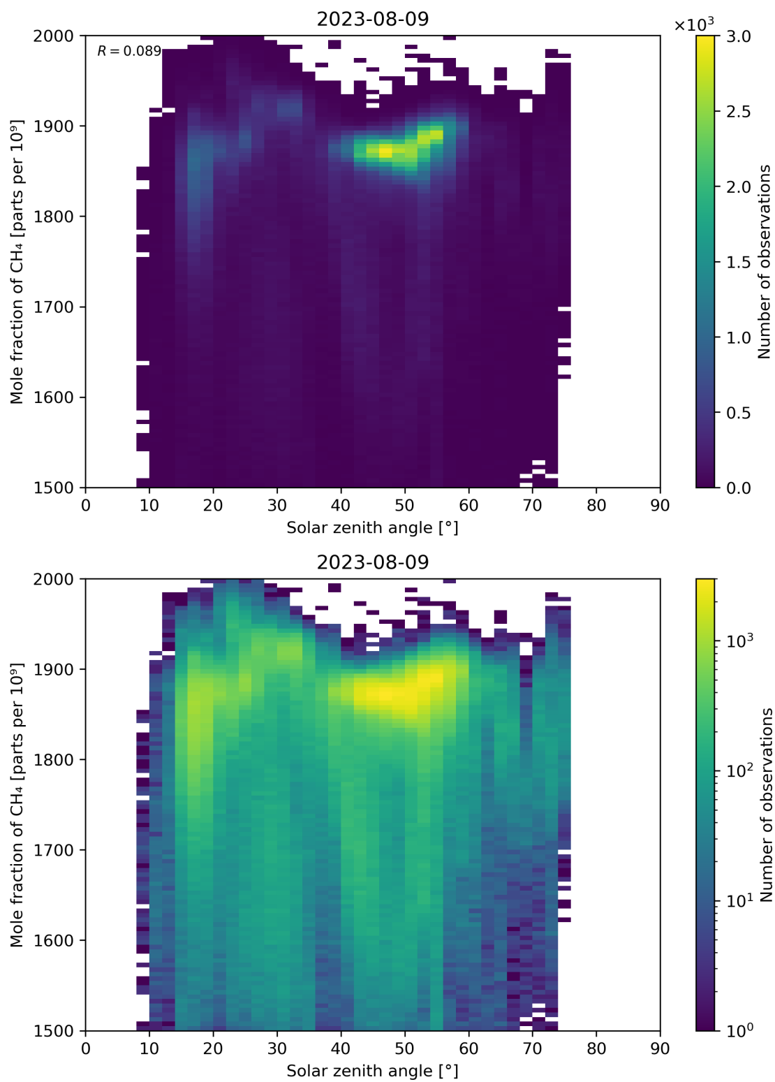
Figure 99: Scatter density plot of “Solar zenith angle” against “Mole fraction of \text{CH}_4 ” for 2023-08-09 to 2023-08-10.
