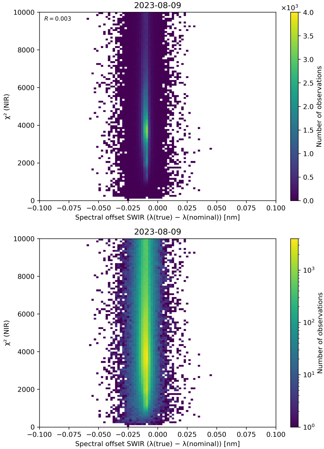
Figure 117: Scatter density plot of “Spectral offset SWIR ( \lambda(\text{true}) - \lambda(\text{nominal}) )” against “ \chi^2 (NIR)” for 2023-08-09 to 2023-08-10.
