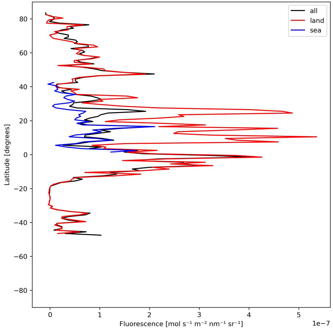
Figure 21: Zonal average of “Fluorescence” for 2023-08-09 to 2023-08-10.
