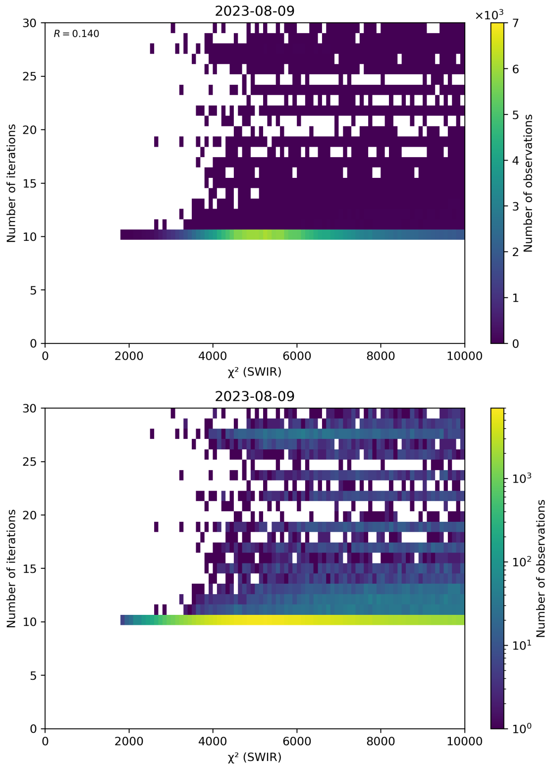
Figure 50: Scatter density plot of “ \chi^2 (SWIR)” against “Number of iterations” for 2023-08-09 to 2023-08-10.
