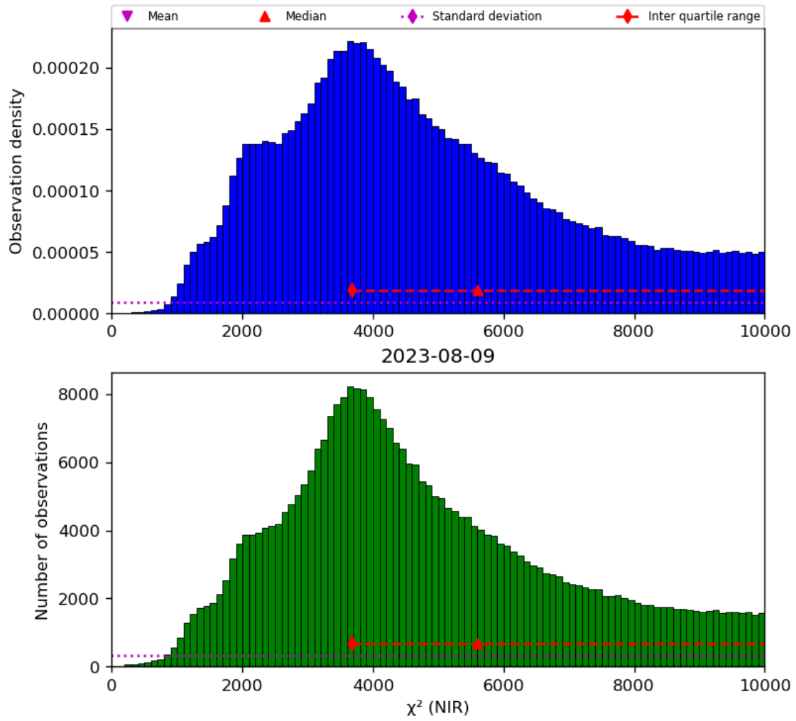
Figure 29: Histogram of “ \chi^2 (NIR)” for 2023-08-09 to 2023-08-10
