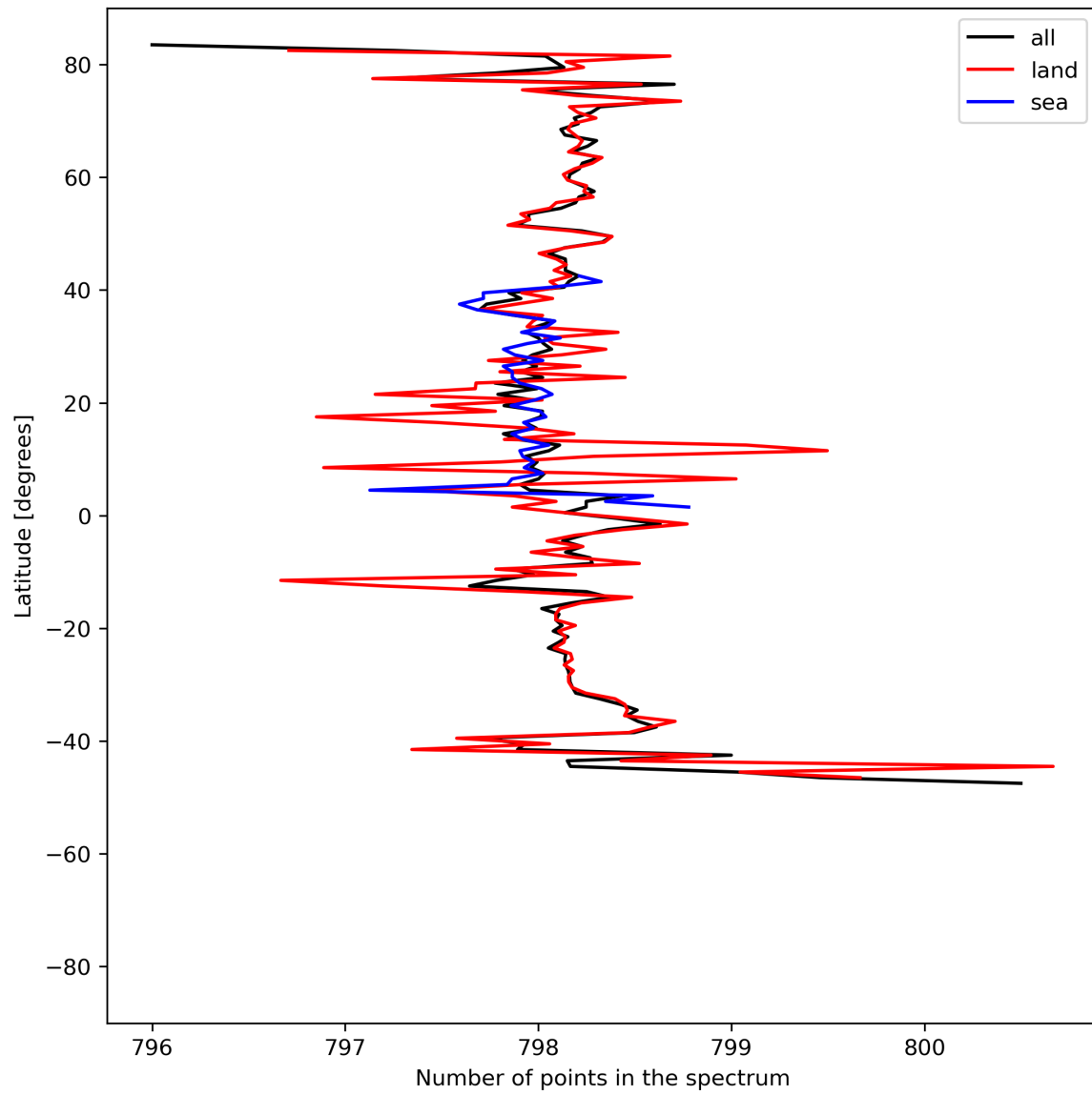
Figure 15: Zonal average of “Number of points in the spectrum” for 2023-08-09 to 2023-08-10.
