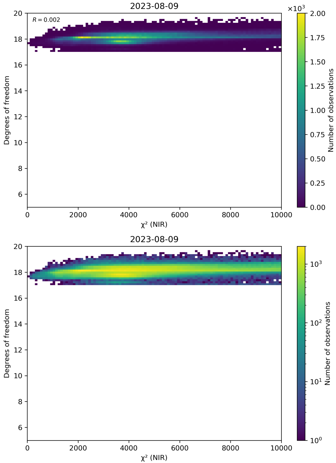
Figure 44: Scatter density plot of “ \chi^2 (NIR)” against “Degrees of freedom” for 2023-08-09 to 2023-08-10.
