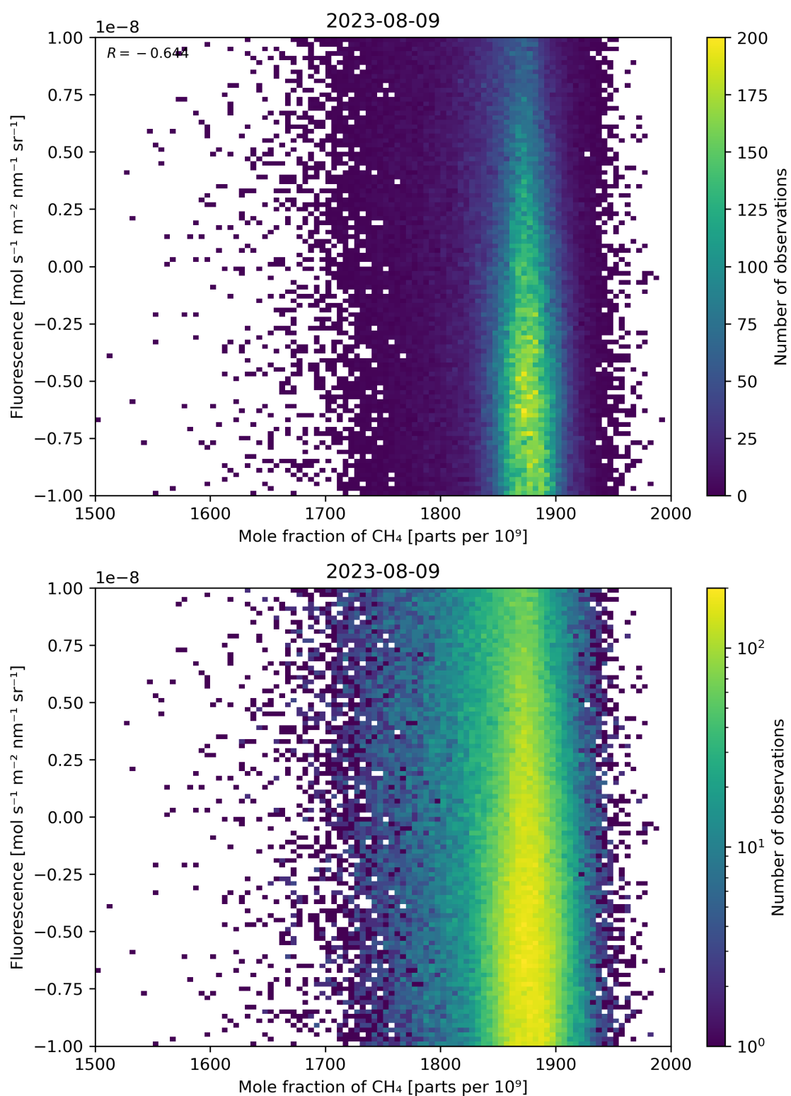
Figure 73: Scatter density plot of “Mole fraction of \text{CH}_4 ” against “Fluorescence” for 2023-08-09 to 2023-08-10.
