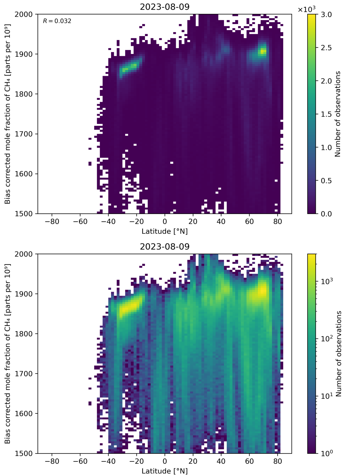
Figure 58: Scatter density plot of “Latitude” against “Bias corrected mole fraction of CH 4 ” for 2023-08-09 to 2023-08-10.
