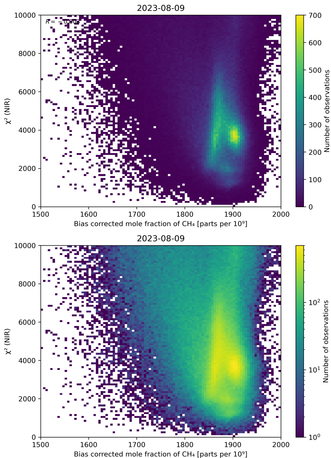
Figure 63: Scatter density plot of “Bias corrected mole fraction of CH 4 ” against “ \chi^2 (NIR)” for 2023-08-09 to 2023-08-10.
