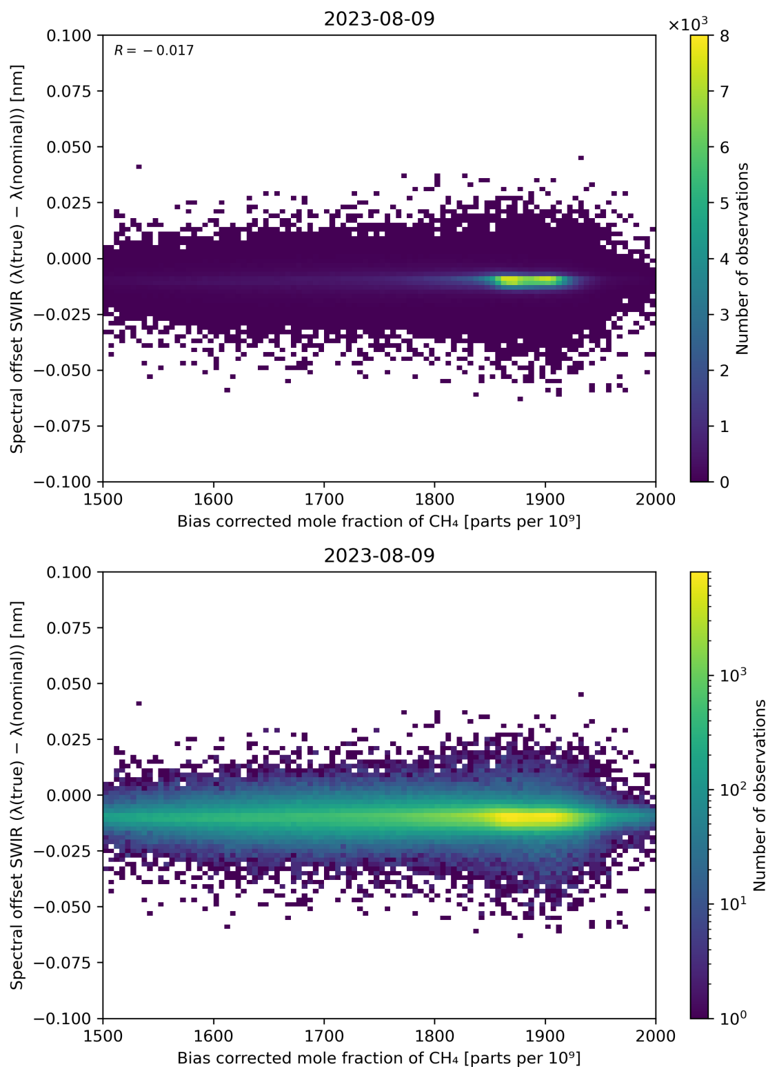
Figure 69: Scatter density plot of “Bias corrected mole fraction of \text{CH}_4 ” against “Spectral offset SWIR ( \lambda(\text{true}) - \lambda(\text{nominal}) )” for 2023-08-09 to 2023-08-10.
