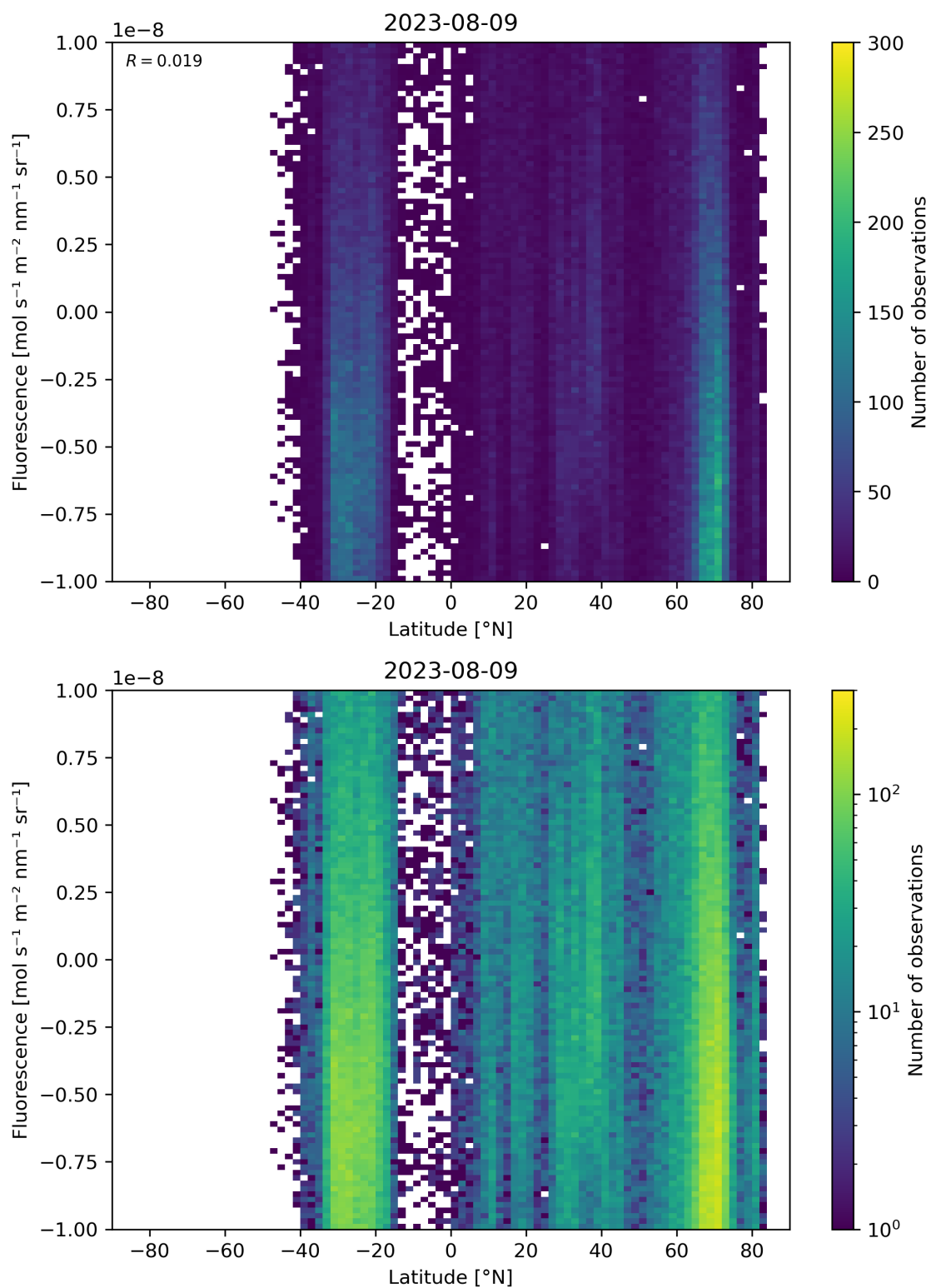
Figure 56: Scatter density plot of “Latitude” against “Fluorescence” for 2023-08-09 to 2023-08-10.
