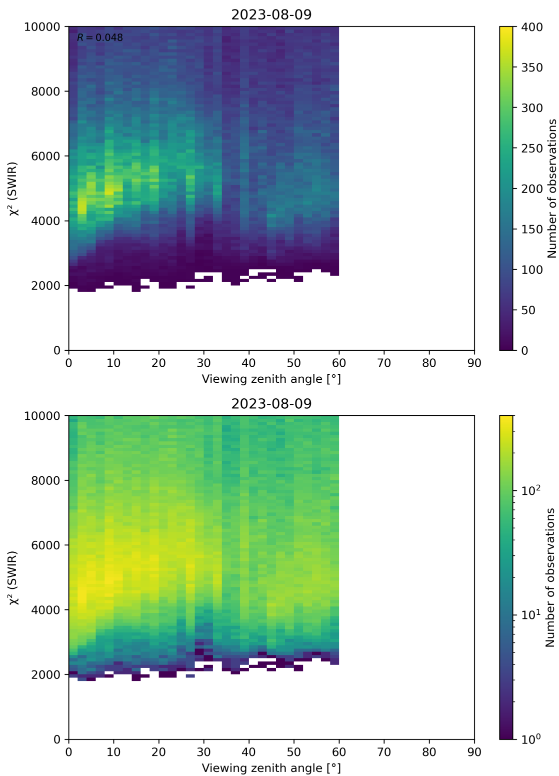
Figure 106: Scatter density plot of “Viewing zenith angle” against “ \chi^2 (SWIR)” for 2023-08-09 to 2023-08-10.
