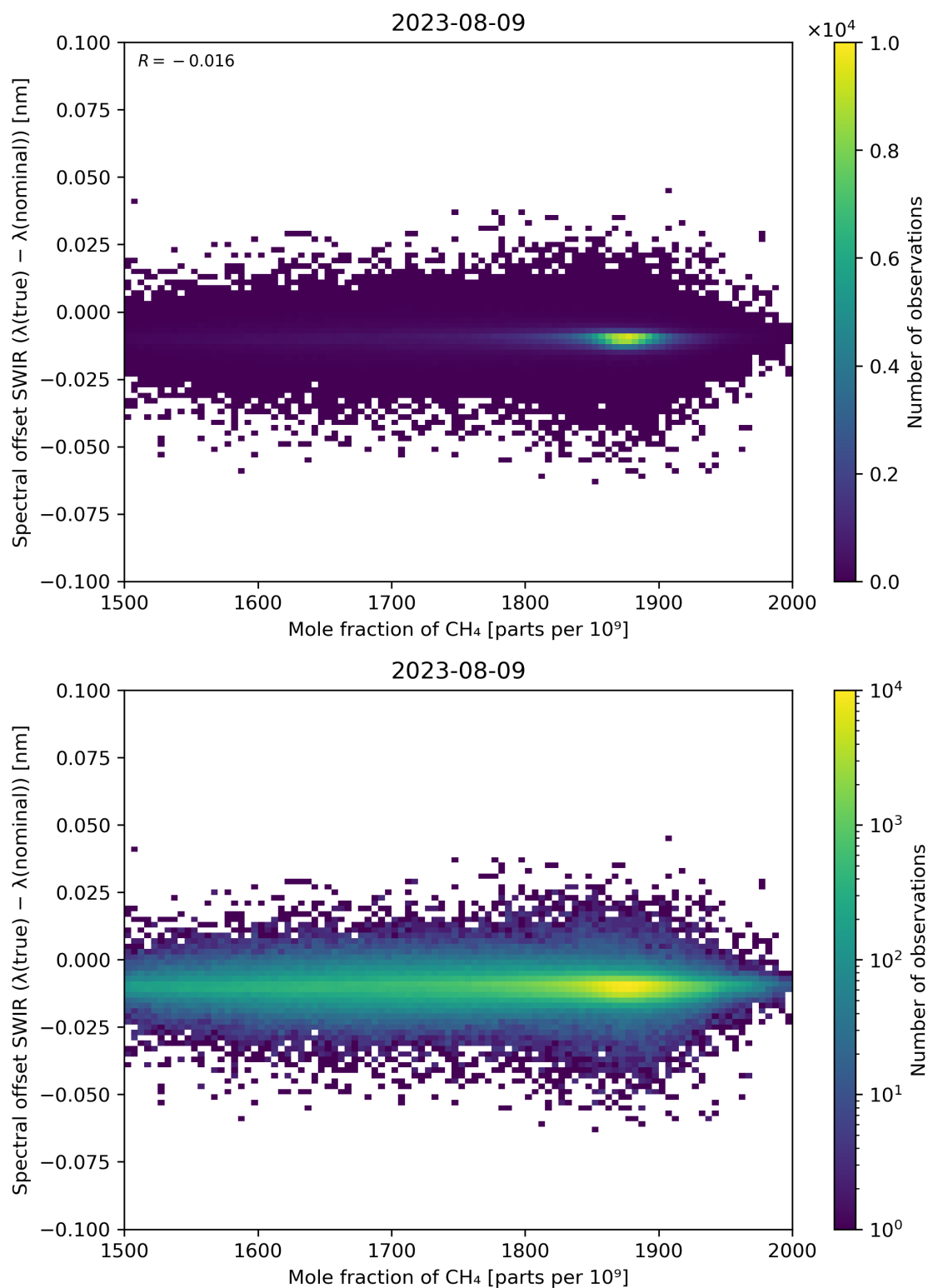
Figure 86: Scatter density plot of “Mole fraction of CH 4 ” against “Spectral offset SWIR ( \lambda(\text{true}) - \lambda(\text{nominal}) )” for 2023-08-09 to 2023-08-10.
