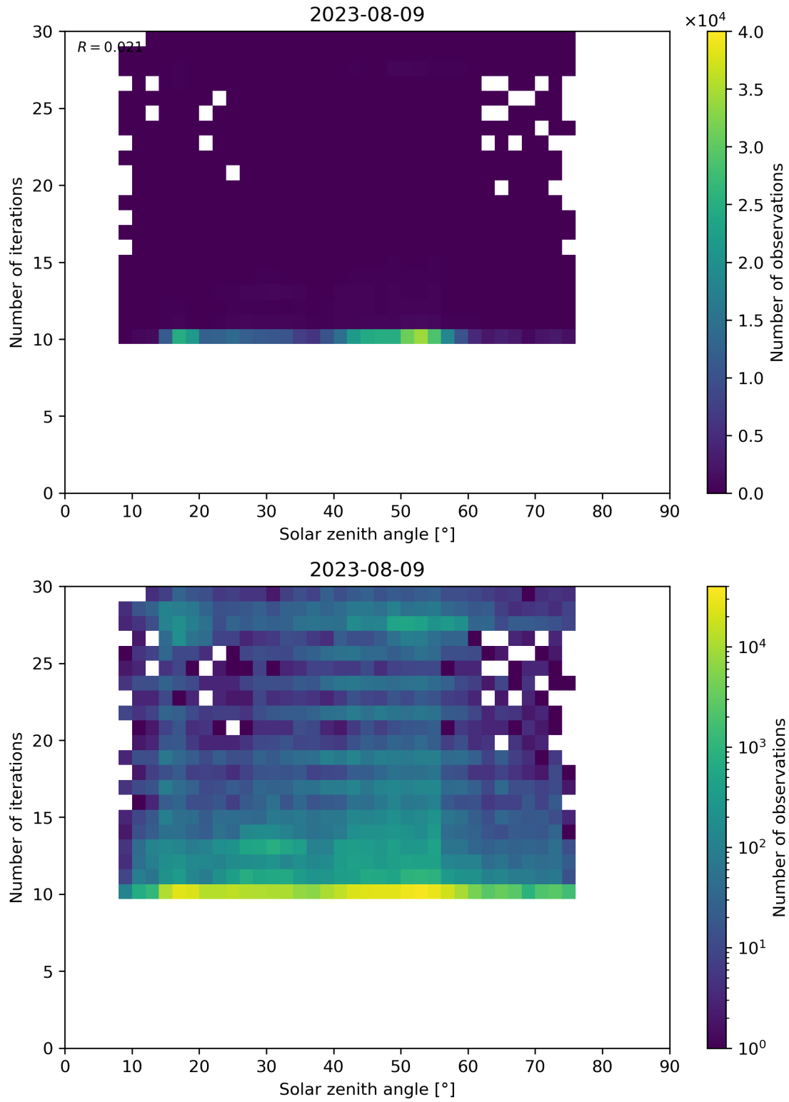
Figure 102: Scatter density plot of “Solar zenith angle” against “Number of iterations” for 2023-08-09 to 2023-08-10.
