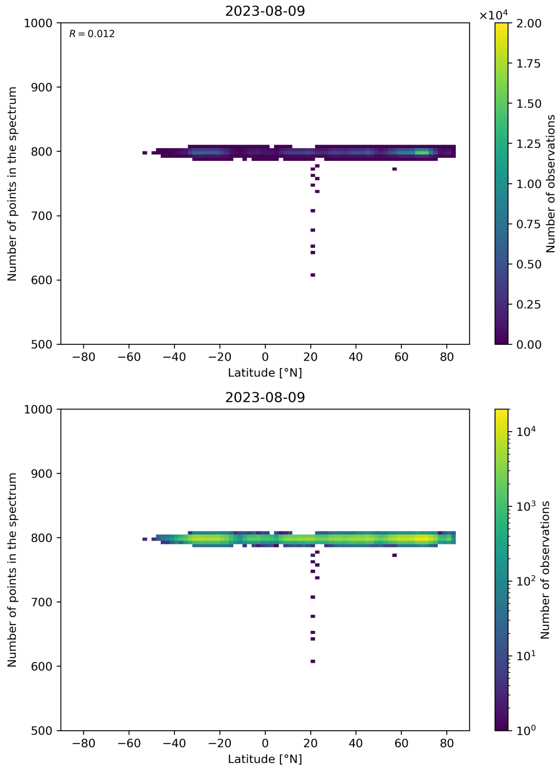
Figure 61: Scatter density plot of “Latitude” against “Number of points in the spectrum” for 2023-08-09 to 2023-08-10.
