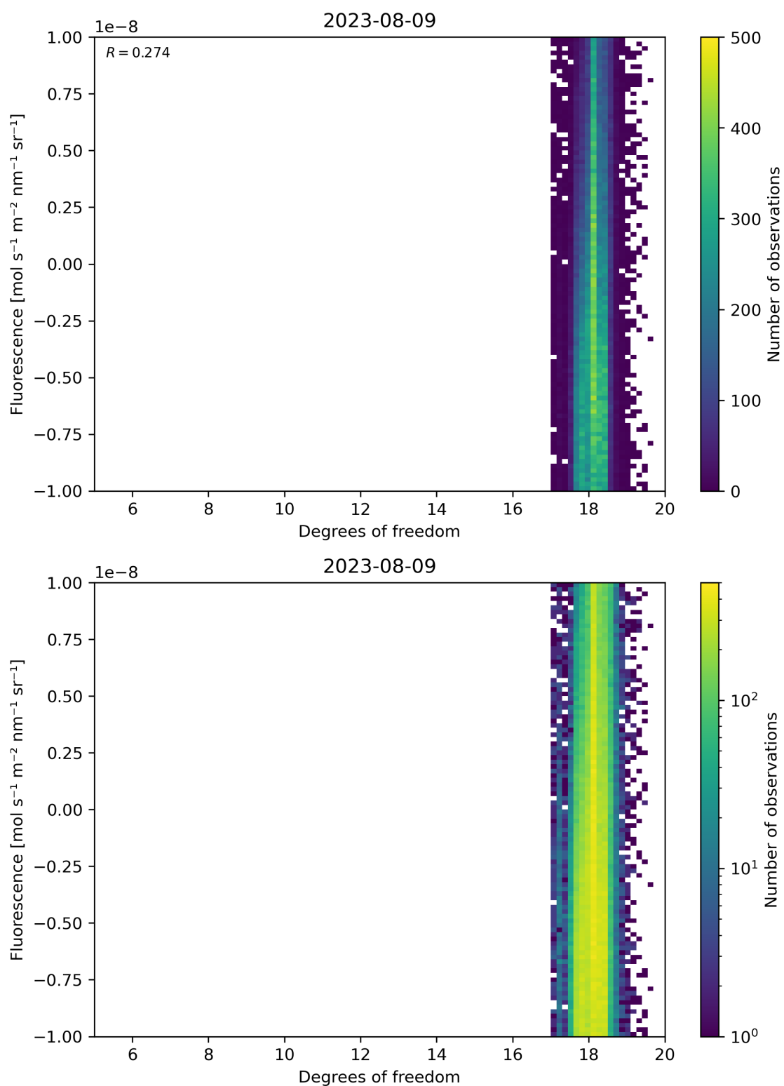
Figure 51: Scatter density plot of “Degrees of freedom” against “Fluorescence” for 2023-08-09 to 2023-08-10.
