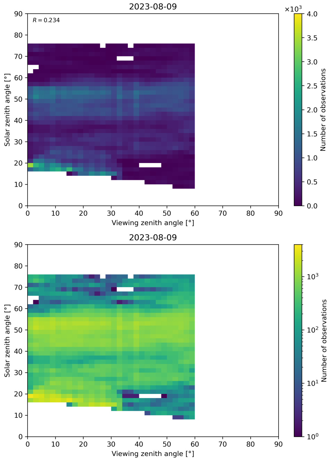
Figure 115: Scatter density plot of “Viewing zenith angle” against “Solar zenith angle” for 2023-08-09 to 2023-08-10.
