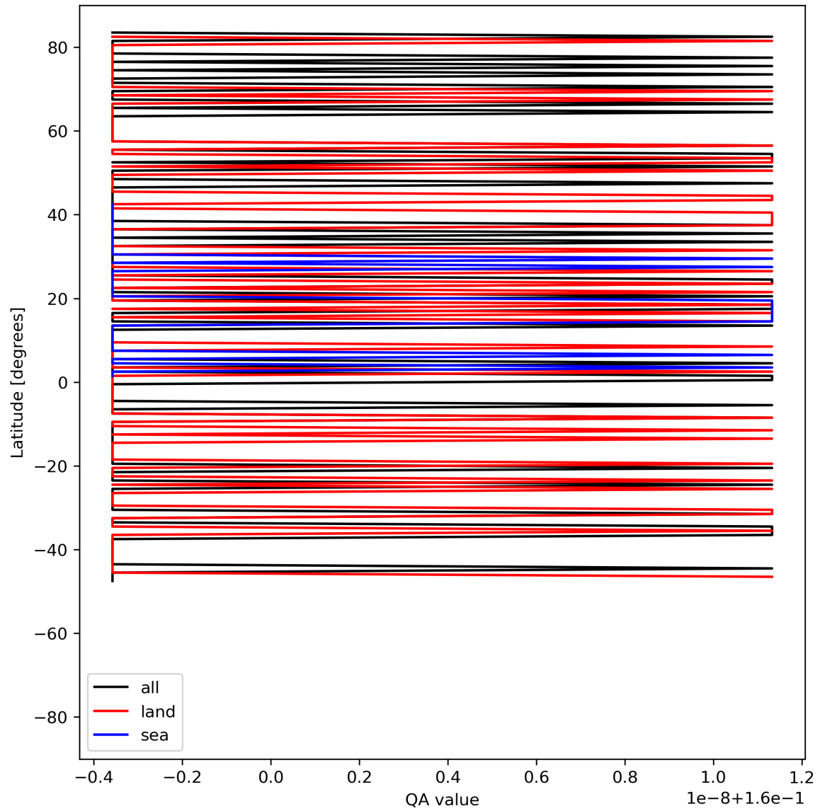
Figure 11: Zonal average of “QA value” for 2023-08-09 to 2023-08-10.
