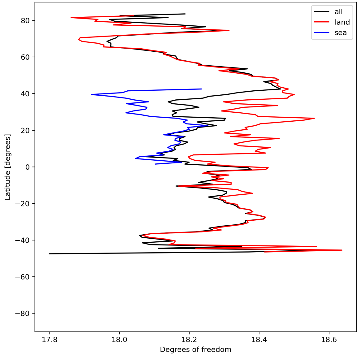
Figure 19: Zonal average of “Degrees of freedom” for 2023-08-09 to 2023-08-10.
