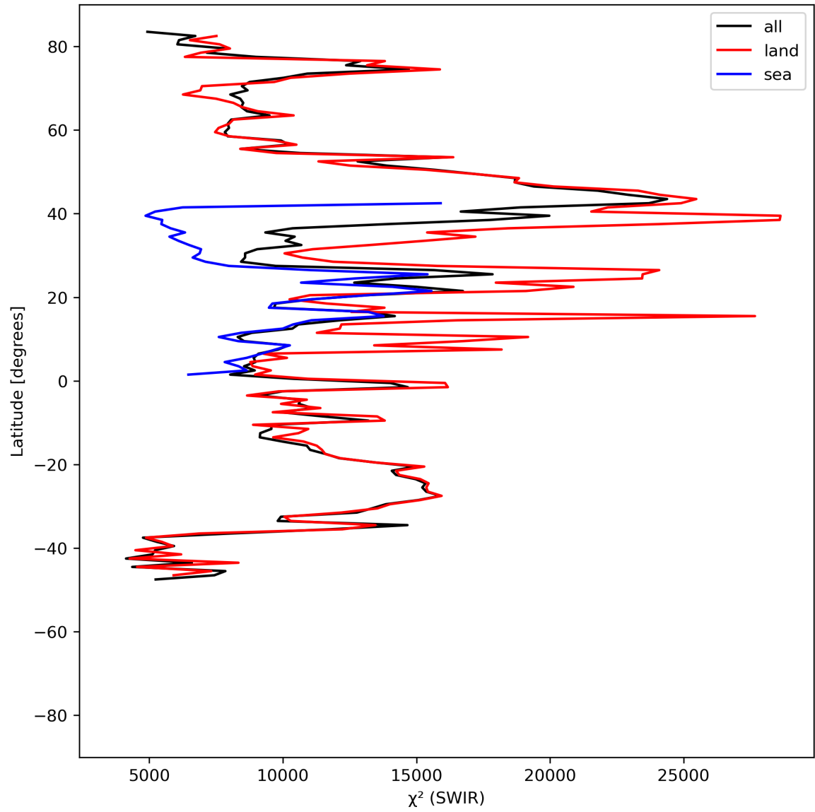
Figure 17: Zonal average of “ \chi^2 (SWIR)” for 2023-08-09 to 2023-08-10.
