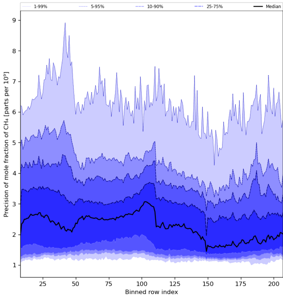
Figure 35: Along track statistics of “Precision of mole fraction of CH 4 ” for 2023-08-09 to 2023-08-10
