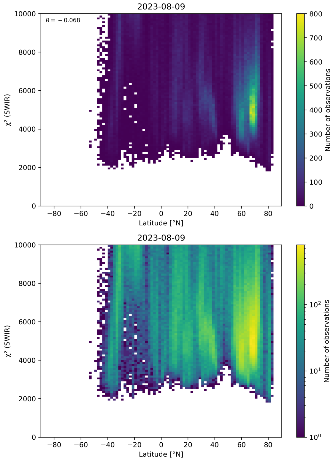
Figure 54: Scatter density plot of “Latitude” against “ \chi^2 (SWIR)” for 2023-08-09 to 2023-08-10.
