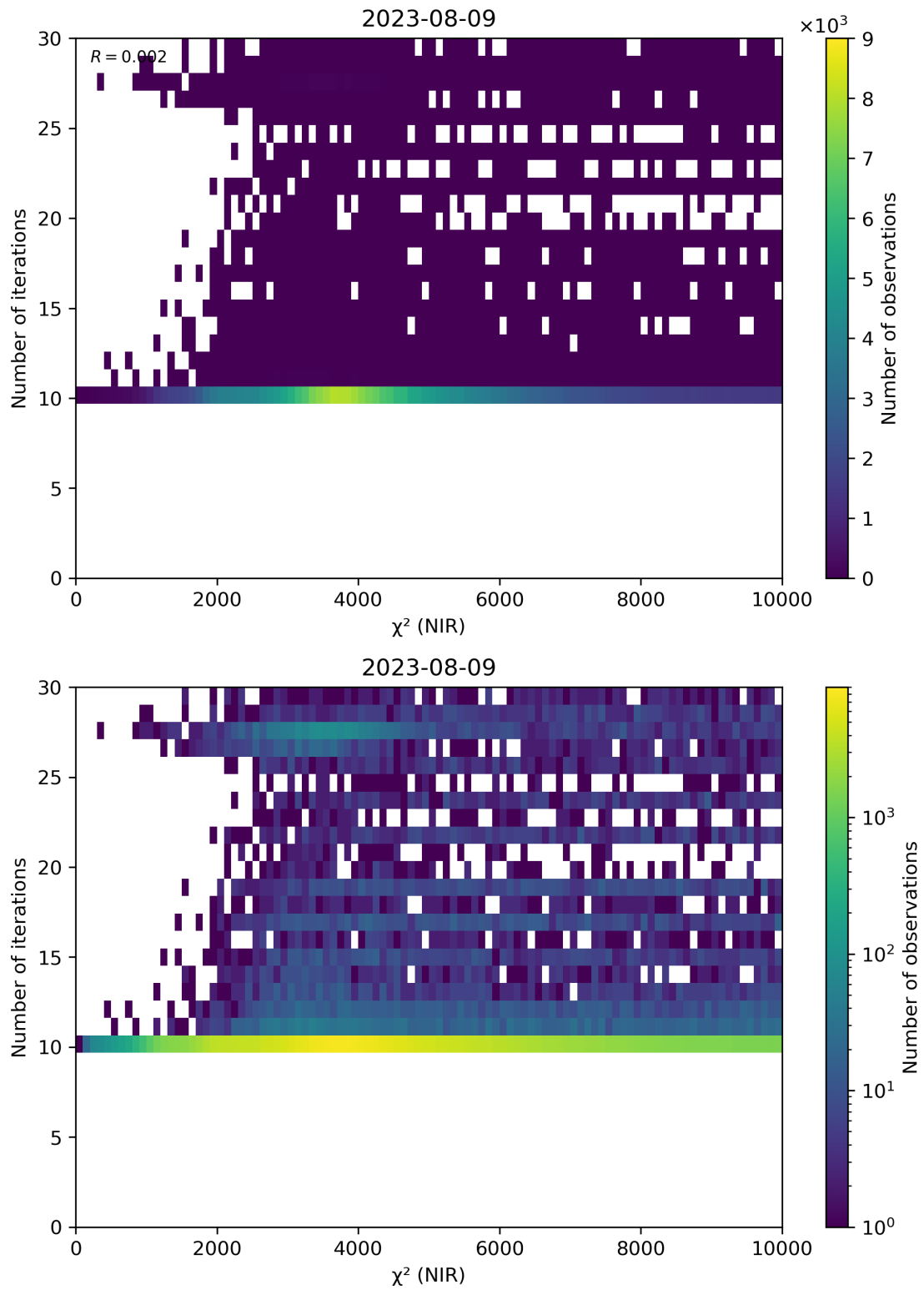
Figure 46: Scatter density plot of “ \chi^2 (NIR)” against “Number of iterations” for 2023-08-09 to 2023-08-10.
