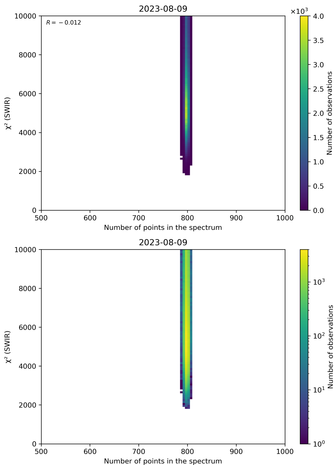
Figure 89: Scatter density plot of “Number of points in the spectrum” against “ \chi^2 (SWIR)” for 2023-08-09 to 2023-08-10.
