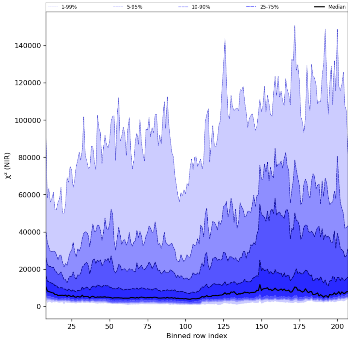
Figure 40: Along track statistics of “ \chi^2 (NIR)” for 2023-08-09 to 2023-08-10
