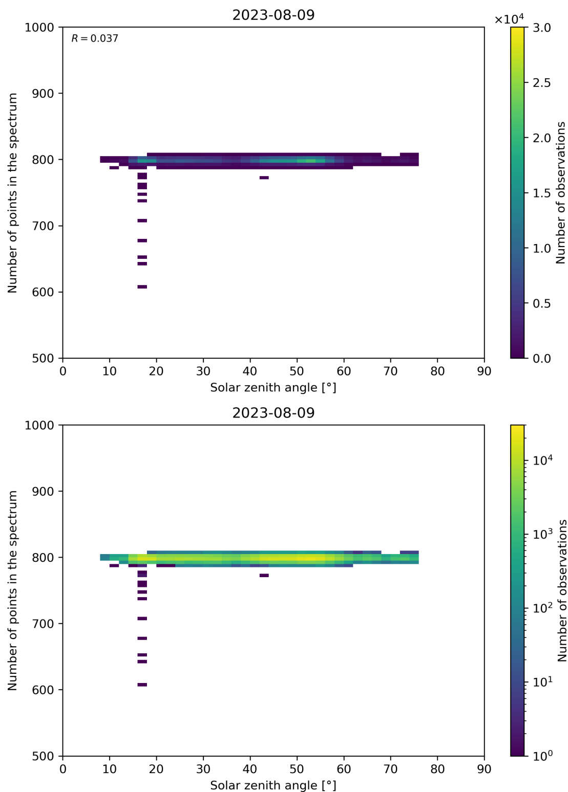
Figure 103: Scatter density plot of “Solar zenith angle” against “Number of points in the spectrum” for 2023-08-09 to 2023-08-10.
