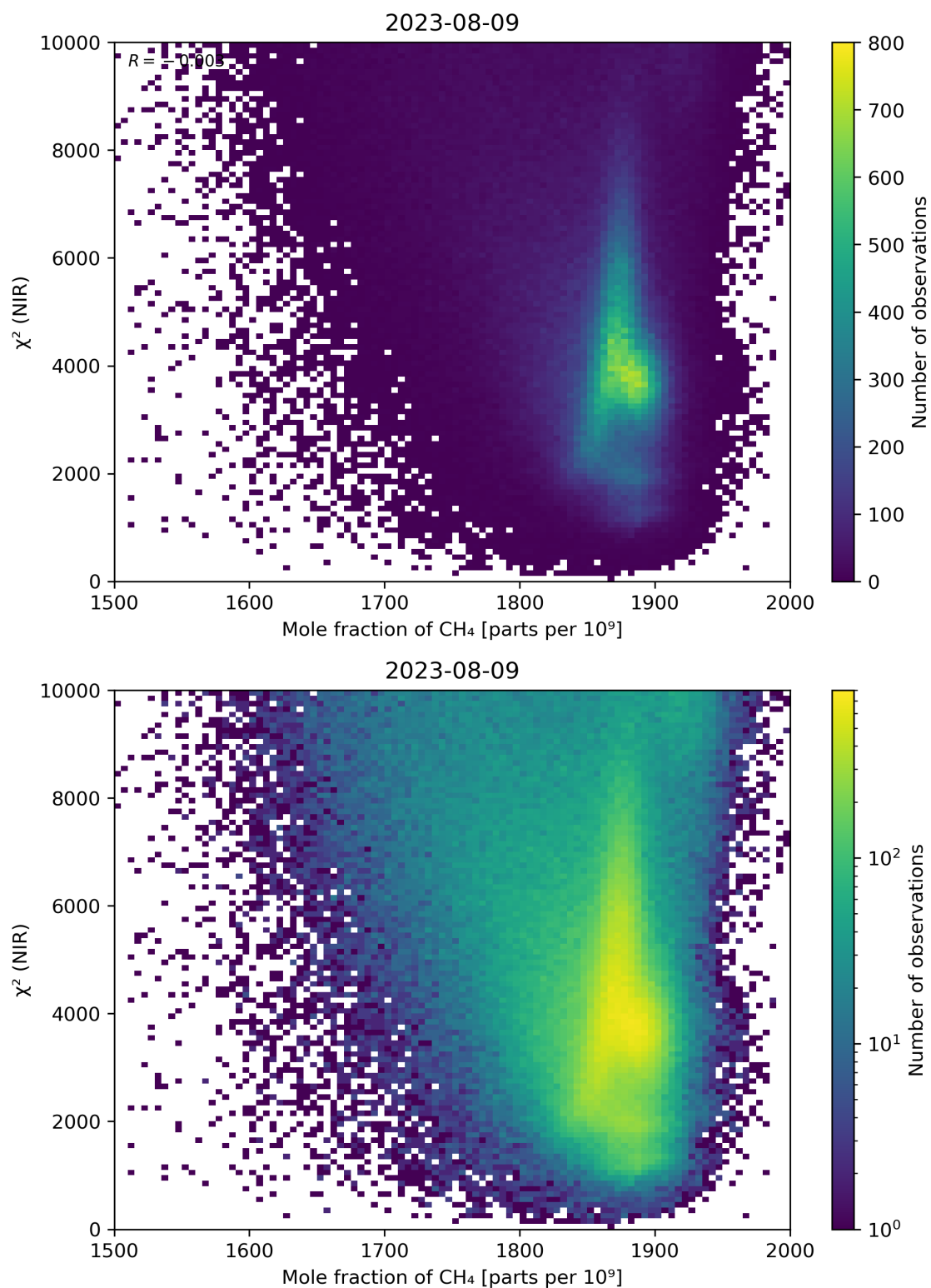
Figure 70: Scatter density plot of “Mole fraction of \text{CH}_4 ” against “ \chi^2 (NIR)” for 2023-08-09 to 2023-08-10.
