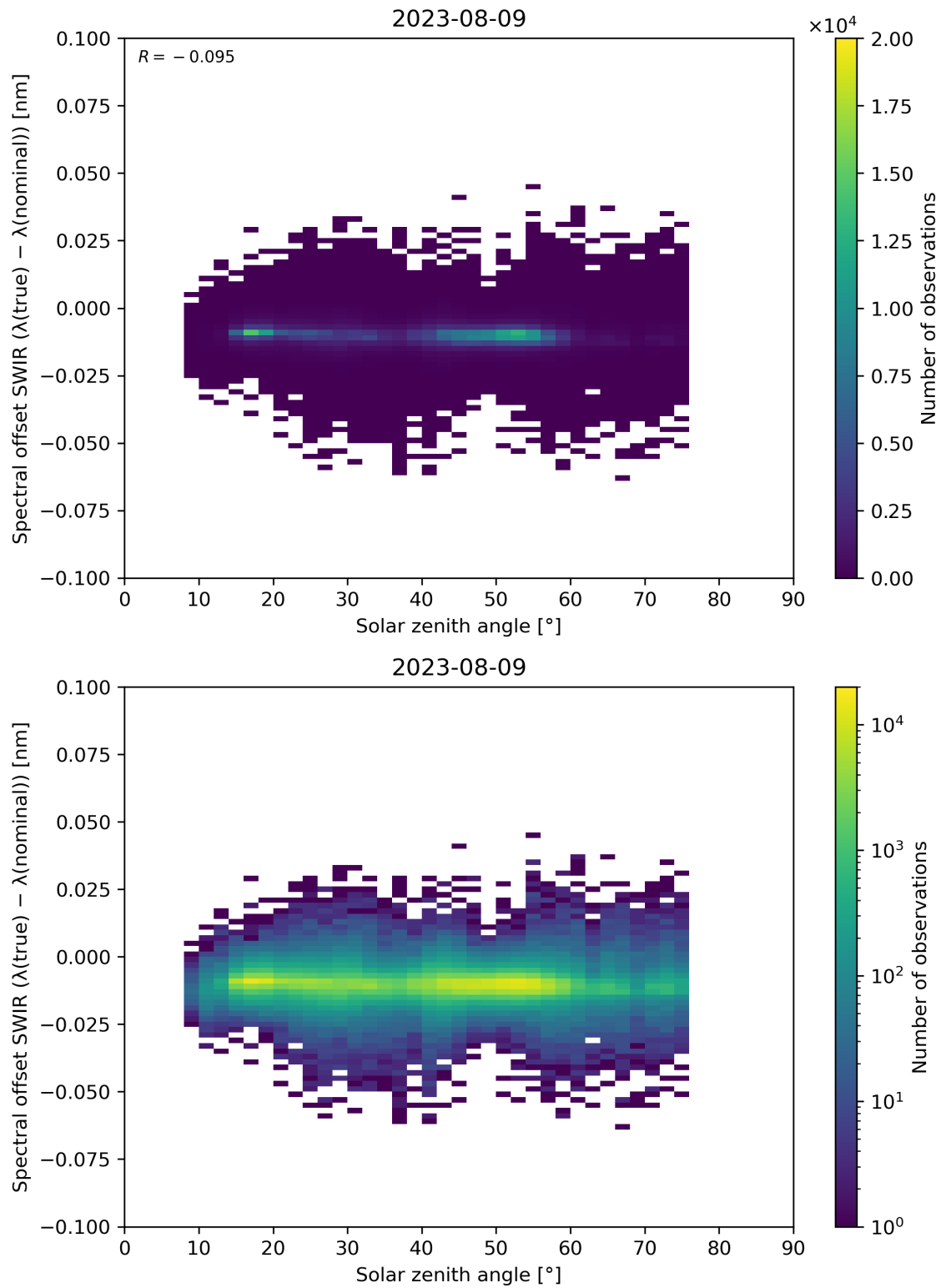
Figure 104: Scatter density plot of “Solar zenith angle” against “Spectral offset SWIR ( \lambda(\text{true}) - \lambda(\text{nominal}) )” for 2023-08-09 to 2023-08-10.
