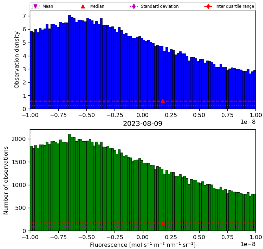
Figure 32: Histogram of “Fluorescence” for 2023-08-09 to 2023-08-10
