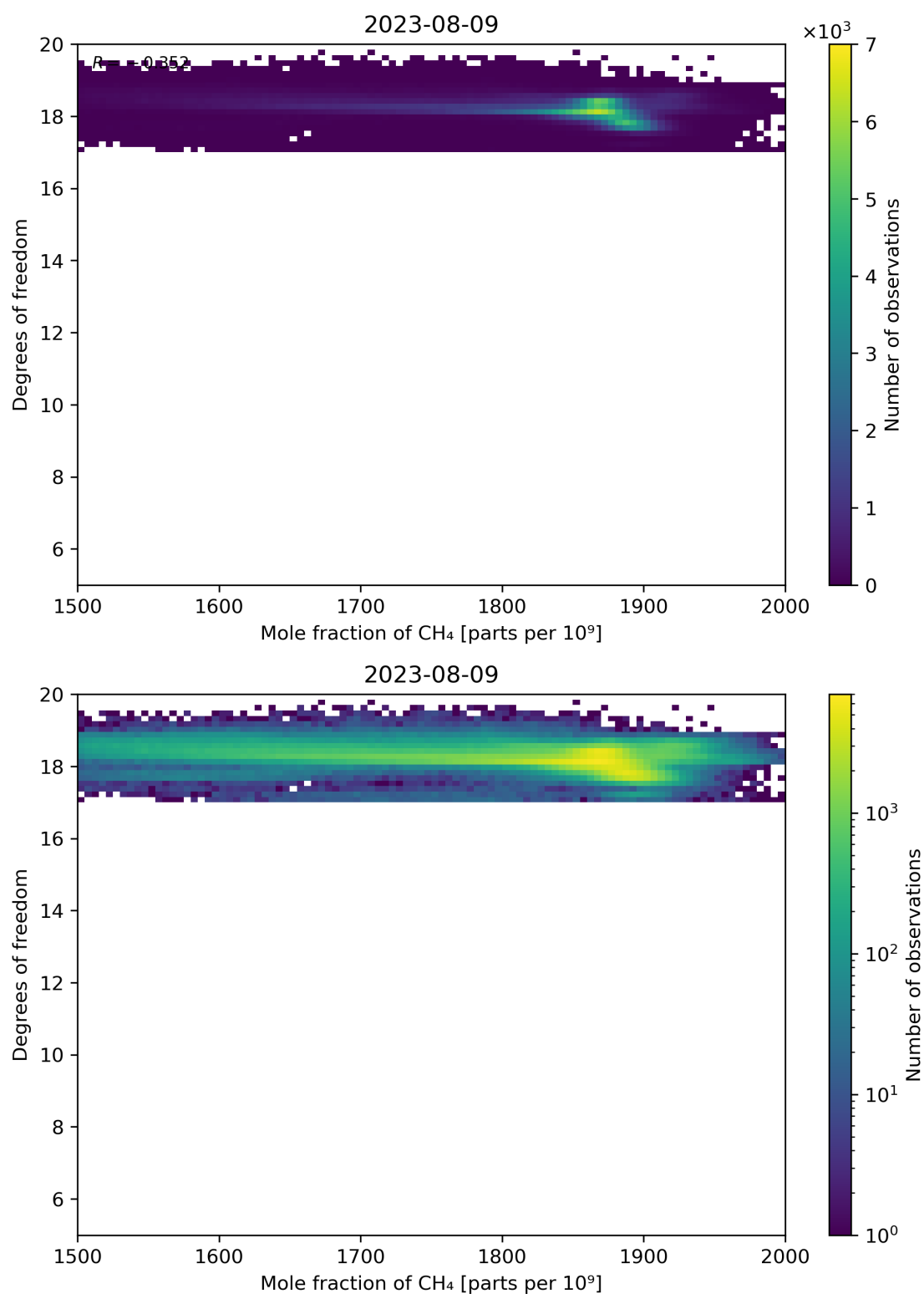
Figure 72: Scatter density plot of “Mole fraction of CH 4 ” against “Degrees of freedom” for 2023-08-09 to 2023-08-10.
