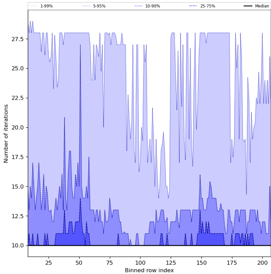
Figure 42: Along track statistics of “Number of iterations” for 2023-08-09 to 2023-08-10
