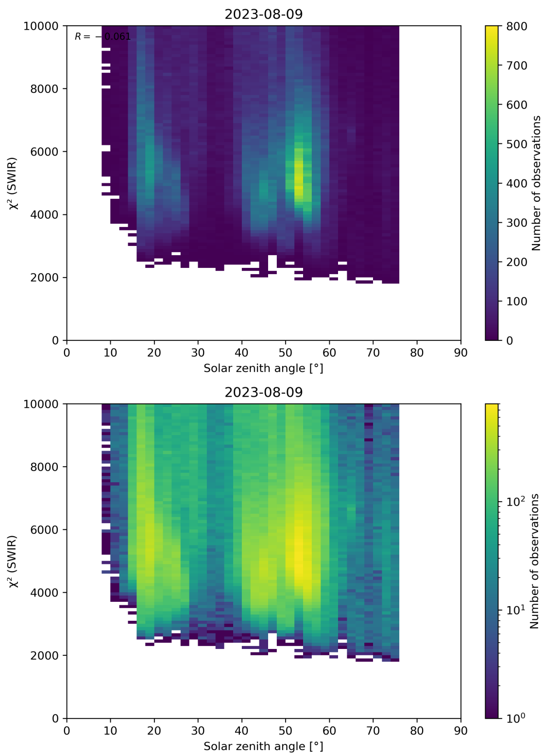
Figure 95: Scatter density plot of “Solar zenith angle” against “ \chi^2 (SWIR)” for 2023-08-09 to 2023-08-10.
