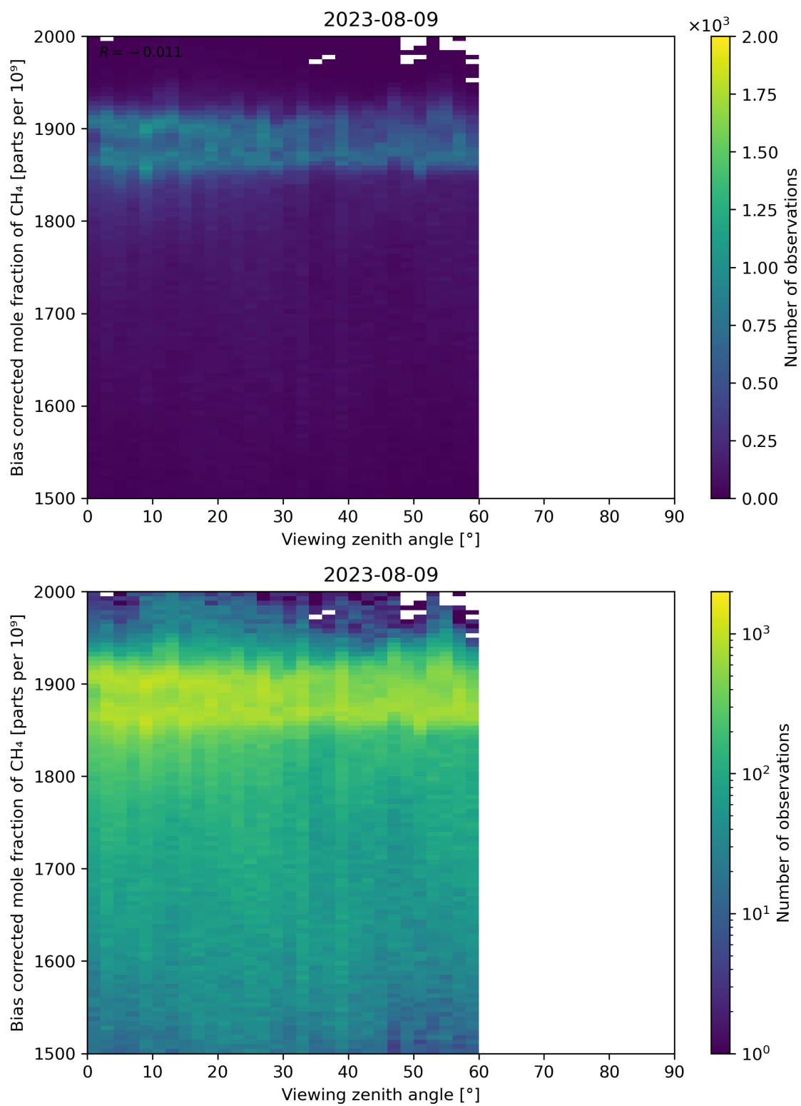
Figure 111: Scatter density plot of “Viewing zenith angle” against “Bias corrected mole fraction of CH 4 ” for 2023-08-09 to 2023-08-10.
