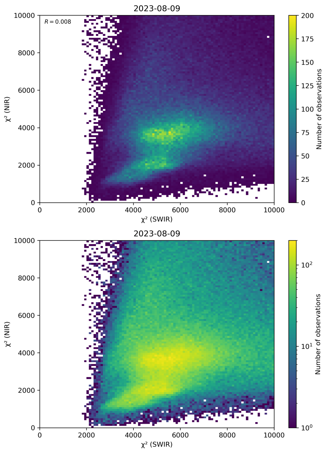
Figure 47: Scatter density plot of “ \chi^2 (SWIR)” against “ \chi^2 (NIR)” for 2023-08-09 to 2023-08-10.
