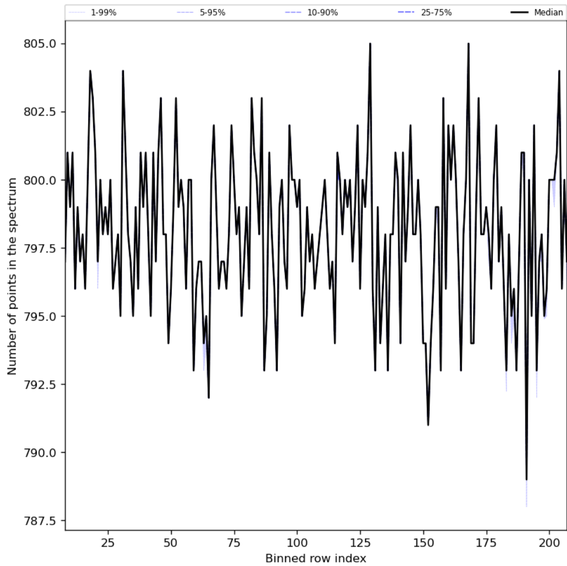
Figure 37: Along track statistics of “Number of points in the spectrum” for 2023-08-09 to 2023-08-10
