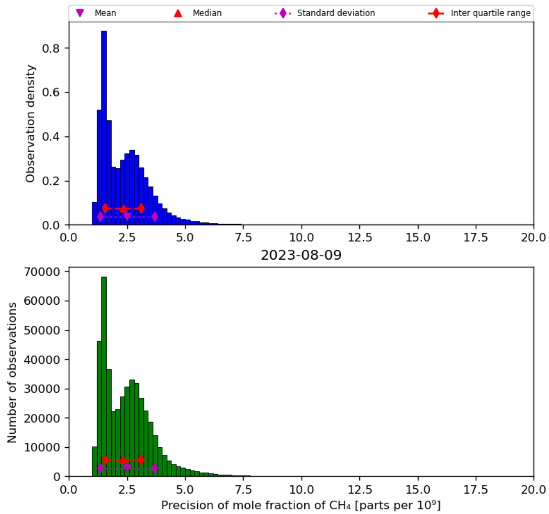
Figure 24: Histogram of “Precision of mole fraction of CH 4 ” for 2023-08-09 to 2023-08-10
