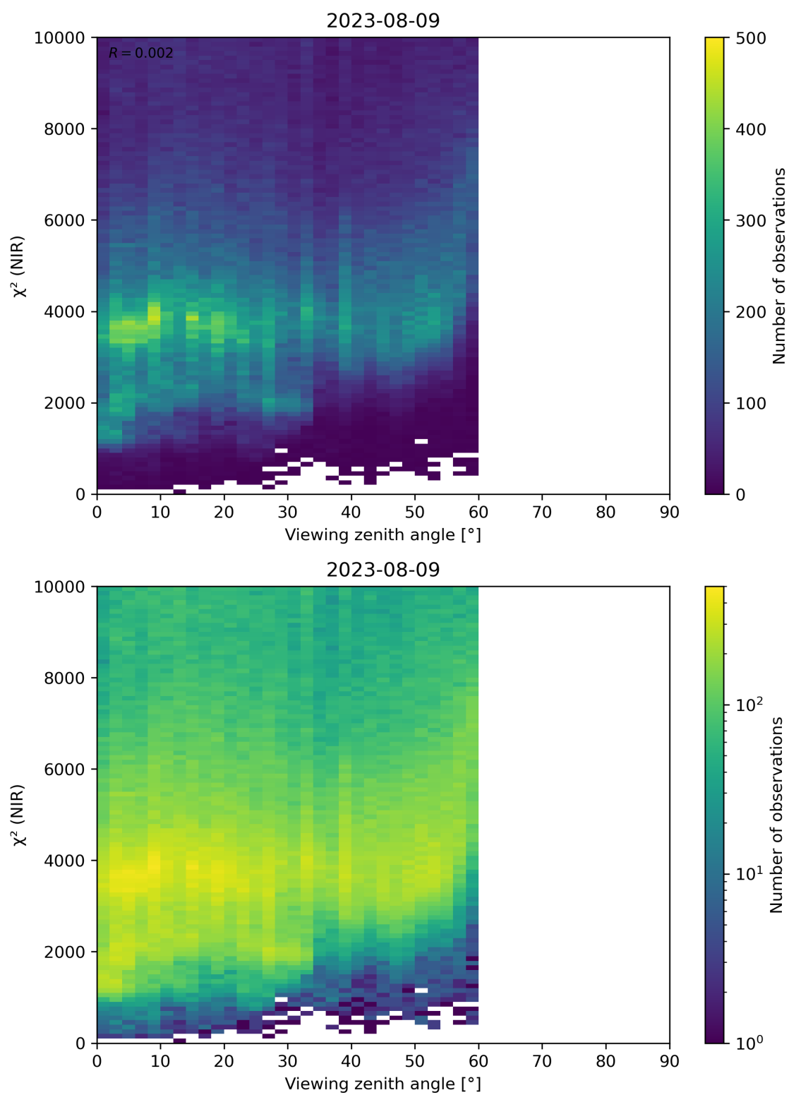
Figure 105: Scatter density plot of “Viewing zenith angle” against “ \chi^2 (NIR)” for 2023-08-09 to 2023-08-10.
