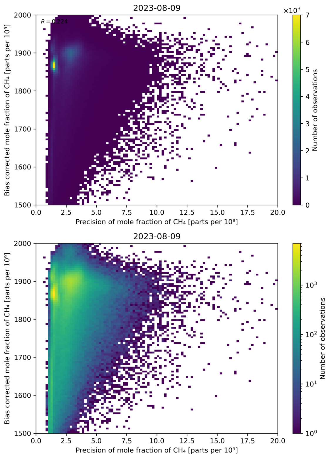
Figure 82: Scatter density plot of “Precision of mole fraction of \text{CH}_4 ” against “Bias corrected mole fraction of \text{CH}_4 ” for 2023-08-09 to 2023-08-10.
