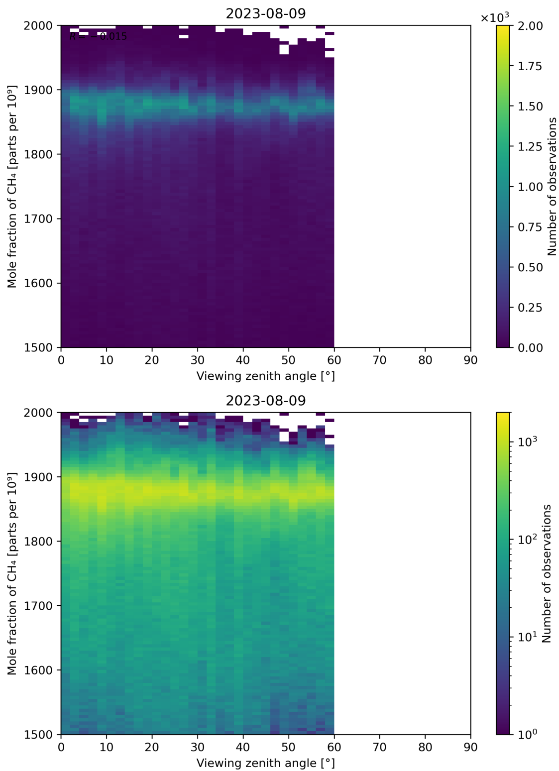
Figure 110: Scatter density plot of “Viewing zenith angle” against “Mole fraction of CH 4 ” for 2023-08-09 to 2023-08-10.
