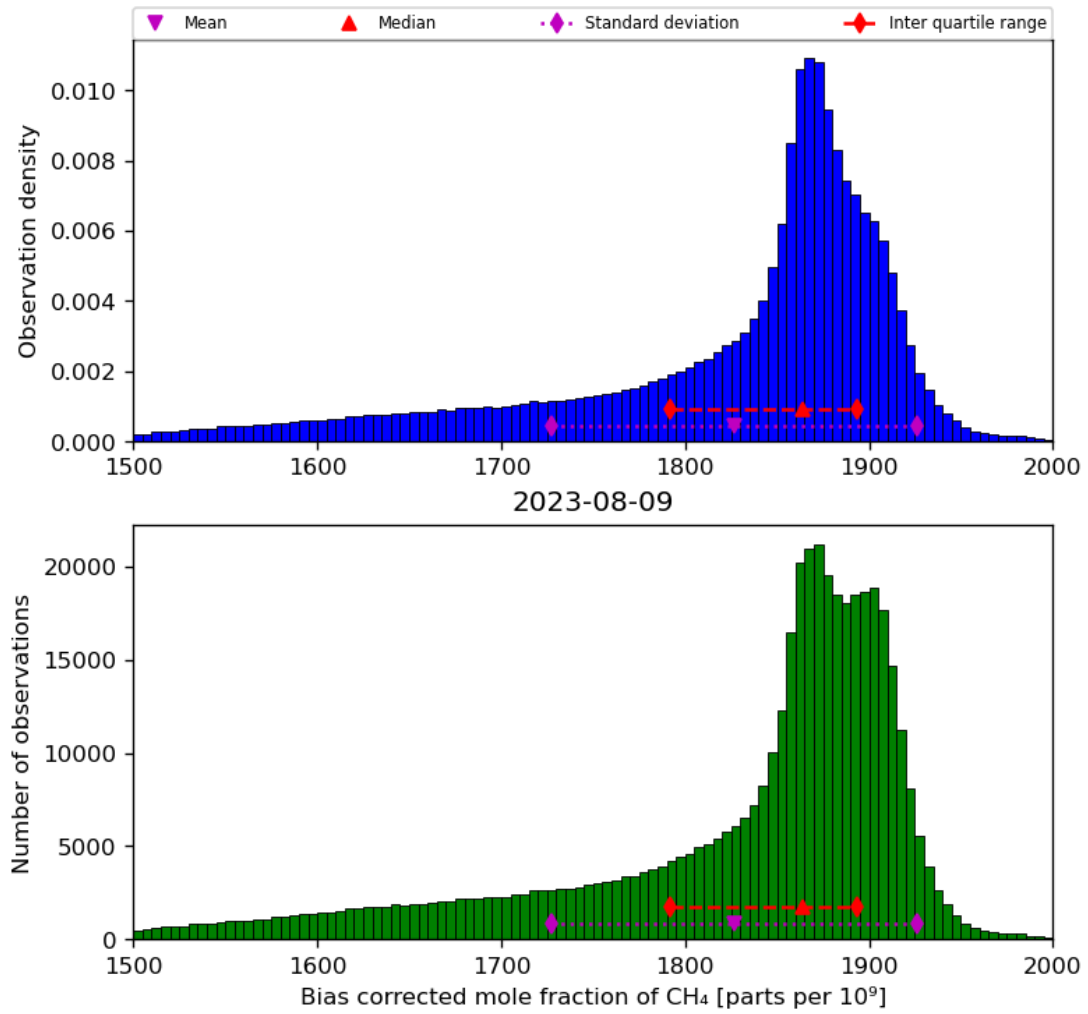
Figure 25: Histogram of “Bias corrected mole fraction of CH 4 ” for 2023-08-09 to 2023-08-10
