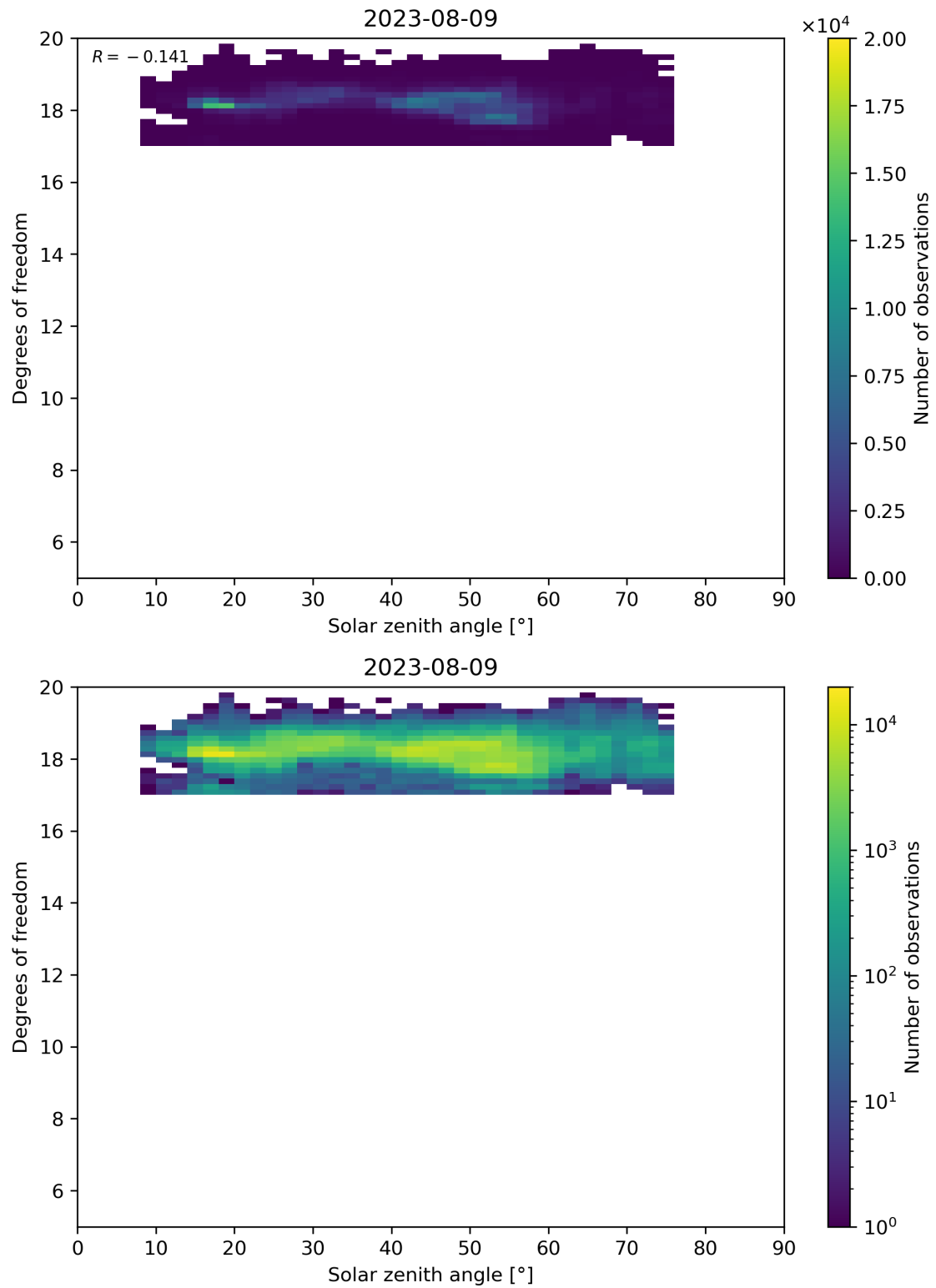
Figure 96: Scatter density plot of “Solar zenith angle” against “Degrees of freedom” for 2023-08-09 to 2023-08-10.
