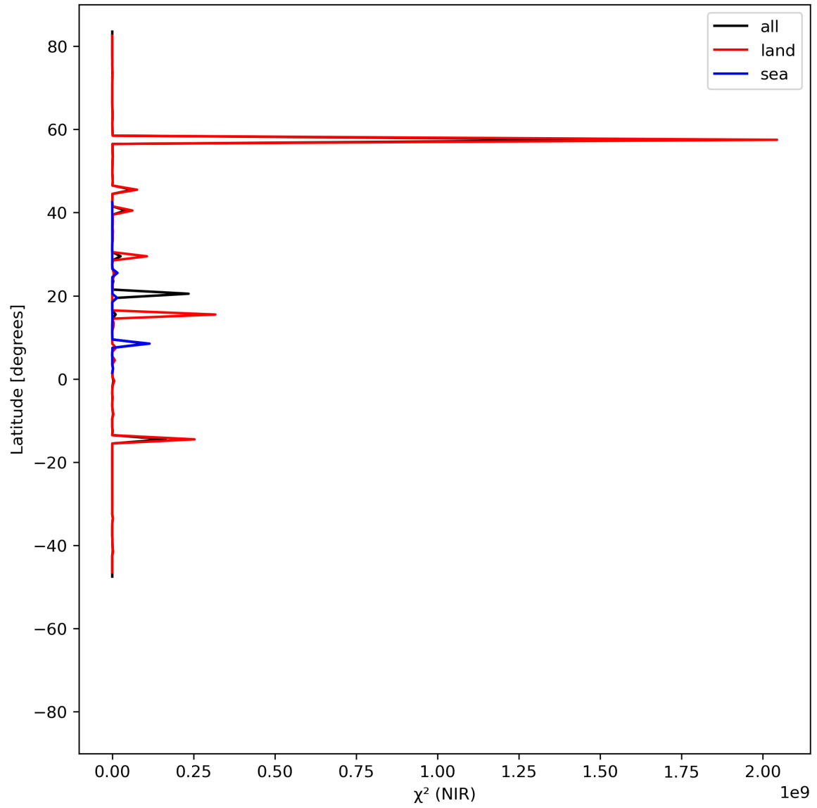
Figure 18: Zonal average of “ \chi^2 (NIR)” for 2023-08-09 to 2023-08-10.
