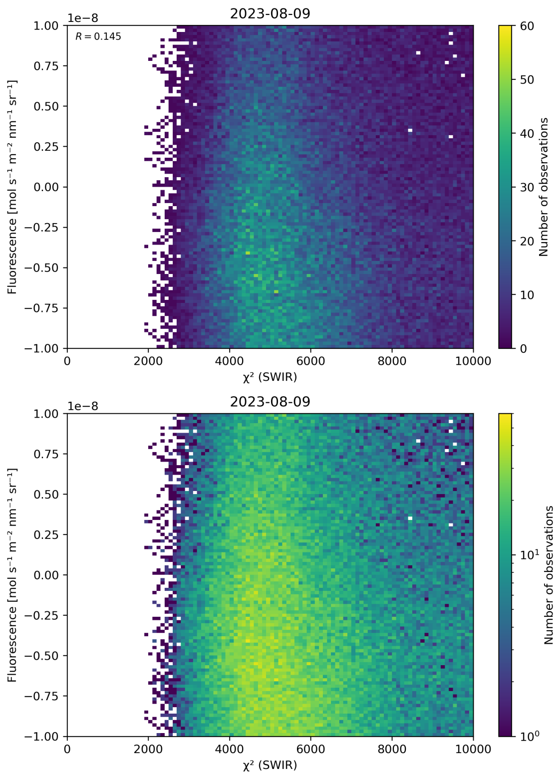
Figure 49: Scatter density plot of “ \chi^2 (SWIR)” against “Fluorescence” for 2023-08-09 to 2023-08-10.
