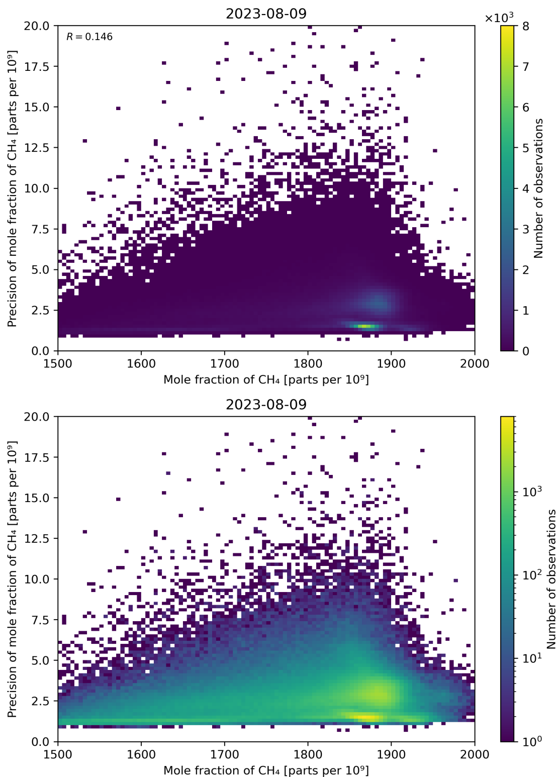
Figure 75: Scatter density plot of “Mole fraction of CH 4 ” against “Precision of mole fraction of CH 4 ” for 2023-08-09 to 2023-08-10.
