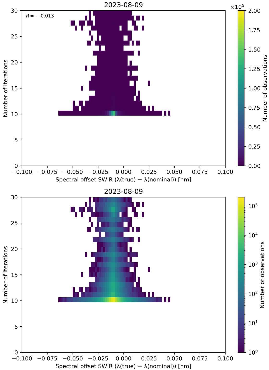
Figure 121: Scatter density plot of “Spectral offset SWIR ( \lambda(\text{true}) - \lambda(\text{nominal}) )” against “Number of iterations” for 2023-08-09 to 2023-08-10.
