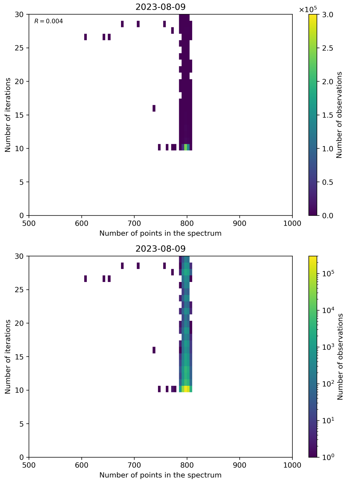
Figure 92: Scatter density plot of “Number of points in the spectrum” against “Number of iterations” for 2023-08-09 to 2023-08-10.
