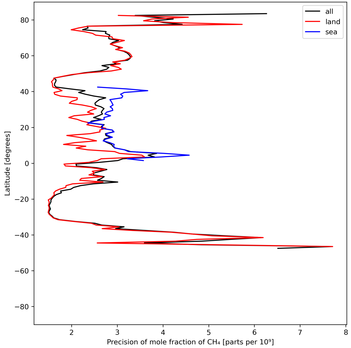
Figure 13: Zonal average of “Precision of mole fraction of CH 4 ” for 2023-08-09 to 2023-08-10.
