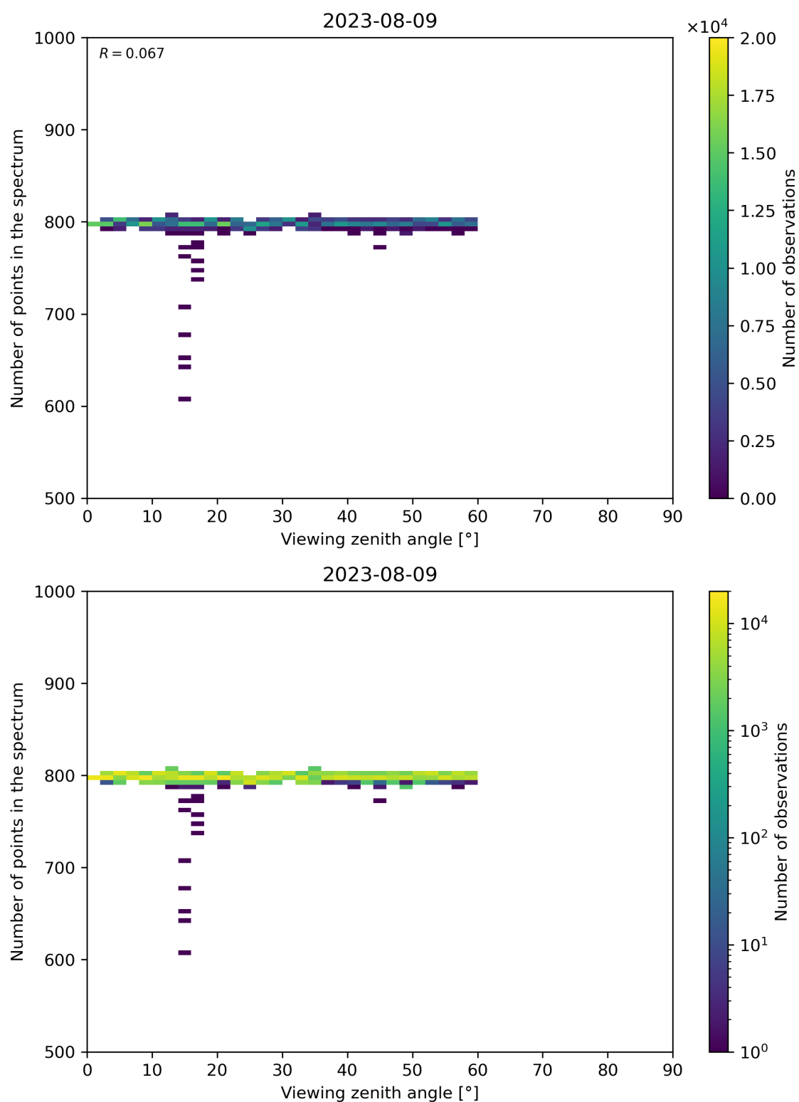
Figure 114: Scatter density plot of “Viewing zenith angle” against “Number of points in the spectrum” for 2023-08-09 to 2023-08-10.
