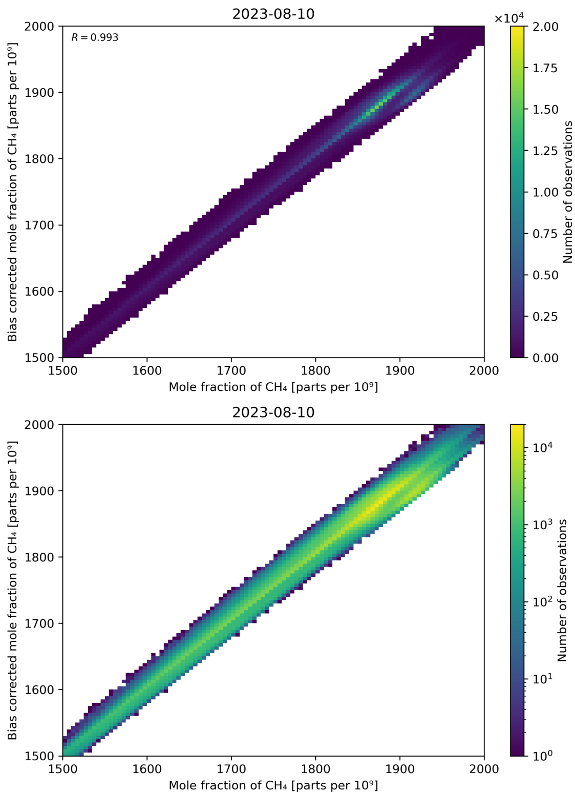
Figure 74: Scatter density plot of “Mole fraction of CH 4 ” against “Bias corrected mole fraction of CH 4 ” for 2023-08-09 to 2023-08-11.
