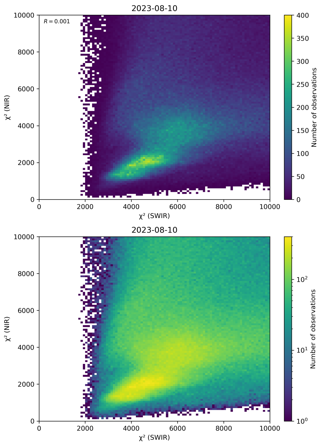
Figure 47: Scatter density plot of “ \chi^2 (SWIR)” against “ \chi^2 (NIR)” for 2023-08-09 to 2023-08-11.
