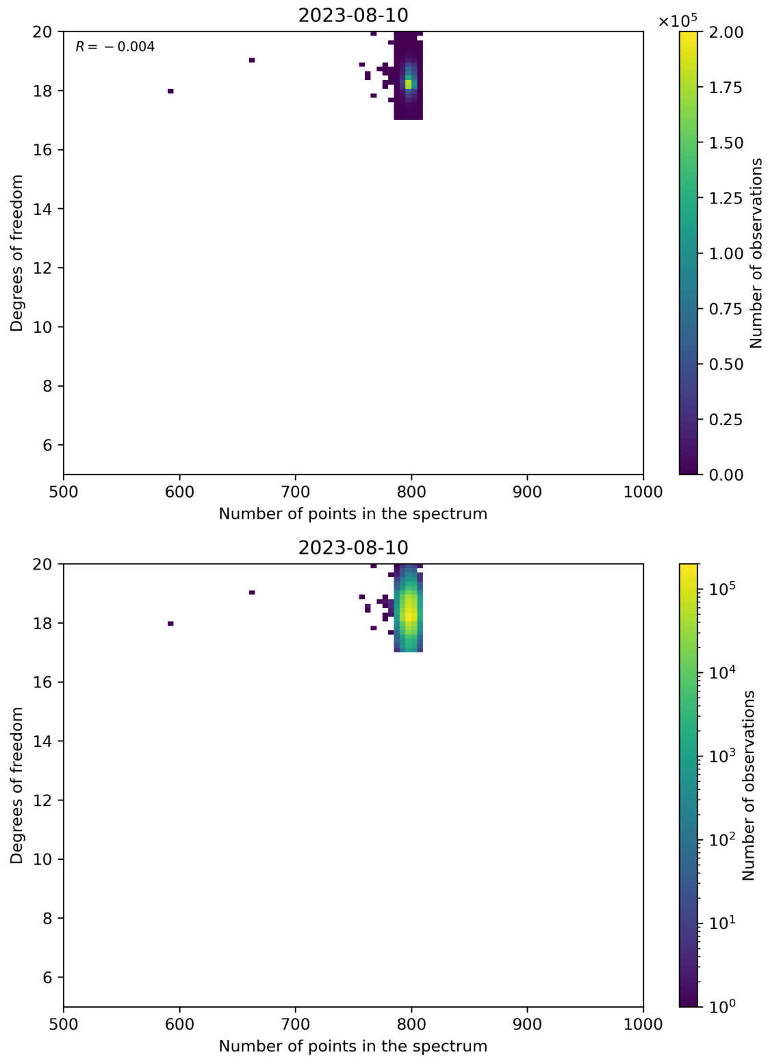
Figure 90: Scatter density plot of “Number of points in the spectrum” against “Degrees of freedom” for 2023-08-09 to 2023-08-11.
