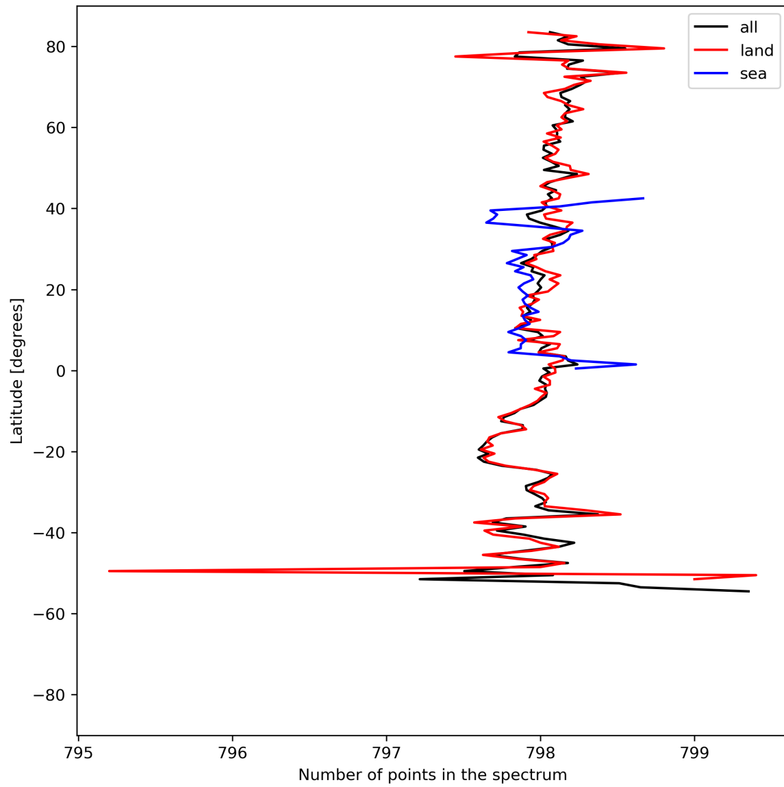
Figure 15: Zonal average of “Number of points in the spectrum” for 2023-08-09 to 2023-08-11.
