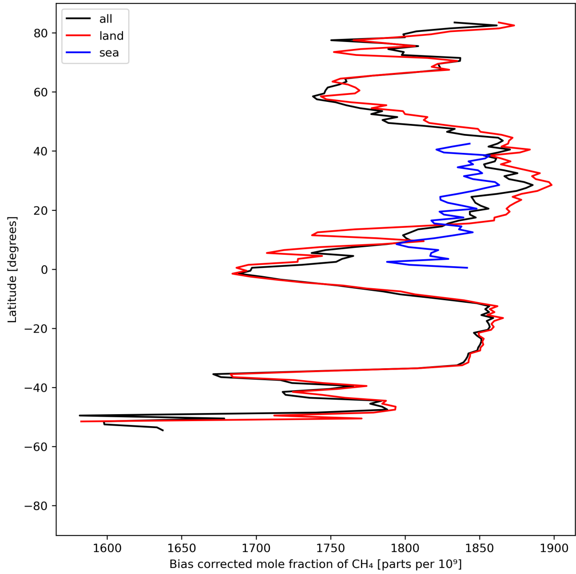
Figure 14: Zonal average of “Bias corrected mole fraction of \text{CH}_4 ” for 2023-08-09 to 2023-08-11.
