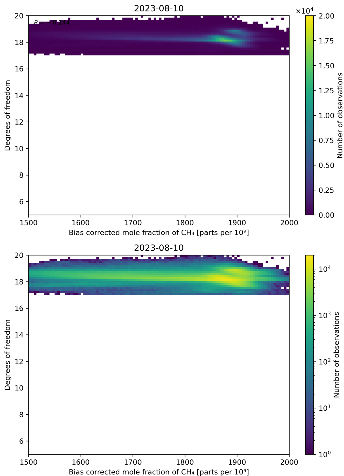
Figure 65: Scatter density plot of “Bias corrected mole fraction of CH 4 ” against “Degrees of freedom” for 2023-08-09 to 2023-08-11.
