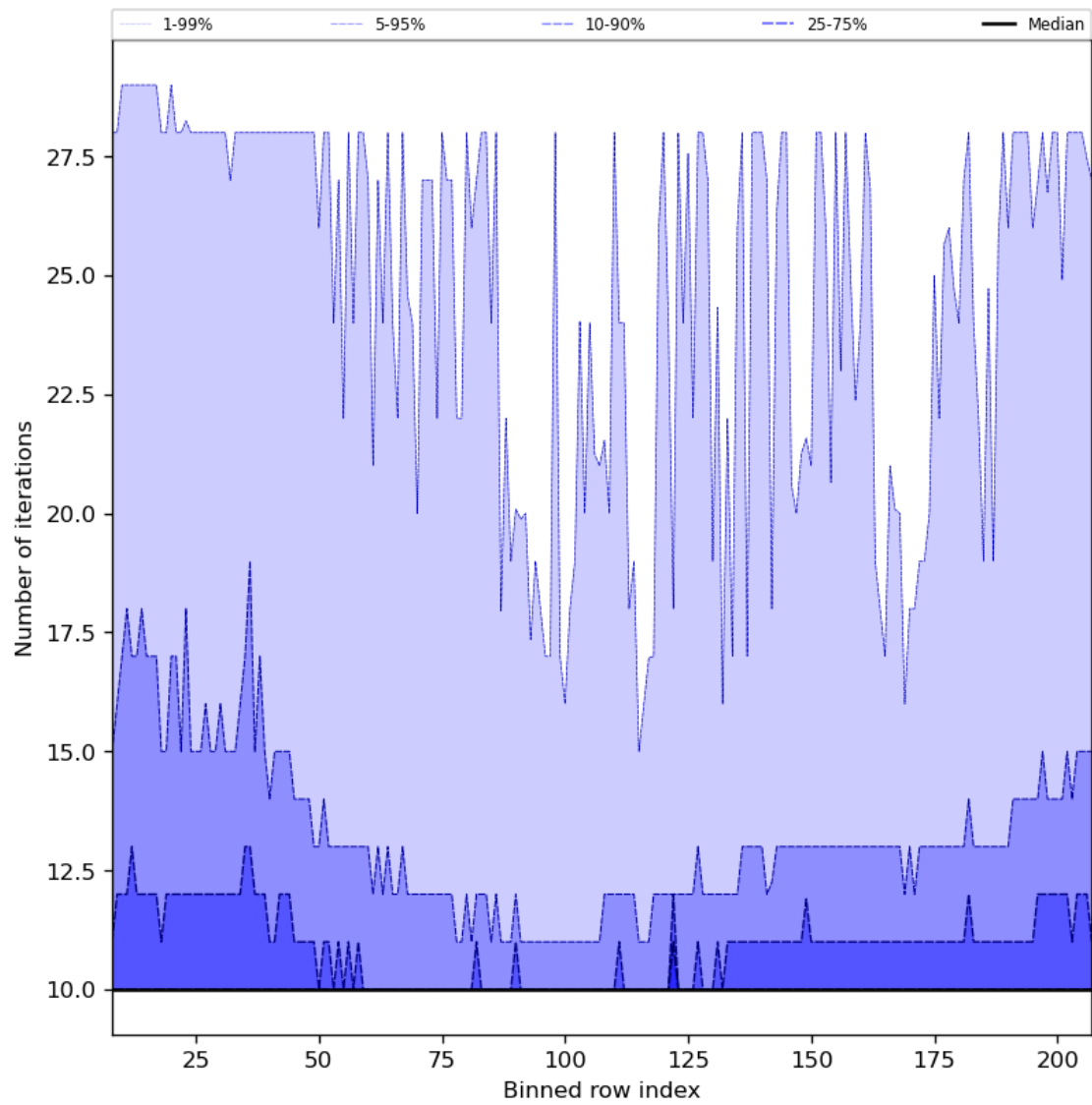
Figure 42: Along track statistics of “Number of iterations” for 2023-08-09 to 2023-08-11
