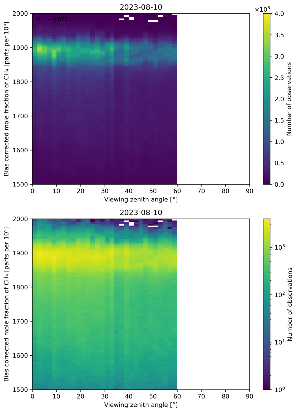
Figure 111: Scatter density plot of “Viewing zenith angle” against “Bias corrected mole fraction of CH 4 ” for 2023-08-09 to 2023-08-11.
