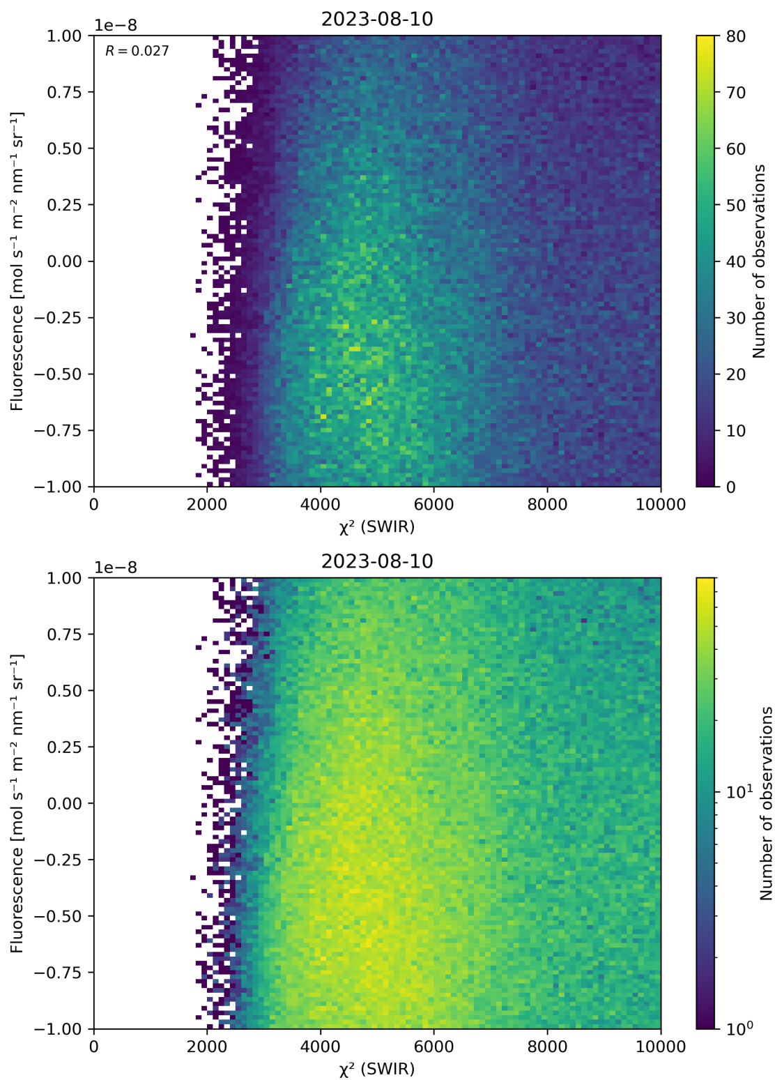
Figure 49: Scatter density plot of “ \chi^2 (SWIR)” against “Fluorescence” for 2023-08-09 to 2023-08-11.
