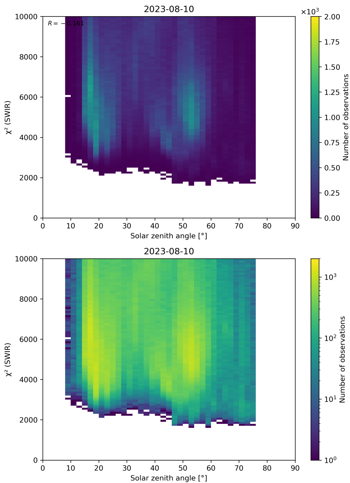
Figure 95: Scatter density plot of “Solar zenith angle” against “ \chi^2 (SWIR)” for 2023-08-09 to 2023-08-11.
