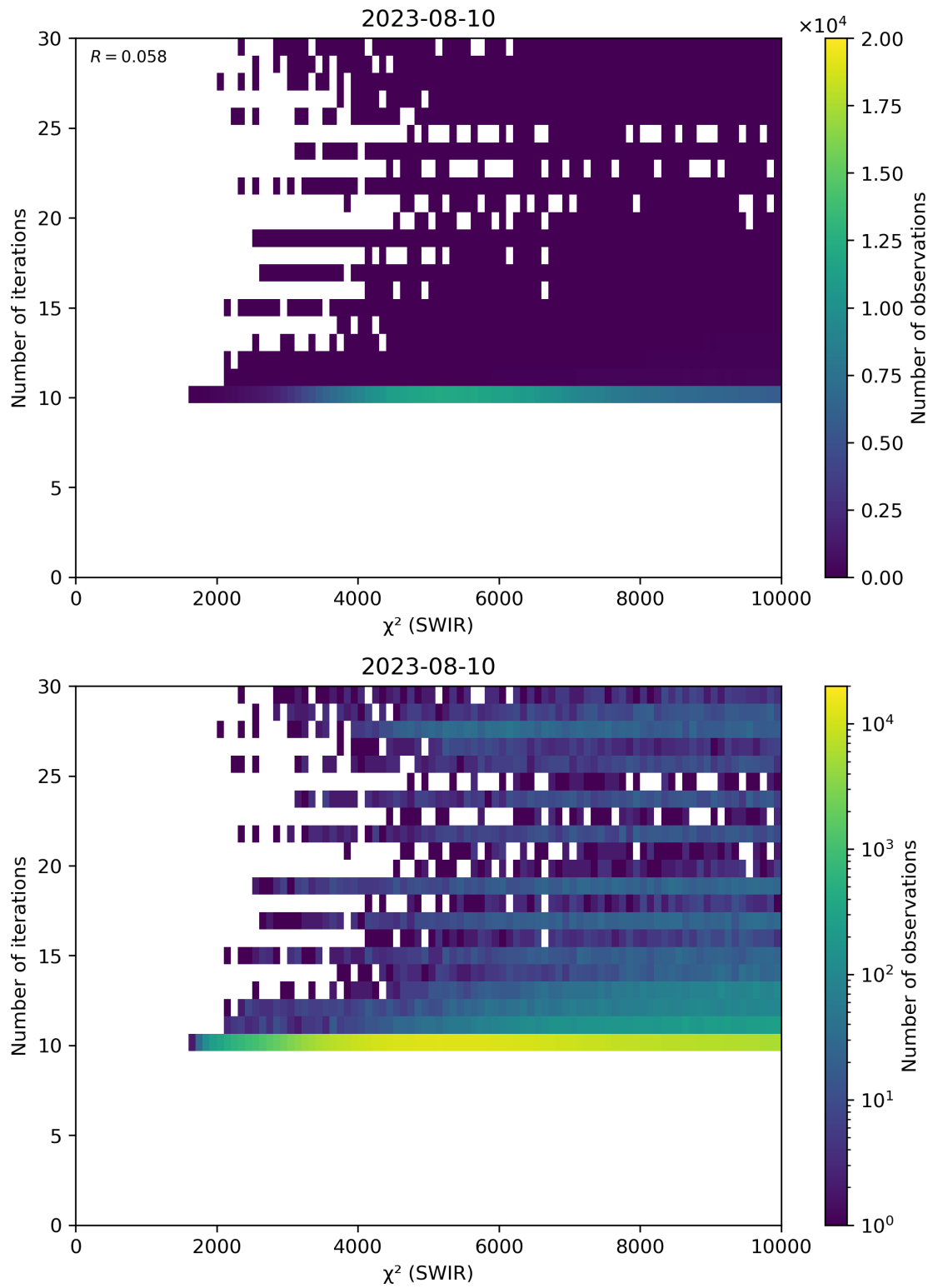
Figure 50: Scatter density plot of “ \chi^2 (SWIR)” against “Number of iterations” for 2023-08-09 to 2023-08-11.
