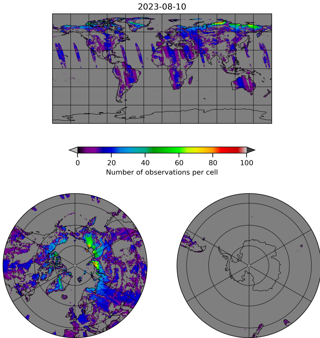
Figure 10: Map of the number of observations for 2023-08-09 to 2023-08-11
