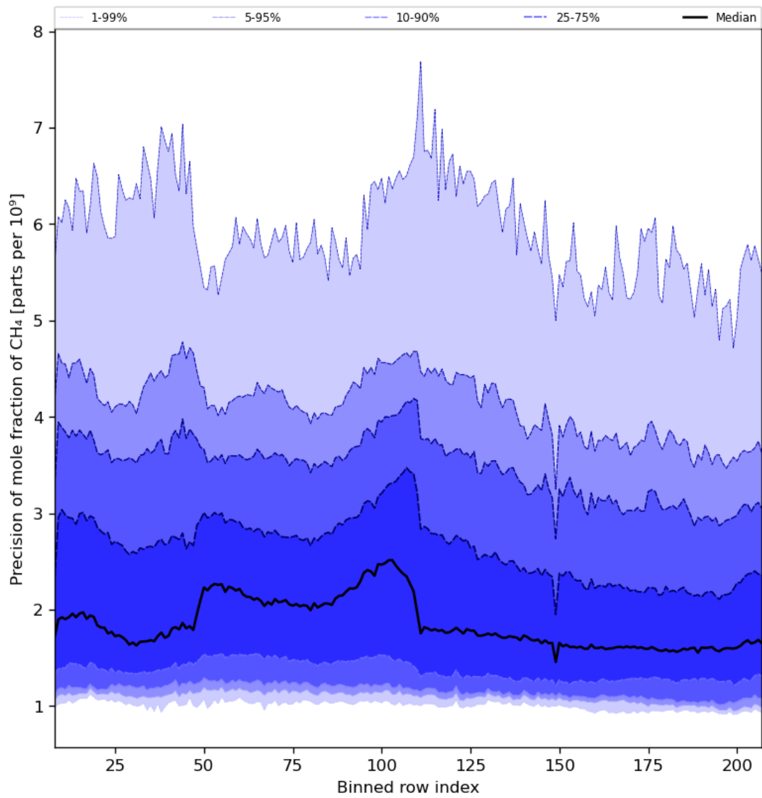
Figure 35: Along track statistics of “Precision of mole fraction of CH 4 ” for 2023-08-09 to 2023-08-11
