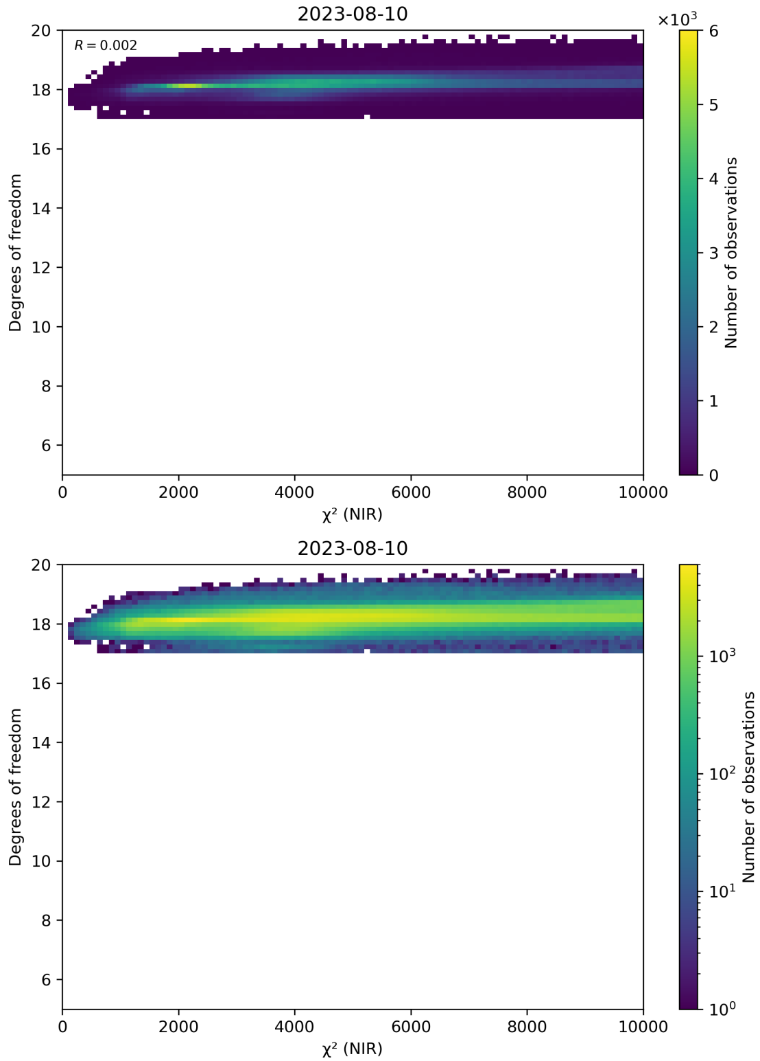
Figure 44: Scatter density plot of “ \chi^2 (NIR)” against “Degrees of freedom” for 2023-08-09 to 2023-08-11.
