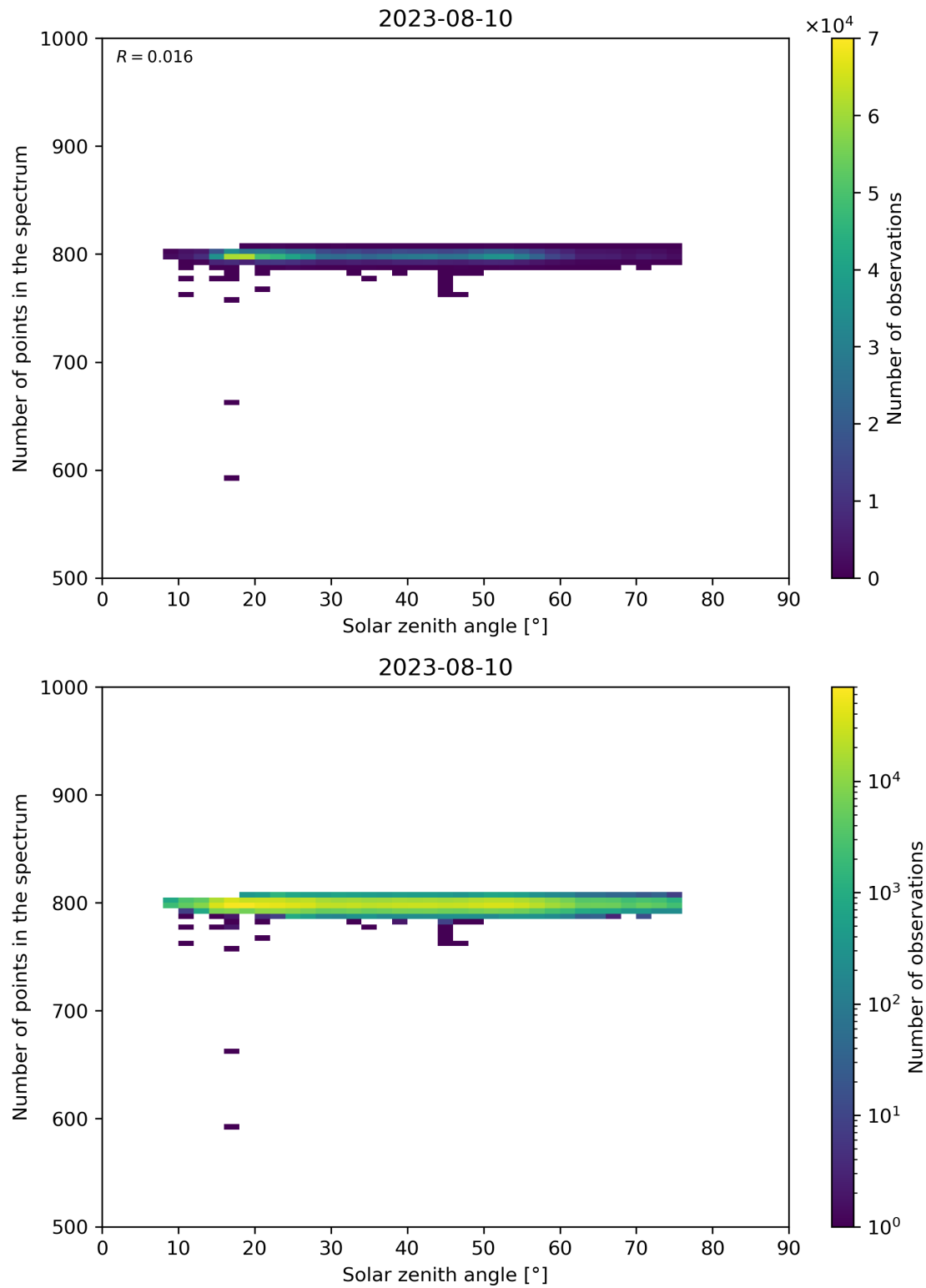
Figure 103: Scatter density plot of “Solar zenith angle” against “Number of points in the spectrum” for 2023-08-09 to 2023-08-11.
