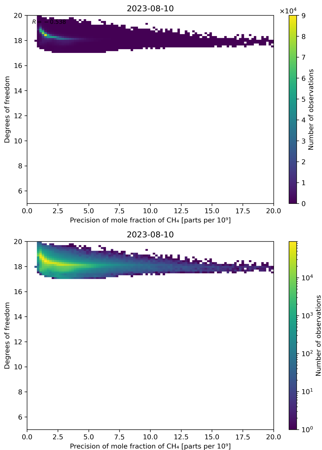
Figure 80: Scatter density plot of “Precision of mole fraction of CH 4 ” against “Degrees of freedom” for 2023-08-09 to 2023-08-11.
