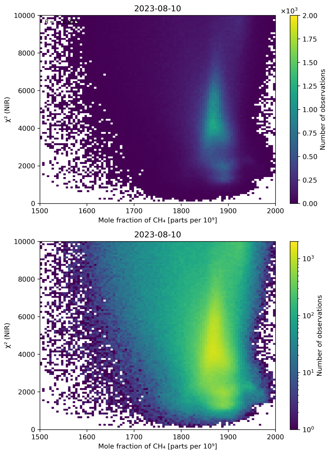
Figure 70: Scatter density plot of “Mole fraction of \text{CH}_4 ” against “ \chi^2 (NIR)” for 2023-08-09 to 2023-08-11.
