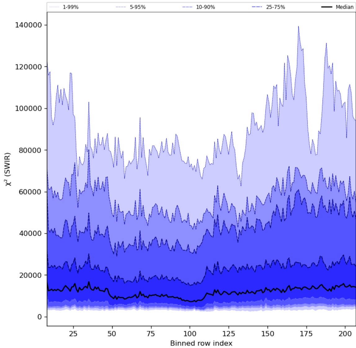
Figure 39: Along track statistics of " \chi^2 (SWIR)" for 2023-08-09 to 2023-08-11
