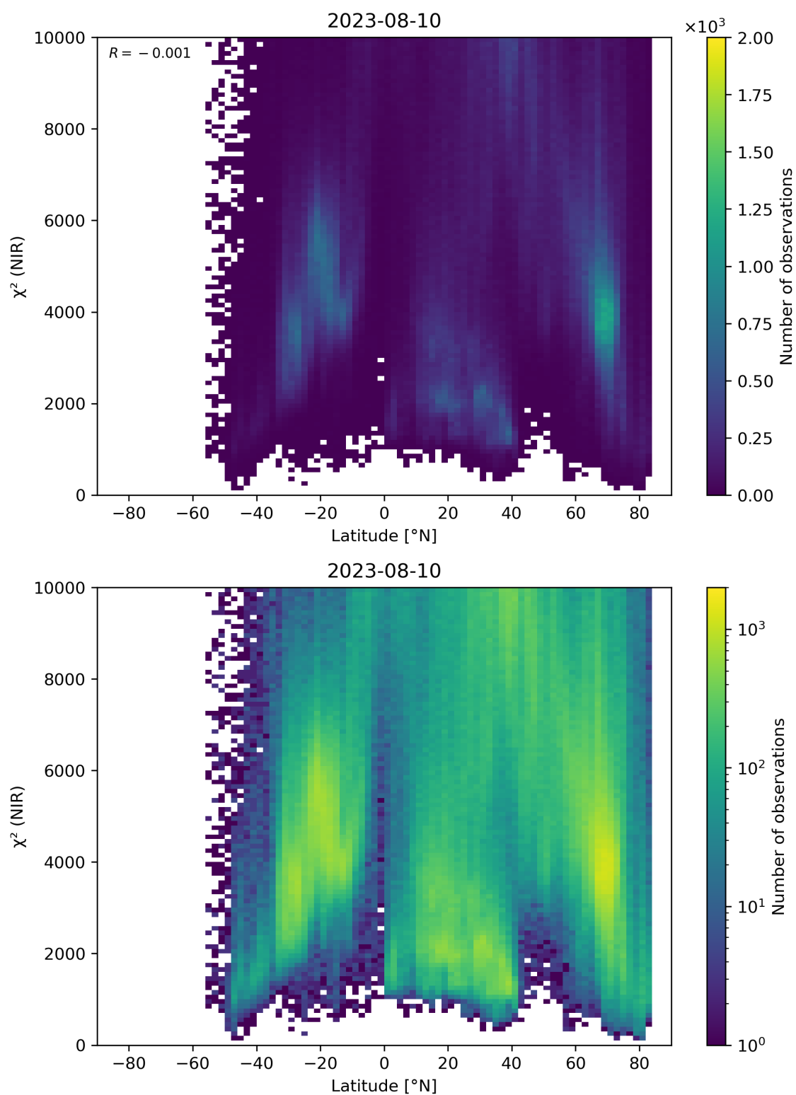
Figure 53: Scatter density plot of “Latitude” against “ \chi^2 (NIR)” for 2023-08-09 to 2023-08-11.
