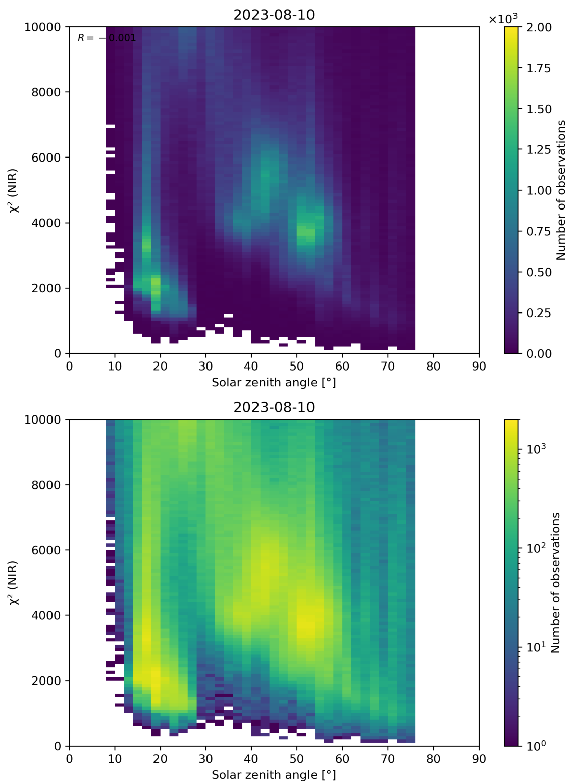
Figure 94: Scatter density plot of “Solar zenith angle” against “ \chi^2 (NIR)” for 2023-08-09 to 2023-08-11.
