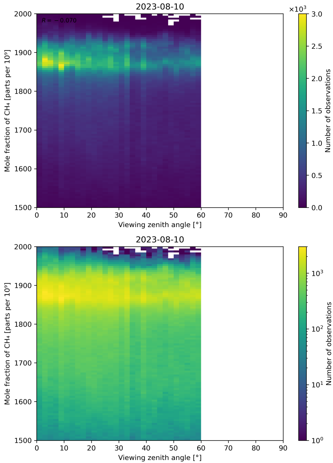
Figure 110: Scatter density plot of “Viewing zenith angle” against “Mole fraction of CH 4 ” for 2023-08-09 to 2023-08-11.
