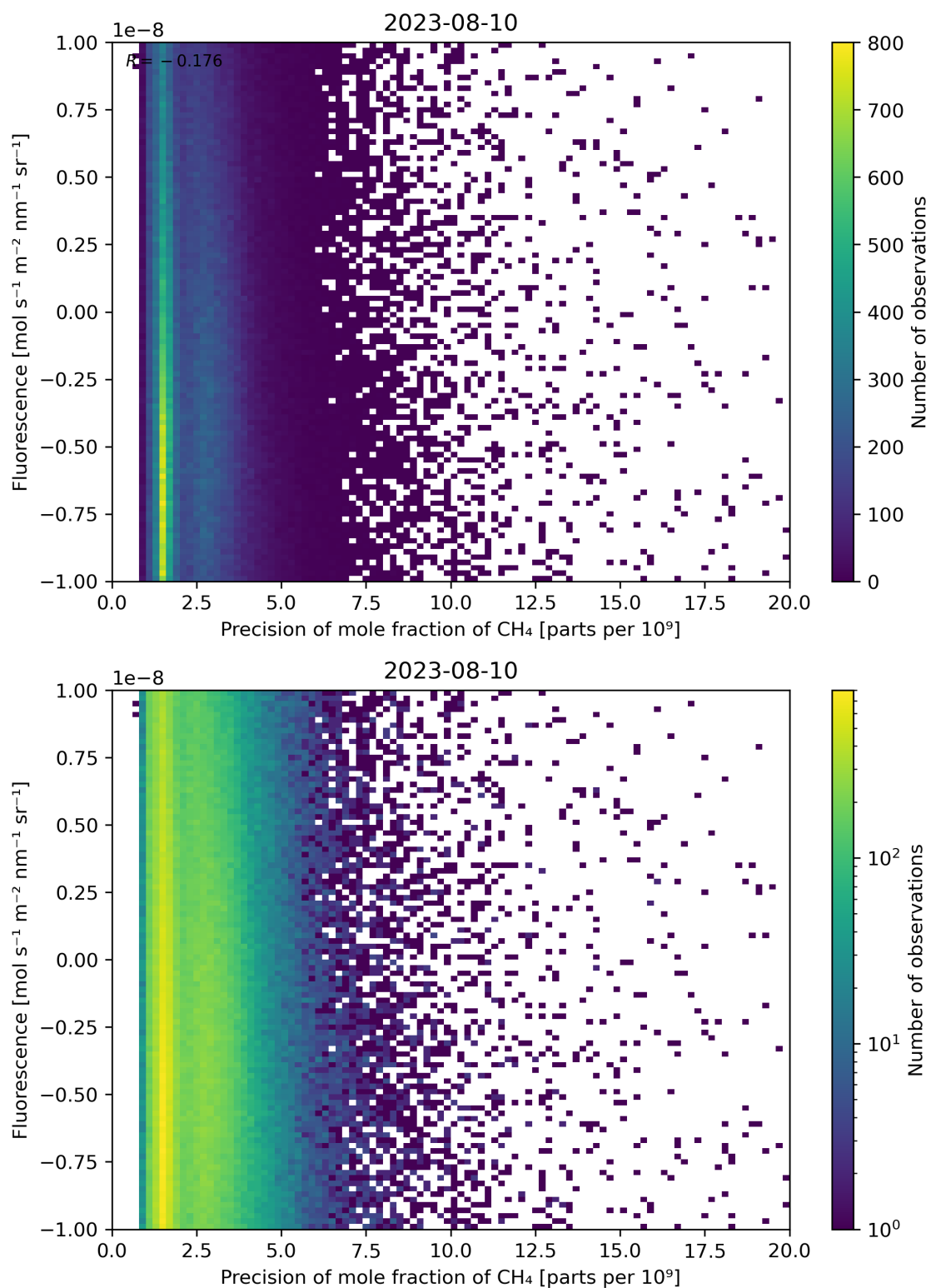
Figure 81: Scatter density plot of “Precision of mole fraction of \text{CH}_4 ” against “Fluorescence” for 2023-08-09 to 2023-08-11.
