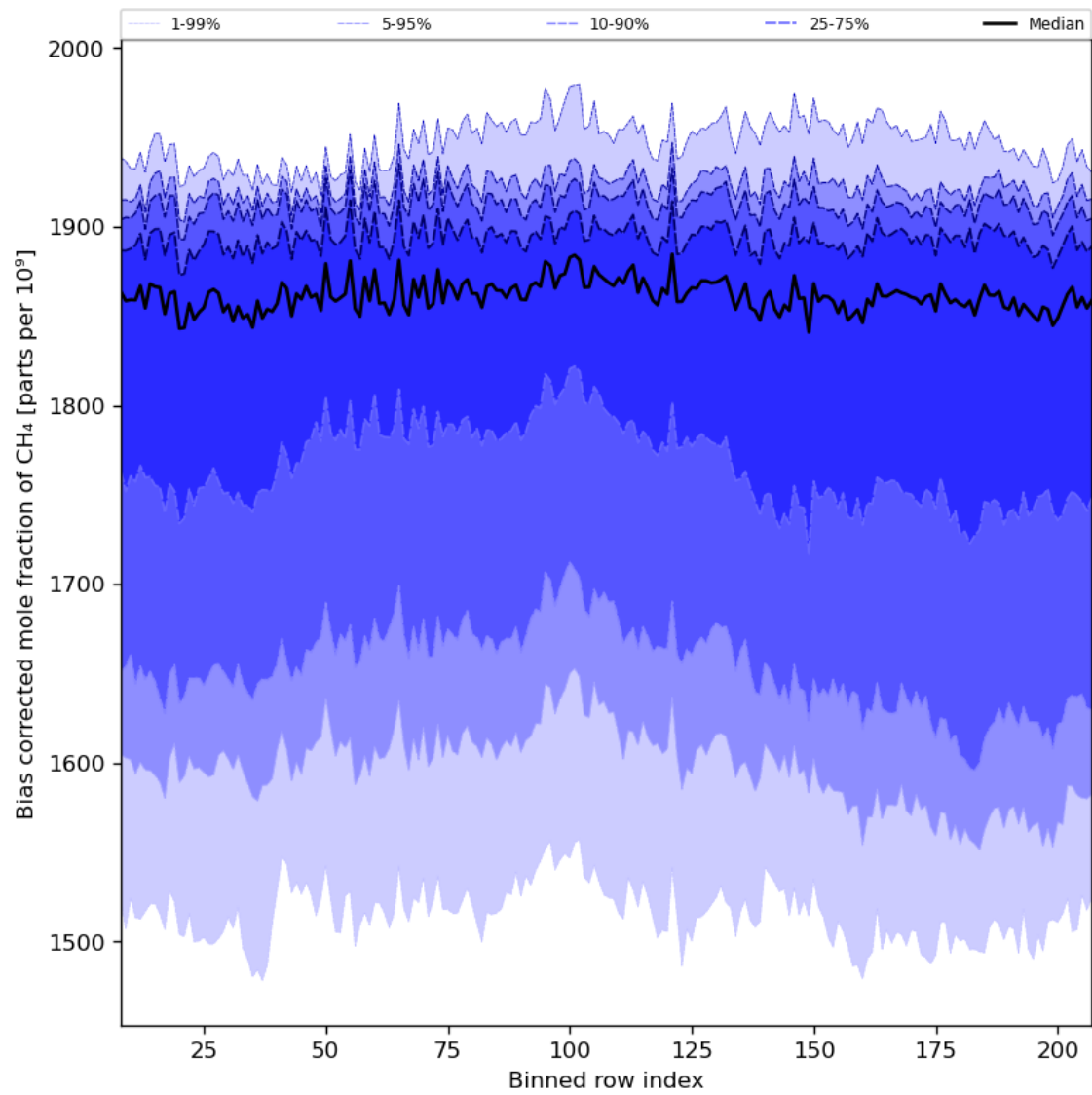
Figure 36: Along track statistics of “Bias corrected mole fraction of CH 4 ” for 2023-08-09 to 2023-08-11
