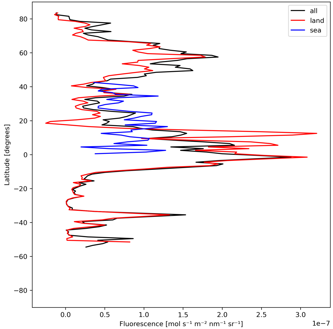
Figure 21: Zonal average of “Fluorescence” for 2023-08-09 to 2023-08-11.
