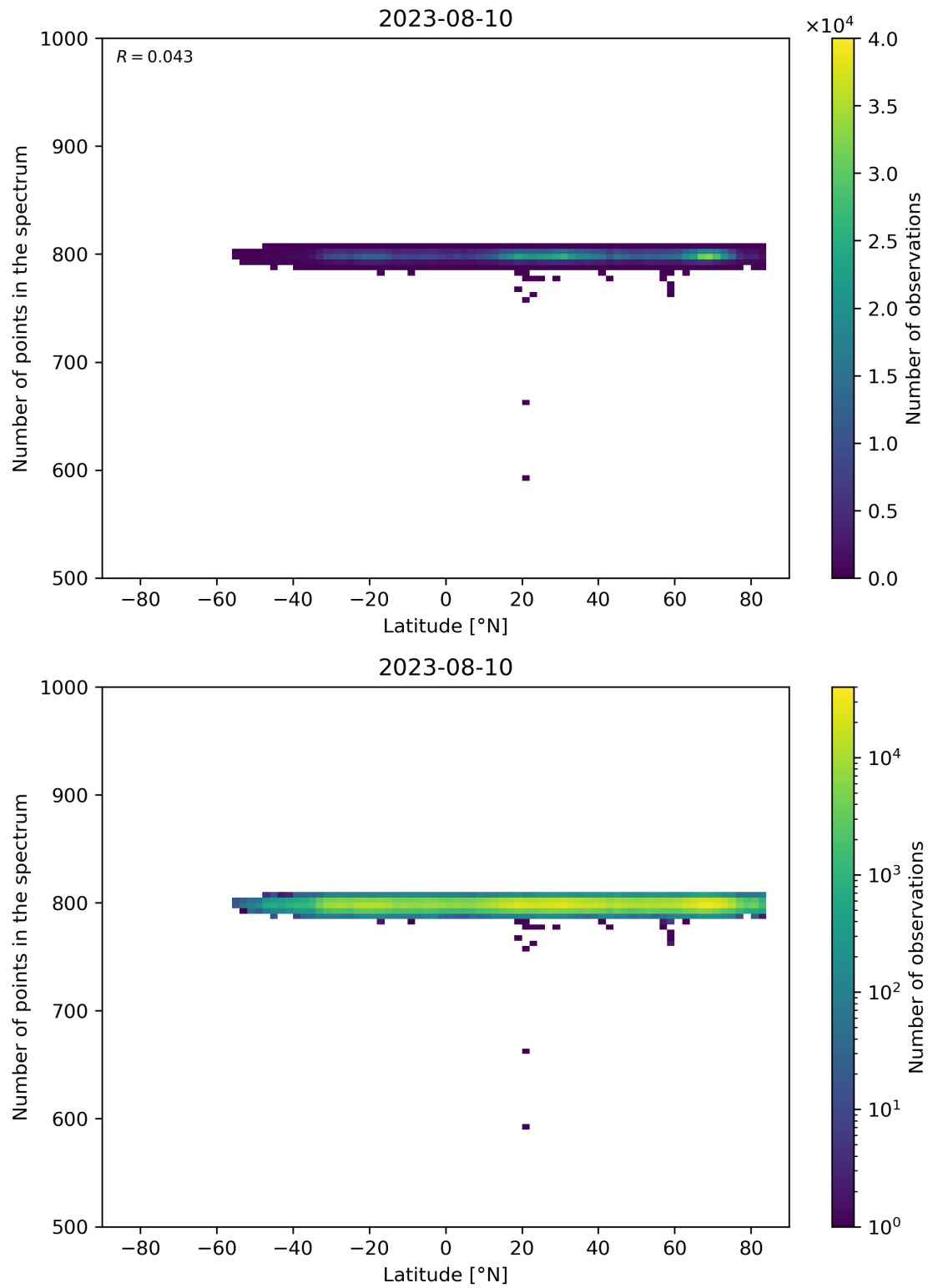
Figure 61: Scatter density plot of “Latitude” against “Number of points in the spectrum” for 2023-08-09 to 2023-08-11.
