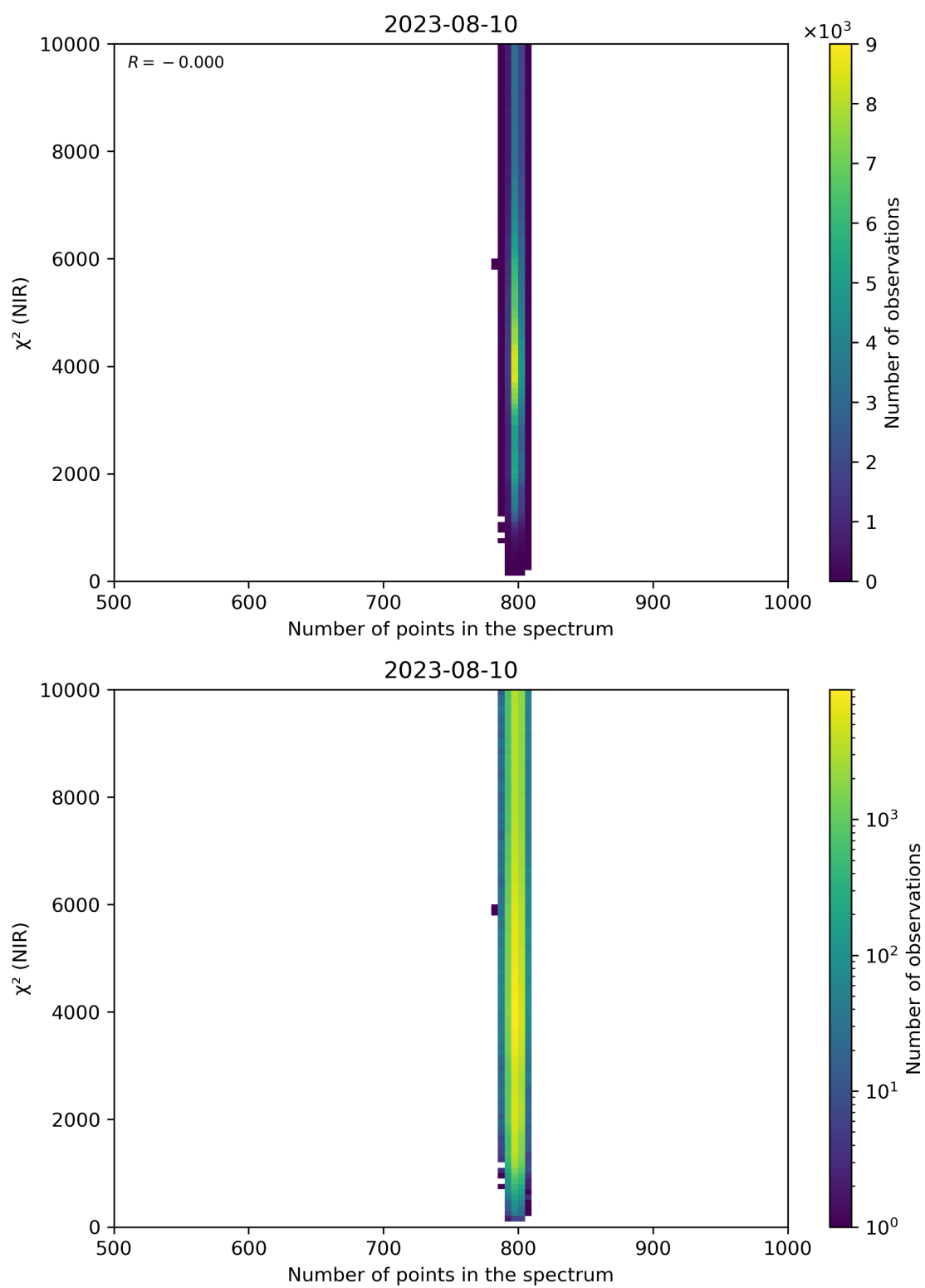
Figure 88: Scatter density plot of “Number of points in the spectrum” against “ \chi^2 (NIR)” for 2023-08-09 to 2023-08-11.
