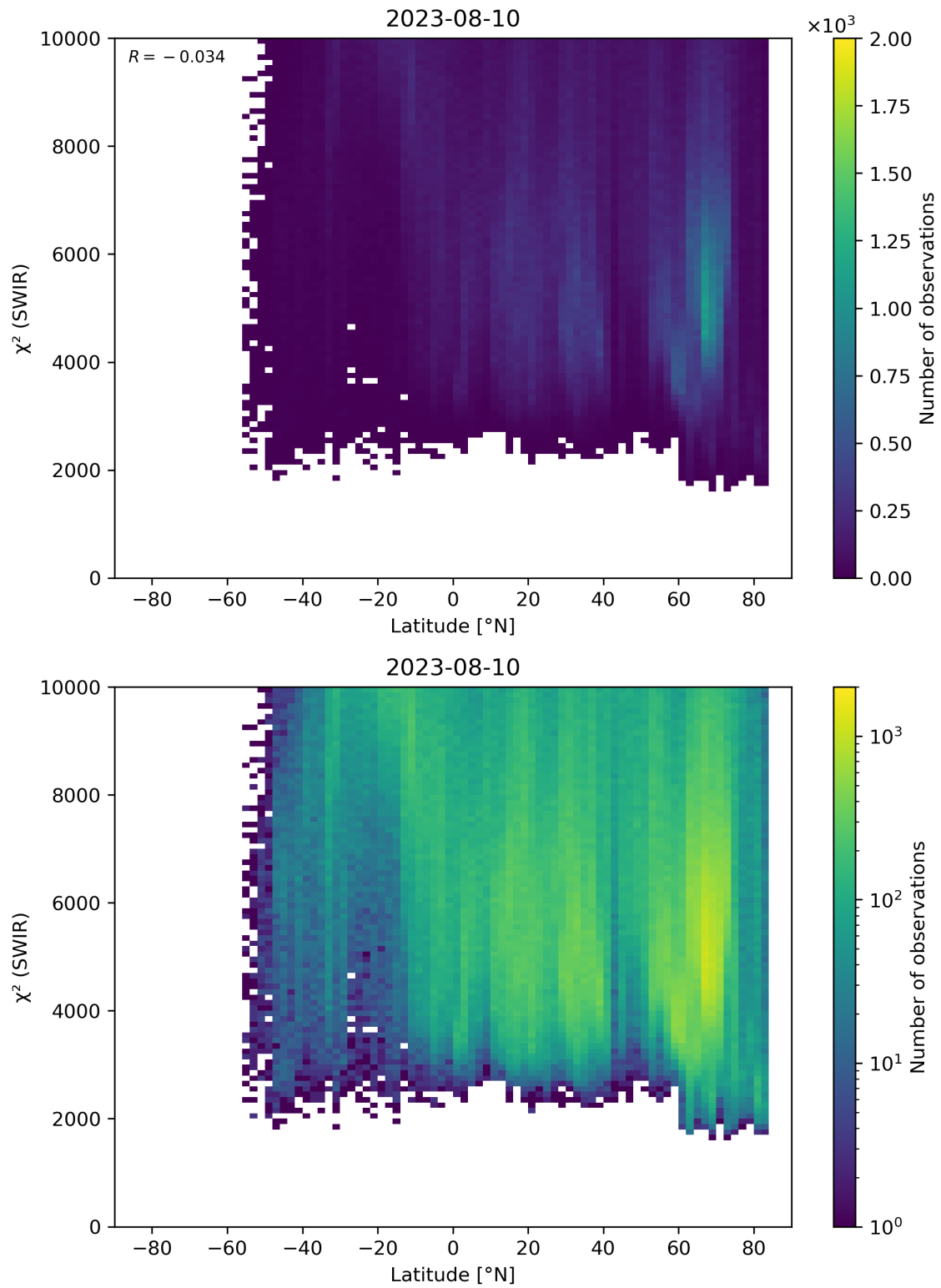
Figure 54: Scatter density plot of “Latitude” against “ \chi^2 (SWIR)” for 2023-08-09 to 2023-08-11.
