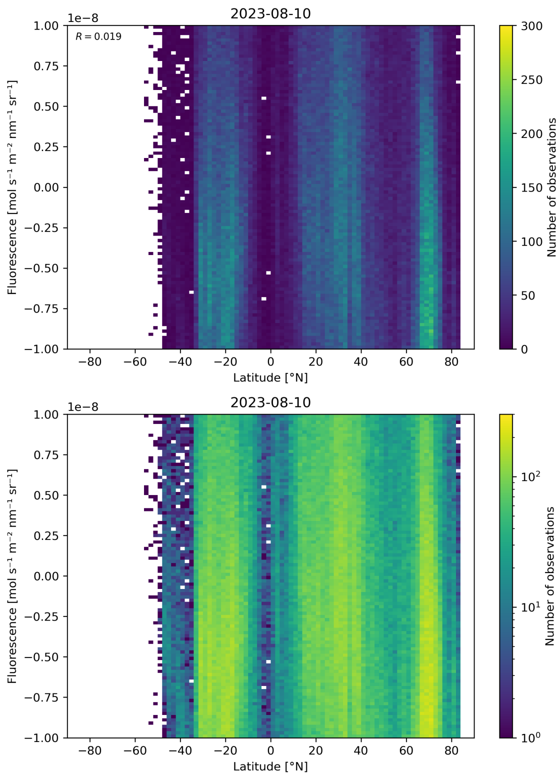
Figure 56: Scatter density plot of “Latitude” against “Fluorescence” for 2023-08-09 to 2023-08-11.
