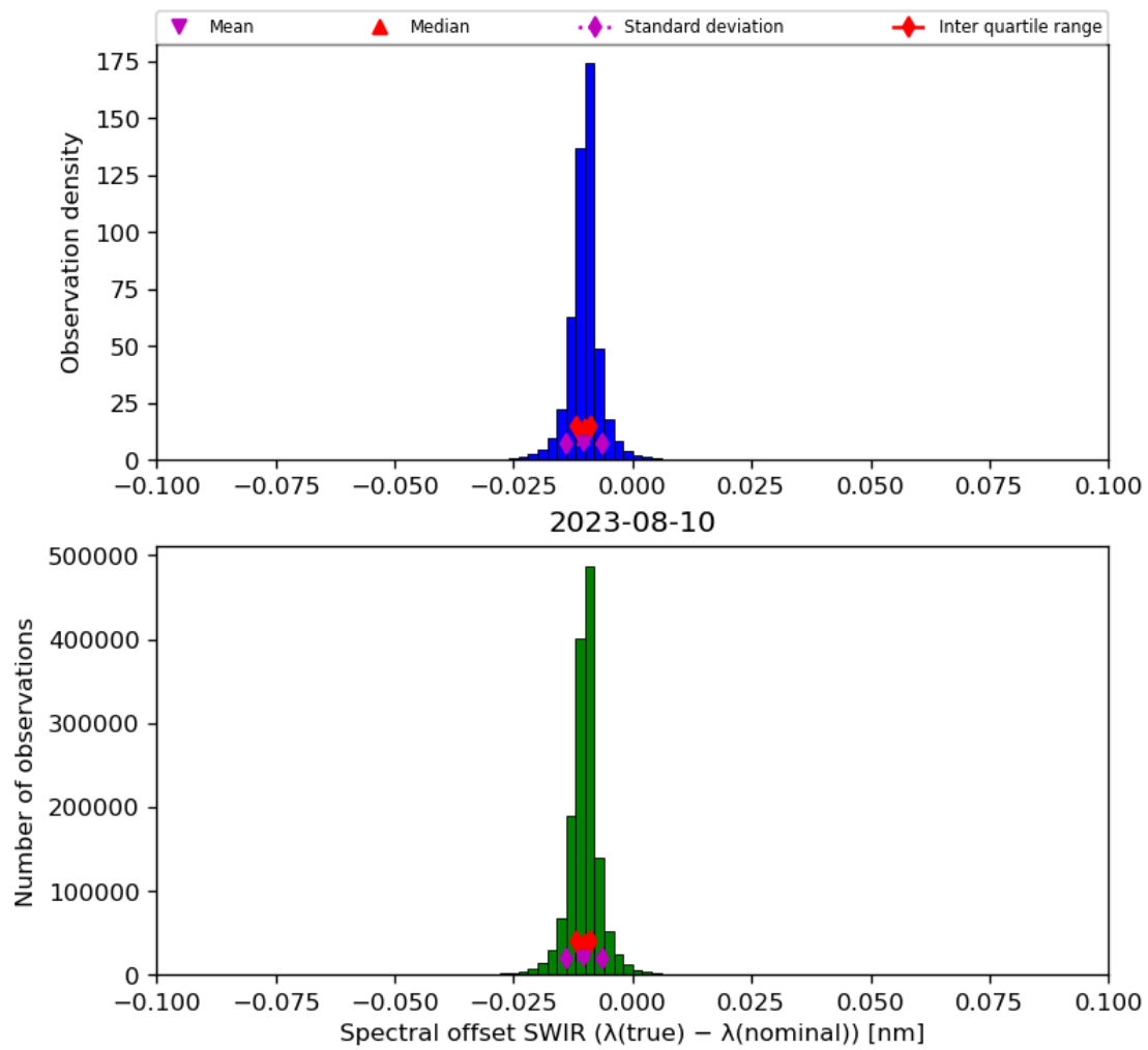
Figure 27: Histogram of “Spectral offset SWIR ( \lambda(\text{true}) - \lambda(\text{nominal}) )” for 2023-08-09 to 2023-08-11
