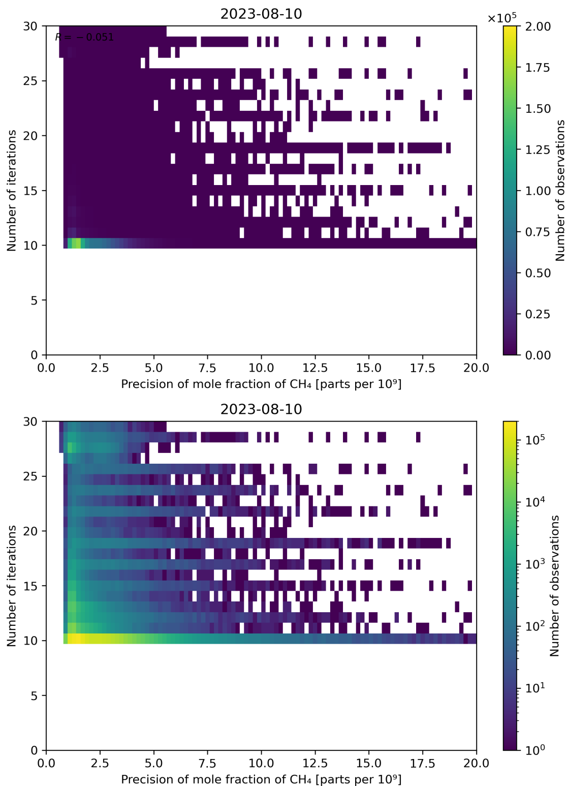
Figure 83: Scatter density plot of “Precision of mole fraction of CH 4 ” against “Number of iterations” for 2023-08-09 to 2023-08-11.
