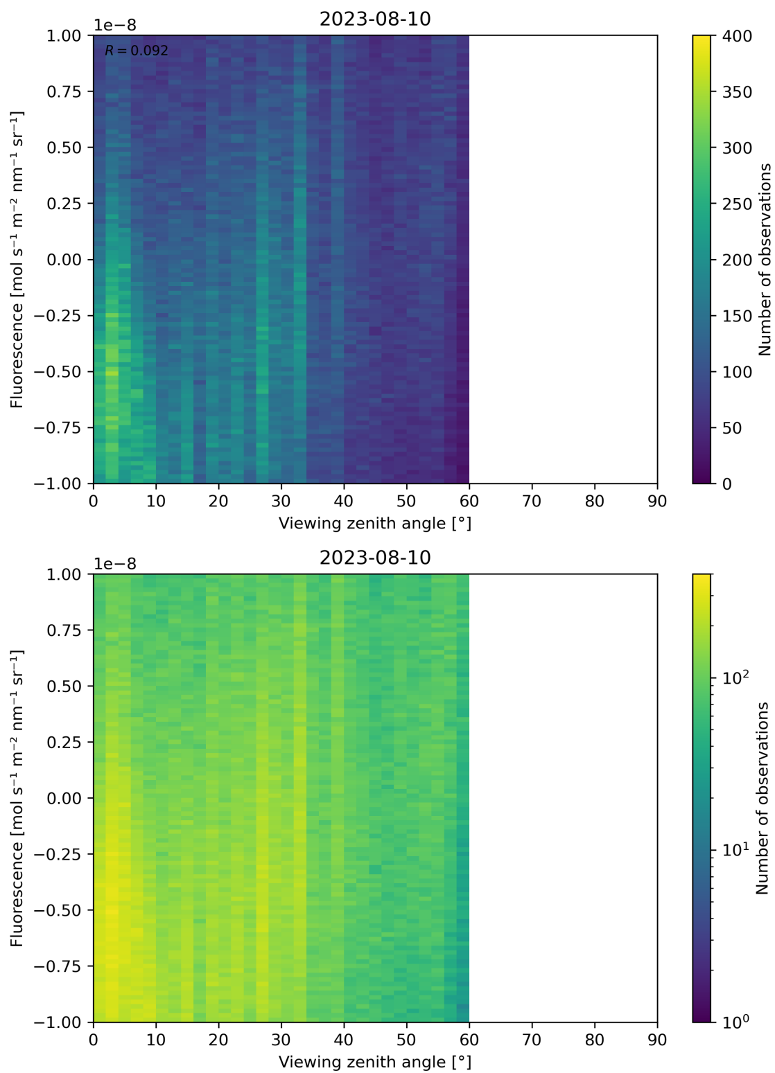
Figure 108: Scatter density plot of “Viewing zenith angle” against “Fluorescence” for 2023-08-09 to 2023-08-11.
