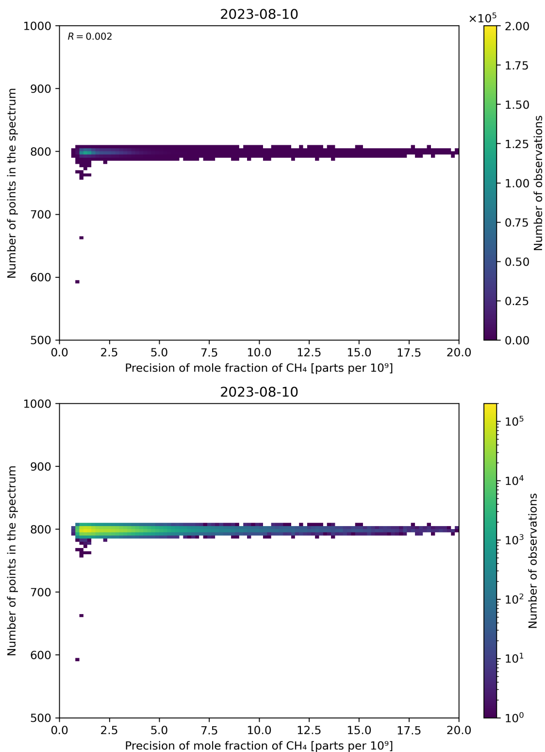
Figure 84: Scatter density plot of “Precision of mole fraction of CH 4 ” against “Number of points in the spectrum” for 2023-08-09 to 2023-08-11.
