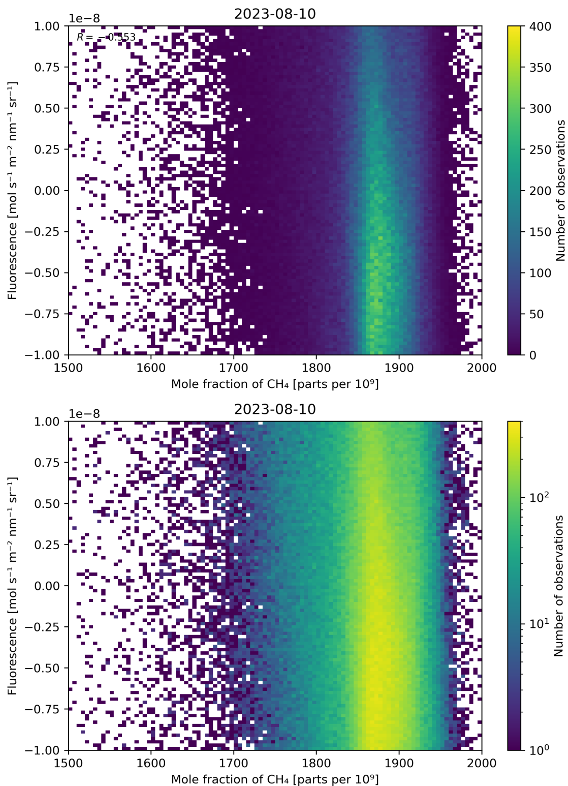
Figure 73: Scatter density plot of “Mole fraction of \text{CH}_4 ” against “Fluorescence” for 2023-08-09 to 2023-08-11.
