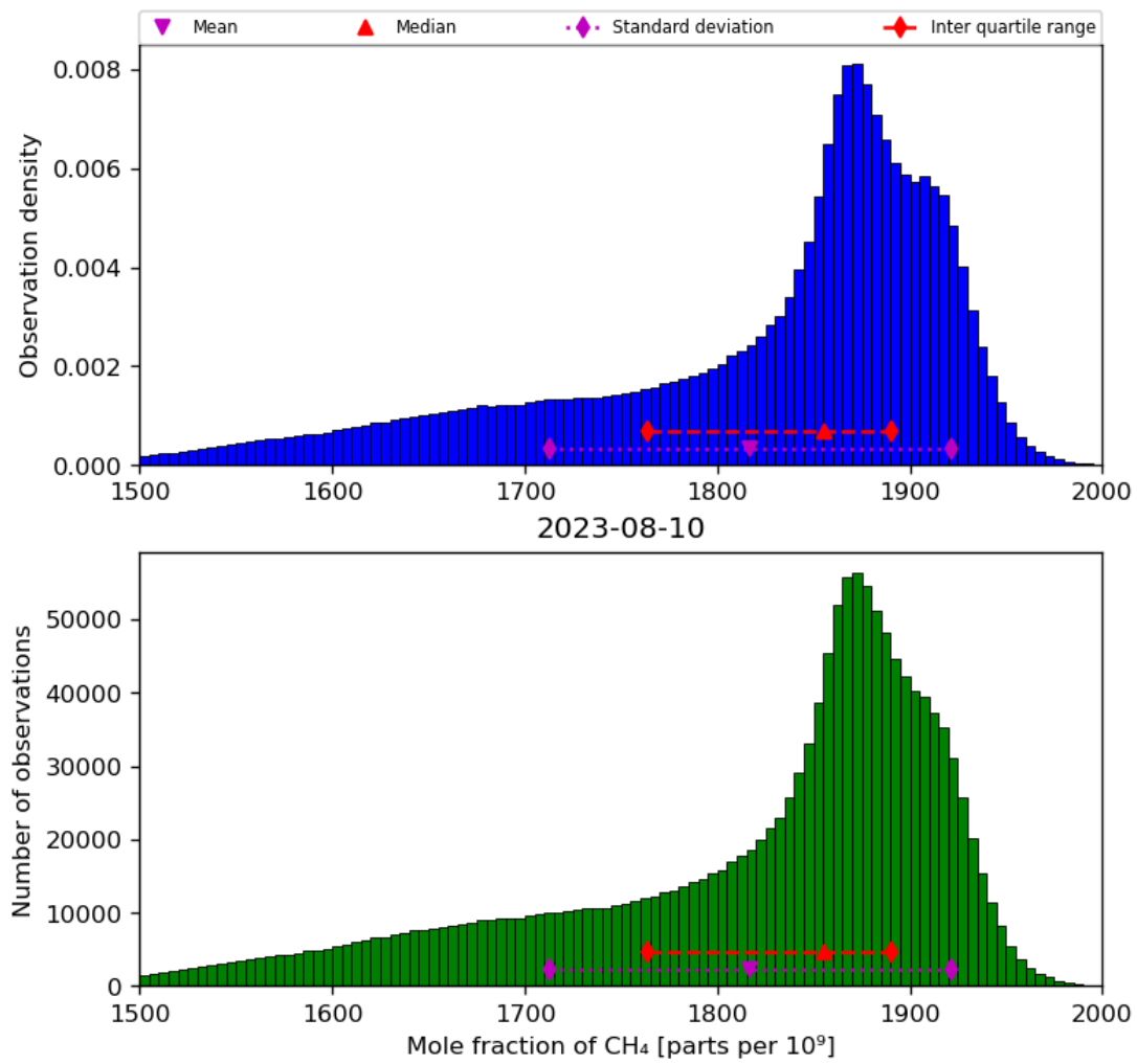
Figure 23: Histogram of “Mole fraction of CH 4 ” for 2023-08-09 to 2023-08-11
