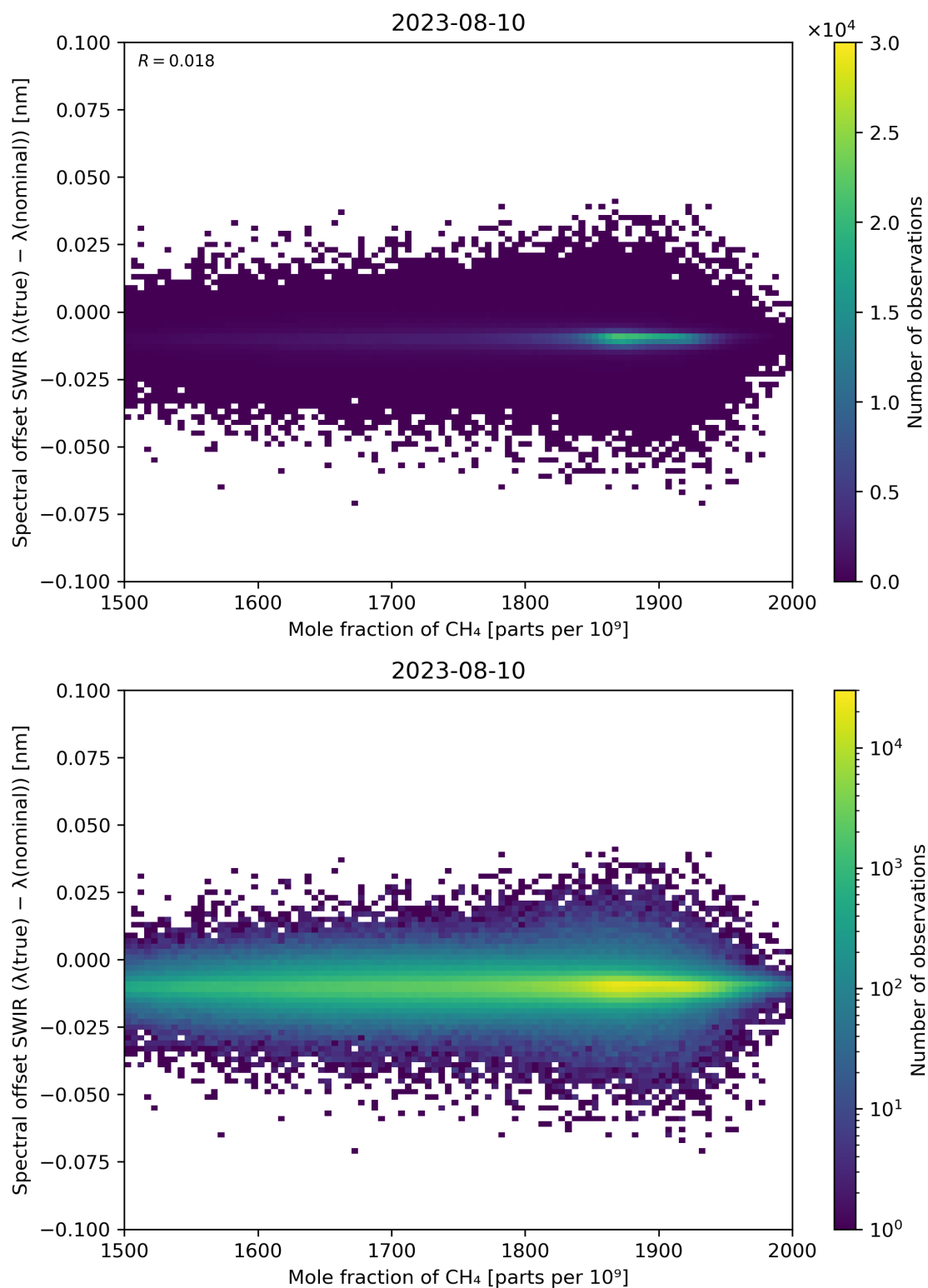
Figure 86: Scatter density plot of “Mole fraction of CH 4 ” against “Spectral offset SWIR ( \lambda(\text{true}) - \lambda(\text{nominal}) )” for 2023-08-09 to 2023-08-11.
