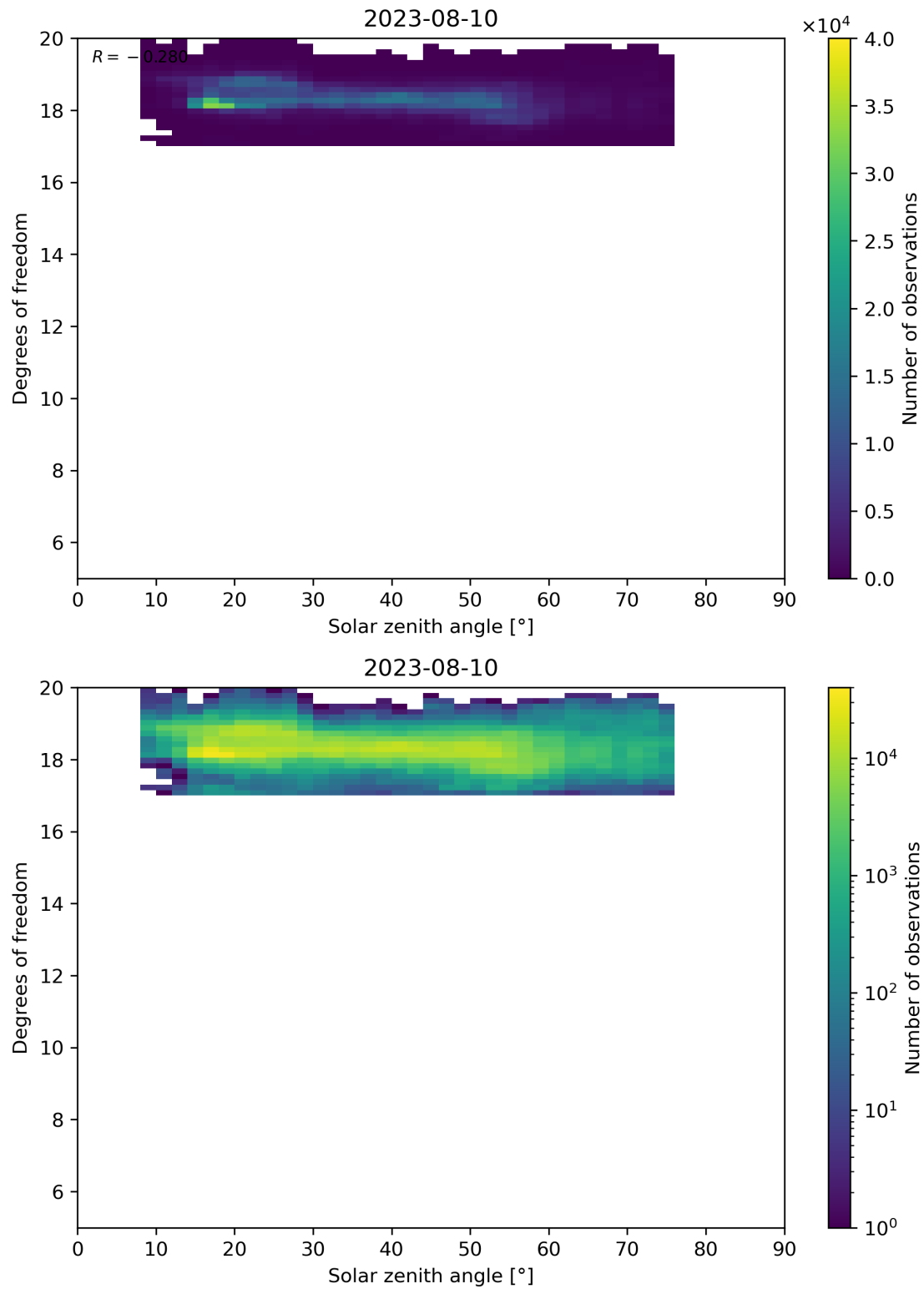
Figure 96: Scatter density plot of “Solar zenith angle” against “Degrees of freedom” for 2023-08-09 to 2023-08-11.
