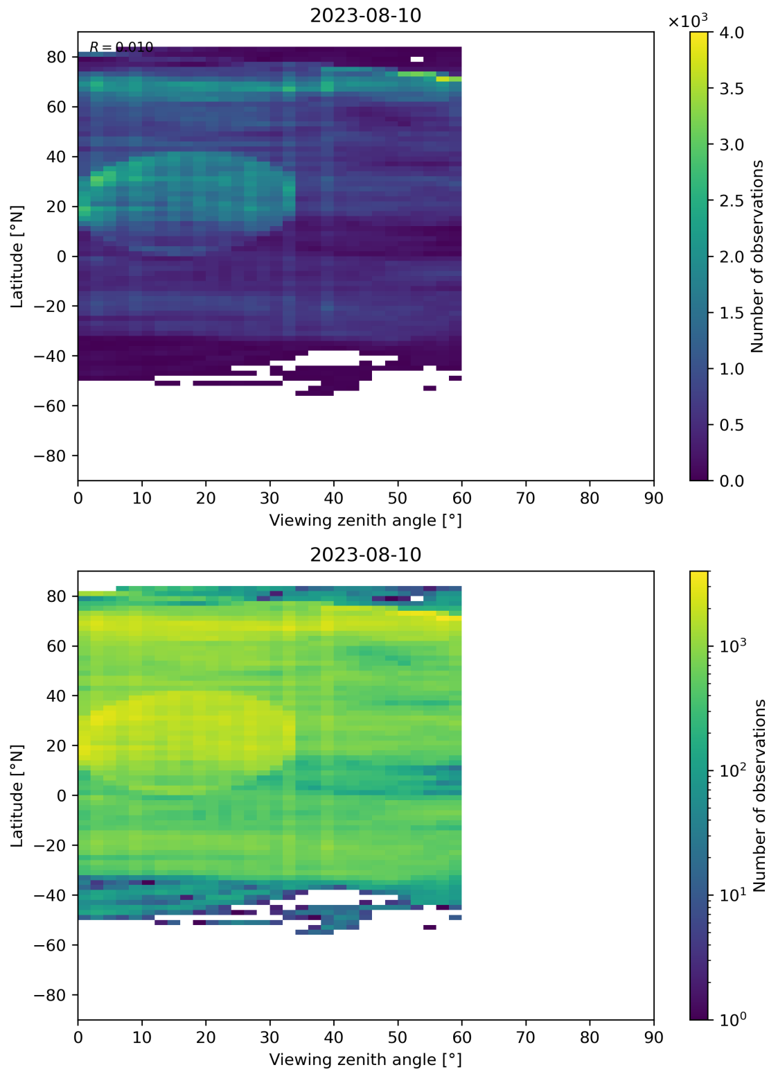
Figure 109: Scatter density plot of “Viewing zenith angle” against “Latitude” for 2023-08-09 to 2023-08-11.
