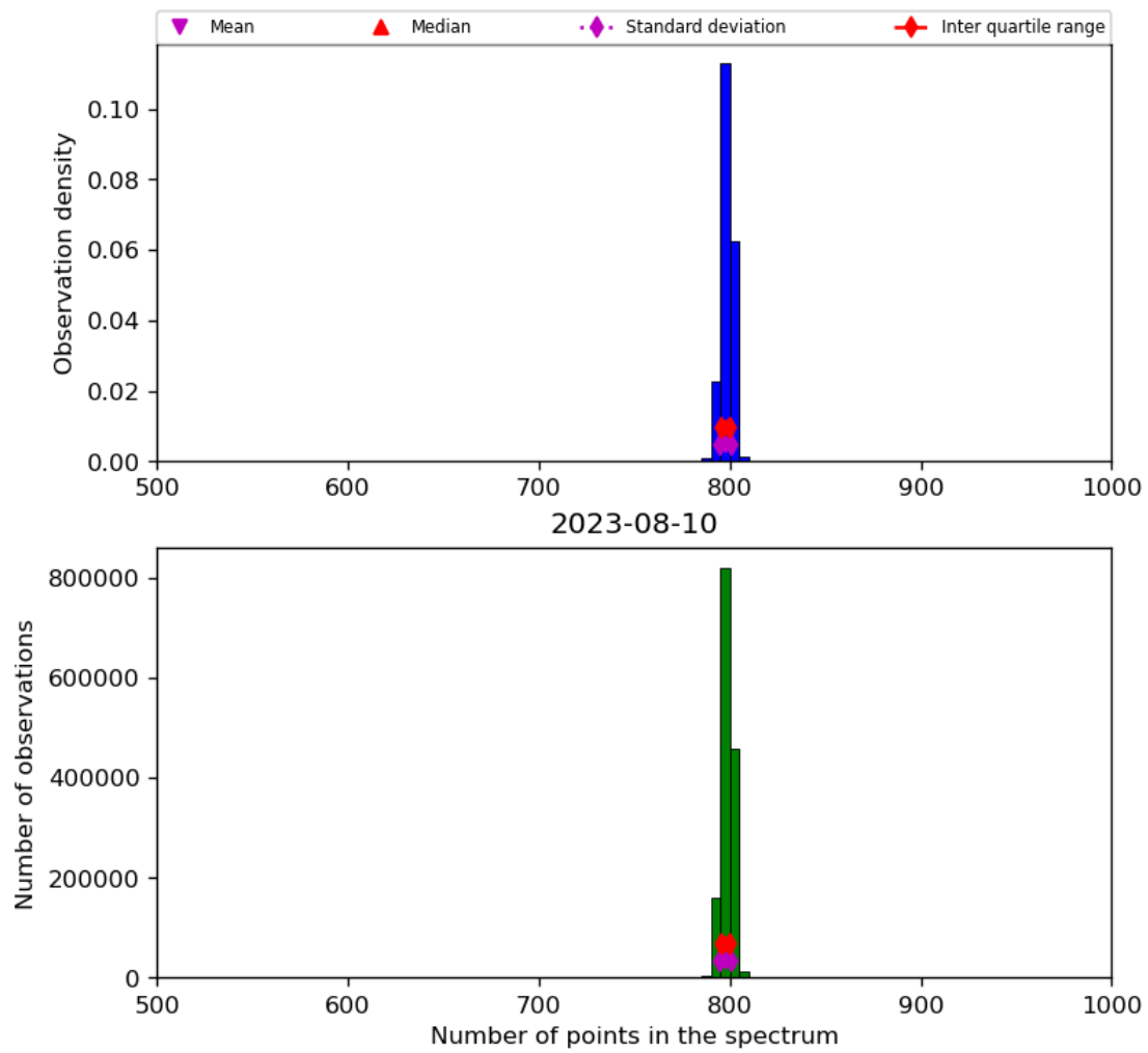
Figure 26: Histogram of “Number of points in the spectrum” for 2023-08-09 to 2023-08-11
