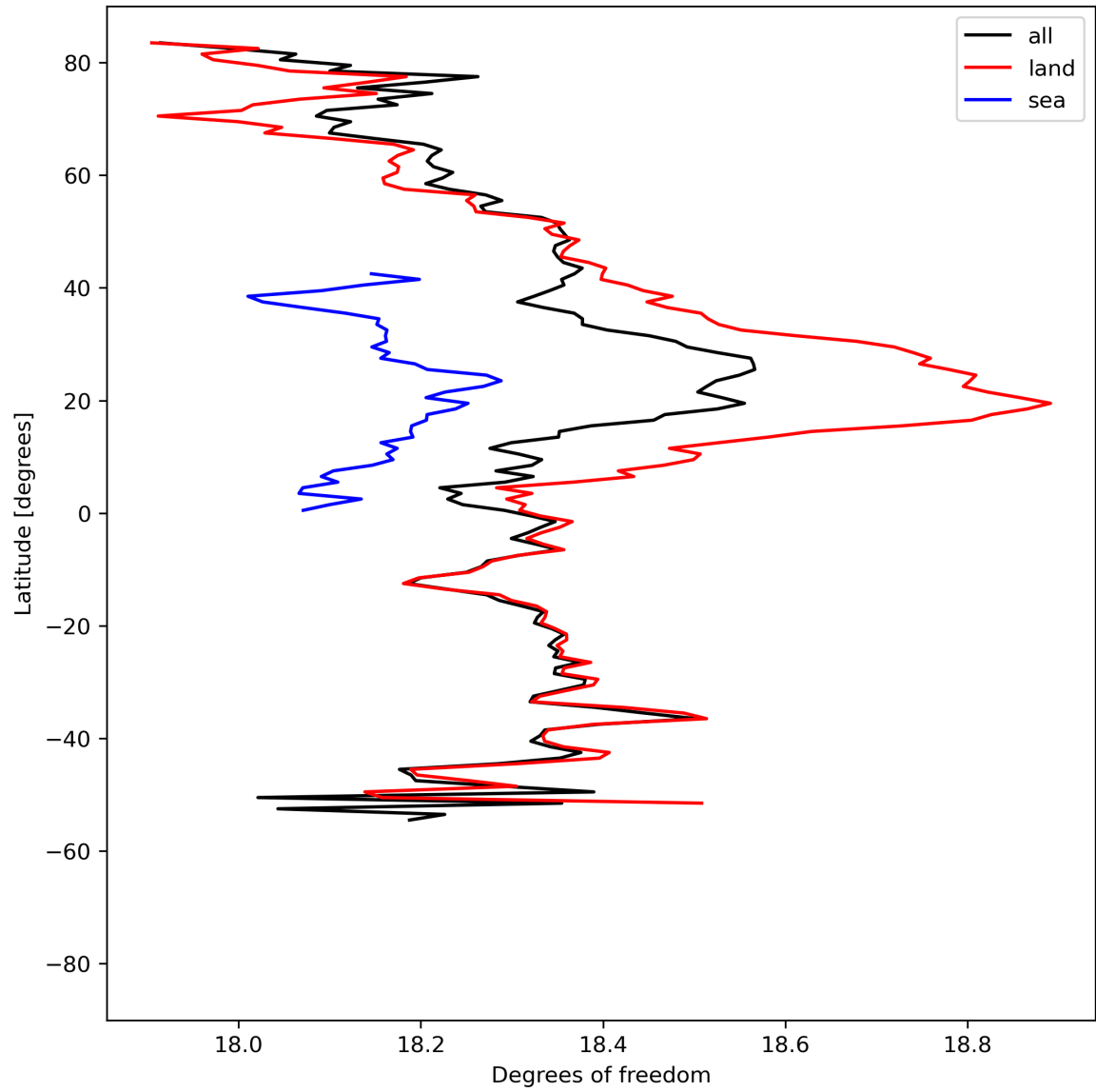
Figure 19: Zonal average of “Degrees of freedom” for 2023-08-09 to 2023-08-11.
