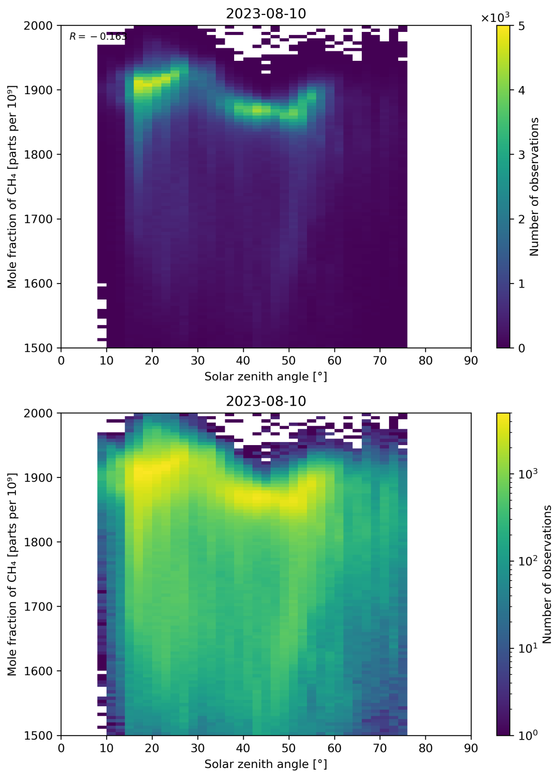
Figure 99: Scatter density plot of “Solar zenith angle” against “Mole fraction of CH 4 ” for 2023-08-09 to 2023-08-11.
