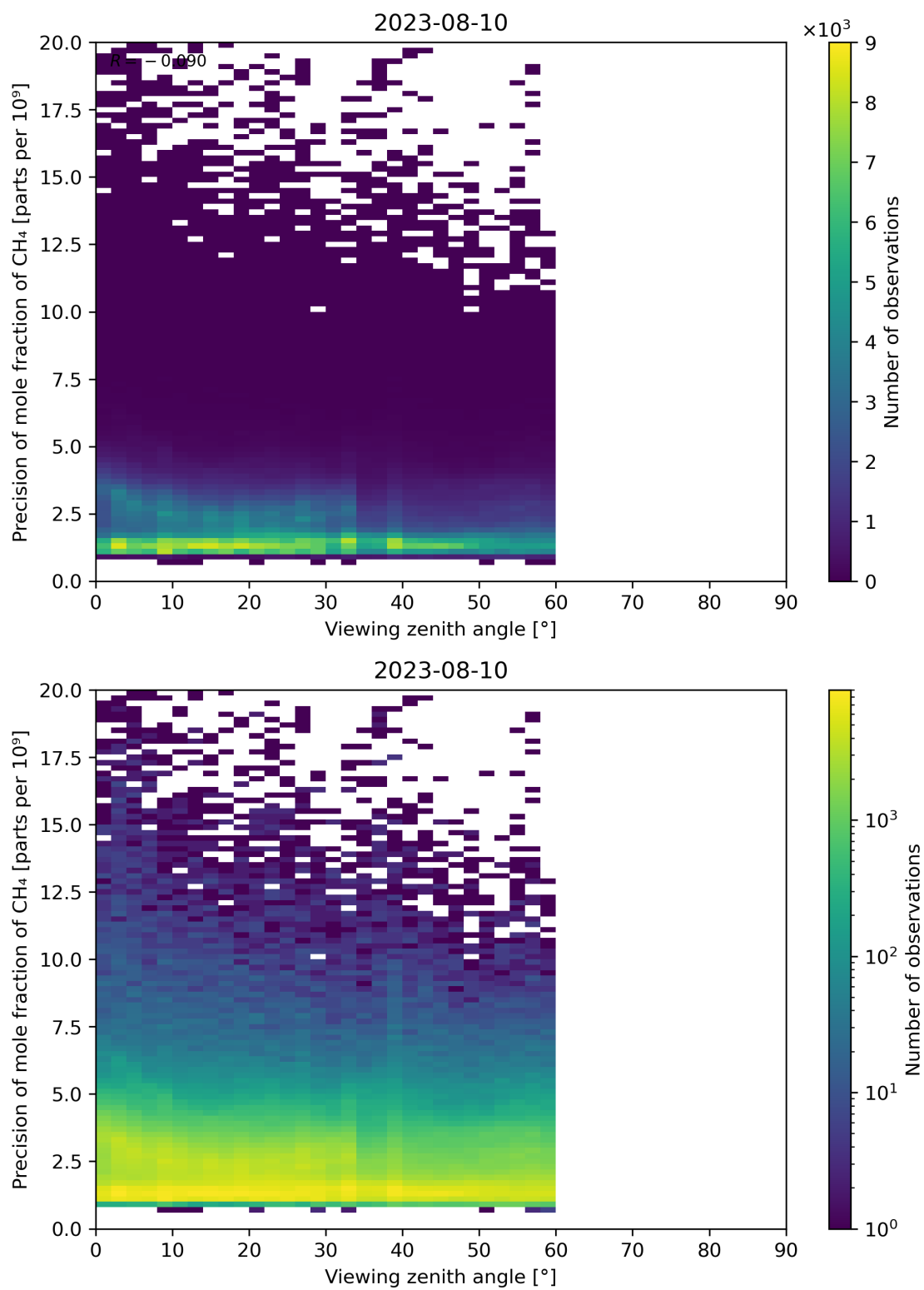
Figure 112: Scatter density plot of “Viewing zenith angle” against “Precision of mole fraction of CH 4 ” for 2023-08-09 to 2023-08-11.
