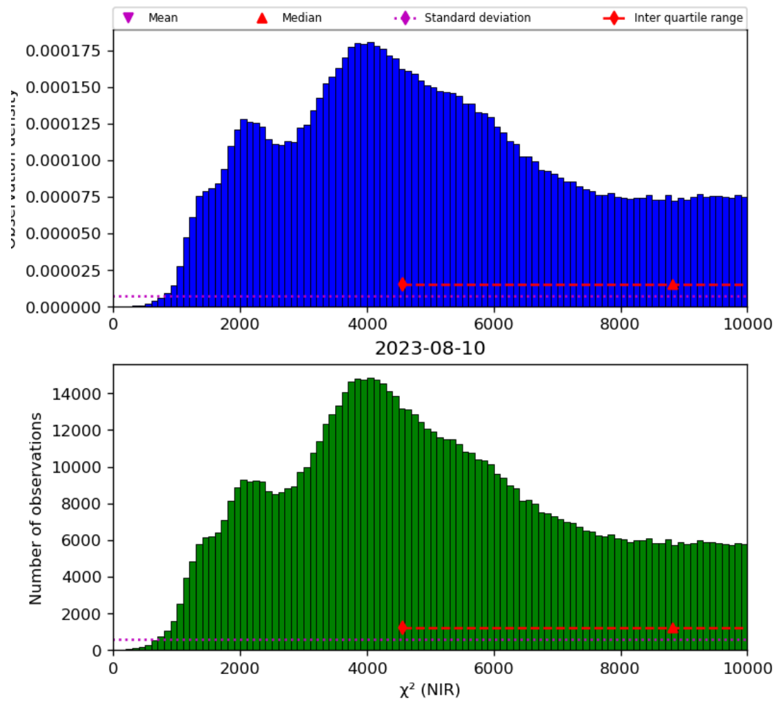
Figure 29: Histogram of “ \chi^2 (NIR)” for 2023-08-09 to 2023-08-11
