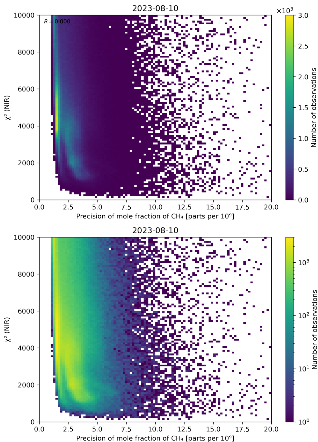
Figure 78: Scatter density plot of “Precision of mole fraction of \text{CH}_4 ” against “ \chi^2 (NIR)” for 2023-08-09 to 2023-08-11.
