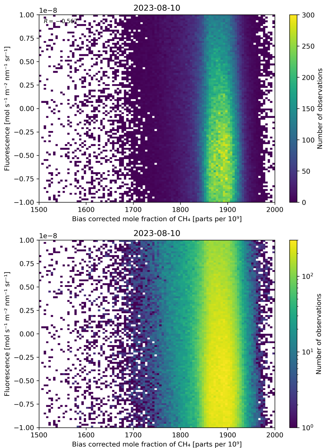
Figure 66: Scatter density plot of “Bias corrected mole fraction of \text{CH}_4 ” against “Fluorescence” for 2023-08-09 to 2023-08-11.
