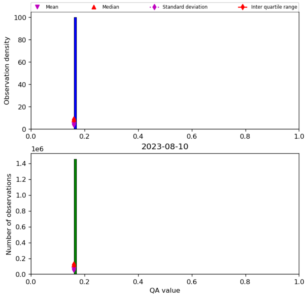
Figure 22: Histogram of “QA value” for 2023-08-09 to 2023-08-11
