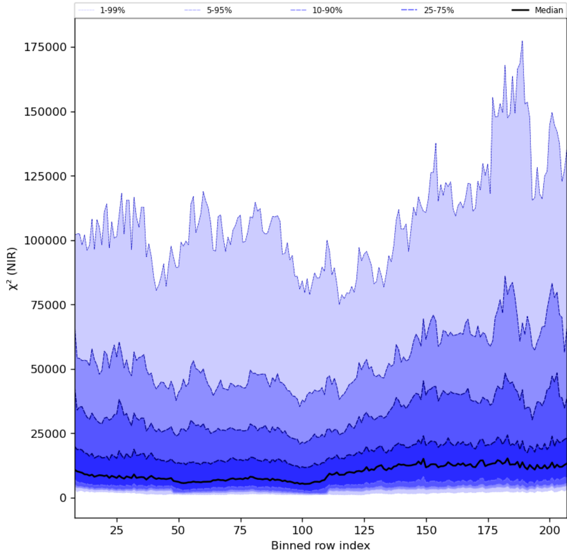
Figure 40: Along track statistics of “ \chi^2 (NIR)” for 2023-08-09 to 2023-08-11
