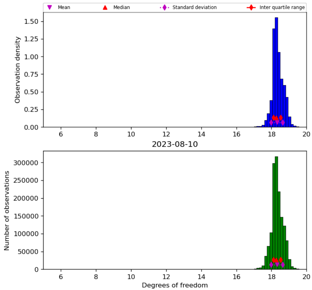
Figure 30: Histogram of “Degrees of freedom” for 2023-08-09 to 2023-08-11
