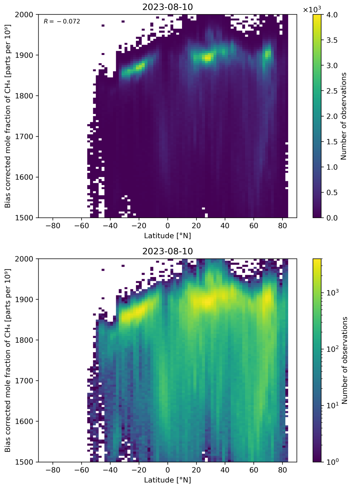
Figure 58: Scatter density plot of “Latitude” against “Bias corrected mole fraction of \text{CH}_4 ” for 2023-08-09 to 2023-08-11.
