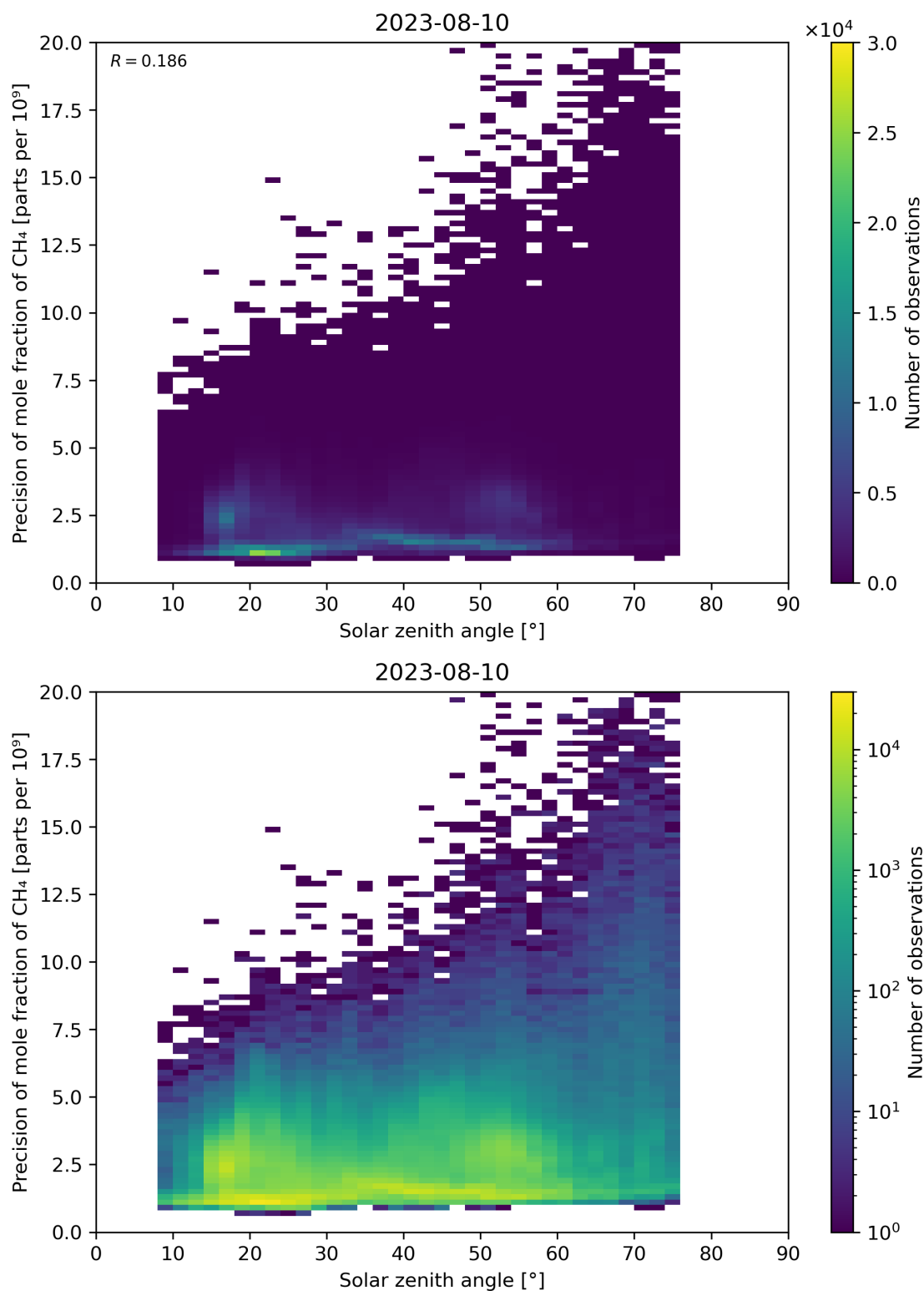
Figure 101: Scatter density plot of “Solar zenith angle” against “Precision of mole fraction of CH 4 ” for 2023-08-09 to 2023-08-11.
