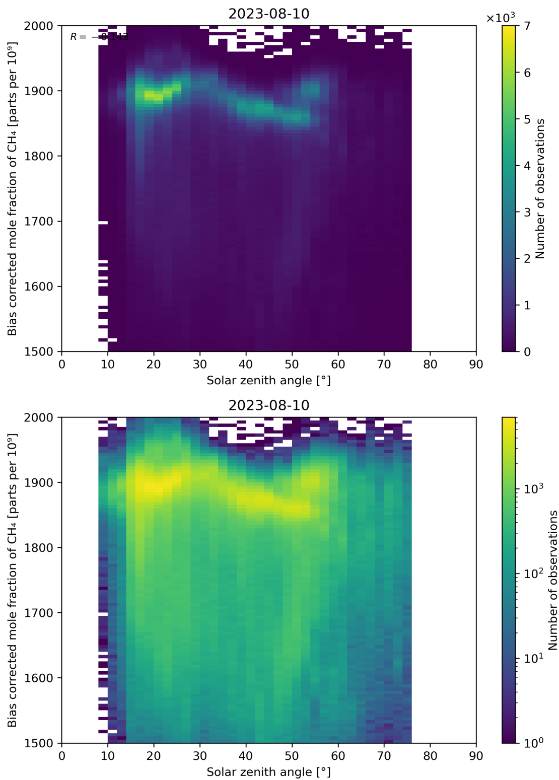
Figure 100: Scatter density plot of “Solar zenith angle” against “Bias corrected mole fraction of \text{CH}_4 ” for 2023-08-09 to 2023-08-11.
