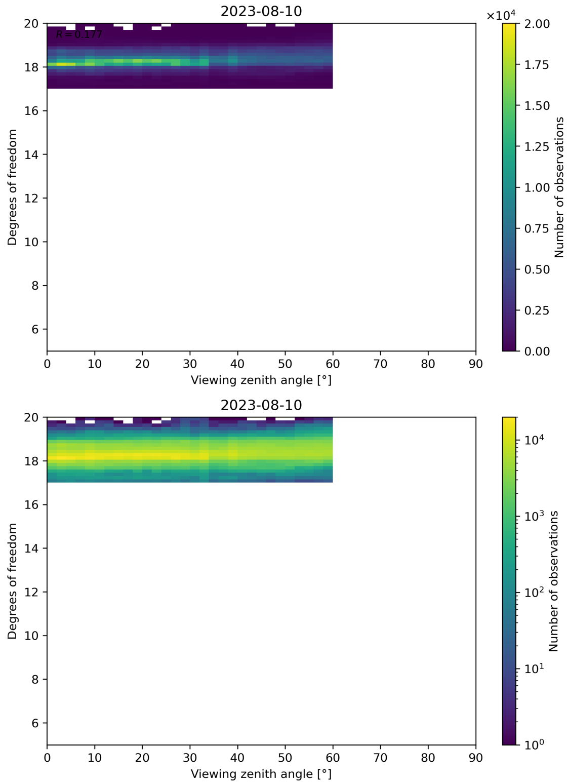
Figure 107: Scatter density plot of “Viewing zenith angle” against “Degrees of freedom” for 2023-08-09 to 2023-08-11.
