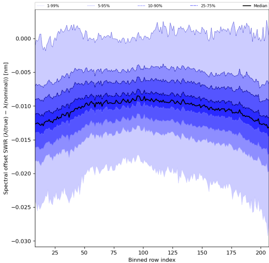
Figure 38: Along track statistics of “Spectral offset SWIR ( \lambda(\text{true}) - \lambda(\text{nominal}) )” for 2023-08-09 to 2023-08-11
