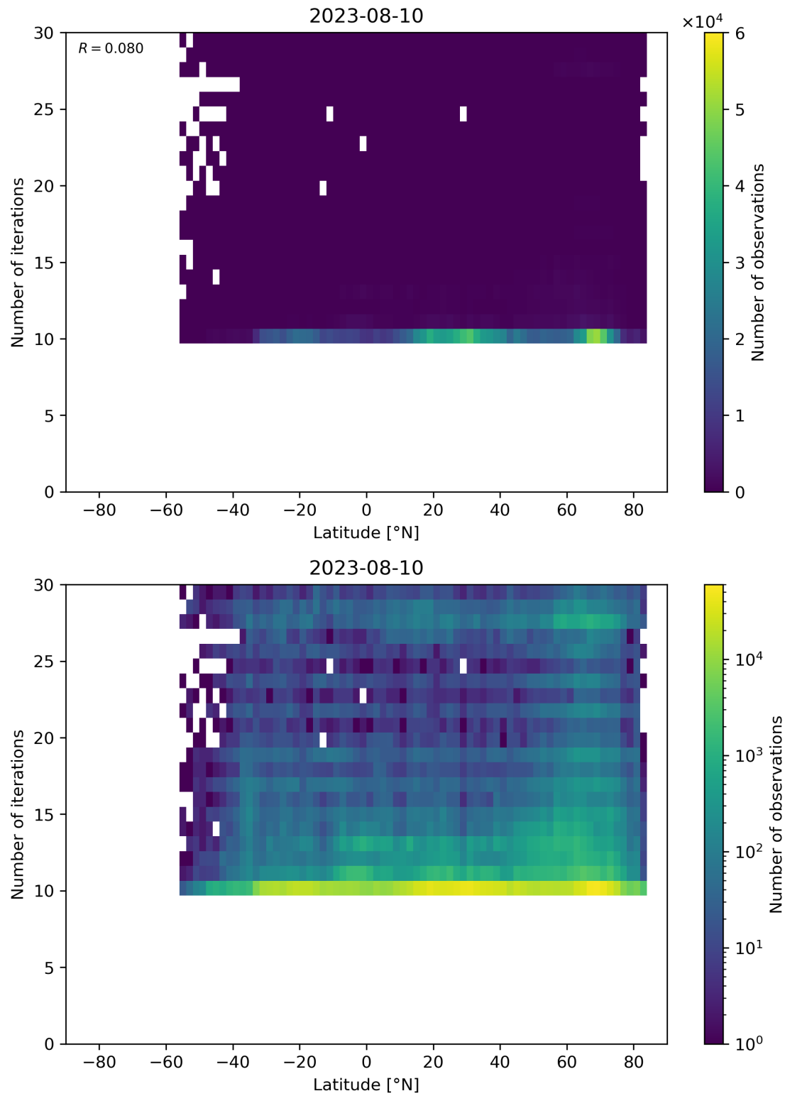
Figure 60: Scatter density plot of “Latitude” against “Number of iterations” for 2023-08-09 to 2023-08-11.
