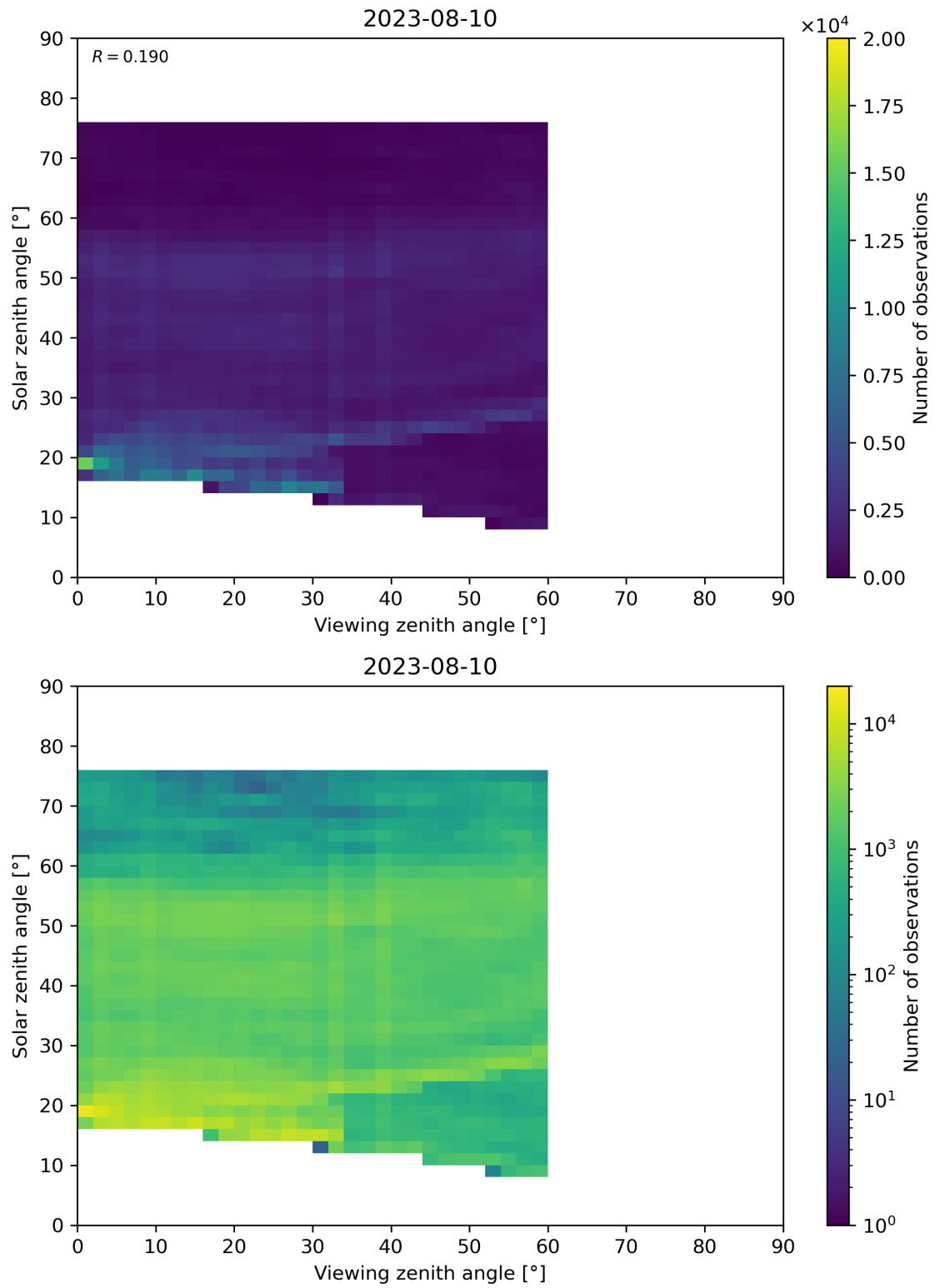
Figure 115: Scatter density plot of “Viewing zenith angle” against “Solar zenith angle” for 2023-08-09 to 2023-08-11.
