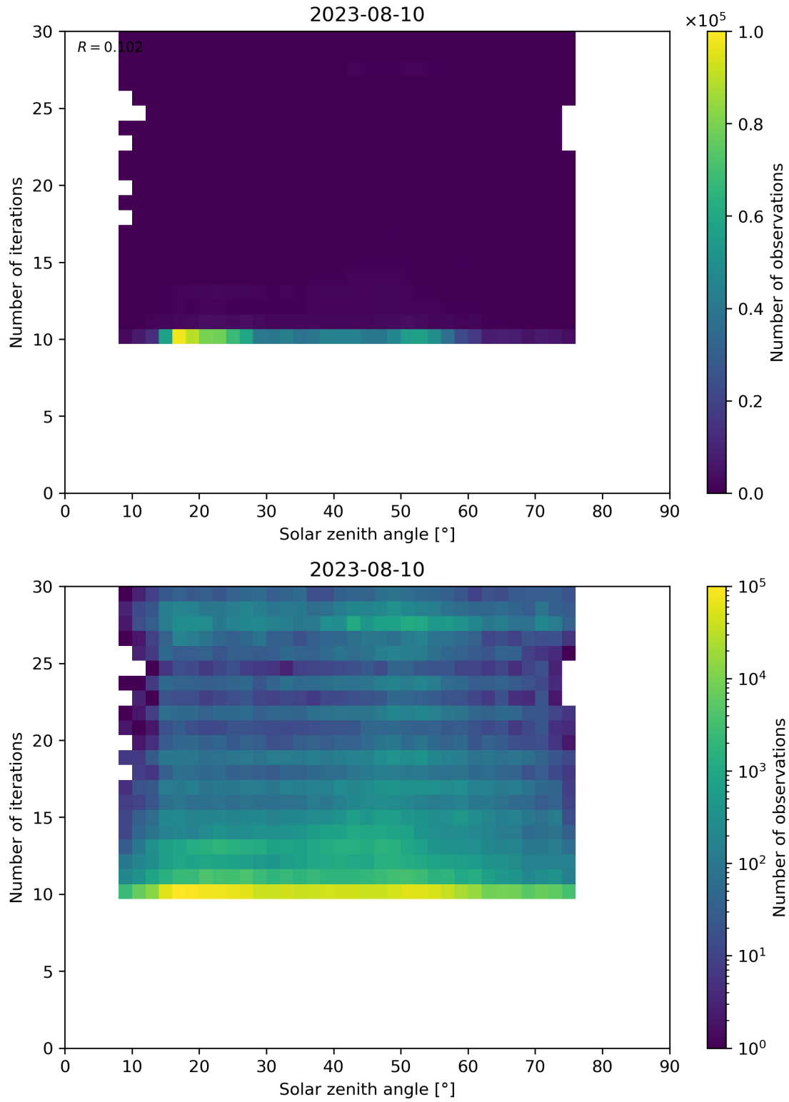
Figure 102: Scatter density plot of “Solar zenith angle” against “Number of iterations” for 2023-08-09 to 2023-08-11.
