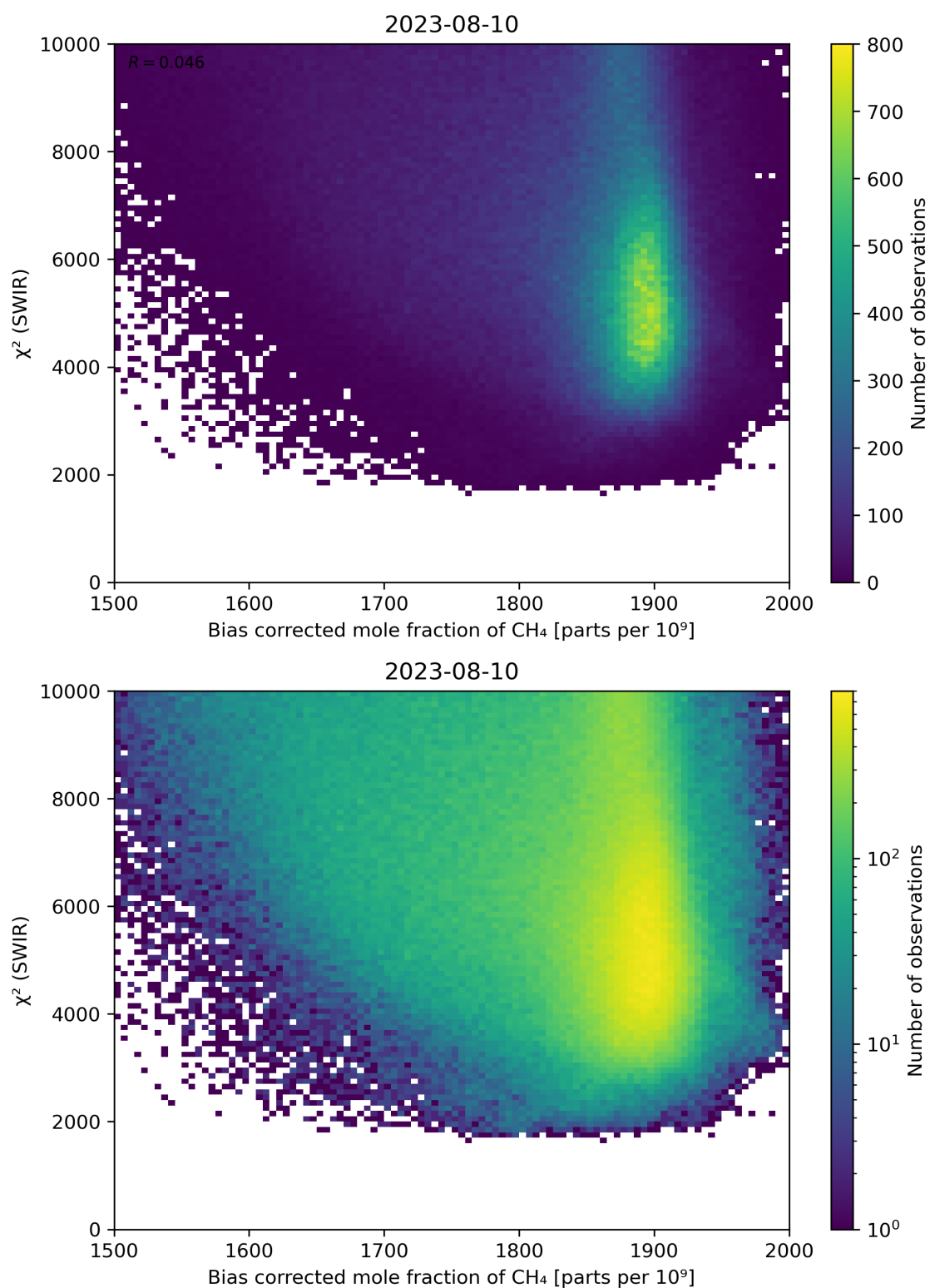
Figure 64: Scatter density plot of “Bias corrected mole fraction of CH 4 ” against “ \chi^2 (SWIR)” for 2023-08-09 to 2023-08-11.
