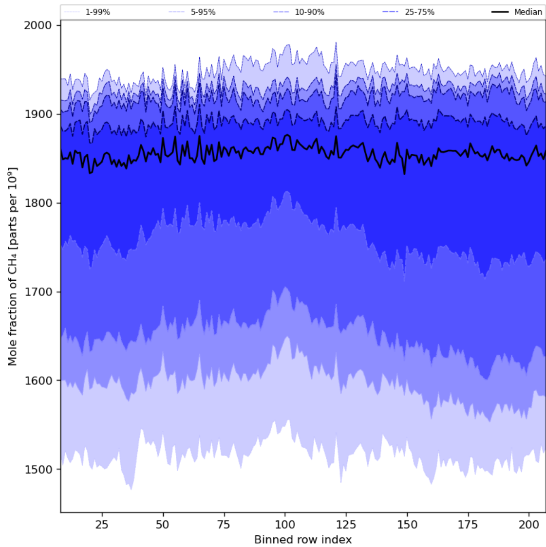
Figure 34: Along track statistics of “Mole fraction of CH 4 ” for 2023-08-09 to 2023-08-11
