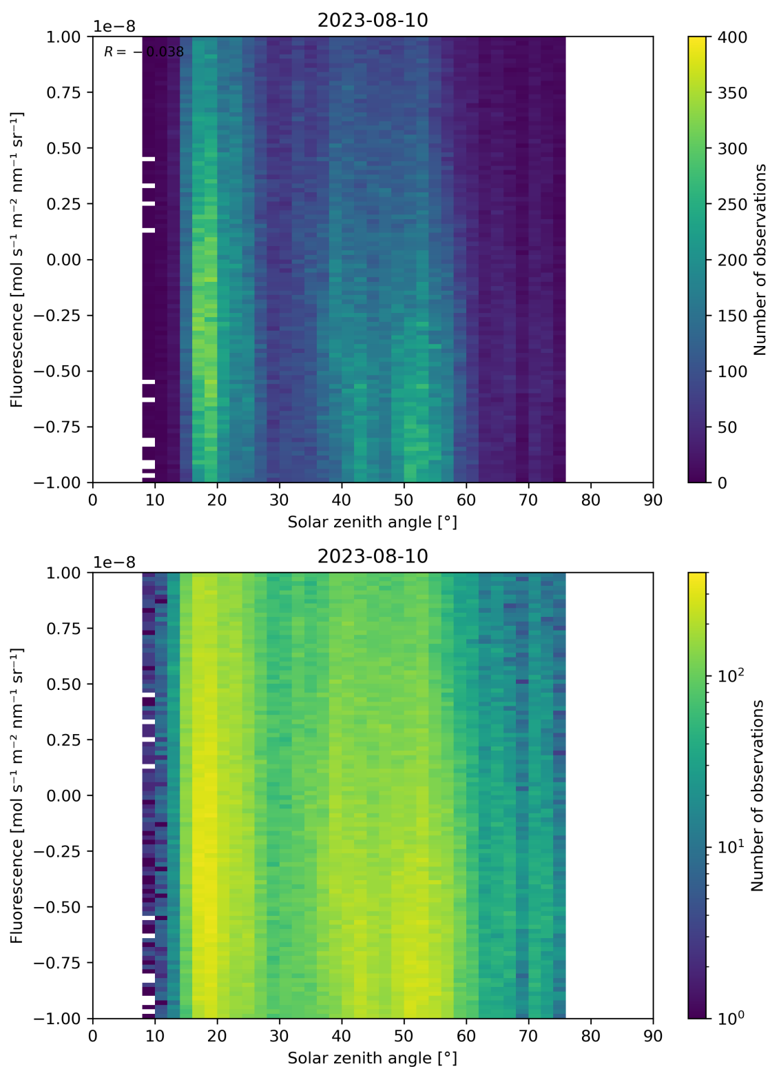
Figure 97: Scatter density plot of “Solar zenith angle” against “Fluorescence” for 2023-08-09 to 2023-08-11.
