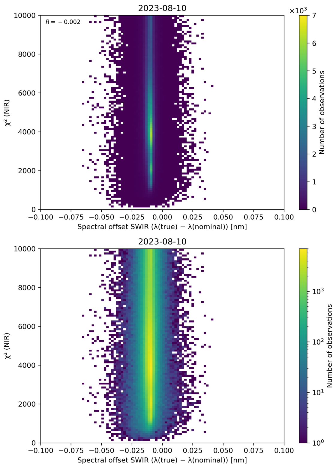
Figure 117: Scatter density plot of “Spectral offset SWIR ( \lambda(\text{true}) - \lambda(\text{nominal}) )” against “ \chi^2 (NIR)” for 2023-08-09 to 2023-08-11.
