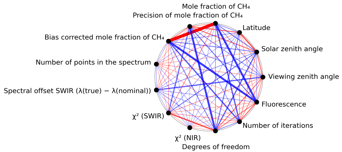
Figure 1: Map of correlation graph for 2023-08-09 to 2023-08-11.
