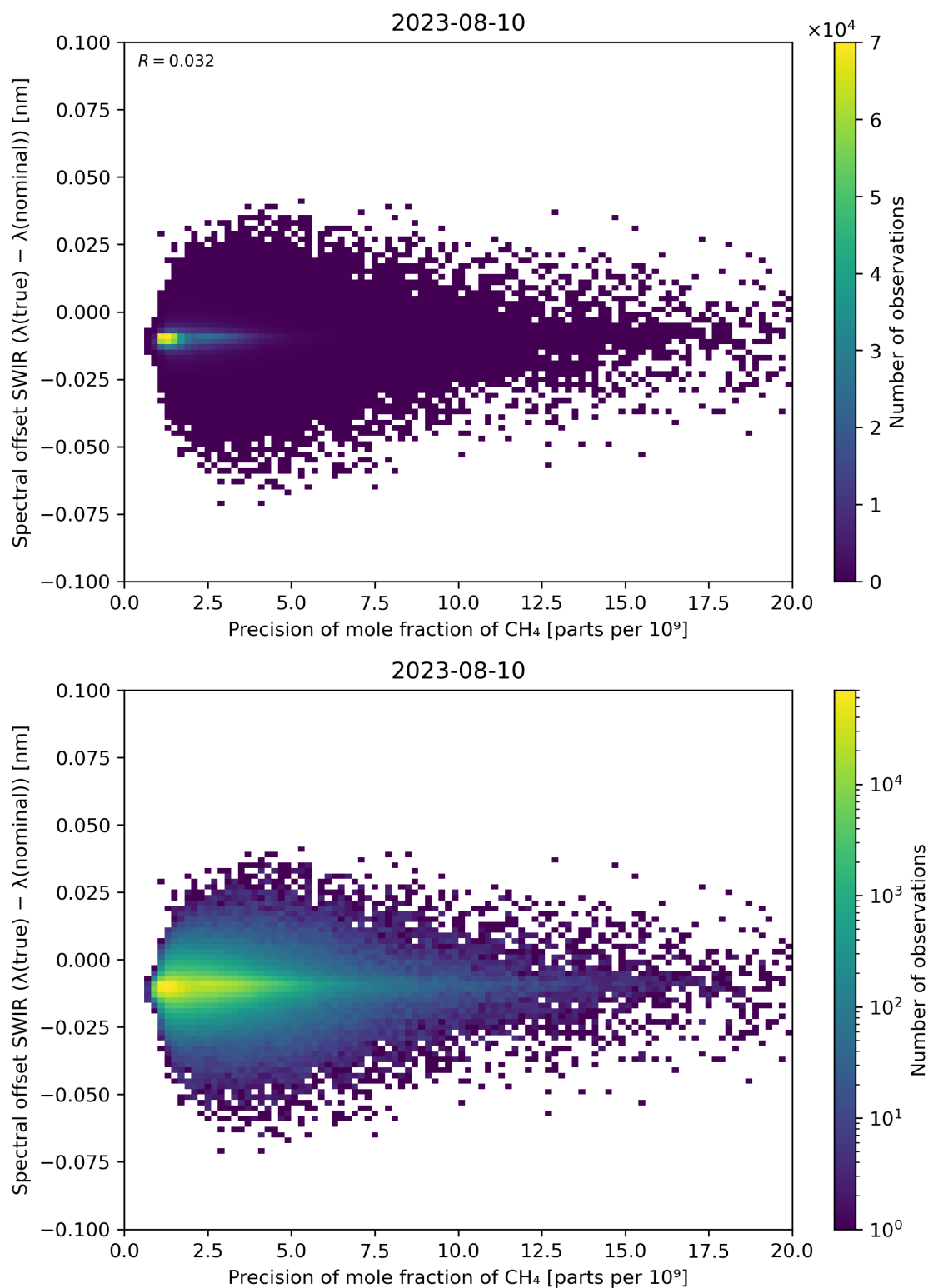
Figure 85: Scatter density plot of “Precision of mole fraction of CH 4 ” against “Spectral offset SWIR ( \lambda(\text{true}) - \lambda(\text{nominal}) )” for 2023-08-09 to 2023-08-11.
