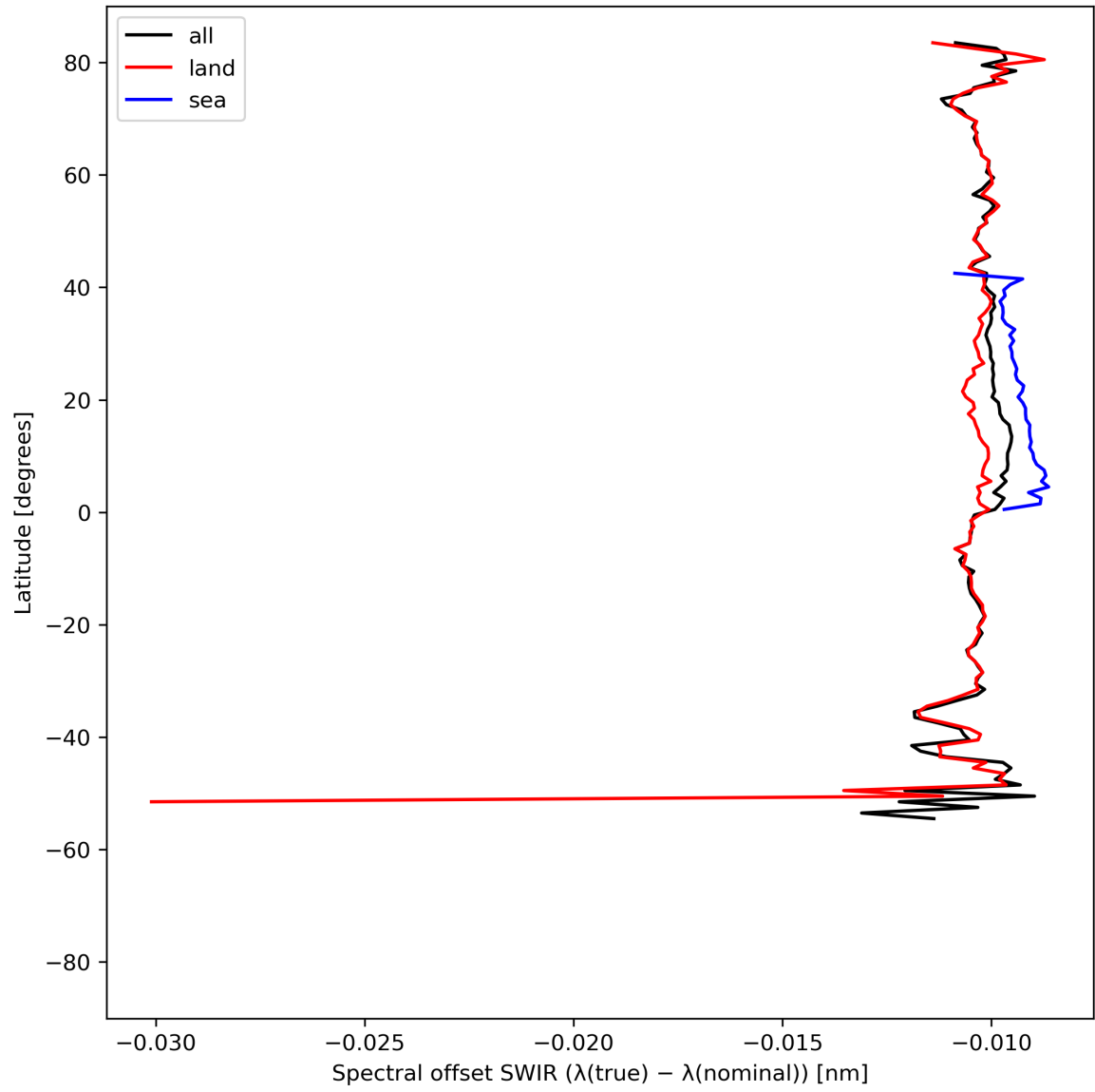
Figure 16: Zonal average of “Spectral offset SWIR ( \lambda(\text{true}) - \lambda(\text{nominal}) )” for 2023-08-09 to 2023-08-11.
