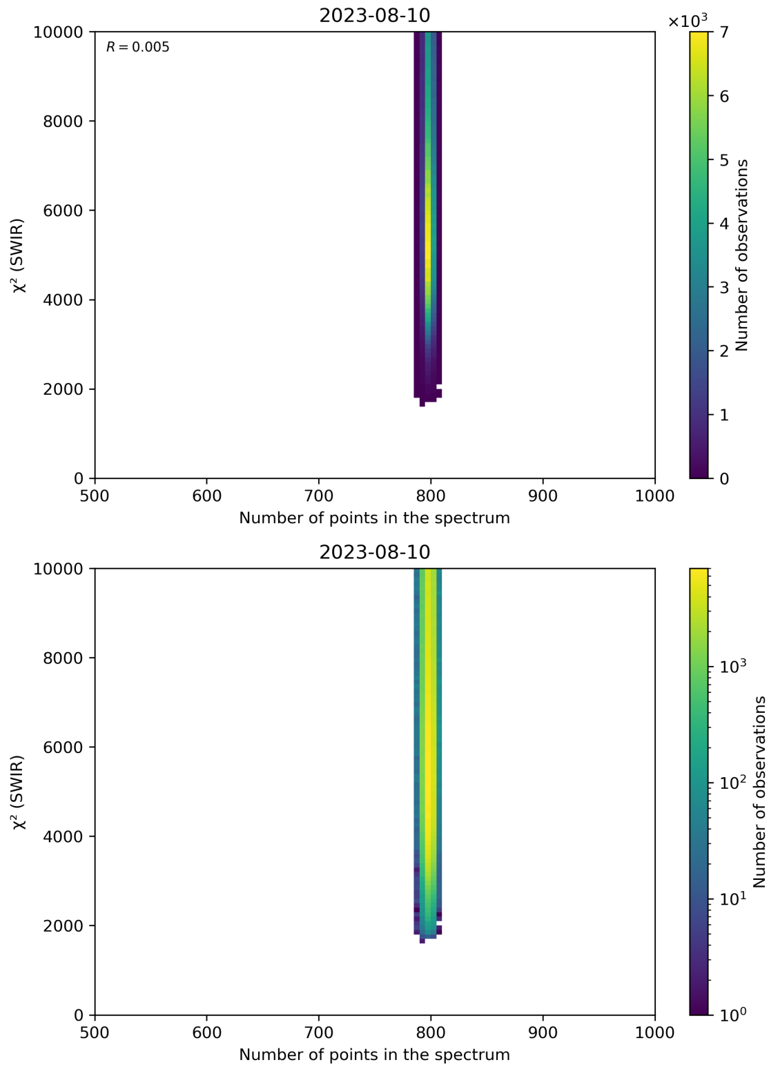
Figure 89: Scatter density plot of “Number of points in the spectrum” against “ \chi^2 (SWIR)” for 2023-08-09 to 2023-08-11.
