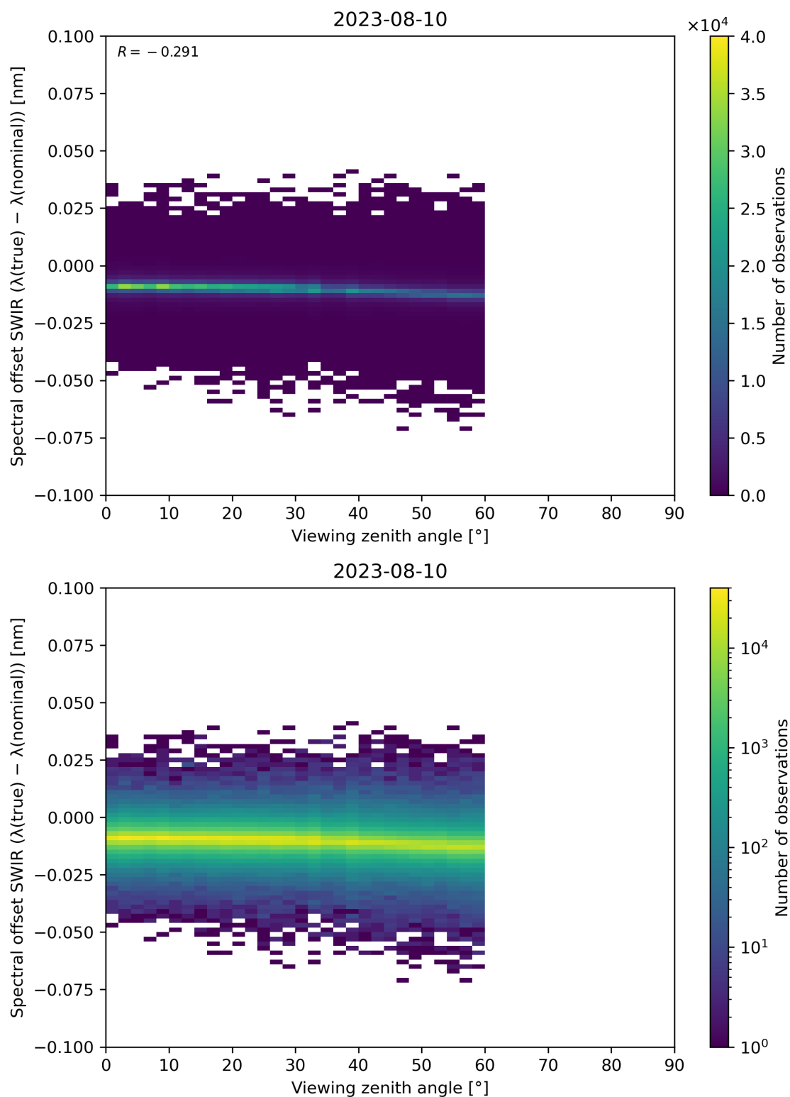
Figure 116: Scatter density plot of “Viewing zenith angle” against “Spectral offset SWIR ( \lambda(\text{true}) - \lambda(\text{nominal}) )” for 2023-08-09 to 2023-08-11.
