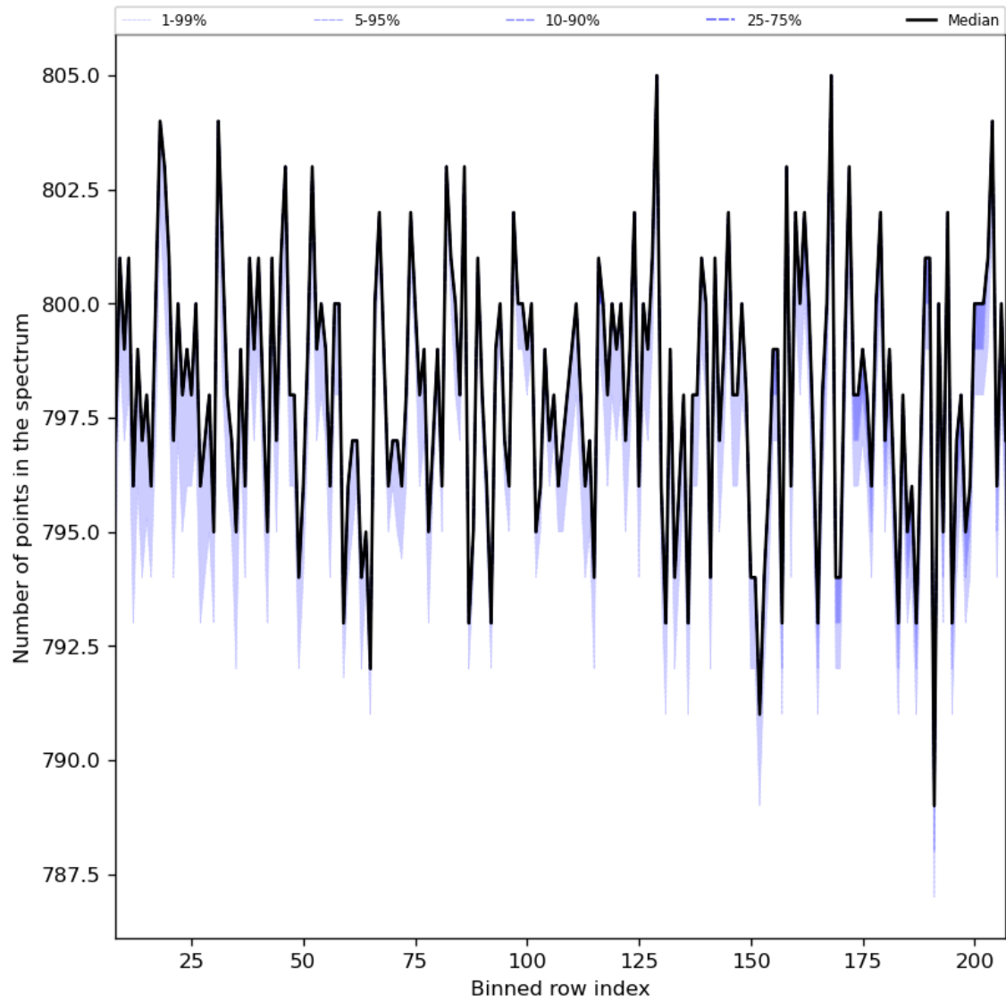
Figure 37: Along track statistics of “Number of points in the spectrum” for 2023-08-09 to 2023-08-11
