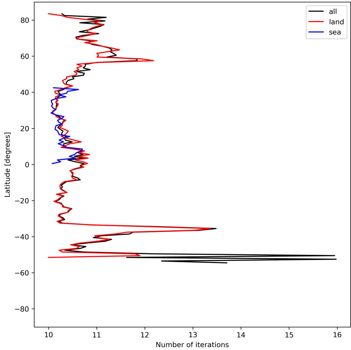
Figure 20: Zonal average of “Number of iterations” for 2023-08-09 to 2023-08-11.
