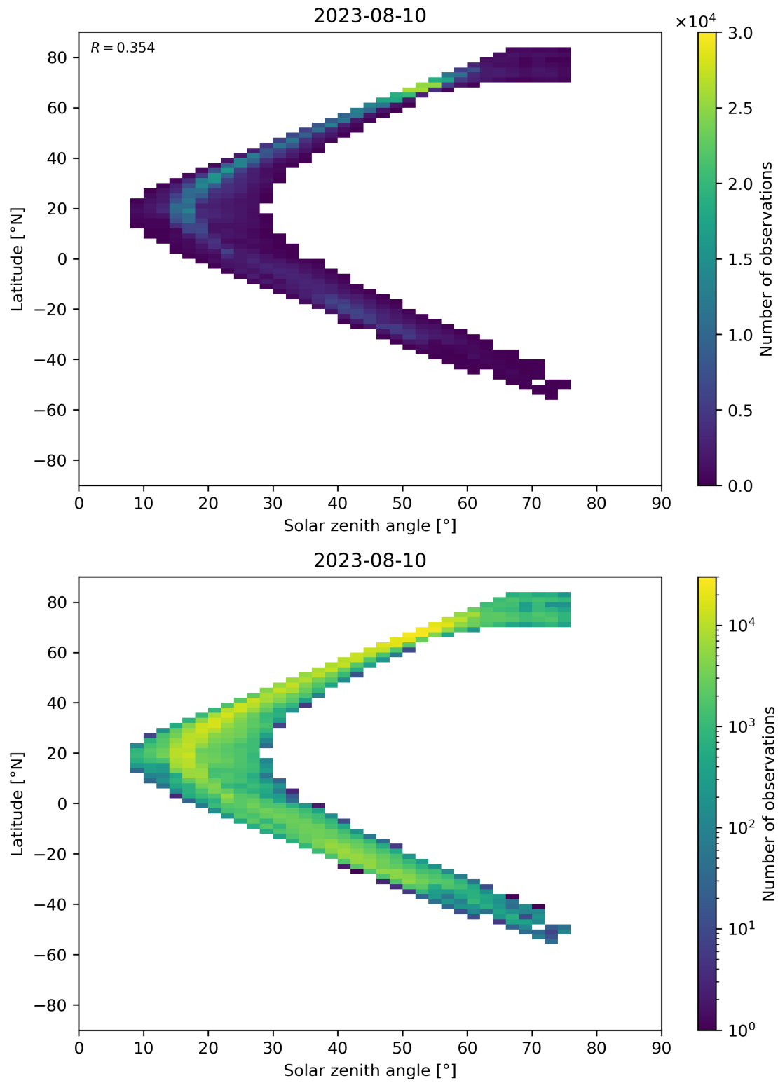
Figure 98: Scatter density plot of “Solar zenith angle” against “Latitude” for 2023-08-09 to 2023-08-11.
