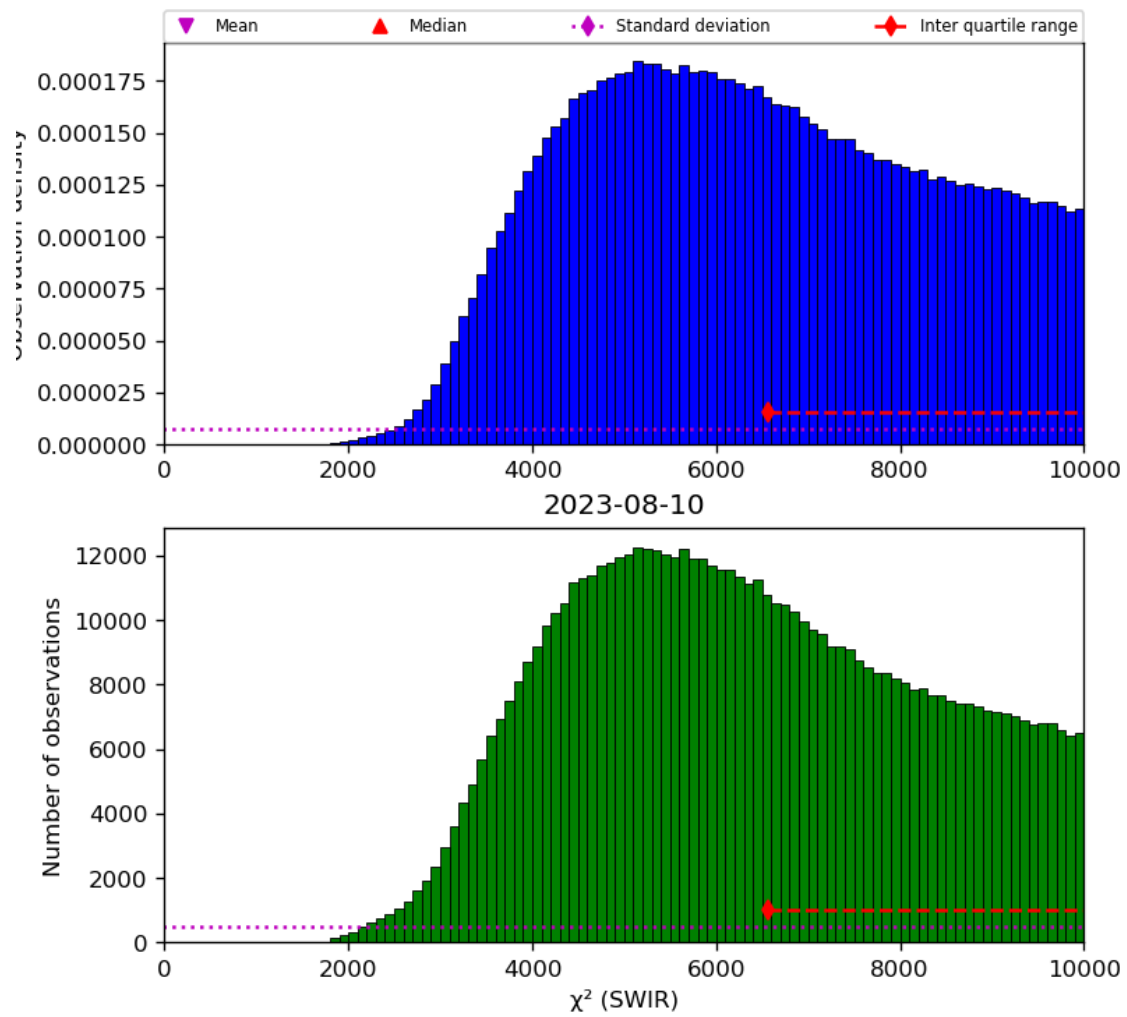
Figure 28: Histogram of “ \chi^2 (SWIR)” for 2023-08-09 to 2023-08-11
