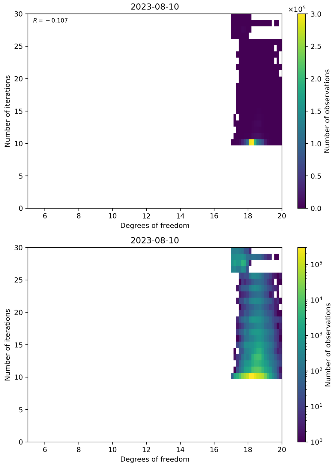
Figure 52: Scatter density plot of “Degrees of freedom” against “Number of iterations” for 2023-08-09 to 2023-08-11.
