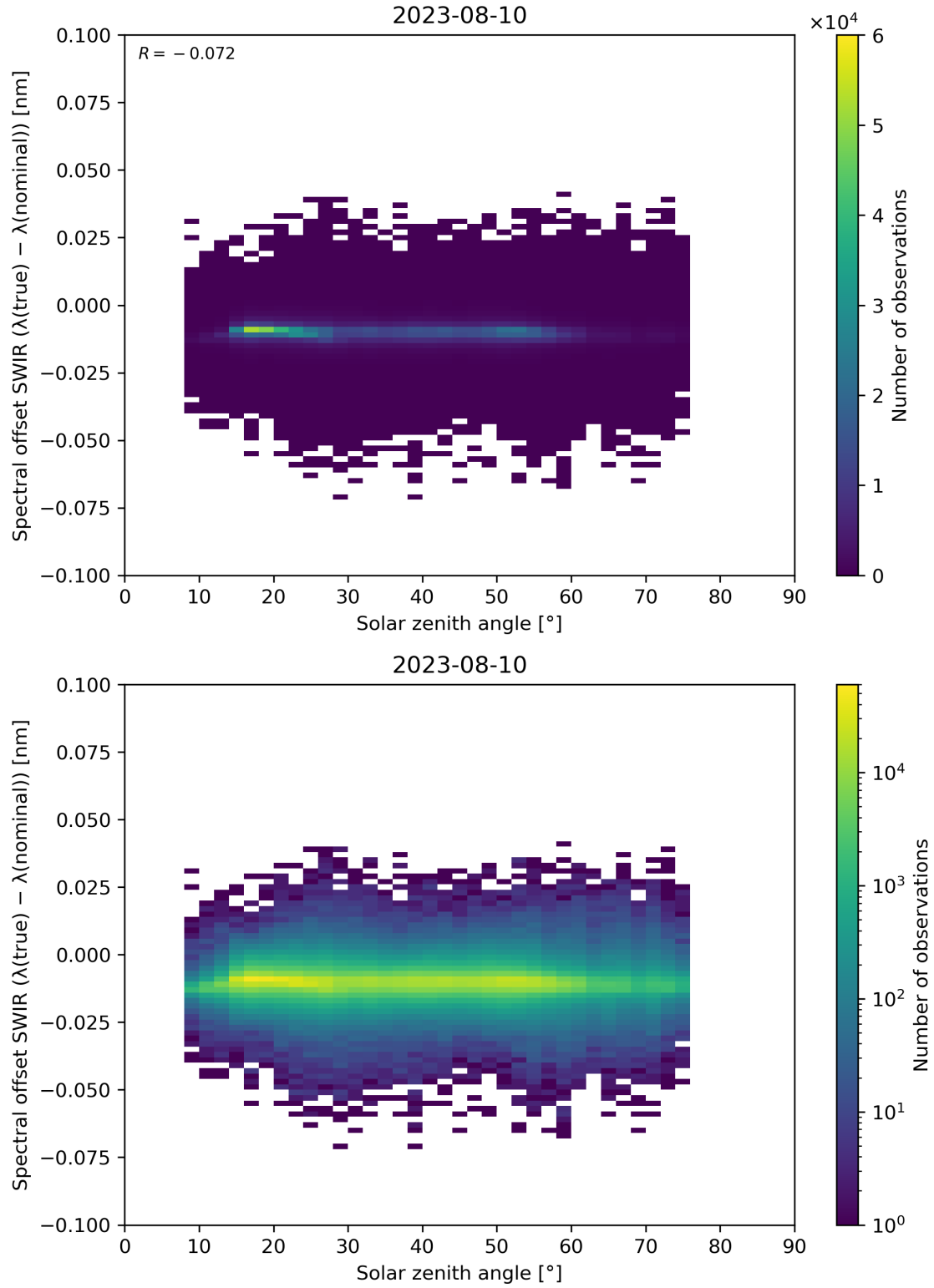
Figure 104: Scatter density plot of “Solar zenith angle” against “Spectral offset SWIR ( \lambda(\text{true}) - \lambda(\text{nominal}) )” for 2023-08-09 to 2023-08-11.
