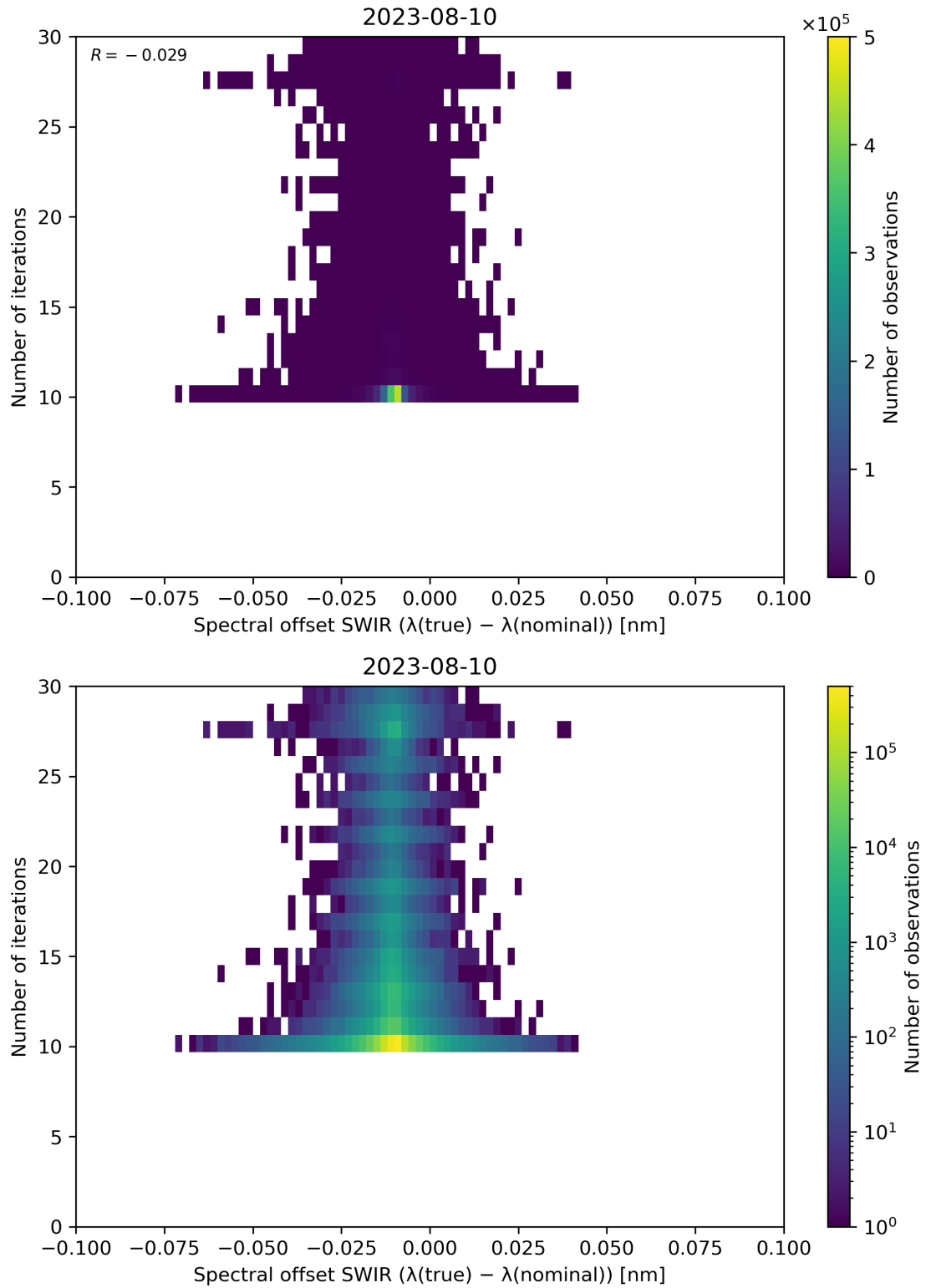
Figure 121: Scatter density plot of “Spectral offset SWIR ( \lambda(\text{true}) - \lambda(\text{nominal}) )” against “Number of iterations” for 2023-08-09 to 2023-08-11.
