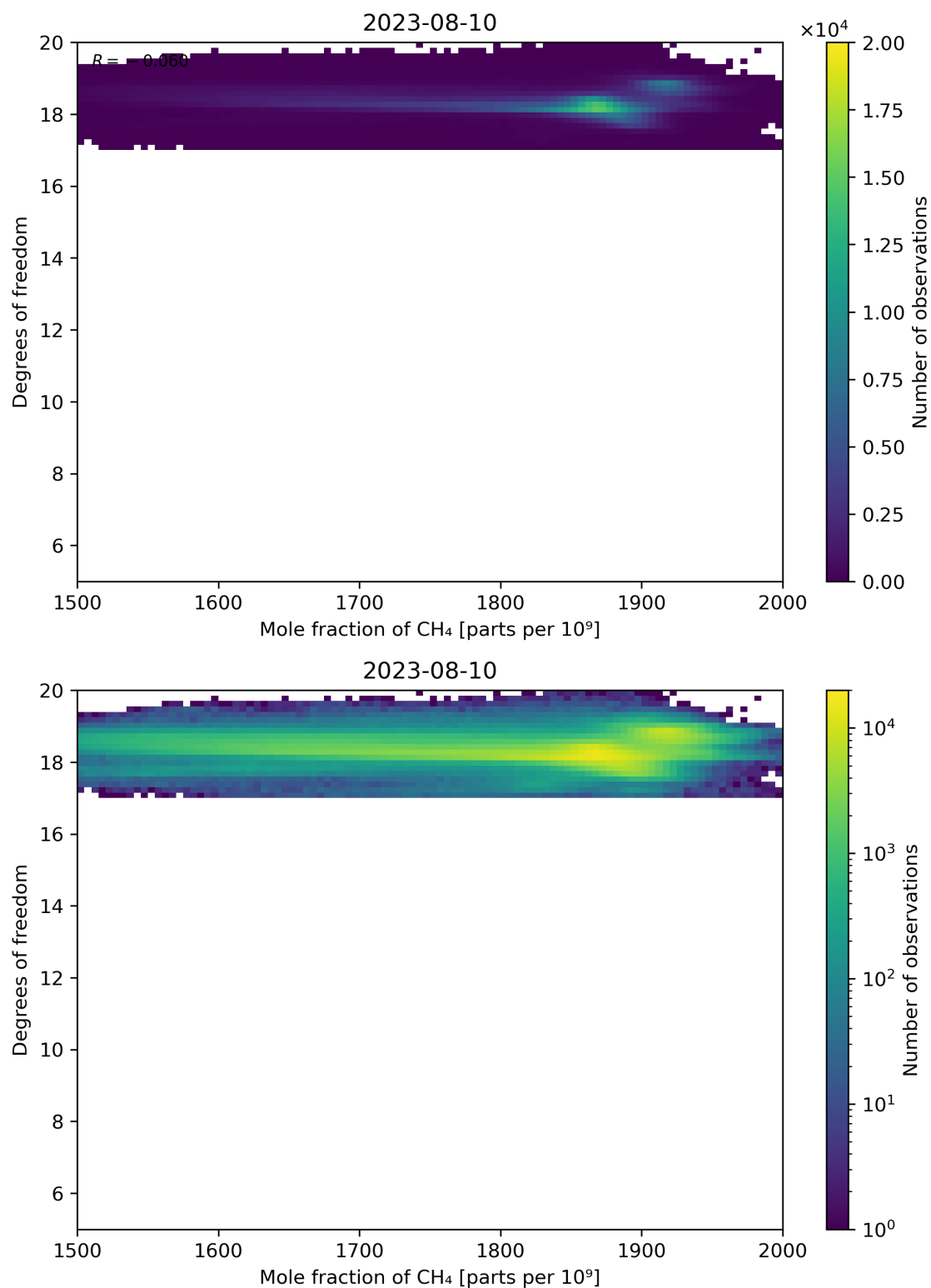
Figure 72: Scatter density plot of “Mole fraction of CH 4 ” against “Degrees of freedom” for 2023-08-09 to 2023-08-11.
