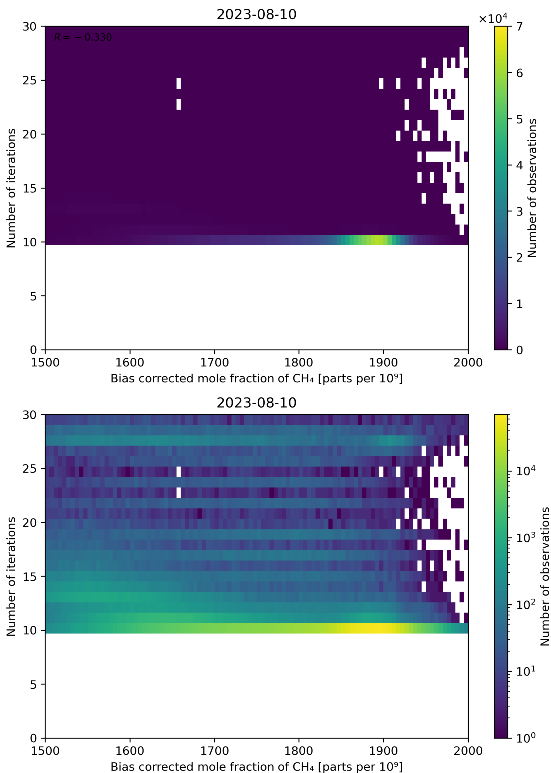
Figure 67: Scatter density plot of “Bias corrected mole fraction of CH 4 ” against “Number of iterations” for 2023-08-09 to 2023-08-11.
