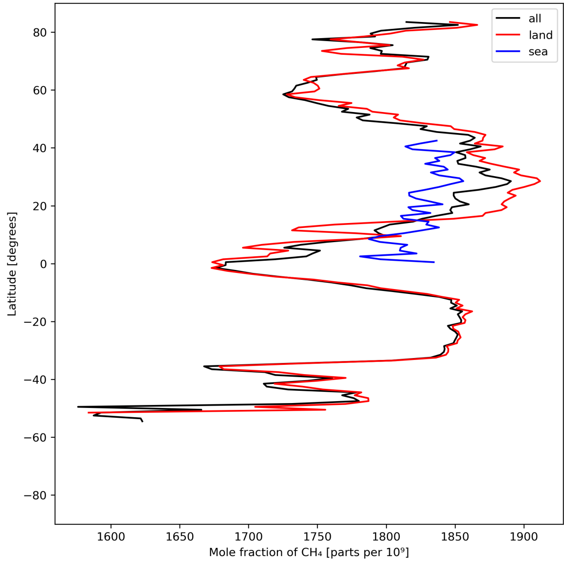
Figure 12: Zonal average of “Mole fraction of \text{CH}_4 ” for 2023-08-09 to 2023-08-11.
