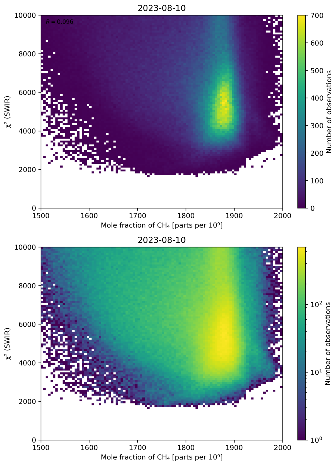
Figure 71: Scatter density plot of “Mole fraction of \text{CH}_4 ” against “ \chi^2 (SWIR)” for 2023-08-09 to 2023-08-11.
