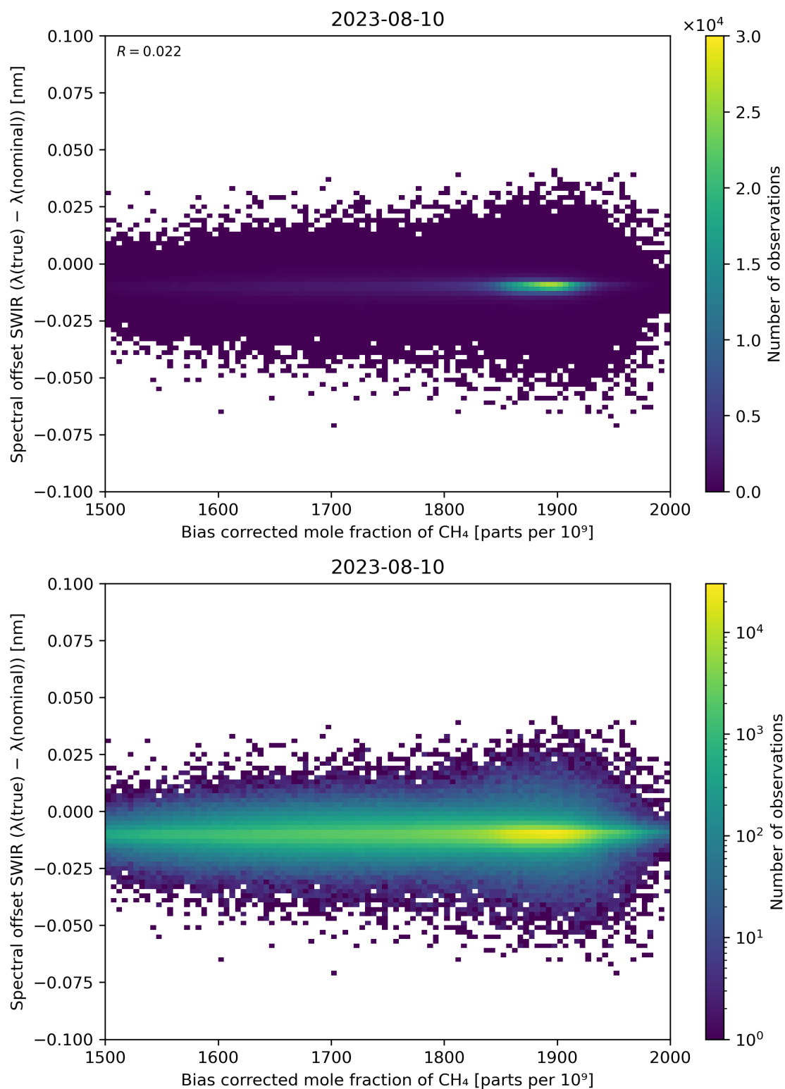
Figure 69: Scatter density plot of “Bias corrected mole fraction of \text{CH}_4 ” against “Spectral offset SWIR ( \lambda(\text{true}) - \lambda(\text{nominal}) )” for 2023-08-09 to 2023-08-11.
