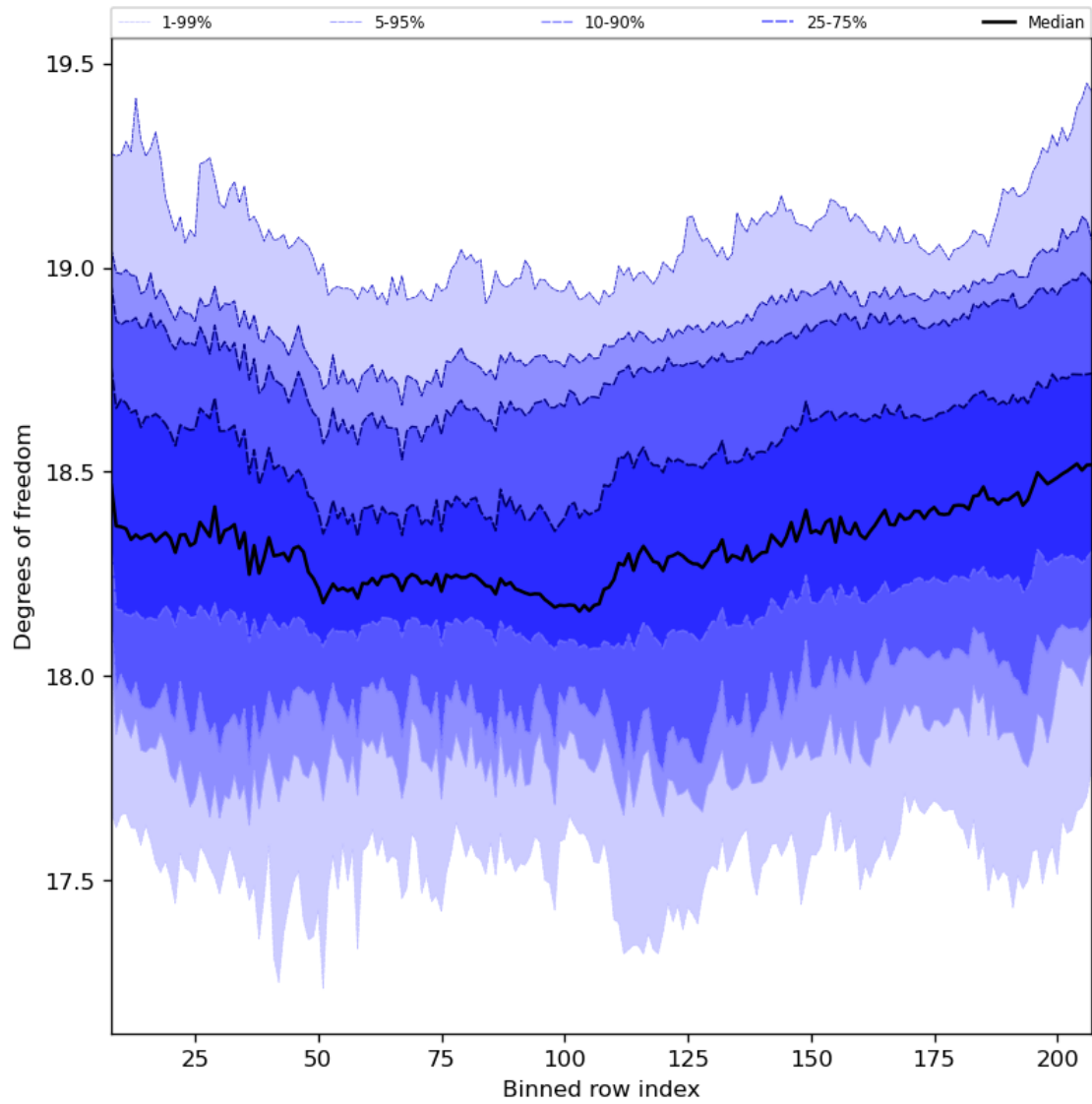
Figure 41: Along track statistics of “Degrees of freedom” for 2023-08-09 to 2023-08-11
