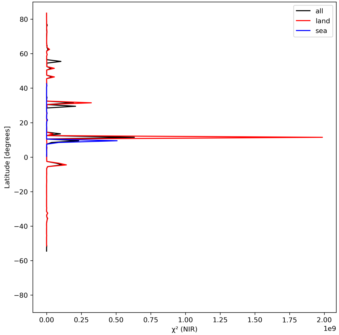
Figure 18: Zonal average of “ \chi^2 (NIR)” for 2023-08-09 to 2023-08-11.
