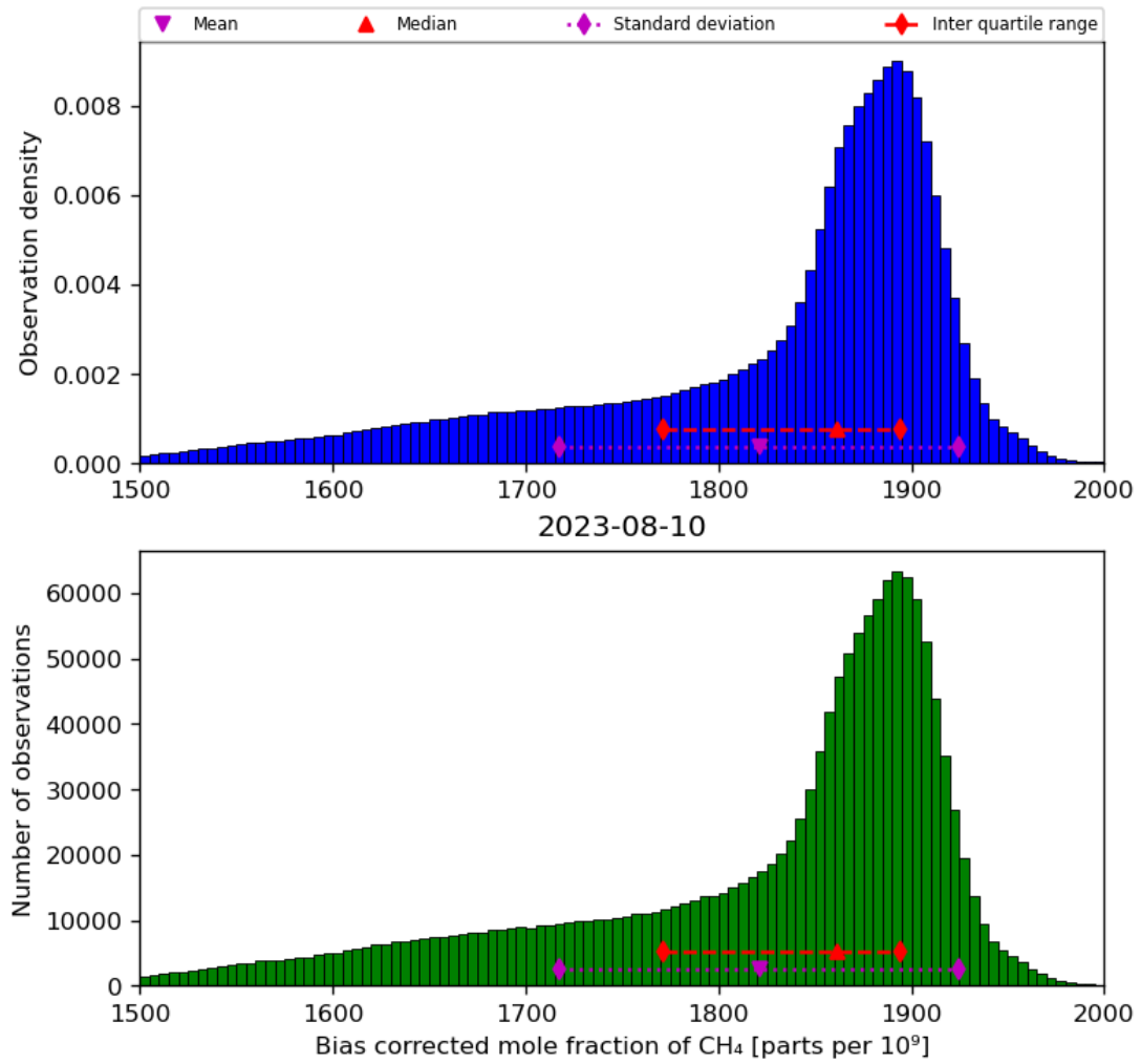
Figure 25: Histogram of “Bias corrected mole fraction of CH 4 ” for 2023-08-09 to 2023-08-11
