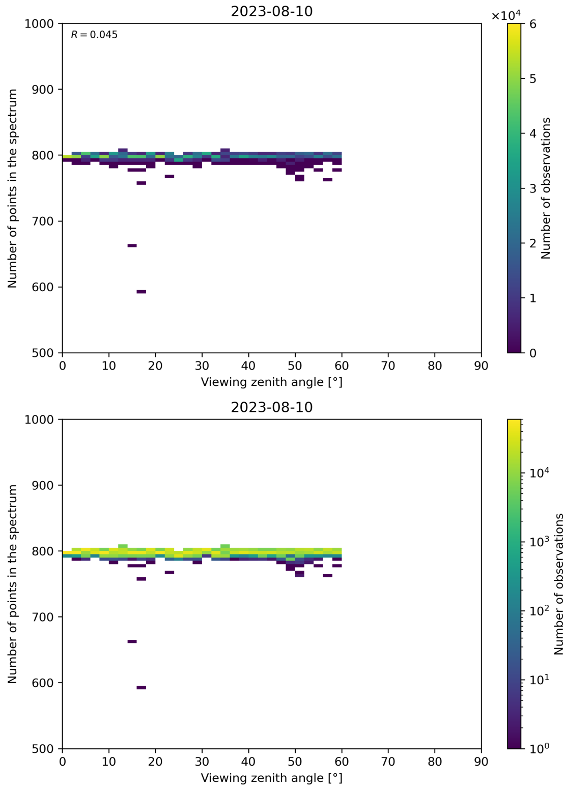
Figure 114: Scatter density plot of “Viewing zenith angle” against “Number of points in the spectrum” for 2023-08-09 to 2023-08-11.
