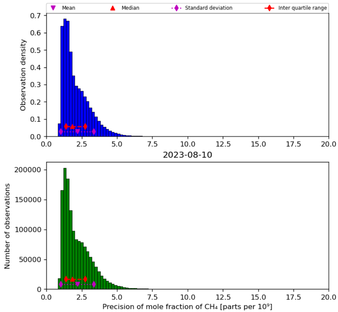
Figure 24: Histogram of “Precision of mole fraction of CH 4 ” for 2023-08-09 to 2023-08-11
