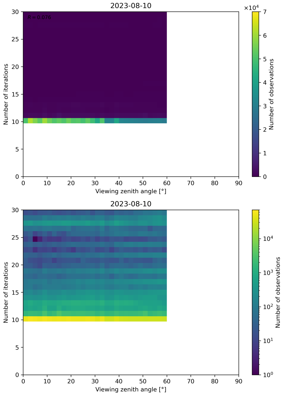
Figure 113: Scatter density plot of “Viewing zenith angle” against “Number of iterations” for 2023-08-09 to 2023-08-11.
