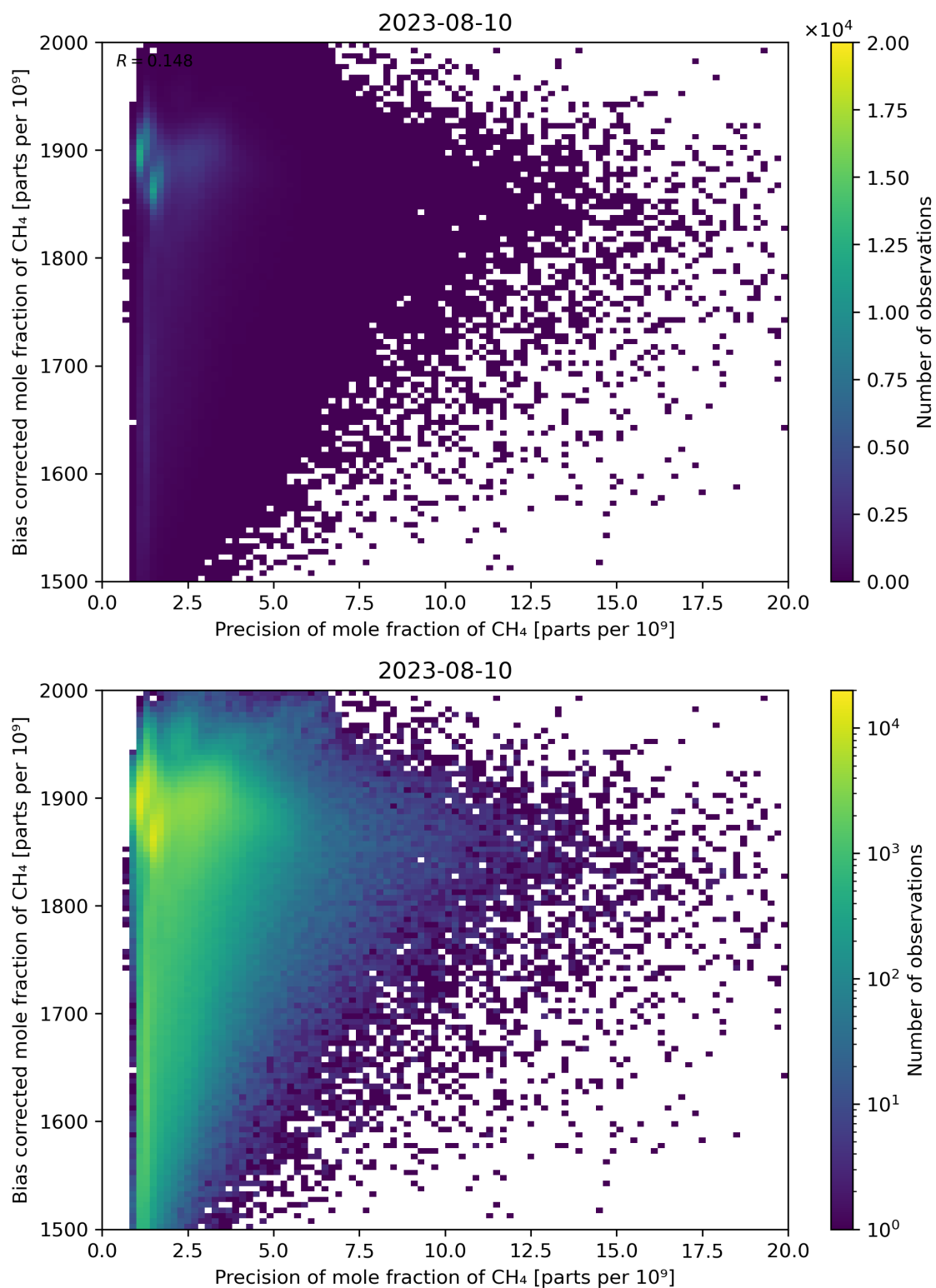
Figure 82: Scatter density plot of “Precision of mole fraction of \text{CH}_4 ” against “Bias corrected mole fraction of \text{CH}_4 ” for 2023-08-09 to 2023-08-11.
