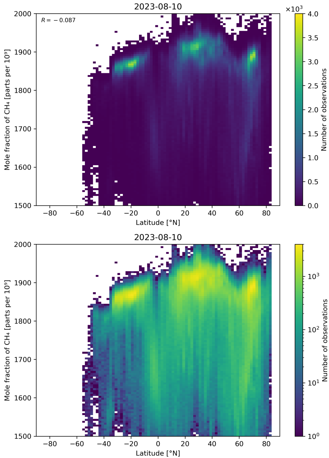
Figure 57: Scatter density plot of “Latitude” against “Mole fraction of CH 4 ” for 2023-08-09 to 2023-08-11.
