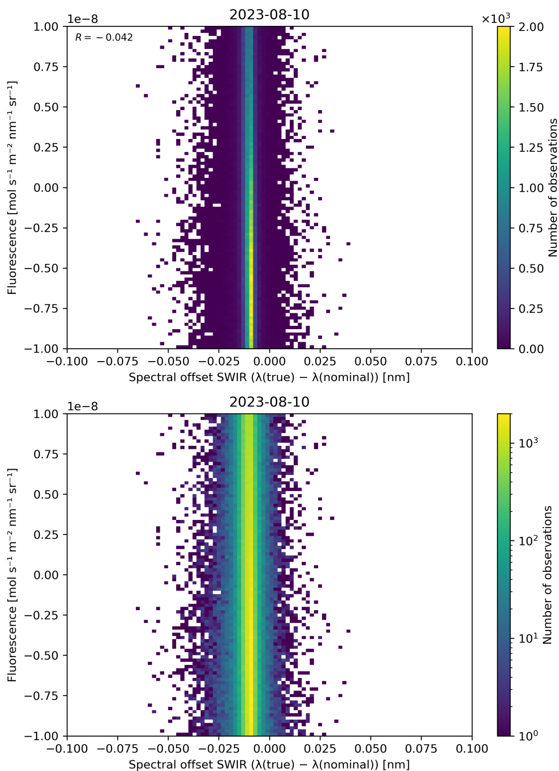
Figure 120: Scatter density plot of “Spectral offset SWIR ( \lambda(\text{true}) - \lambda(\text{nominal}) )” against “Fluorescence” for 2023-08-09 to 2023-08-11.
