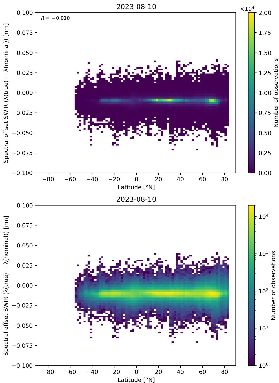
Figure 62: Scatter density plot of “Latitude” against “Spectral offset SWIR ( \lambda(\text{true}) - \lambda(\text{nominal}) )” for 2023-08-09 to 2023-08-11.
