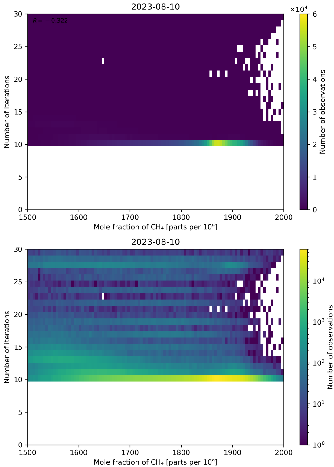
Figure 76: Scatter density plot of “Mole fraction of CH 4 ” against “Number of iterations” for 2023-08-09 to 2023-08-11.
