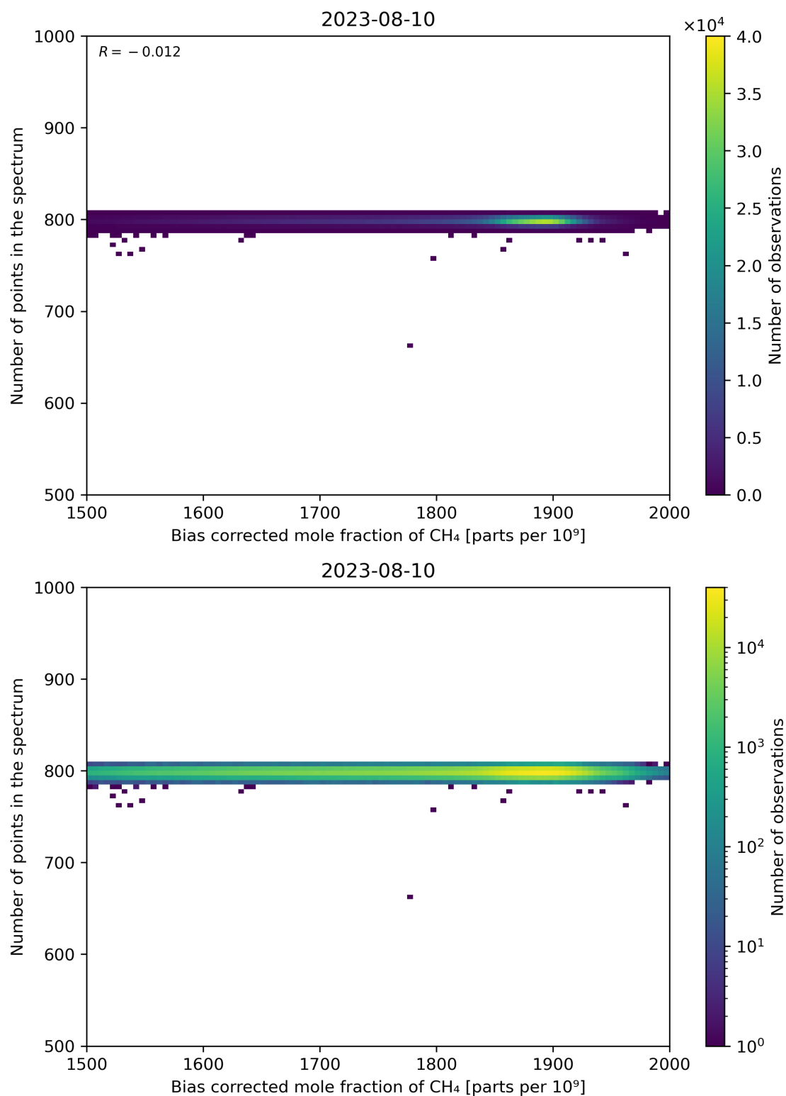
Figure 68: Scatter density plot of “Bias corrected mole fraction of CH 4 ” against “Number of points in the spectrum” for 2023-08-09 to 2023-08-11.
