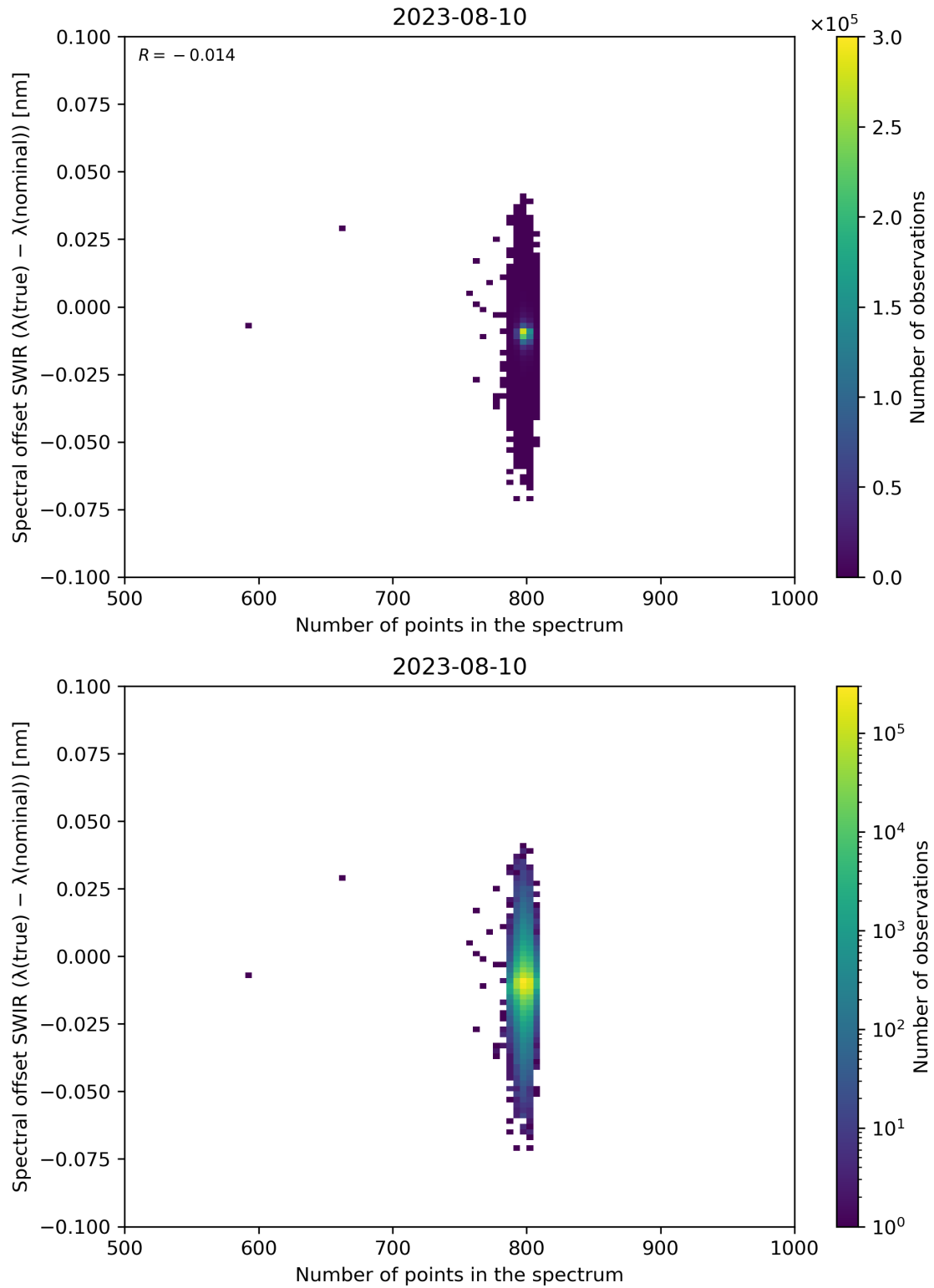
Figure 93: Scatter density plot of “Number of points in the spectrum” against “Spectral offset SWIR ( \lambda(\text{true}) - \lambda(\text{nominal}) )” for 2023-08-09 to 2023-08-11.
