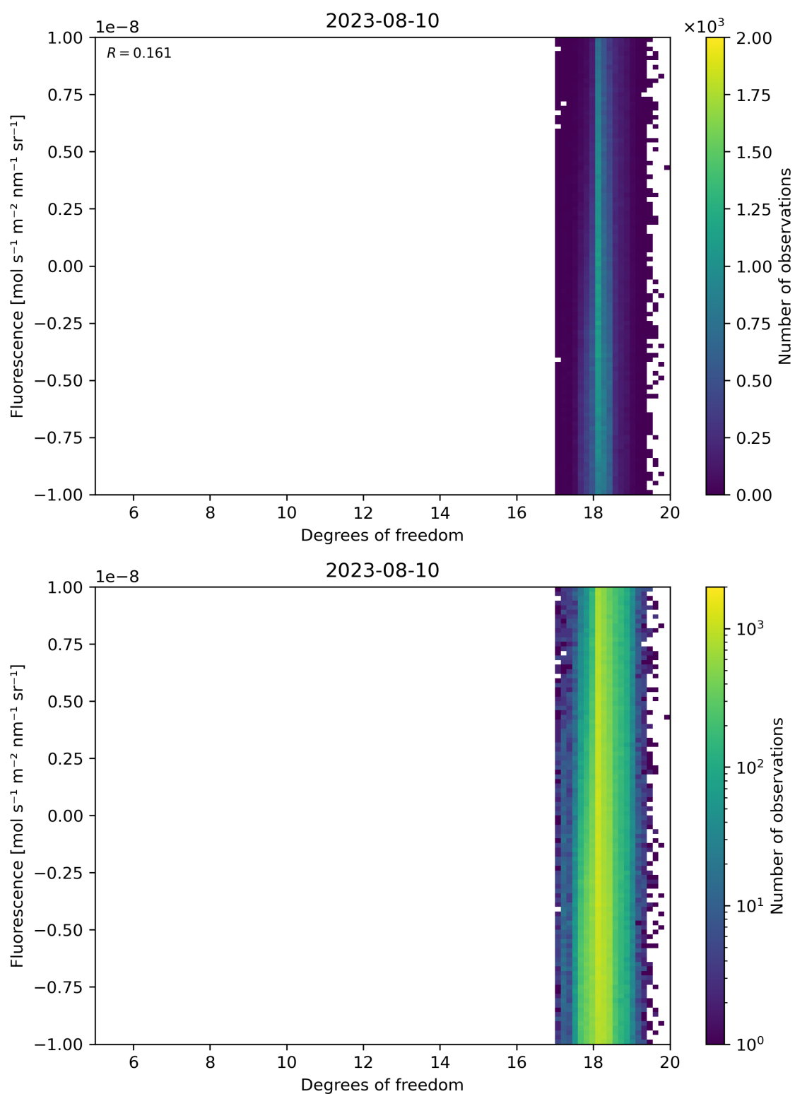
Figure 51: Scatter density plot of “Degrees of freedom” against “Fluorescence” for 2023-08-09 to 2023-08-11.
