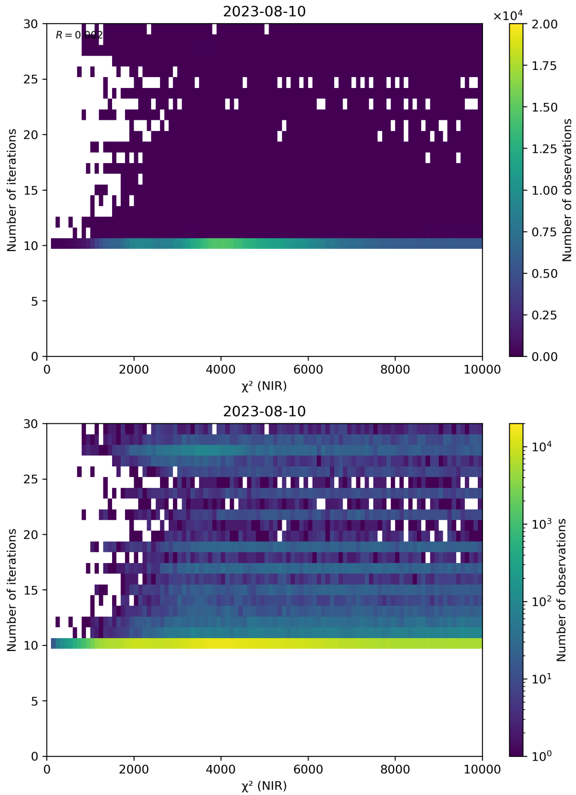
Figure 46: Scatter density plot of “ \chi^2 (NIR)” against “Number of iterations” for 2023-08-09 to 2023-08-11.
