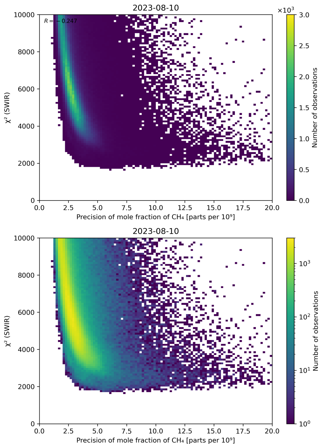
Figure 79: Scatter density plot of “Precision of mole fraction of \text{CH}_4 ” against “ \chi^2 (SWIR)” for 2023-08-09 to 2023-08-11.
