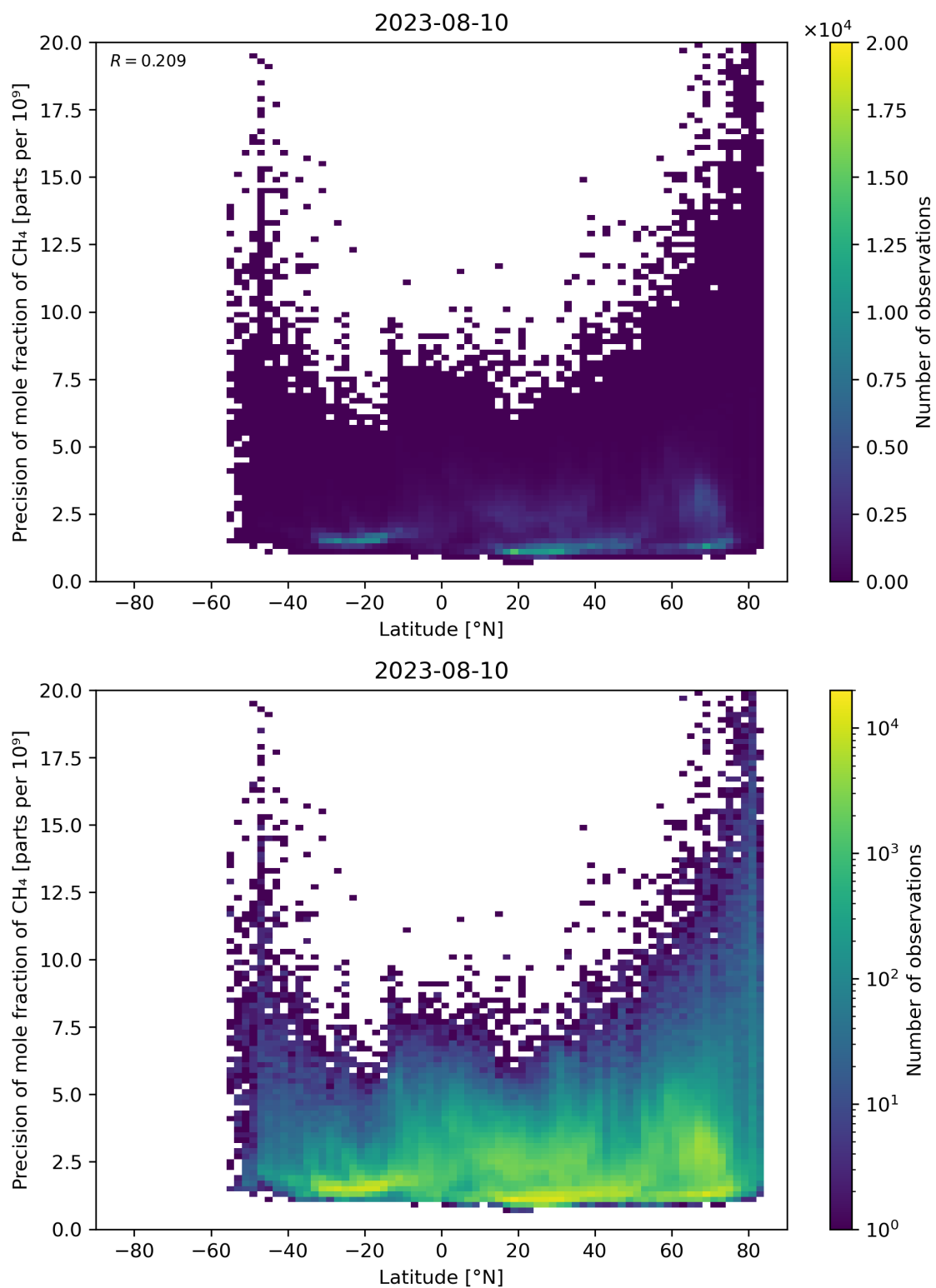
Figure 59: Scatter density plot of “Latitude” against “Precision of mole fraction of \text{CH}_4 ” for 2023-08-09 to 2023-08-11.
