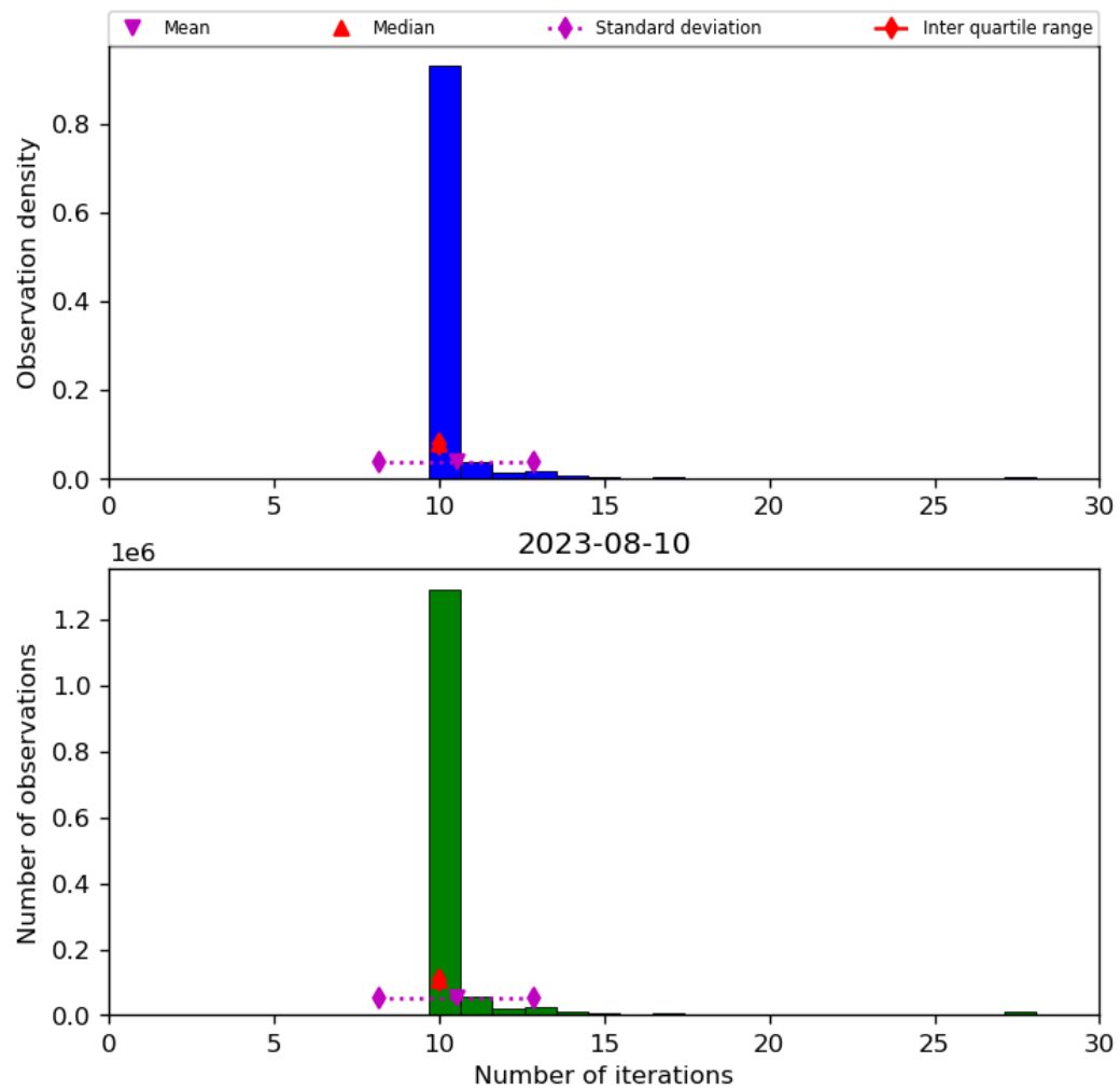
Figure 31: Histogram of “Number of iterations” for 2023-08-09 to 2023-08-11
