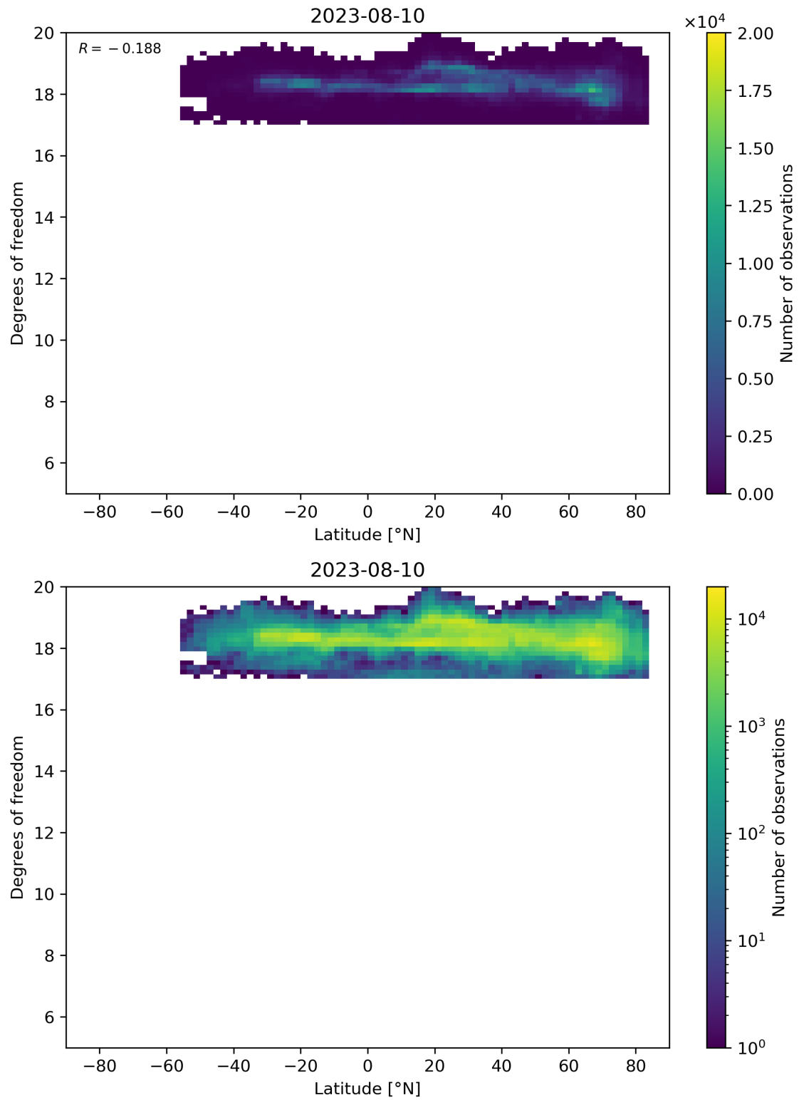
Figure 55: Scatter density plot of “Latitude” against “Degrees of freedom” for 2023-08-09 to 2023-08-11.
