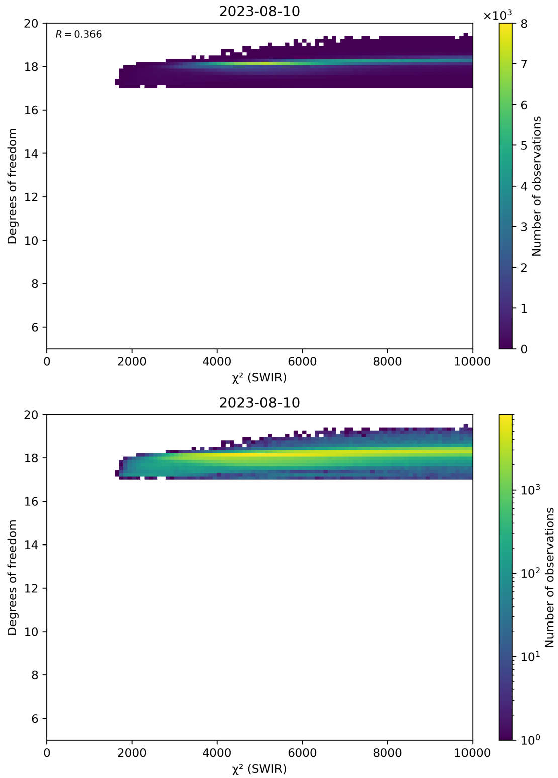
Figure 48: Scatter density plot of “ \chi^2 (SWIR)” against “Degrees of freedom” for 2023-08-09 to 2023-08-11.
