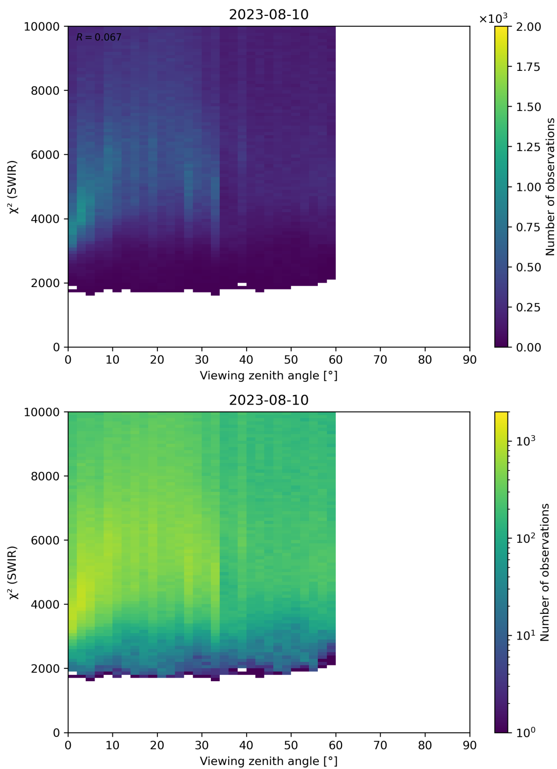
Figure 106: Scatter density plot of “Viewing zenith angle” against “ \chi^2 (SWIR)” for 2023-08-09 to 2023-08-11.
