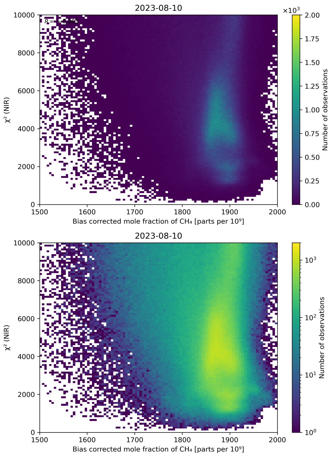
Figure 63: Scatter density plot of “Bias corrected mole fraction of CH 4 ” against “ \chi^2 (NIR)” for 2023-08-09 to 2023-08-11.
