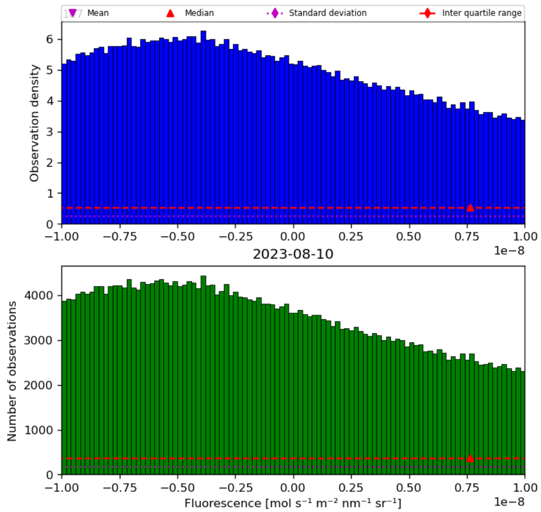
Figure 32: Histogram of “Fluorescence” for 2023-08-09 to 2023-08-11
