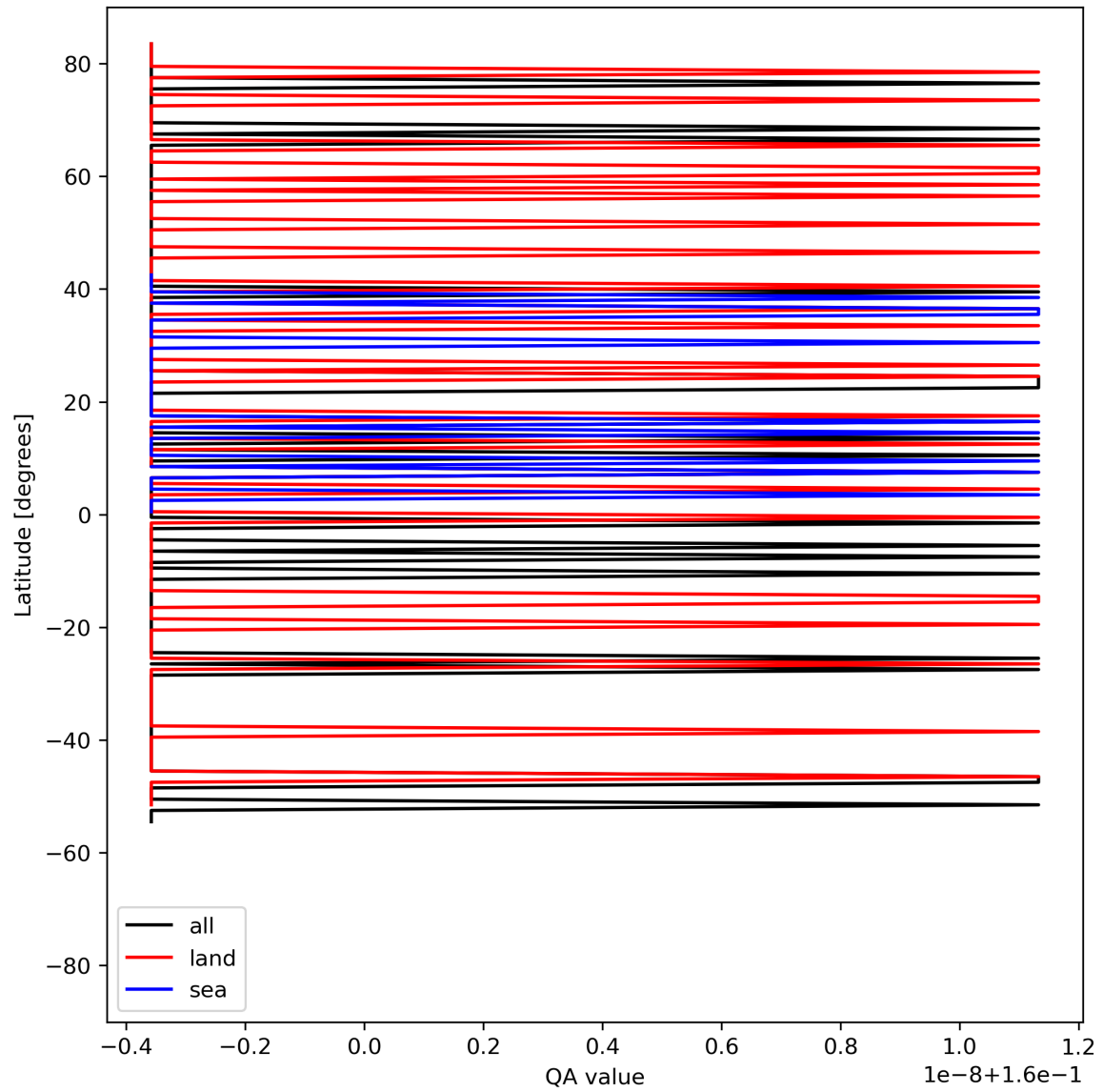
Figure 11: Zonal average of “QA value” for 2023-08-09 to 2023-08-11.
