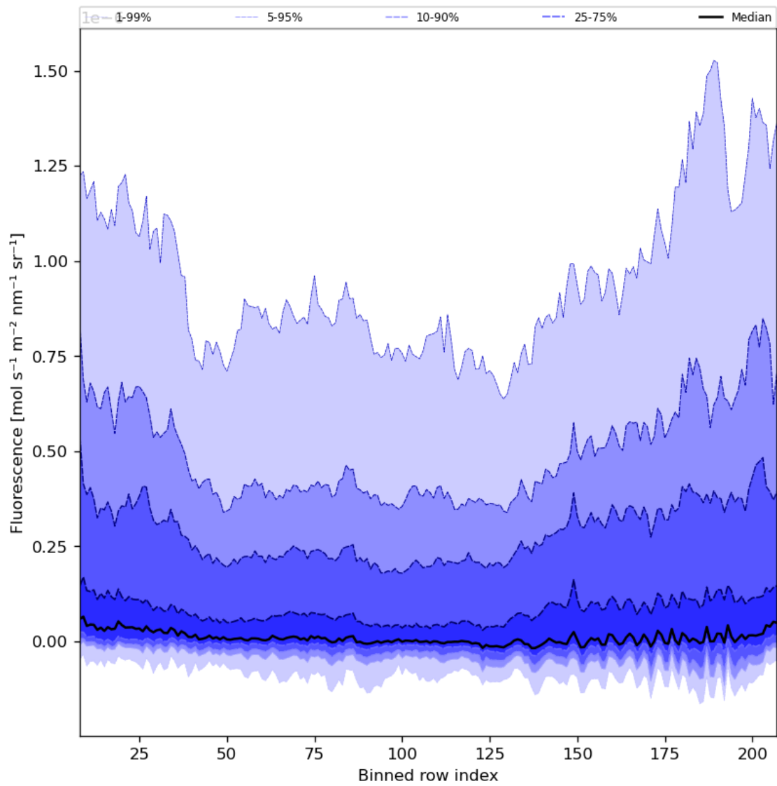
Figure 43: Along track statistics of “Fluorescence” for 2023-08-09 to 2023-08-11
