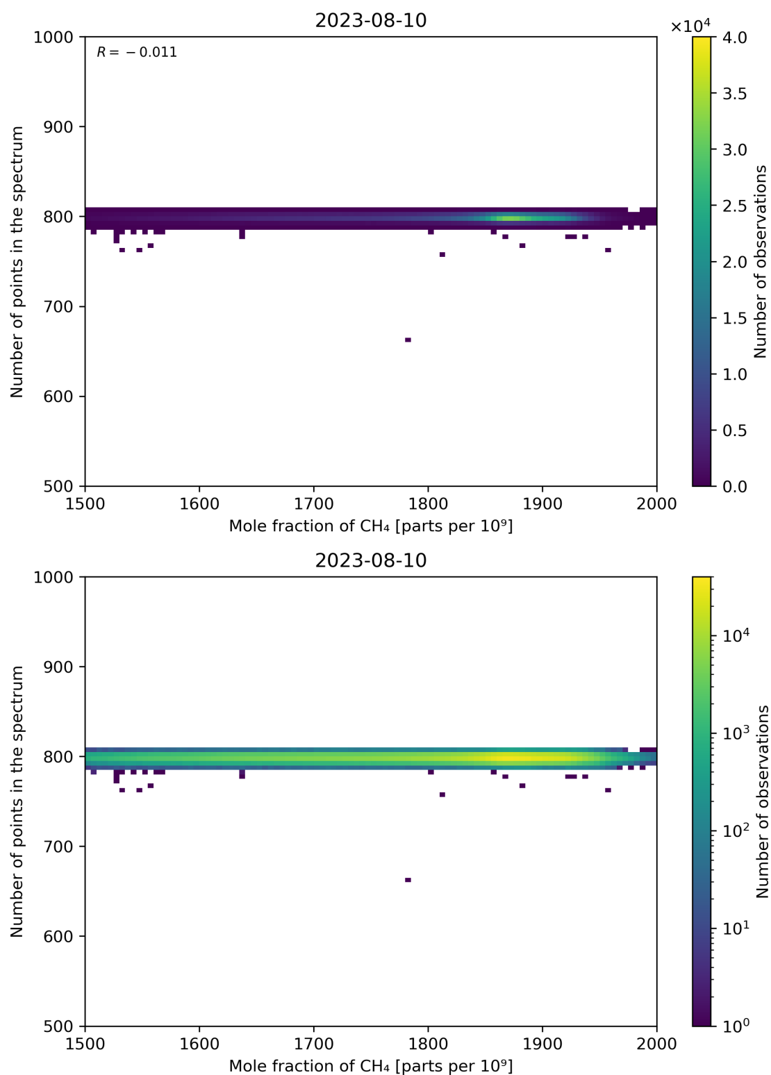
Figure 77: Scatter density plot of “Mole fraction of CH 4 ” against “Number of points in the spectrum” for 2023-08-09 to 2023-08-11.
