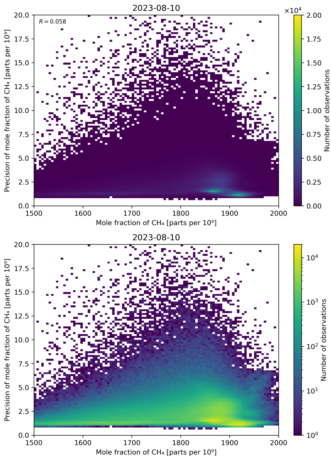
Figure 75: Scatter density plot of “Mole fraction of CH 4 ” against “Precision of mole fraction of CH 4 ” for 2023-08-09 to 2023-08-11.
