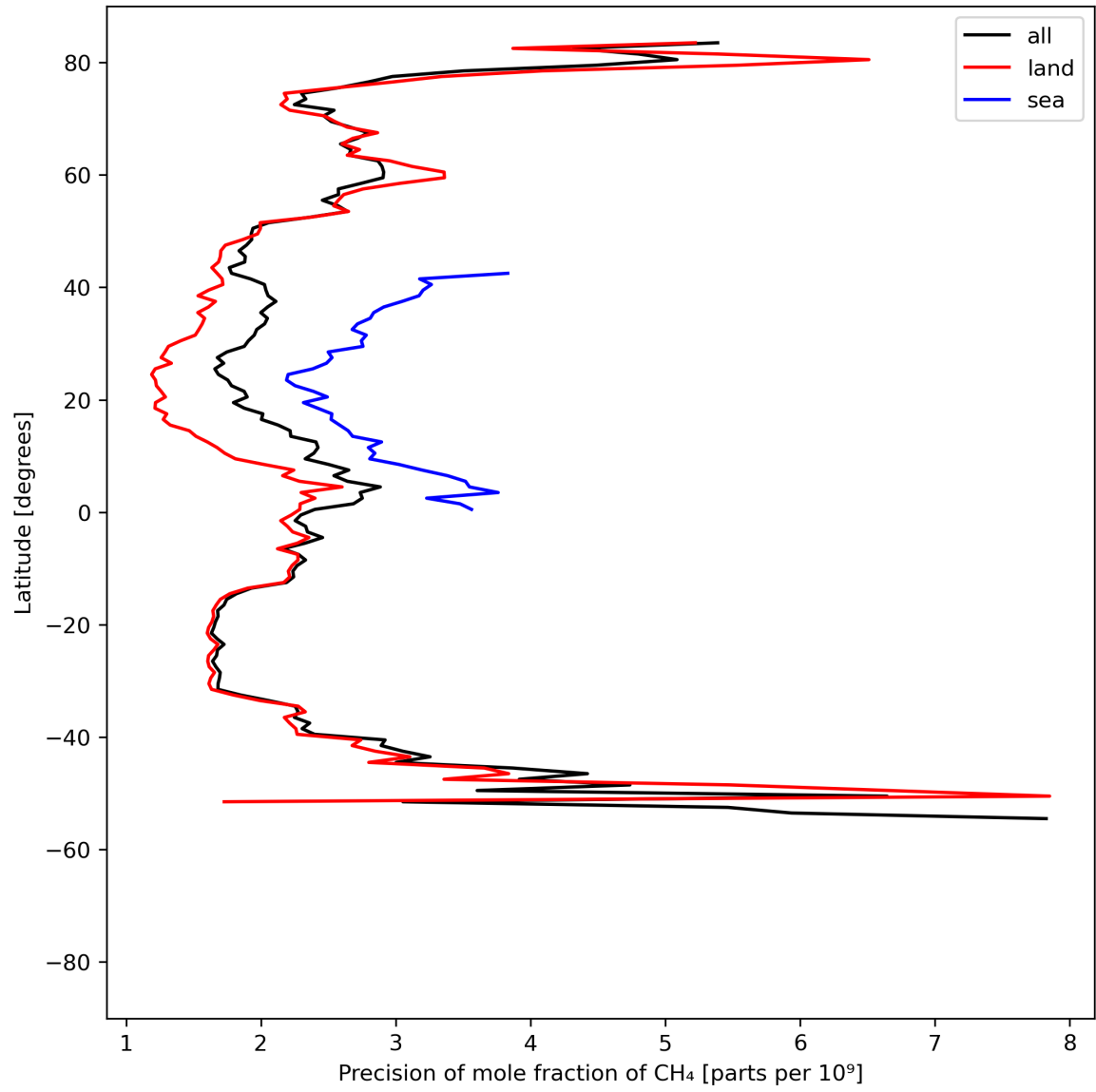
Figure 13: Zonal average of “Precision of mole fraction of CH 4 ” for 2023-08-09 to 2023-08-11.
