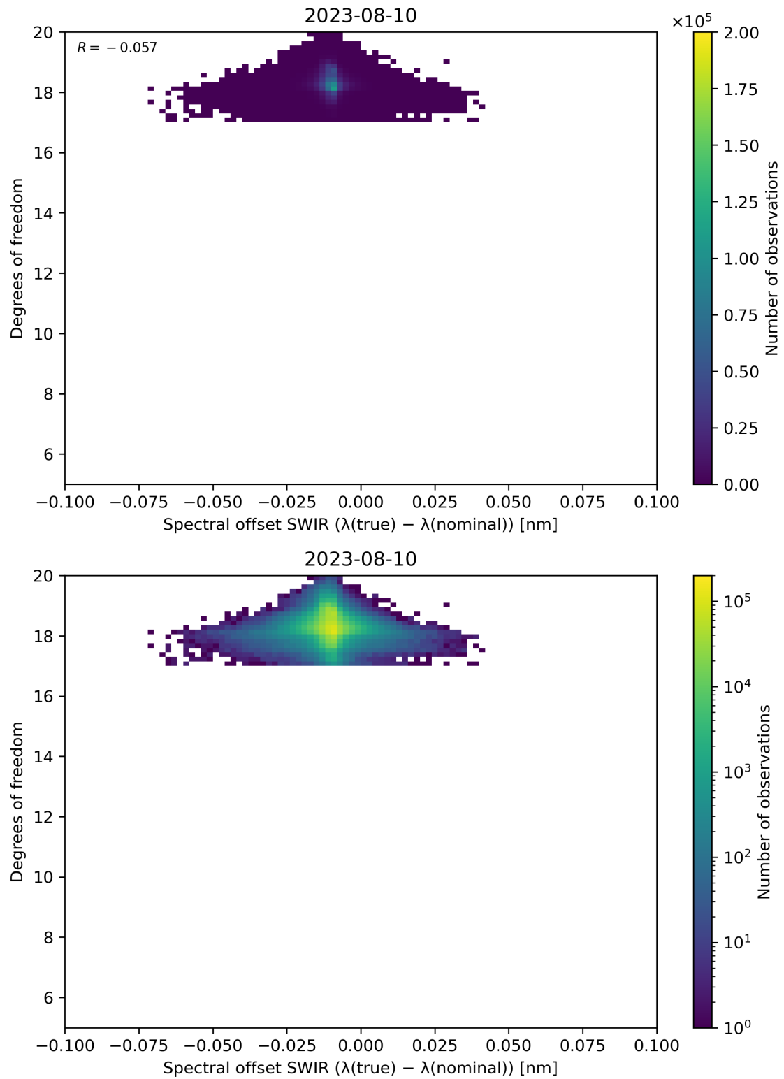
Figure 119: Scatter density plot of “Spectral offset SWIR ( \lambda(\text{true}) - \lambda(\text{nominal}) )” against “Degrees of freedom” for 2023-08-09 to 2023-08-11.
