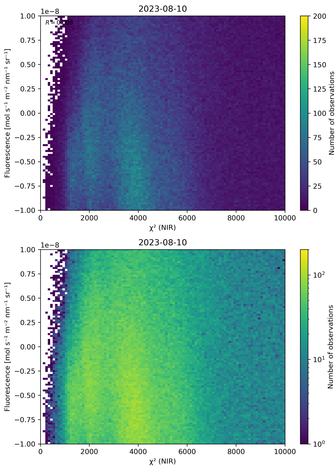
Figure 45: Scatter density plot of “ \chi^2 (NIR)” against “Fluorescence” for 2023-08-09 to 2023-08-11.
