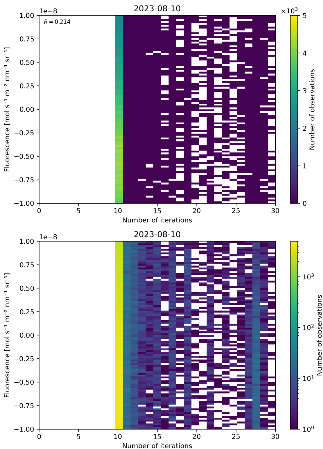
Figure 87: Scatter density plot of “Number of iterations” against “Fluorescence” for 2023-08-09 to 2023-08-11.
