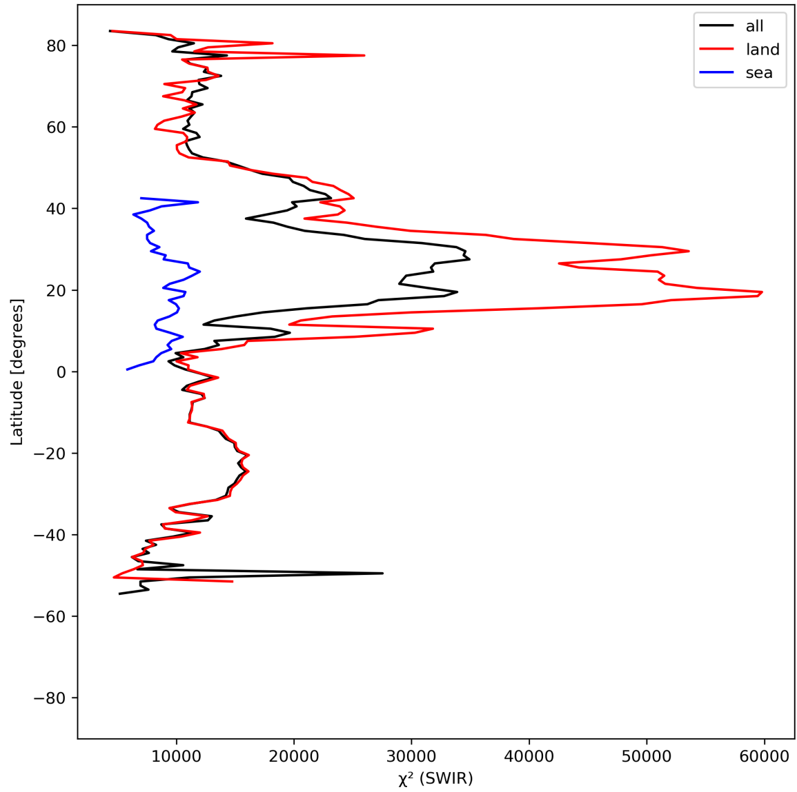
Figure 17: Zonal average of “ \chi^2 (SWIR)” for 2023-08-09 to 2023-08-11.
