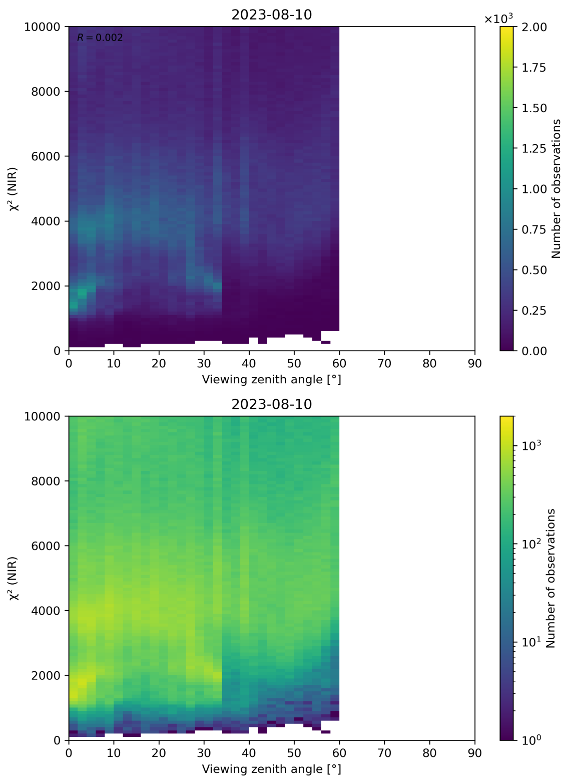
Figure 105: Scatter density plot of “Viewing zenith angle” against “ \chi^2 (NIR)” for 2023-08-09 to 2023-08-11.
