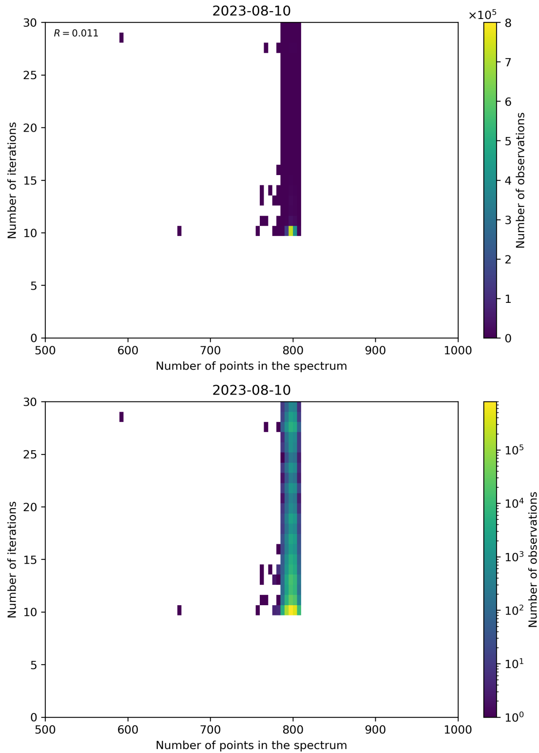
Figure 92: Scatter density plot of “Number of points in the spectrum” against “Number of iterations” for 2023-08-09 to 2023-08-11.
