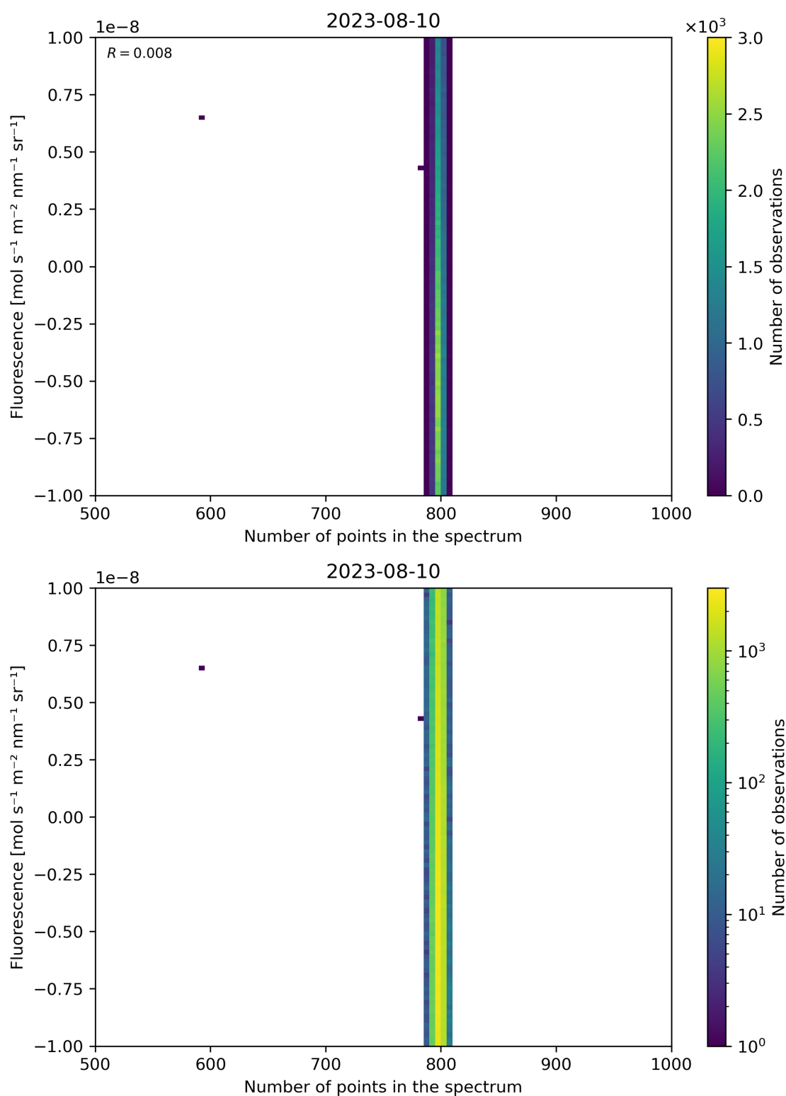
Figure 91: Scatter density plot of “Number of points in the spectrum” against “Fluorescence” for 2023-08-09 to 2023-08-11.
