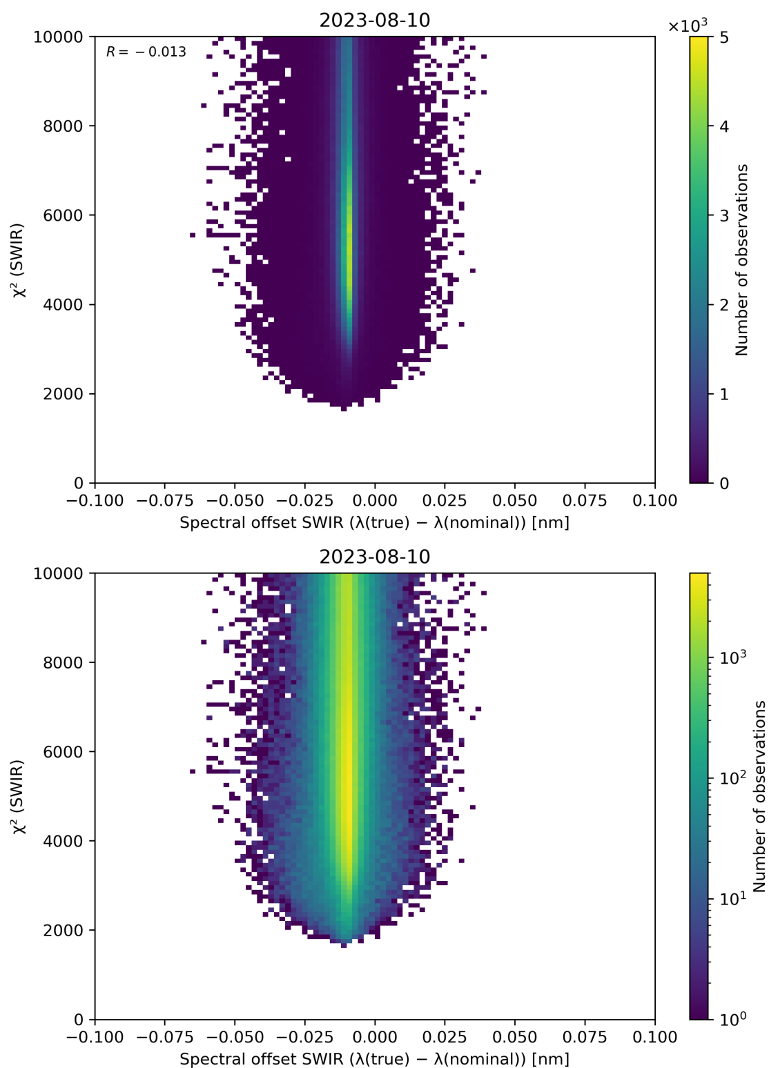
Figure 118: Scatter density plot of “Spectral offset SWIR ( \lambda(\text{true}) - \lambda(\text{nominal}) )” against “ \chi^2 (SWIR)” for 2023-08-09 to 2023-08-11.
