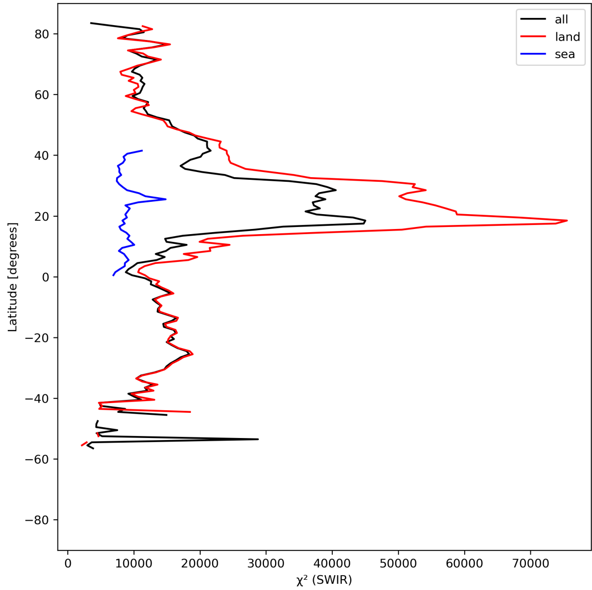
Figure 17: Zonal average of “ \chi^2 (SWIR)” for 2023-08-11 to 2023-08-13.
