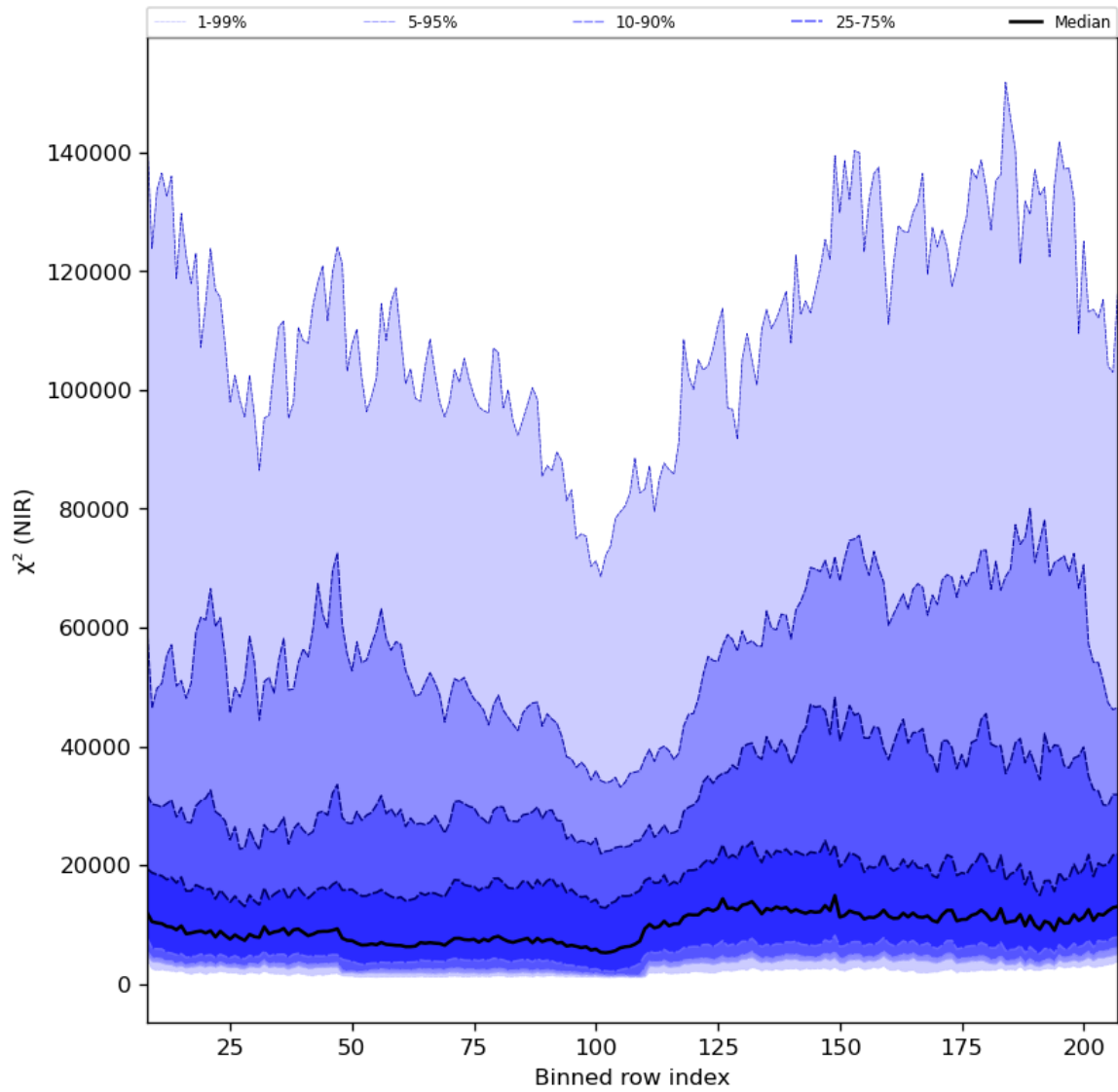
Figure 40: Along track statistics of “ \chi^2 (NIR)” for 2023-08-11 to 2023-08-13
