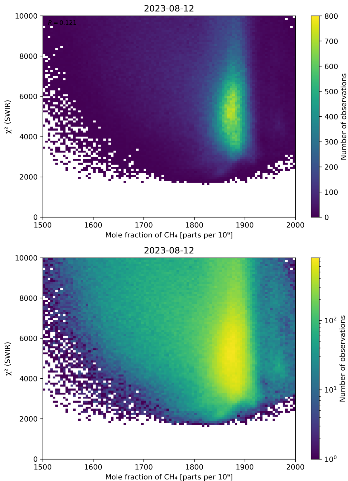
Figure 71: Scatter density plot of “Mole fraction of CH 4 ” against “ \chi^2 (SWIR)” for 2023-08-11 to 2023-08-13.
