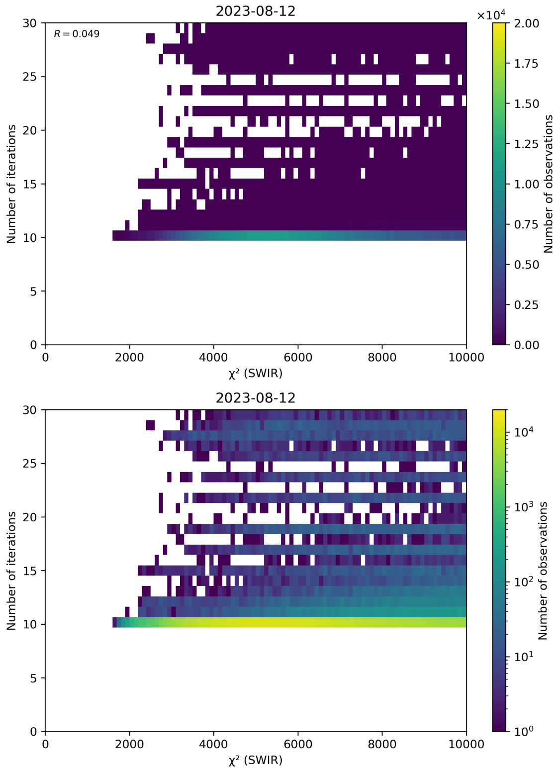
Figure 50: Scatter density plot of “ \chi^2 (SWIR)” against “Number of iterations” for 2023-08-11 to 2023-08-13.
