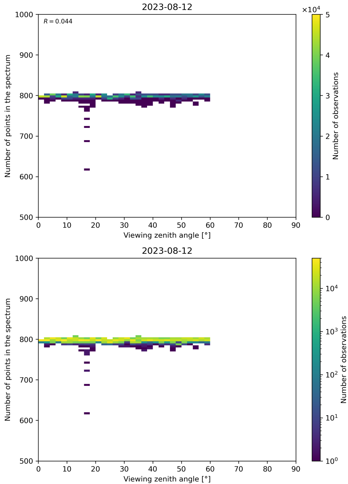
Figure 114: Scatter density plot of “Viewing zenith angle” against “Number of points in the spectrum” for 2023-08-11 to 2023-08-13.
