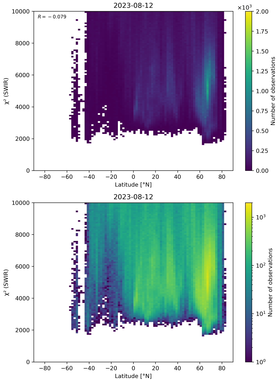
Figure 54: Scatter density plot of “Latitude” against “ \chi^2 (SWIR)” for 2023-08-11 to 2023-08-13.
