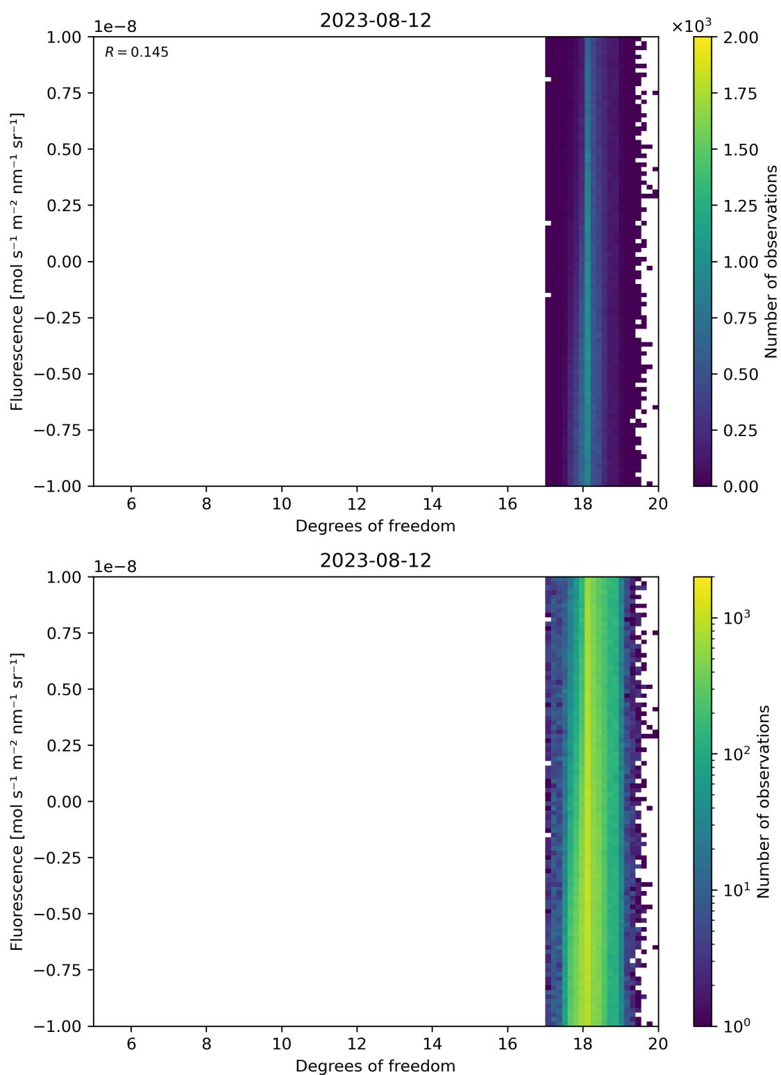
Figure 51: Scatter density plot of “Degrees of freedom” against “Fluorescence” for 2023-08-11 to 2023-08-13.
