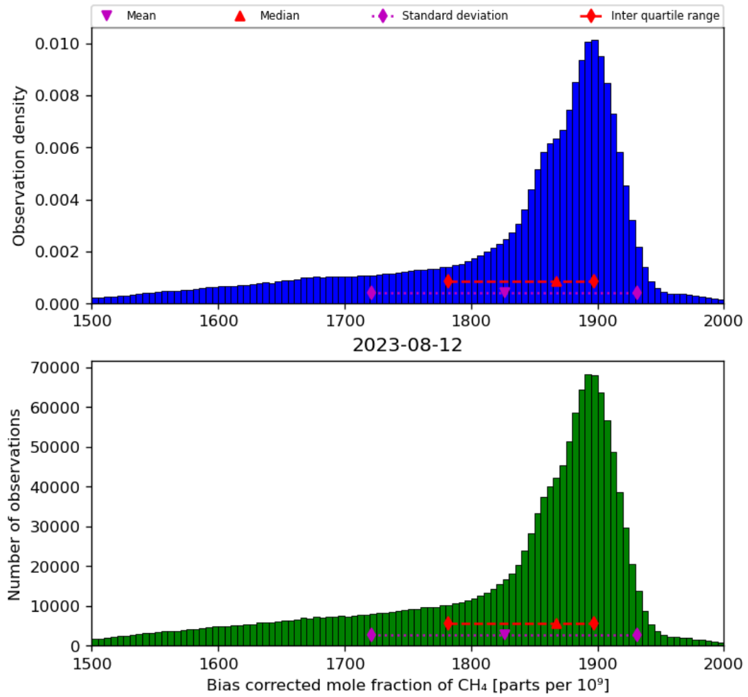
Figure 25: Histogram of “Bias corrected mole fraction of CH 4 ” for 2023-08-11 to 2023-08-13
