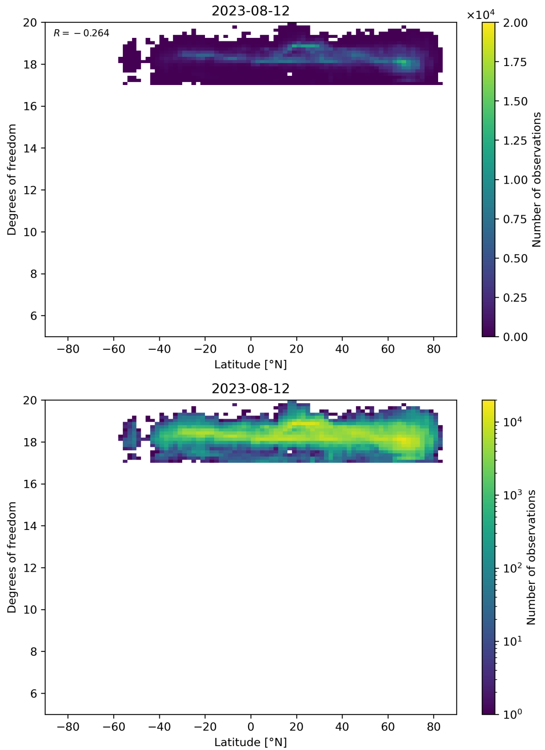
Figure 55: Scatter density plot of “Latitude” against “Degrees of freedom” for 2023-08-11 to 2023-08-13.
