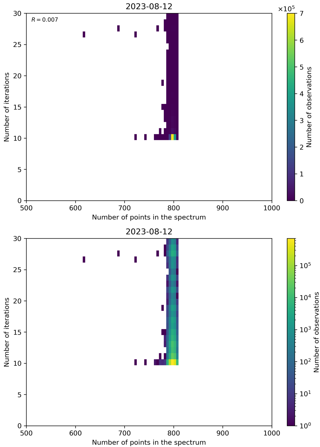
Figure 92: Scatter density plot of “Number of points in the spectrum” against “Number of iterations” for 2023-08-11 to 2023-08-13.
