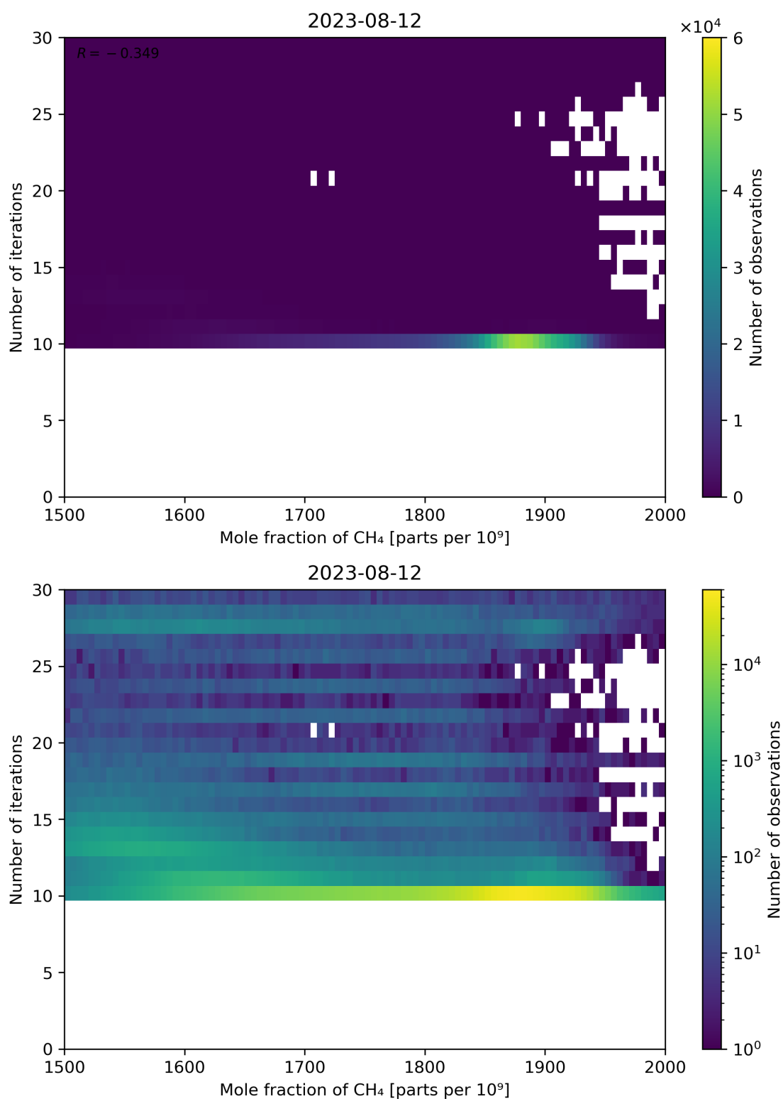
Figure 76: Scatter density plot of “Mole fraction of CH 4 ” against “Number of iterations” for 2023-08-11 to 2023-08-13.
