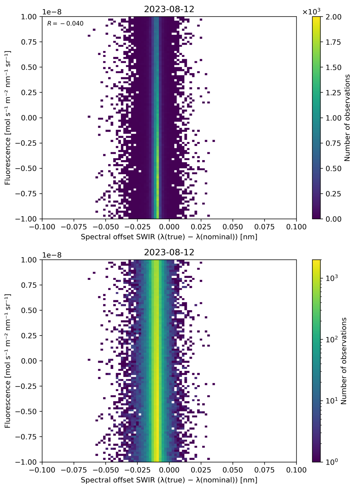
Figure 120: Scatter density plot of “Spectral offset SWIR ( \lambda(\text{true}) - \lambda(\text{nominal}) )” against “Fluorescence” for 2023-08-11 to 2023-08-13.
