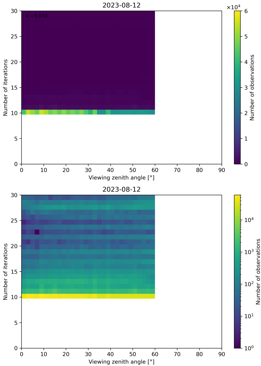
Figure 113: Scatter density plot of “Viewing zenith angle” against “Number of iterations” for 2023-08-11 to 2023-08-13.
