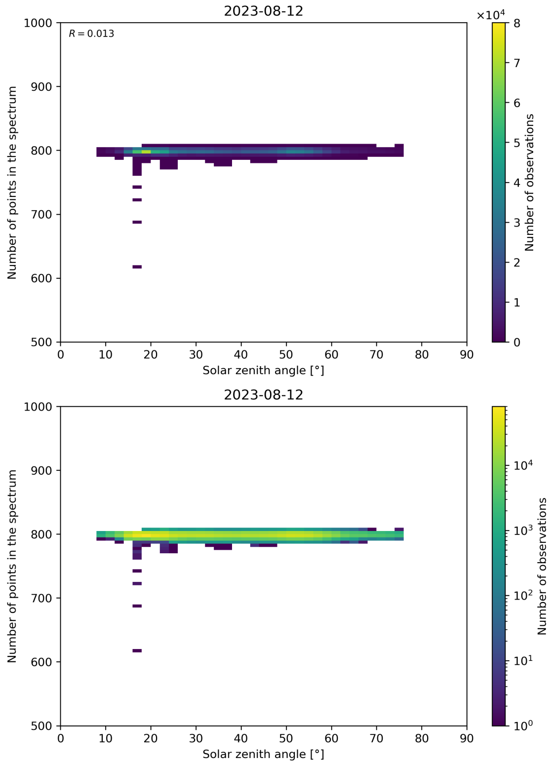
Figure 103: Scatter density plot of “Solar zenith angle” against “Number of points in the spectrum” for 2023-08-11 to 2023-08-13.
