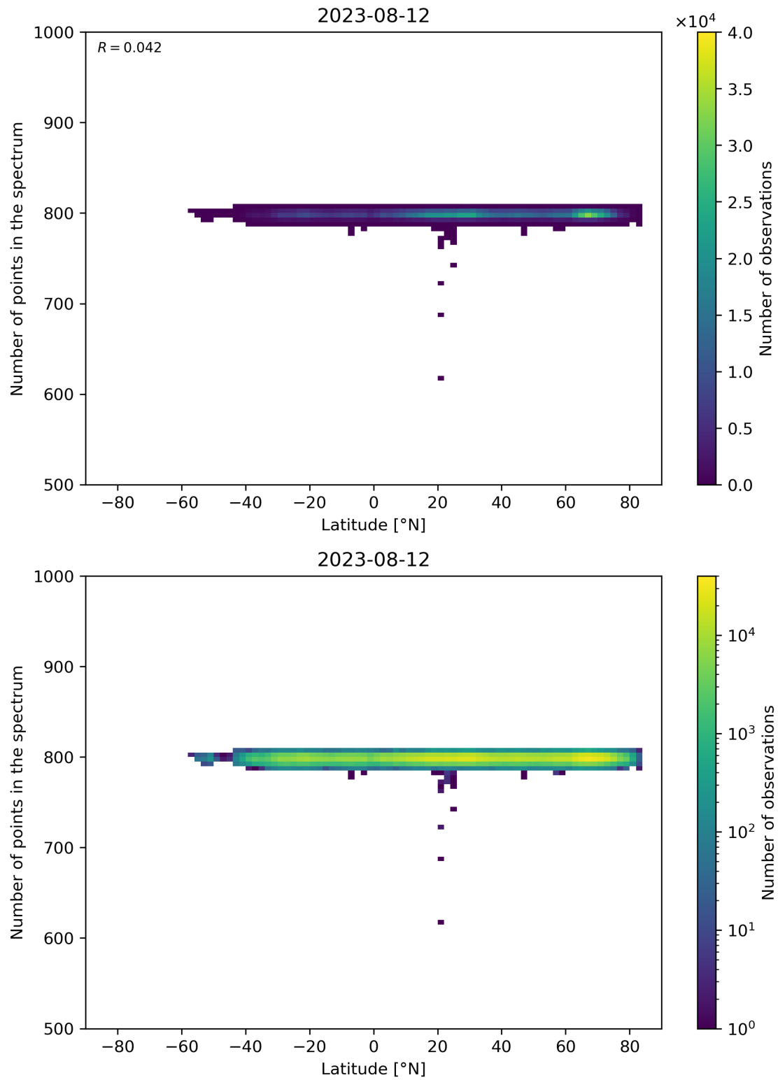
Figure 61: Scatter density plot of “Latitude” against “Number of points in the spectrum” for 2023-08-11 to 2023-08-13.
