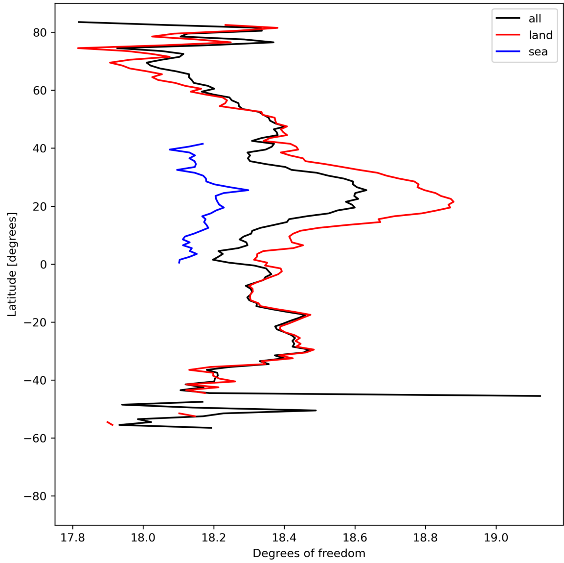
Figure 19: Zonal average of “Degrees of freedom” for 2023-08-11 to 2023-08-13.
