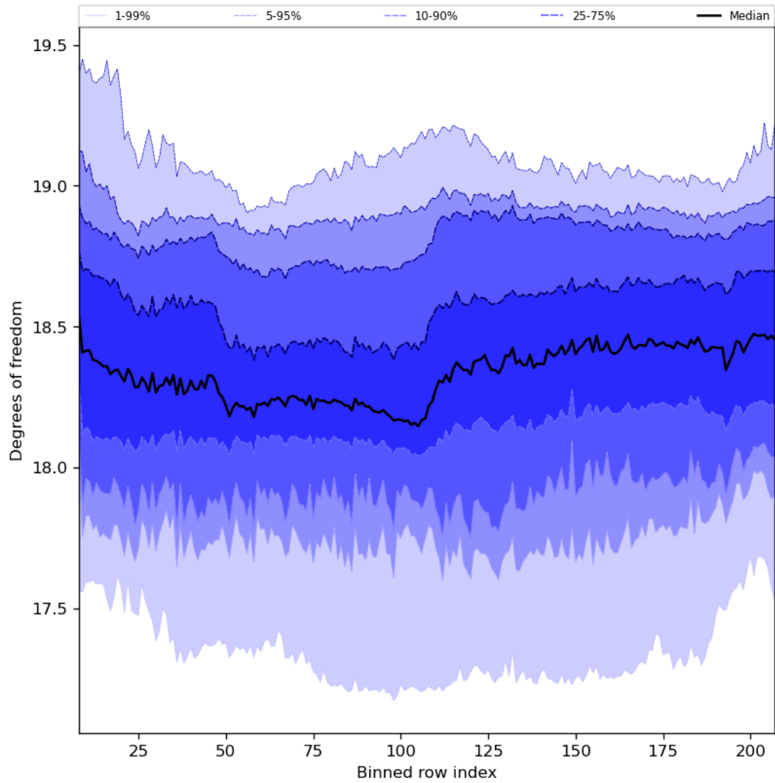
Figure 41: Along track statistics of “Degrees of freedom” for 2023-08-11 to 2023-08-13
