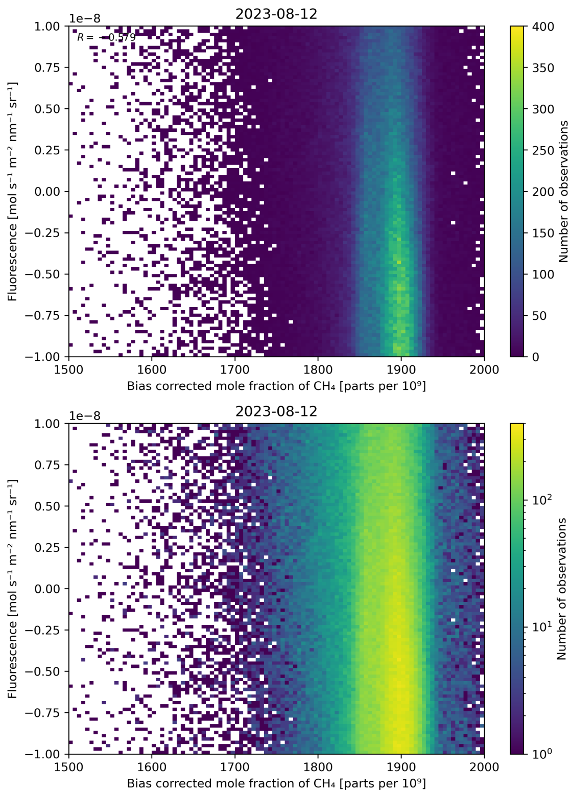
Figure 66: Scatter density plot of “Bias corrected mole fraction of \text{CH}_4 ” against “Fluorescence” for 2023-08-11 to 2023-08-13.
