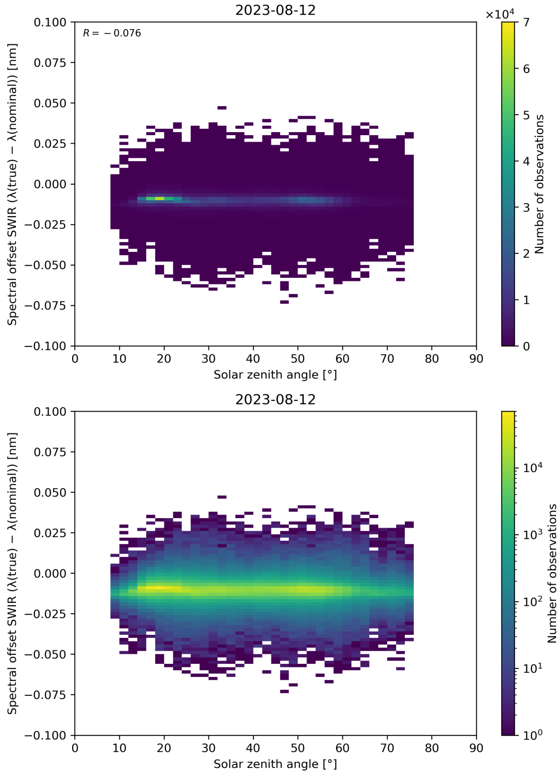
Figure 104: Scatter density plot of “Solar zenith angle” against “Spectral offset SWIR ( \lambda(\text{true}) - \lambda(\text{nominal}) )” for 2023-08-11 to 2023-08-13.
