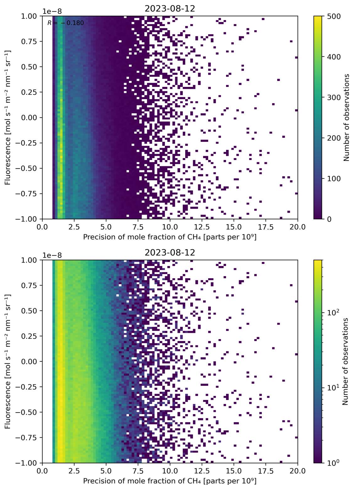
Figure 81: Scatter density plot of “Precision of mole fraction of \text{CH}_4 ” against “Fluorescence” for 2023-08-11 to 2023-08-13.
