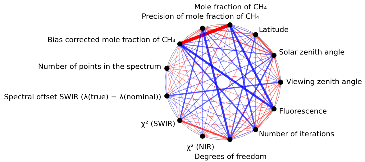
Figure 1: Map of correlation graph for 2023-08-11 to 2023-08-13.
