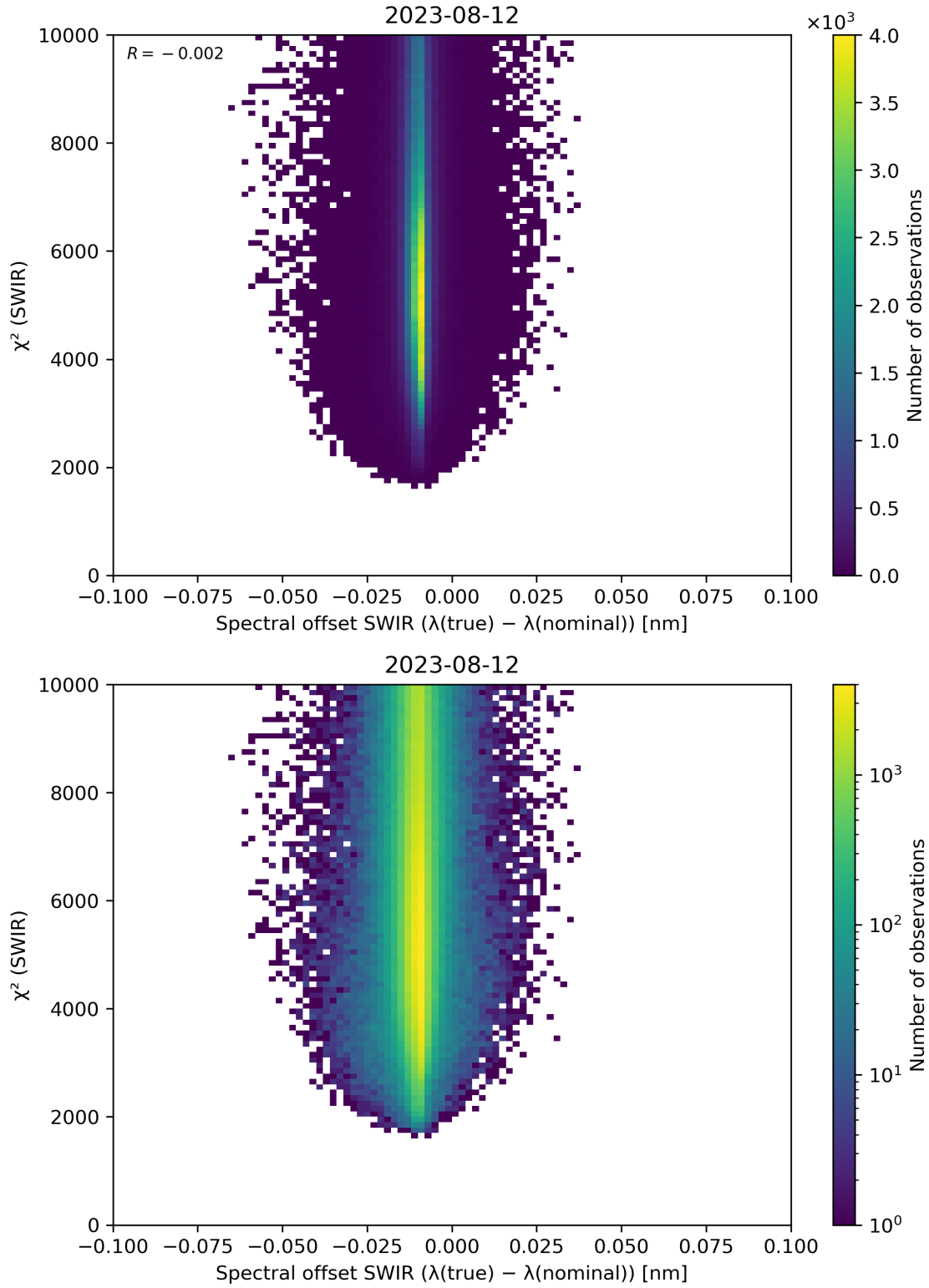
Figure 118: Scatter density plot of “Spectral offset SWIR ( \lambda(\text{true}) - \lambda(\text{nominal}) )” against “ \chi^2 (SWIR)” for 2023-08-11 to 2023-08-13.
