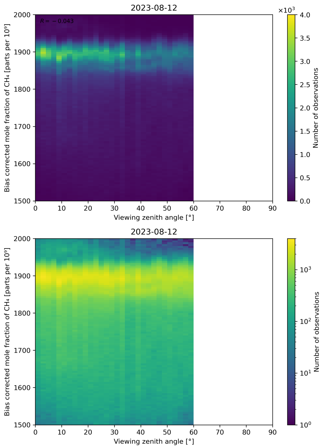
Figure 111: Scatter density plot of “Viewing zenith angle” against “Bias corrected mole fraction of CH 4 ” for 2023-08-11 to 2023-08-13.
