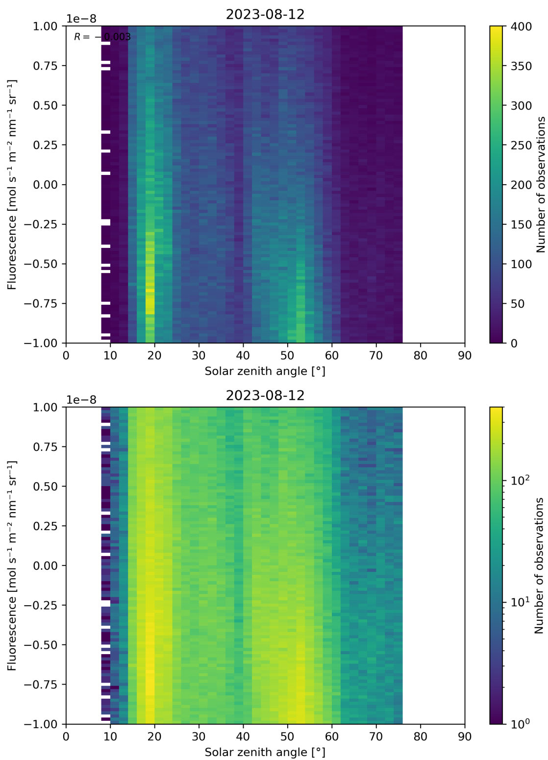
Figure 97: Scatter density plot of “Solar zenith angle” against “Fluorescence” for 2023-08-11 to 2023-08-13.
