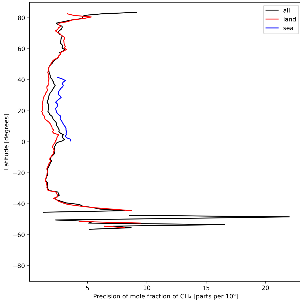
Figure 13: Zonal average of “Precision of mole fraction of CH 4 ” for 2023-08-11 to 2023-08-13.
