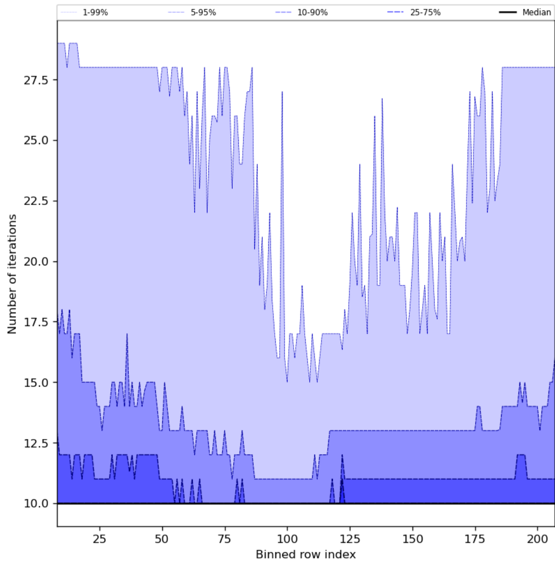
Figure 42: Along track statistics of “Number of iterations” for 2023-08-11 to 2023-08-13
