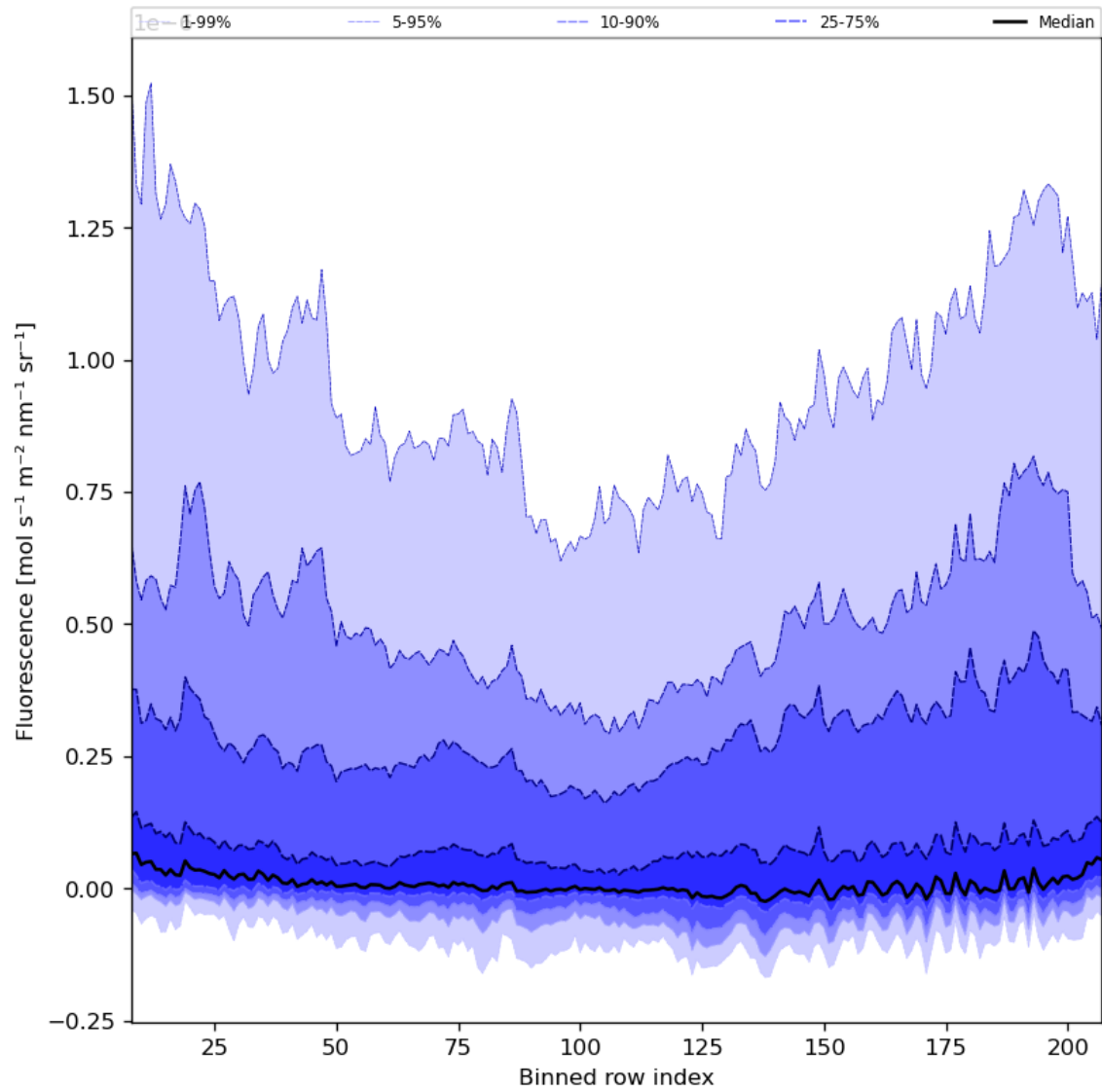
Figure 43: Along track statistics of “Fluorescence” for 2023-08-11 to 2023-08-13
