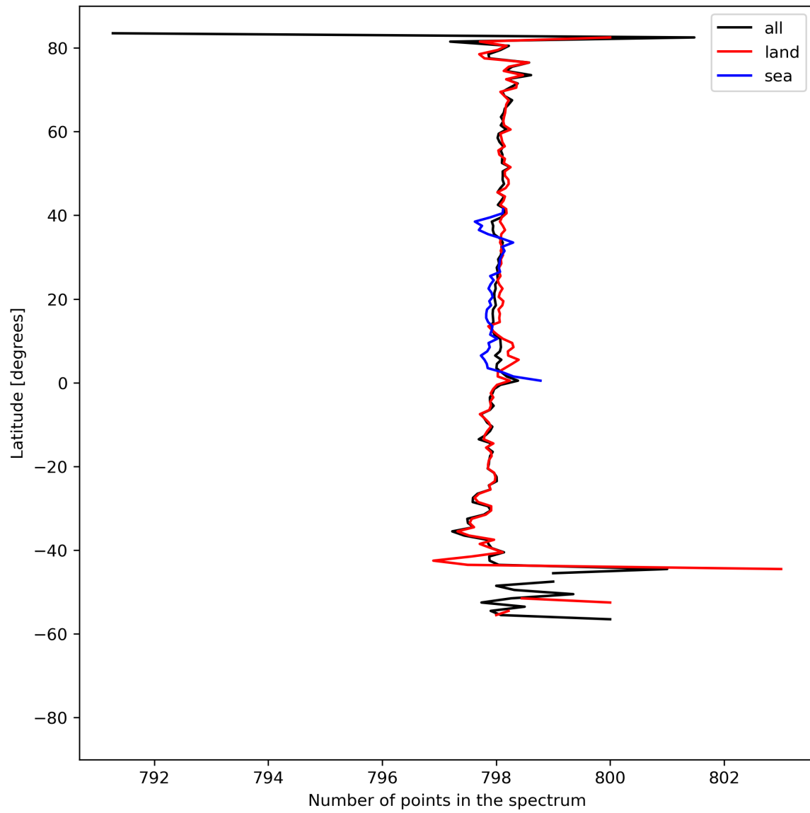
Figure 15: Zonal average of “Number of points in the spectrum” for 2023-08-11 to 2023-08-13.
