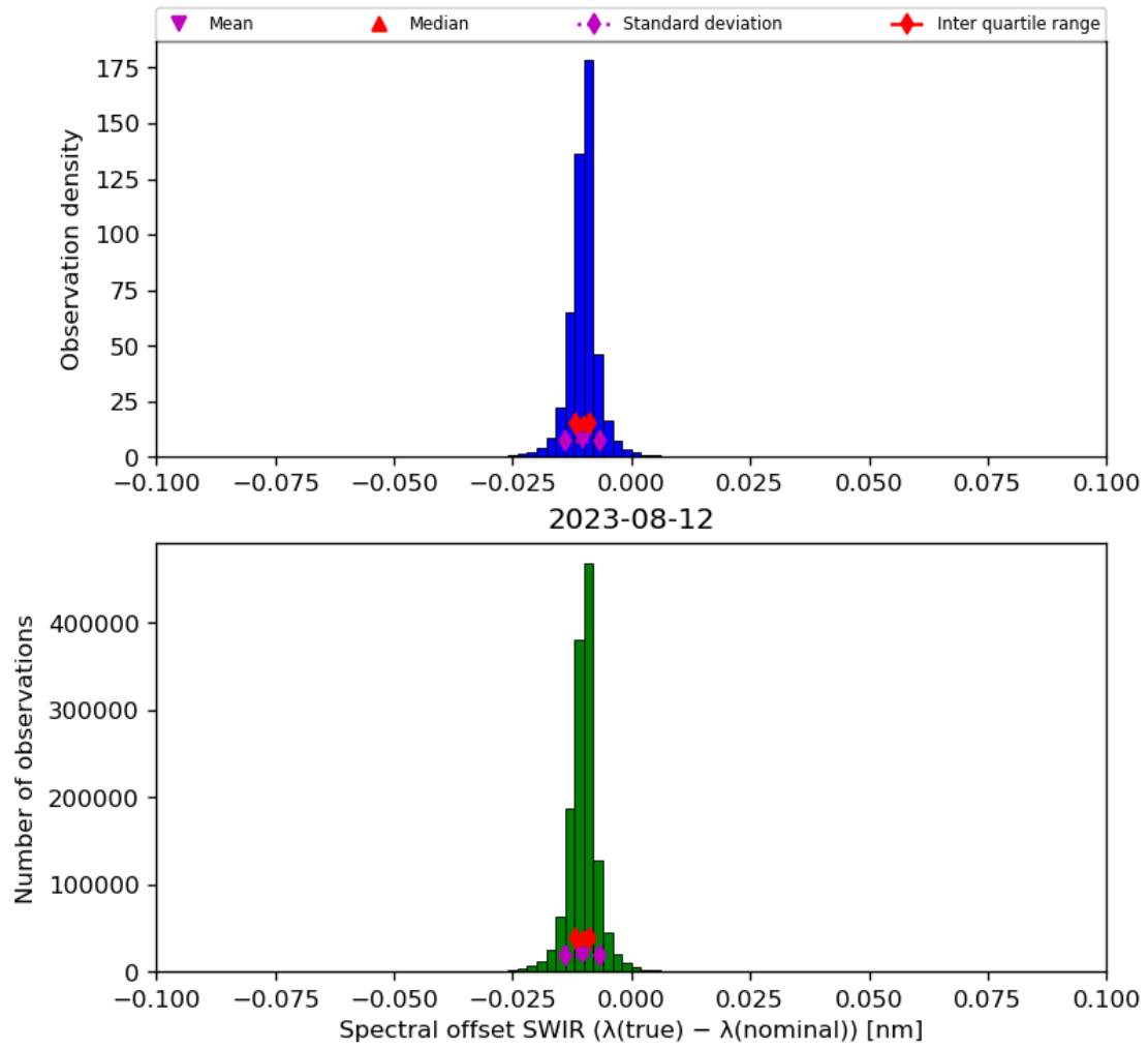
Figure 27: Histogram of “Spectral offset SWIR ( \lambda(\text{true}) - \lambda(\text{nominal}) )” for 2023-08-11 to 2023-08-13
