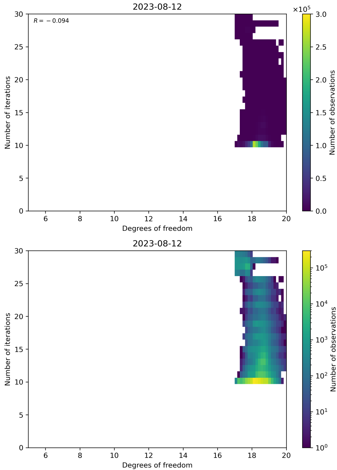
Figure 52: Scatter density plot of “Degrees of freedom” against “Number of iterations” for 2023-08-11 to 2023-08-13.
