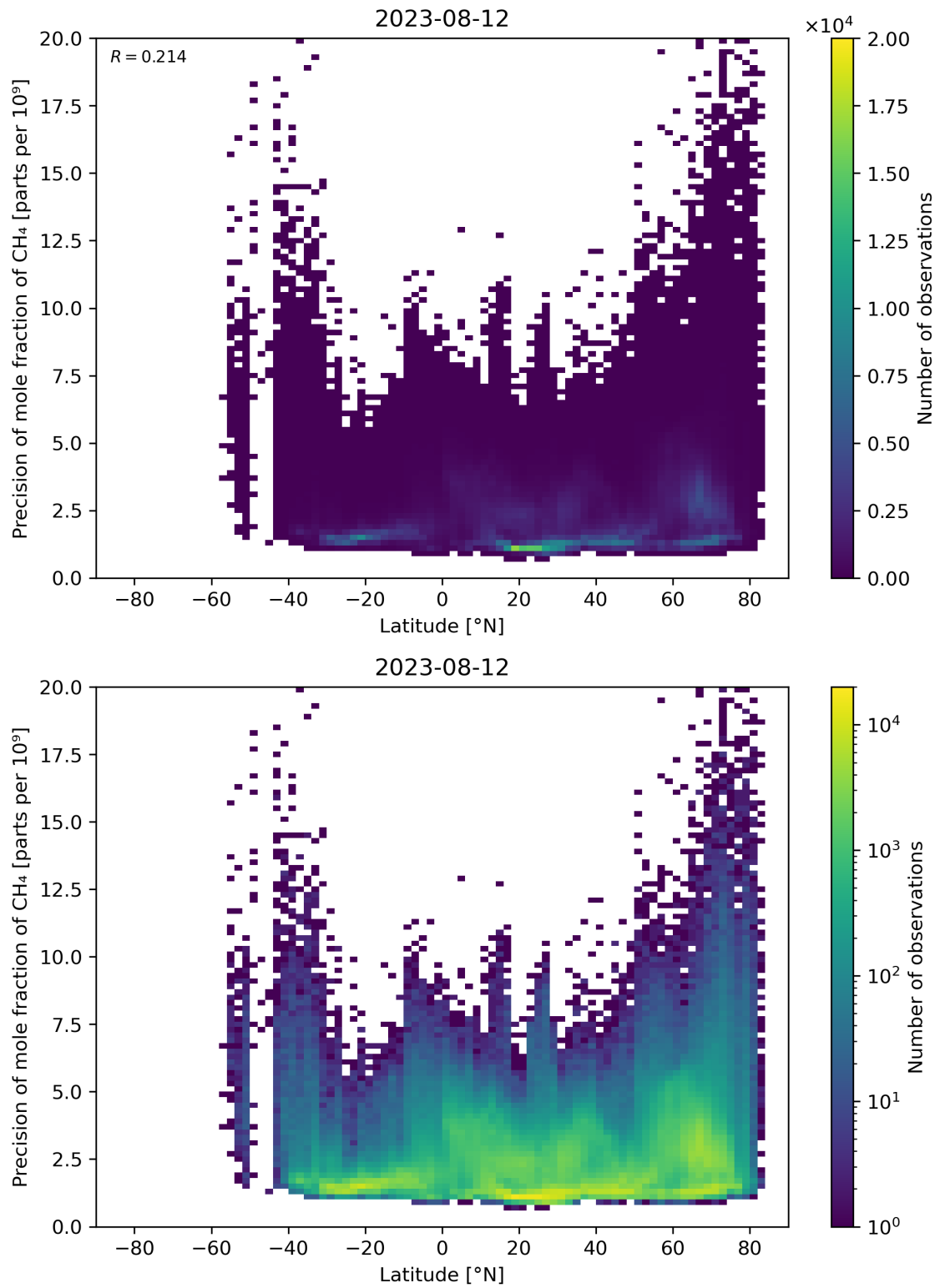
Figure 59: Scatter density plot of “Latitude” against “Precision of mole fraction of \text{CH}_4 ” for 2023-08-11 to 2023-08-13.
