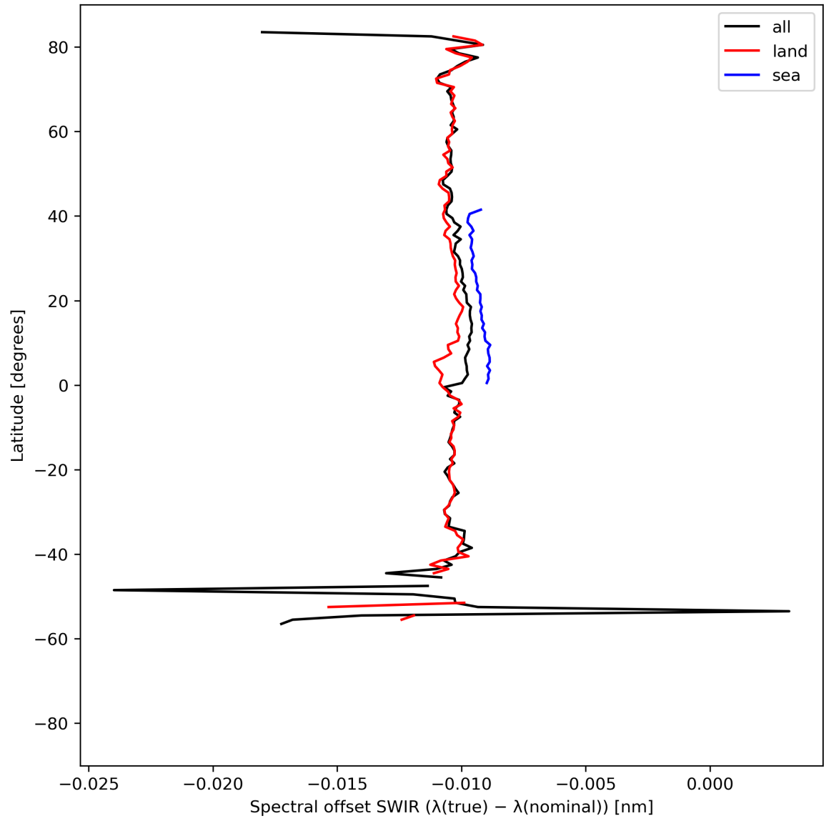
Figure 16: Zonal average of “Spectral offset SWIR ( \lambda(\text{true}) - \lambda(\text{nominal}) )” for 2023-08-11 to 2023-08-13.
