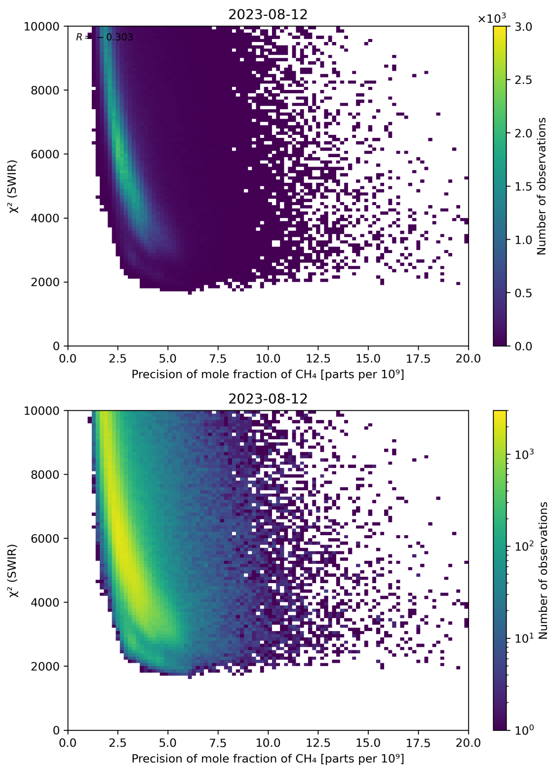
Figure 79: Scatter density plot of “Precision of mole fraction of CH 4 ” against “ \chi^2 (SWIR)” for 2023-08-11 to 2023-08-13.
