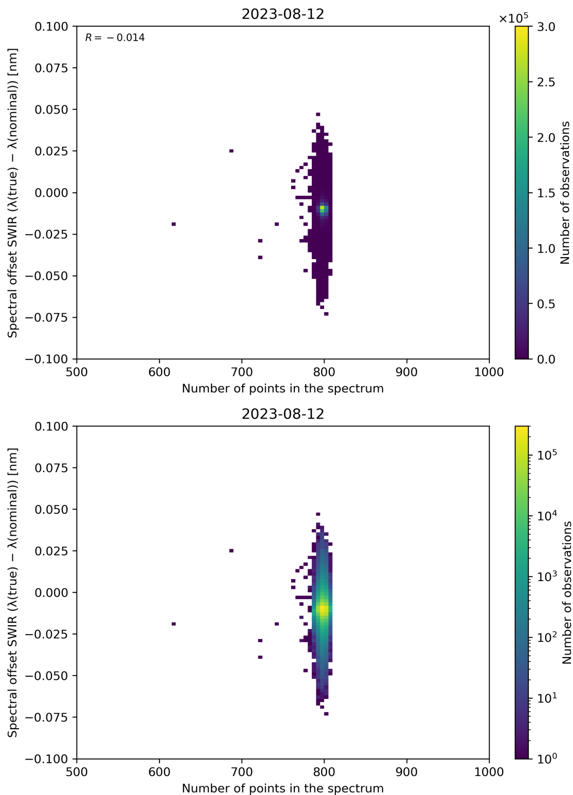
Figure 93: Scatter density plot of “Number of points in the spectrum” against “Spectral offset SWIR ( \lambda(\text{true}) - \lambda(\text{nominal}) )” for 2023-08-11 to 2023-08-13.
