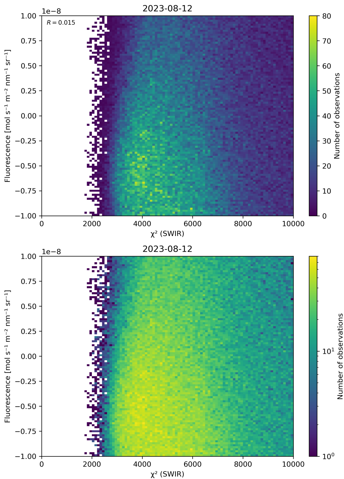
Figure 49: Scatter density plot of “ \chi^2 (SWIR)” against “Fluorescence” for 2023-08-11 to 2023-08-13.
