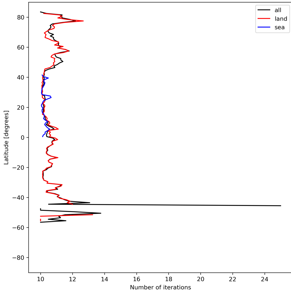
Figure 20: Zonal average of “Number of iterations” for 2023-08-11 to 2023-08-13.
