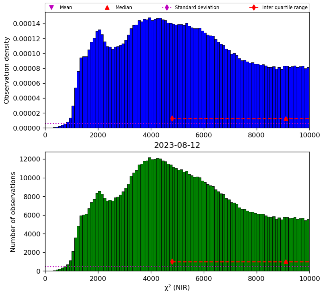
Figure 29: Histogram of “ \chi^2 (NIR)” for 2023-08-11 to 2023-08-13
