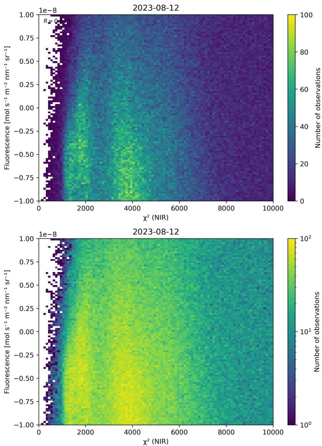
Figure 45: Scatter density plot of “ \chi^2 (NIR)” against “Fluorescence” for 2023-08-11 to 2023-08-13.
