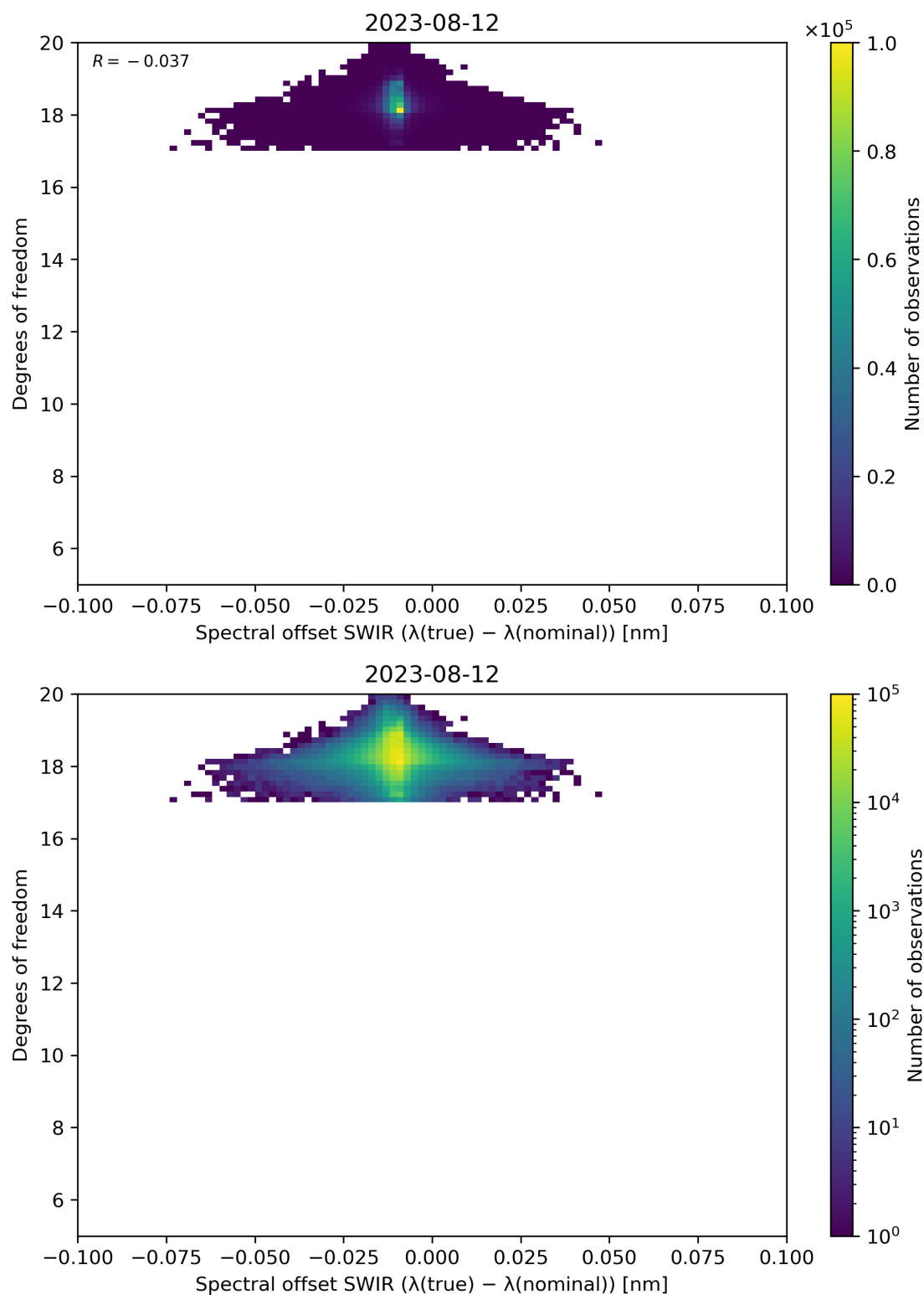
Figure 119: Scatter density plot of “Spectral offset SWIR ( \lambda(\text{true}) - \lambda(\text{nominal}) )” against “Degrees of freedom” for 2023-08-11 to 2023-08-13.
