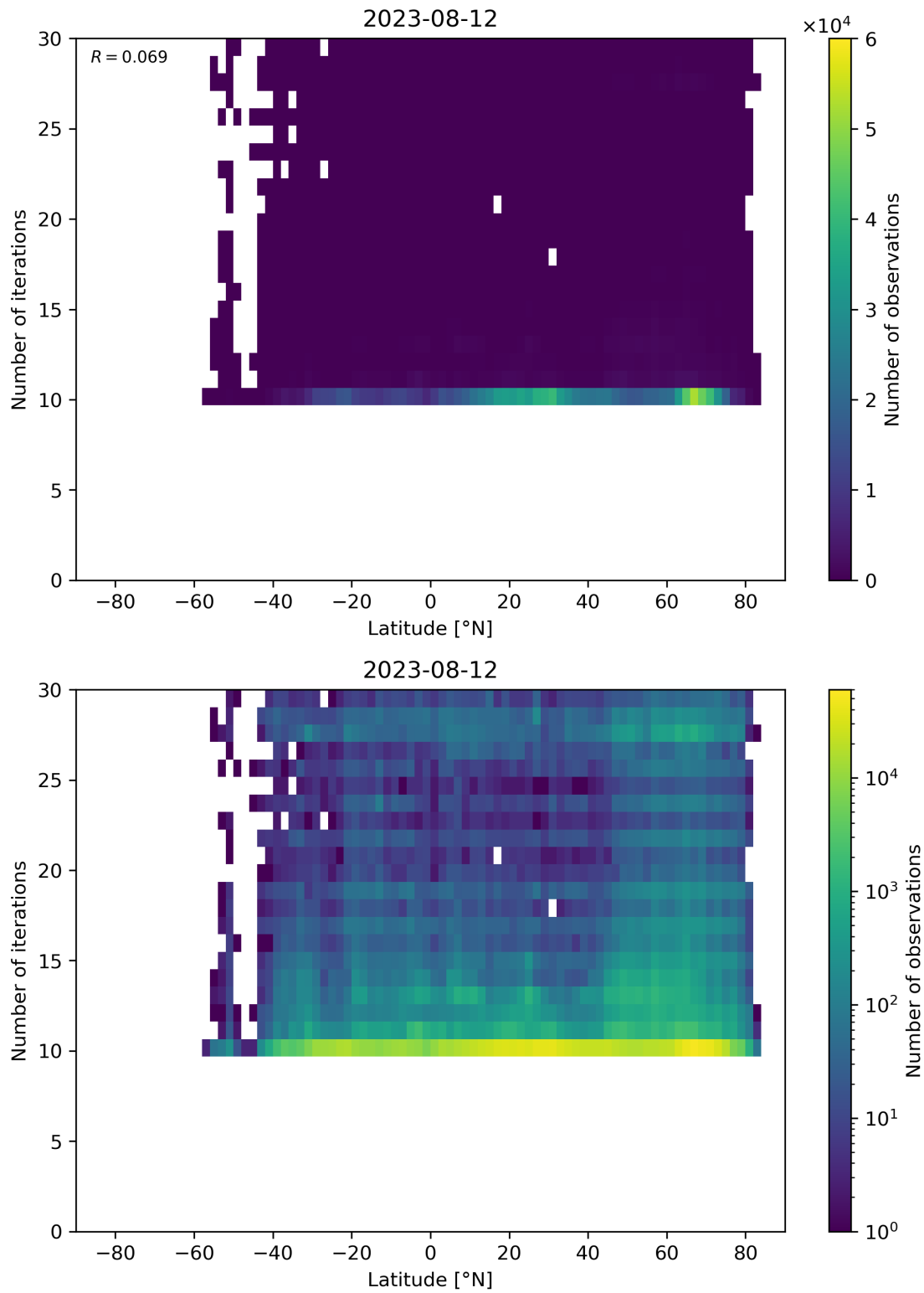
Figure 60: Scatter density plot of “Latitude” against “Number of iterations” for 2023-08-11 to 2023-08-13.
