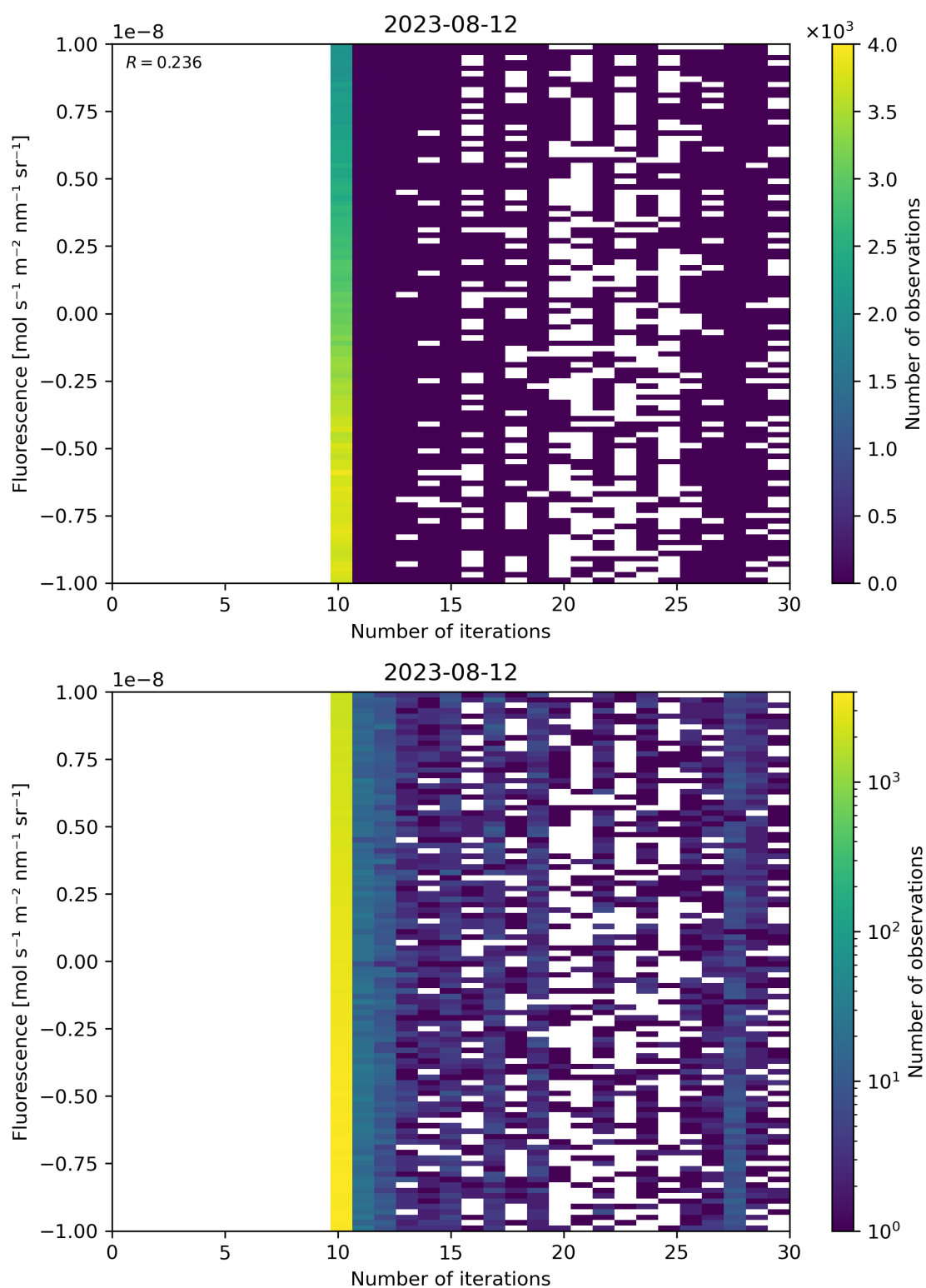
Figure 87: Scatter density plot of “Number of iterations” against “Fluorescence” for 2023-08-11 to 2023-08-13.
