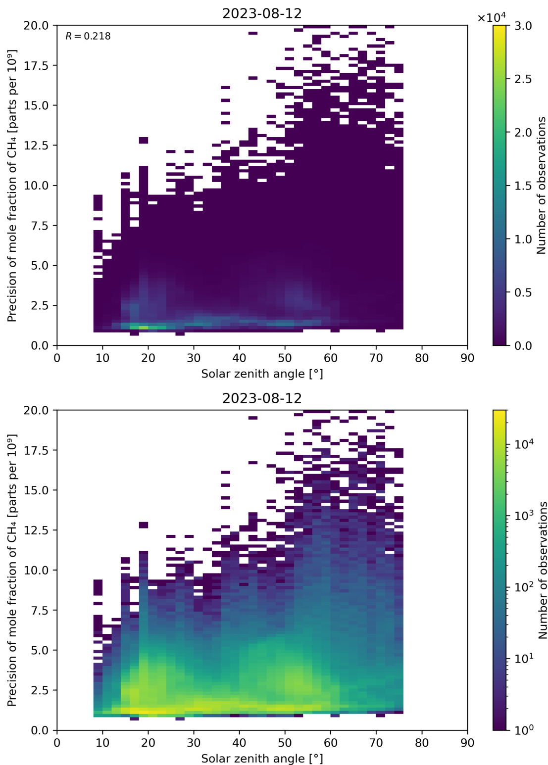
Figure 101: Scatter density plot of “Solar zenith angle” against “Precision of mole fraction of CH 4 ” for 2023-08-11 to 2023-08-13.
