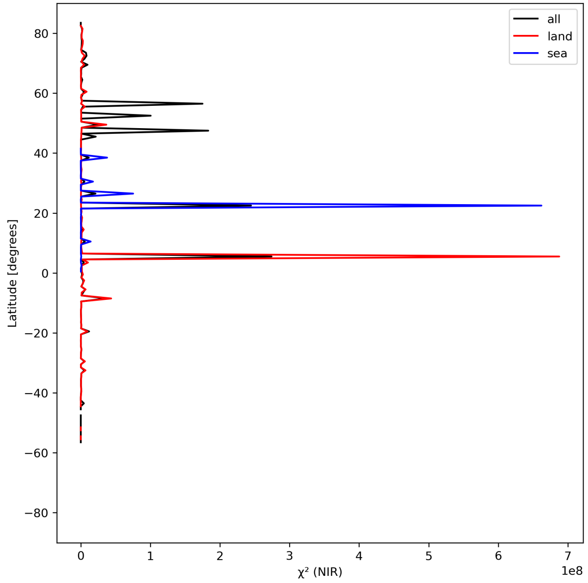
Figure 18: Zonal average of “ \chi^2 (NIR)” for 2023-08-11 to 2023-08-13.
