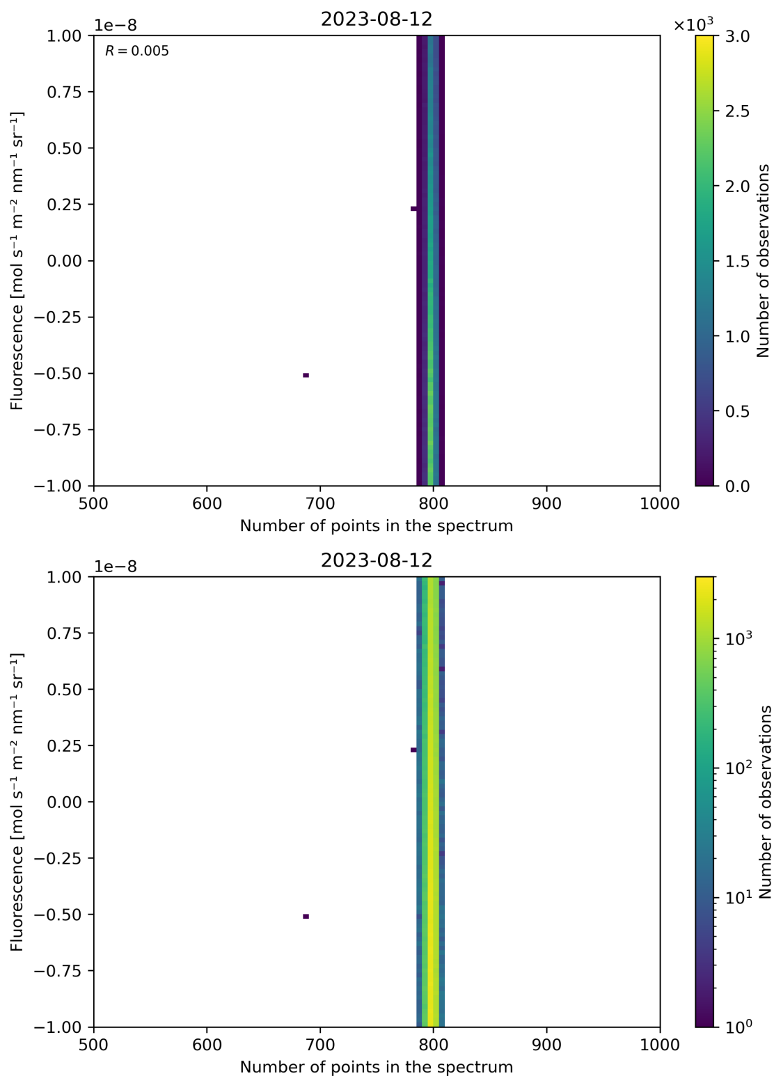
Figure 91: Scatter density plot of “Number of points in the spectrum” against “Fluorescence” for 2023-08-11 to 2023-08-13.
