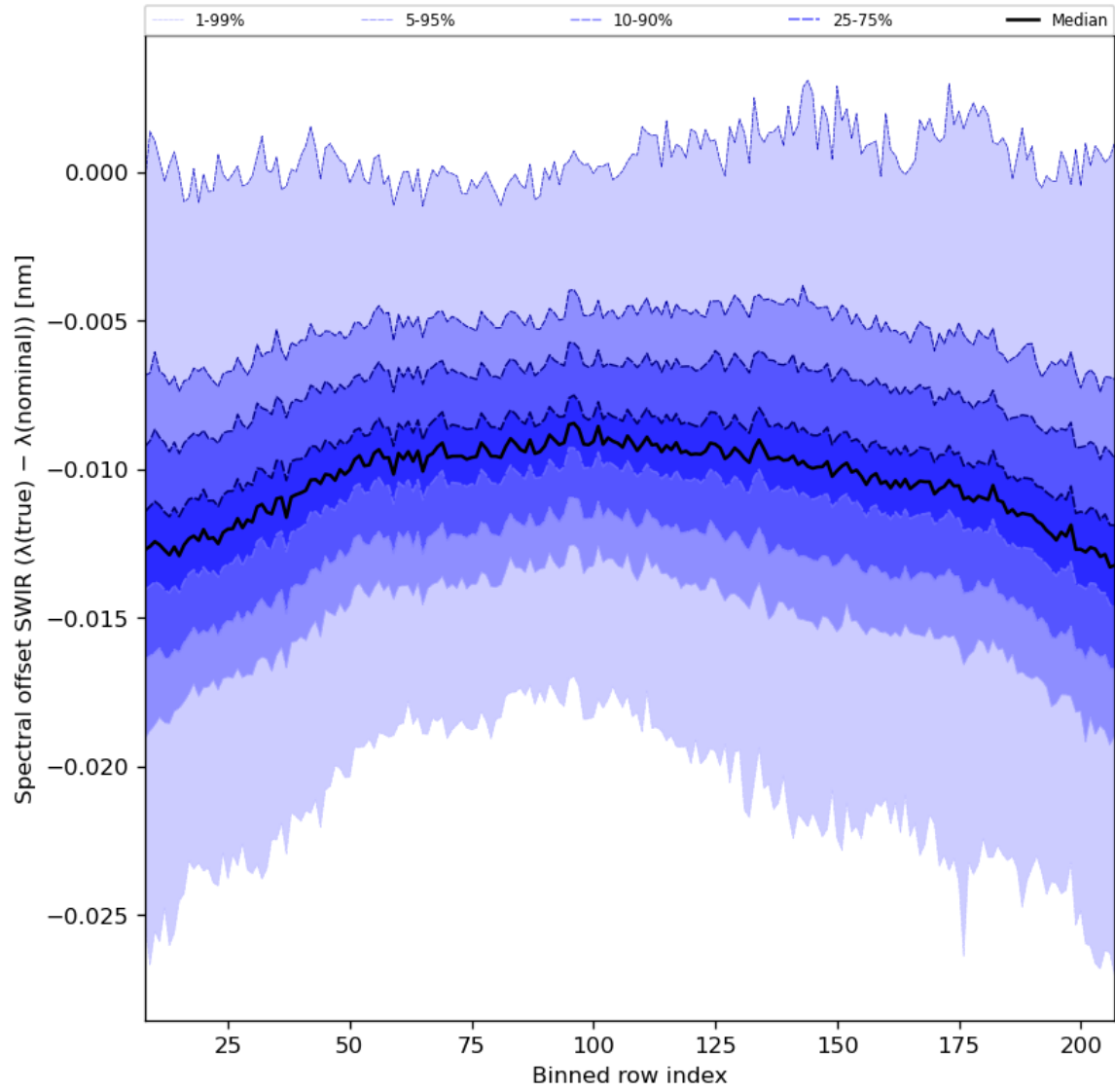
Figure 38: Along track statistics of “Spectral offset SWIR ( \lambda(\text{true}) - \lambda(\text{nominal}) )” for 2023-08-11 to 2023-08-13
