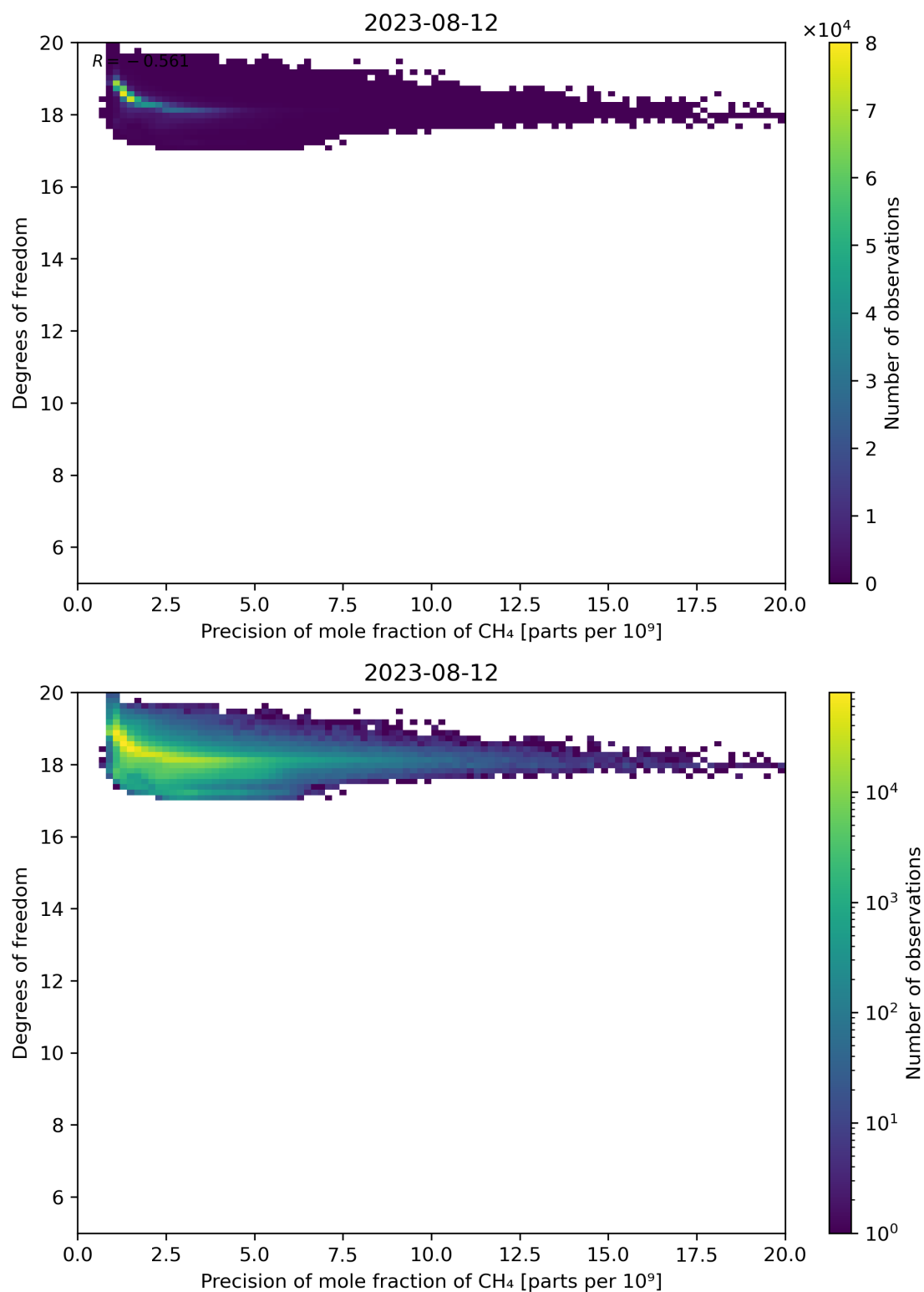
Figure 80: Scatter density plot of “Precision of mole fraction of CH 4 ” against “Degrees of freedom” for 2023-08-11 to 2023-08-13.
