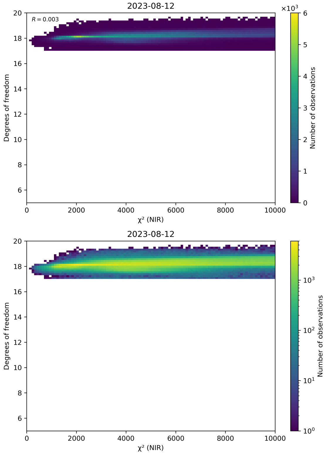
Figure 44: Scatter density plot of “ \chi^2 (NIR)” against “Degrees of freedom” for 2023-08-11 to 2023-08-13.
