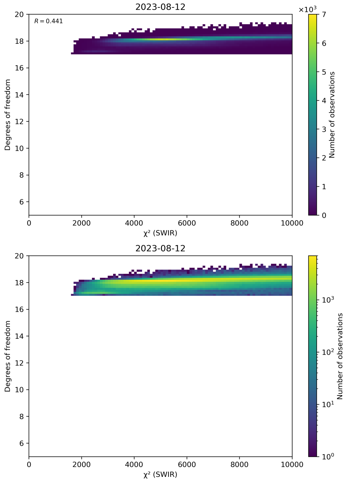
Figure 48: Scatter density plot of “ \chi^2 (SWIR)” against “Degrees of freedom” for 2023-08-11 to 2023-08-13.
