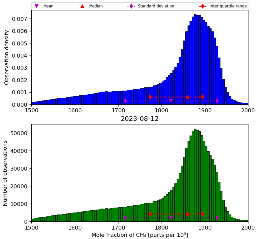
Figure 23: Histogram of “Mole fraction of CH 4 ” for 2023-08-11 to 2023-08-13
