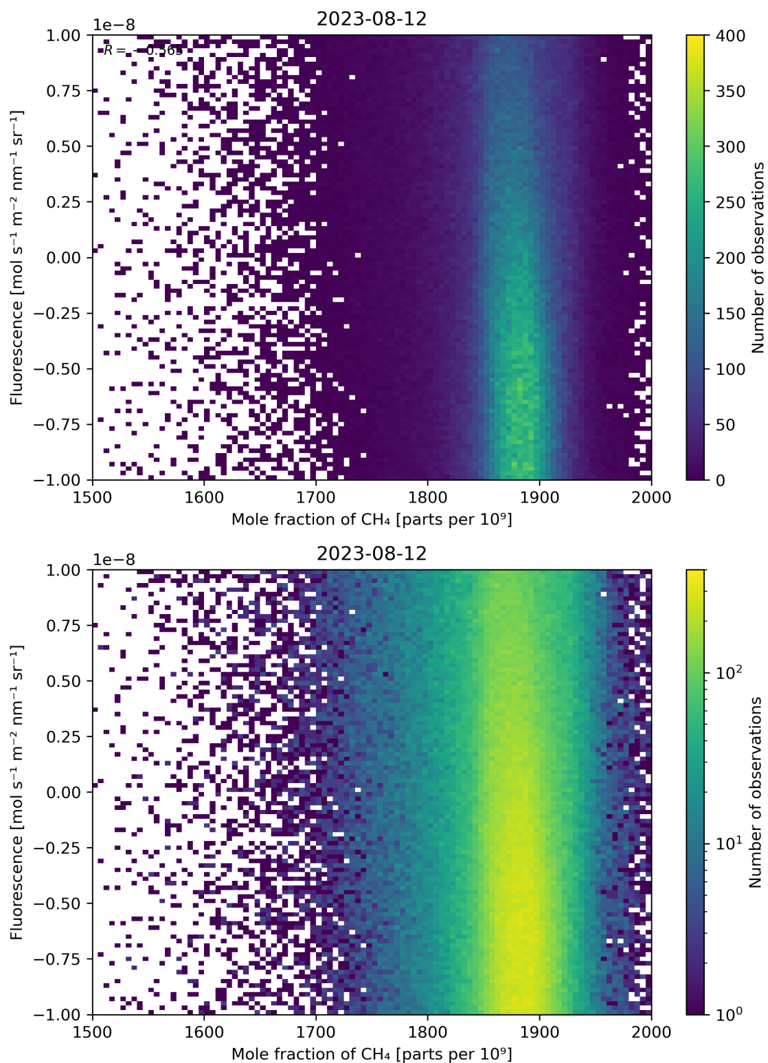
Figure 73: Scatter density plot of “Mole fraction of \text{CH}_4 ” against “Fluorescence” for 2023-08-11 to 2023-08-13.
