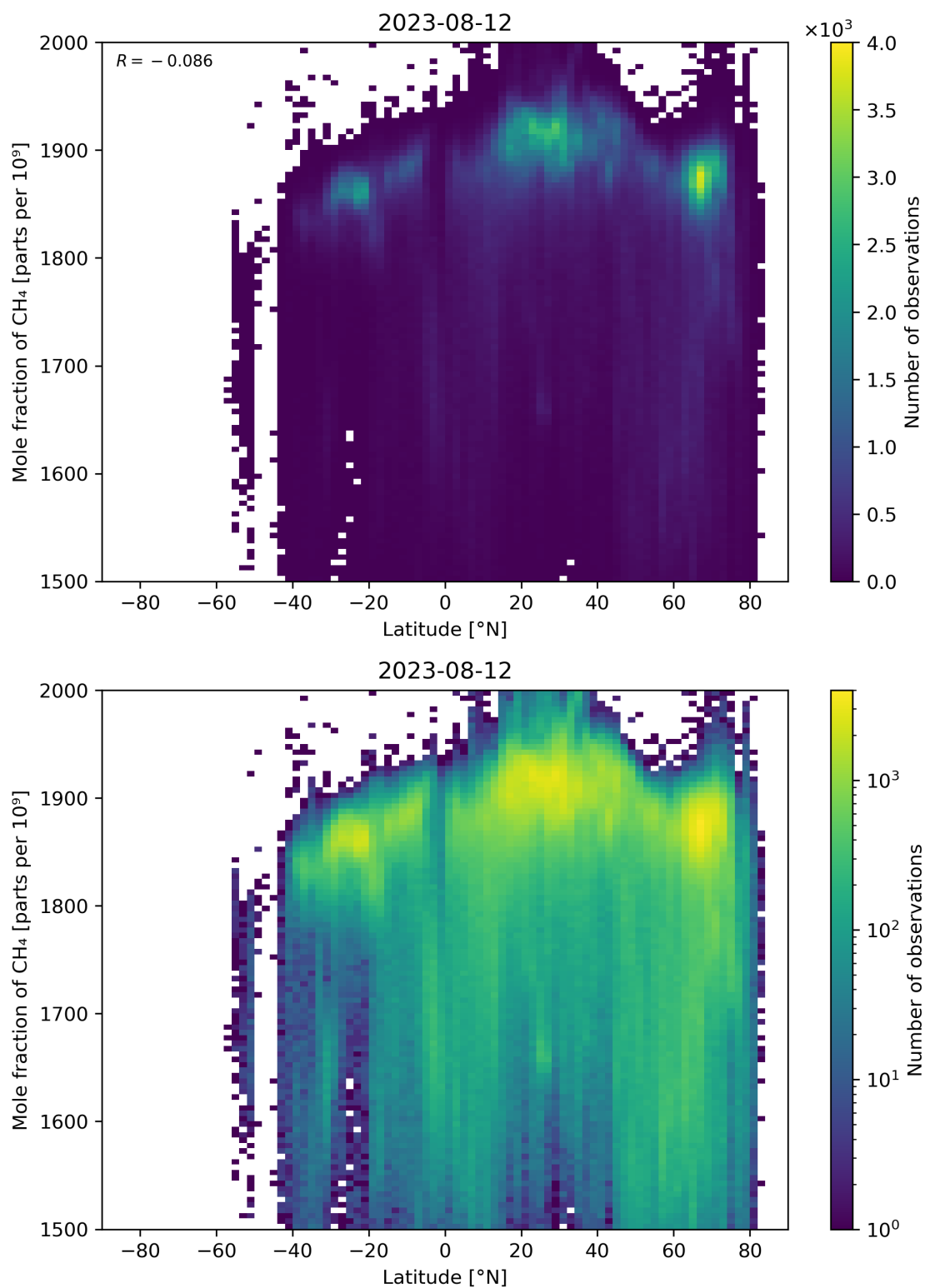
Figure 57: Scatter density plot of “Latitude” against “Mole fraction of \text{CH}_4 ” for 2023-08-11 to 2023-08-13.
