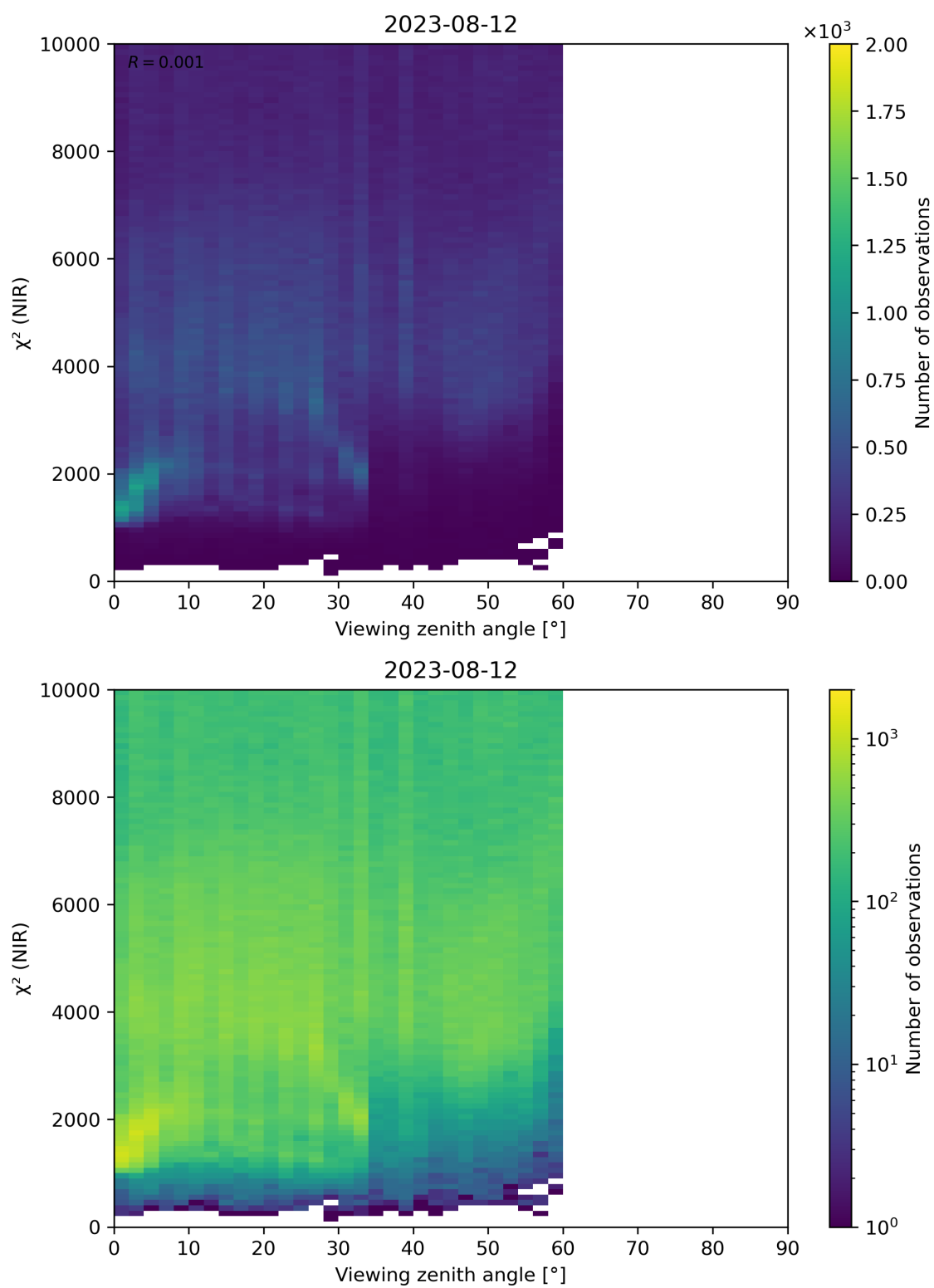
Figure 105: Scatter density plot of “Viewing zenith angle” against “ \chi^2 (NIR)” for 2023-08-11 to 2023-08-13.
