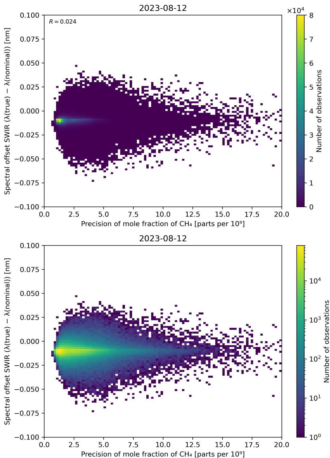
Figure 85: Scatter density plot of “Precision of mole fraction of CH 4 ” against “Spectral offset SWIR ( \lambda(\text{true}) - \lambda(\text{nominal}) )” for 2023-08-11 to 2023-08-13.
