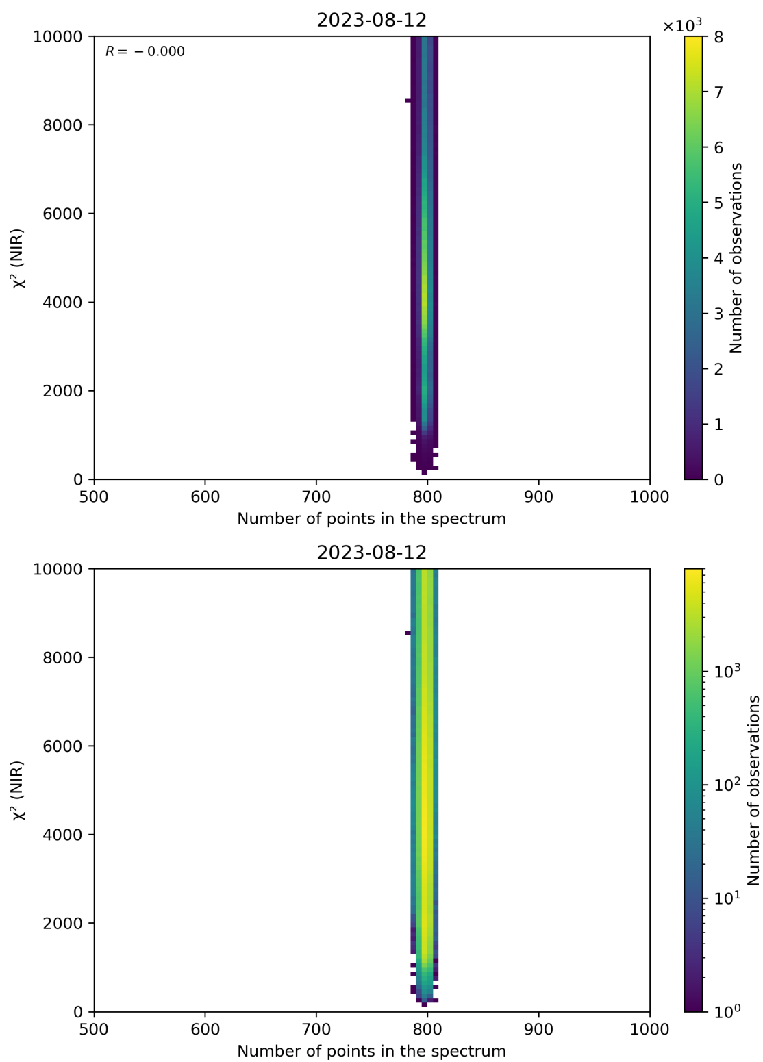
Figure 88: Scatter density plot of “Number of points in the spectrum” against “ \chi^2 (NIR)” for 2023-08-11 to 2023-08-13.
