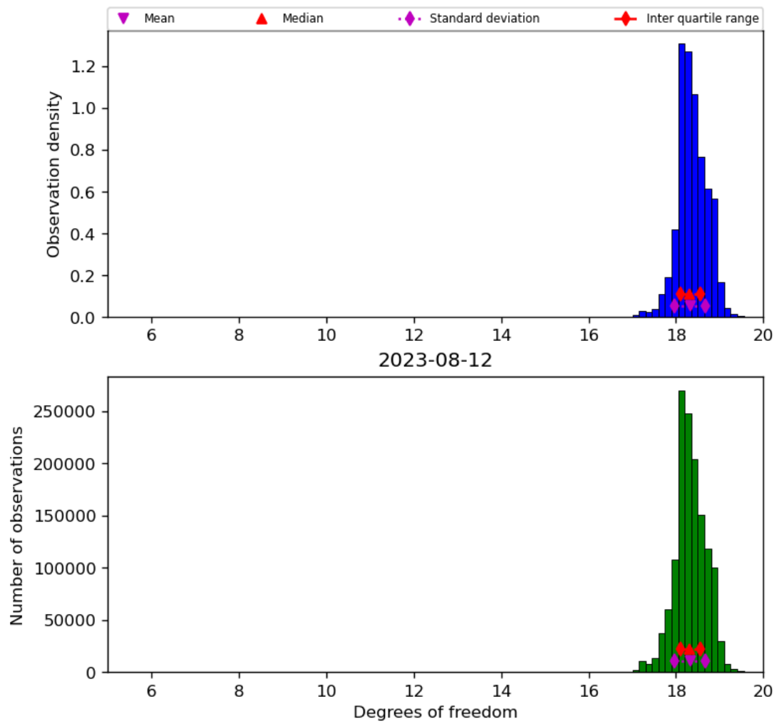
Figure 30: Histogram of “Degrees of freedom” for 2023-08-11 to 2023-08-13
