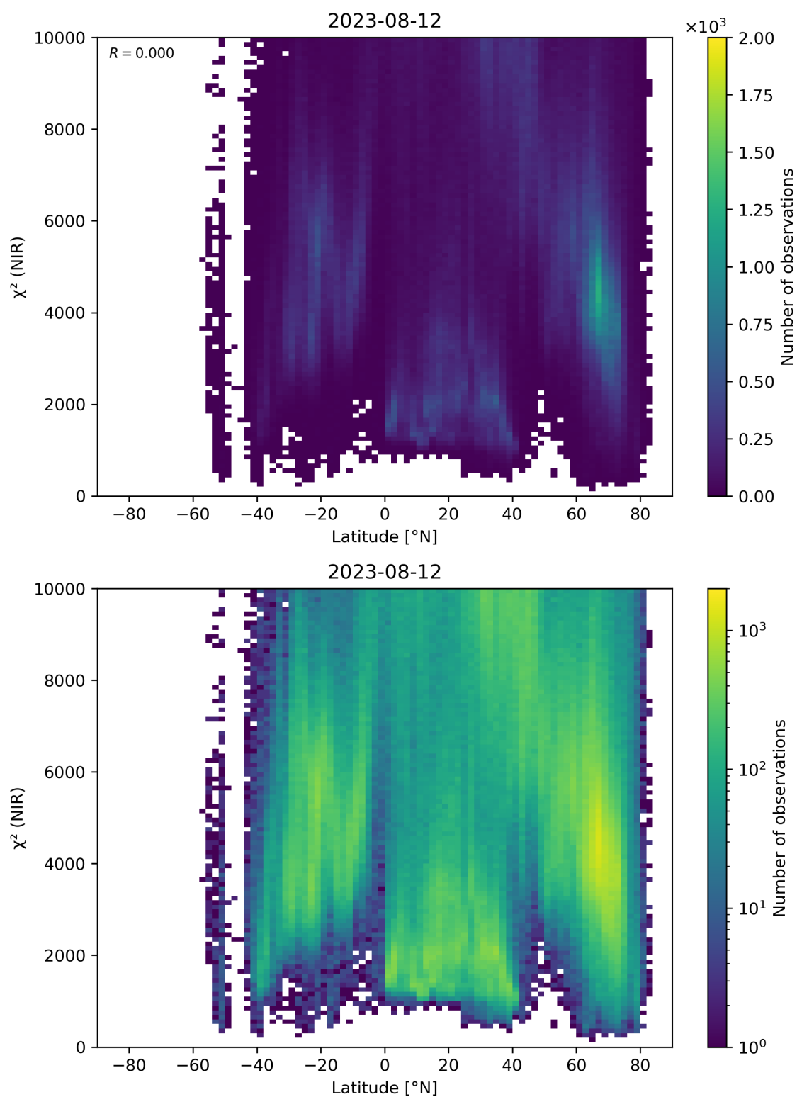
Figure 53: Scatter density plot of “Latitude” against “ \chi^2 (NIR)” for 2023-08-11 to 2023-08-13.
