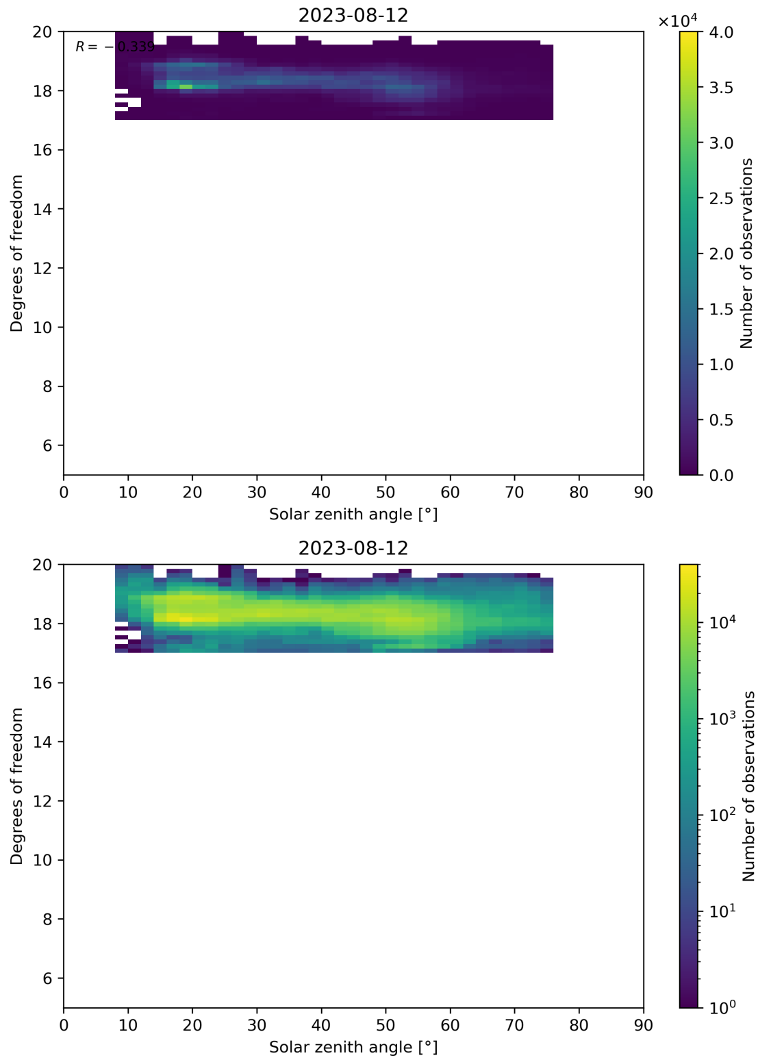
Figure 96: Scatter density plot of “Solar zenith angle” against “Degrees of freedom” for 2023-08-11 to 2023-08-13.
