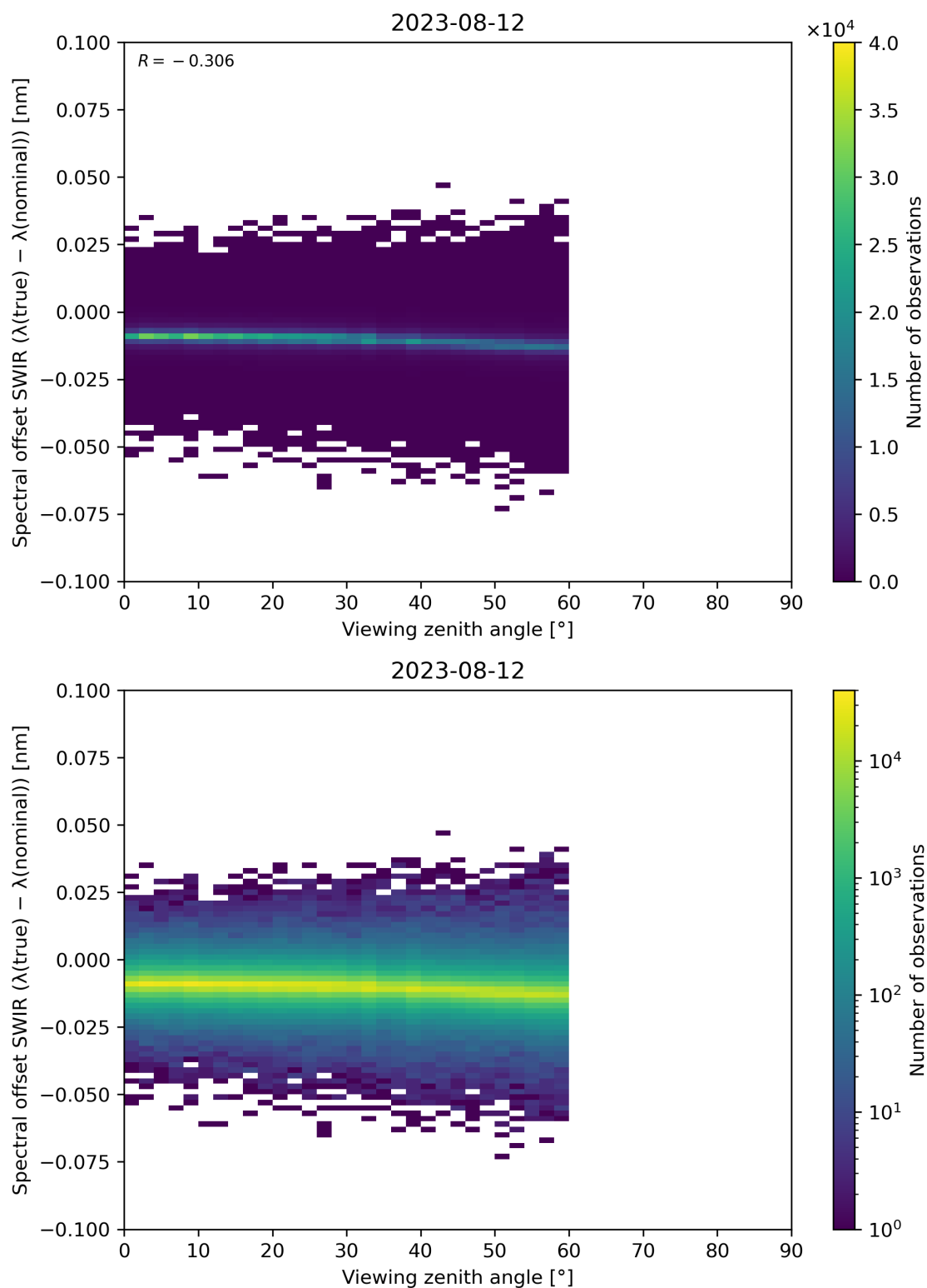
Figure 116: Scatter density plot of “Viewing zenith angle” against “Spectral offset SWIR ( \lambda(\text{true}) - \lambda(\text{nominal}) )” for 2023-08-11 to 2023-08-13.
