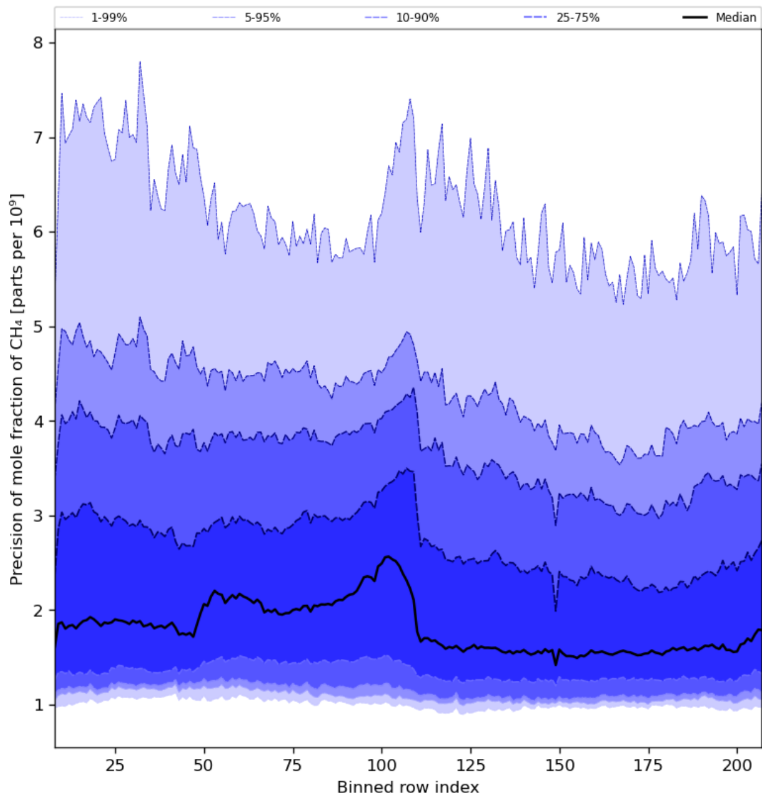
Figure 35: Along track statistics of “Precision of mole fraction of CH 4 ” for 2023-08-11 to 2023-08-13
