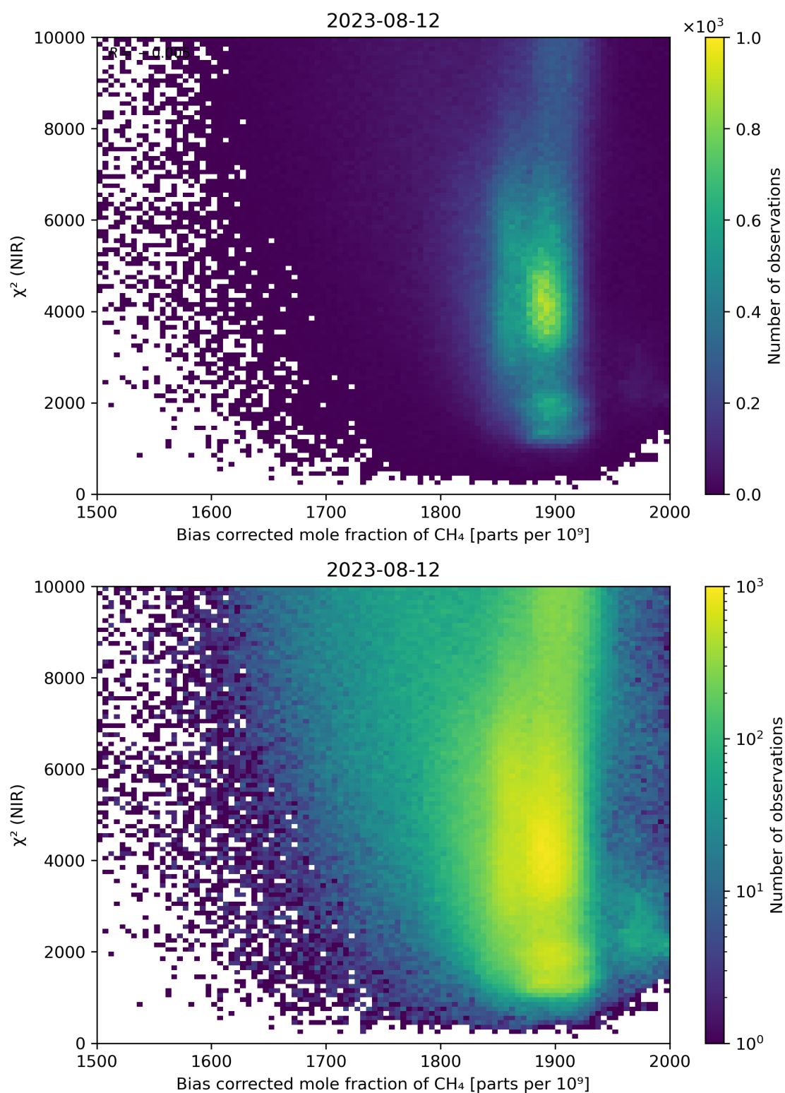
Figure 63: Scatter density plot of “Bias corrected mole fraction of CH 4 ” against “ \chi^2 (NIR)” for 2023-08-11 to 2023-08-13.
