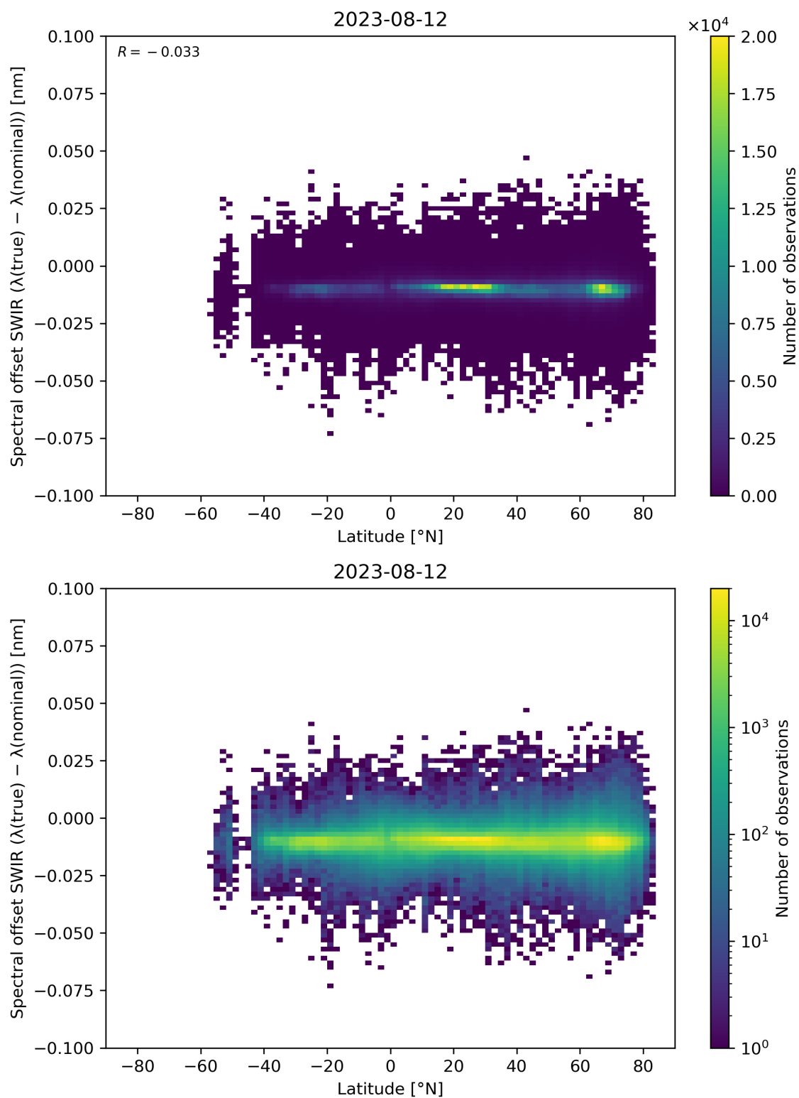
Figure 62: Scatter density plot of “Latitude” against “Spectral offset SWIR ( \lambda(\text{true}) - \lambda(\text{nominal}) )” for 2023-08-11 to 2023-08-13.
