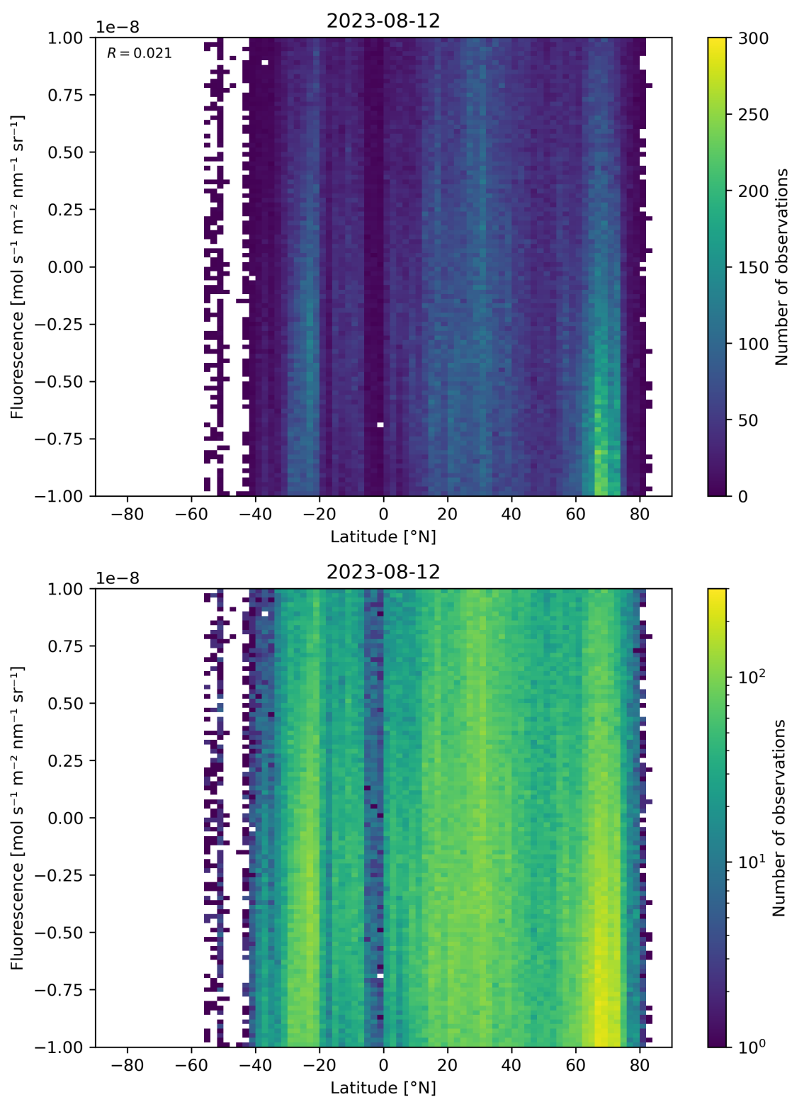
Figure 56: Scatter density plot of “Latitude” against “Fluorescence” for 2023-08-11 to 2023-08-13.
