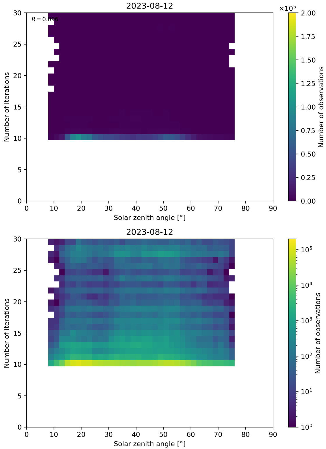
Figure 102: Scatter density plot of “Solar zenith angle” against “Number of iterations” for 2023-08-11 to 2023-08-13.
