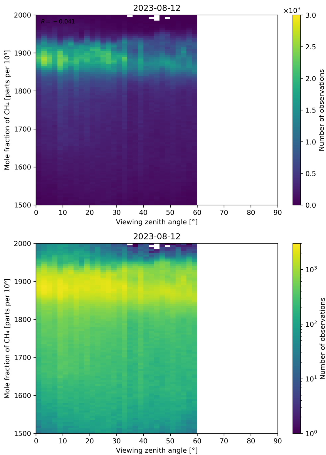
Figure 110: Scatter density plot of “Viewing zenith angle” against “Mole fraction of CH 4 ” for 2023-08-11 to 2023-08-13.
