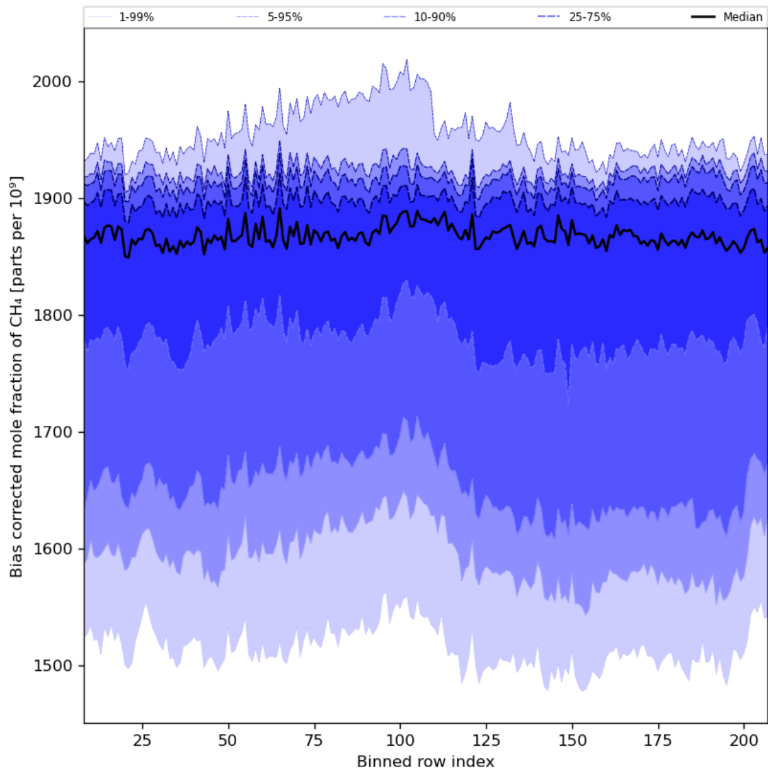
Figure 36: Along track statistics of “Bias corrected mole fraction of \text{CH}_4 ” for 2023-08-11 to 2023-08-13
