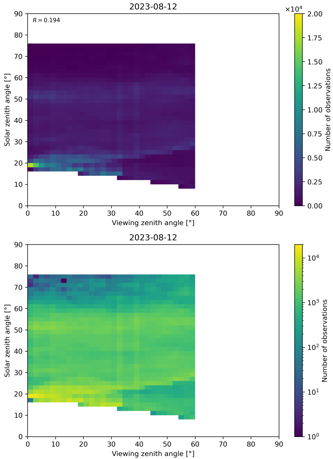
Figure 115: Scatter density plot of “Viewing zenith angle” against “Solar zenith angle” for 2023-08-11 to 2023-08-13.
