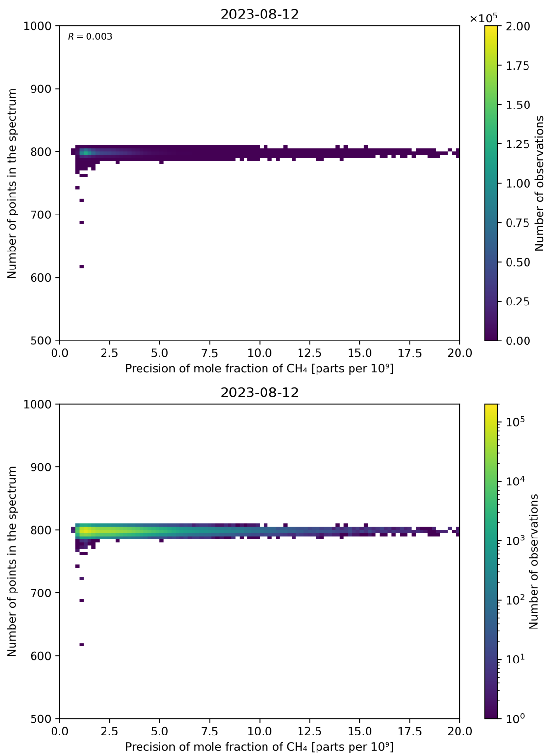
Figure 84: Scatter density plot of “Precision of mole fraction of \text{CH}_4 ” against “Number of points in the spectrum” for 2023-08-11 to 2023-08-13.
