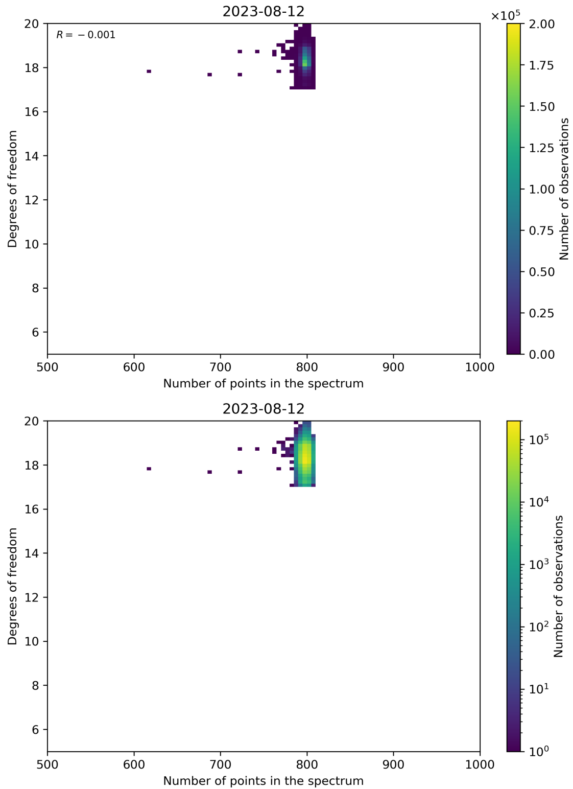
Figure 90: Scatter density plot of “Number of points in the spectrum” against “Degrees of freedom” for 2023-08-11 to 2023-08-13.
