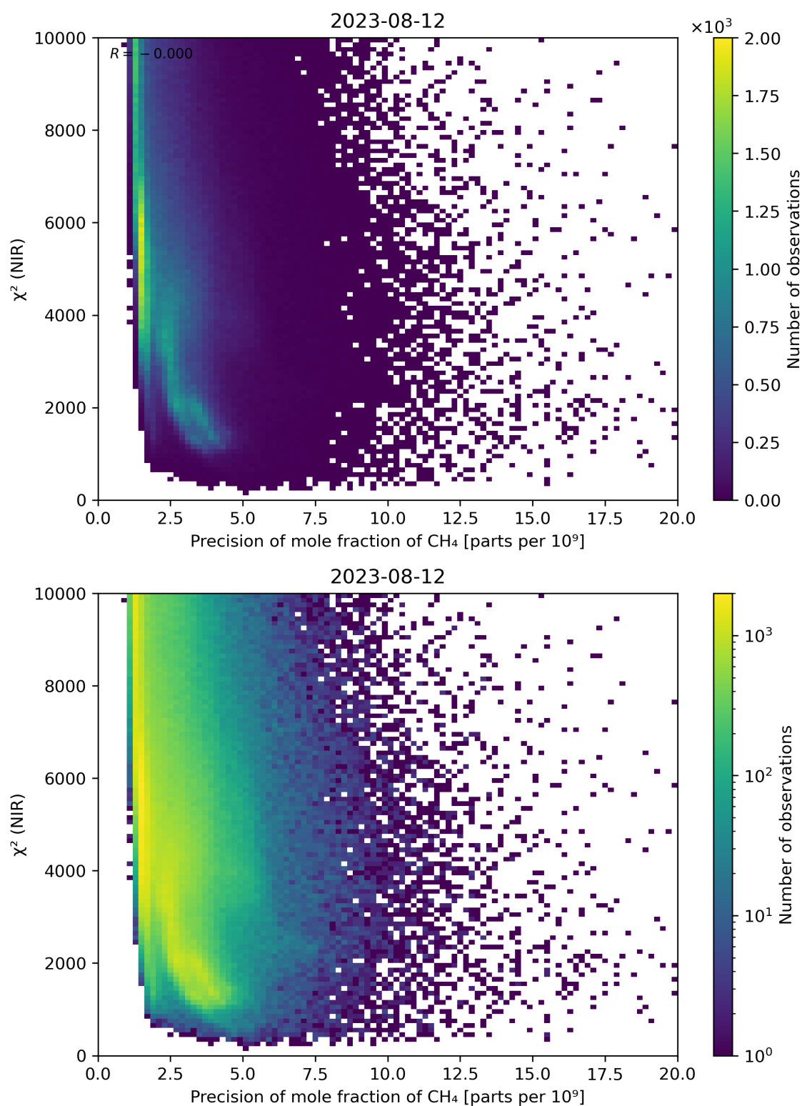
Figure 78: Scatter density plot of “Precision of mole fraction of CH 4 ” against “ \chi^2 (NIR)” for 2023-08-11 to 2023-08-13.
