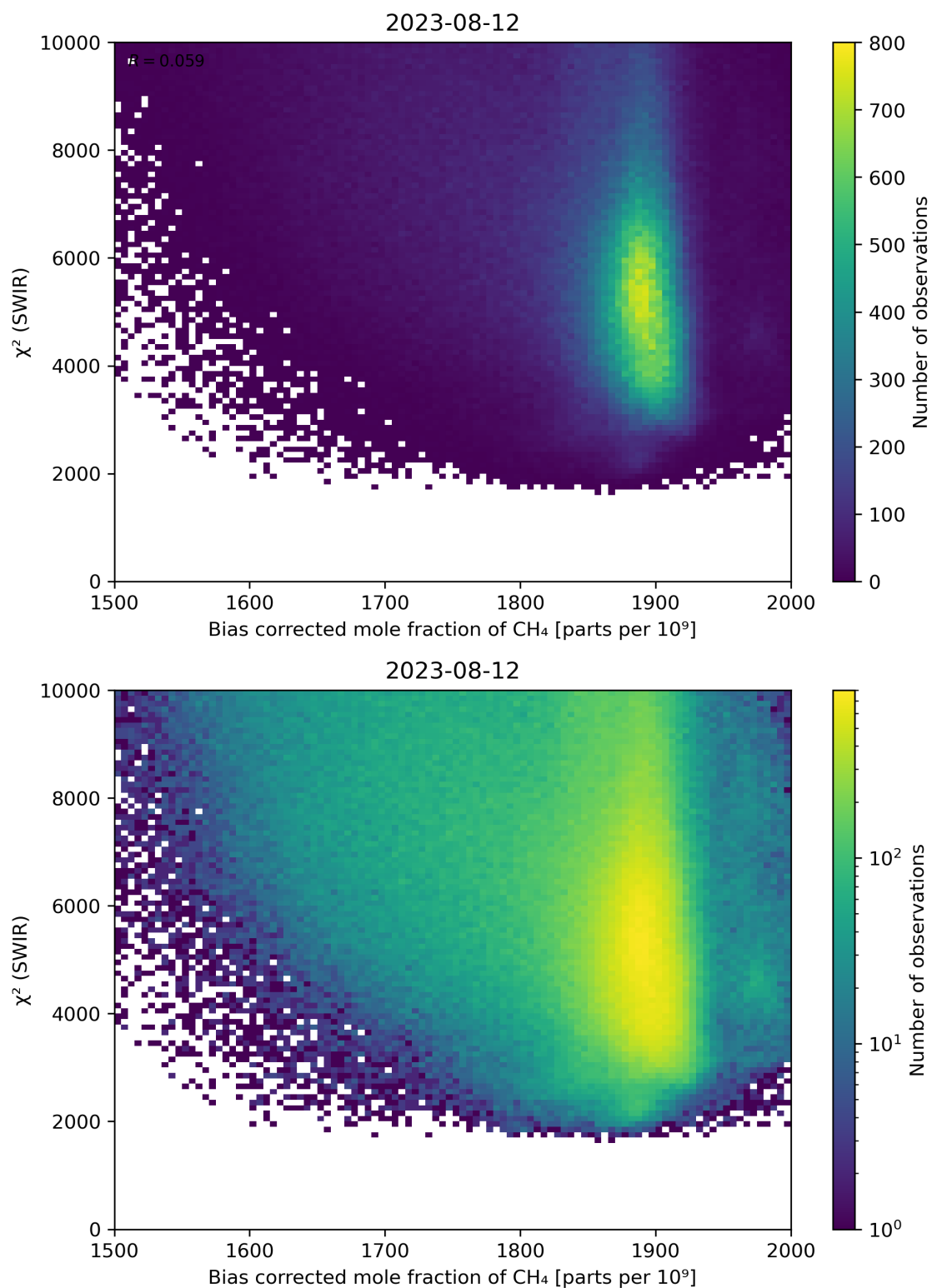
Figure 64: Scatter density plot of “Bias corrected mole fraction of CH 4 ” against “ \chi^2 (SWIR)” for 2023-08-11 to 2023-08-13.
