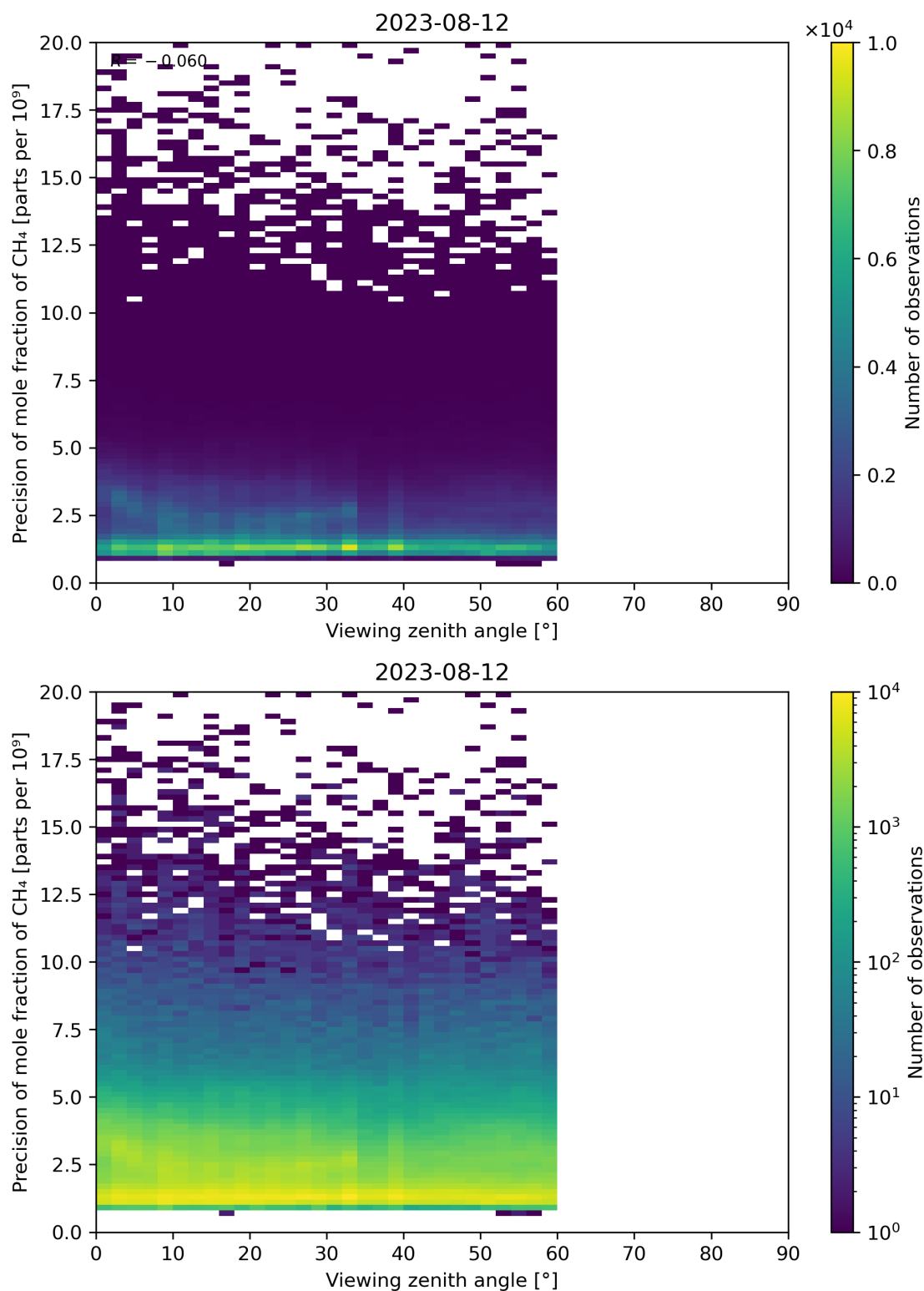
Figure 112: Scatter density plot of “Viewing zenith angle” against “Precision of mole fraction of CH 4 ” for 2023-08-11 to 2023-08-13.
