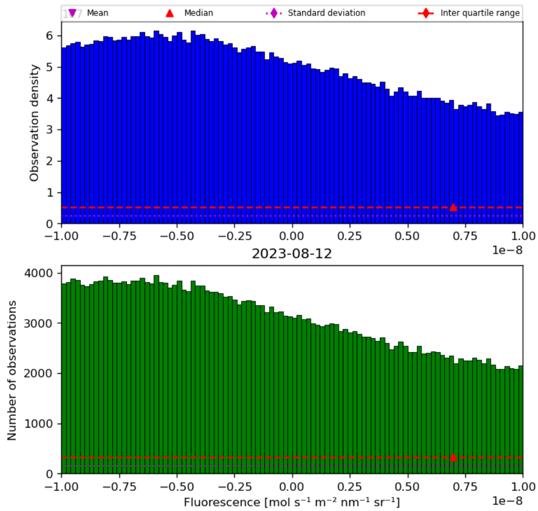
Figure 32: Histogram of “Fluorescence” for 2023-08-11 to 2023-08-13
