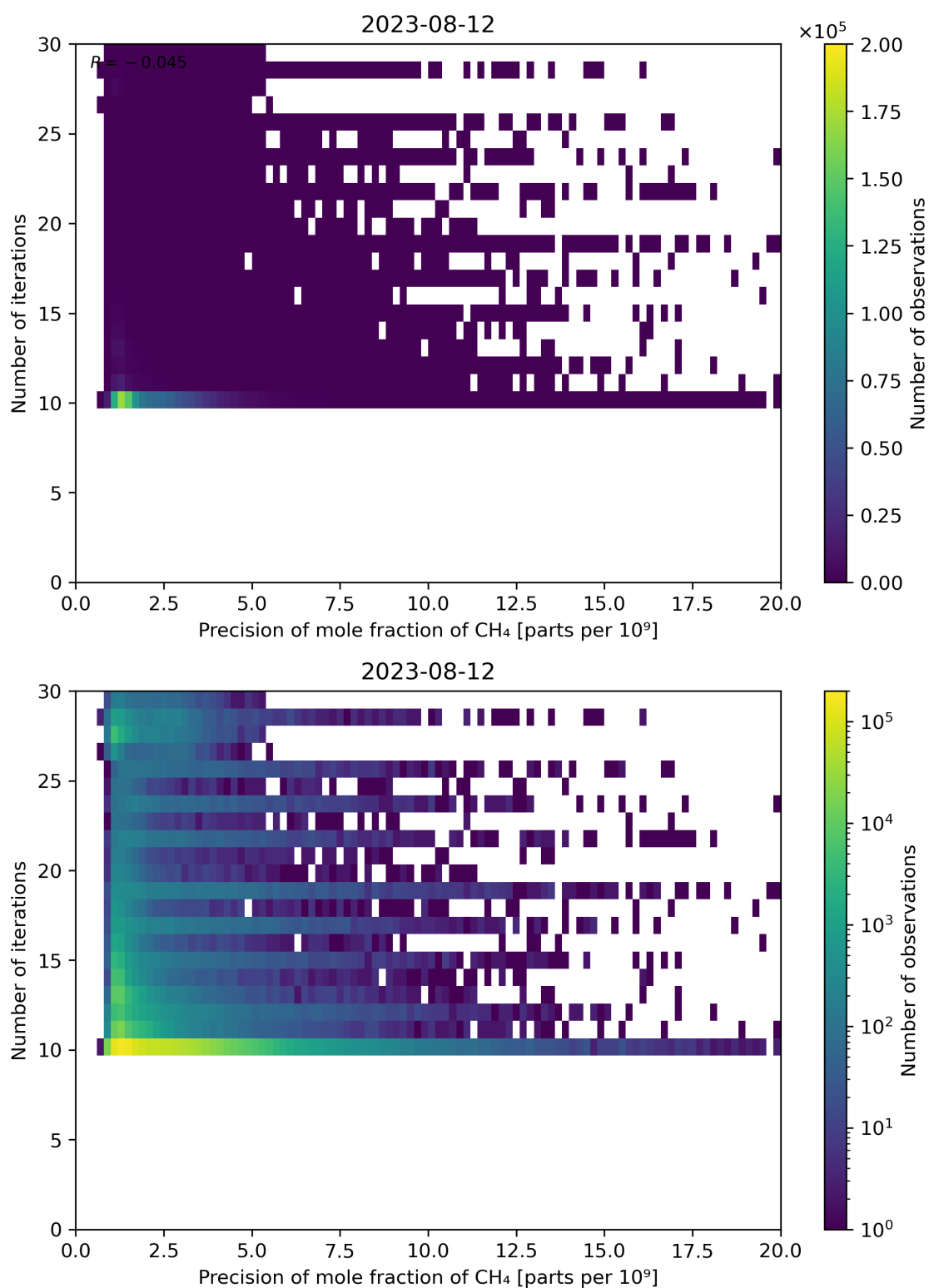
Figure 83: Scatter density plot of “Precision of mole fraction of CH 4 ” against “Number of iterations” for 2023-08-11 to 2023-08-13.
