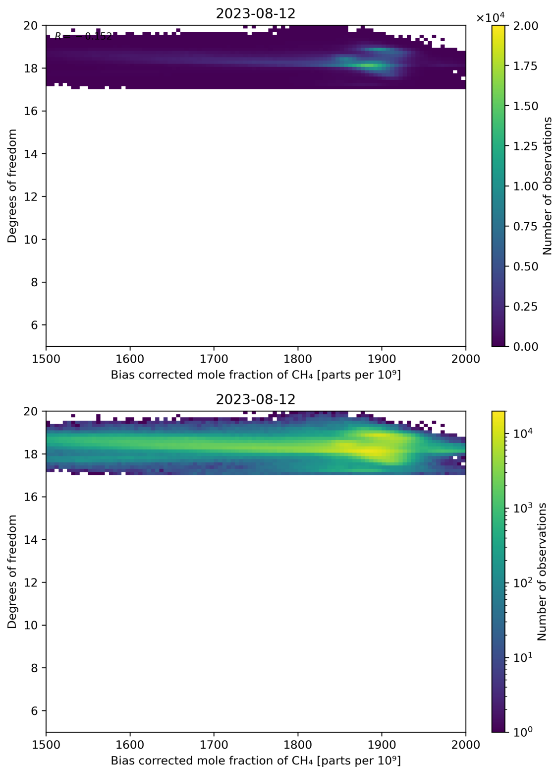
Figure 65: Scatter density plot of “Bias corrected mole fraction of CH 4 ” against “Degrees of freedom” for 2023-08-11 to 2023-08-13.
