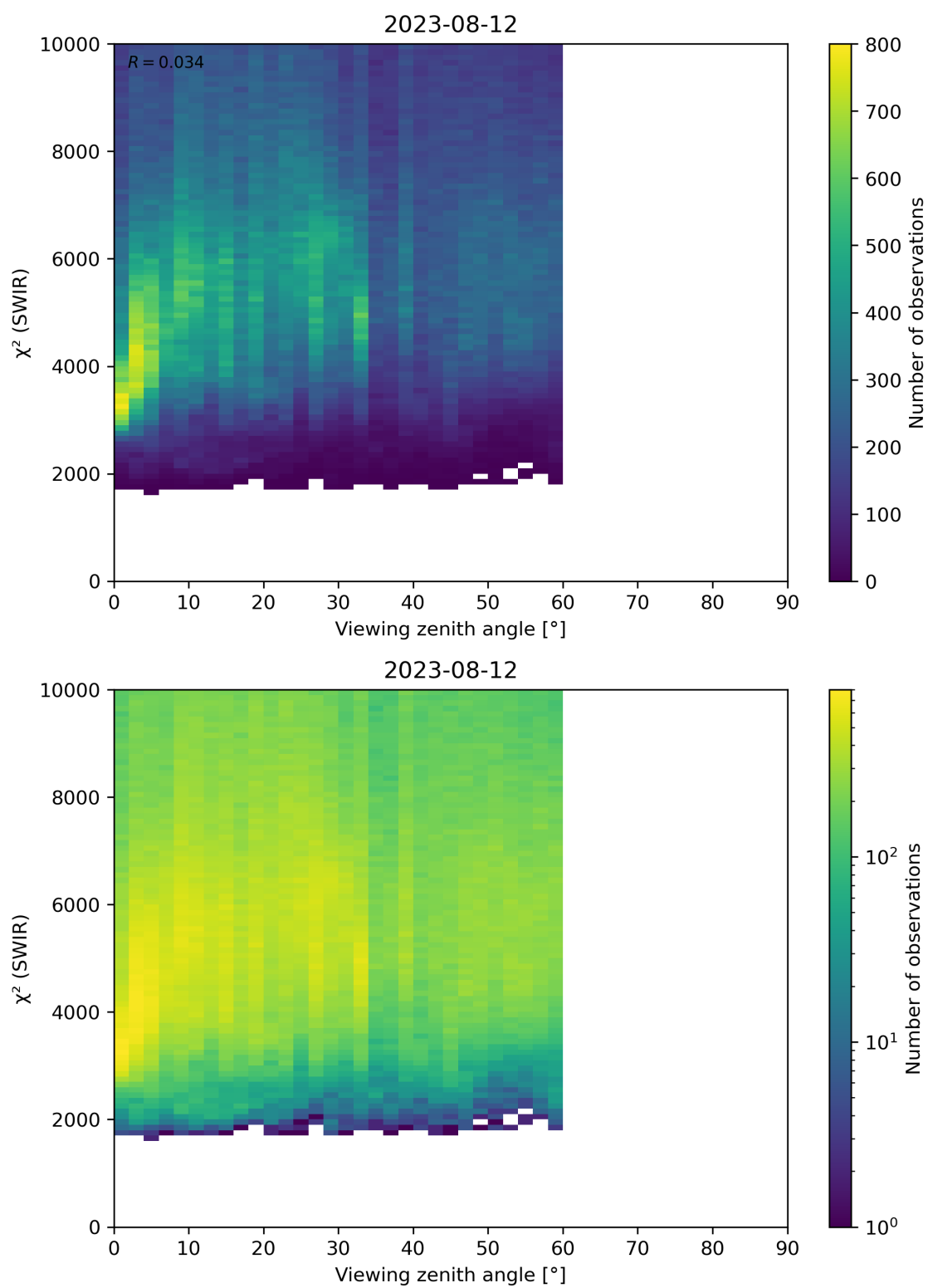
Figure 106: Scatter density plot of “Viewing zenith angle” against “ \chi^2 (SWIR)” for 2023-08-11 to 2023-08-13.
