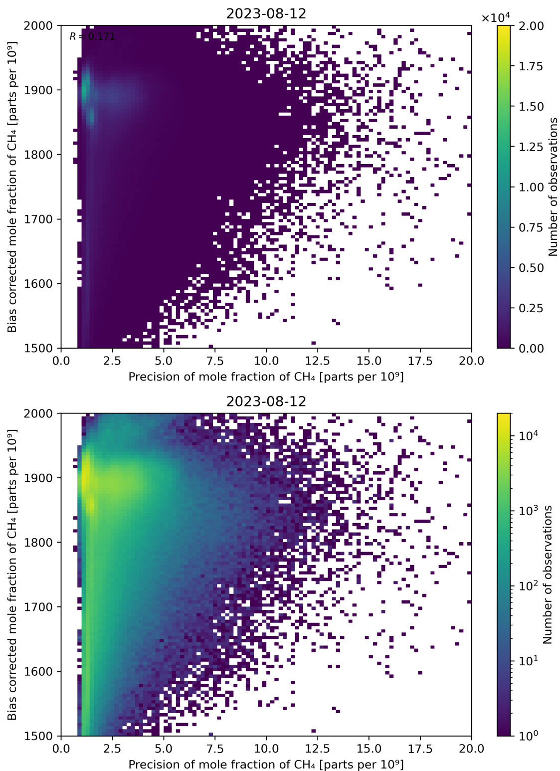
Figure 82: Scatter density plot of “Precision of mole fraction of CH 4 ” against “Bias corrected mole fraction of CH 4 ” for 2023-08-11 to 2023-08-13.
