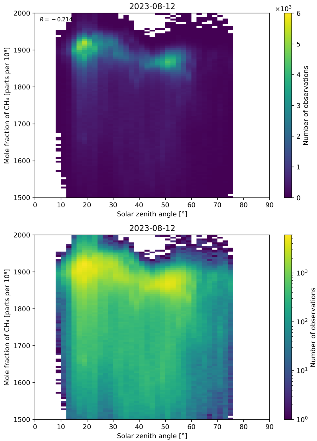
Figure 99: Scatter density plot of “Solar zenith angle” against “Mole fraction of CH 4 ” for 2023-08-11 to 2023-08-13.
