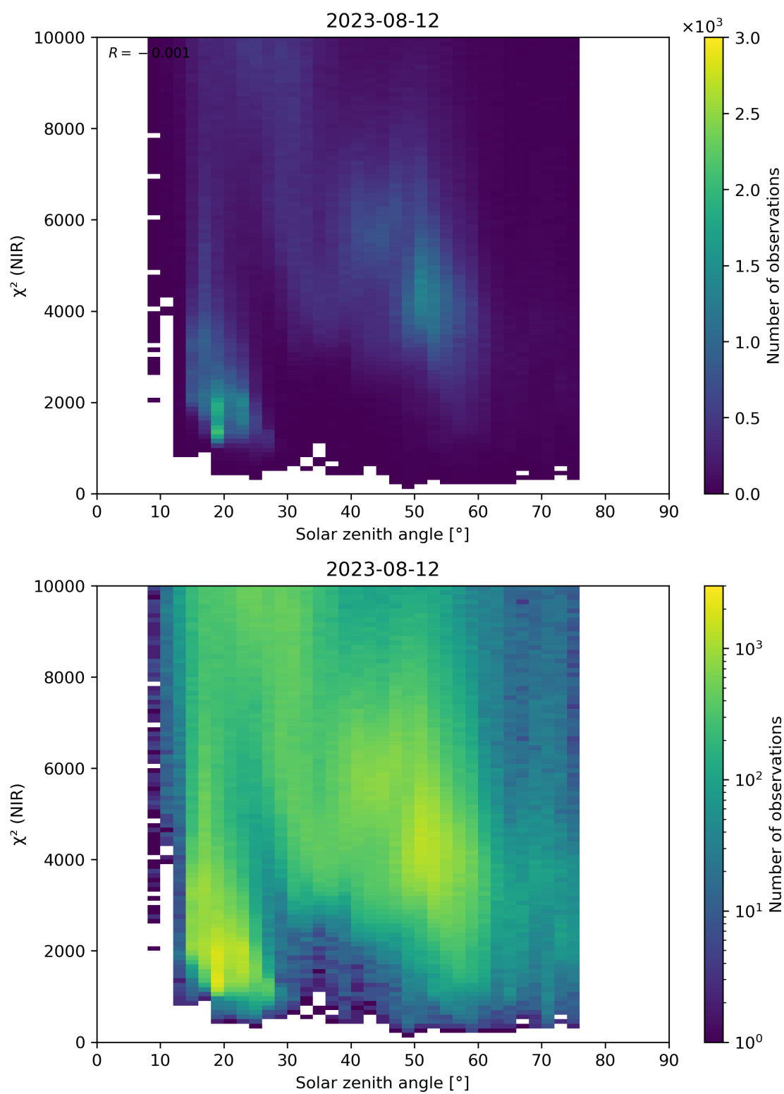
Figure 94: Scatter density plot of “Solar zenith angle” against “ \chi^2 (NIR)” for 2023-08-11 to 2023-08-13.
