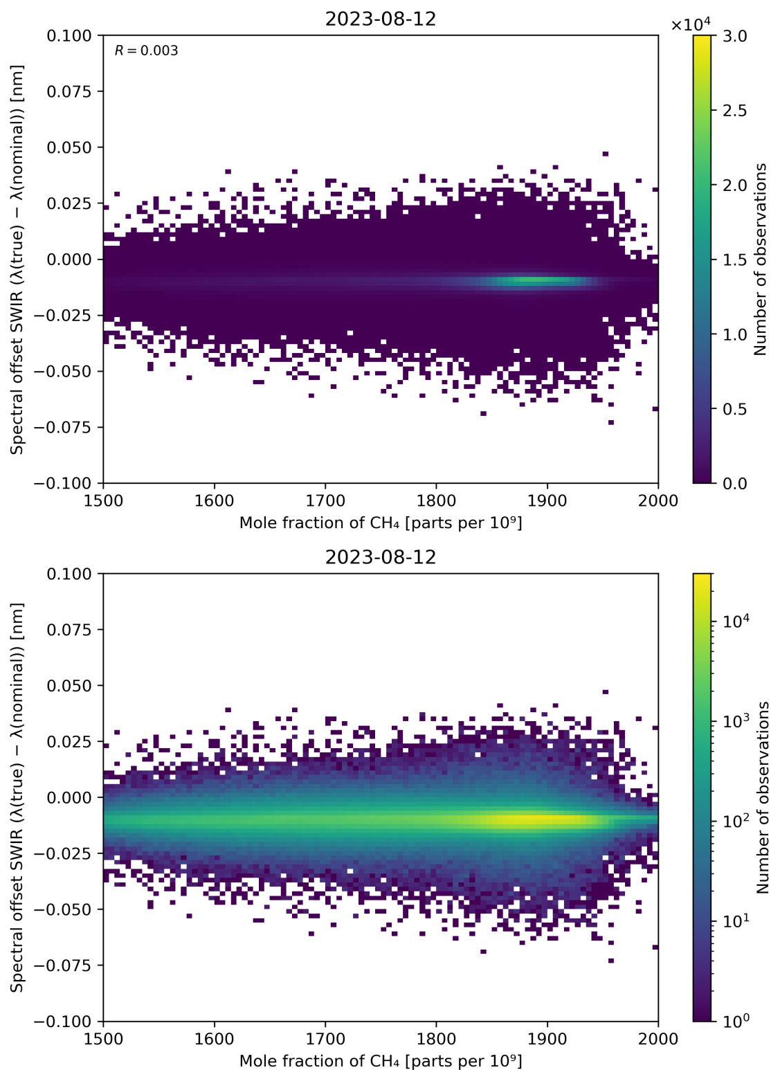
Figure 86: Scatter density plot of “Mole fraction of CH 4 ” against “Spectral offset SWIR ( \lambda(\text{true}) - \lambda(\text{nominal}) )” for 2023-08-11 to 2023-08-13.
