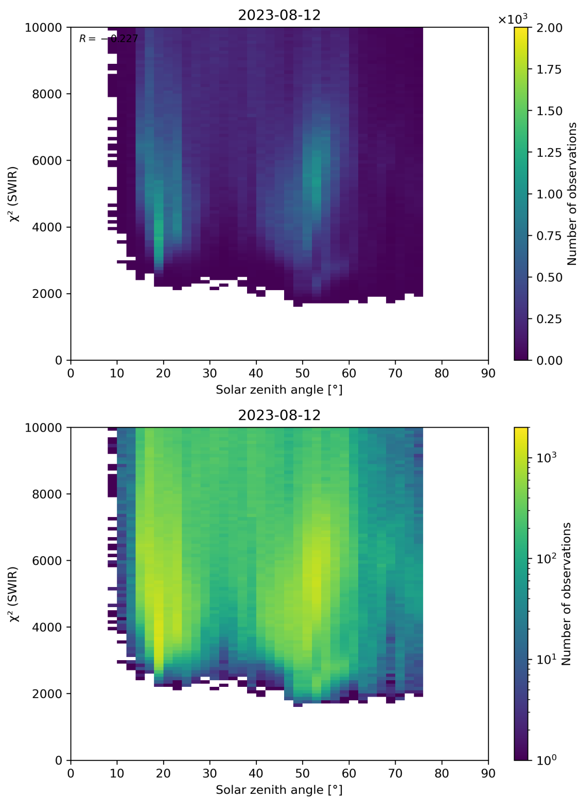
Figure 95: Scatter density plot of “Solar zenith angle” against “ \chi^2 (SWIR)” for 2023-08-11 to 2023-08-13.
