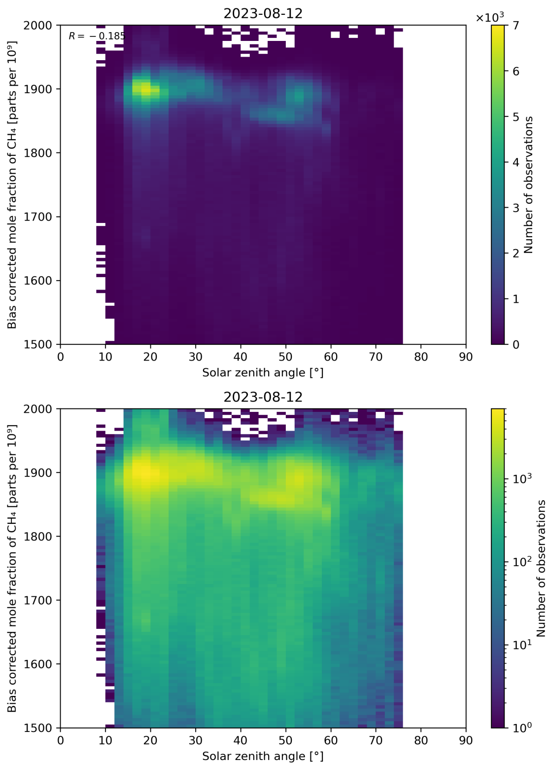
Figure 100: Scatter density plot of “Solar zenith angle” against “Bias corrected mole fraction of CH 4 ” for 2023-08-11 to 2023-08-13.
