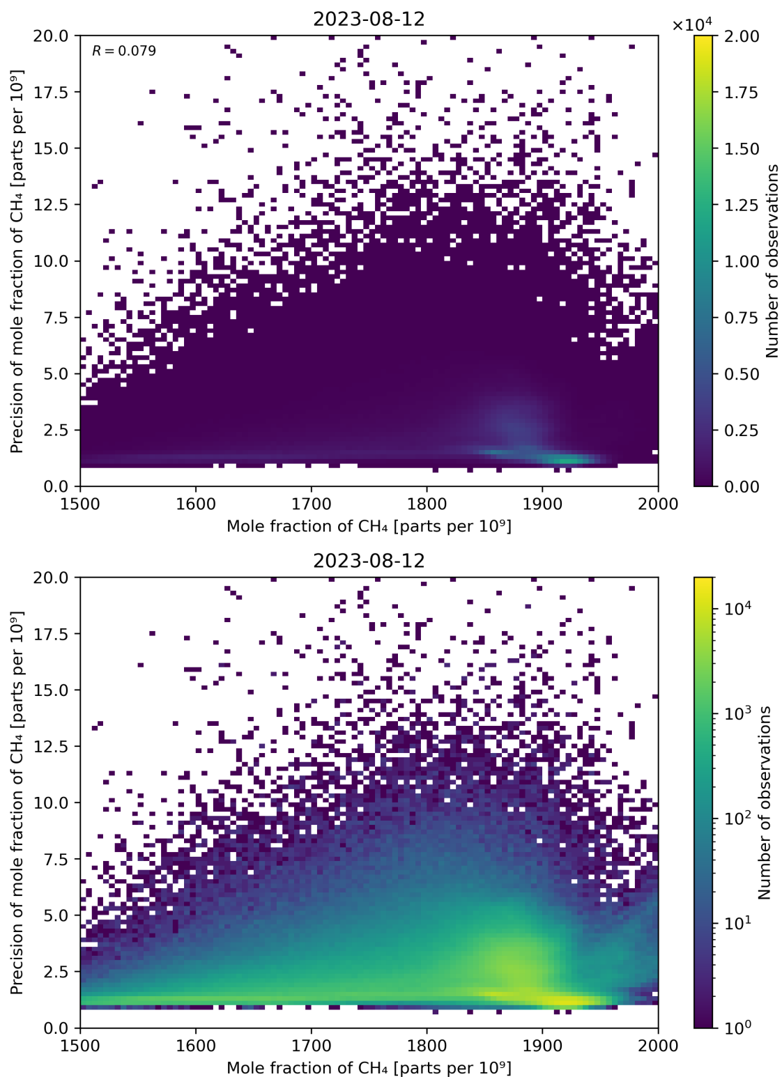
Figure 75: Scatter density plot of “Mole fraction of CH 4 ” against “Precision of mole fraction of CH 4 ” for 2023-08-11 to 2023-08-13.
