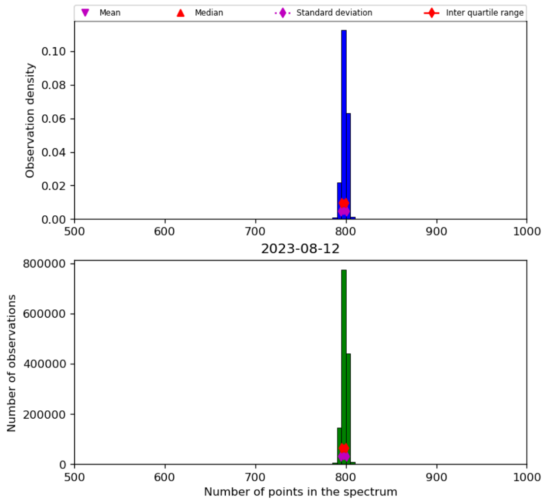
Figure 26: Histogram of “Number of points in the spectrum” for 2023-08-11 to 2023-08-13
