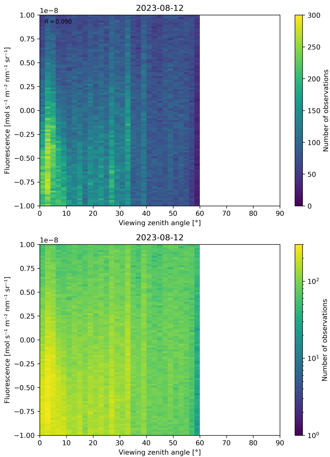
Figure 108: Scatter density plot of “Viewing zenith angle” against “Fluorescence” for 2023-08-11 to 2023-08-13.
