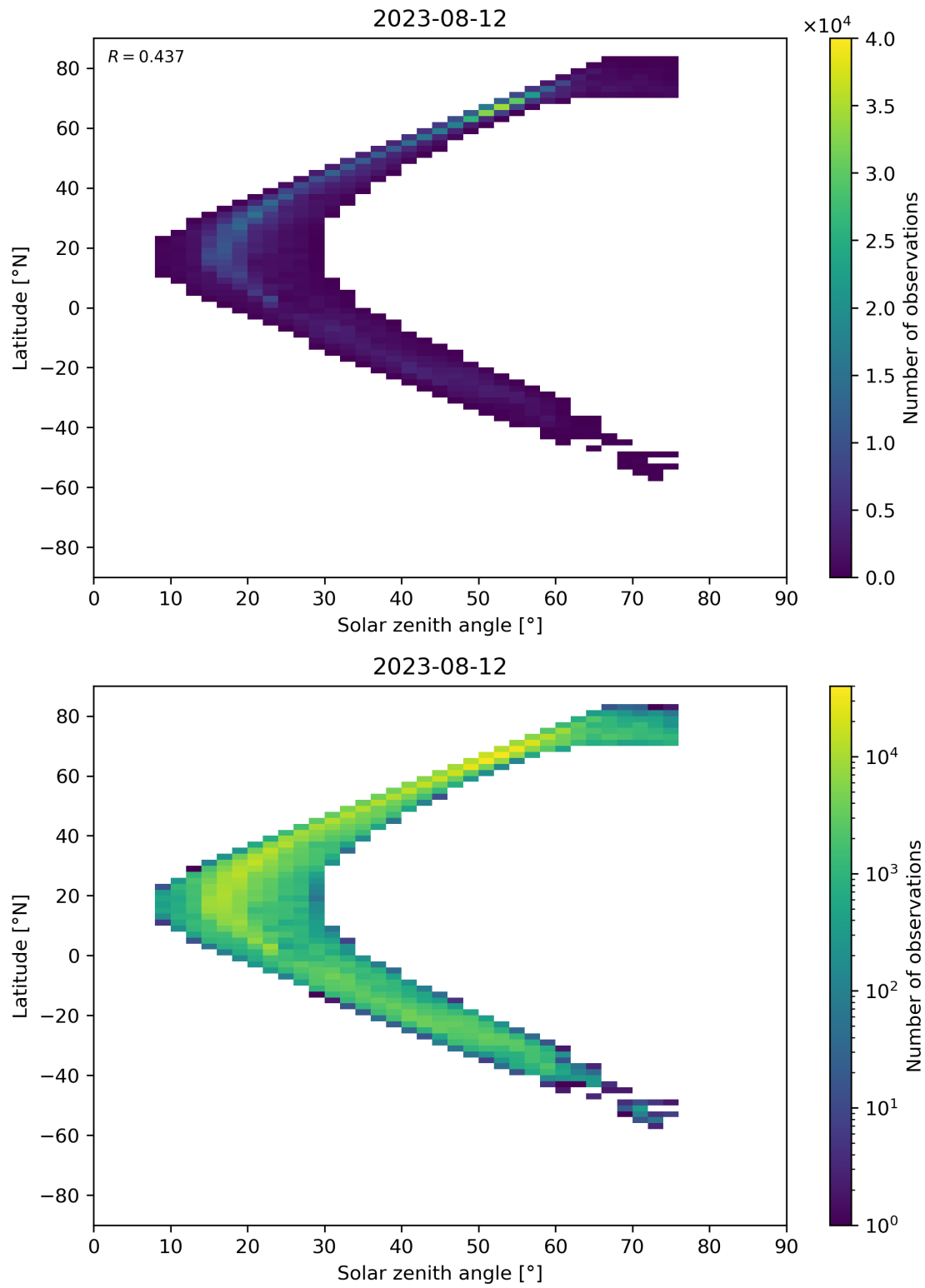
Figure 98: Scatter density plot of “Solar zenith angle” against “Latitude” for 2023-08-11 to 2023-08-13.
