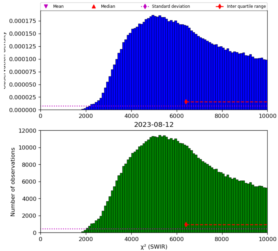
Figure 28: Histogram of “ \chi^2 (SWIR)” for 2023-08-11 to 2023-08-13
