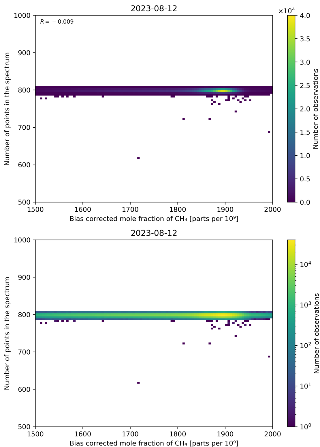
Figure 68: Scatter density plot of “Bias corrected mole fraction of CH 4 ” against “Number of points in the spectrum” for 2023-08-11 to 2023-08-13.
