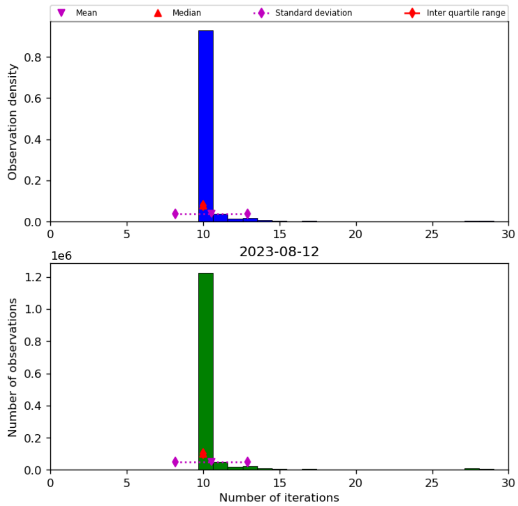
Figure 31: Histogram of “Number of iterations” for 2023-08-11 to 2023-08-13
