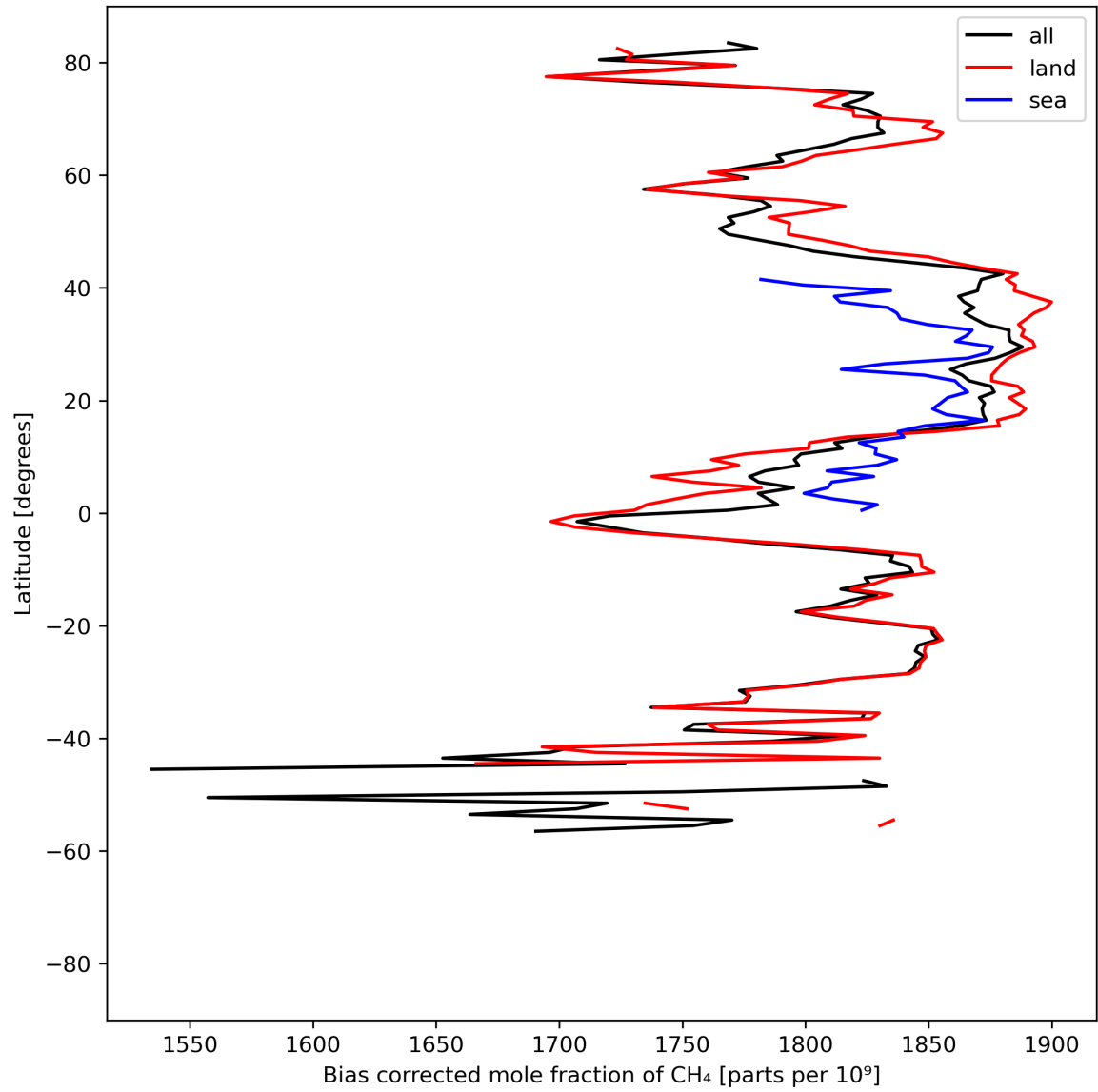
Figure 14: Zonal average of “Bias corrected mole fraction of \text{CH}_4 ” for 2023-08-11 to 2023-08-13.
