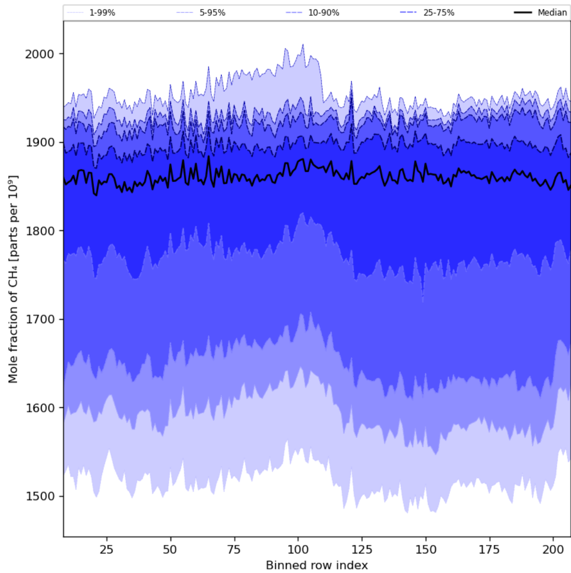
Figure 34: Along track statistics of “Mole fraction of CH 4 ” for 2023-08-11 to 2023-08-13
