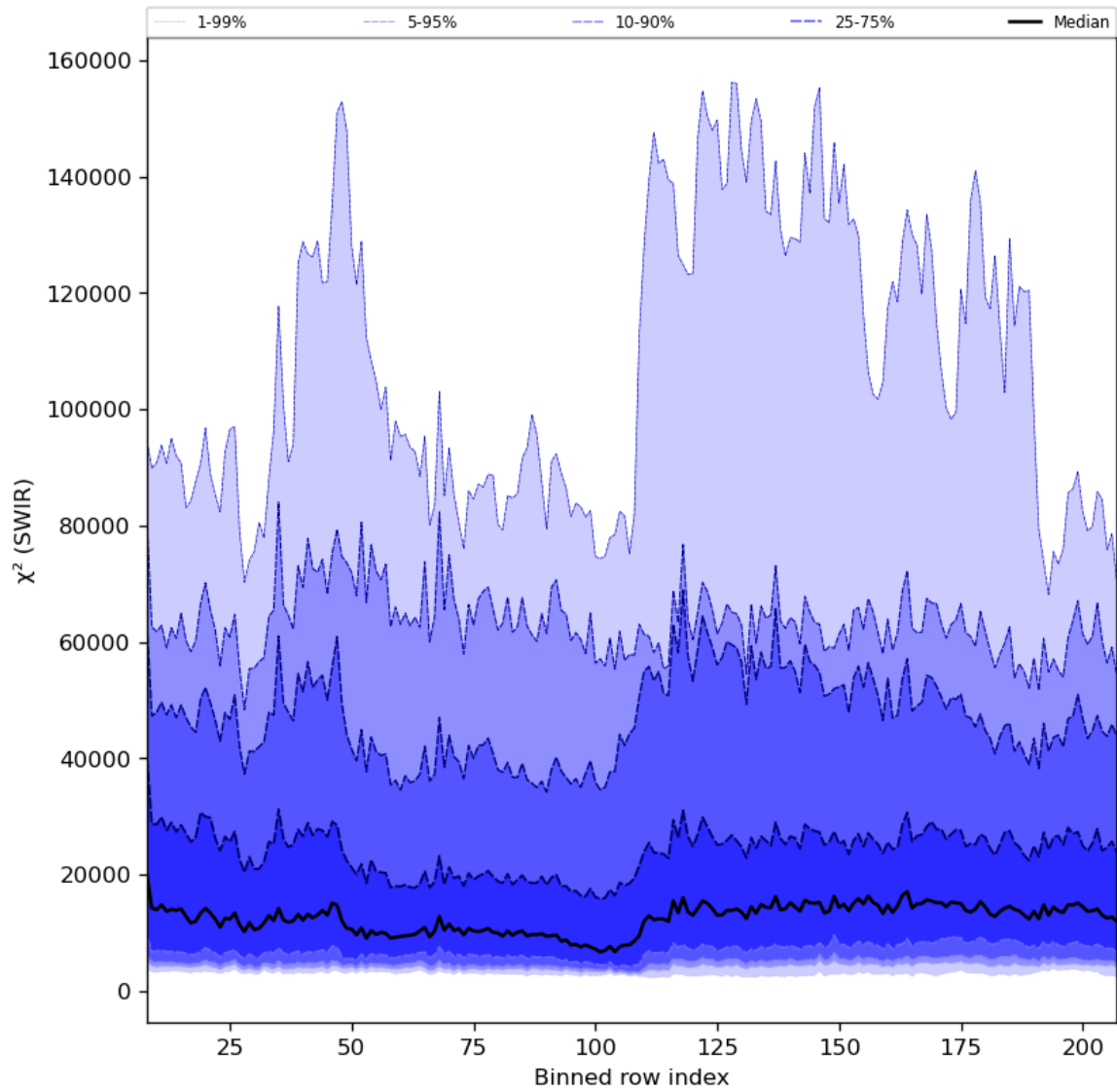
Figure 39: Along track statistics of “ \chi^2 (SWIR)” for 2023-08-11 to 2023-08-13
