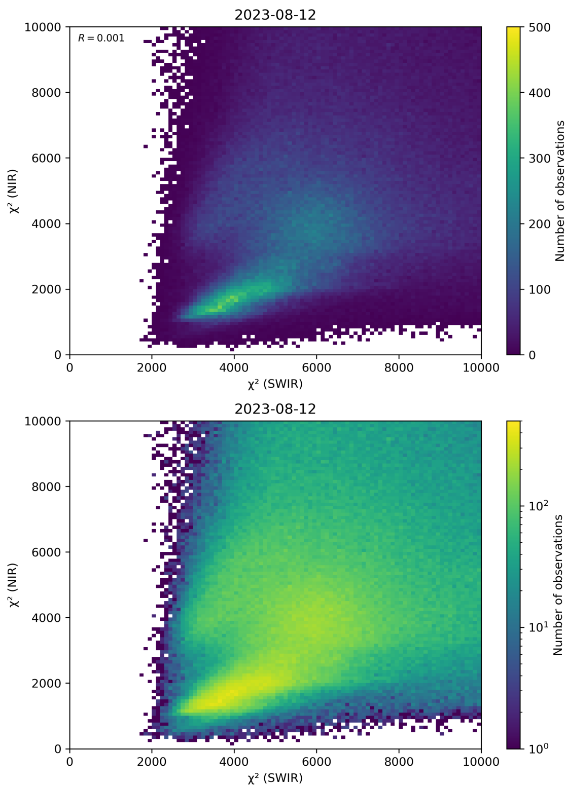
Figure 47: Scatter density plot of “ \chi^2 (SWIR)” against “ \chi^2 (NIR)” for 2023-08-11 to 2023-08-13.
