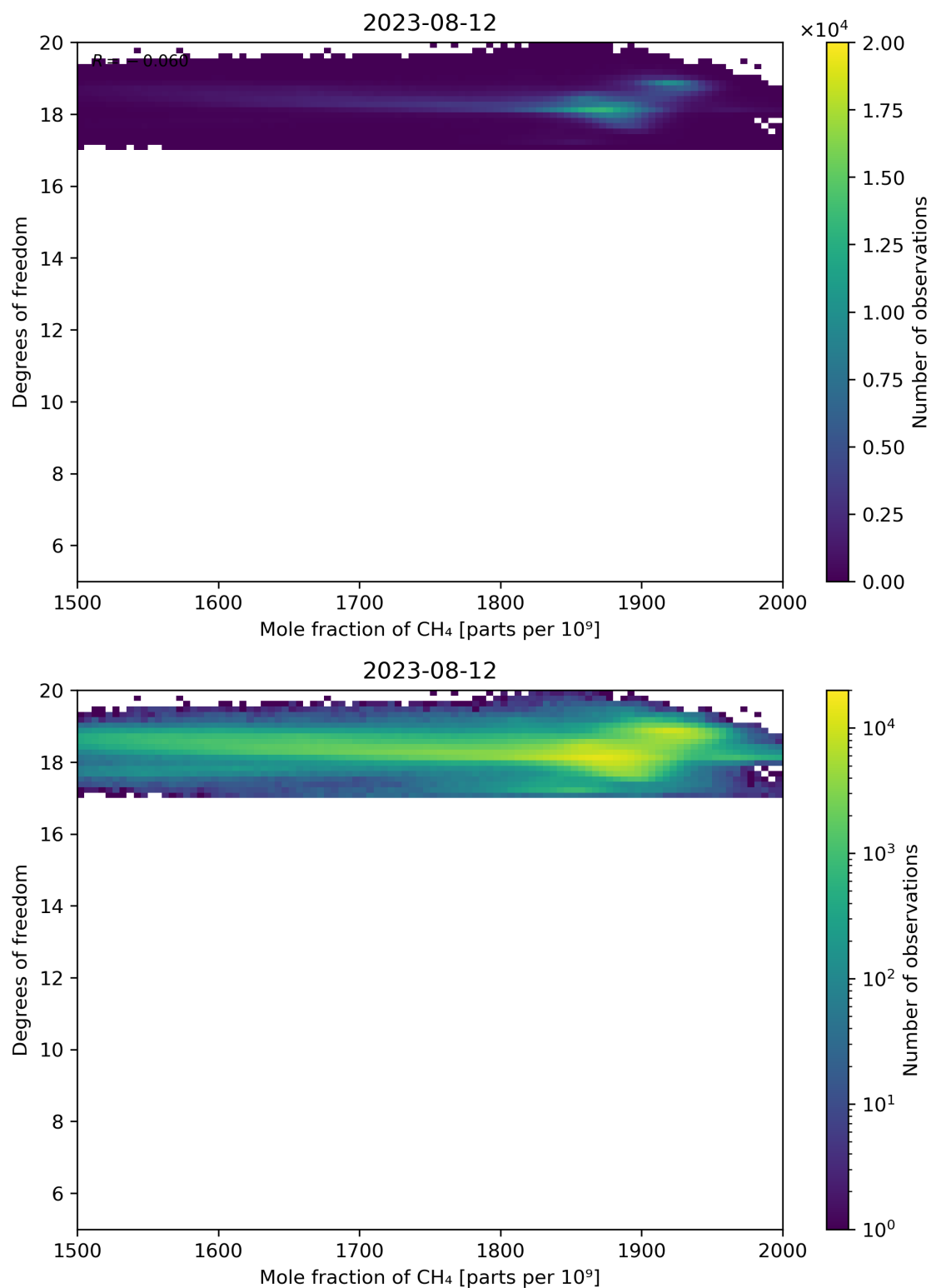
Figure 72: Scatter density plot of “Mole fraction of CH 4 ” against “Degrees of freedom” for 2023-08-11 to 2023-08-13.
