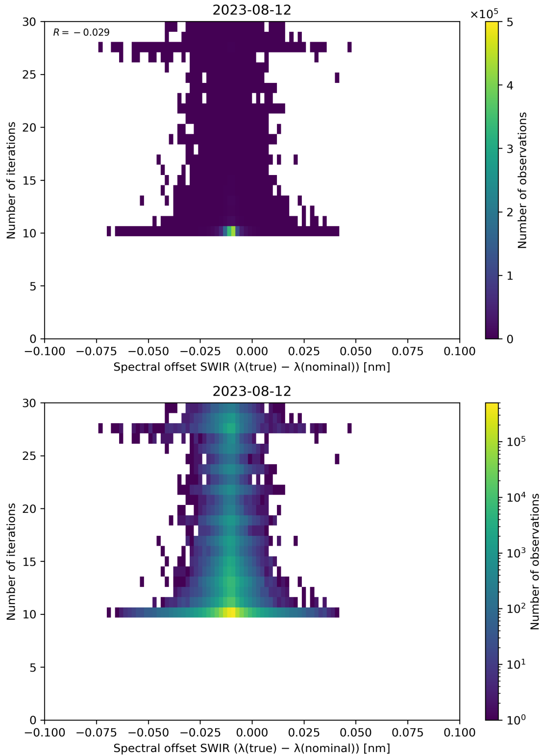
Figure 121: Scatter density plot of “Spectral offset SWIR ( \lambda(\text{true}) - \lambda(\text{nominal}) )” against “Number of iterations” for 2023-08-11 to 2023-08-13.
