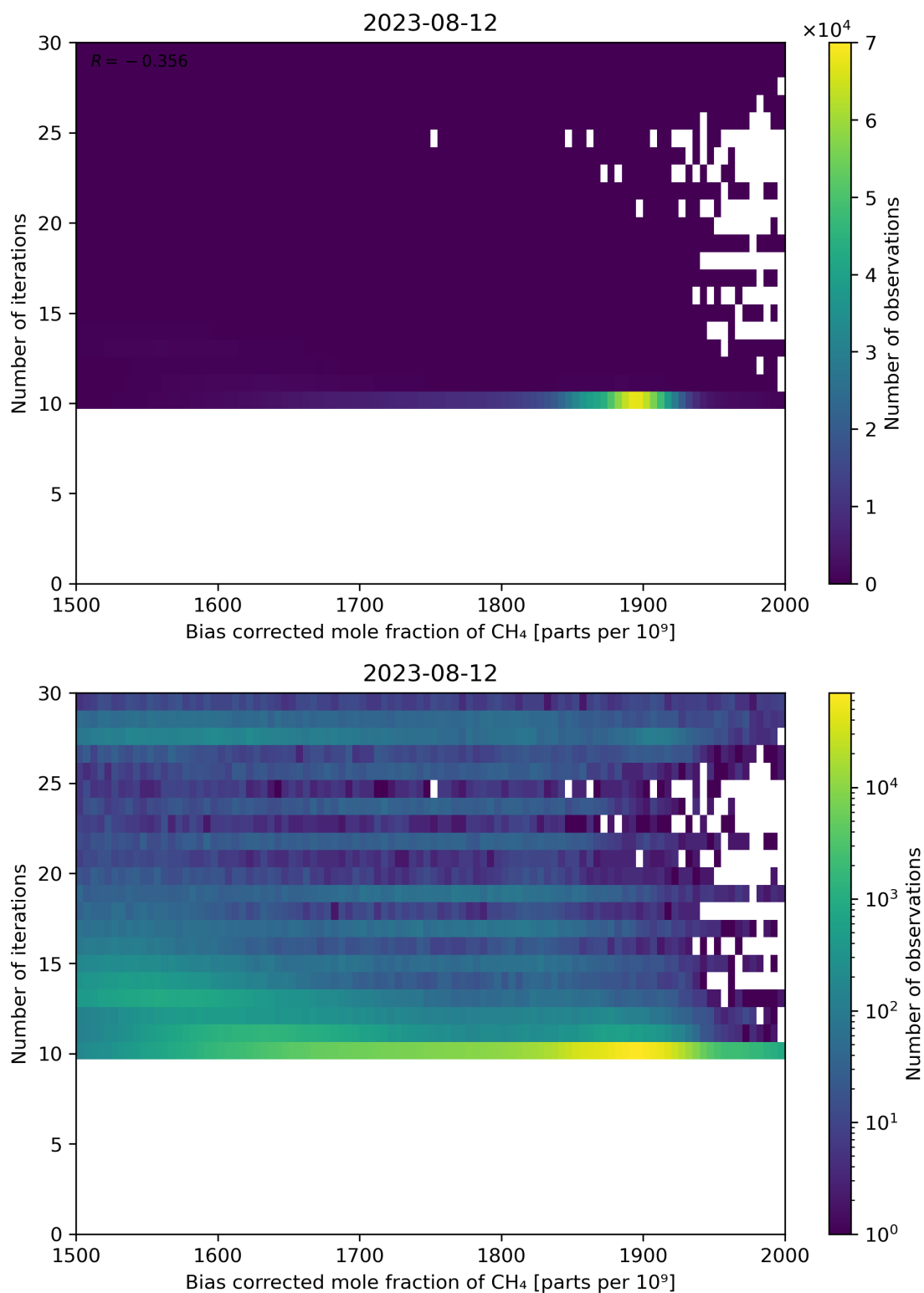
Figure 67: Scatter density plot of “Bias corrected mole fraction of \text{CH}_4 ” against “Number of iterations” for 2023-08-11 to 2023-08-13.
