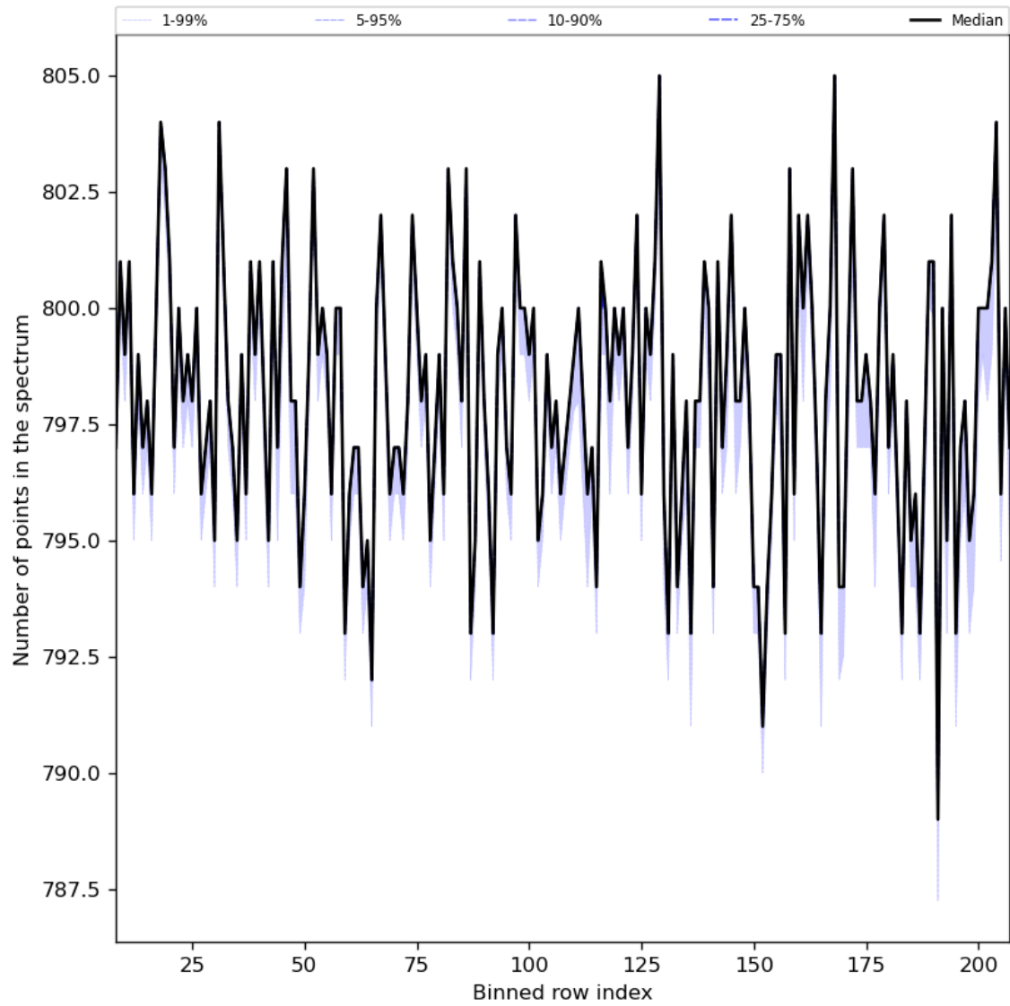
Figure 37: Along track statistics of “Number of points in the spectrum” for 2023-08-11 to 2023-08-13
