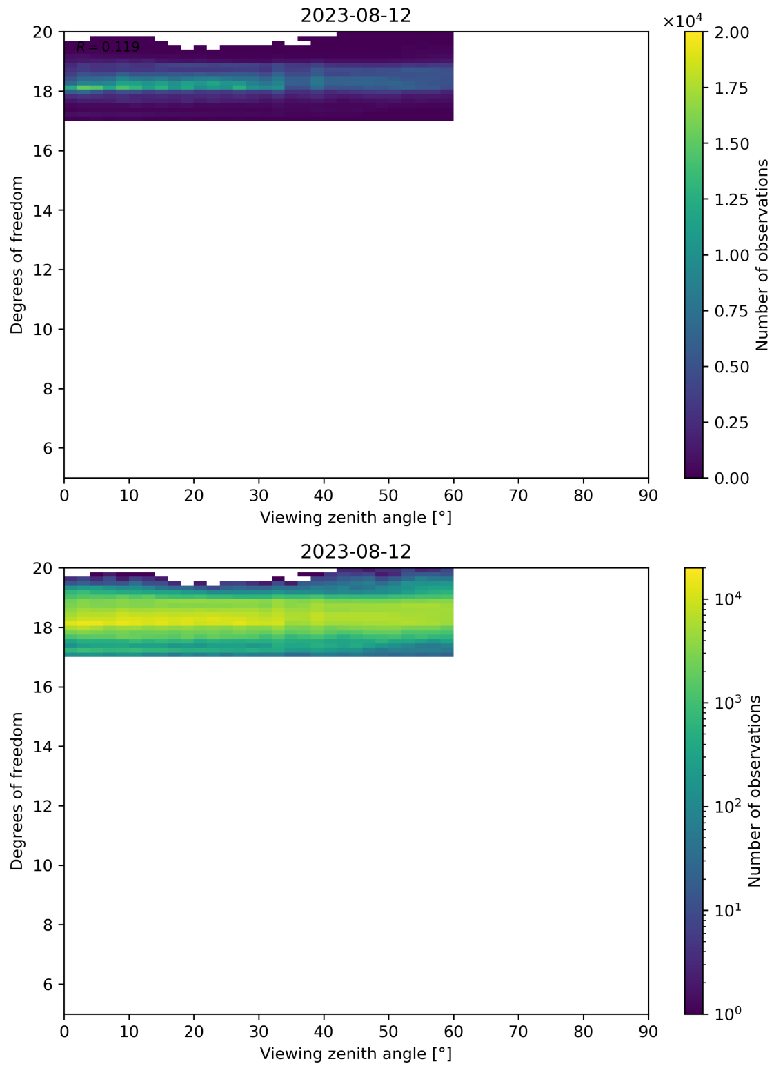
Figure 107: Scatter density plot of “Viewing zenith angle” against “Degrees of freedom” for 2023-08-11 to 2023-08-13.
