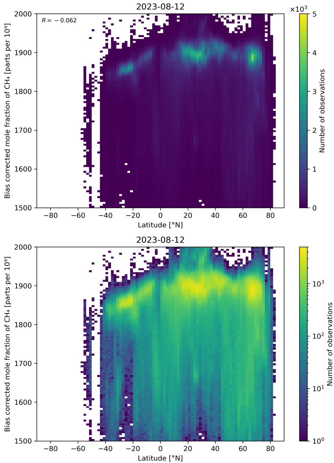
Figure 58: Scatter density plot of “Latitude” against “Bias corrected mole fraction of \text{CH}_4 ” for 2023-08-11 to 2023-08-13.
