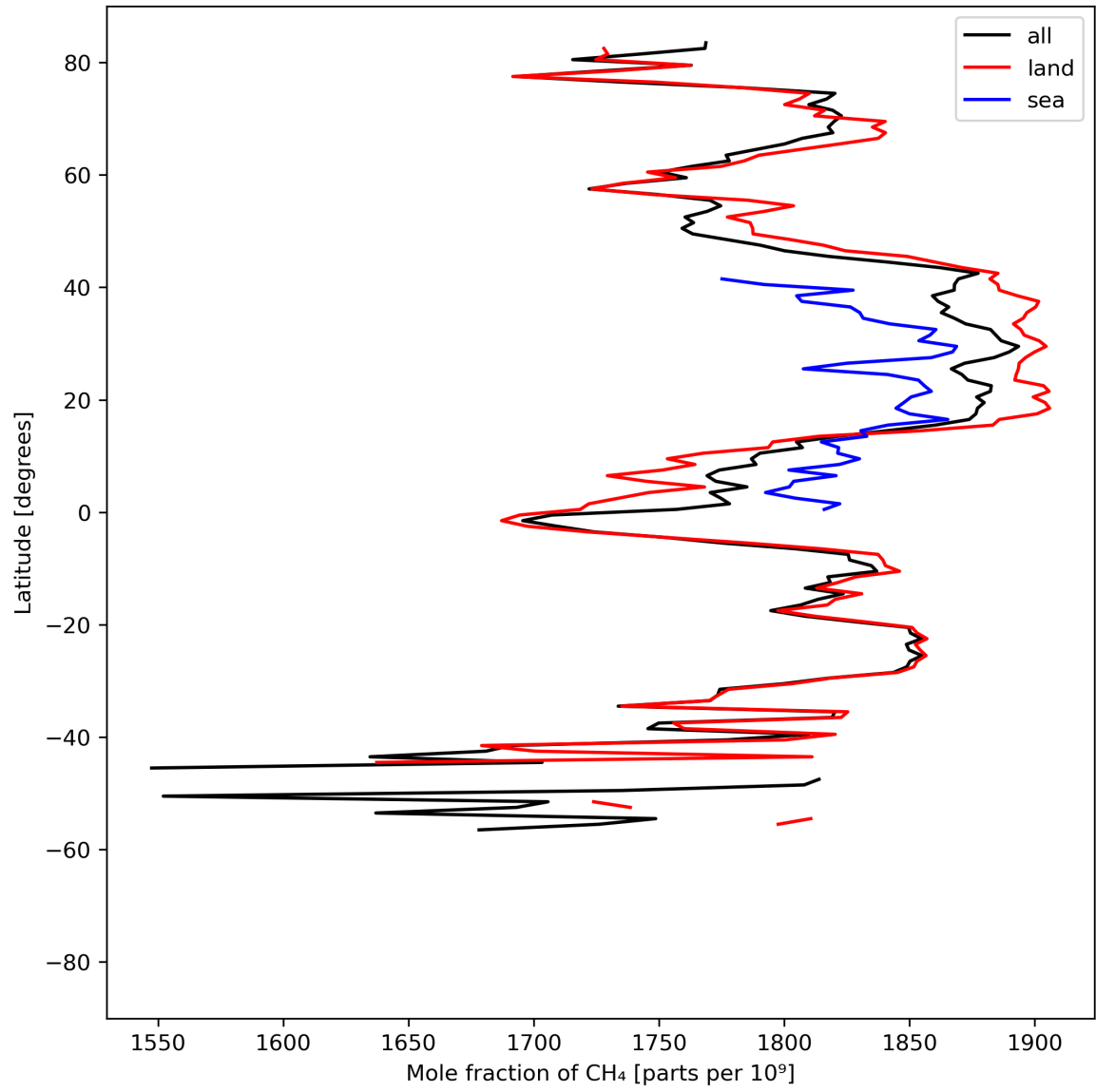
Figure 12: Zonal average of “Mole fraction of \text{CH}_4 ” for 2023-08-11 to 2023-08-13.
