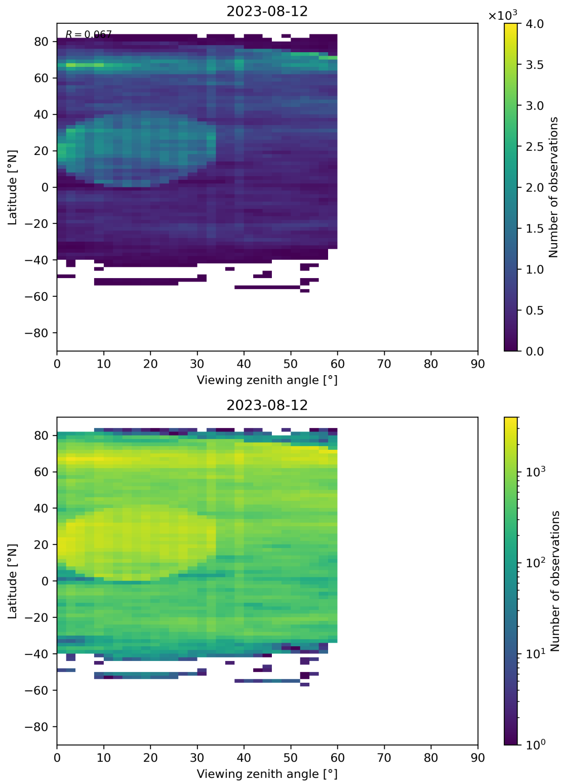
Figure 109: Scatter density plot of “Viewing zenith angle” against “Latitude” for 2023-08-11 to 2023-08-13.
