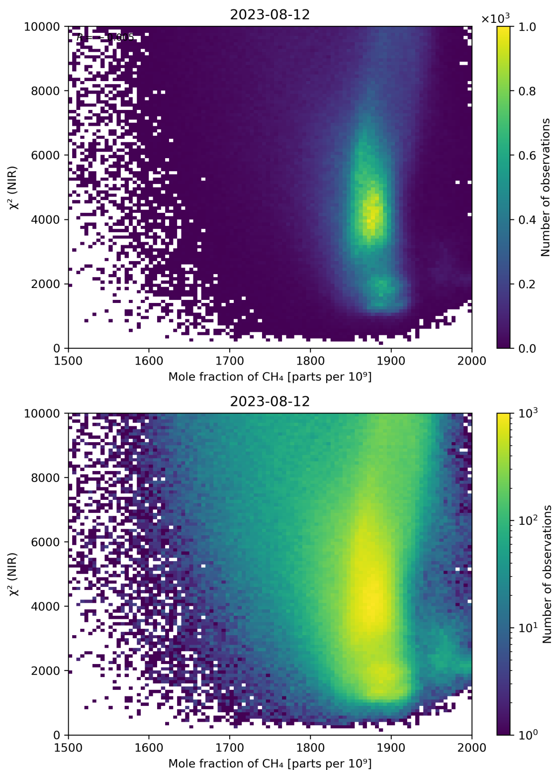
Figure 70: Scatter density plot of “Mole fraction of \text{CH}_4 ” against “ \chi^2 (NIR)” for 2023-08-11 to 2023-08-13.
