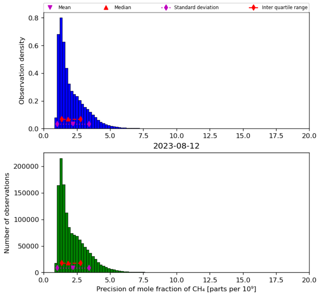
Figure 24: Histogram of “Precision of mole fraction of CH 4 ” for 2023-08-11 to 2023-08-13
