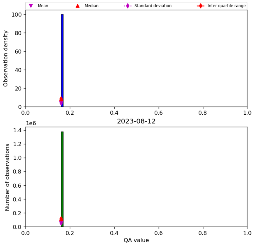
Figure 22: Histogram of “QA value” for 2023-08-11 to 2023-08-13
