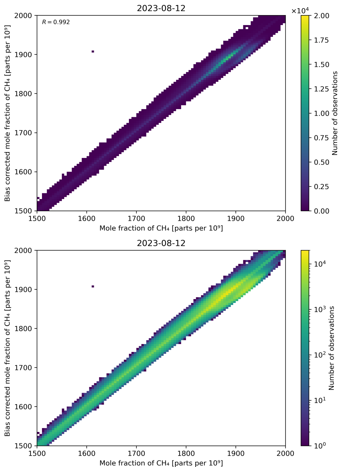
Figure 74: Scatter density plot of “Mole fraction of CH 4 ” against “Bias corrected mole fraction of CH 4 ” for 2023-08-11 to 2023-08-13.
