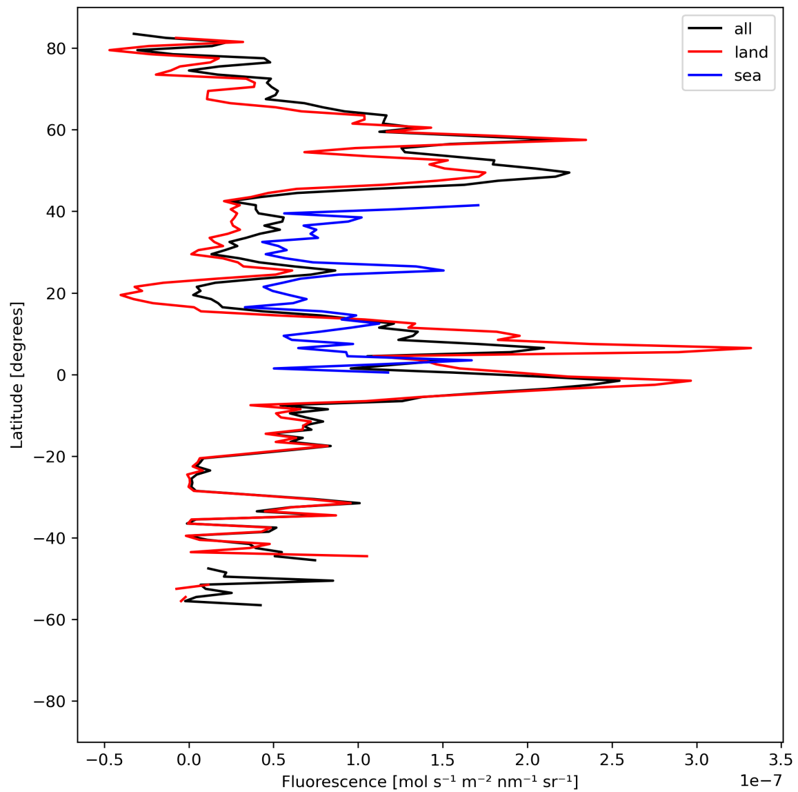
Figure 21: Zonal average of “Fluorescence” for 2023-08-11 to 2023-08-13.
