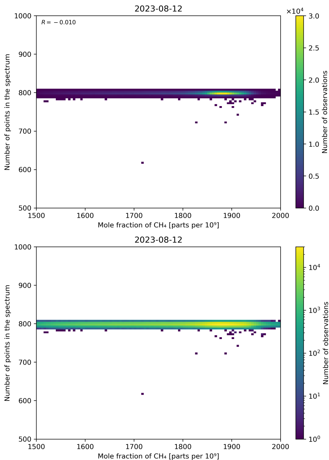
Figure 77: Scatter density plot of “Mole fraction of CH 4 ” against “Number of points in the spectrum” for 2023-08-11 to 2023-08-13.
