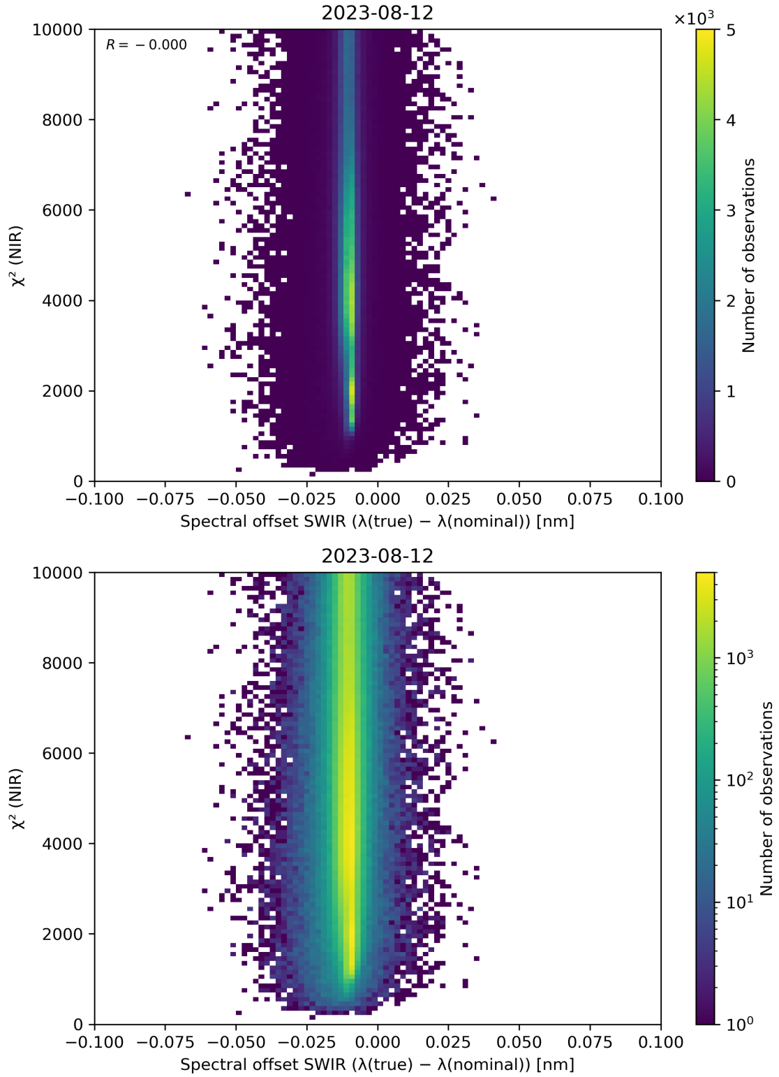
Figure 117: Scatter density plot of “Spectral offset SWIR ( \lambda(\text{true}) - \lambda(\text{nominal}) )” against “ \chi^2 (NIR)” for 2023-08-11 to 2023-08-13.
