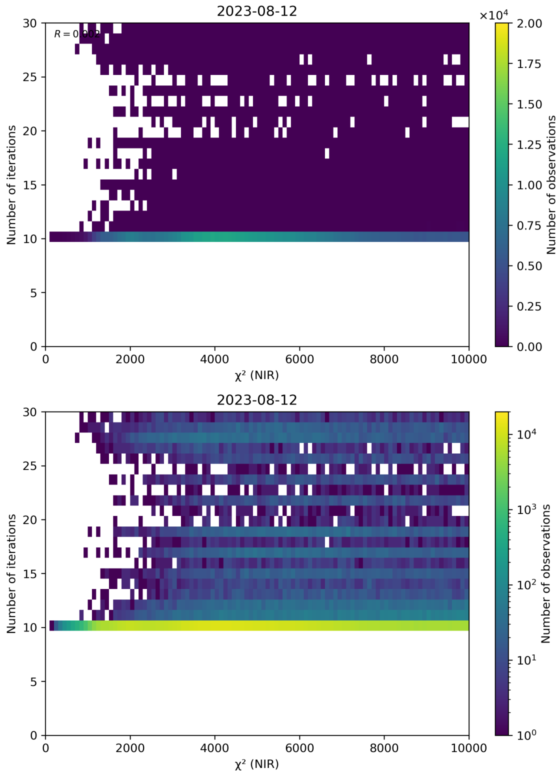
Figure 46: Scatter density plot of “ \chi^2 (NIR)” against “Number of iterations” for 2023-08-11 to 2023-08-13.
