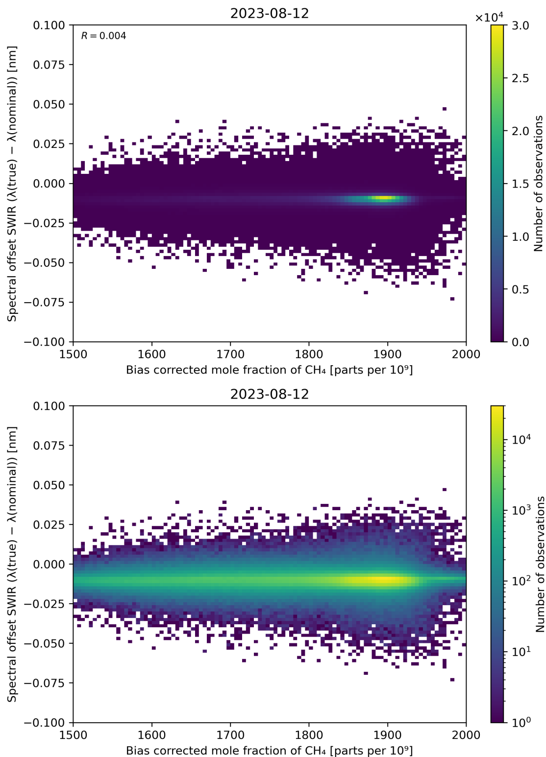
Figure 69: Scatter density plot of “Bias corrected mole fraction of \text{CH}_4 ” against “Spectral offset SWIR ( \lambda(\text{true}) - \lambda(\text{nominal}) )” for 2023-08-11 to 2023-08-13.
