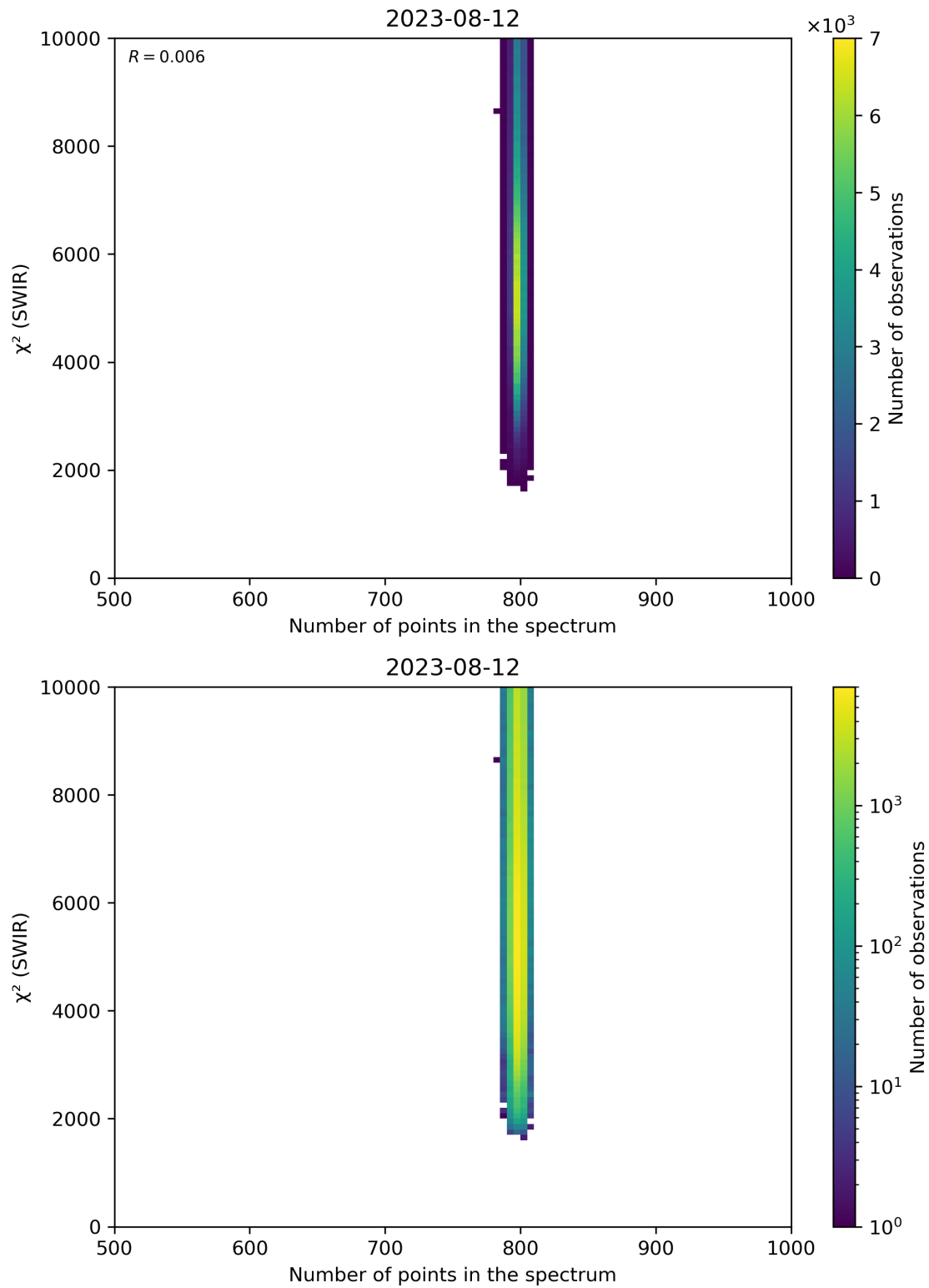
Figure 89: Scatter density plot of “Number of points in the spectrum” against “ \chi^2 (SWIR)” for 2023-08-11 to 2023-08-13.
