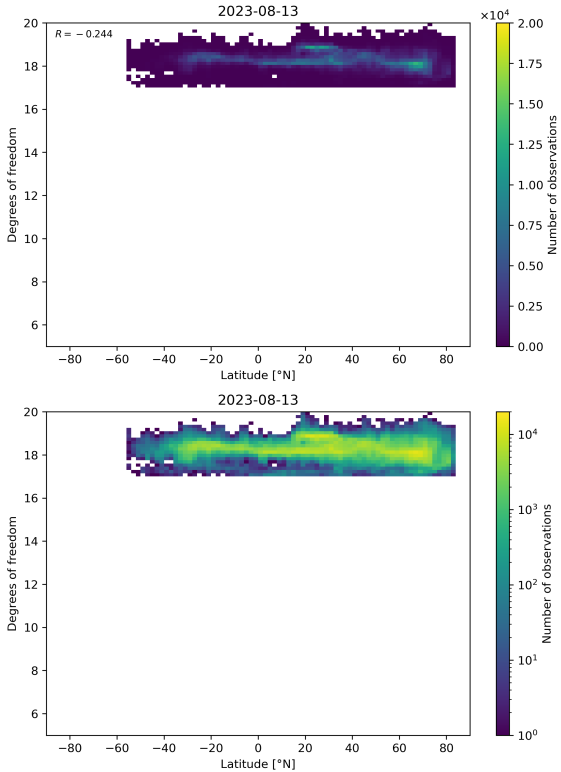
Figure 55: Scatter density plot of “Latitude” against “Degrees of freedom” for 2023-08-12 to 2023-08-14.
