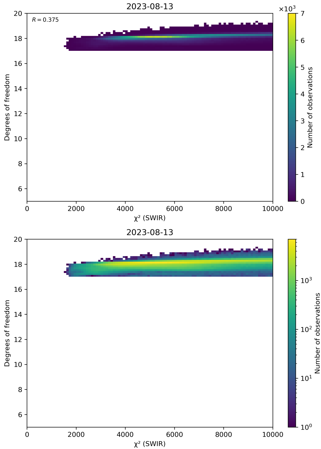
Figure 48: Scatter density plot of “ \chi^2 (SWIR)” against “Degrees of freedom” for 2023-08-12 to 2023-08-14.
