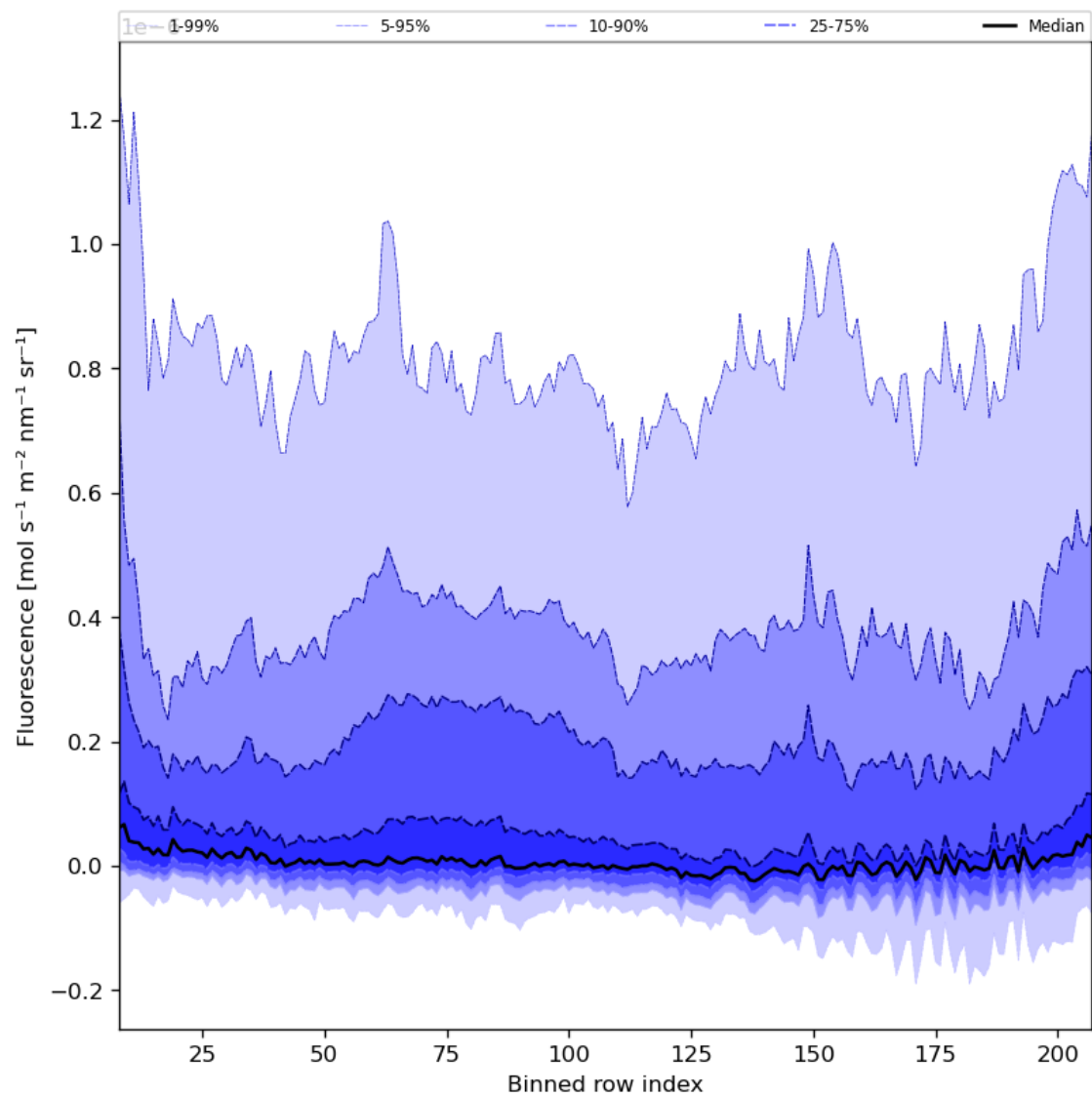
Figure 43: Along track statistics of “Fluorescence” for 2023-08-12 to 2023-08-14
