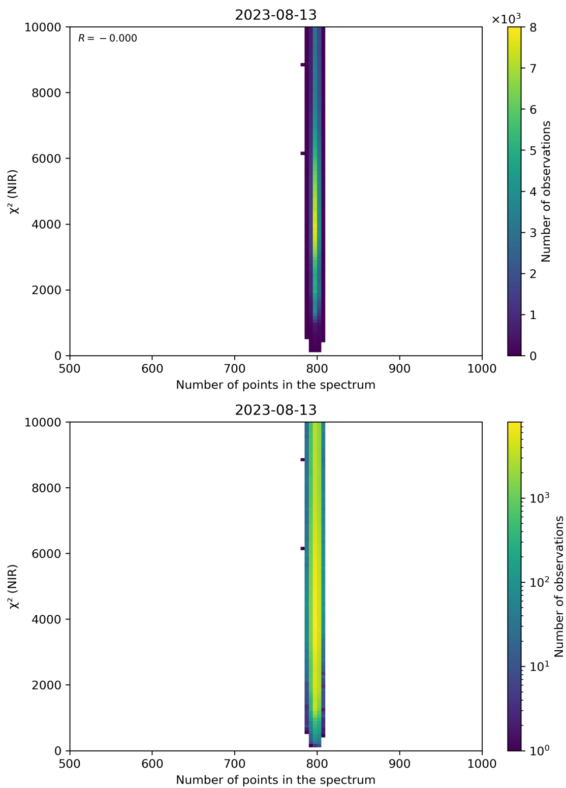
Figure 88: Scatter density plot of “Number of points in the spectrum” against “ \chi^2 (NIR)” for 2023-08-12 to 2023-08-14.
