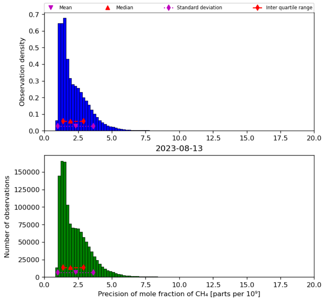
Figure 24: Histogram of “Precision of mole fraction of CH 4 ” for 2023-08-12 to 2023-08-14
