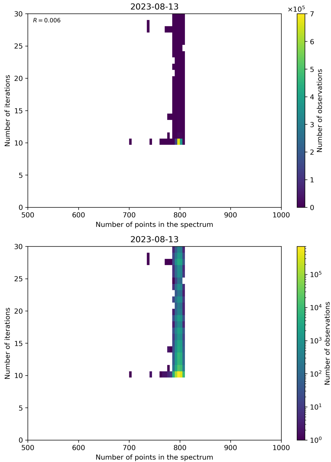
Figure 92: Scatter density plot of “Number of points in the spectrum” against “Number of iterations” for 2023-08-12 to 2023-08-14.
