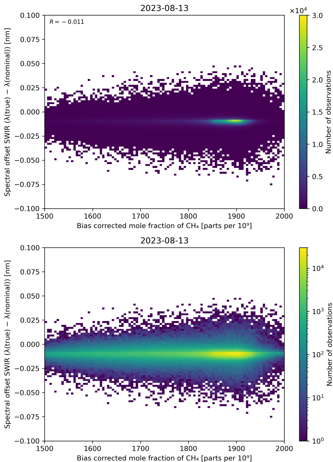
Figure 69: Scatter density plot of “Bias corrected mole fraction of \text{CH}_4 ” against “Spectral offset SWIR ( \lambda(\text{true}) - \lambda(\text{nominal}) )” for 2023-08-12 to 2023-08-14.
