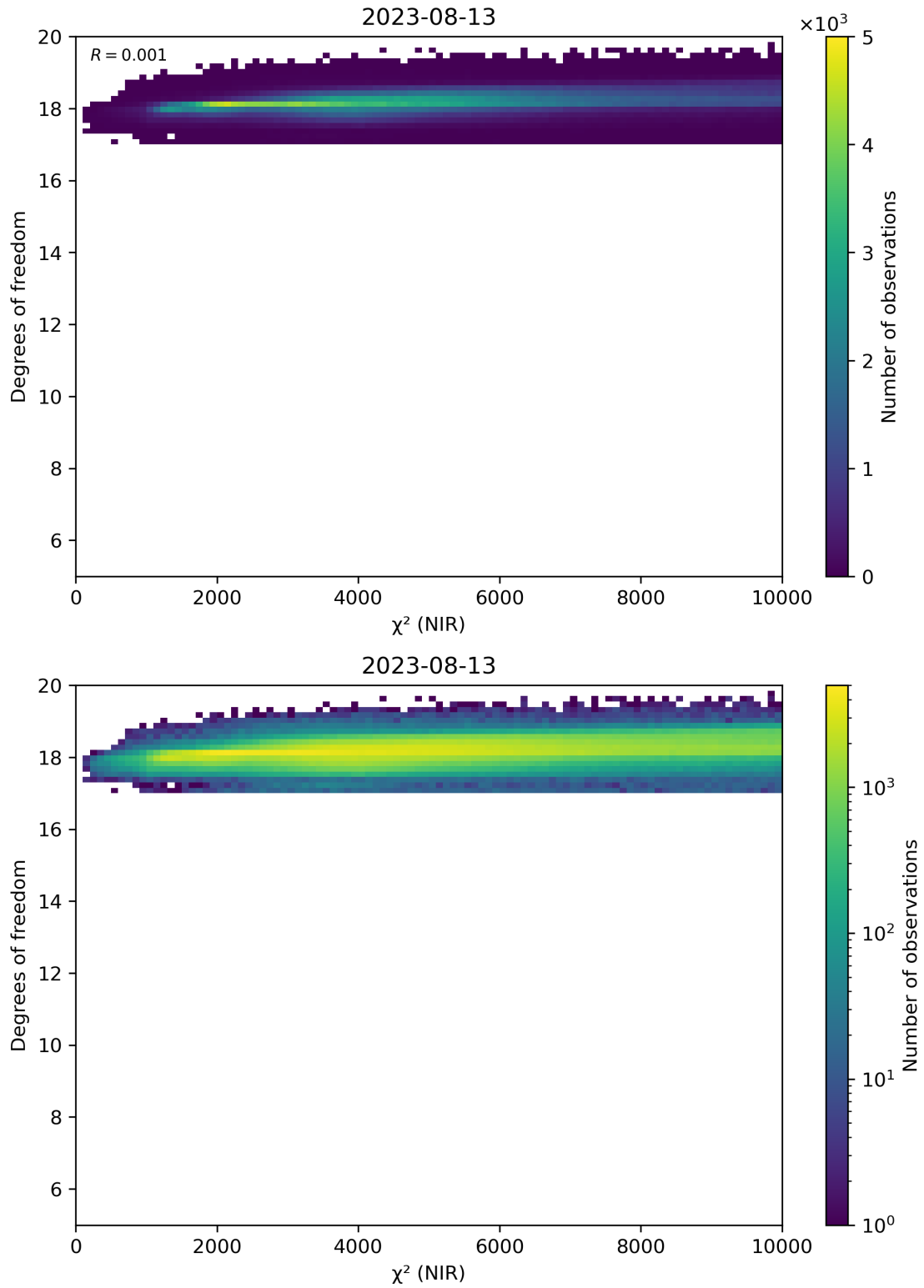
Figure 44: Scatter density plot of “ \chi^2 (NIR)” against “Degrees of freedom” for 2023-08-12 to 2023-08-14.
