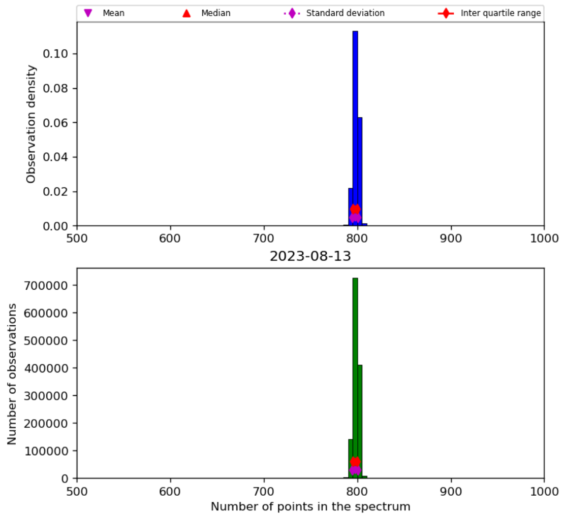
Figure 26: Histogram of “Number of points in the spectrum” for 2023-08-12 to 2023-08-14
