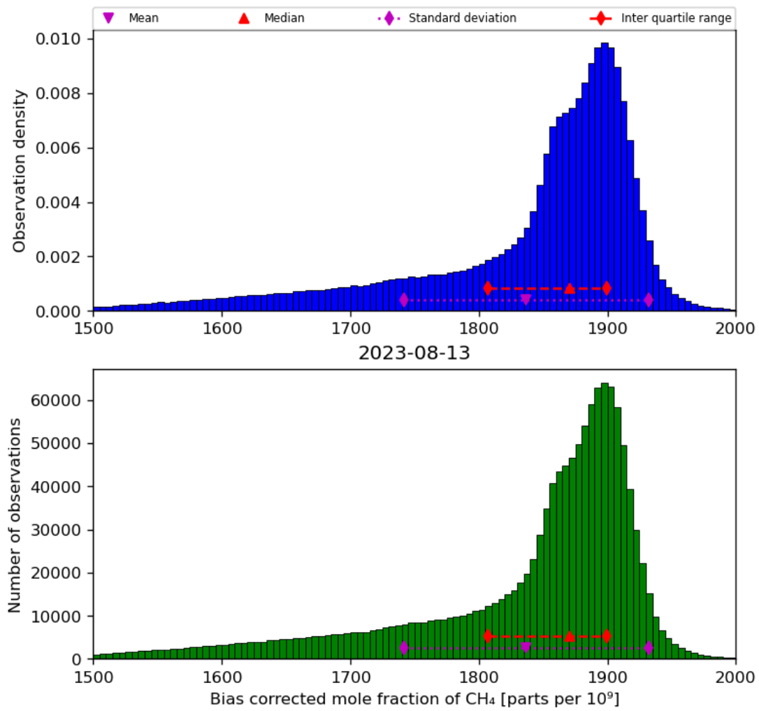
Figure 25: Histogram of “Bias corrected mole fraction of CH 4 ” for 2023-08-12 to 2023-08-14
