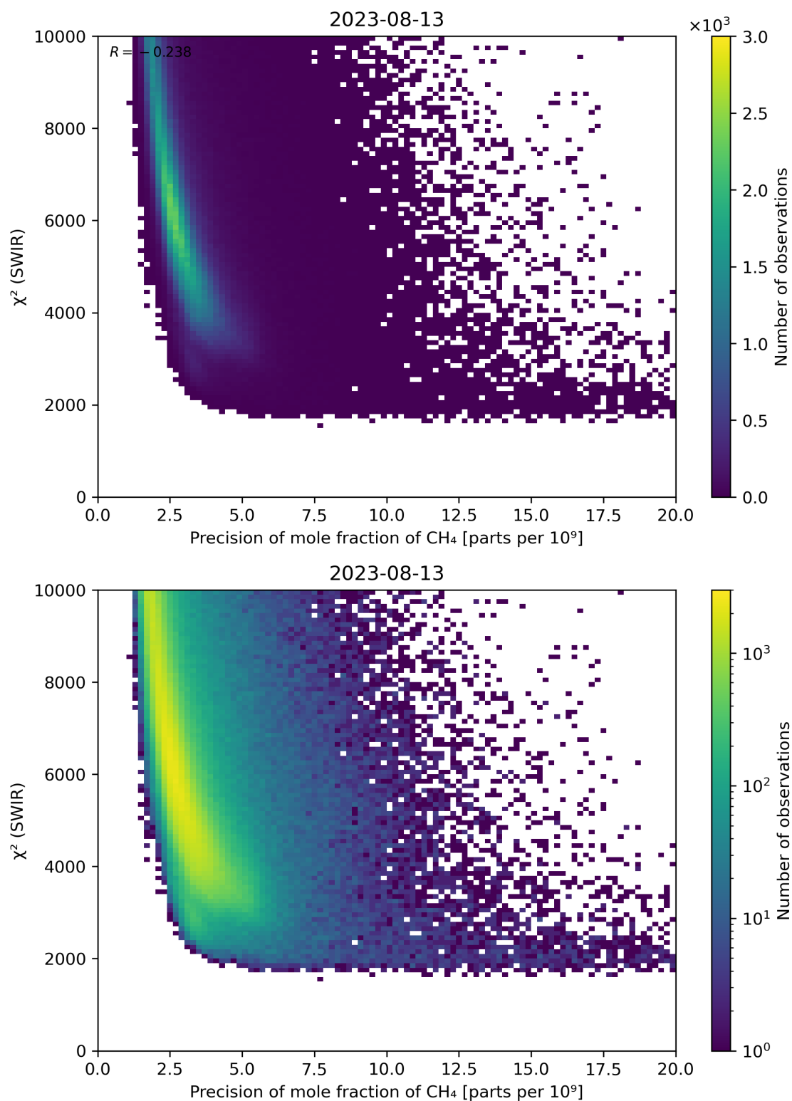
Figure 79: Scatter density plot of “Precision of mole fraction of CH 4 ” against “ \chi^2 (SWIR)” for 2023-08-12 to 2023-08-14.
