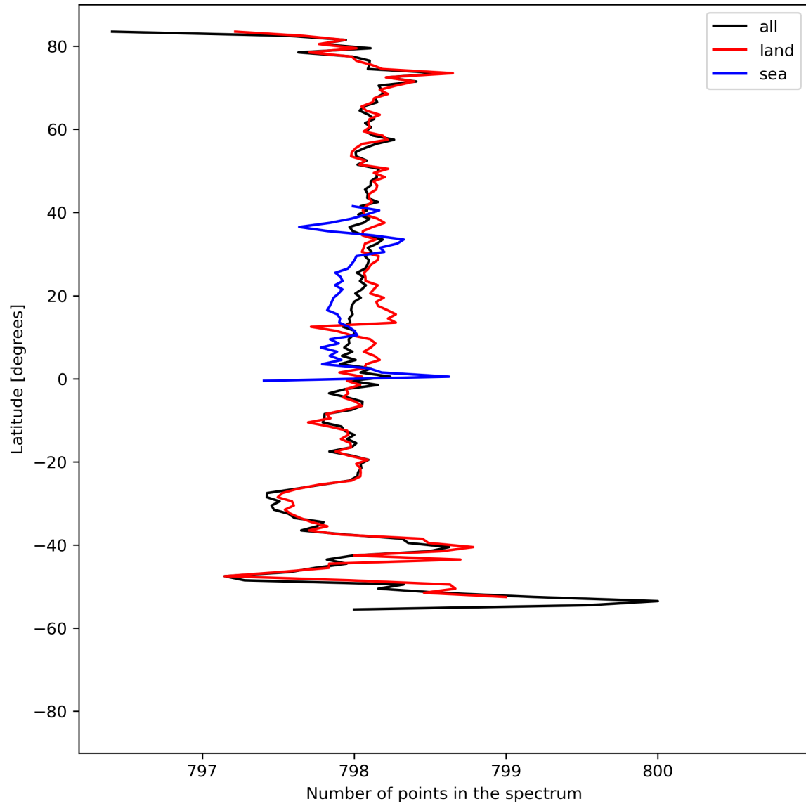
Figure 15: Zonal average of “Number of points in the spectrum” for 2023-08-12 to 2023-08-14.
