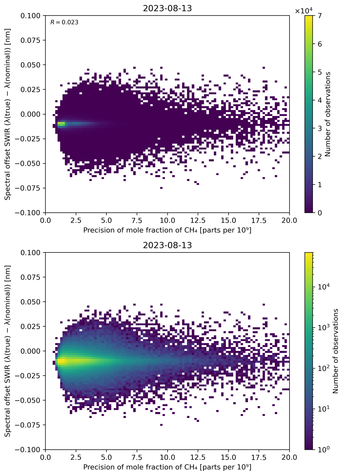
Figure 85: Scatter density plot of “Precision of mole fraction of CH 4 ” against “Spectral offset SWIR ( \lambda(\text{true}) - \lambda(\text{nominal}) )” for 2023-08-12 to 2023-08-14.
