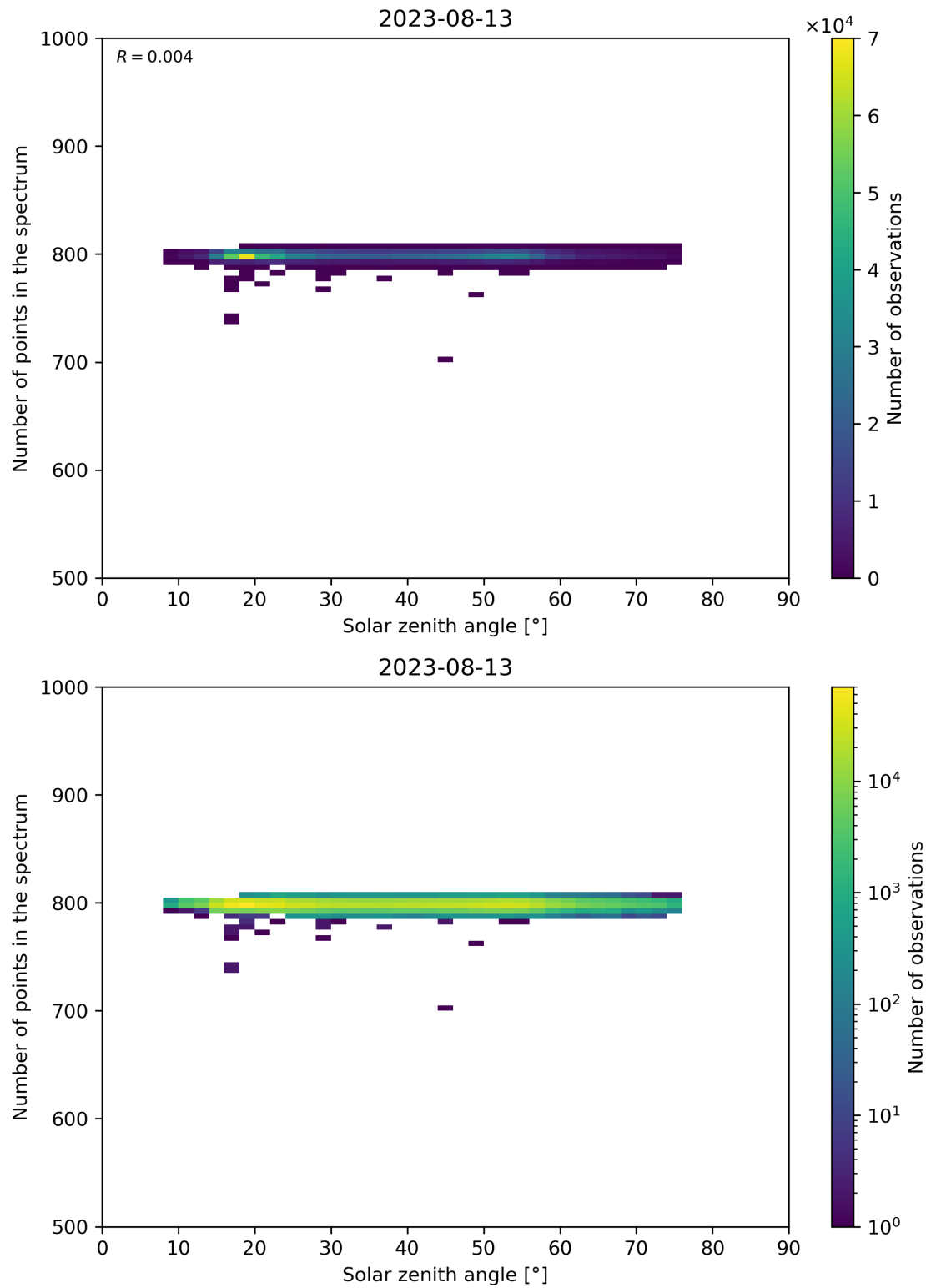
Figure 103: Scatter density plot of “Solar zenith angle” against “Number of points in the spectrum” for 2023-08-12 to 2023-08-14.
