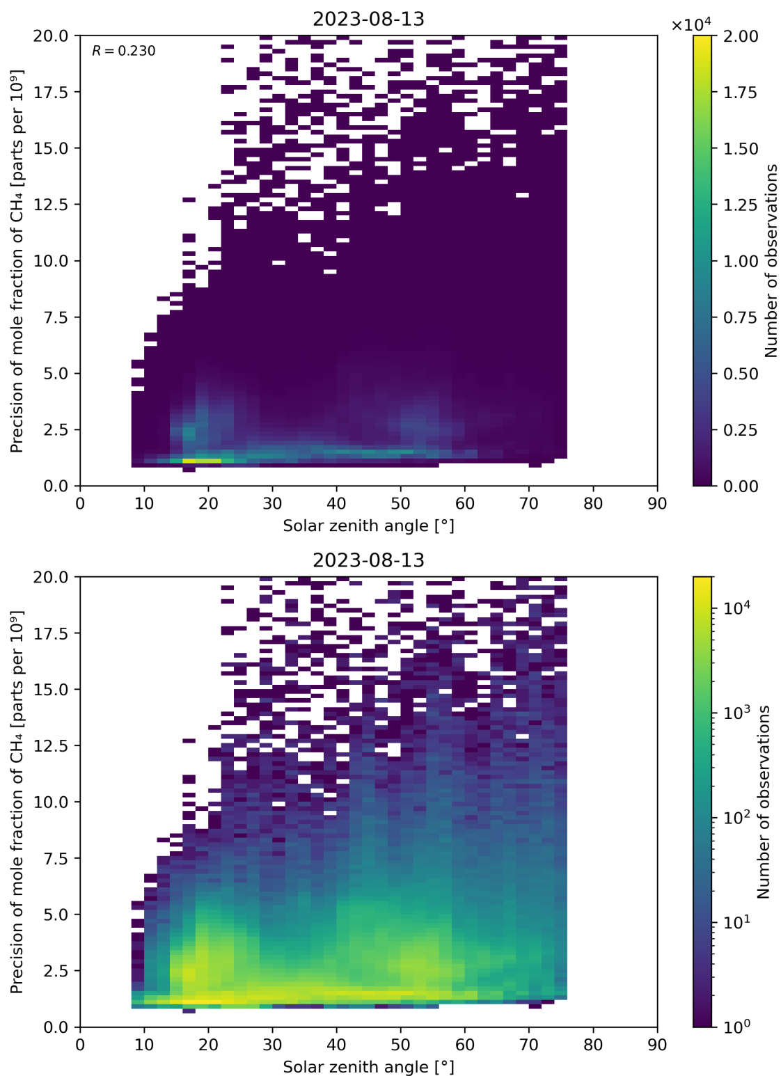
Figure 101: Scatter density plot of “Solar zenith angle” against “Precision of mole fraction of \text{CH}_4 ” for 2023-08-12 to 2023-08-14.
