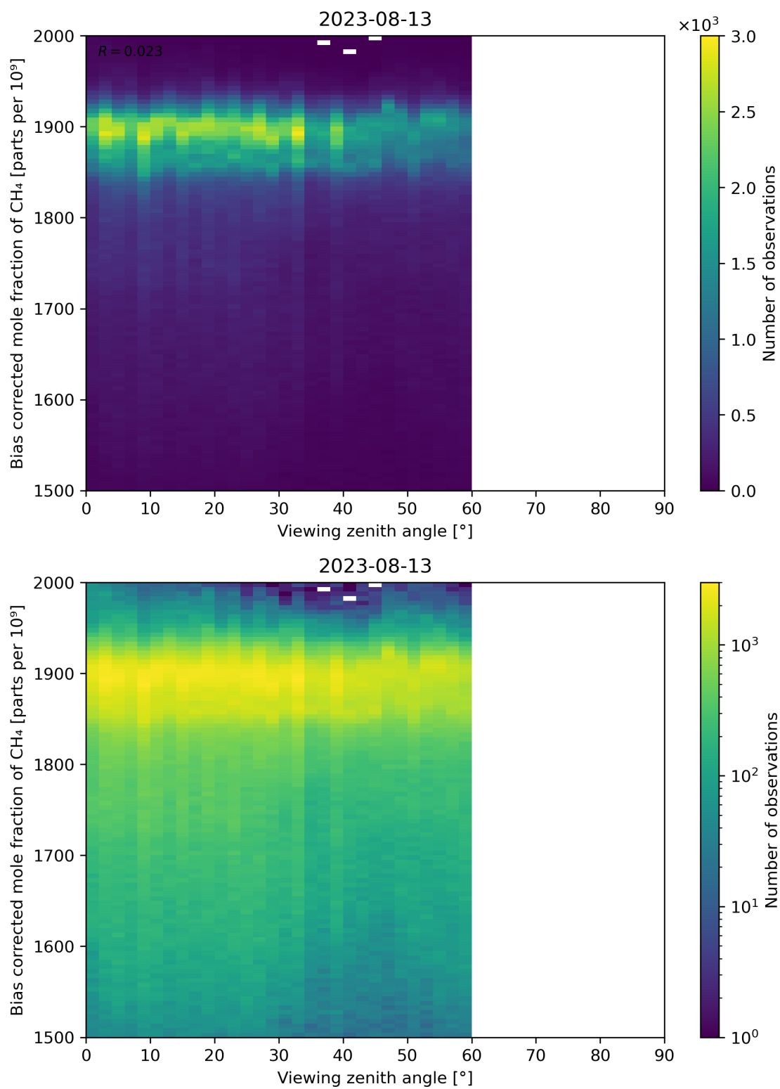
Figure 111: Scatter density plot of “Viewing zenith angle” against “Bias corrected mole fraction of CH 4 ” for 2023-08-12 to 2023-08-14.
