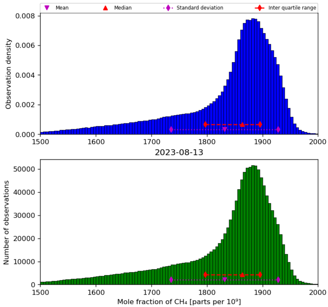
Figure 23: Histogram of “Mole fraction of CH 4 ” for 2023-08-12 to 2023-08-14
