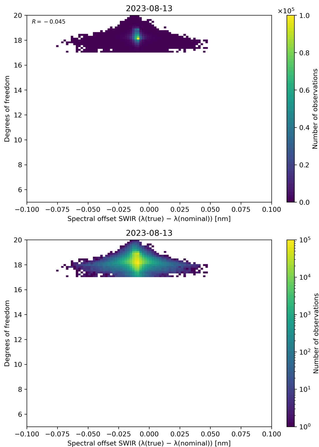
Figure 119: Scatter density plot of “Spectral offset SWIR ( \lambda(\text{true}) - \lambda(\text{nominal}) )” against “Degrees of freedom” for 2023-08-12 to 2023-08-14.
