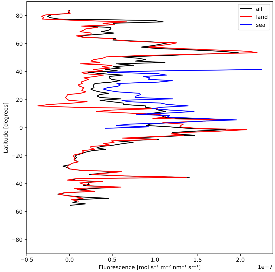
Figure 21: Zonal average of “Fluorescence” for 2023-08-12 to 2023-08-14.
