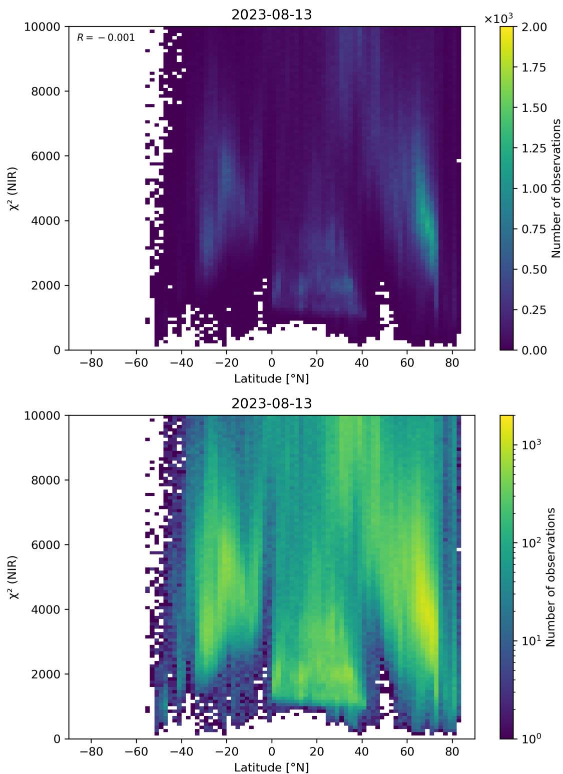
Figure 53: Scatter density plot of “Latitude” against “ \chi^2 (NIR)” for 2023-08-12 to 2023-08-14.
