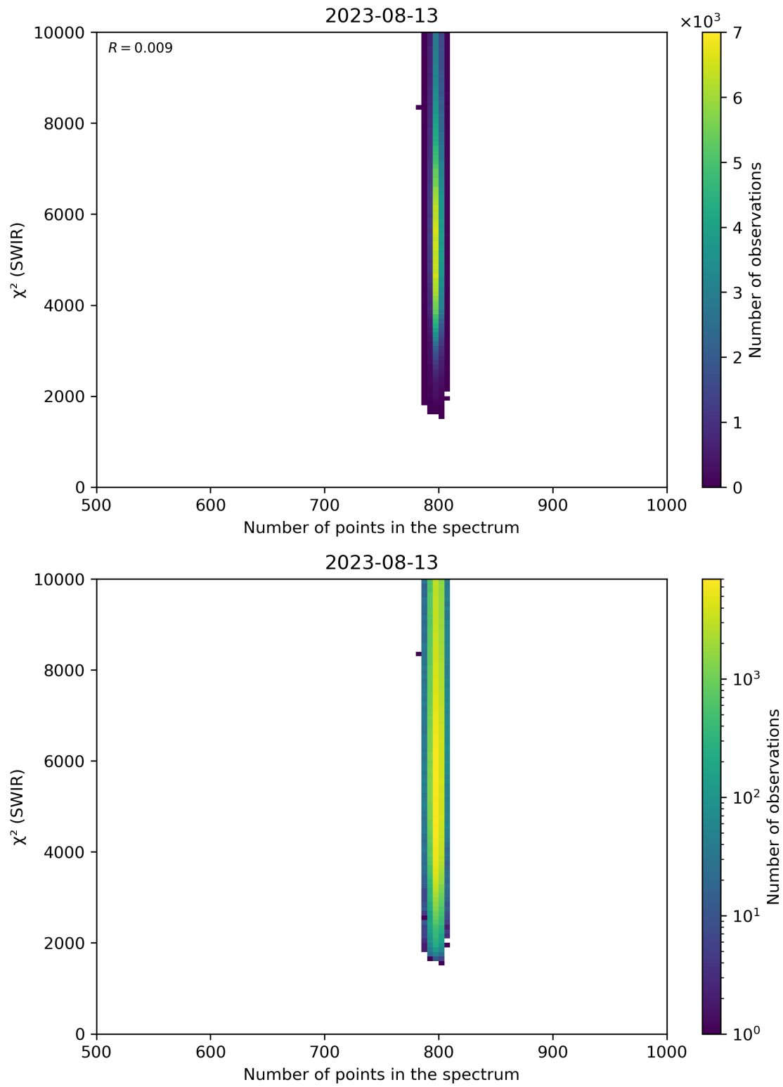
Figure 89: Scatter density plot of “Number of points in the spectrum” against “ \chi^2 (SWIR)” for 2023-08-12 to 2023-08-14.
