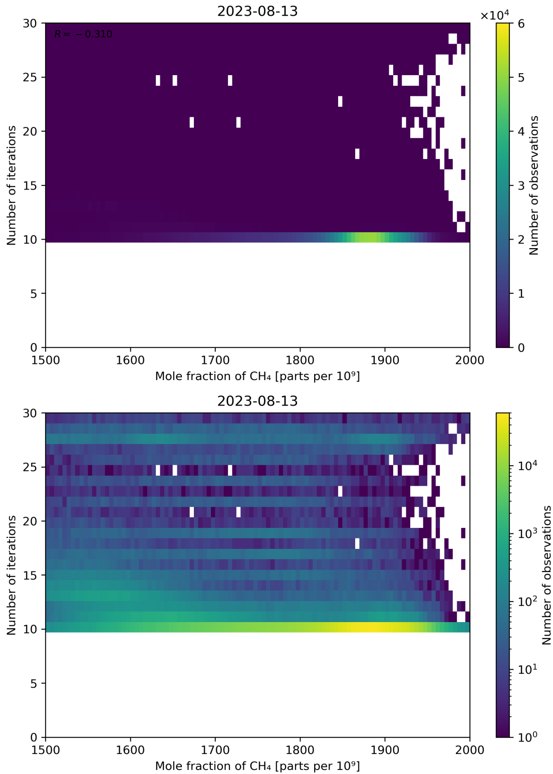
Figure 76: Scatter density plot of “Mole fraction of CH 4 ” against “Number of iterations” for 2023-08-12 to 2023-08-14.
