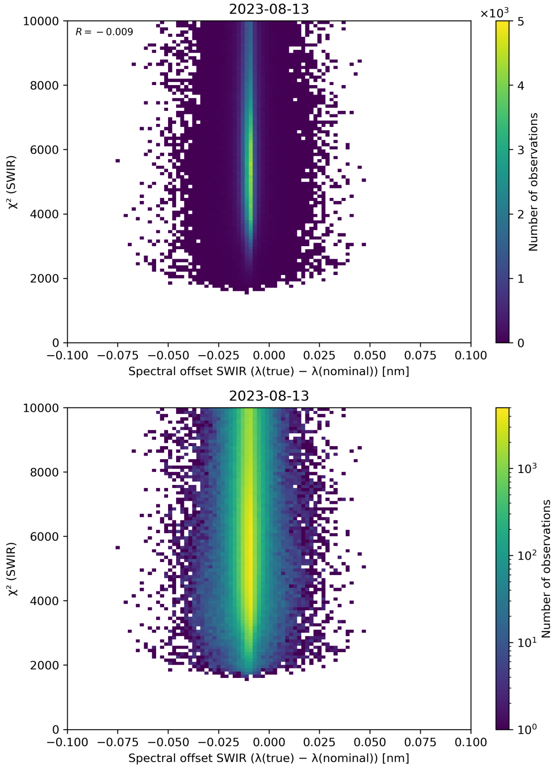
Figure 118: Scatter density plot of “Spectral offset SWIR ( \lambda(\text{true}) - \lambda(\text{nominal}) )” against “ \chi^2 (SWIR)” for 2023-08-12 to 2023-08-14.
