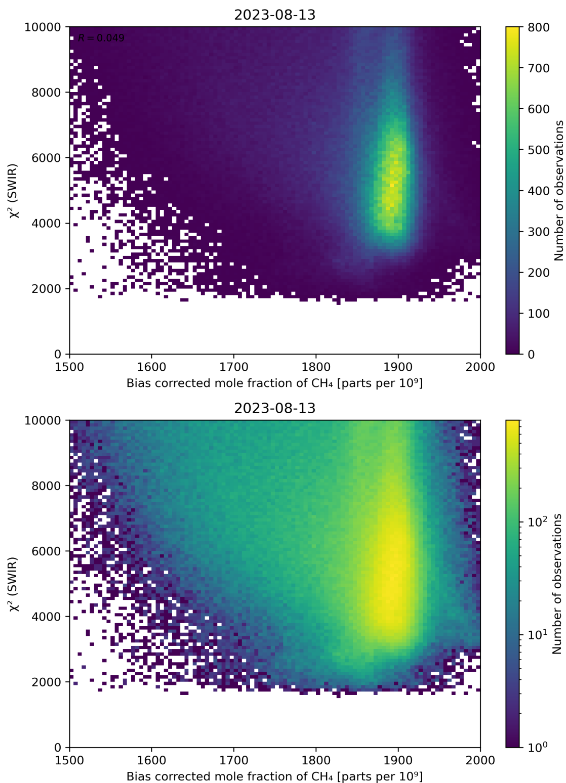
Figure 64: Scatter density plot of “Bias corrected mole fraction of \text{CH}_4 ” against “ \chi^2 (SWIR)” for 2023-08-12 to 2023-08-14.
