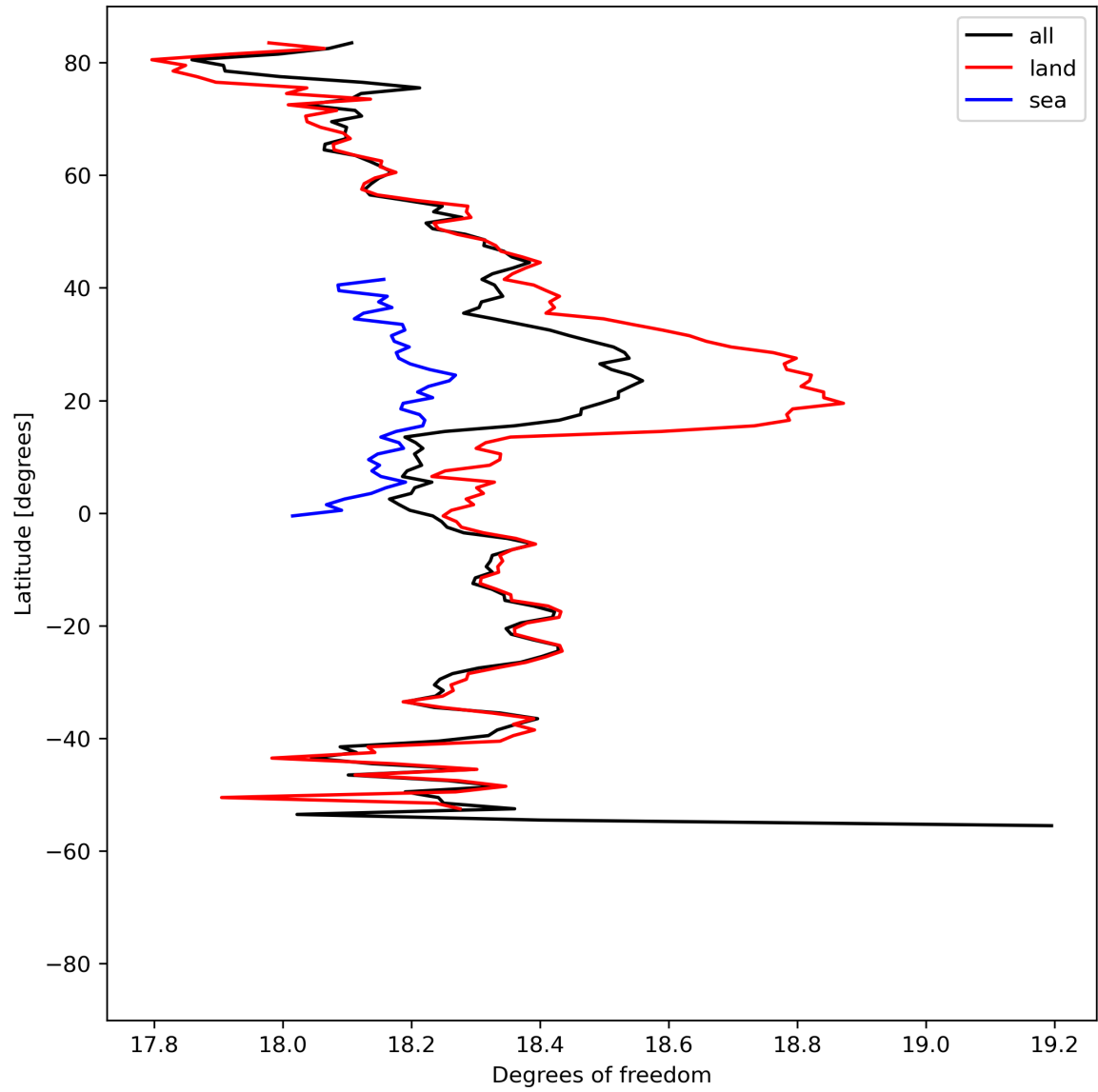
Figure 19: Zonal average of “Degrees of freedom” for 2023-08-12 to 2023-08-14.
