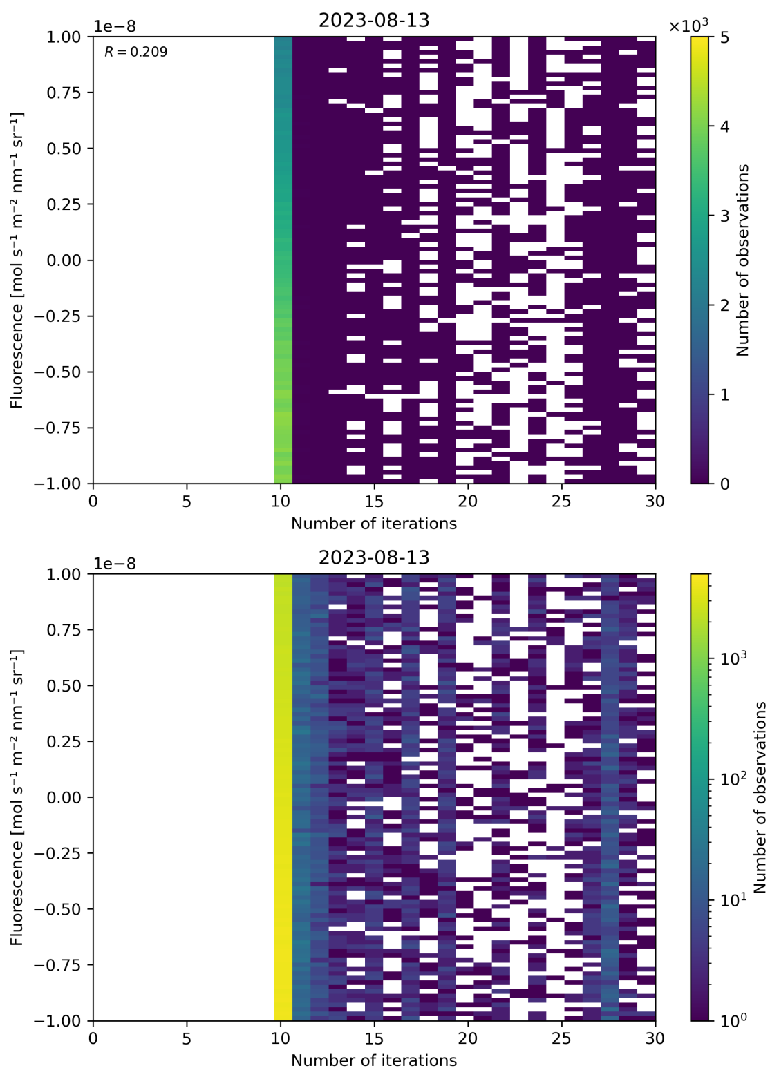
Figure 87: Scatter density plot of “Number of iterations” against “Fluorescence” for 2023-08-12 to 2023-08-14.
