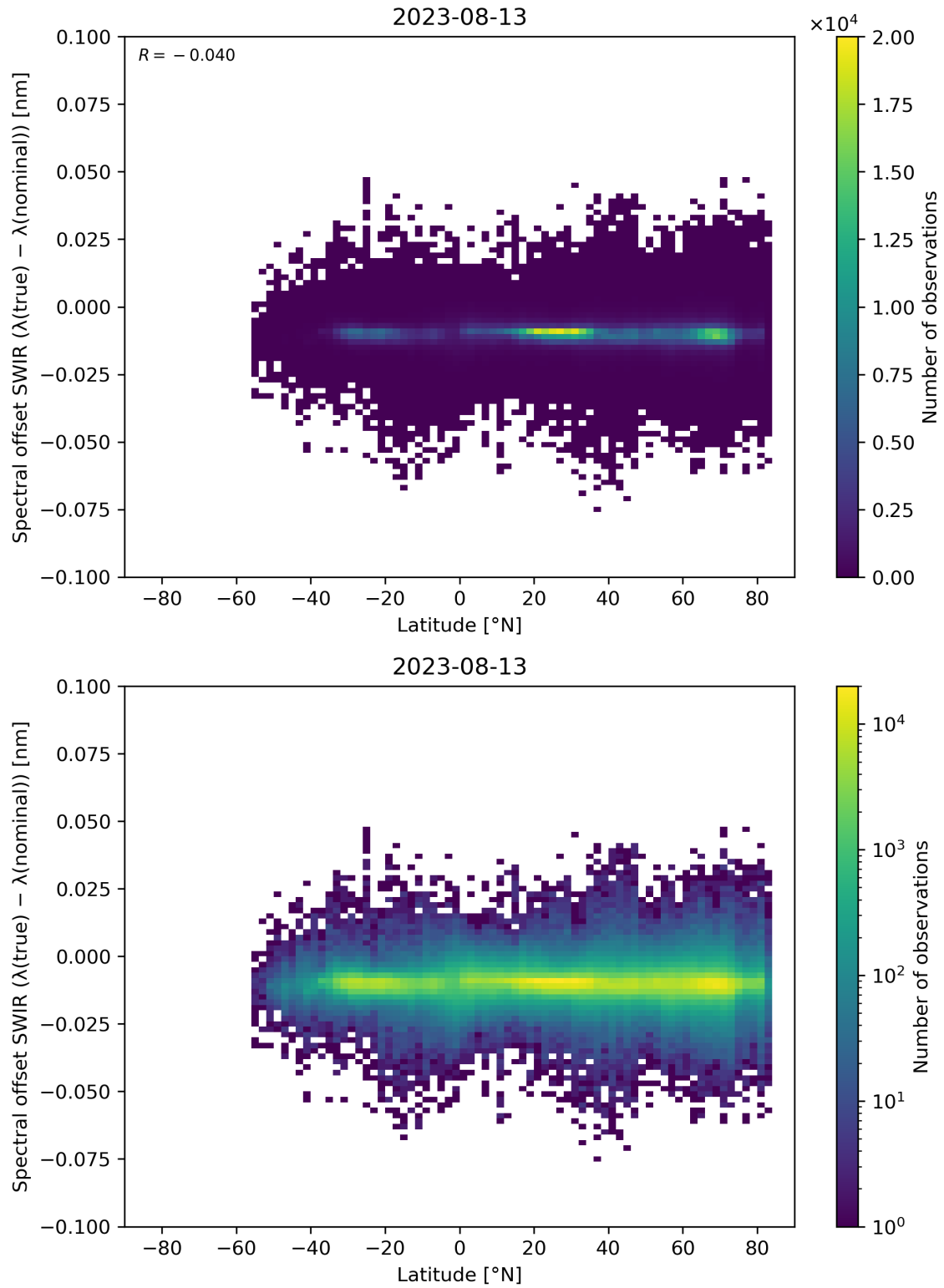
Figure 62: Scatter density plot of “Latitude” against “Spectral offset SWIR ( \lambda(\text{true}) - \lambda(\text{nominal}) )” for 2023-08-12 to 2023-08-14.
