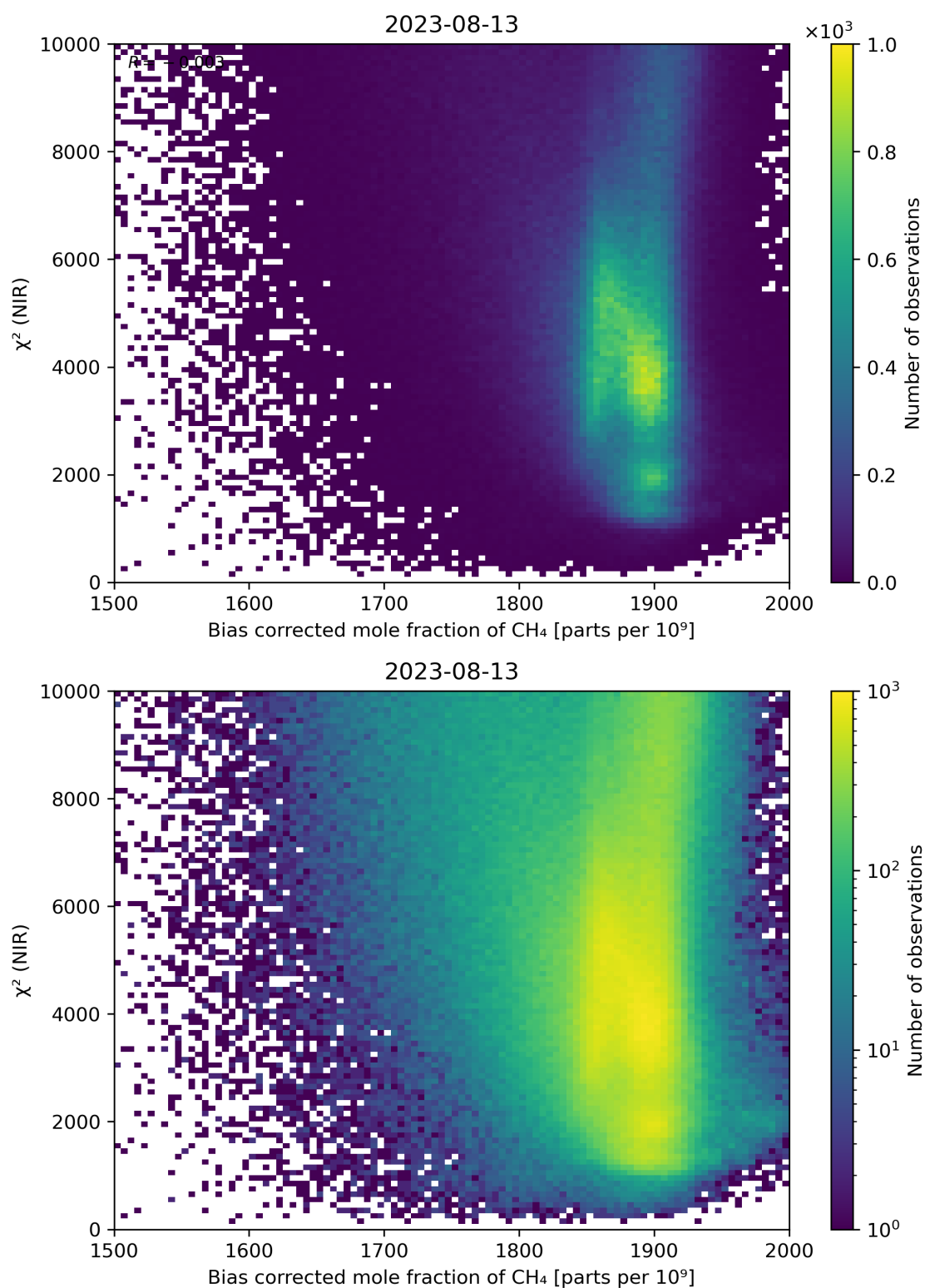
Figure 63: Scatter density plot of “Bias corrected mole fraction of CH 4 ” against “ \chi^2 (NIR)” for 2023-08-12 to 2023-08-14.
