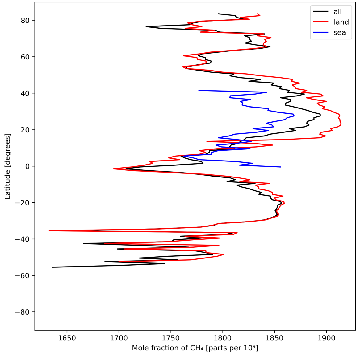
Figure 12: Zonal average of “Mole fraction of \text{CH}_4 ” for 2023-08-12 to 2023-08-14.
