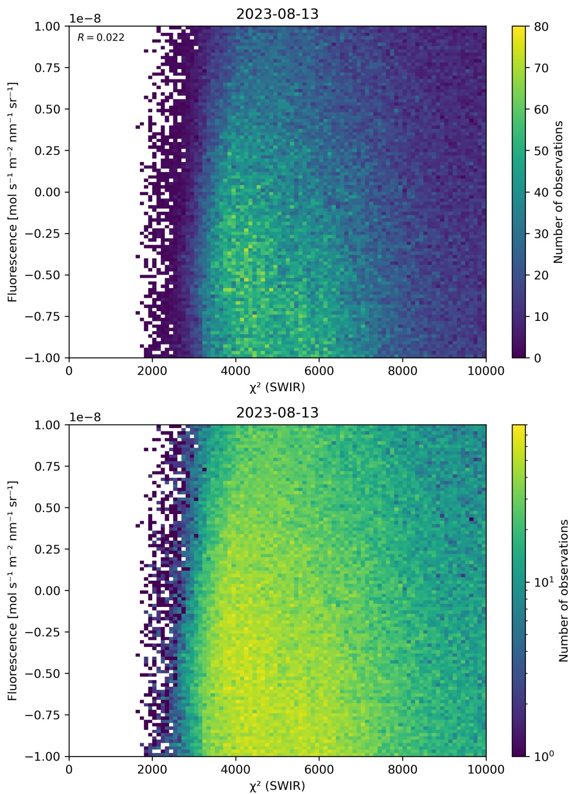
Figure 49: Scatter density plot of “ \chi^2 (SWIR)” against “Fluorescence” for 2023-08-12 to 2023-08-14.
