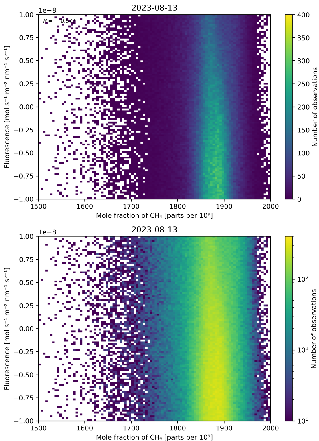
Figure 73: Scatter density plot of “Mole fraction of \text{CH}_4 ” against “Fluorescence” for 2023-08-12 to 2023-08-14.
