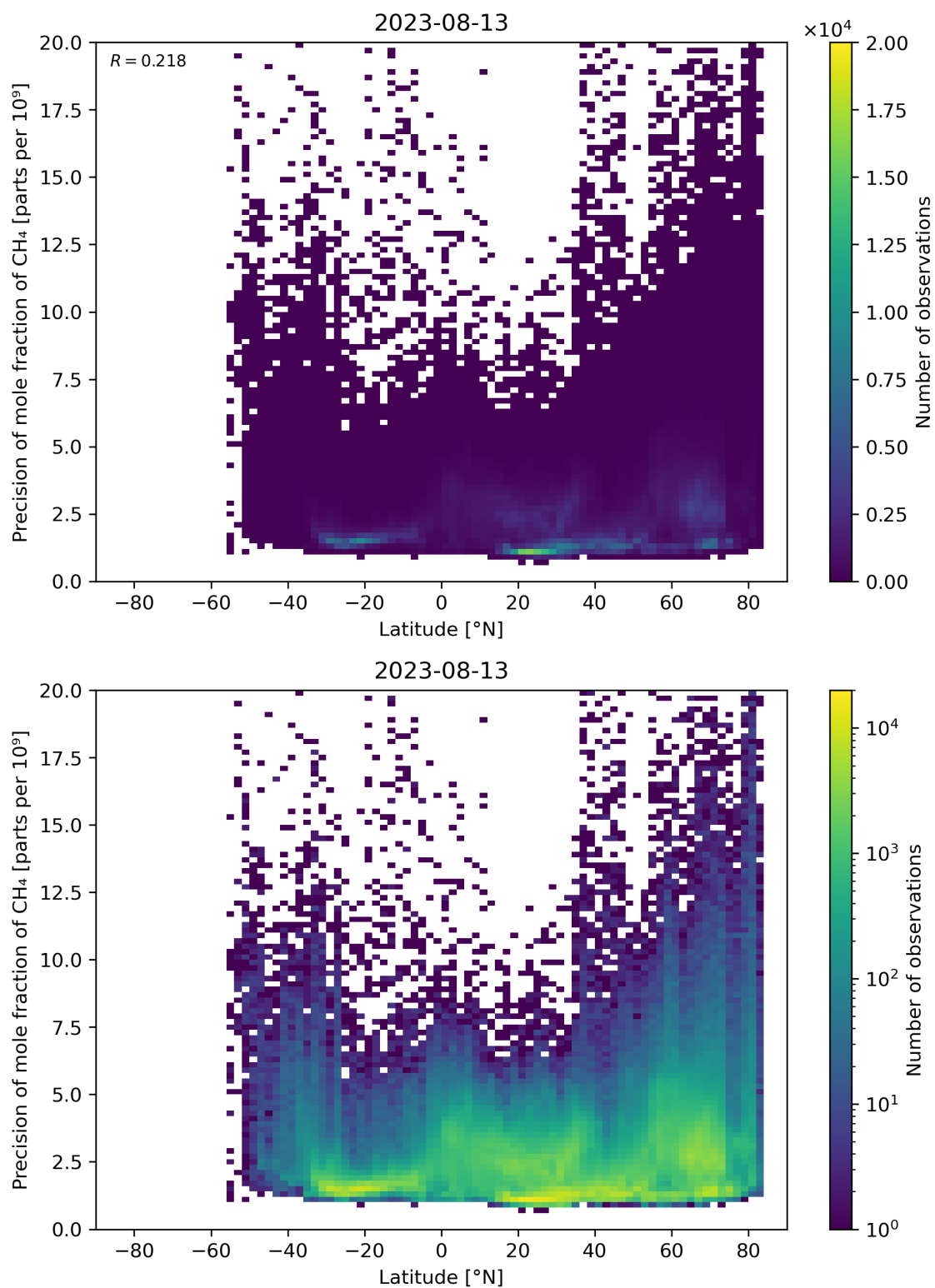
Figure 59: Scatter density plot of “Latitude” against “Precision of mole fraction of \text{CH}_4 ” for 2023-08-12 to 2023-08-14.
