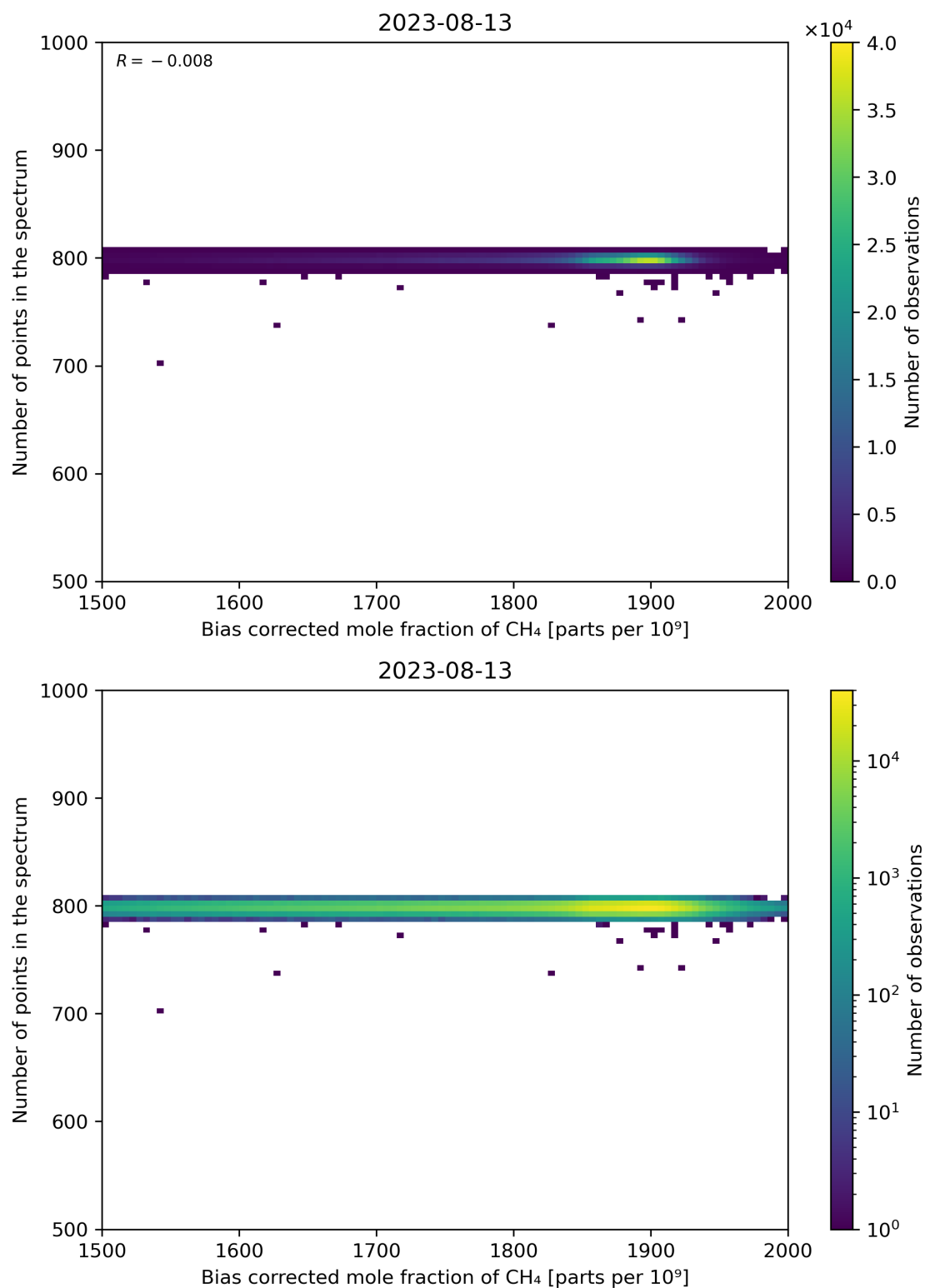
Figure 68: Scatter density plot of “Bias corrected mole fraction of CH 4 ” against “Number of points in the spectrum” for 2023-08-12 to 2023-08-14.
