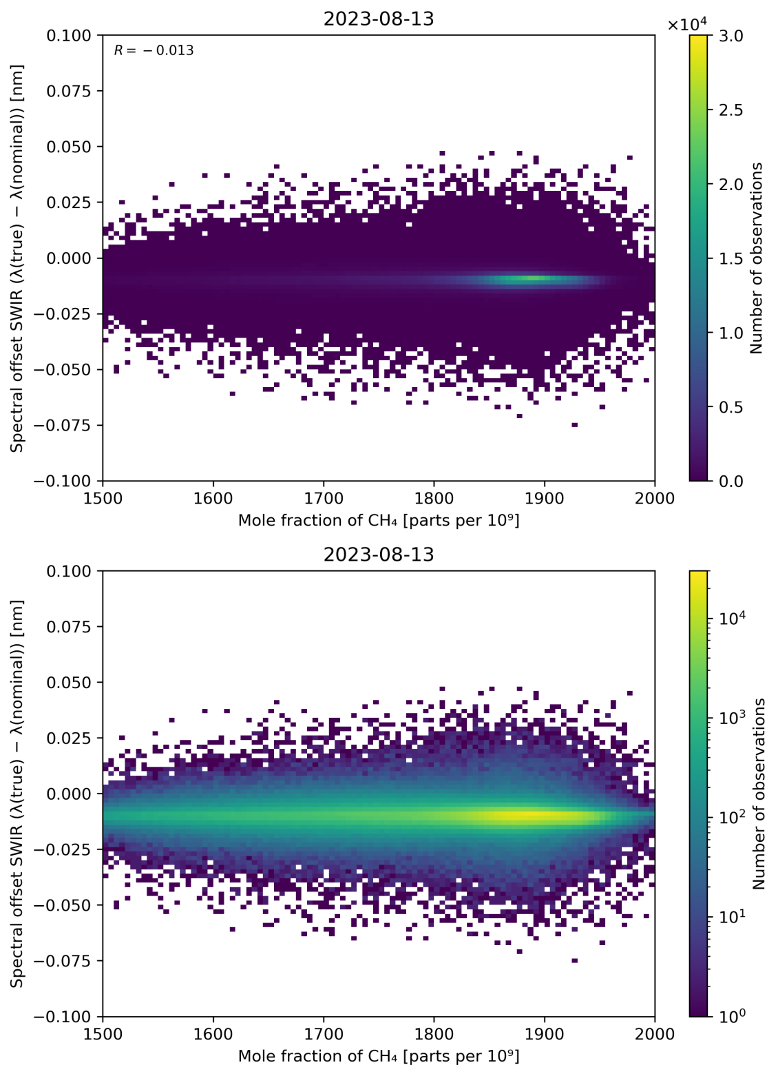
Figure 86: Scatter density plot of “Mole fraction of CH 4 ” against “Spectral offset SWIR ( \lambda(\text{true}) - \lambda(\text{nominal}) )” for 2023-08-12 to 2023-08-14.
