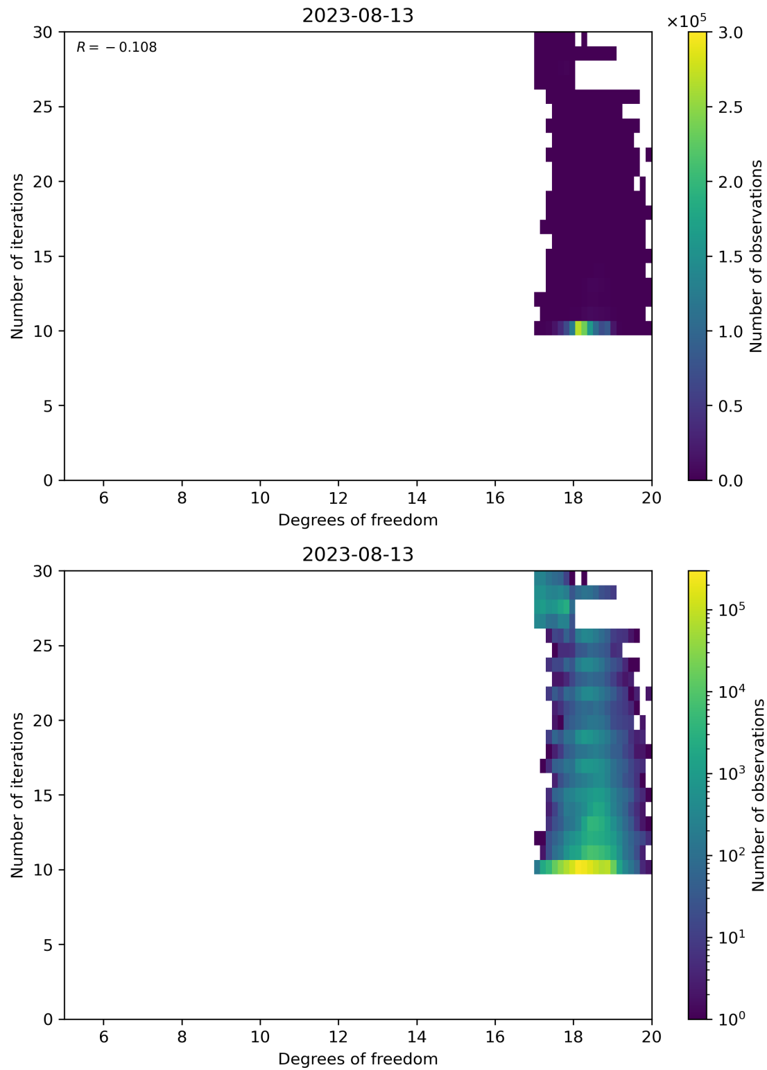
Figure 52: Scatter density plot of “Degrees of freedom” against “Number of iterations” for 2023-08-12 to 2023-08-14.
