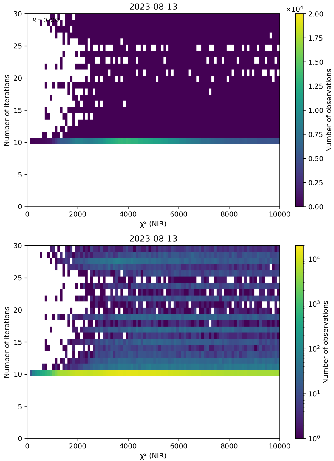
Figure 46: Scatter density plot of “ \chi^2 (NIR)” against “Number of iterations” for 2023-08-12 to 2023-08-14.
