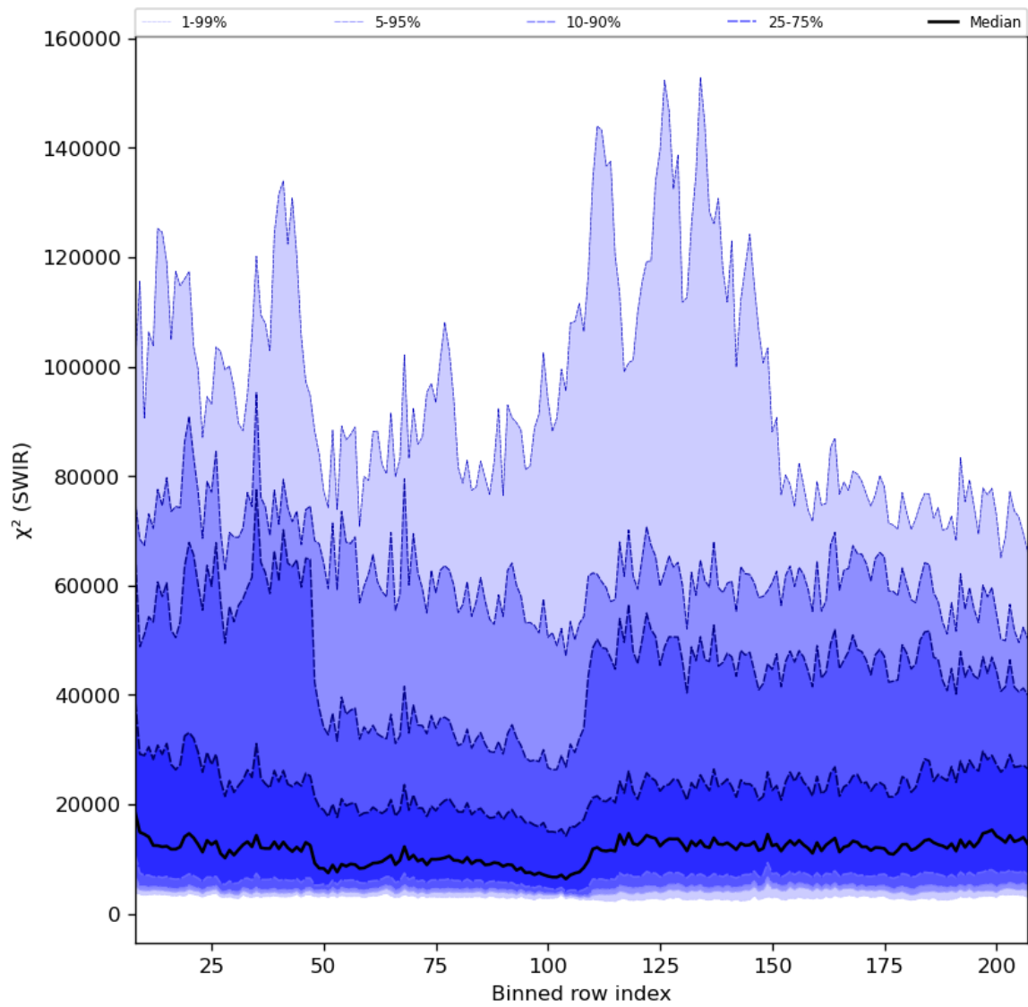
Figure 39: Along track statistics of “ \chi^2 (SWIR)” for 2023-08-12 to 2023-08-14
