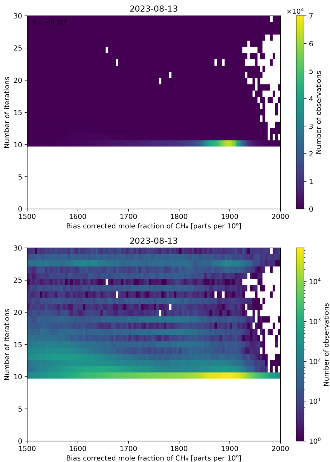
Figure 67: Scatter density plot of “Bias corrected mole fraction of CH 4 ” against “Number of iterations” for 2023-08-12 to 2023-08-14.
