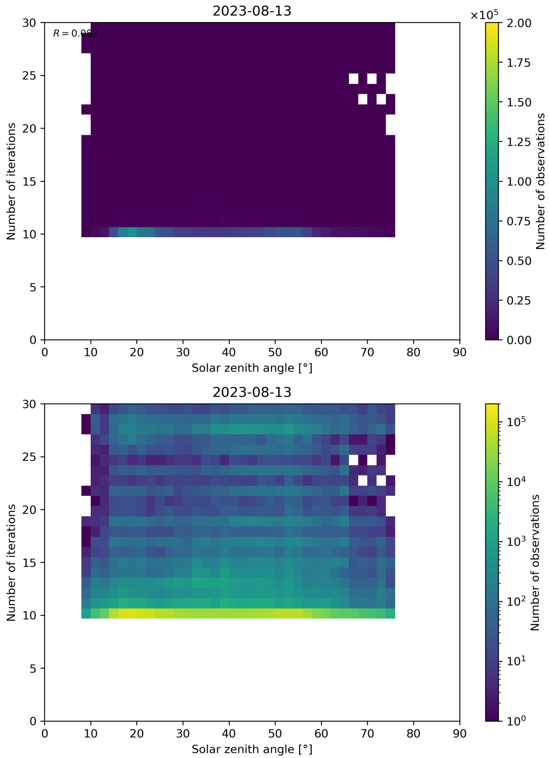
Figure 102: Scatter density plot of “Solar zenith angle” against “Number of iterations” for 2023-08-12 to 2023-08-14.
