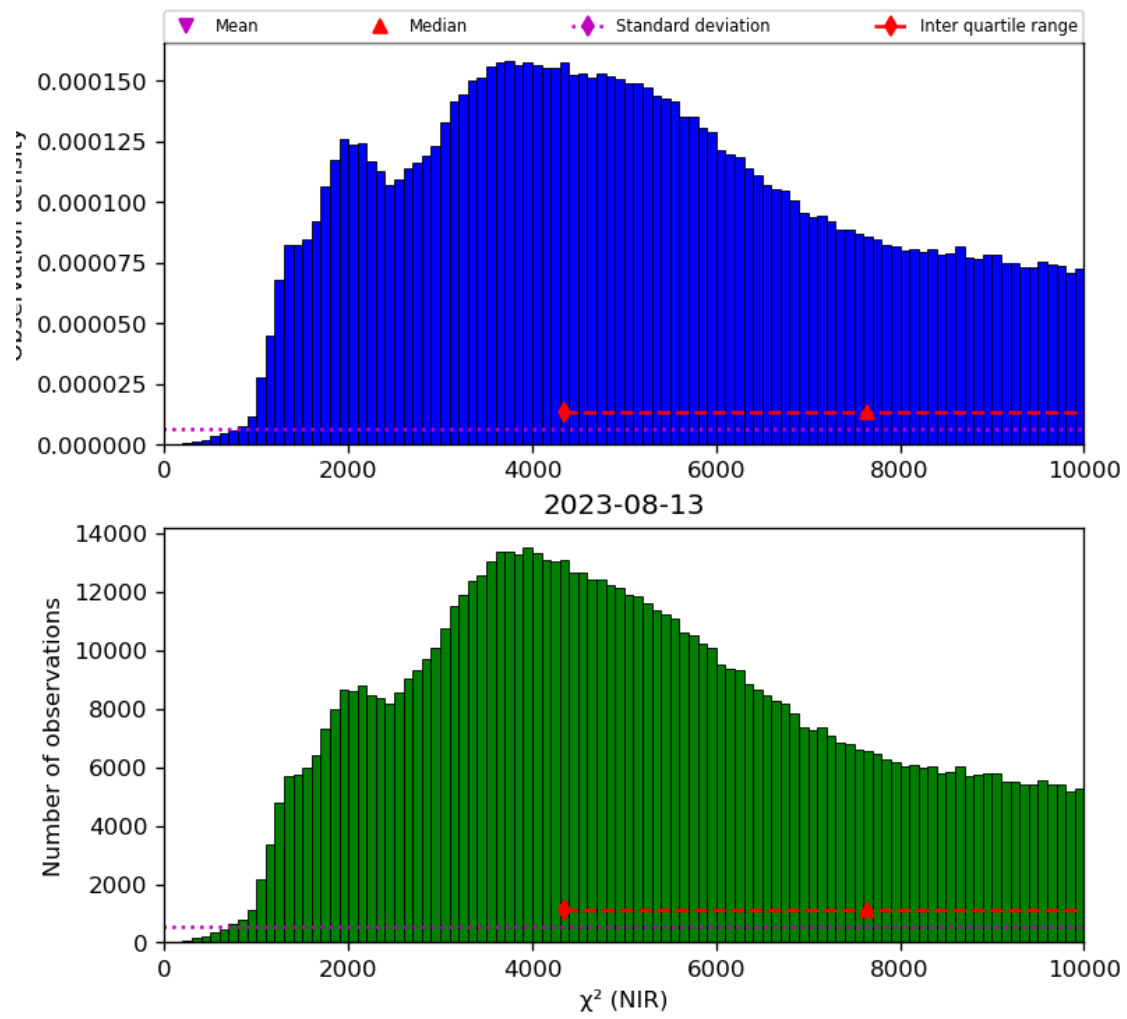
Figure 29: Histogram of “ \chi^2 (NIR)” for 2023-08-12 to 2023-08-14
