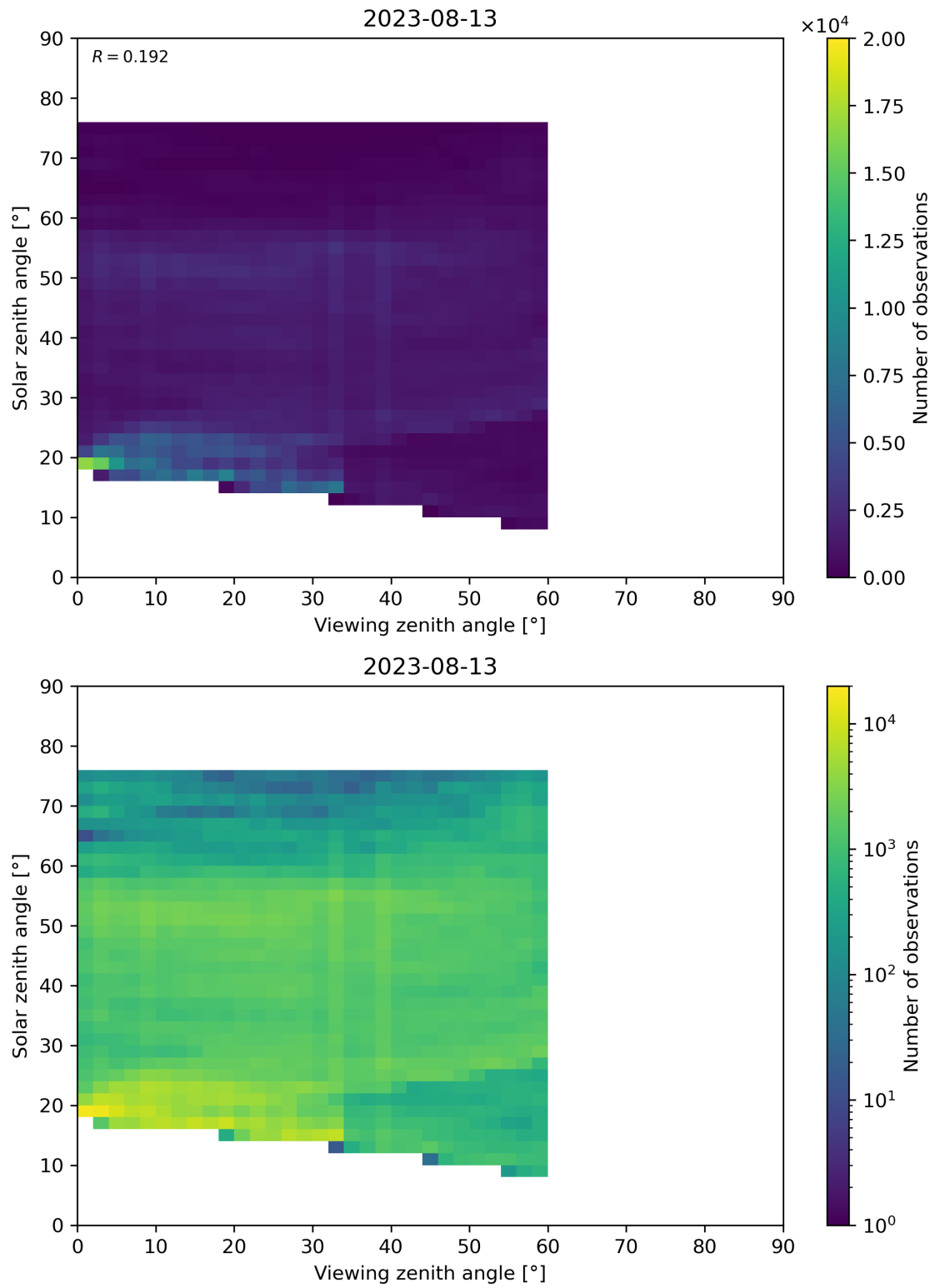
Figure 115: Scatter density plot of “Viewing zenith angle” against “Solar zenith angle” for 2023-08-12 to 2023-08-14.
