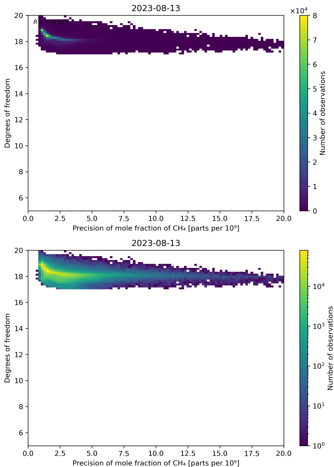
Figure 80: Scatter density plot of “Precision of mole fraction of CH 4 ” against “Degrees of freedom” for 2023-08-12 to 2023-08-14.
