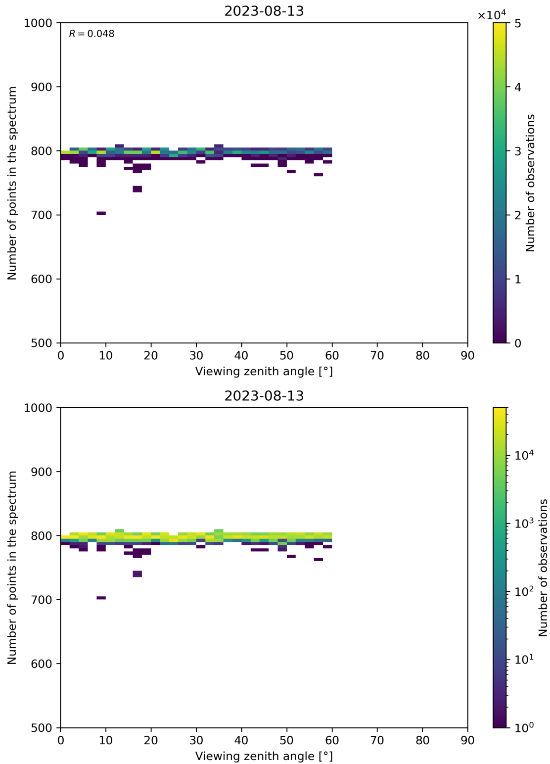
Figure 114: Scatter density plot of “Viewing zenith angle” against “Number of points in the spectrum” for 2023-08-12 to 2023-08-14.
