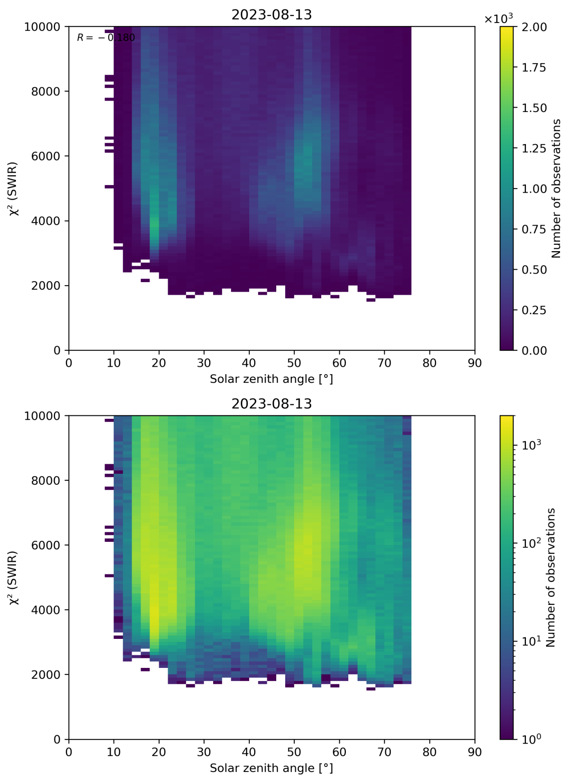
Figure 95: Scatter density plot of “Solar zenith angle” against “ \chi^2 (SWIR)” for 2023-08-12 to 2023-08-14.
