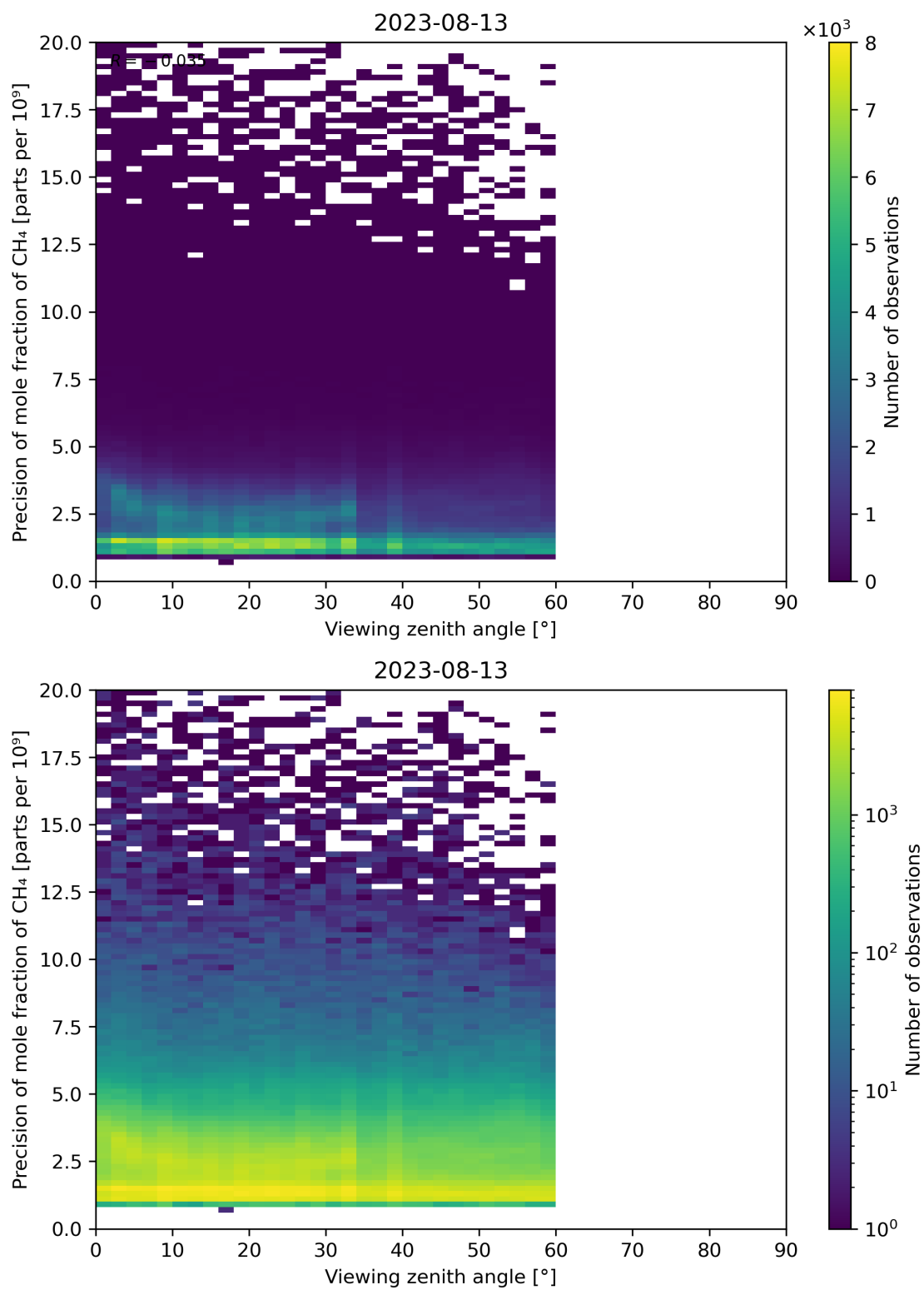
Figure 112: Scatter density plot of “Viewing zenith angle” against “Precision of mole fraction of CH 4 ” for 2023-08-12 to 2023-08-14.
