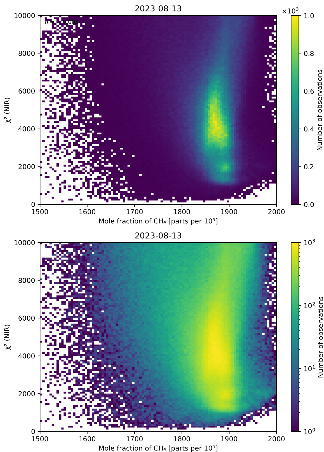
Figure 70: Scatter density plot of “Mole fraction of CH 4 ” against “ \chi^2 (NIR)” for 2023-08-12 to 2023-08-14.
