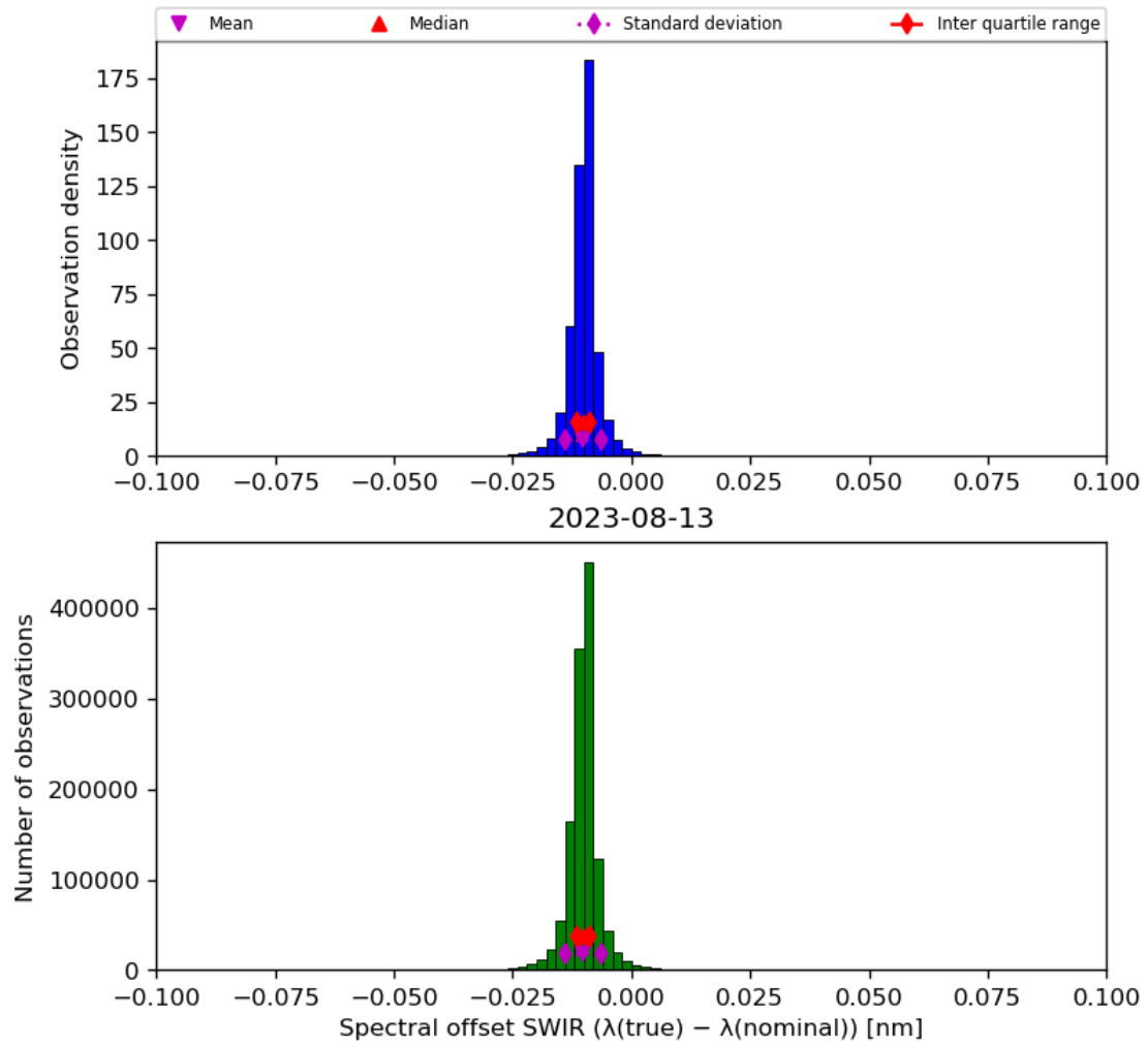
Figure 27: Histogram of “Spectral offset SWIR ( \lambda(\text{true}) - \lambda(\text{nominal}) )” for 2023-08-12 to 2023-08-14
