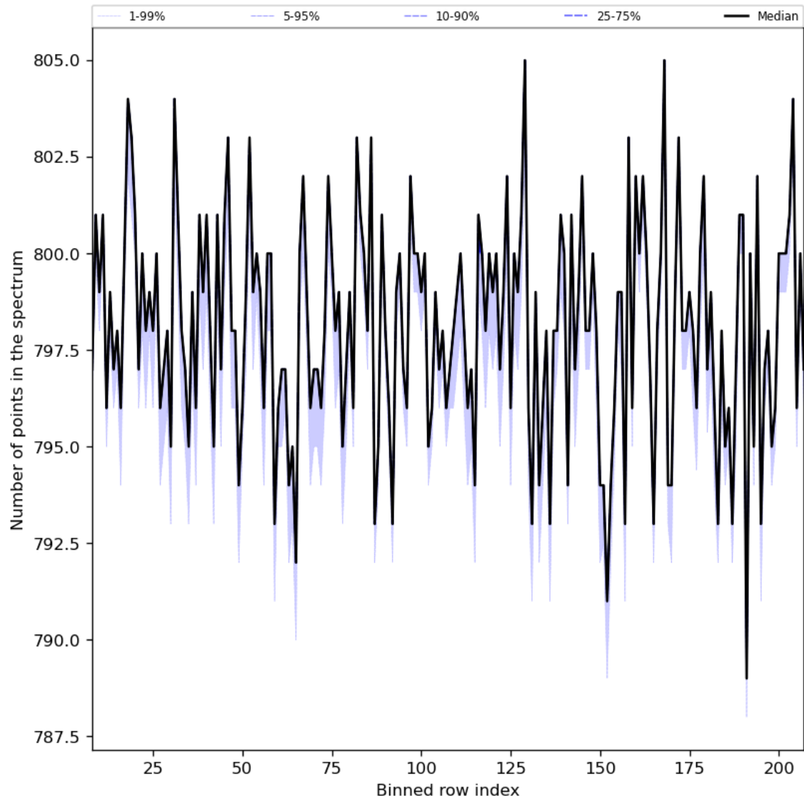
Figure 37: Along track statistics of “Number of points in the spectrum” for 2023-08-12 to 2023-08-14
