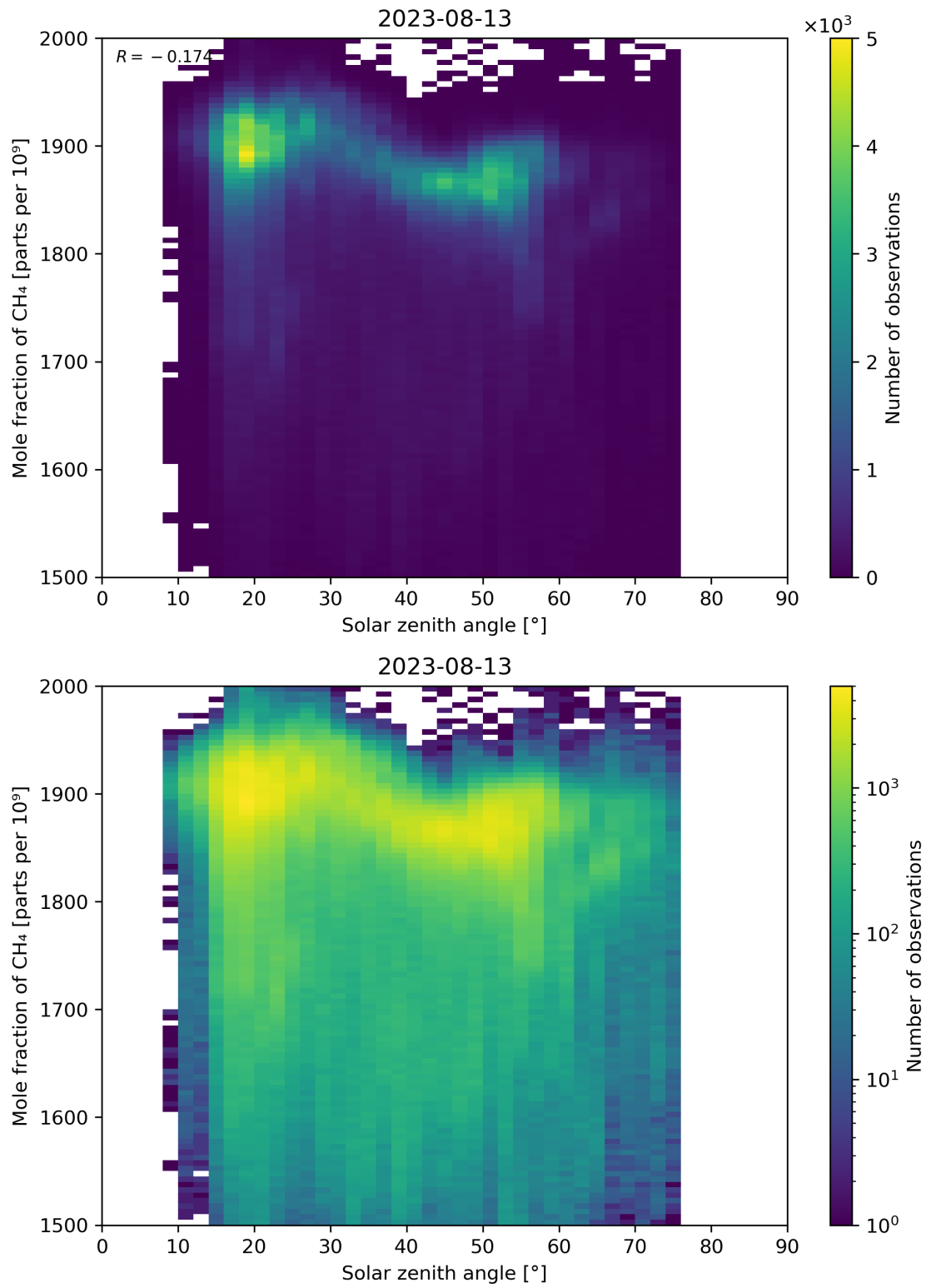
Figure 99: Scatter density plot of “Solar zenith angle” against “Mole fraction of CH 4 ” for 2023-08-12 to 2023-08-14.
