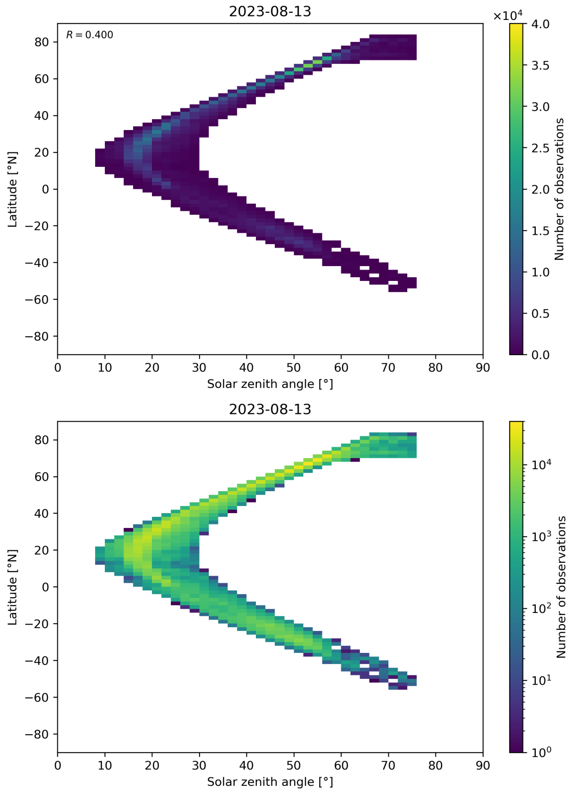
Figure 98: Scatter density plot of “Solar zenith angle” against “Latitude” for 2023-08-12 to 2023-08-14.
