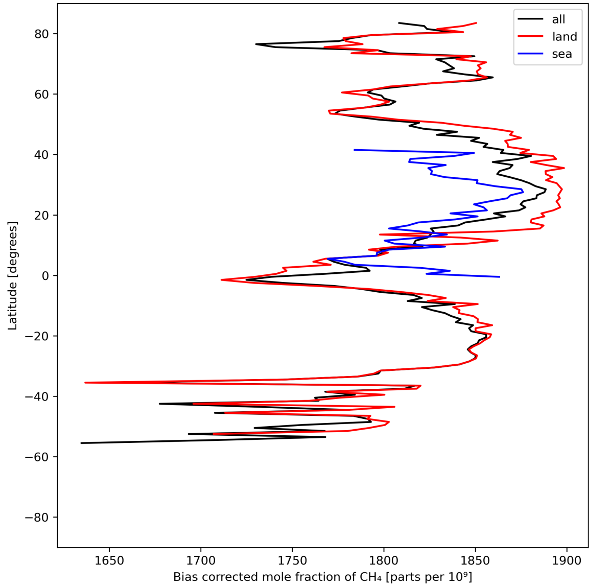
Figure 14: Zonal average of “Bias corrected mole fraction of CH 4 ” for 2023-08-12 to 2023-08-14.
