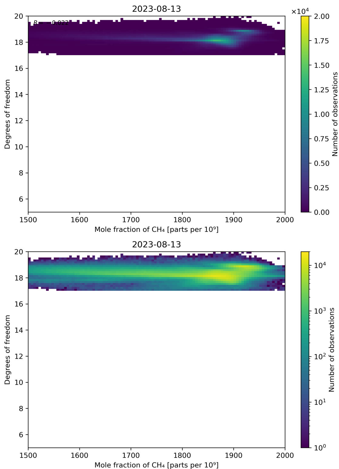
Figure 72: Scatter density plot of “Mole fraction of CH 4 ” against “Degrees of freedom” for 2023-08-12 to 2023-08-14.
