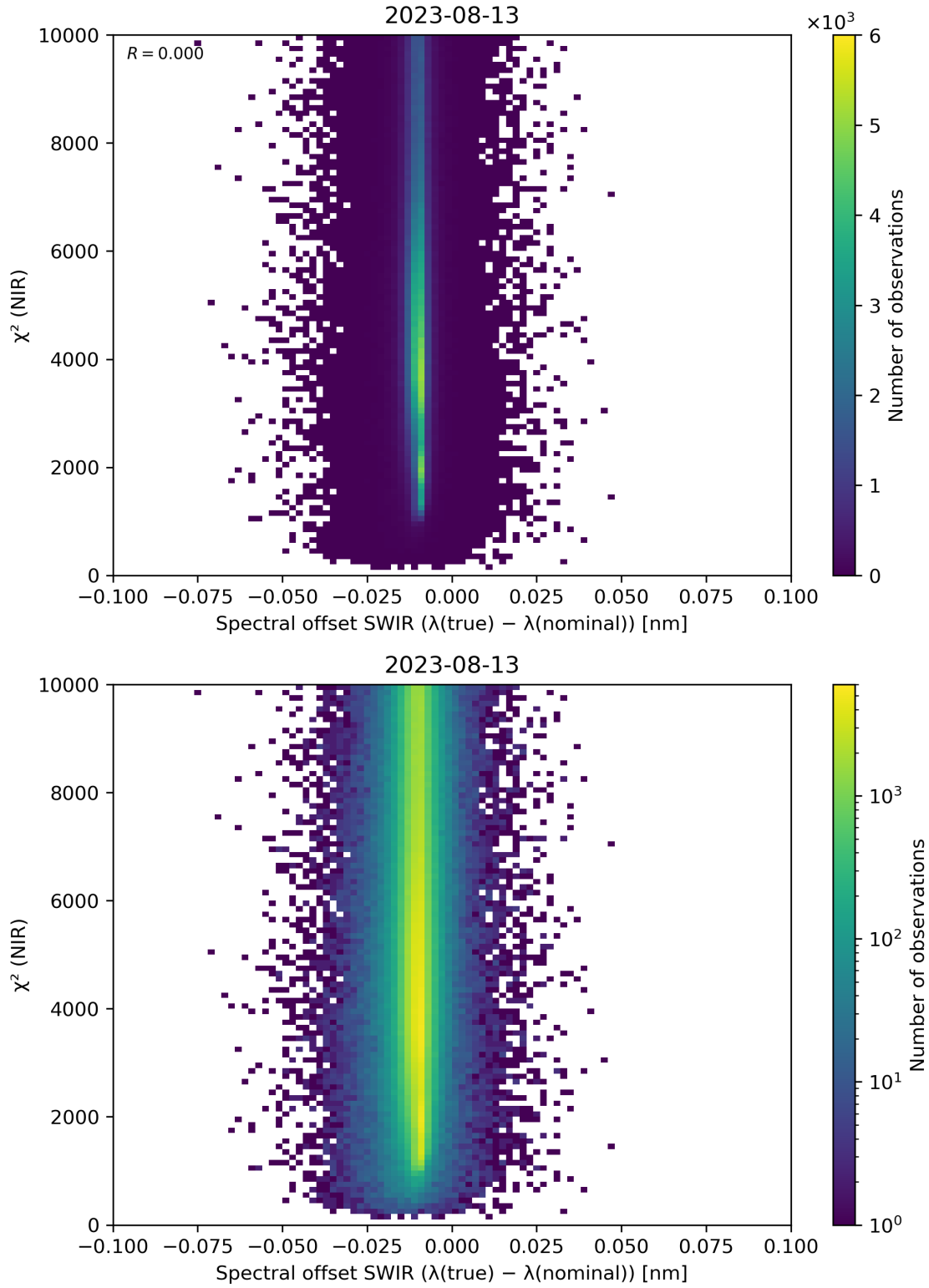
Figure 117: Scatter density plot of “Spectral offset SWIR ( \lambda(\text{true}) - \lambda(\text{nominal}) )” against “ \chi^2 (NIR)” for 2023-08-12 to 2023-08-14.
