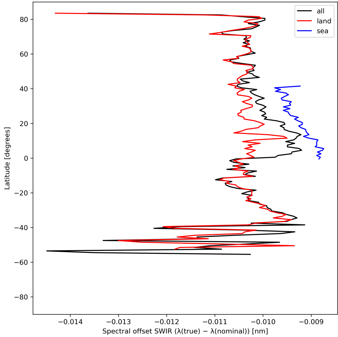
Figure 16: Zonal average of “Spectral offset SWIR ( \lambda(\text{true}) - \lambda(\text{nominal}) )” for 2023-08-12 to 2023-08-14.
