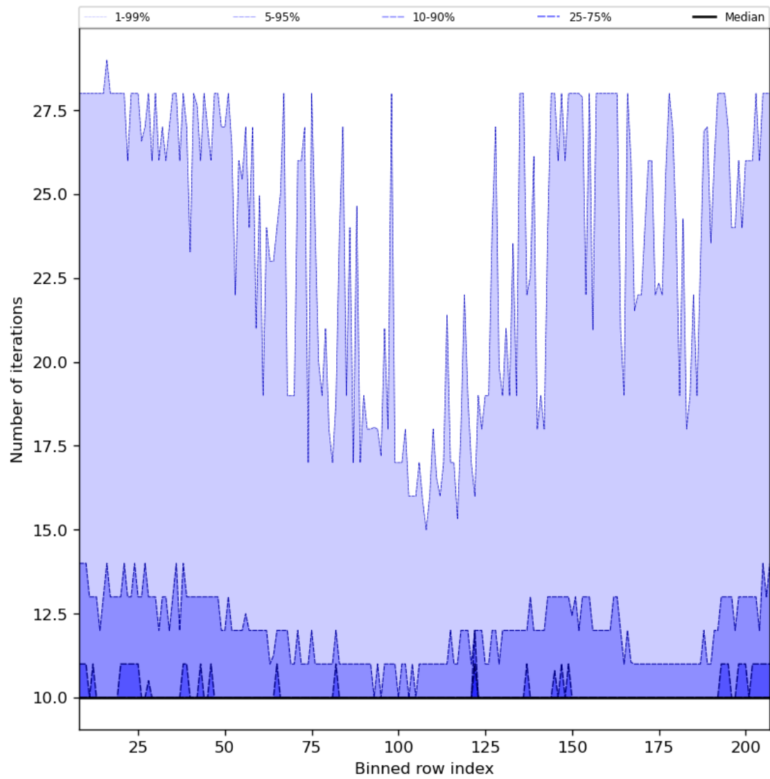
Figure 42: Along track statistics of “Number of iterations” for 2023-08-12 to 2023-08-14
