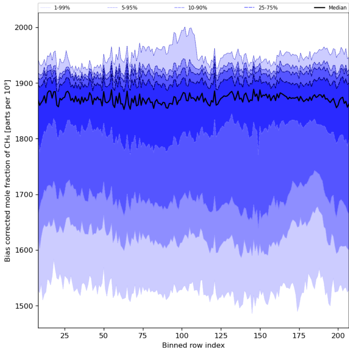
Figure 36: Along track statistics of “Bias corrected mole fraction of CH 4 ” for 2023-08-12 to 2023-08-14
