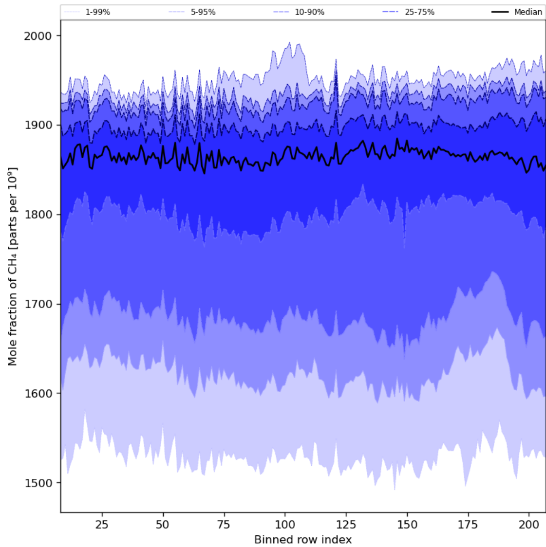
Figure 34: Along track statistics of “Mole fraction of CH 4 ” for 2023-08-12 to 2023-08-14
