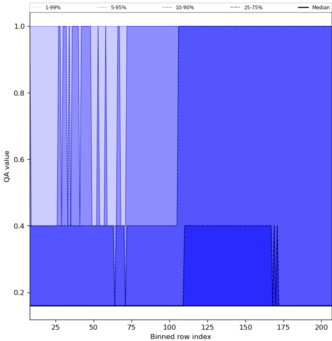
Figure 33: Along track statistics of “QA value” for 2023-08-12 to 2023-08-14
