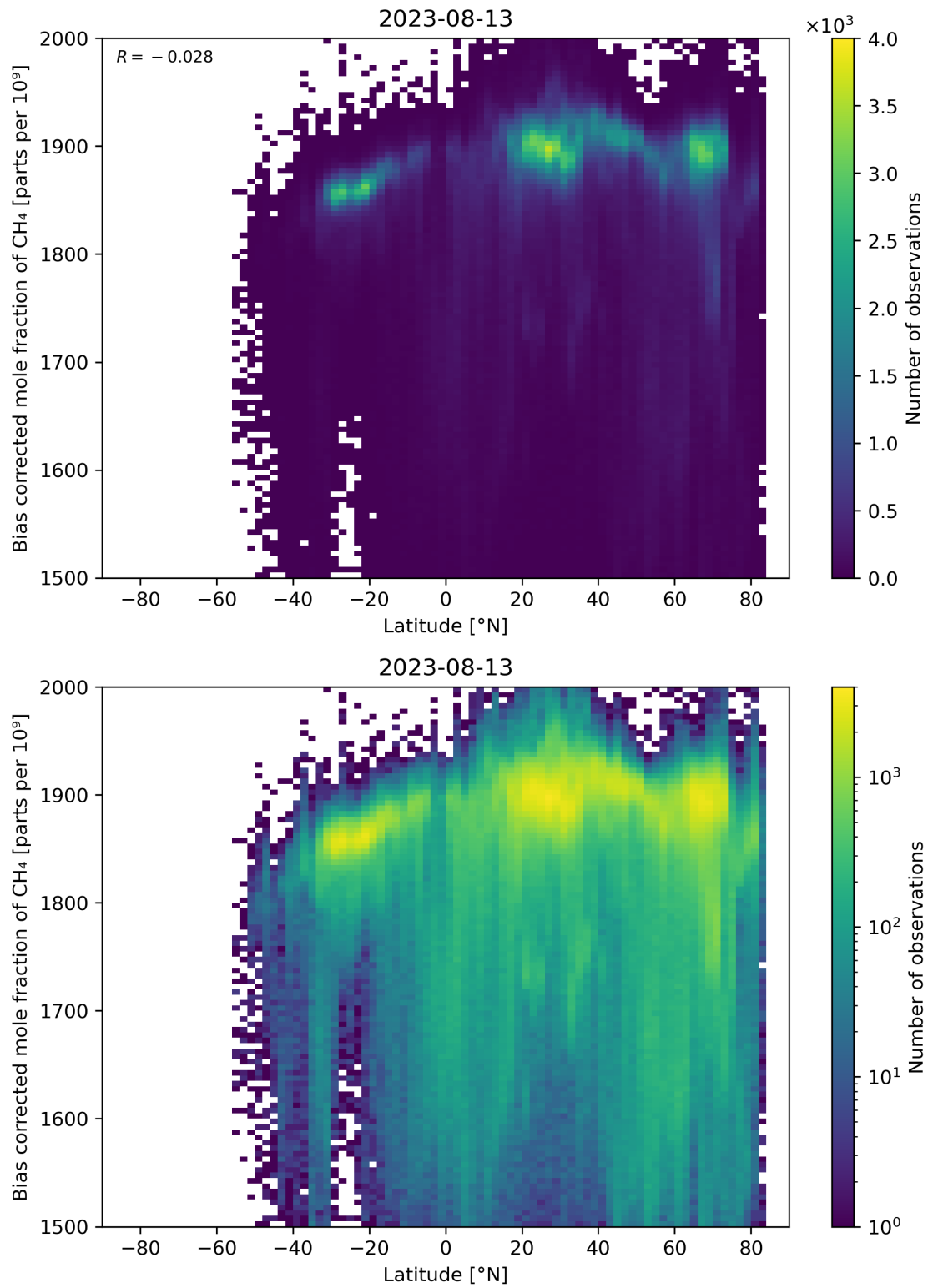
Figure 58: Scatter density plot of “Latitude” against “Bias corrected mole fraction of \text{CH}_4 ” for 2023-08-12 to 2023-08-14.
