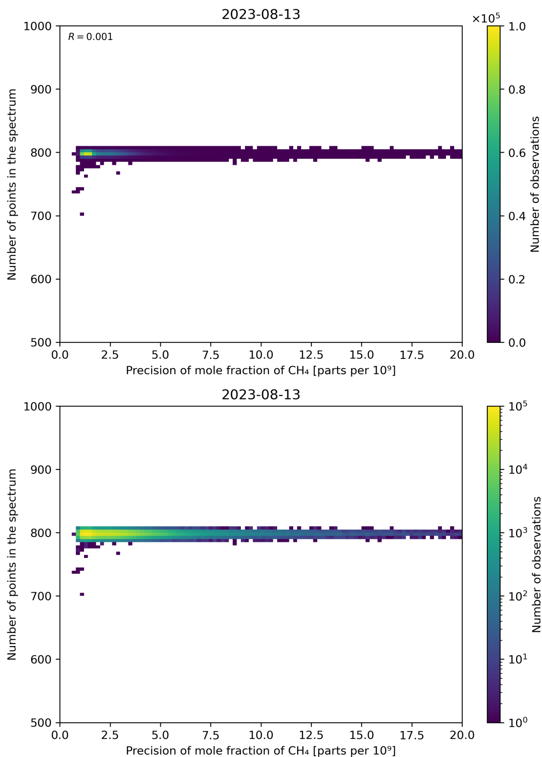
Figure 84: Scatter density plot of “Precision of mole fraction of CH 4 ” against “Number of points in the spectrum” for 2023-08-12 to 2023-08-14.
