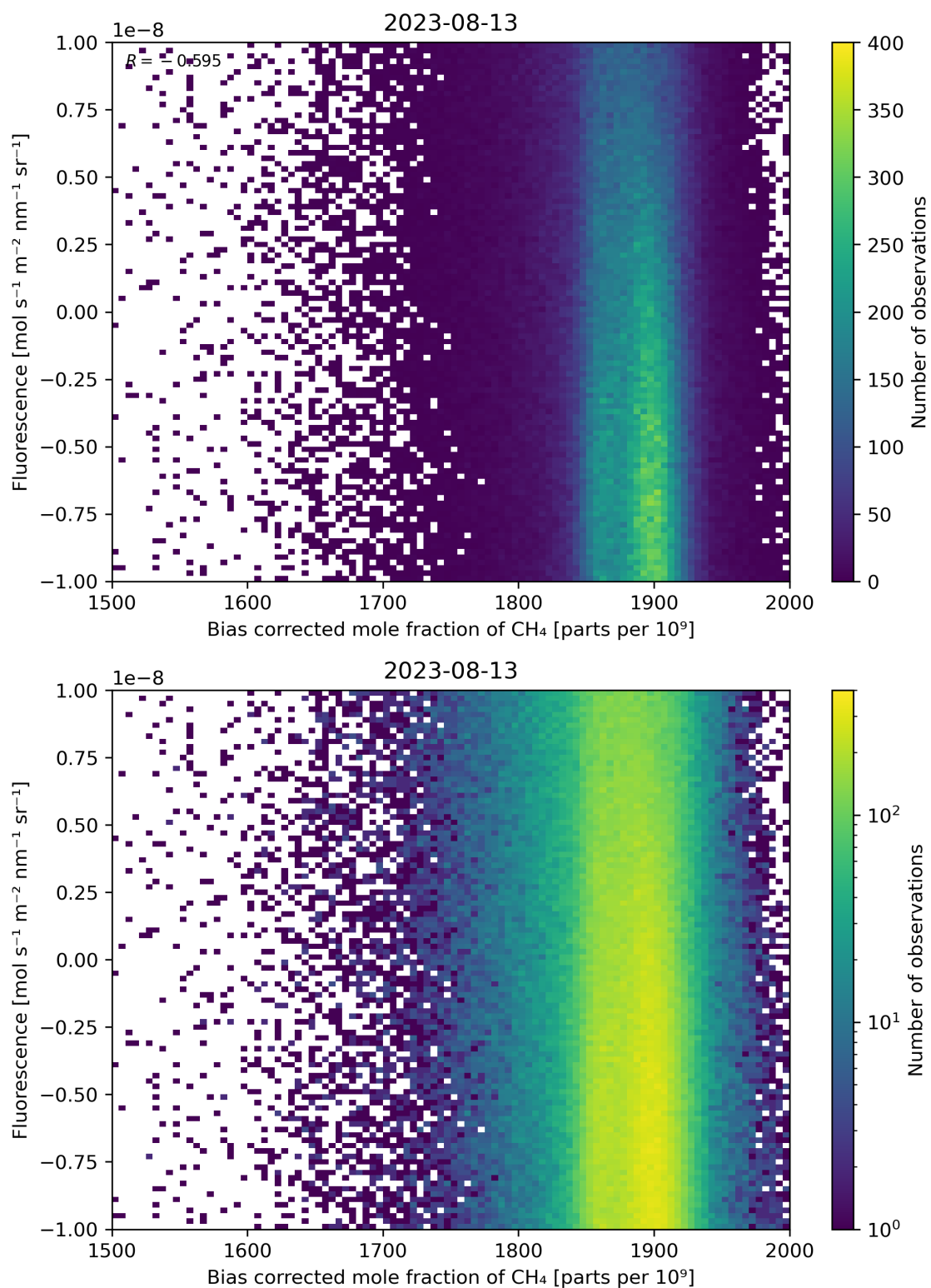
Figure 66: Scatter density plot of “Bias corrected mole fraction of \text{CH}_4 ” against “Fluorescence” for 2023-08-12 to 2023-08-14.
