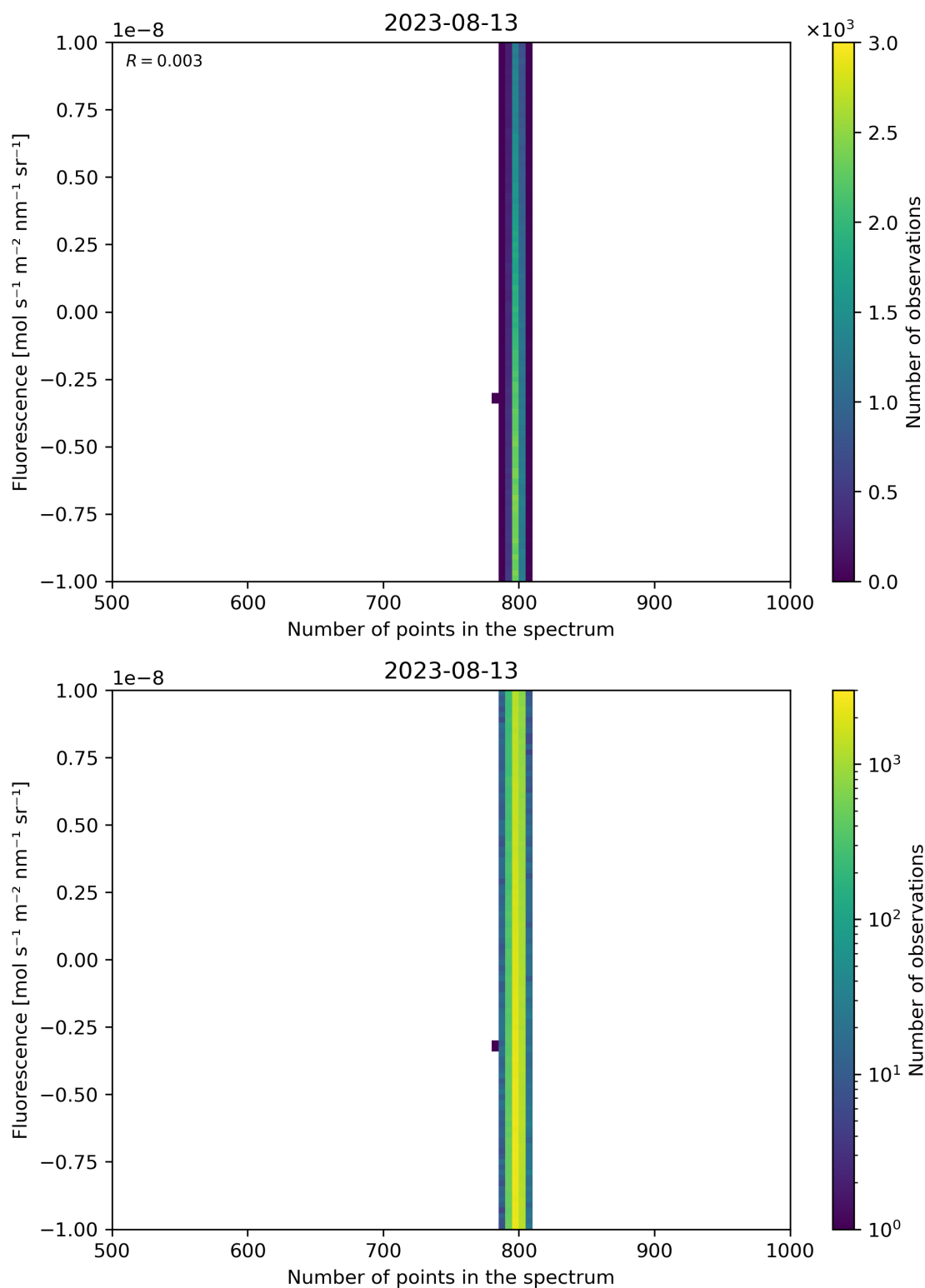
Figure 91: Scatter density plot of “Number of points in the spectrum” against “Fluorescence” for 2023-08-12 to 2023-08-14.
