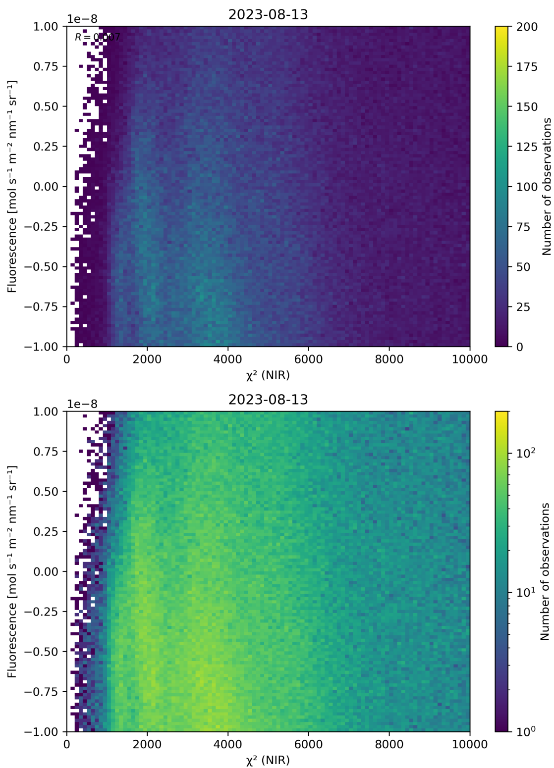
Figure 45: Scatter density plot of “ \chi^2 (NIR)” against “Fluorescence” for 2023-08-12 to 2023-08-14.
