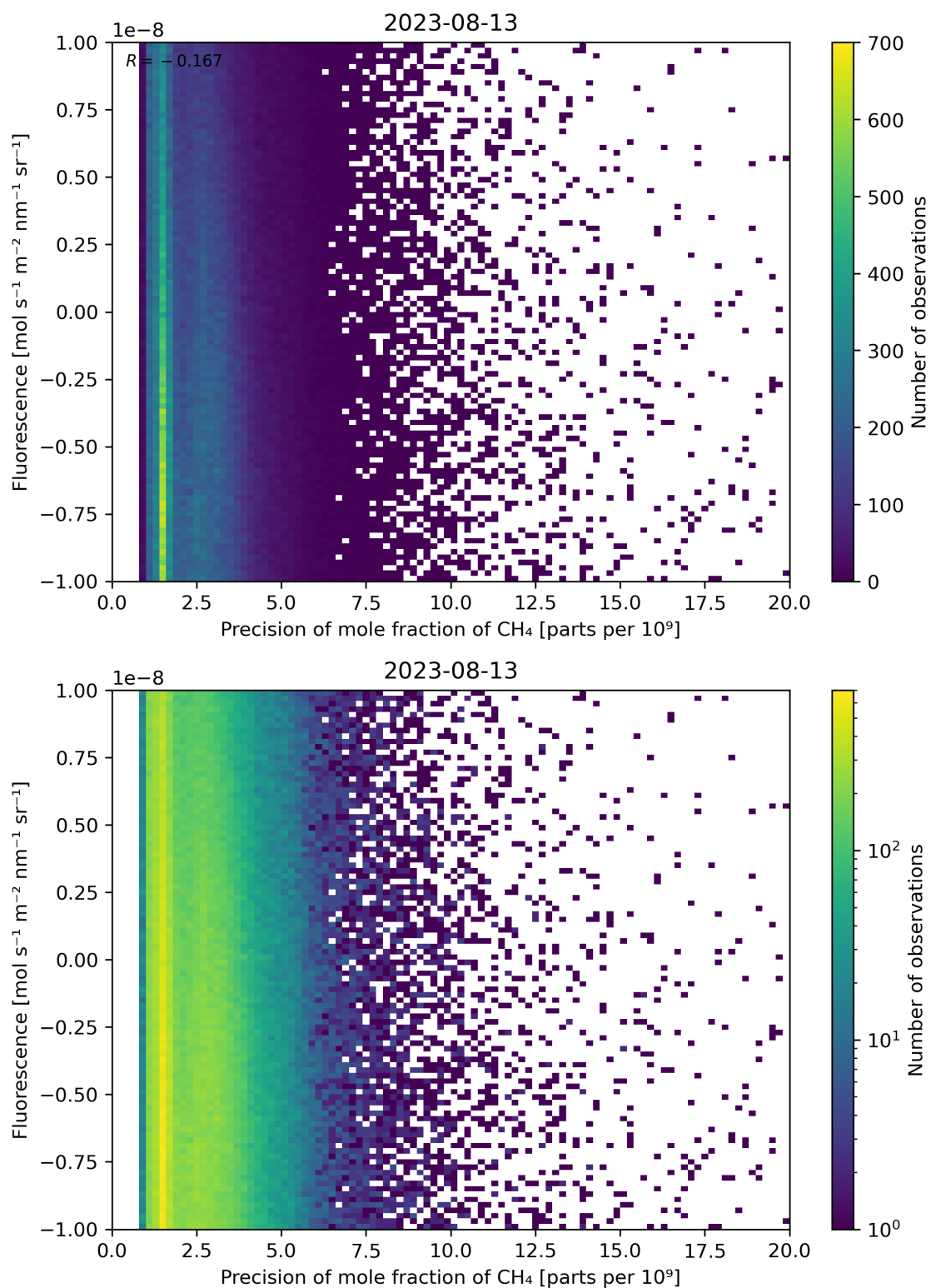
Figure 81: Scatter density plot of “Precision of mole fraction of \text{CH}_4 ” against “Fluorescence” for 2023-08-12 to 2023-08-14.
