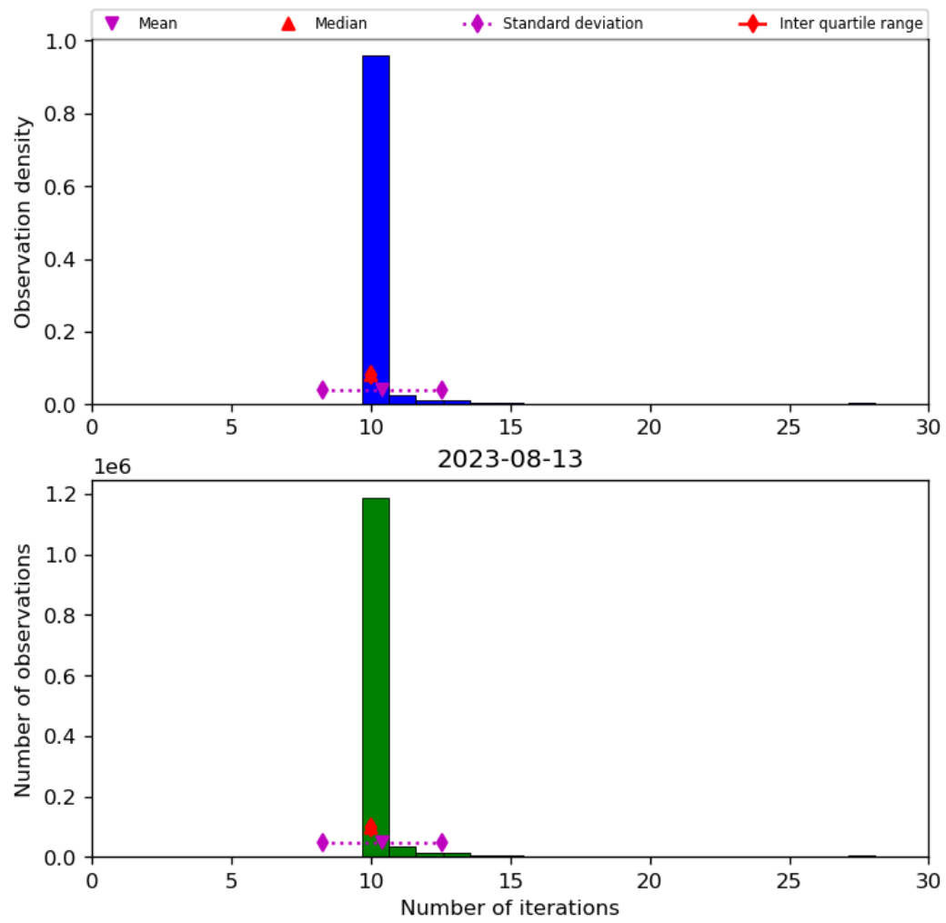
Figure 31: Histogram of “Number of iterations” for 2023-08-12 to 2023-08-14
