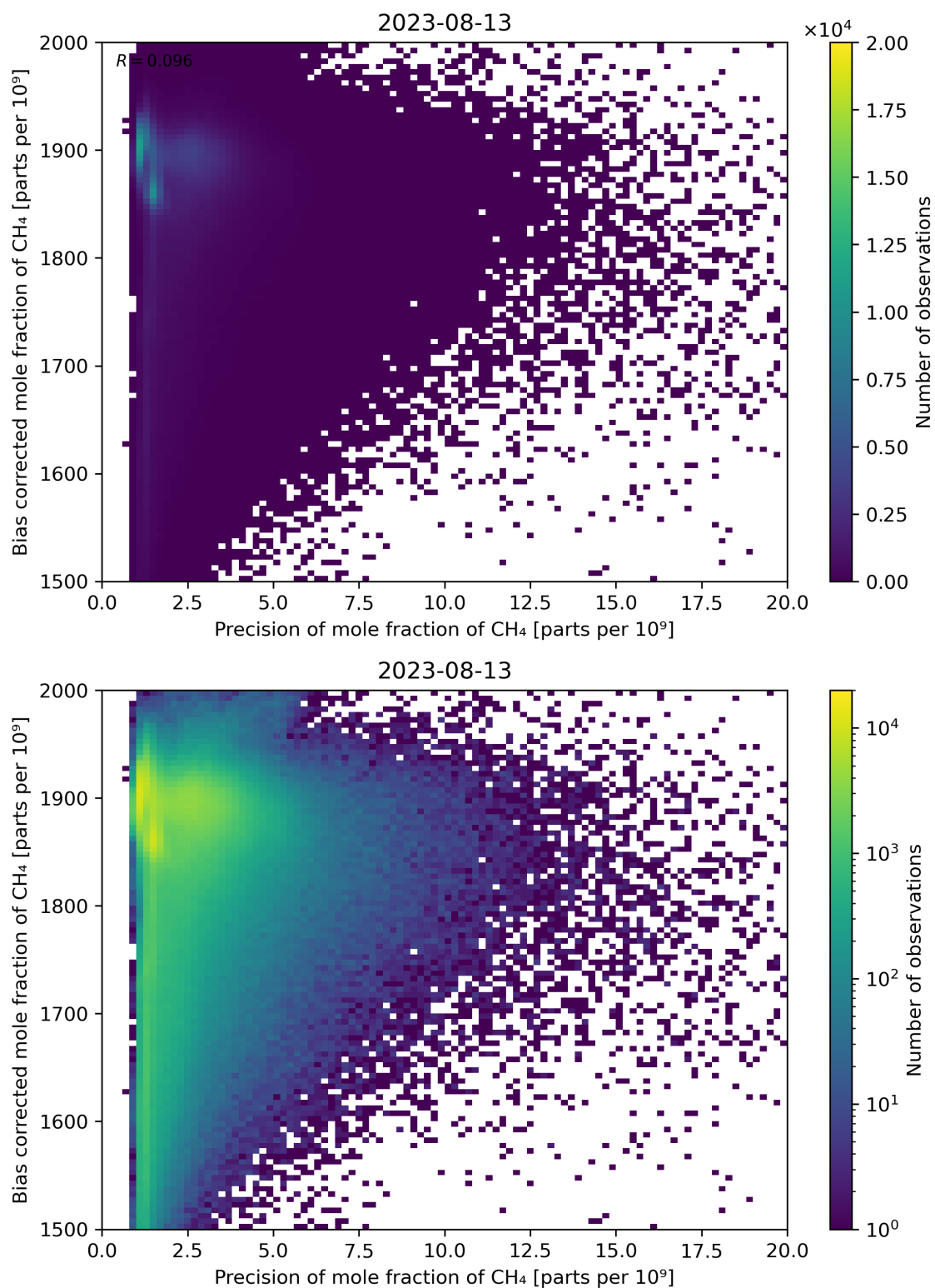
Figure 82: Scatter density plot of “Precision of mole fraction of CH 4 ” against “Bias corrected mole fraction of CH 4 ” for 2023-08-12 to 2023-08-14.
