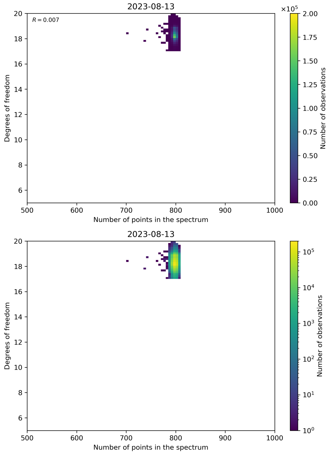
Figure 90: Scatter density plot of “Number of points in the spectrum” against “Degrees of freedom” for 2023-08-12 to 2023-08-14.
