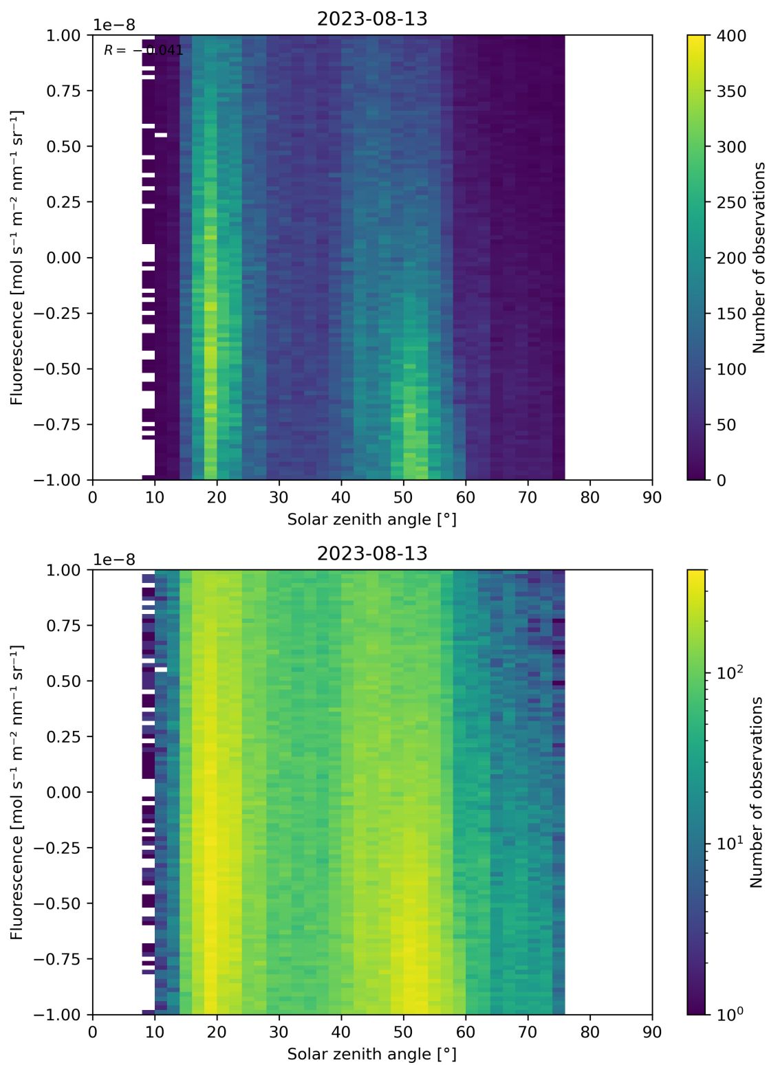
Figure 97: Scatter density plot of “Solar zenith angle” against “Fluorescence” for 2023-08-12 to 2023-08-14.
