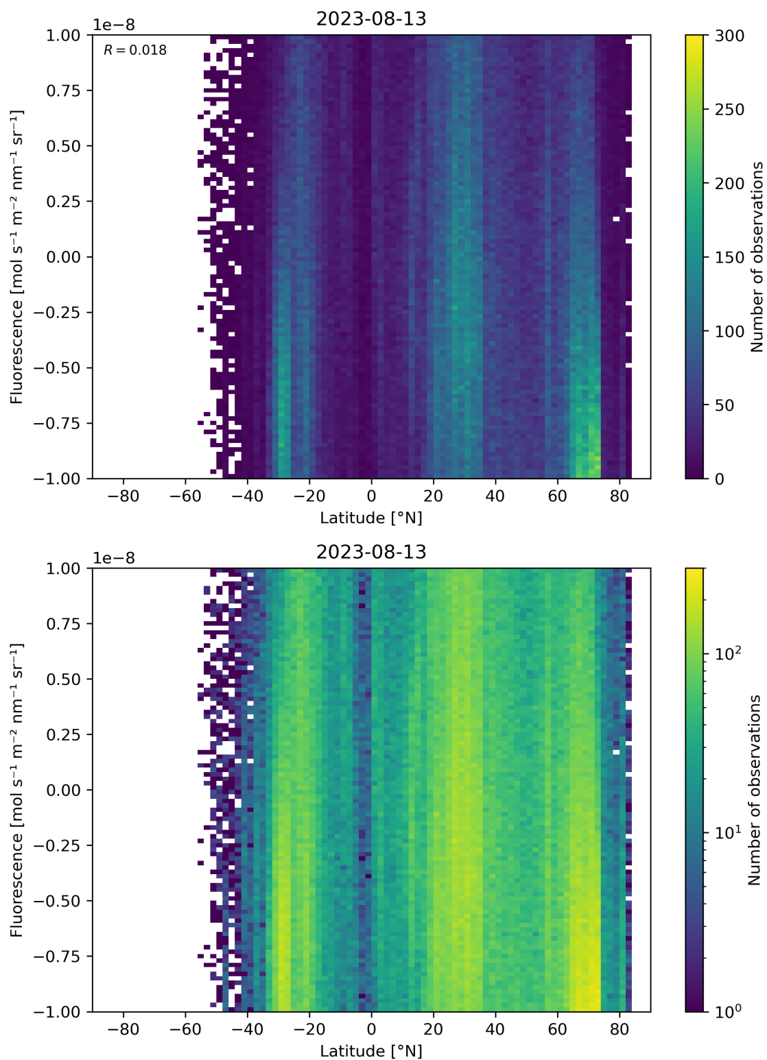
Figure 56: Scatter density plot of “Latitude” against “Fluorescence” for 2023-08-12 to 2023-08-14.
