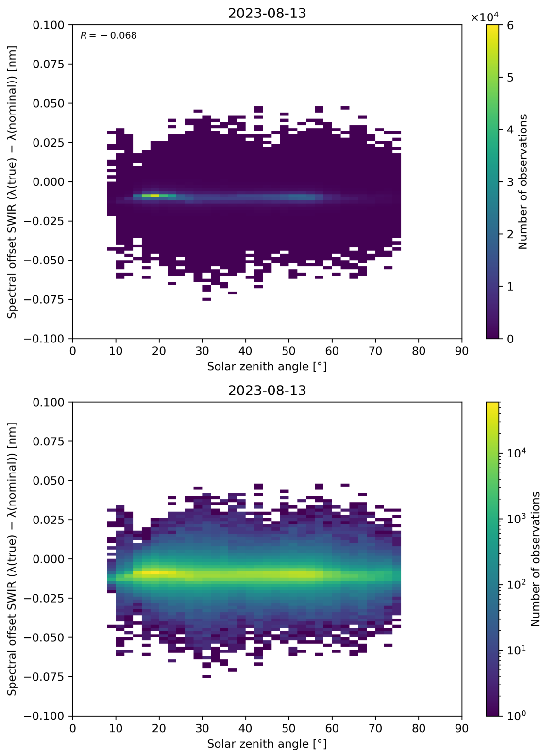
Figure 104: Scatter density plot of “Solar zenith angle” against “Spectral offset SWIR ( \lambda(\text{true}) - \lambda(\text{nominal}) )” for 2023-08-12 to 2023-08-14.
