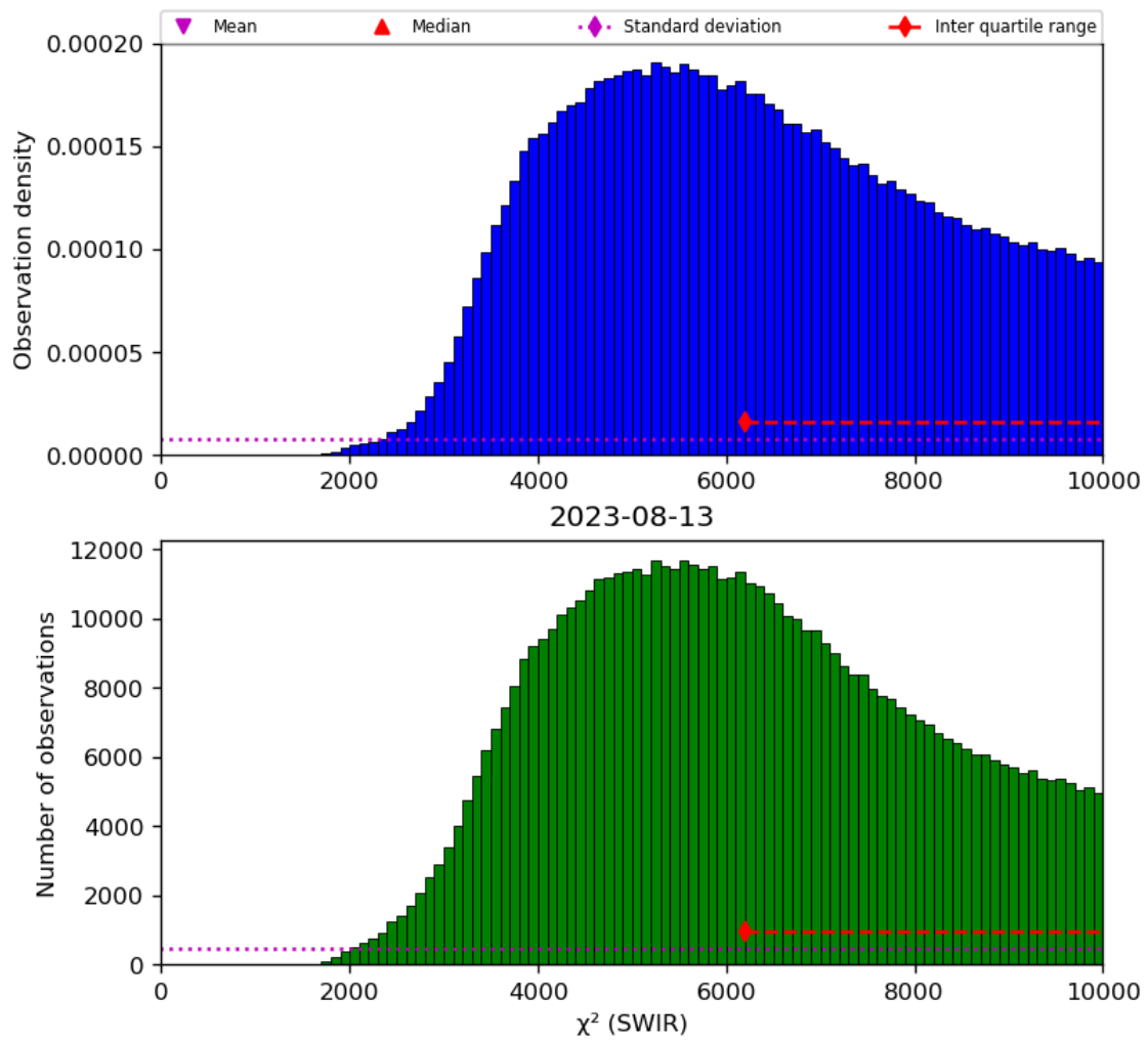
Figure 28: Histogram of “ \chi^2 (SWIR)” for 2023-08-12 to 2023-08-14
