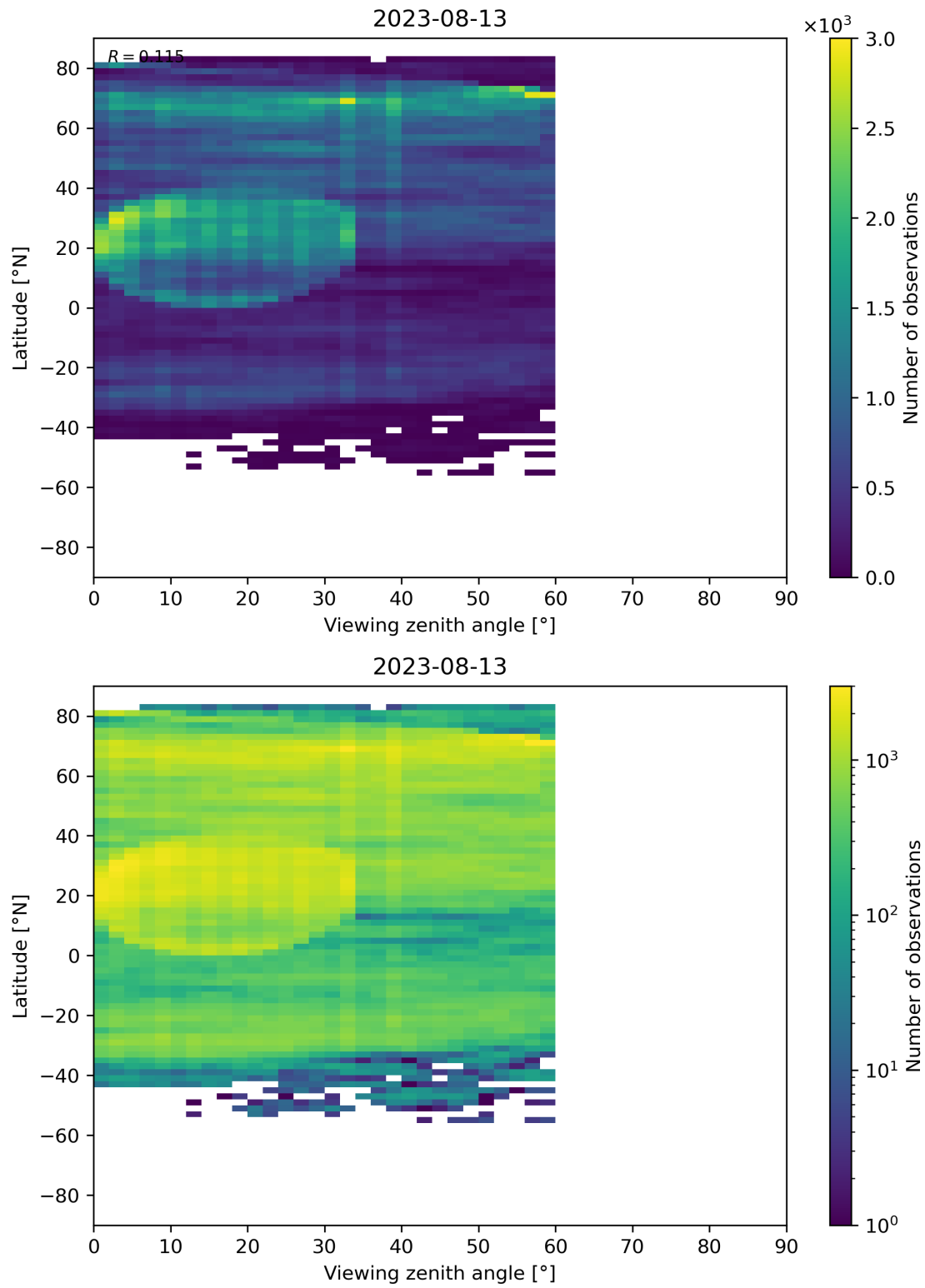
Figure 109: Scatter density plot of “Viewing zenith angle” against “Latitude” for 2023-08-12 to 2023-08-14.
