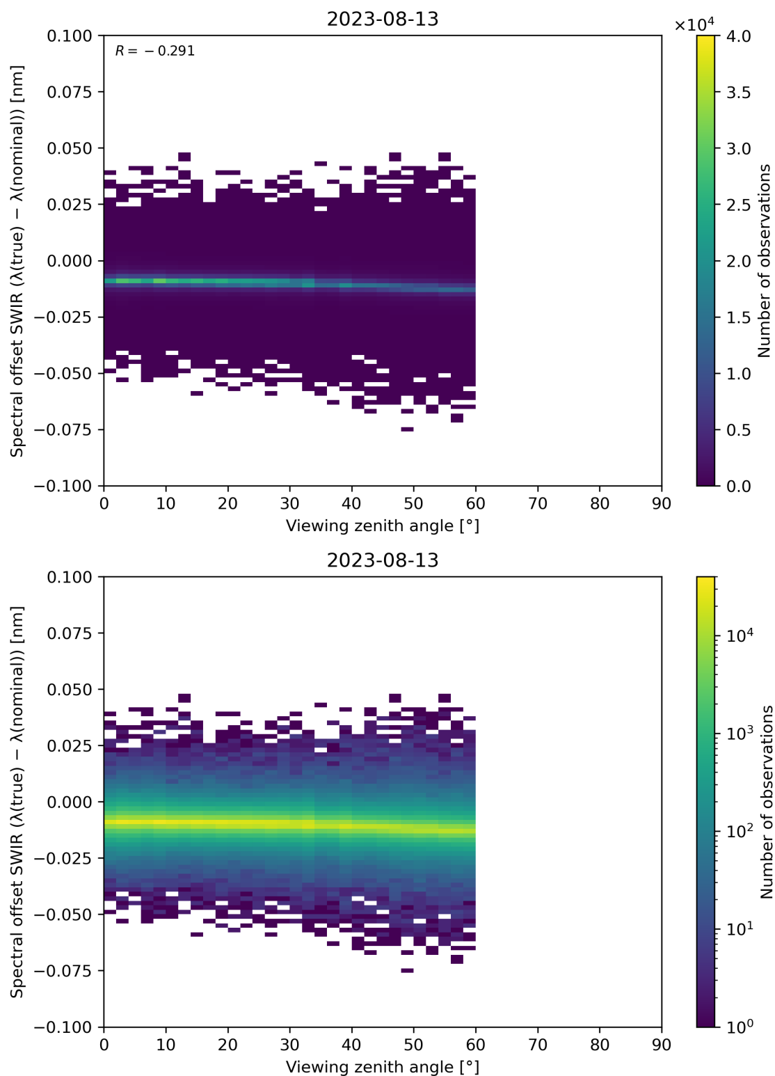
Figure 116: Scatter density plot of “Viewing zenith angle” against “Spectral offset SWIR ( \lambda(\text{true}) - \lambda(\text{nominal}) )” for 2023-08-12 to 2023-08-14.
