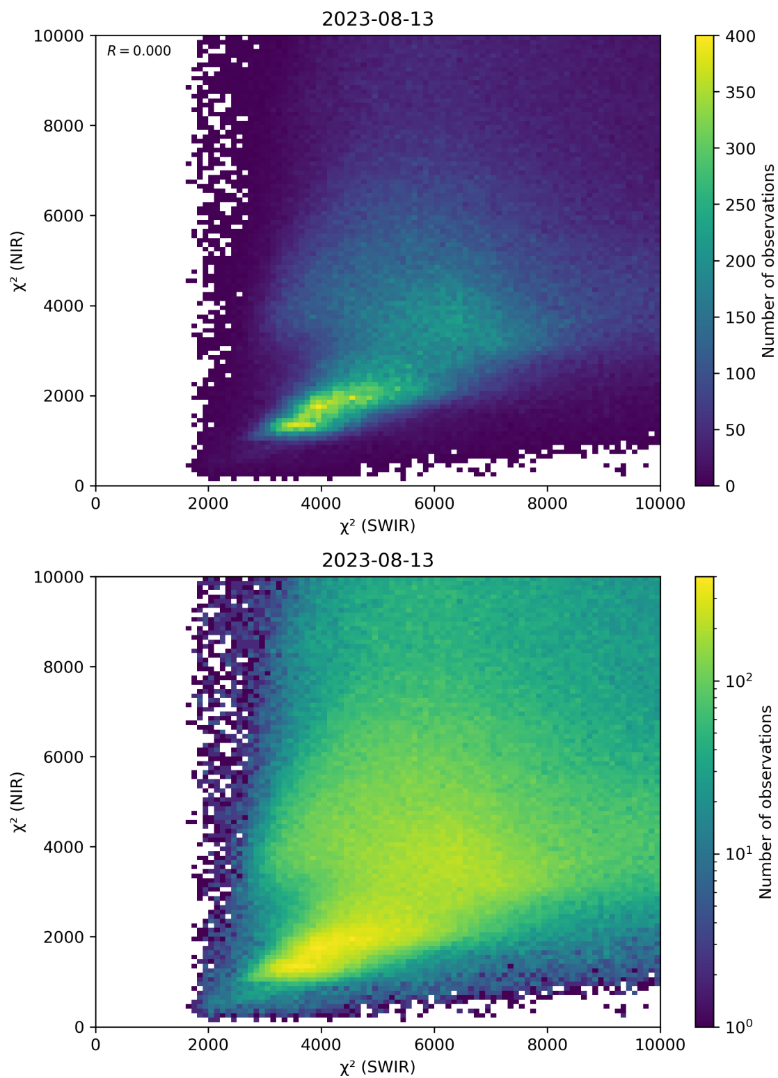
Figure 47: Scatter density plot of “ \chi^2 (SWIR)” against “ \chi^2 (NIR)” for 2023-08-12 to 2023-08-14.
