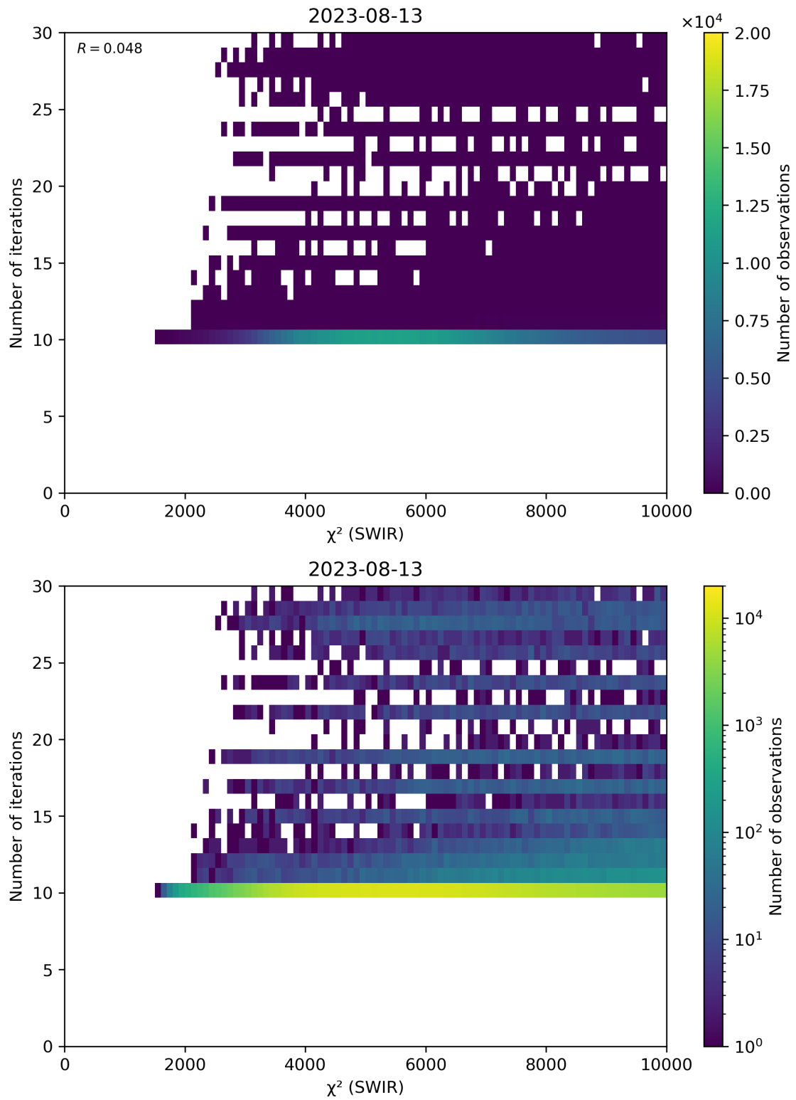
Figure 50: Scatter density plot of “ \chi^2 (SWIR)” against “Number of iterations” for 2023-08-12 to 2023-08-14.
