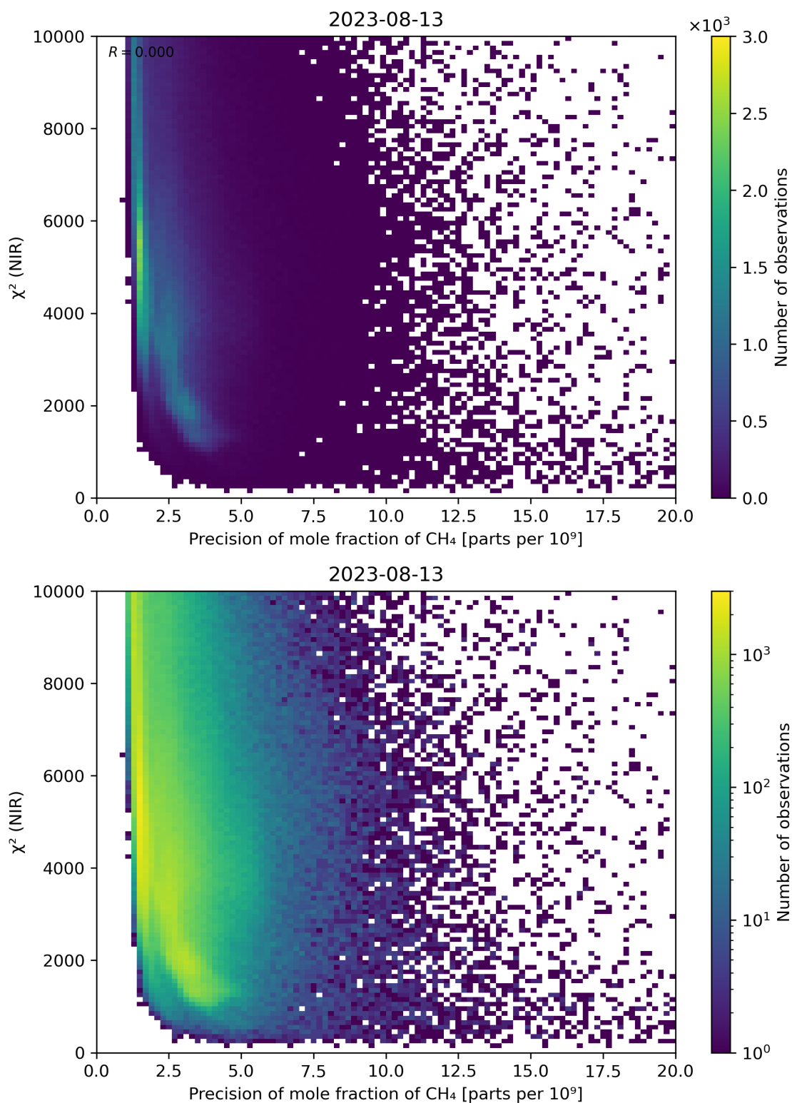
Figure 78: Scatter density plot of “Precision of mole fraction of CH 4 ” against “ \chi^2 (NIR)” for 2023-08-12 to 2023-08-14.
