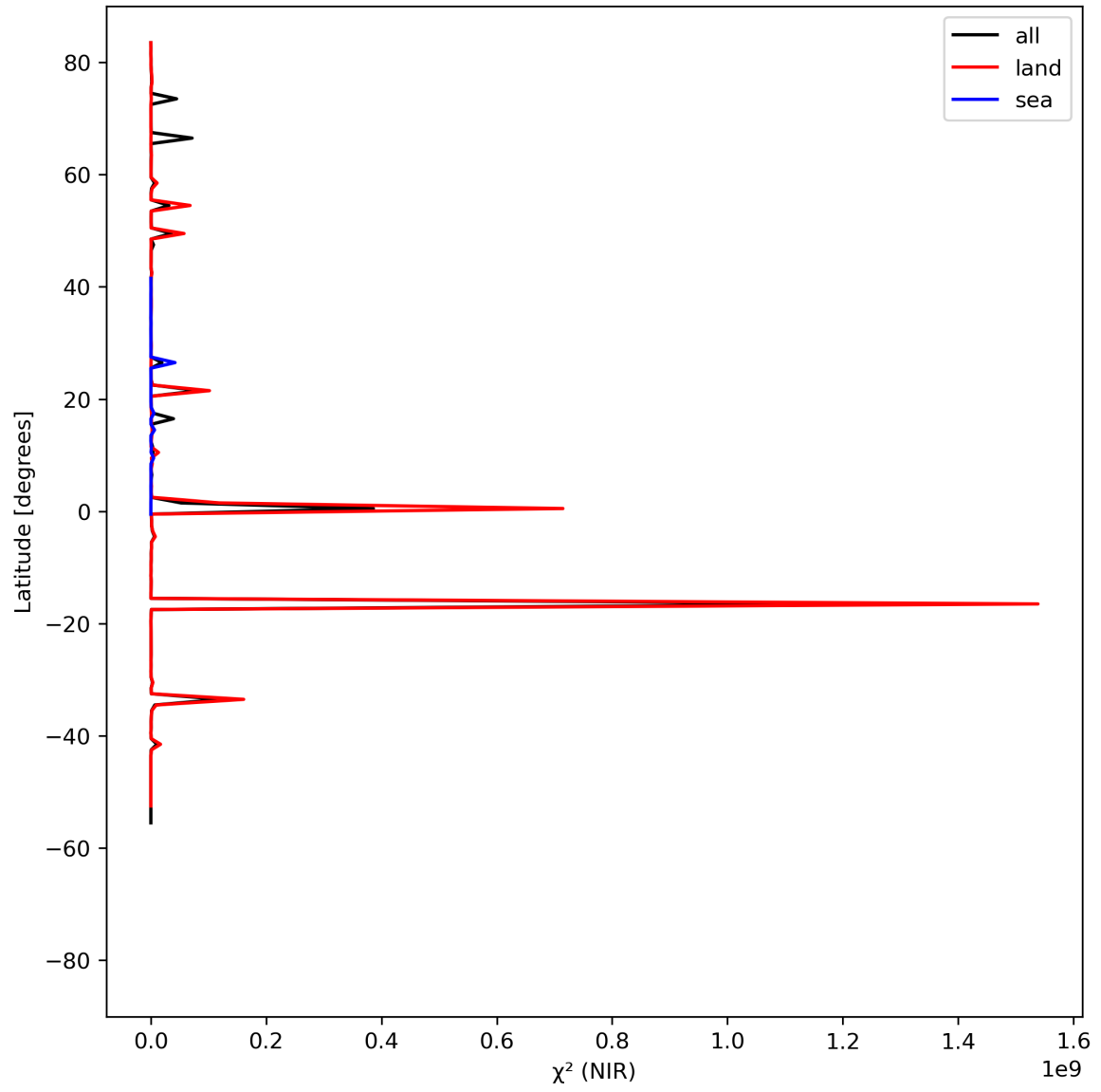
Figure 18: Zonal average of “ \chi^2 (NIR)” for 2023-08-12 to 2023-08-14.
