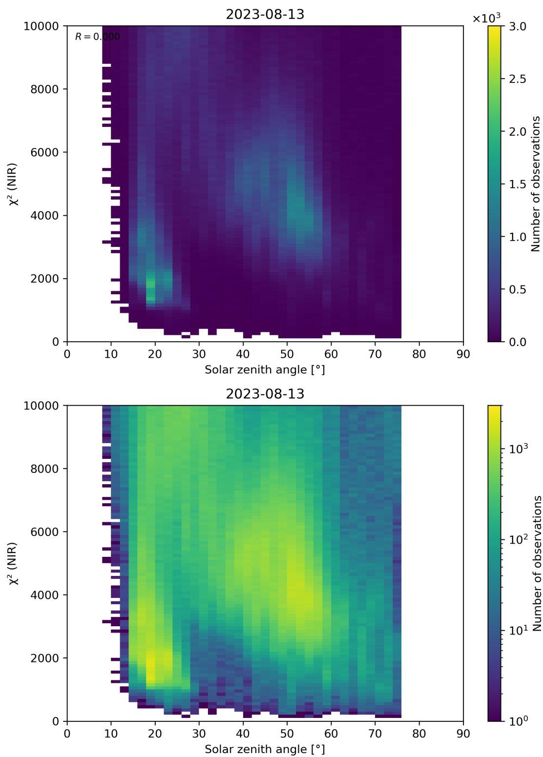
Figure 94: Scatter density plot of “Solar zenith angle” against “ \chi^2 (NIR)” for 2023-08-12 to 2023-08-14.
