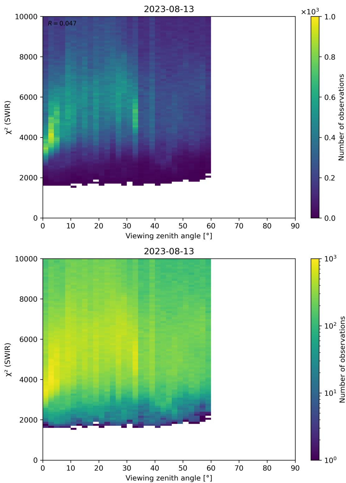
Figure 106: Scatter density plot of “Viewing zenith angle” against “ \chi^2 (SWIR)” for 2023-08-12 to 2023-08-14.
