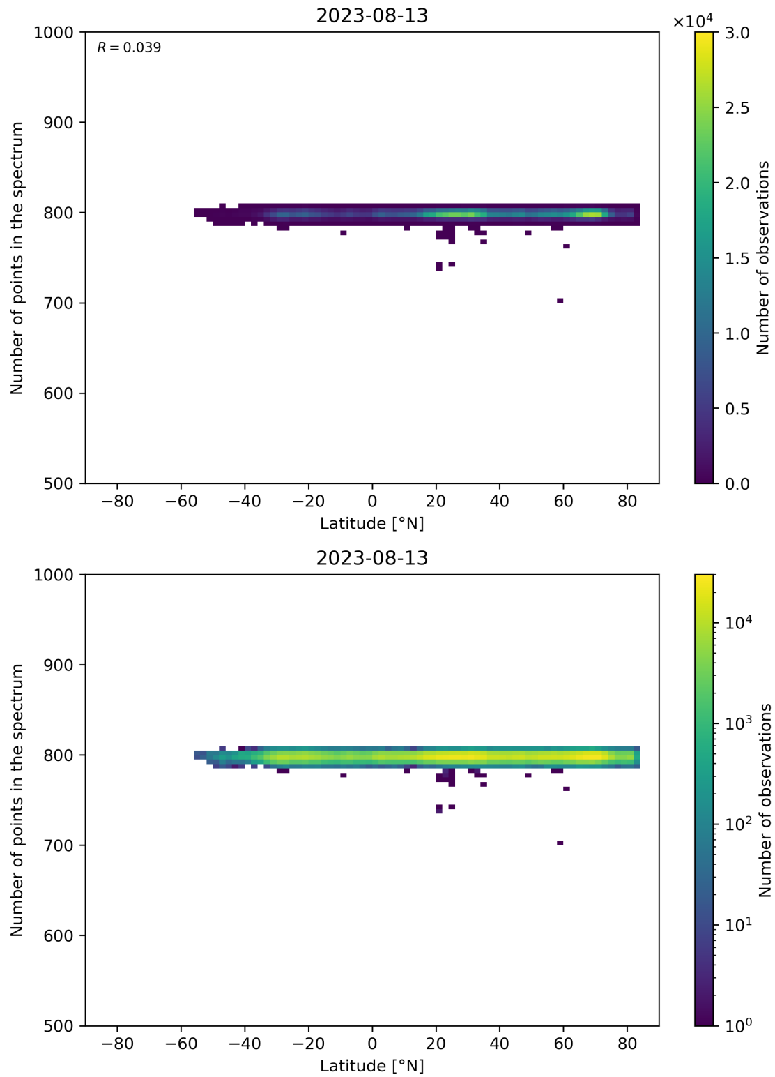
Figure 61: Scatter density plot of “Latitude” against “Number of points in the spectrum” for 2023-08-12 to 2023-08-14.
