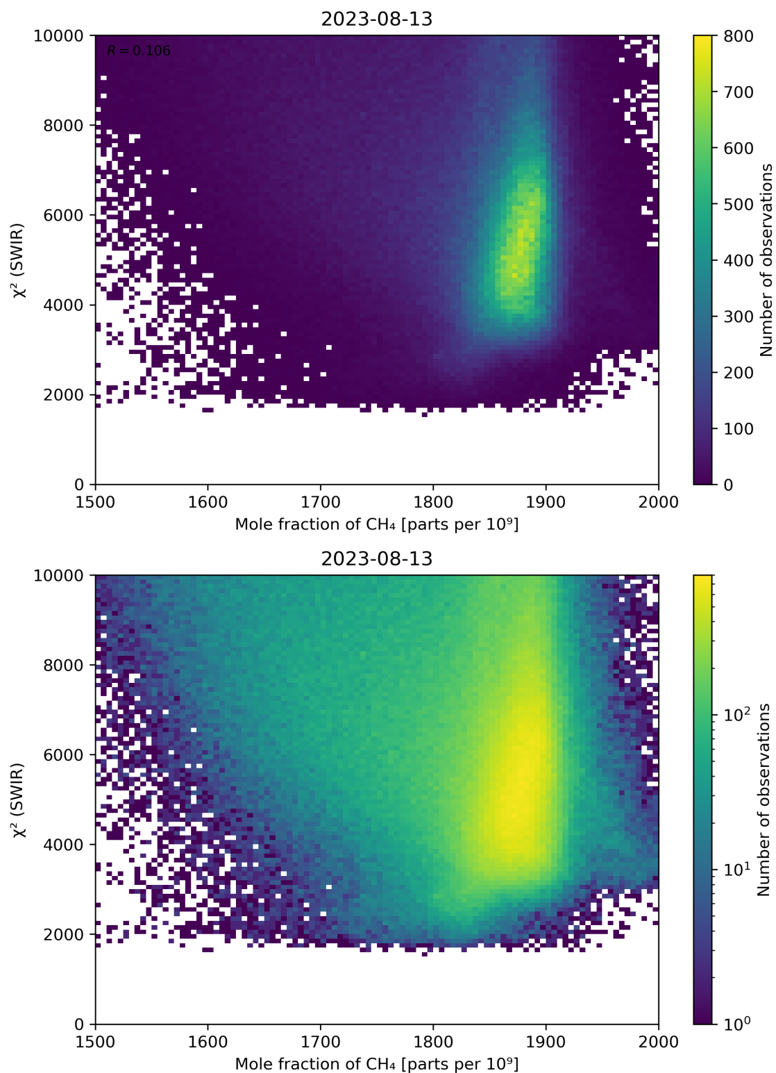
Figure 71: Scatter density plot of “Mole fraction of \text{CH}_4 ” against “ \chi^2 (SWIR)” for 2023-08-12 to 2023-08-14.
