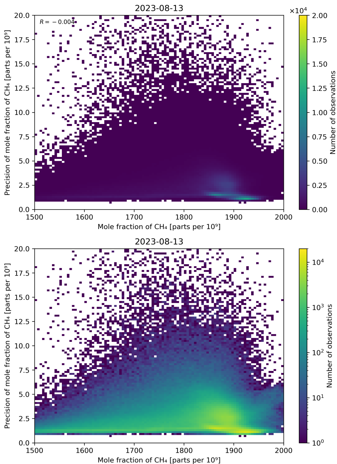
Figure 75: Scatter density plot of “Mole fraction of CH 4 ” against “Precision of mole fraction of CH 4 ” for 2023-08-12 to 2023-08-14.
