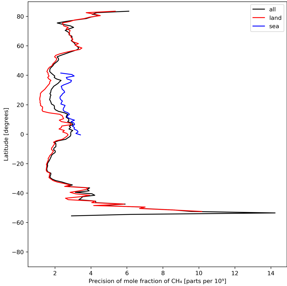
Figure 13: Zonal average of “Precision of mole fraction of CH 4 ” for 2023-08-12 to 2023-08-14.
