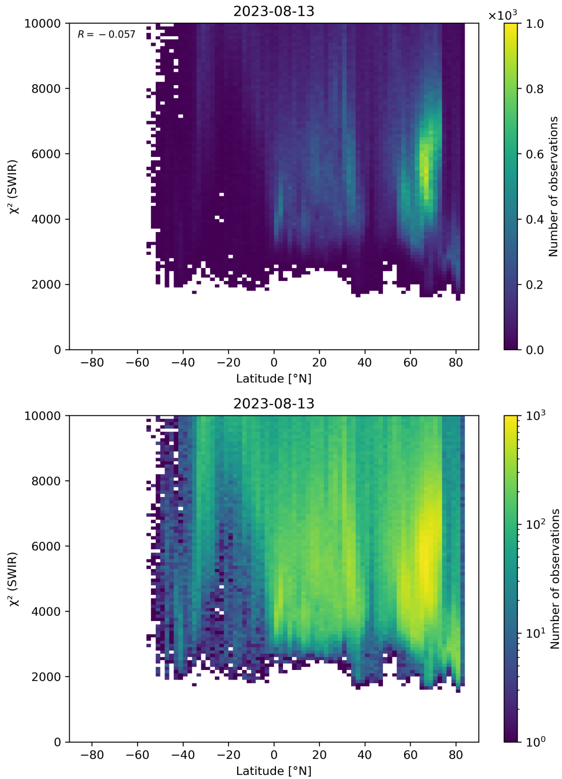
Figure 54: Scatter density plot of “Latitude” against “ \chi^2 (SWIR)” for 2023-08-12 to 2023-08-14.
