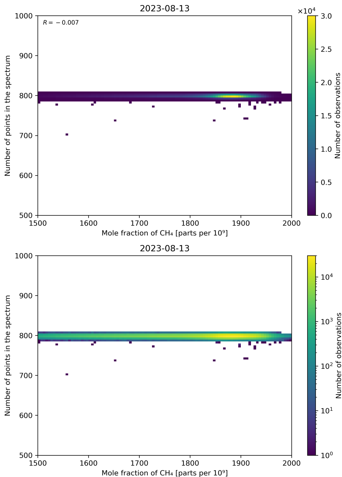
Figure 77: Scatter density plot of “Mole fraction of CH 4 ” against “Number of points in the spectrum” for 2023-08-12 to 2023-08-14.
