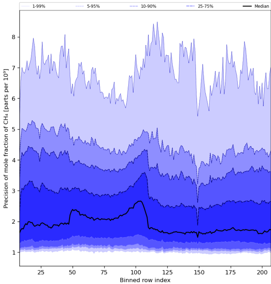
Figure 35: Along track statistics of “Precision of mole fraction of CH 4 ” for 2023-08-12 to 2023-08-14
