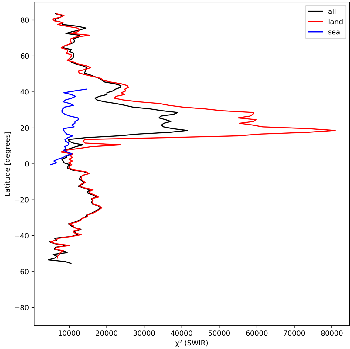
Figure 17: Zonal average of “ \chi^2 (SWIR)” for 2023-08-12 to 2023-08-14.
