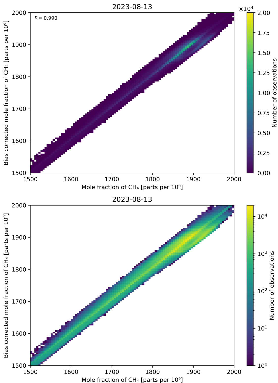
Figure 74: Scatter density plot of “Mole fraction of CH 4 ” against “Bias corrected mole fraction of CH 4 ” for 2023-08-12 to 2023-08-14.
