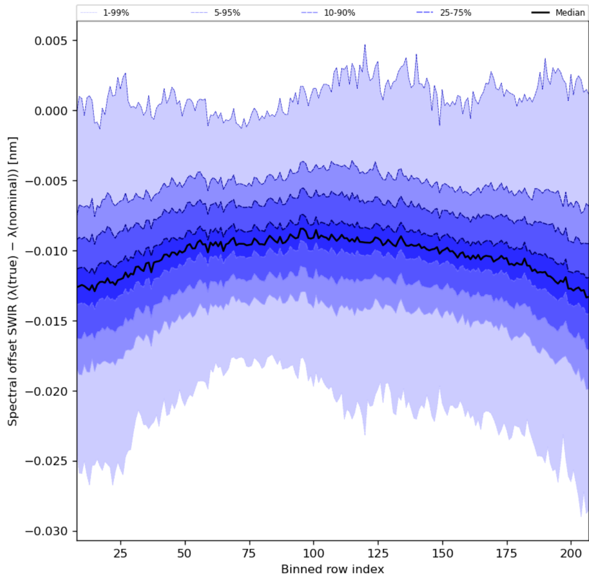
Figure 38: Along track statistics of “Spectral offset SWIR ( \lambda(\text{true}) - \lambda(\text{nominal}) )” for 2023-08-12 to 2023-08-14
