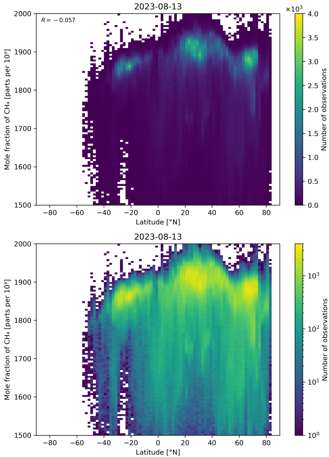
Figure 57: Scatter density plot of “Latitude” against “Mole fraction of CH 4 ” for 2023-08-12 to 2023-08-14.
