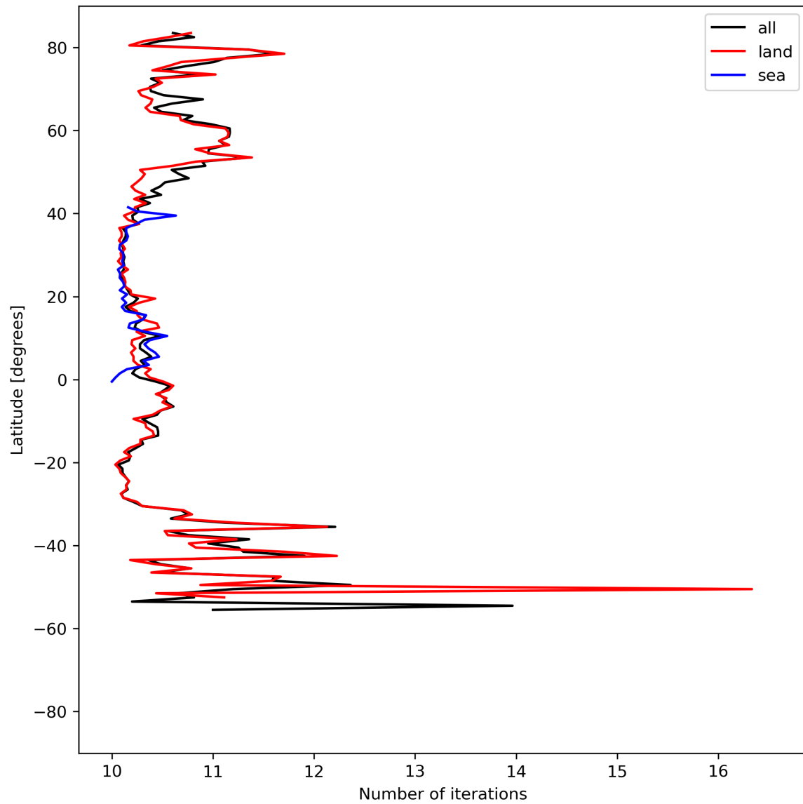
Figure 20: Zonal average of “Number of iterations” for 2023-08-12 to 2023-08-14.
