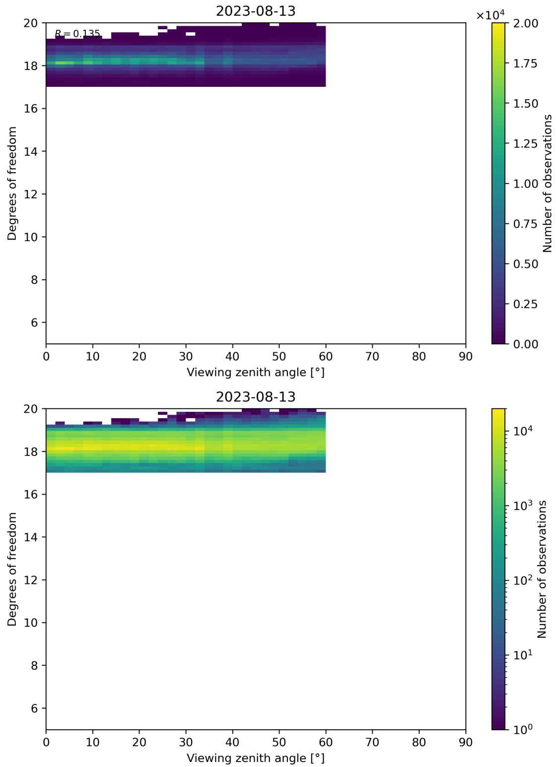
Figure 107: Scatter density plot of “Viewing zenith angle” against “Degrees of freedom” for 2023-08-12 to 2023-08-14.
