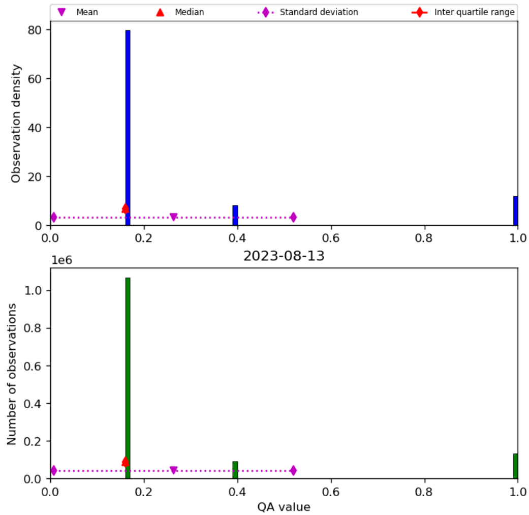
Figure 22: Histogram of “QA value” for 2023-08-12 to 2023-08-14
