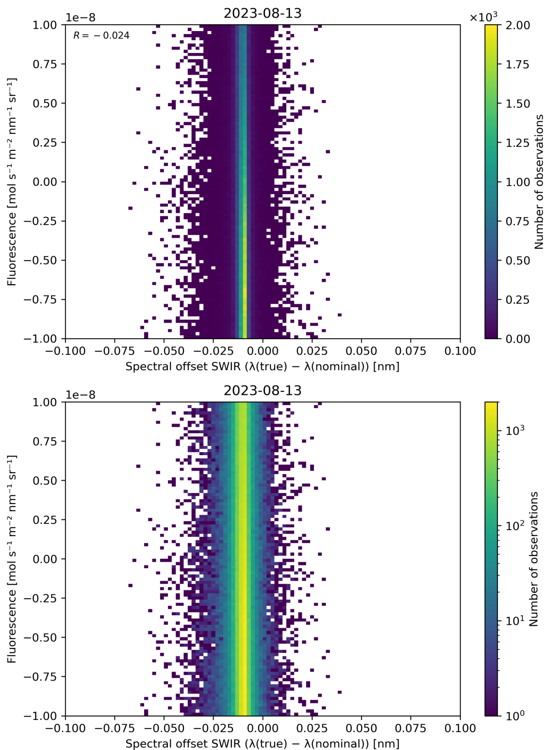
Figure 120: Scatter density plot of “Spectral offset SWIR ( \lambda(\text{true}) - \lambda(\text{nominal}) )” against “Fluorescence” for 2023-08-12 to 2023-08-14.
