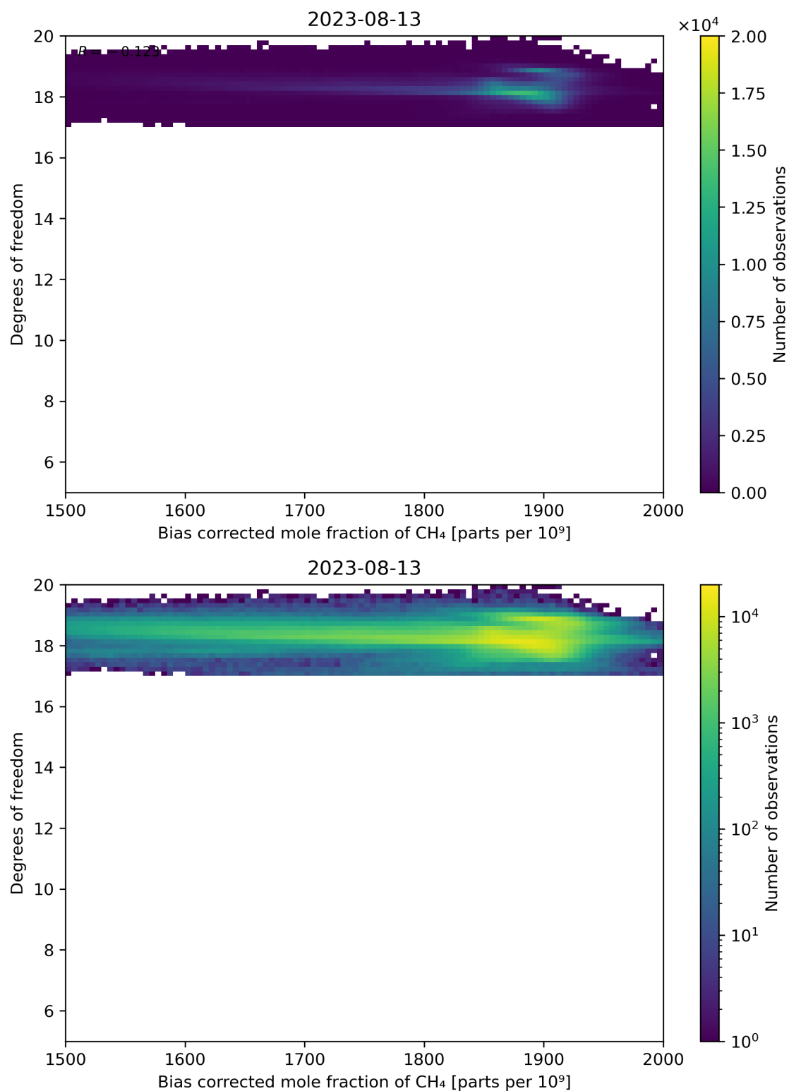
Figure 65: Scatter density plot of “Bias corrected mole fraction of CH 4 ” against “Degrees of freedom” for 2023-08-12 to 2023-08-14.
