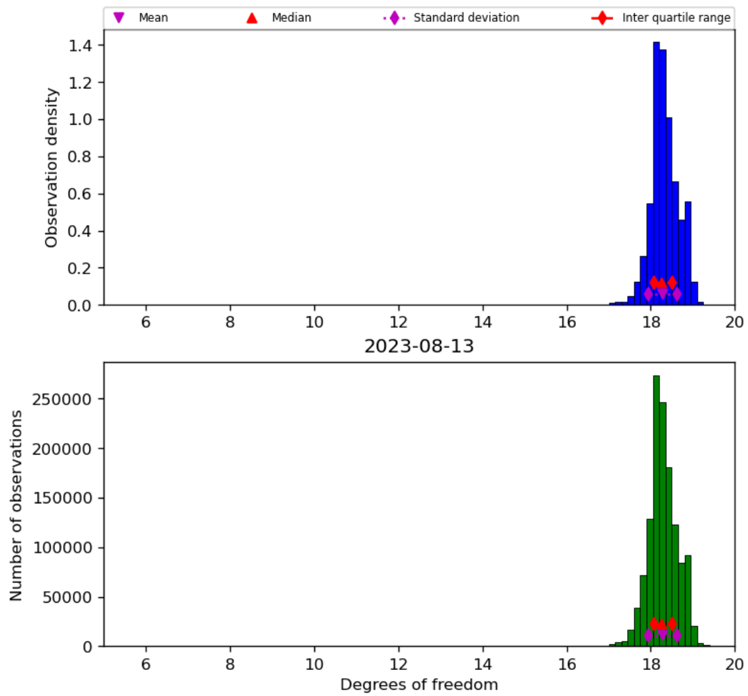
Figure 30: Histogram of “Degrees of freedom” for 2023-08-12 to 2023-08-14
