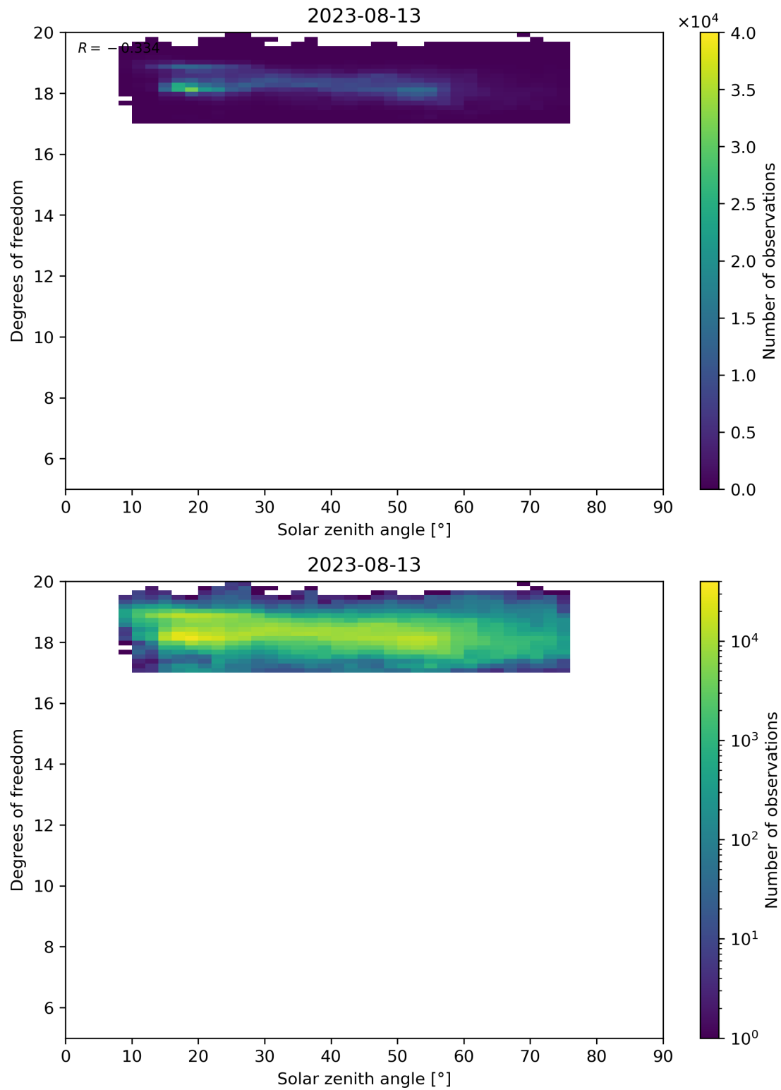
Figure 96: Scatter density plot of “Solar zenith angle” against “Degrees of freedom” for 2023-08-12 to 2023-08-14.
