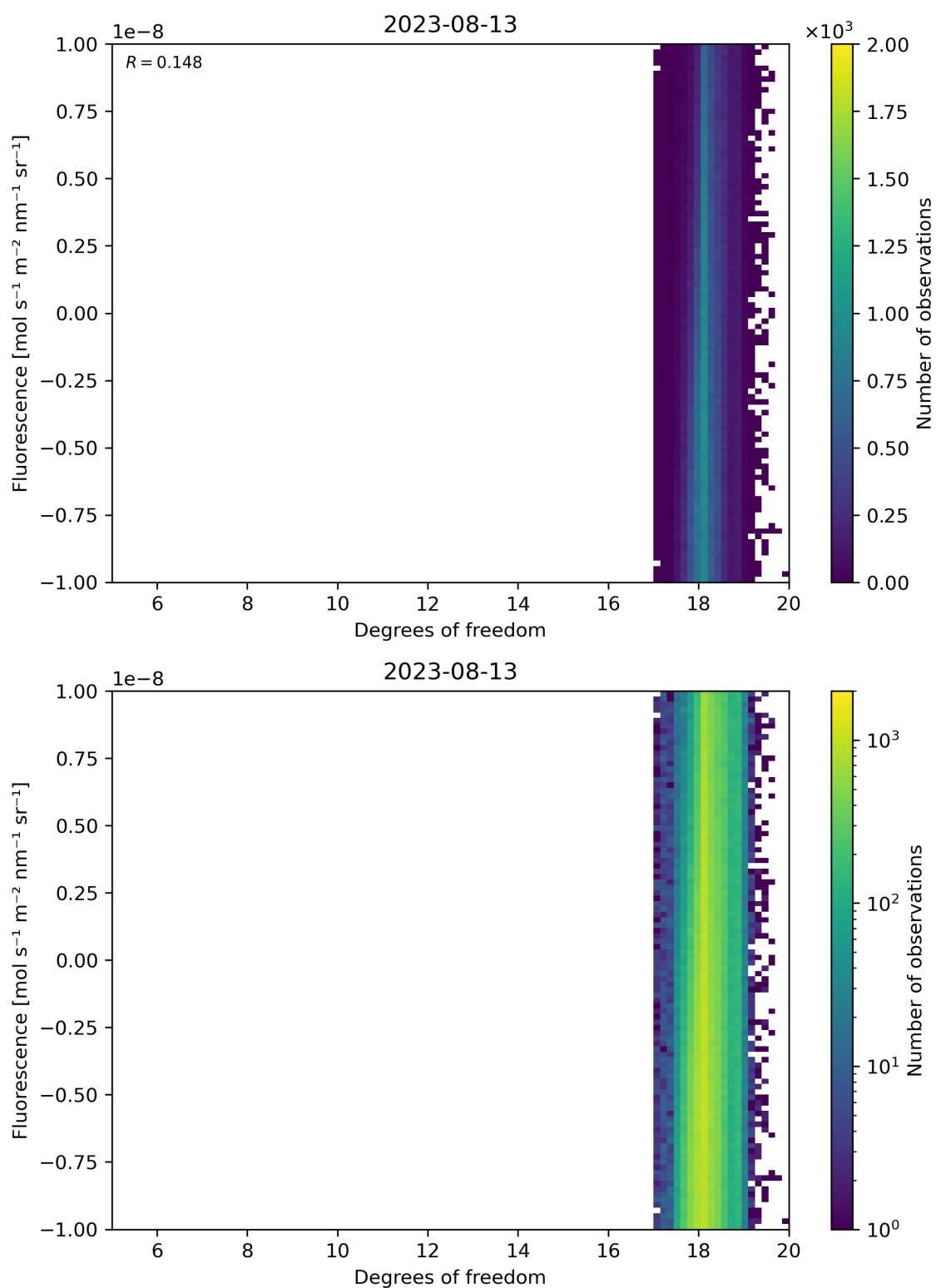
Figure 51: Scatter density plot of “Degrees of freedom” against “Fluorescence” for 2023-08-12 to 2023-08-14.
