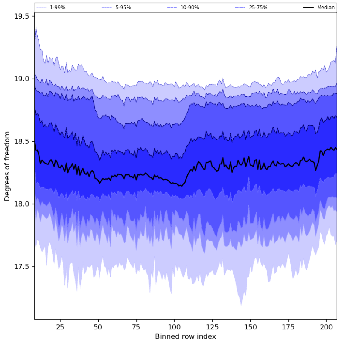
Figure 41: Along track statistics of “Degrees of freedom” for 2023-08-12 to 2023-08-14
