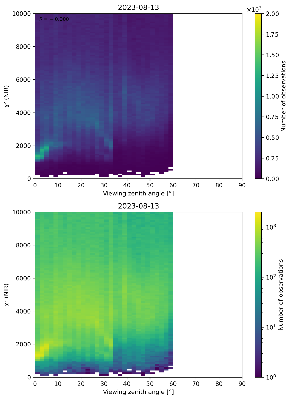
Figure 105: Scatter density plot of “Viewing zenith angle” against “ \chi^2 (NIR)” for 2023-08-12 to 2023-08-14.
