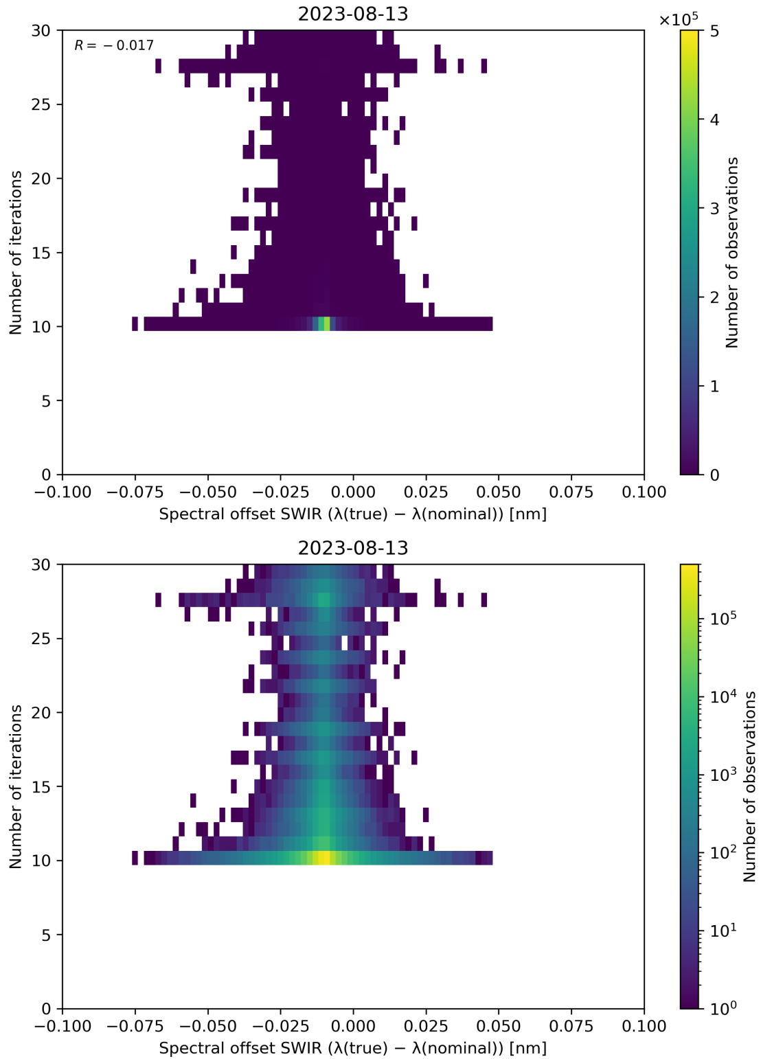
Figure 121: Scatter density plot of “Spectral offset SWIR ( \lambda(\text{true}) - \lambda(\text{nominal}) )” against “Number of iterations” for 2023-08-12 to 2023-08-14.
