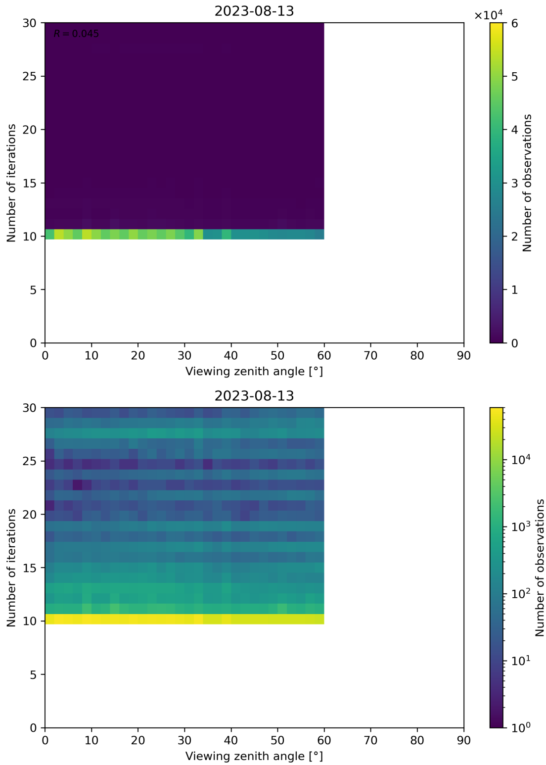
Figure 113: Scatter density plot of “Viewing zenith angle” against “Number of iterations” for 2023-08-12 to 2023-08-14.
