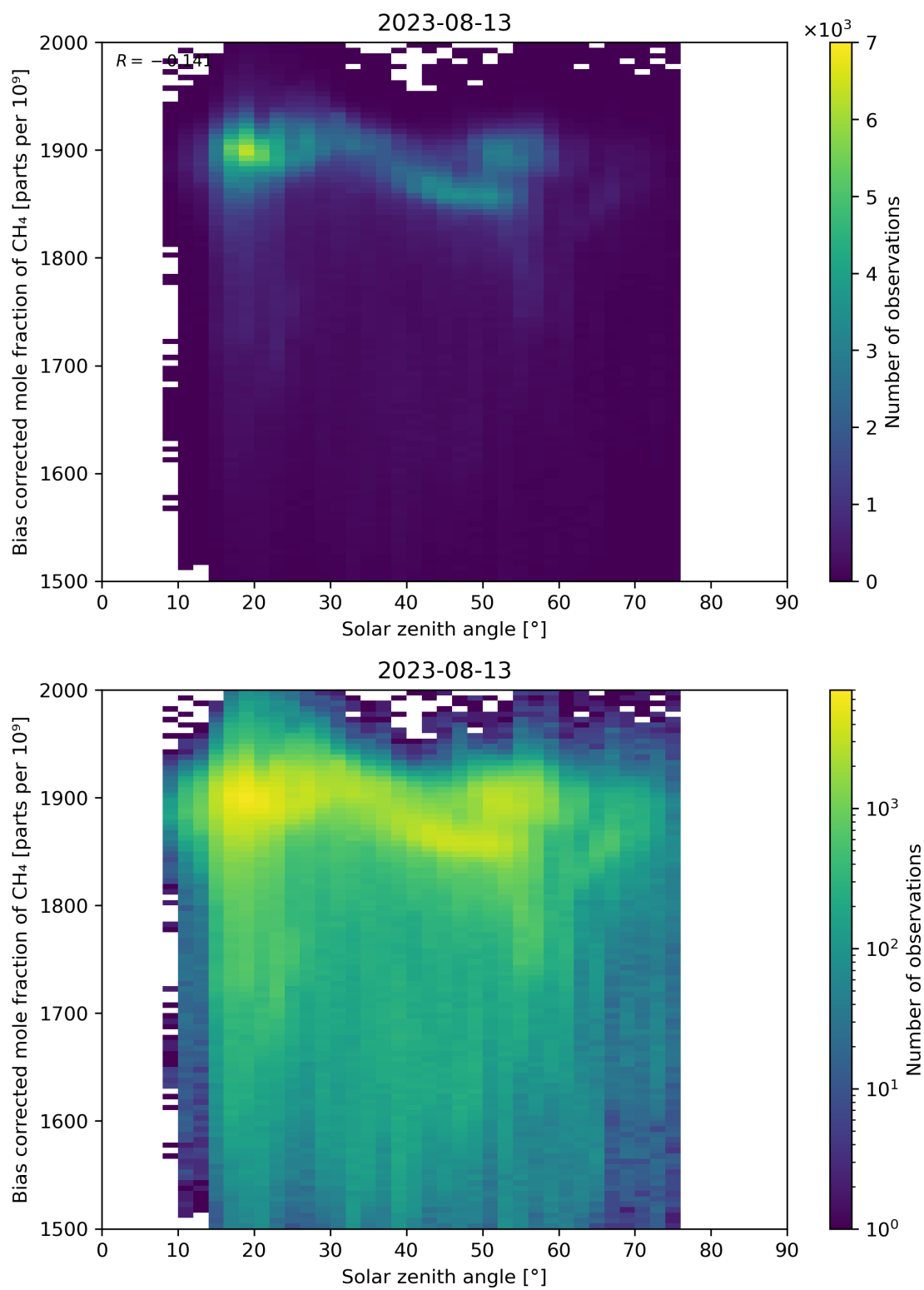
Figure 100: Scatter density plot of “Solar zenith angle” against “Bias corrected mole fraction of CH 4 ” for 2023-08-12 to 2023-08-14.
