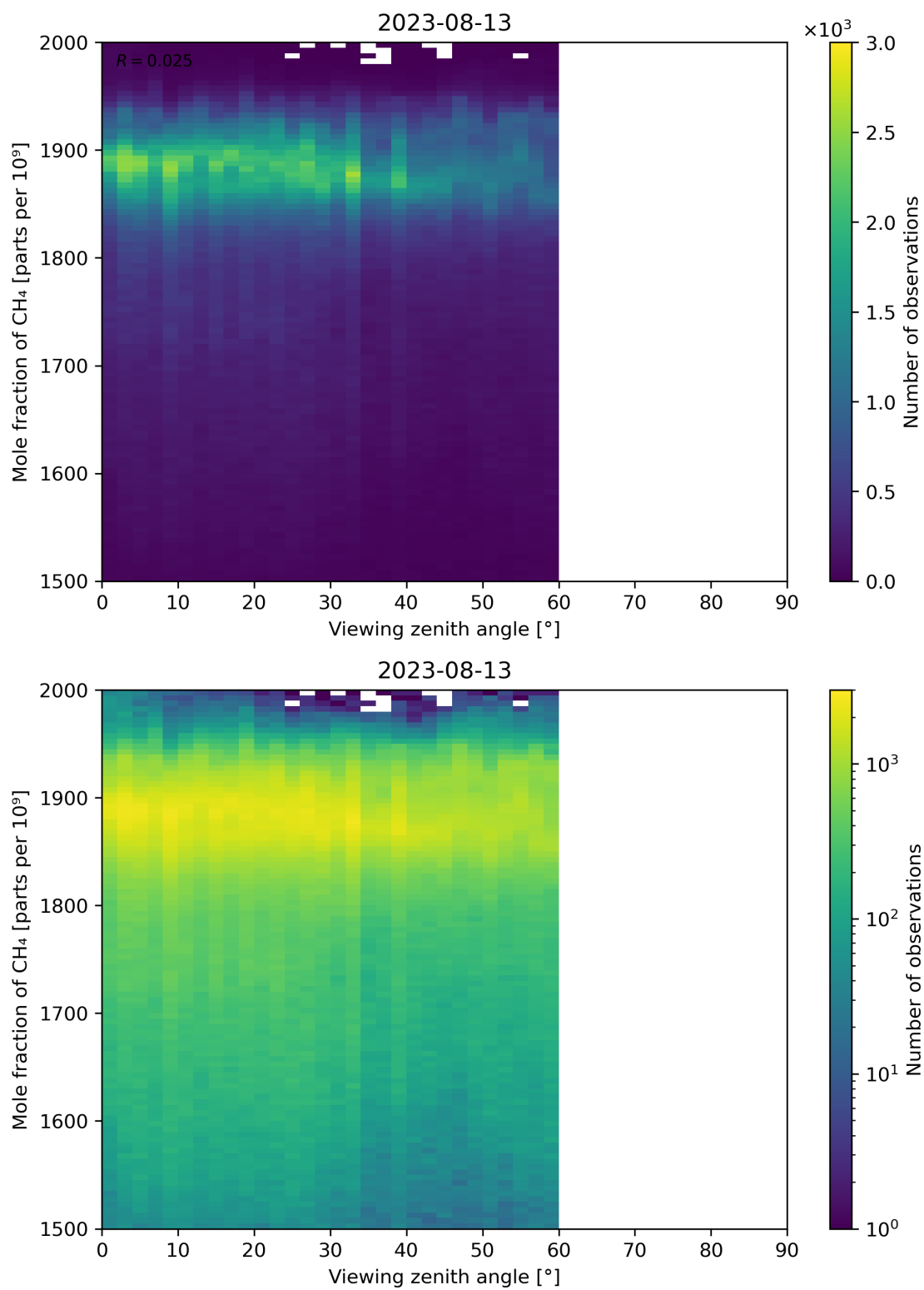
Figure 110: Scatter density plot of “Viewing zenith angle” against “Mole fraction of CH 4 ” for 2023-08-12 to 2023-08-14.
