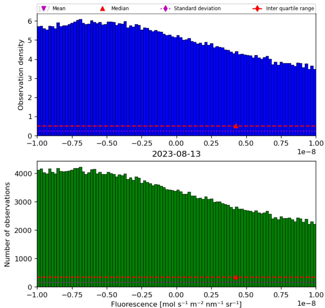
Figure 32: Histogram of “Fluorescence” for 2023-08-12 to 2023-08-14
