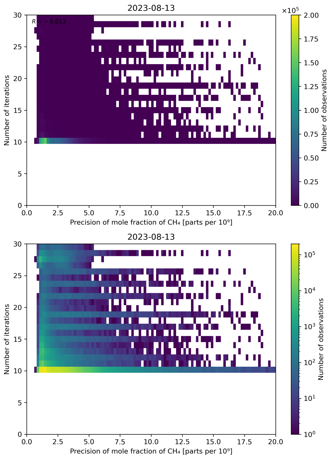
Figure 83: Scatter density plot of “Precision of mole fraction of CH 4 ” against “Number of iterations” for 2023-08-12 to 2023-08-14.
