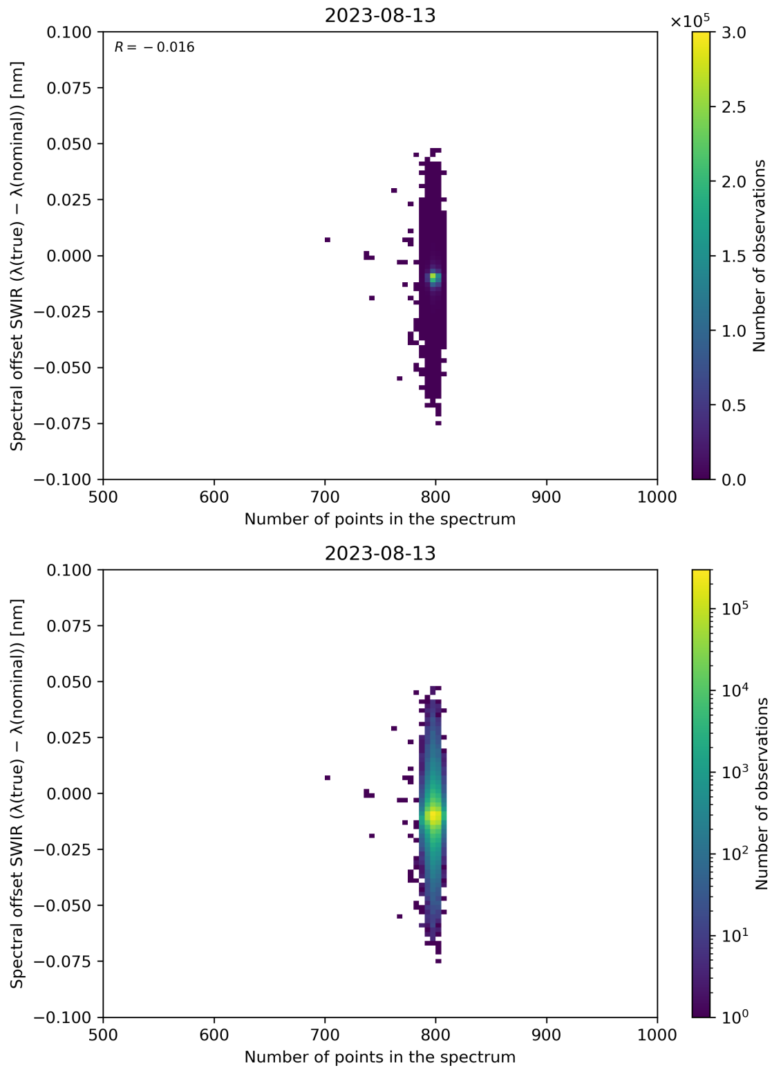
Figure 93: Scatter density plot of “Number of points in the spectrum” against “Spectral offset SWIR ( \lambda(\text{true}) - \lambda(\text{nominal}) )” for 2023-08-12 to 2023-08-14.
