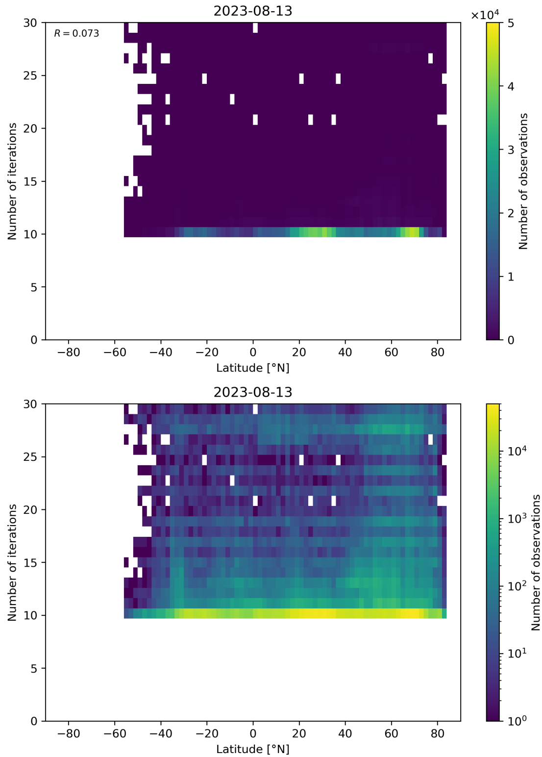
Figure 60: Scatter density plot of “Latitude” against “Number of iterations” for 2023-08-12 to 2023-08-14.
