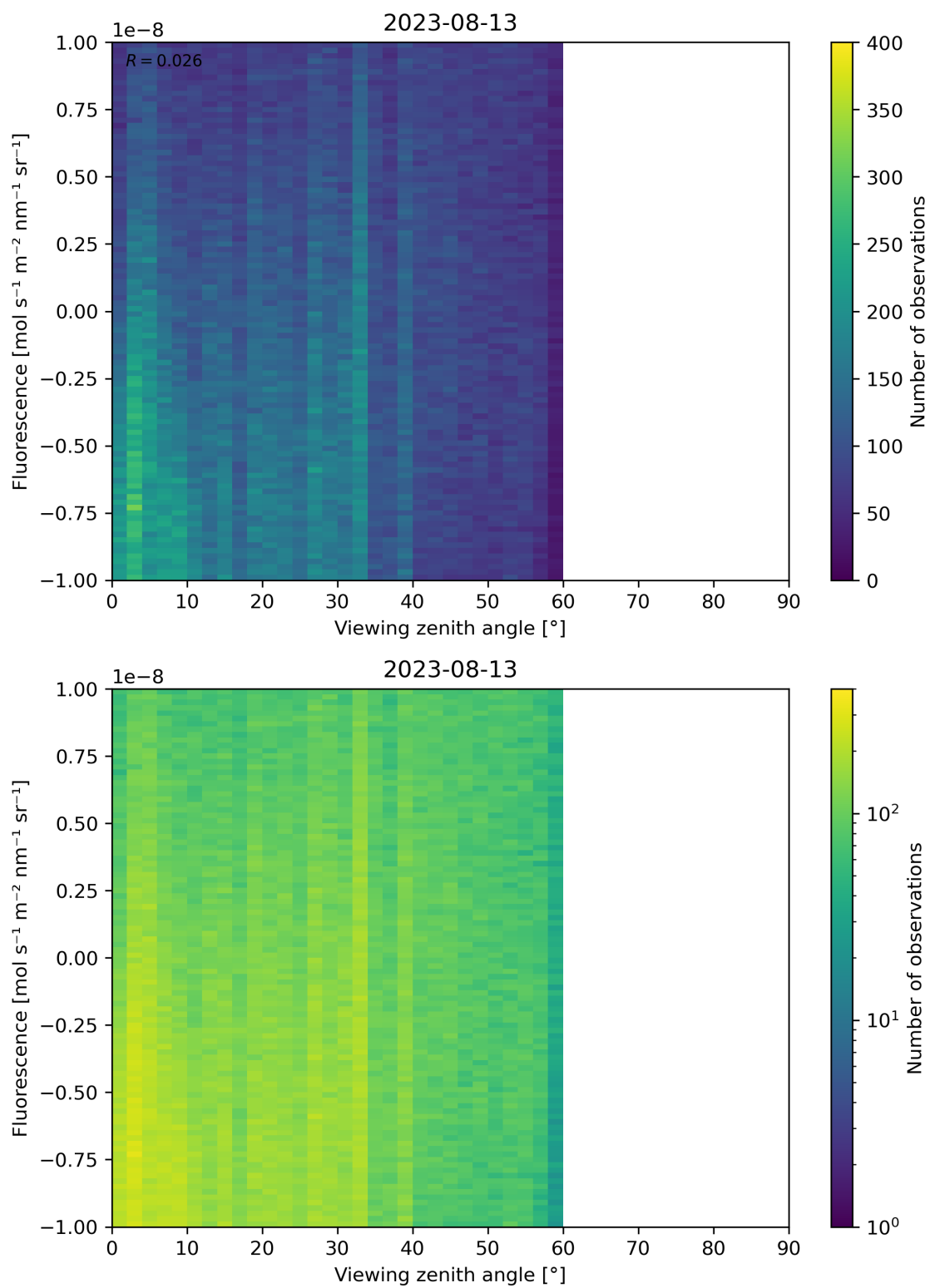
Figure 108: Scatter density plot of “Viewing zenith angle” against “Fluorescence” for 2023-08-12 to 2023-08-14.
