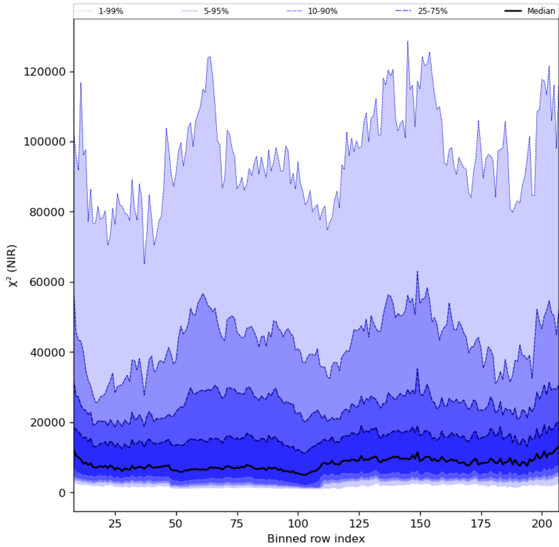
Figure 40: Along track statistics of “ \chi^2 (NIR)” for 2023-08-12 to 2023-08-14
