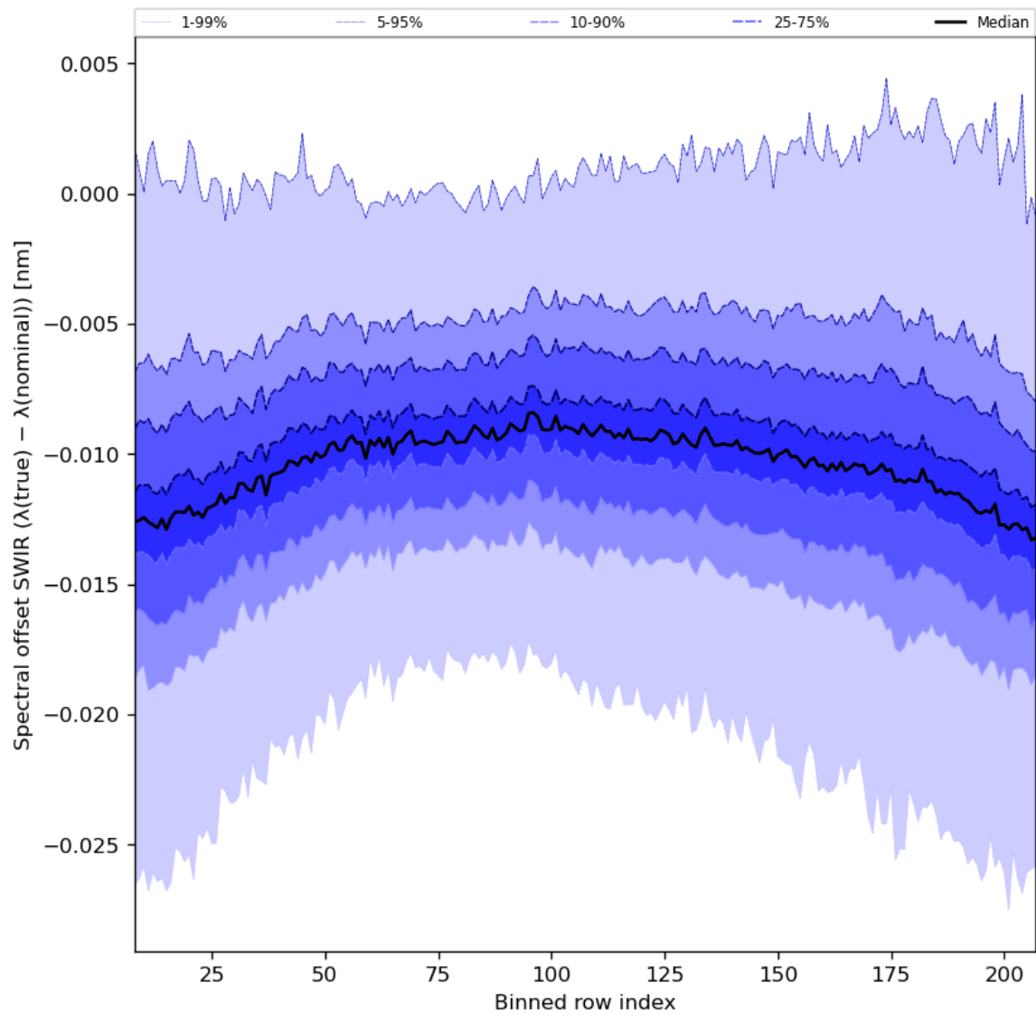
Figure 38: Along track statistics of “Spectral offset SWIR ( \lambda(\text{true}) - \lambda(\text{nominal}) )” for 2023-08-14 to 2023-08-15
