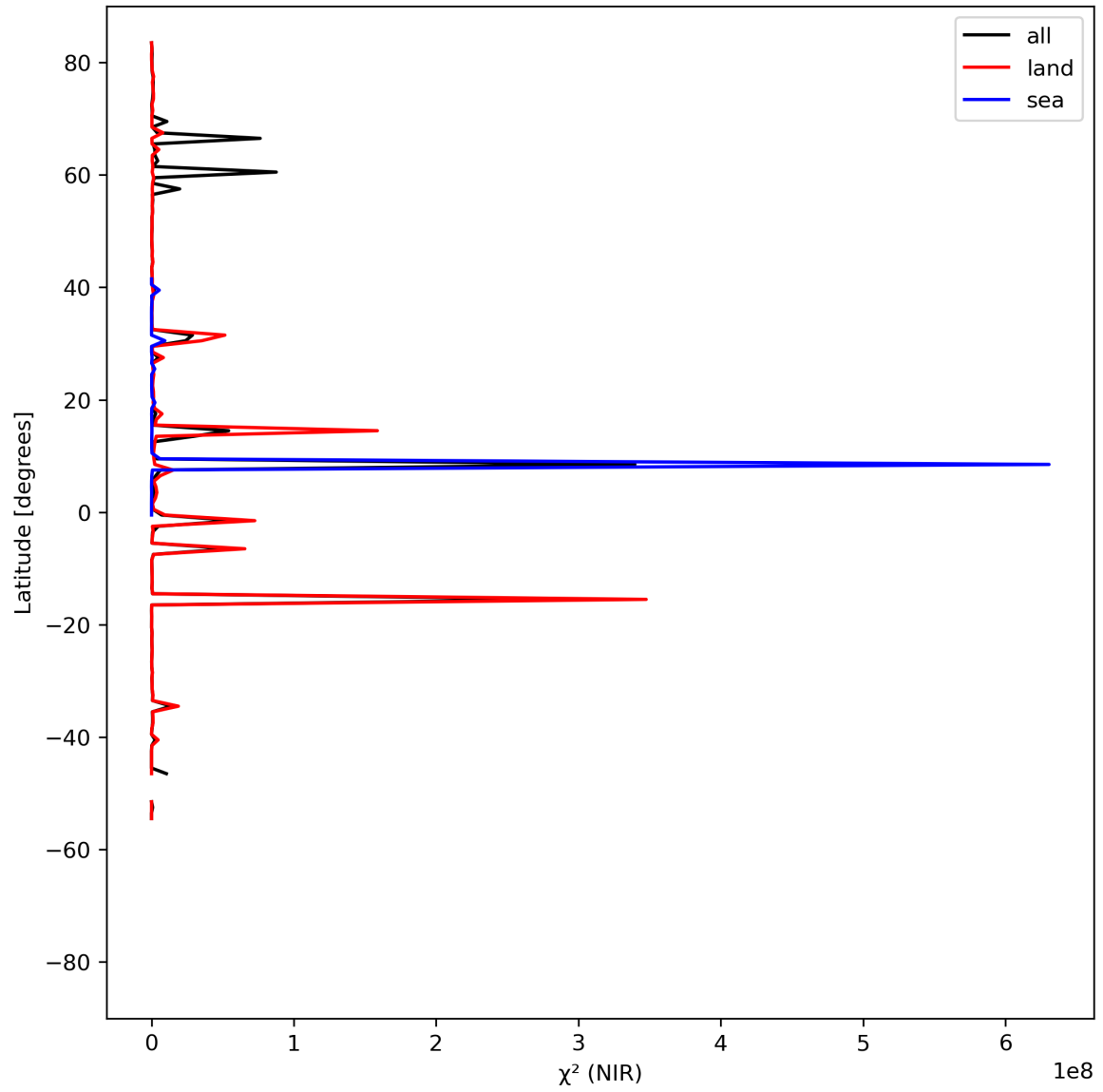
Figure 18: Zonal average of “ \chi^2 (NIR)” for 2023-08-14 to 2023-08-15.
