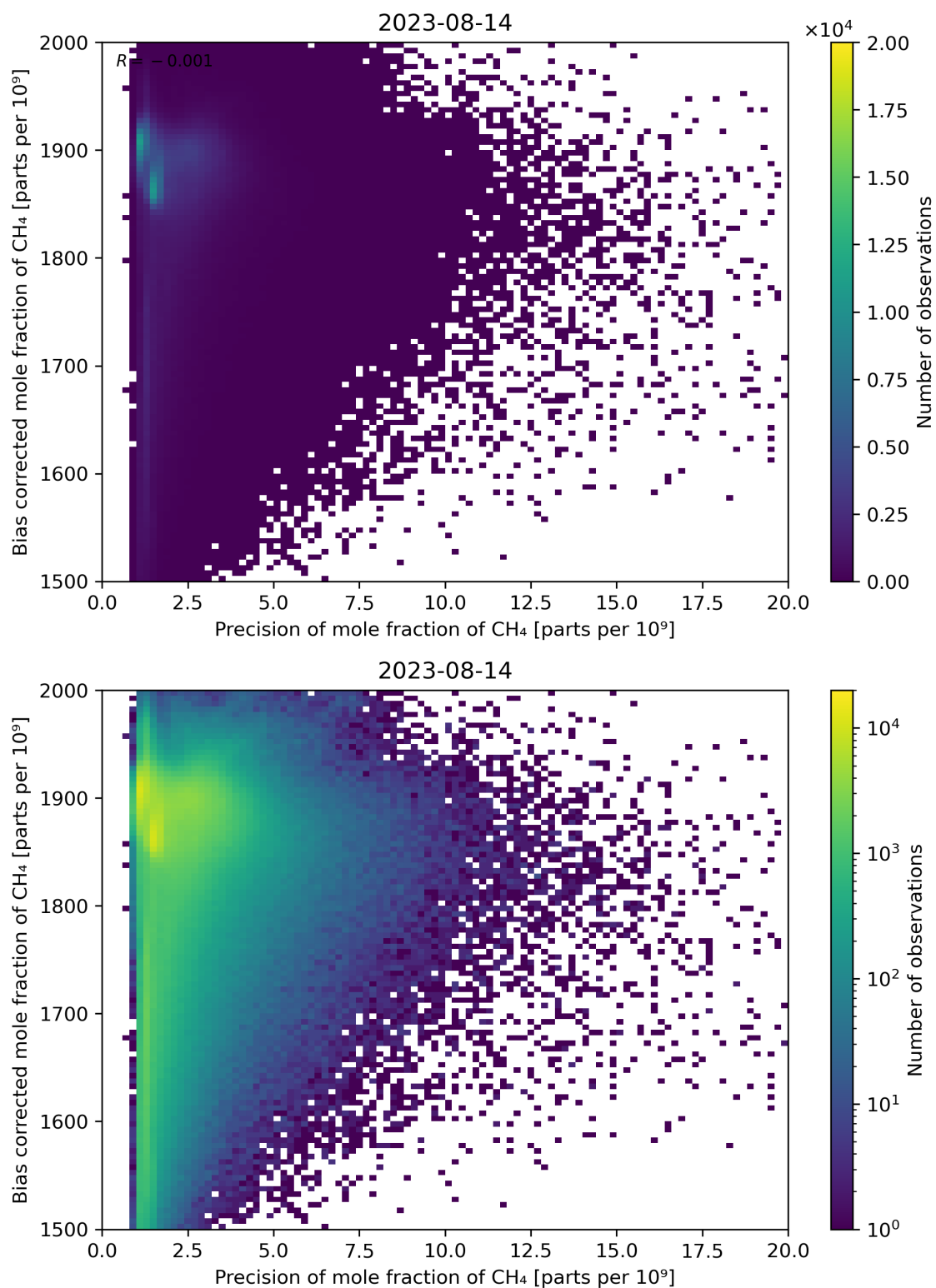
Figure 82: Scatter density plot of “Precision of mole fraction of CH 4 ” against “Bias corrected mole fraction of CH 4 ” for 2023-08-14 to 2023-08-15.
