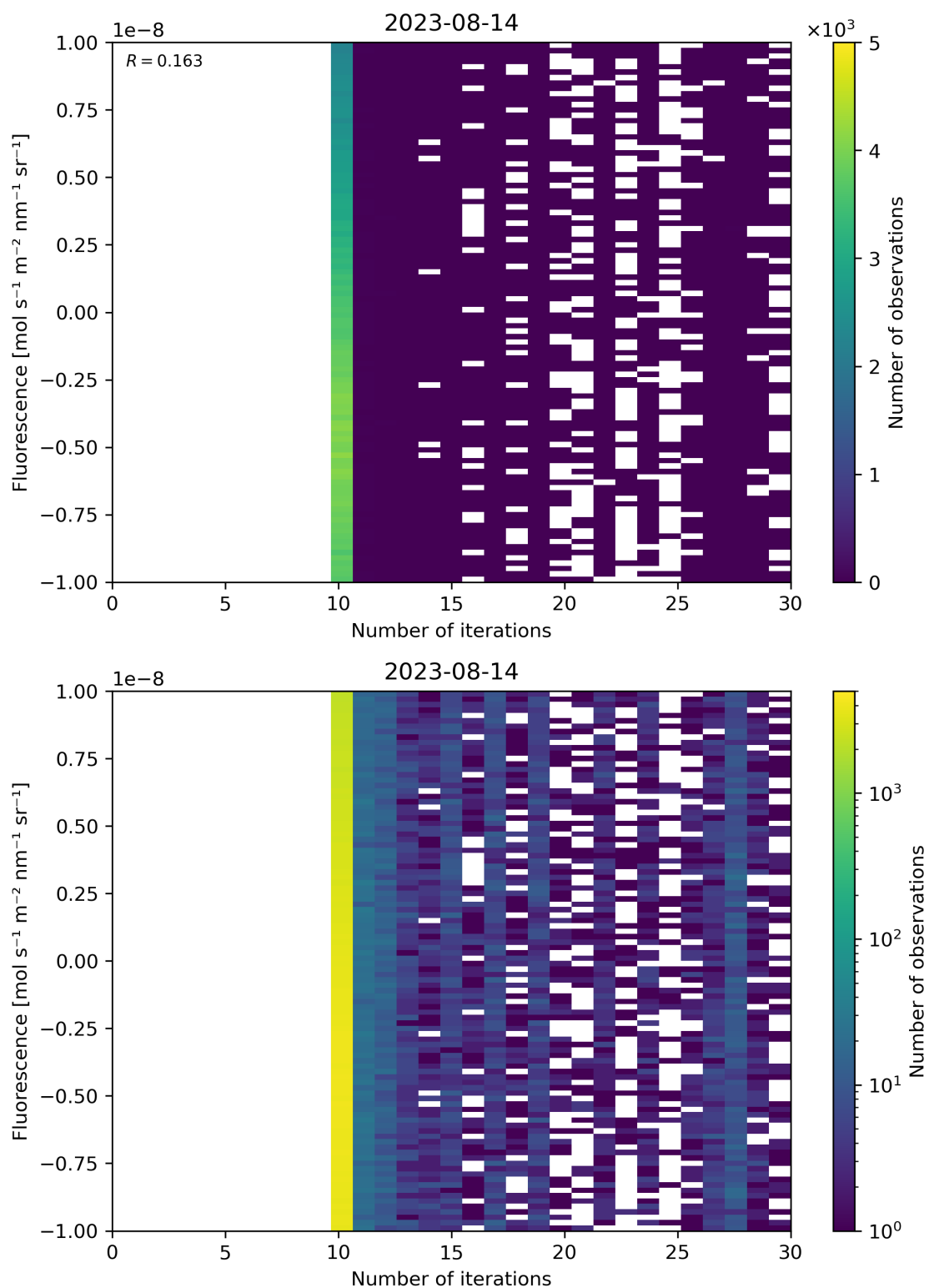
Figure 87: Scatter density plot of “Number of iterations” against “Fluorescence” for 2023-08-14 to 2023-08-15.
