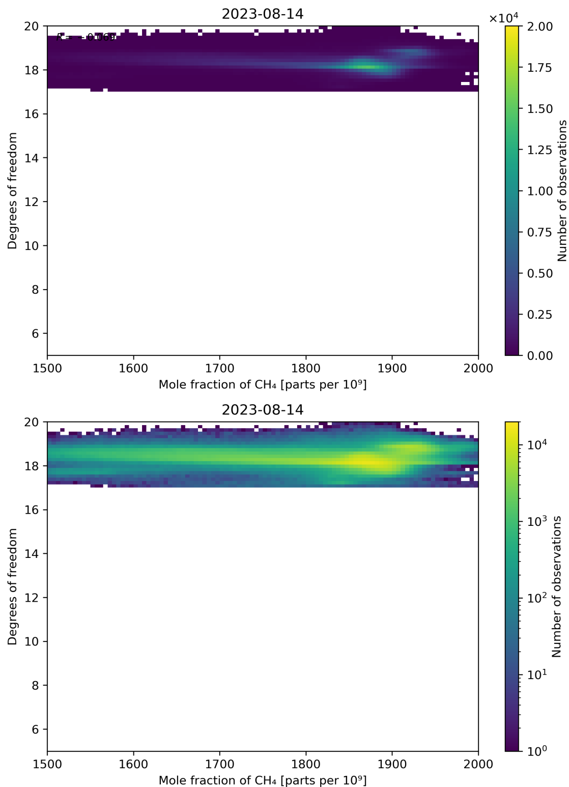
Figure 72: Scatter density plot of “Mole fraction of CH 4 ” against “Degrees of freedom” for 2023-08-14 to 2023-08-15.
