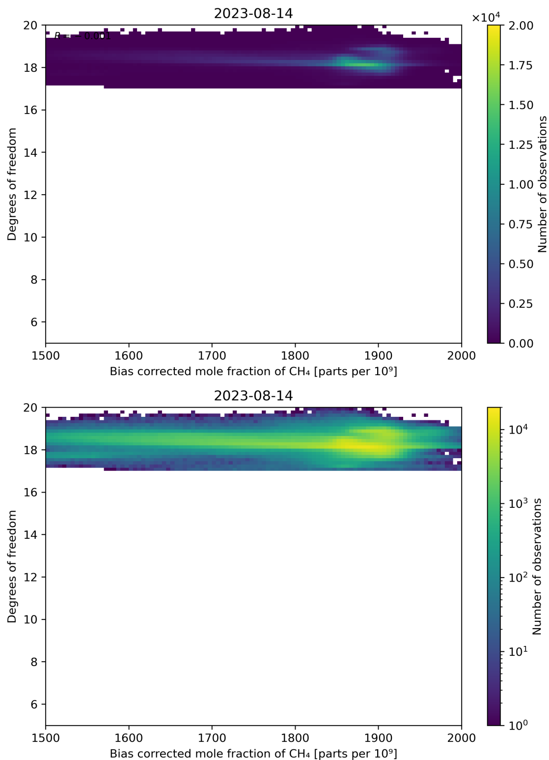
Figure 65: Scatter density plot of “Bias corrected mole fraction of CH 4 ” against “Degrees of freedom” for 2023-08-14 to 2023-08-15.
