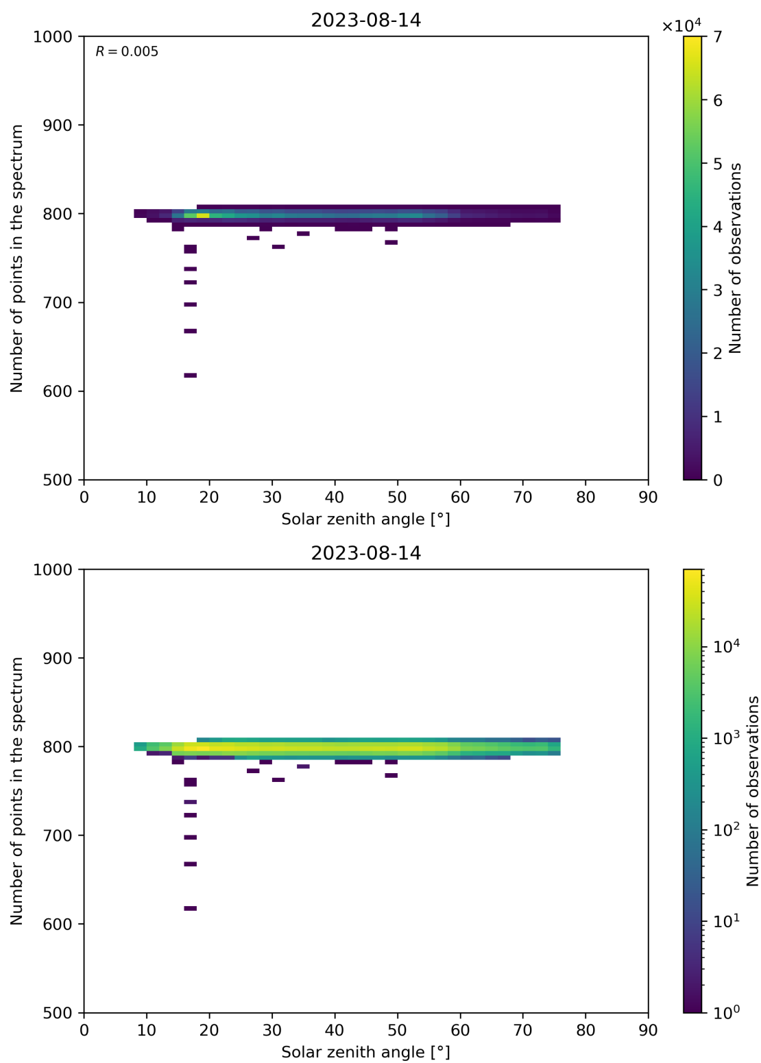
Figure 103: Scatter density plot of “Solar zenith angle” against “Number of points in the spectrum” for 2023-08-14 to 2023-08-15.
