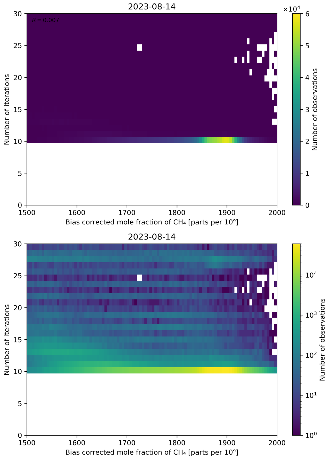
Figure 67: Scatter density plot of “Bias corrected mole fraction of CH 4 ” against “Number of iterations” for 2023-08-14 to 2023-08-15.
