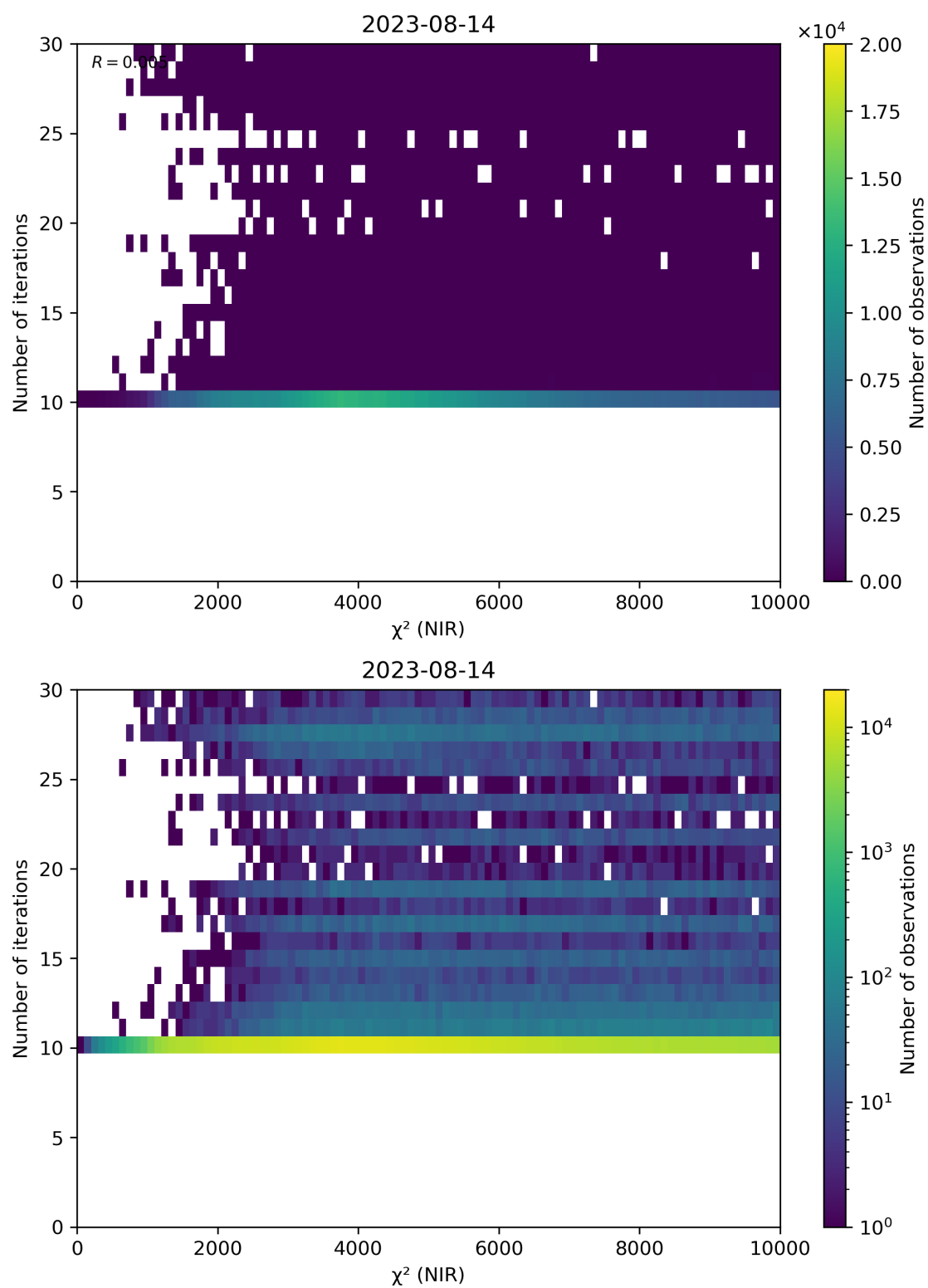
Figure 46: Scatter density plot of “ \chi^2 (NIR)” against “Number of iterations” for 2023-08-14 to 2023-08-15.
