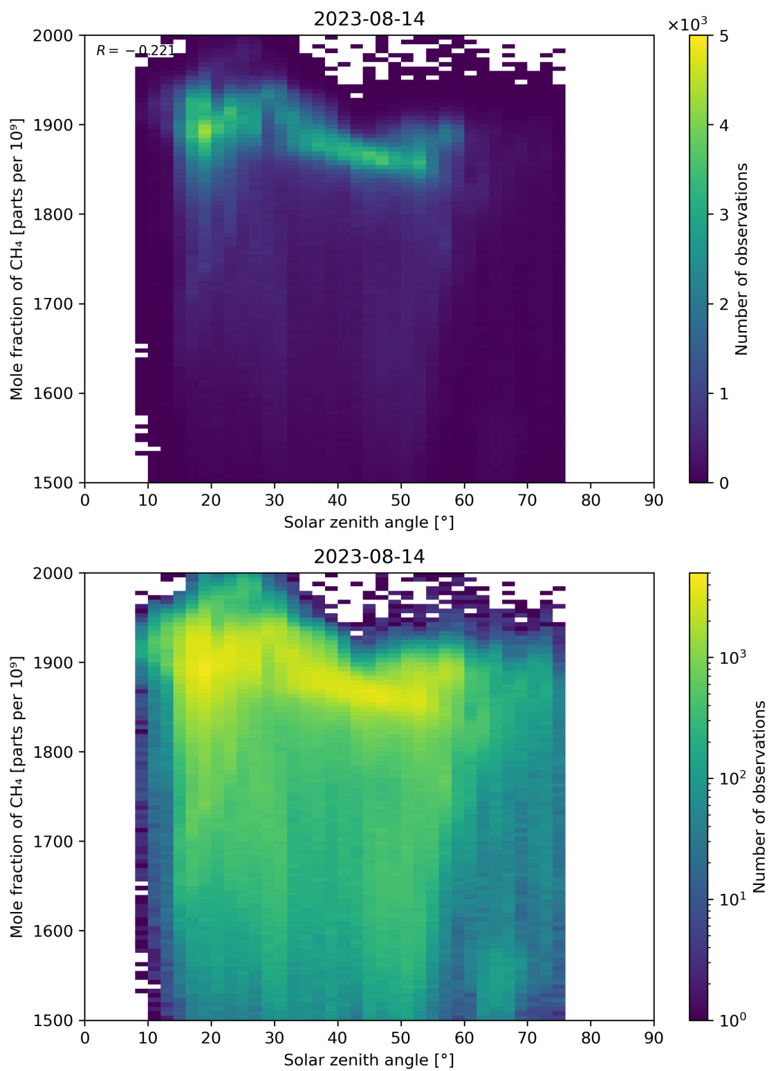
Figure 99: Scatter density plot of “Solar zenith angle” against “Mole fraction of CH 4 ” for 2023-08-14 to 2023-08-15.
