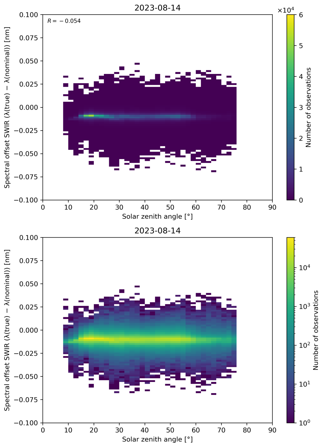
Figure 104: Scatter density plot of “Solar zenith angle” against “Spectral offset SWIR ( \lambda(\text{true}) - \lambda(\text{nominal}) )” for 2023-08-14 to 2023-08-15.
