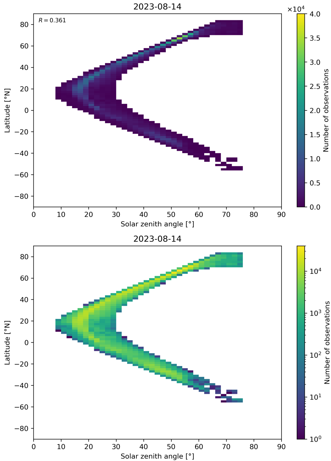
Figure 98: Scatter density plot of “Solar zenith angle” against “Latitude” for 2023-08-14 to 2023-08-15.
