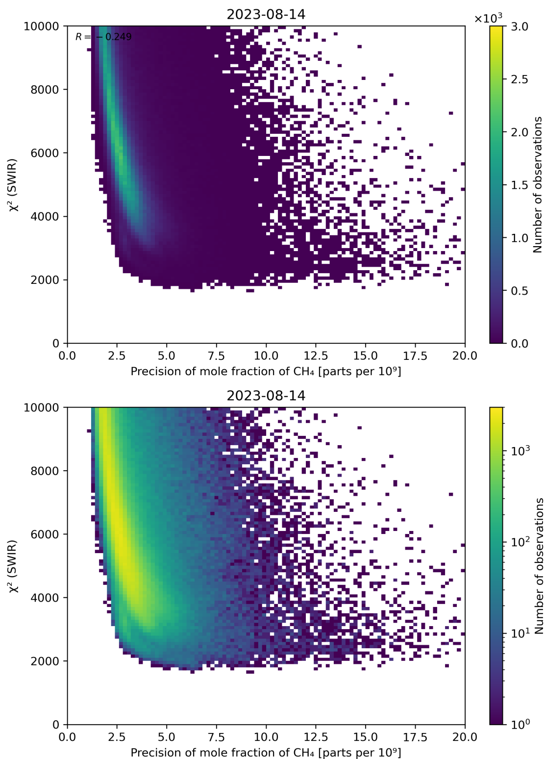
Figure 79: Scatter density plot of “Precision of mole fraction of \text{CH}_4 ” against “ \chi^2 (SWIR)” for 2023-08-14 to 2023-08-15.
