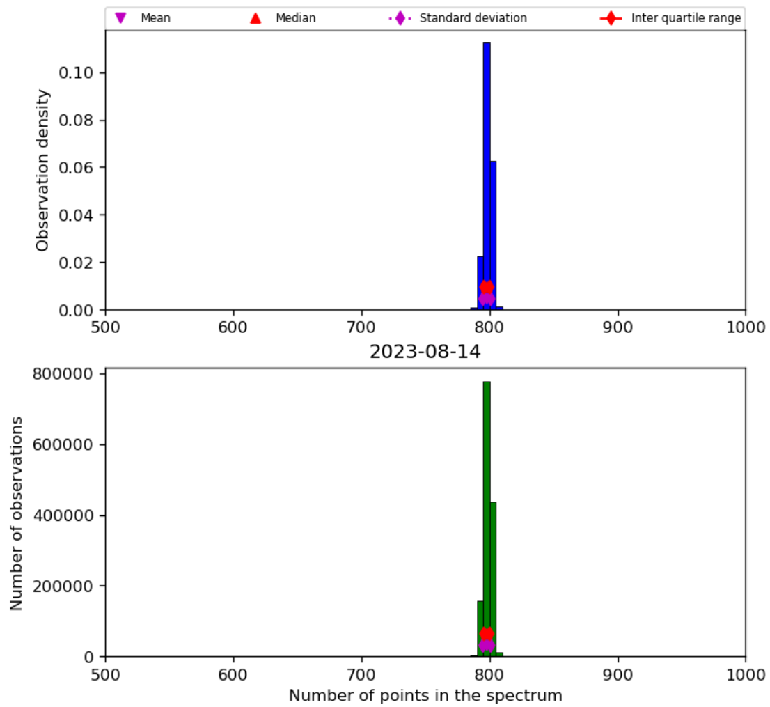
Figure 26: Histogram of “Number of points in the spectrum” for 2023-08-14 to 2023-08-15
