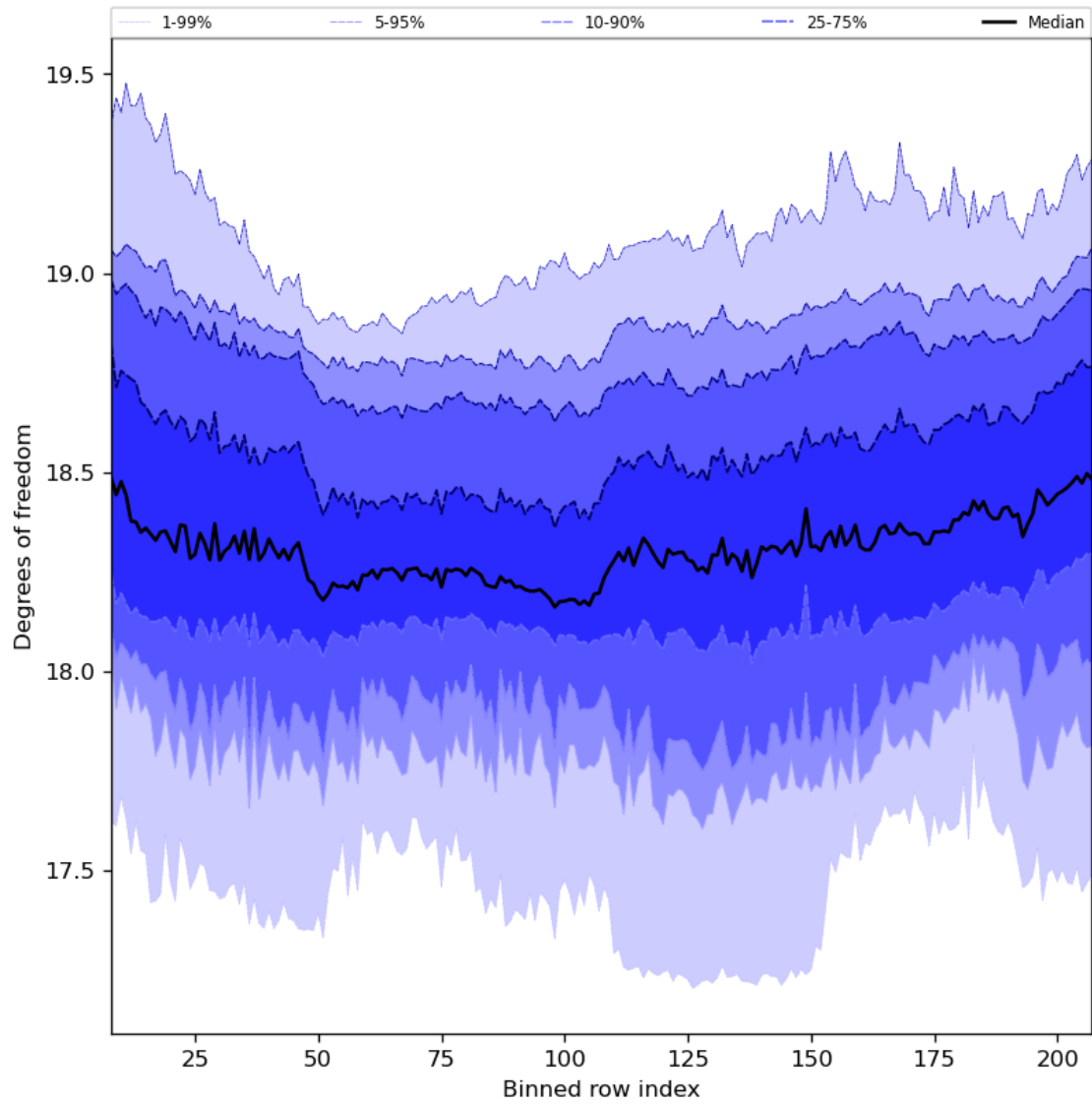
Figure 41: Along track statistics of “Degrees of freedom” for 2023-08-14 to 2023-08-15
