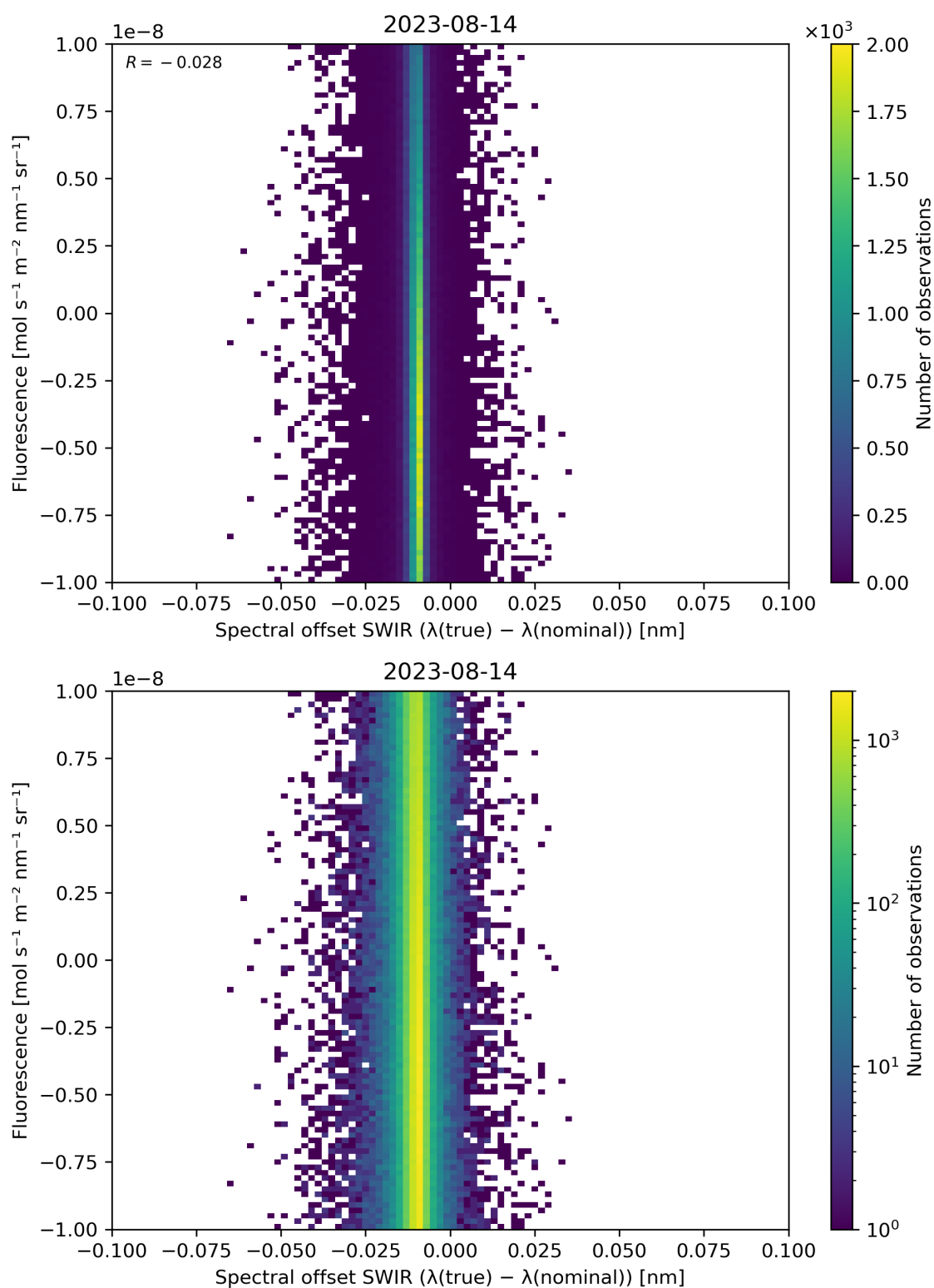
Figure 120: Scatter density plot of “Spectral offset SWIR ( \lambda(\text{true}) - \lambda(\text{nominal}) )” against “Fluorescence” for 2023-08-14 to 2023-08-15.
