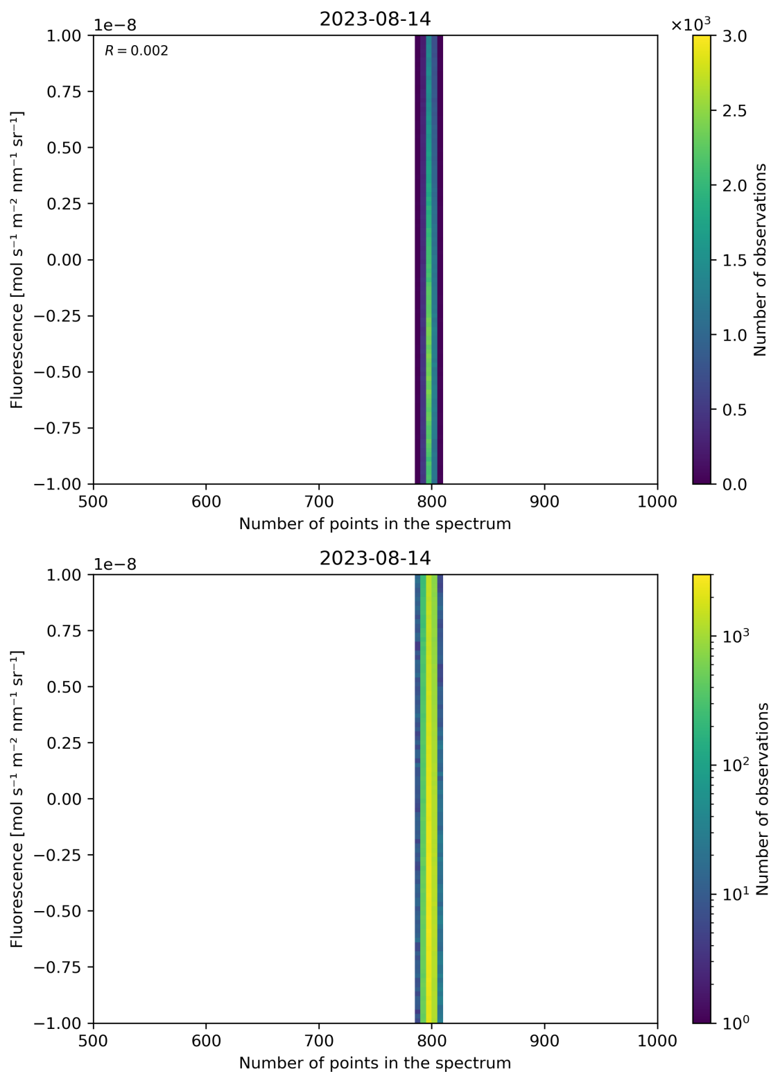
Figure 91: Scatter density plot of “Number of points in the spectrum” against “Fluorescence” for 2023-08-14 to 2023-08-15.
