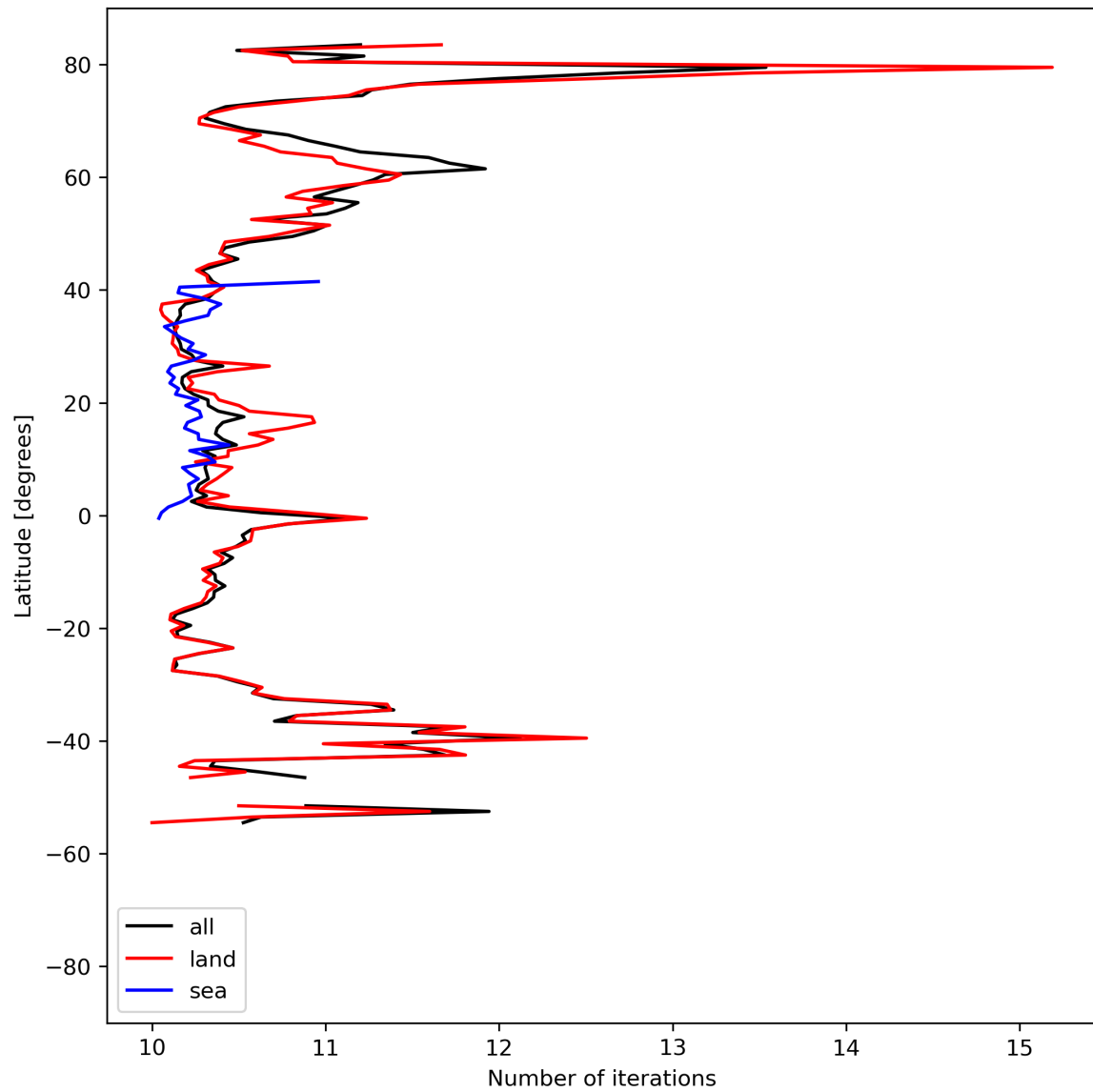
Figure 20: Zonal average of “Number of iterations” for 2023-08-14 to 2023-08-15.
