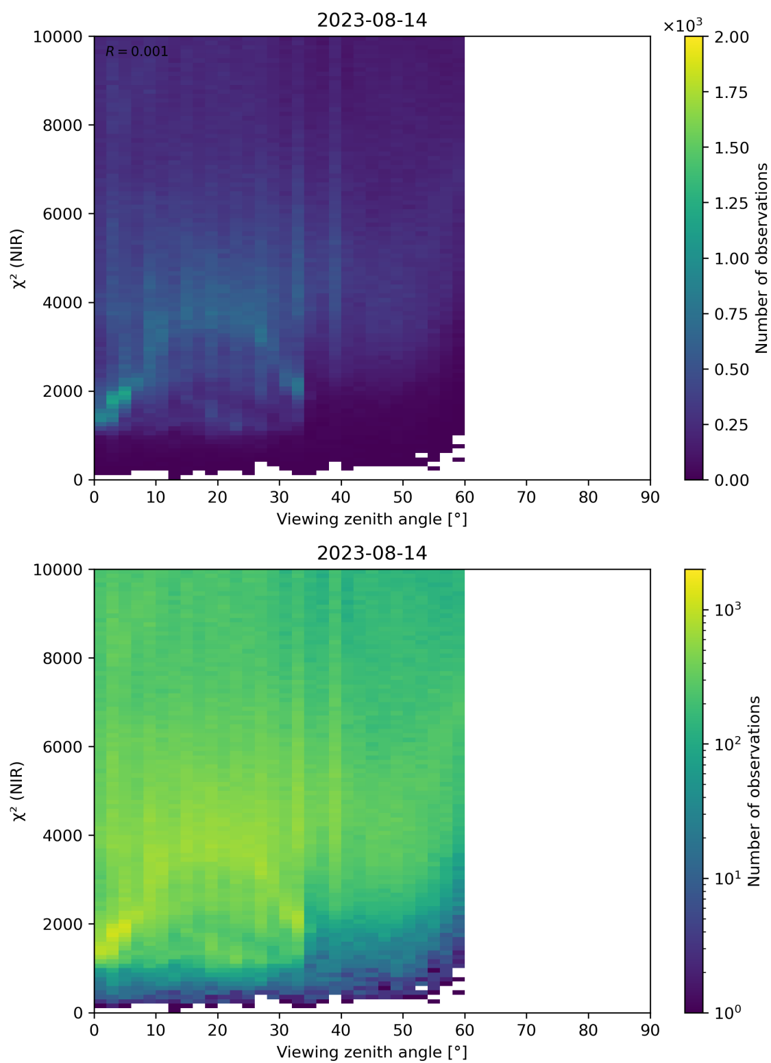
Figure 105: Scatter density plot of “Viewing zenith angle” against “ \chi^2 (NIR)” for 2023-08-14 to 2023-08-15.
