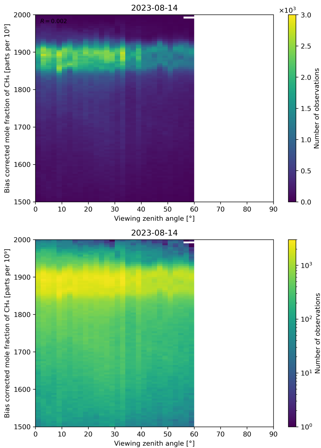
Figure 111: Scatter density plot of “Viewing zenith angle” against “Bias corrected mole fraction of CH 4 ” for 2023-08-14 to 2023-08-15.
