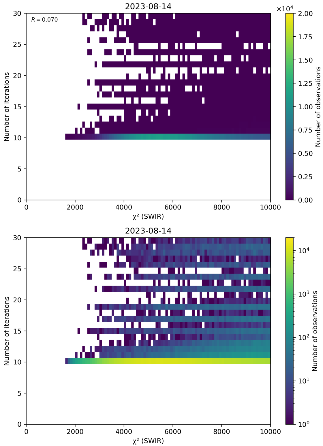
Figure 50: Scatter density plot of “ \chi^2 (SWIR)” against “Number of iterations” for 2023-08-14 to 2023-08-15.
