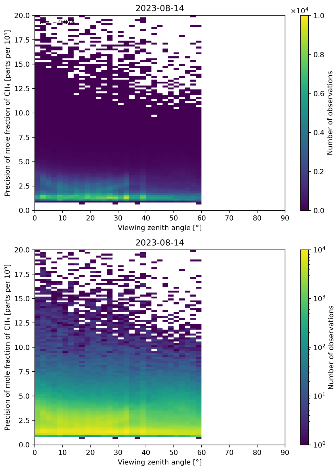
Figure 112: Scatter density plot of “Viewing zenith angle” against “Precision of mole fraction of CH 4 ” for 2023-08-14 to 2023-08-15.
