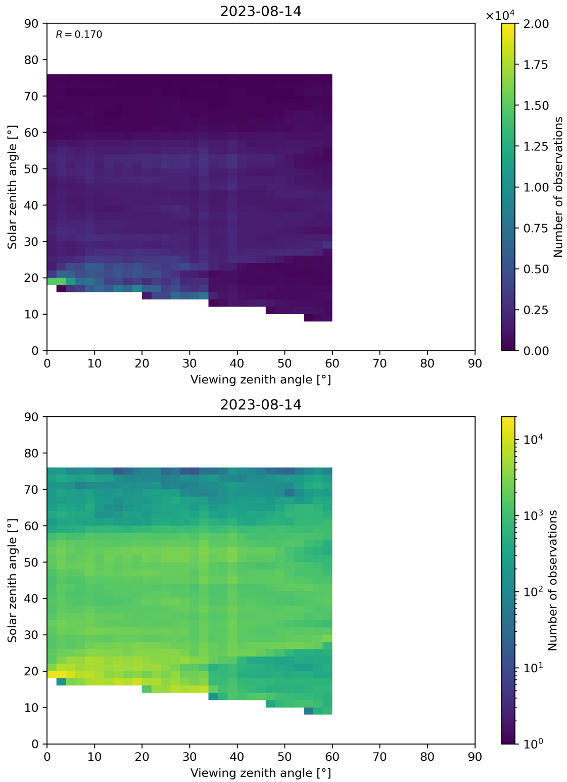
Figure 115: Scatter density plot of “Viewing zenith angle” against “Solar zenith angle” for 2023-08-14 to 2023-08-15.
