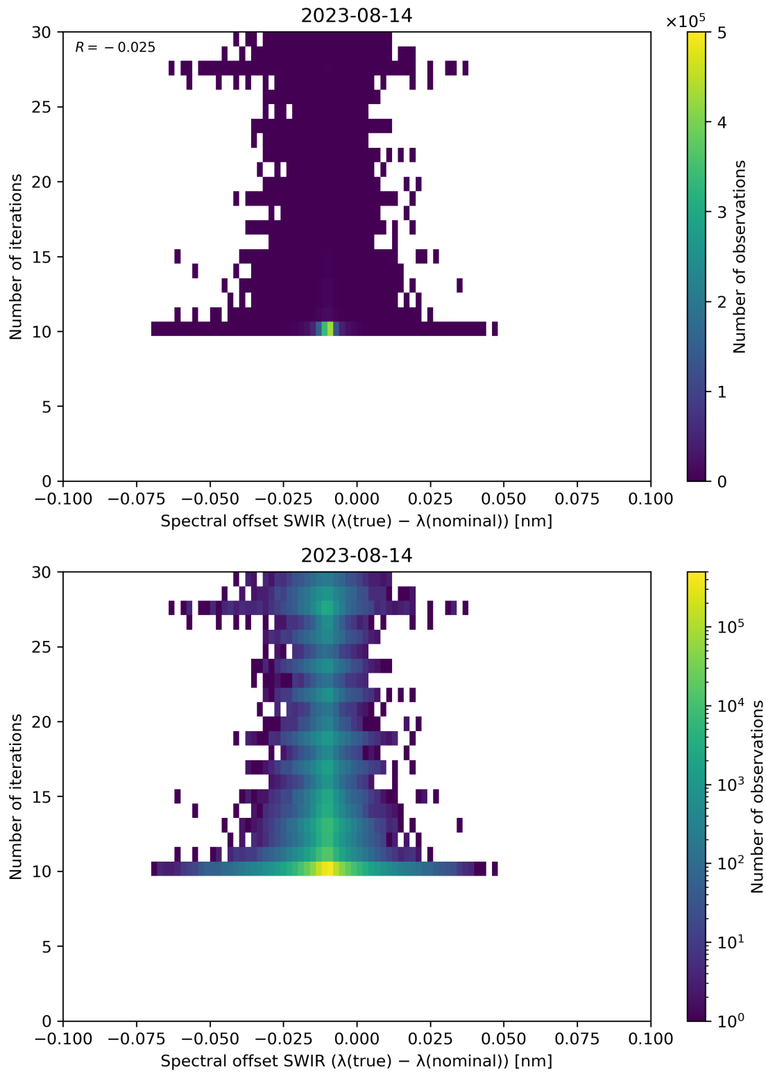
Figure 121: Scatter density plot of “Spectral offset SWIR ( \lambda(\text{true}) - \lambda(\text{nominal}) )” against “Number of iterations” for 2023-08-14 to 2023-08-15.
