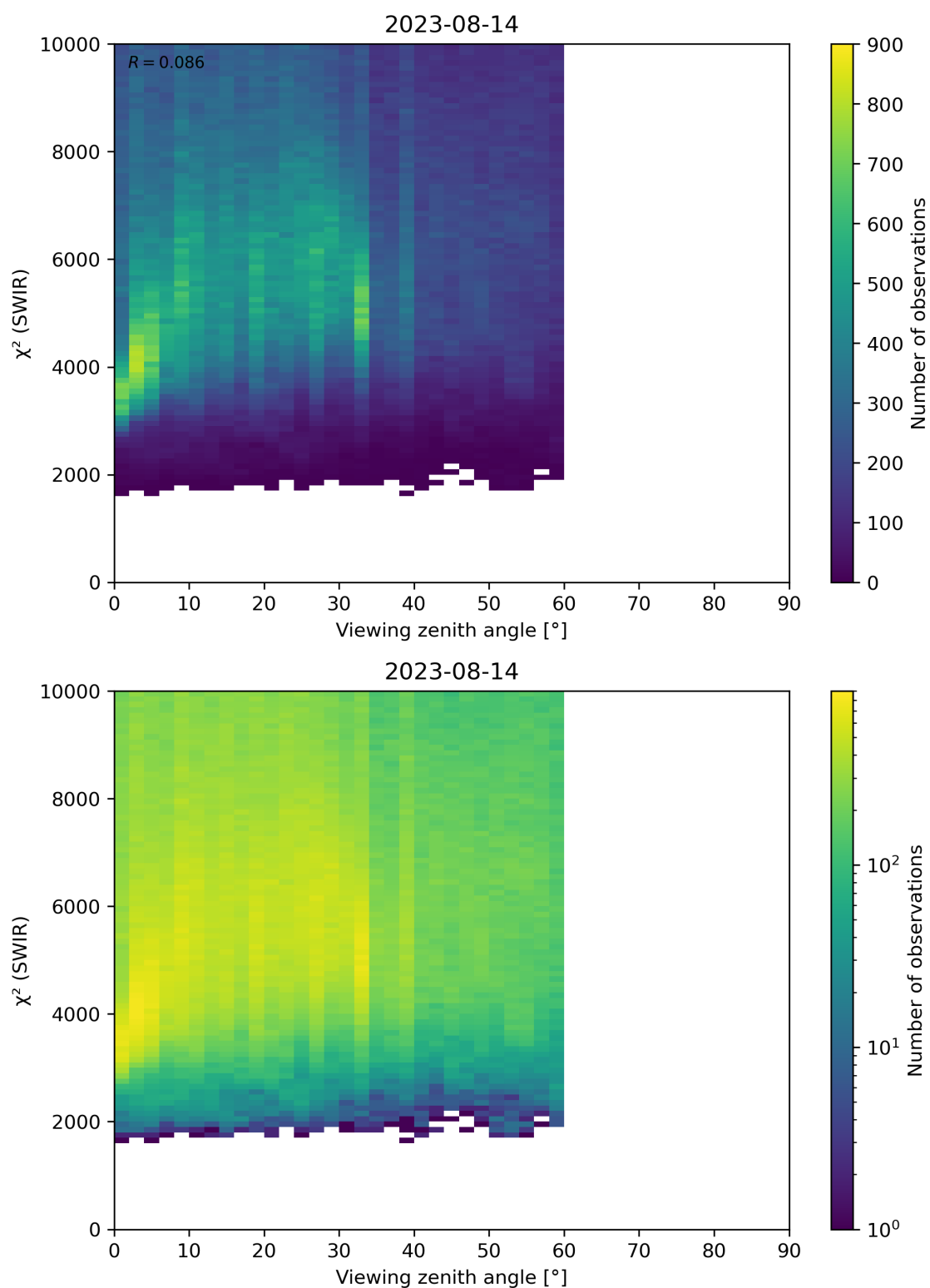
Figure 106: Scatter density plot of “Viewing zenith angle” against “ \chi^2 (SWIR)” for 2023-08-14 to 2023-08-15.
