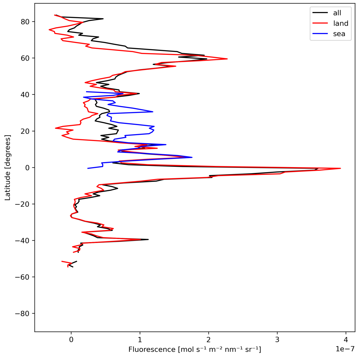
Figure 21: Zonal average of “Fluorescence” for 2023-08-14 to 2023-08-15.
