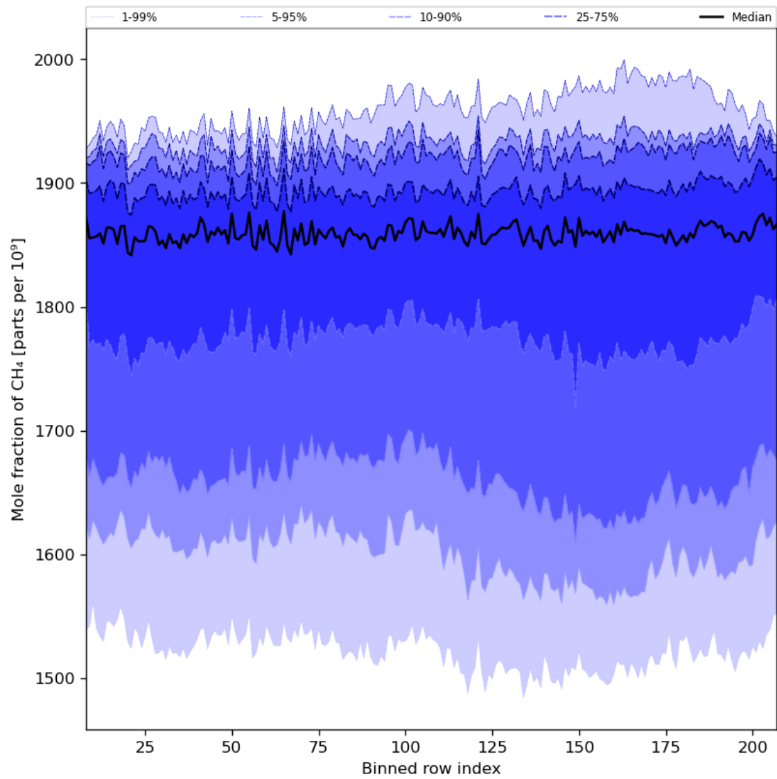
Figure 34: Along track statistics of “Mole fraction of CH 4 ” for 2023-08-14 to 2023-08-15
