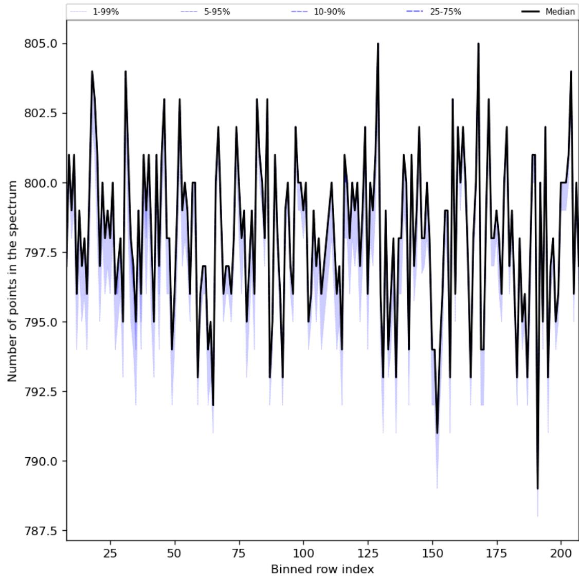
Figure 37: Along track statistics of “Number of points in the spectrum” for 2023-08-14 to 2023-08-15
