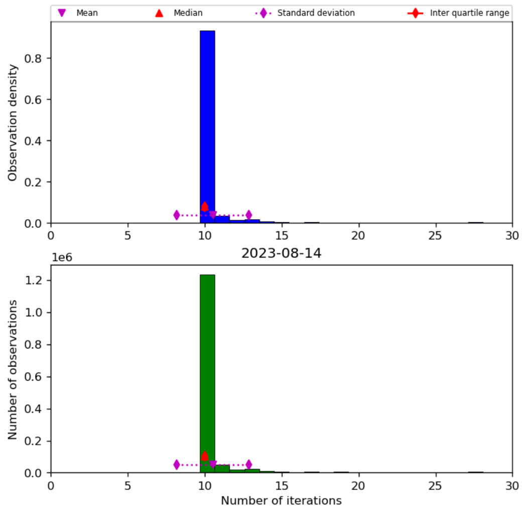
Figure 31: Histogram of “Number of iterations” for 2023-08-14 to 2023-08-15
