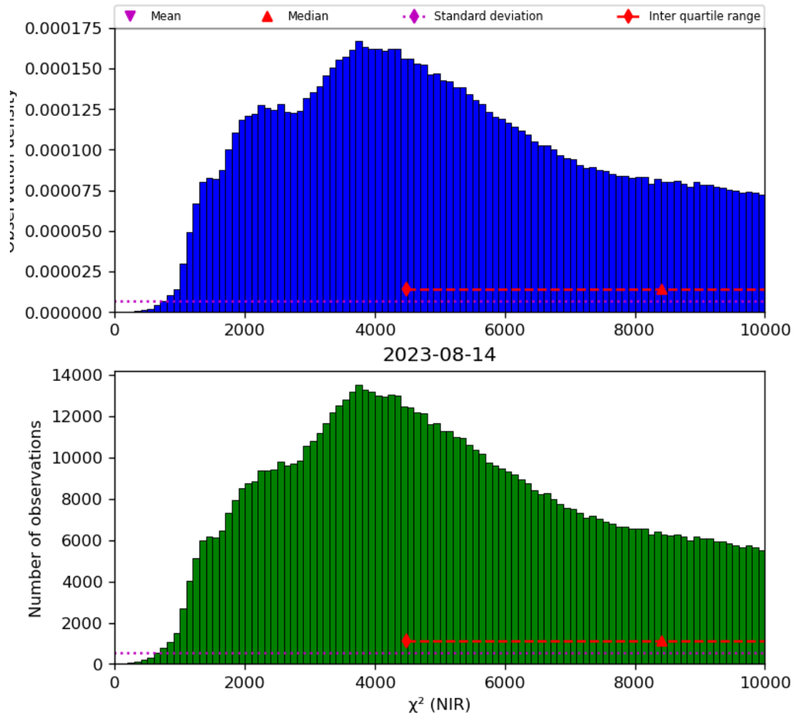
Figure 29: Histogram of “ \chi^2 (NIR)” for 2023-08-14 to 2023-08-15
