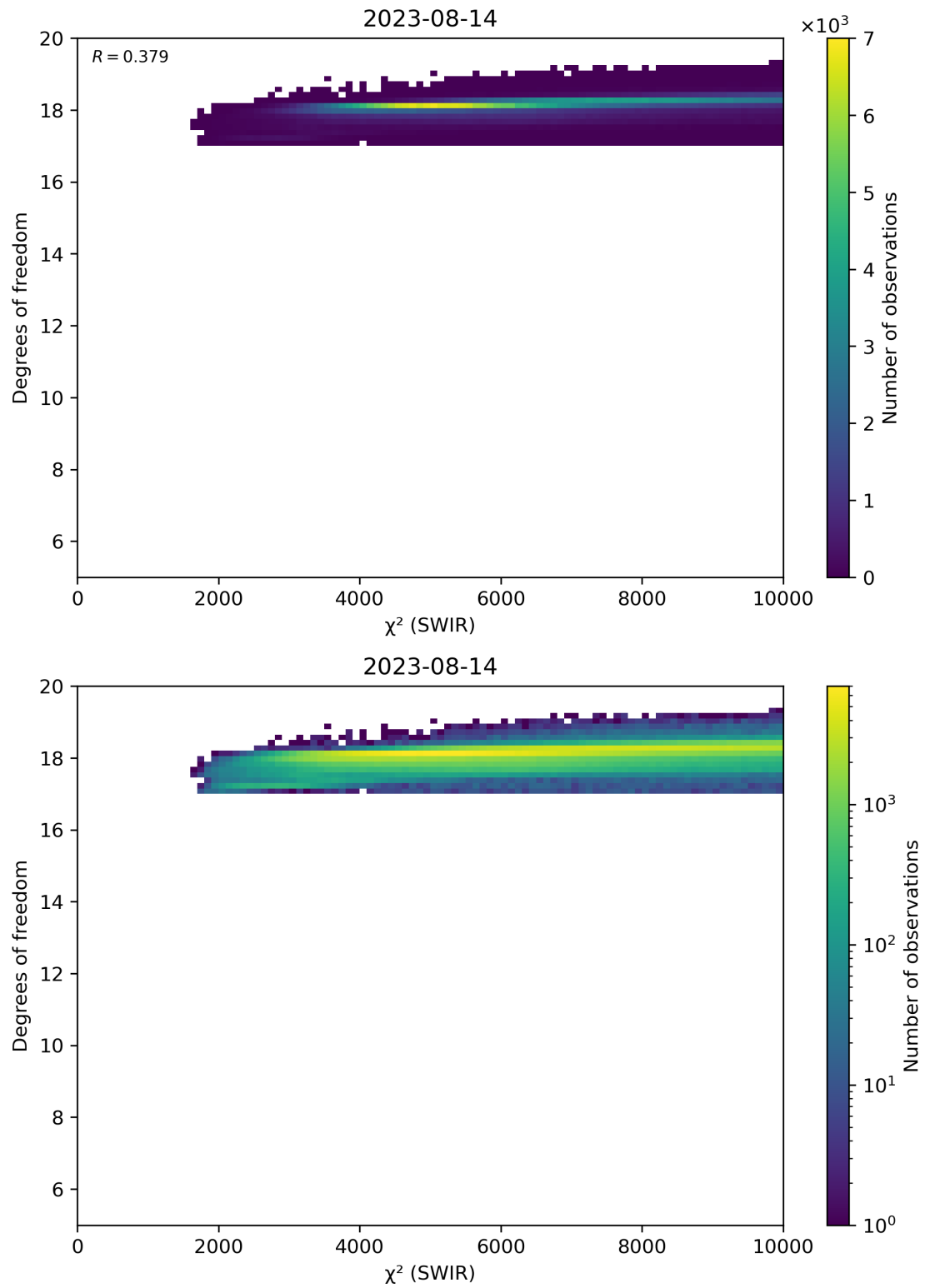
Figure 48: Scatter density plot of “ \chi^2 (SWIR)” against “Degrees of freedom” for 2023-08-14 to 2023-08-15.
