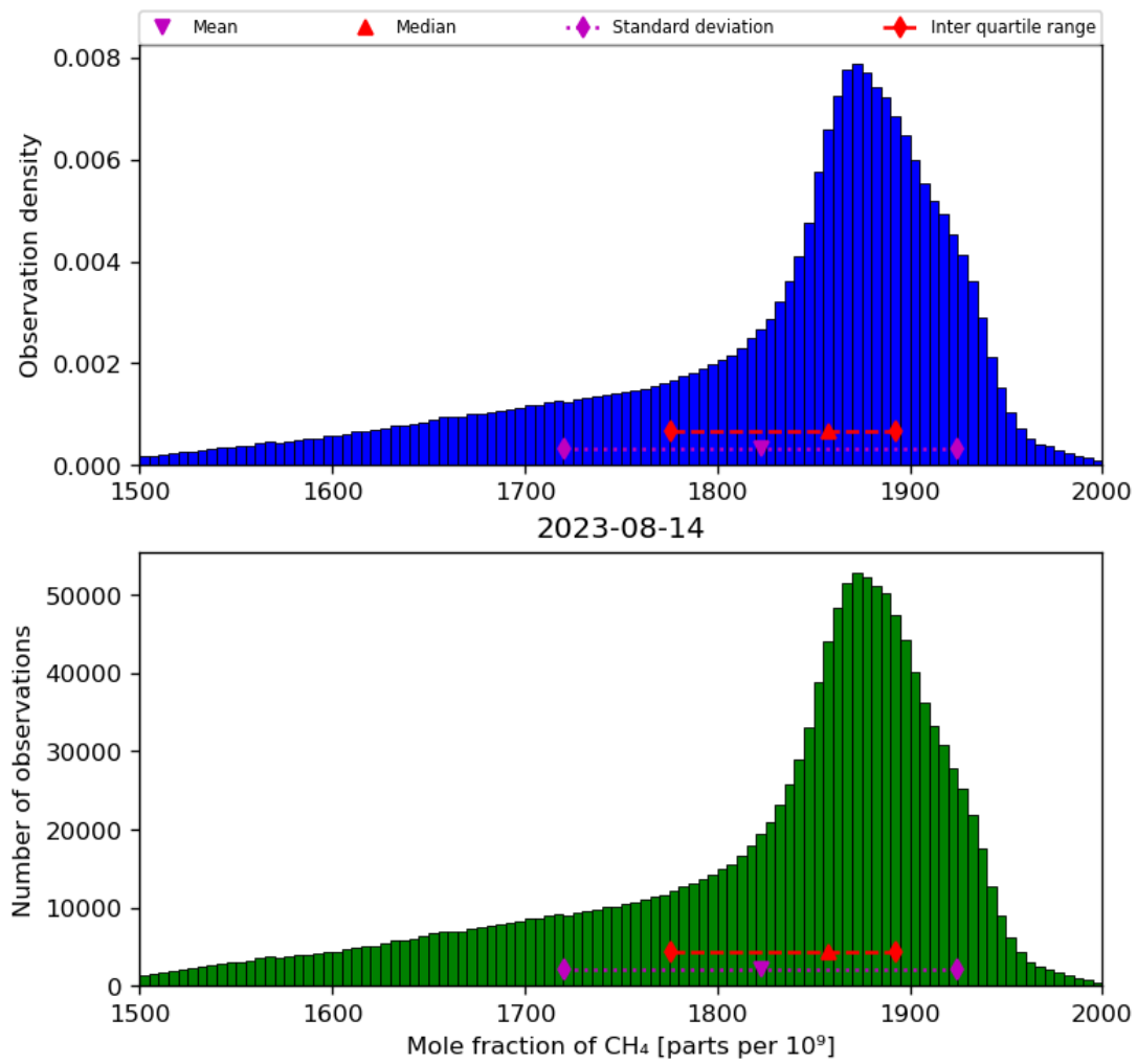
Figure 23: Histogram of “Mole fraction of CH 4 ” for 2023-08-14 to 2023-08-15
