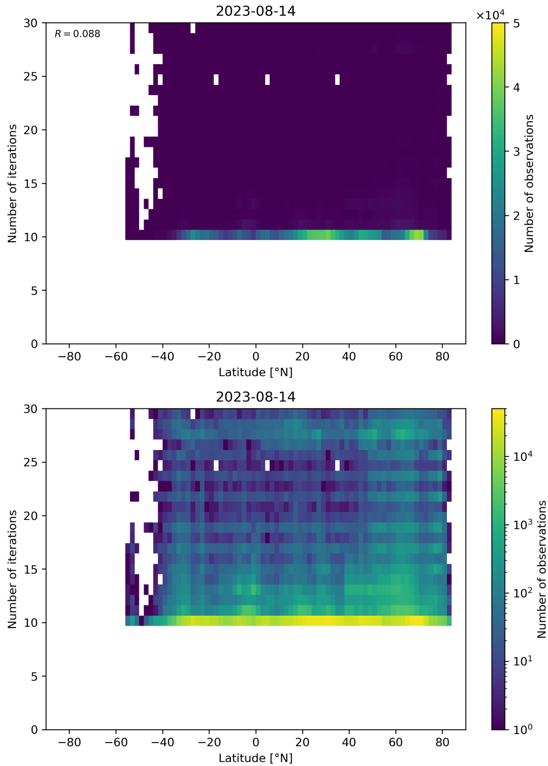
Figure 60: Scatter density plot of “Latitude” against “Number of iterations” for 2023-08-14 to 2023-08-15.
