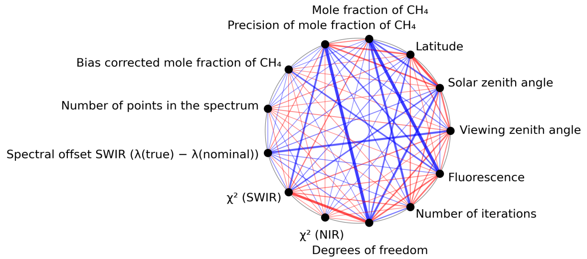
Figure 1: Map of correlation graph for 2023-08-14 to 2023-08-15.
