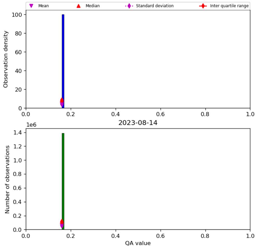
Figure 22: Histogram of “QA value” for 2023-08-14 to 2023-08-15
