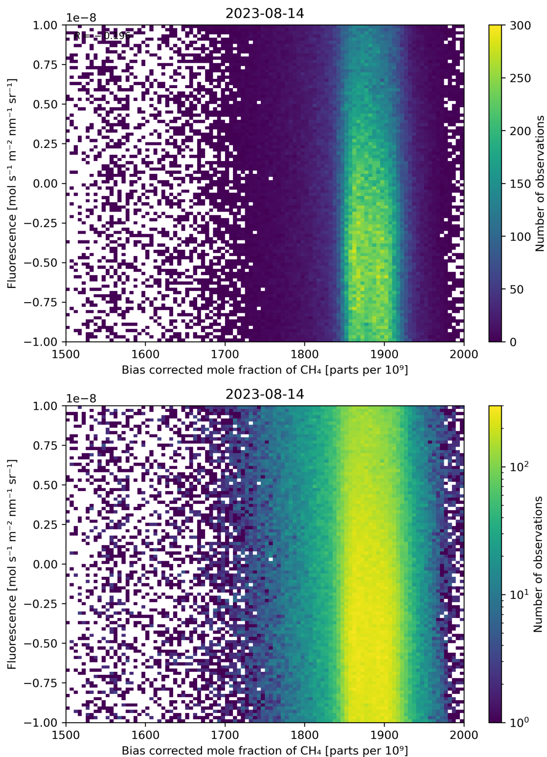
Figure 66: Scatter density plot of “Bias corrected mole fraction of \text{CH}_4 ” against “Fluorescence” for 2023-08-14 to 2023-08-15.
