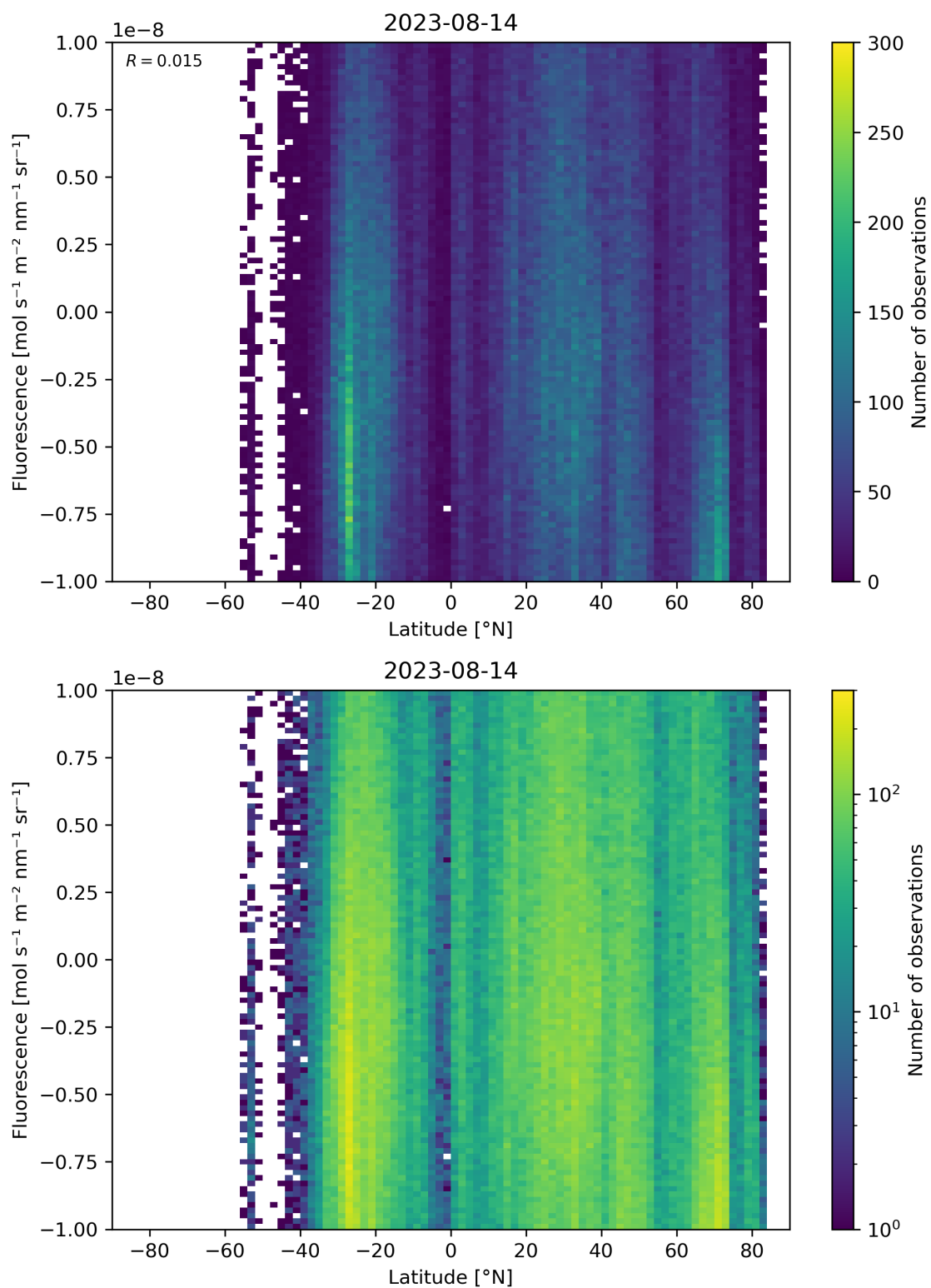
Figure 56: Scatter density plot of “Latitude” against “Fluorescence” for 2023-08-14 to 2023-08-15.
