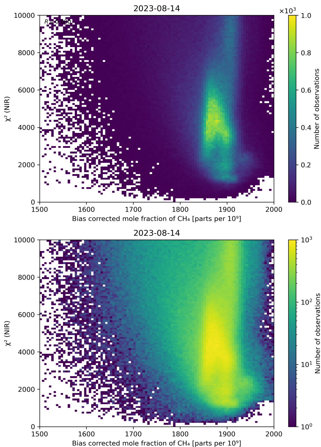
Figure 63: Scatter density plot of “Bias corrected mole fraction of \text{CH}_4 ” against “ \chi^2 (NIR)” for 2023-08-14 to 2023-08-15.
