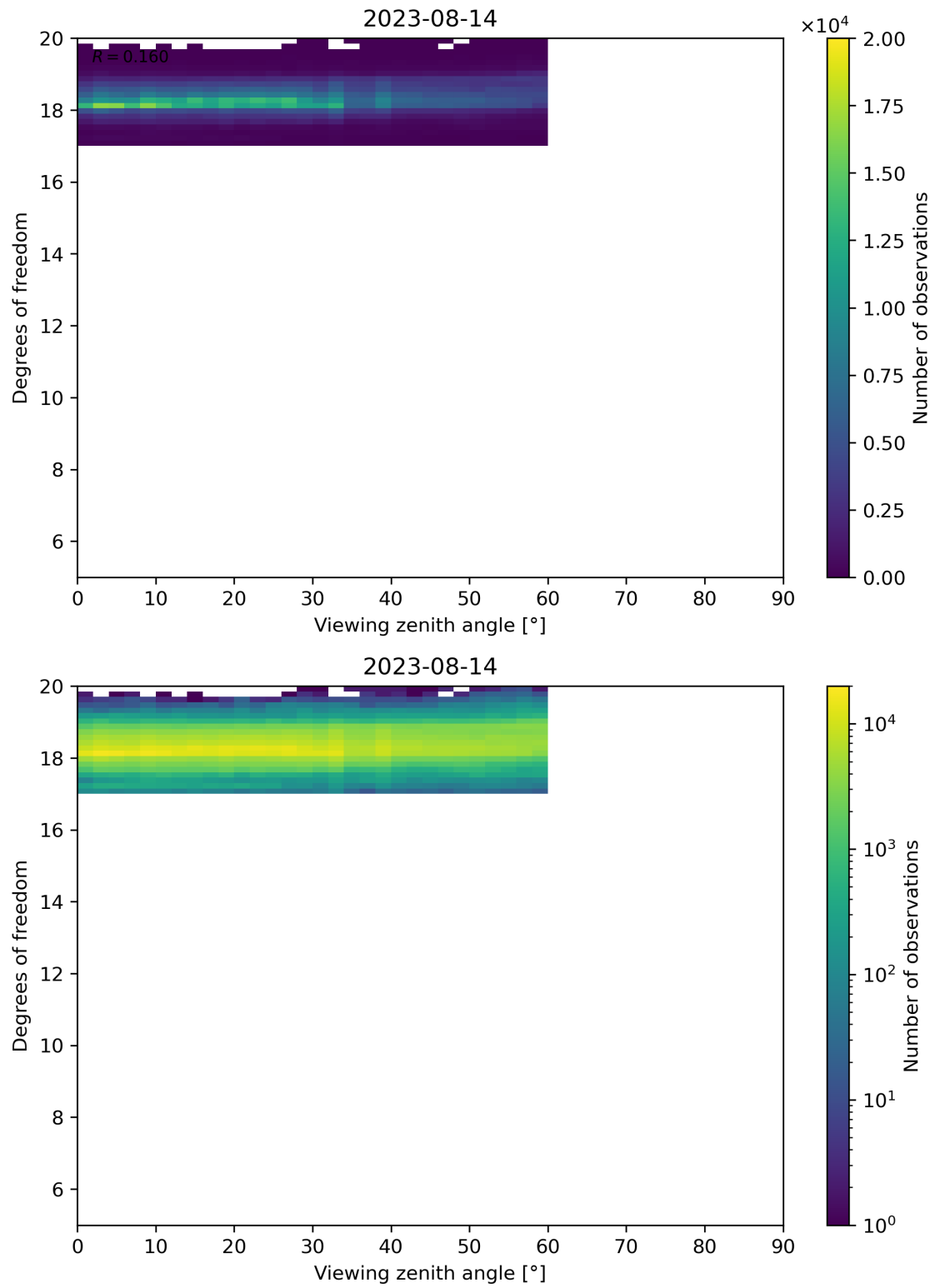
Figure 107: Scatter density plot of “Viewing zenith angle” against “Degrees of freedom” for 2023-08-14 to 2023-08-15.
