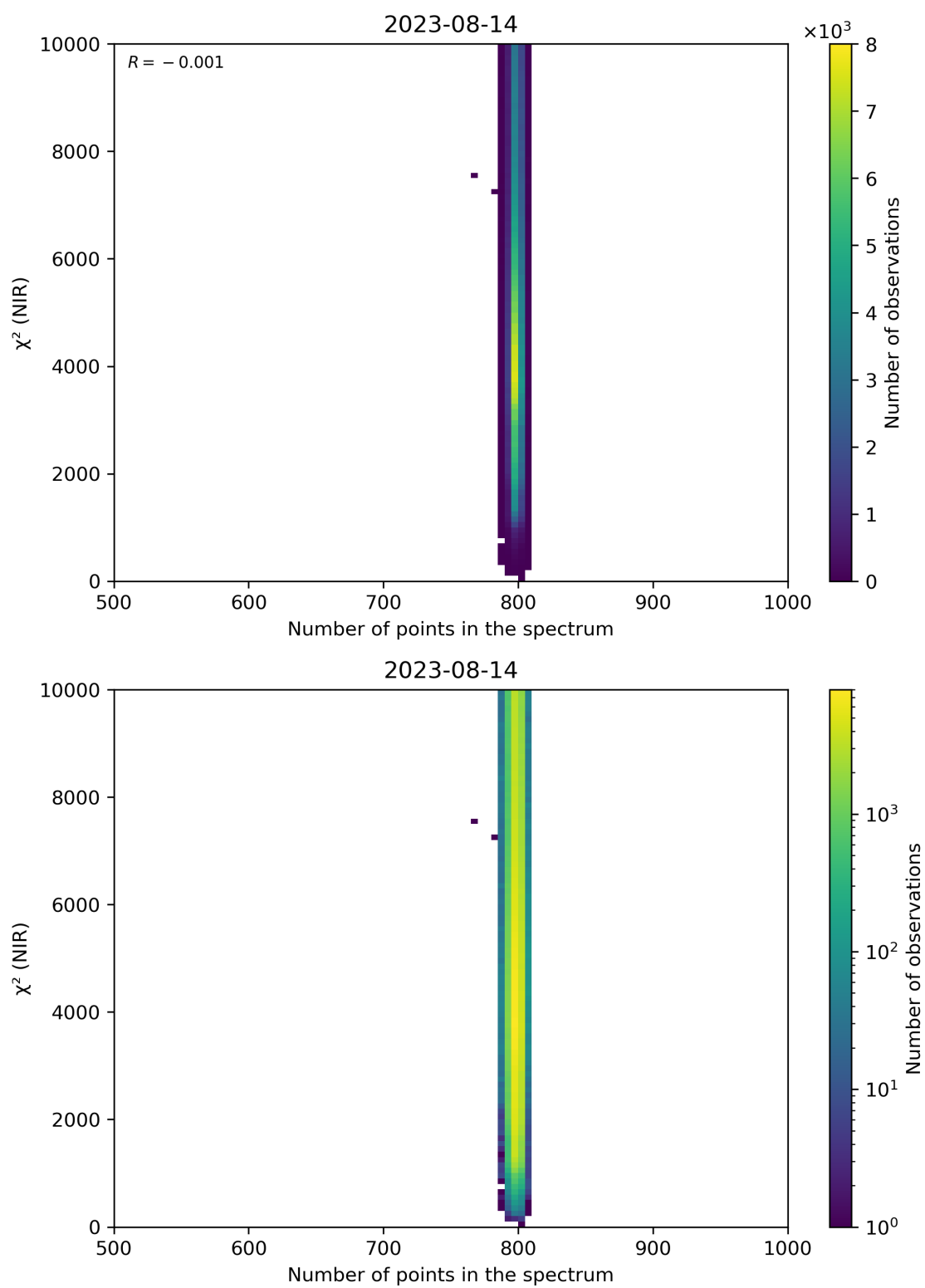
Figure 88: Scatter density plot of “Number of points in the spectrum” against “ \chi^2 (NIR)” for 2023-08-14 to 2023-08-15.
