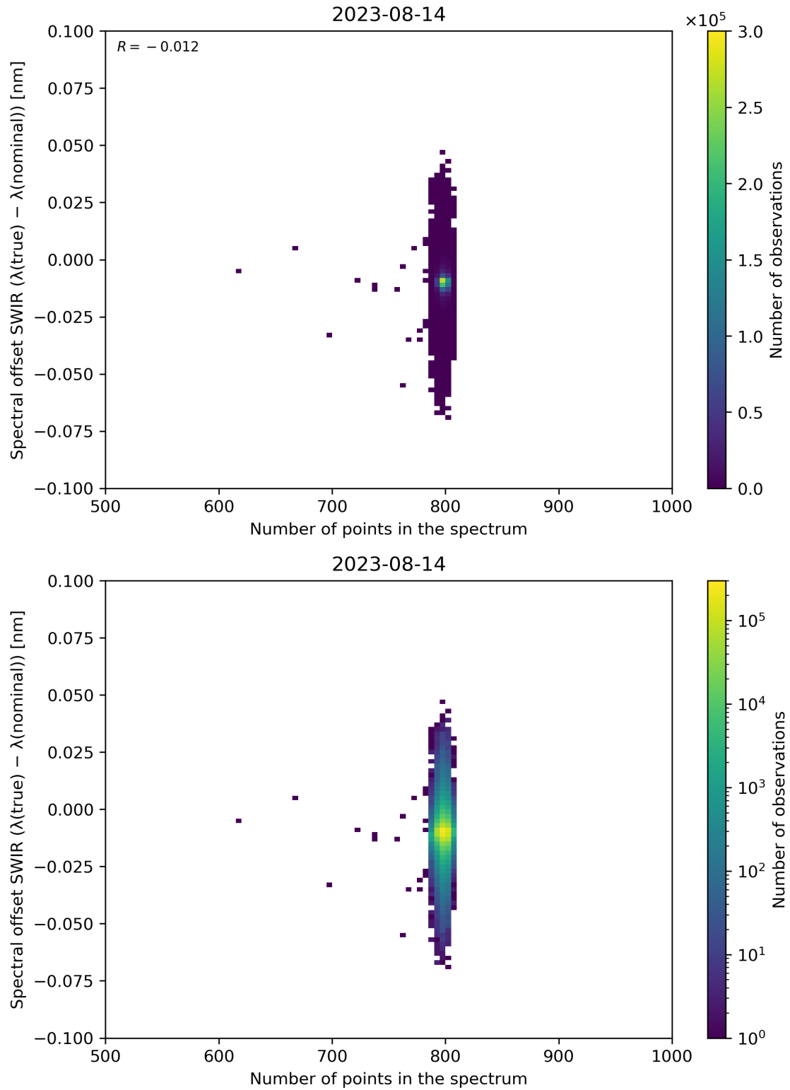
Figure 93: Scatter density plot of “Number of points in the spectrum” against “Spectral offset SWIR ( \lambda(\text{true}) - \lambda(\text{nominal}) )” for 2023-08-14 to 2023-08-15.
