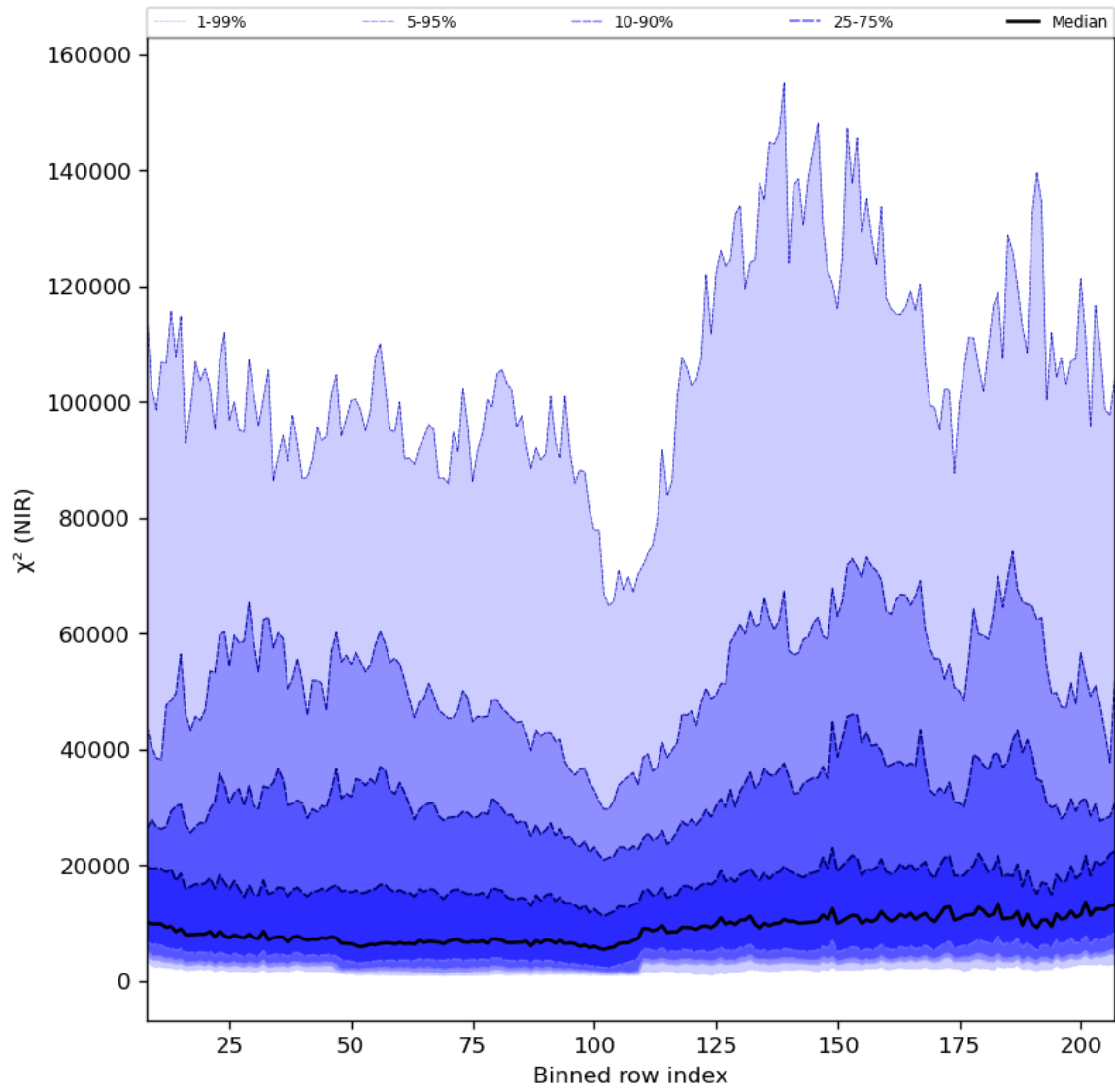
Figure 40: Along track statistics of " \chi^2 (NIR)" for 2023-08-14 to 2023-08-15
