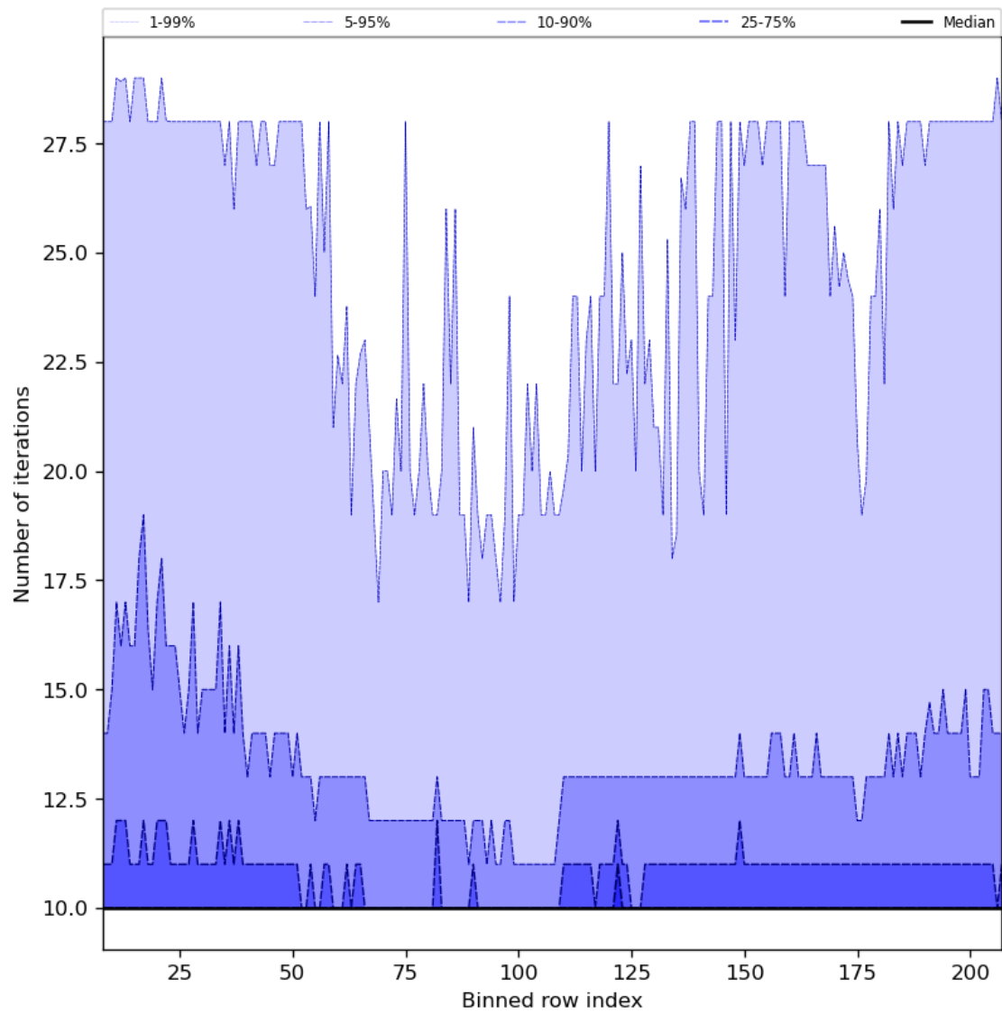
Figure 42: Along track statistics of “Number of iterations” for 2023-08-14 to 2023-08-15
