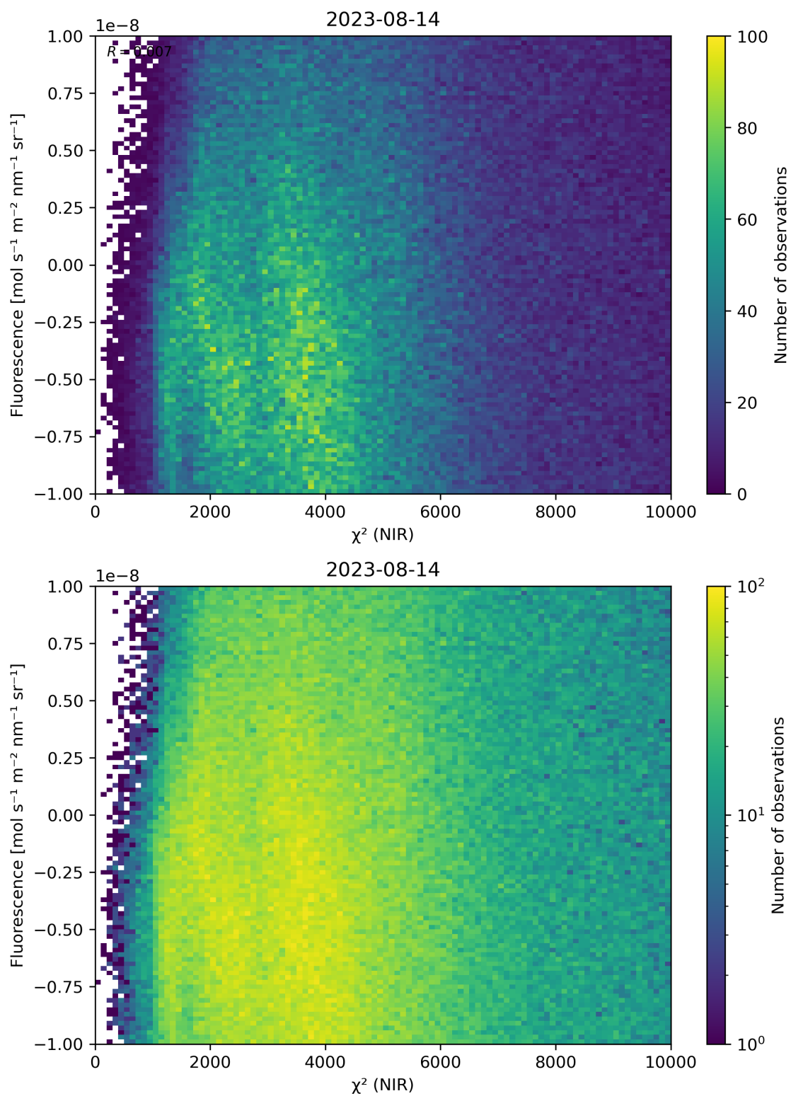
Figure 45: Scatter density plot of “ \chi^2 (NIR)” against “Fluorescence” for 2023-08-14 to 2023-08-15.
