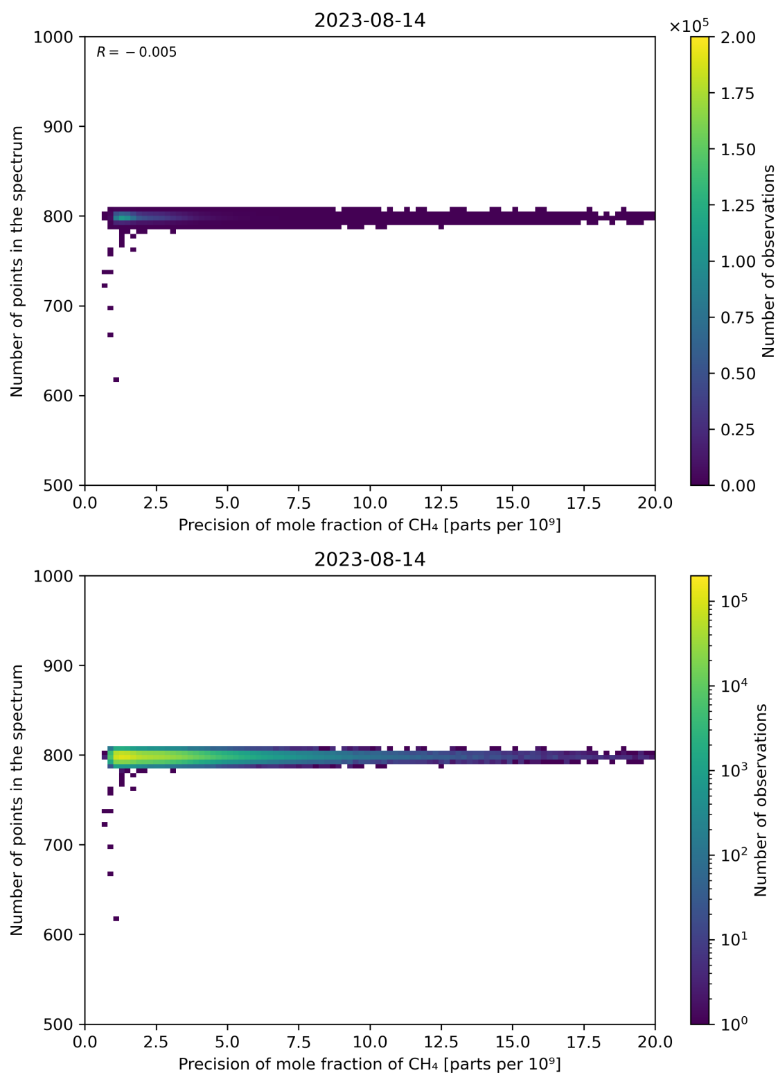
Figure 84: Scatter density plot of “Precision of mole fraction of CH 4 ” against “Number of points in the spectrum” for 2023-08-14 to 2023-08-15.
