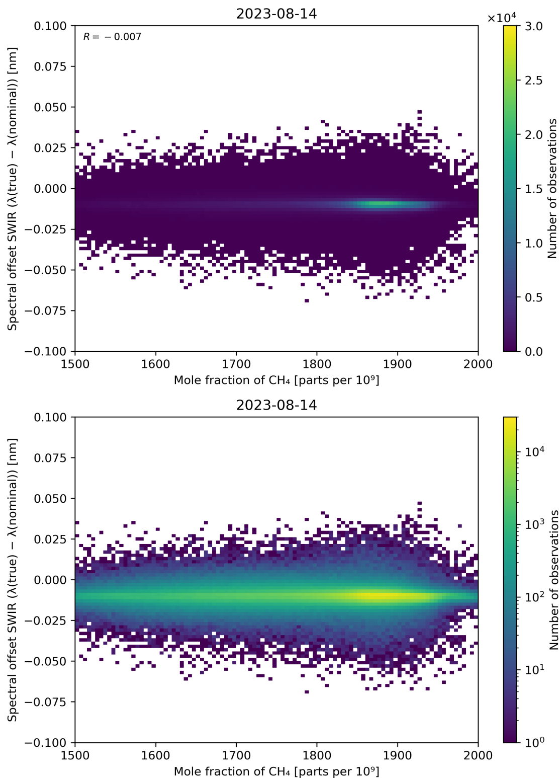
Figure 86: Scatter density plot of “Mole fraction of CH 4 ” against “Spectral offset SWIR ( \lambda(\text{true}) - \lambda(\text{nominal}) )” for 2023-08-14 to 2023-08-15.
