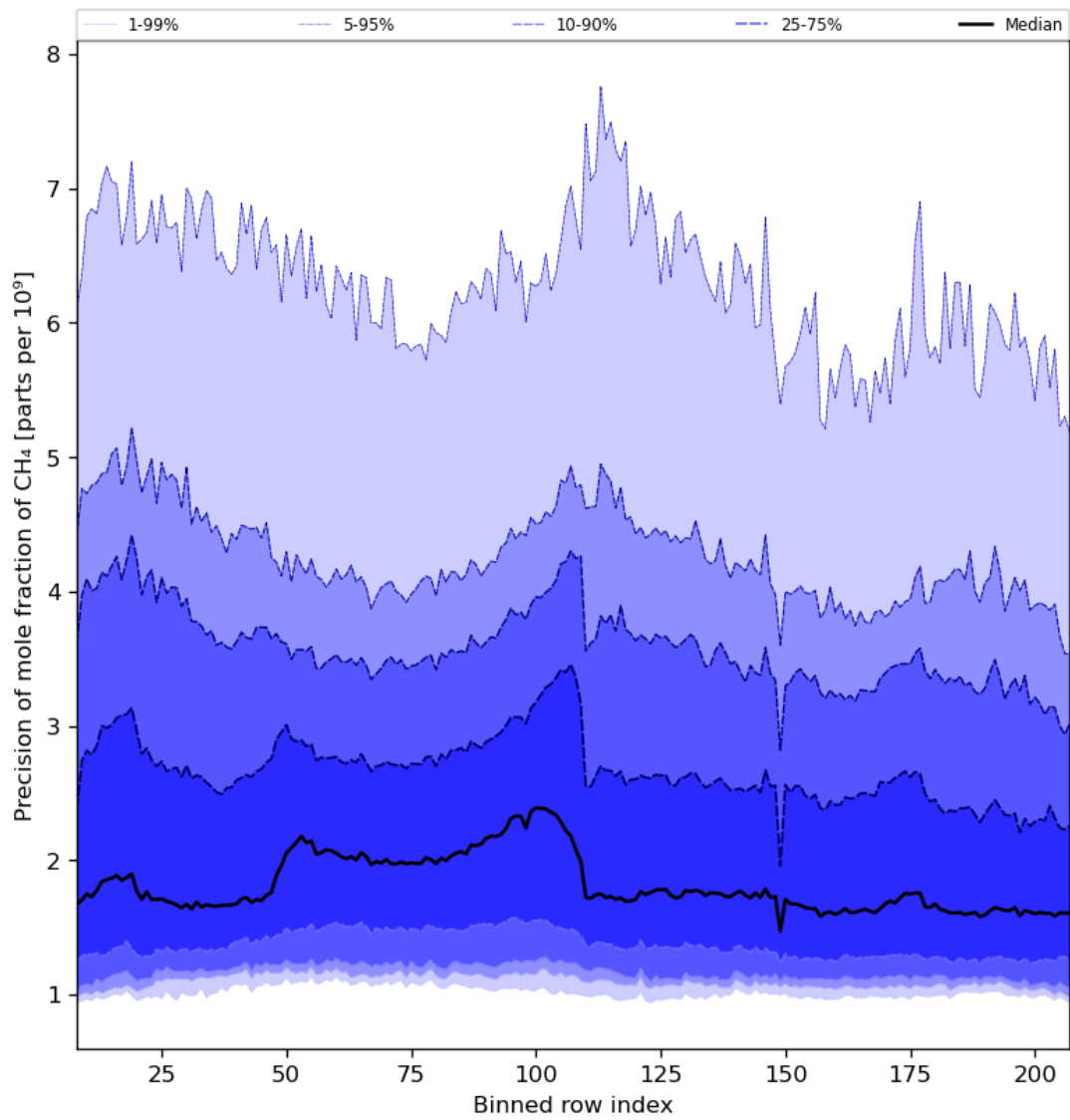
Figure 35: Along track statistics of “Precision of mole fraction of CH 4 ” for 2023-08-14 to 2023-08-15
