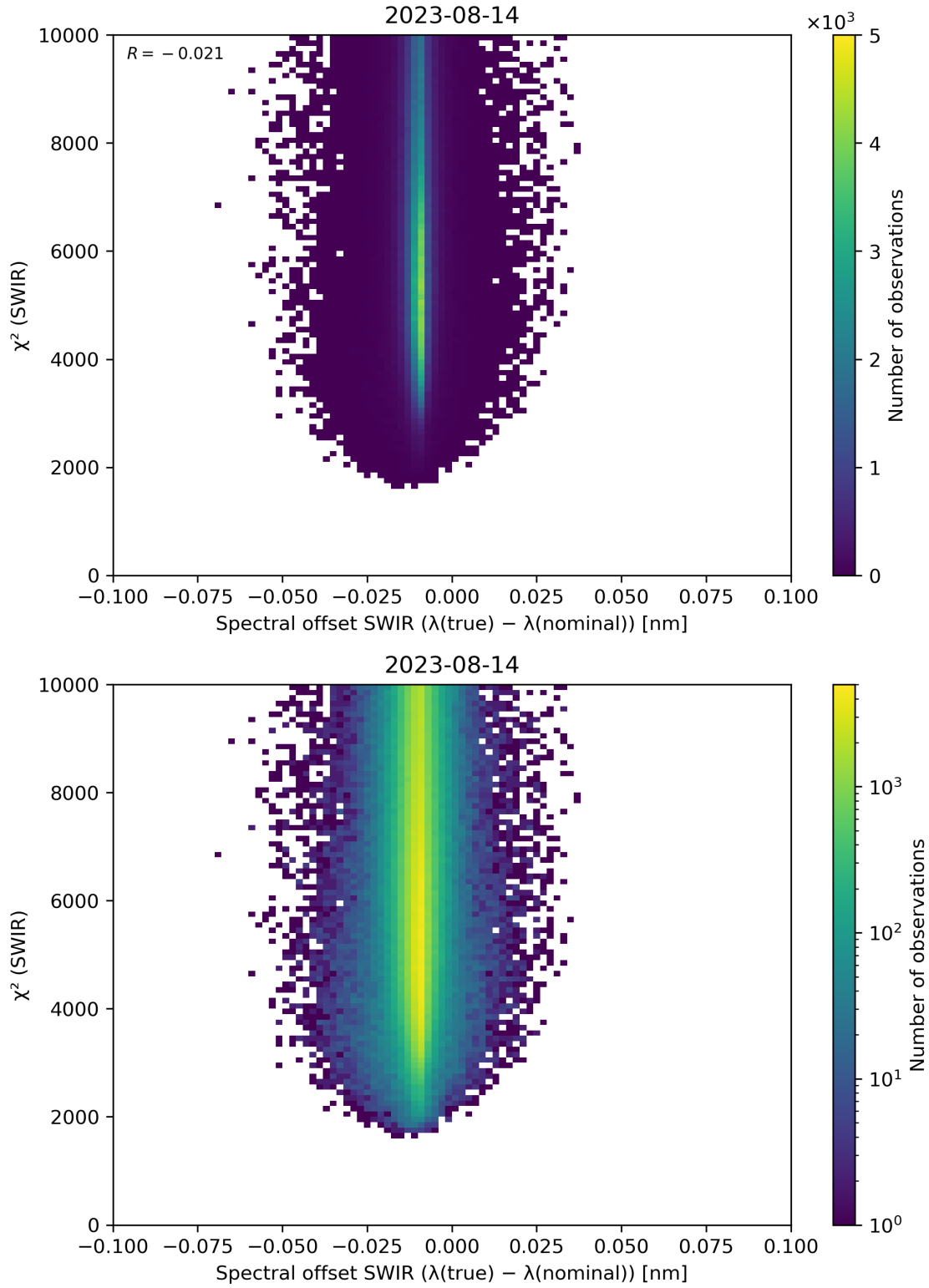
Figure 118: Scatter density plot of “Spectral offset SWIR ( \lambda(\text{true}) - \lambda(\text{nominal}) )” against “ \chi^2 (SWIR)” for 2023-08-14 to 2023-08-15.
