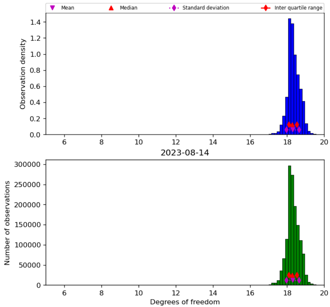
Figure 30: Histogram of “Degrees of freedom” for 2023-08-14 to 2023-08-15
