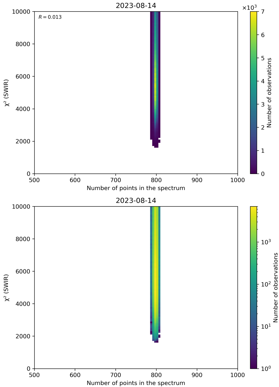
Figure 89: Scatter density plot of “Number of points in the spectrum” against “ \chi^2 (SWIR)” for 2023-08-14 to 2023-08-15.
