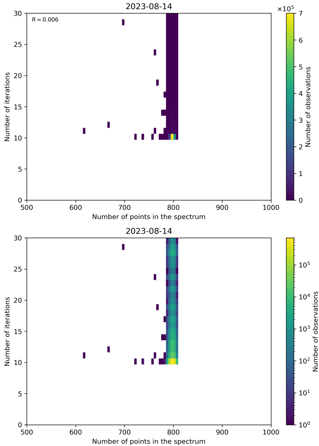
Figure 92: Scatter density plot of “Number of points in the spectrum” against “Number of iterations” for 2023-08-14 to 2023-08-15.
