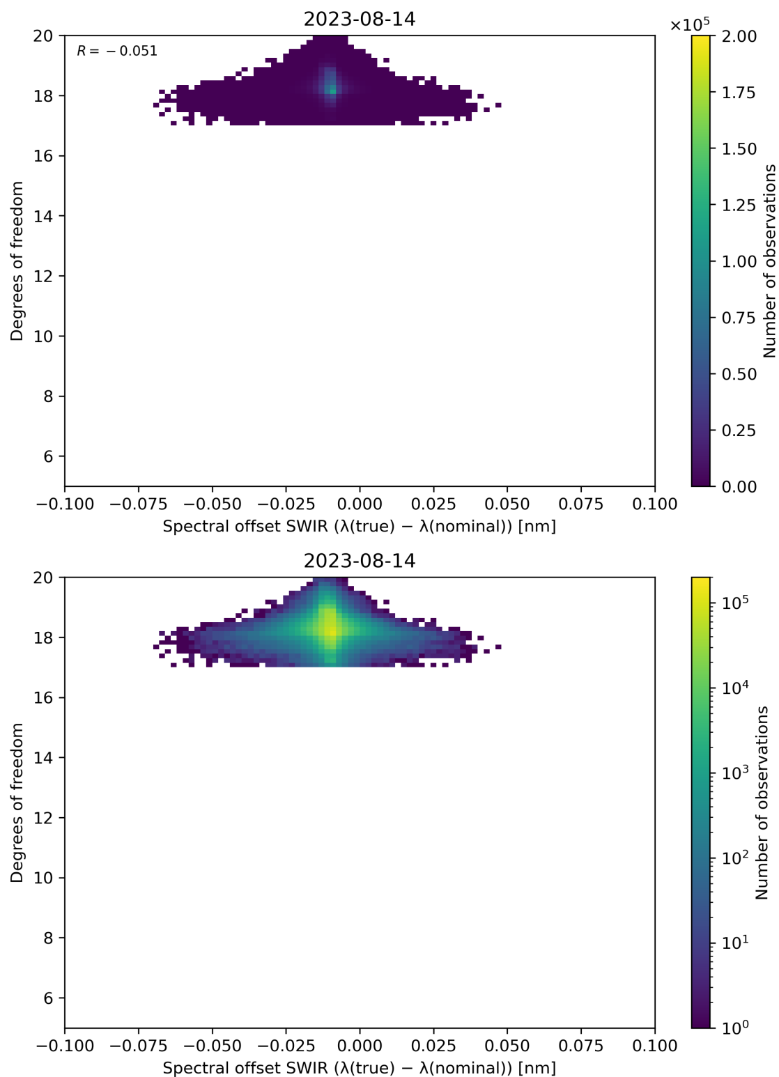
Figure 119: Scatter density plot of “Spectral offset SWIR ( \lambda(\text{true}) - \lambda(\text{nominal}) )” against “Degrees of freedom” for 2023-08-14 to 2023-08-15.
