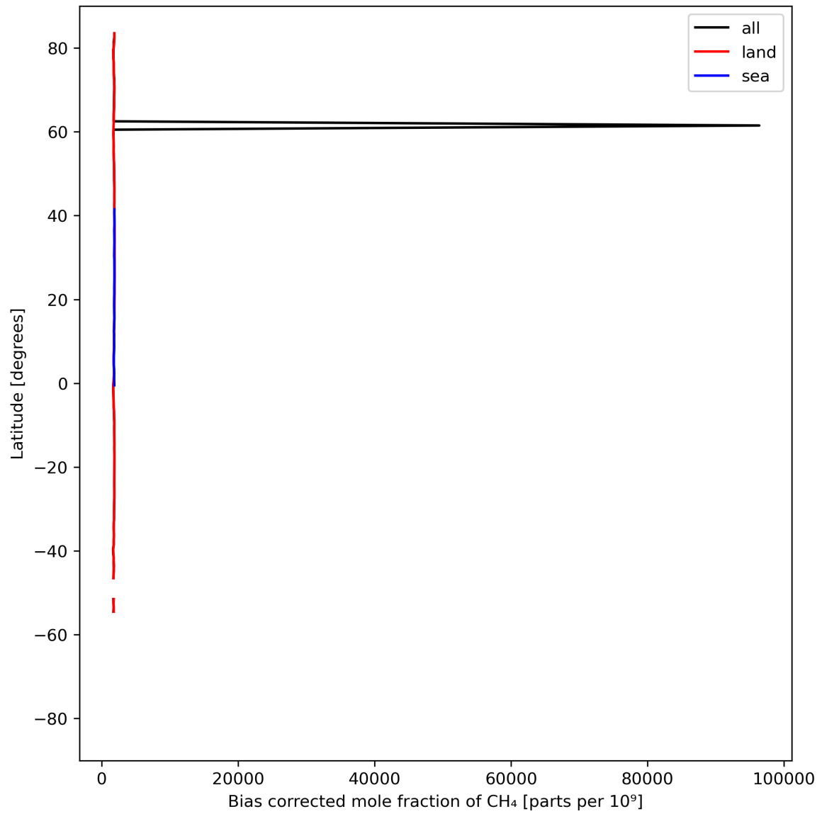
Figure 14: Zonal average of “Bias corrected mole fraction of CH 4 ” for 2023-08-14 to 2023-08-15.
