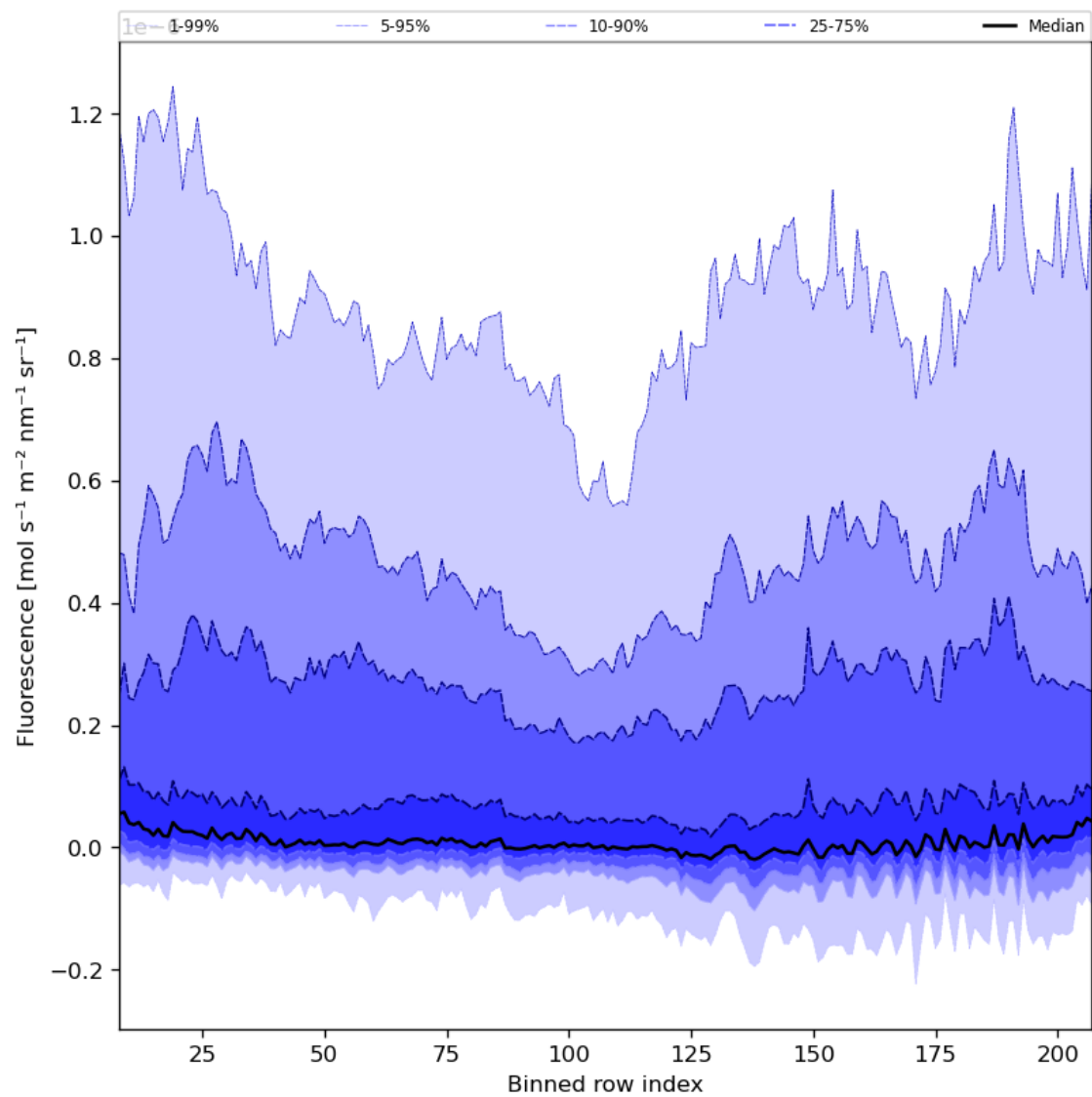
Figure 43: Along track statistics of “Fluorescence” for 2023-08-14 to 2023-08-15
