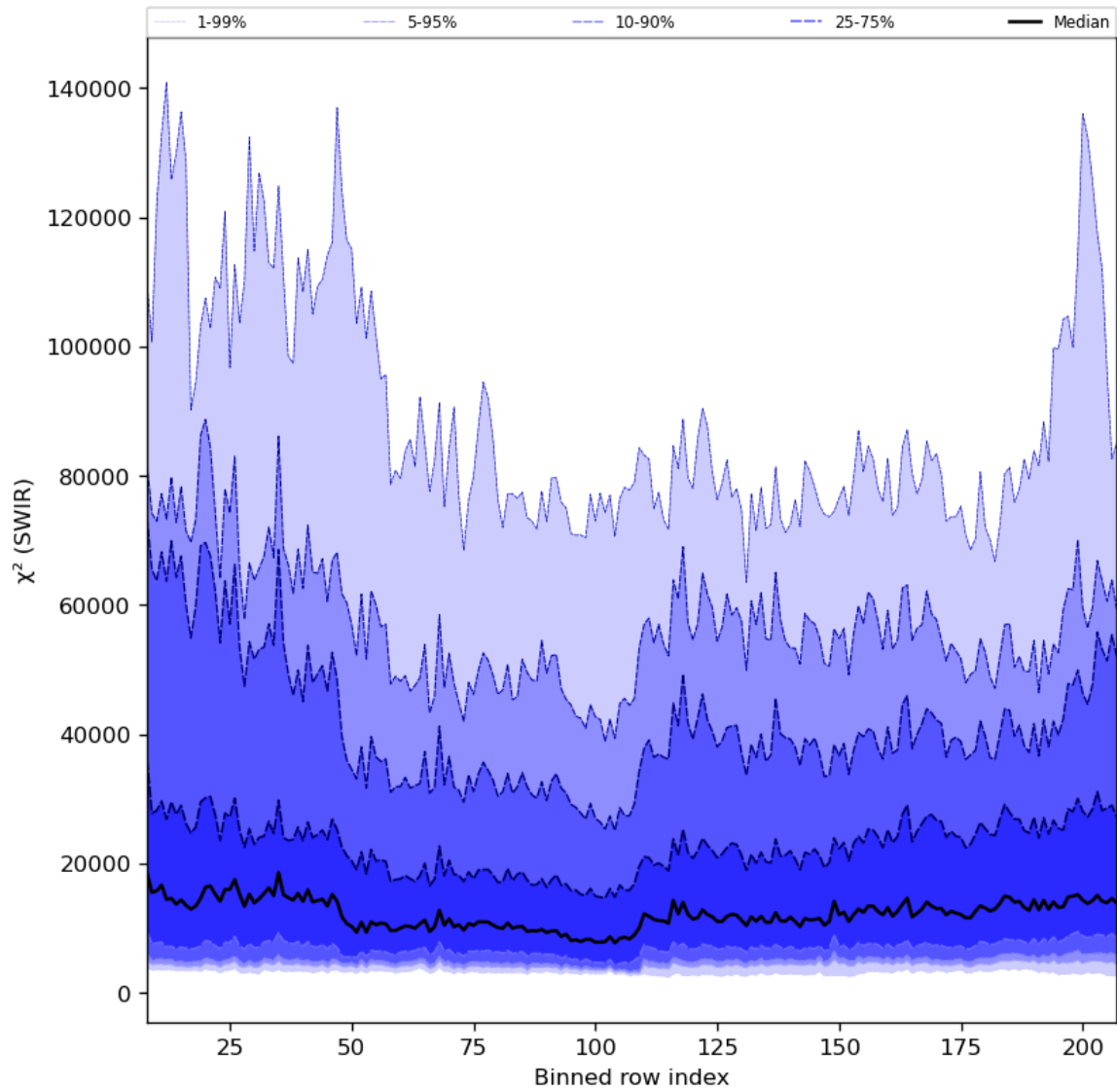
Figure 39: Along track statistics of “ \chi^2 (SWIR)” for 2023-08-14 to 2023-08-15
