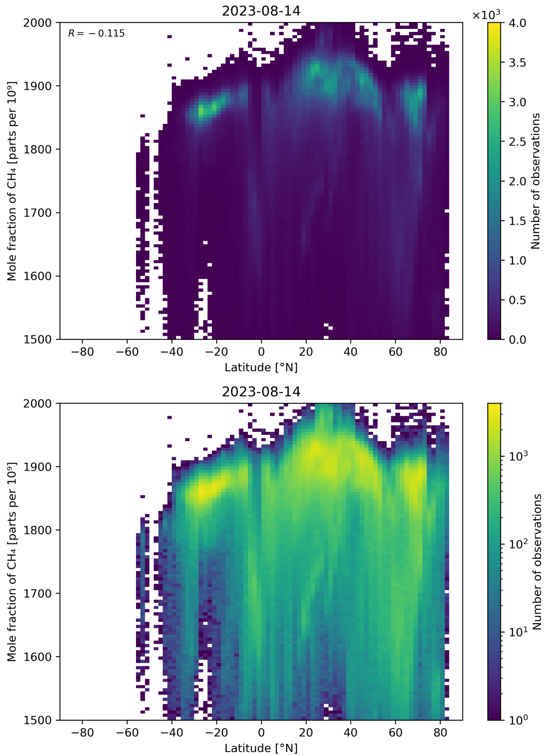
Figure 57: Scatter density plot of “Latitude” against “Mole fraction of \text{CH}_4 ” for 2023-08-14 to 2023-08-15.
