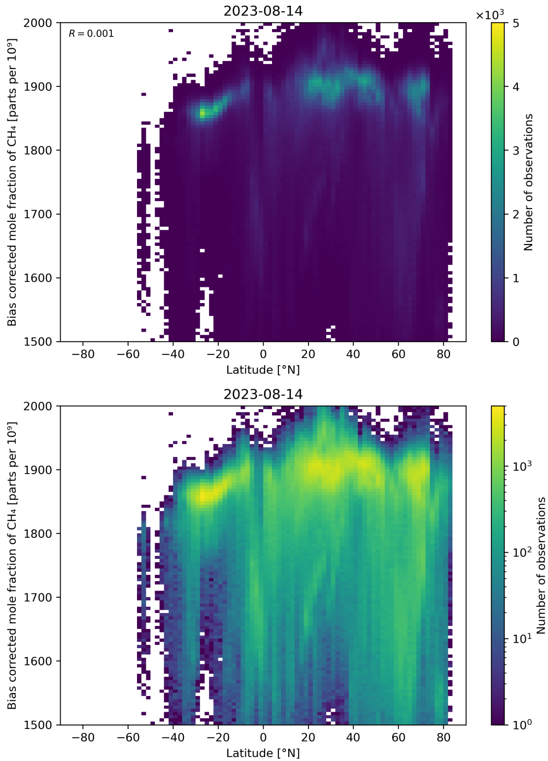
Figure 58: Scatter density plot of “Latitude” against “Bias corrected mole fraction of CH 4 ” for 2023-08-14 to 2023-08-15.
