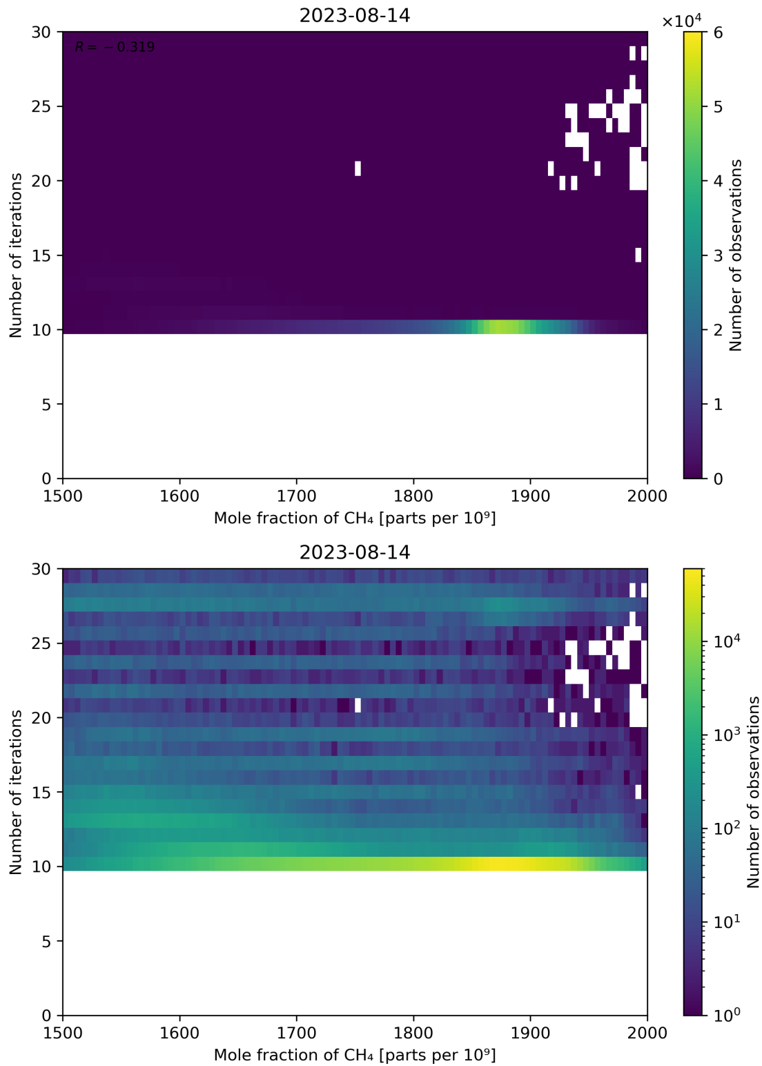
Figure 76: Scatter density plot of “Mole fraction of CH 4 ” against “Number of iterations” for 2023-08-14 to 2023-08-15.
