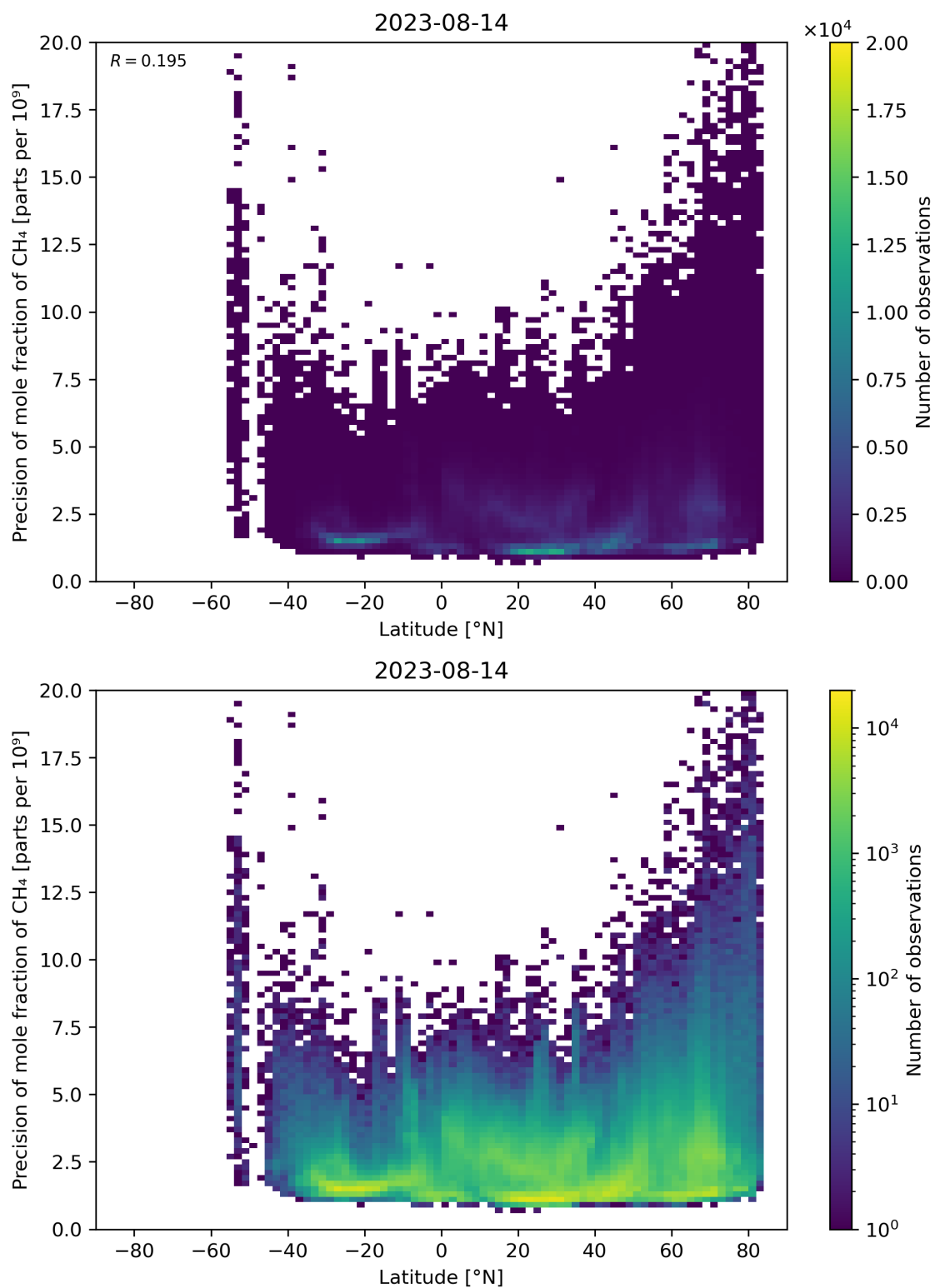
Figure 59: Scatter density plot of “Latitude” against “Precision of mole fraction of \text{CH}_4 ” for 2023-08-14 to 2023-08-15.
