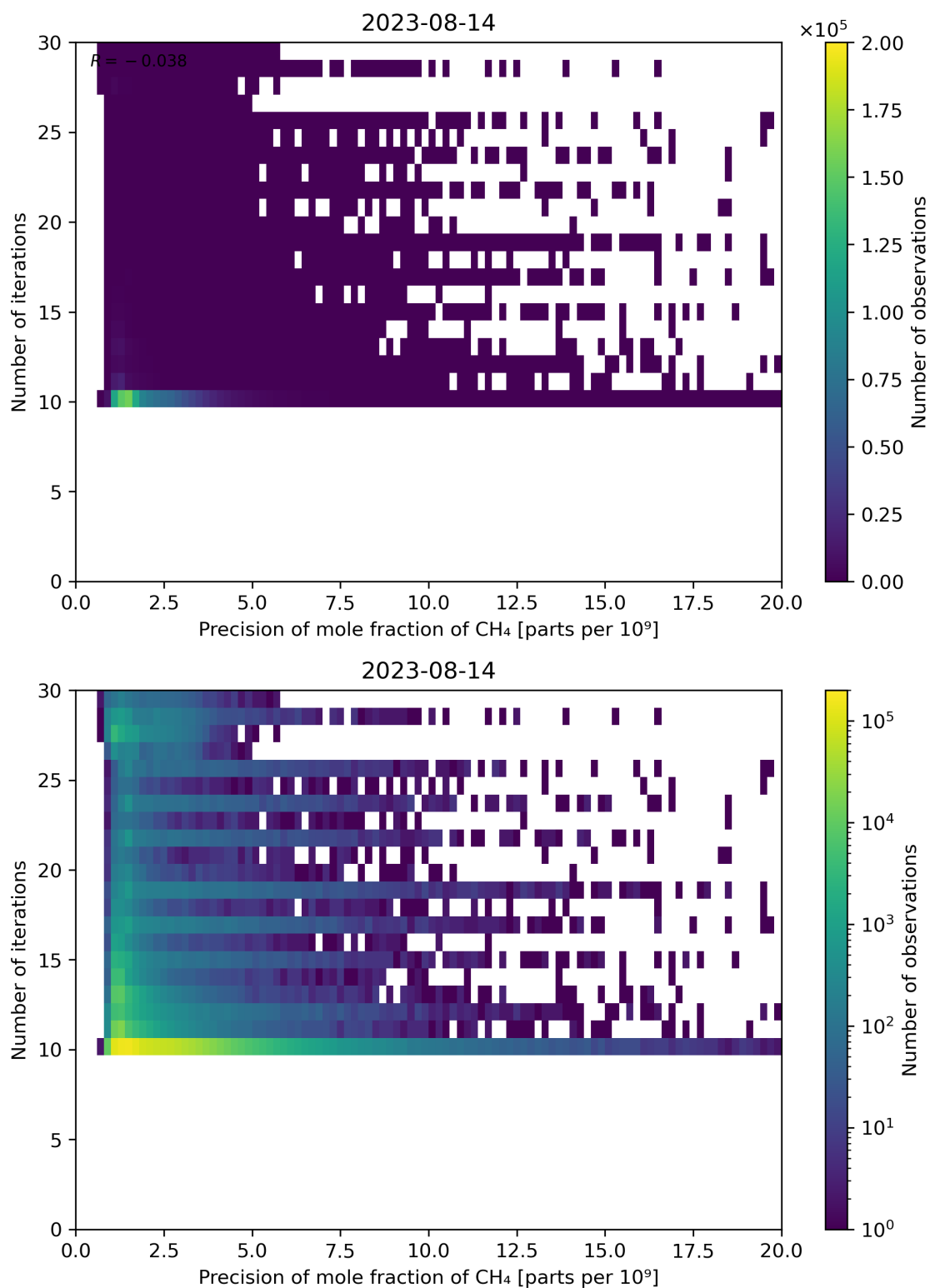
Figure 83: Scatter density plot of “Precision of mole fraction of CH 4 ” against “Number of iterations” for 2023-08-14 to 2023-08-15.
