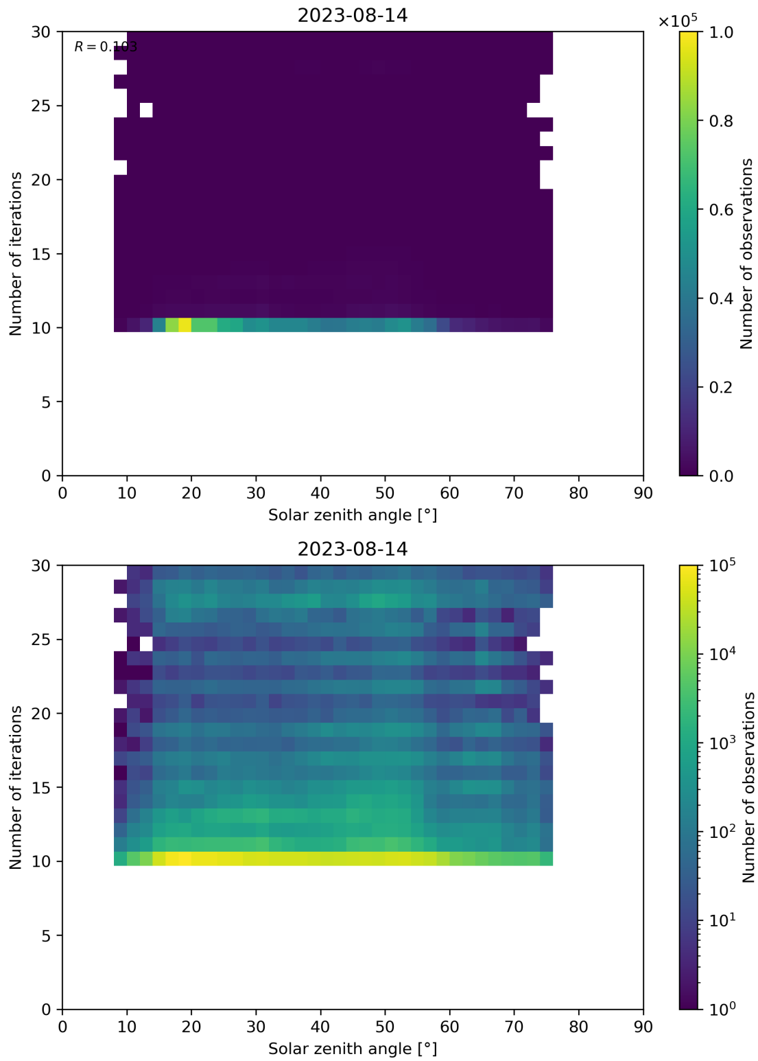
Figure 102: Scatter density plot of “Solar zenith angle” against “Number of iterations” for 2023-08-14 to 2023-08-15.
