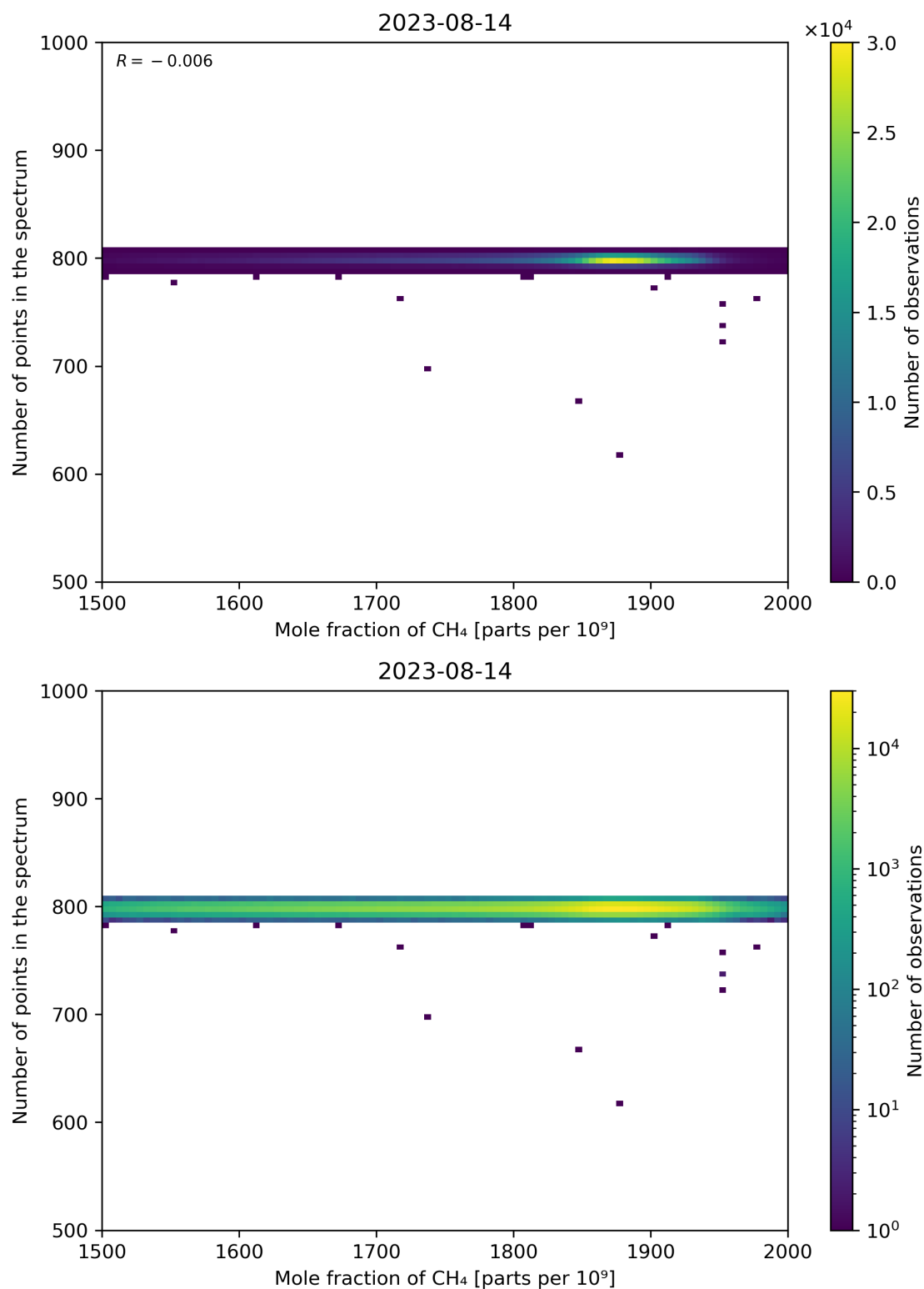
Figure 77: Scatter density plot of “Mole fraction of CH 4 ” against “Number of points in the spectrum” for 2023-08-14 to 2023-08-15.
