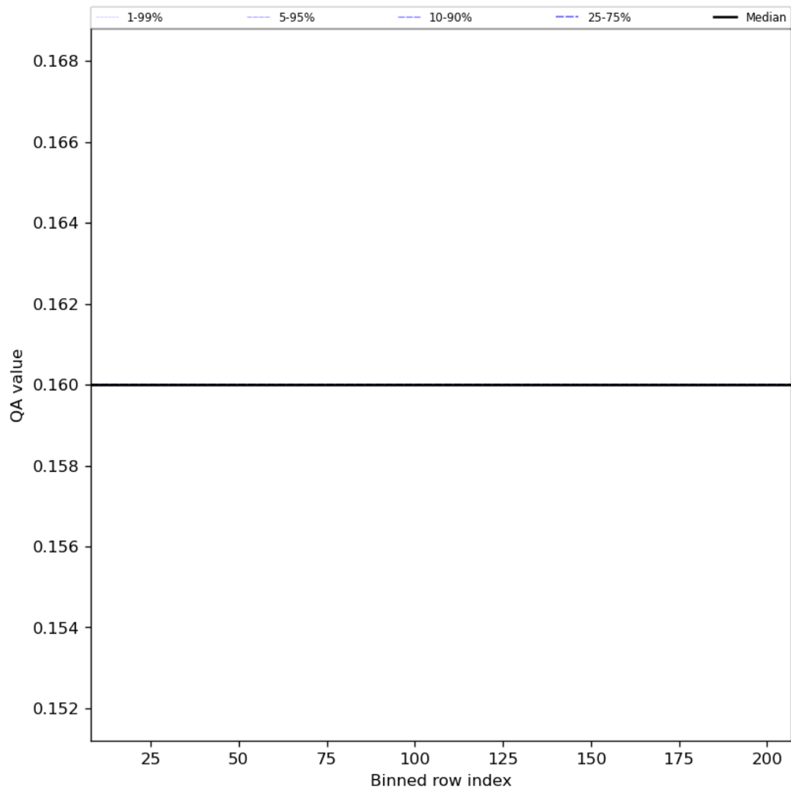
Figure 33: Along track statistics of “QA value” for 2023-08-14 to 2023-08-15
