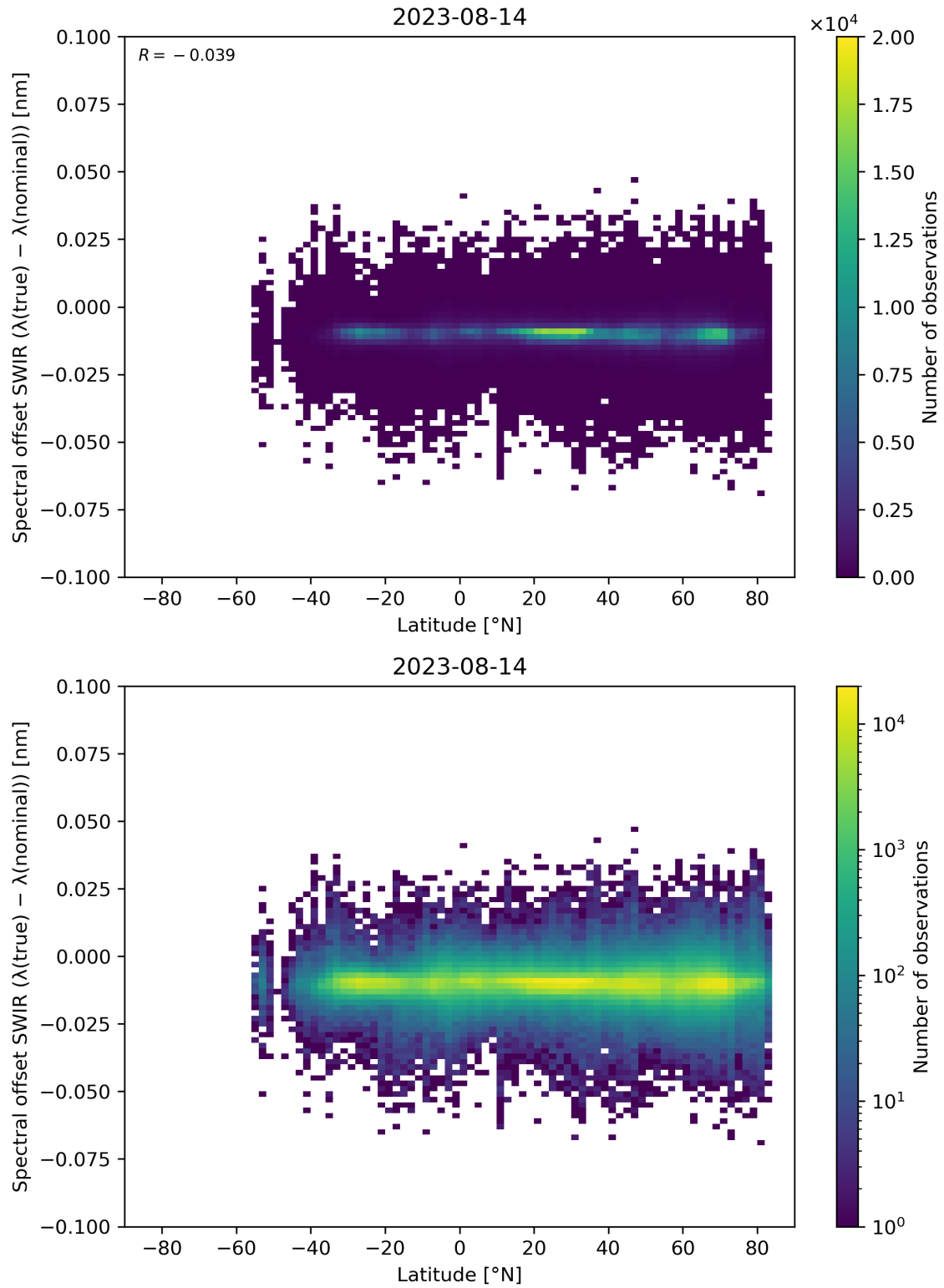
Figure 62: Scatter density plot of “Latitude” against “Spectral offset SWIR ( \lambda(\text{true}) - \lambda(\text{nominal}) )” for 2023-08-14 to 2023-08-15.
