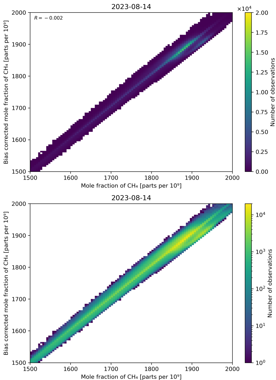
Figure 74: Scatter density plot of “Mole fraction of CH 4 ” against “Bias corrected mole fraction of CH 4 ” for 2023-08-14 to 2023-08-15.
