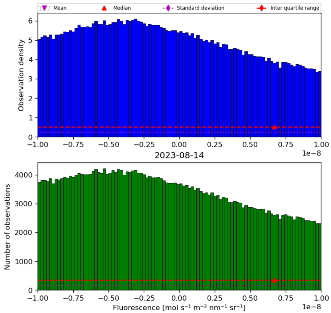
Figure 32: Histogram of “Fluorescence” for 2023-08-14 to 2023-08-15
