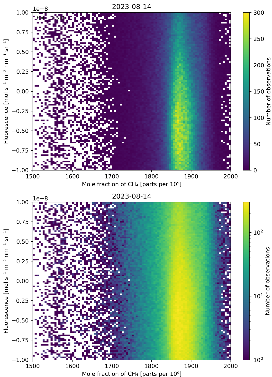
Figure 73: Scatter density plot of “Mole fraction of \text{CH}_4 ” against “Fluorescence” for 2023-08-14 to 2023-08-15.
