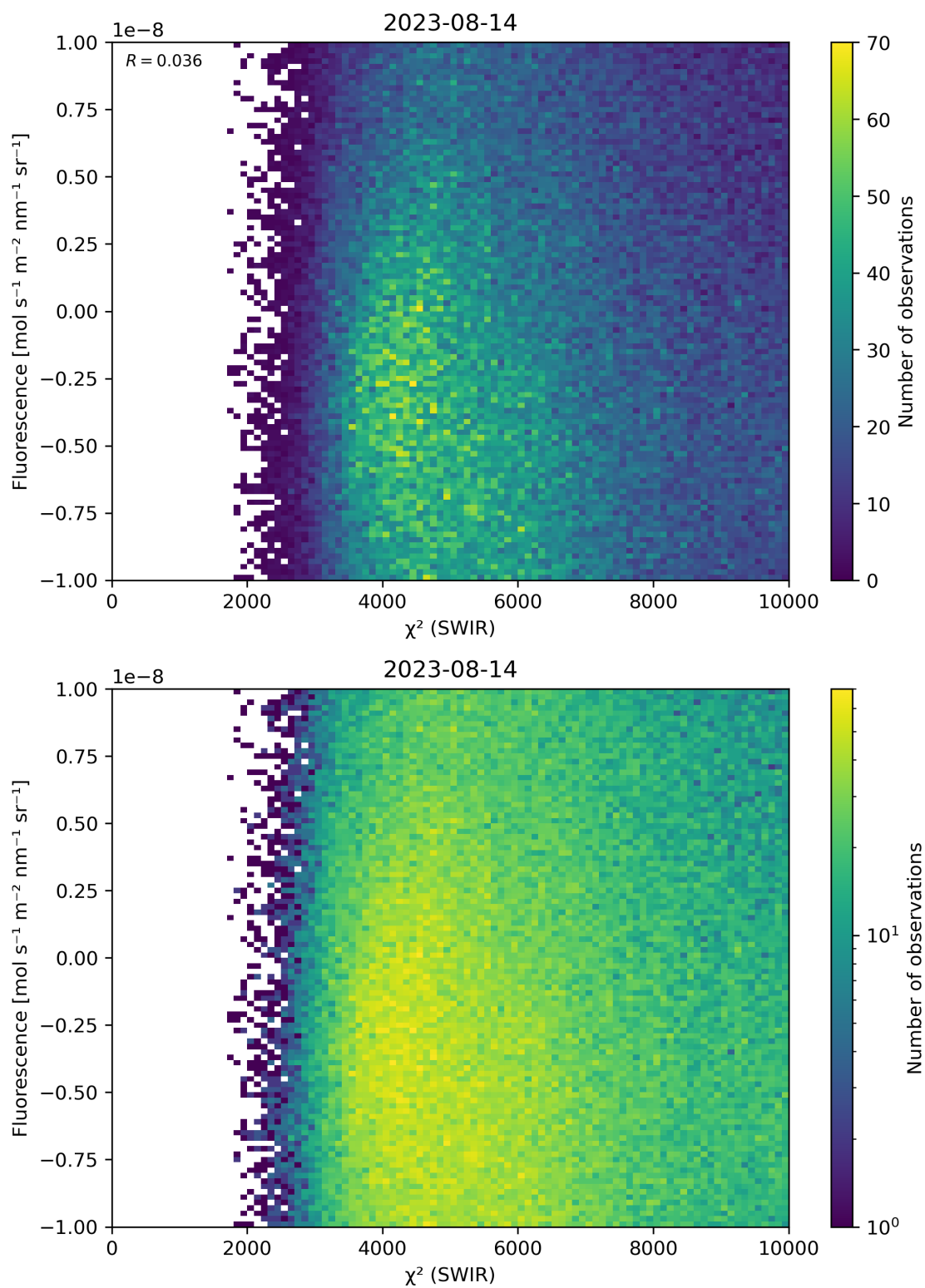
Figure 49: Scatter density plot of “ \chi^2 (SWIR)” against “Fluorescence” for 2023-08-14 to 2023-08-15.
