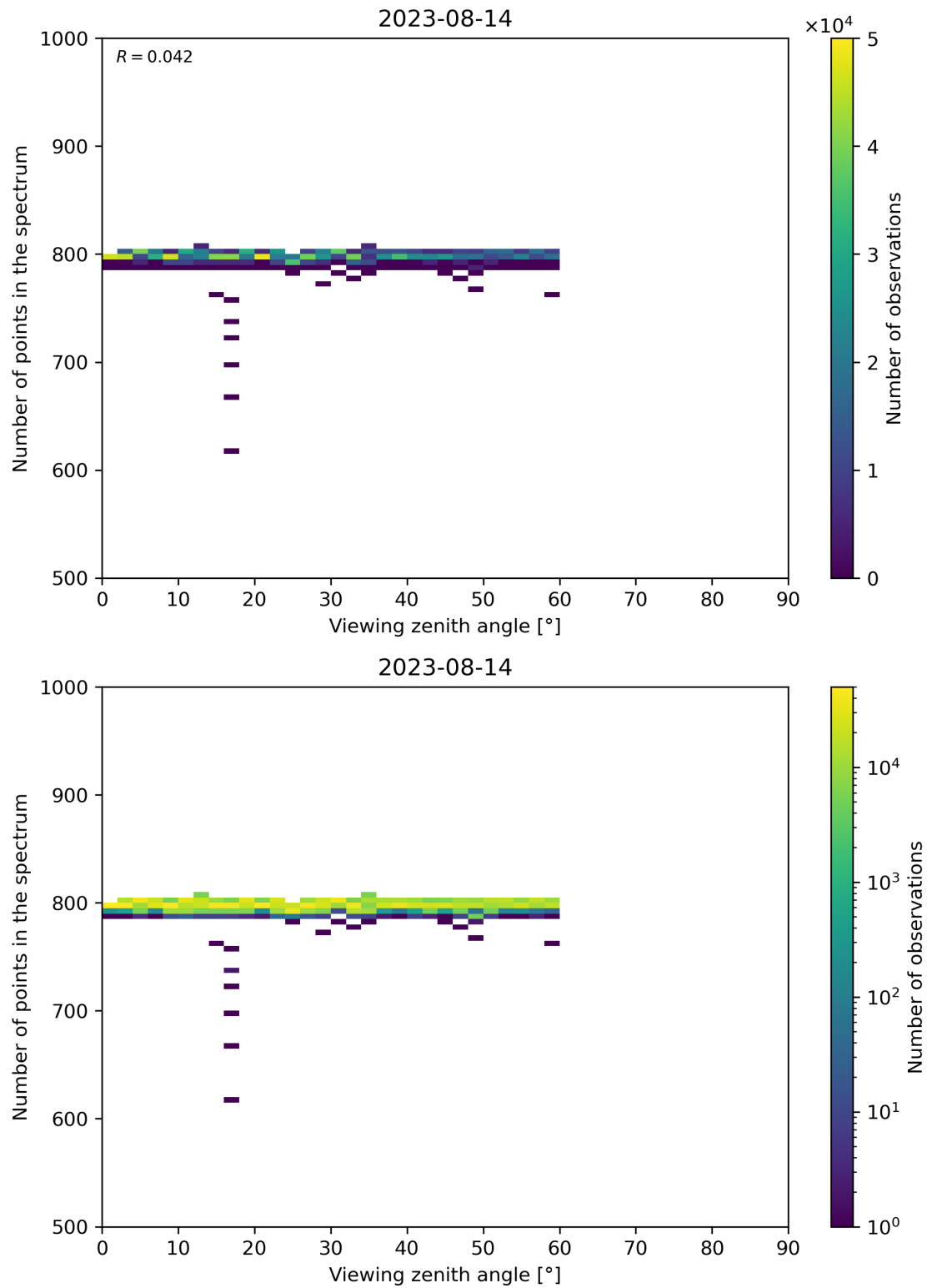
Figure 114: Scatter density plot of “Viewing zenith angle” against “Number of points in the spectrum” for 2023-08-14 to 2023-08-15.
