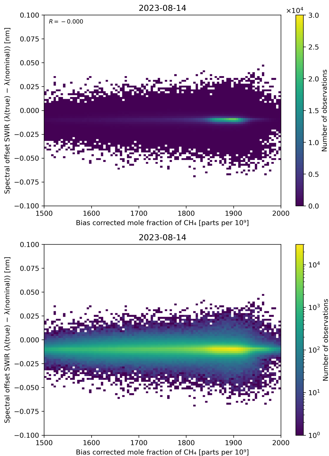
Figure 69: Scatter density plot of “Bias corrected mole fraction of \text{CH}_4 ” against “Spectral offset SWIR ( \lambda(\text{true}) - \lambda(\text{nominal}) )” for 2023-08-14 to 2023-08-15.
