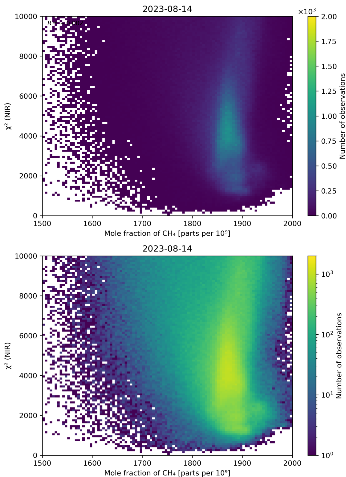
Figure 70: Scatter density plot of “Mole fraction of \text{CH}_4 ” against “ \chi^2 (NIR)” for 2023-08-14 to 2023-08-15.
