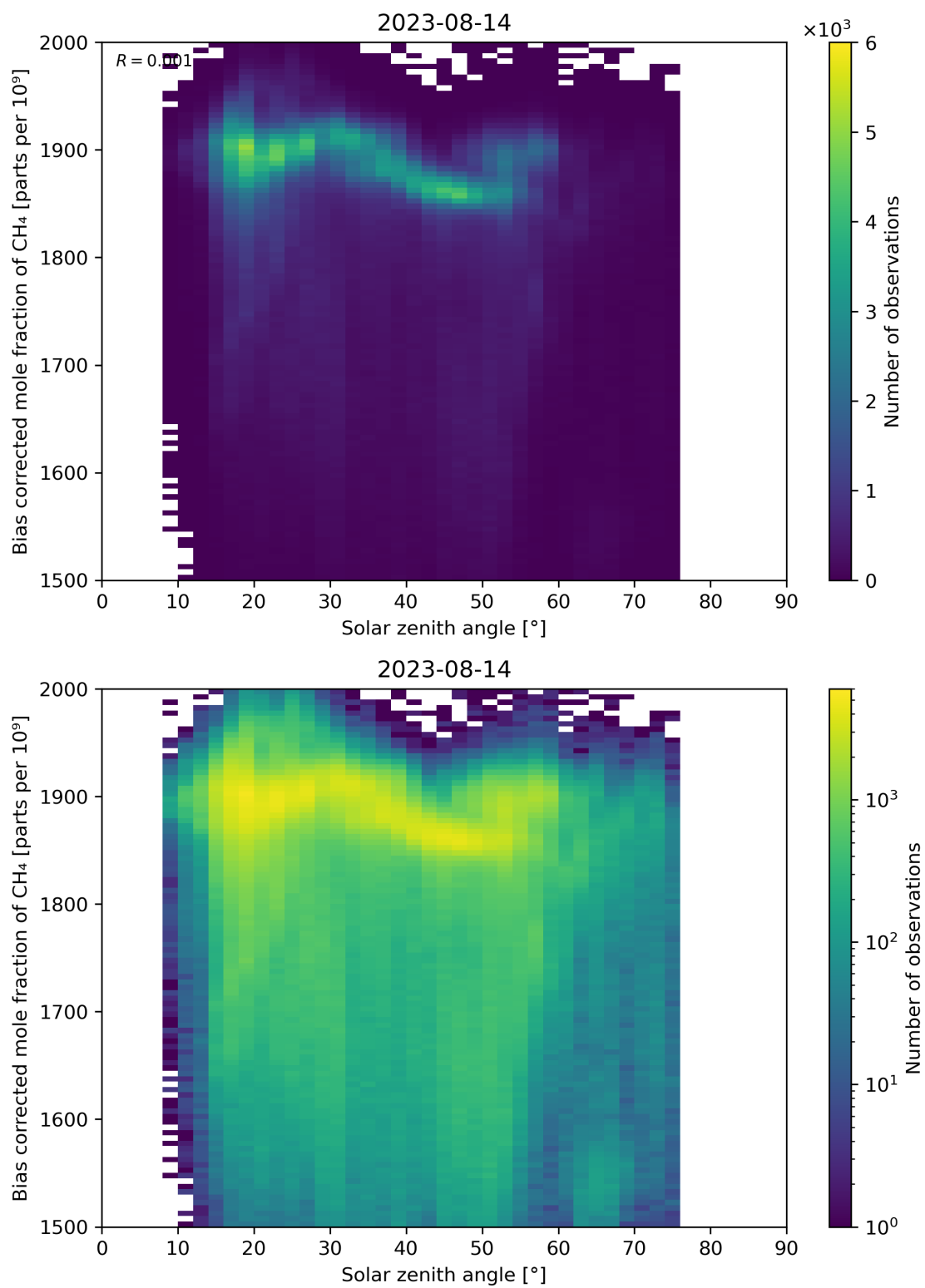
Figure 100: Scatter density plot of “Solar zenith angle” against “Bias corrected mole fraction of CH 4 ” for 2023-08-14 to 2023-08-15.
