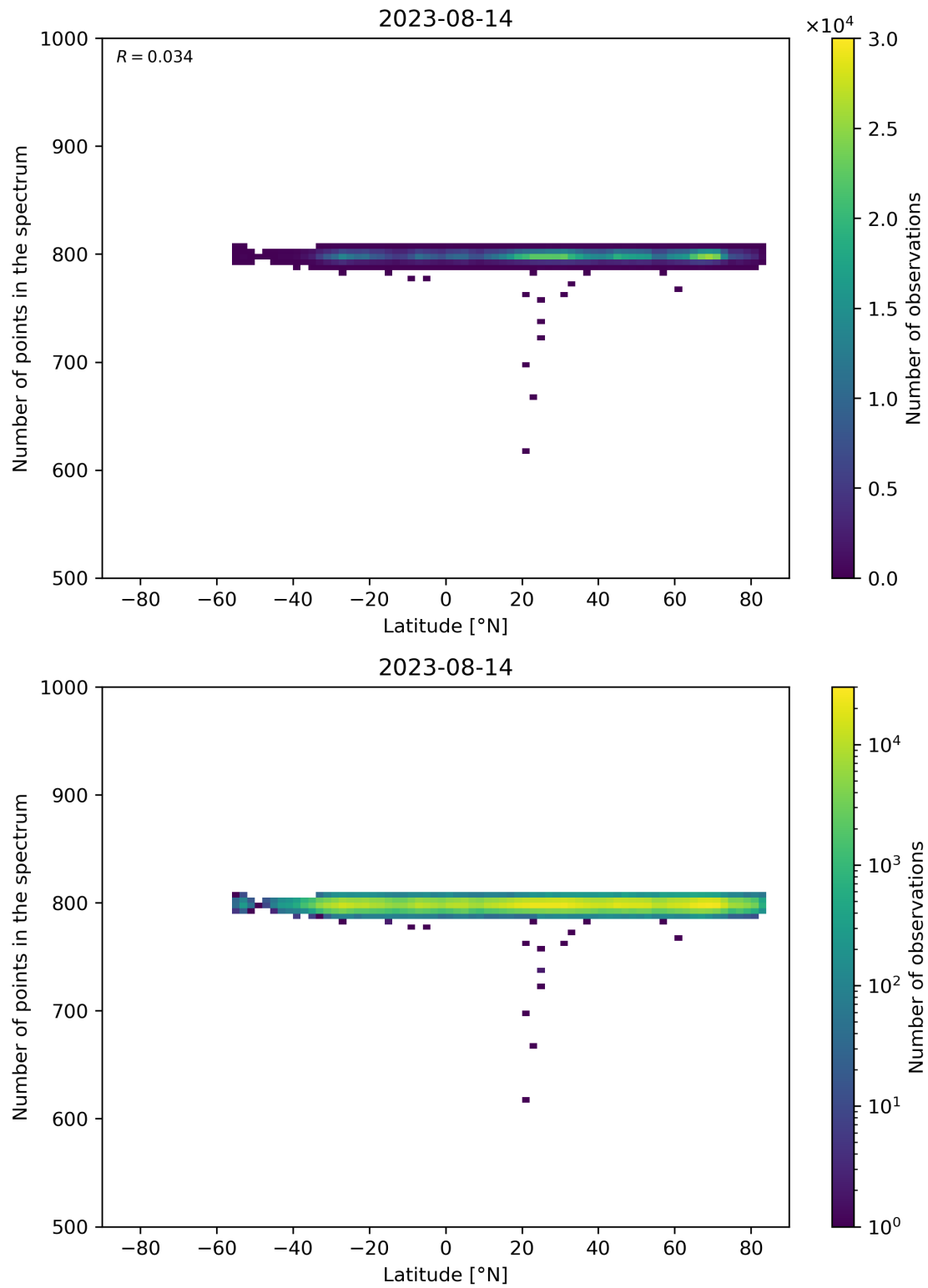
Figure 61: Scatter density plot of “Latitude” against “Number of points in the spectrum” for 2023-08-14 to 2023-08-15.
