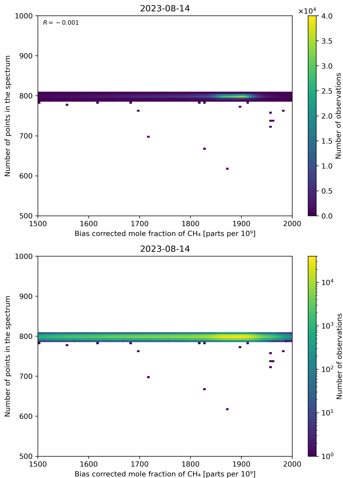
Figure 68: Scatter density plot of “Bias corrected mole fraction of CH 4 ” against “Number of points in the spectrum” for 2023-08-14 to 2023-08-15.
