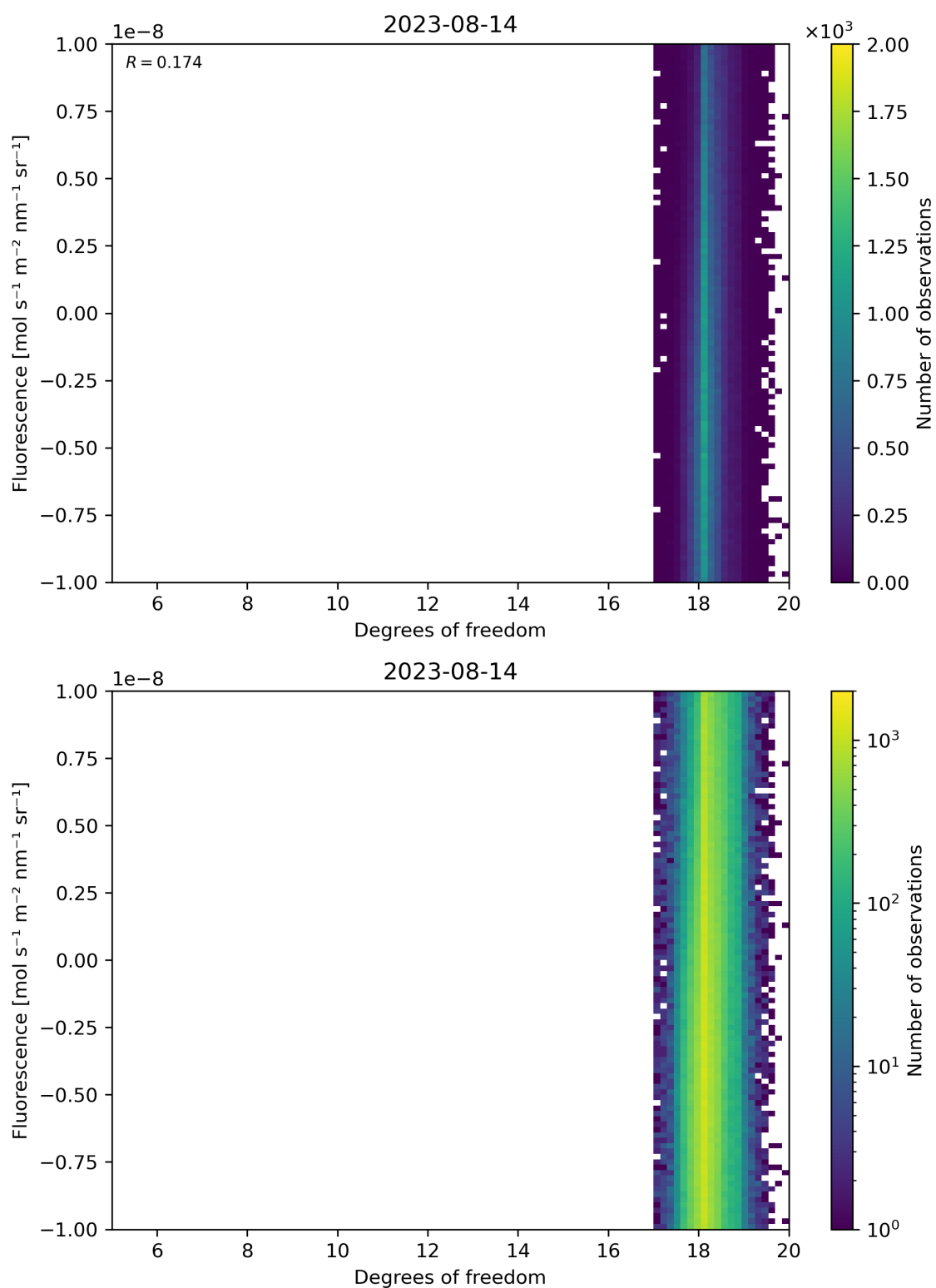
Figure 51: Scatter density plot of “Degrees of freedom” against “Fluorescence” for 2023-08-14 to 2023-08-15.
