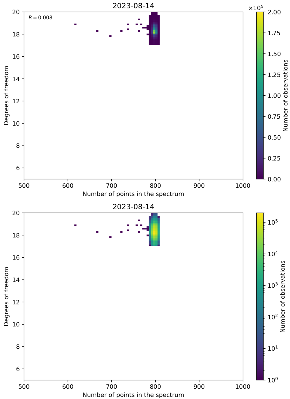
Figure 90: Scatter density plot of “Number of points in the spectrum” against “Degrees of freedom” for 2023-08-14 to 2023-08-15.
