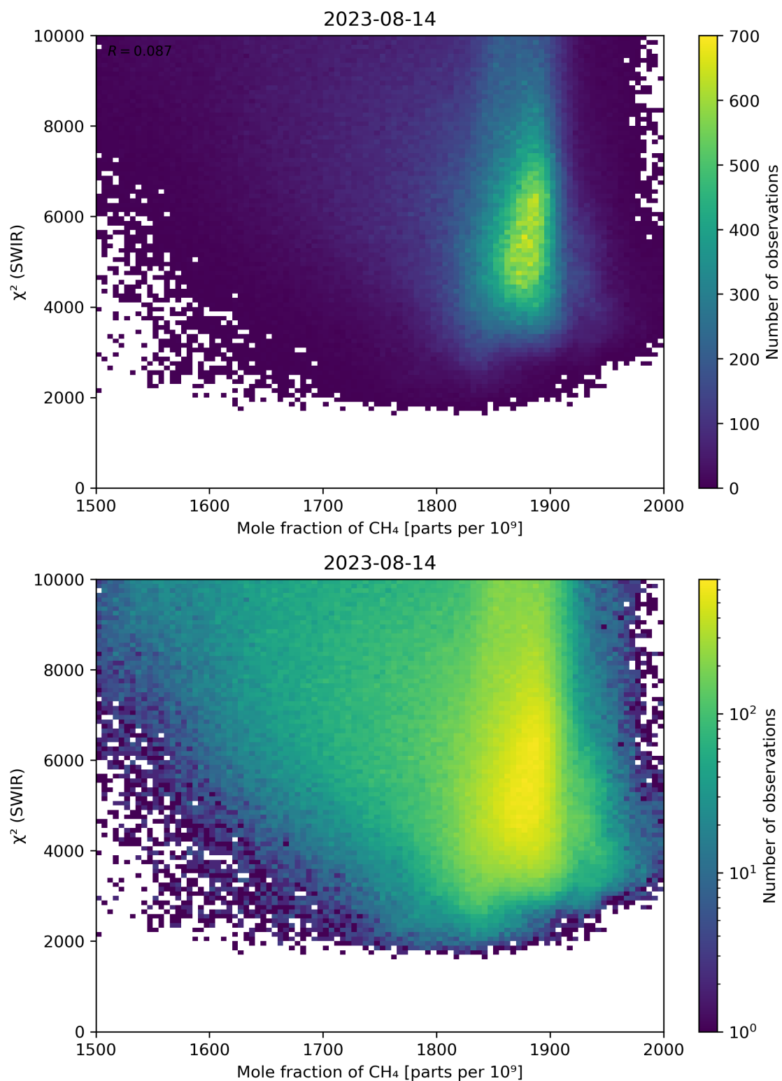
Figure 71: Scatter density plot of “Mole fraction of \text{CH}_4 ” against “ \chi^2 (SWIR)” for 2023-08-14 to 2023-08-15.
