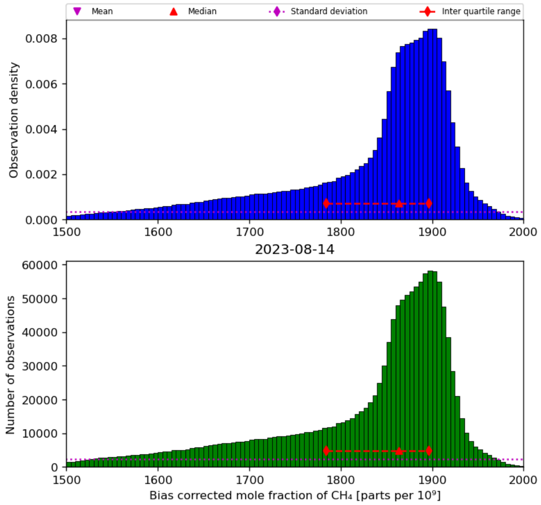
Figure 25: Histogram of “Bias corrected mole fraction of CH 4 ” for 2023-08-14 to 2023-08-15
