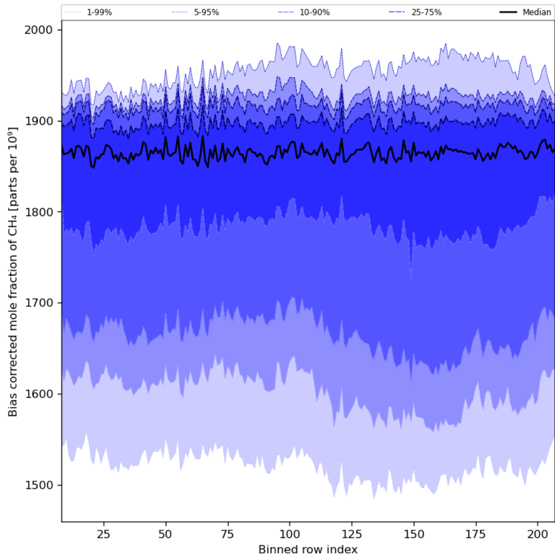
Figure 36: Along track statistics of “Bias corrected mole fraction of CH 4 ” for 2023-08-14 to 2023-08-15
