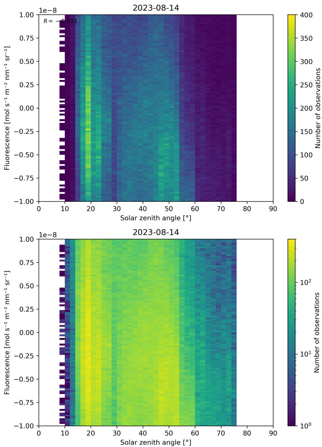
Figure 97: Scatter density plot of “Solar zenith angle” against “Fluorescence” for 2023-08-14 to 2023-08-15.
