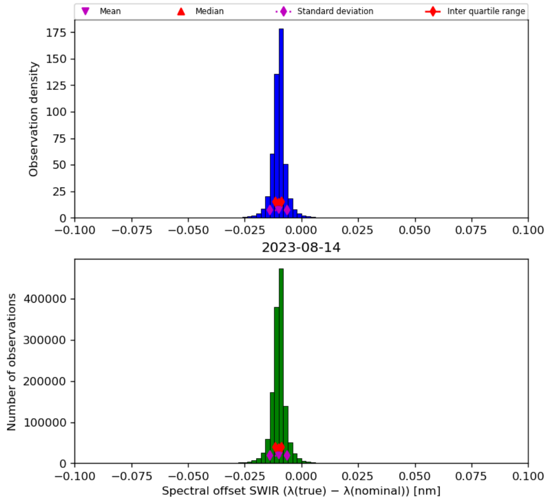
Figure 27: Histogram of “Spectral offset SWIR ( \lambda(\text{true}) - \lambda(\text{nominal}) )” for 2023-08-14 to 2023-08-15
