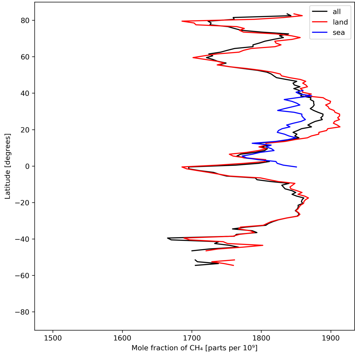
Figure 12: Zonal average of “Mole fraction of \text{CH}_4 ” for 2023-08-14 to 2023-08-15.
