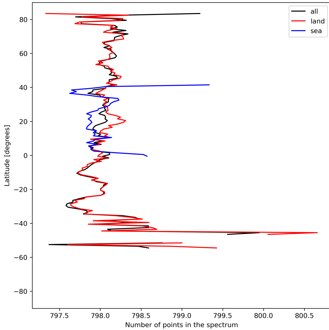
Figure 15: Zonal average of “Number of points in the spectrum” for 2023-08-14 to 2023-08-15.
