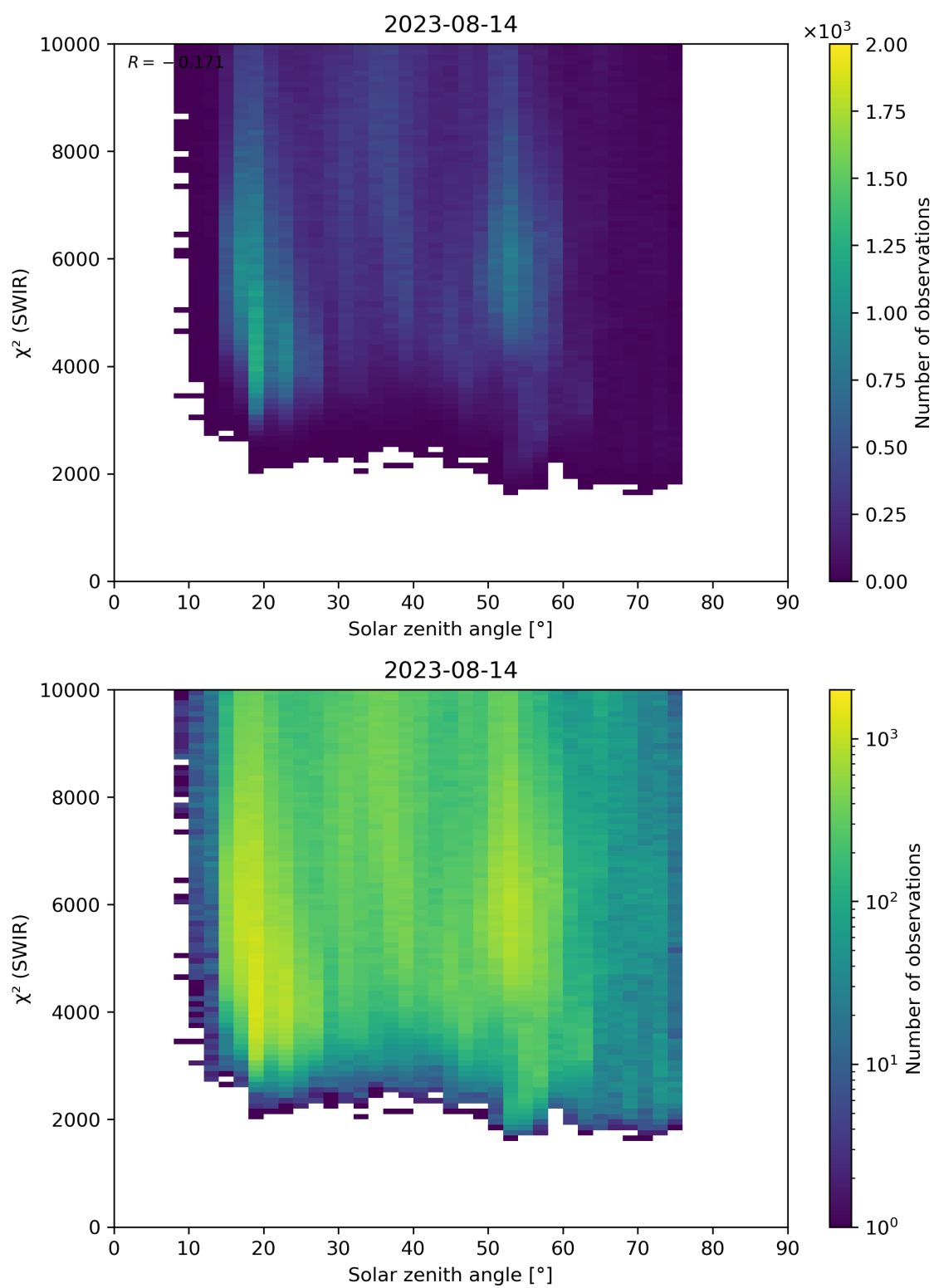
Figure 95: Scatter density plot of “Solar zenith angle” against “ \chi^2 (SWIR)” for 2023-08-14 to 2023-08-15.
