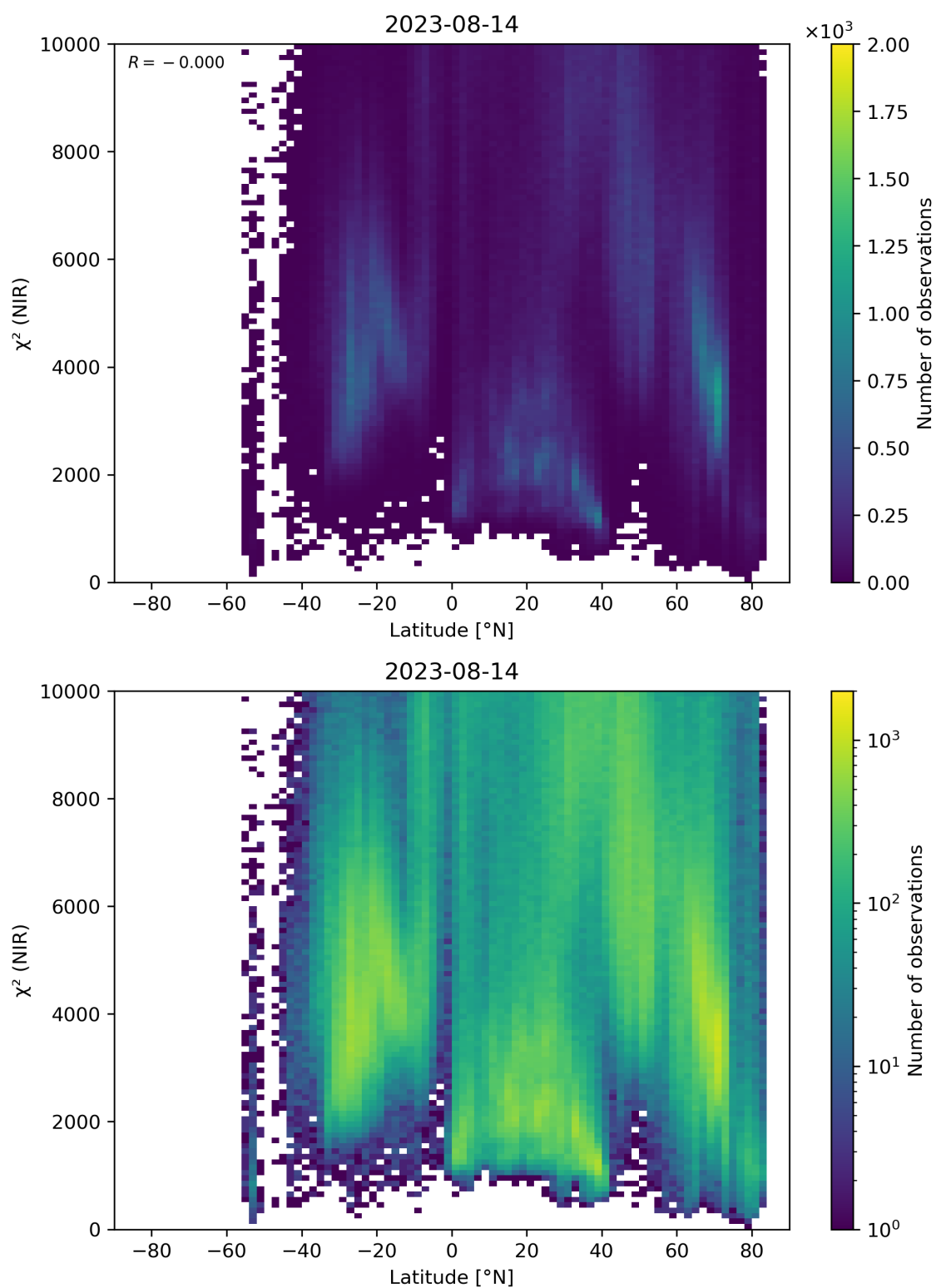
Figure 53: Scatter density plot of “Latitude” against “ \chi^2 (NIR)” for 2023-08-14 to 2023-08-15.
