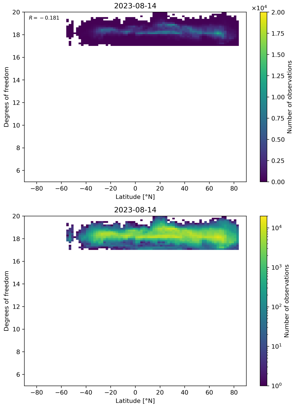
Figure 55: Scatter density plot of “Latitude” against “Degrees of freedom” for 2023-08-14 to 2023-08-15.
