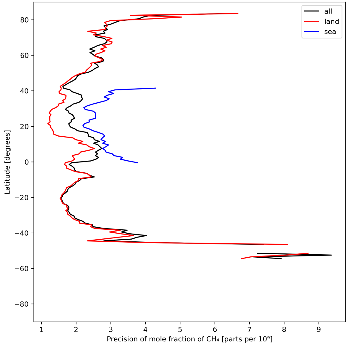
Figure 13: Zonal average of “Precision of mole fraction of CH 4 ” for 2023-08-14 to 2023-08-15.
