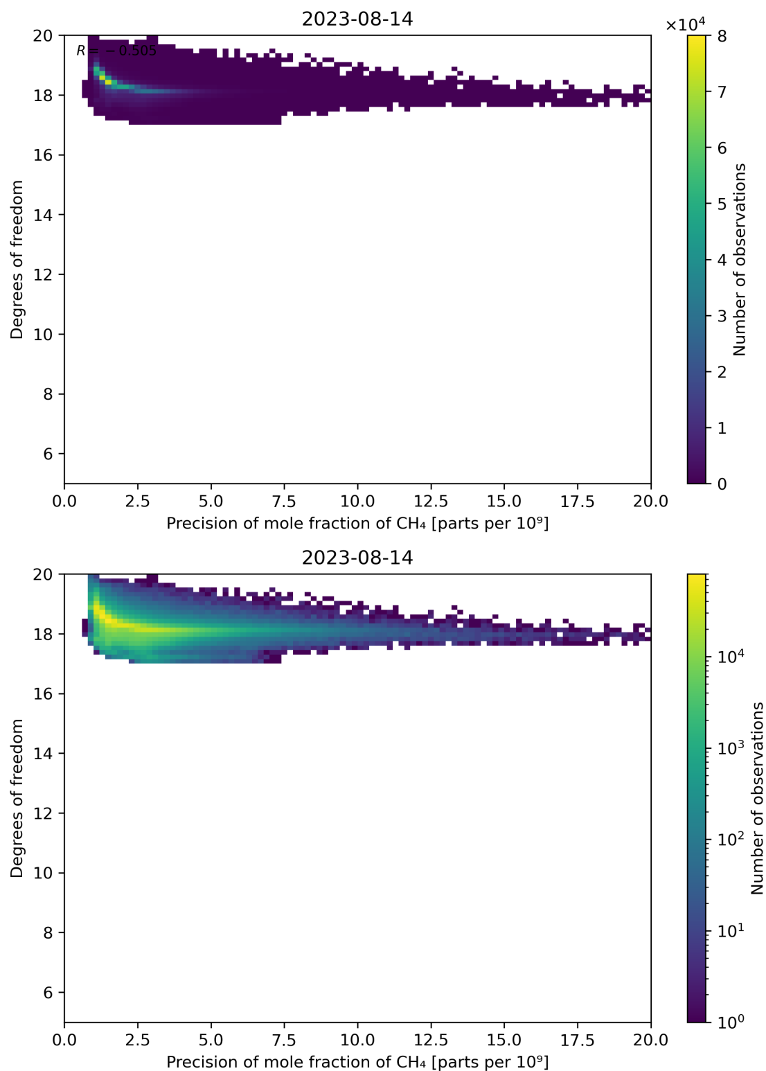
Figure 80: Scatter density plot of “Precision of mole fraction of CH 4 ” against “Degrees of freedom” for 2023-08-14 to 2023-08-15.
