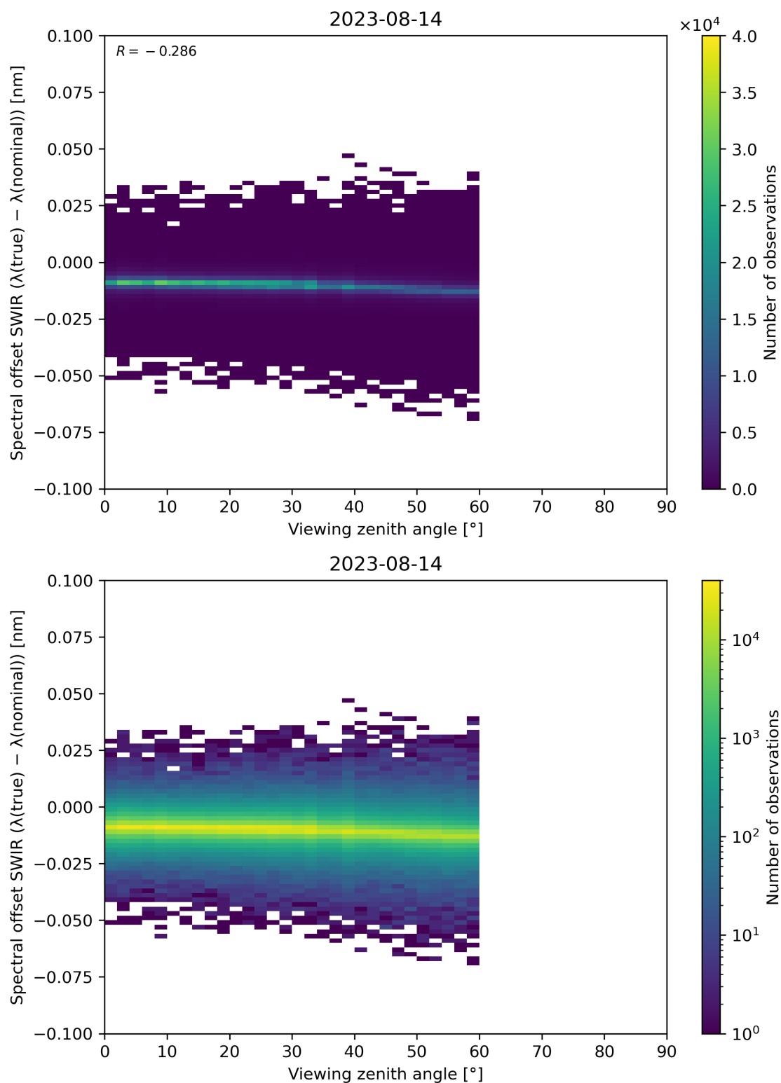
Figure 116: Scatter density plot of “Viewing zenith angle” against “Spectral offset SWIR ( \lambda(\text{true}) - \lambda(\text{nominal}) )” for 2023-08-14 to 2023-08-15.
