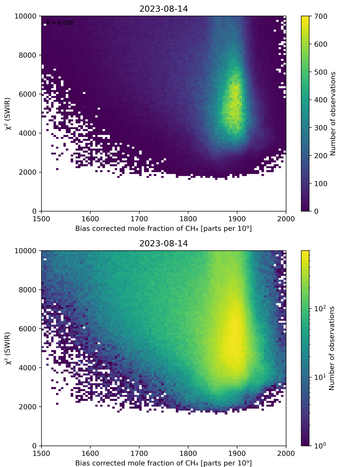
Figure 64: Scatter density plot of “Bias corrected mole fraction of \text{CH}_4 ” against “ \chi^2 (SWIR)” for 2023-08-14 to 2023-08-15.
