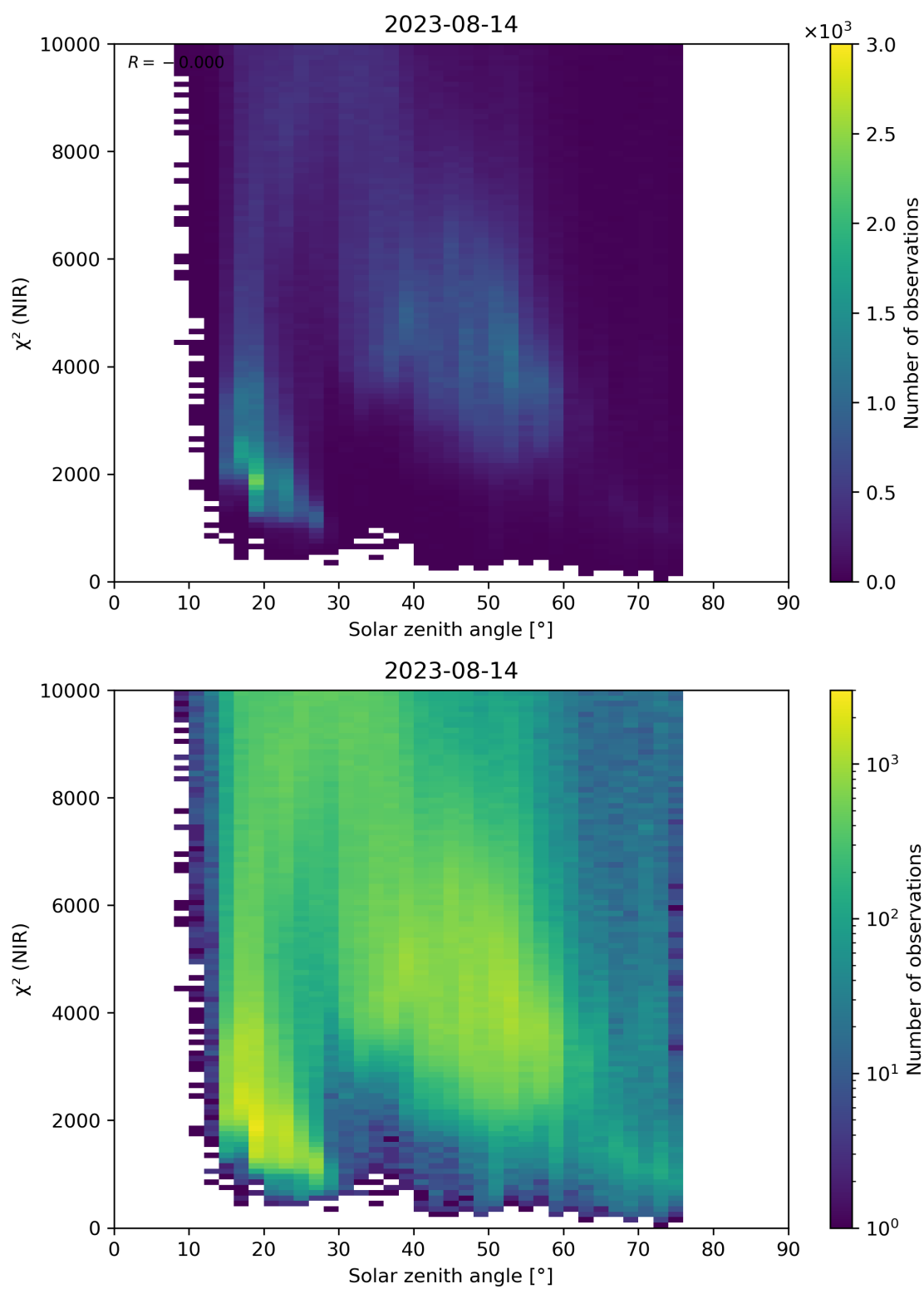
Figure 94: Scatter density plot of “Solar zenith angle” against “ \chi^2 (NIR)” for 2023-08-14 to 2023-08-15.
