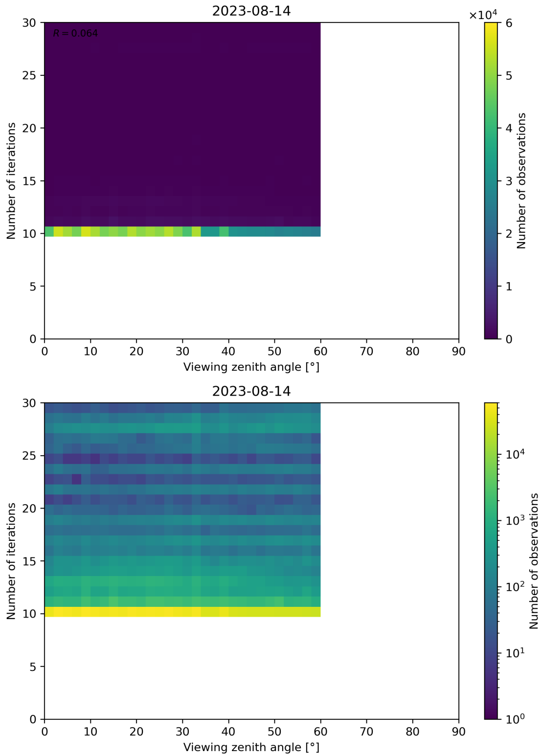
Figure 113: Scatter density plot of “Viewing zenith angle” against “Number of iterations” for 2023-08-14 to 2023-08-15.
