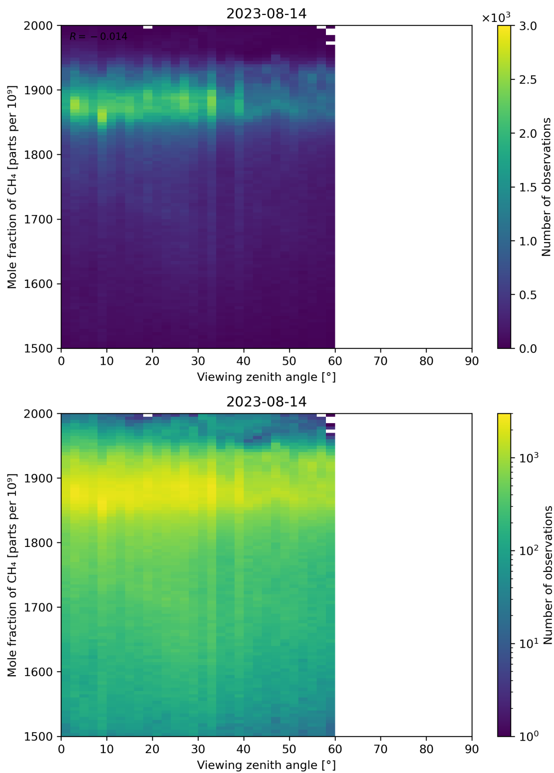
Figure 110: Scatter density plot of “Viewing zenith angle” against “Mole fraction of CH 4 ” for 2023-08-14 to 2023-08-15.
