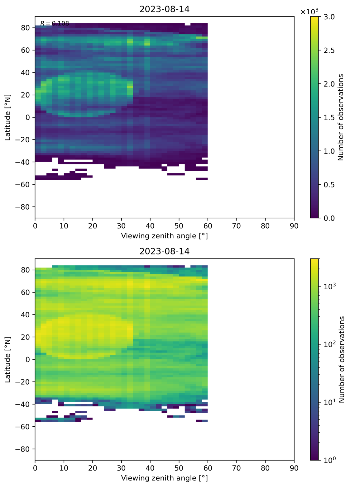
Figure 109: Scatter density plot of “Viewing zenith angle” against “Latitude” for 2023-08-14 to 2023-08-15.
