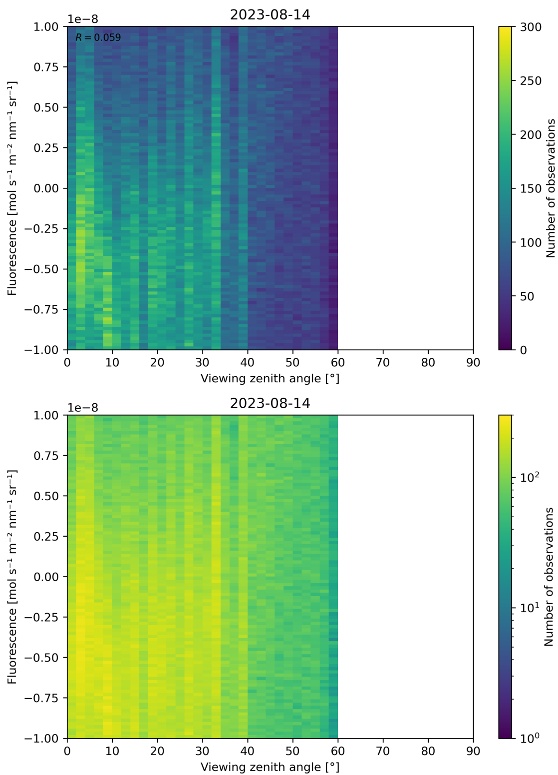
Figure 108: Scatter density plot of “Viewing zenith angle” against “Fluorescence” for 2023-08-14 to 2023-08-15.
