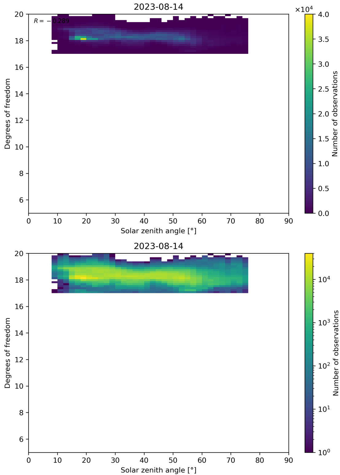
Figure 96: Scatter density plot of “Solar zenith angle” against “Degrees of freedom” for 2023-08-14 to 2023-08-15.
