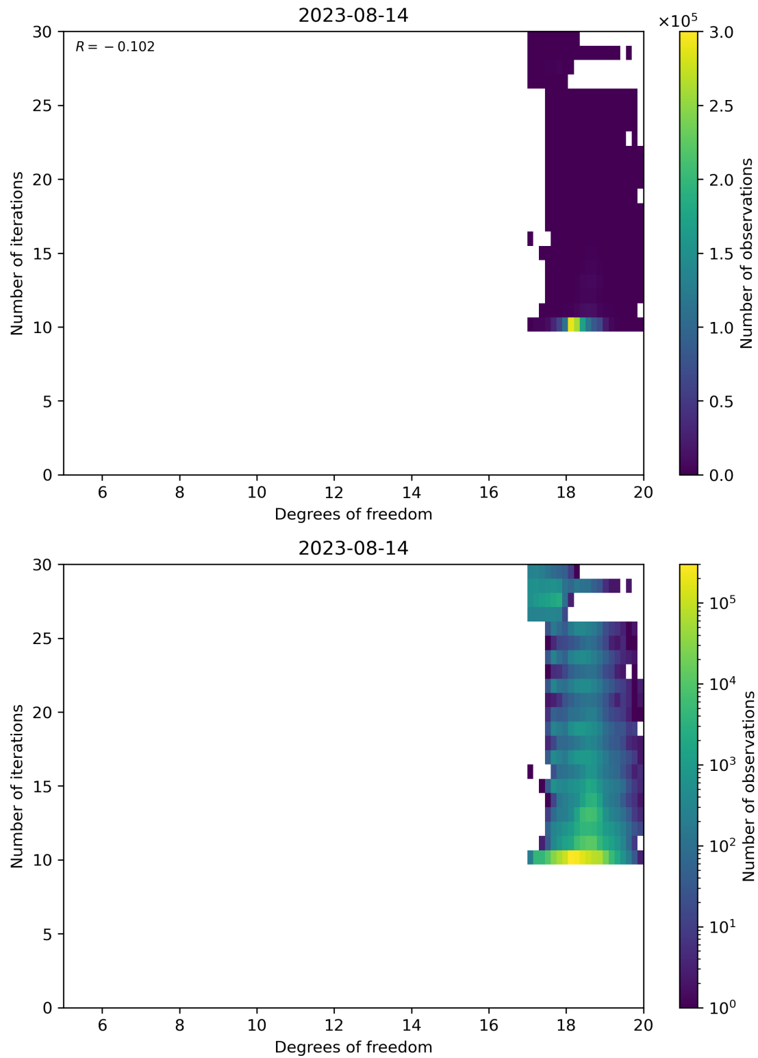
Figure 52: Scatter density plot of “Degrees of freedom” against “Number of iterations” for 2023-08-14 to 2023-08-15.
