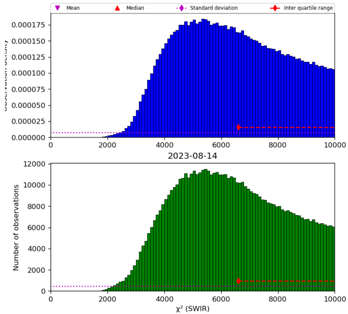
Figure 28: Histogram of “ \chi^2 (SWIR)” for 2023-08-14 to 2023-08-15
