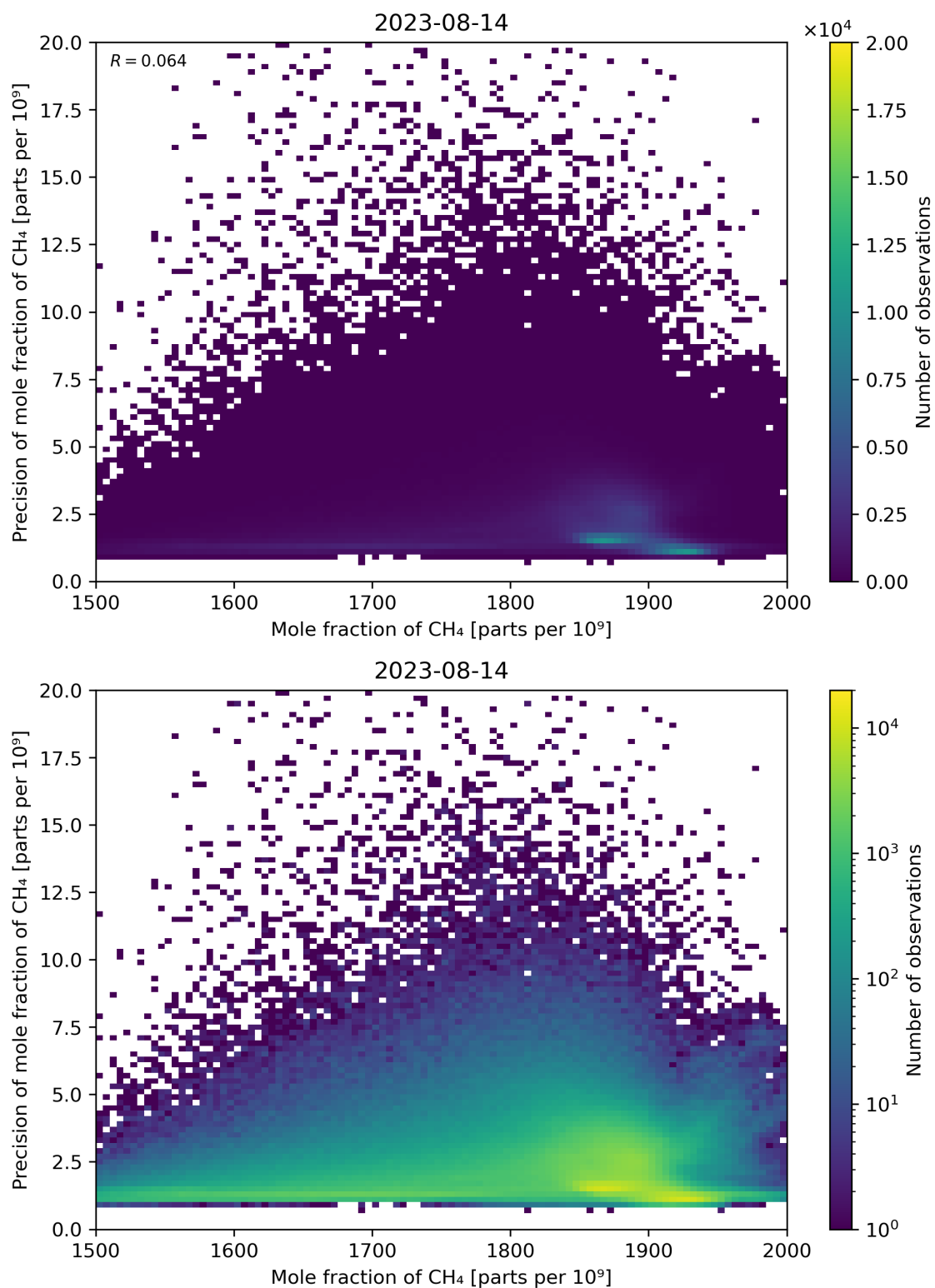
Figure 75: Scatter density plot of “Mole fraction of CH 4 ” against “Precision of mole fraction of CH 4 ” for 2023-08-14 to 2023-08-15.
