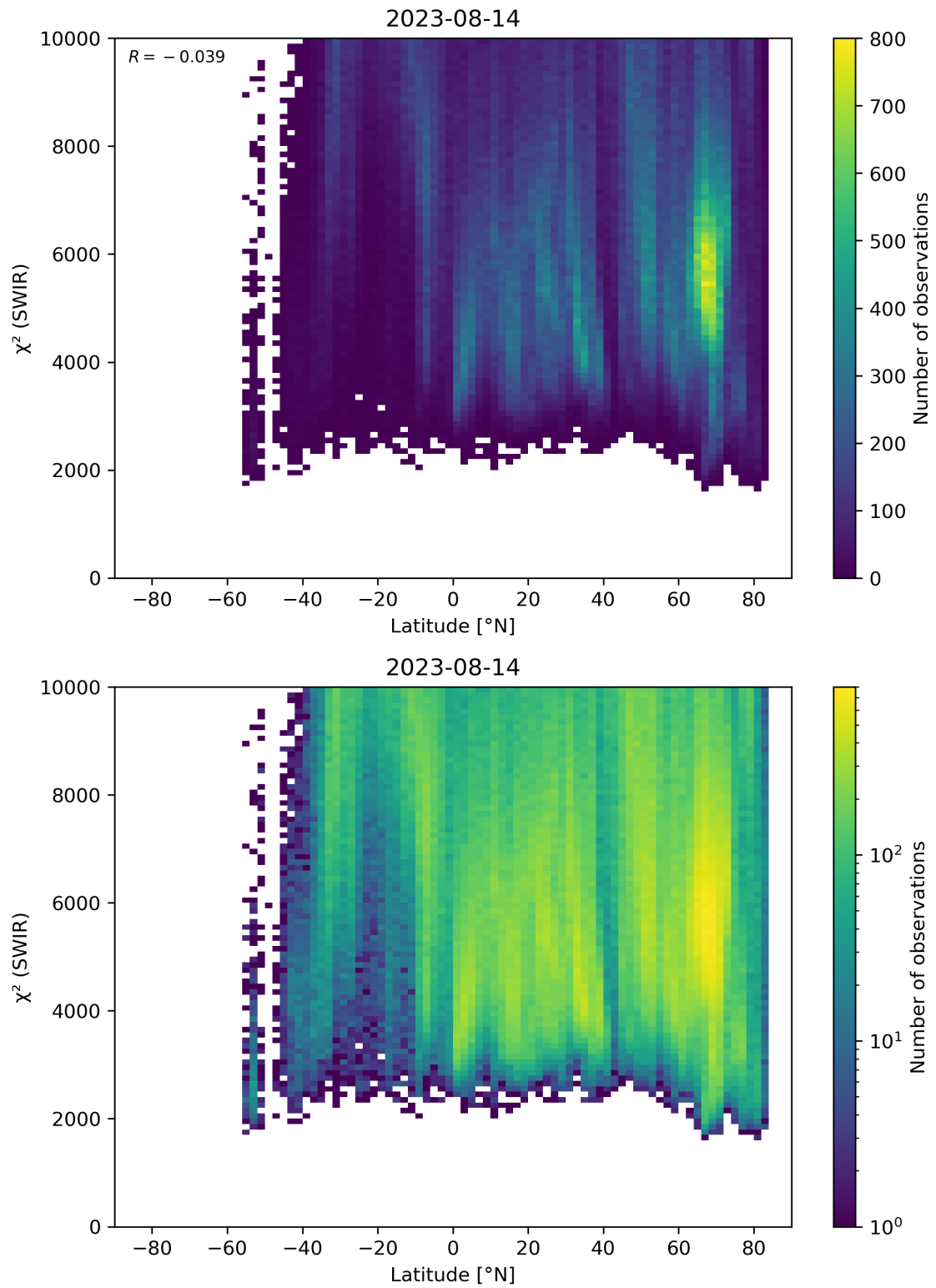
Figure 54: Scatter density plot of “Latitude” against “ \chi^2 (SWIR)” for 2023-08-14 to 2023-08-15.
