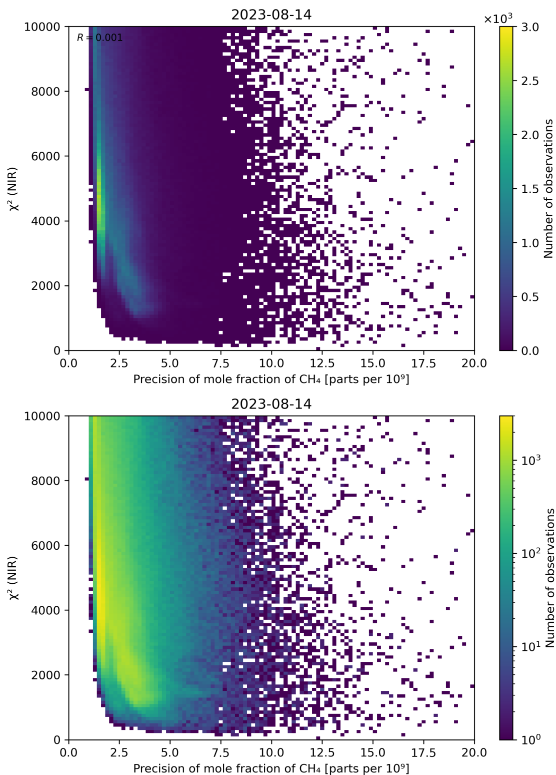
Figure 78: Scatter density plot of “Precision of mole fraction of \text{CH}_4 ” against “ \chi^2 (NIR)” for 2023-08-14 to 2023-08-15.
