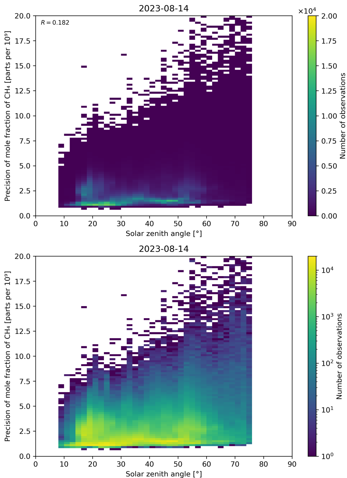
Figure 101: Scatter density plot of “Solar zenith angle” against “Precision of mole fraction of \text{CH}_4 ” for 2023-08-14 to 2023-08-15.
