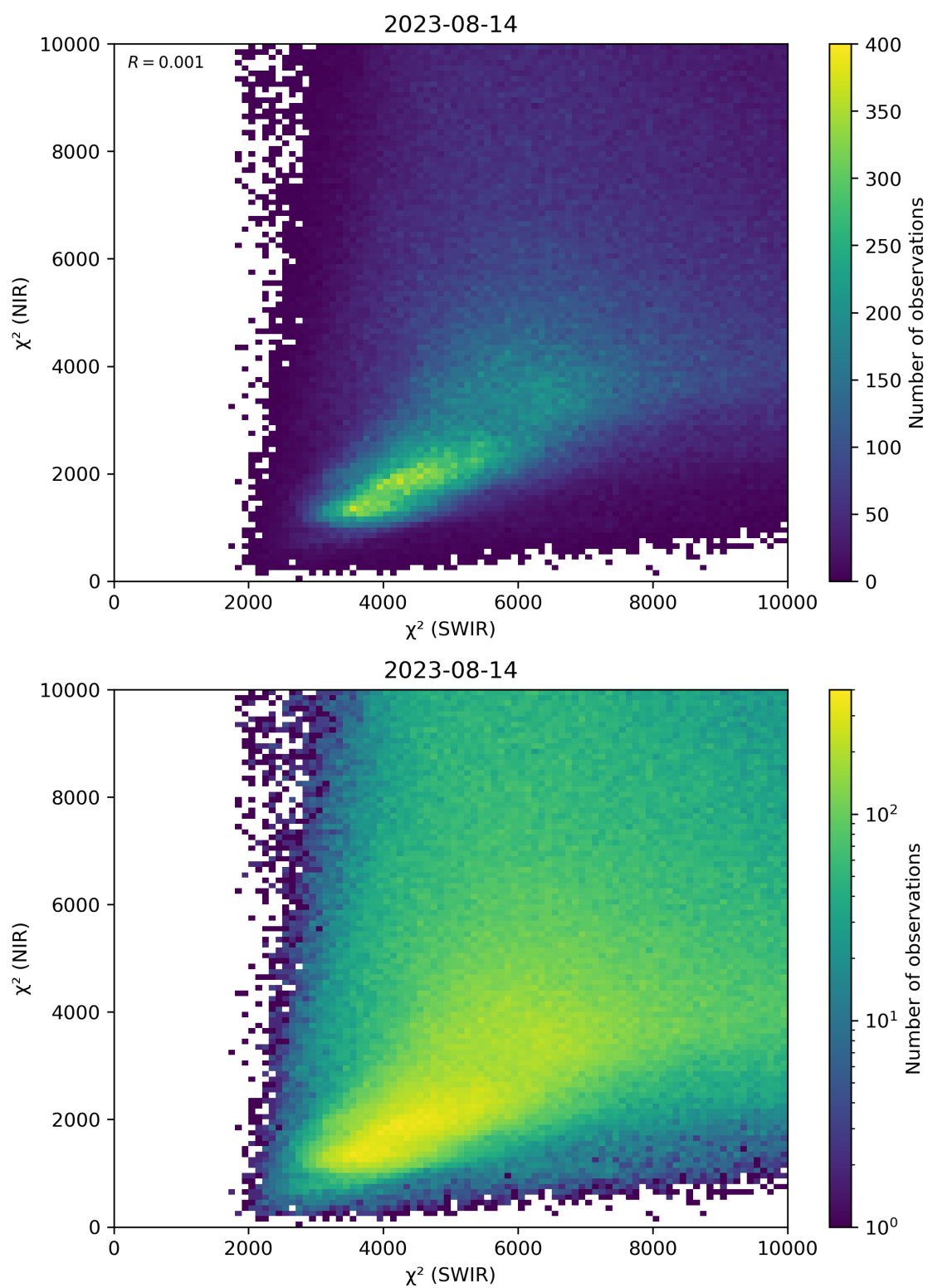
Figure 47: Scatter density plot of “ \chi^2 (SWIR)” against “ \chi^2 (NIR)” for 2023-08-14 to 2023-08-15.
