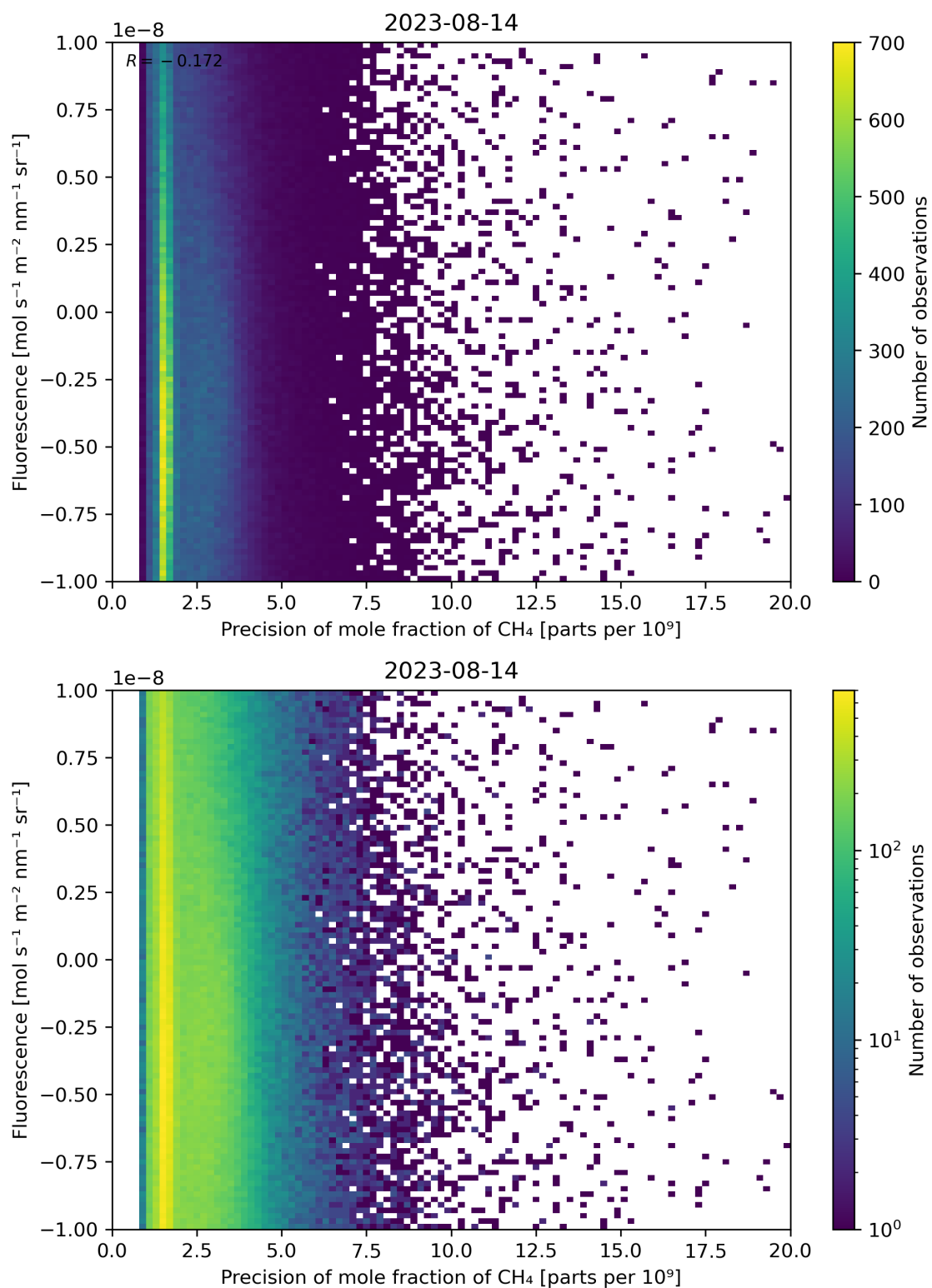
Figure 81: Scatter density plot of “Precision of mole fraction of \text{CH}_4 ” against “Fluorescence” for 2023-08-14 to 2023-08-15.
