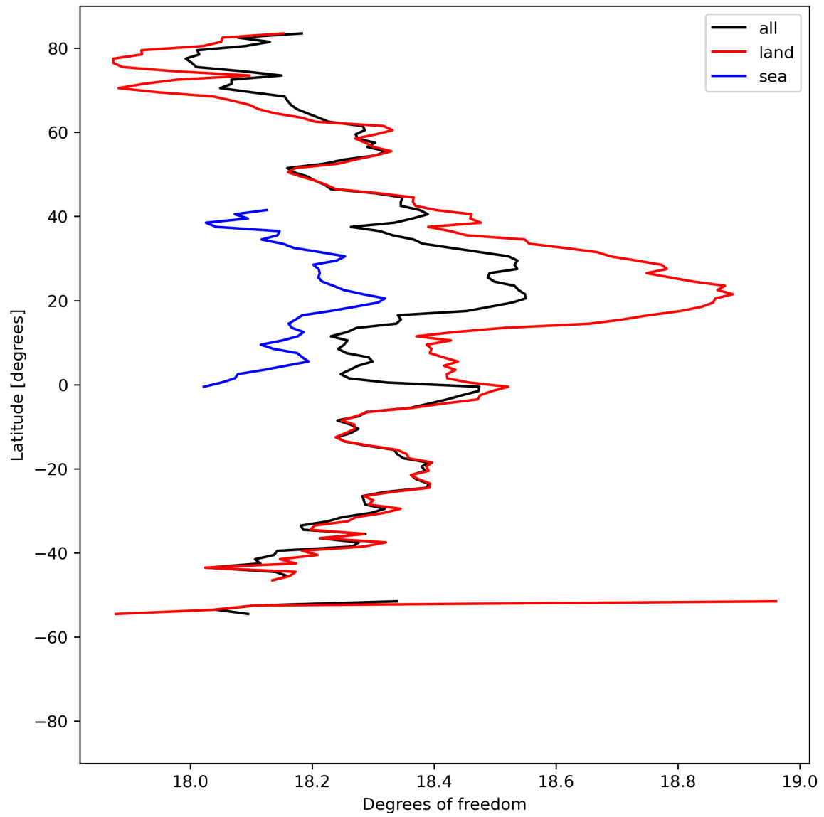
Figure 19: Zonal average of “Degrees of freedom” for 2023-08-14 to 2023-08-15.
