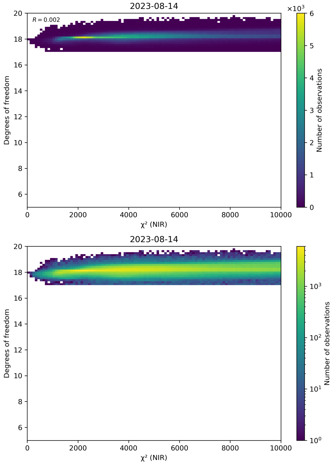
Figure 44: Scatter density plot of “ \chi^2 (NIR)” against “Degrees of freedom” for 2023-08-14 to 2023-08-15.
