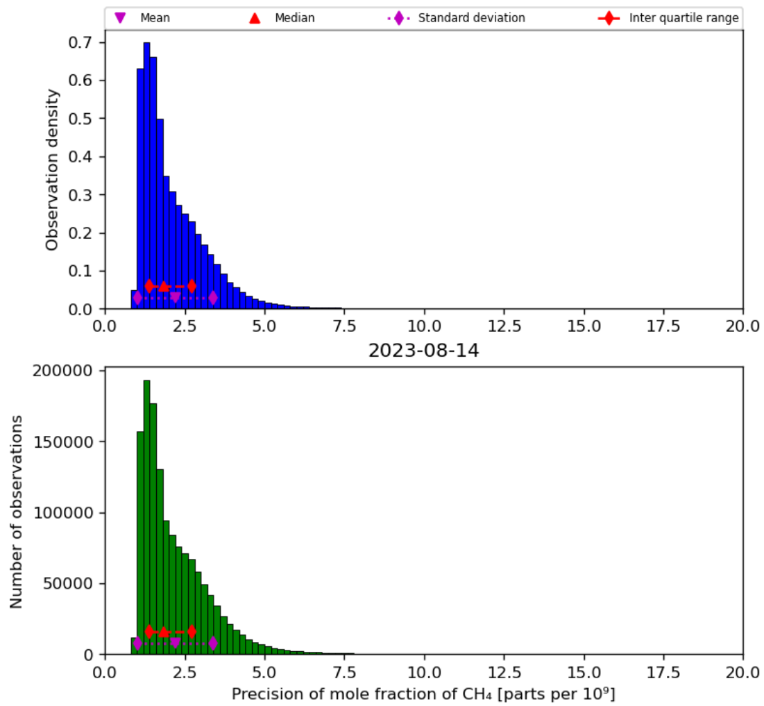
Figure 24: Histogram of “Precision of mole fraction of CH 4 ” for 2023-08-14 to 2023-08-15
