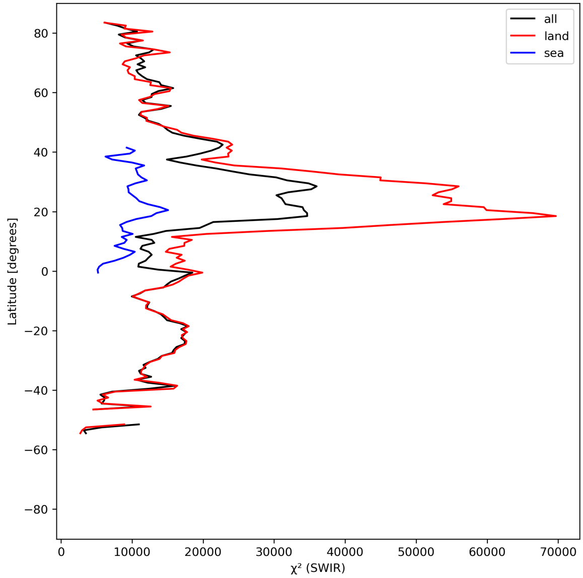
Figure 17: Zonal average of “ \chi^2 (SWIR)” for 2023-08-14 to 2023-08-15.
