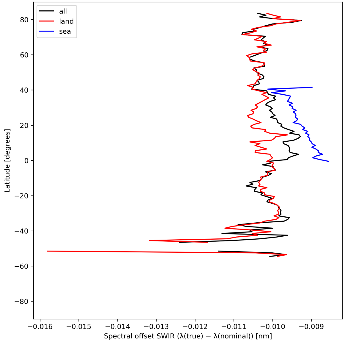
Figure 16: Zonal average of “Spectral offset SWIR ( \lambda(\text{true}) - \lambda(\text{nominal}) )” for 2023-08-14 to 2023-08-15.
