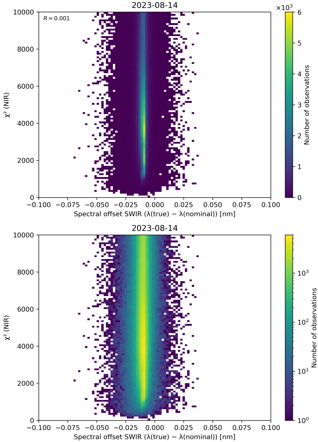
Figure 117: Scatter density plot of “Spectral offset SWIR ( \lambda(\text{true}) - \lambda(\text{nominal}) )” against “ \chi^2 (NIR)” for 2023-08-14 to 2023-08-15.
