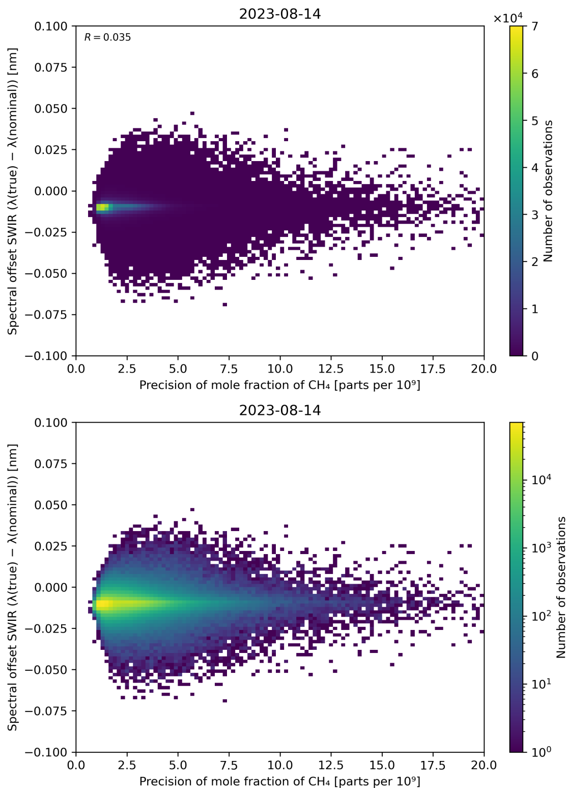
Figure 85: Scatter density plot of “Precision of mole fraction of \text{CH}_4 ” against “Spectral offset SWIR ( \lambda(\text{true}) - \lambda(\text{nominal}) )” for 2023-08-14 to 2023-08-15.
