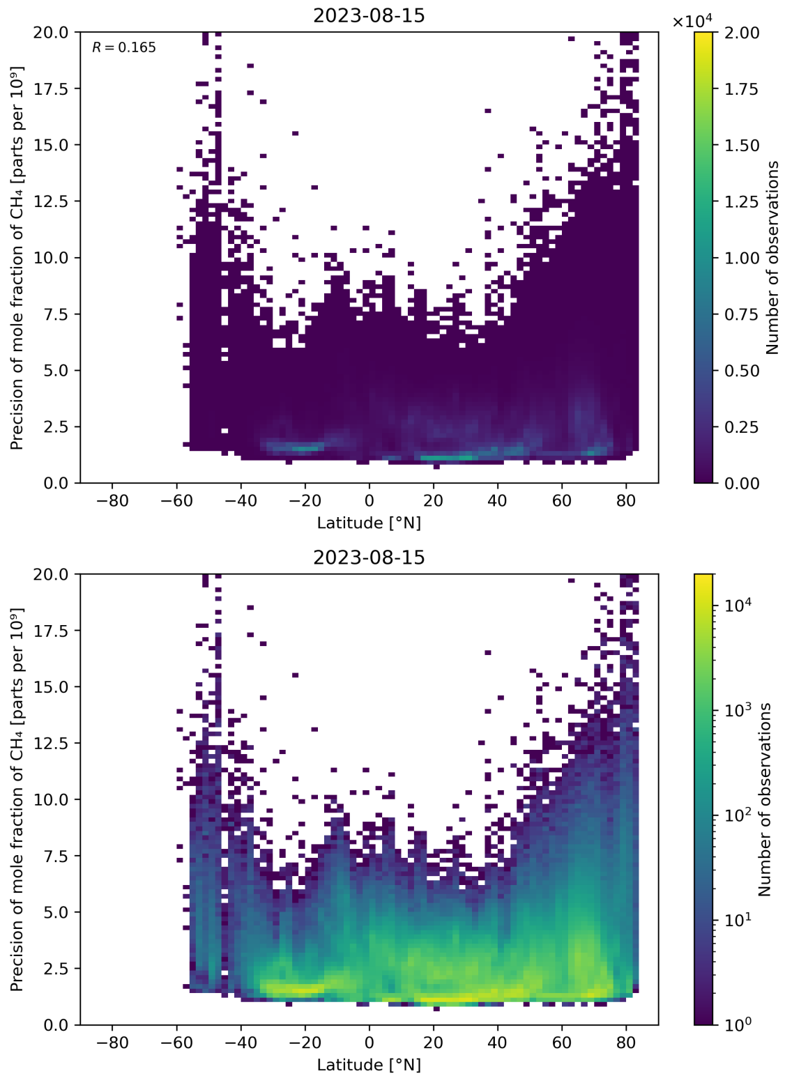
Figure 59: Scatter density plot of “Latitude” against “Precision of mole fraction of CH 4 ” for 2023-08-14 to 2023-08-16.
