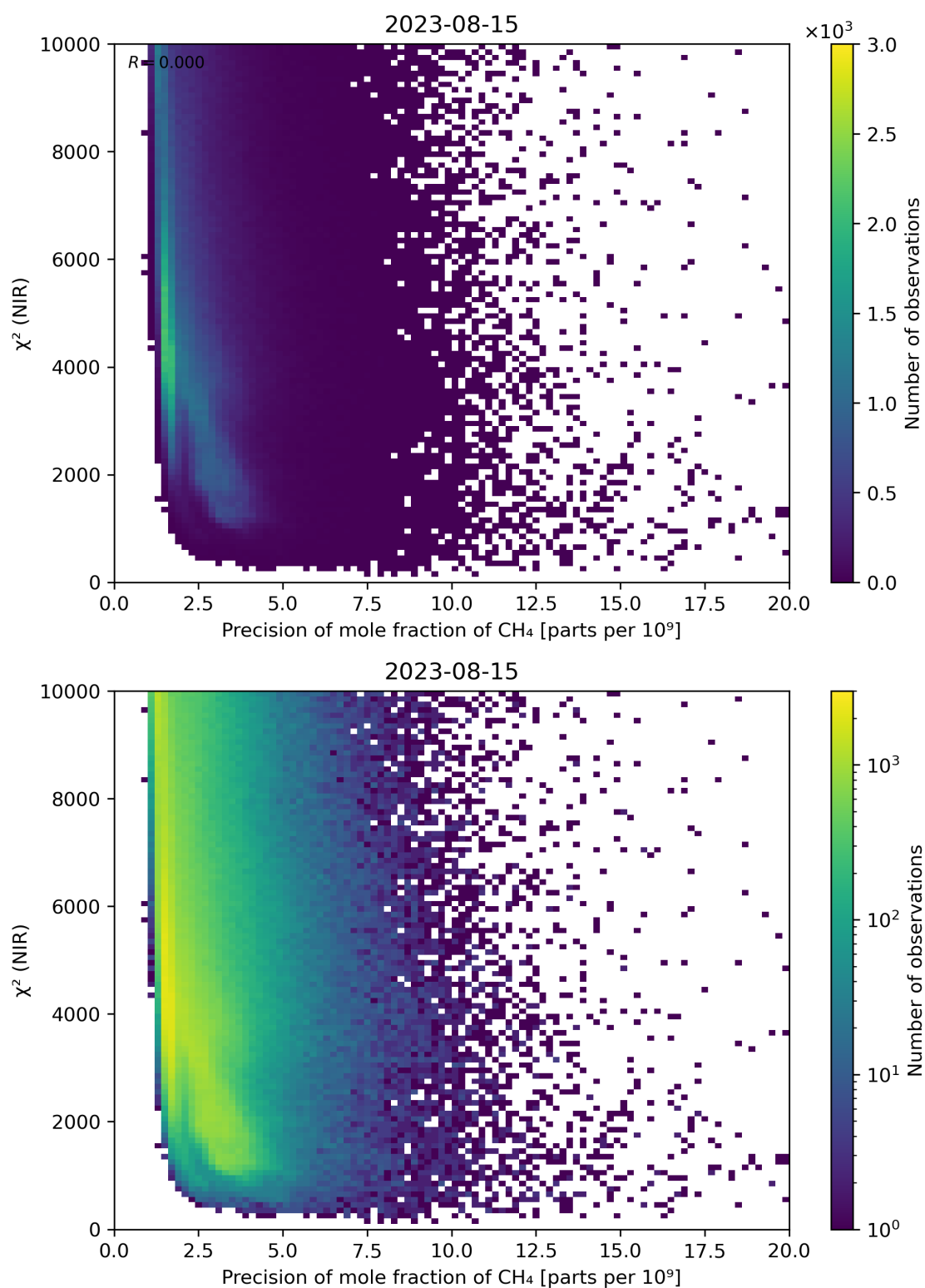
Figure 78: Scatter density plot of “Precision of mole fraction of CH 4 ” against “ \chi^2 (NIR)” for 2023-08-14 to 2023-08-16.
