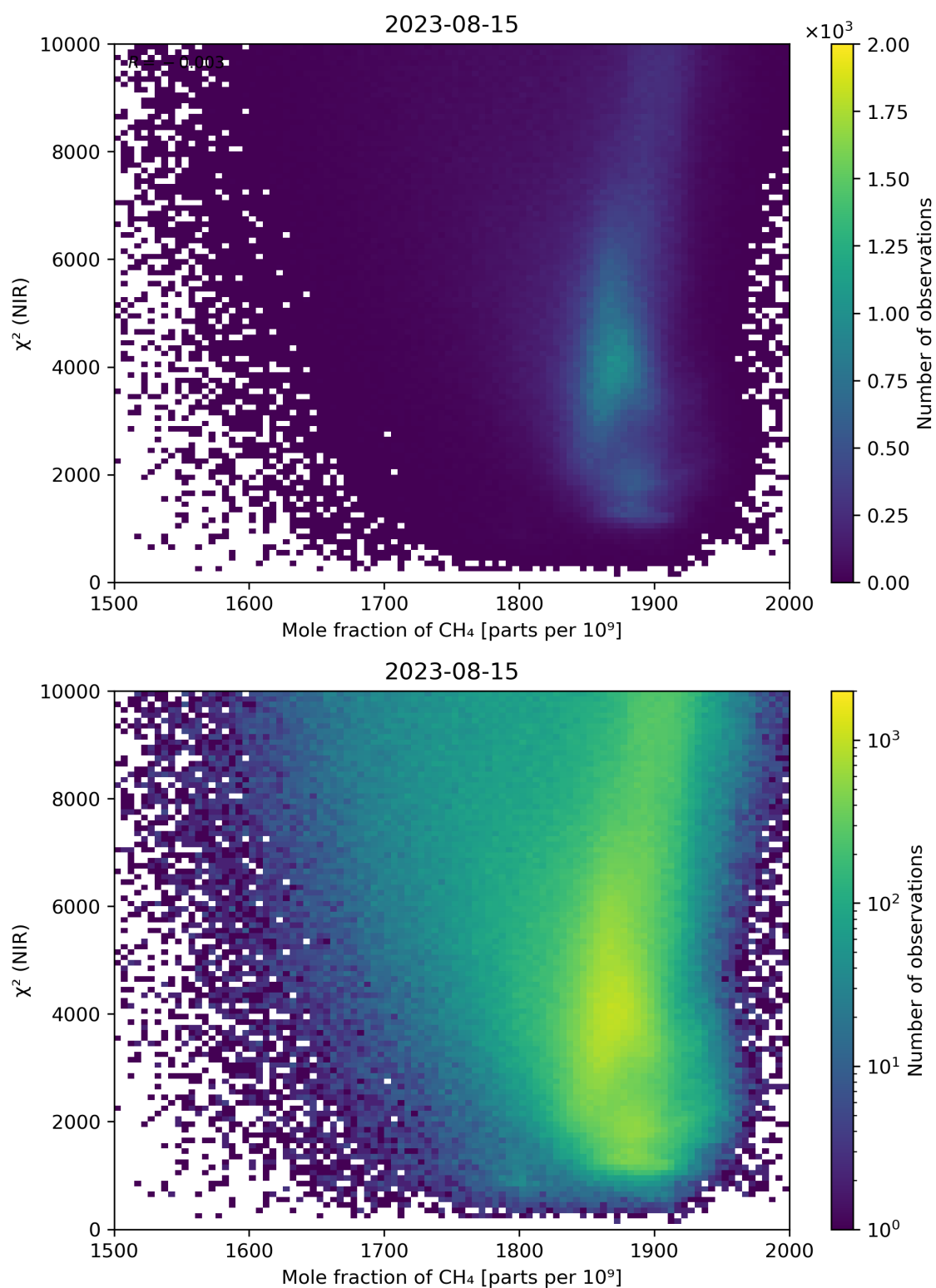
Figure 70: Scatter density plot of “Mole fraction of CH 4 ” against “ \chi^2 (NIR)” for 2023-08-14 to 2023-08-16.
