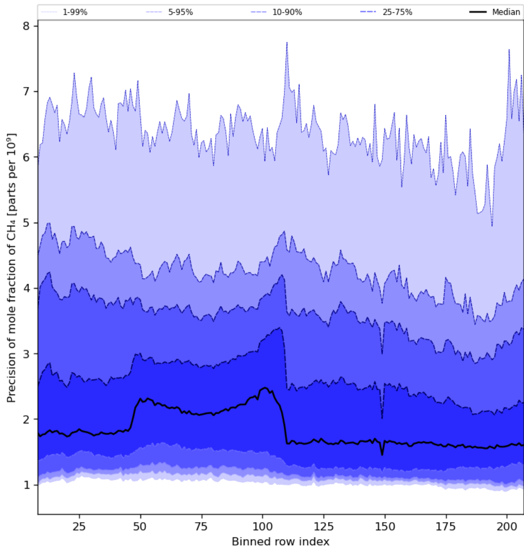
Figure 35: Along track statistics of “Precision of mole fraction of CH 4 ” for 2023-08-14 to 2023-08-16
