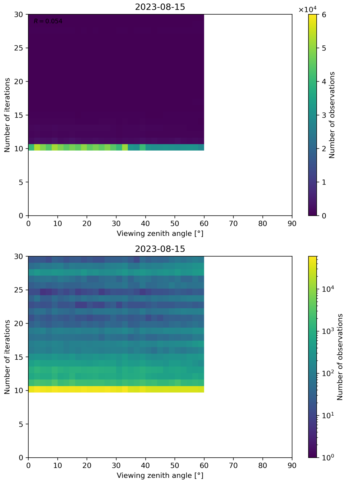
Figure 113: Scatter density plot of “Viewing zenith angle” against “Number of iterations” for 2023-08-14 to 2023-08-16.
