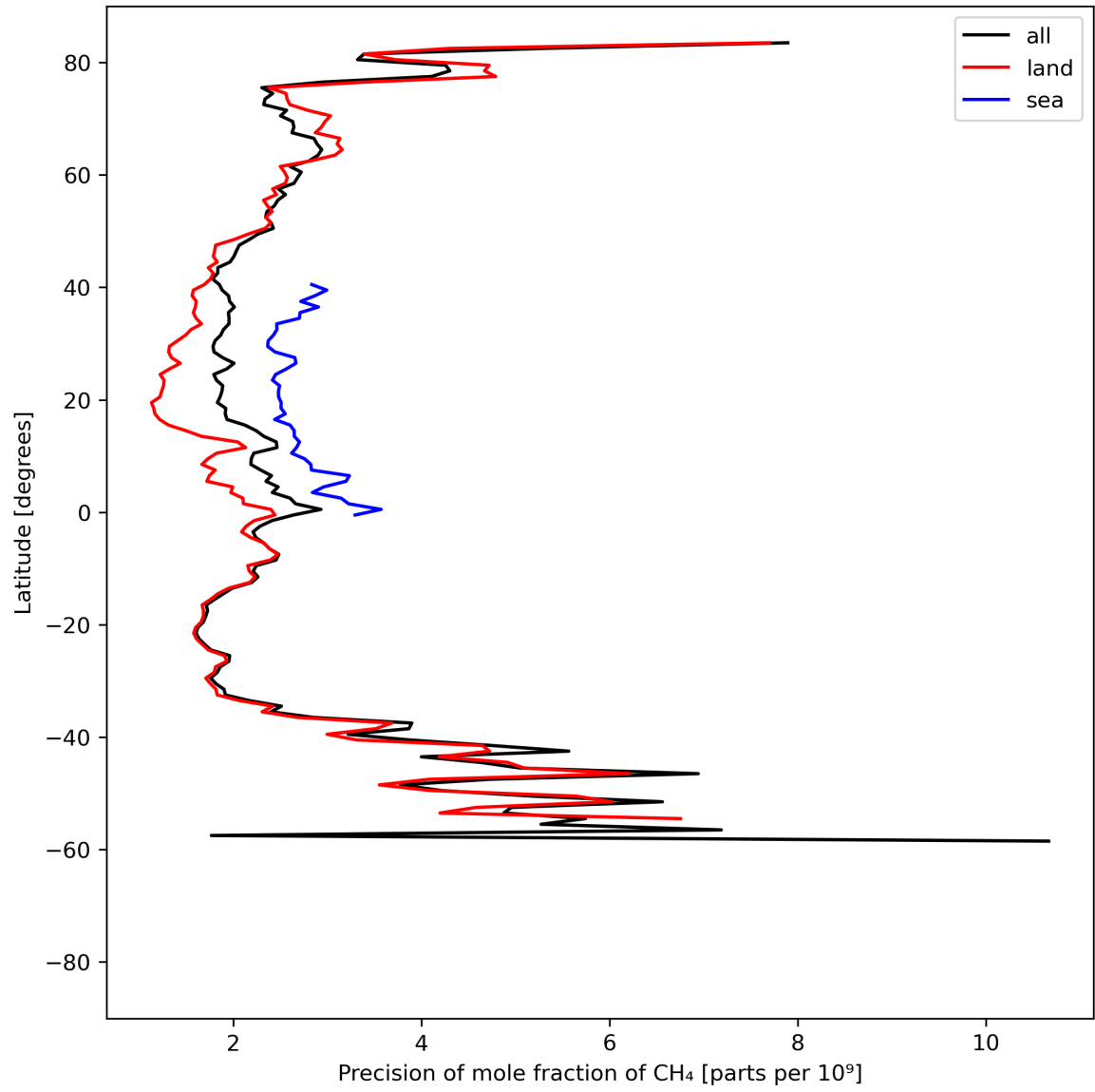
Figure 13: Zonal average of “Precision of mole fraction of CH 4 ” for 2023-08-14 to 2023-08-16.
