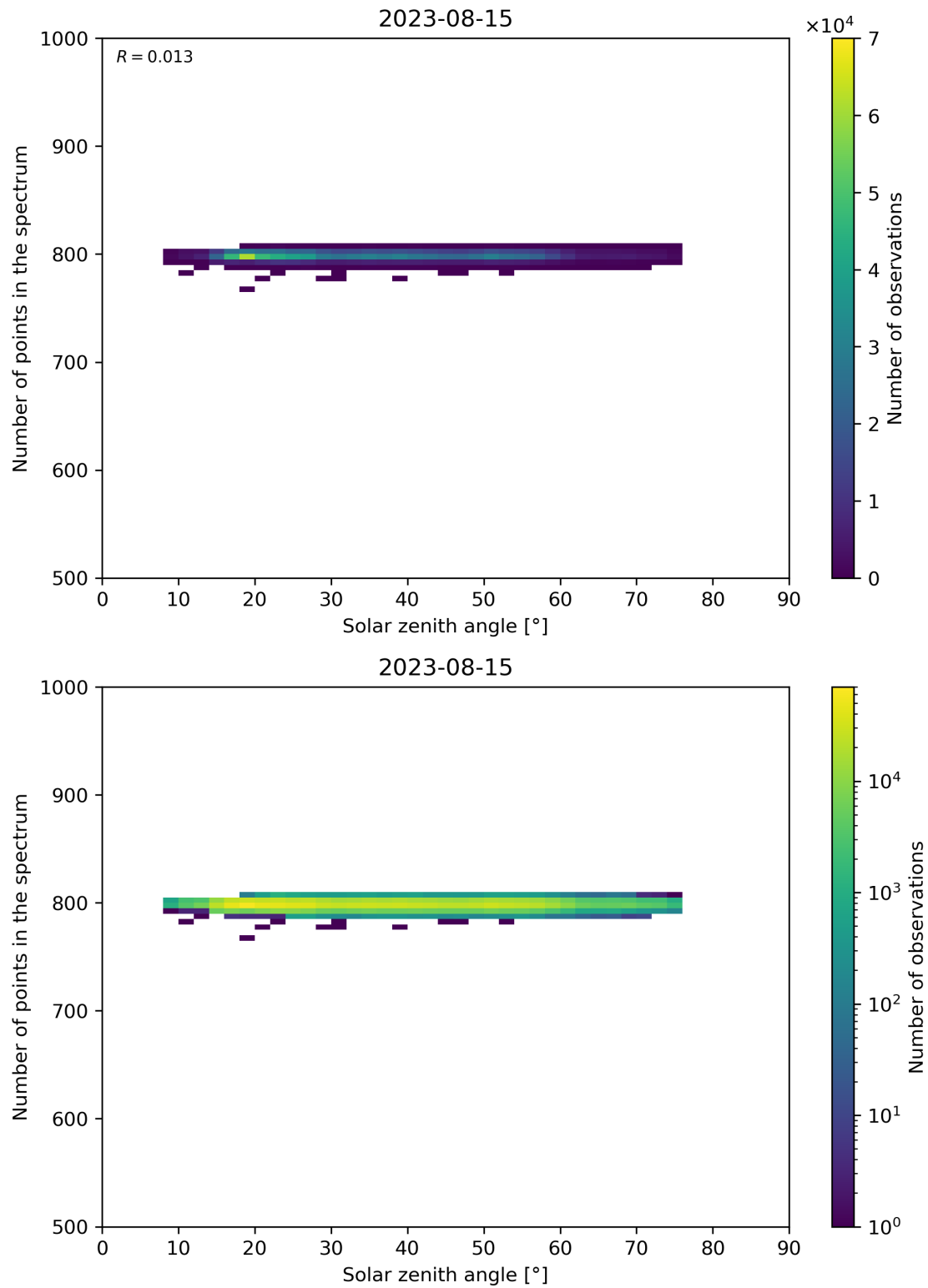
Figure 103: Scatter density plot of “Solar zenith angle” against “Number of points in the spectrum” for 2023-08-14 to 2023-08-16.
