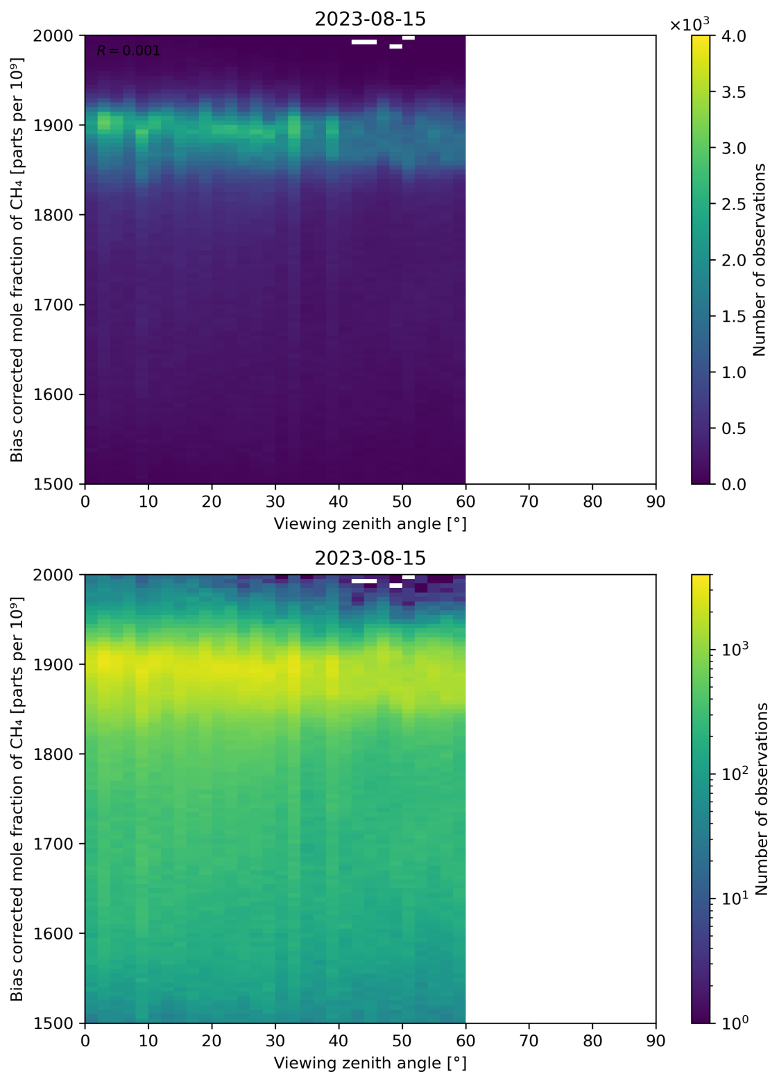
Figure 111: Scatter density plot of “Viewing zenith angle” against “Bias corrected mole fraction of CH 4 ” for 2023-08-14 to 2023-08-16.
