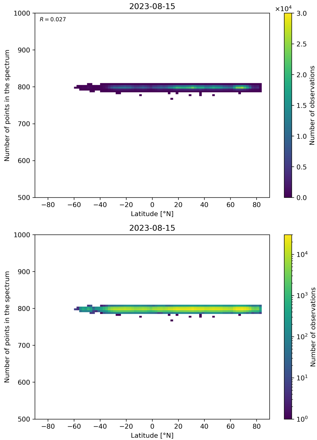
Figure 61: Scatter density plot of “Latitude” against “Number of points in the spectrum” for 2023-08-14 to 2023-08-16.
