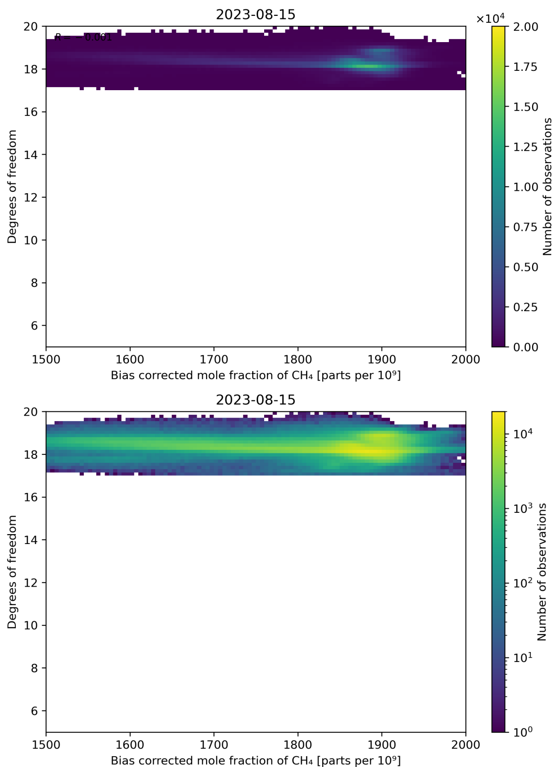
Figure 65: Scatter density plot of “Bias corrected mole fraction of CH 4 ” against “Degrees of freedom” for 2023-08-14 to 2023-08-16.
