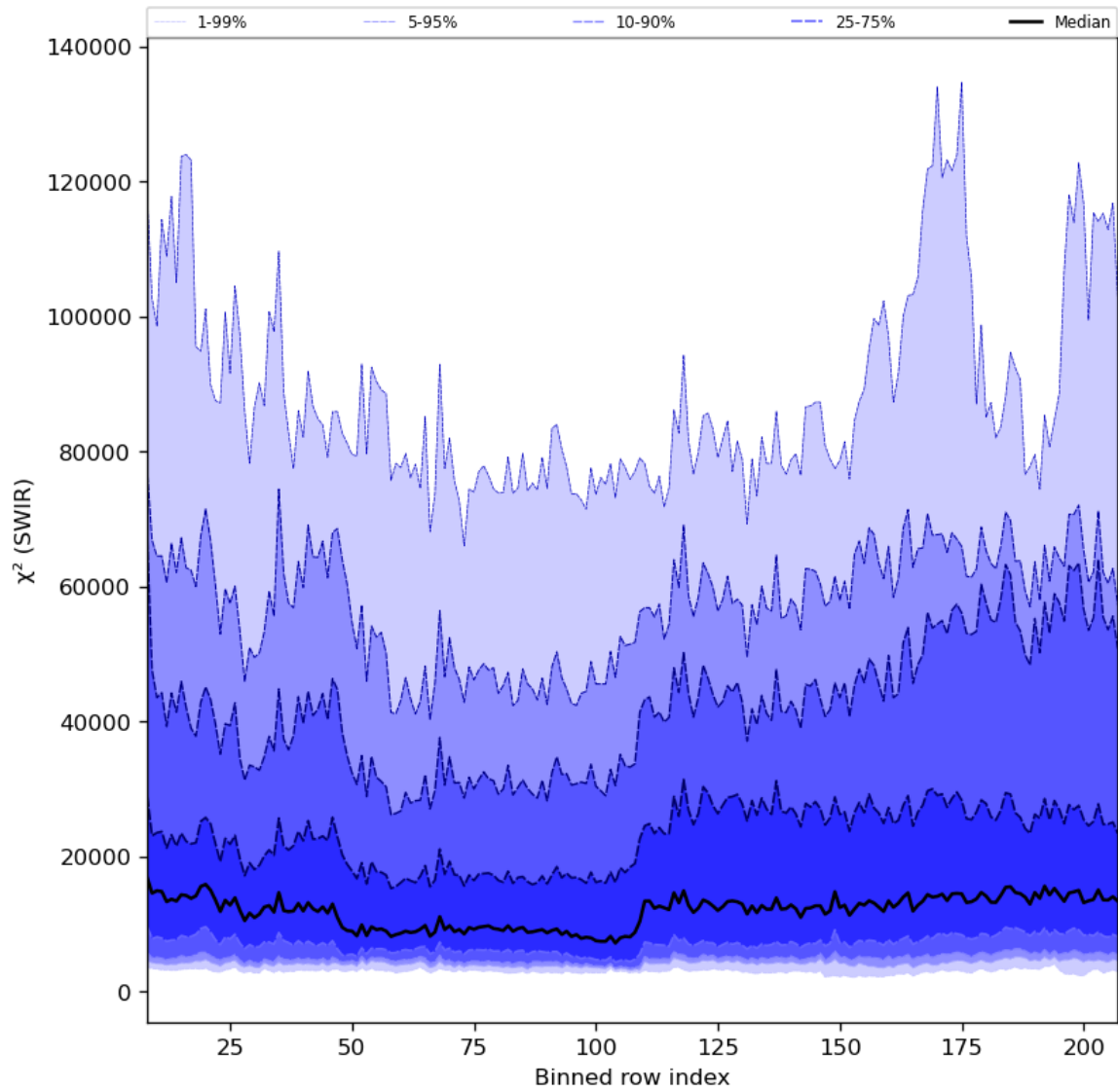
Figure 39: Along track statistics of “ \chi^2 (SWIR)” for 2023-08-14 to 2023-08-16
