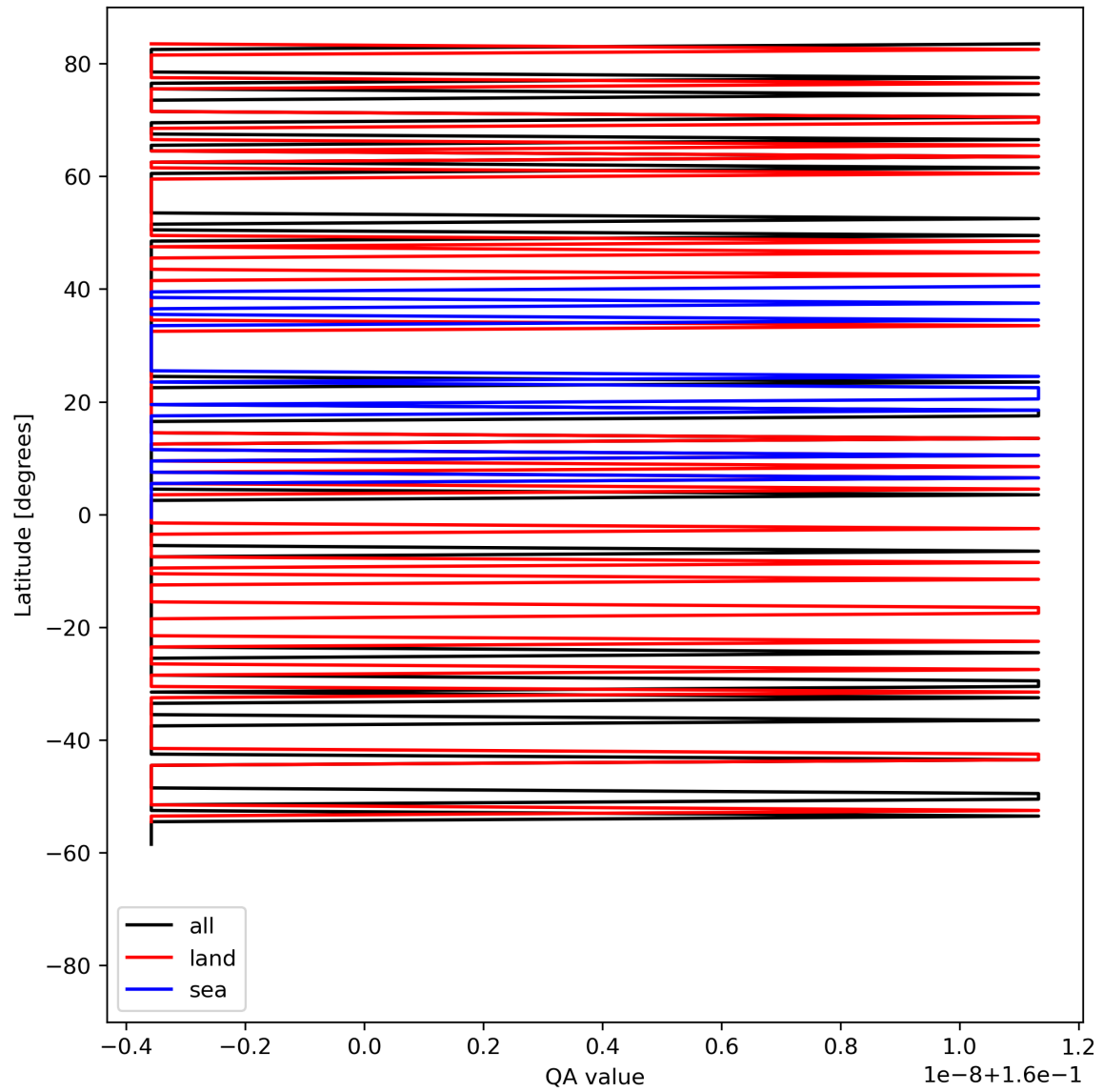
Figure 11: Zonal average of “QA value” for 2023-08-14 to 2023-08-16.
