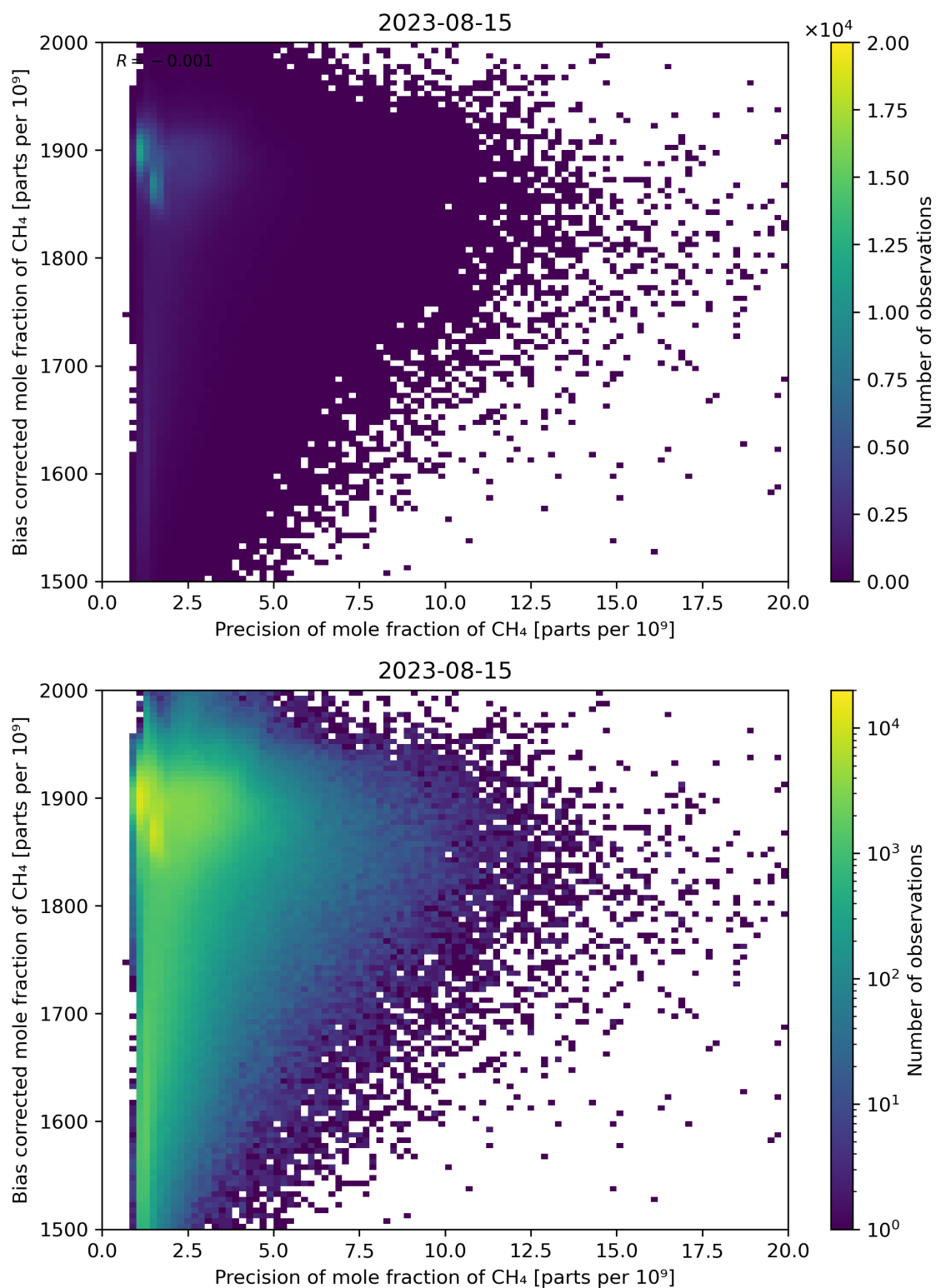
Figure 82: Scatter density plot of “Precision of mole fraction of CH 4 ” against “Bias corrected mole fraction of CH 4 ” for 2023-08-14 to 2023-08-16.
