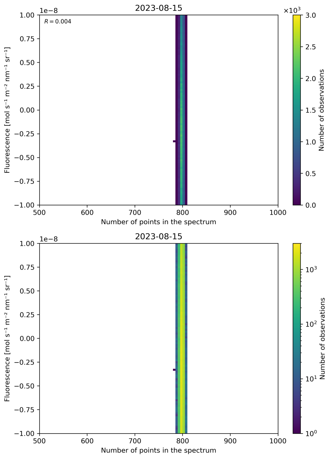
Figure 91: Scatter density plot of “Number of points in the spectrum” against “Fluorescence” for 2023-08-14 to 2023-08-16.
