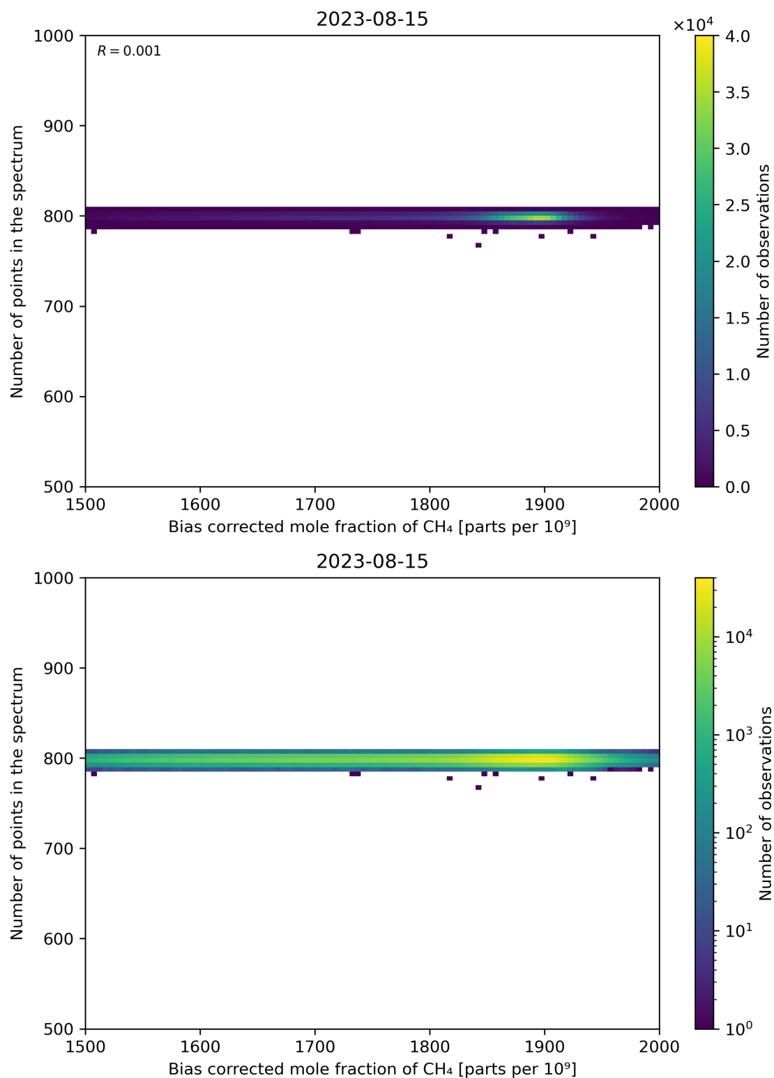
Figure 68: Scatter density plot of “Bias corrected mole fraction of CH 4 ” against “Number of points in the spectrum” for 2023-08-14 to 2023-08-16.
