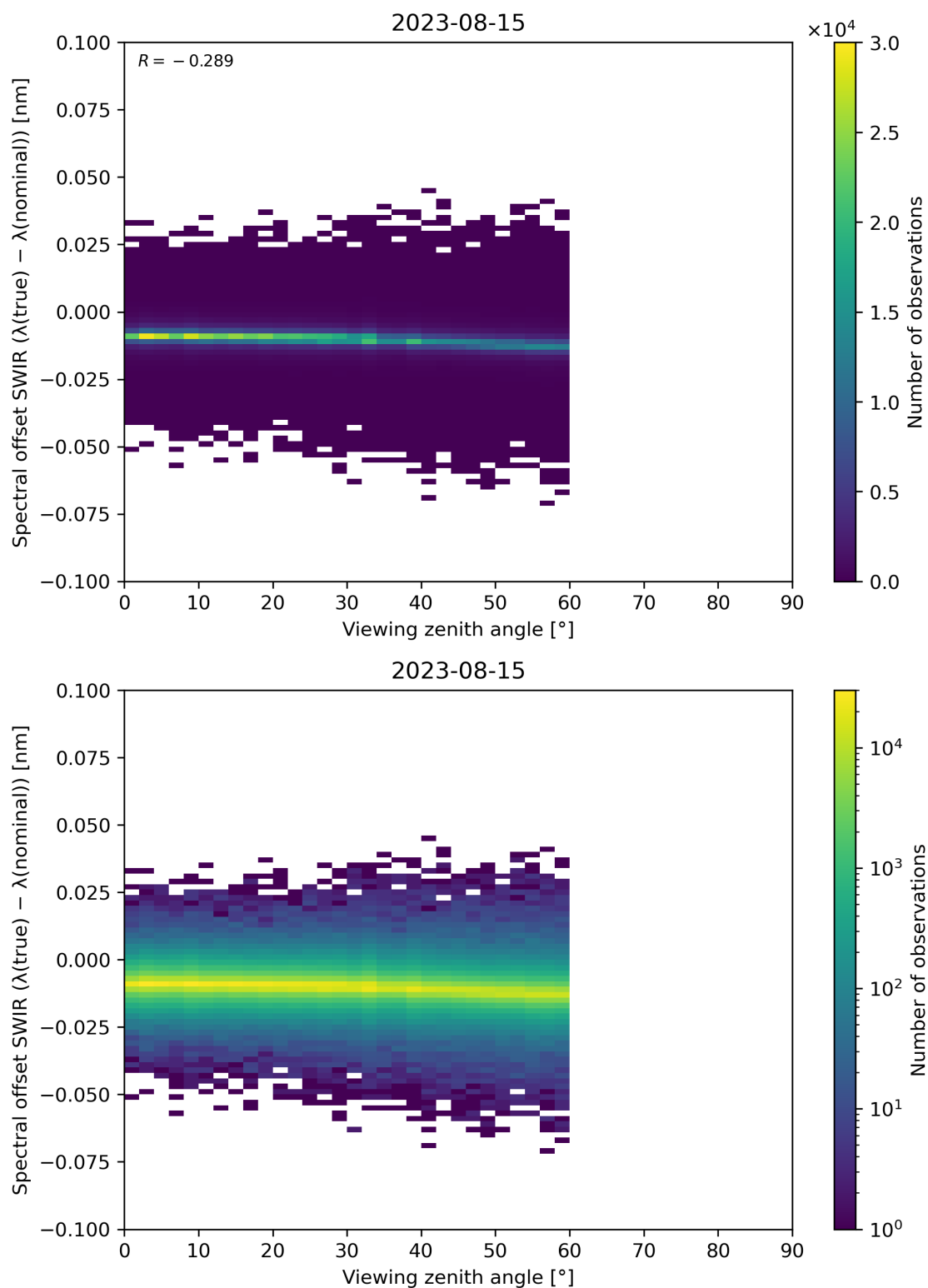
Figure 116: Scatter density plot of “Viewing zenith angle” against “Spectral offset SWIR ( \lambda(\text{true}) - \lambda(\text{nominal}) )” for 2023-08-14 to 2023-08-16.
