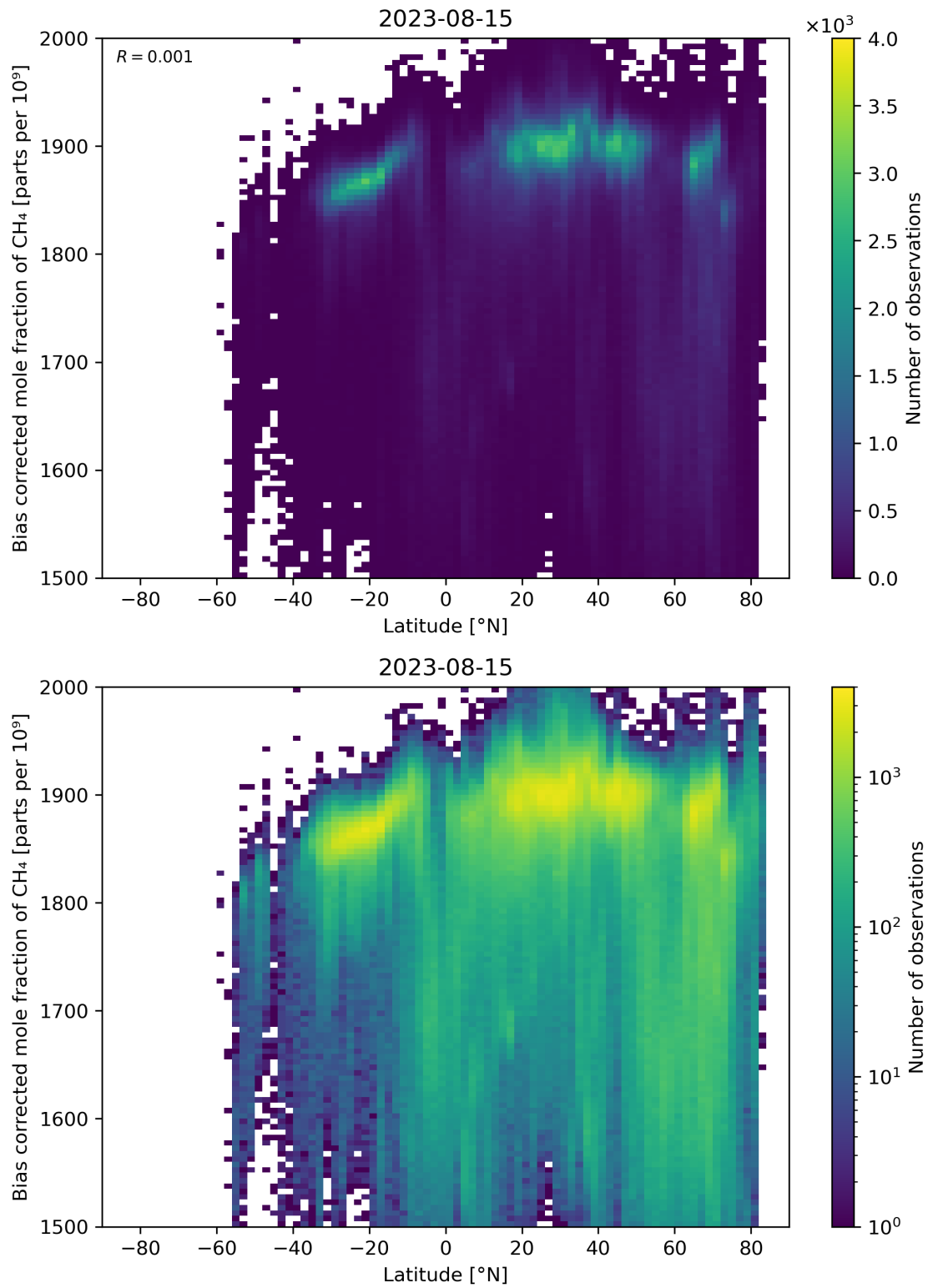
Figure 58: Scatter density plot of “Latitude” against “Bias corrected mole fraction of \text{CH}_4 ” for 2023-08-14 to 2023-08-16.
