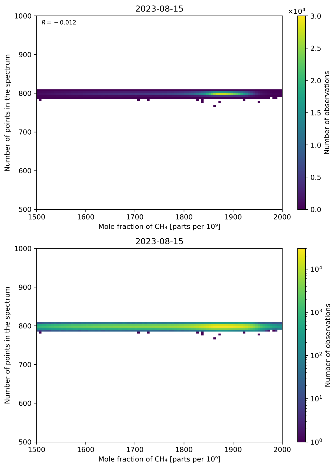
Figure 77: Scatter density plot of “Mole fraction of CH 4 ” against “Number of points in the spectrum” for 2023-08-14 to 2023-08-16.
