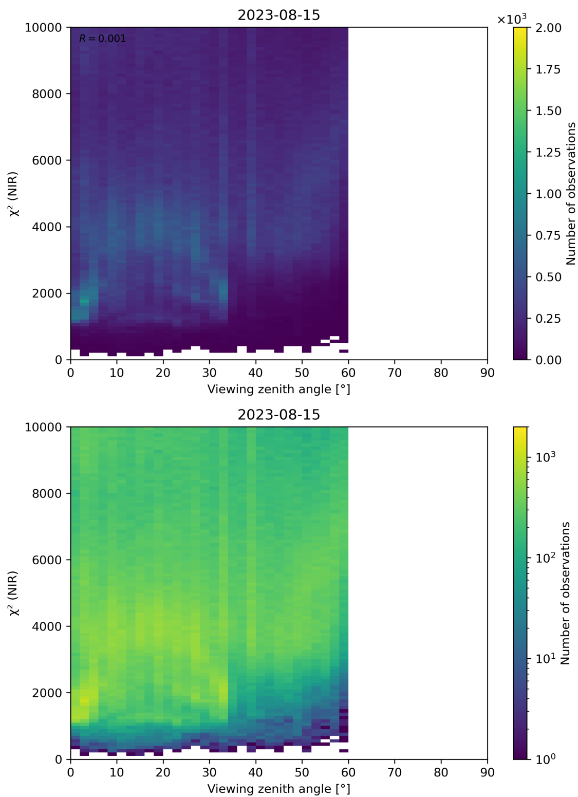
Figure 105: Scatter density plot of “Viewing zenith angle” against “ \chi^2 (NIR)” for 2023-08-14 to 2023-08-16.
