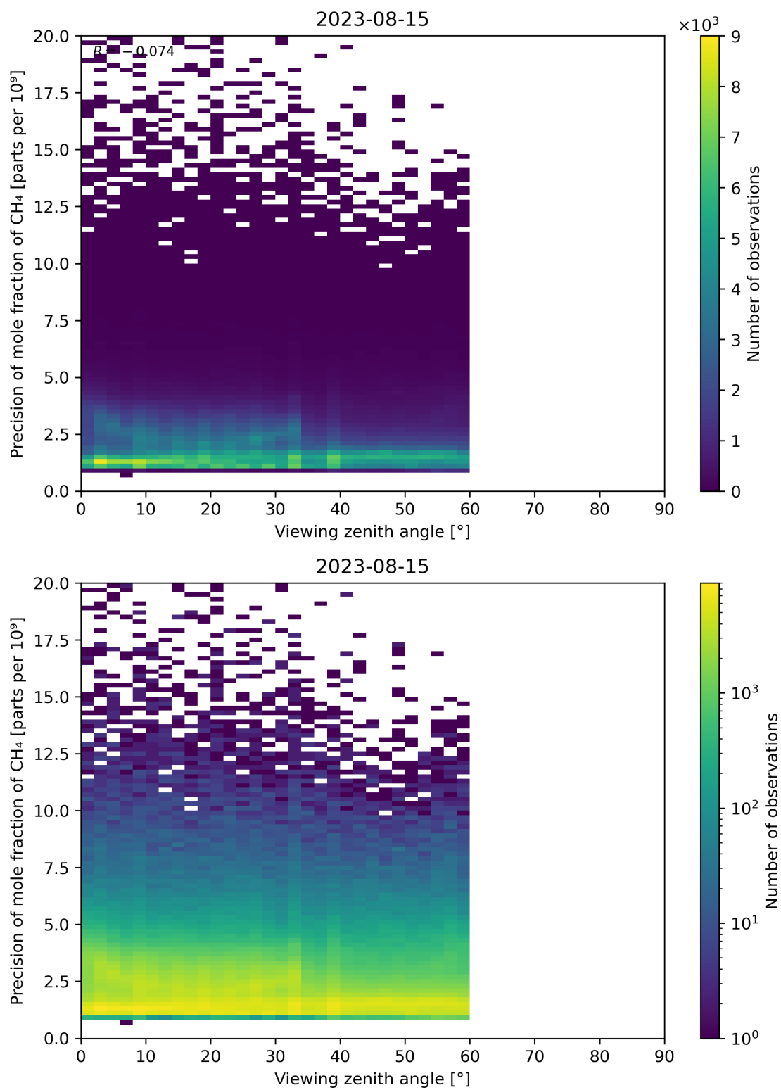
Figure 112: Scatter density plot of “Viewing zenith angle” against “Precision of mole fraction of CH 4 ” for 2023-08-14 to 2023-08-16.
