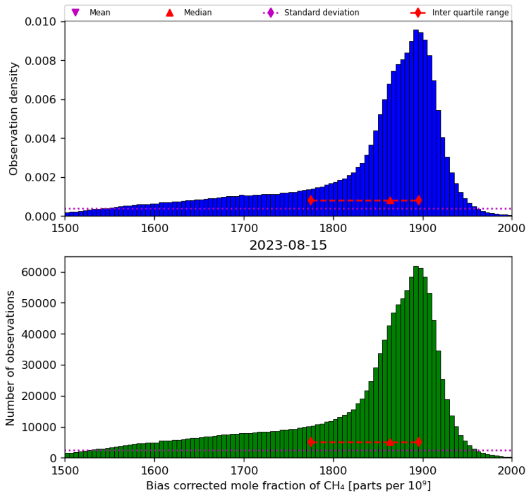
Figure 25: Histogram of “Bias corrected mole fraction of CH 4 ” for 2023-08-14 to 2023-08-16
