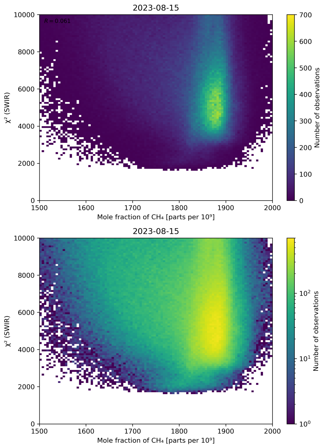
Figure 71: Scatter density plot of “Mole fraction of \text{CH}_4 ” against “ \chi^2 (SWIR)” for 2023-08-14 to 2023-08-16.
