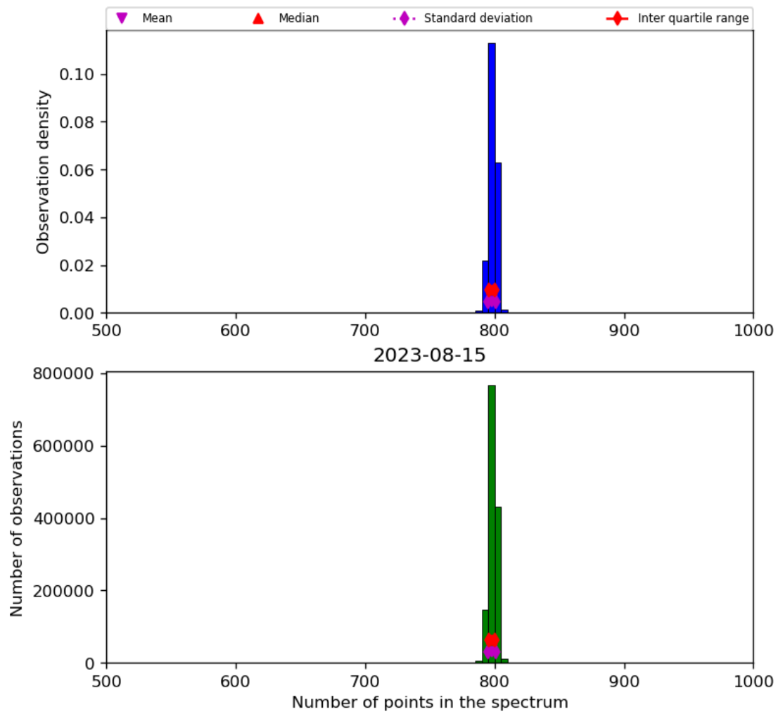
Figure 26: Histogram of “Number of points in the spectrum” for 2023-08-14 to 2023-08-16
