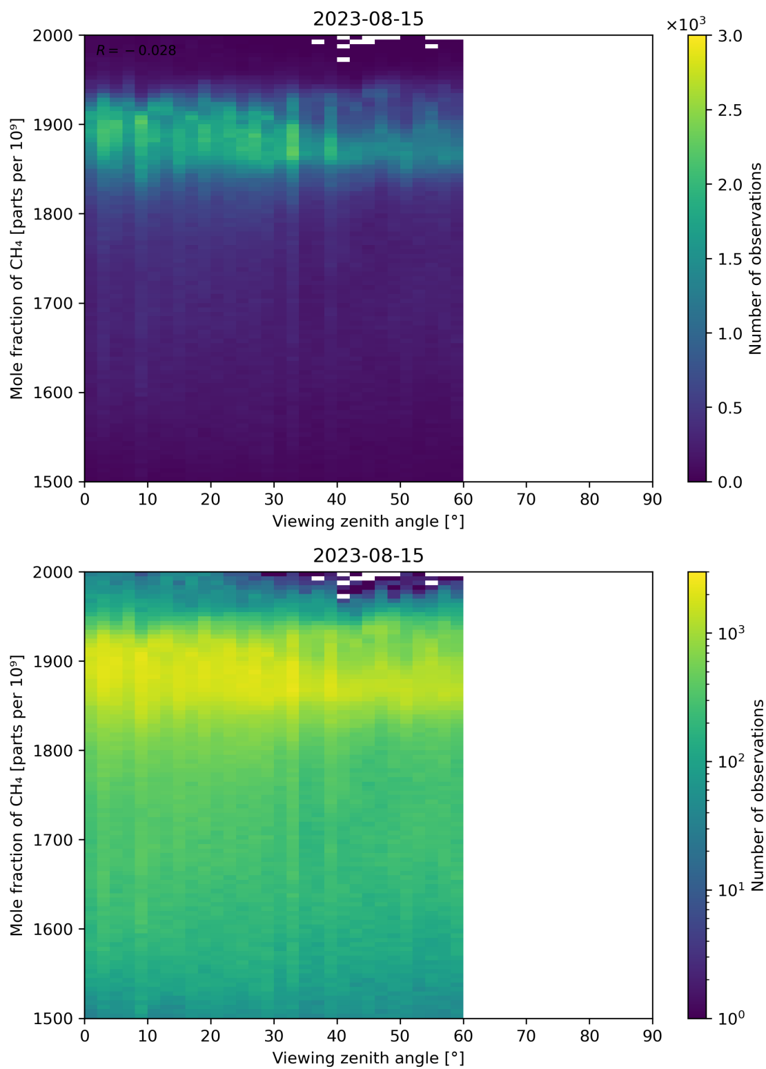
Figure 110: Scatter density plot of “Viewing zenith angle” against “Mole fraction of CH 4 ” for 2023-08-14 to 2023-08-16.
