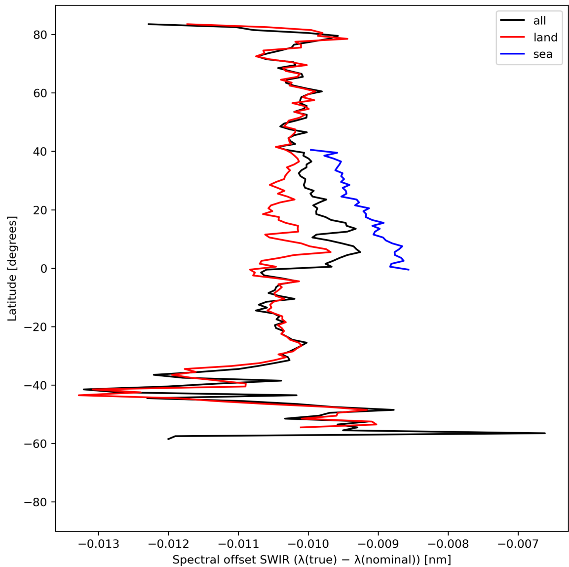
Figure 16: Zonal average of “Spectral offset SWIR ( \lambda(\text{true}) - \lambda(\text{nominal}) )” for 2023-08-14 to 2023-08-16.
