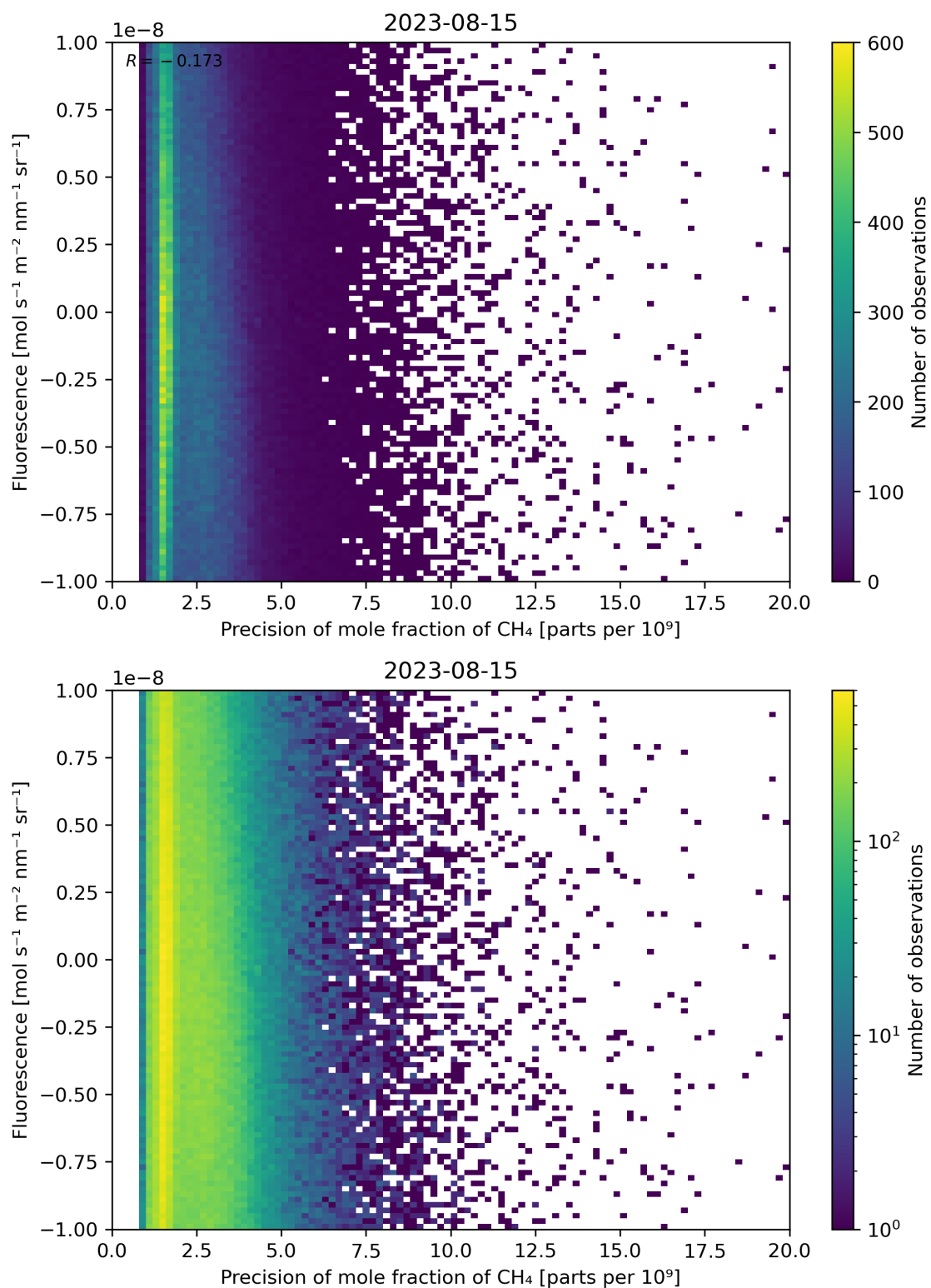
Figure 81: Scatter density plot of “Precision of mole fraction of \text{CH}_4 ” against “Fluorescence” for 2023-08-14 to 2023-08-16.
