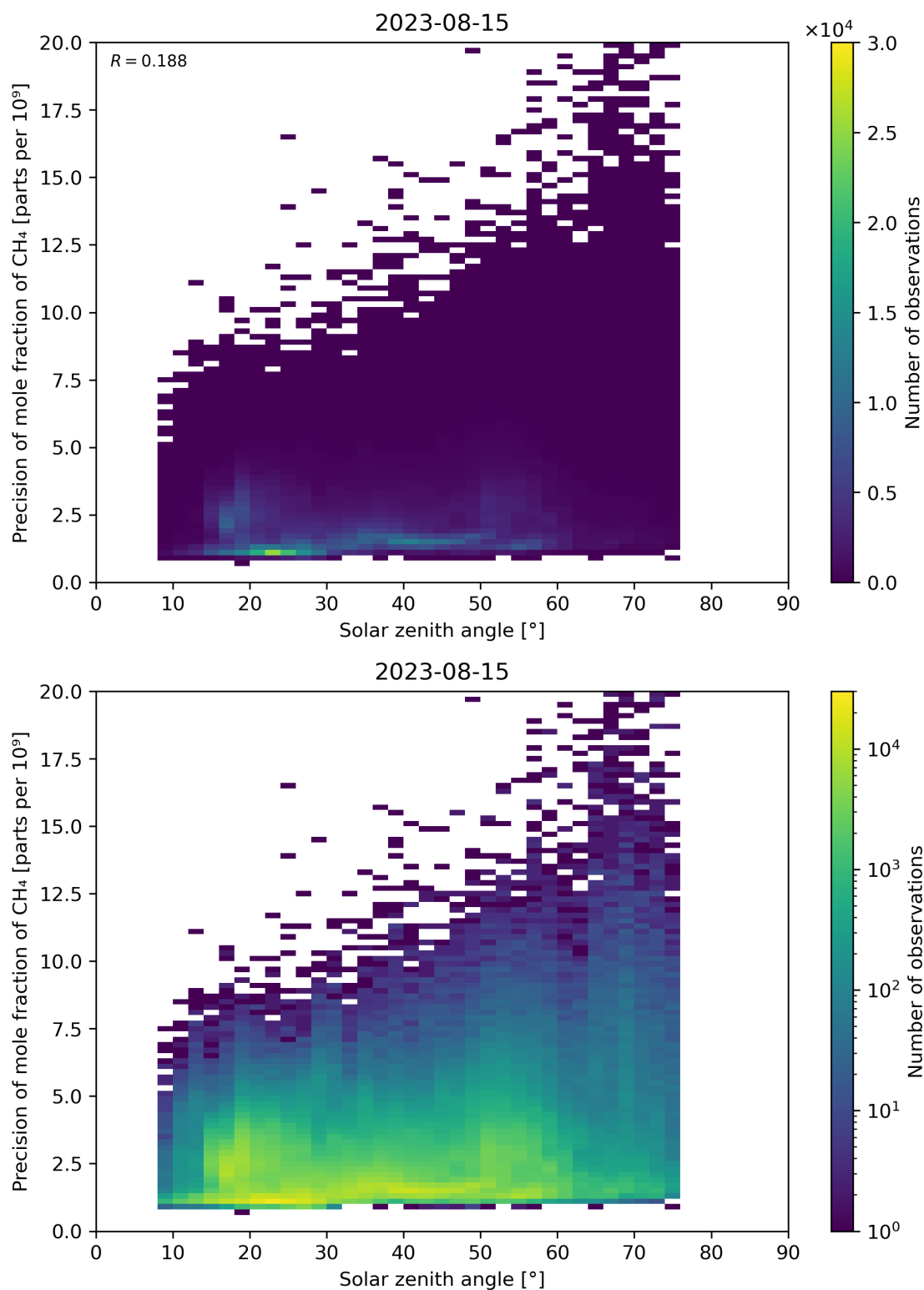
Figure 101: Scatter density plot of “Solar zenith angle” against “Precision of mole fraction of CH 4 ” for 2023-08-14 to 2023-08-16.
