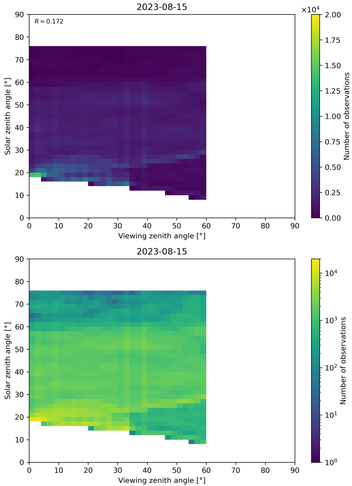
Figure 115: Scatter density plot of “Viewing zenith angle” against “Solar zenith angle” for 2023-08-14 to 2023-08-16.
