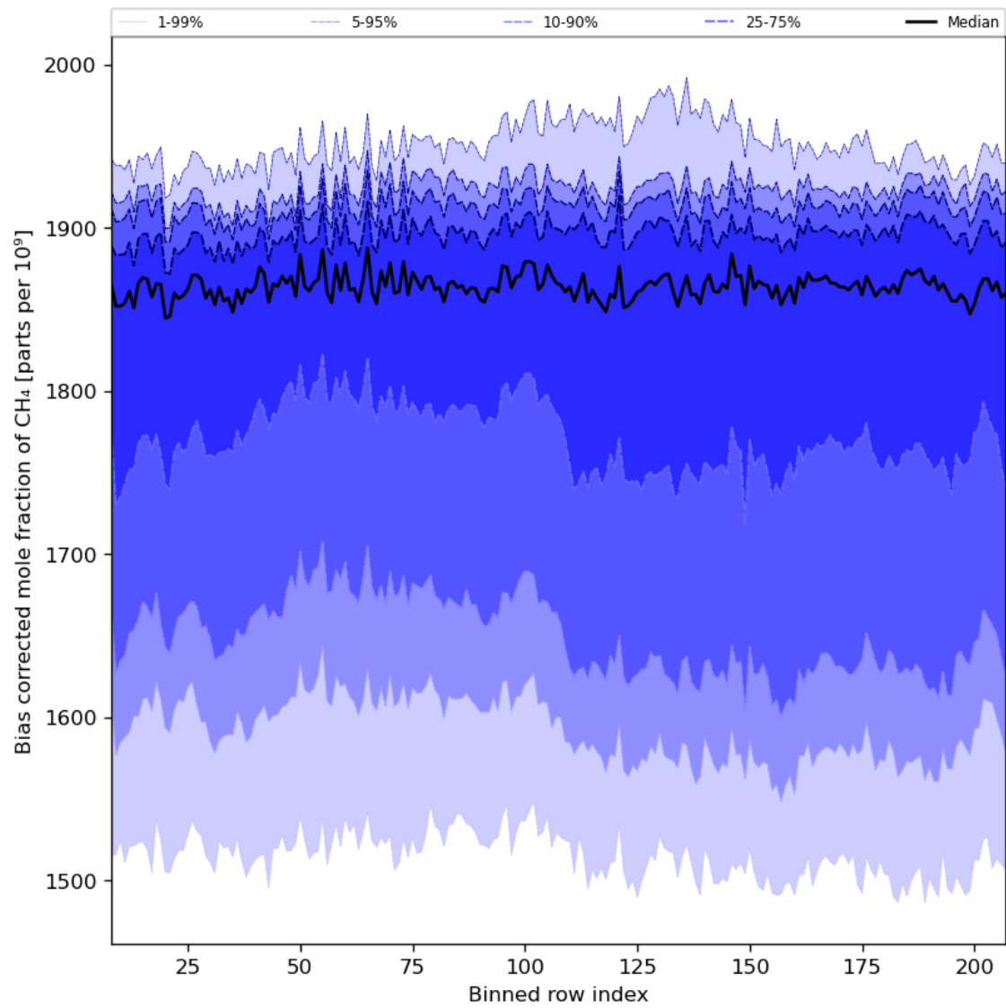
Figure 36: Along track statistics of “Bias corrected mole fraction of CH 4 ” for 2023-08-14 to 2023-08-16
