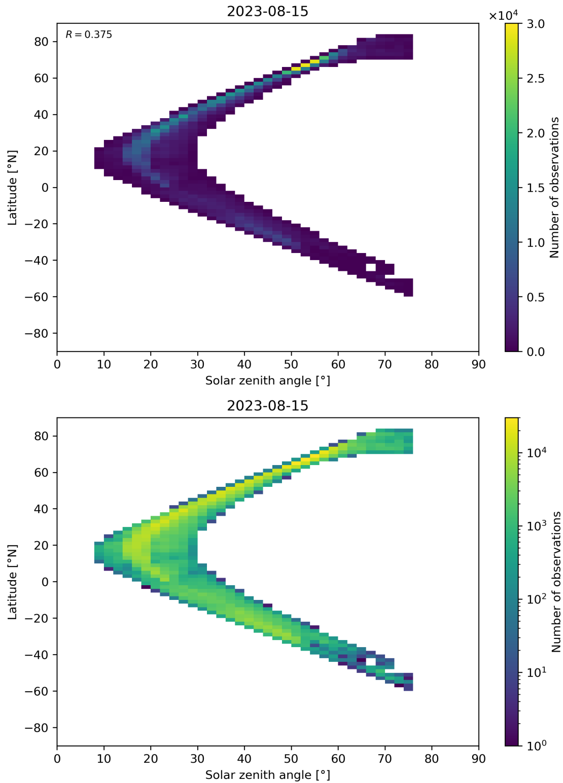
Figure 98: Scatter density plot of “Solar zenith angle” against “Latitude” for 2023-08-14 to 2023-08-16.
