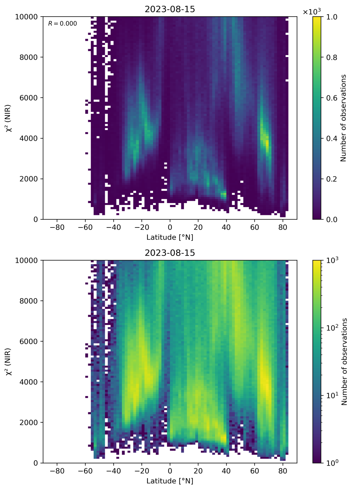
Figure 53: Scatter density plot of “Latitude” against “ \chi^2 (NIR)” for 2023-08-14 to 2023-08-16.
