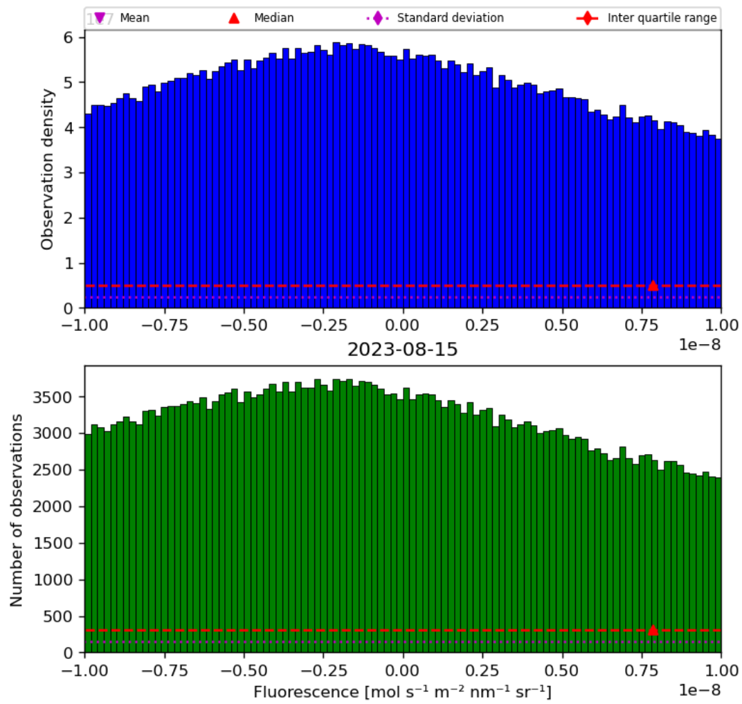
Figure 32: Histogram of “Fluorescence” for 2023-08-14 to 2023-08-16
