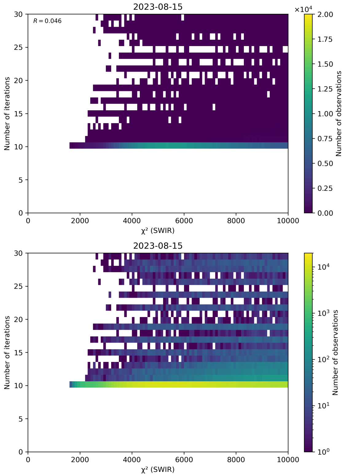
Figure 50: Scatter density plot of “ \chi^2 (SWIR)” against “Number of iterations” for 2023-08-14 to 2023-08-16.
