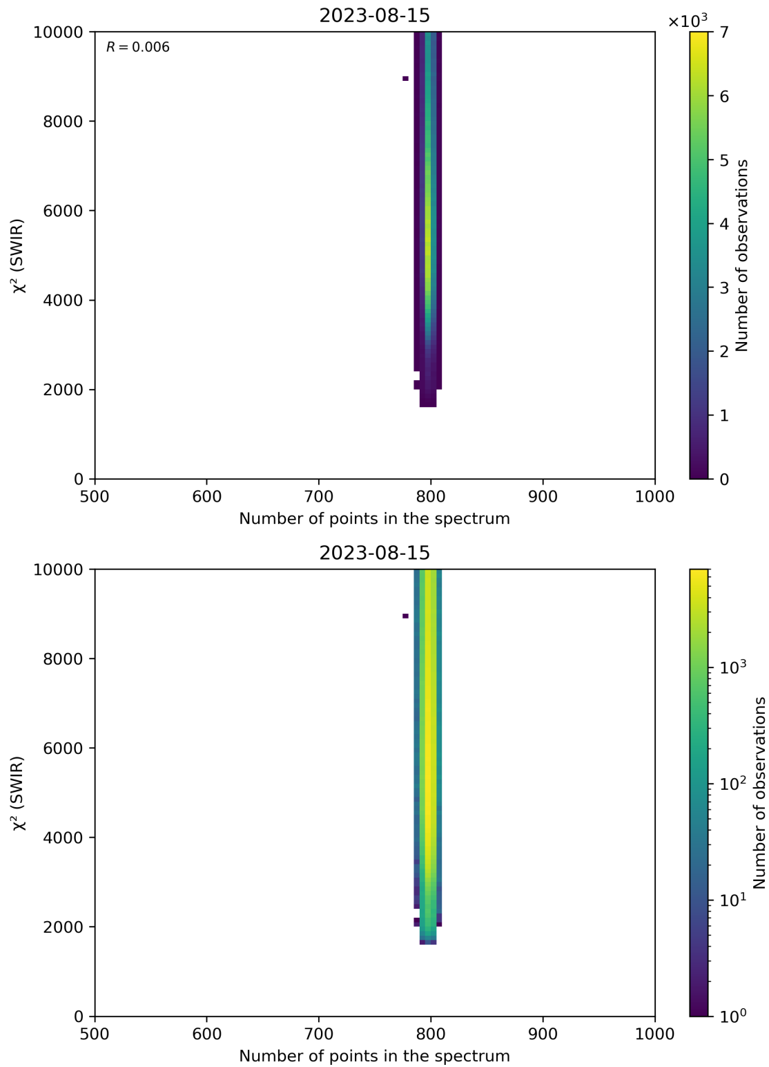
Figure 89: Scatter density plot of “Number of points in the spectrum” against “ \chi^2 (SWIR)” for 2023-08-14 to 2023-08-16.
