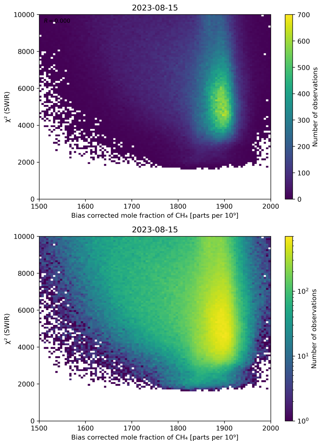
Figure 64: Scatter density plot of “Bias corrected mole fraction of \text{CH}_4 ” against “ \chi^2 (SWIR)” for 2023-08-14 to 2023-08-16.
