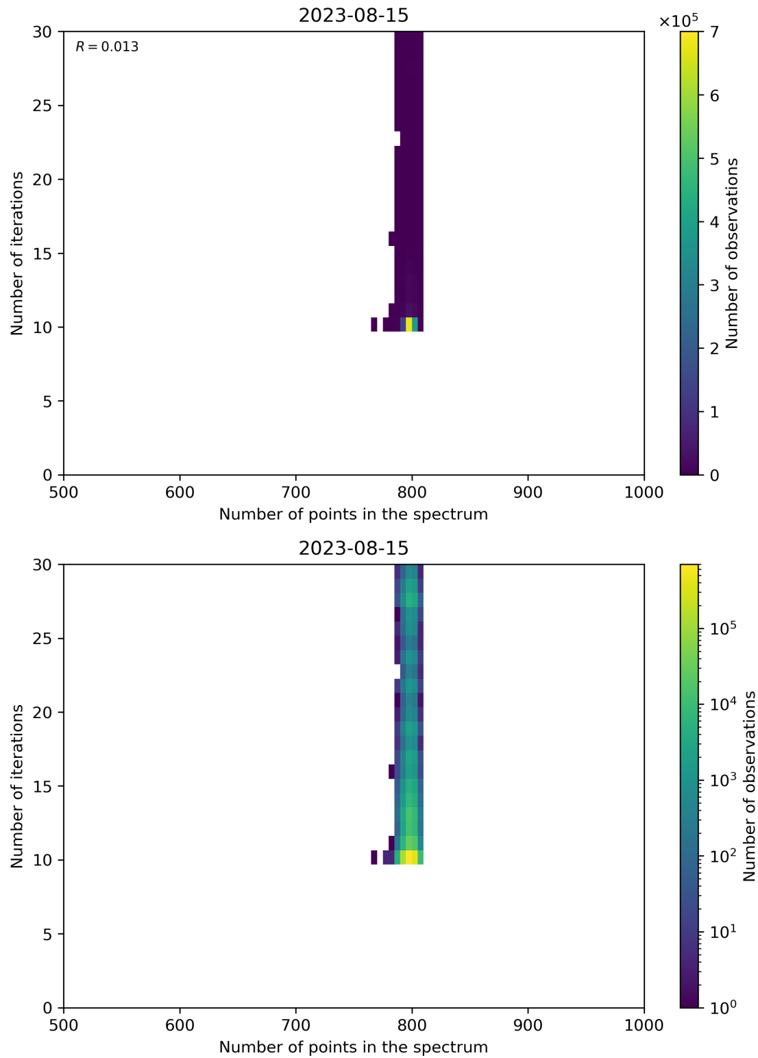
Figure 92: Scatter density plot of “Number of points in the spectrum” against “Number of iterations” for 2023-08-14 to 2023-08-16.
