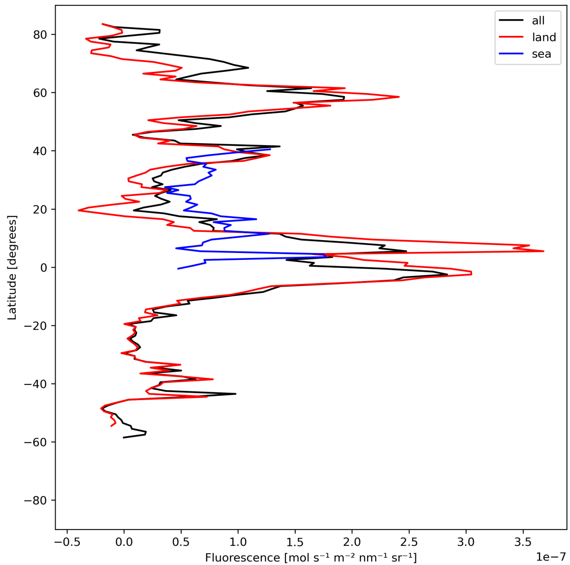
Figure 21: Zonal average of “Fluorescence” for 2023-08-14 to 2023-08-16.
