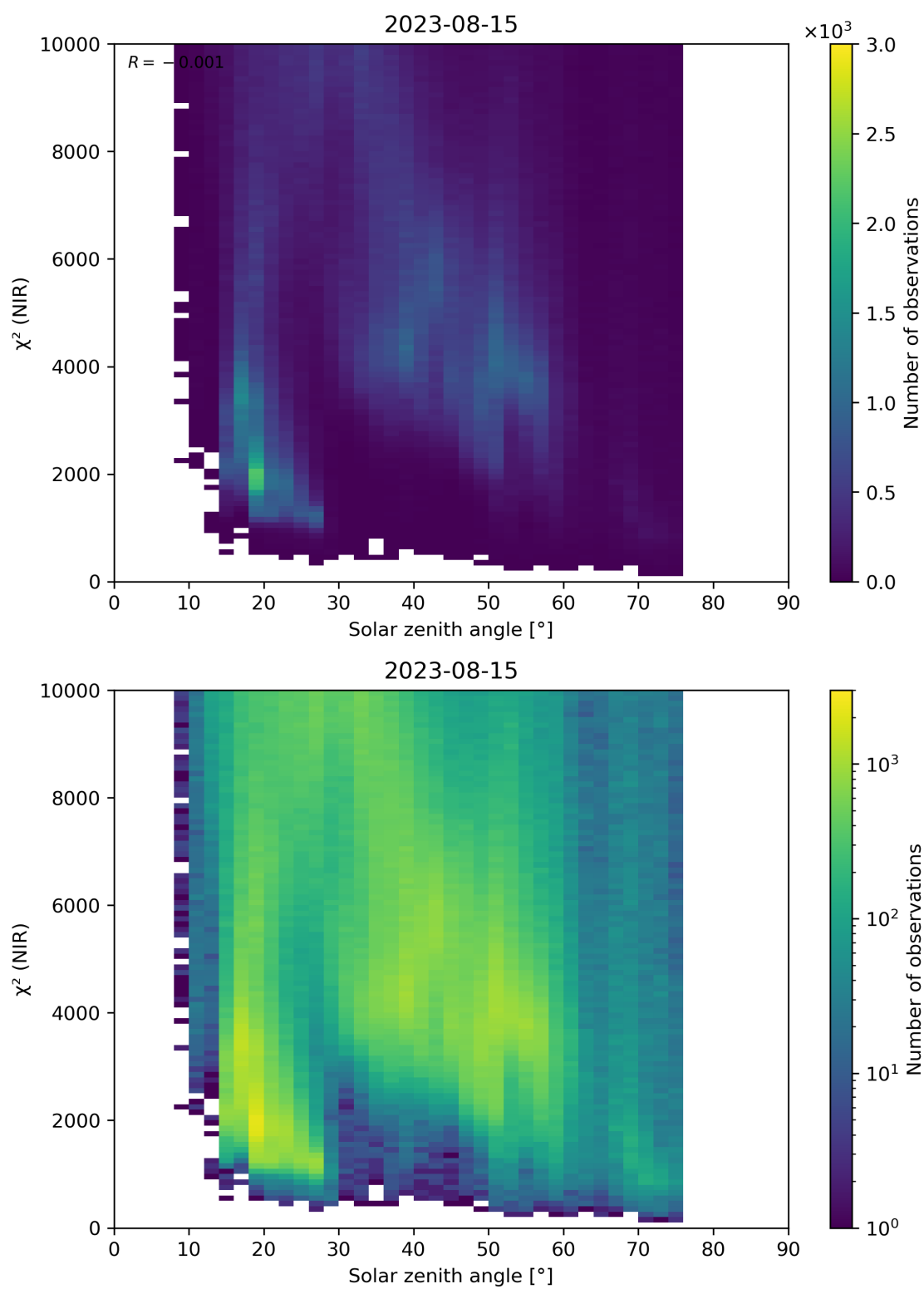
Figure 94: Scatter density plot of “Solar zenith angle” against “ \chi^2 (NIR)” for 2023-08-14 to 2023-08-16.
