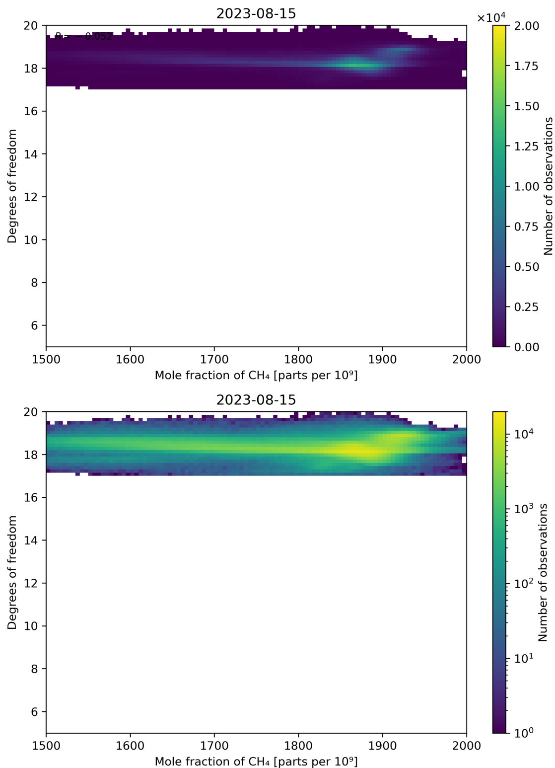
Figure 72: Scatter density plot of “Mole fraction of CH 4 ” against “Degrees of freedom” for 2023-08-14 to 2023-08-16.
