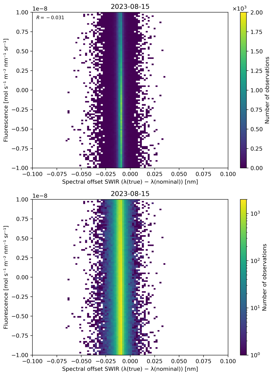
Figure 120: Scatter density plot of “Spectral offset SWIR ( \lambda(\text{true}) - \lambda(\text{nominal}) )” against “Fluorescence” for 2023-08-14 to 2023-08-16.
