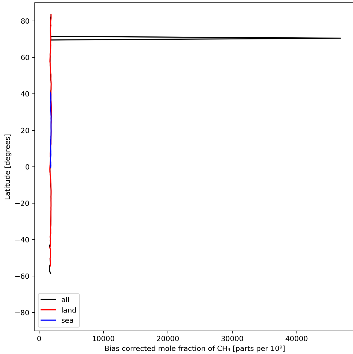
Figure 14: Zonal average of “Bias corrected mole fraction of CH 4 ” for 2023-08-14 to 2023-08-16.
