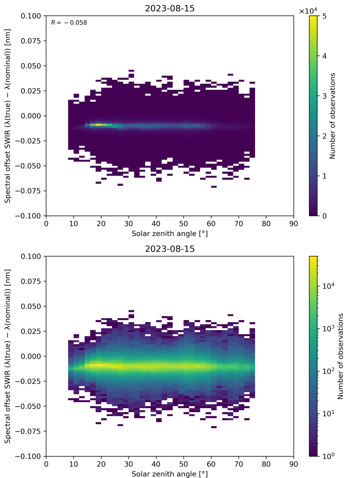
Figure 104: Scatter density plot of “Solar zenith angle” against “Spectral offset SWIR ( \lambda(\text{true}) - \lambda(\text{nominal}) )” for 2023-08-14 to 2023-08-16.
