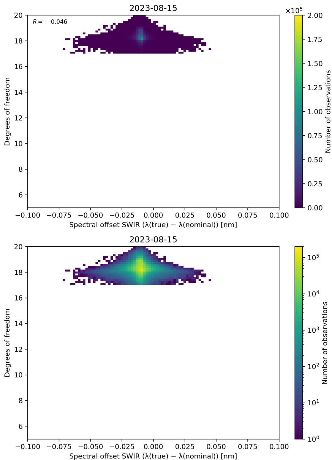
Figure 119: Scatter density plot of “Spectral offset SWIR ( \lambda(\text{true}) - \lambda(\text{nominal}) )” against “Degrees of freedom” for 2023-08-14 to 2023-08-16.
