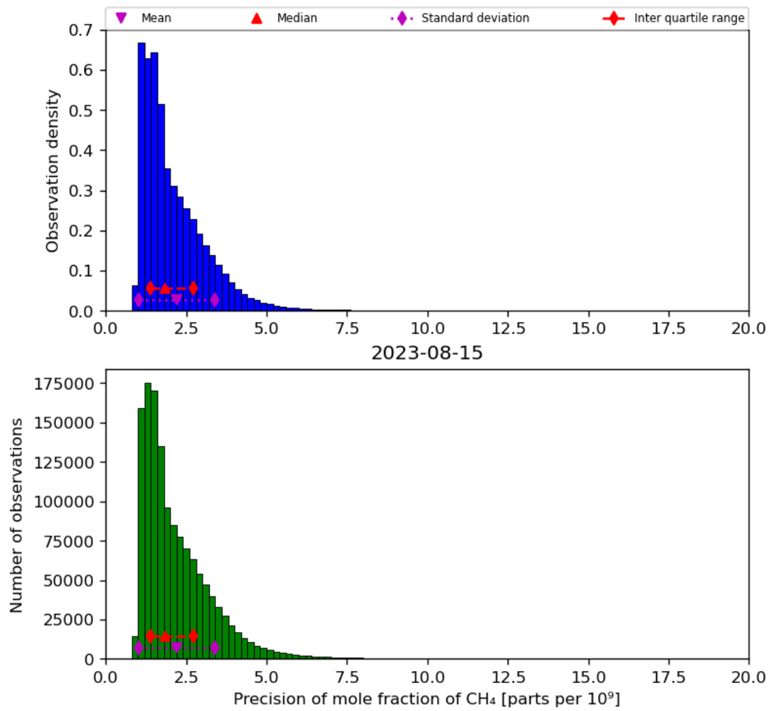
Figure 24: Histogram of “Precision of mole fraction of CH 4 ” for 2023-08-14 to 2023-08-16
