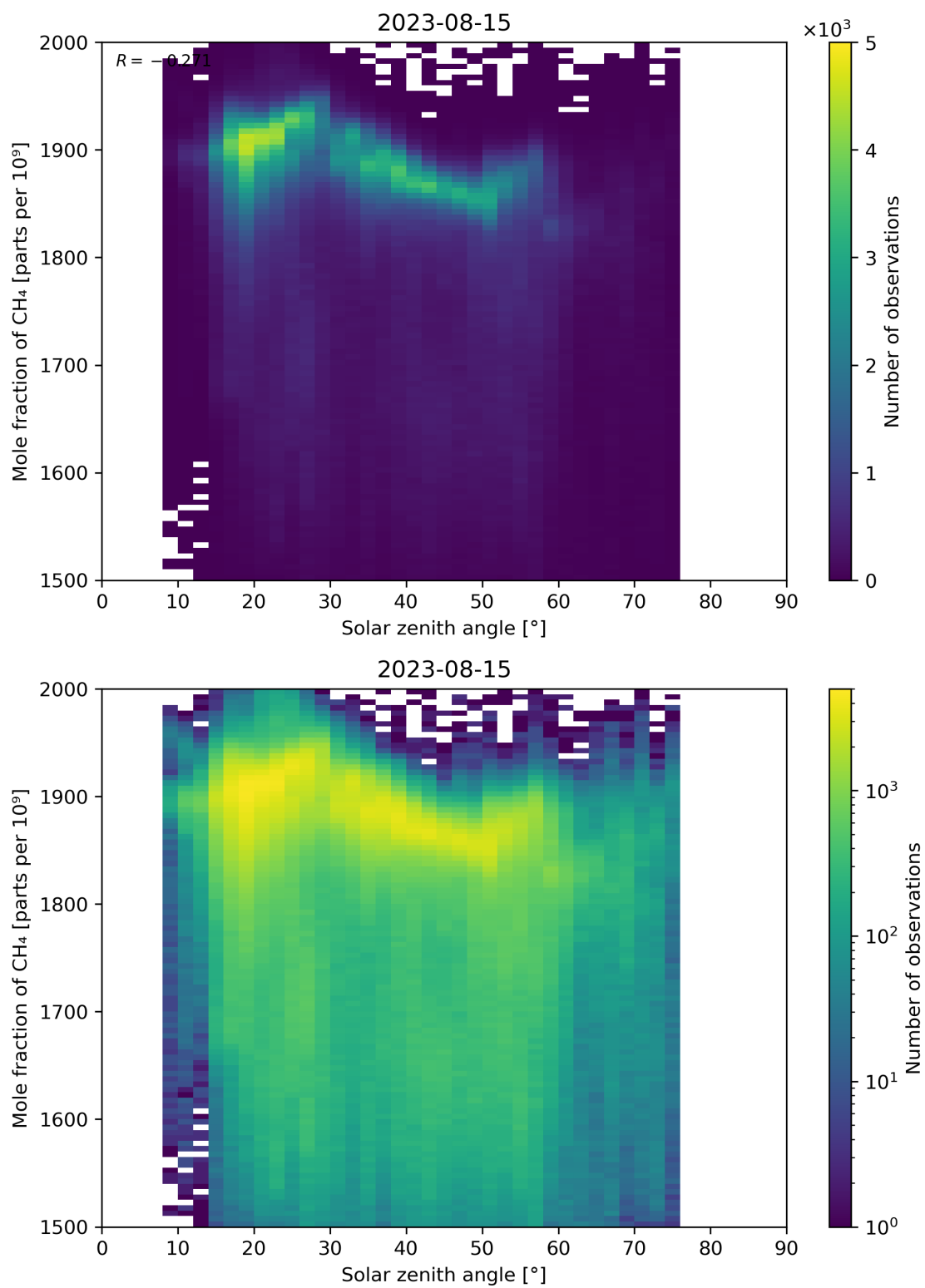
Figure 99: Scatter density plot of “Solar zenith angle” against “Mole fraction of CH 4 ” for 2023-08-14 to 2023-08-16.
