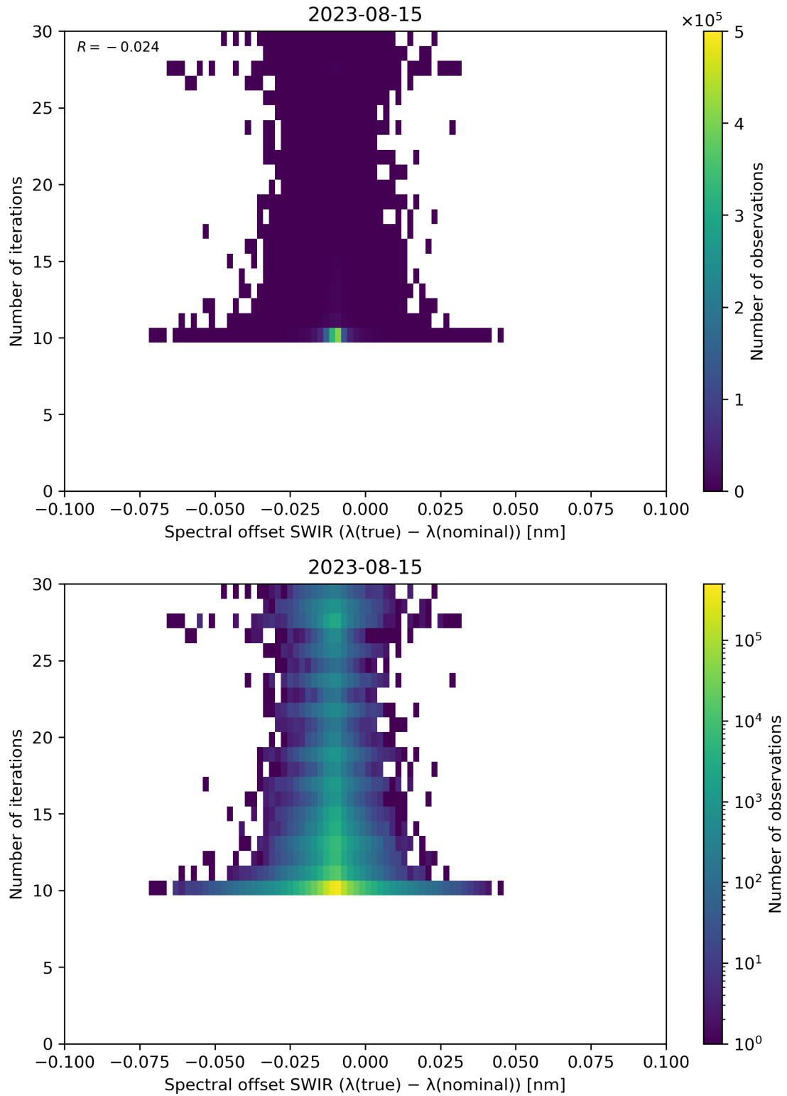
Figure 121: Scatter density plot of “Spectral offset SWIR ( \lambda(\text{true}) - \lambda(\text{nominal}) )” against “Number of iterations” for 2023-08-14 to 2023-08-16.
