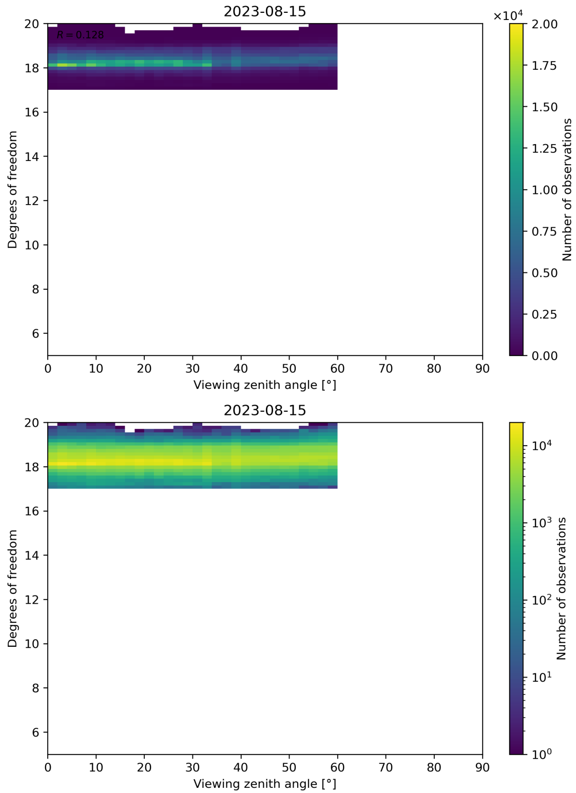
Figure 107: Scatter density plot of “Viewing zenith angle” against “Degrees of freedom” for 2023-08-14 to 2023-08-16.
