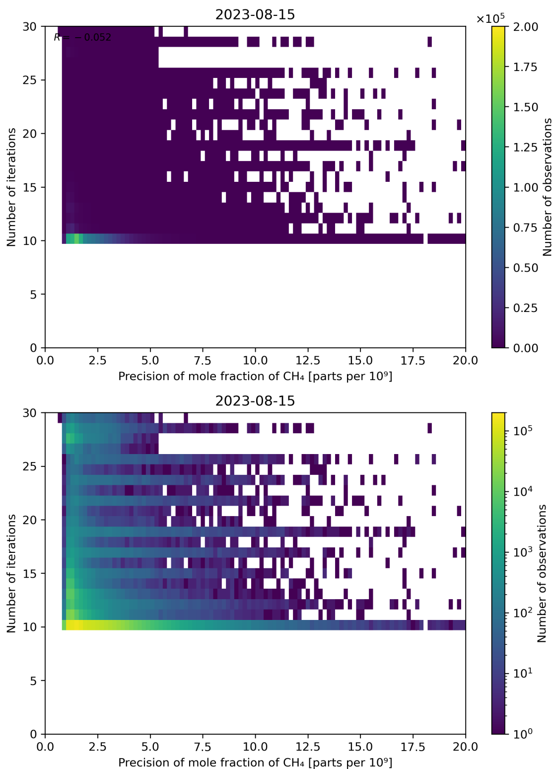
Figure 83: Scatter density plot of “Precision of mole fraction of CH 4 ” against “Number of iterations” for 2023-08-14 to 2023-08-16.
