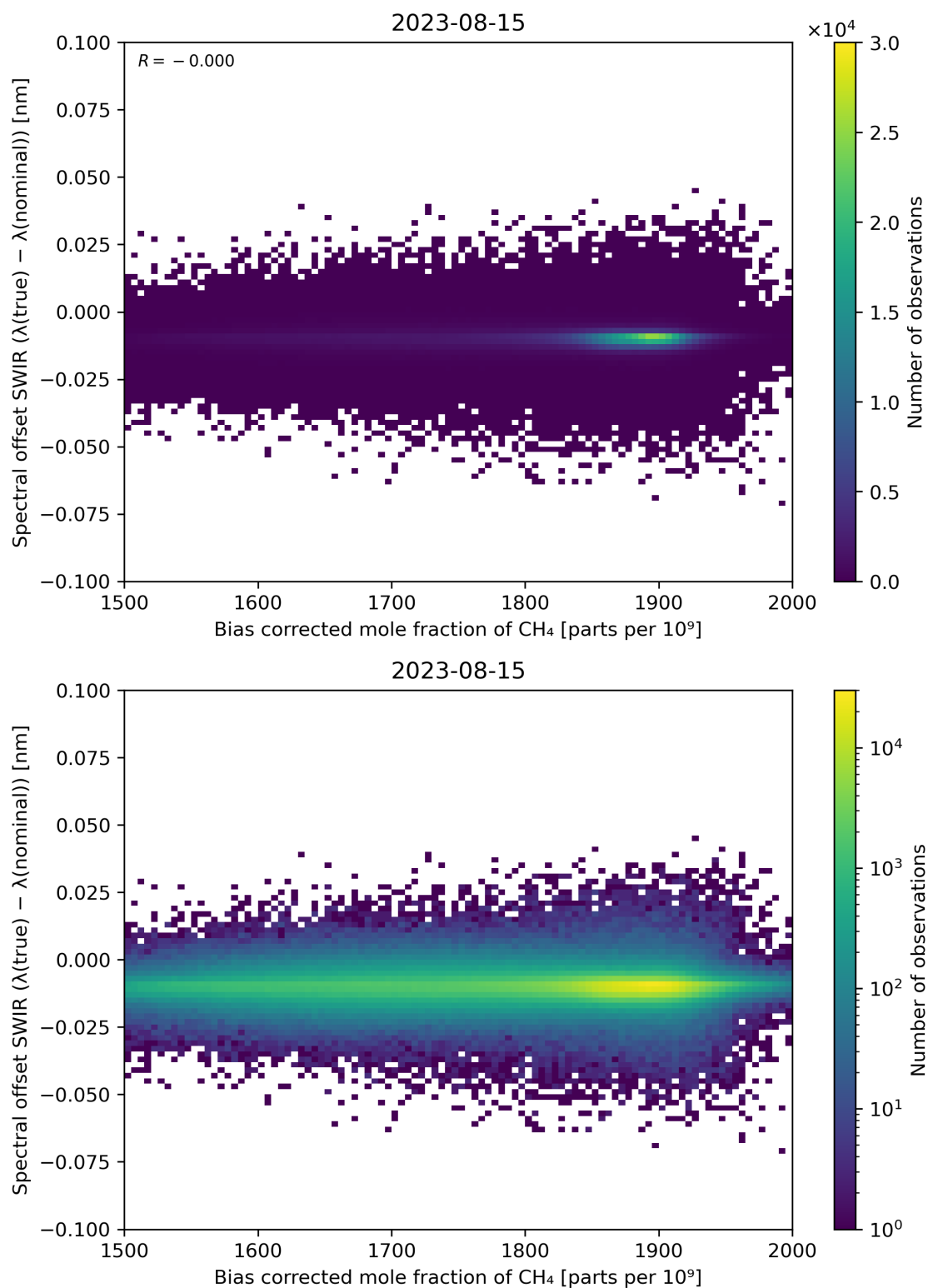
Figure 69: Scatter density plot of “Bias corrected mole fraction of \text{CH}_4 ” against “Spectral offset SWIR ( \lambda(\text{true}) - \lambda(\text{nominal}) )” for 2023-08-14 to 2023-08-16.
