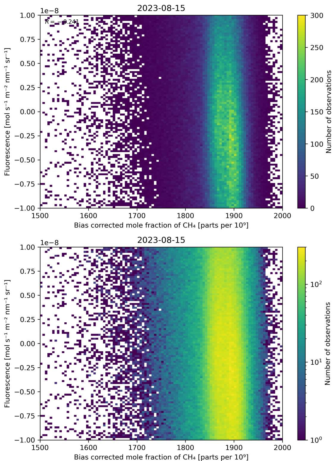
Figure 66: Scatter density plot of “Bias corrected mole fraction of CH 4 ” against “Fluorescence” for 2023-08-14 to 2023-08-16.
