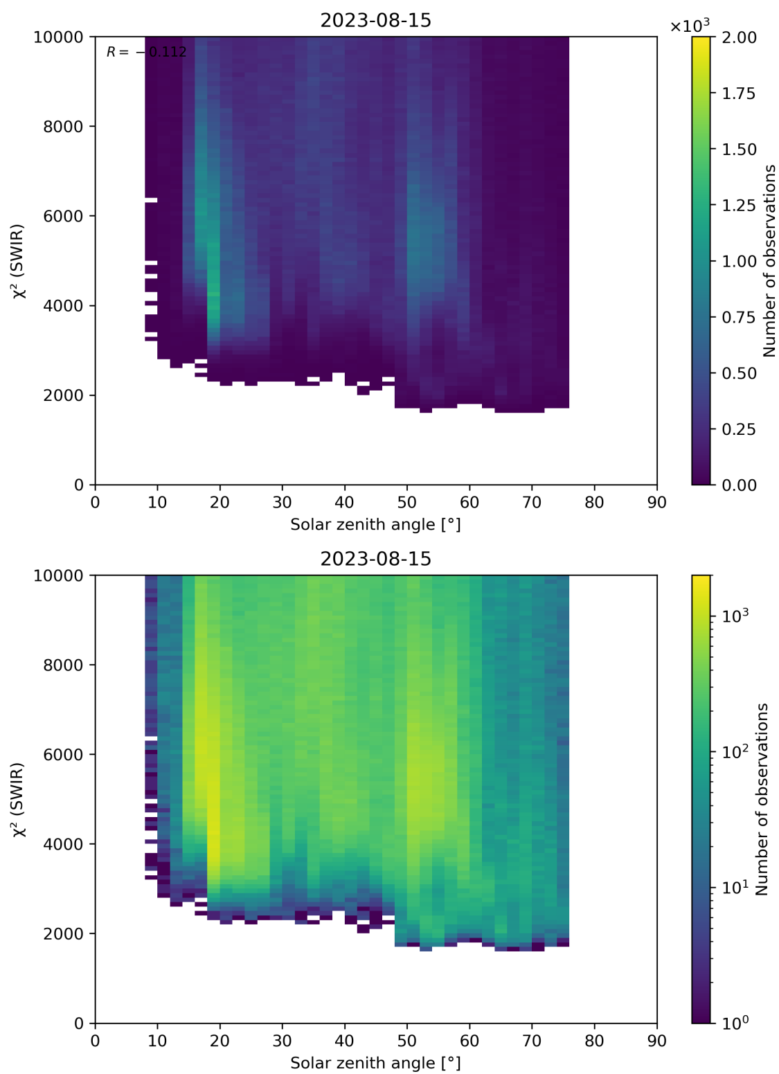
Figure 95: Scatter density plot of “Solar zenith angle” against “ \chi^2 (SWIR)” for 2023-08-14 to 2023-08-16.
