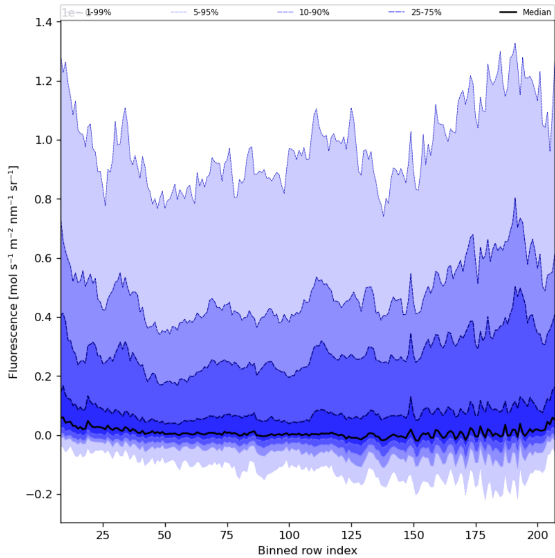
Figure 43: Along track statistics of “Fluorescence” for 2023-08-14 to 2023-08-16
