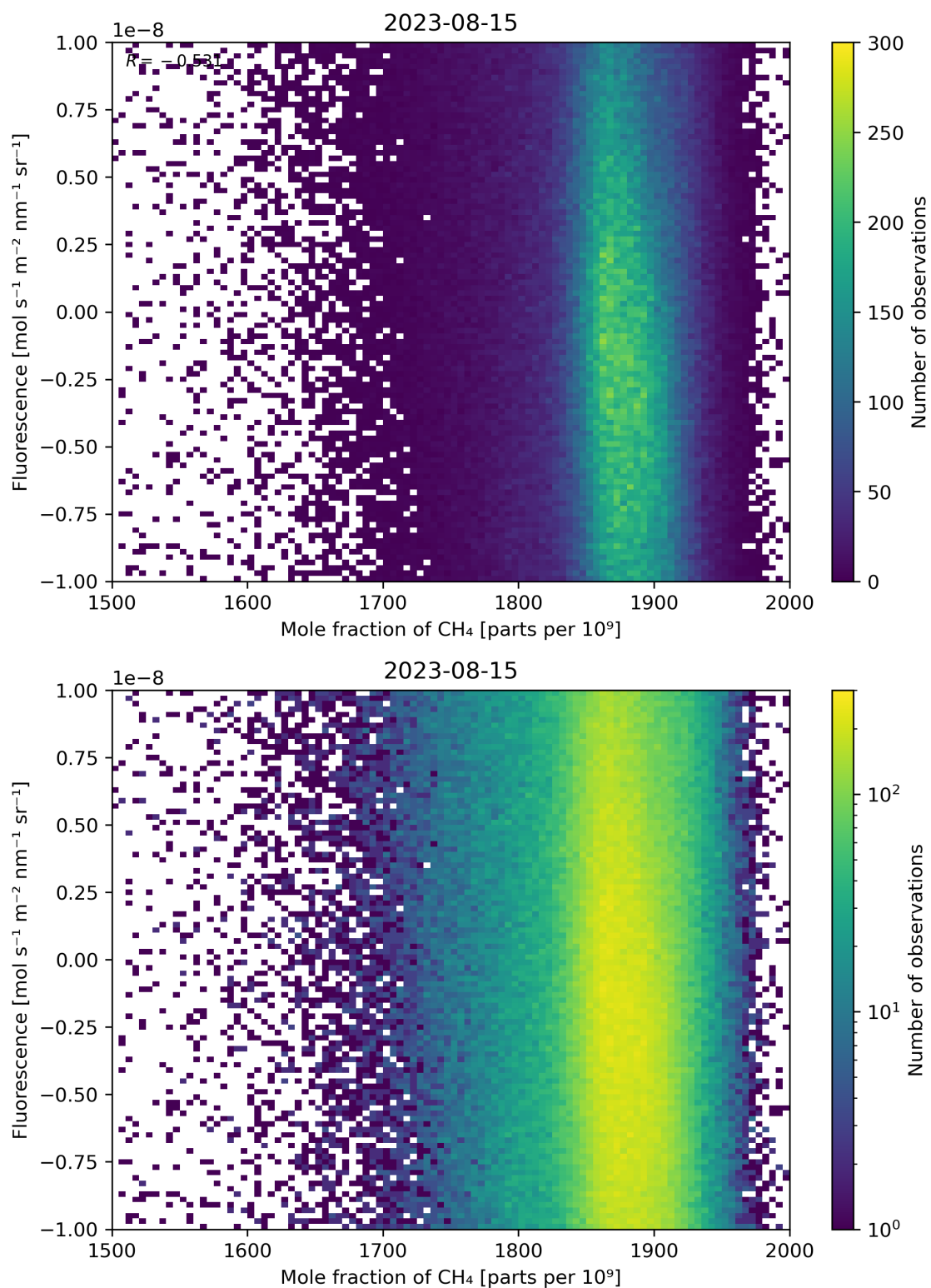
Figure 73: Scatter density plot of “Mole fraction of \text{CH}_4 ” against “Fluorescence” for 2023-08-14 to 2023-08-16.
