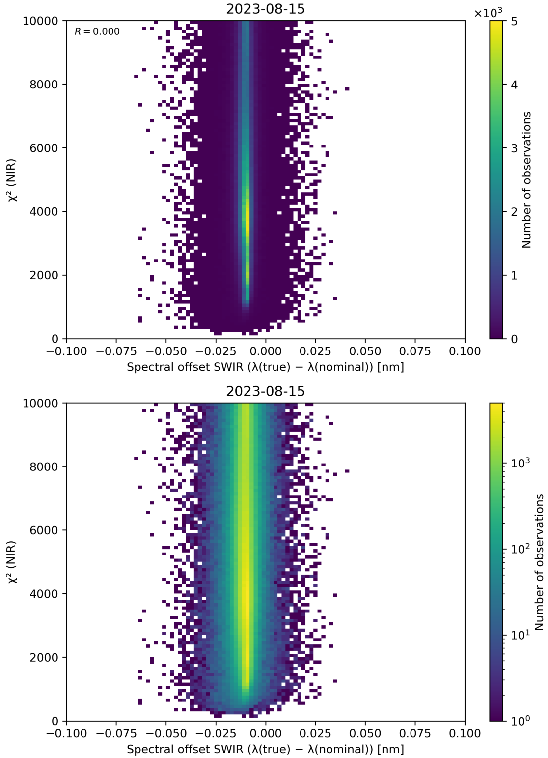
Figure 117: Scatter density plot of “Spectral offset SWIR ( \lambda(\text{true}) - \lambda(\text{nominal}) )” against “ \chi^2 (NIR)” for 2023-08-14 to 2023-08-16.
