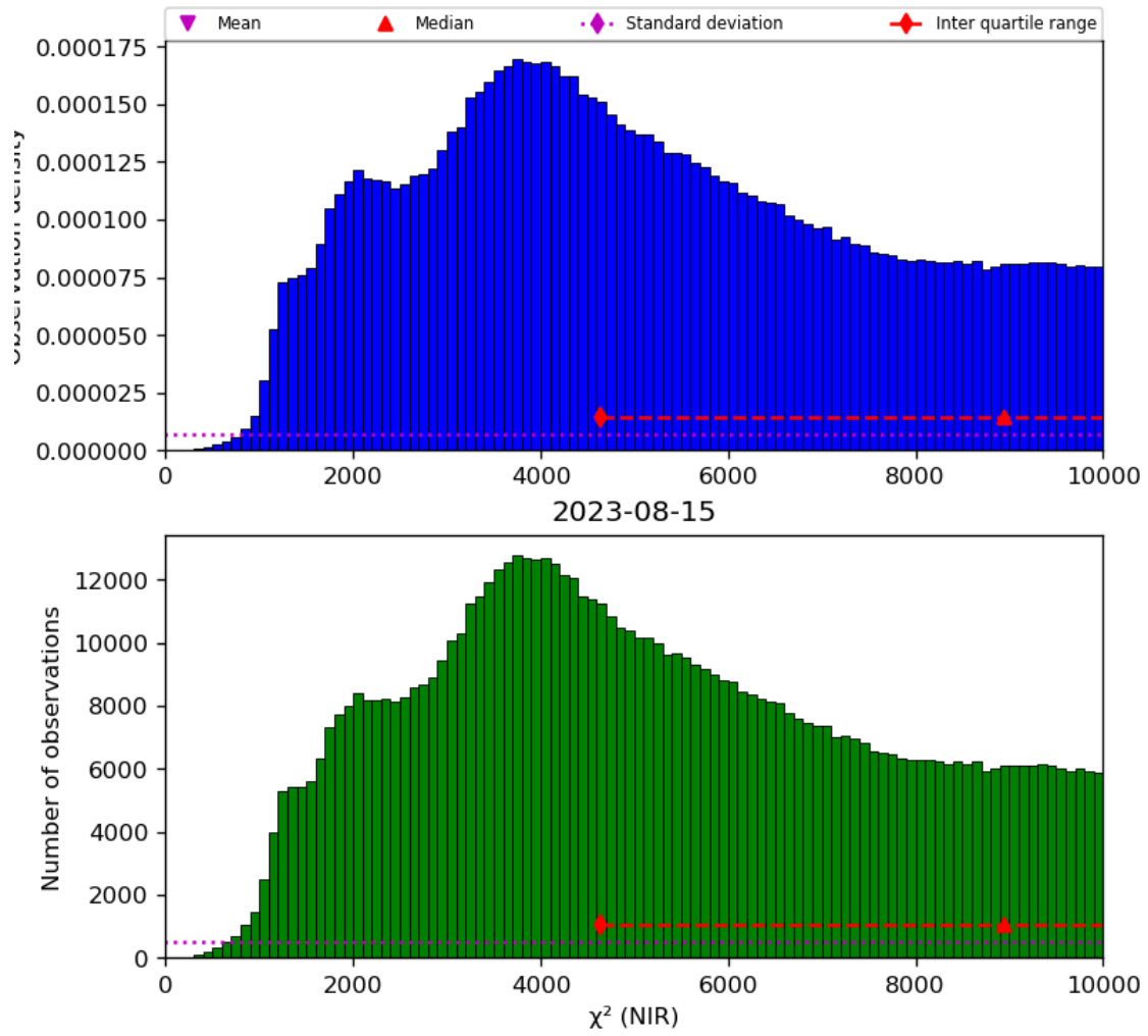
Figure 29: Histogram of “ \chi^2 (NIR)” for 2023-08-14 to 2023-08-16
