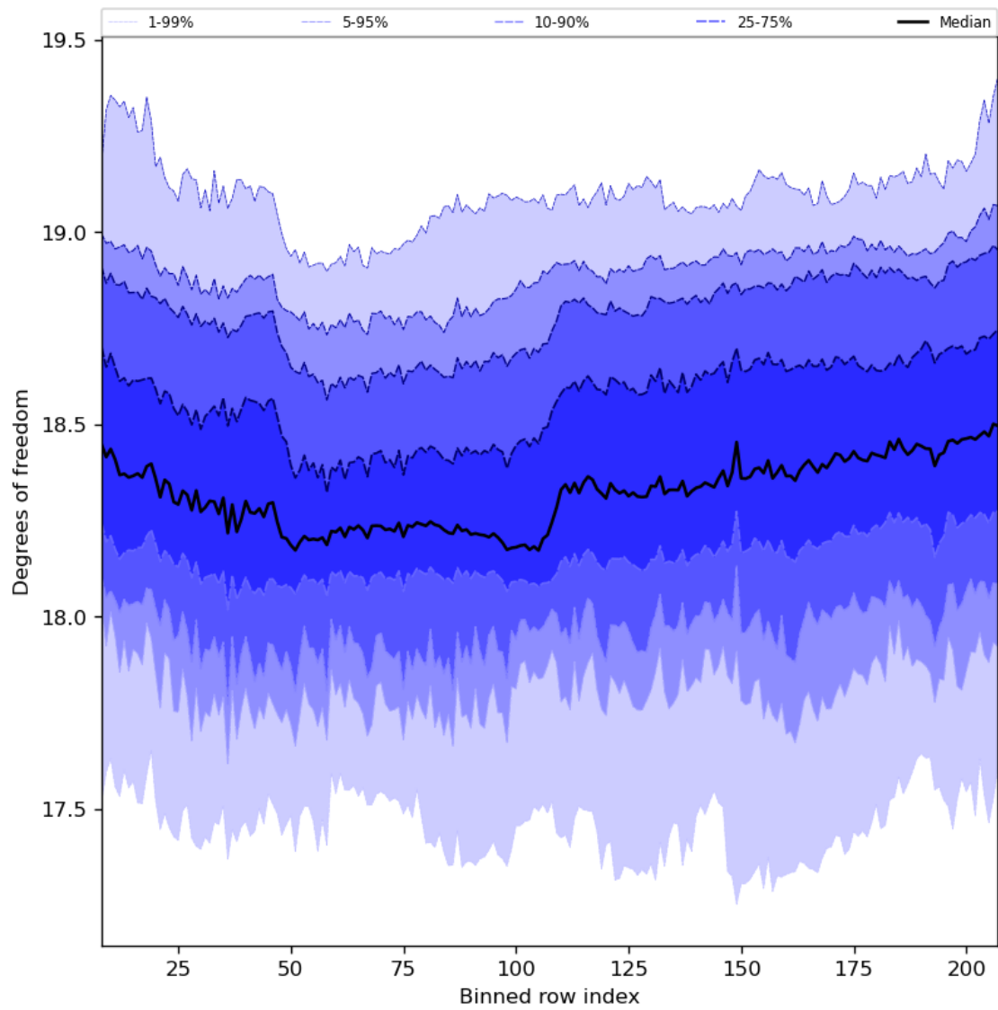
Figure 41: Along track statistics of “Degrees of freedom” for 2023-08-14 to 2023-08-16
