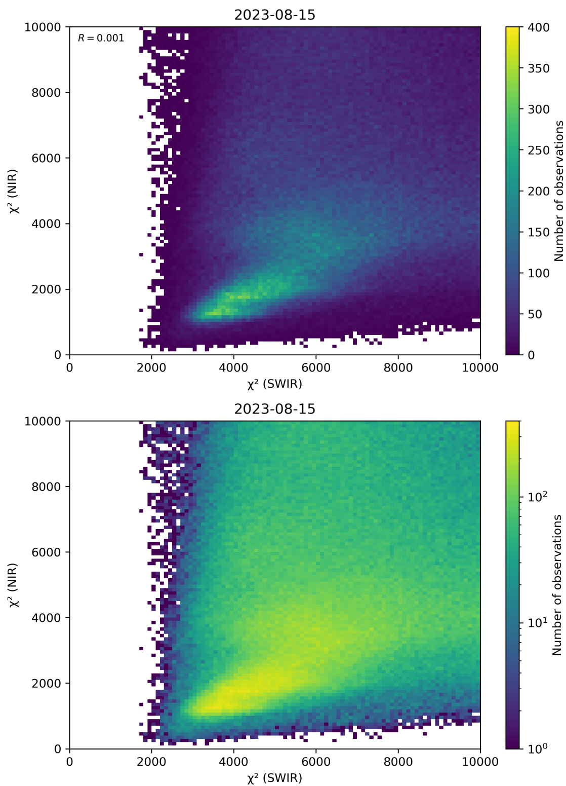
Figure 47: Scatter density plot of “ \chi^2 (SWIR)” against “ \chi^2 (NIR)” for 2023-08-14 to 2023-08-16.
