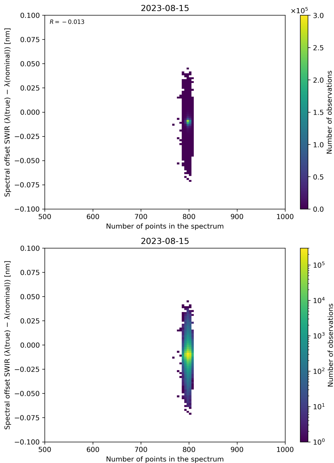
Figure 93: Scatter density plot of “Number of points in the spectrum” against “Spectral offset SWIR ( \lambda(\text{true}) - \lambda(\text{nominal}) )” for 2023-08-14 to 2023-08-16.
