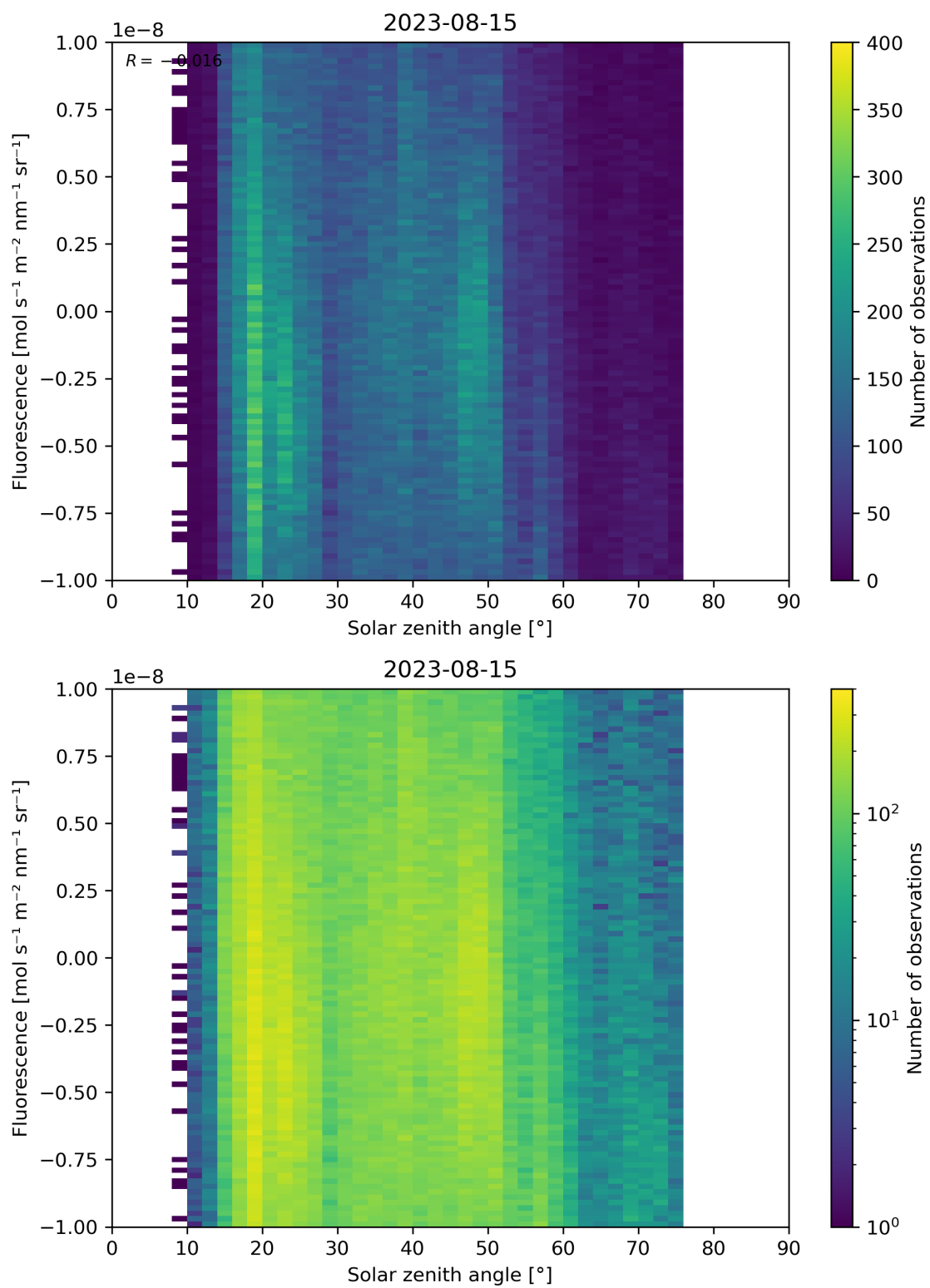
Figure 97: Scatter density plot of “Solar zenith angle” against “Fluorescence” for 2023-08-14 to 2023-08-16.
