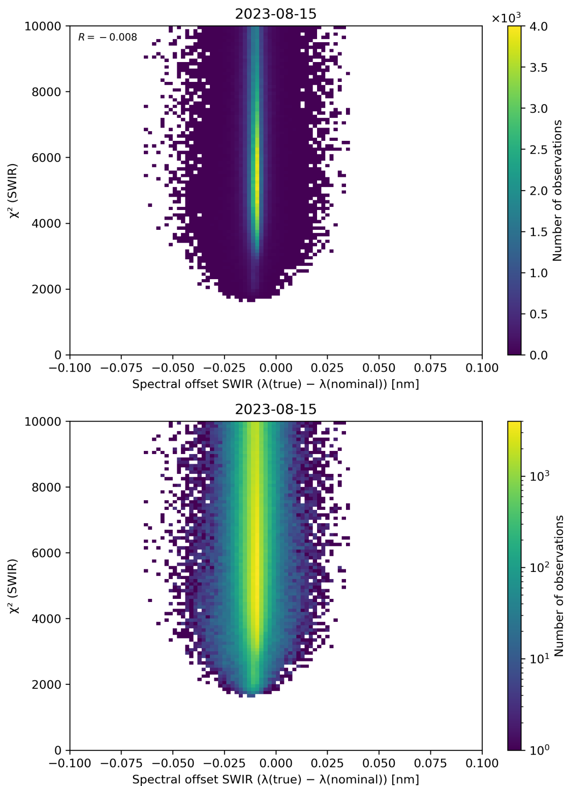
Figure 118: Scatter density plot of “Spectral offset SWIR ( \lambda(\text{true}) - \lambda(\text{nominal}) )” against “ \chi^2 (SWIR)” for 2023-08-14 to 2023-08-16.
