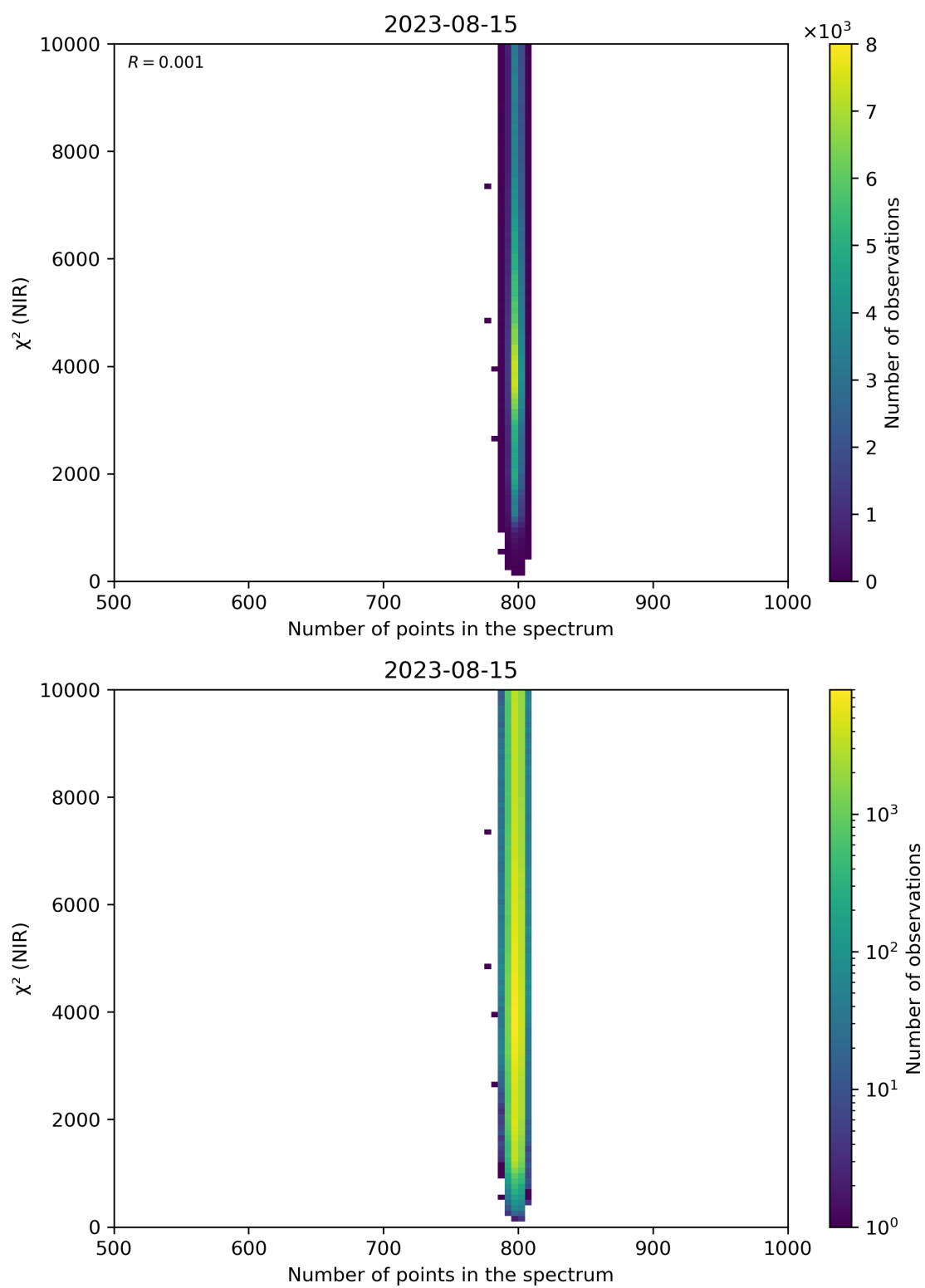
Figure 88: Scatter density plot of “Number of points in the spectrum” against “ \chi^2 (NIR)” for 2023-08-14 to 2023-08-16.
