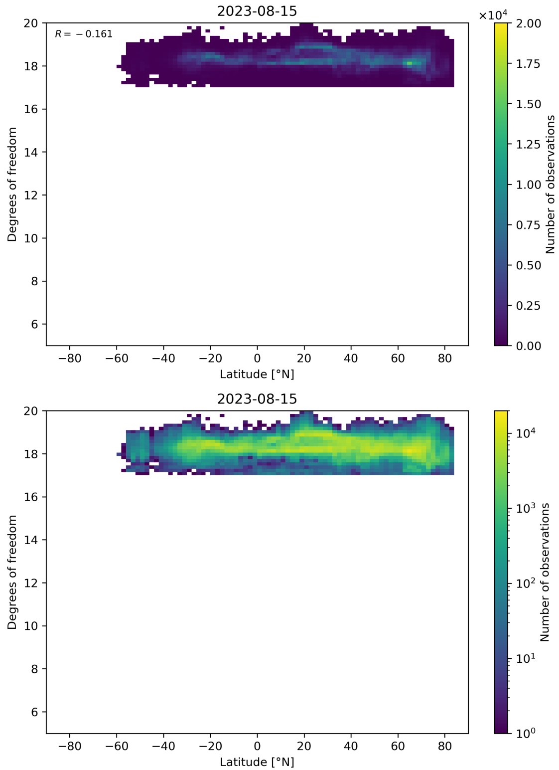
Figure 55: Scatter density plot of “Latitude” against “Degrees of freedom” for 2023-08-14 to 2023-08-16.
