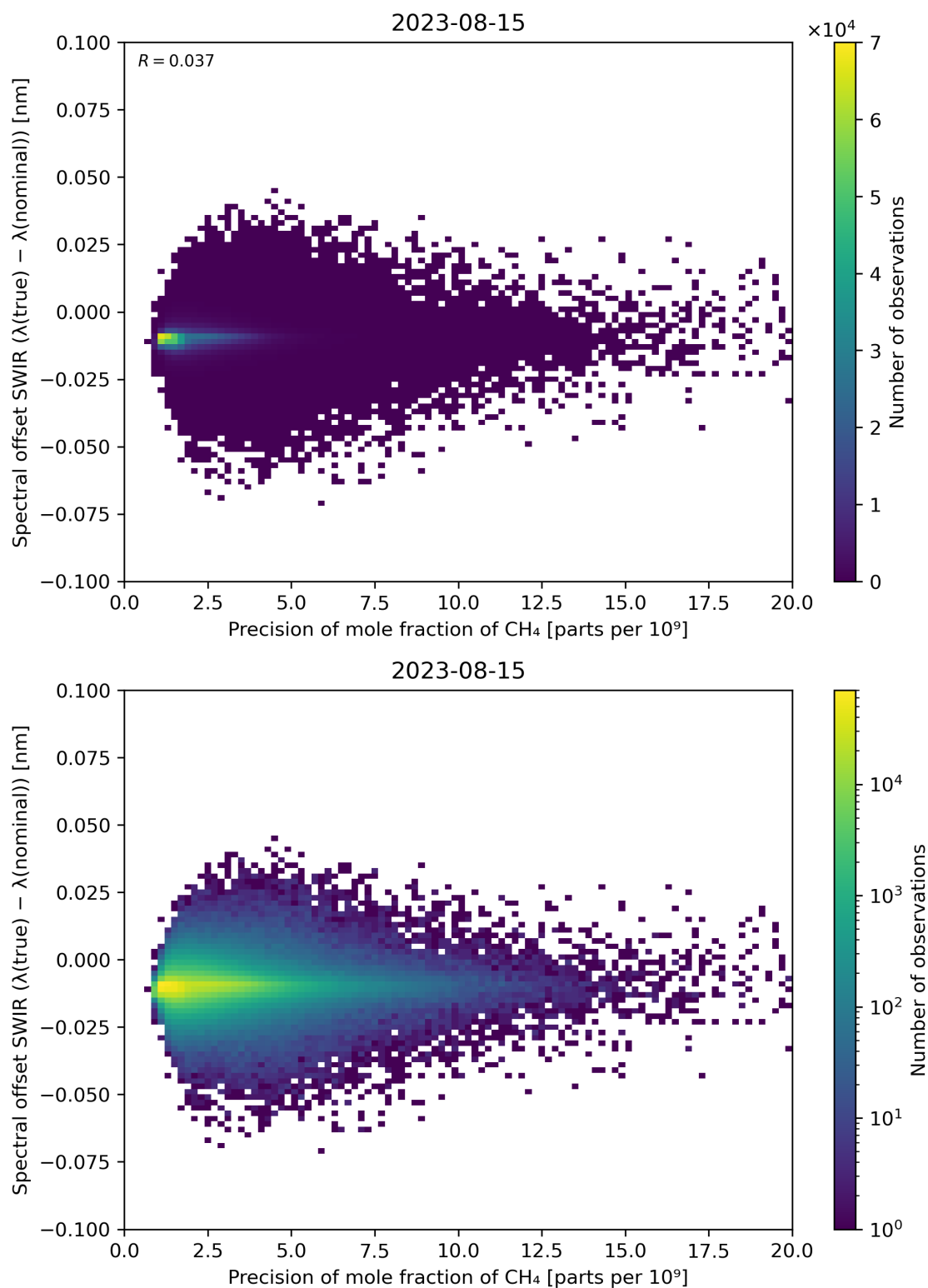
Figure 85: Scatter density plot of “Precision of mole fraction of \text{CH}_4 ” against “Spectral offset SWIR ( \lambda(\text{true}) - \lambda(\text{nominal}) )” for 2023-08-14 to 2023-08-16.
