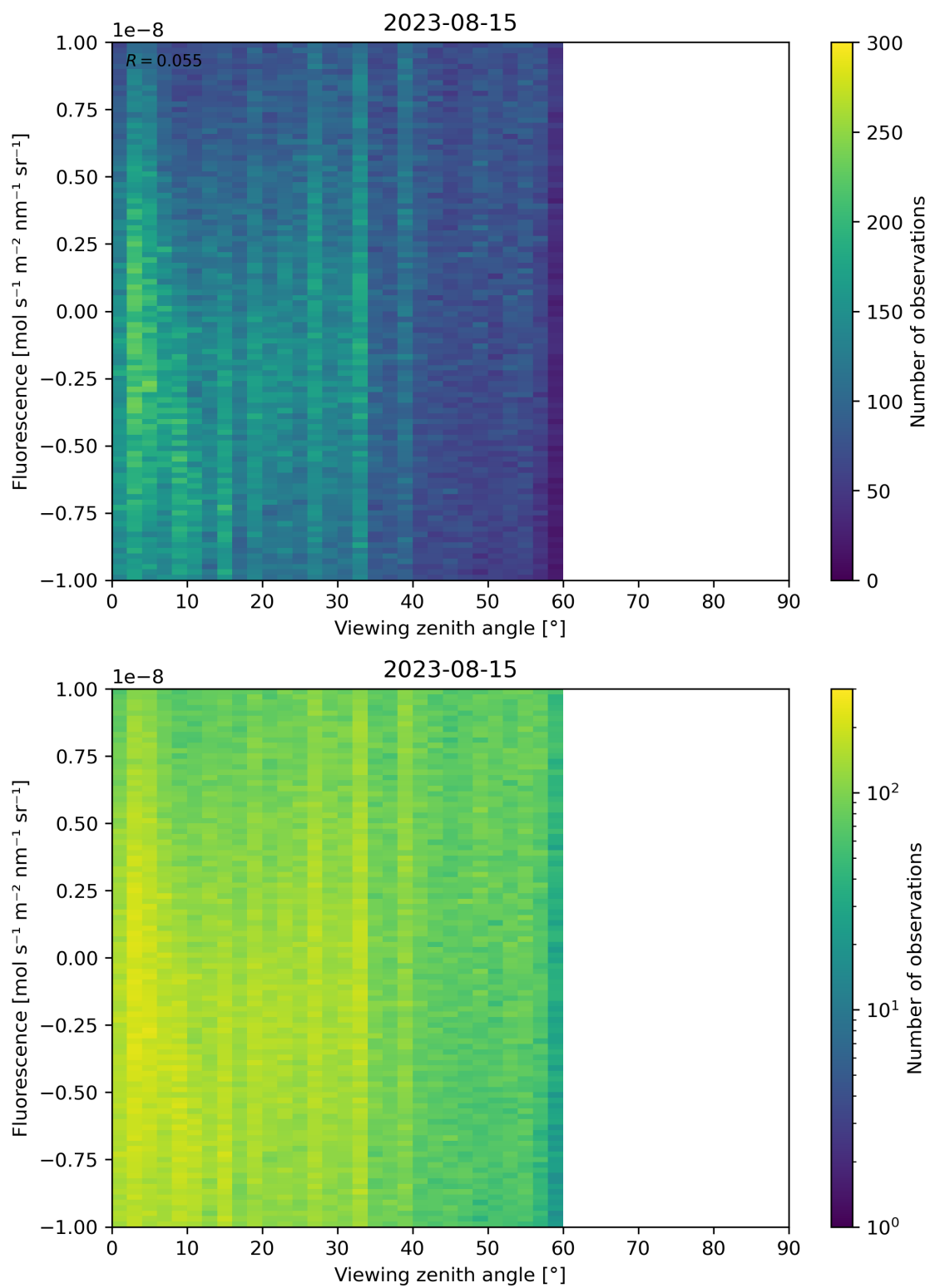
Figure 108: Scatter density plot of “Viewing zenith angle” against “Fluorescence” for 2023-08-14 to 2023-08-16.
