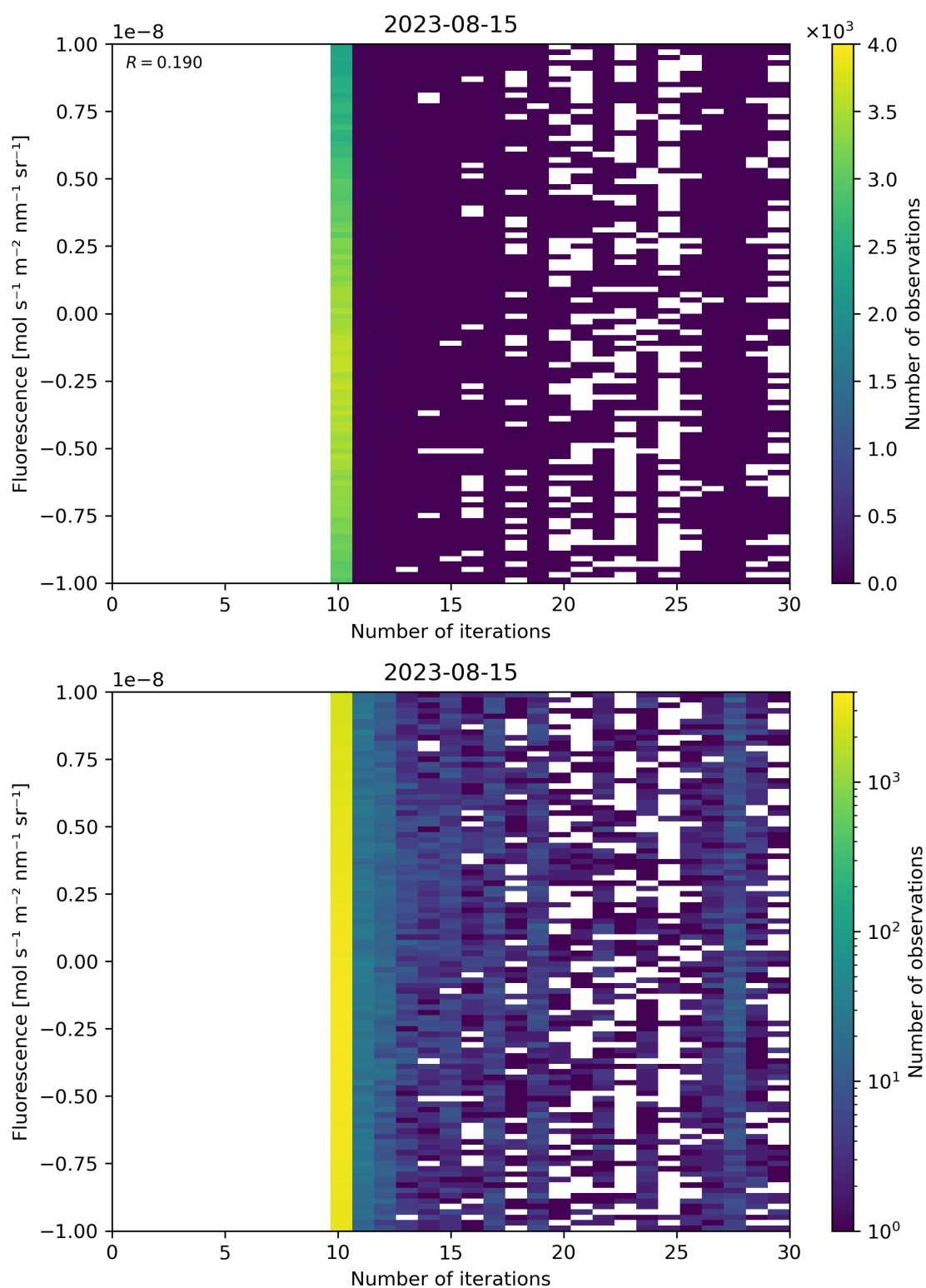
Figure 87: Scatter density plot of “Number of iterations” against “Fluorescence” for 2023-08-14 to 2023-08-16.
