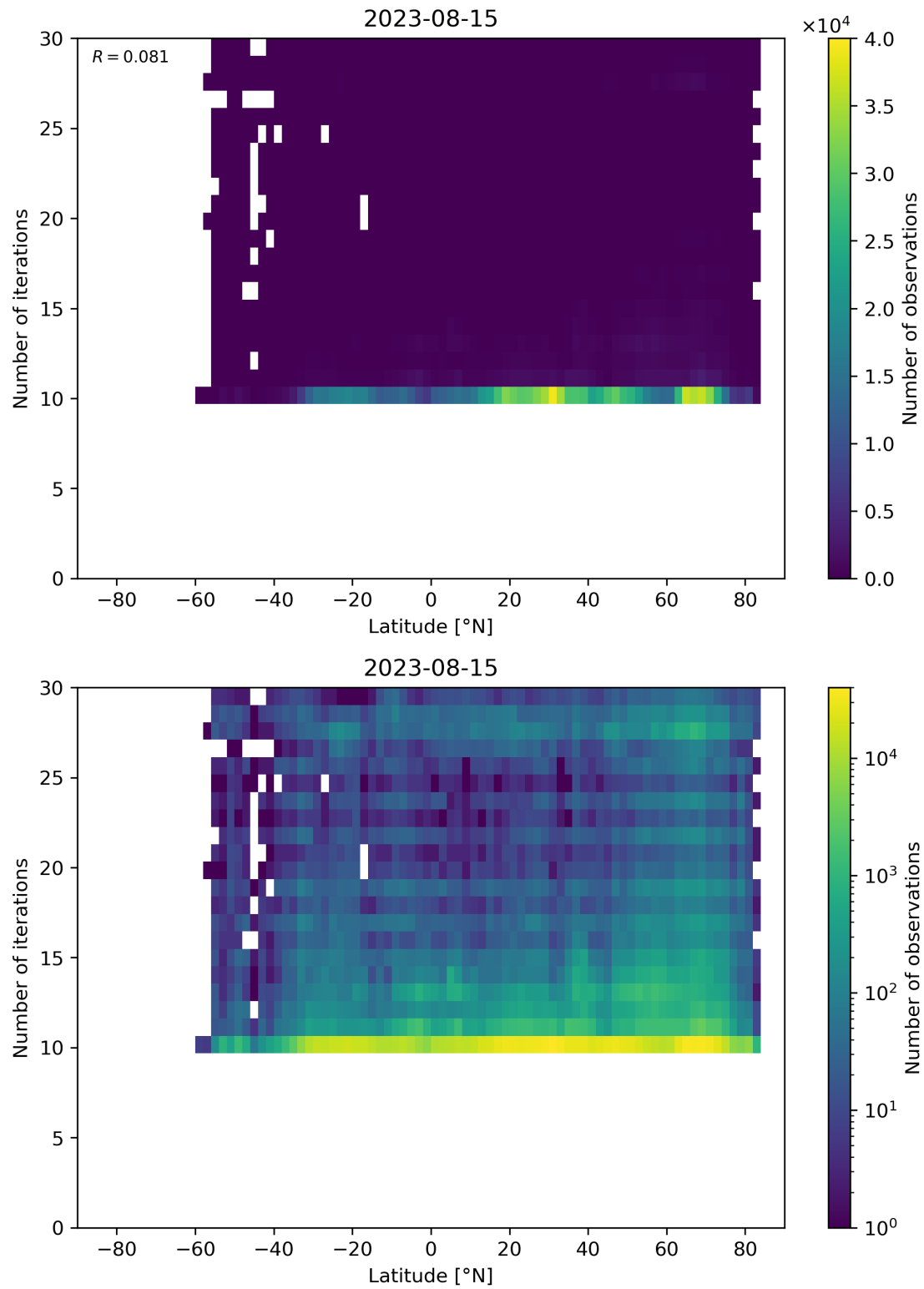
Figure 60: Scatter density plot of “Latitude” against “Number of iterations” for 2023-08-14 to 2023-08-16.
