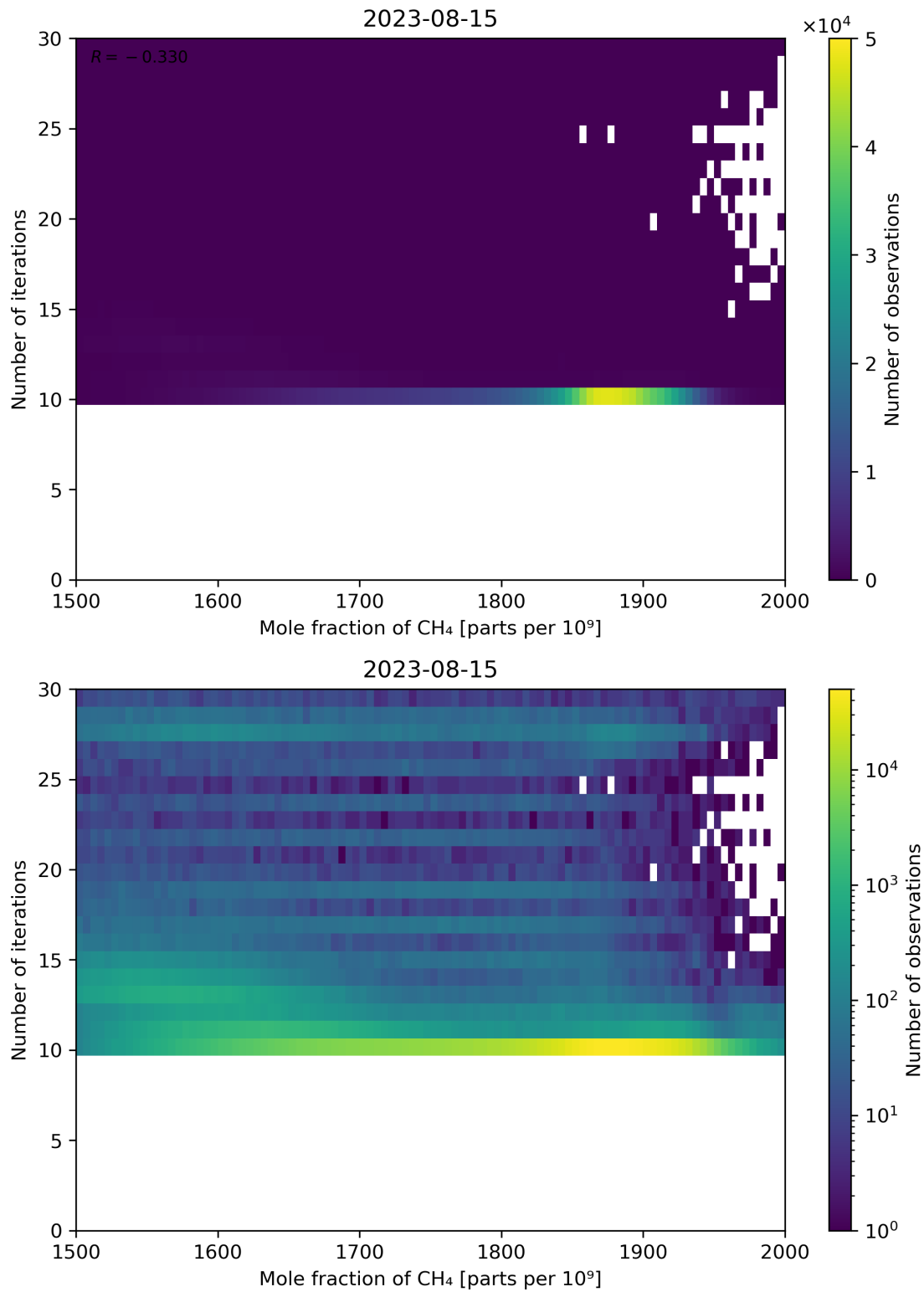
Figure 76: Scatter density plot of “Mole fraction of CH 4 ” against “Number of iterations” for 2023-08-14 to 2023-08-16.
