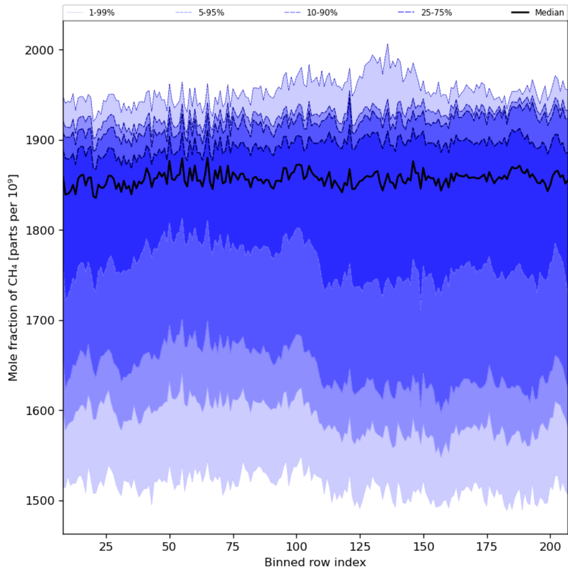
Figure 34: Along track statistics of “Mole fraction of CH 4 ” for 2023-08-14 to 2023-08-16
