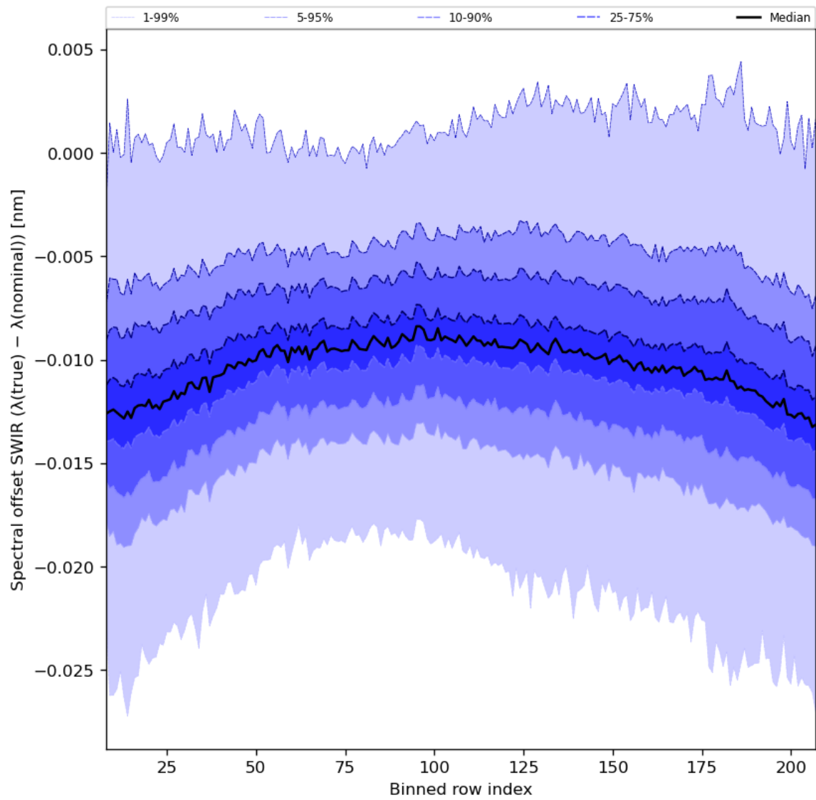
Figure 38: Along track statistics of “Spectral offset SWIR ( \lambda(\text{true}) - \lambda(\text{nominal}) )” for 2023-08-14 to 2023-08-16
