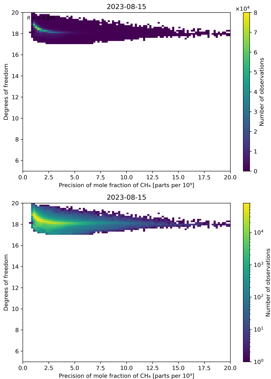
Figure 80: Scatter density plot of “Precision of mole fraction of CH 4 ” against “Degrees of freedom” for 2023-08-14 to 2023-08-16.
