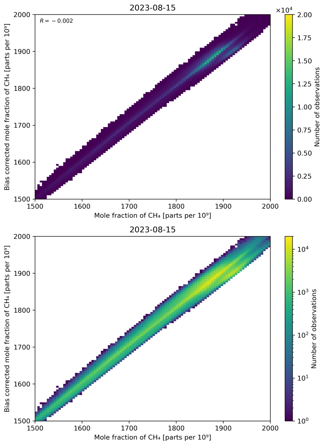
Figure 74: Scatter density plot of “Mole fraction of CH 4 ” against “Bias corrected mole fraction of CH 4 ” for 2023-08-14 to 2023-08-16.
