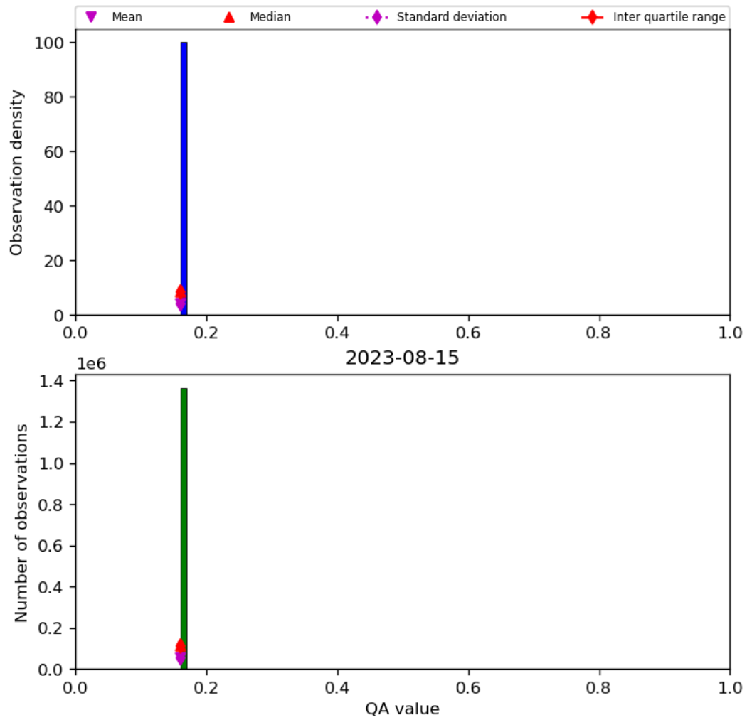
Figure 22: Histogram of “QA value” for 2023-08-14 to 2023-08-16
