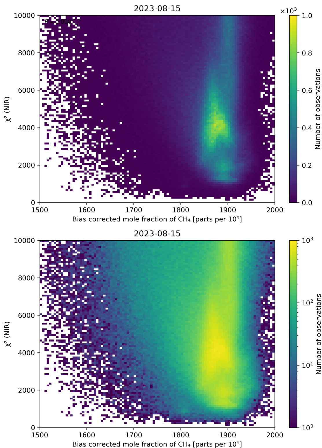
Figure 63: Scatter density plot of “Bias corrected mole fraction of CH 4 ” against “ \chi^2 (NIR)” for 2023-08-14 to 2023-08-16.
