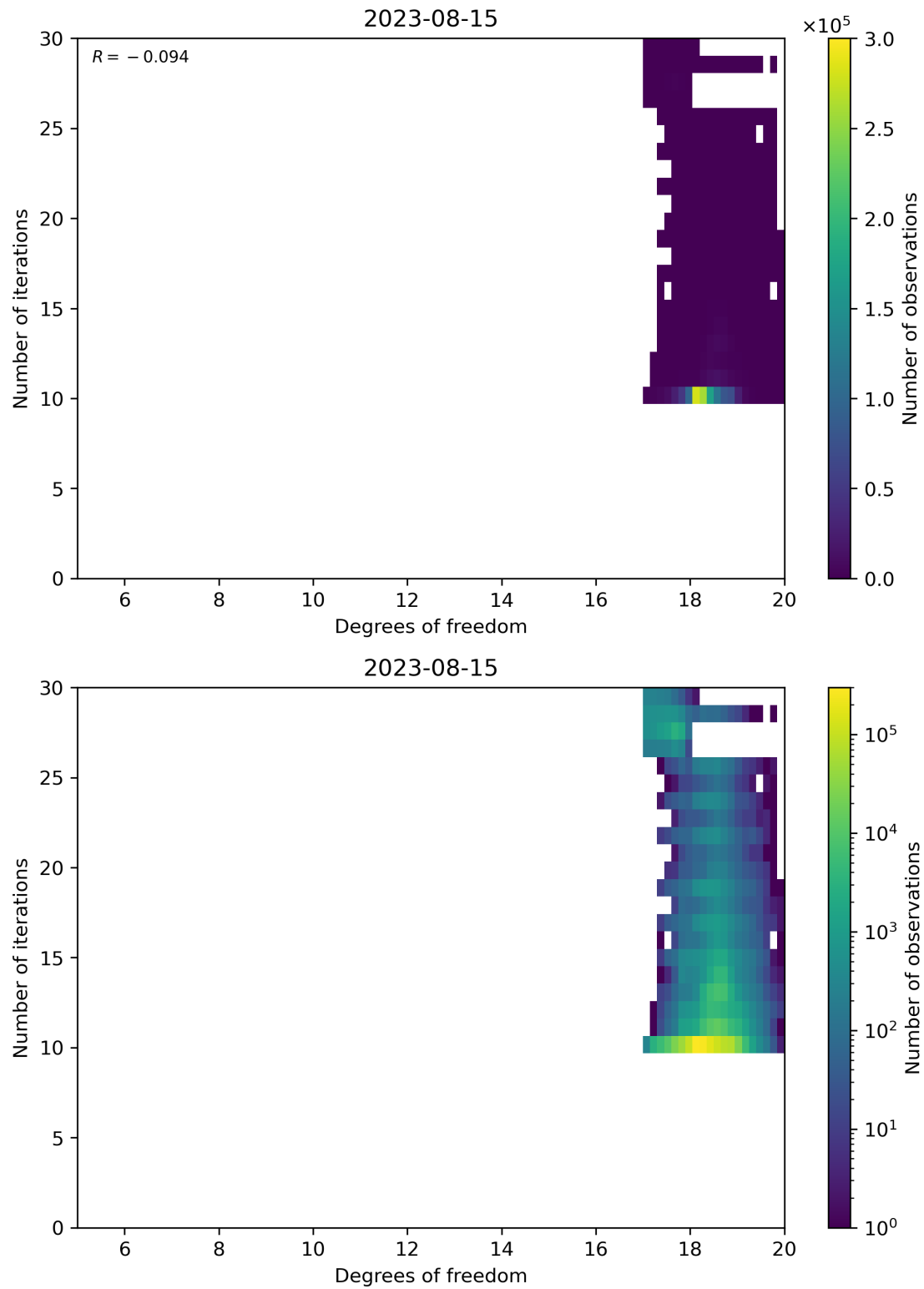
Figure 52: Scatter density plot of “Degrees of freedom” against “Number of iterations” for 2023-08-14 to 2023-08-16.
