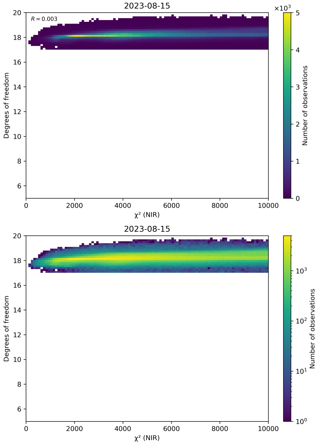
Figure 44: Scatter density plot of “ \chi^2 (NIR)” against “Degrees of freedom” for 2023-08-14 to 2023-08-16.
