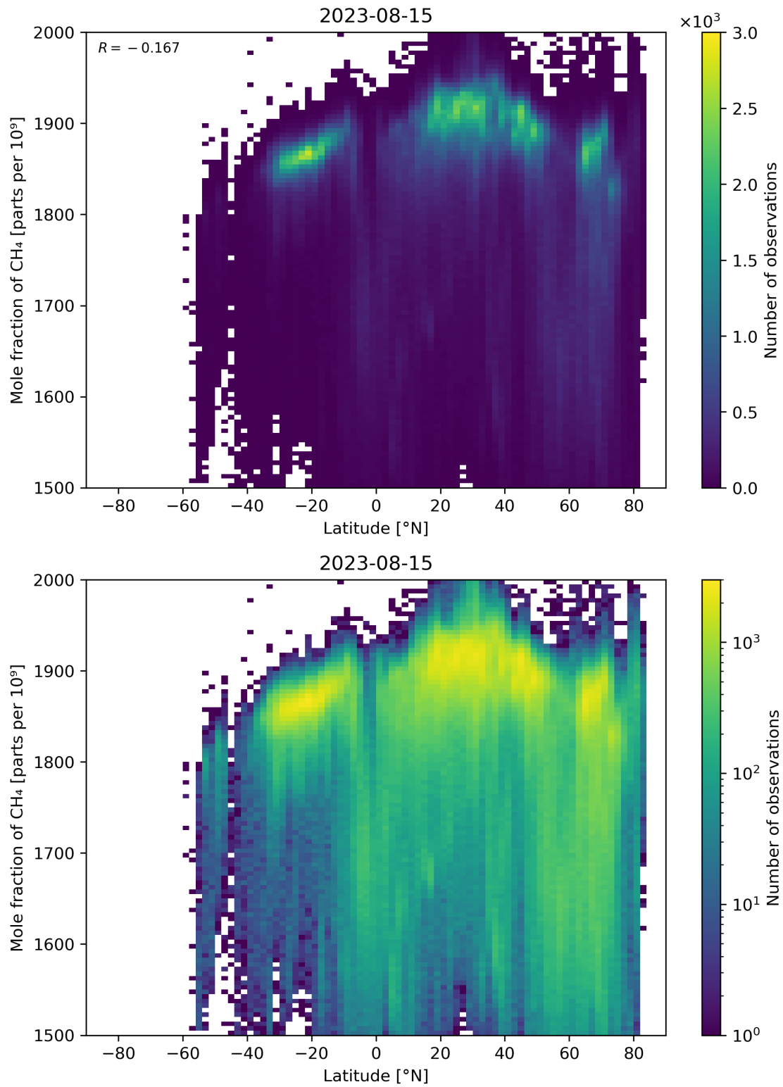
Figure 57: Scatter density plot of “Latitude” against “Mole fraction of CH 4 ” for 2023-08-14 to 2023-08-16.
