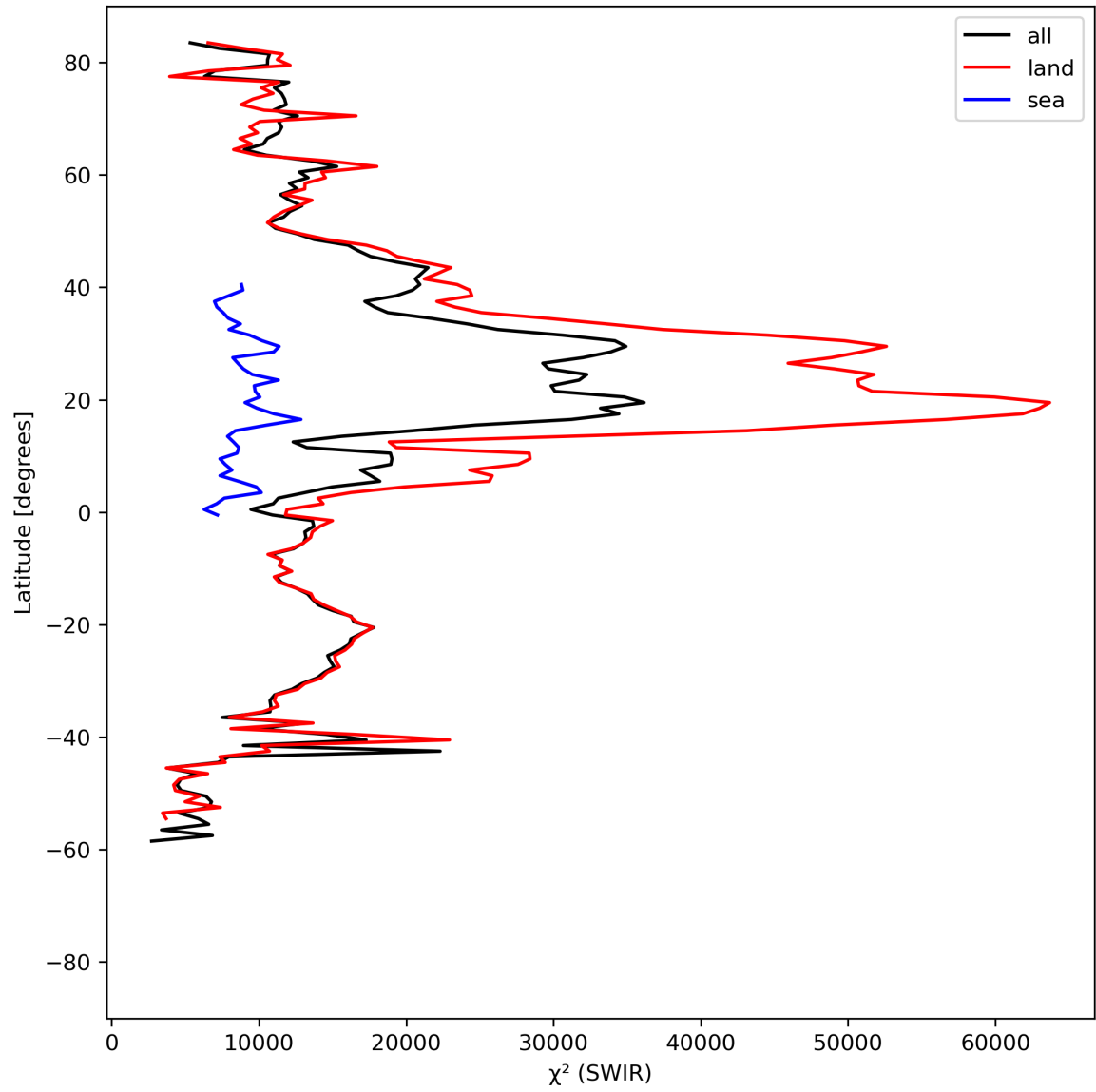
Figure 17: Zonal average of “ \chi^2 (SWIR)” for 2023-08-14 to 2023-08-16.
