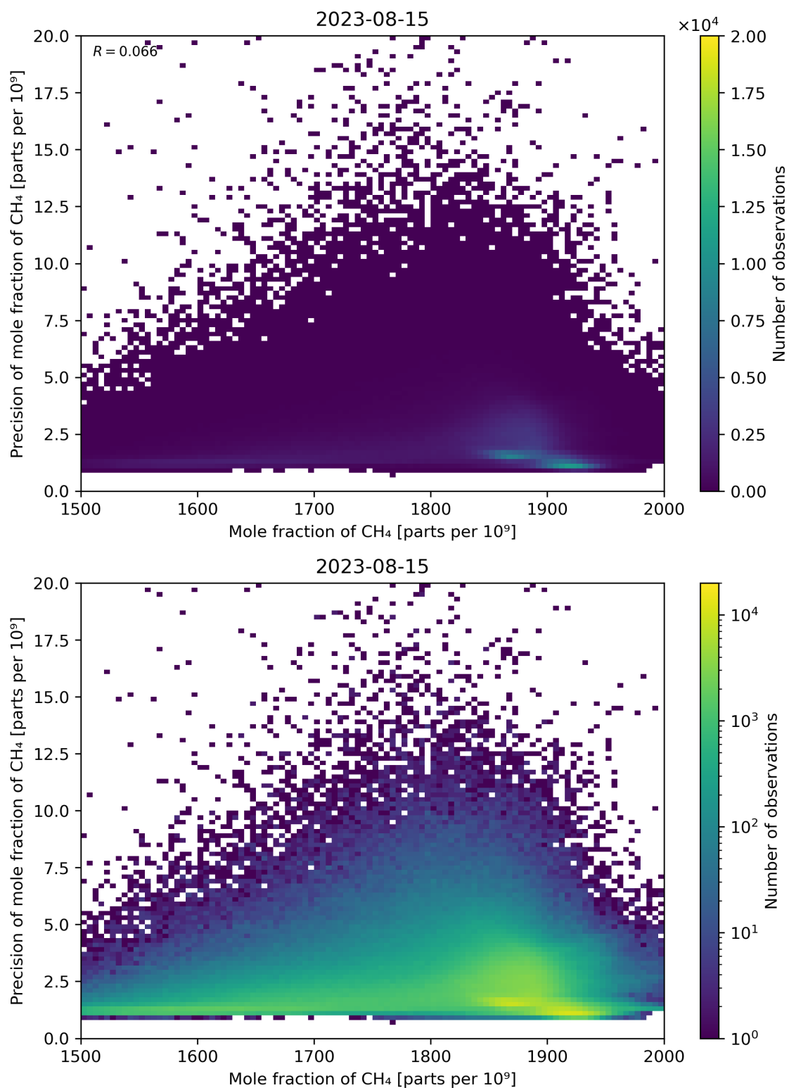
Figure 75: Scatter density plot of “Mole fraction of CH 4 ” against “Precision of mole fraction of CH 4 ” for 2023-08-14 to 2023-08-16.
