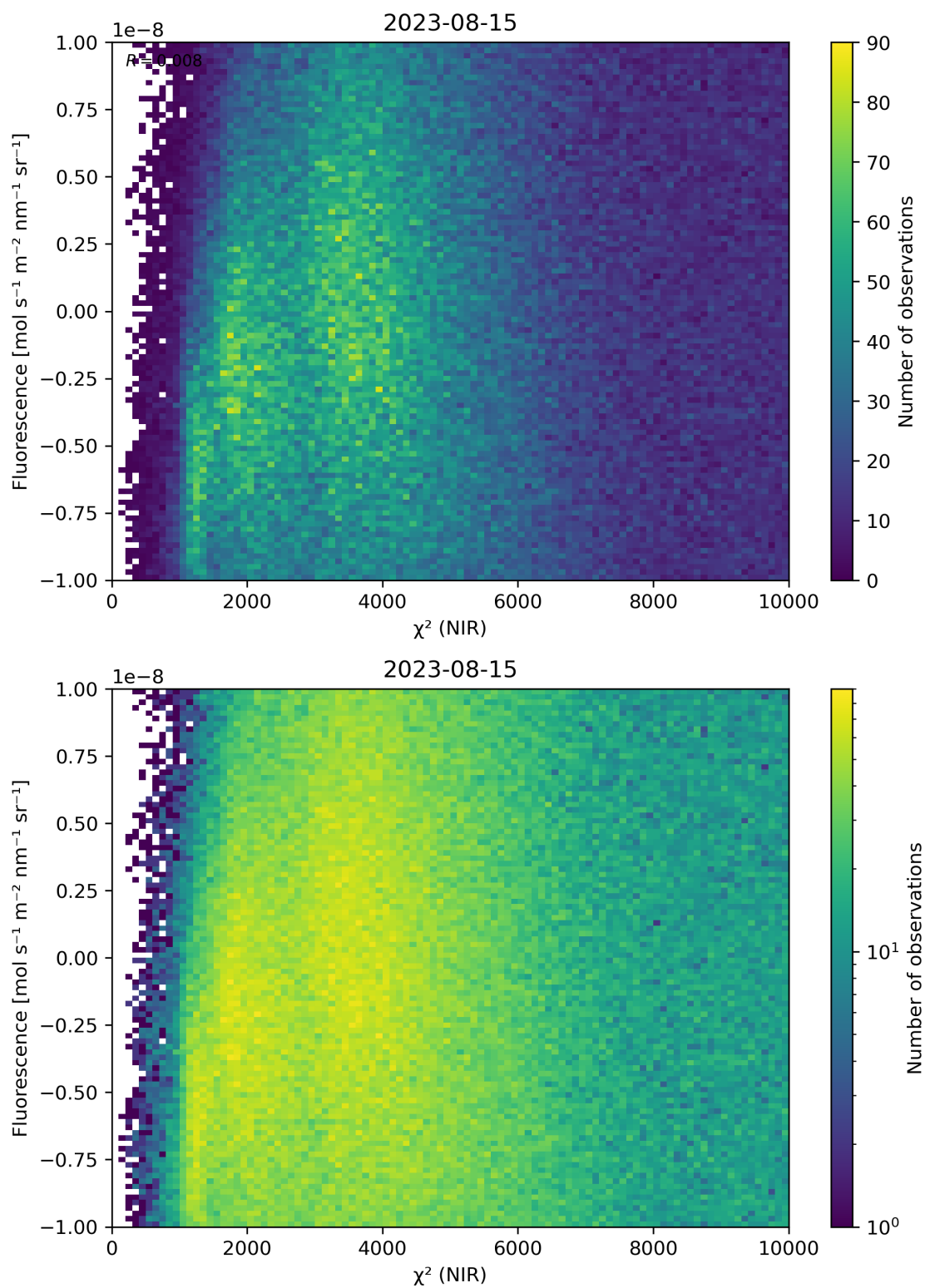
Figure 45: Scatter density plot of “ \chi^2 (NIR)” against “Fluorescence” for 2023-08-14 to 2023-08-16.
