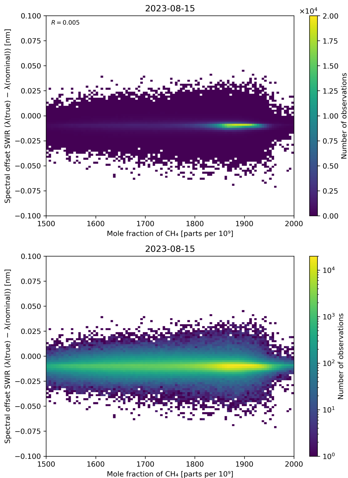
Figure 86: Scatter density plot of “Mole fraction of CH 4 ” against “Spectral offset SWIR ( \lambda(\text{true}) - \lambda(\text{nominal}) )” for 2023-08-14 to 2023-08-16.
