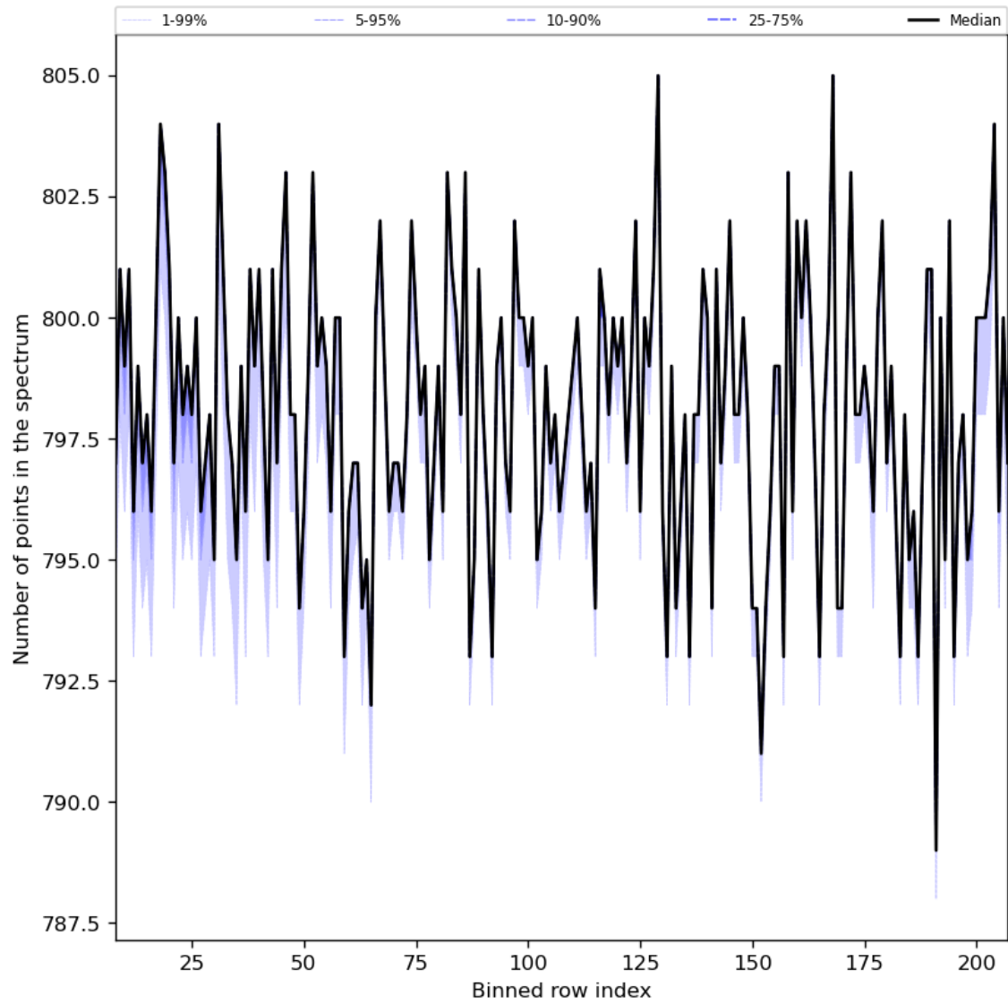
Figure 37: Along track statistics of “Number of points in the spectrum” for 2023-08-14 to 2023-08-16
