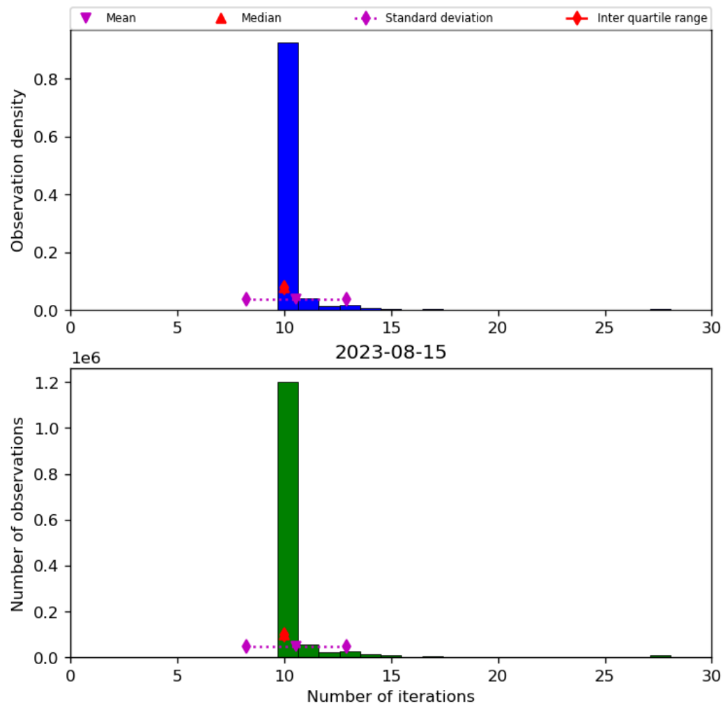
Figure 31: Histogram of “Number of iterations” for 2023-08-14 to 2023-08-16
