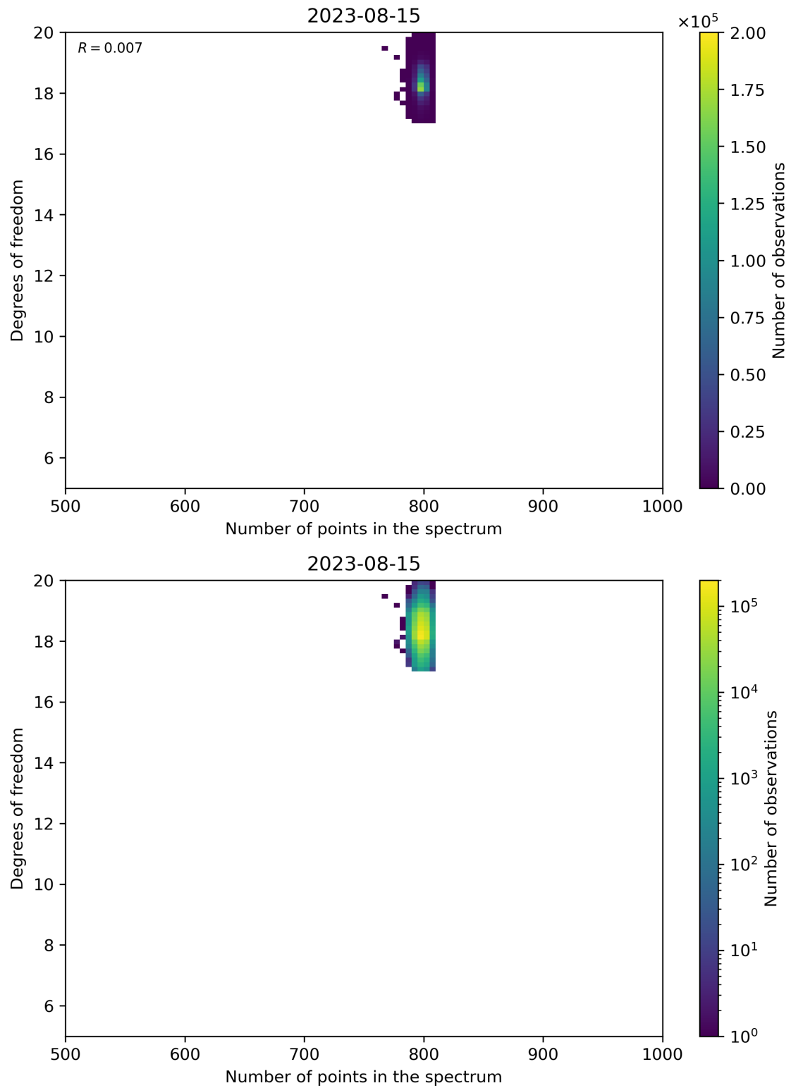
Figure 90: Scatter density plot of “Number of points in the spectrum” against “Degrees of freedom” for 2023-08-14 to 2023-08-16.
