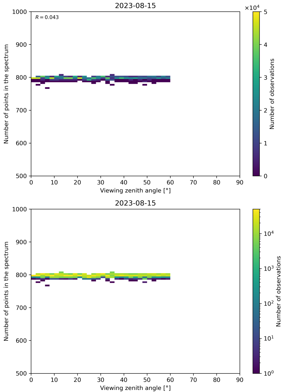
Figure 114: Scatter density plot of “Viewing zenith angle” against “Number of points in the spectrum” for 2023-08-14 to 2023-08-16.
