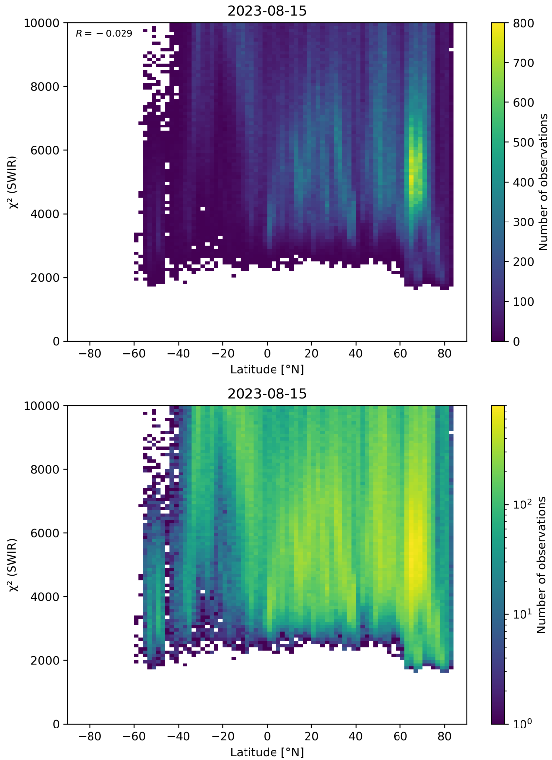
Figure 54: Scatter density plot of “Latitude” against “ \chi^2 (SWIR)” for 2023-08-14 to 2023-08-16.
