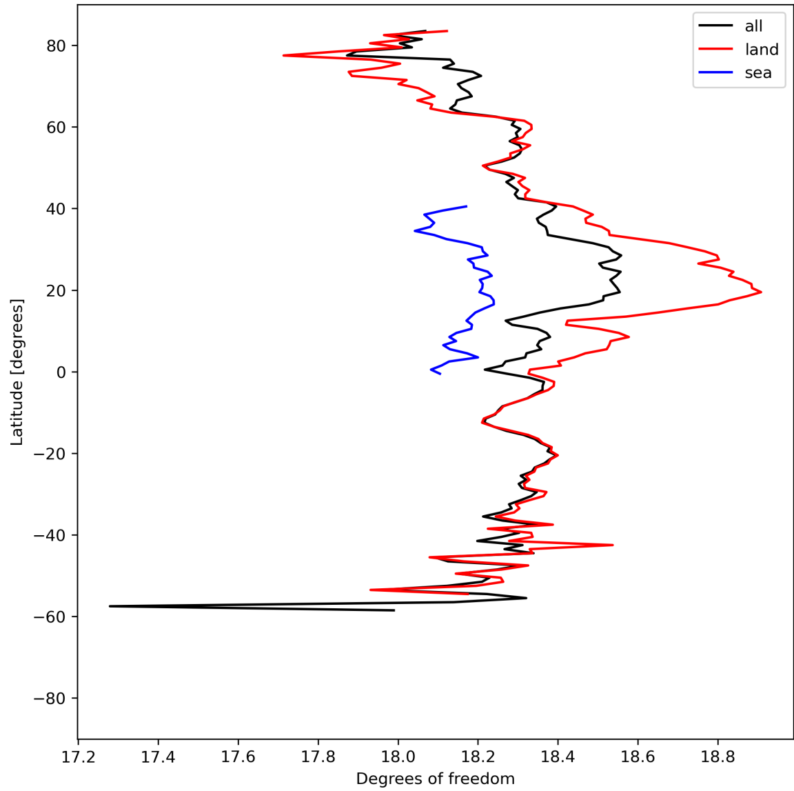
Figure 19: Zonal average of “Degrees of freedom” for 2023-08-14 to 2023-08-16.
