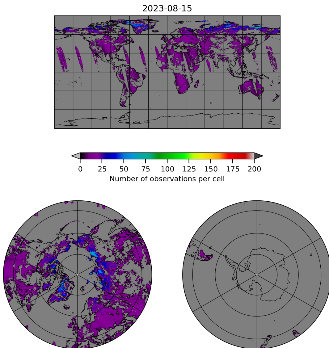
Figure 10: Map of the number of observations for 2023-08-14 to 2023-08-16
