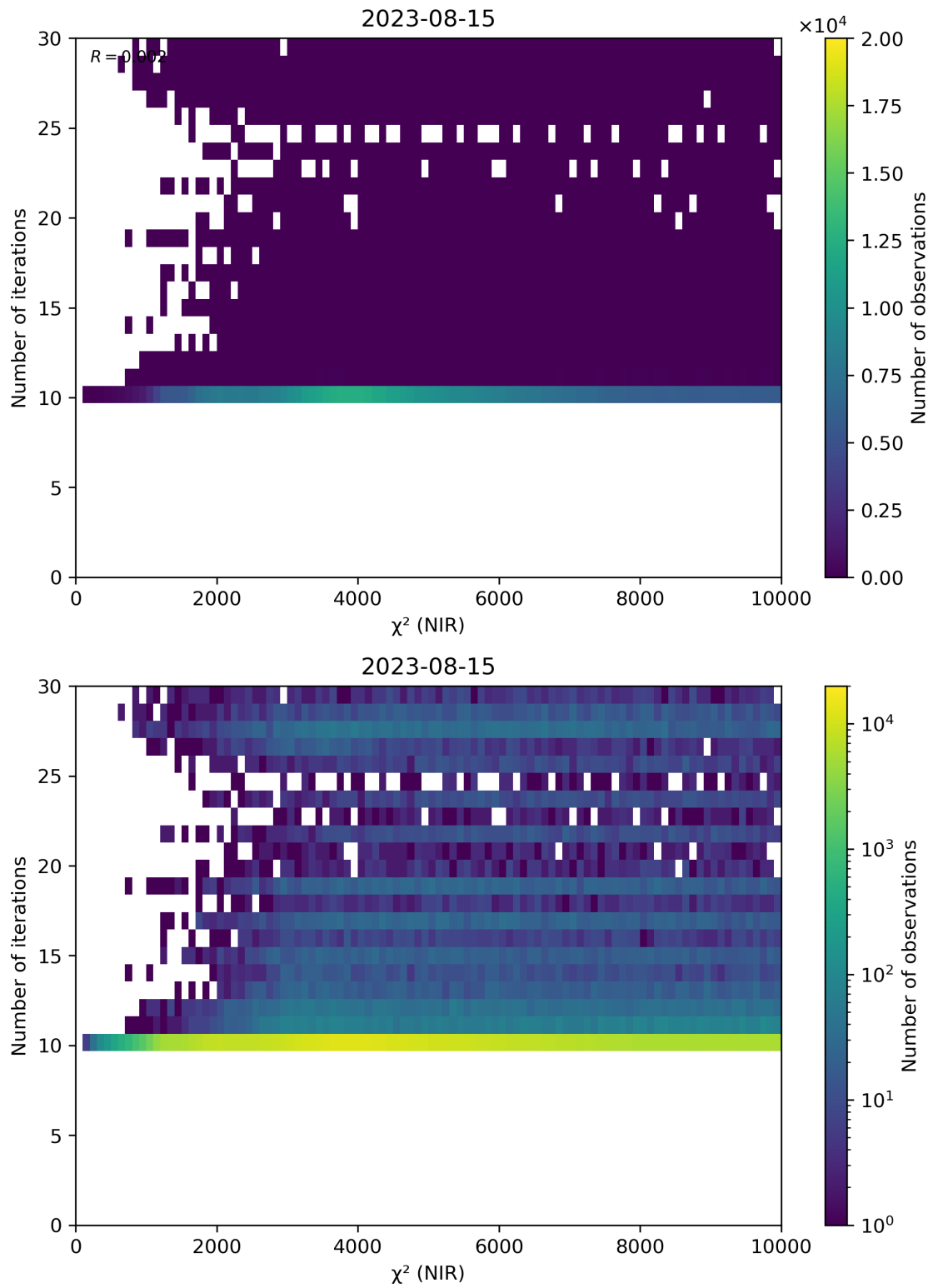
Figure 46: Scatter density plot of “ \chi^2 (NIR)” against “Number of iterations” for 2023-08-14 to 2023-08-16.
