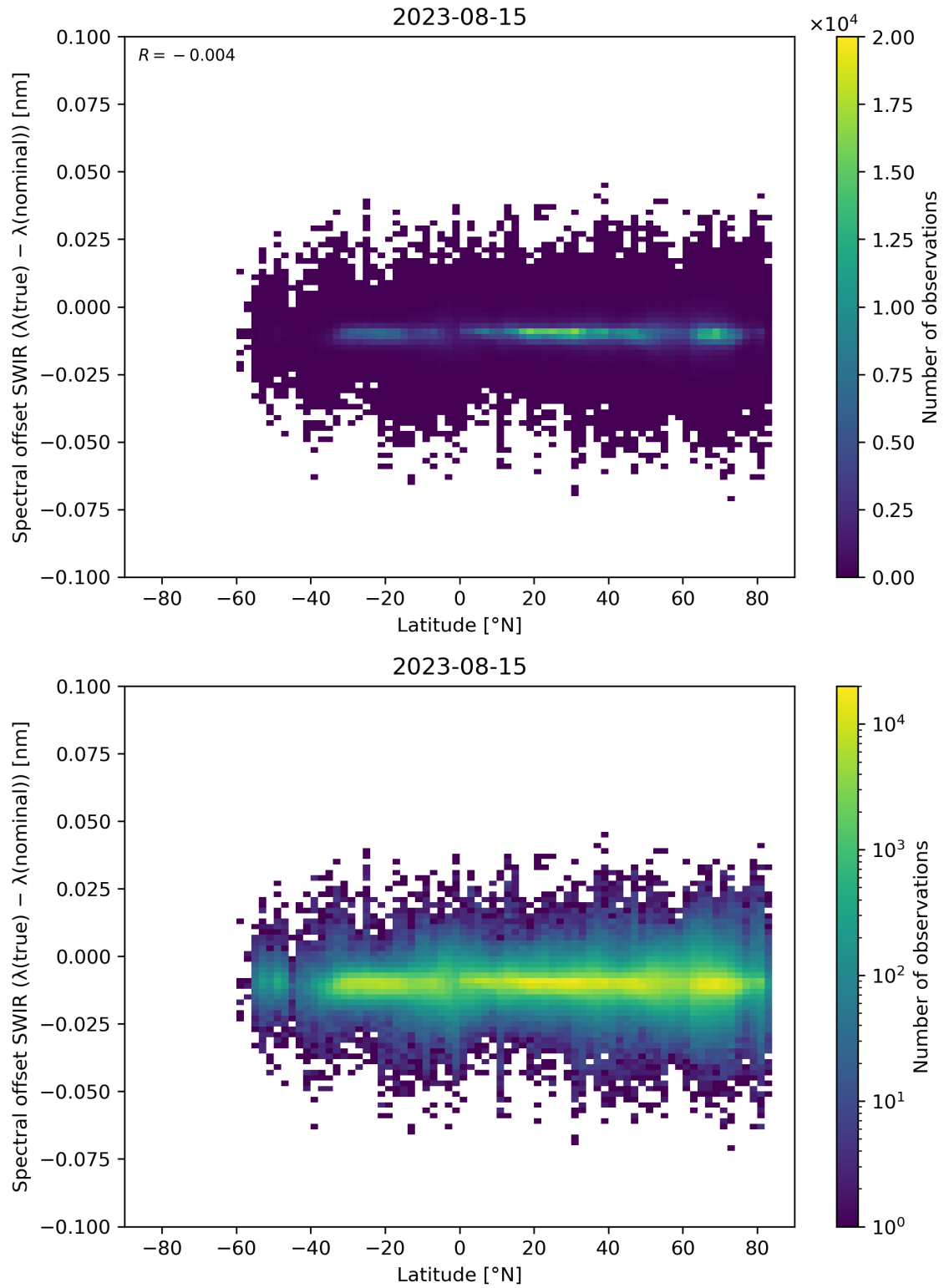
Figure 62: Scatter density plot of “Latitude” against “Spectral offset SWIR ( \lambda(\text{true}) - \lambda(\text{nominal}) )” for 2023-08-14 to 2023-08-16.
