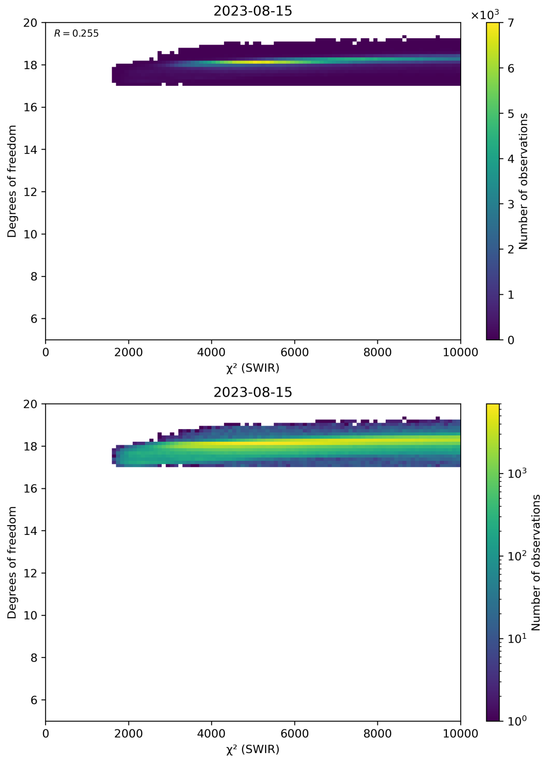
Figure 48: Scatter density plot of “ \chi^2 (SWIR)” against “Degrees of freedom” for 2023-08-14 to 2023-08-16.
