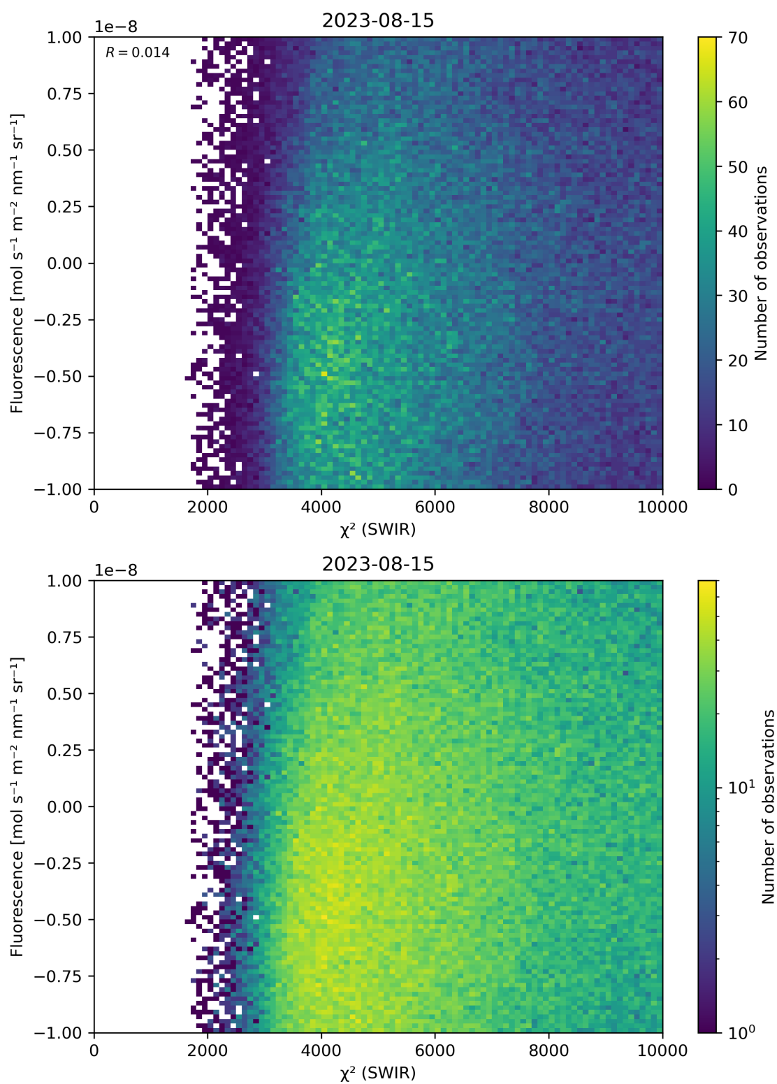
Figure 49: Scatter density plot of “ \chi^2 (SWIR)” against “Fluorescence” for 2023-08-14 to 2023-08-16.
