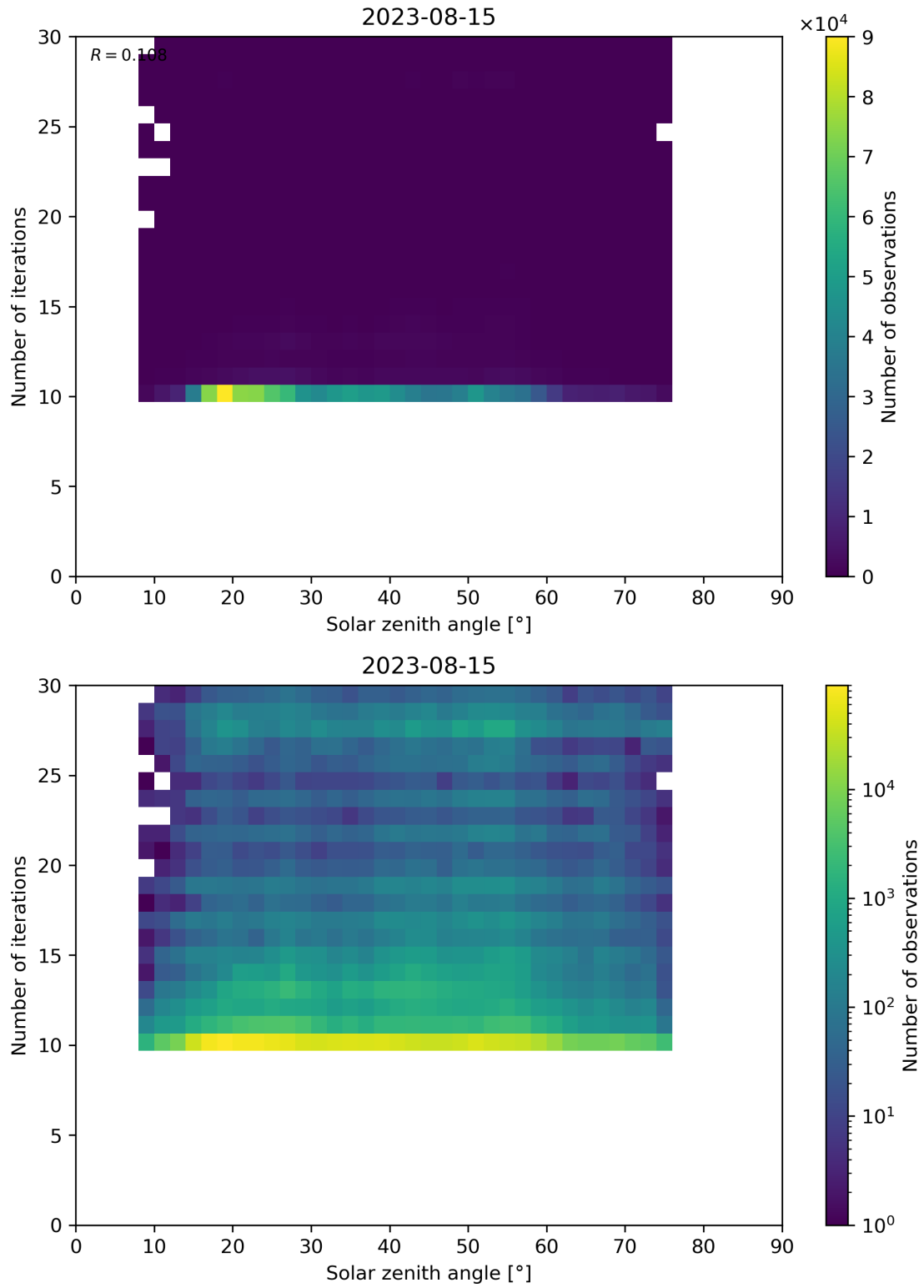
Figure 102: Scatter density plot of “Solar zenith angle” against “Number of iterations” for 2023-08-14 to 2023-08-16.
