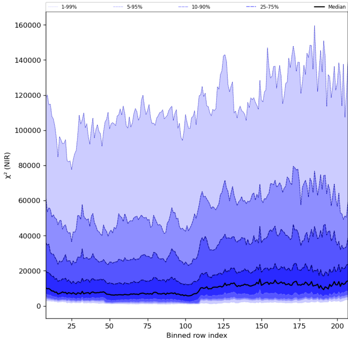
Figure 40: Along track statistics of “ \chi^2 (NIR)” for 2023-08-14 to 2023-08-16
