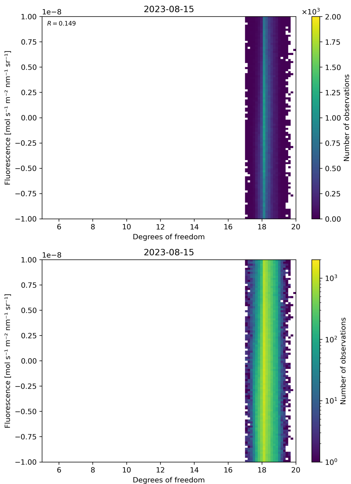
Figure 51: Scatter density plot of “Degrees of freedom” against “Fluorescence” for 2023-08-14 to 2023-08-16.
