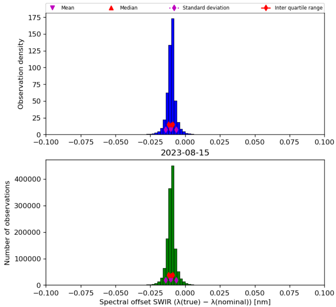
Figure 27: Histogram of “Spectral offset SWIR ( \lambda(\text{true}) - \lambda(\text{nominal}) )” for 2023-08-14 to 2023-08-16
