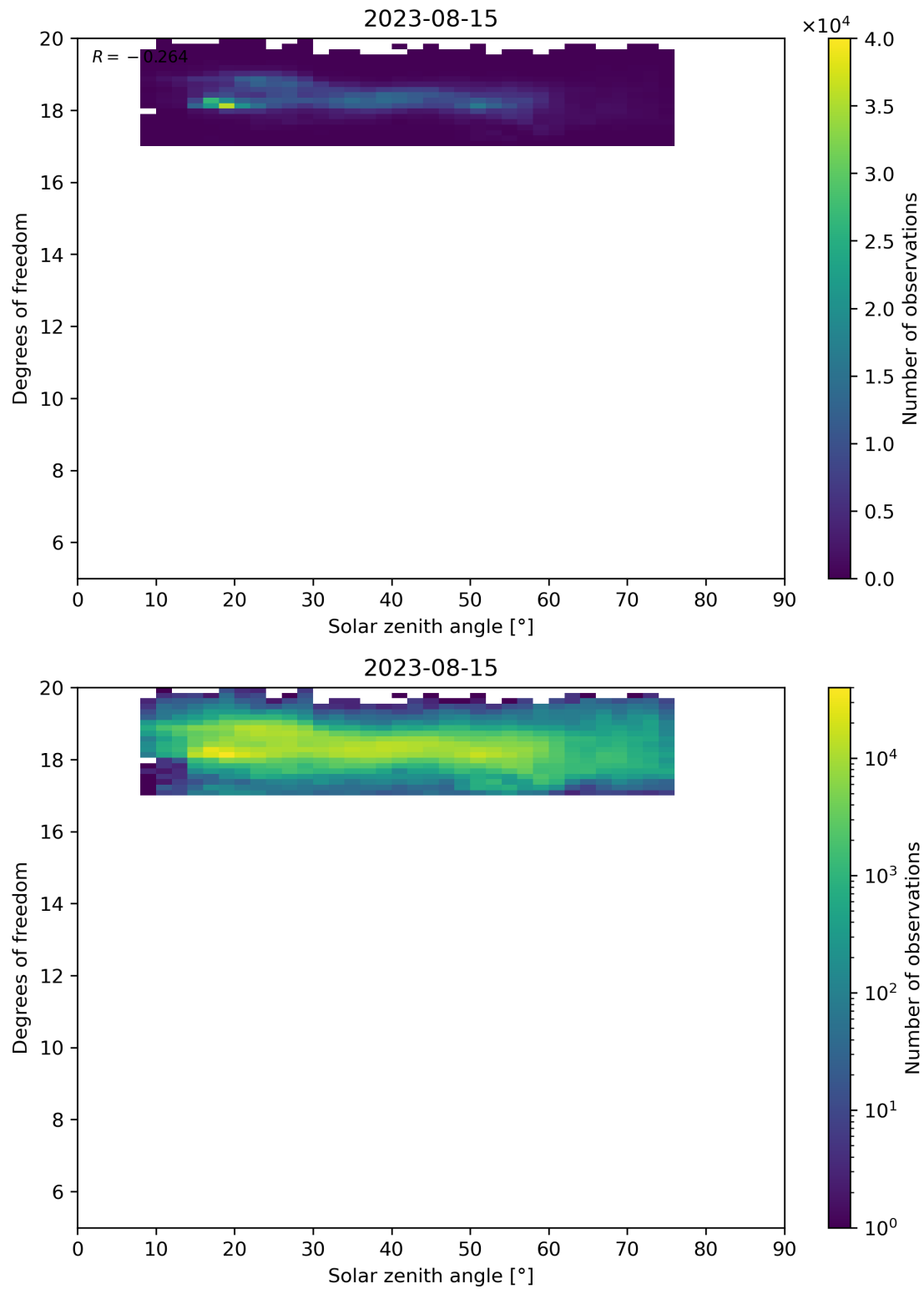
Figure 96: Scatter density plot of “Solar zenith angle” against “Degrees of freedom” for 2023-08-14 to 2023-08-16.
