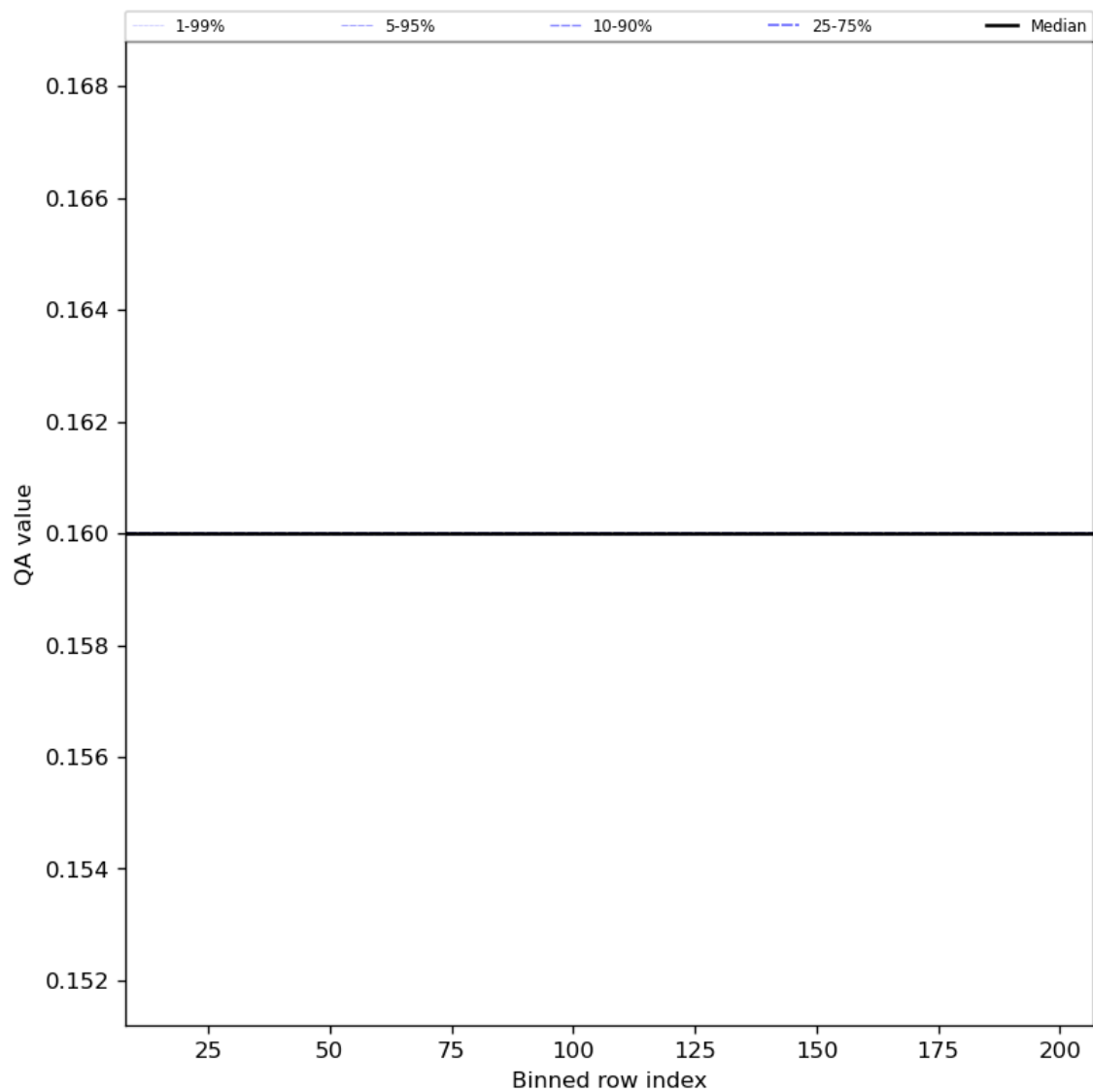
Figure 33: Along track statistics of “QA value” for 2023-08-14 to 2023-08-16
