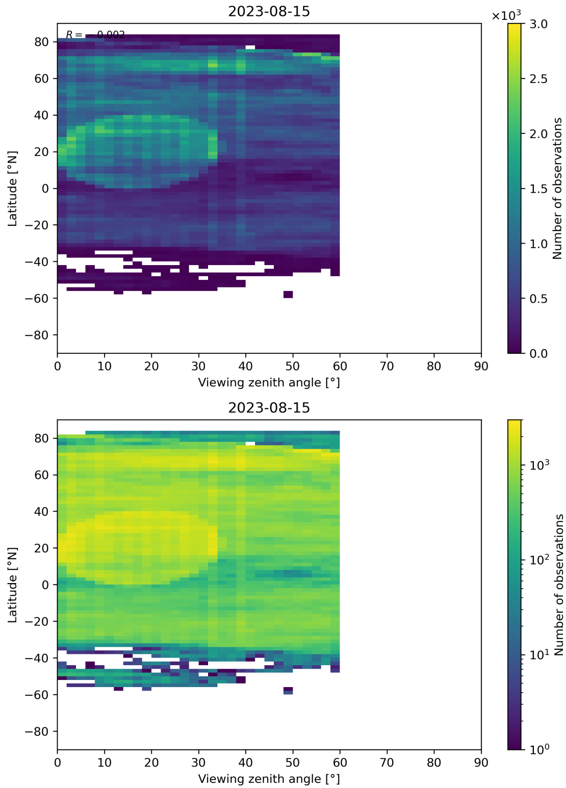
Figure 109: Scatter density plot of “Viewing zenith angle” against “Latitude” for 2023-08-14 to 2023-08-16.
