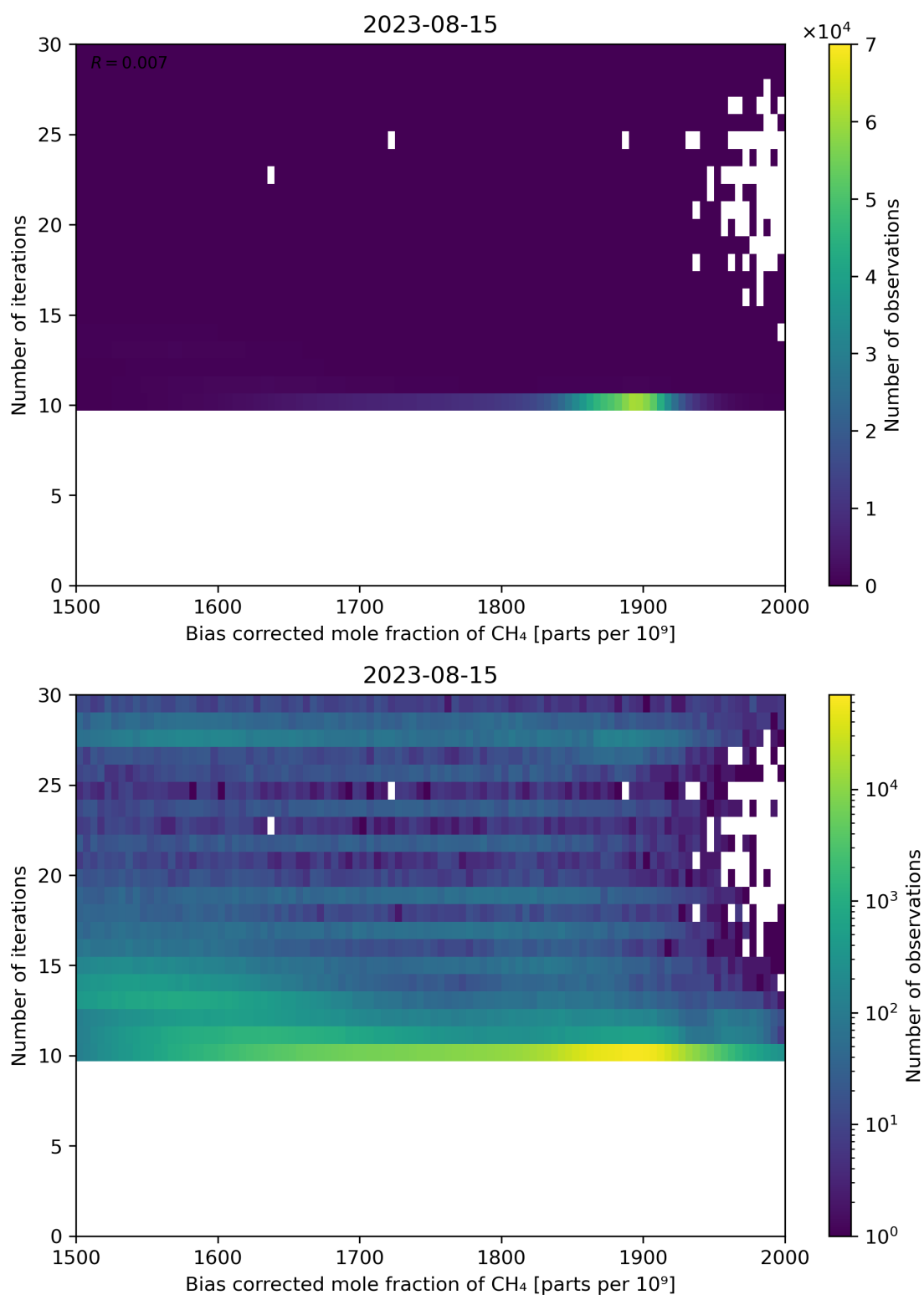
Figure 67: Scatter density plot of “Bias corrected mole fraction of CH 4 ” against “Number of iterations” for 2023-08-14 to 2023-08-16.
