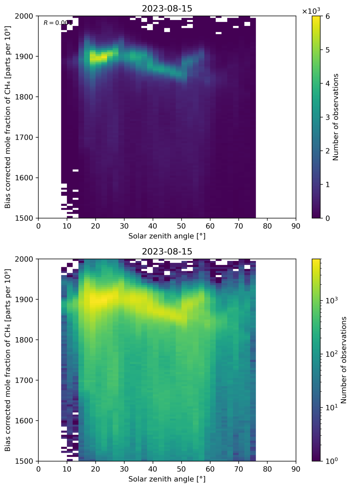
Figure 100: Scatter density plot of “Solar zenith angle” against “Bias corrected mole fraction of CH 4 ” for 2023-08-14 to 2023-08-16.
