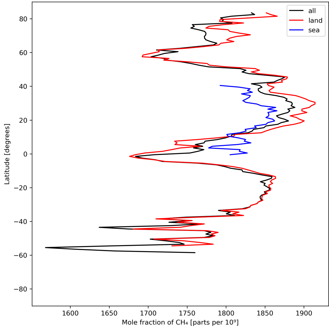
Figure 12: Zonal average of “Mole fraction of CH 4 ” for 2023-08-14 to 2023-08-16.
