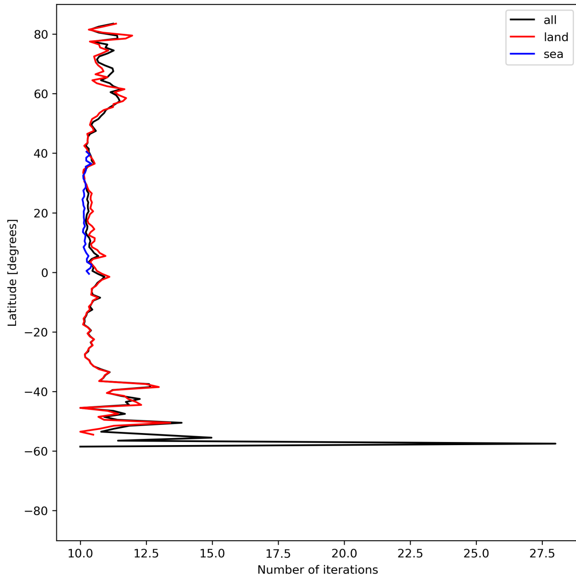
Figure 20: Zonal average of “Number of iterations” for 2023-08-14 to 2023-08-16.
