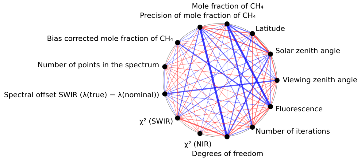
Figure 1: Map of correlation graph for 2023-08-14 to 2023-08-16.
