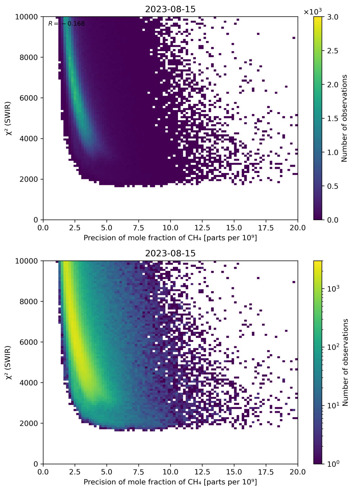
Figure 79: Scatter density plot of “Precision of mole fraction of CH 4 ” against “ \chi^2 (SWIR)” for 2023-08-14 to 2023-08-16.
