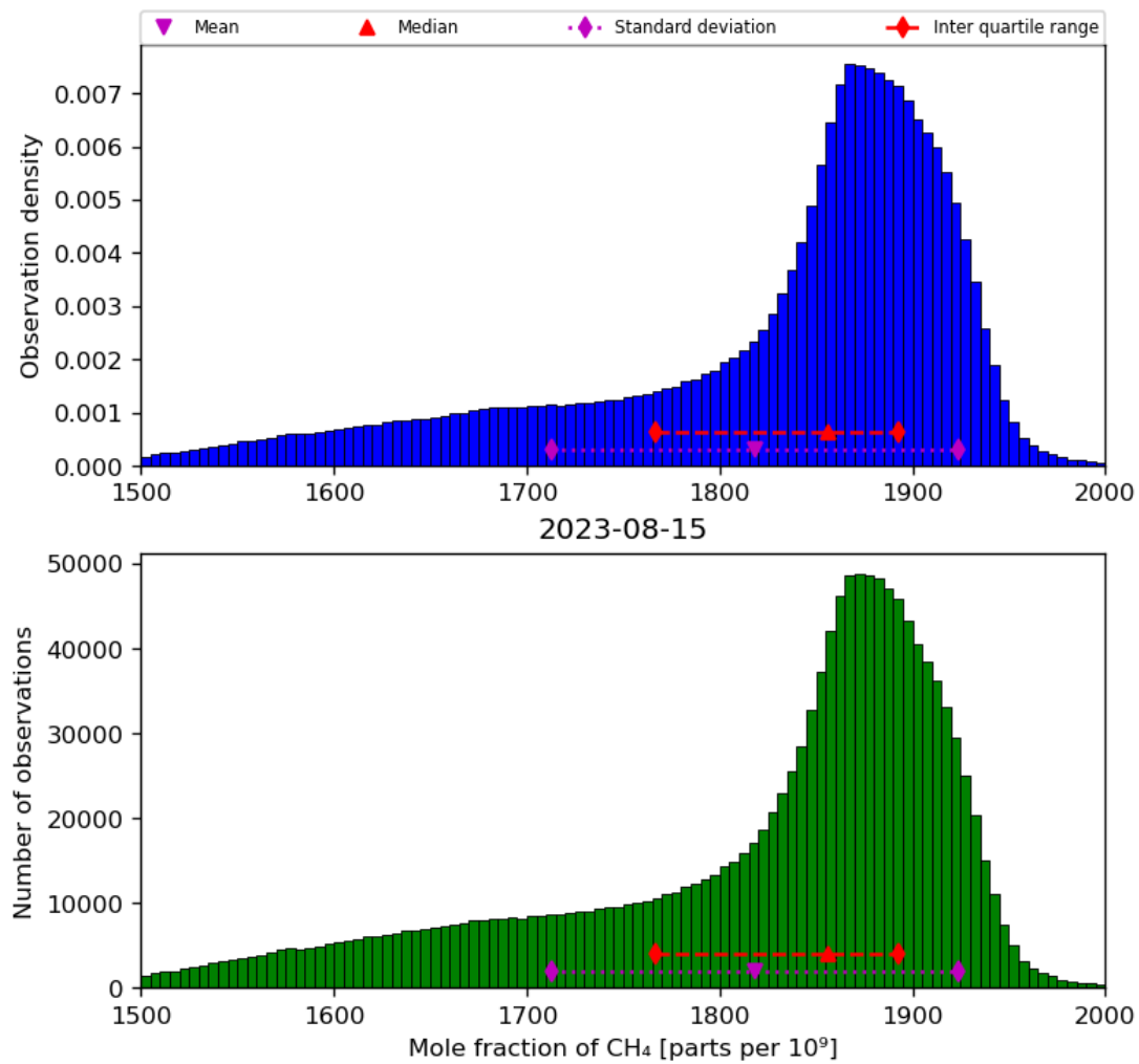
Figure 23: Histogram of “Mole fraction of CH 4 ” for 2023-08-14 to 2023-08-16
