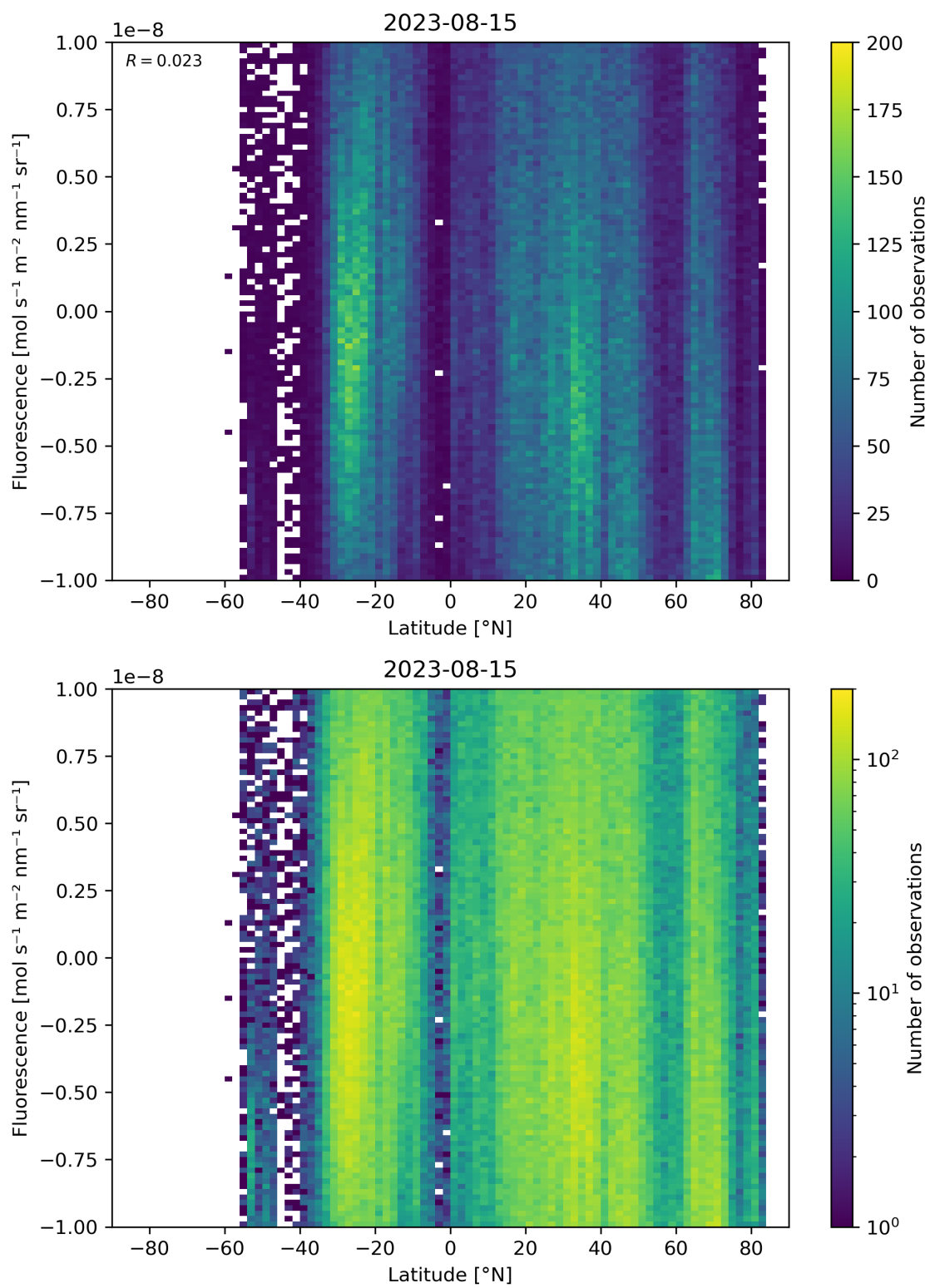
Figure 56: Scatter density plot of “Latitude” against “Fluorescence” for 2023-08-14 to 2023-08-16.
