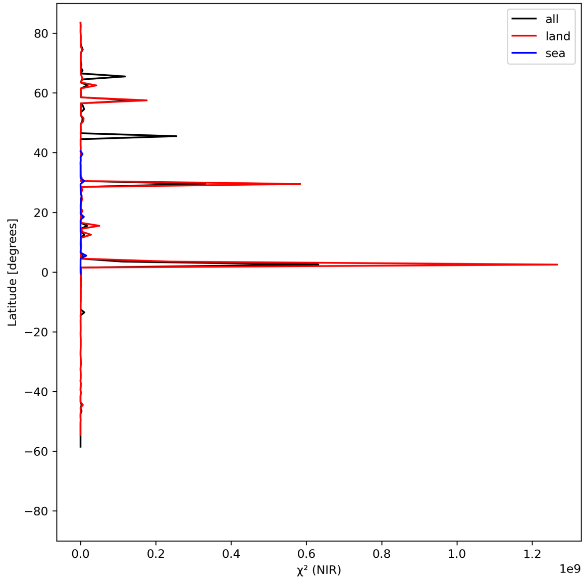
Figure 18: Zonal average of “ \chi^2 (NIR)” for 2023-08-14 to 2023-08-16.
