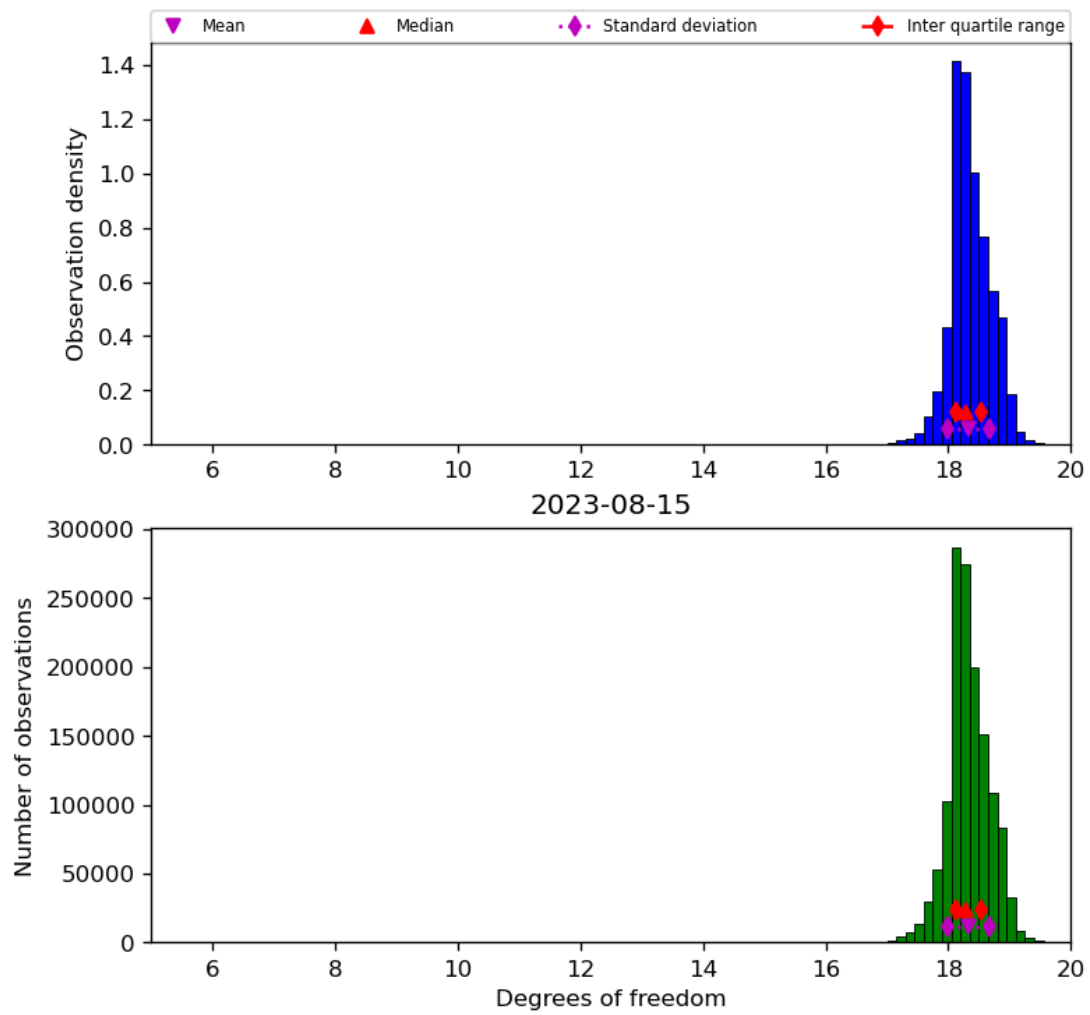
Figure 30: Histogram of “Degrees of freedom” for 2023-08-14 to 2023-08-16
