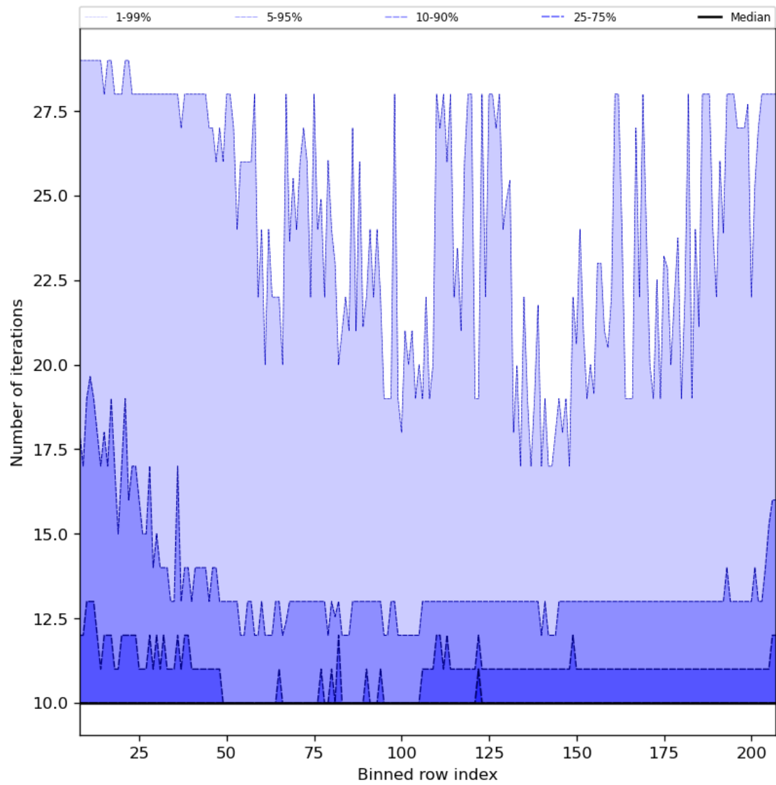
Figure 42: Along track statistics of “Number of iterations” for 2023-08-14 to 2023-08-16
