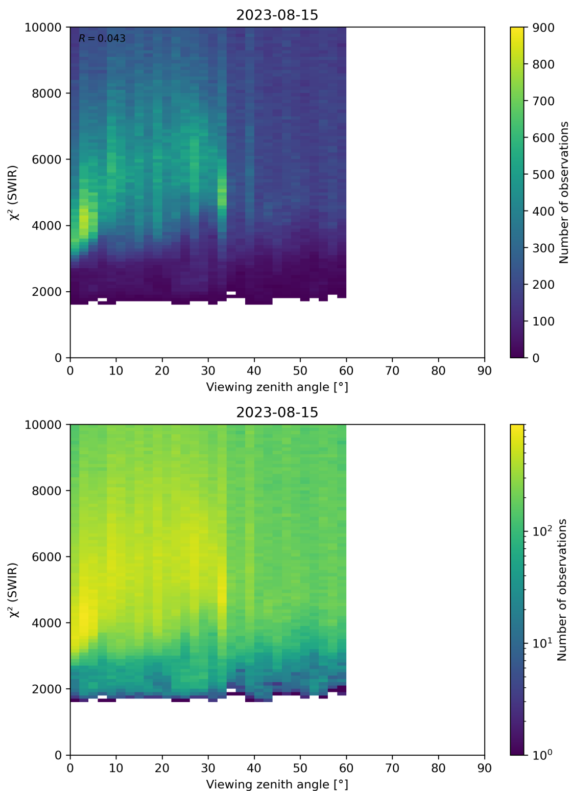
Figure 106: Scatter density plot of “Viewing zenith angle” against “ \chi^2 (SWIR)” for 2023-08-14 to 2023-08-16.
