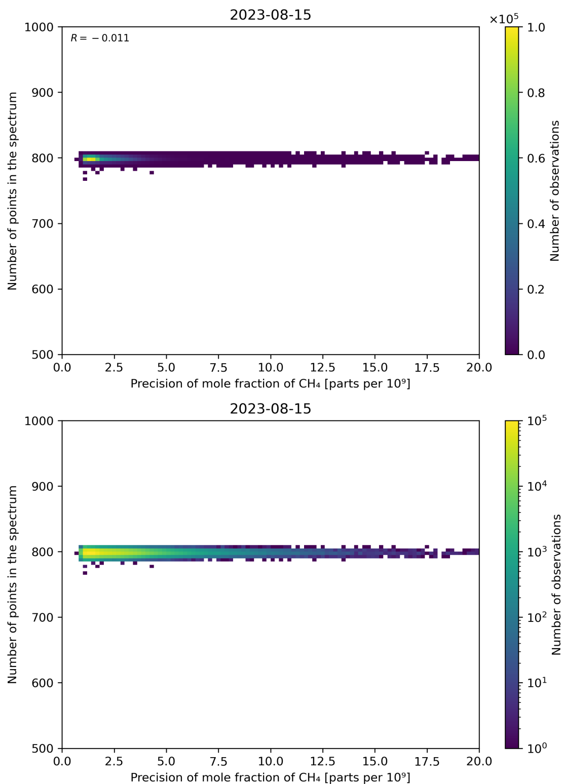
Figure 84: Scatter density plot of “Precision of mole fraction of CH 4 ” against “Number of points in the spectrum” for 2023-08-14 to 2023-08-16.
