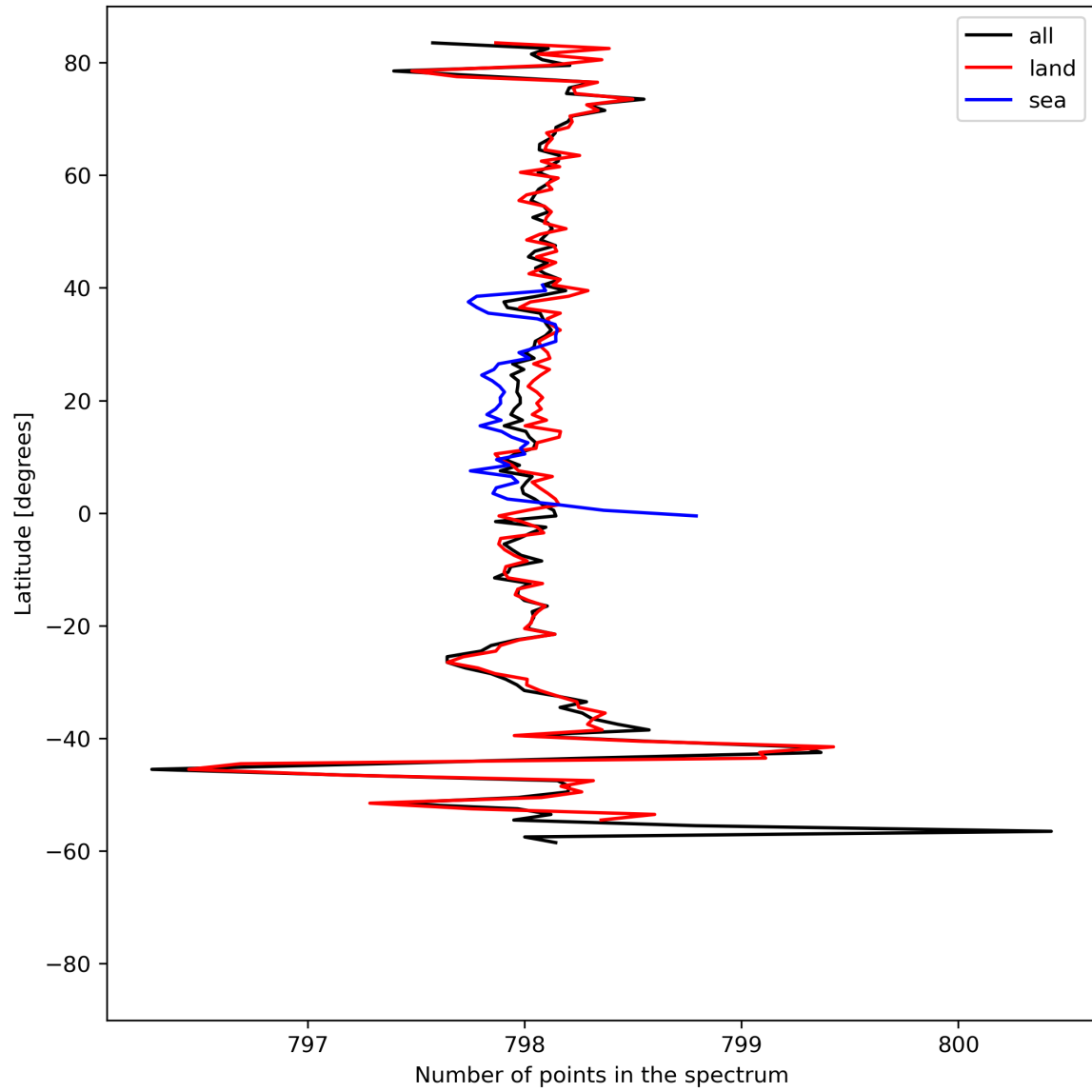
Figure 15: Zonal average of “Number of points in the spectrum” for 2023-08-14 to 2023-08-16.
