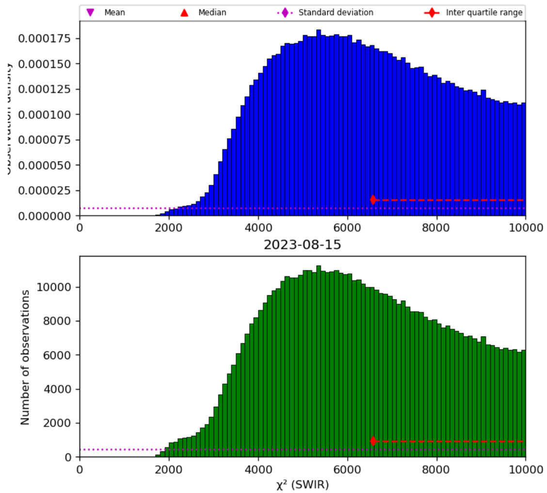
Figure 28: Histogram of “ \chi^2 (SWIR)” for 2023-08-14 to 2023-08-16
