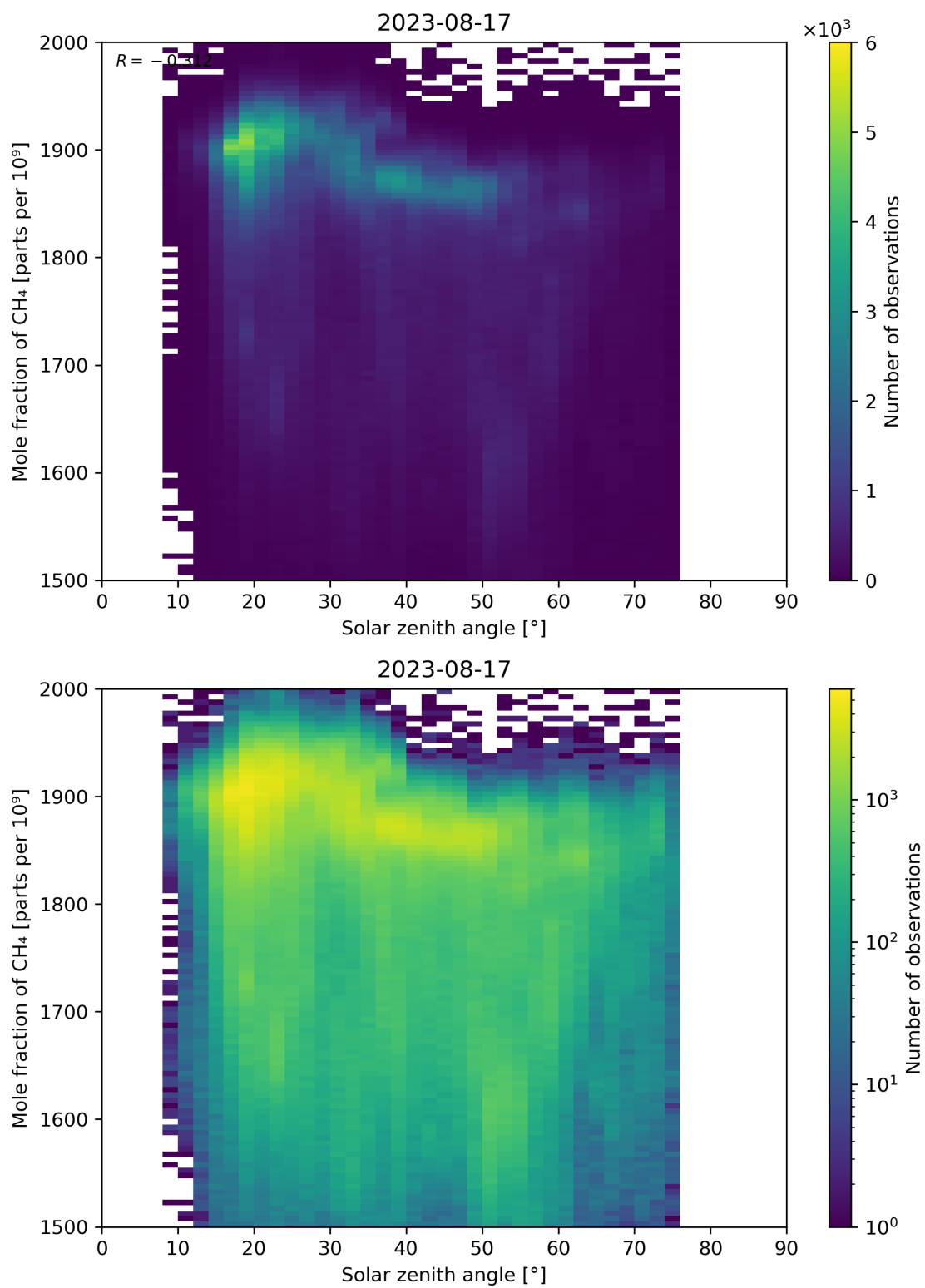
Figure 99: Scatter density plot of “Solar zenith angle” against “Mole fraction of CH 4 ” for 2023-08-16 to 2023-08-18.
