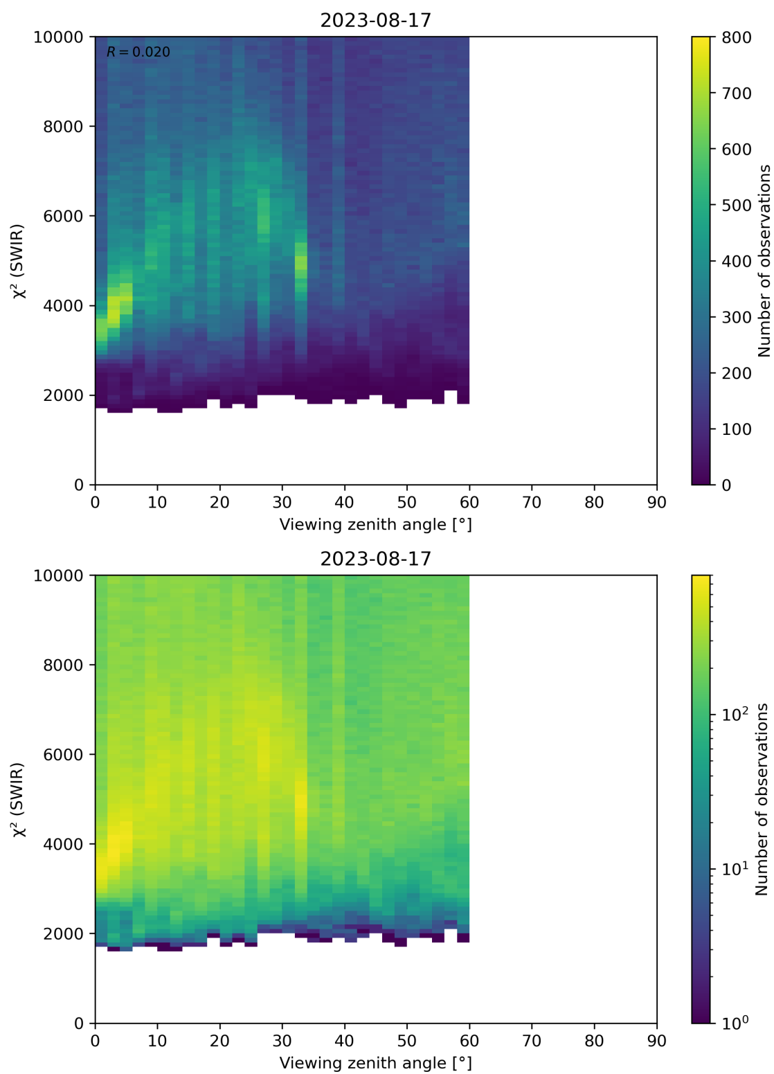
Figure 106: Scatter density plot of “Viewing zenith angle” against “ \chi^2 (SWIR)” for 2023-08-16 to 2023-08-18.
