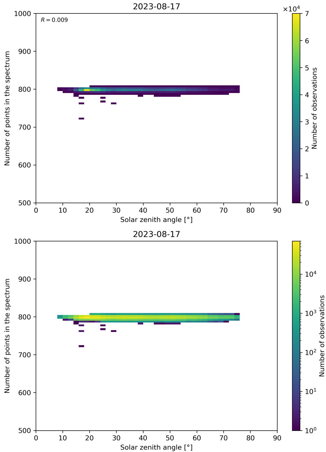
Figure 103: Scatter density plot of “Solar zenith angle” against “Number of points in the spectrum” for 2023-08-16 to 2023-08-18.
