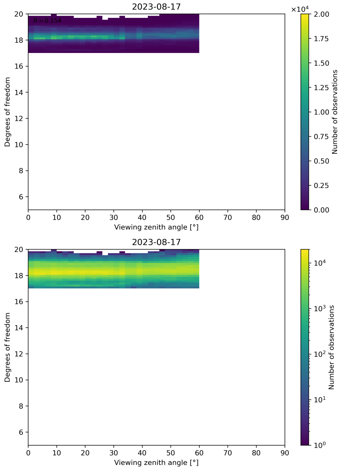
Figure 107: Scatter density plot of “Viewing zenith angle” against “Degrees of freedom” for 2023-08-16 to 2023-08-18.
