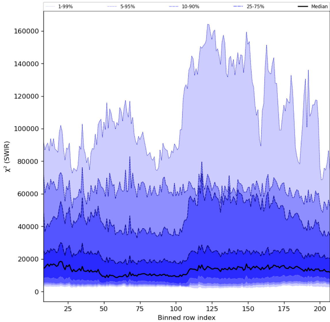
Figure 39: Along track statistics of " \chi^2 (SWIR)" for 2023-08-16 to 2023-08-18
