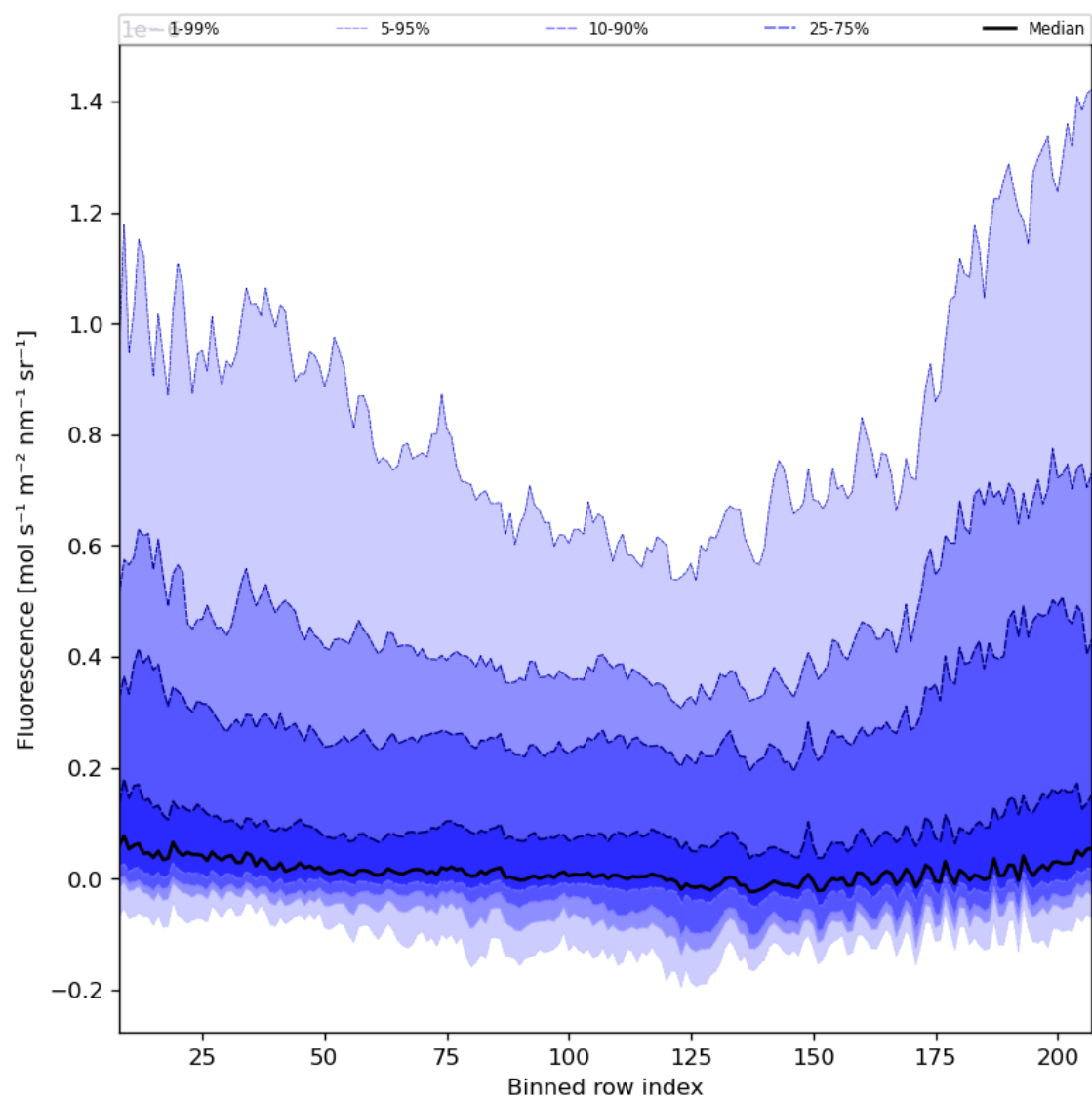
Figure 43: Along track statistics of “Fluorescence” for 2023-08-16 to 2023-08-18
