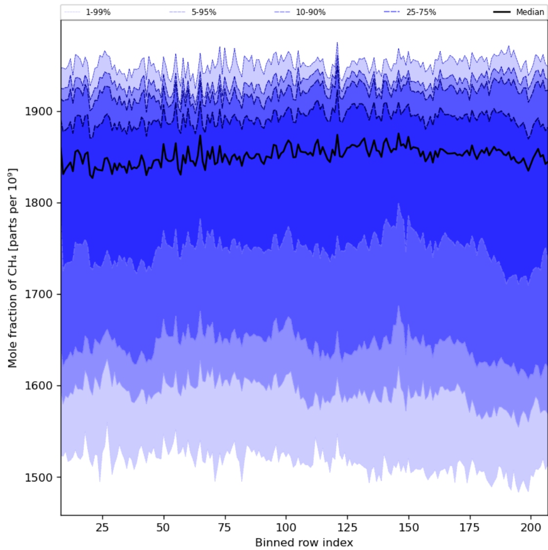
Figure 34: Along track statistics of “Mole fraction of CH 4 ” for 2023-08-16 to 2023-08-18
