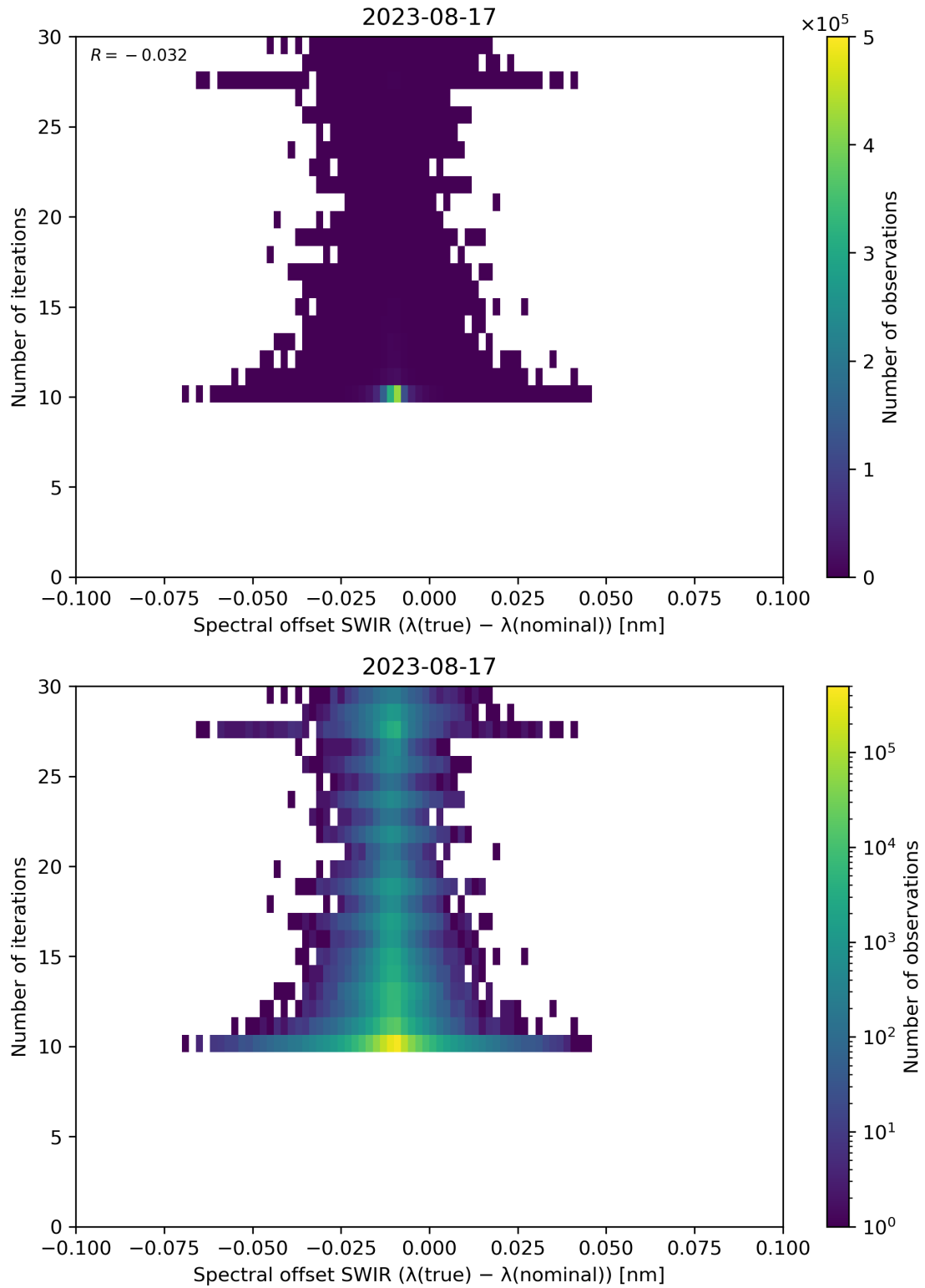
Figure 121: Scatter density plot of “Spectral offset SWIR ( \lambda(\text{true}) - \lambda(\text{nominal}) )” against “Number of iterations” for 2023-08-16 to 2023-08-18.
