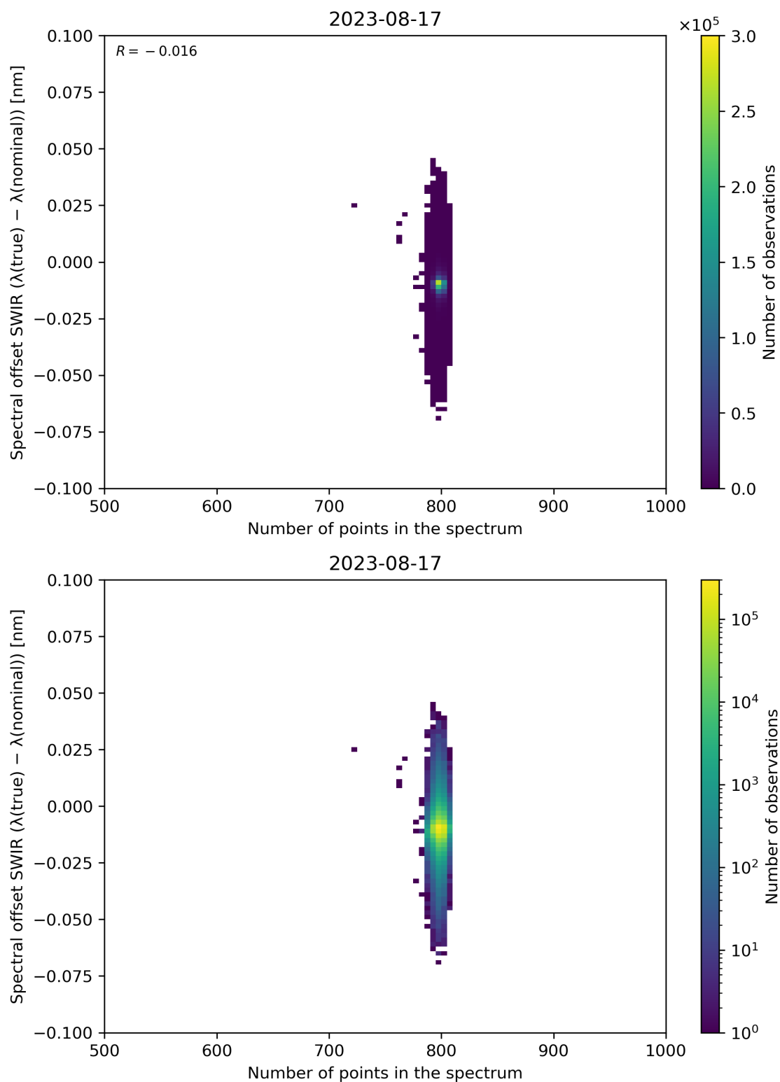
Figure 93: Scatter density plot of “Number of points in the spectrum” against “Spectral offset SWIR ( \lambda(\text{true}) - \lambda(\text{nominal}) )” for 2023-08-16 to 2023-08-18.
