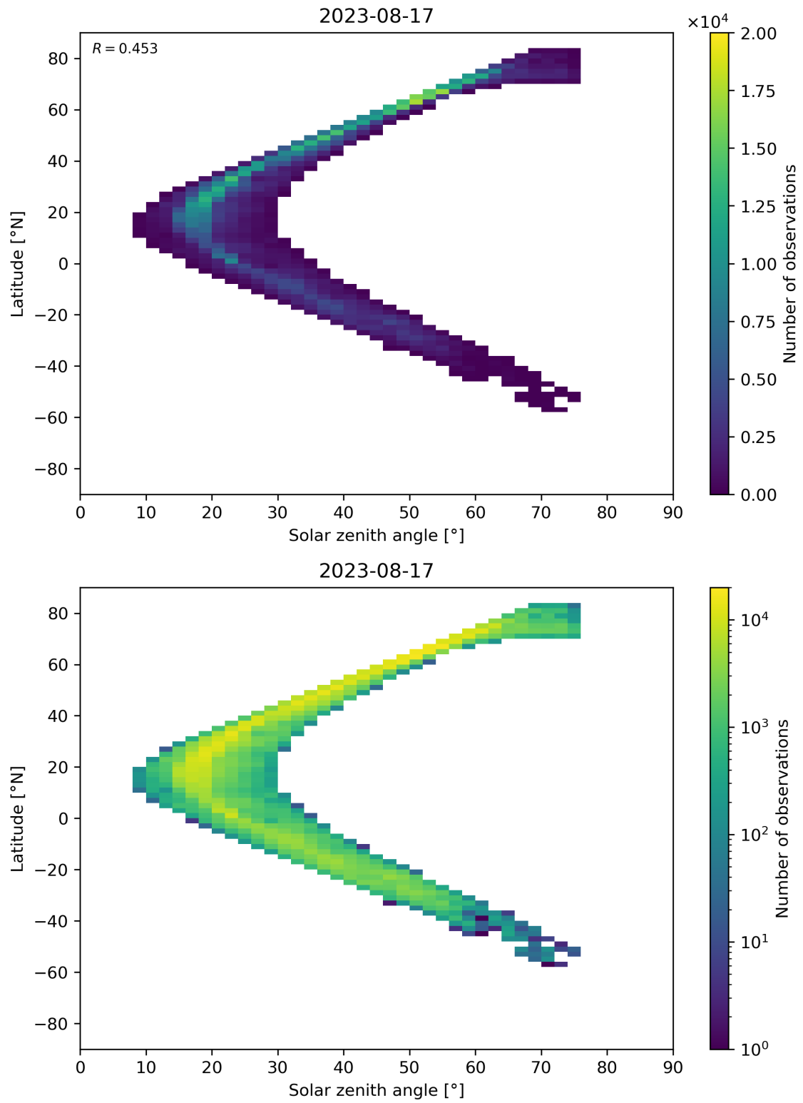
Figure 98: Scatter density plot of “Solar zenith angle” against “Latitude” for 2023-08-16 to 2023-08-18.
