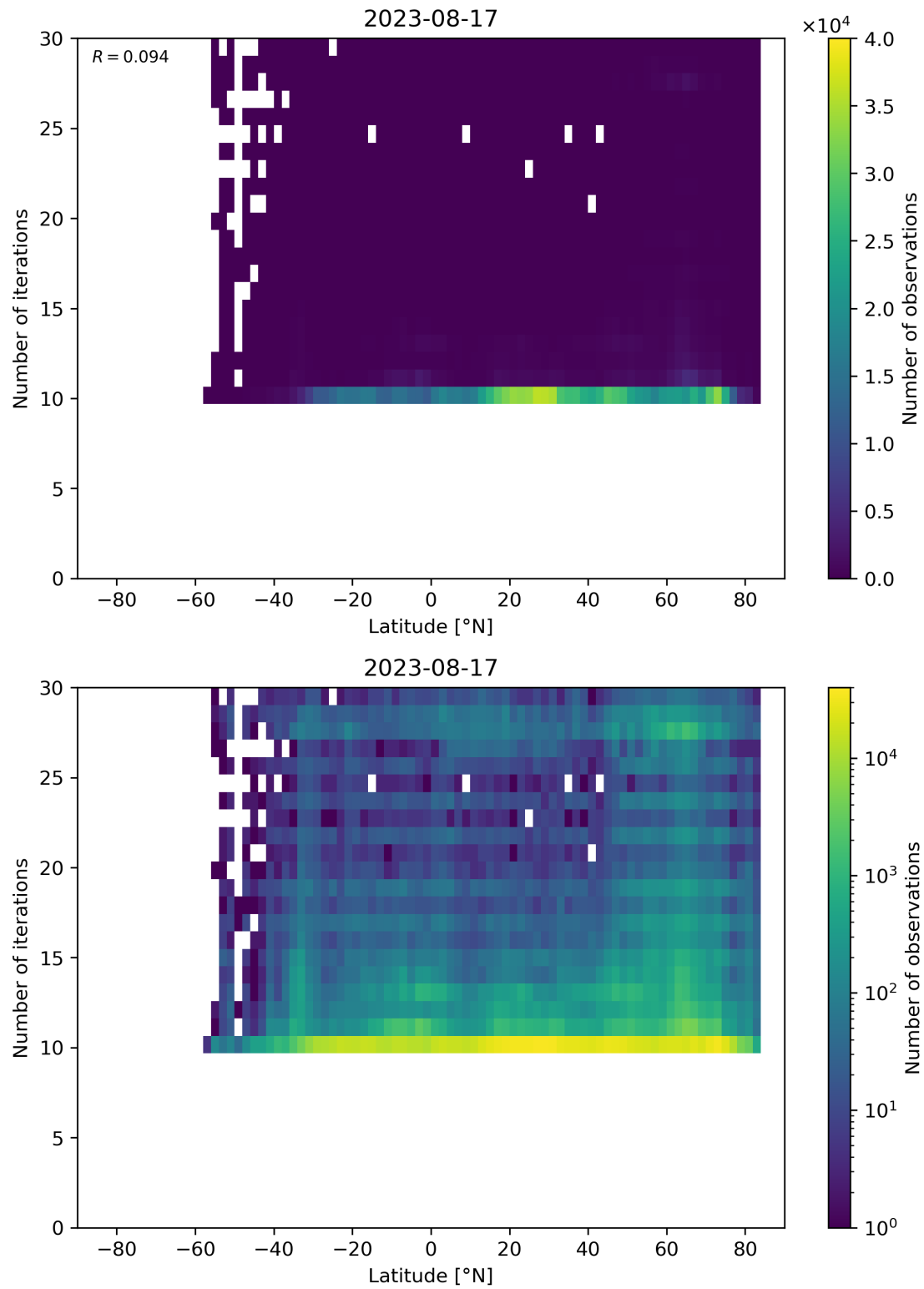
Figure 60: Scatter density plot of “Latitude” against “Number of iterations” for 2023-08-16 to 2023-08-18.
