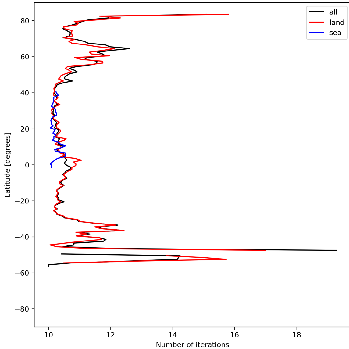
Figure 20: Zonal average of “Number of iterations” for 2023-08-16 to 2023-08-18.
