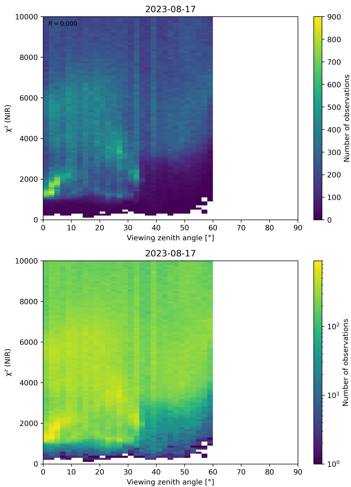
Figure 105: Scatter density plot of “Viewing zenith angle” against “ \chi^2 (NIR)” for 2023-08-16 to 2023-08-18.
