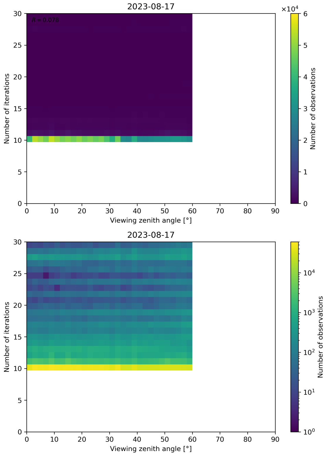
Figure 113: Scatter density plot of “Viewing zenith angle” against “Number of iterations” for 2023-08-16 to 2023-08-18.
