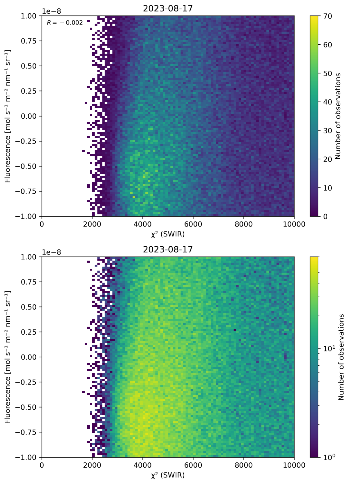
Figure 49: Scatter density plot of “ \chi^2 (SWIR)” against “Fluorescence” for 2023-08-16 to 2023-08-18.
