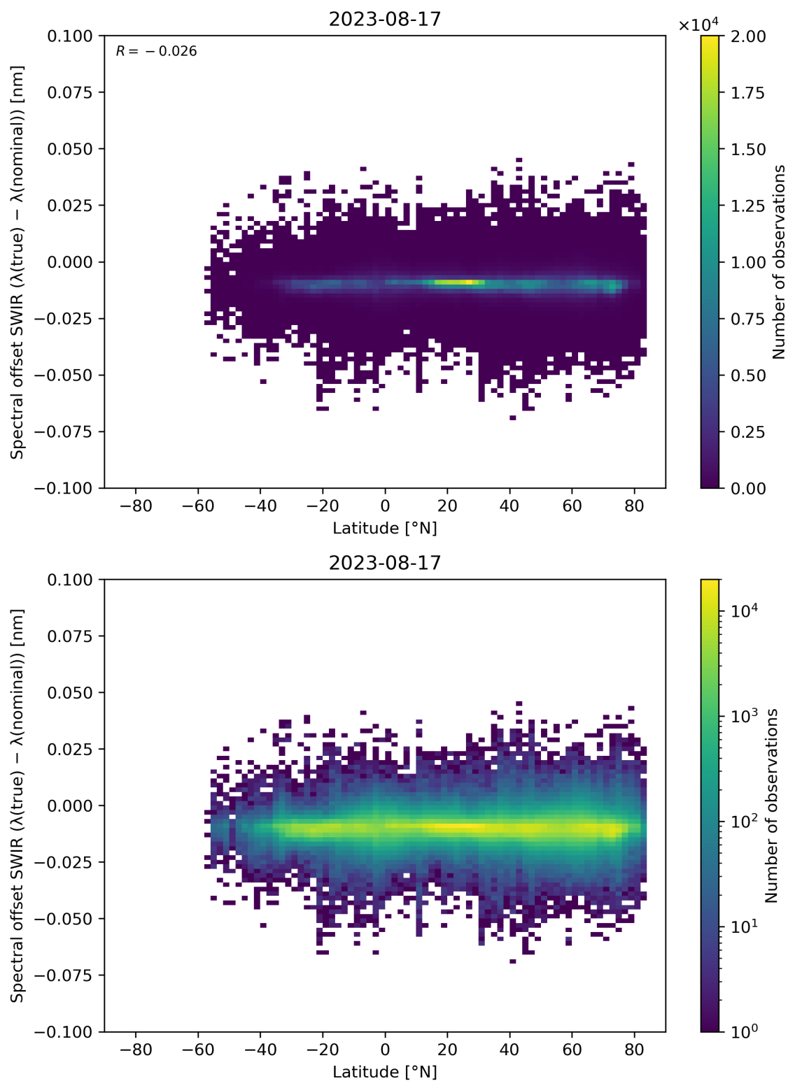
Figure 62: Scatter density plot of “Latitude” against “Spectral offset SWIR ( \lambda(\text{true}) - \lambda(\text{nominal}) )” for 2023-08-16 to 2023-08-18.
