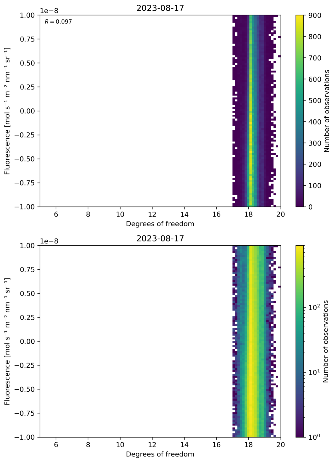
Figure 51: Scatter density plot of “Degrees of freedom” against “Fluorescence” for 2023-08-16 to 2023-08-18.
