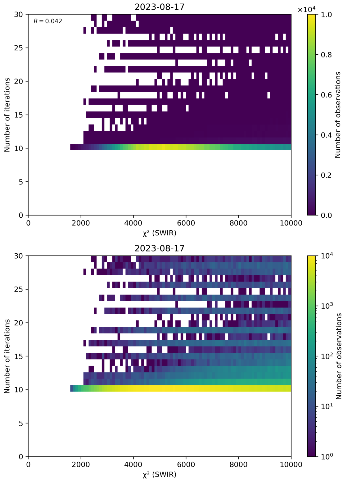
Figure 50: Scatter density plot of “ \chi^2 (SWIR)” against “Number of iterations” for 2023-08-16 to 2023-08-18.
