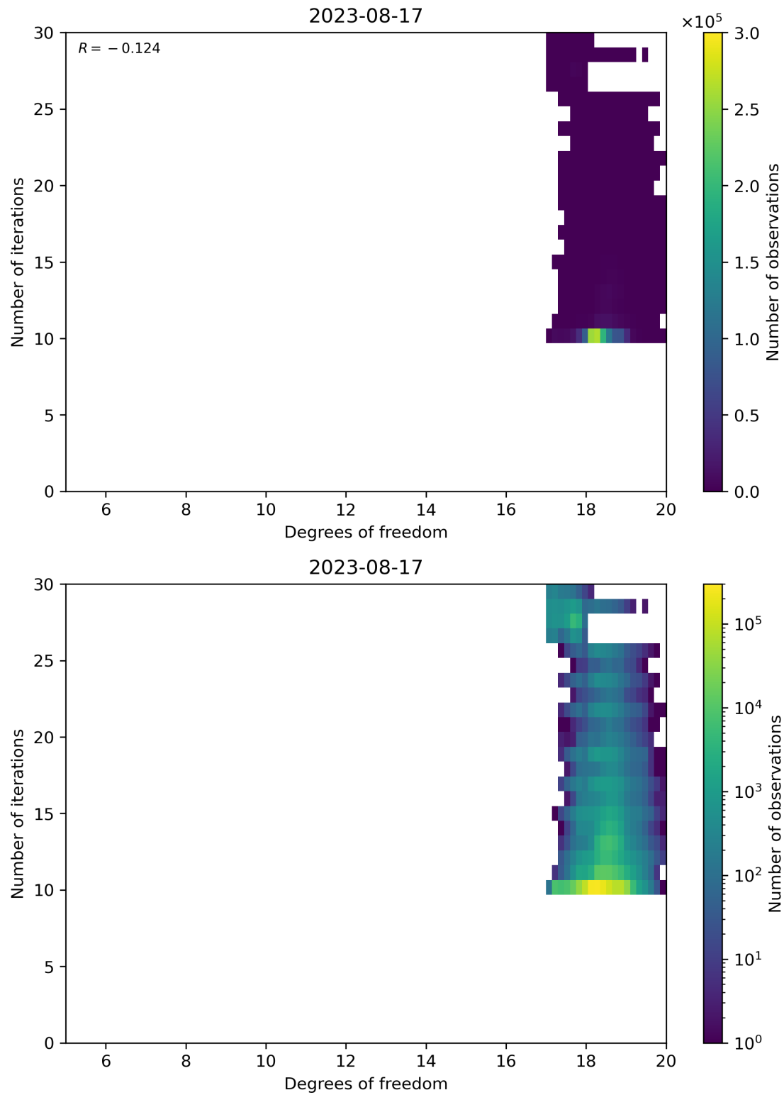
Figure 52: Scatter density plot of “Degrees of freedom” against “Number of iterations” for 2023-08-16 to 2023-08-18.
