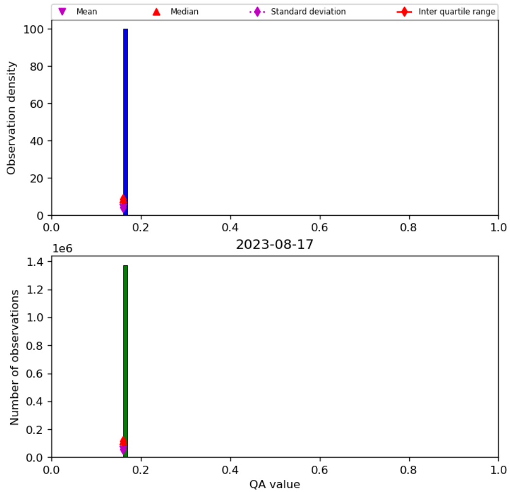
Figure 22: Histogram of “QA value” for 2023-08-16 to 2023-08-18
