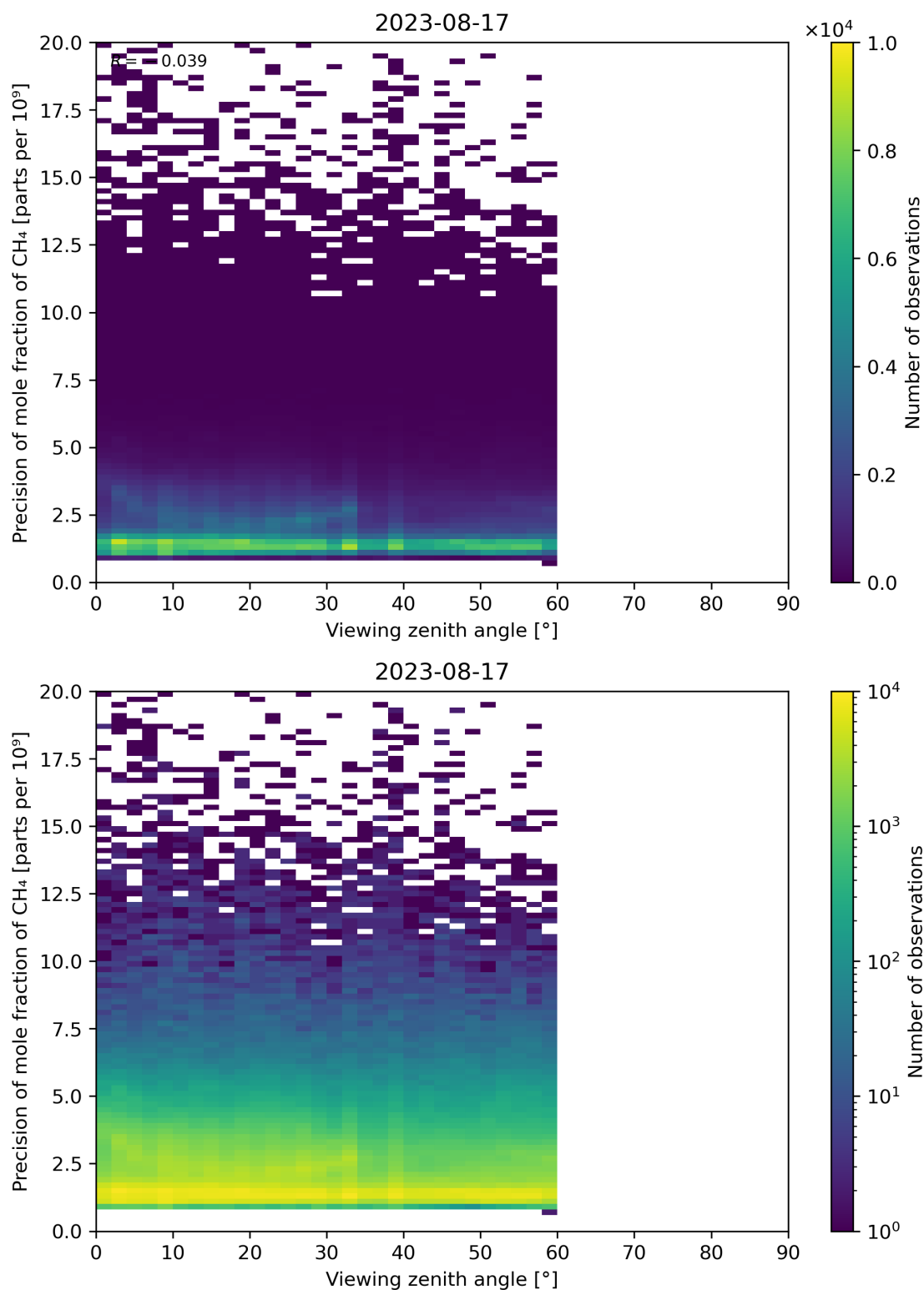
Figure 112: Scatter density plot of “Viewing zenith angle” against “Precision of mole fraction of CH 4 ” for 2023-08-16 to 2023-08-18.
