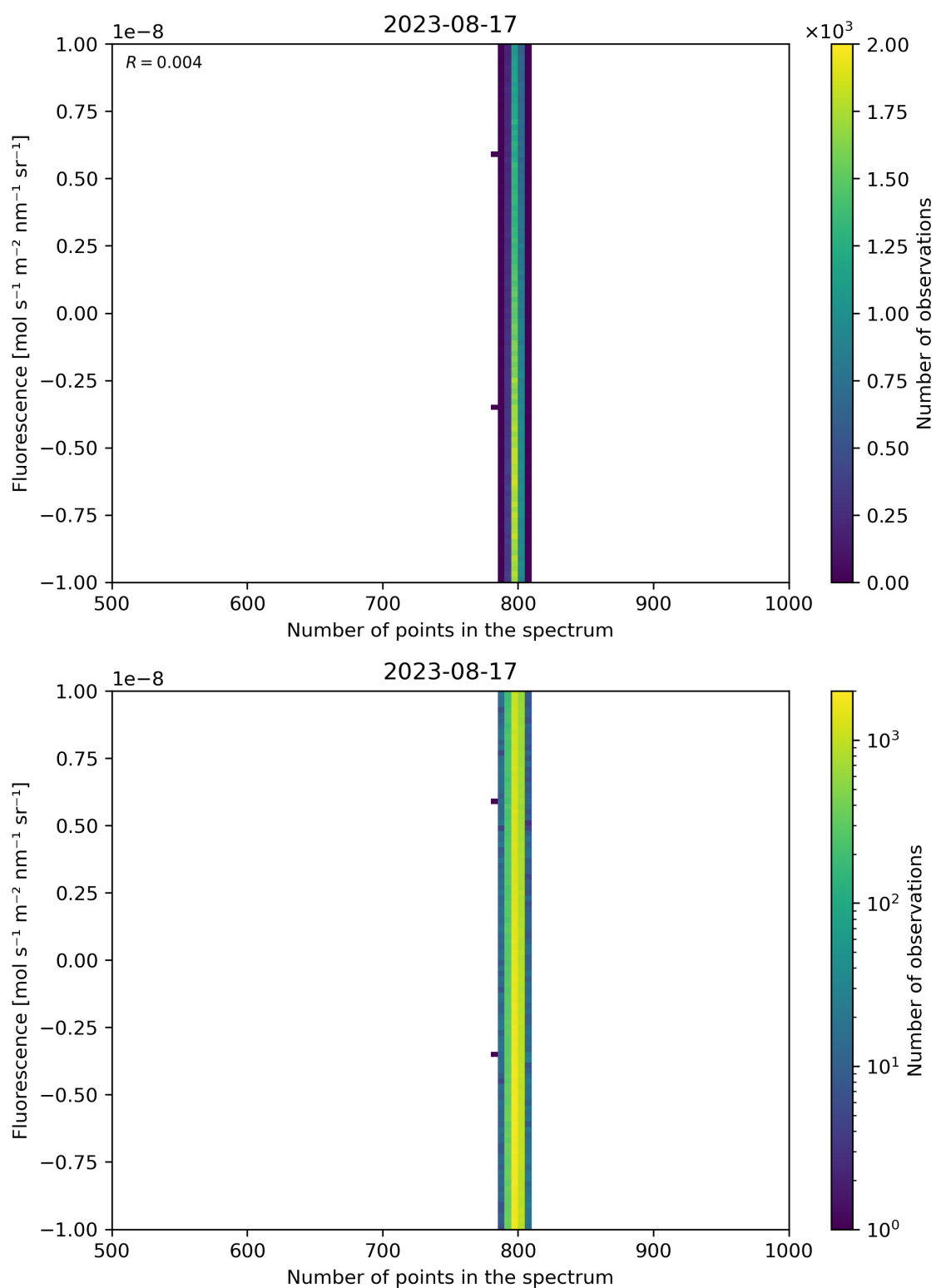
Figure 91: Scatter density plot of “Number of points in the spectrum” against “Fluorescence” for 2023-08-16 to 2023-08-18.
