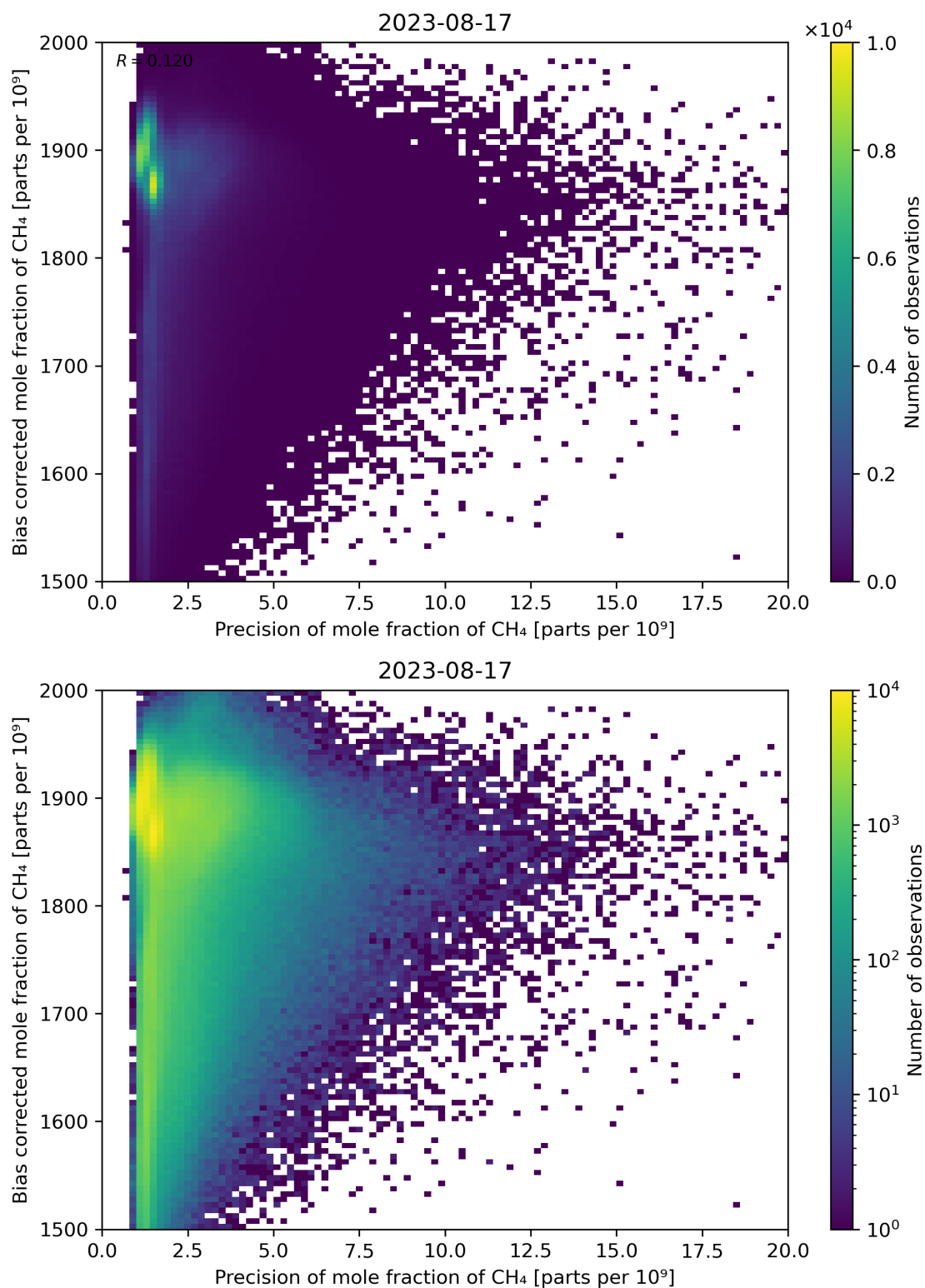
Figure 82: Scatter density plot of “Precision of mole fraction of \text{CH}_4 ” against “Bias corrected mole fraction of \text{CH}_4 ” for 2023-08-16 to 2023-08-18.
