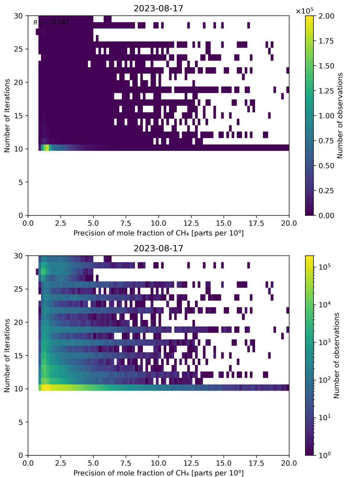
Figure 83: Scatter density plot of “Precision of mole fraction of CH 4 ” against “Number of iterations” for 2023-08-16 to 2023-08-18.
