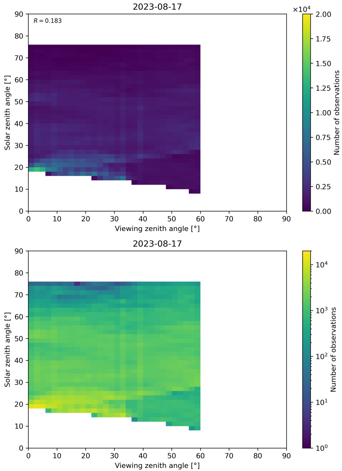
Figure 115: Scatter density plot of “Viewing zenith angle” against “Solar zenith angle” for 2023-08-16 to 2023-08-18.
