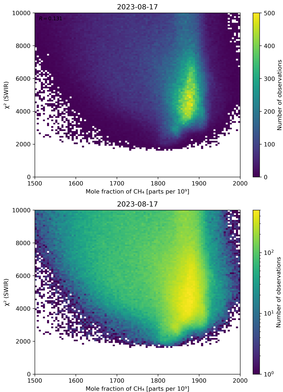
Figure 71: Scatter density plot of “Mole fraction of \text{CH}_4 ” against “ \chi^2 (SWIR)” for 2023-08-16 to 2023-08-18.
