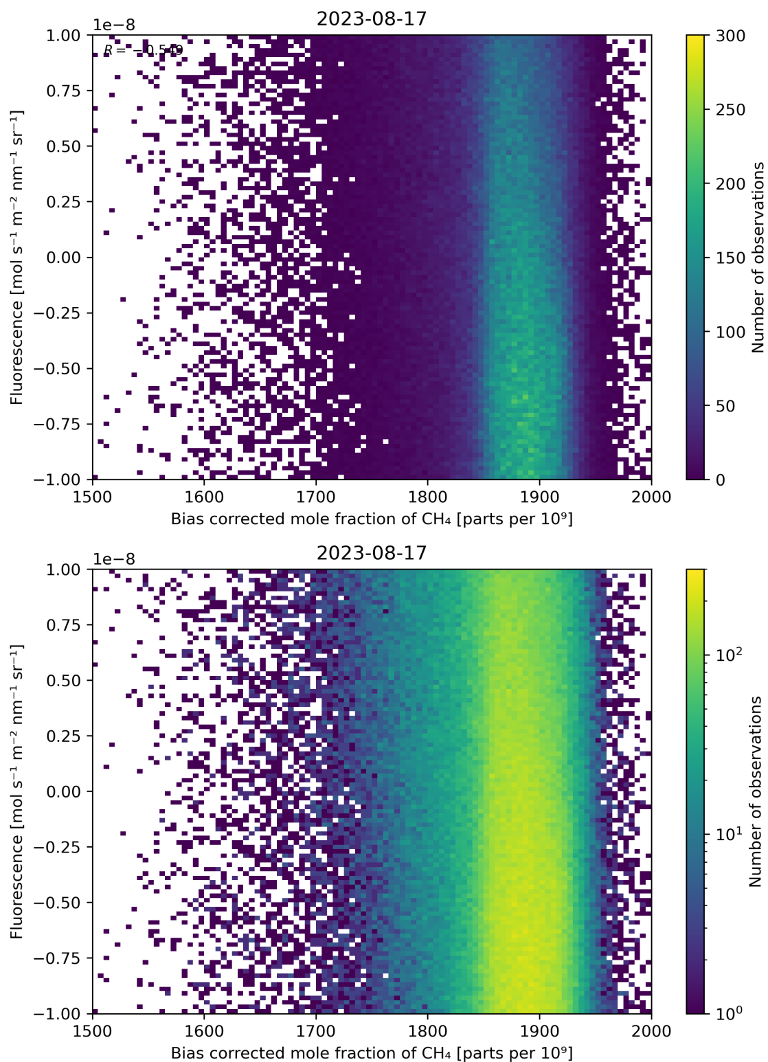
Figure 66: Scatter density plot of “Bias corrected mole fraction of \text{CH}_4 ” against “Fluorescence” for 2023-08-16 to 2023-08-18.
