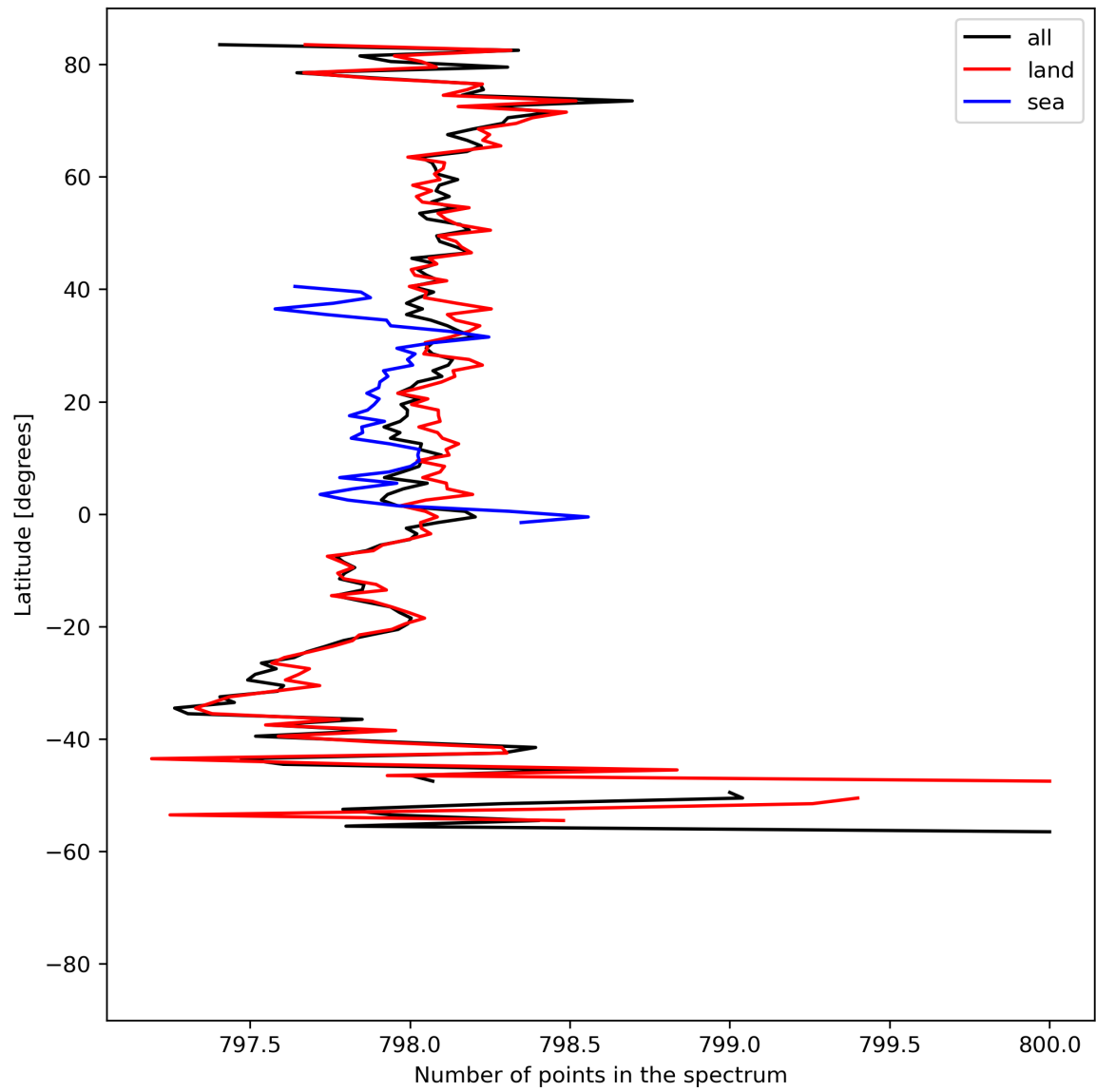
Figure 15: Zonal average of “Number of points in the spectrum” for 2023-08-16 to 2023-08-18.
