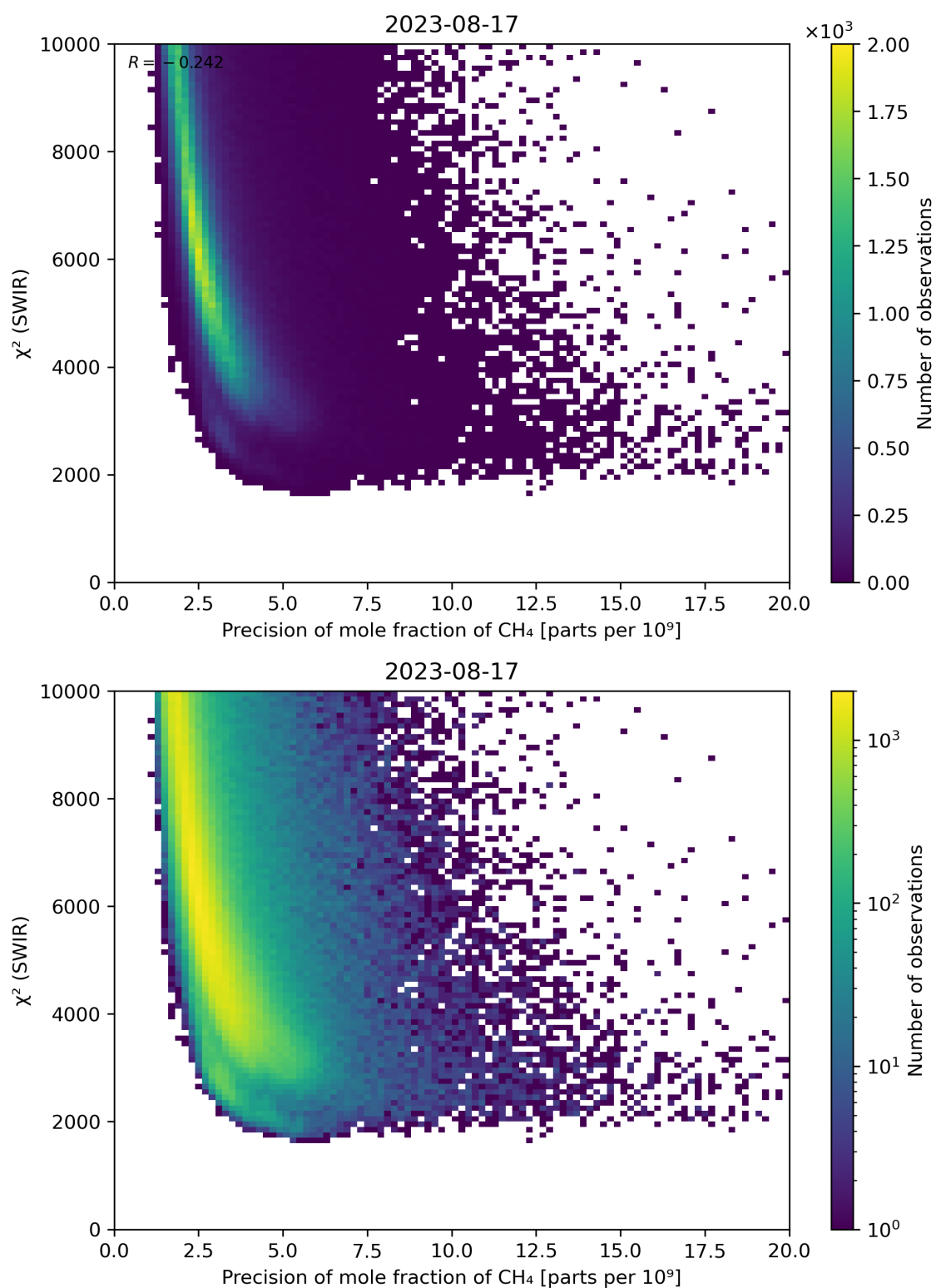
Figure 79: Scatter density plot of “Precision of mole fraction of \text{CH}_4 ” against “ \chi^2 (SWIR)” for 2023-08-16 to 2023-08-18.
