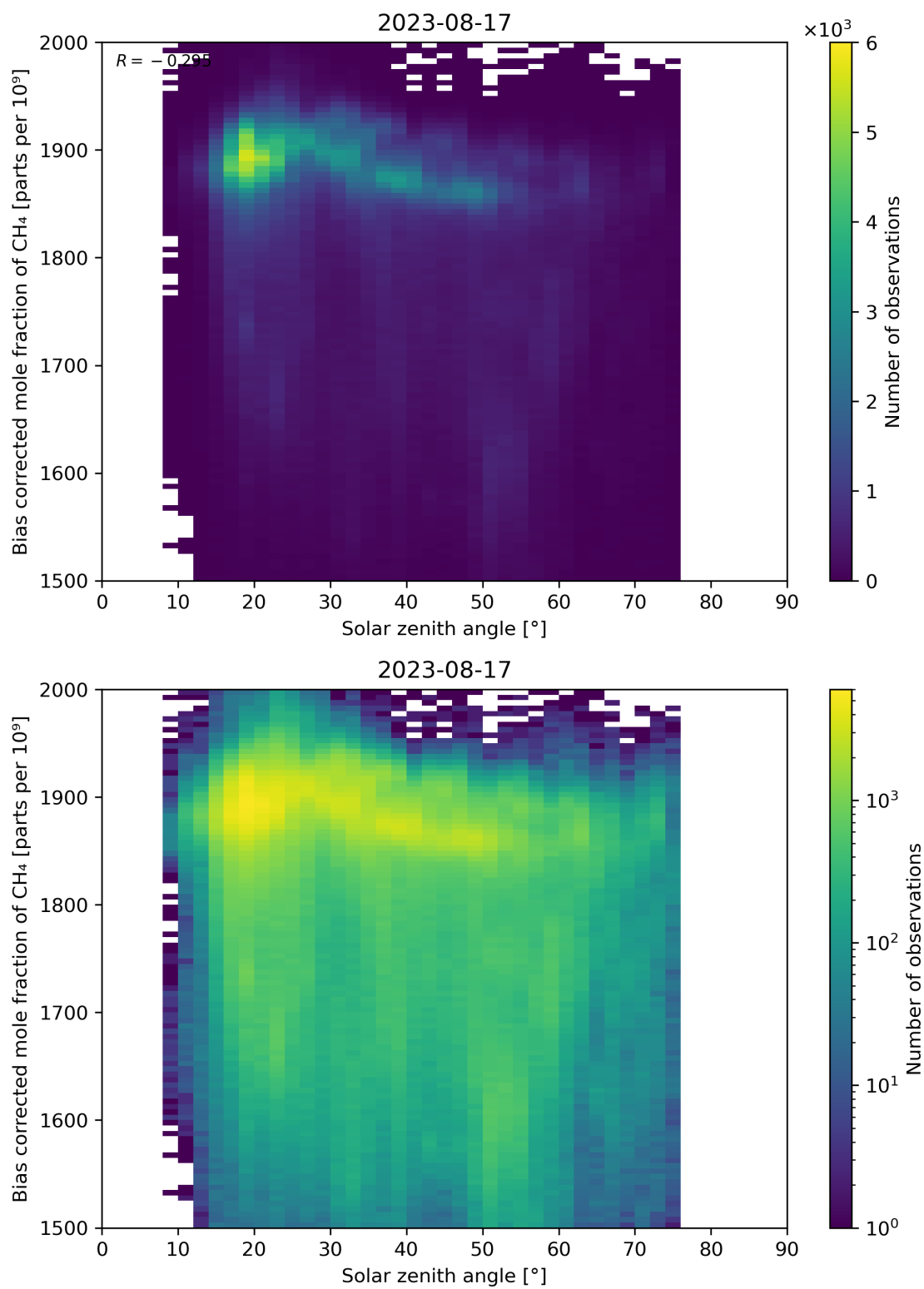
Figure 100: Scatter density plot of “Solar zenith angle” against “Bias corrected mole fraction of CH 4 ” for 2023-08-16 to 2023-08-18.
