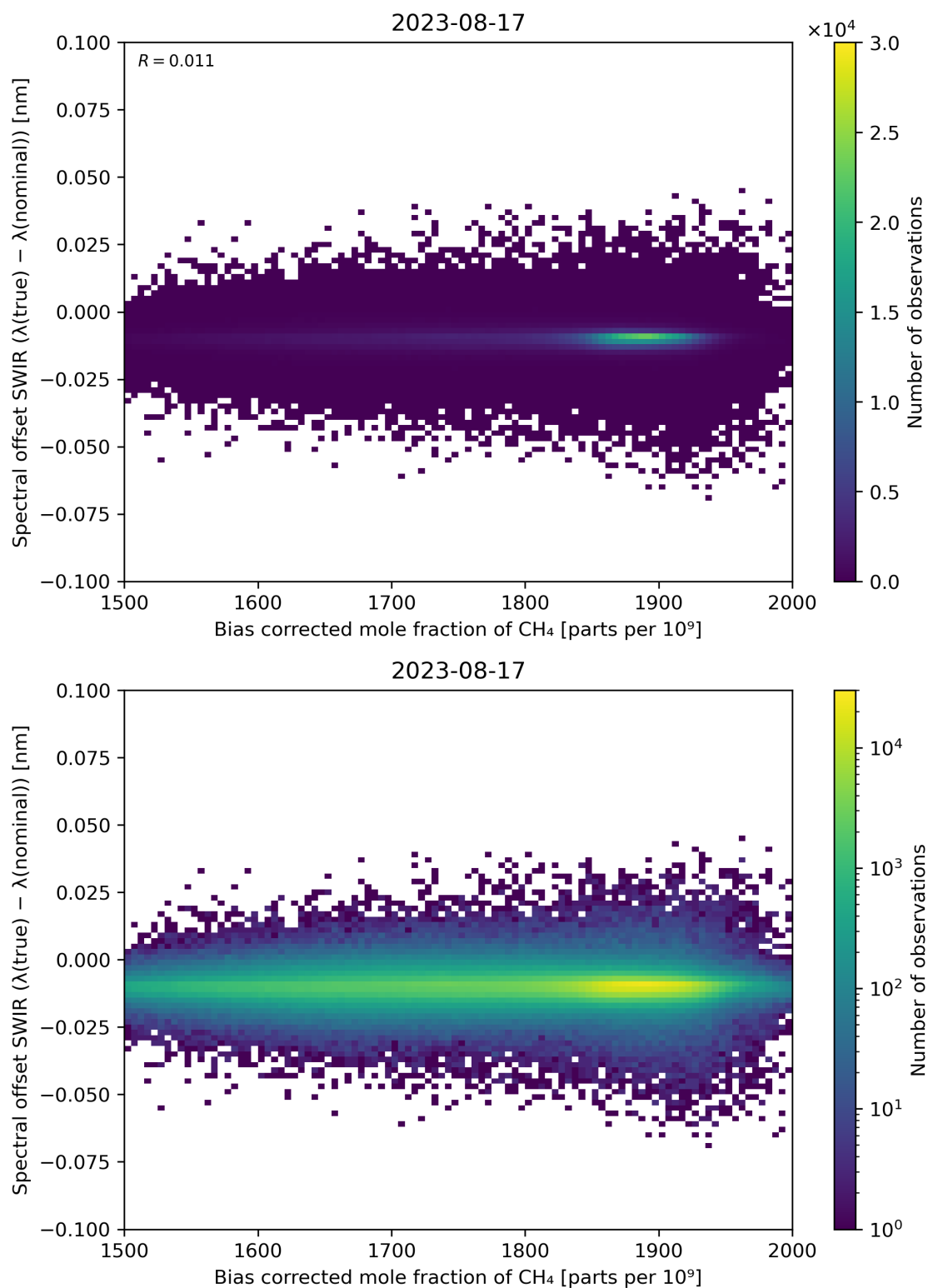
Figure 69: Scatter density plot of “Bias corrected mole fraction of \text{CH}_4 ” against “Spectral offset SWIR ( \lambda(\text{true}) - \lambda(\text{nominal}) )” for 2023-08-16 to 2023-08-18.
