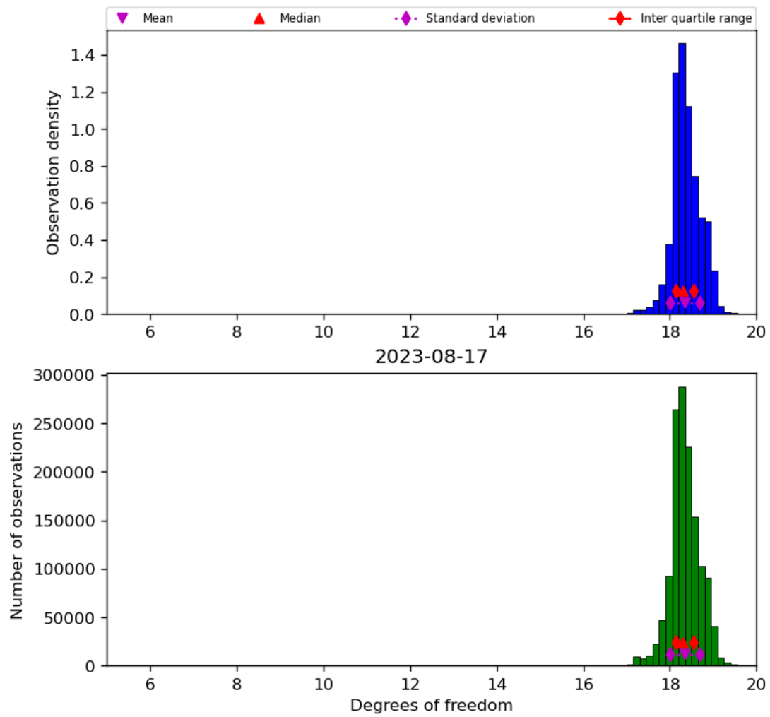
Figure 30: Histogram of “Degrees of freedom” for 2023-08-16 to 2023-08-18
