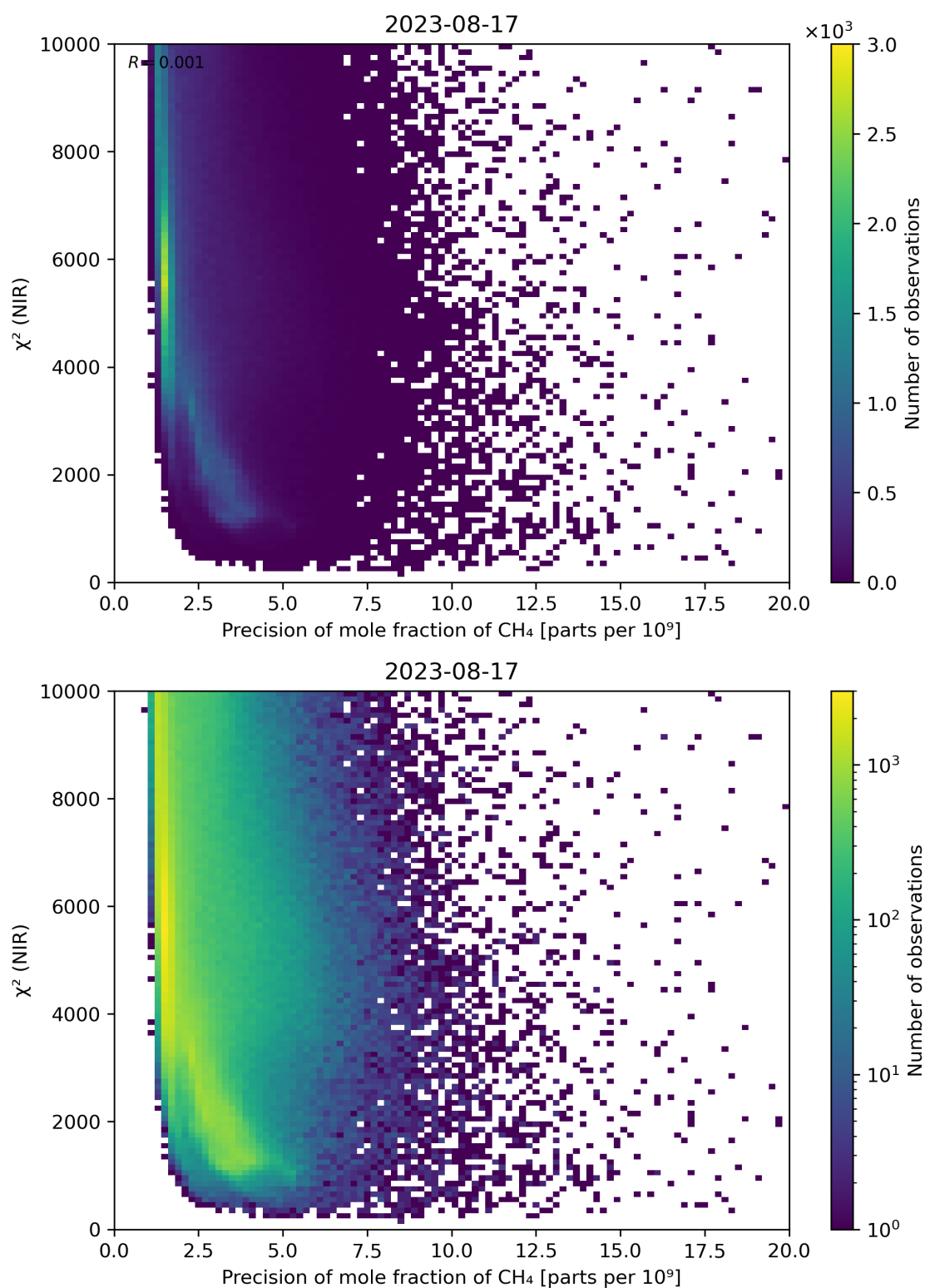
Figure 78: Scatter density plot of “Precision of mole fraction of \text{CH}_4 ” against “ \chi^2 (NIR)” for 2023-08-16 to 2023-08-18.
