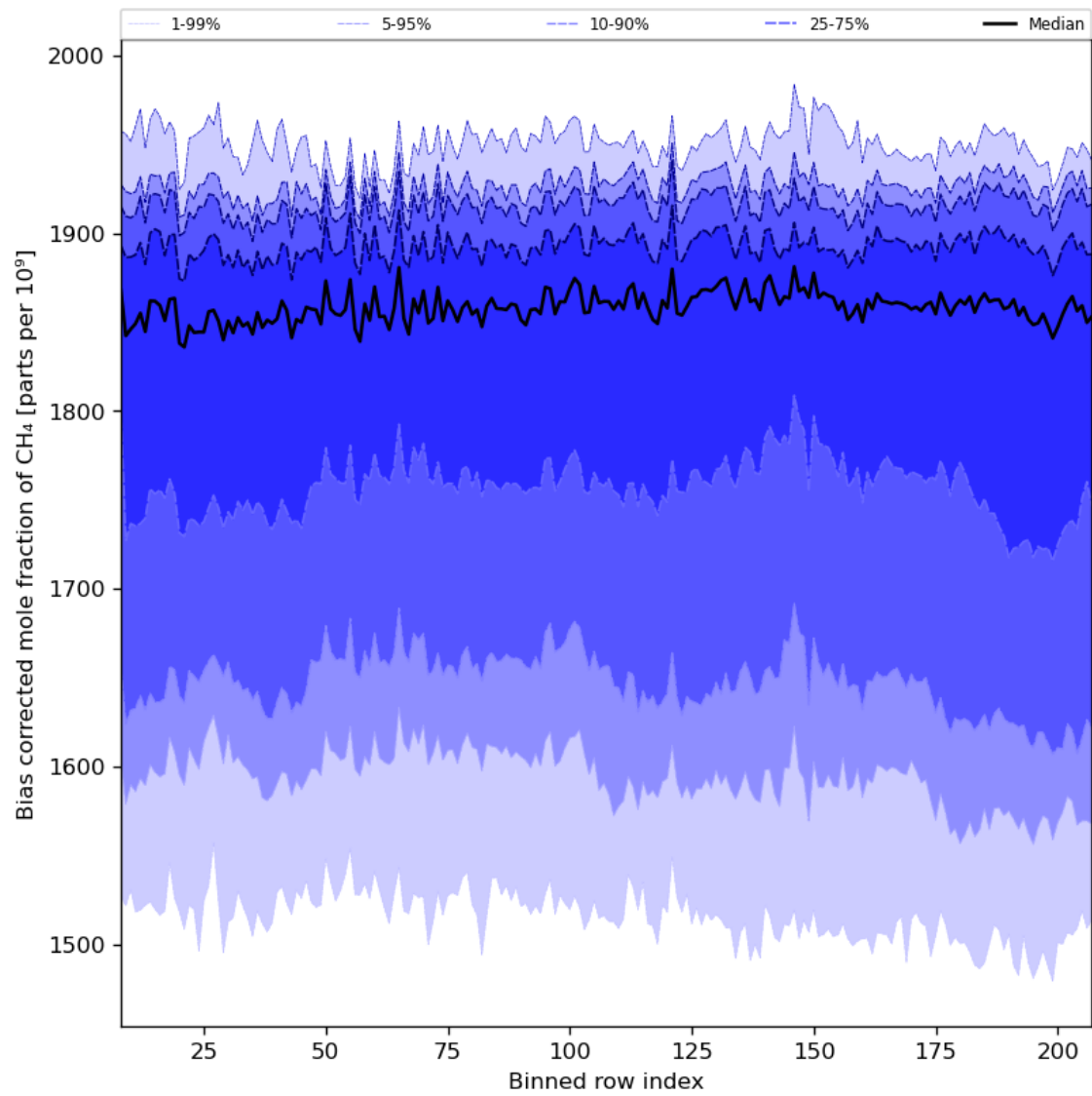
Figure 36: Along track statistics of “Bias corrected mole fraction of \text{CH}_4 ” for 2023-08-16 to 2023-08-18
