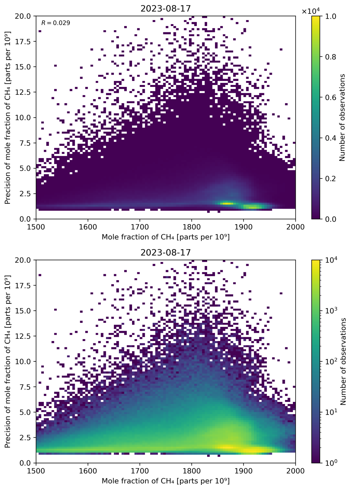
Figure 75: Scatter density plot of “Mole fraction of CH 4 ” against “Precision of mole fraction of CH 4 ” for 2023-08-16 to 2023-08-18.
