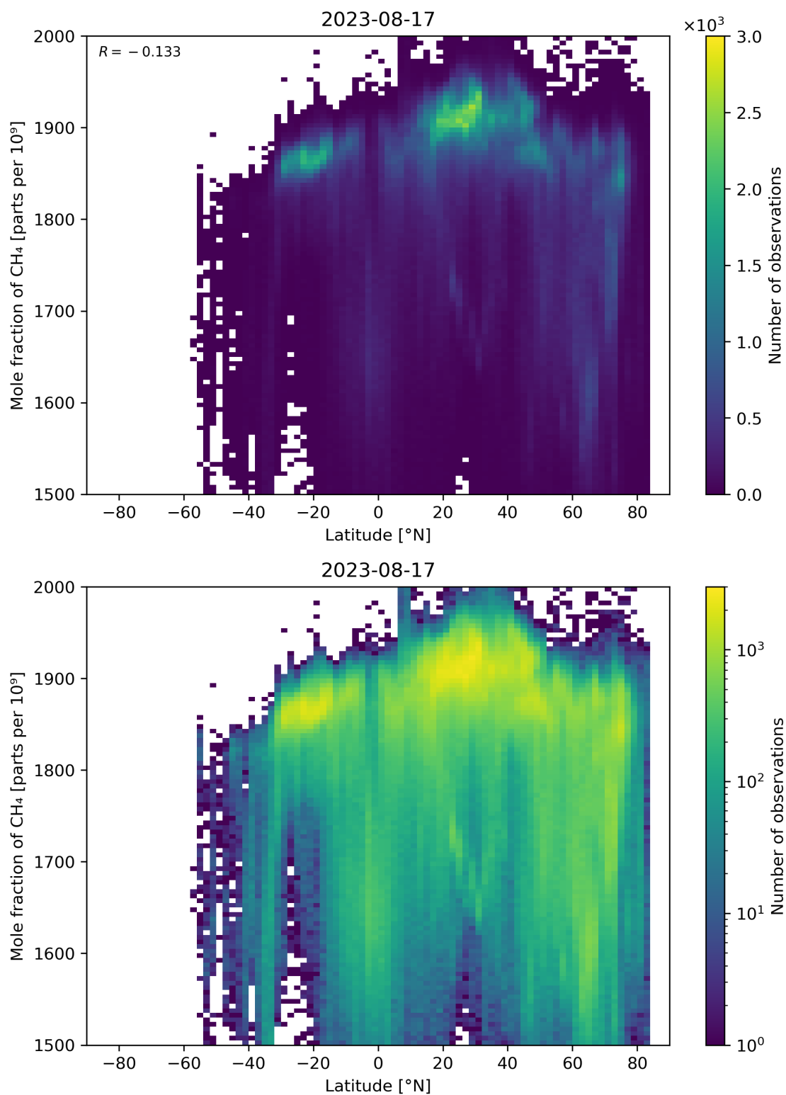
Figure 57: Scatter density plot of “Latitude” against “Mole fraction of CH 4 ” for 2023-08-16 to 2023-08-18.
