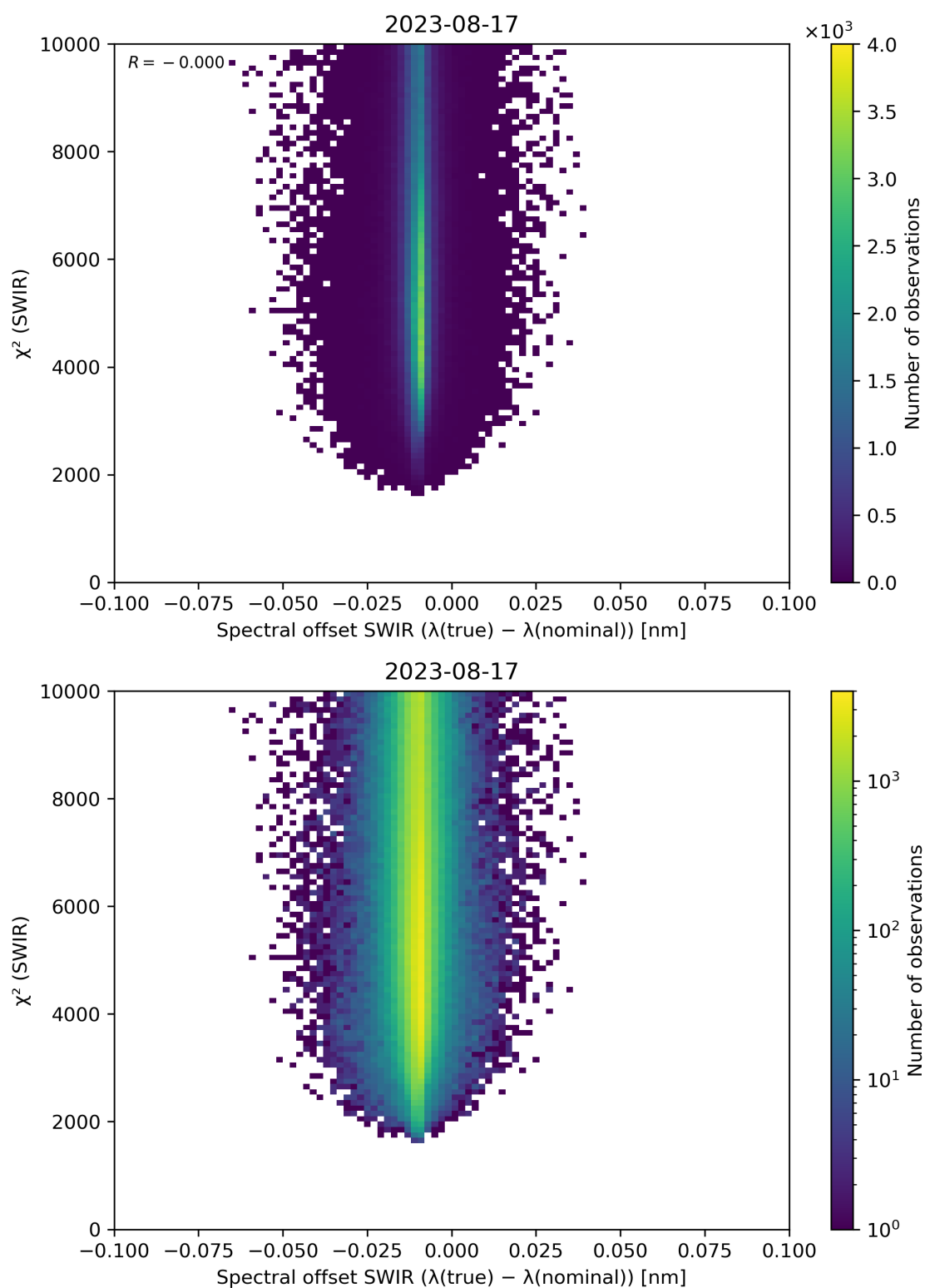
Figure 118: Scatter density plot of “Spectral offset SWIR ( \lambda(\text{true}) - \lambda(\text{nominal}) )” against “ \chi^2 (SWIR)” for 2023-08-16 to 2023-08-18.
