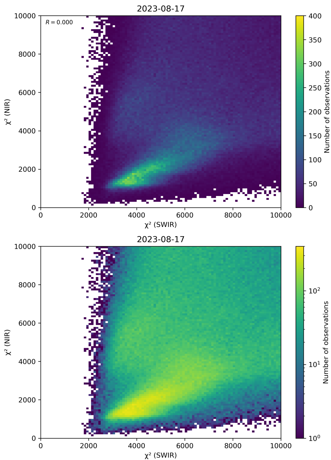
Figure 47: Scatter density plot of “ \chi^2 (SWIR)” against “ \chi^2 (NIR)” for 2023-08-16 to 2023-08-18.
