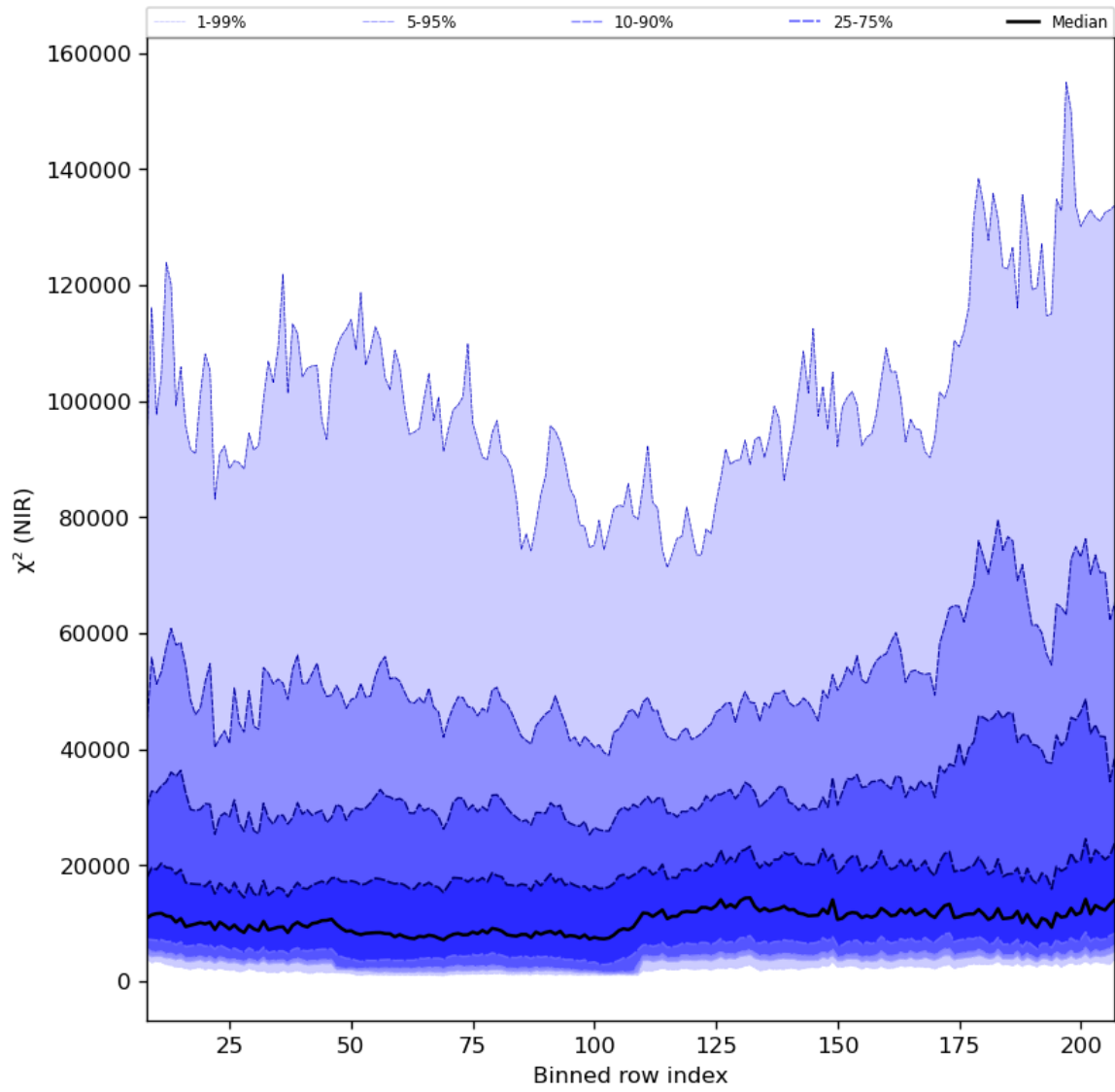
Figure 40: Along track statistics of “ \chi^2 (NIR)” for 2023-08-16 to 2023-08-18
