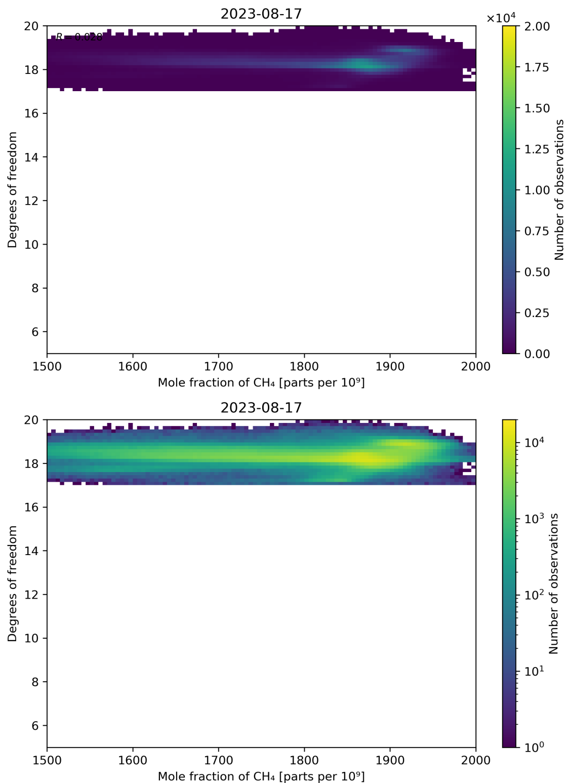
Figure 72: Scatter density plot of “Mole fraction of CH 4 ” against “Degrees of freedom” for 2023-08-16 to 2023-08-18.
