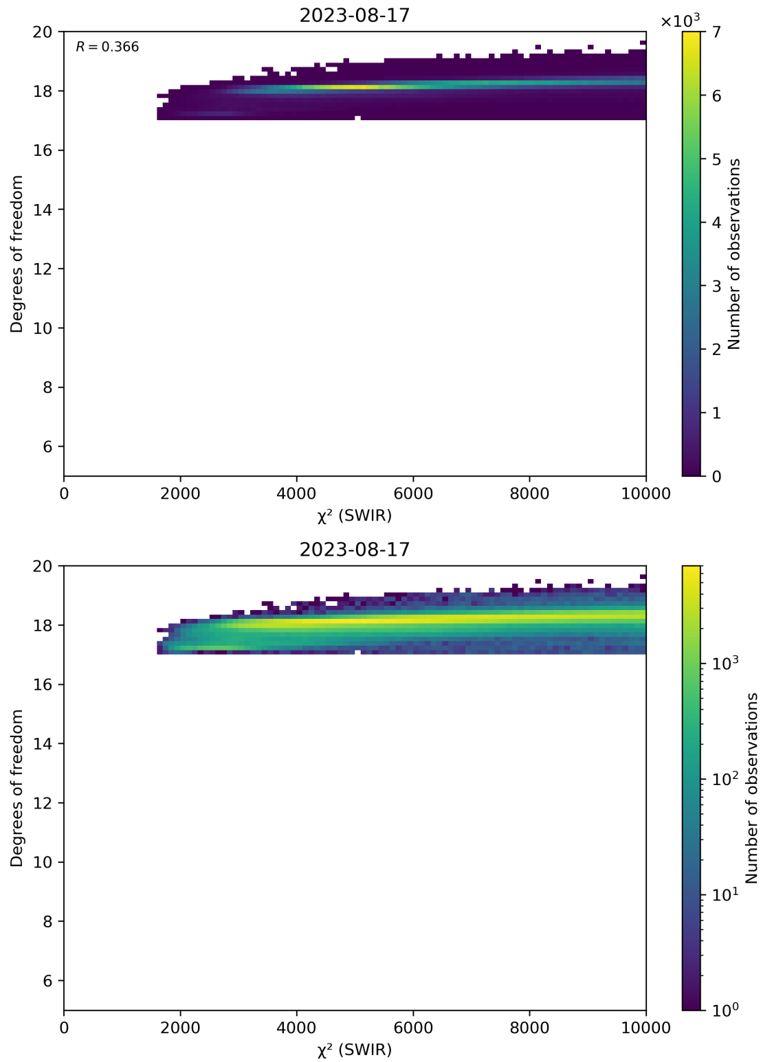
Figure 48: Scatter density plot of “ \chi^2 (SWIR)” against “Degrees of freedom” for 2023-08-16 to 2023-08-18.
