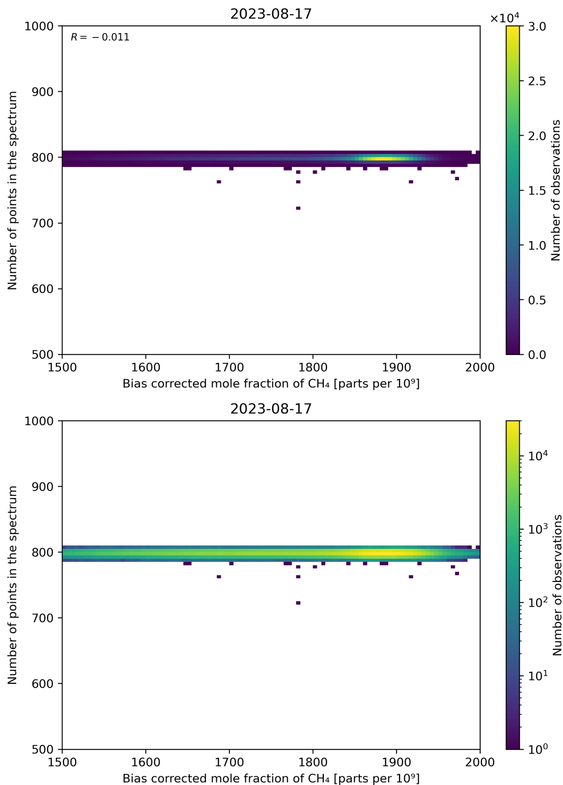
Figure 68: Scatter density plot of “Bias corrected mole fraction of CH 4 ” against “Number of points in the spectrum” for 2023-08-16 to 2023-08-18.
