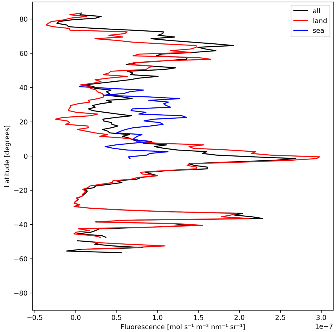
Figure 21: Zonal average of “Fluorescence” for 2023-08-16 to 2023-08-18.
