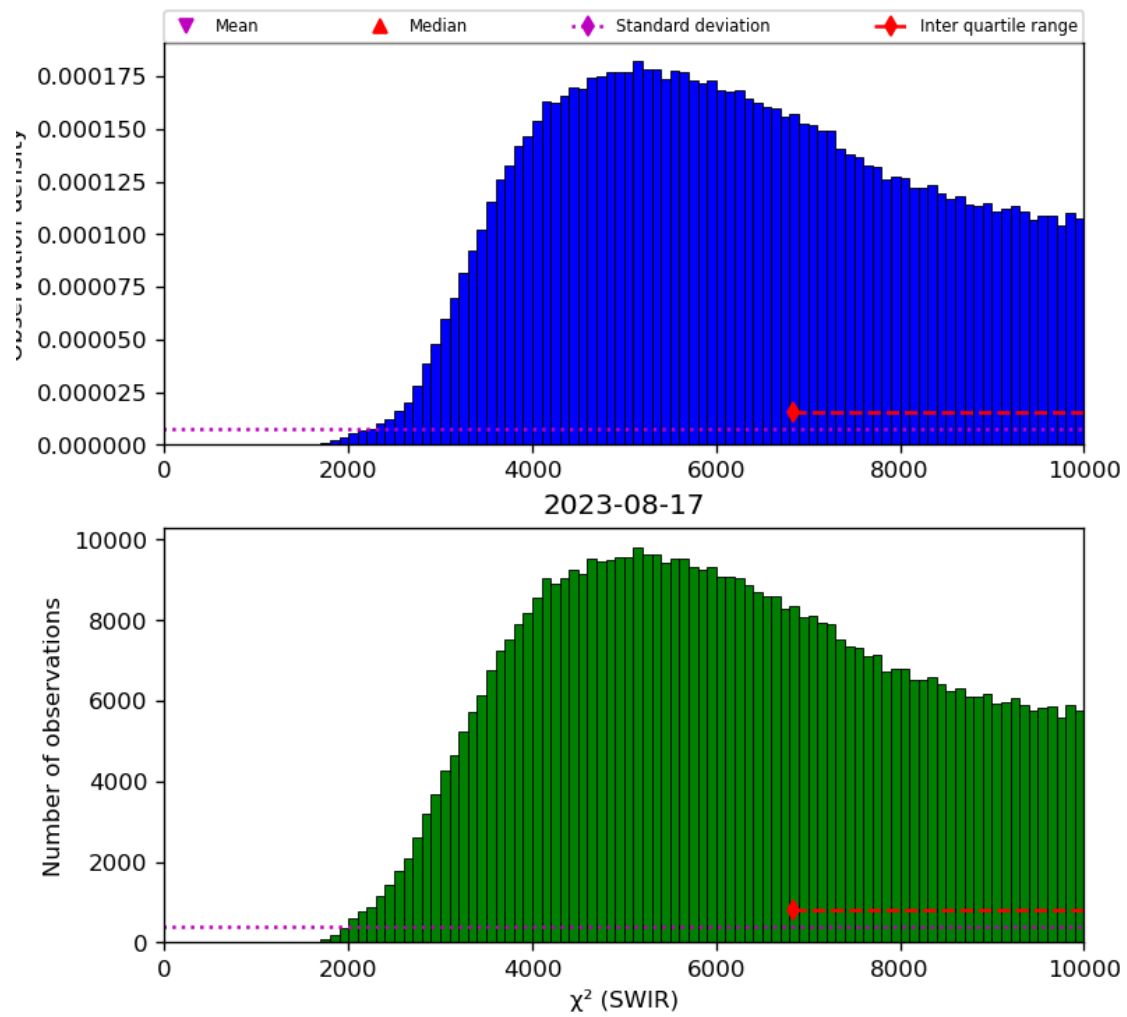
Figure 28: Histogram of " \chi^2 (SWIR)" for 2023-08-16 to 2023-08-18
