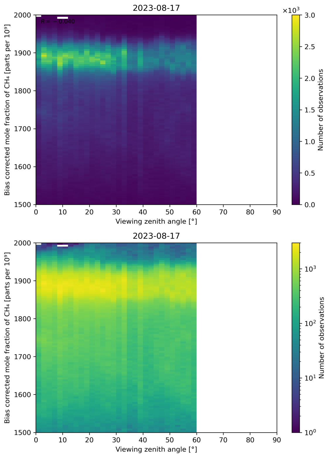
Figure 111: Scatter density plot of “Viewing zenith angle” against “Bias corrected mole fraction of CH 4 ” for 2023-08-16 to 2023-08-18.
