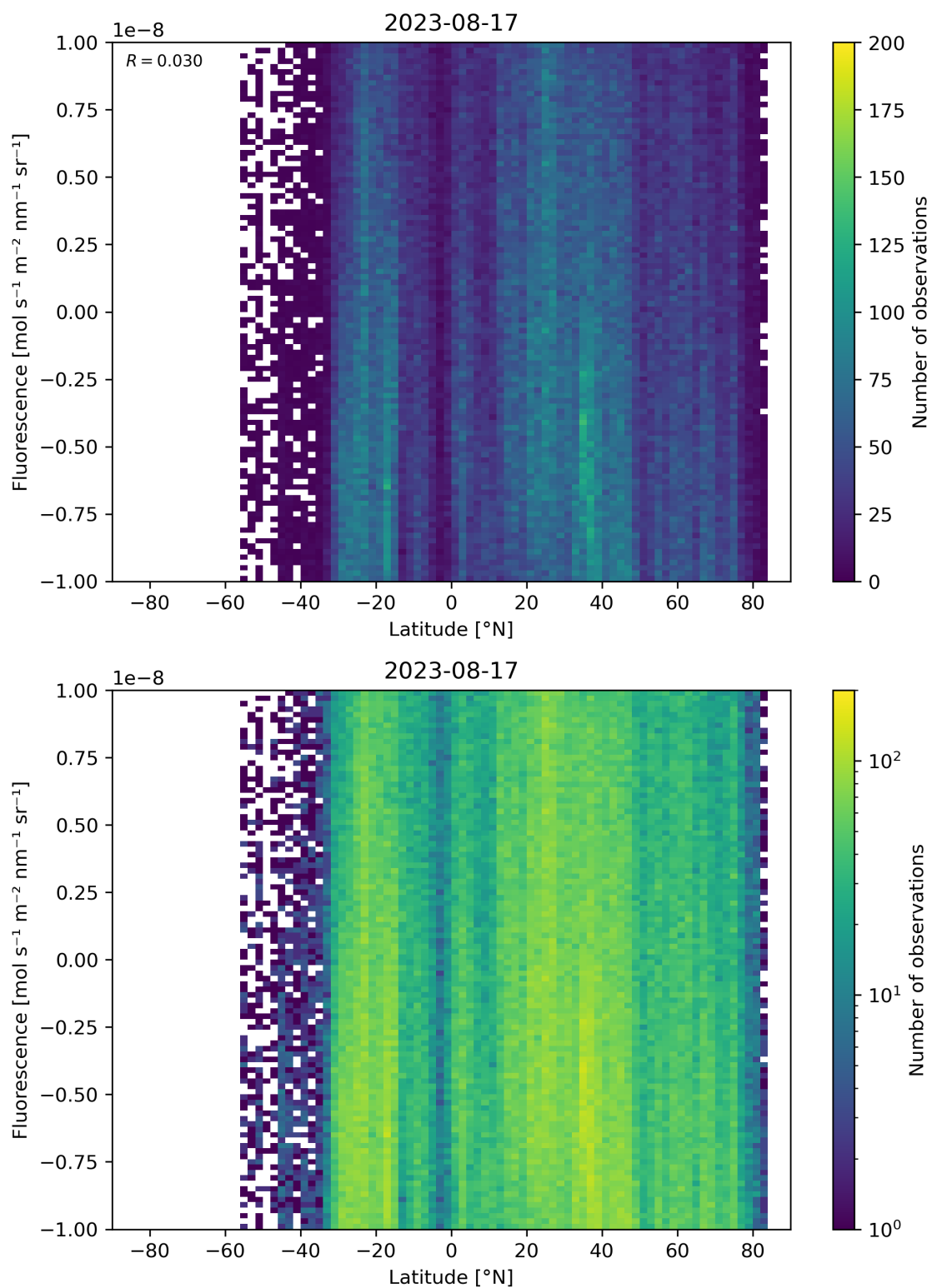
Figure 56: Scatter density plot of “Latitude” against “Fluorescence” for 2023-08-16 to 2023-08-18.
