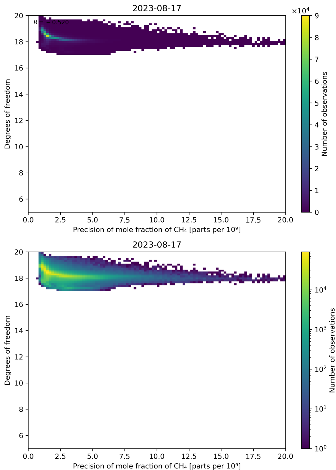
Figure 80: Scatter density plot of “Precision of mole fraction of CH 4 ” against “Degrees of freedom” for 2023-08-16 to 2023-08-18.
