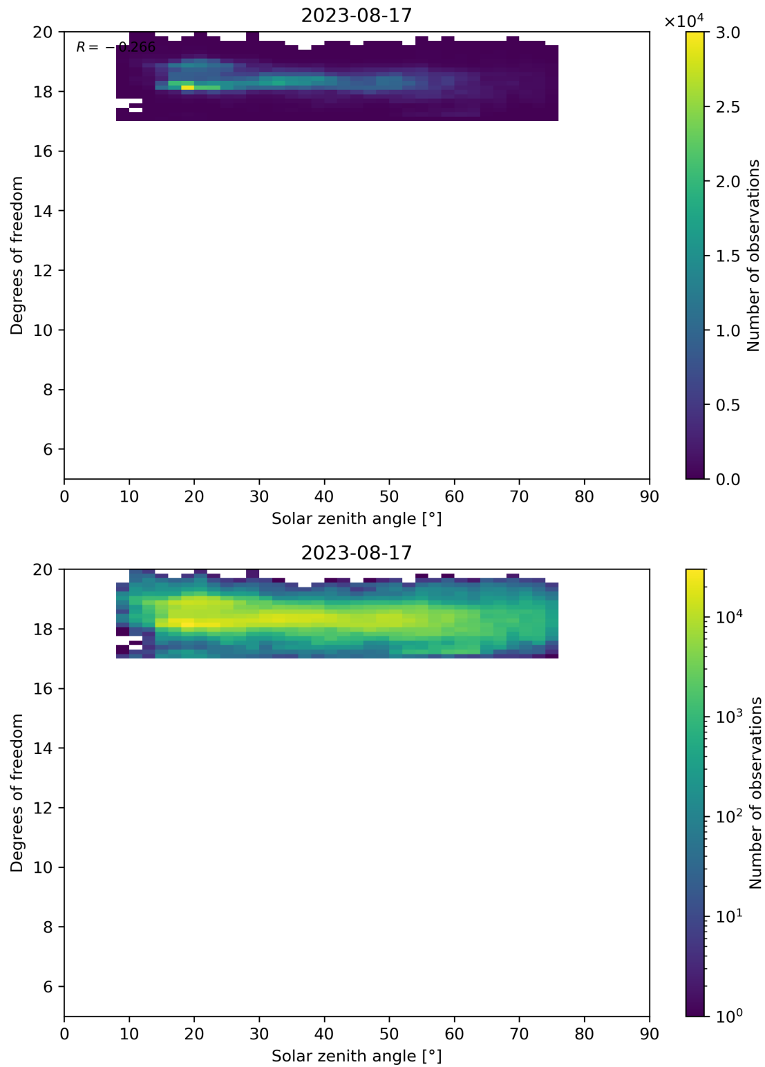
Figure 96: Scatter density plot of “Solar zenith angle” against “Degrees of freedom” for 2023-08-16 to 2023-08-18.
