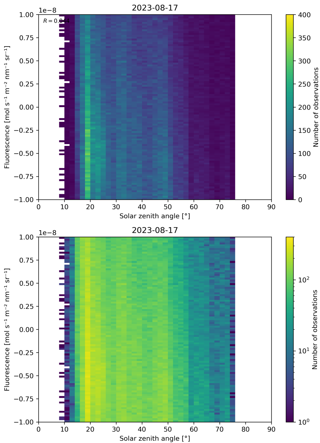
Figure 97: Scatter density plot of “Solar zenith angle” against “Fluorescence” for 2023-08-16 to 2023-08-18.
