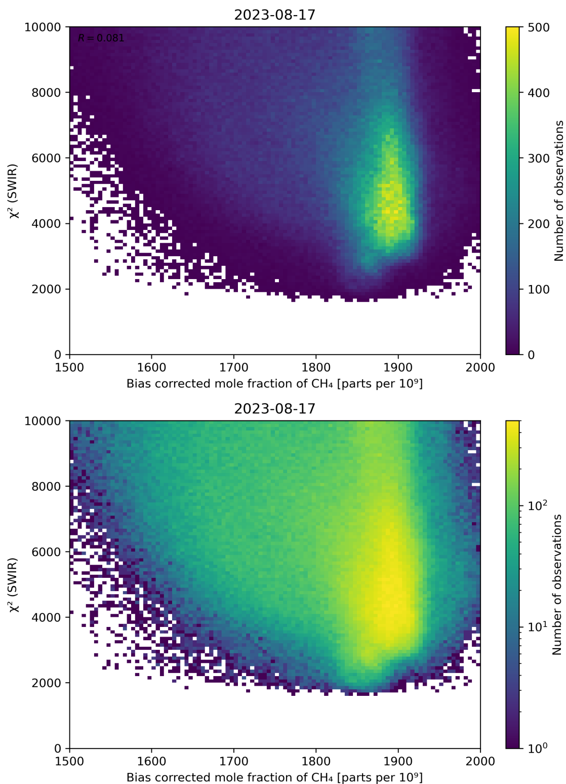
Figure 64: Scatter density plot of “Bias corrected mole fraction of CH 4 ” against “ \chi^2 (SWIR)” for 2023-08-16 to 2023-08-18.
