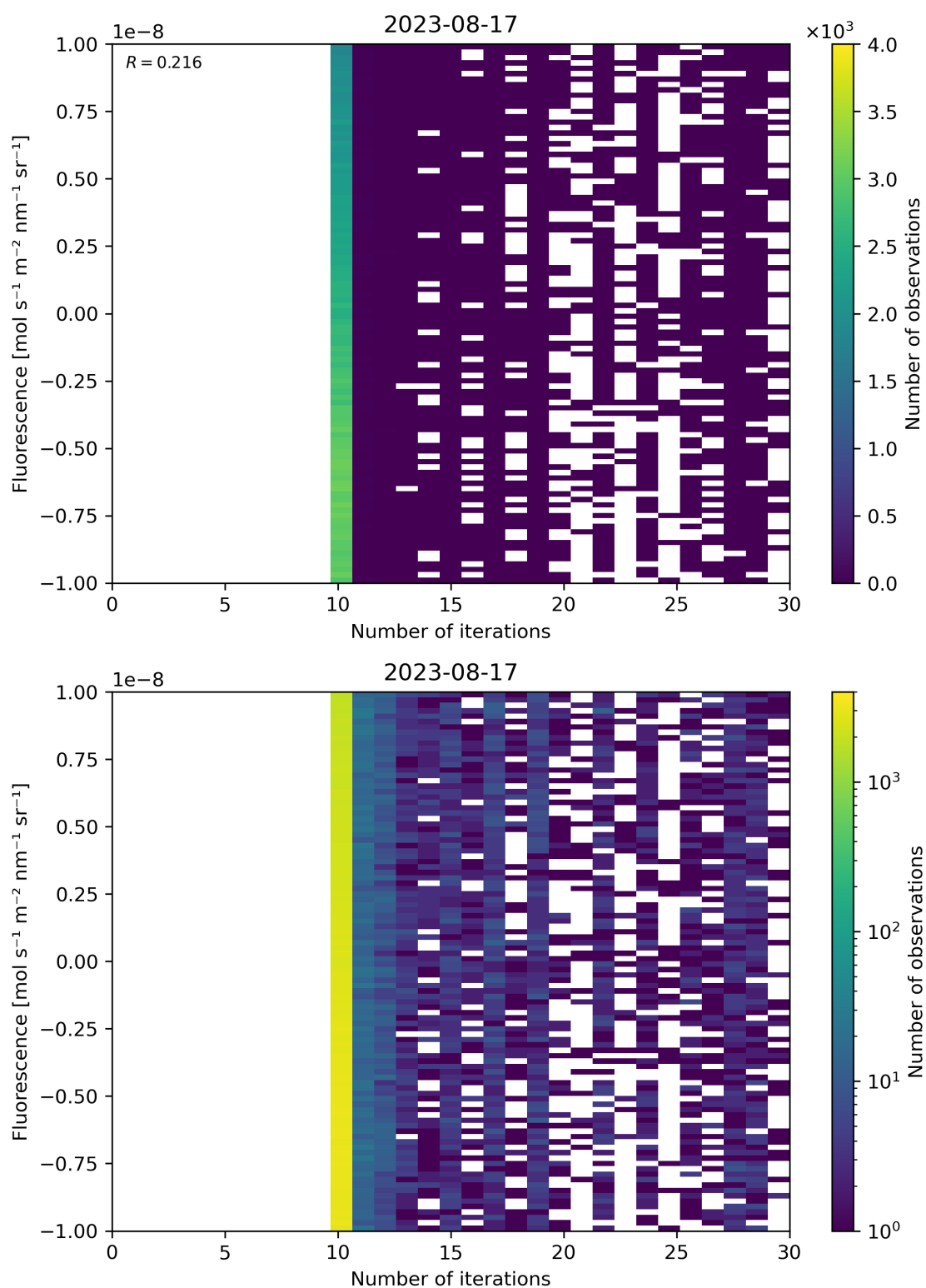
Figure 87: Scatter density plot of “Number of iterations” against “Fluorescence” for 2023-08-16 to 2023-08-18.
