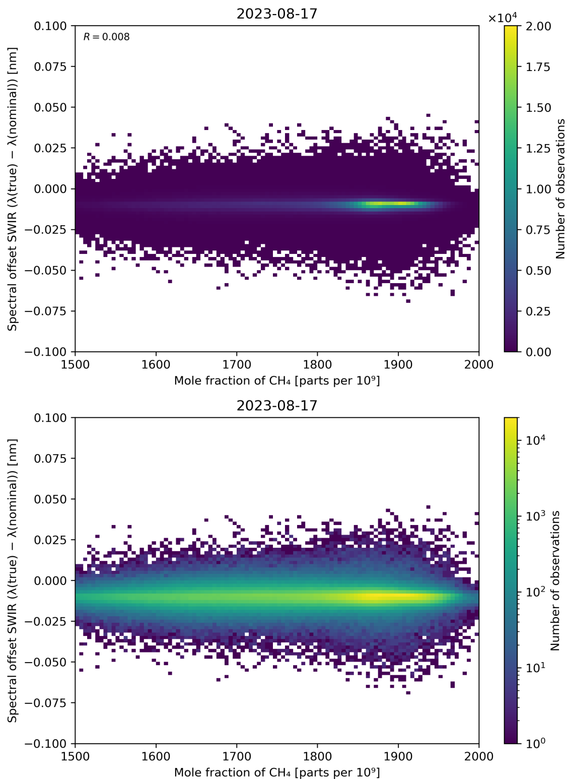
Figure 86: Scatter density plot of “Mole fraction of CH 4 ” against “Spectral offset SWIR ( \lambda(\text{true}) - \lambda(\text{nominal}) )” for 2023-08-16 to 2023-08-18.
