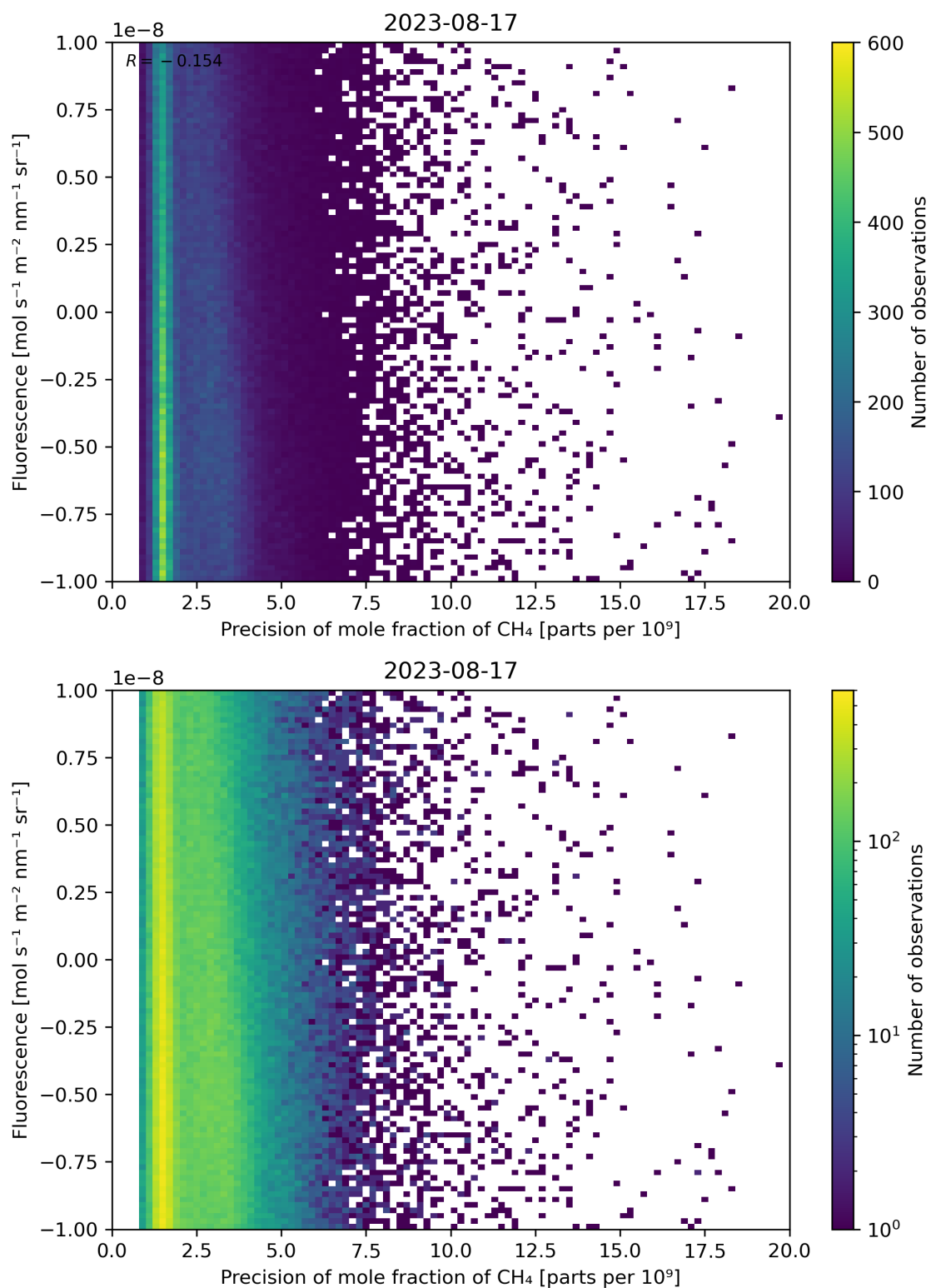
Figure 81: Scatter density plot of “Precision of mole fraction of CH 4 ” against “Fluorescence” for 2023-08-16 to 2023-08-18.
