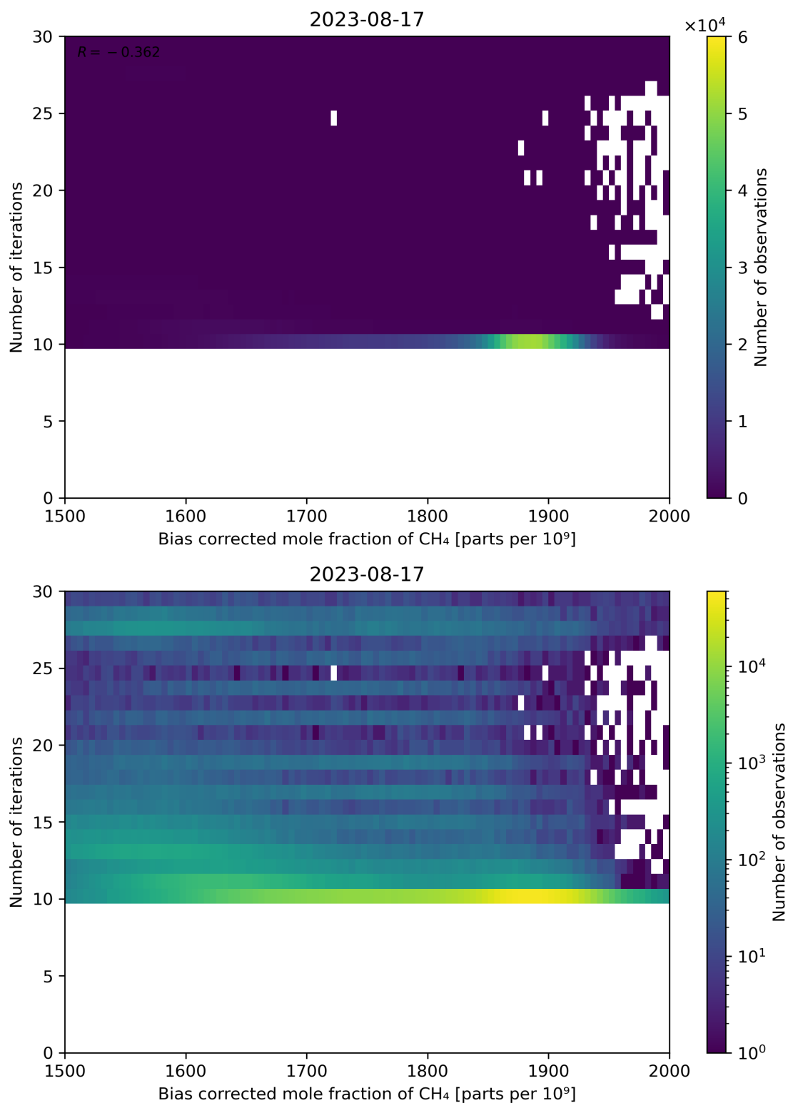
Figure 67: Scatter density plot of “Bias corrected mole fraction of CH 4 ” against “Number of iterations” for 2023-08-16 to 2023-08-18.
