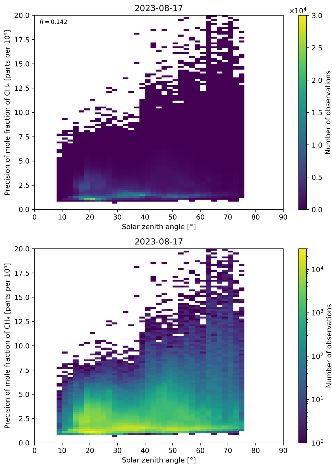
Figure 101: Scatter density plot of “Solar zenith angle” against “Precision of mole fraction of \text{CH}_4 ” for 2023-08-16 to 2023-08-18.
