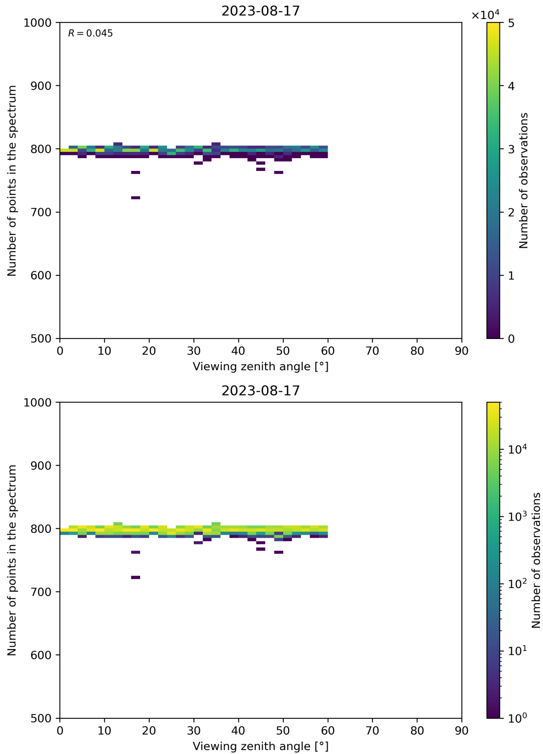
Figure 114: Scatter density plot of “Viewing zenith angle” against “Number of points in the spectrum” for 2023-08-16 to 2023-08-18.
