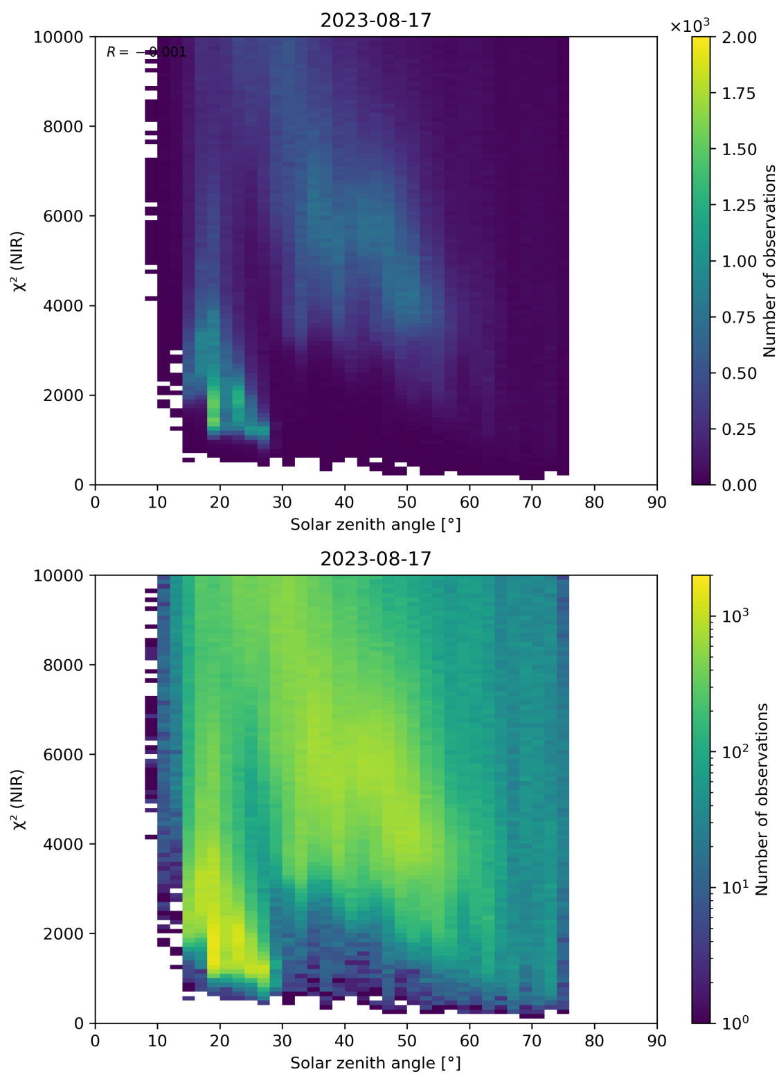
Figure 94: Scatter density plot of “Solar zenith angle” against “ \chi^2 (NIR)” for 2023-08-16 to 2023-08-18.
