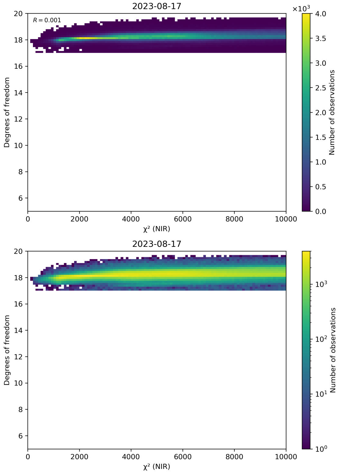
Figure 44: Scatter density plot of “ \chi^2 (NIR)” against “Degrees of freedom” for 2023-08-16 to 2023-08-18.
