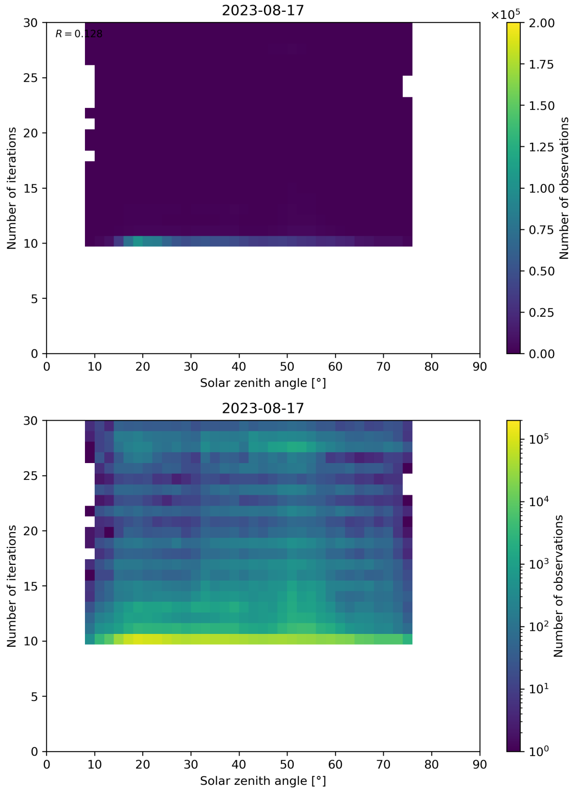
Figure 102: Scatter density plot of “Solar zenith angle” against “Number of iterations” for 2023-08-16 to 2023-08-18.
