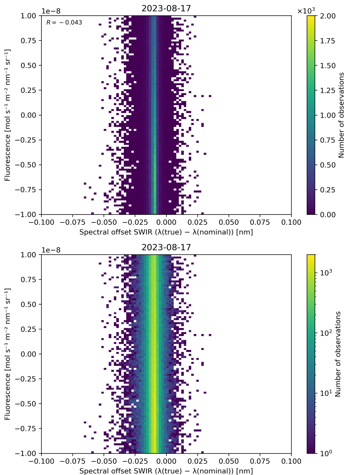
Figure 120: Scatter density plot of “Spectral offset SWIR ( \lambda(\text{true}) - \lambda(\text{nominal}) )” against “Fluorescence” for 2023-08-16 to 2023-08-18.
