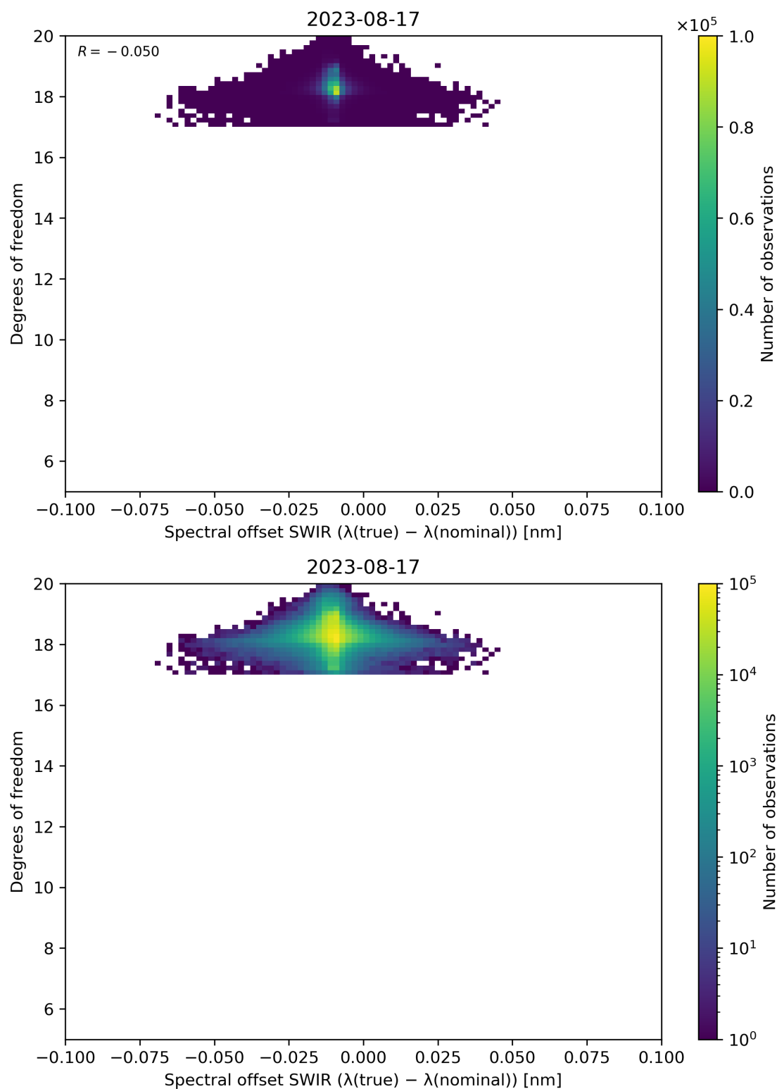
Figure 119: Scatter density plot of “Spectral offset SWIR ( \lambda(\text{true}) - \lambda(\text{nominal}) )” against “Degrees of freedom” for 2023-08-16 to 2023-08-18.
