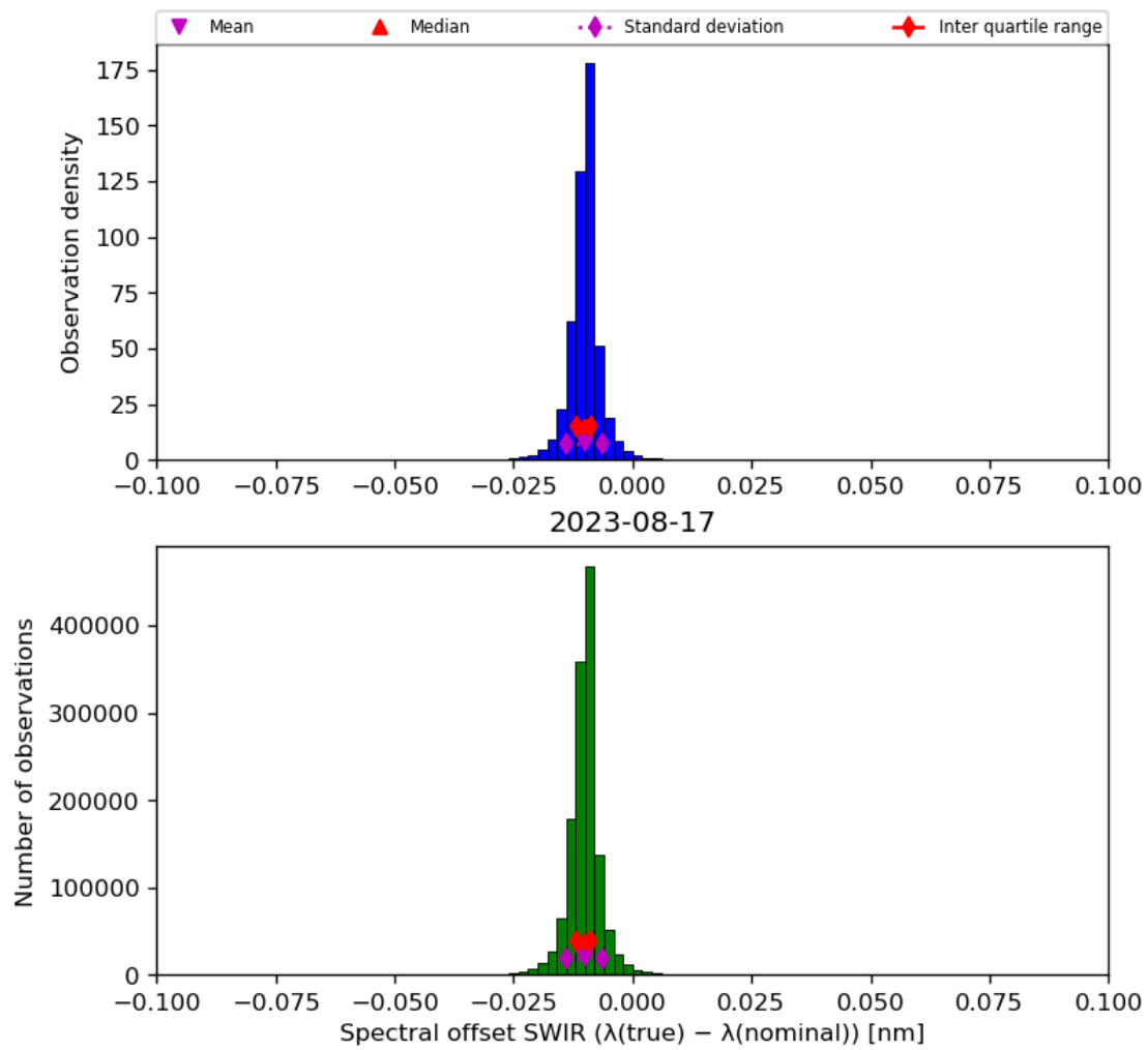
Figure 27: Histogram of “Spectral offset SWIR ( \lambda(\text{true}) - \lambda(\text{nominal}) )” for 2023-08-16 to 2023-08-18
