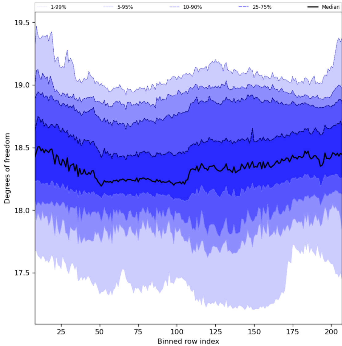
Figure 41: Along track statistics of “Degrees of freedom” for 2023-08-16 to 2023-08-18
