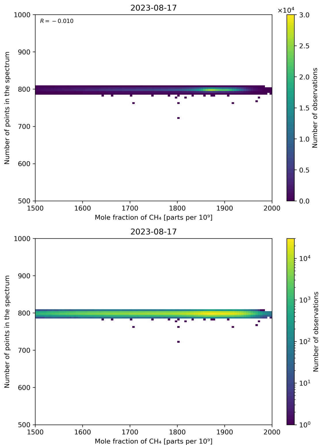
Figure 77: Scatter density plot of “Mole fraction of CH 4 ” against “Number of points in the spectrum” for 2023-08-16 to 2023-08-18.
