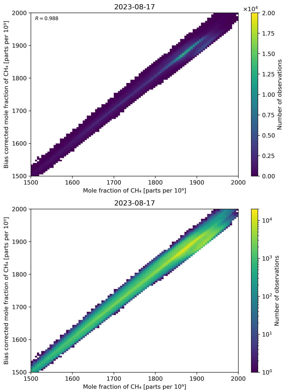
Figure 74: Scatter density plot of “Mole fraction of CH 4 ” against “Bias corrected mole fraction of CH 4 ” for 2023-08-16 to 2023-08-18.
