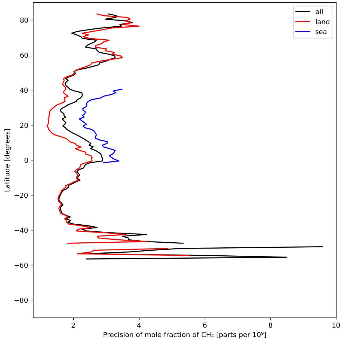
Figure 13: Zonal average of “Precision of mole fraction of CH 4 ” for 2023-08-16 to 2023-08-18.
