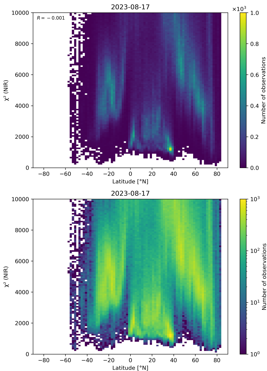
Figure 53: Scatter density plot of “Latitude” against “ \chi^2 (NIR)” for 2023-08-16 to 2023-08-18.
