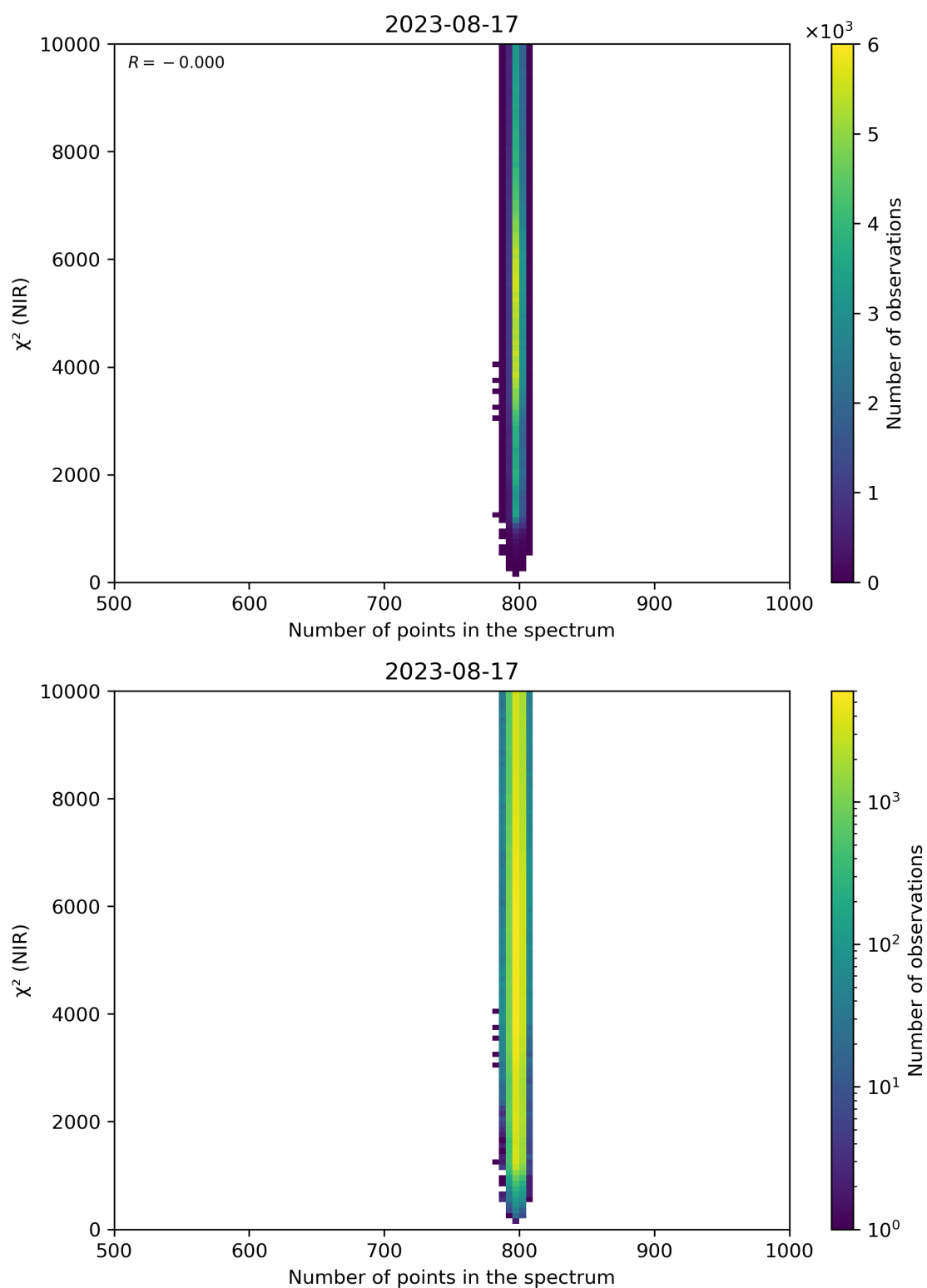
Figure 88: Scatter density plot of “Number of points in the spectrum” against “ \chi^2 (NIR)” for 2023-08-16 to 2023-08-18.
