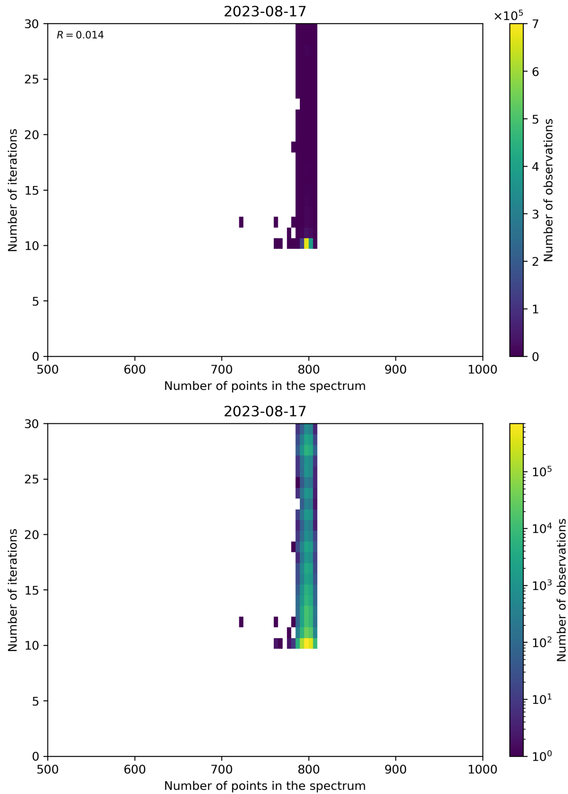
Figure 92: Scatter density plot of “Number of points in the spectrum” against “Number of iterations” for 2023-08-16 to 2023-08-18.
