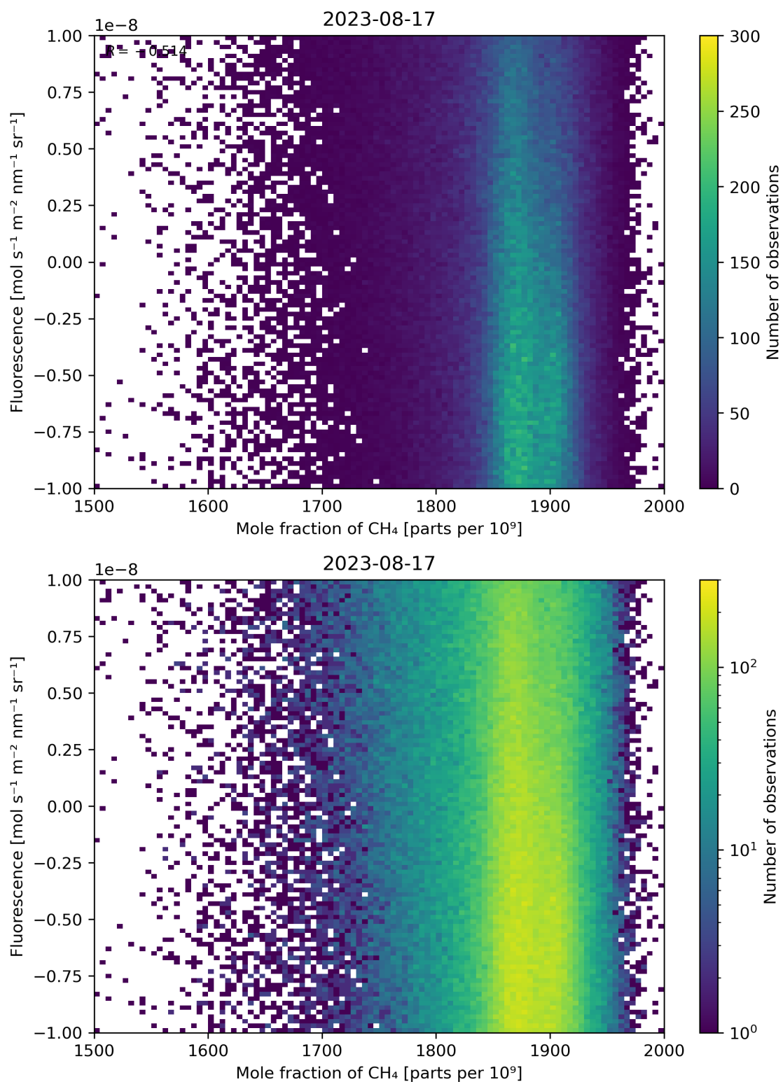
Figure 73: Scatter density plot of “Mole fraction of \text{CH}_4 ” against “Fluorescence” for 2023-08-16 to 2023-08-18.
