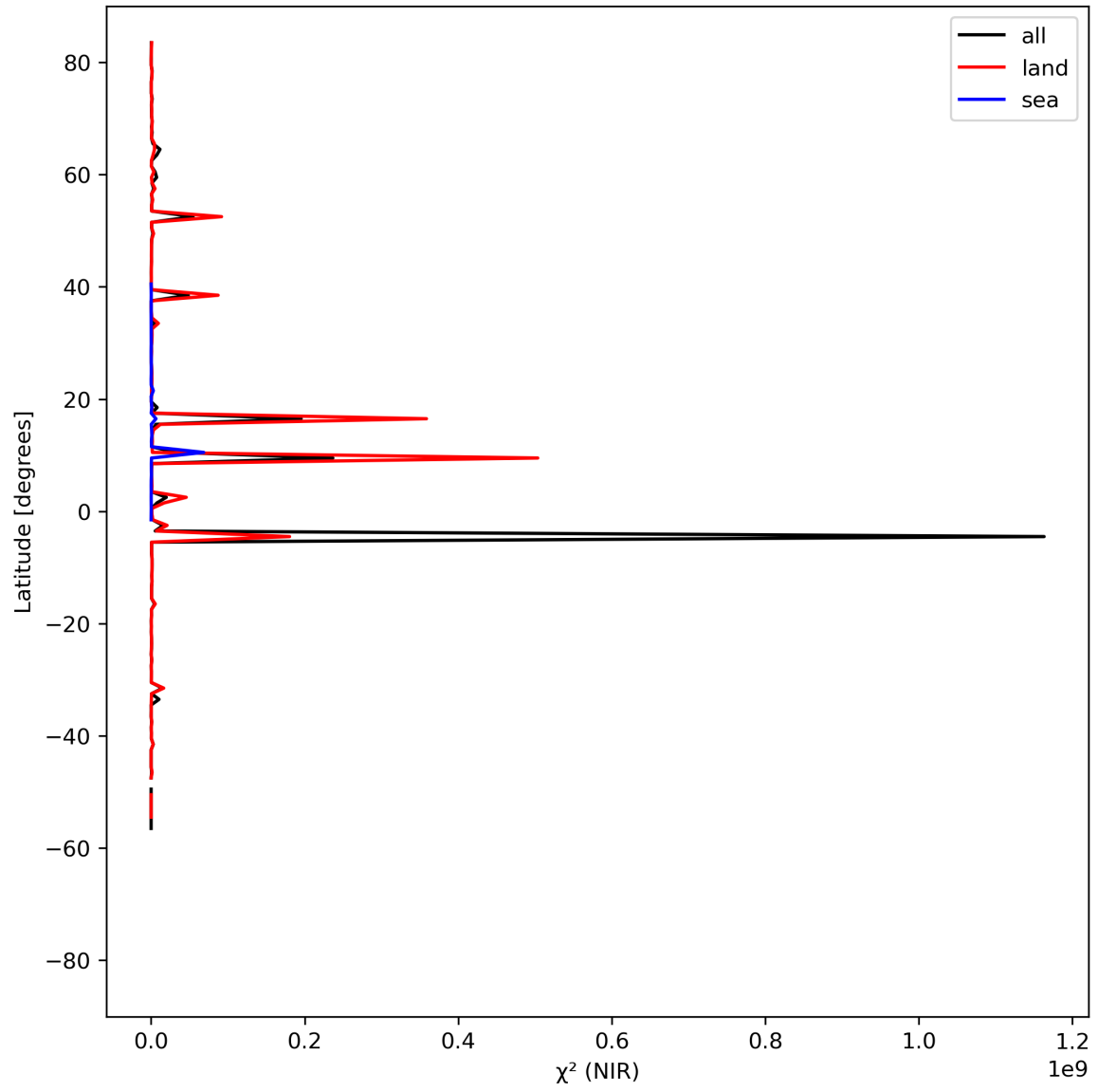
Figure 18: Zonal average of “ \chi^2 (NIR)” for 2023-08-16 to 2023-08-18.
