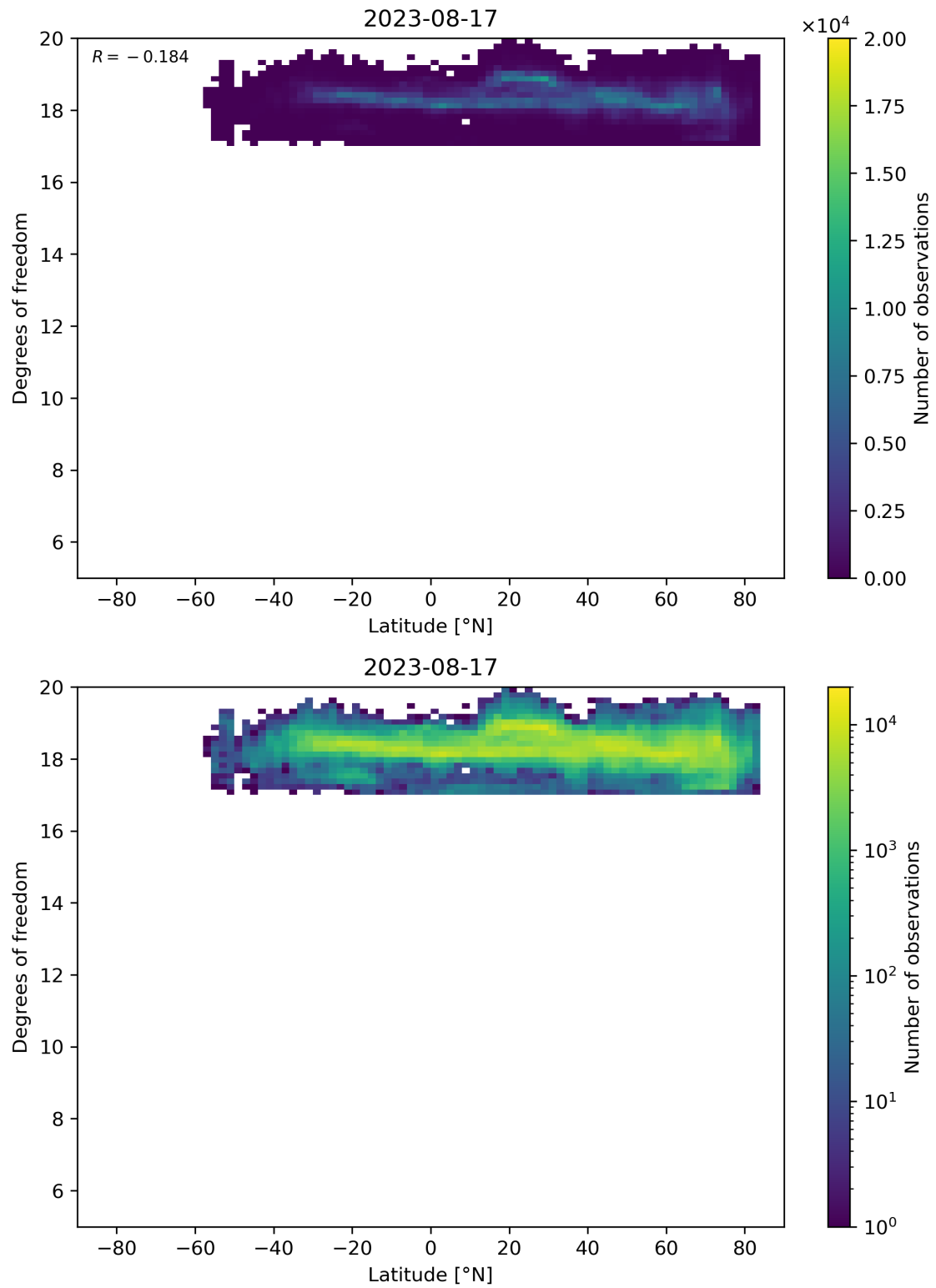
Figure 55: Scatter density plot of “Latitude” against “Degrees of freedom” for 2023-08-16 to 2023-08-18.
