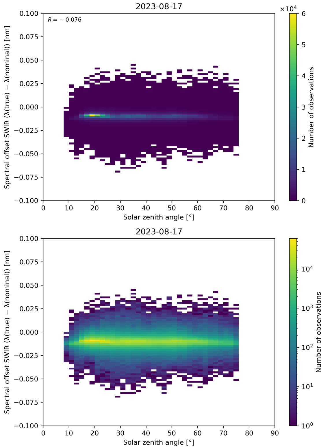
Figure 104: Scatter density plot of “Solar zenith angle” against “Spectral offset SWIR ( \lambda(\text{true}) - \lambda(\text{nominal}) )” for 2023-08-16 to 2023-08-18.
