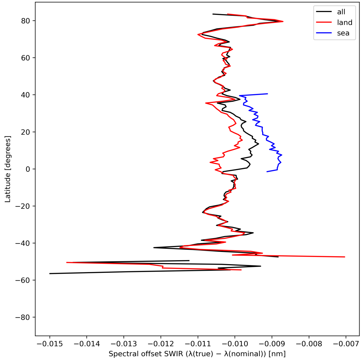
Figure 16: Zonal average of “Spectral offset SWIR ( \lambda(\text{true}) - \lambda(\text{nominal}) )” for 2023-08-16 to 2023-08-18.
