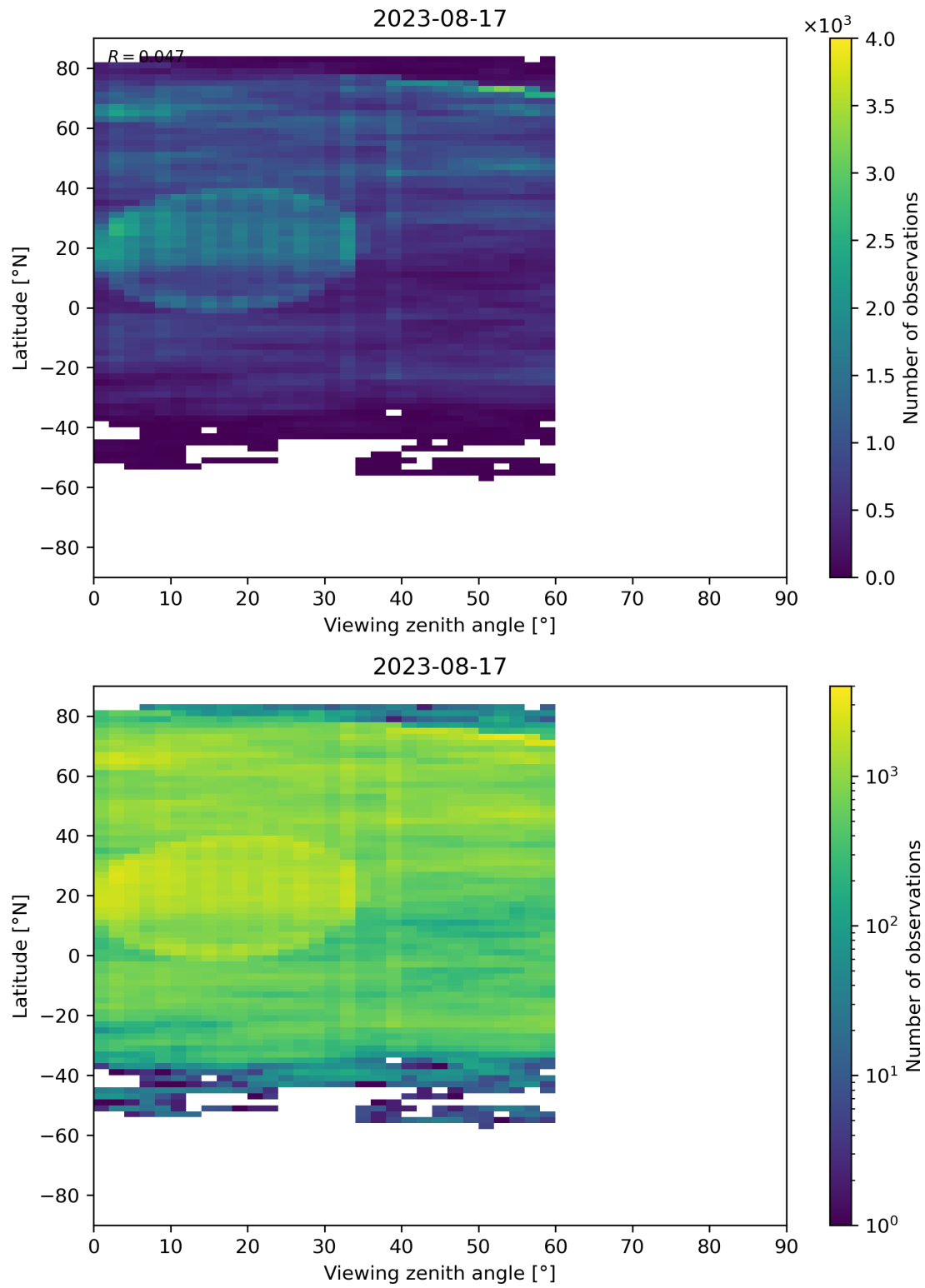
Figure 109: Scatter density plot of “Viewing zenith angle” against “Latitude” for 2023-08-16 to 2023-08-18.
