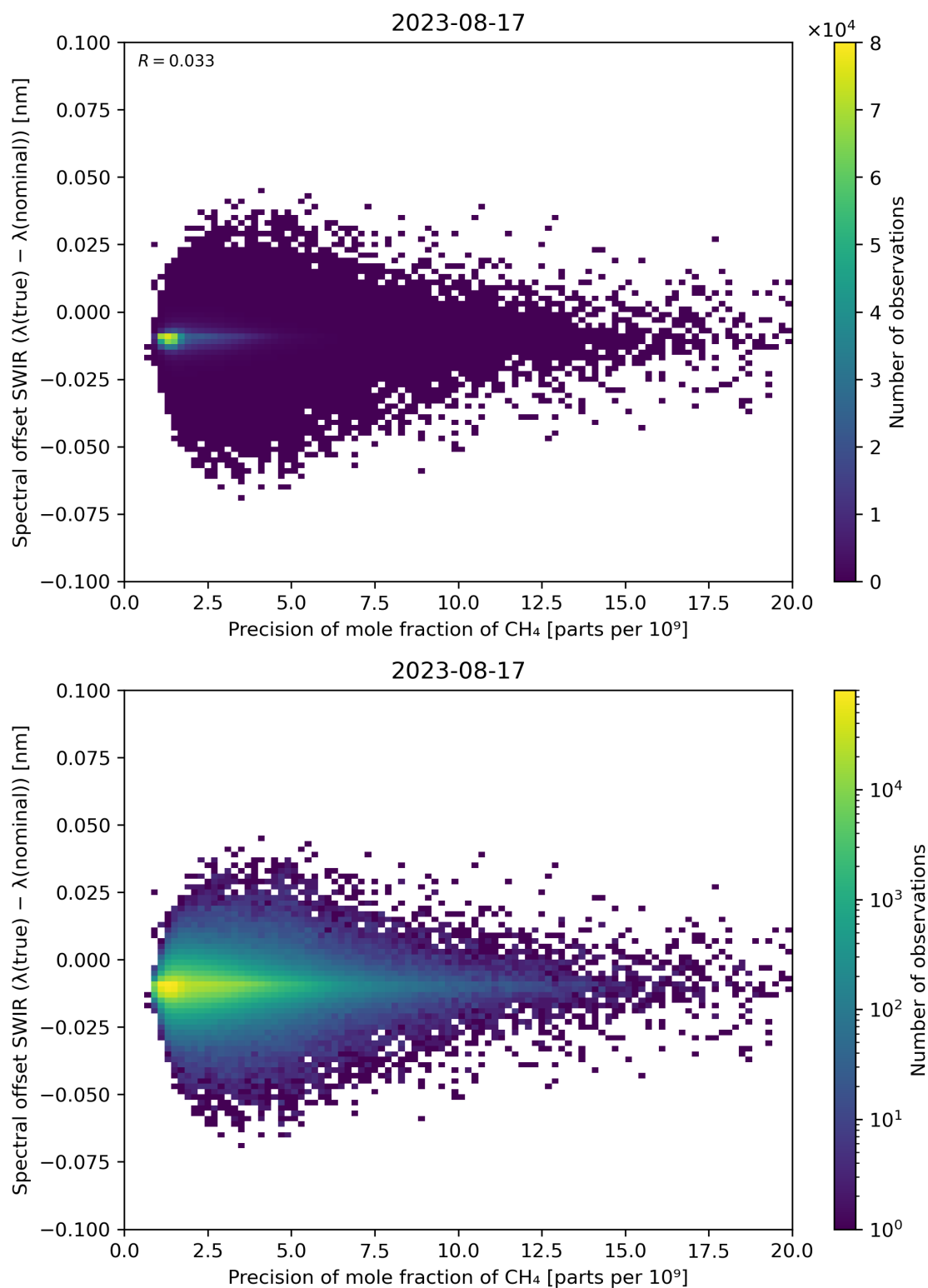
Figure 85: Scatter density plot of “Precision of mole fraction of \text{CH}_4 ” against “Spectral offset SWIR ( \lambda(\text{true}) - \lambda(\text{nominal}) )” for 2023-08-16 to 2023-08-18.
