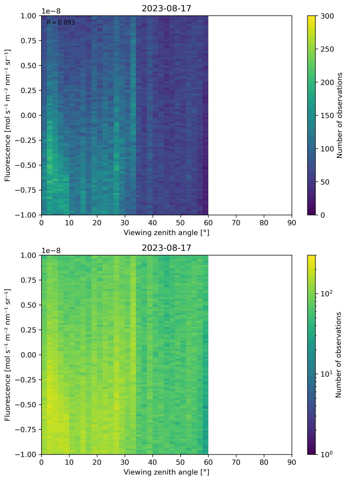
Figure 108: Scatter density plot of “Viewing zenith angle” against “Fluorescence” for 2023-08-16 to 2023-08-18.
