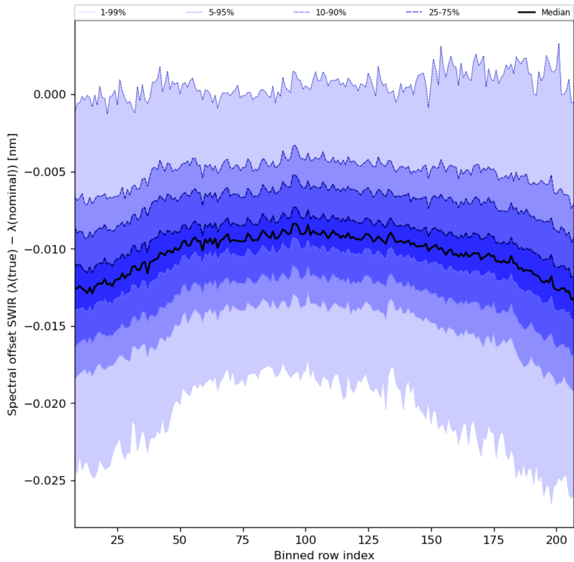
Figure 38: Along track statistics of “Spectral offset SWIR ( \lambda(\text{true}) - \lambda(\text{nominal}) )” for 2023-08-16 to 2023-08-18
