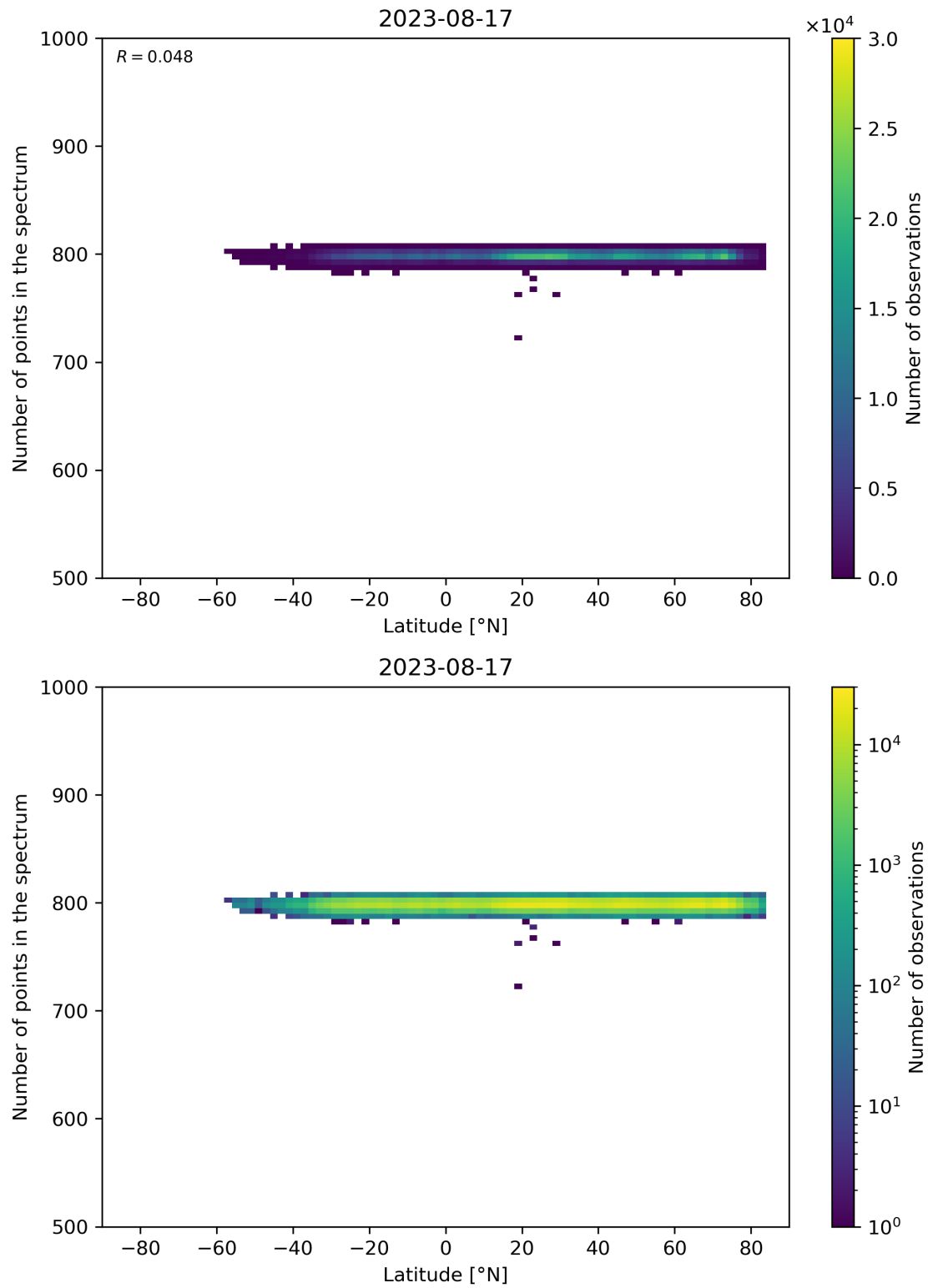
Figure 61: Scatter density plot of “Latitude” against “Number of points in the spectrum” for 2023-08-16 to 2023-08-18.
