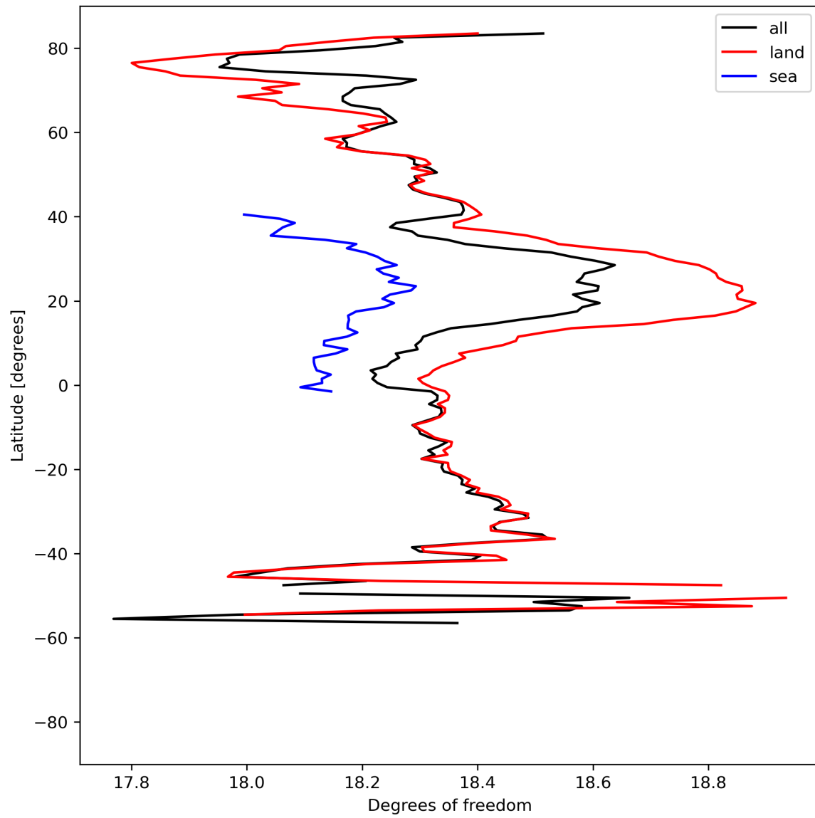
Figure 19: Zonal average of “Degrees of freedom” for 2023-08-16 to 2023-08-18.
