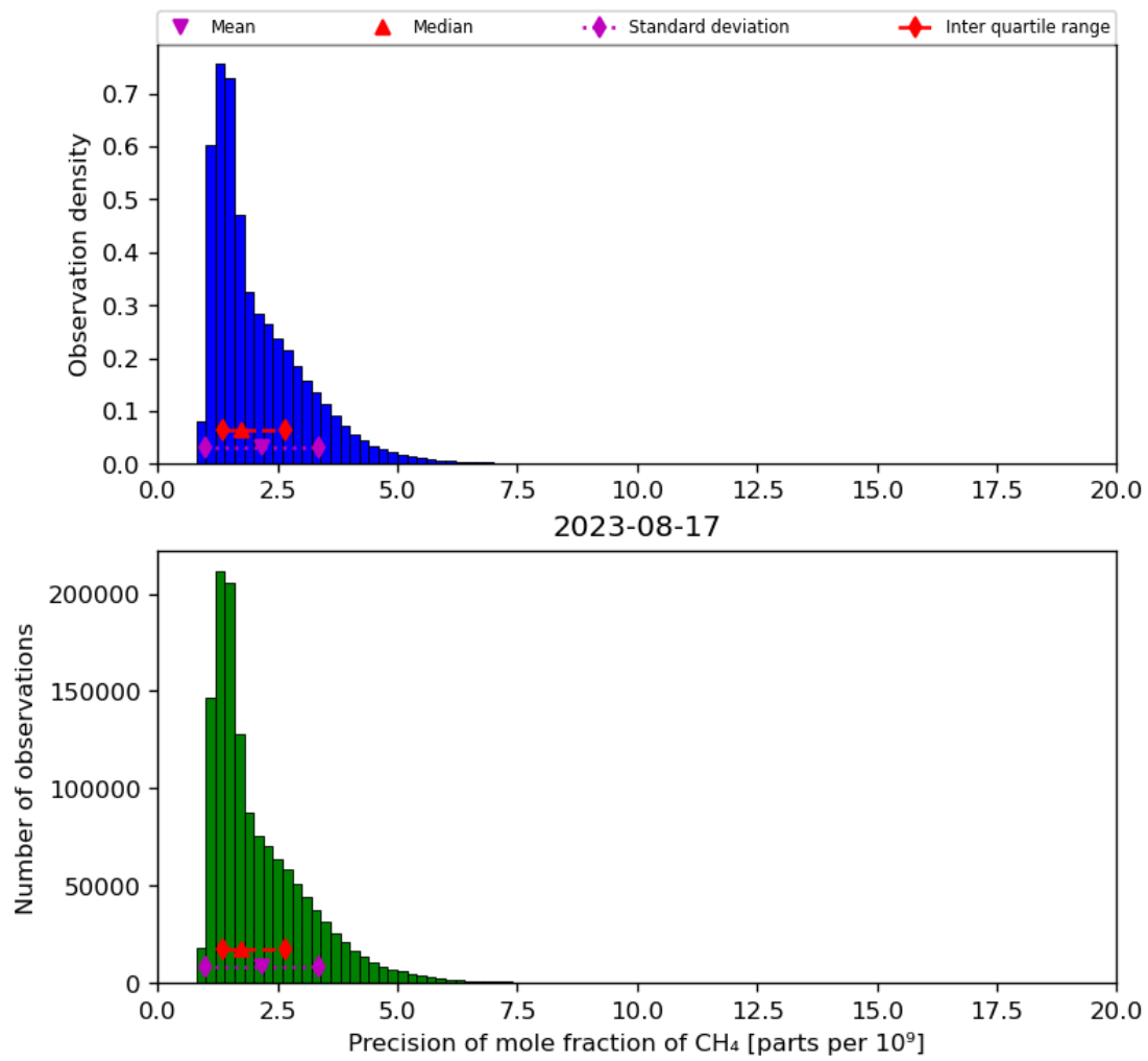
Figure 24: Histogram of “Precision of mole fraction of CH 4 ” for 2023-08-16 to 2023-08-18
