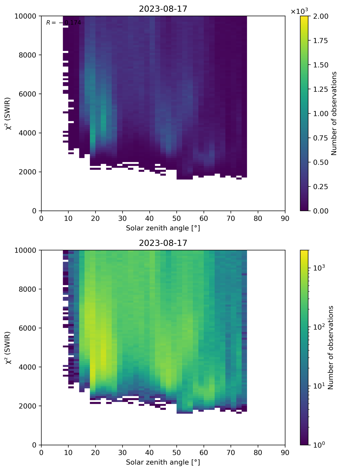
Figure 95: Scatter density plot of “Solar zenith angle” against “ \chi^2 (SWIR)” for 2023-08-16 to 2023-08-18.
