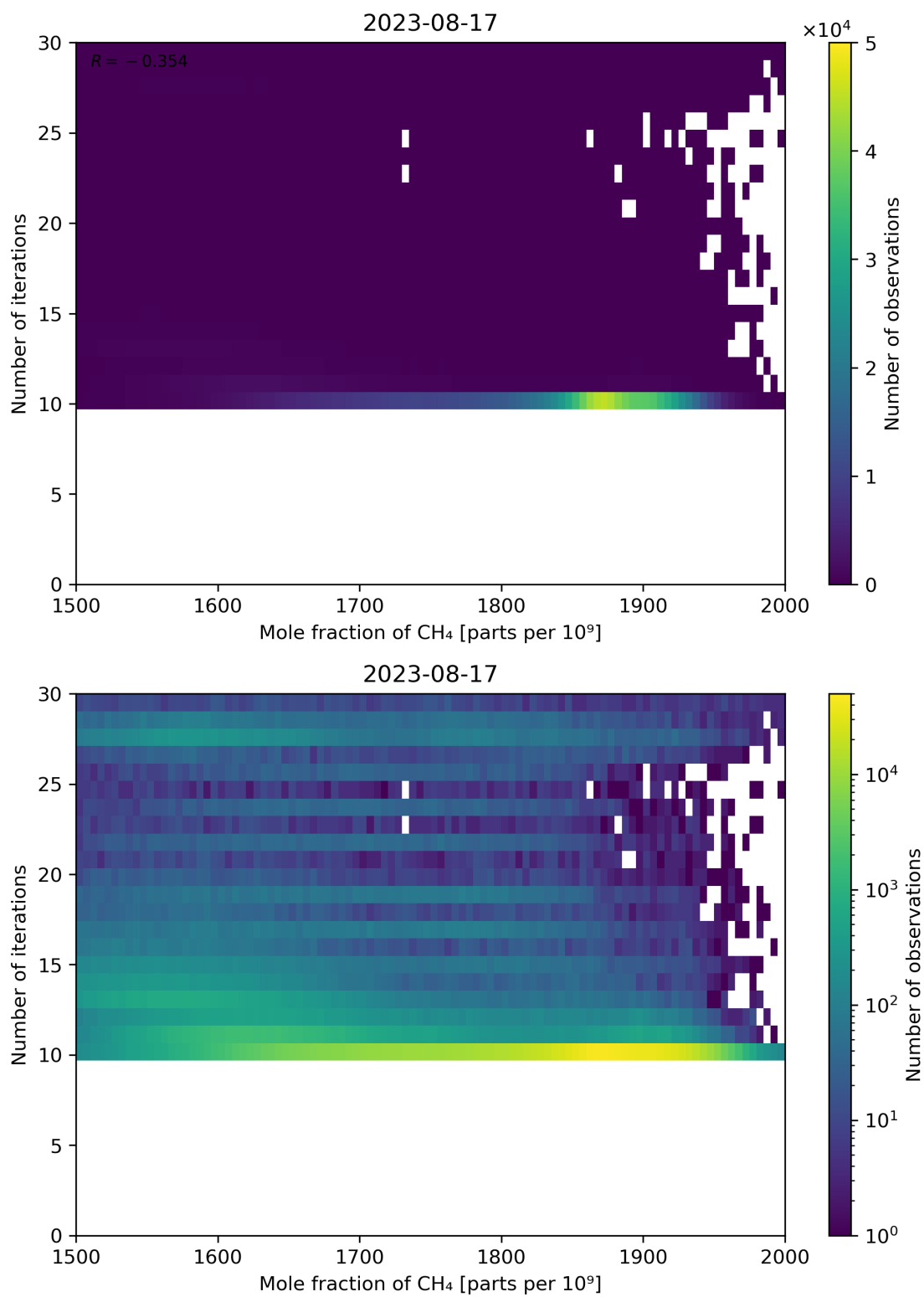
Figure 76: Scatter density plot of “Mole fraction of CH 4 ” against “Number of iterations” for 2023-08-16 to 2023-08-18.
