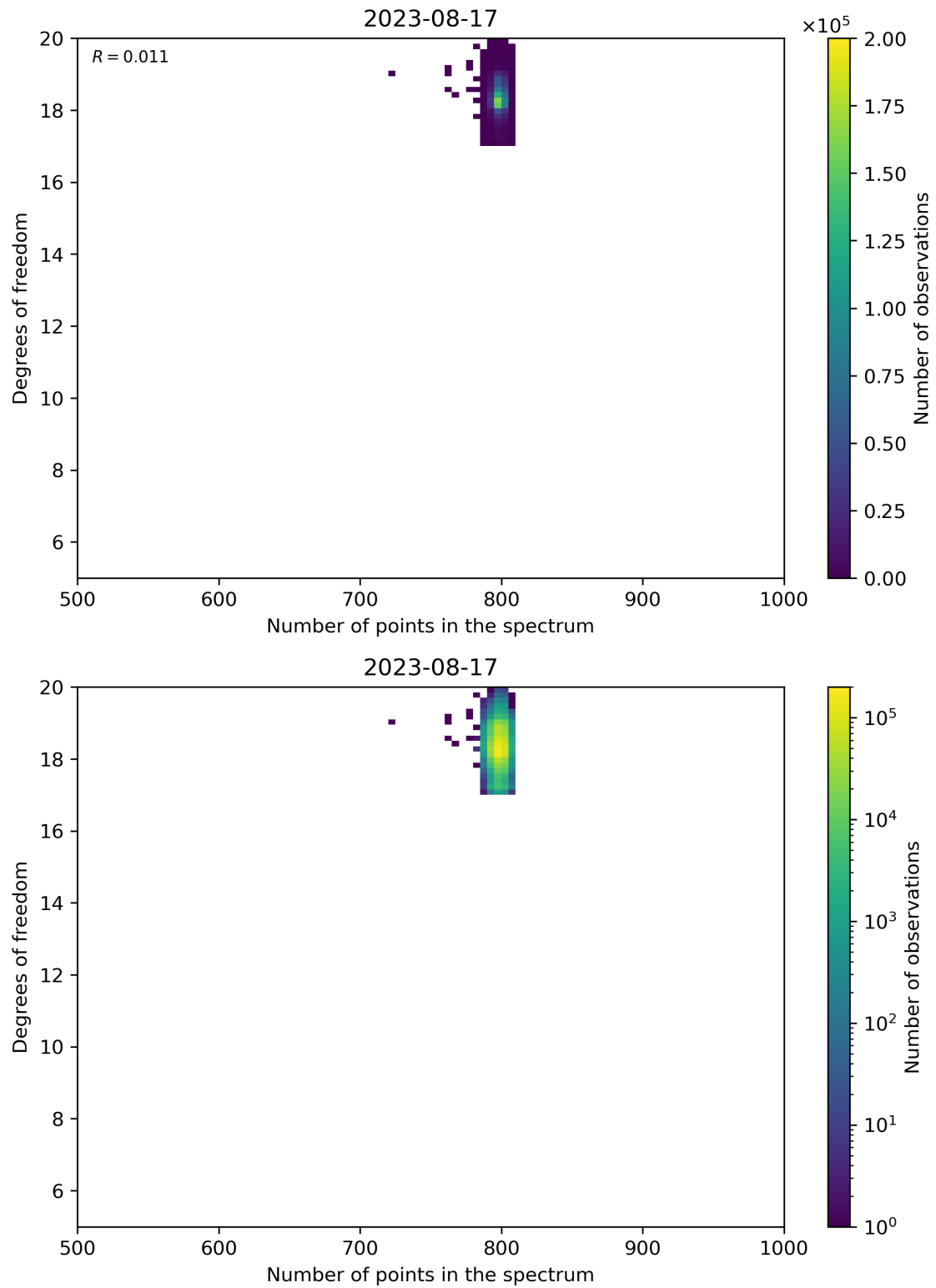
Figure 90: Scatter density plot of “Number of points in the spectrum” against “Degrees of freedom” for 2023-08-16 to 2023-08-18.
