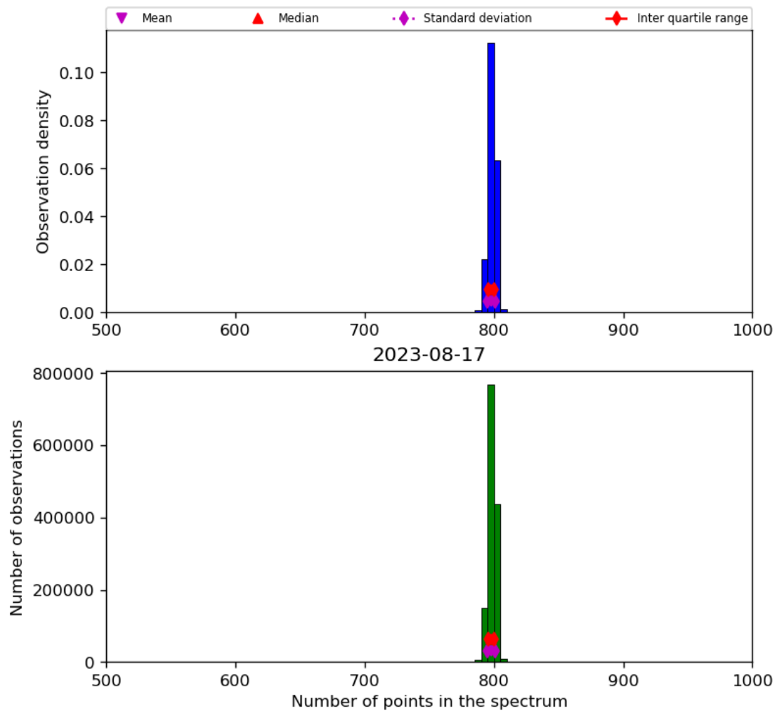
Figure 26: Histogram of “Number of points in the spectrum” for 2023-08-16 to 2023-08-18
