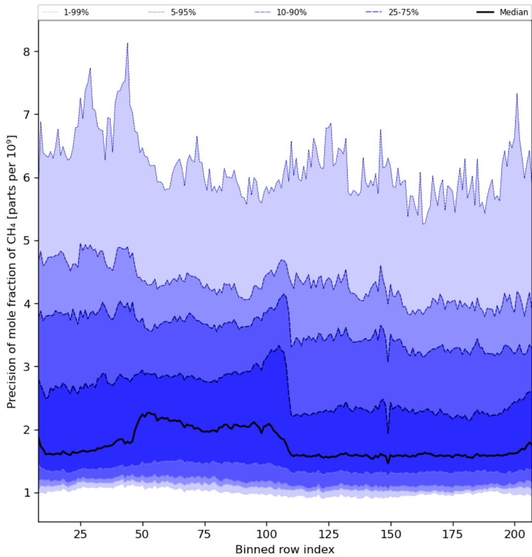
Figure 35: Along track statistics of “Precision of mole fraction of CH 4 ” for 2023-08-16 to 2023-08-18
