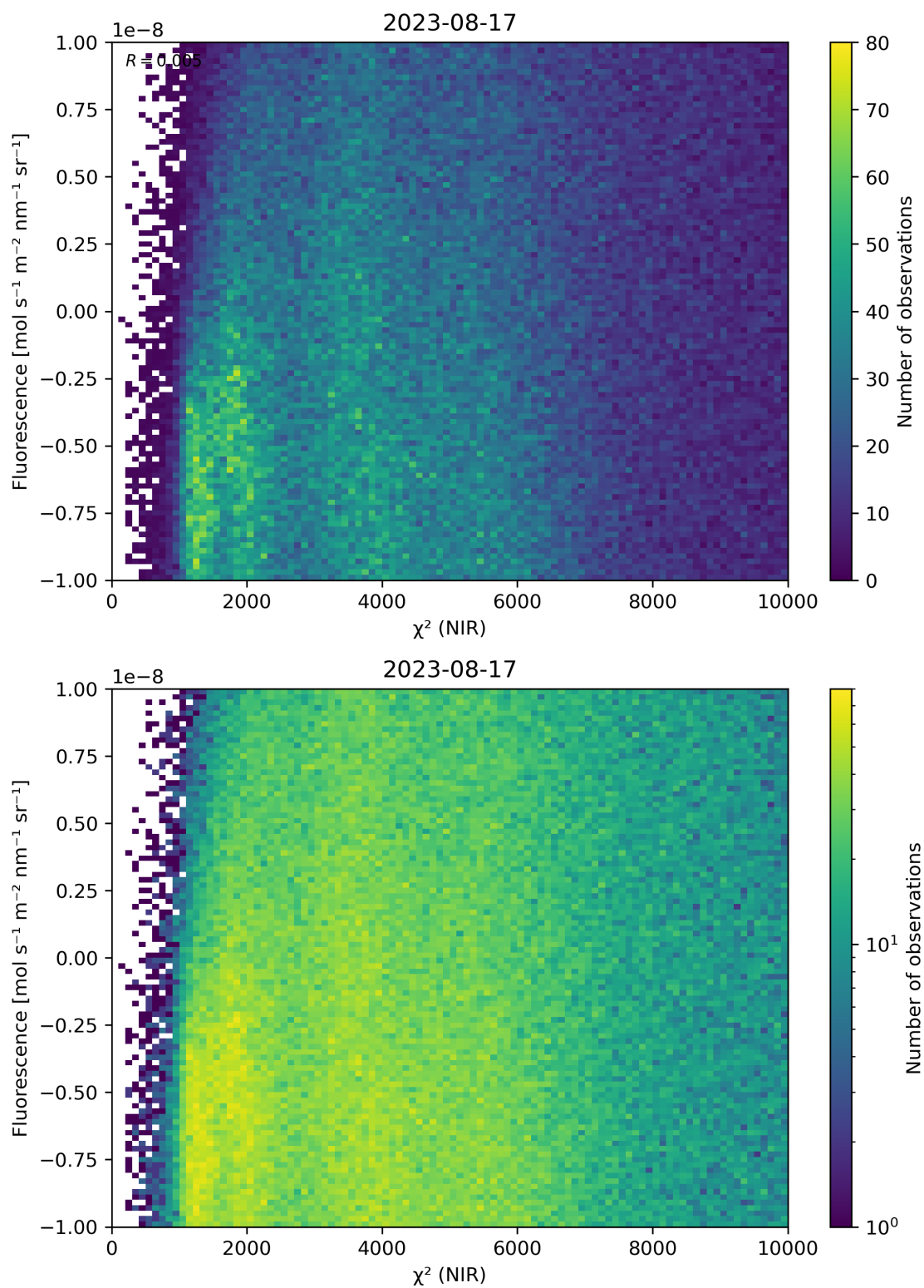
Figure 45: Scatter density plot of “ \chi^2 (NIR)” against “Fluorescence” for 2023-08-16 to 2023-08-18.
