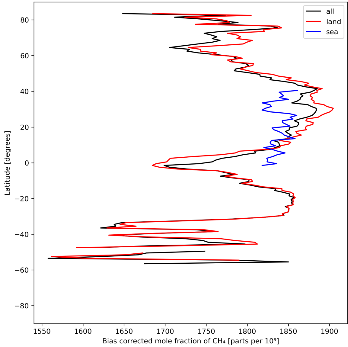
Figure 14: Zonal average of “Bias corrected mole fraction of CH 4 ” for 2023-08-16 to 2023-08-18.
