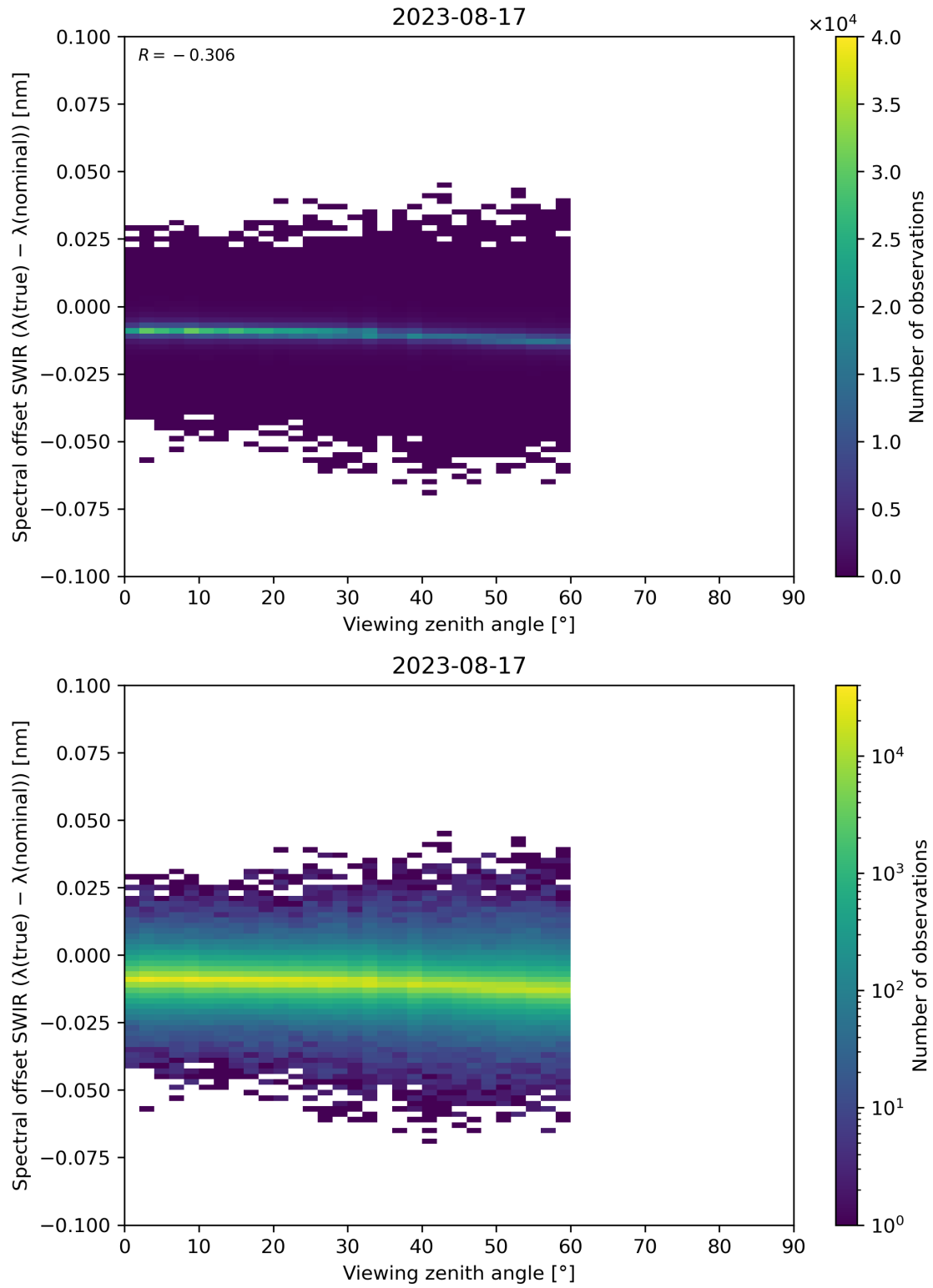
Figure 116: Scatter density plot of “Viewing zenith angle” against “Spectral offset SWIR ( \lambda(\text{true}) - \lambda(\text{nominal}) )” for 2023-08-16 to 2023-08-18.
