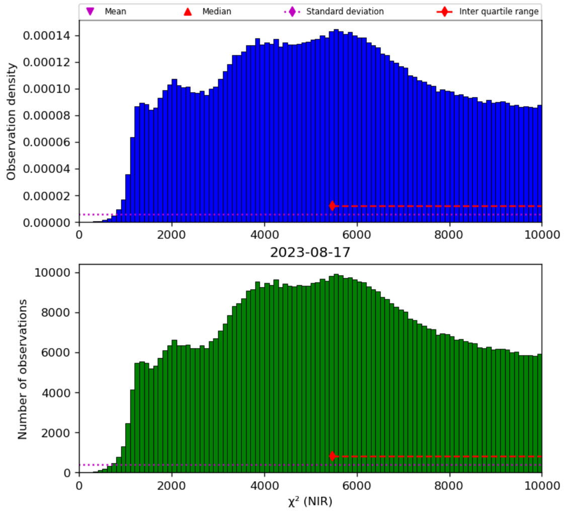
Figure 29: Histogram of “ \chi^2 (NIR)” for 2023-08-16 to 2023-08-18
