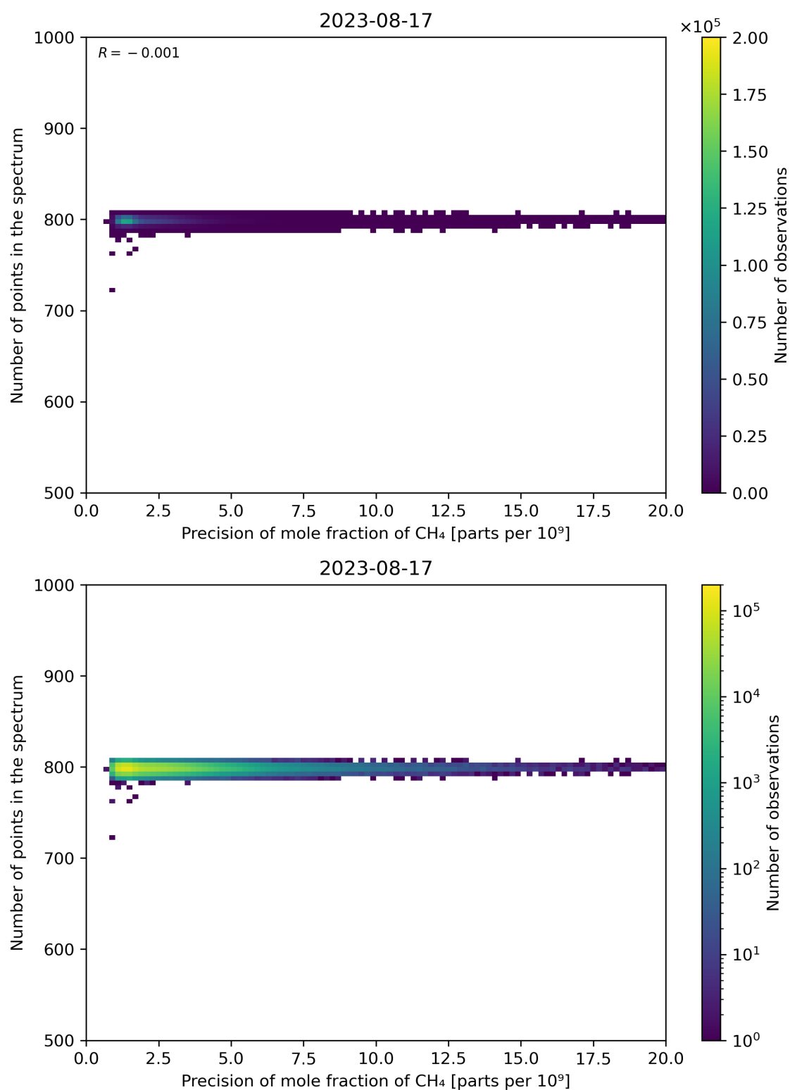
Figure 84: Scatter density plot of “Precision of mole fraction of CH 4 ” against “Number of points in the spectrum” for 2023-08-16 to 2023-08-18.
