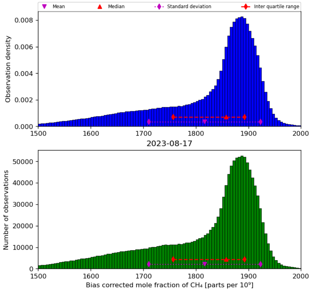
Figure 25: Histogram of “Bias corrected mole fraction of CH 4 ” for 2023-08-16 to 2023-08-18
