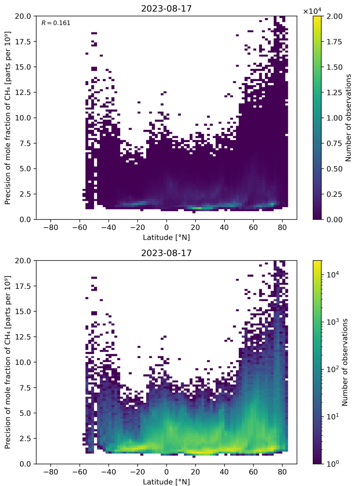
Figure 59: Scatter density plot of “Latitude” against “Precision of mole fraction of CH 4 ” for 2023-08-16 to 2023-08-18.
