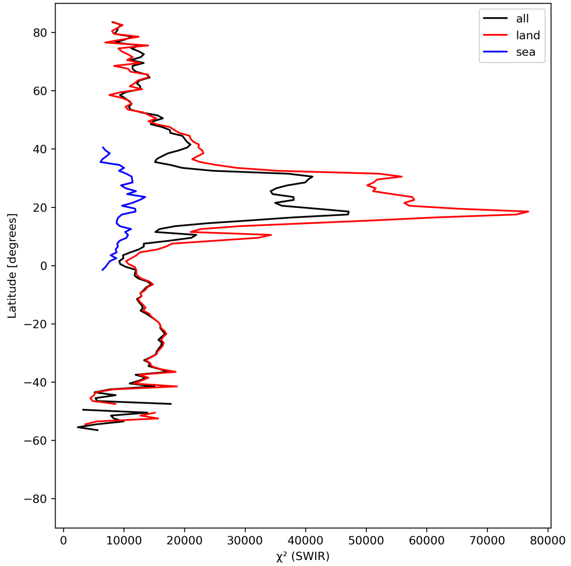
Figure 17: Zonal average of “ \chi^2 (SWIR)” for 2023-08-16 to 2023-08-18.
