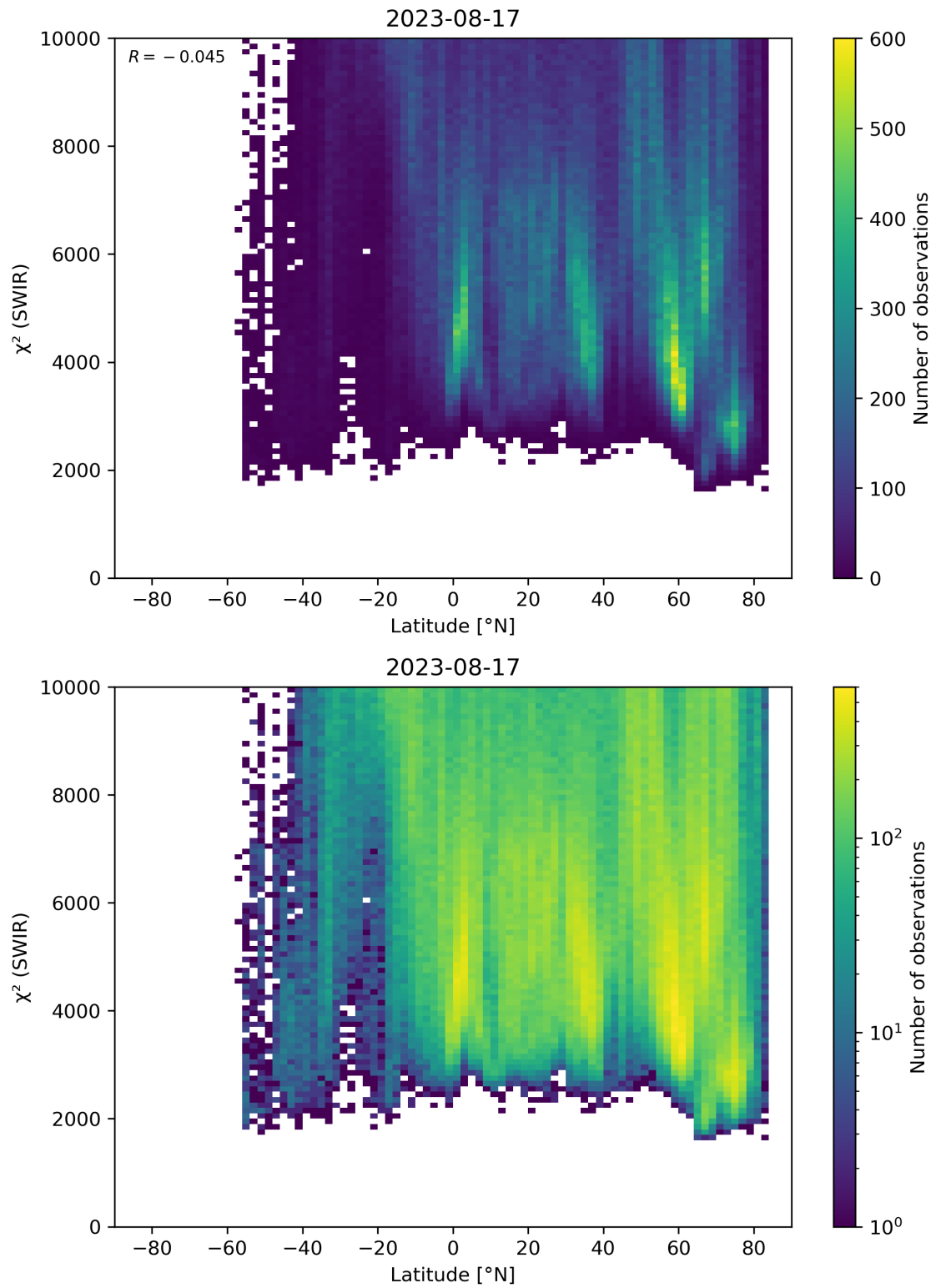
Figure 54: Scatter density plot of “Latitude” against “ \chi^2 (SWIR)” for 2023-08-16 to 2023-08-18.
