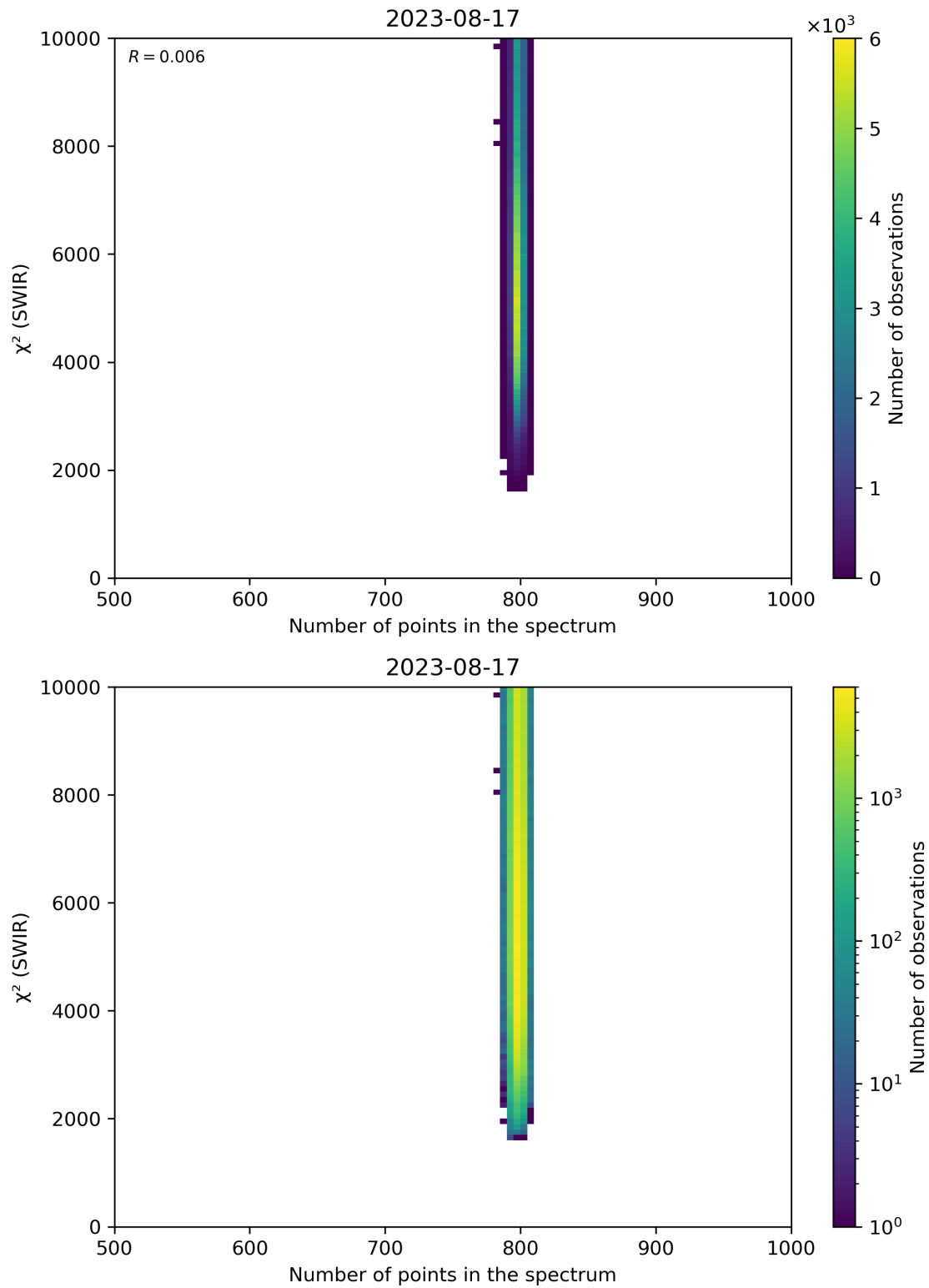
Figure 89: Scatter density plot of “Number of points in the spectrum” against “ \chi^2 (SWIR)” for 2023-08-16 to 2023-08-18.
