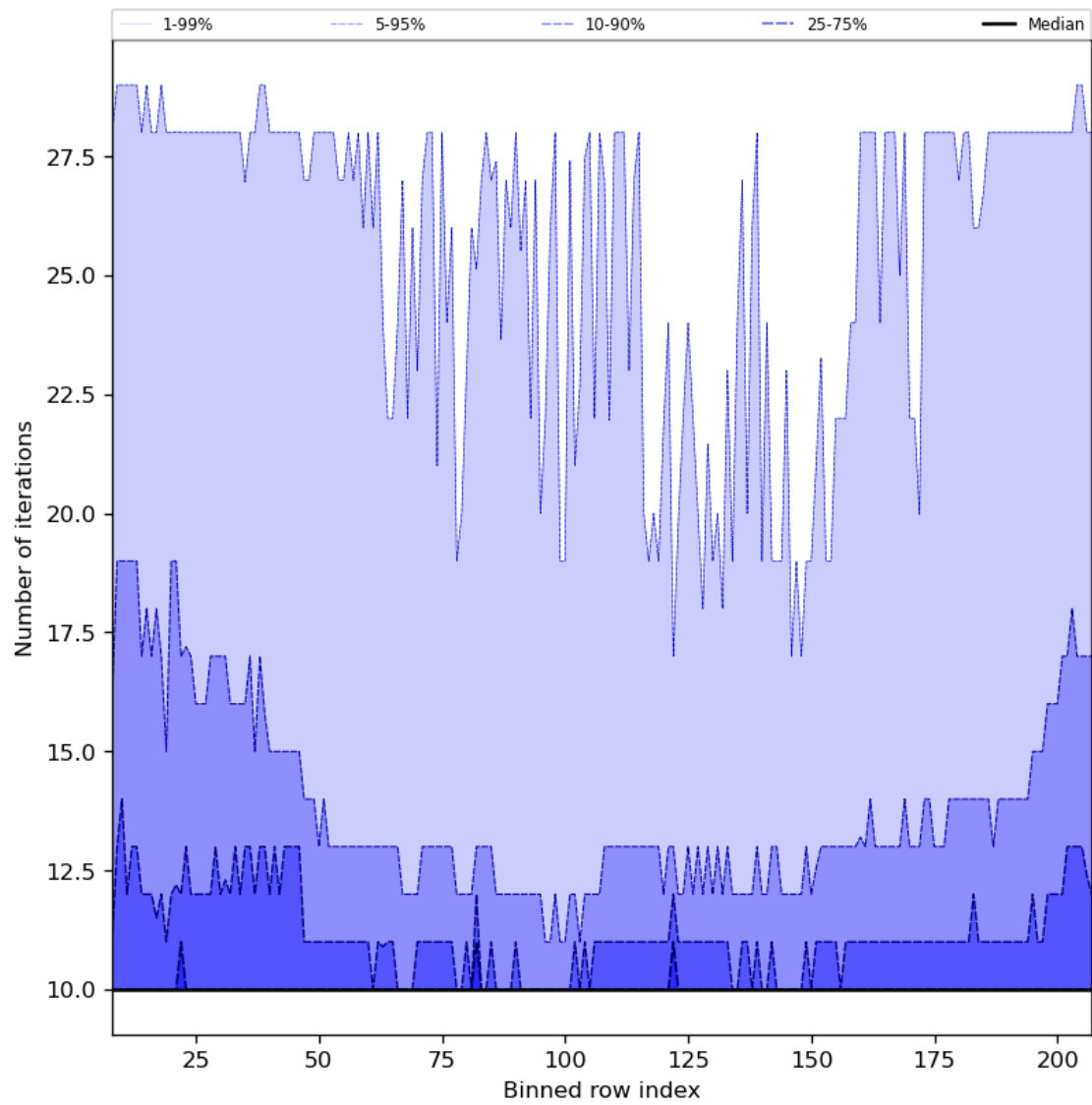
Figure 42: Along track statistics of “Number of iterations” for 2023-08-16 to 2023-08-18
