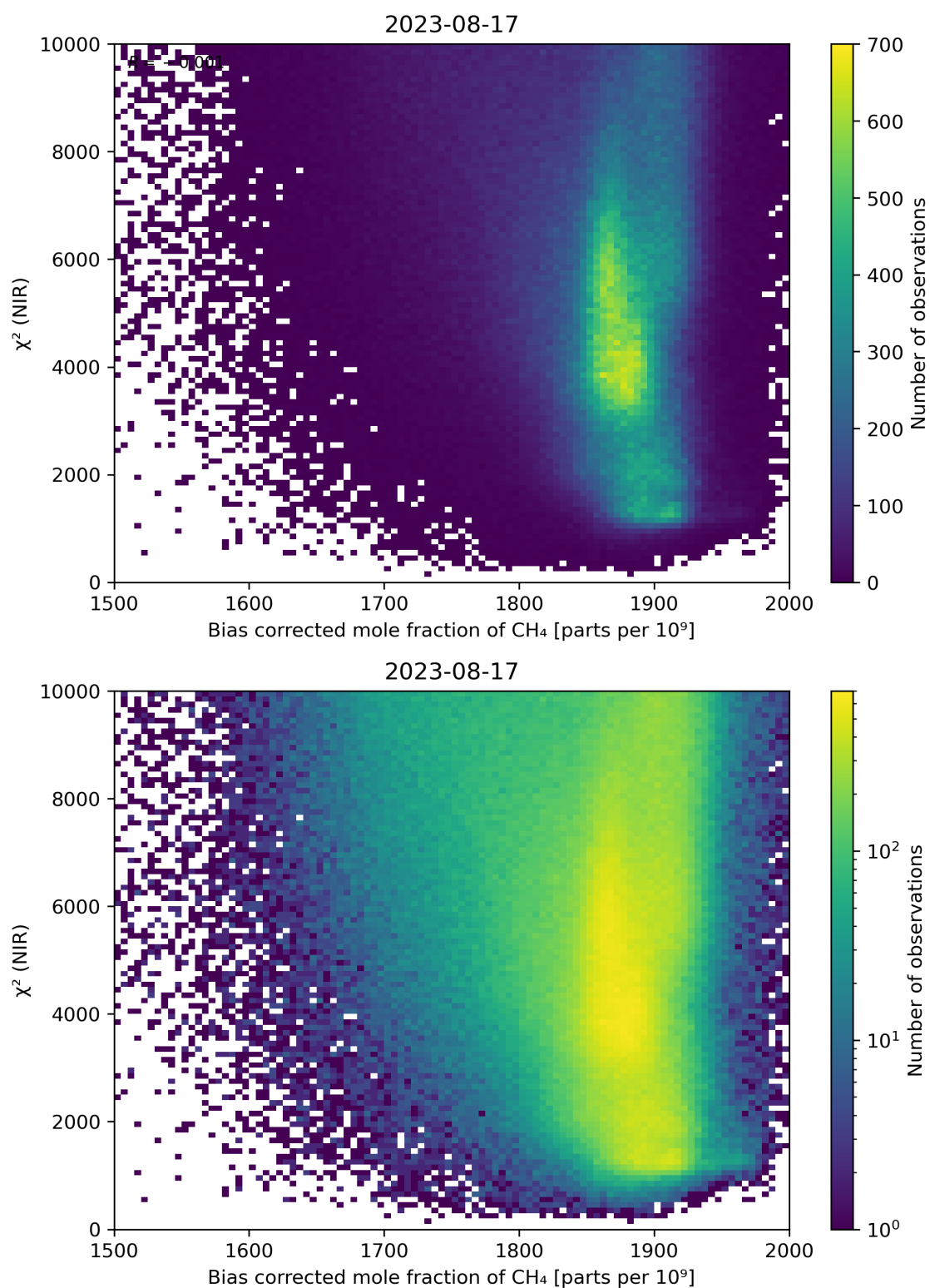
Figure 63: Scatter density plot of “Bias corrected mole fraction of CH 4 ” against “ \chi^2 (NIR)” for 2023-08-16 to 2023-08-18.
