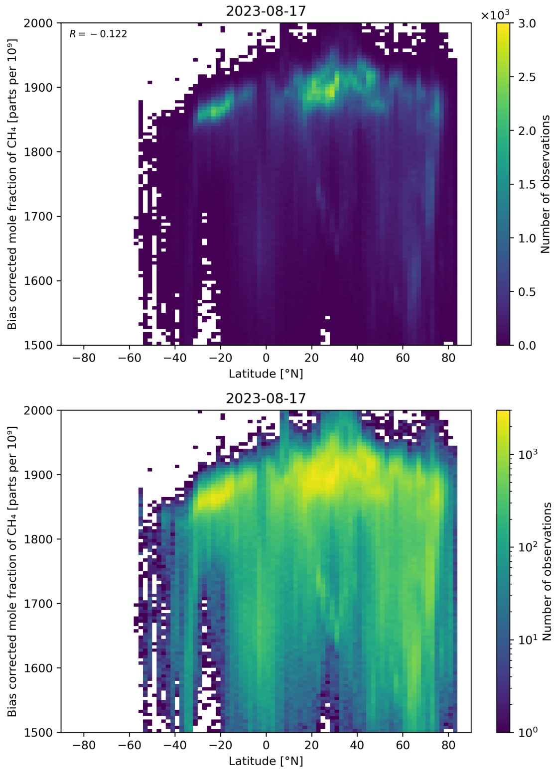
Figure 58: Scatter density plot of “Latitude” against “Bias corrected mole fraction of \text{CH}_4 ” for 2023-08-16 to 2023-08-18.
