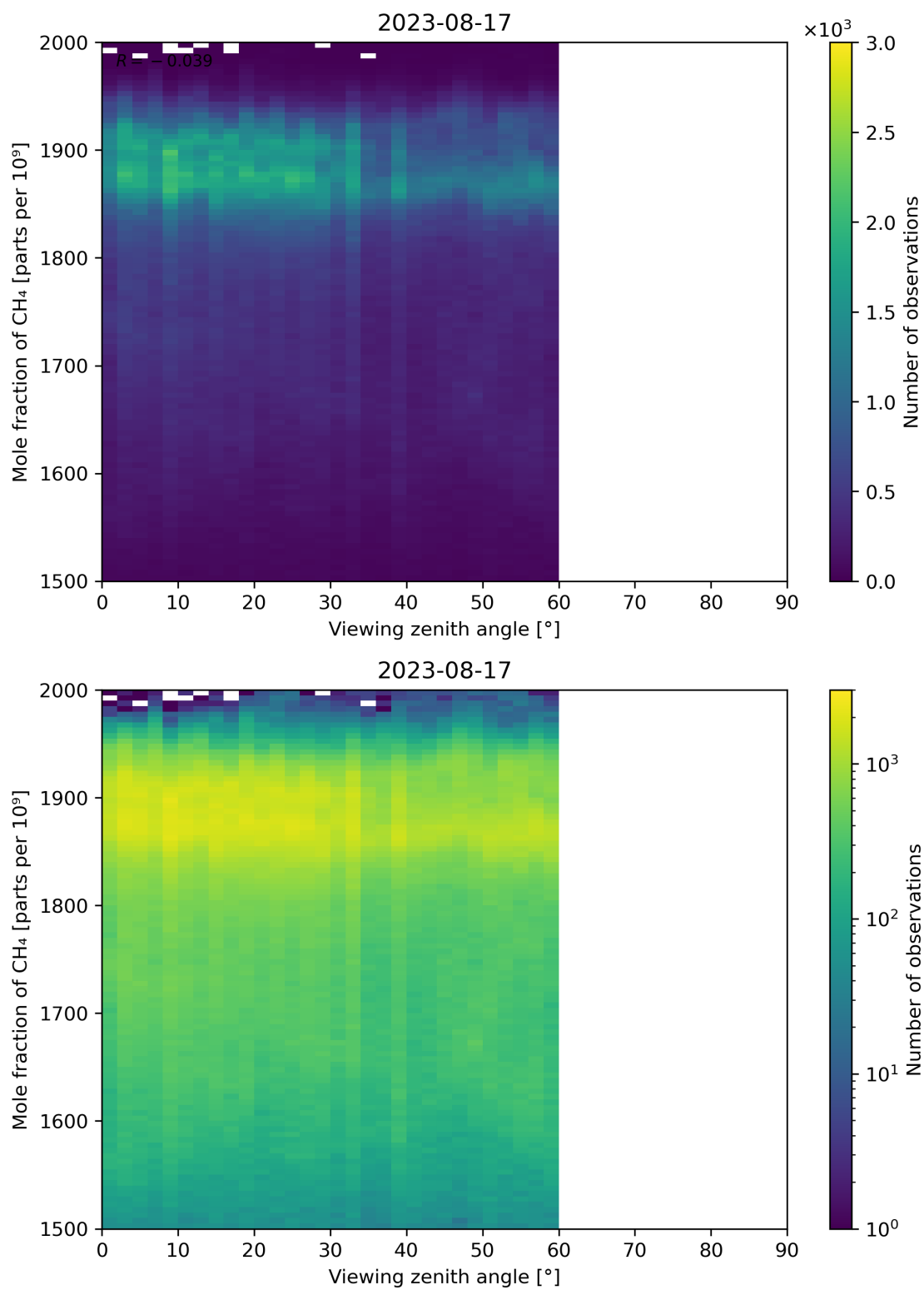
Figure 110: Scatter density plot of “Viewing zenith angle” against “Mole fraction of CH 4 ” for 2023-08-16 to 2023-08-18.
