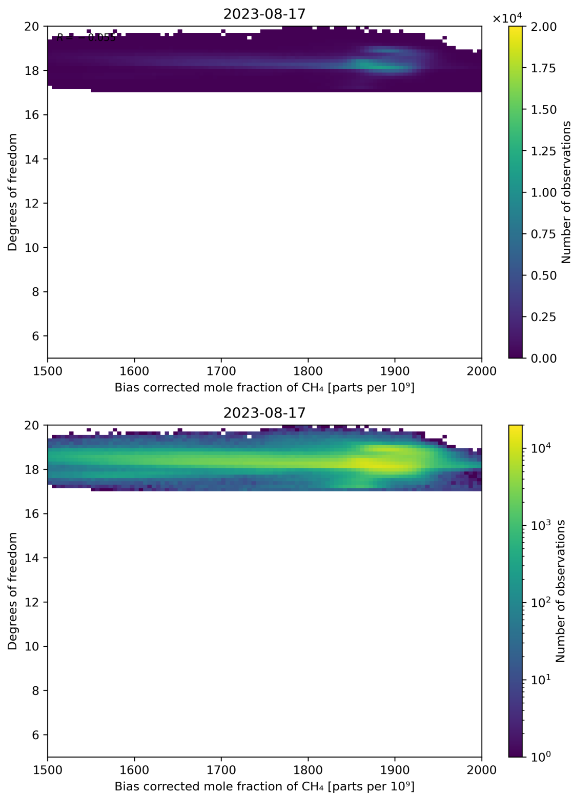
Figure 65: Scatter density plot of “Bias corrected mole fraction of CH 4 ” against “Degrees of freedom” for 2023-08-16 to 2023-08-18.
