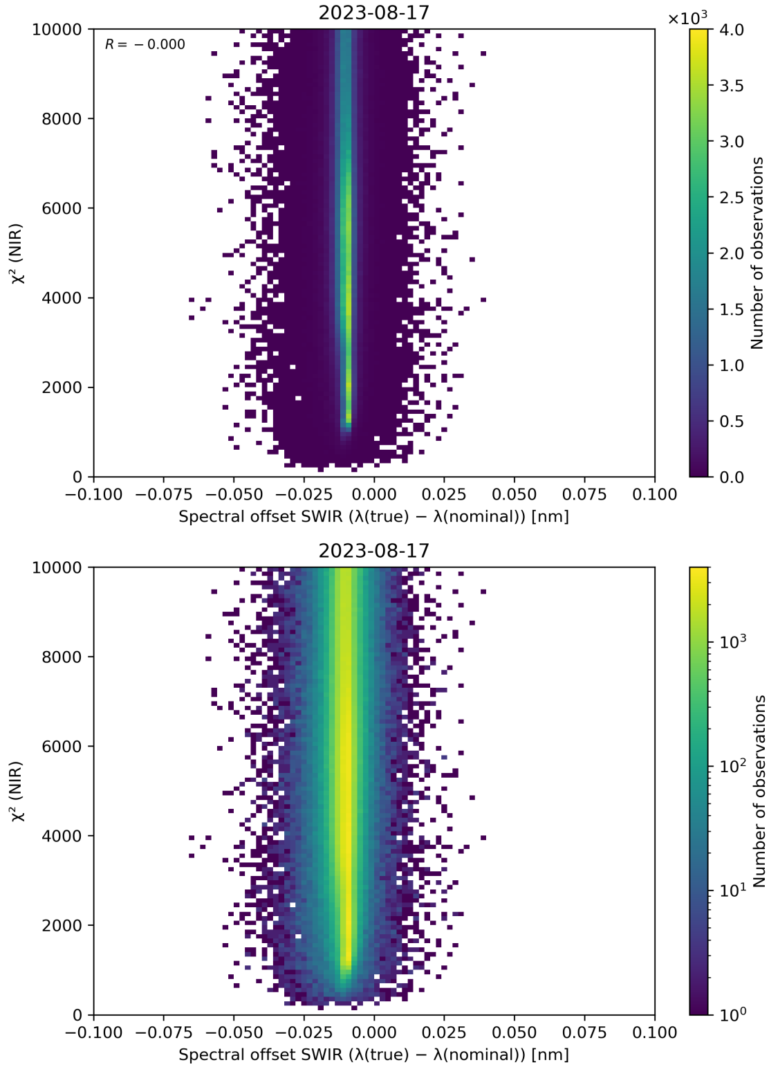
Figure 117: Scatter density plot of “Spectral offset SWIR ( \lambda(\text{true}) - \lambda(\text{nominal}) )” against “ \chi^2 (NIR)” for 2023-08-16 to 2023-08-18.
