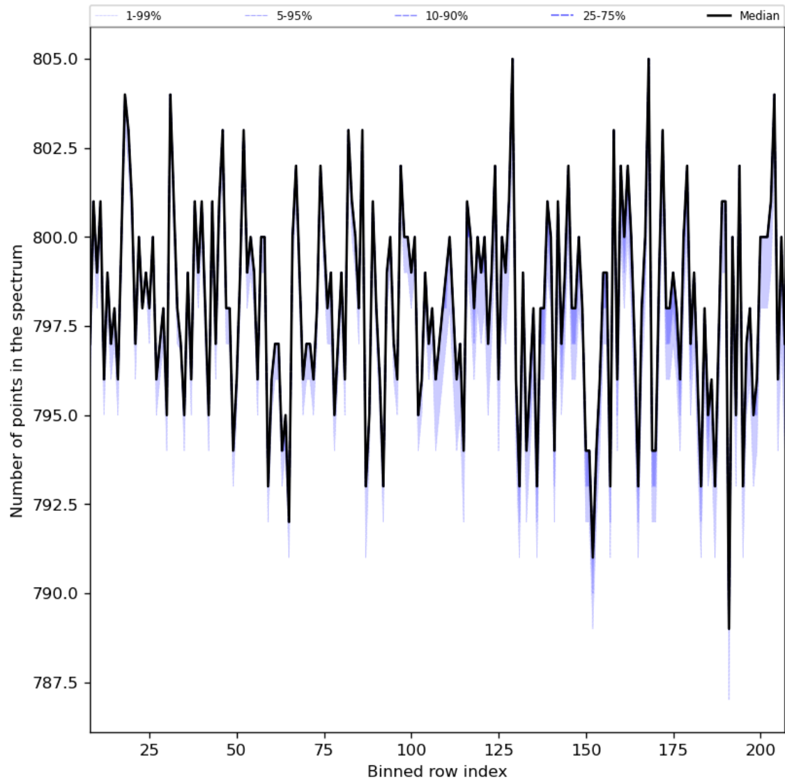
Figure 37: Along track statistics of “Number of points in the spectrum” for 2023-08-16 to 2023-08-18
