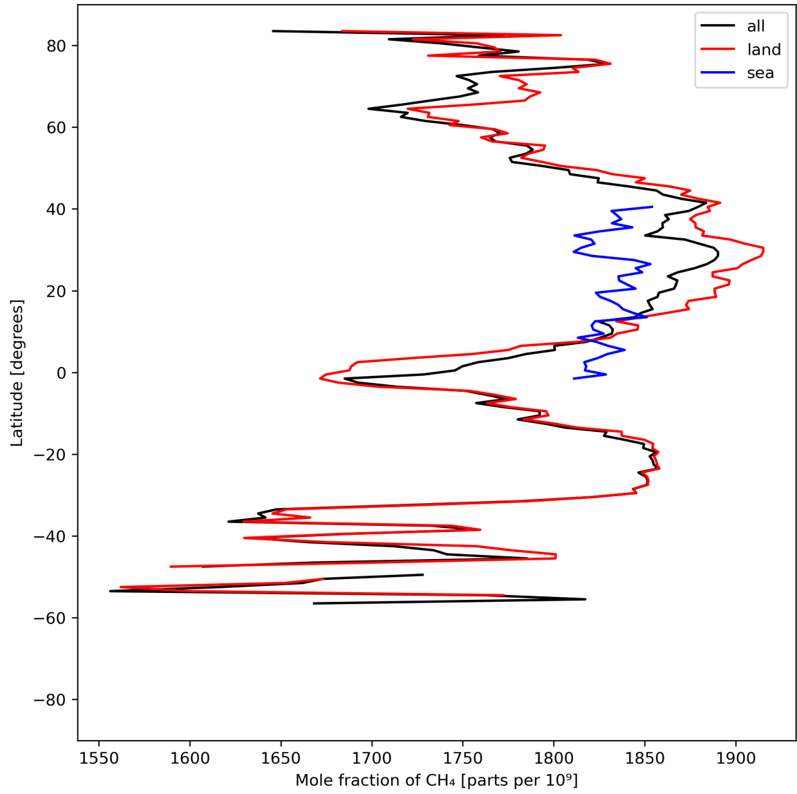
Figure 12: Zonal average of “Mole fraction of \text{CH}_4 ” for 2023-08-16 to 2023-08-18.
