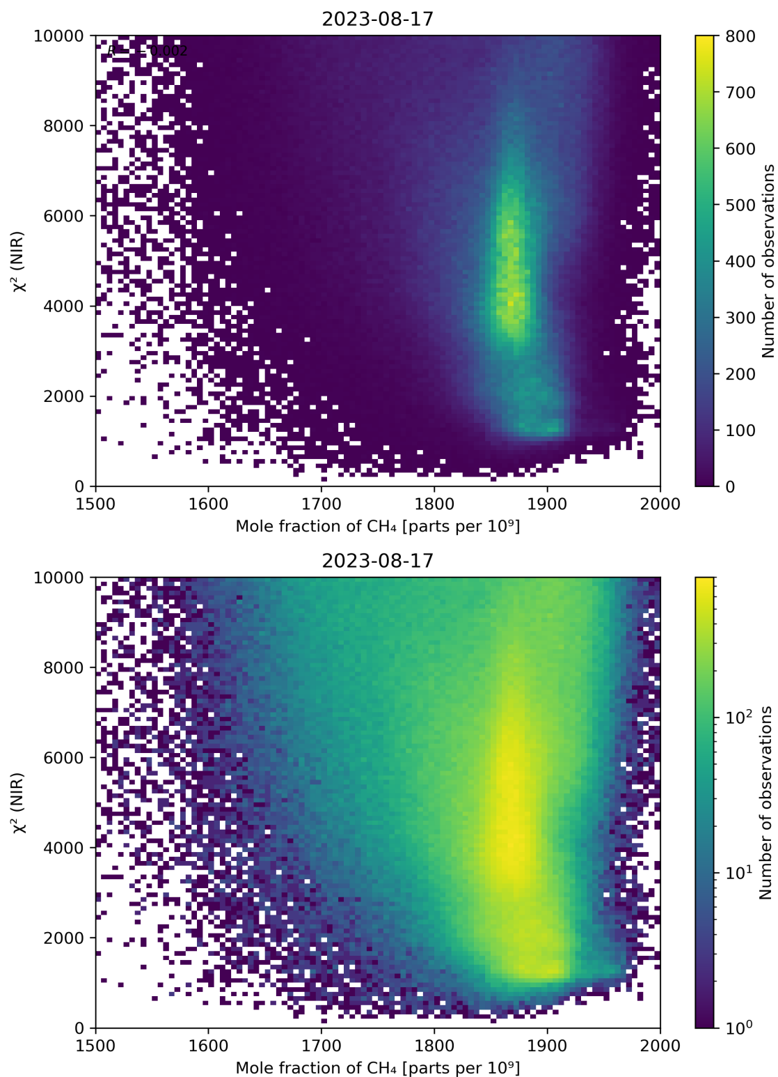
Figure 70: Scatter density plot of “Mole fraction of CH 4 ” against “ \chi^2 (NIR)” for 2023-08-16 to 2023-08-18.
