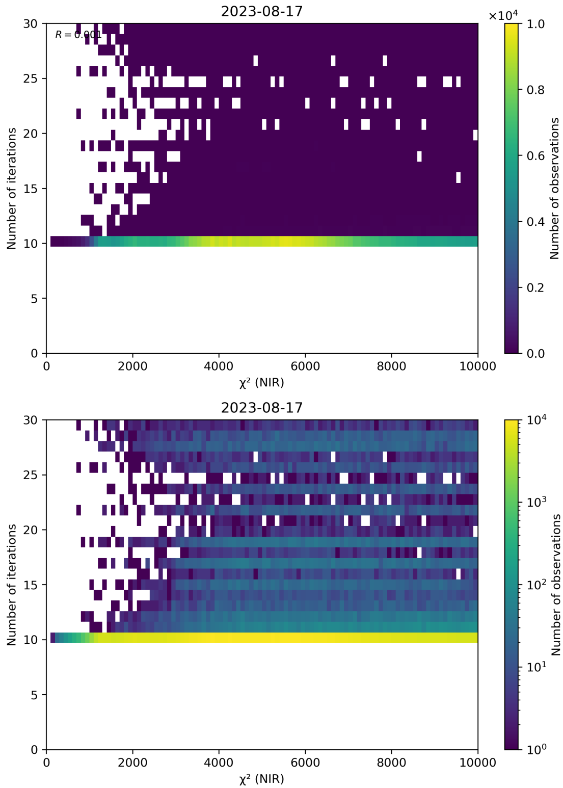
Figure 46: Scatter density plot of “ \chi^2 (NIR)” against “Number of iterations” for 2023-08-16 to 2023-08-18.
