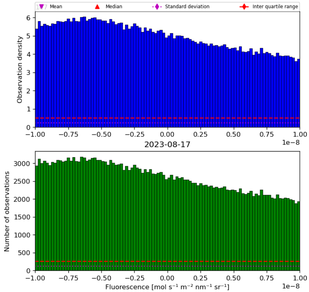
Figure 32: Histogram of “Fluorescence” for 2023-08-16 to 2023-08-18
