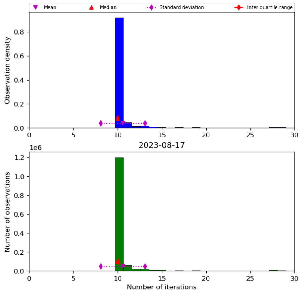
Figure 31: Histogram of “Number of iterations” for 2023-08-16 to 2023-08-18
