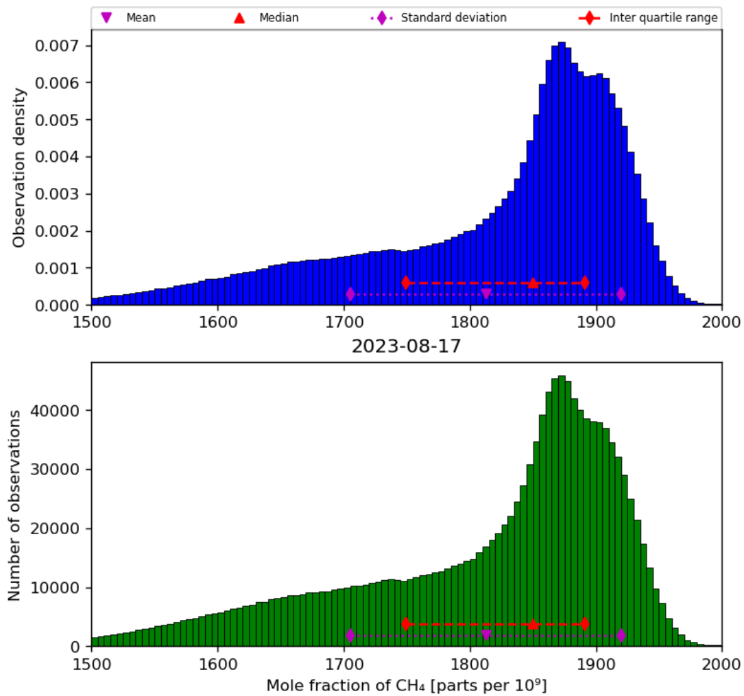
Figure 23: Histogram of “Mole fraction of CH 4 ” for 2023-08-16 to 2023-08-18
