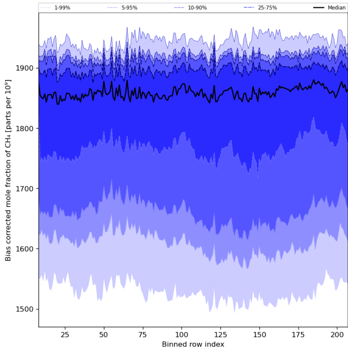
Figure 36: Along track statistics of “Bias corrected mole fraction of CH 4 ” for 2023-08-17 to 2023-08-19
