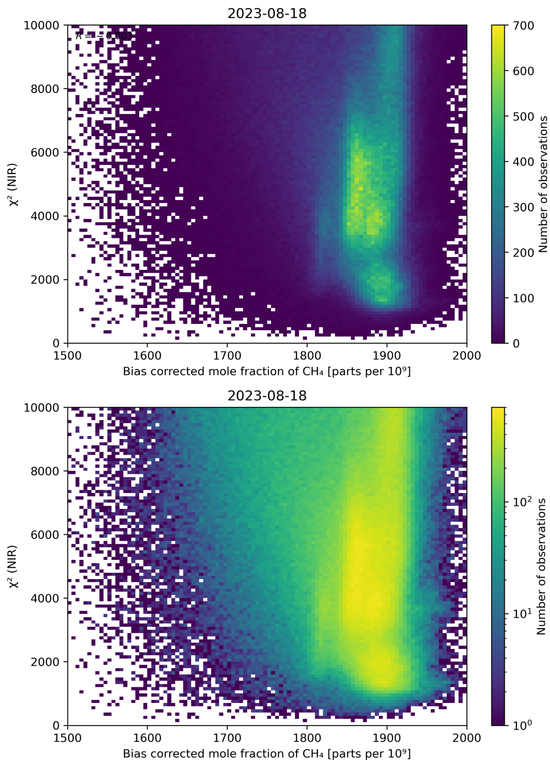
Figure 63: Scatter density plot of “Bias corrected mole fraction of CH 4 ” against “ \chi^2 (NIR)” for 2023-08-17 to 2023-08-19.
