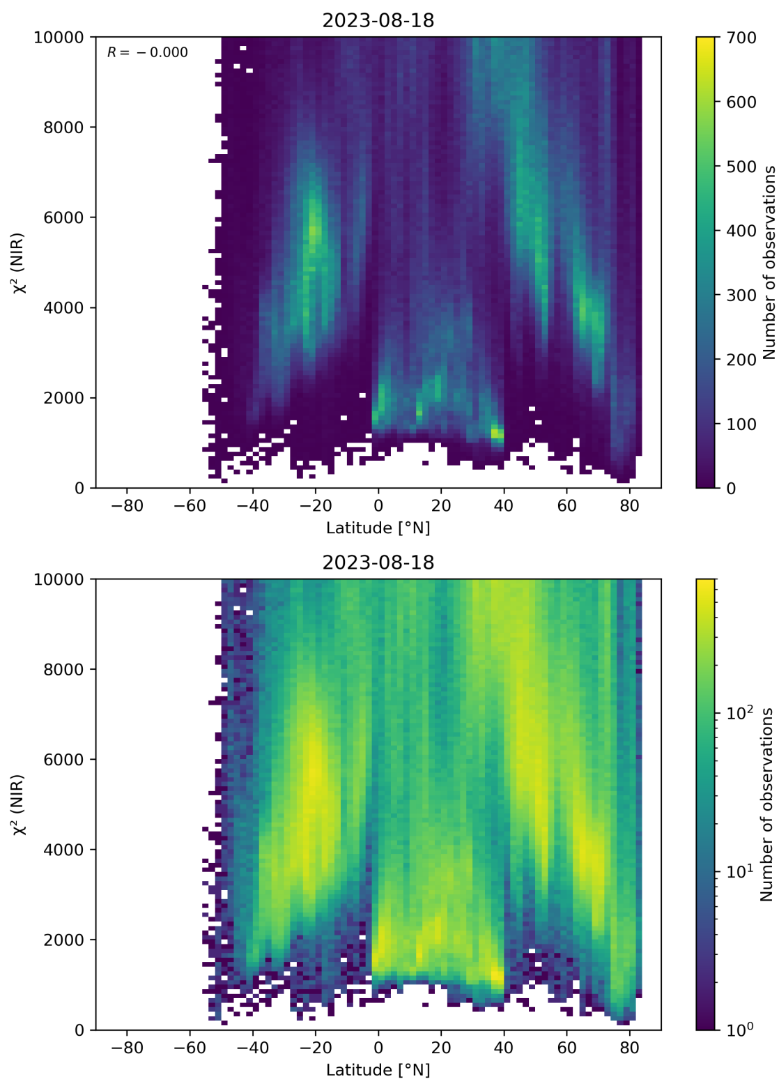
Figure 53: Scatter density plot of “Latitude” against “ \chi^2 (NIR)” for 2023-08-17 to 2023-08-19.
