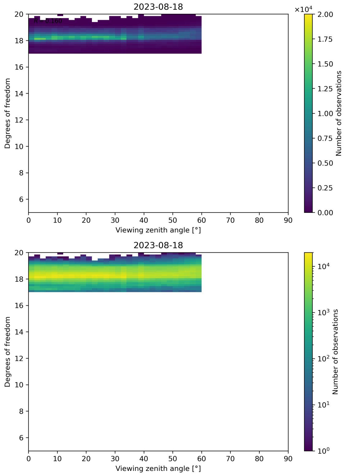
Figure 107: Scatter density plot of “Viewing zenith angle” against “Degrees of freedom” for 2023-08-17 to 2023-08-19.
