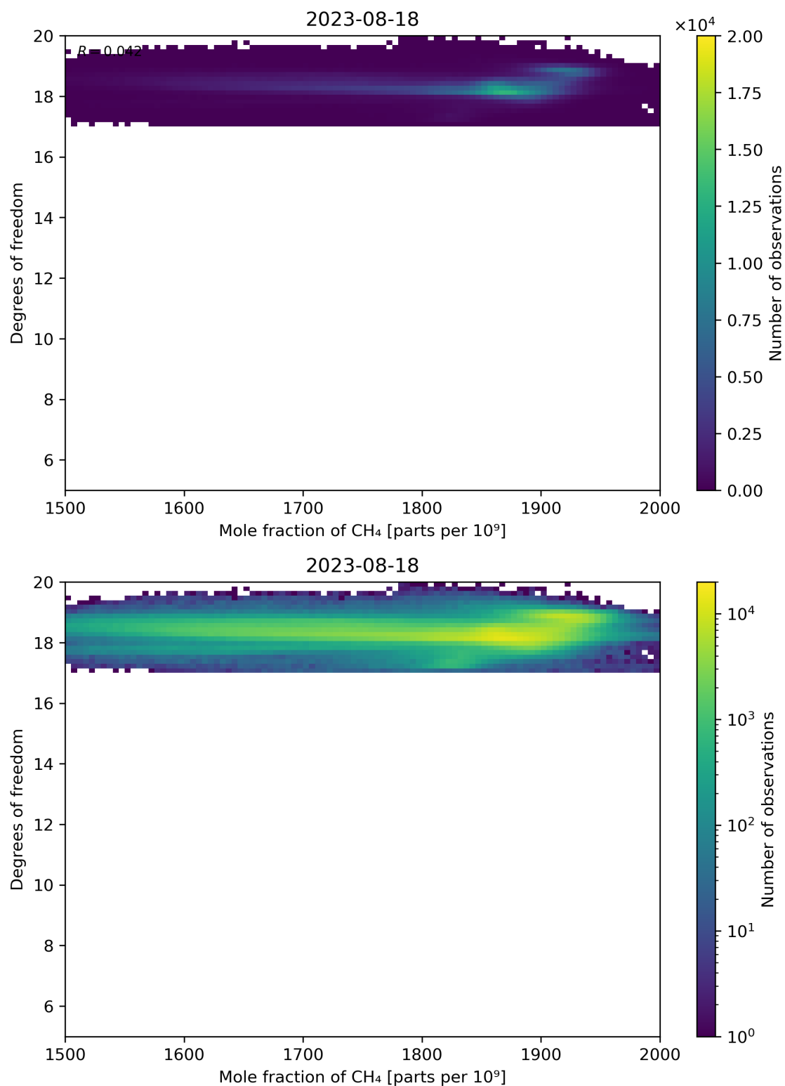
Figure 72: Scatter density plot of “Mole fraction of CH 4 ” against “Degrees of freedom” for 2023-08-17 to 2023-08-19.
