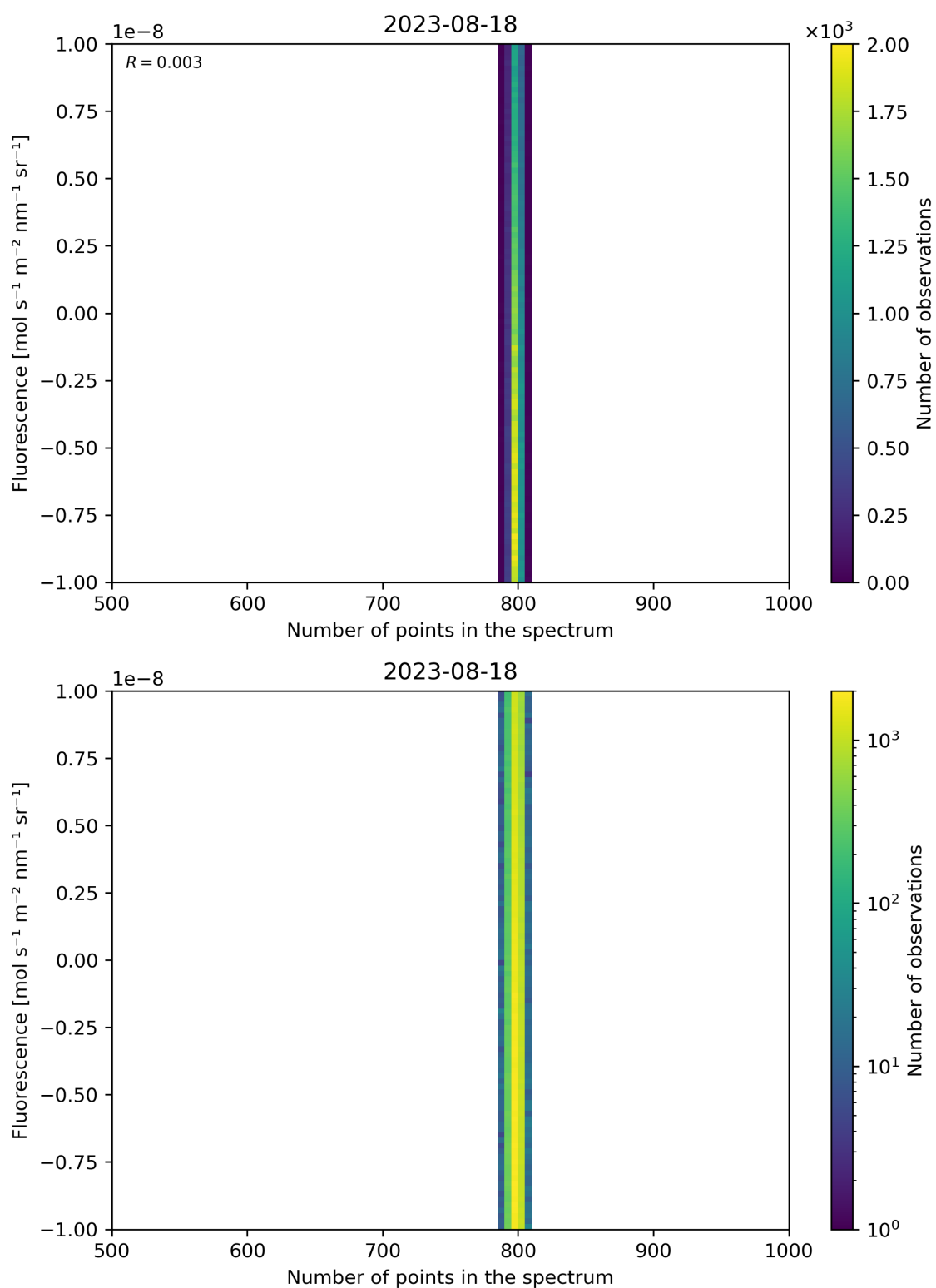
Figure 91: Scatter density plot of “Number of points in the spectrum” against “Fluorescence” for 2023-08-17 to 2023-08-19.
