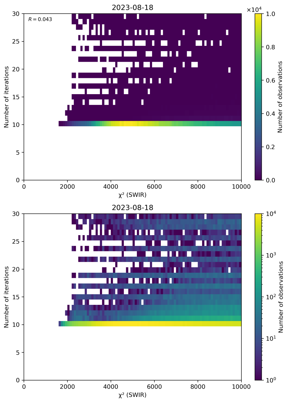
Figure 50: Scatter density plot of “ \chi^2 (SWIR)” against “Number of iterations” for 2023-08-17 to 2023-08-19.
