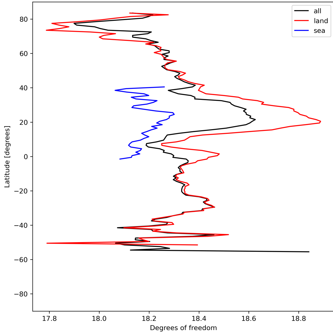
Figure 19: Zonal average of “Degrees of freedom” for 2023-08-17 to 2023-08-19.
