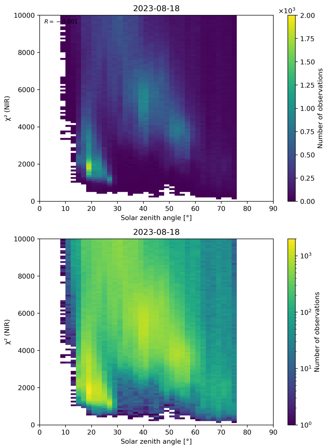
Figure 94: Scatter density plot of “Solar zenith angle” against “ \chi^2 (NIR)” for 2023-08-17 to 2023-08-19.
