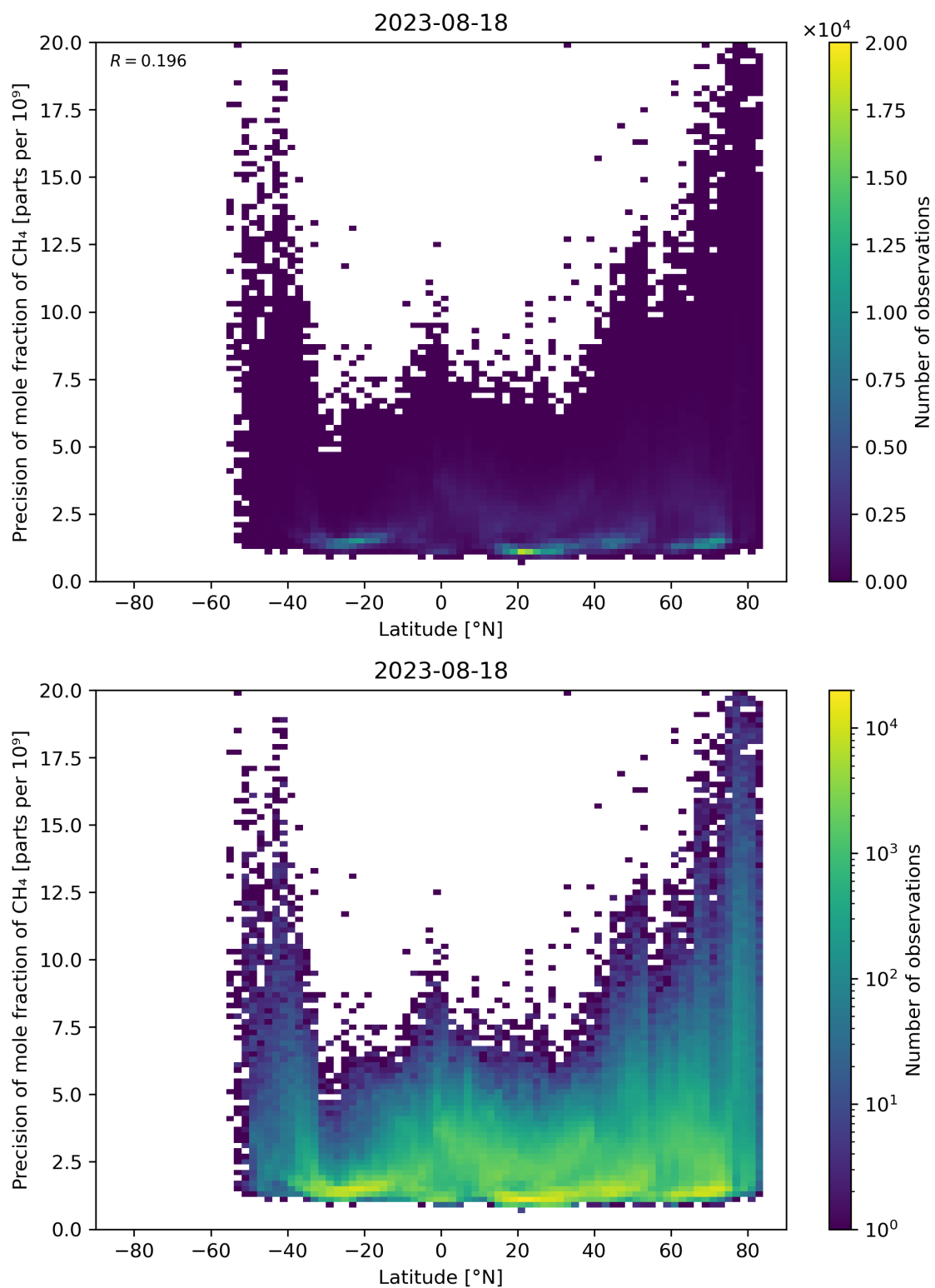
Figure 59: Scatter density plot of “Latitude” against “Precision of mole fraction of \text{CH}_4 ” for 2023-08-17 to 2023-08-19.
