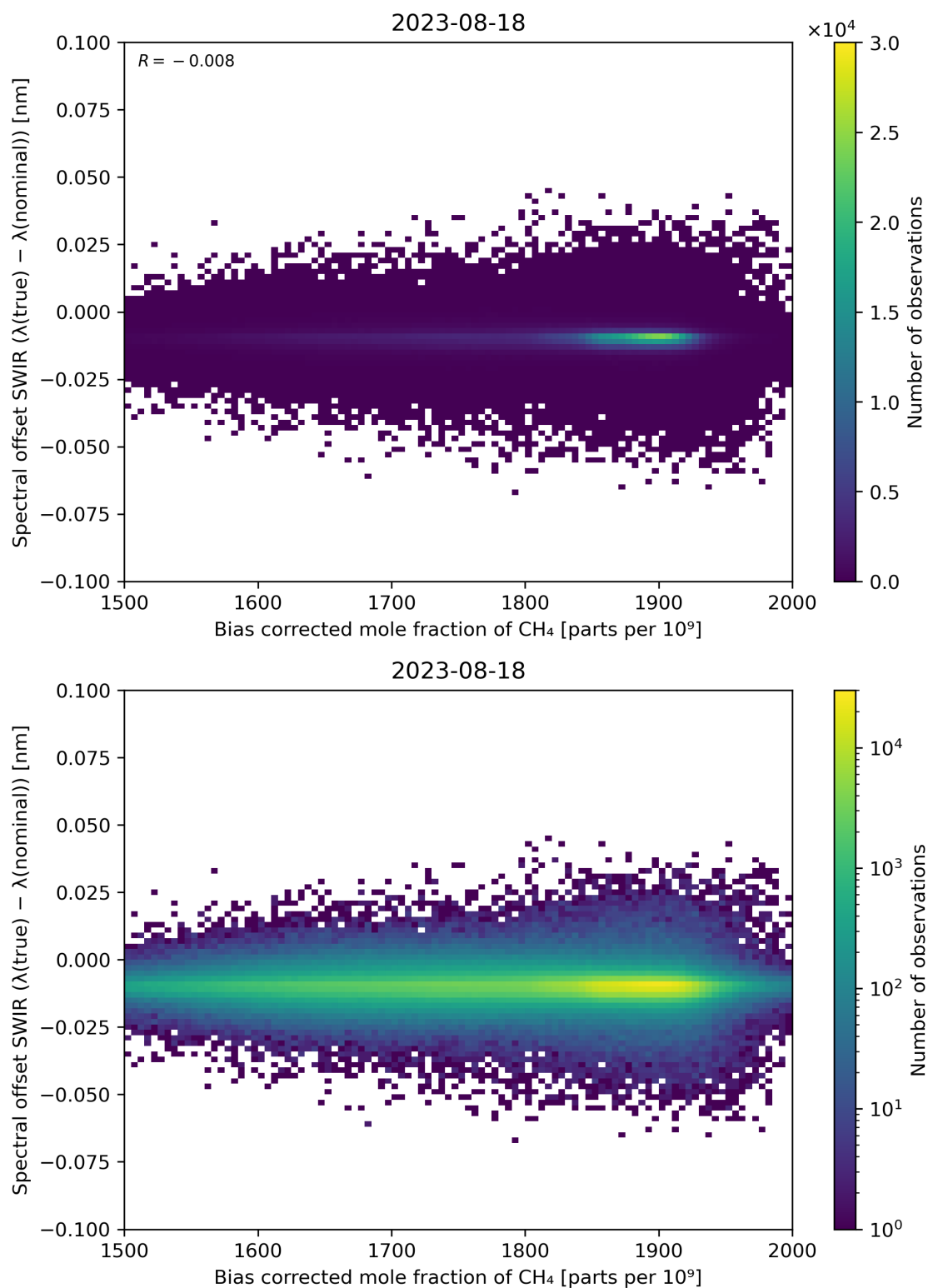
Figure 69: Scatter density plot of “Bias corrected mole fraction of \text{CH}_4 ” against “Spectral offset SWIR ( \lambda(\text{true}) - \lambda(\text{nominal}) )” for 2023-08-17 to 2023-08-19.
