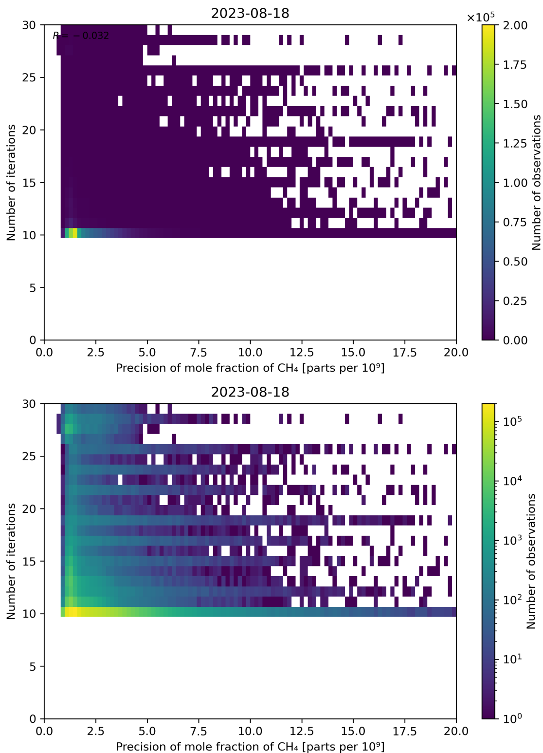
Figure 83: Scatter density plot of “Precision of mole fraction of CH 4 ” against “Number of iterations” for 2023-08-17 to 2023-08-19.
