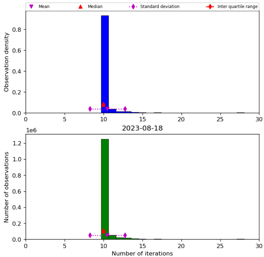
Figure 31: Histogram of “Number of iterations” for 2023-08-17 to 2023-08-19
