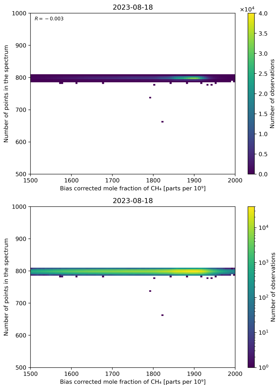
Figure 68: Scatter density plot of “Bias corrected mole fraction of CH 4 ” against “Number of points in the spectrum” for 2023-08-17 to 2023-08-19.
