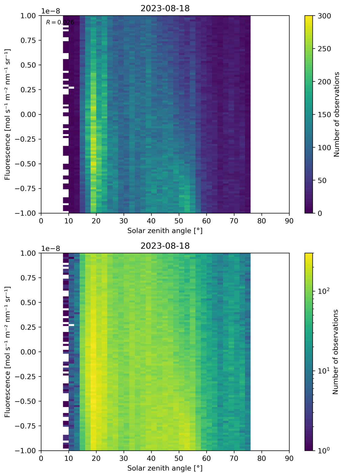
Figure 97: Scatter density plot of “Solar zenith angle” against “Fluorescence” for 2023-08-17 to 2023-08-19.
