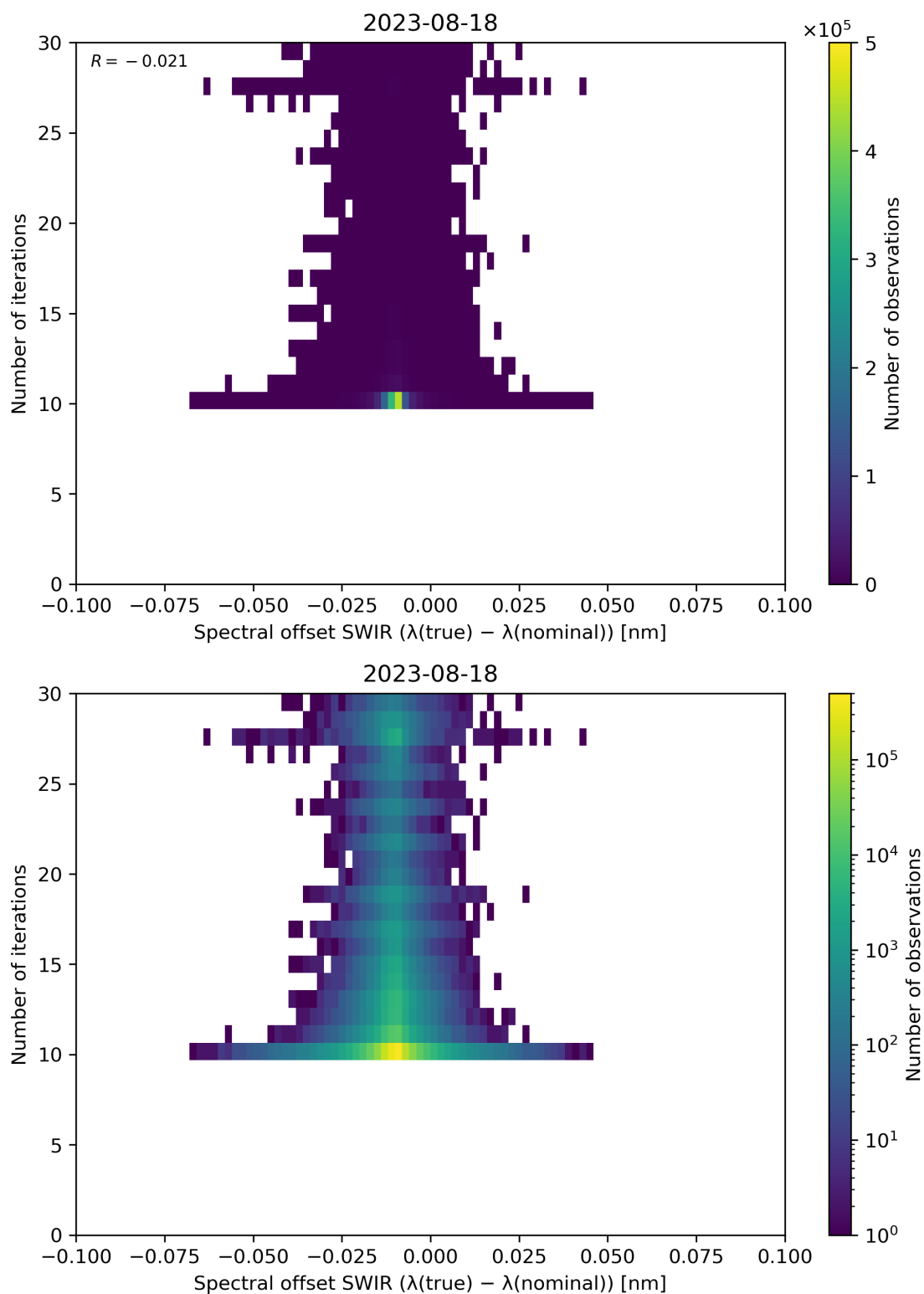
Figure 121: Scatter density plot of “Spectral offset SWIR ( \lambda(\text{true}) - \lambda(\text{nominal}) )” against “Number of iterations” for 2023-08-17 to 2023-08-19.
