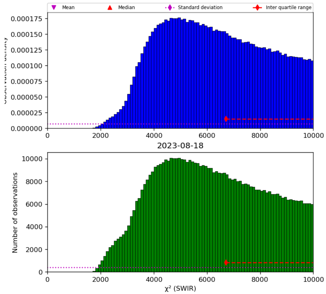
Figure 28: Histogram of “ \chi^2 (SWIR)” for 2023-08-17 to 2023-08-19
