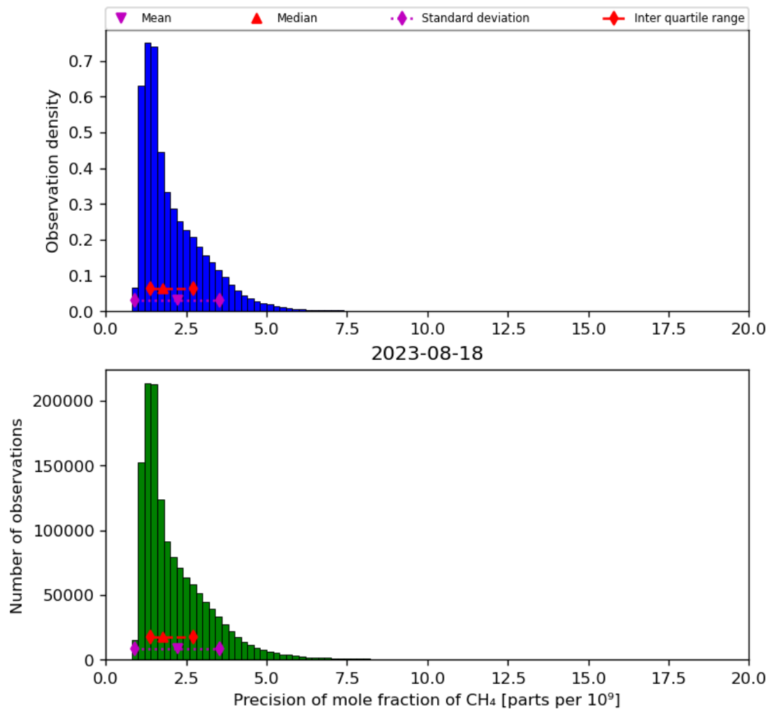
Figure 24: Histogram of “Precision of mole fraction of CH 4 ” for 2023-08-17 to 2023-08-19
