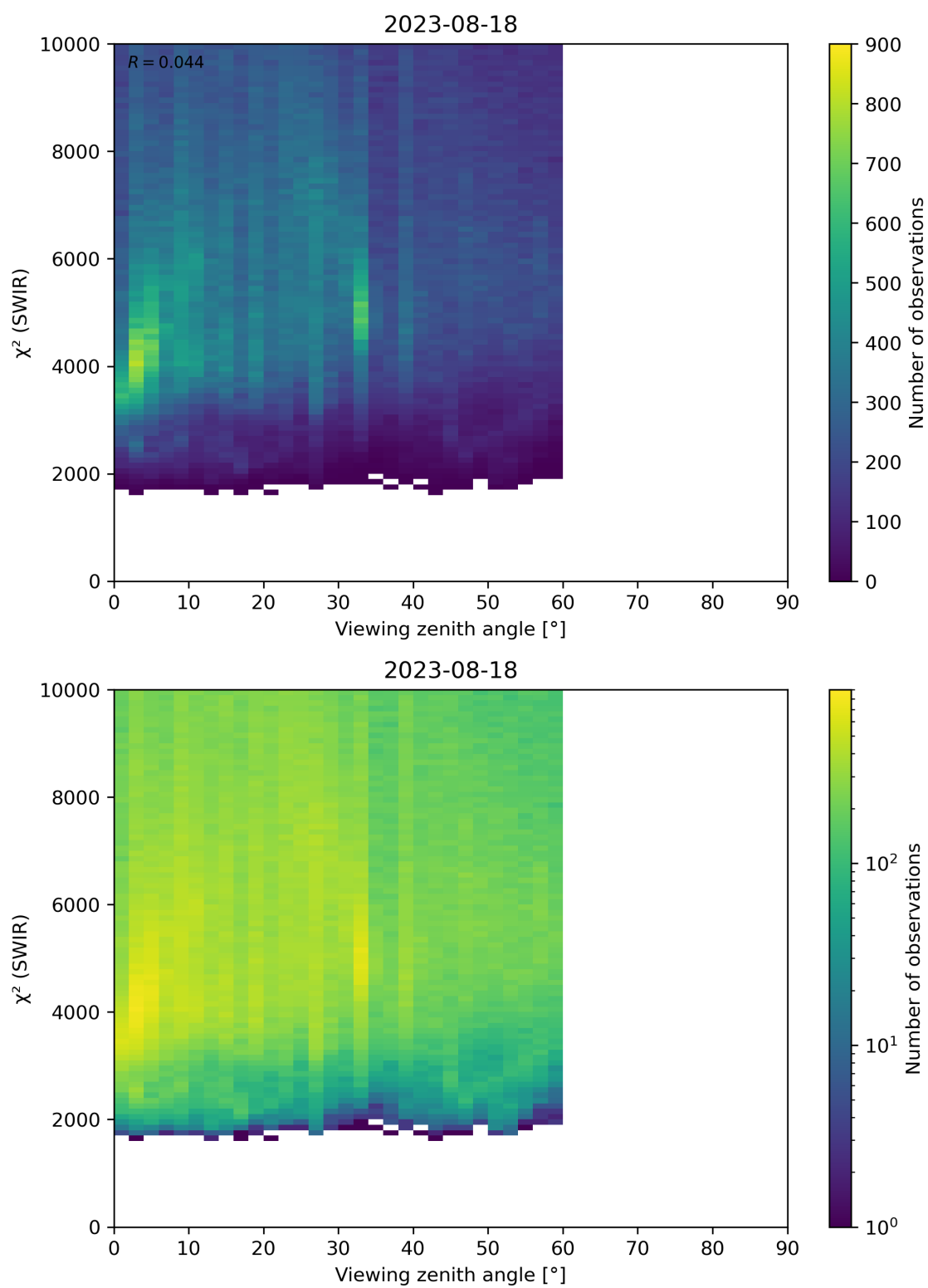
Figure 106: Scatter density plot of “Viewing zenith angle” against “ \chi^2 (SWIR)” for 2023-08-17 to 2023-08-19.
