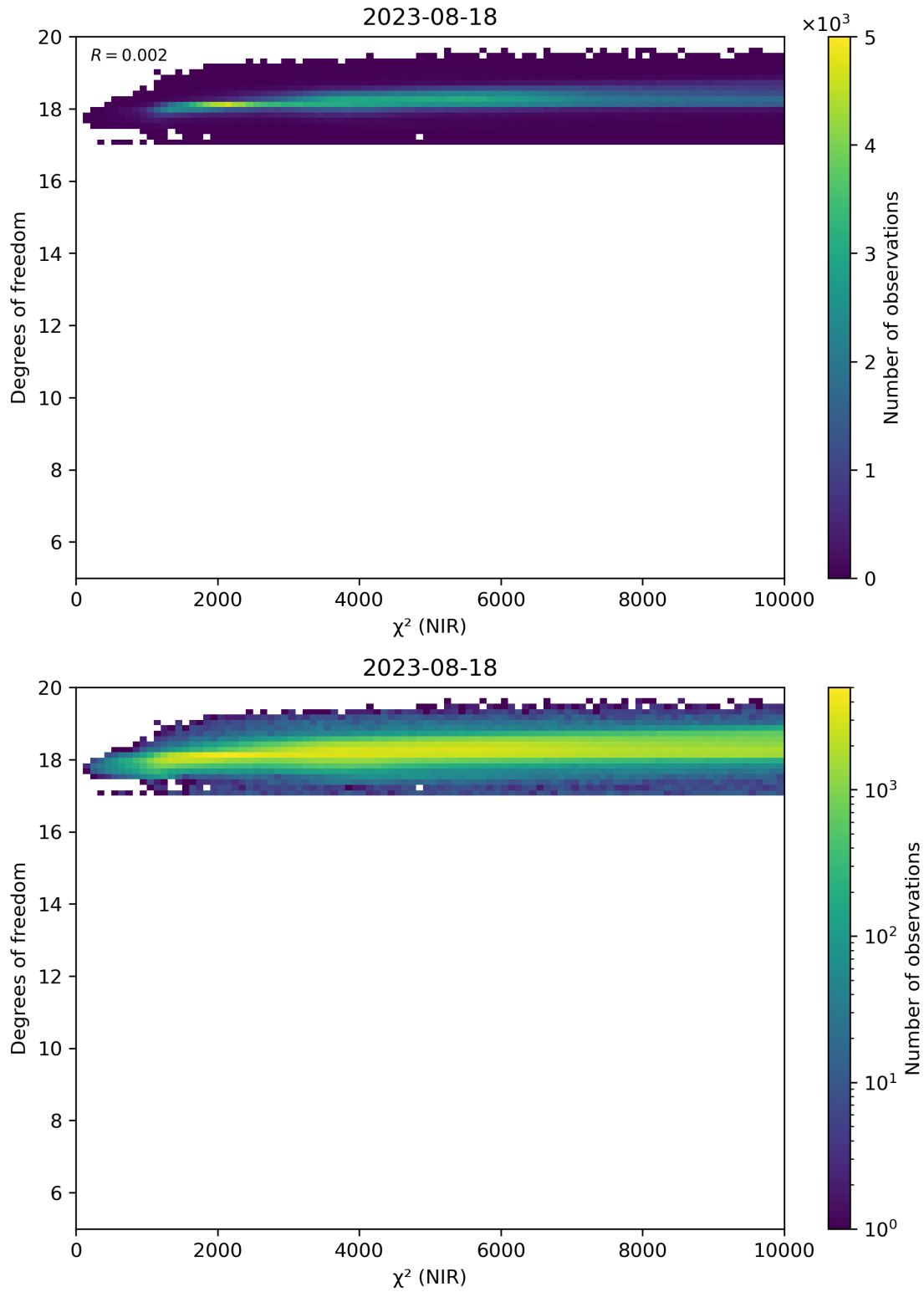
Figure 44: Scatter density plot of “ \chi^2 (NIR)” against “Degrees of freedom” for 2023-08-17 to 2023-08-19.
