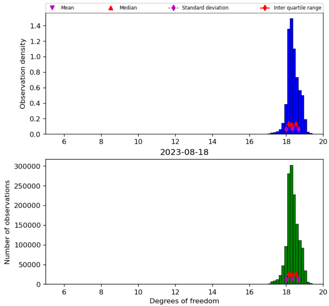
Figure 30: Histogram of “Degrees of freedom” for 2023-08-17 to 2023-08-19
