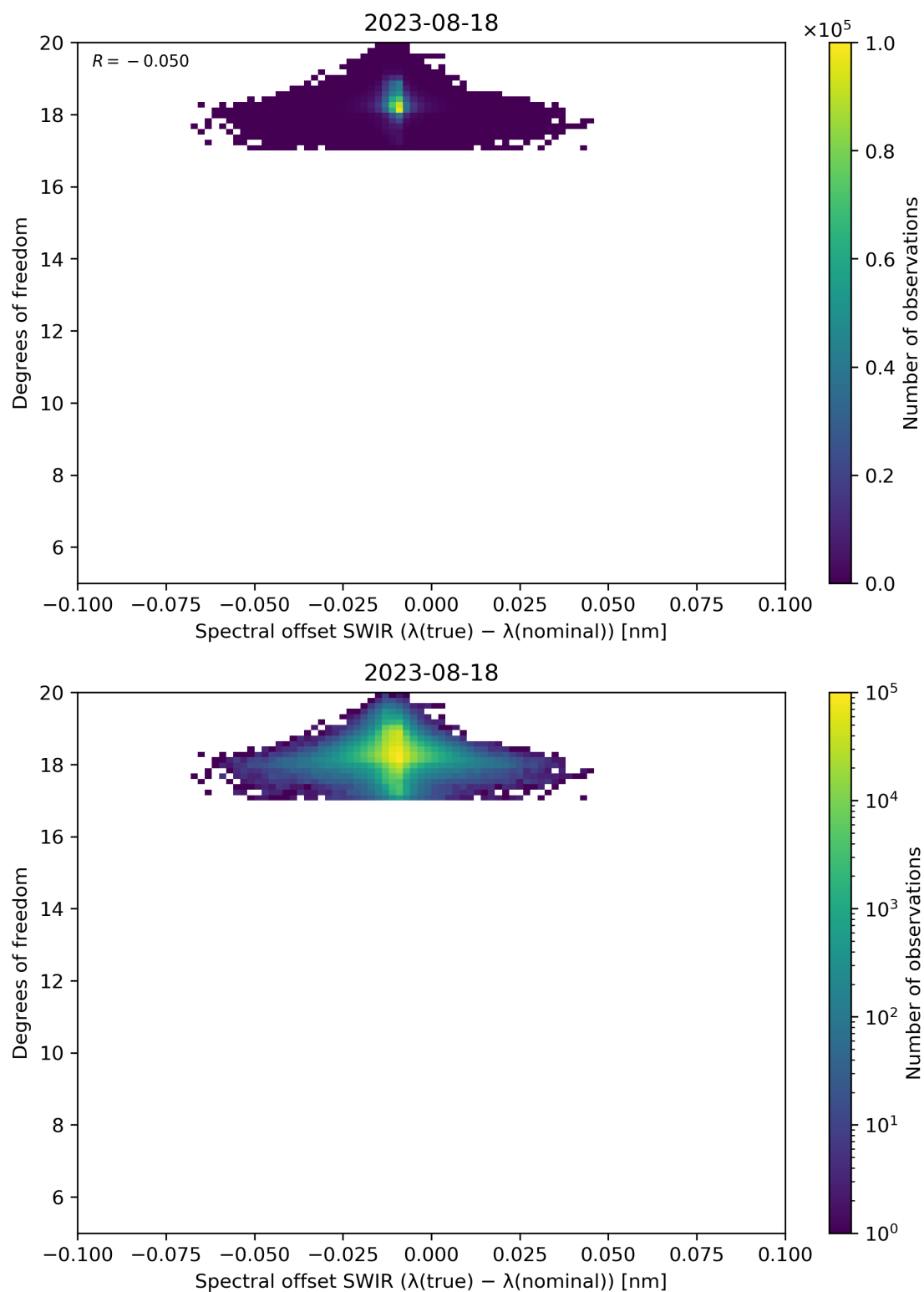
Figure 119: Scatter density plot of “Spectral offset SWIR ( \lambda(\text{true}) - \lambda(\text{nominal}) )” against “Degrees of freedom” for 2023-08-17 to 2023-08-19.
