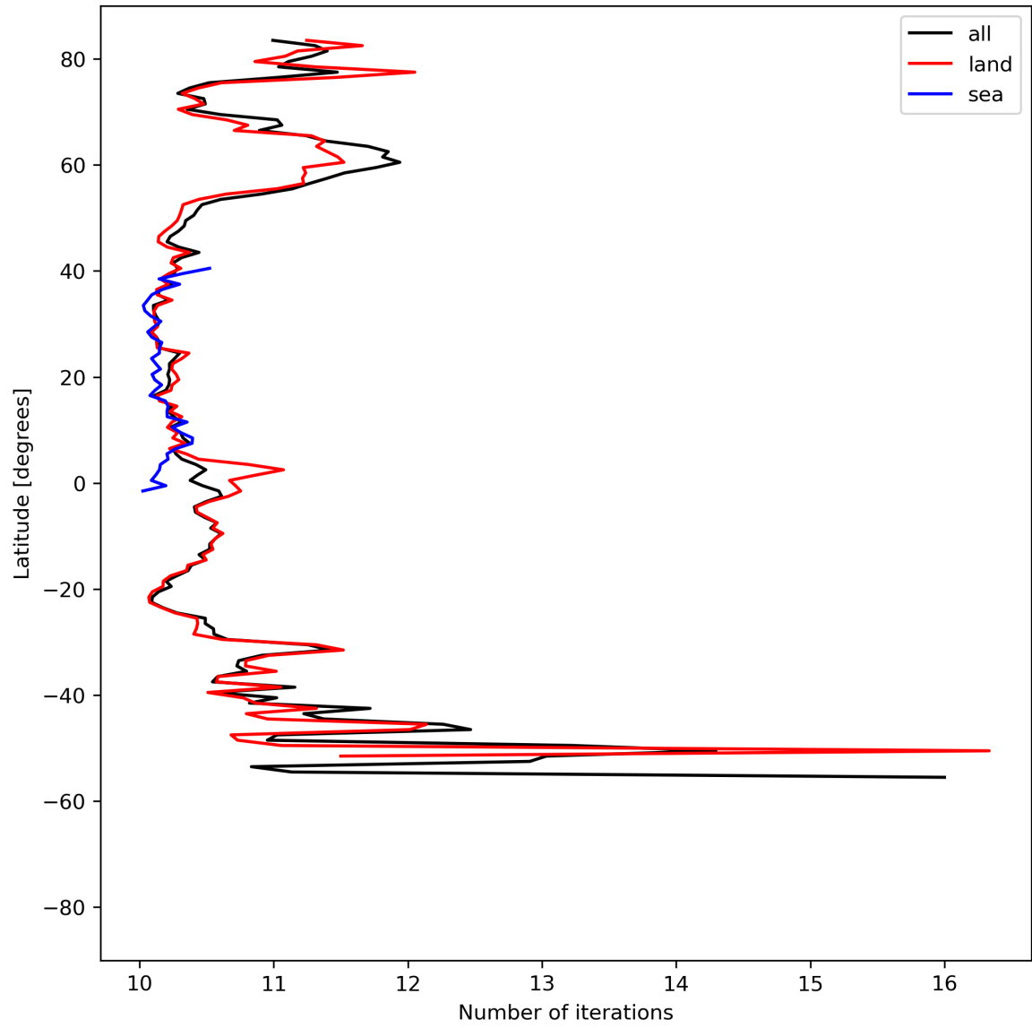
Figure 20: Zonal average of “Number of iterations” for 2023-08-17 to 2023-08-19.
