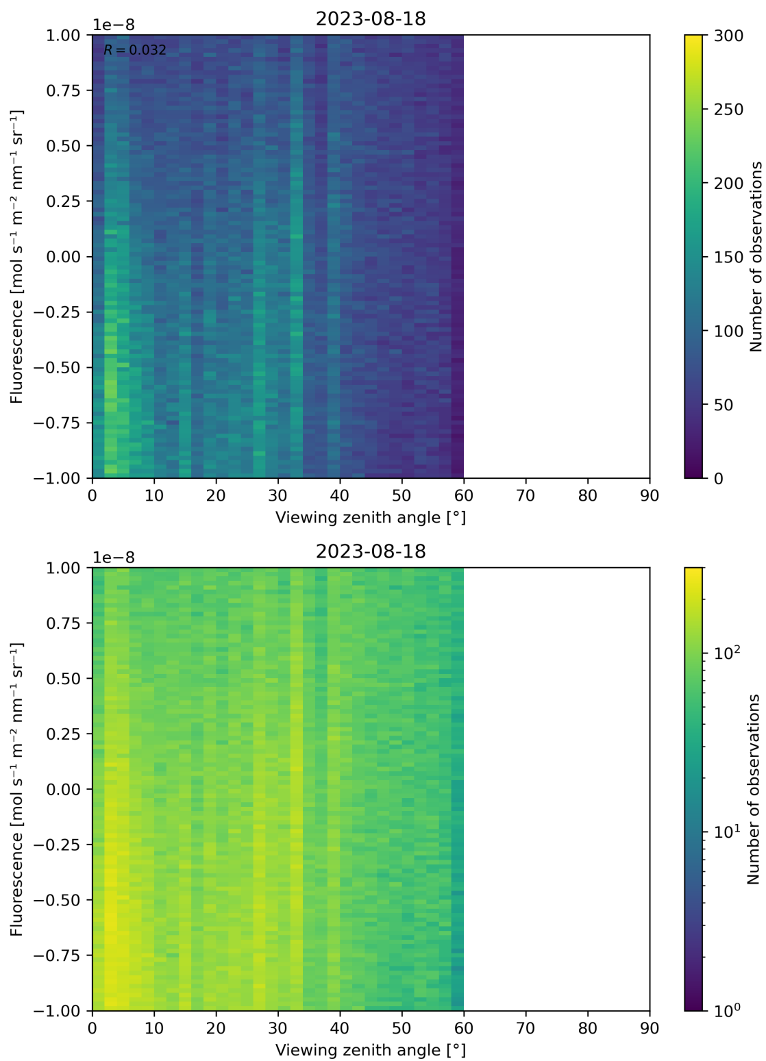
Figure 108: Scatter density plot of “Viewing zenith angle” against “Fluorescence” for 2023-08-17 to 2023-08-19.
