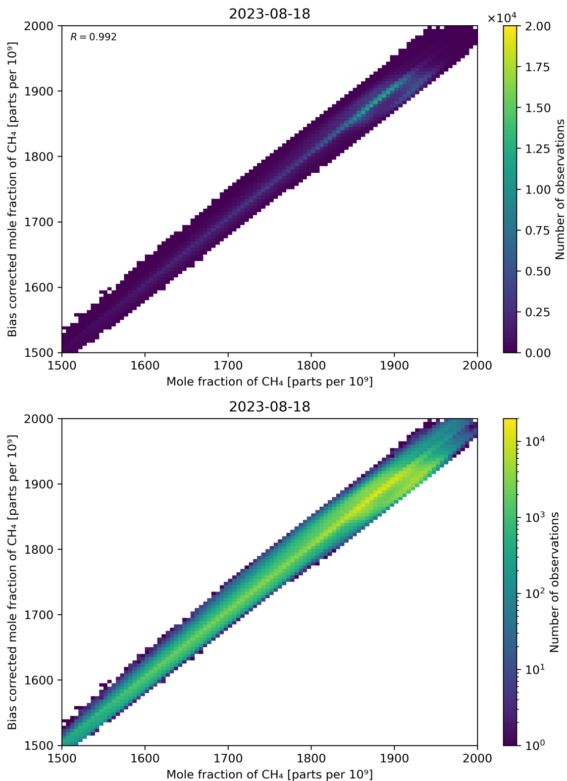
Figure 74: Scatter density plot of “Mole fraction of CH 4 ” against “Bias corrected mole fraction of CH 4 ” for 2023-08-17 to 2023-08-19.
