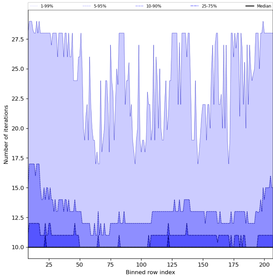
Figure 42: Along track statistics of “Number of iterations” for 2023-08-17 to 2023-08-19
