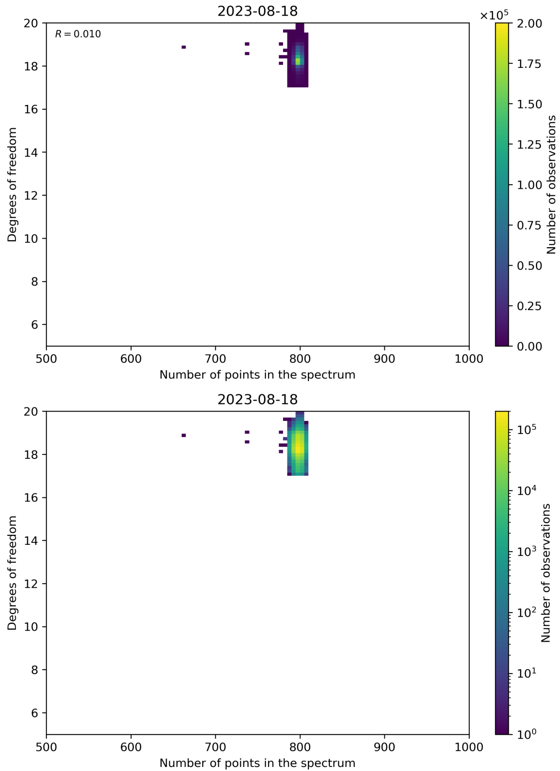
Figure 90: Scatter density plot of “Number of points in the spectrum” against “Degrees of freedom” for 2023-08-17 to 2023-08-19.
