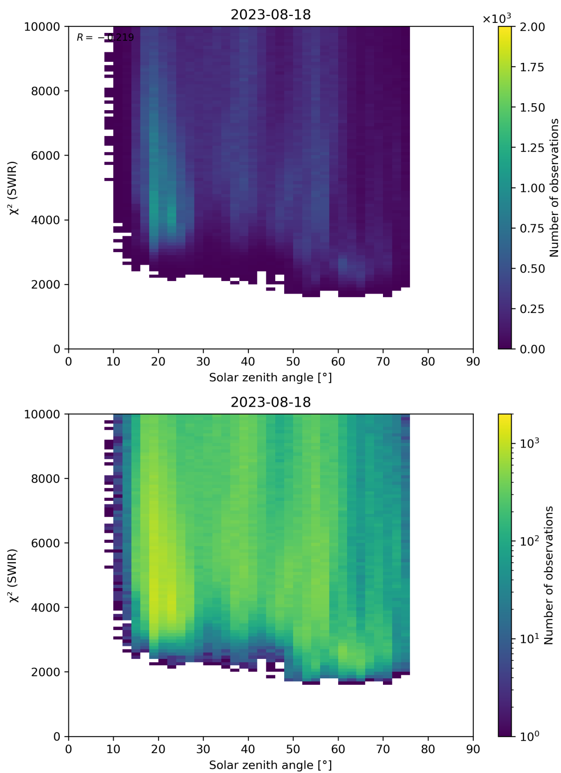
Figure 95: Scatter density plot of “Solar zenith angle” against “ \chi^2 (SWIR)” for 2023-08-17 to 2023-08-19.
