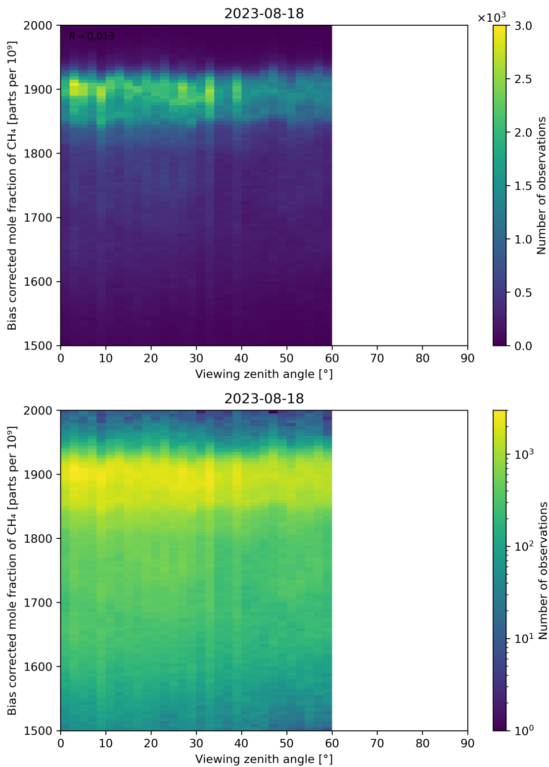
Figure 111: Scatter density plot of “Viewing zenith angle” against “Bias corrected mole fraction of CH 4 ” for 2023-08-17 to 2023-08-19.
