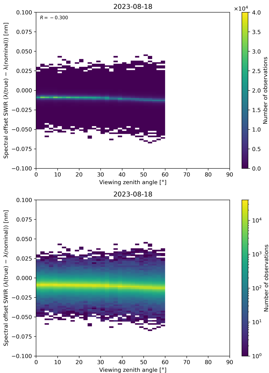
Figure 116: Scatter density plot of “Viewing zenith angle” against “Spectral offset SWIR ( \lambda(\text{true}) - \lambda(\text{nominal}) )” for 2023-08-17 to 2023-08-19.
