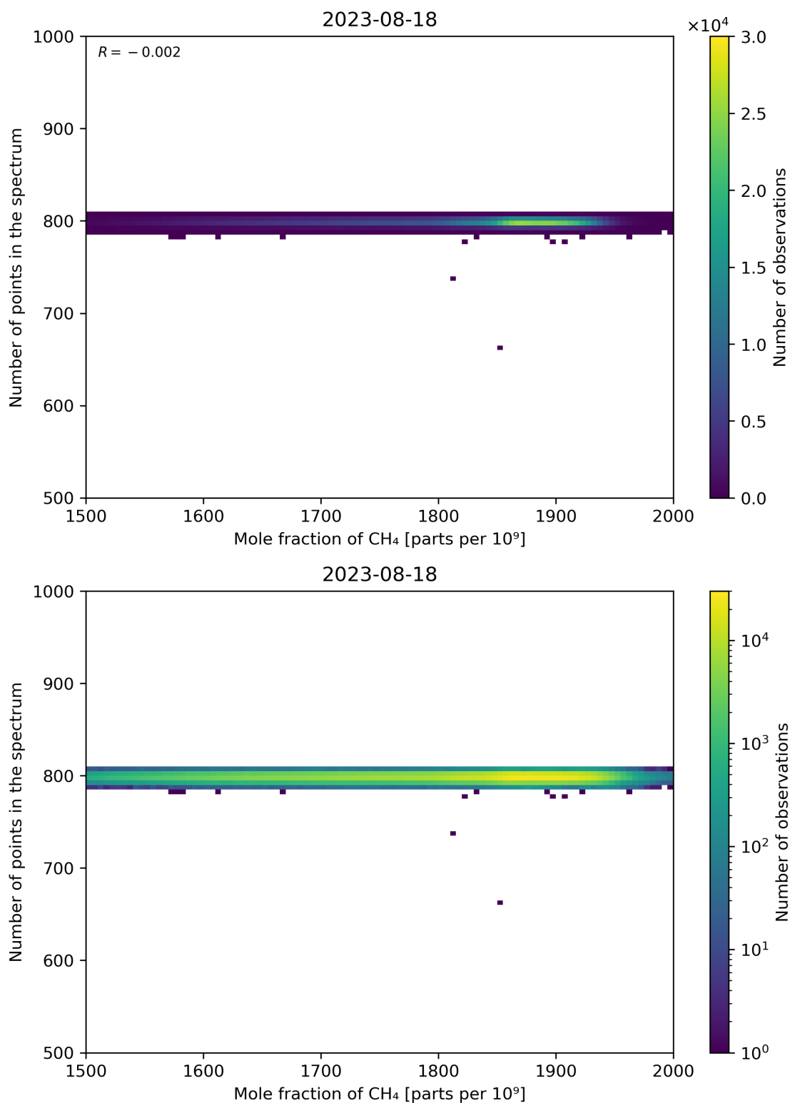
Figure 77: Scatter density plot of “Mole fraction of CH 4 ” against “Number of points in the spectrum” for 2023-08-17 to 2023-08-19.
