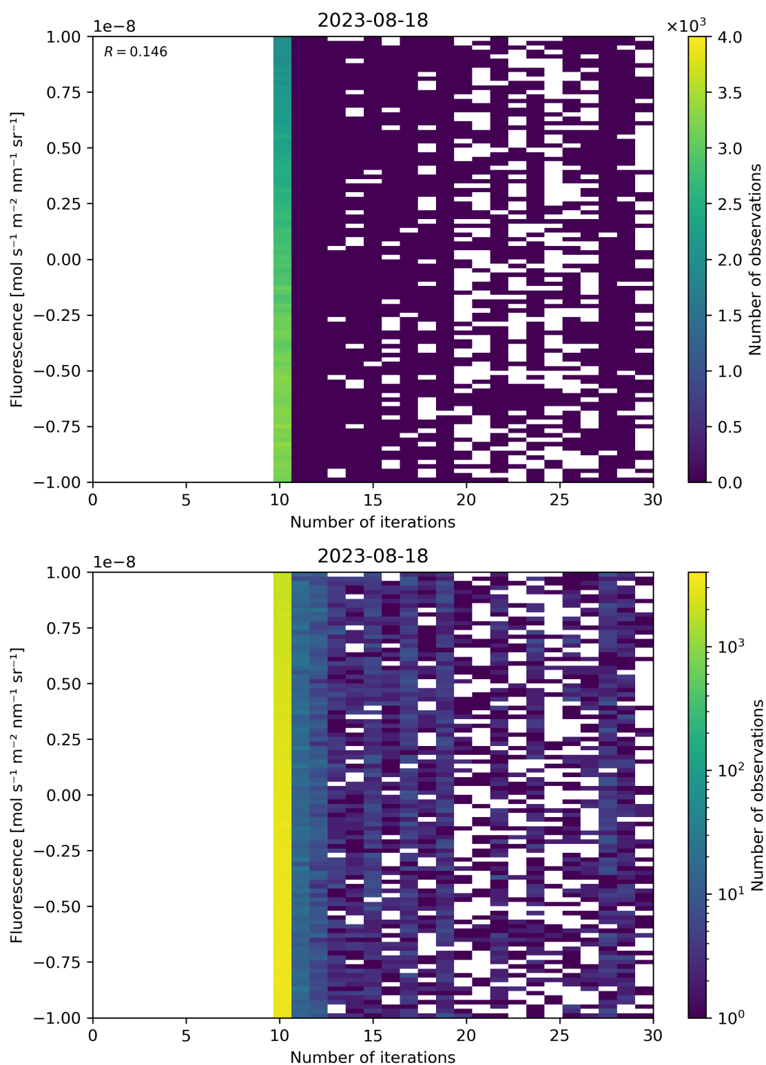
Figure 87: Scatter density plot of “Number of iterations” against “Fluorescence” for 2023-08-17 to 2023-08-19.
