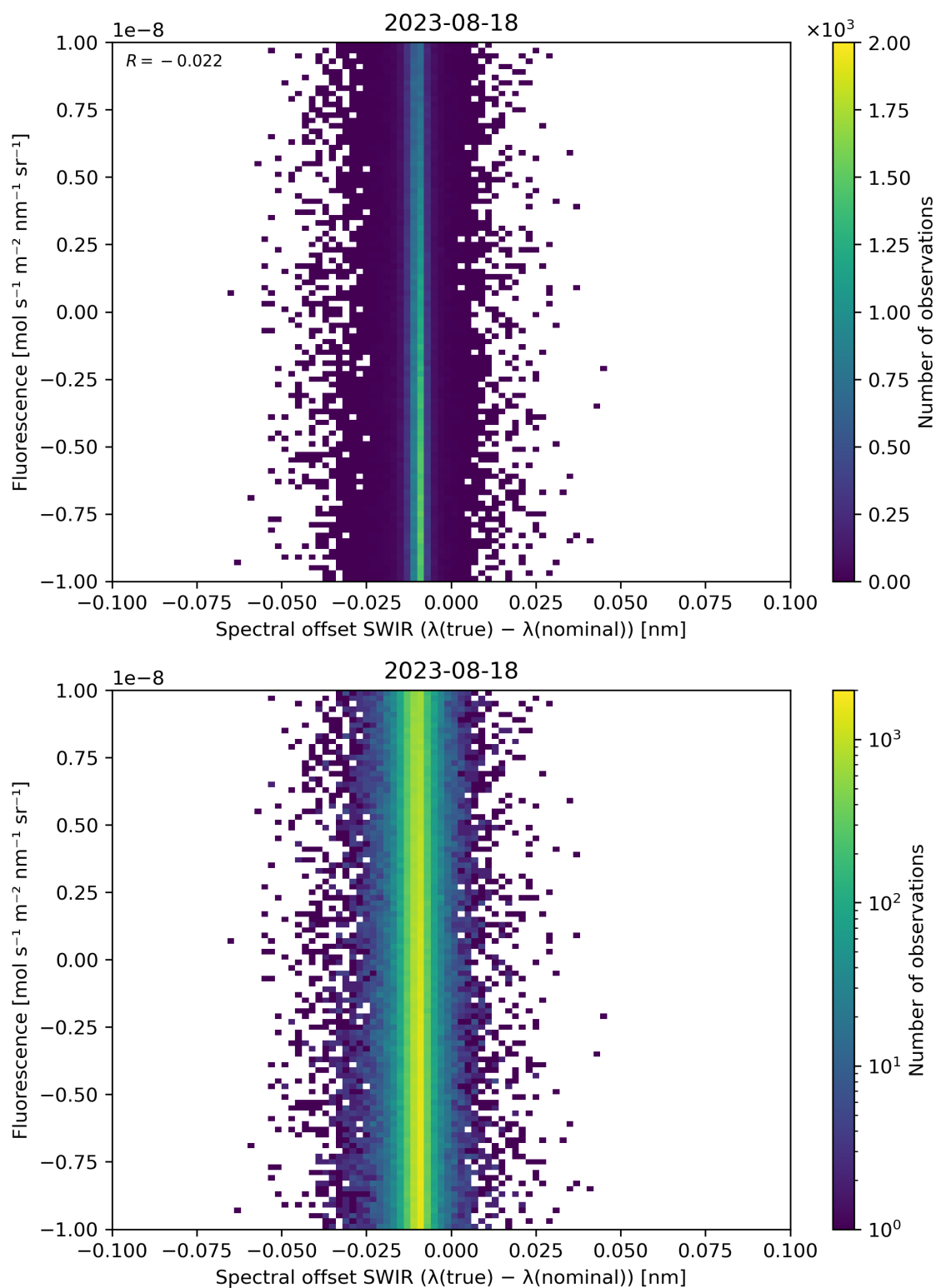
Figure 120: Scatter density plot of “Spectral offset SWIR ( \lambda(\text{true}) - \lambda(\text{nominal}) )” against “Fluorescence” for 2023-08-17 to 2023-08-19.
