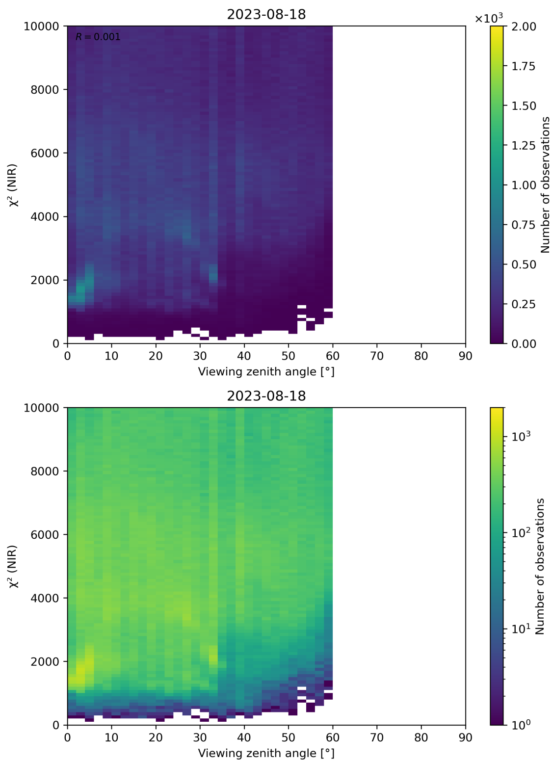
Figure 105: Scatter density plot of “Viewing zenith angle” against “ \chi^2 (NIR)” for 2023-08-17 to 2023-08-19.
