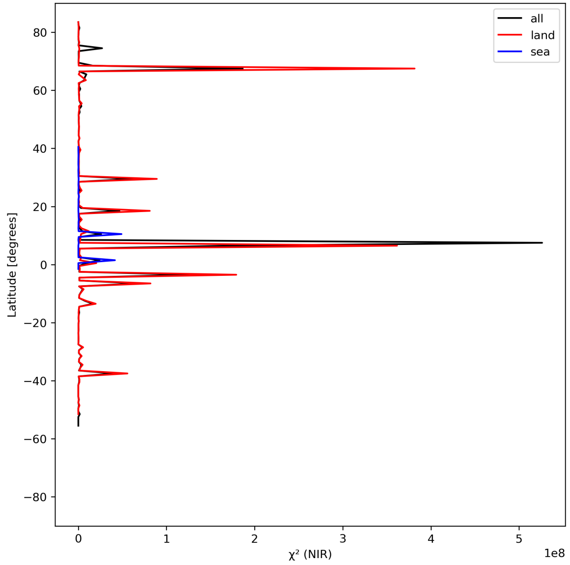
Figure 18: Zonal average of “ \chi^2 (NIR)” for 2023-08-17 to 2023-08-19.
