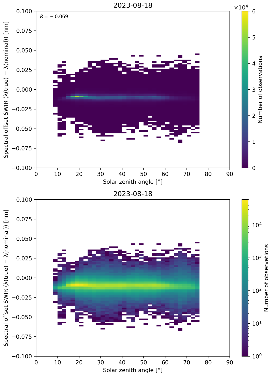
Figure 104: Scatter density plot of “Solar zenith angle” against “Spectral offset SWIR ( \lambda(\text{true}) - \lambda(\text{nominal}) )” for 2023-08-17 to 2023-08-19.
