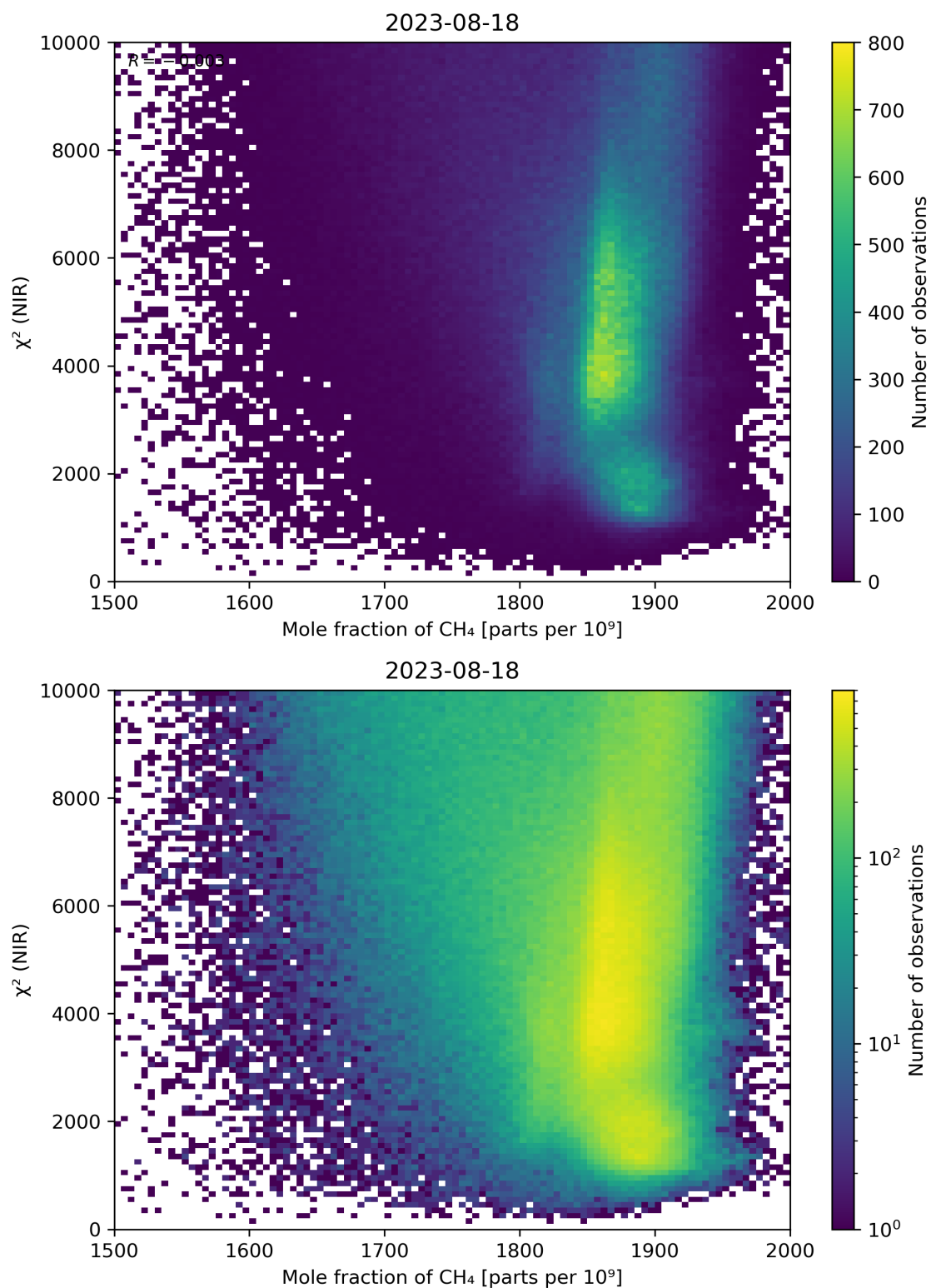
Figure 70: Scatter density plot of “Mole fraction of CH 4 ” against “ \chi^2 (NIR)” for 2023-08-17 to 2023-08-19.
