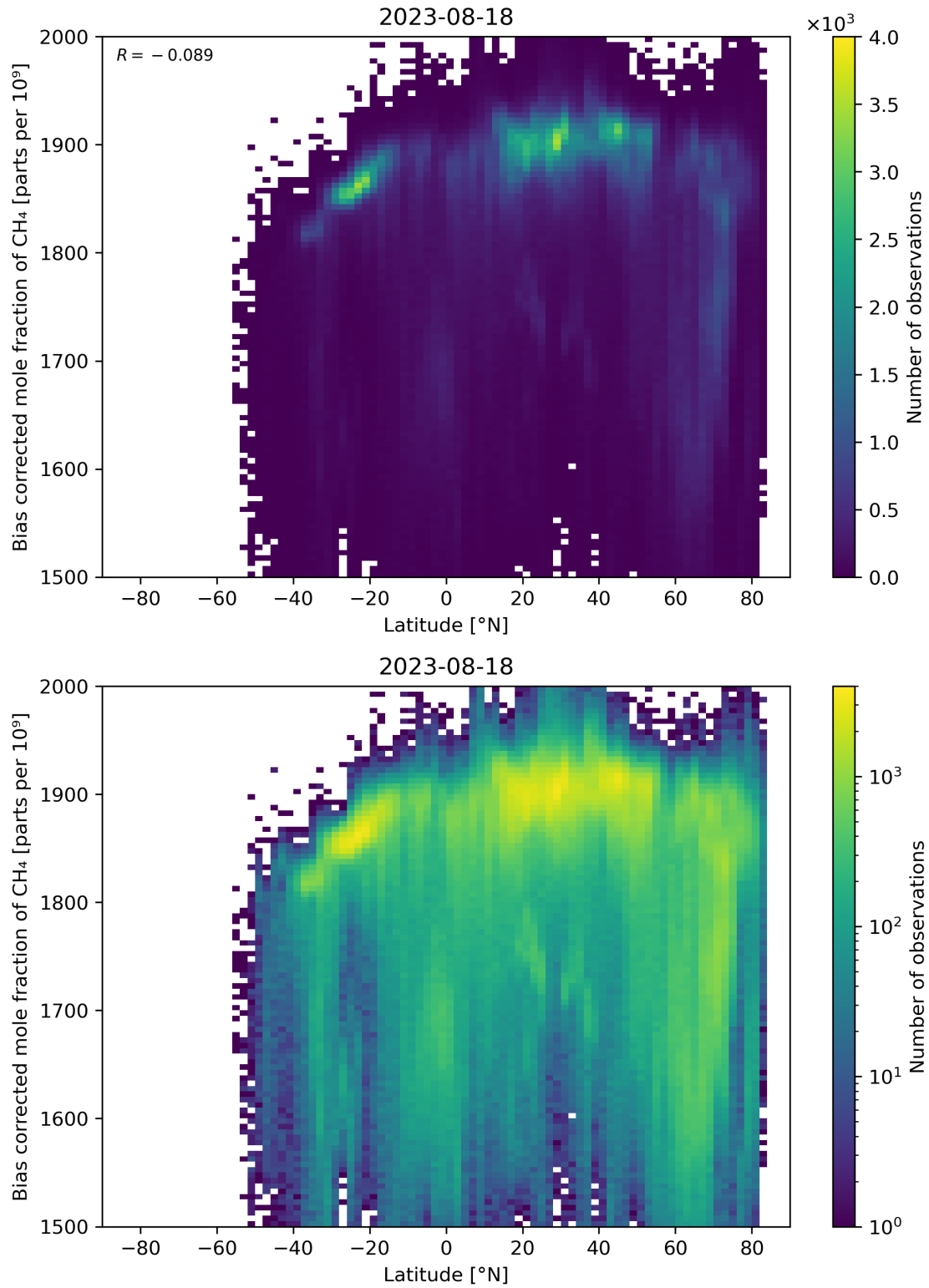
Figure 58: Scatter density plot of “Latitude” against “Bias corrected mole fraction of \text{CH}_4 ” for 2023-08-17 to 2023-08-19.
