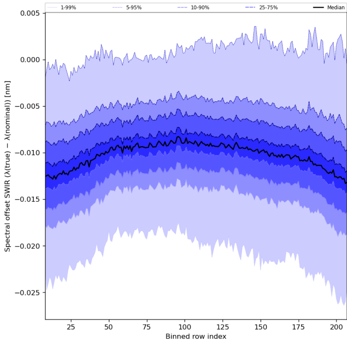
Figure 38: Along track statistics of “Spectral offset SWIR ( \lambda(\text{true}) - \lambda(\text{nominal}) )” for 2023-08-17 to 2023-08-19
