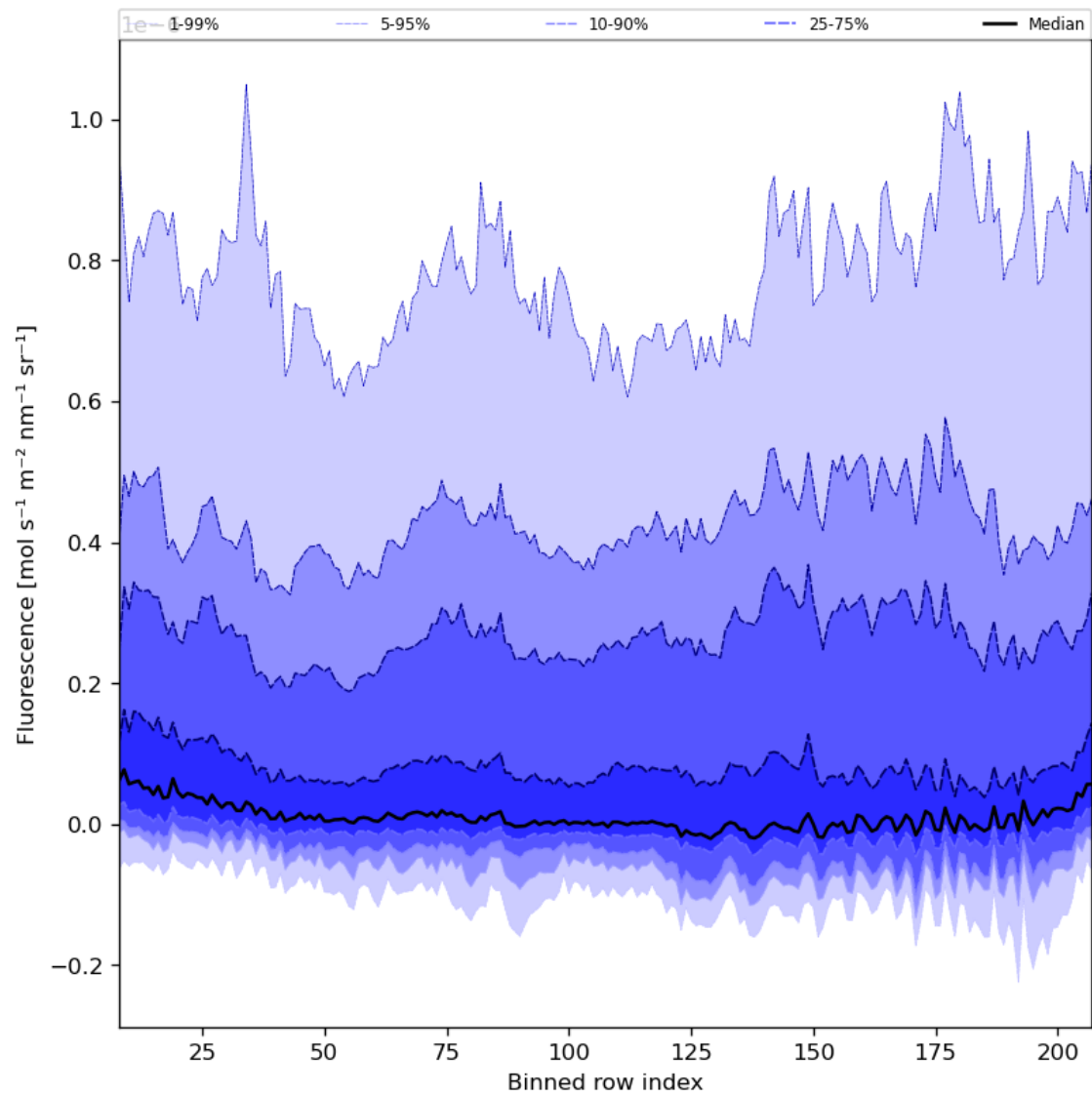
Figure 43: Along track statistics of “Fluorescence” for 2023-08-17 to 2023-08-19
