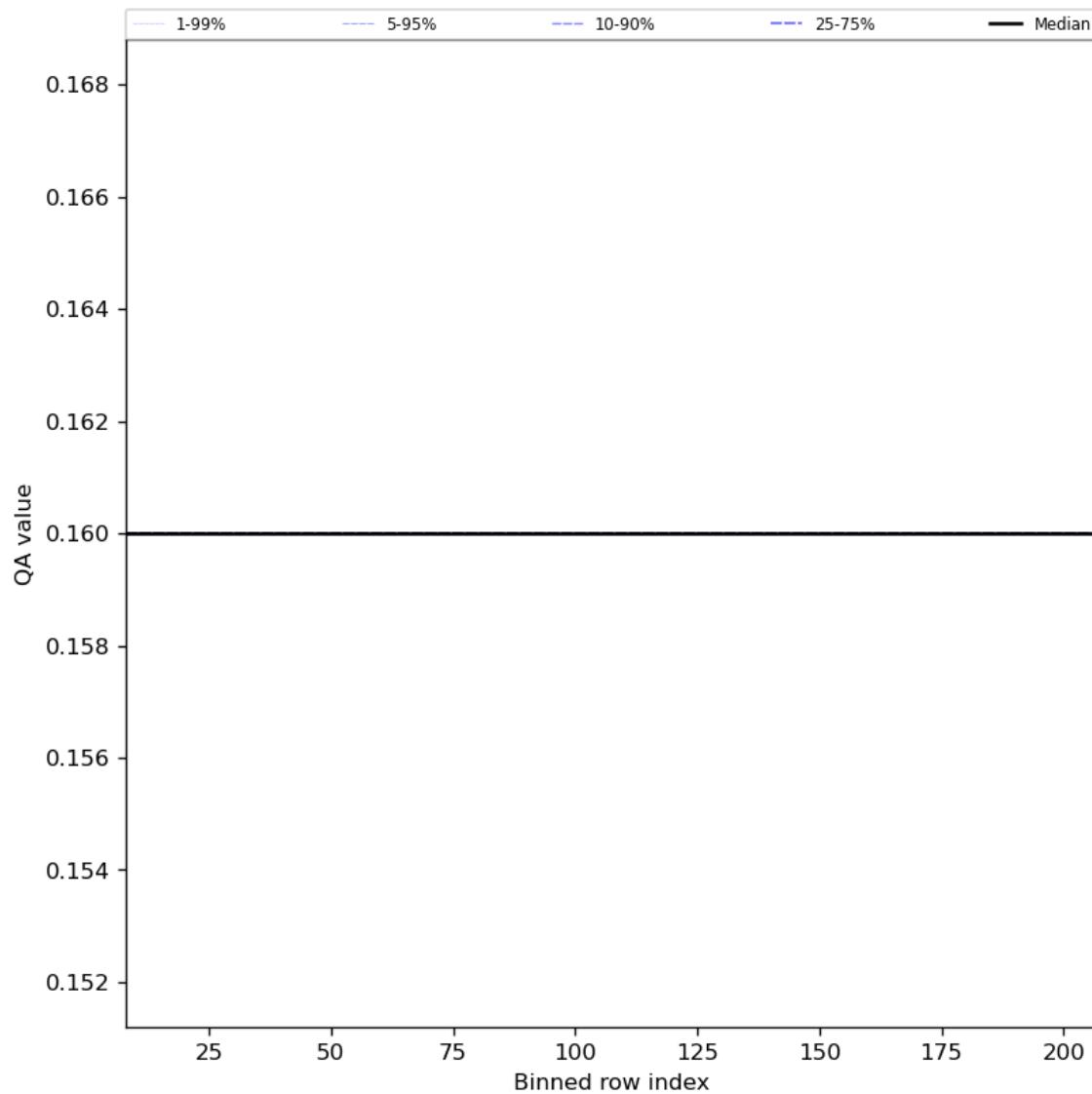
Figure 33: Along track statistics of “QA value” for 2023-08-17 to 2023-08-19
