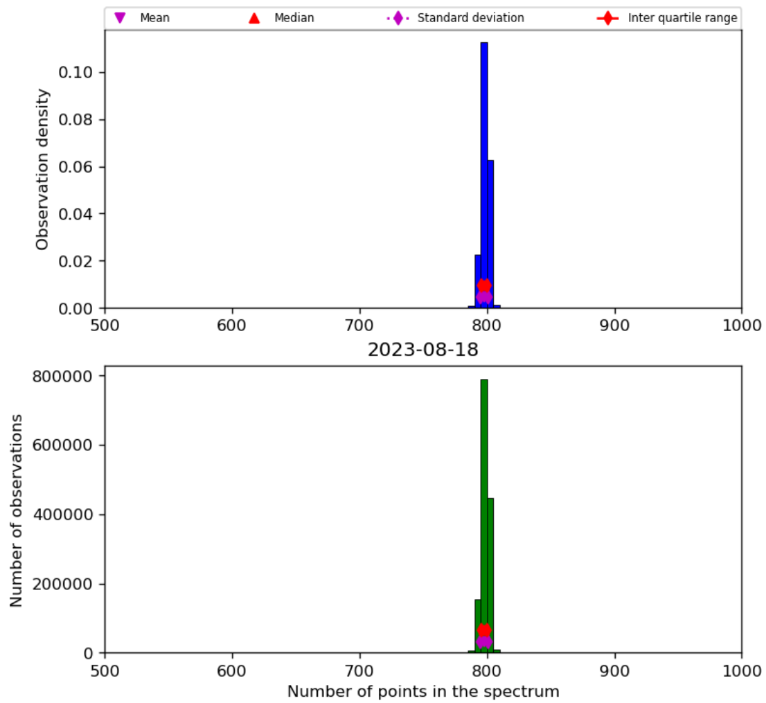
Figure 26: Histogram of “Number of points in the spectrum” for 2023-08-17 to 2023-08-19
