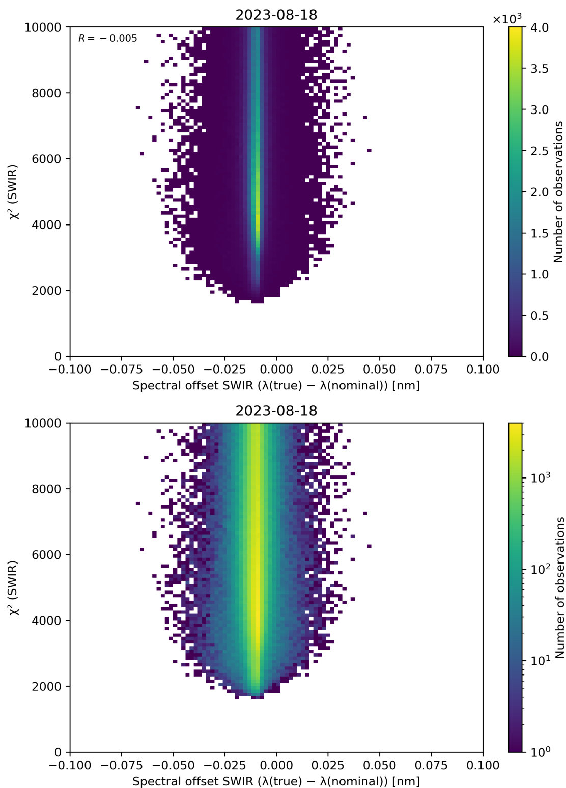
Figure 118: Scatter density plot of “Spectral offset SWIR ( \lambda(\text{true}) - \lambda(\text{nominal}) )” against “ \chi^2 (SWIR)” for 2023-08-17 to 2023-08-19.
