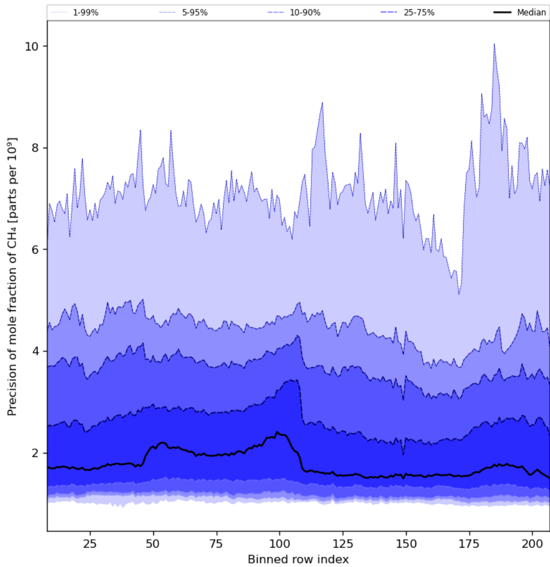
Figure 35: Along track statistics of “Precision of mole fraction of CH 4 ” for 2023-08-17 to 2023-08-19
