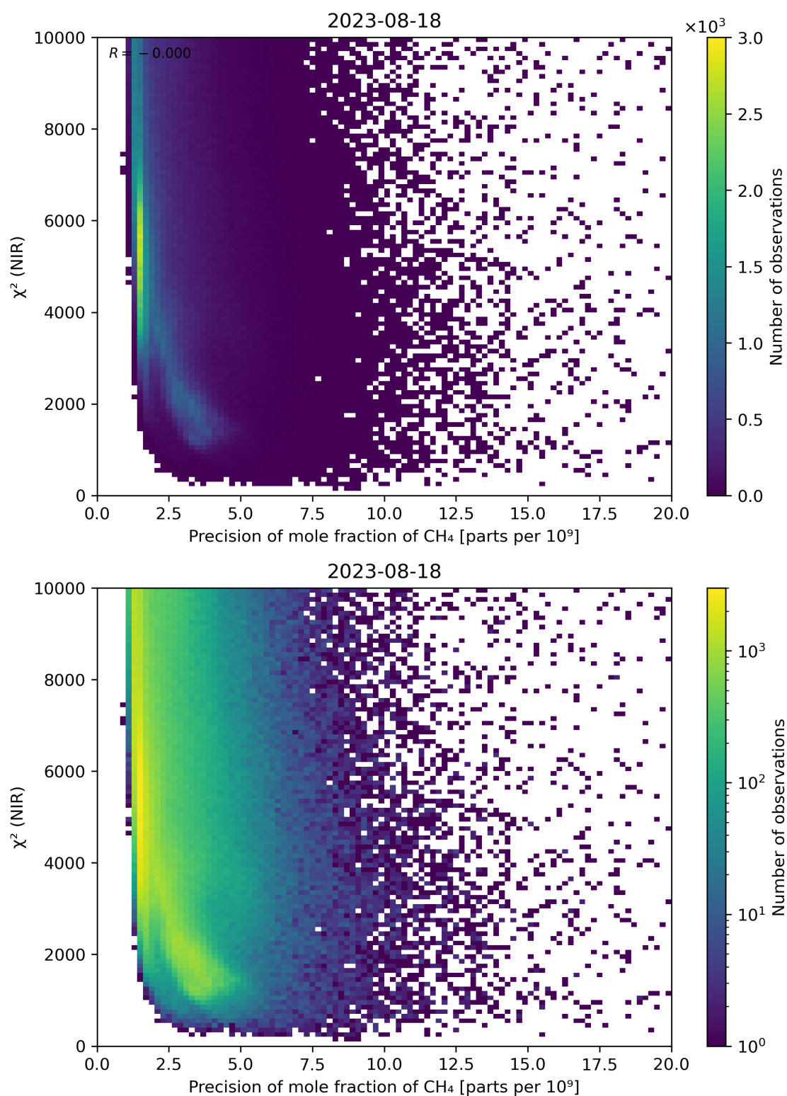
Figure 78: Scatter density plot of “Precision of mole fraction of CH 4 ” against “ \chi^2 (NIR)” for 2023-08-17 to 2023-08-19.
