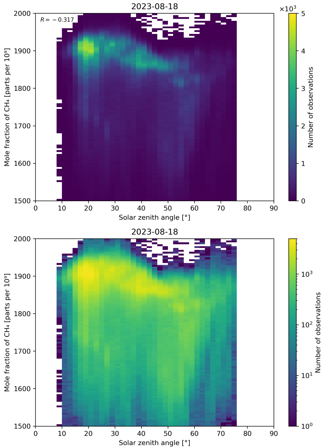
Figure 99: Scatter density plot of “Solar zenith angle” against “Mole fraction of CH 4 ” for 2023-08-17 to 2023-08-19.
