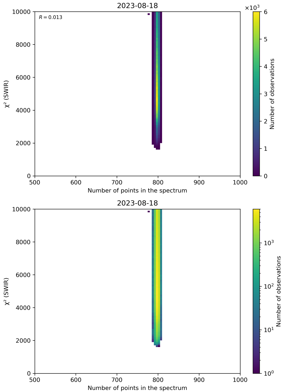
Figure 89: Scatter density plot of “Number of points in the spectrum” against “ \chi^2 (SWIR)” for 2023-08-17 to 2023-08-19.
