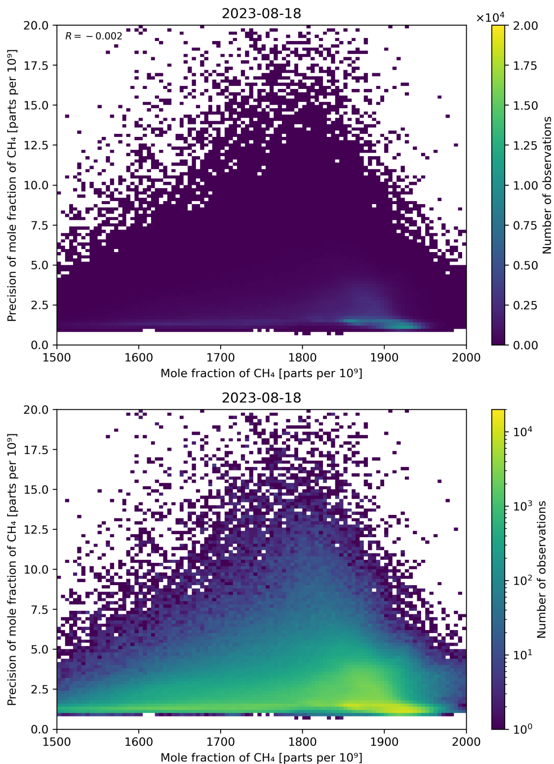
Figure 75: Scatter density plot of “Mole fraction of CH 4 ” against “Precision of mole fraction of CH 4 ” for 2023-08-17 to 2023-08-19.
