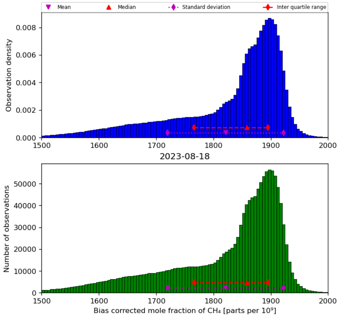
Figure 25: Histogram of “Bias corrected mole fraction of CH 4 ” for 2023-08-17 to 2023-08-19
