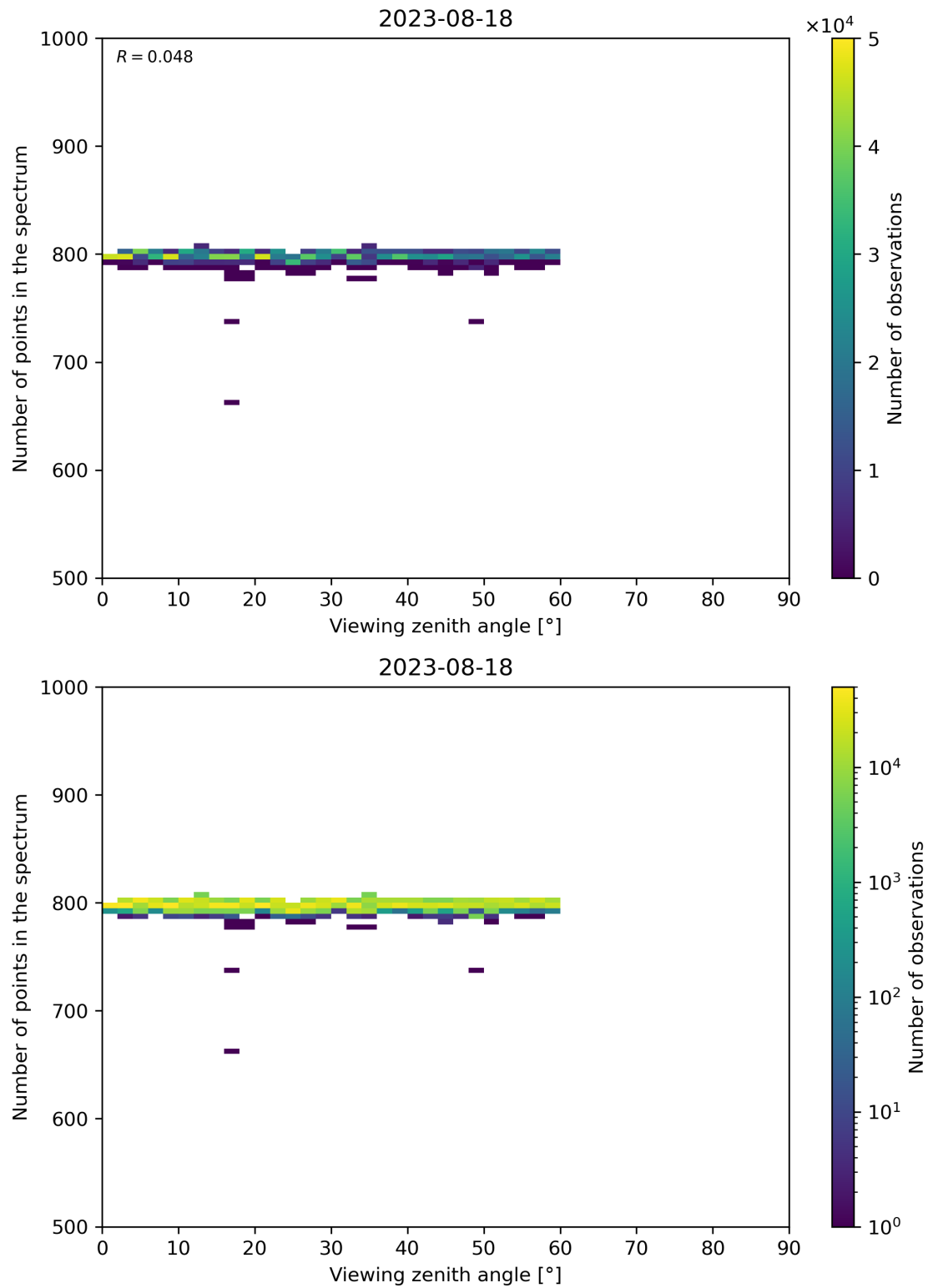
Figure 114: Scatter density plot of “Viewing zenith angle” against “Number of points in the spectrum” for 2023-08-17 to 2023-08-19.
