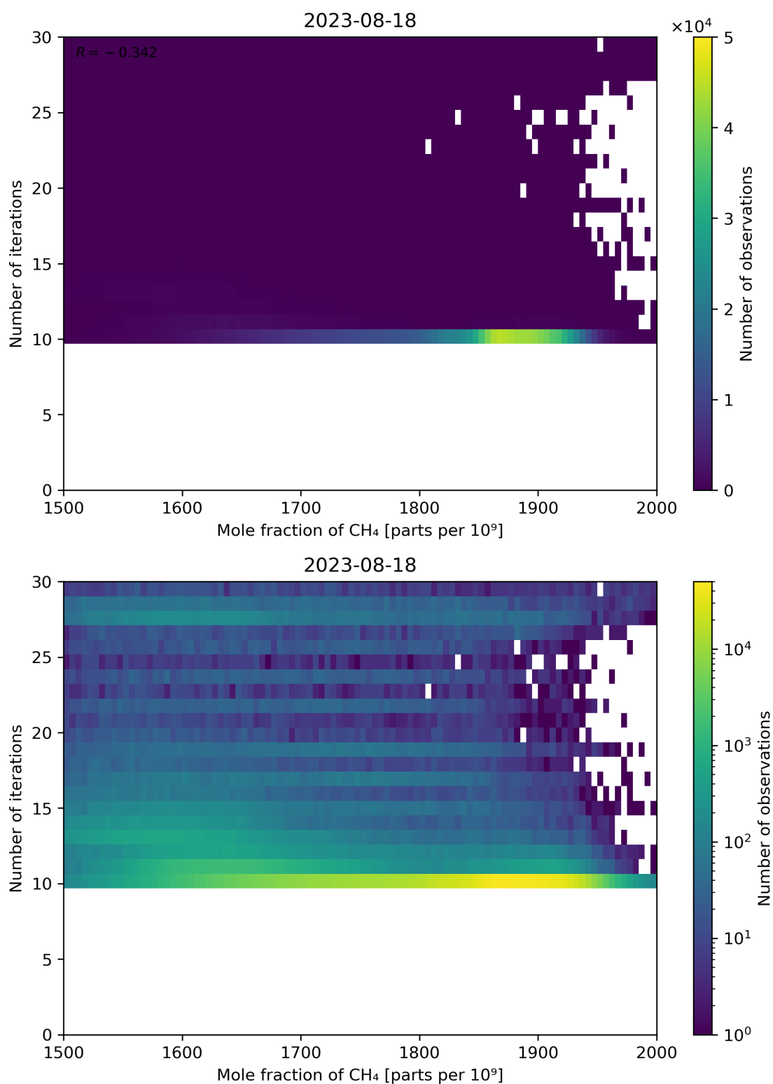
Figure 76: Scatter density plot of “Mole fraction of CH 4 ” against “Number of iterations” for 2023-08-17 to 2023-08-19.
