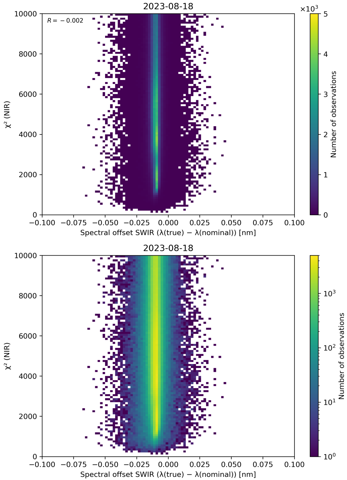
Figure 117: Scatter density plot of “Spectral offset SWIR ( \lambda(\text{true}) - \lambda(\text{nominal}) )” against “ \chi^2 (NIR)” for 2023-08-17 to 2023-08-19.
