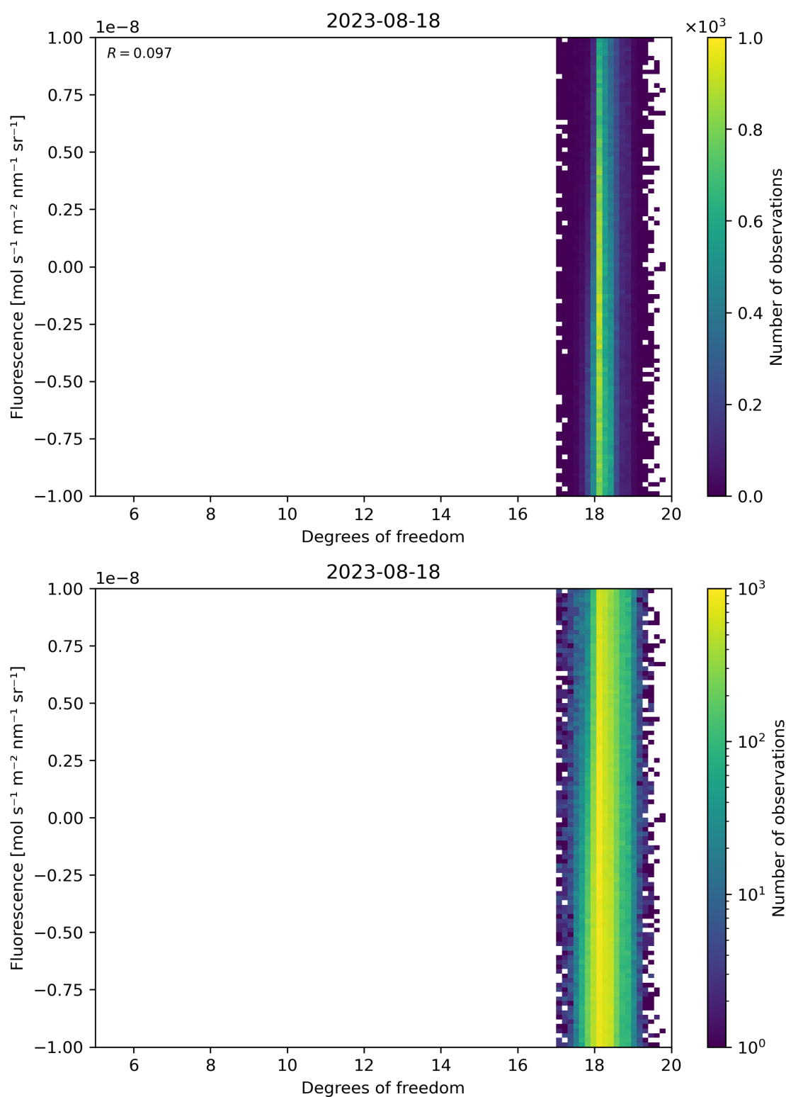
Figure 51: Scatter density plot of “Degrees of freedom” against “Fluorescence” for 2023-08-17 to 2023-08-19.
