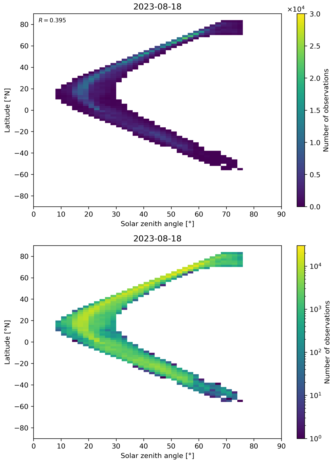
Figure 98: Scatter density plot of “Solar zenith angle” against “Latitude” for 2023-08-17 to 2023-08-19.
