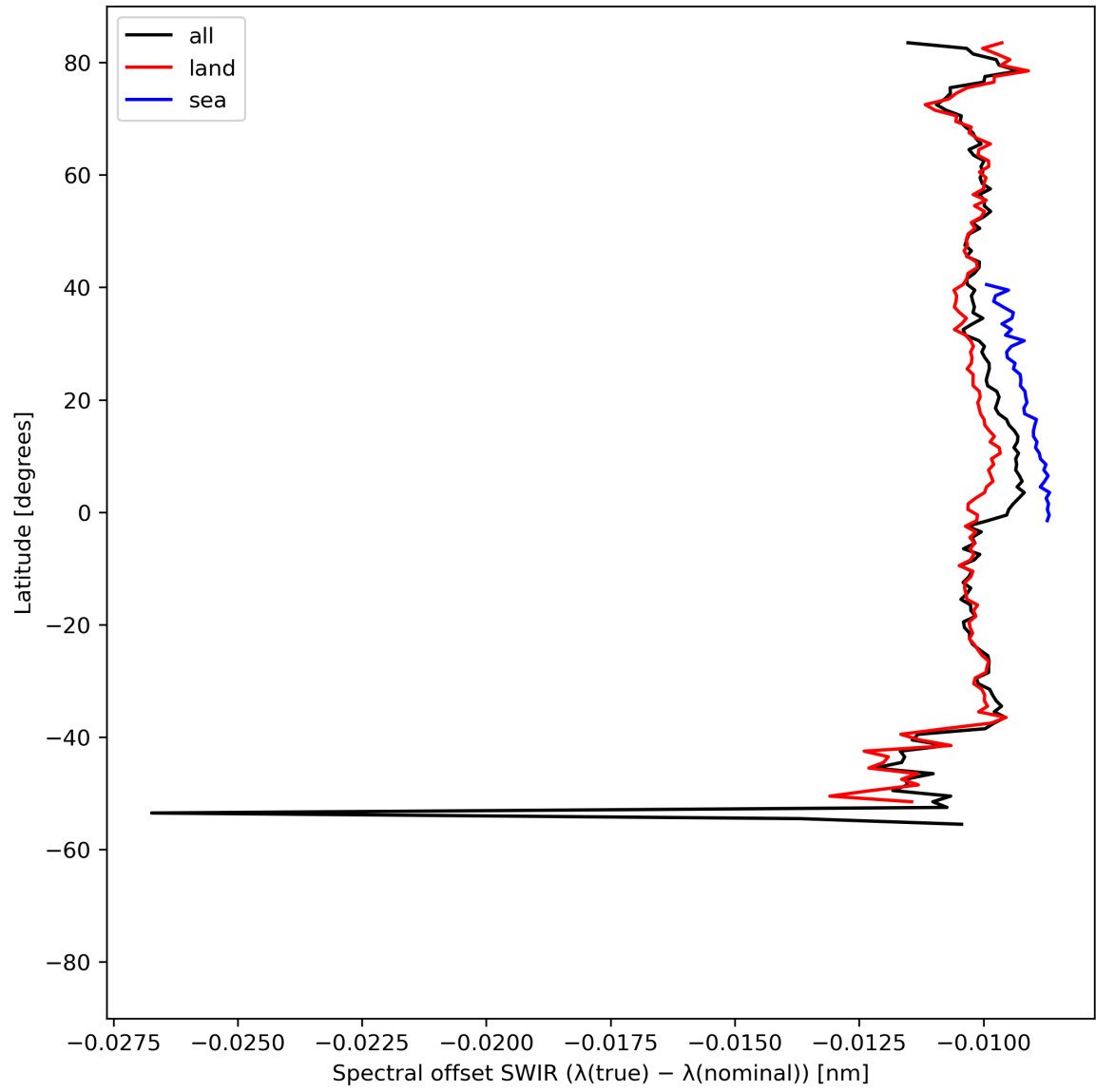
Figure 16: Zonal average of “Spectral offset SWIR ( \lambda(\text{true}) - \lambda(\text{nominal}) )” for 2023-08-17 to 2023-08-19.
