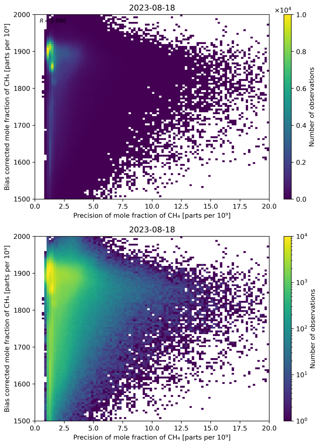
Figure 82: Scatter density plot of “Precision of mole fraction of CH 4 ” against “Bias corrected mole fraction of CH 4 ” for 2023-08-17 to 2023-08-19.
