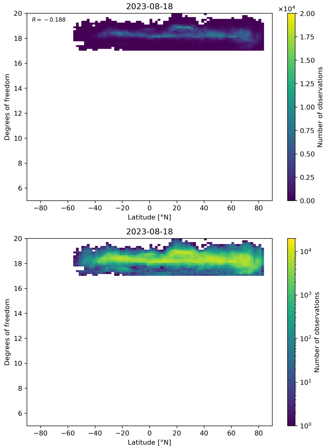
Figure 55: Scatter density plot of “Latitude” against “Degrees of freedom” for 2023-08-17 to 2023-08-19.
