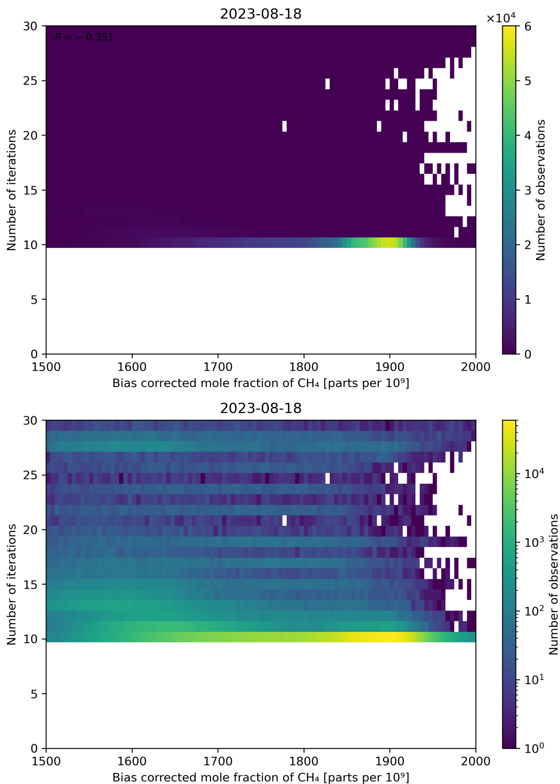
Figure 67: Scatter density plot of “Bias corrected mole fraction of CH 4 ” against “Number of iterations” for 2023-08-17 to 2023-08-19.
