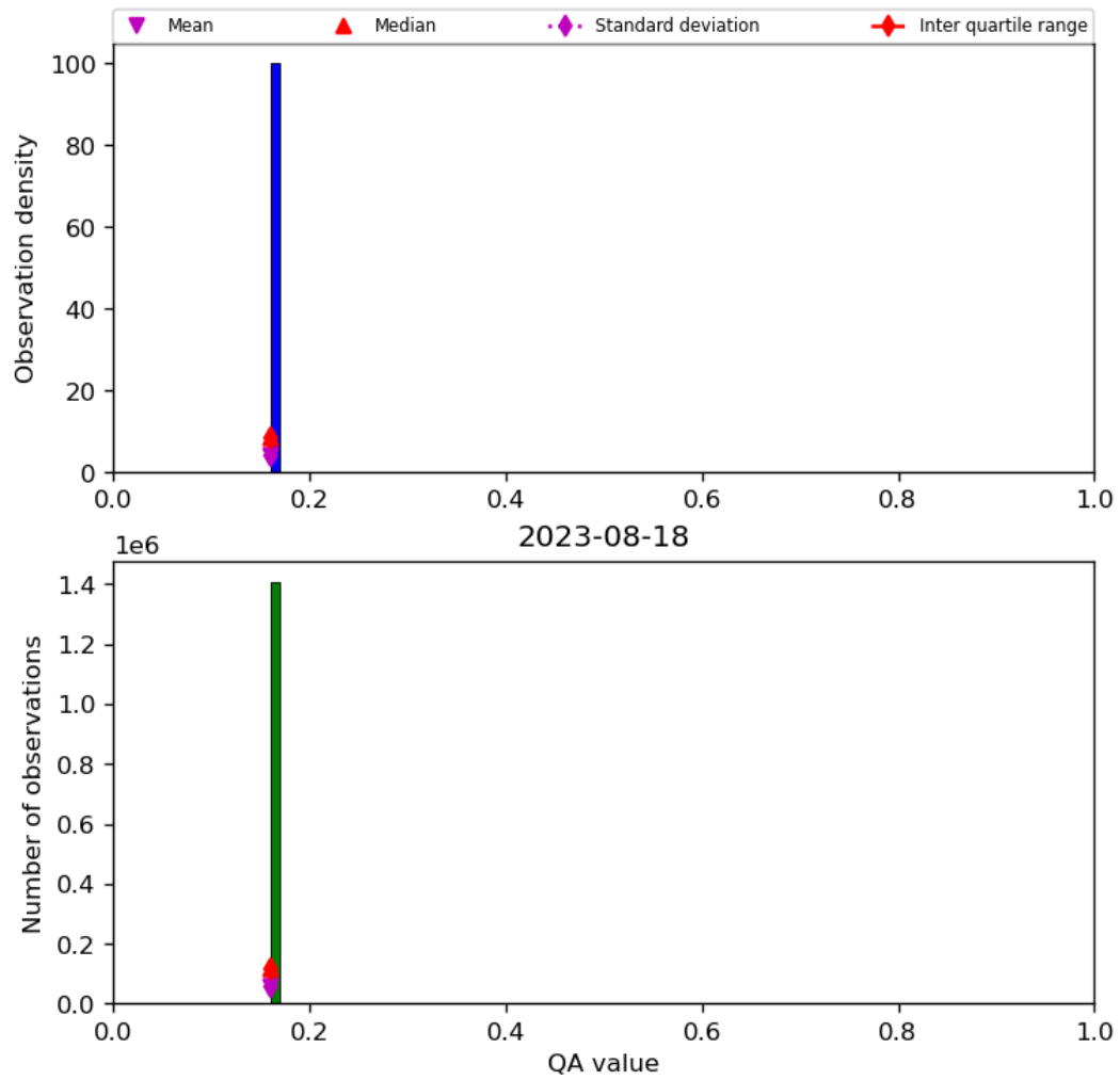
Figure 22: Histogram of “QA value” for 2023-08-17 to 2023-08-19
