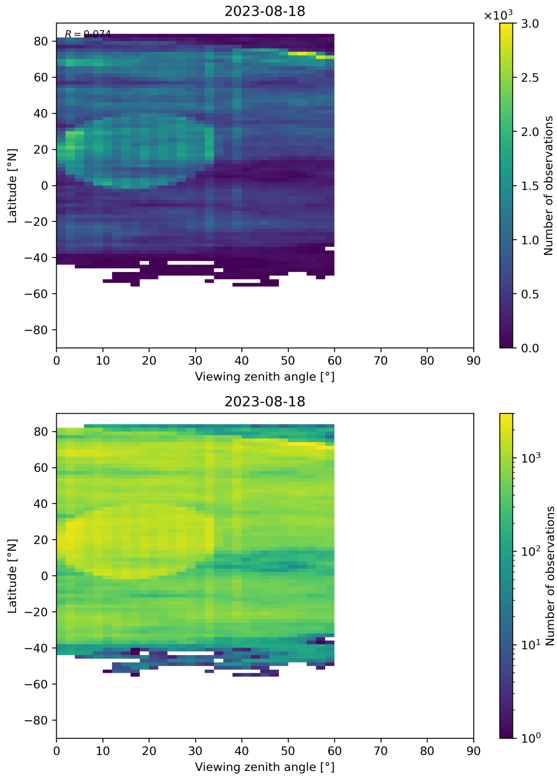
Figure 109: Scatter density plot of “Viewing zenith angle” against “Latitude” for 2023-08-17 to 2023-08-19.
