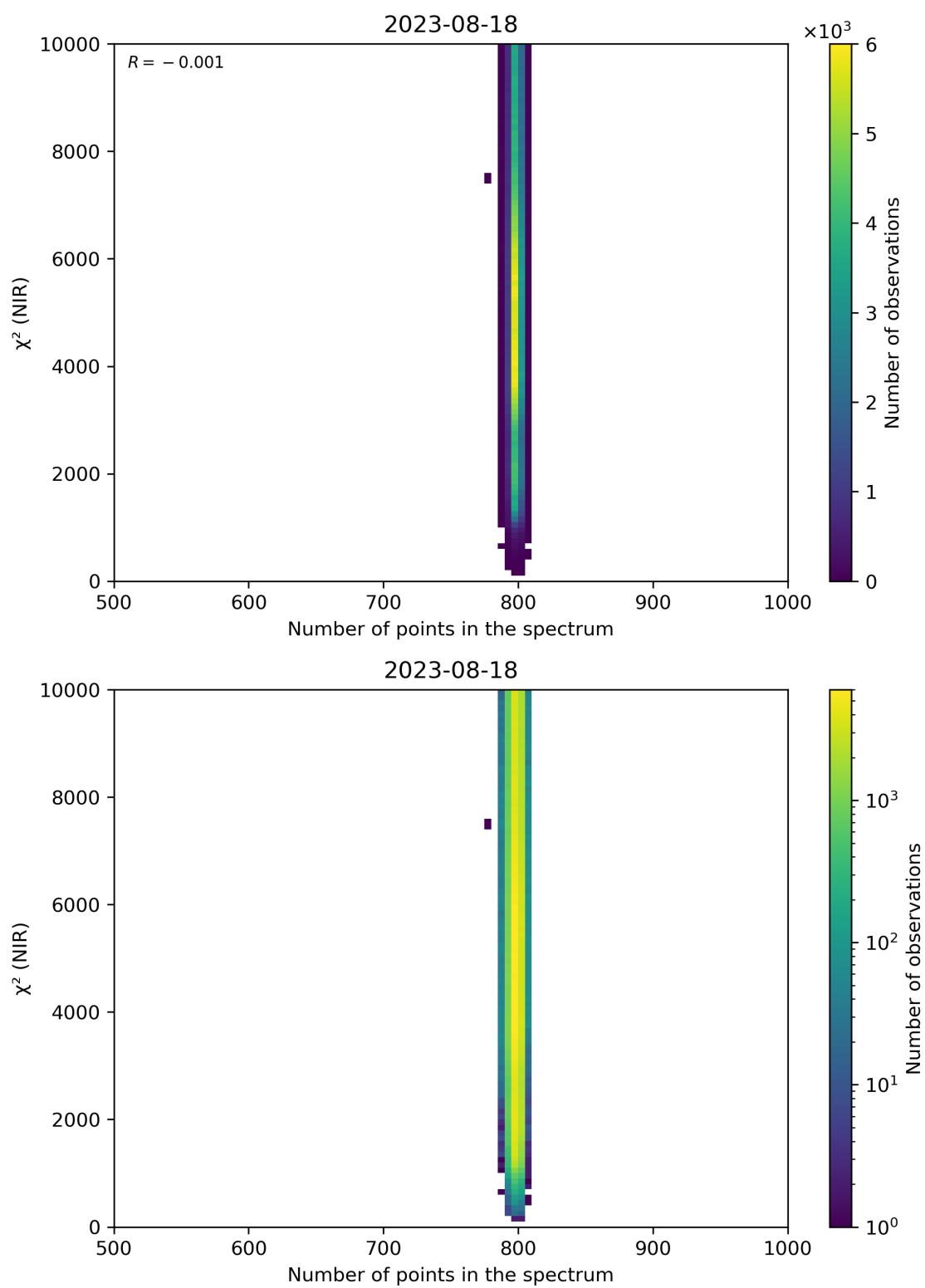
Figure 88: Scatter density plot of “Number of points in the spectrum” against “ \chi^2 (NIR)” for 2023-08-17 to 2023-08-19.
