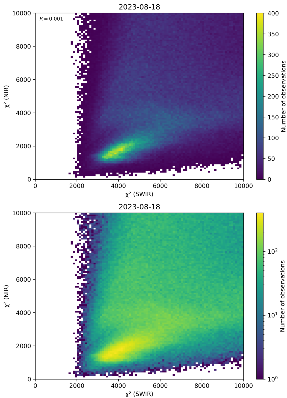
Figure 47: Scatter density plot of “ \chi^2 (SWIR)” against “ \chi^2 (NIR)” for 2023-08-17 to 2023-08-19.
