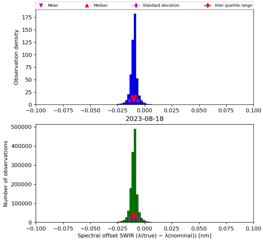
Figure 27: Histogram of “Spectral offset SWIR ( \lambda(\text{true}) - \lambda(\text{nominal}) )” for 2023-08-17 to 2023-08-19
