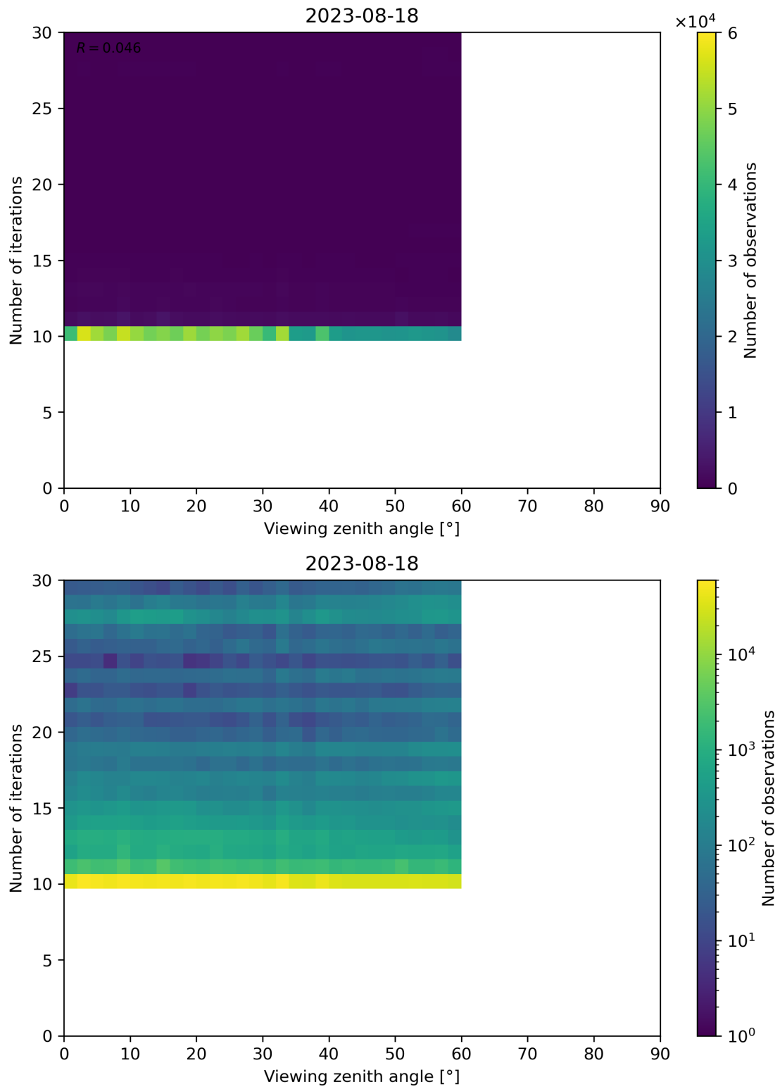
Figure 113: Scatter density plot of “Viewing zenith angle” against “Number of iterations” for 2023-08-17 to 2023-08-19.
