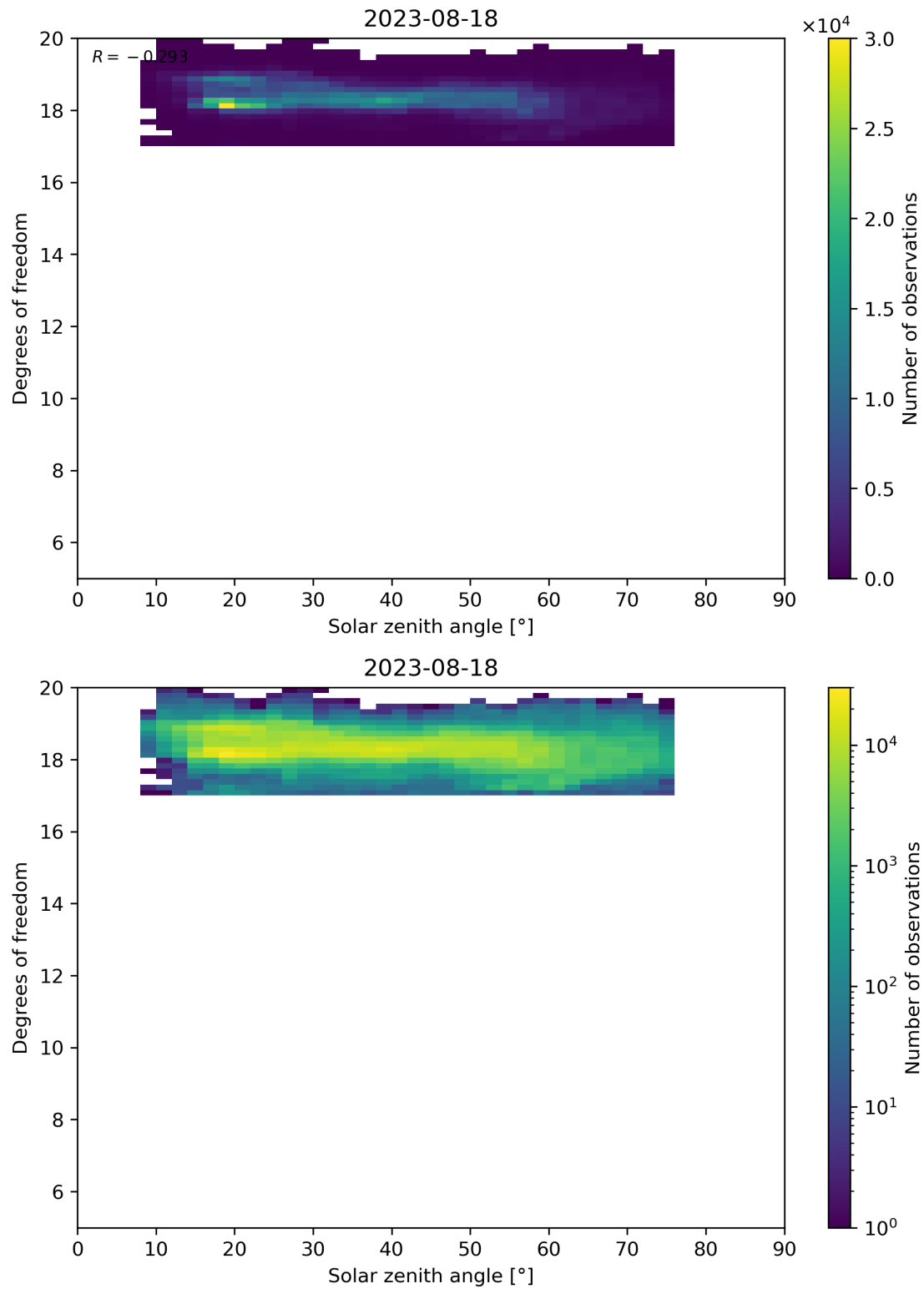
Figure 96: Scatter density plot of “Solar zenith angle” against “Degrees of freedom” for 2023-08-17 to 2023-08-19.
