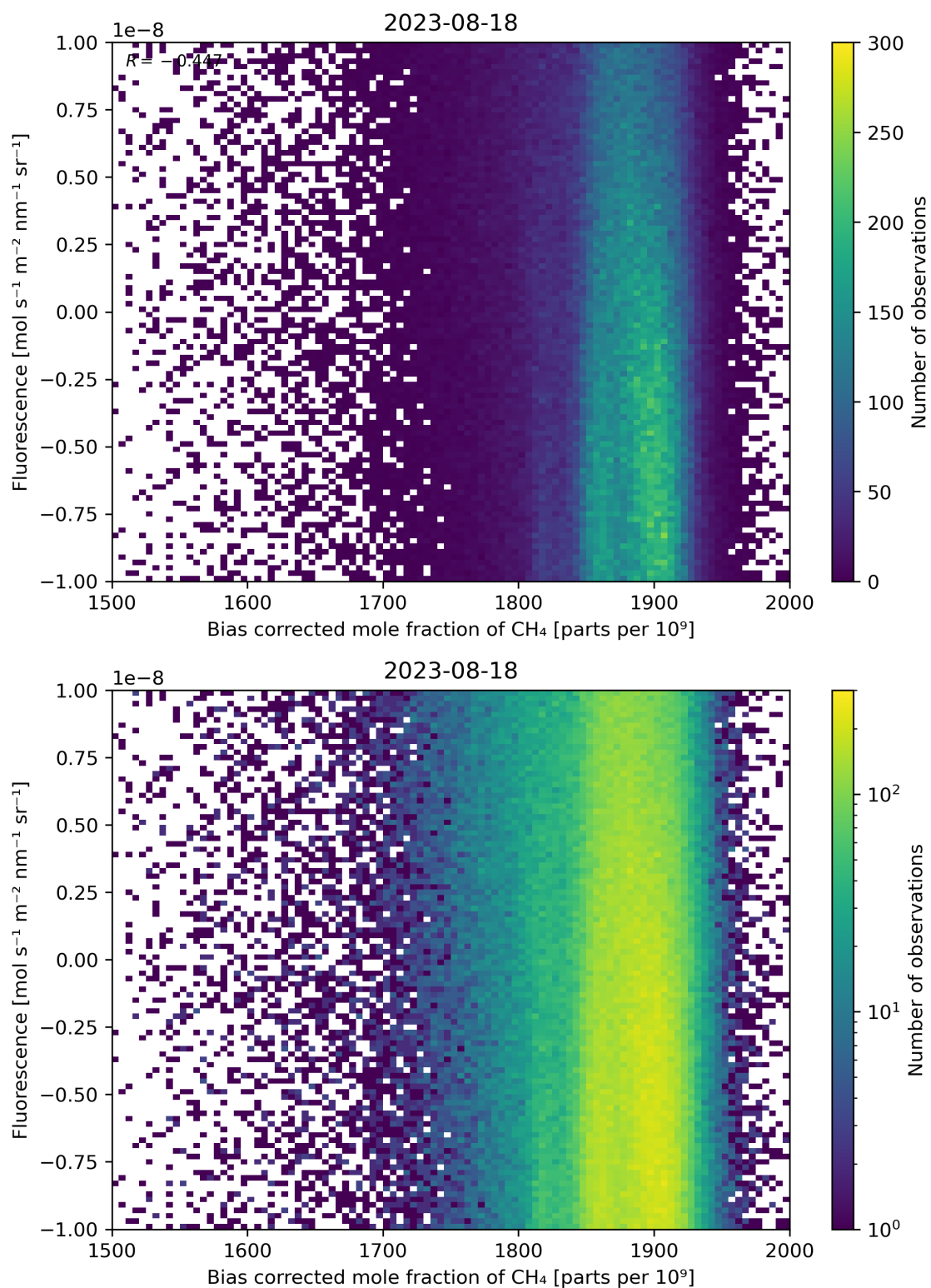
Figure 66: Scatter density plot of “Bias corrected mole fraction of \text{CH}_4 ” against “Fluorescence” for 2023-08-17 to 2023-08-19.
