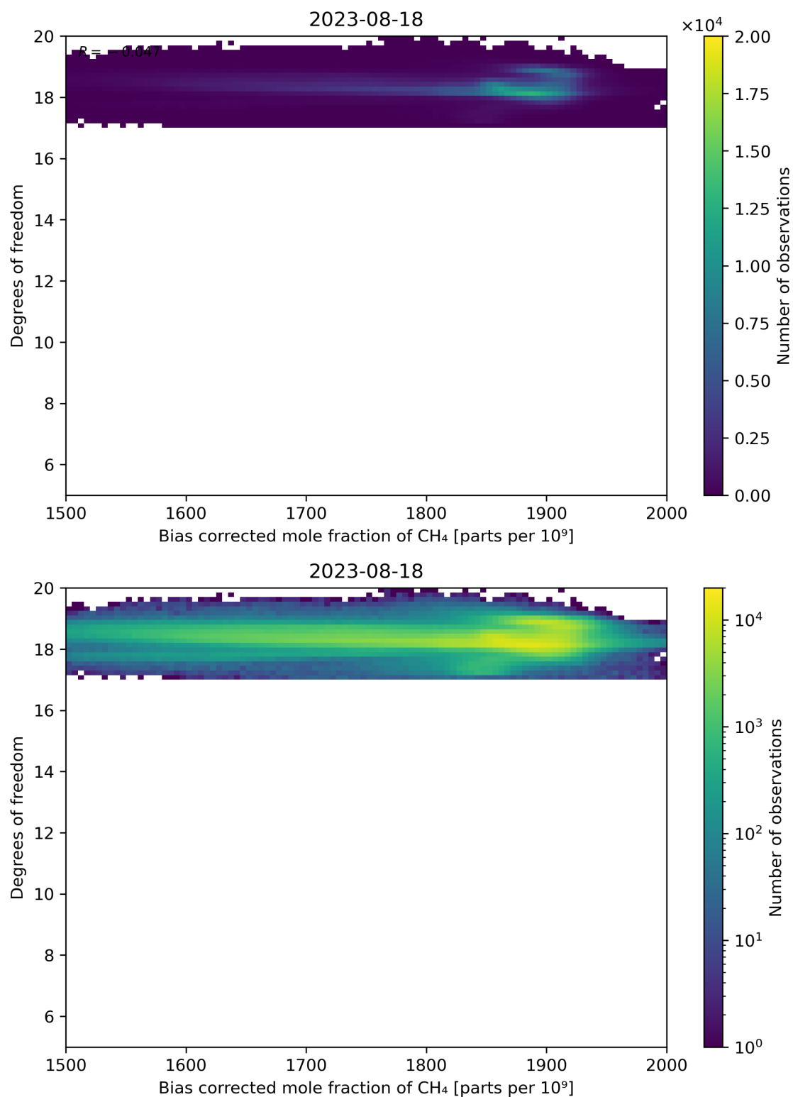
Figure 65: Scatter density plot of “Bias corrected mole fraction of CH 4 ” against “Degrees of freedom” for 2023-08-17 to 2023-08-19.
