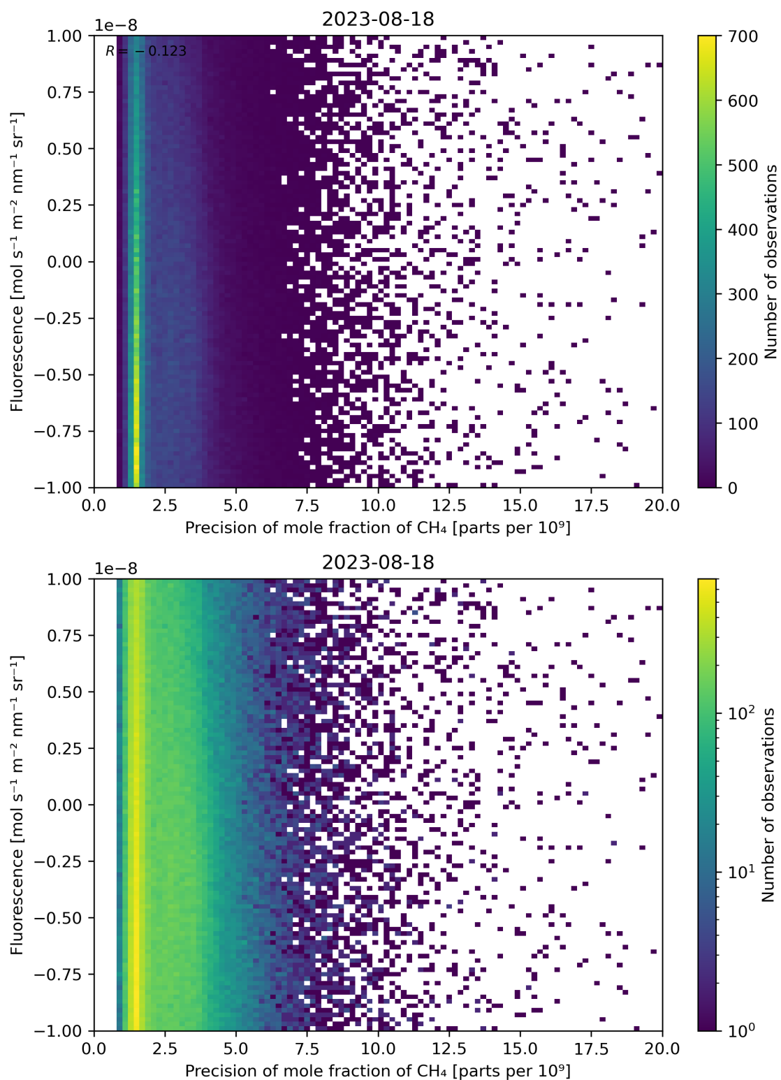
Figure 81: Scatter density plot of “Precision of mole fraction of \text{CH}_4 ” against “Fluorescence” for 2023-08-17 to 2023-08-19.
