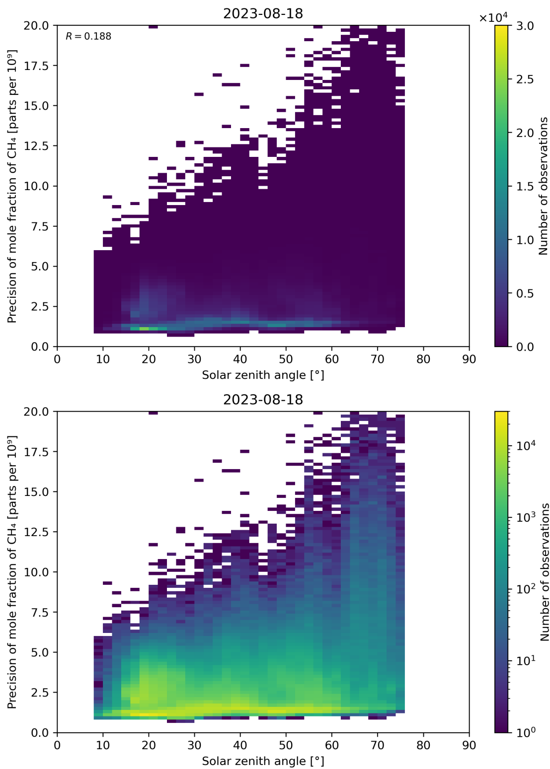
Figure 101: Scatter density plot of “Solar zenith angle” against “Precision of mole fraction of CH 4 ” for 2023-08-17 to 2023-08-19.
