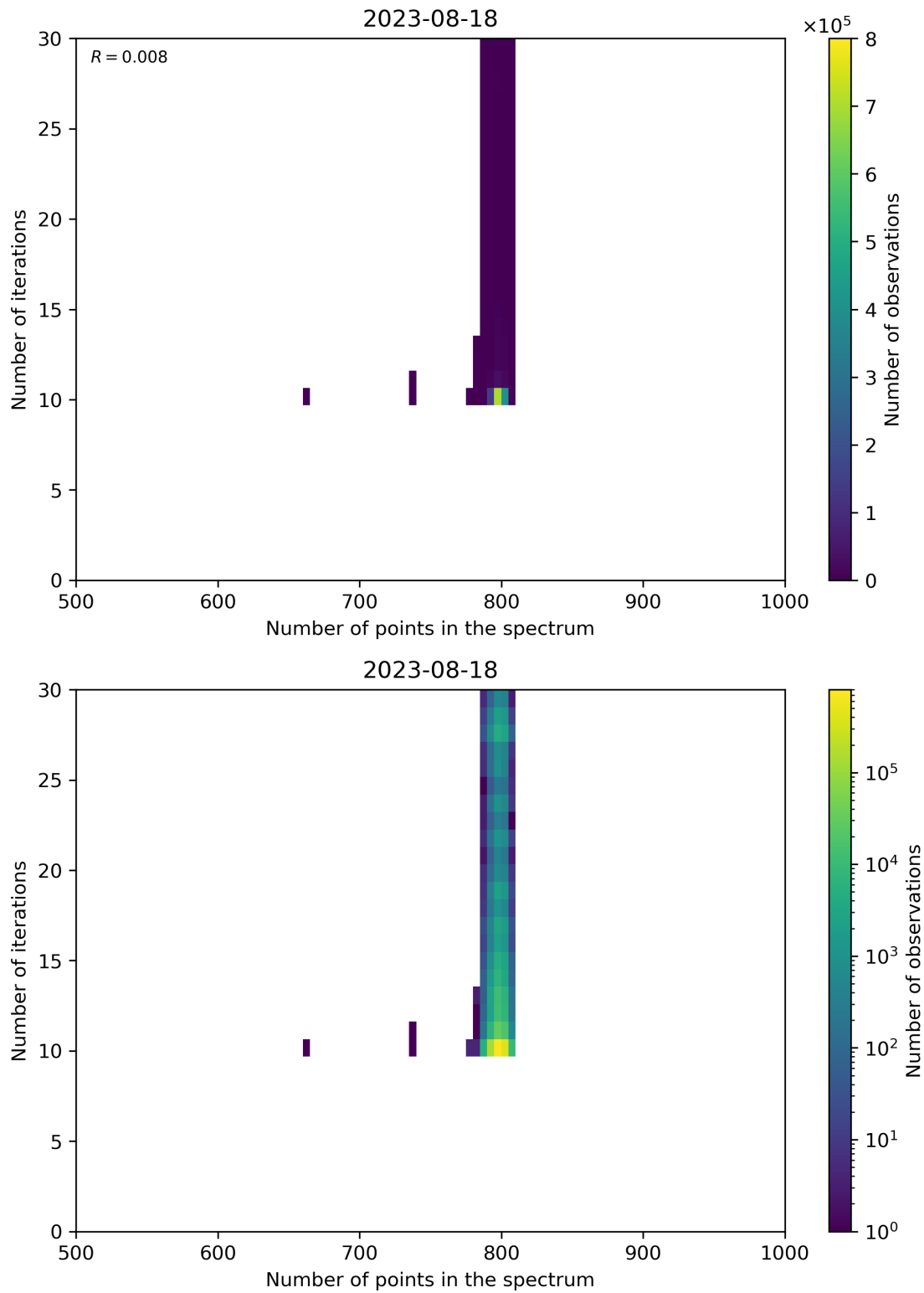
Figure 92: Scatter density plot of “Number of points in the spectrum” against “Number of iterations” for 2023-08-17 to 2023-08-19.
