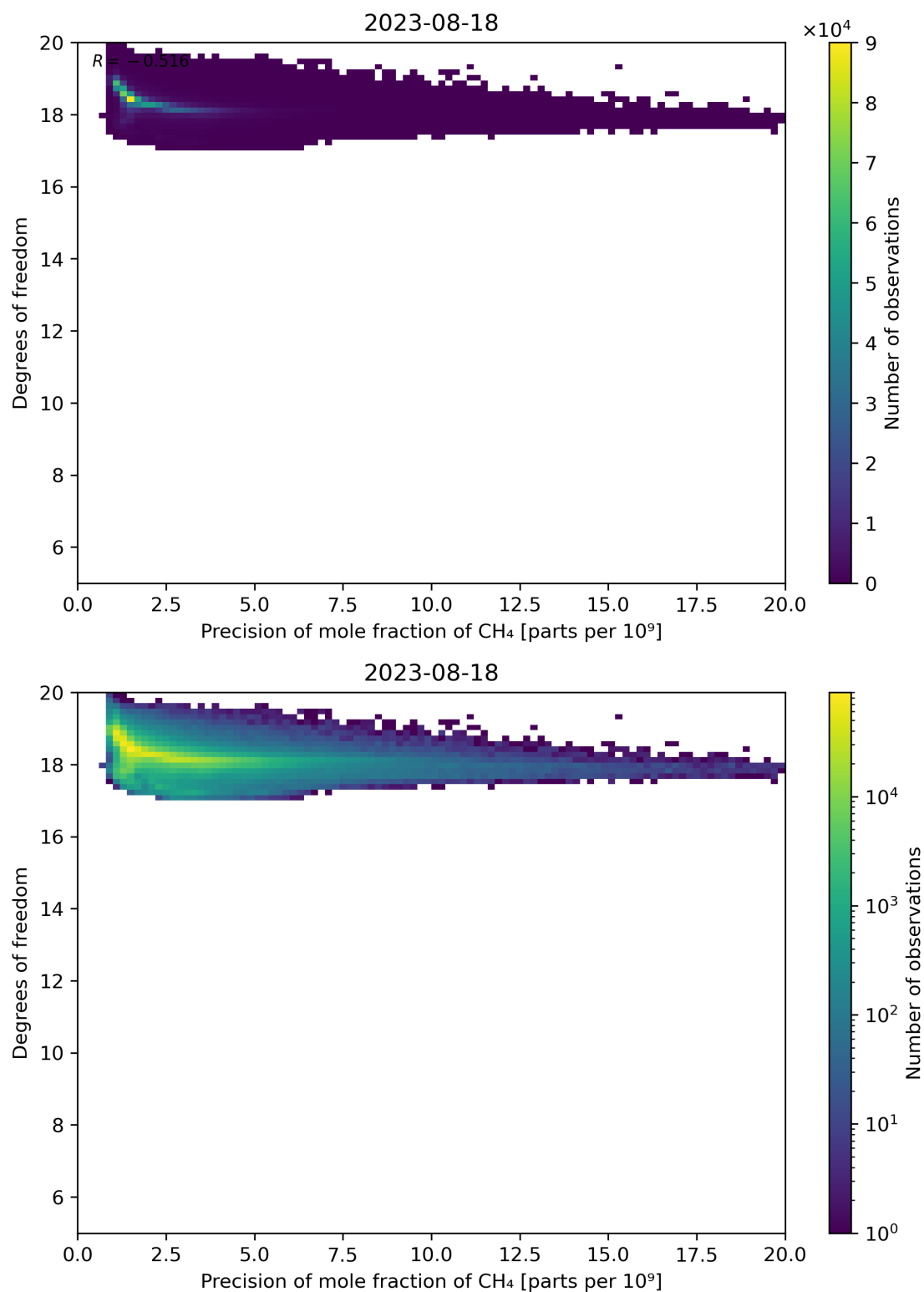
Figure 80: Scatter density plot of “Precision of mole fraction of CH 4 ” against “Degrees of freedom” for 2023-08-17 to 2023-08-19.
