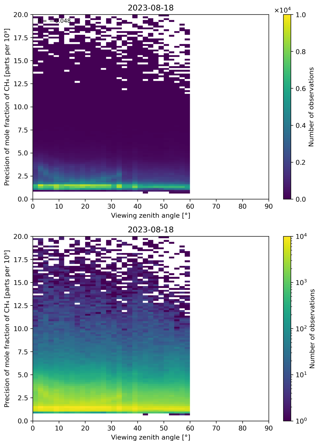
Figure 112: Scatter density plot of “Viewing zenith angle” against “Precision of mole fraction of CH 4 ” for 2023-08-17 to 2023-08-19.
