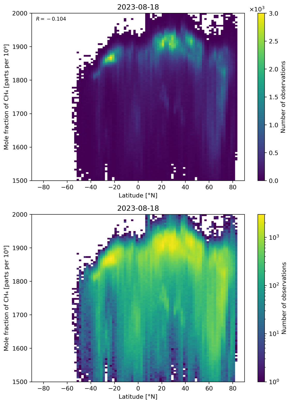
Figure 57: Scatter density plot of “Latitude” against “Mole fraction of CH 4 ” for 2023-08-17 to 2023-08-19.
