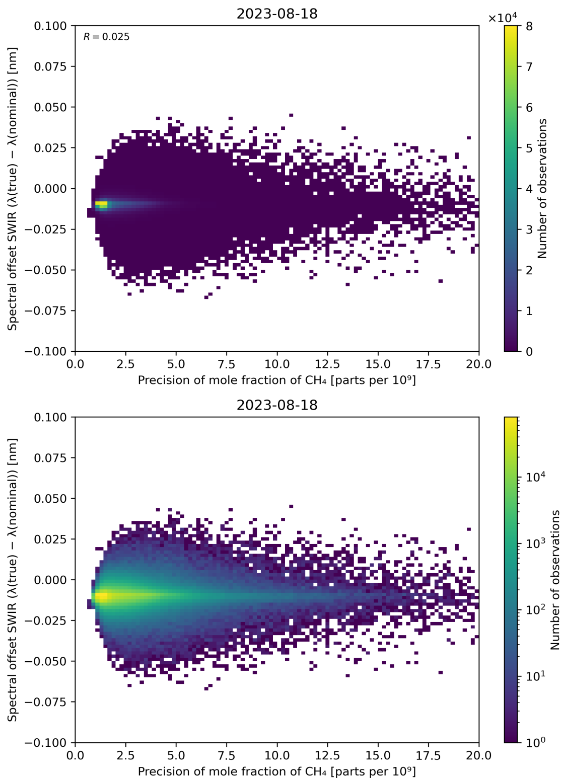
Figure 85: Scatter density plot of “Precision of mole fraction of CH 4 ” against “Spectral offset SWIR ( \lambda(\text{true}) - \lambda(\text{nominal}) )” for 2023-08-17 to 2023-08-19.
