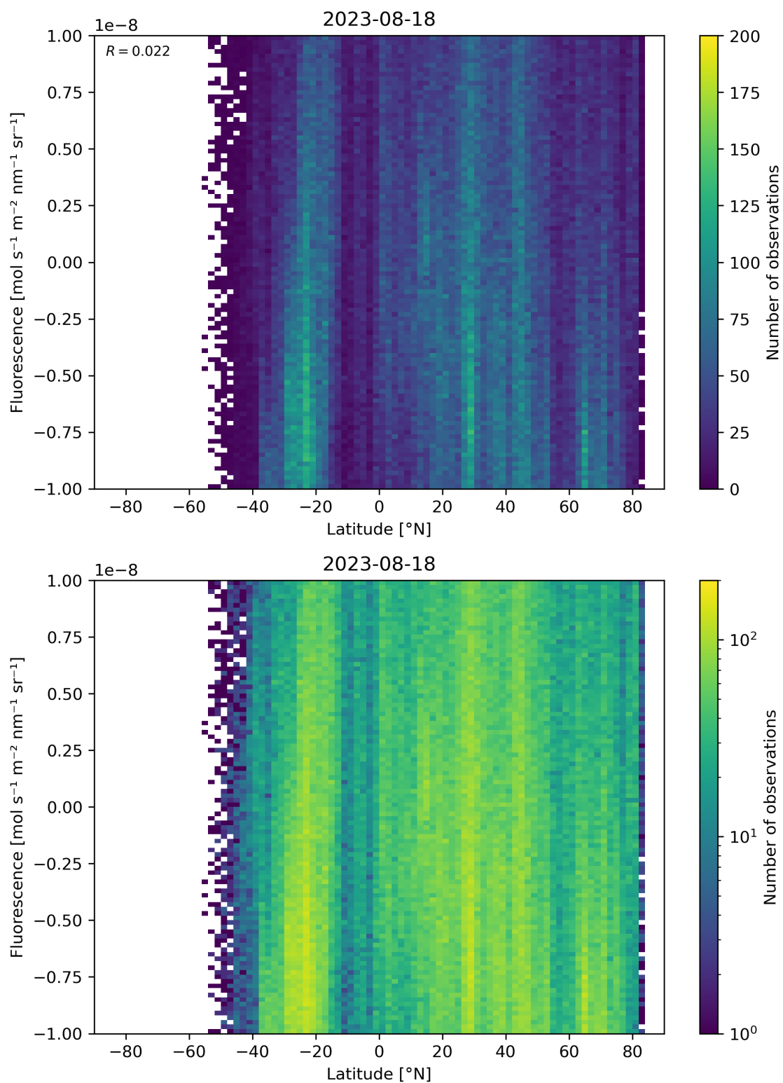
Figure 56: Scatter density plot of “Latitude” against “Fluorescence” for 2023-08-17 to 2023-08-19.
