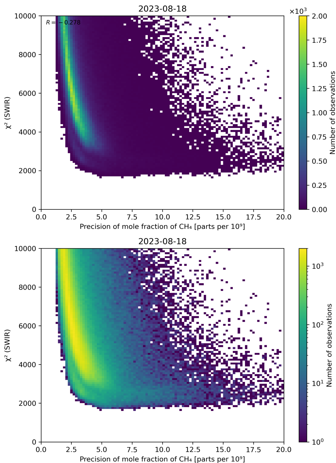
Figure 79: Scatter density plot of “Precision of mole fraction of \text{CH}_4 ” against “ \chi^2 (SWIR)” for 2023-08-17 to 2023-08-19.
