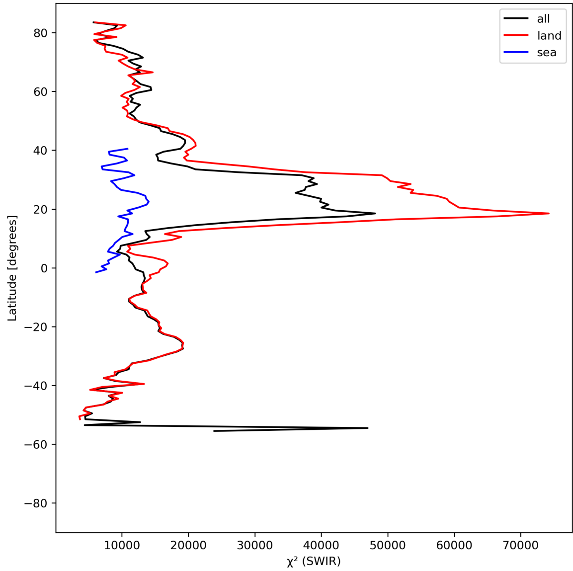
Figure 17: Zonal average of “ \chi^2 (SWIR)” for 2023-08-17 to 2023-08-19.
