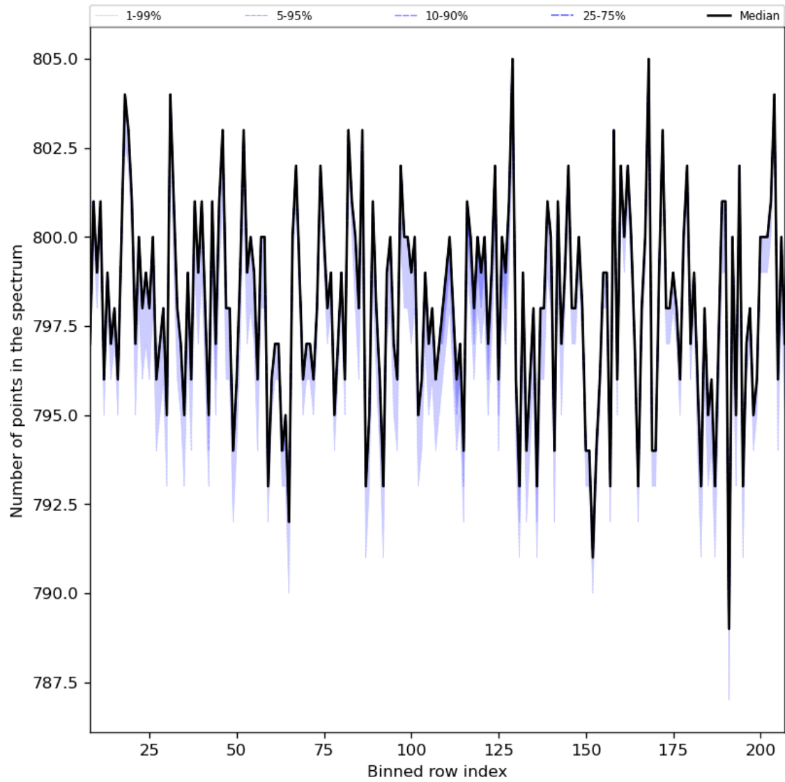
Figure 37: Along track statistics of “Number of points in the spectrum” for 2023-08-17 to 2023-08-19
