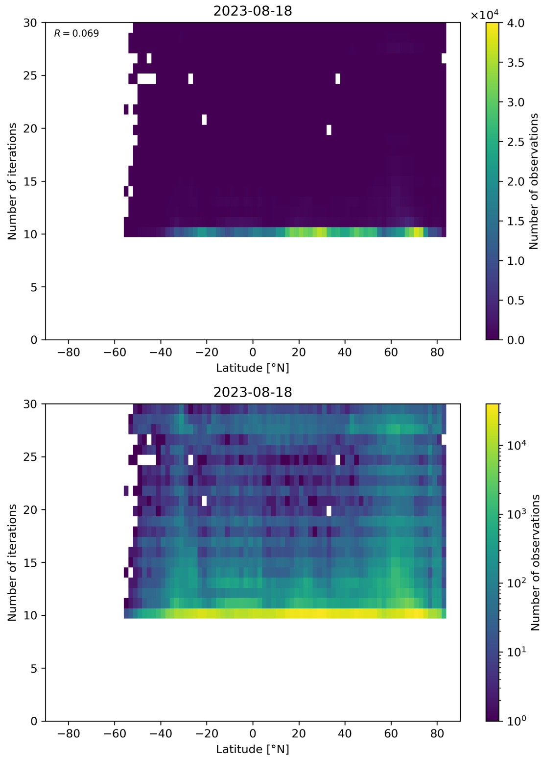
Figure 60: Scatter density plot of “Latitude” against “Number of iterations” for 2023-08-17 to 2023-08-19.
