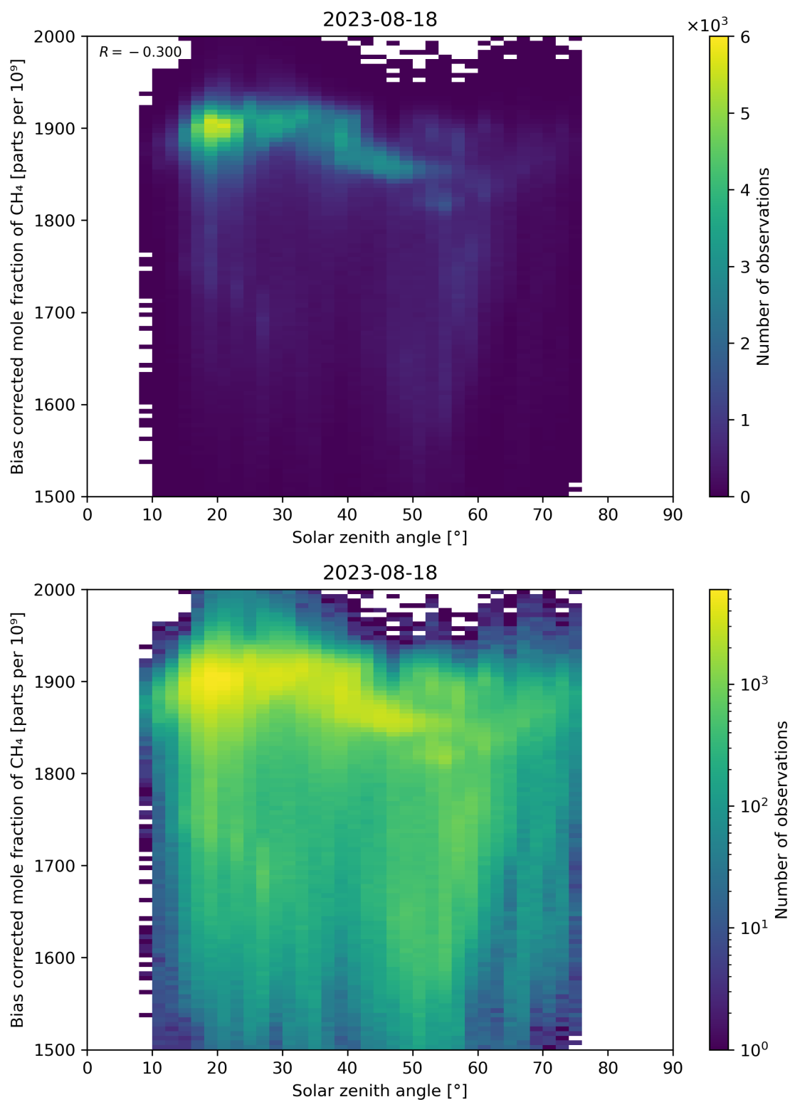
Figure 100: Scatter density plot of “Solar zenith angle” against “Bias corrected mole fraction of CH 4 ” for 2023-08-17 to 2023-08-19.
