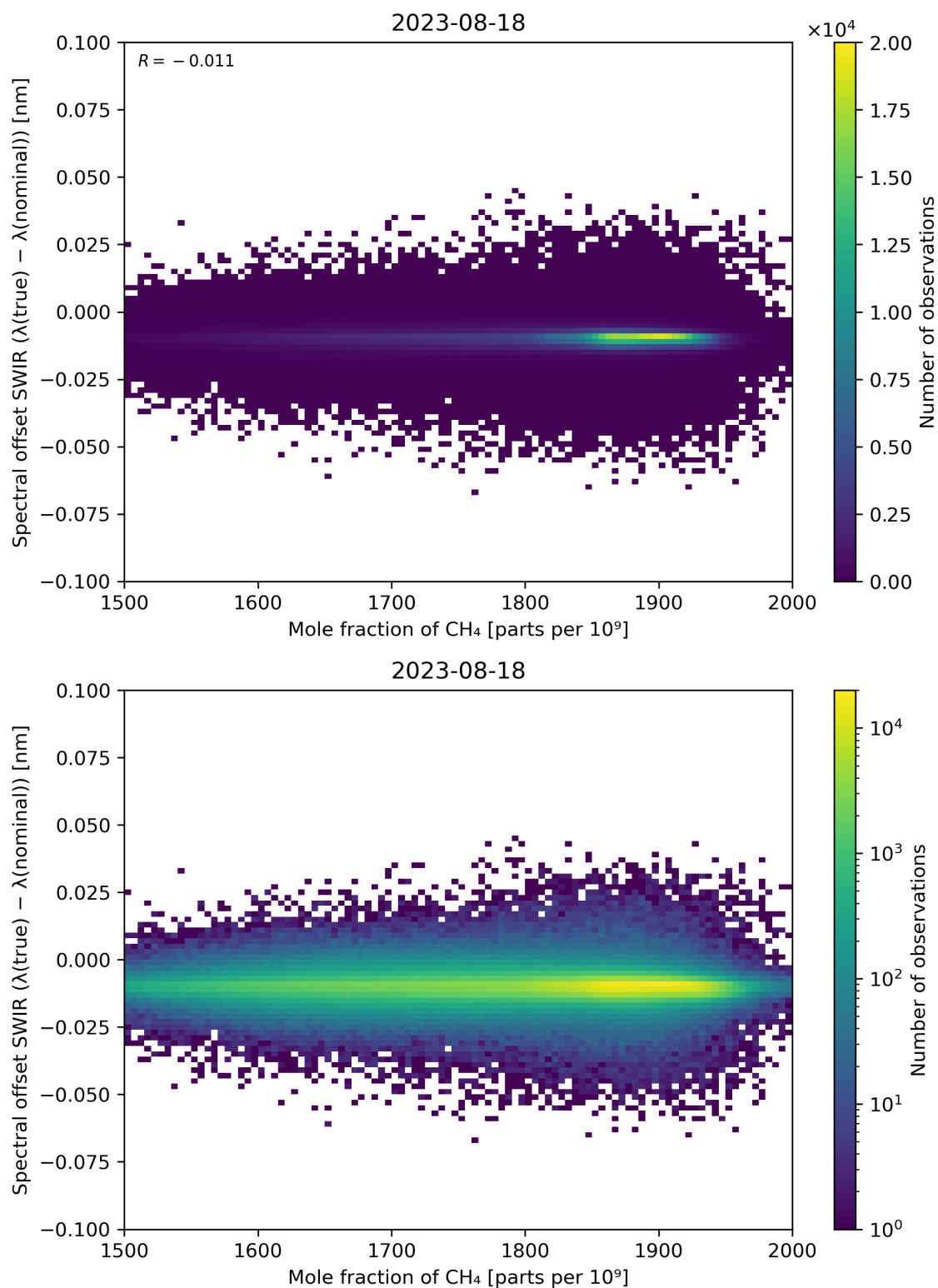
Figure 86: Scatter density plot of “Mole fraction of CH 4 ” against “Spectral offset SWIR ( \lambda(\text{true}) - \lambda(\text{nominal}) )” for 2023-08-17 to 2023-08-19.
