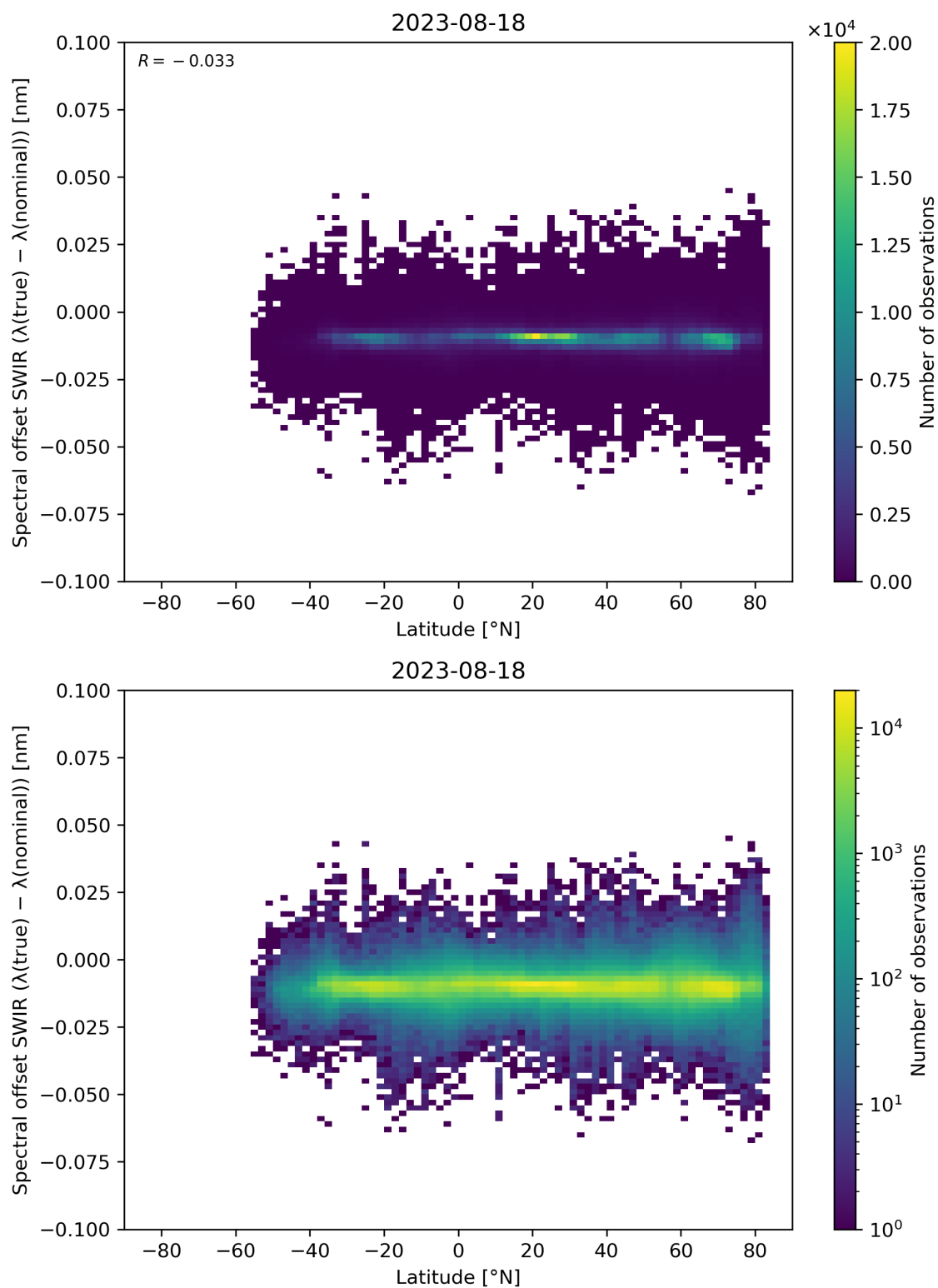
Figure 62: Scatter density plot of “Latitude” against “Spectral offset SWIR ( \lambda(\text{true}) - \lambda(\text{nominal}) )” for 2023-08-17 to 2023-08-19.
