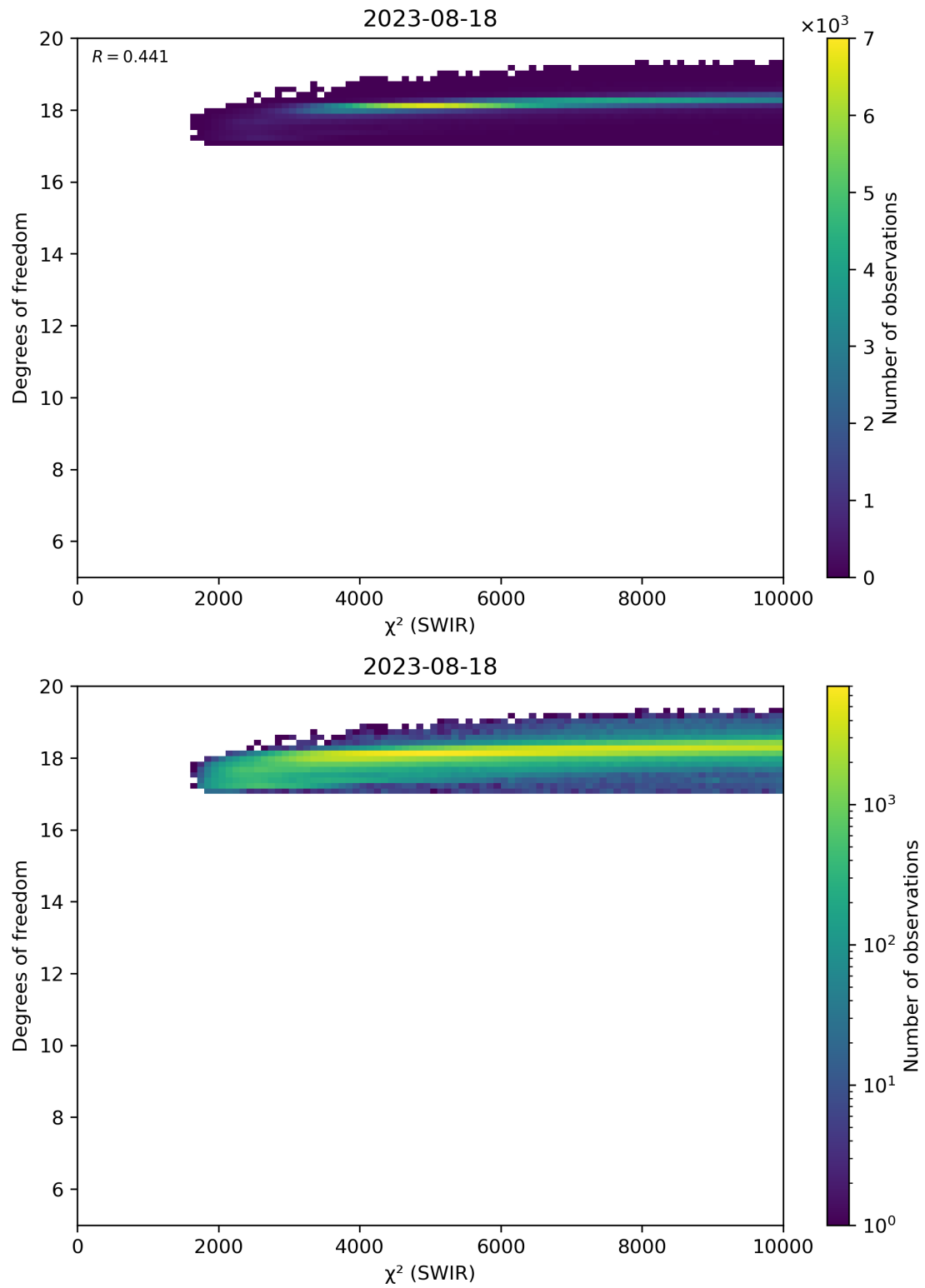
Figure 48: Scatter density plot of “ \chi^2 (SWIR)” against “Degrees of freedom” for 2023-08-17 to 2023-08-19.
