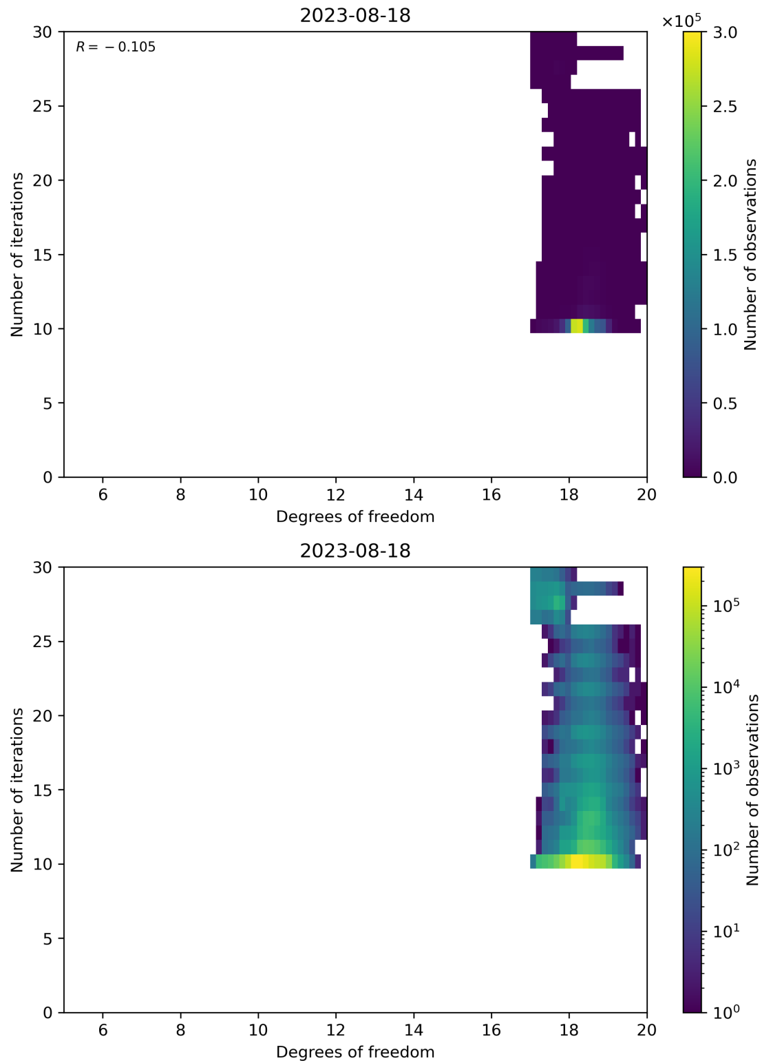
Figure 52: Scatter density plot of “Degrees of freedom” against “Number of iterations” for 2023-08-17 to 2023-08-19.
