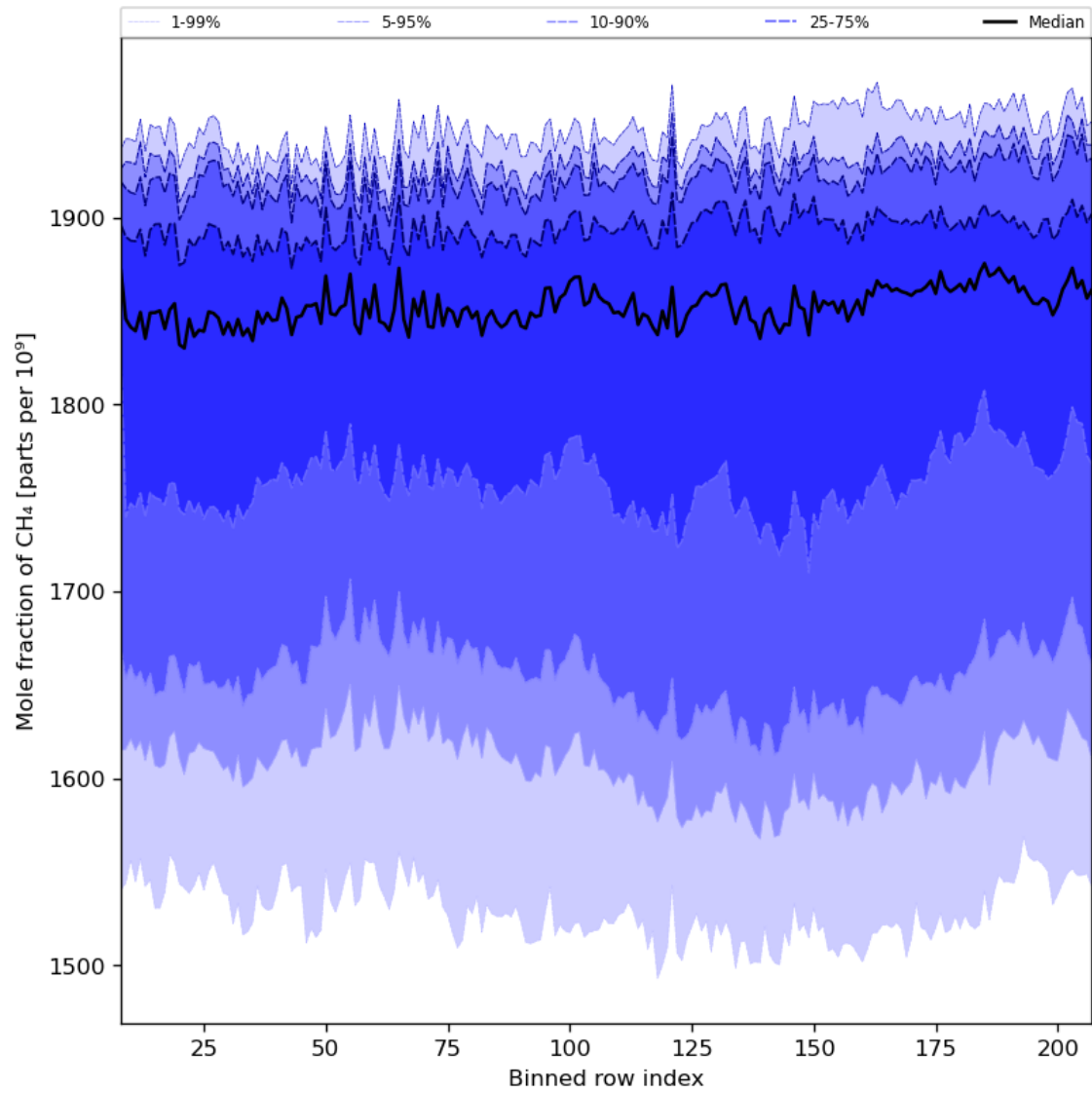
Figure 34: Along track statistics of “Mole fraction of CH 4 ” for 2023-08-17 to 2023-08-19
