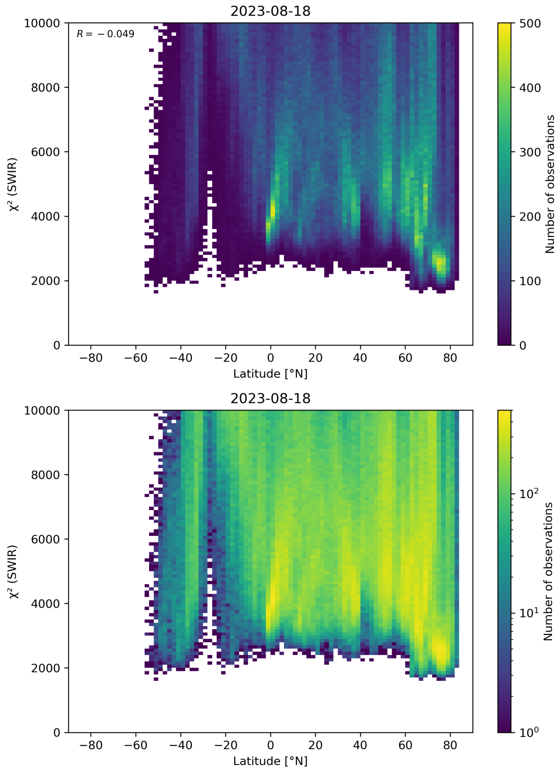
Figure 54: Scatter density plot of “Latitude” against “ \chi^2 (SWIR)” for 2023-08-17 to 2023-08-19.
