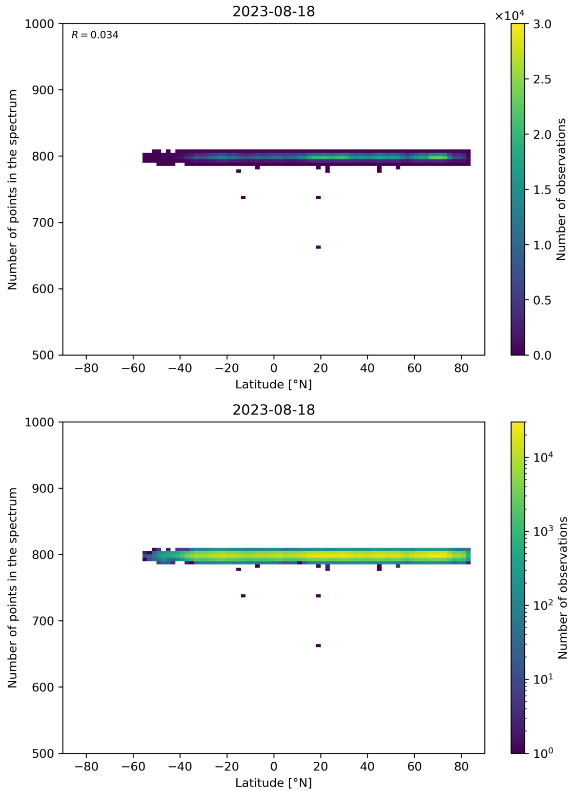
Figure 61: Scatter density plot of “Latitude” against “Number of points in the spectrum” for 2023-08-17 to 2023-08-19.
