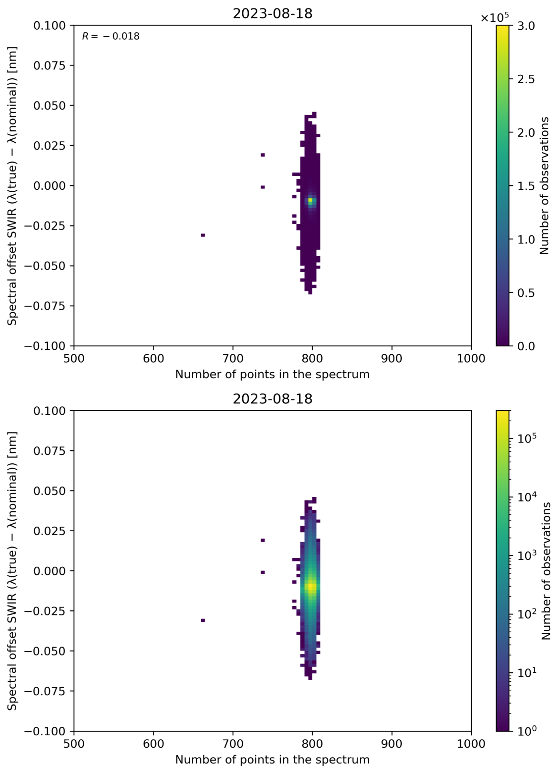
Figure 93: Scatter density plot of “Number of points in the spectrum” against “Spectral offset SWIR ( \lambda(\text{true}) - \lambda(\text{nominal}) )” for 2023-08-17 to 2023-08-19.
