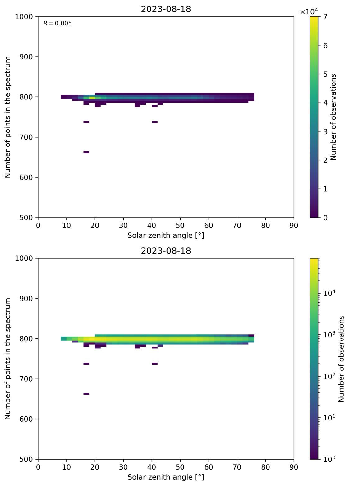
Figure 103: Scatter density plot of “Solar zenith angle” against “Number of points in the spectrum” for 2023-08-17 to 2023-08-19.
