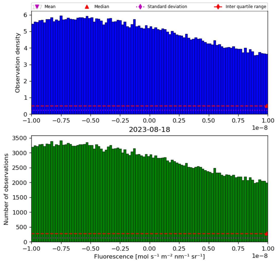
Figure 32: Histogram of “Fluorescence” for 2023-08-17 to 2023-08-19
