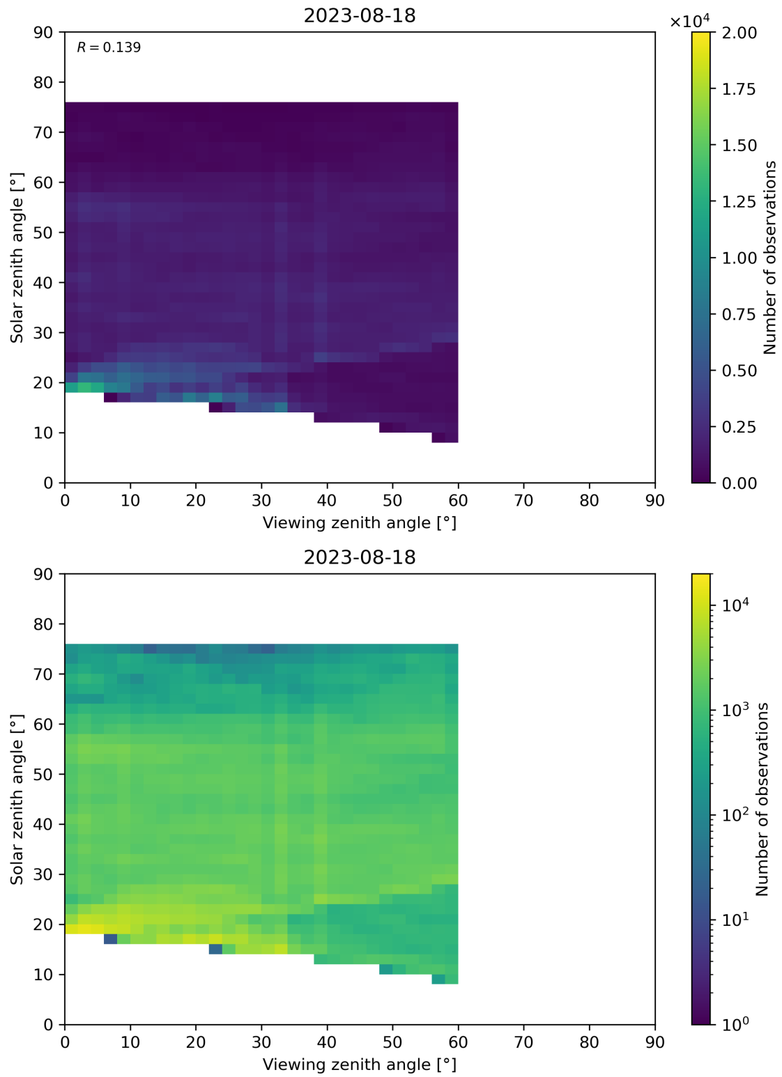
Figure 115: Scatter density plot of “Viewing zenith angle” against “Solar zenith angle” for 2023-08-17 to 2023-08-19.
