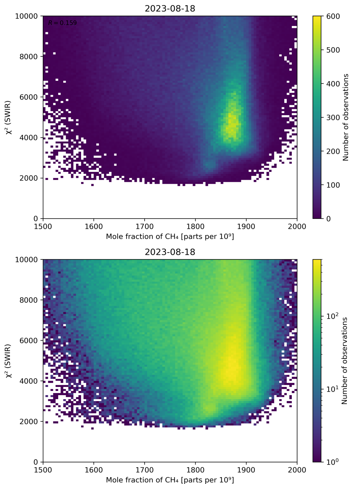
Figure 71: Scatter density plot of “Mole fraction of \text{CH}_4 ” against “ \chi^2 (SWIR)” for 2023-08-17 to 2023-08-19.
