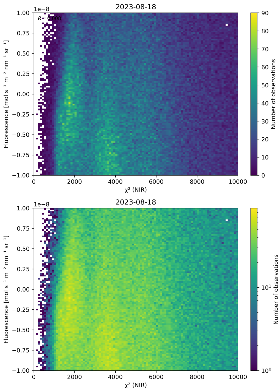
Figure 45: Scatter density plot of “ \chi^2 (NIR)” against “Fluorescence” for 2023-08-17 to 2023-08-19.
