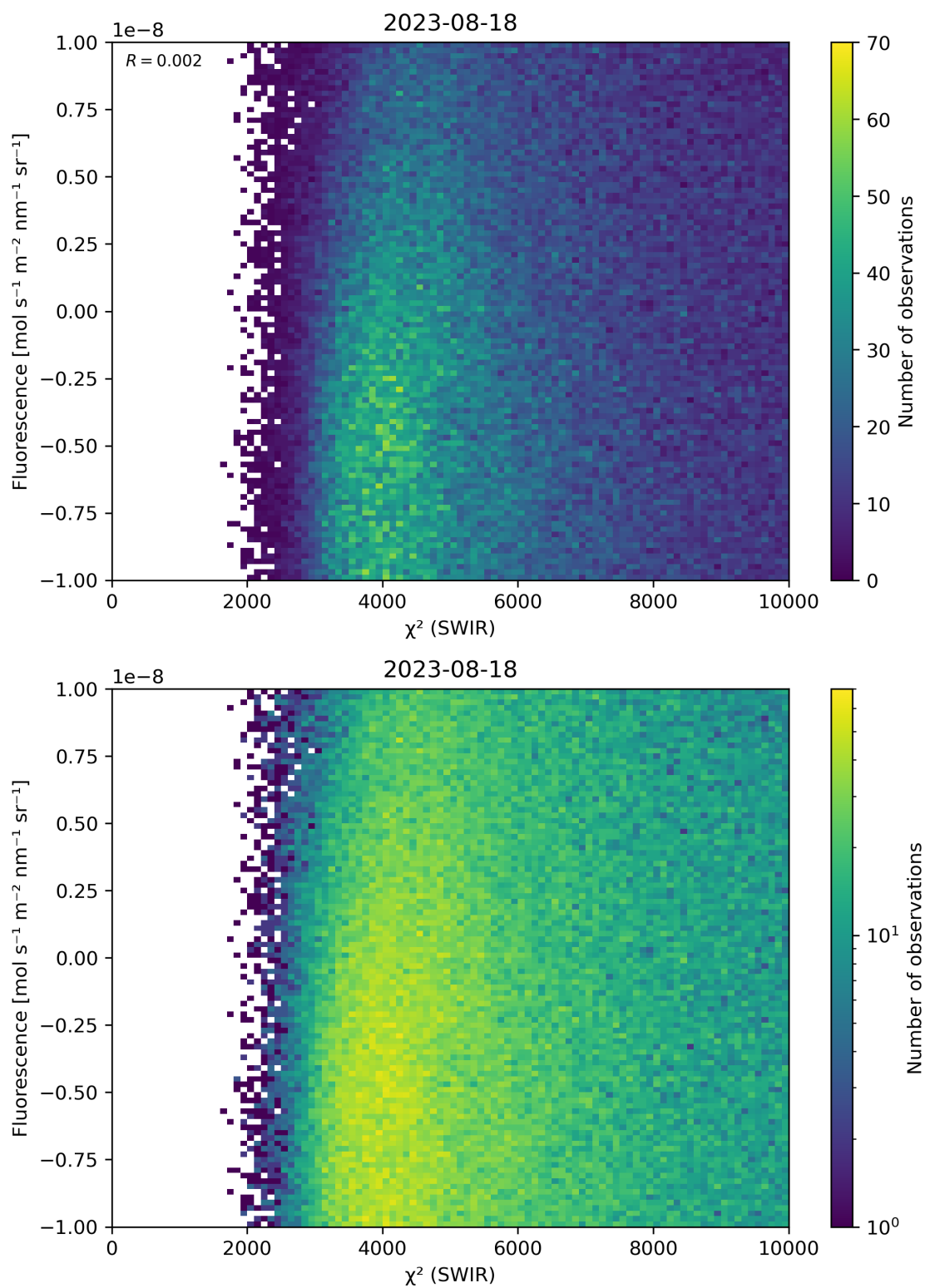
Figure 49: Scatter density plot of “ \chi^2 (SWIR)” against “Fluorescence” for 2023-08-17 to 2023-08-19.
