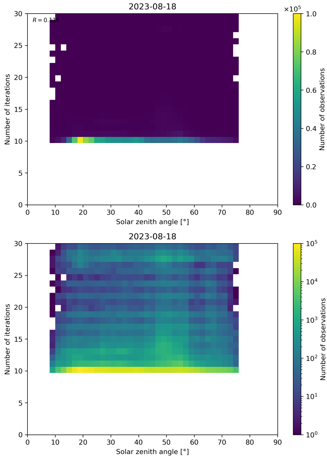
Figure 102: Scatter density plot of “Solar zenith angle” against “Number of iterations” for 2023-08-17 to 2023-08-19.
