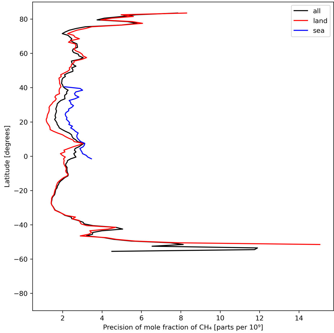
Figure 13: Zonal average of “Precision of mole fraction of CH 4 ” for 2023-08-17 to 2023-08-19.
