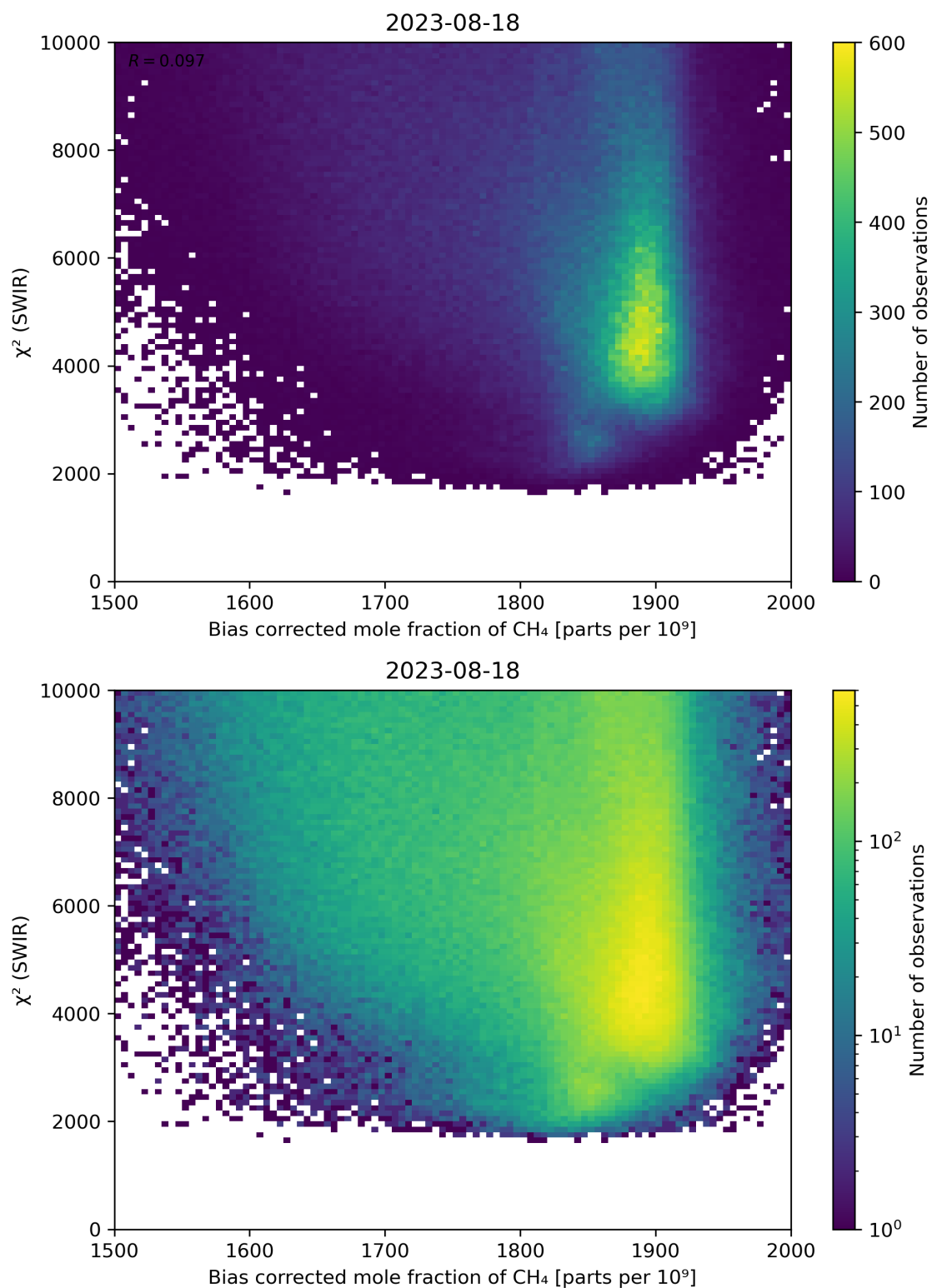
Figure 64: Scatter density plot of “Bias corrected mole fraction of CH 4 ” against “ \chi^2 (SWIR)” for 2023-08-17 to 2023-08-19.
