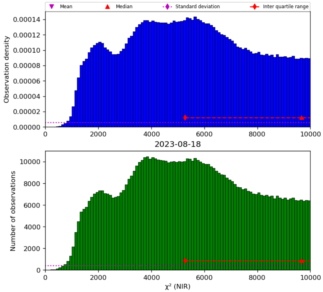
Figure 29: Histogram of " \chi^2 (NIR)" for 2023-08-17 to 2023-08-19
