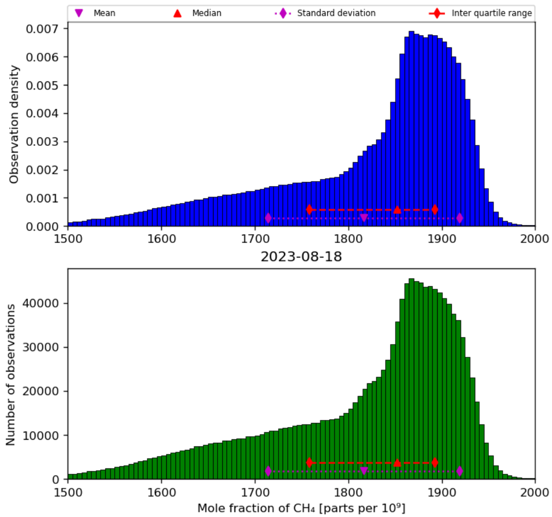
Figure 23: Histogram of “Mole fraction of CH 4 ” for 2023-08-17 to 2023-08-19
