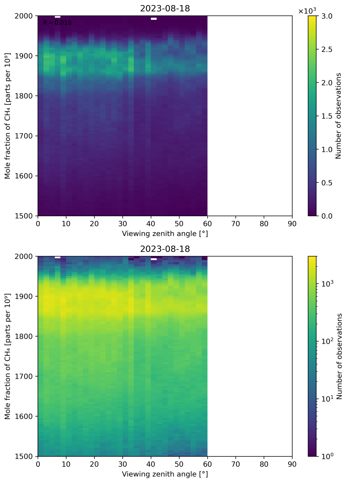
Figure 110: Scatter density plot of “Viewing zenith angle” against “Mole fraction of CH 4 ” for 2023-08-17 to 2023-08-19.
