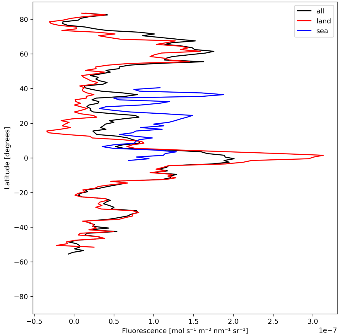
Figure 21: Zonal average of “Fluorescence” for 2023-08-17 to 2023-08-19.
