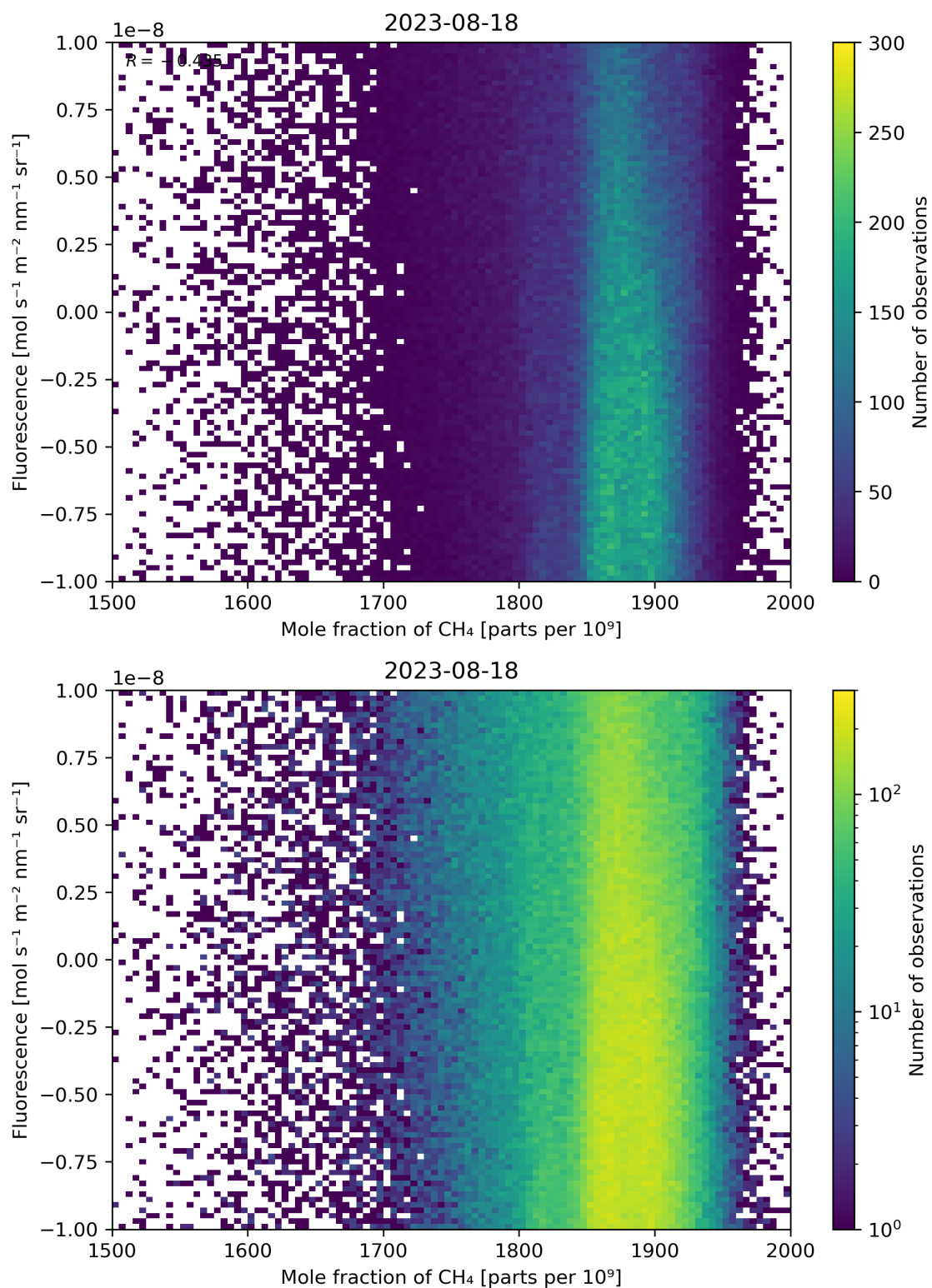
Figure 73: Scatter density plot of “Mole fraction of \text{CH}_4 ” against “Fluorescence” for 2023-08-17 to 2023-08-19.
