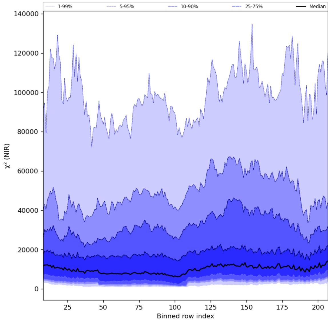
Figure 40: Along track statistics of “ \chi^2 (NIR)” for 2023-08-17 to 2023-08-19
