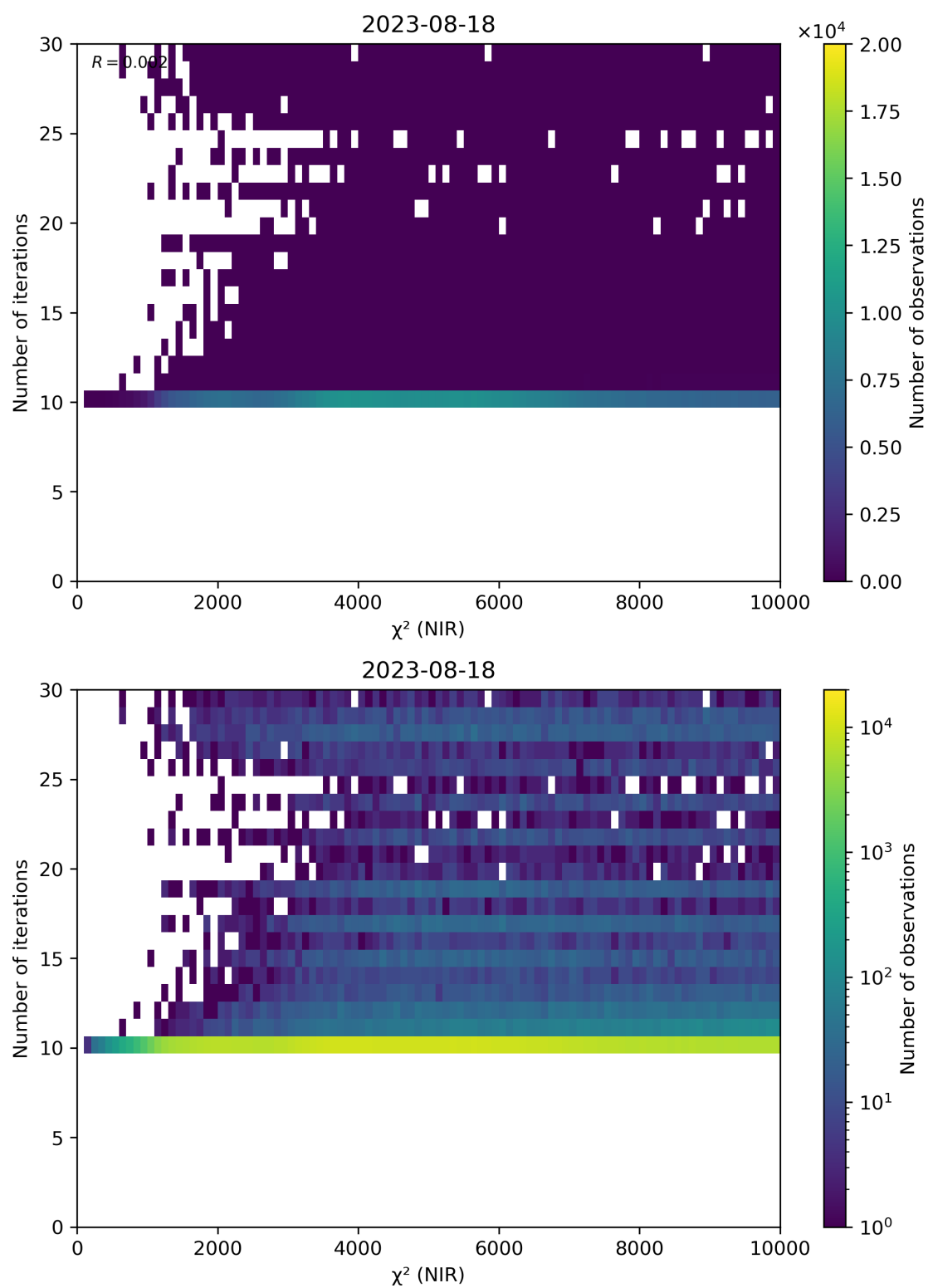
Figure 46: Scatter density plot of “ \chi^2 (NIR)” against “Number of iterations” for 2023-08-17 to 2023-08-19.
