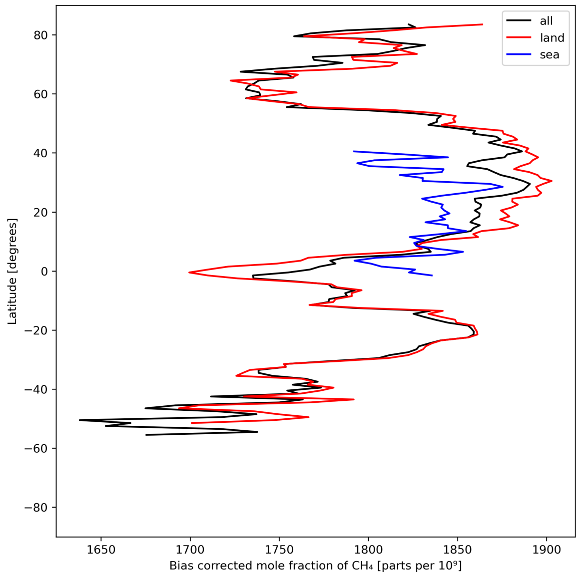
Figure 14: Zonal average of “Bias corrected mole fraction of \text{CH}_4 ” for 2023-08-17 to 2023-08-19.
