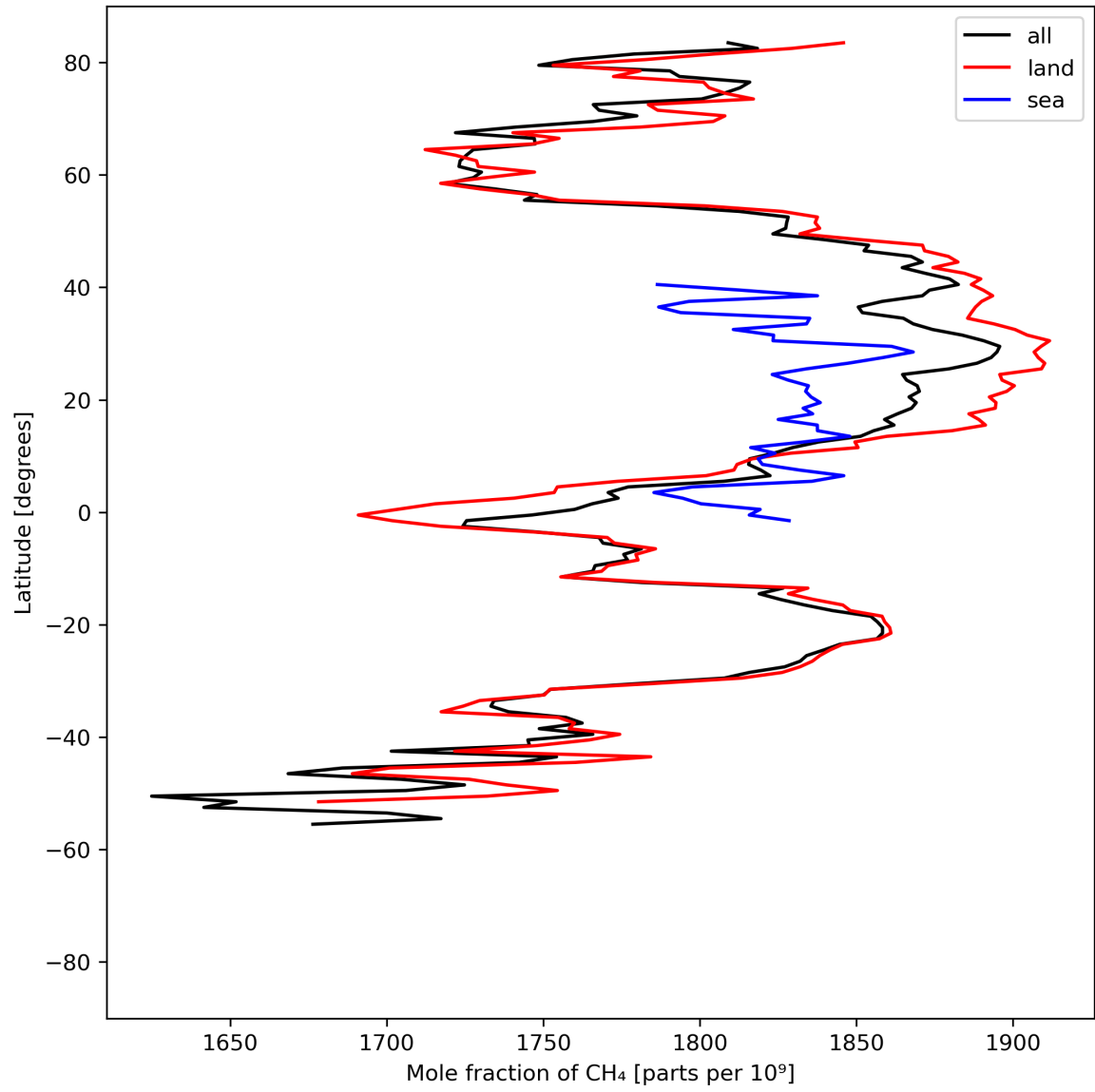
Figure 12: Zonal average of “Mole fraction of \text{CH}_4 ” for 2023-08-17 to 2023-08-19.
