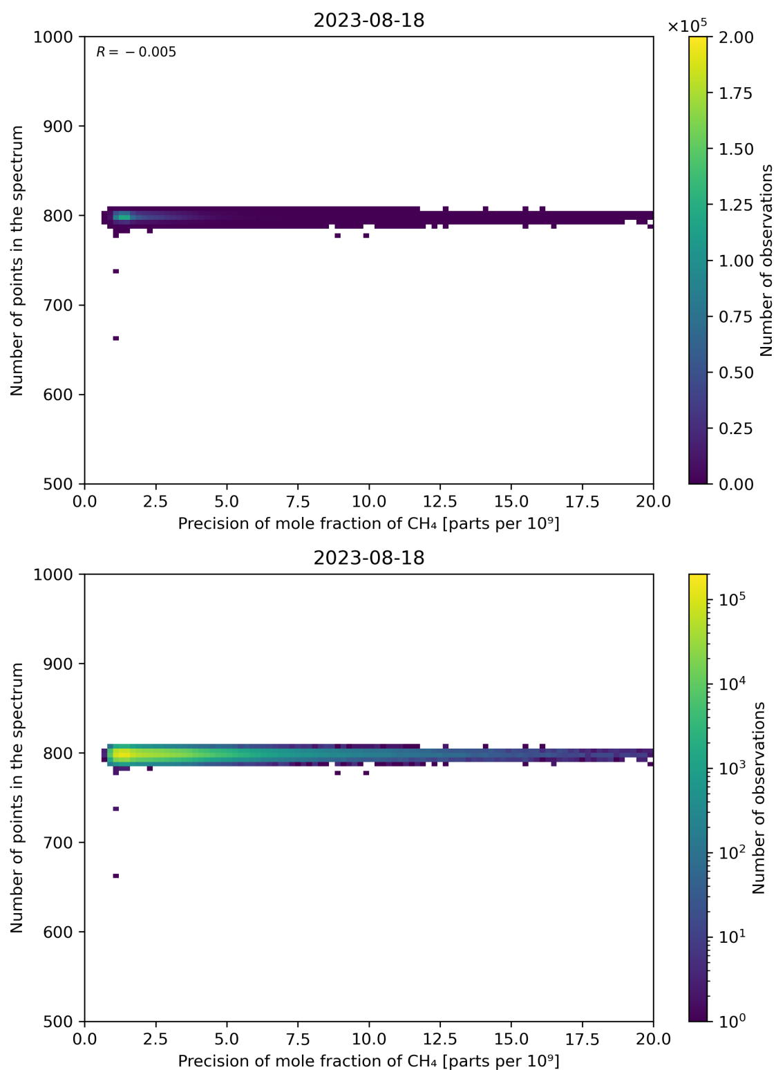
Figure 84: Scatter density plot of “Precision of mole fraction of \text{CH}_4 ” against “Number of points in the spectrum” for 2023-08-17 to 2023-08-19.
