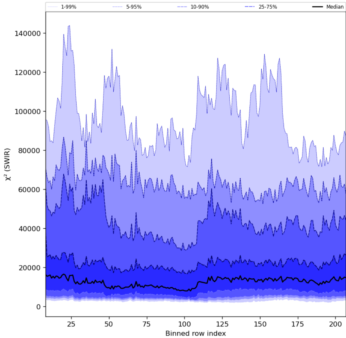
Figure 39: Along track statistics of “ \chi^2 (SWIR)” for 2023-08-17 to 2023-08-19
