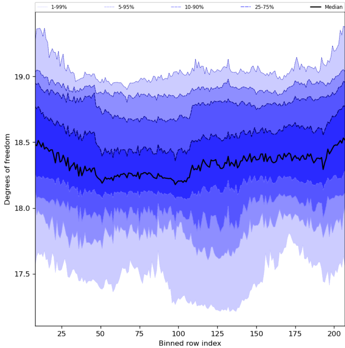
Figure 41: Along track statistics of “Degrees of freedom” for 2023-08-17 to 2023-08-19
