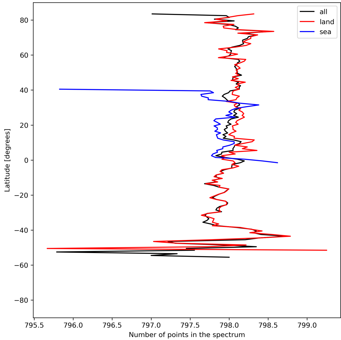
Figure 15: Zonal average of “Number of points in the spectrum” for 2023-08-17 to 2023-08-19.
