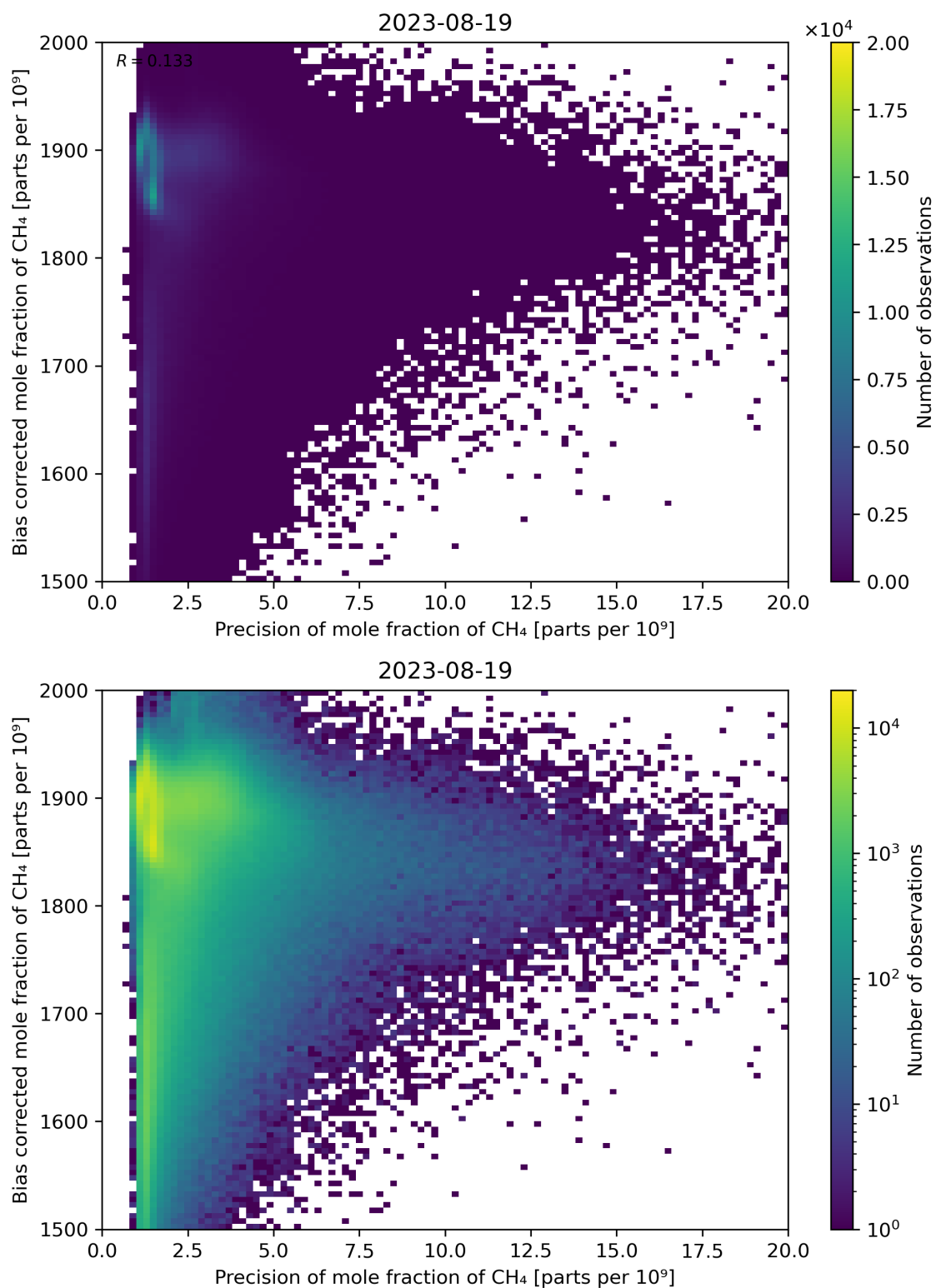
Figure 82: Scatter density plot of “Precision of mole fraction of CH 4 ” against “Bias corrected mole fraction of CH 4 ” for 2023-08-18 to 2023-08-20.
