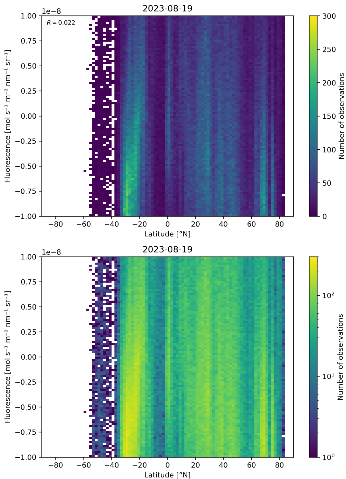
Figure 56: Scatter density plot of “Latitude” against “Fluorescence” for 2023-08-18 to 2023-08-20.
