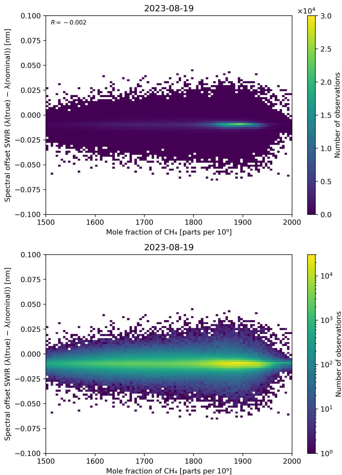
Figure 86: Scatter density plot of “Mole fraction of CH 4 ” against “Spectral offset SWIR ( \lambda(\text{true}) - \lambda(\text{nominal}) )” for 2023-08-18 to 2023-08-20.
