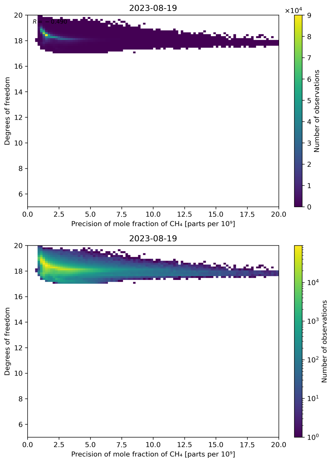
Figure 80: Scatter density plot of “Precision of mole fraction of CH 4 ” against “Degrees of freedom” for 2023-08-18 to 2023-08-20.
