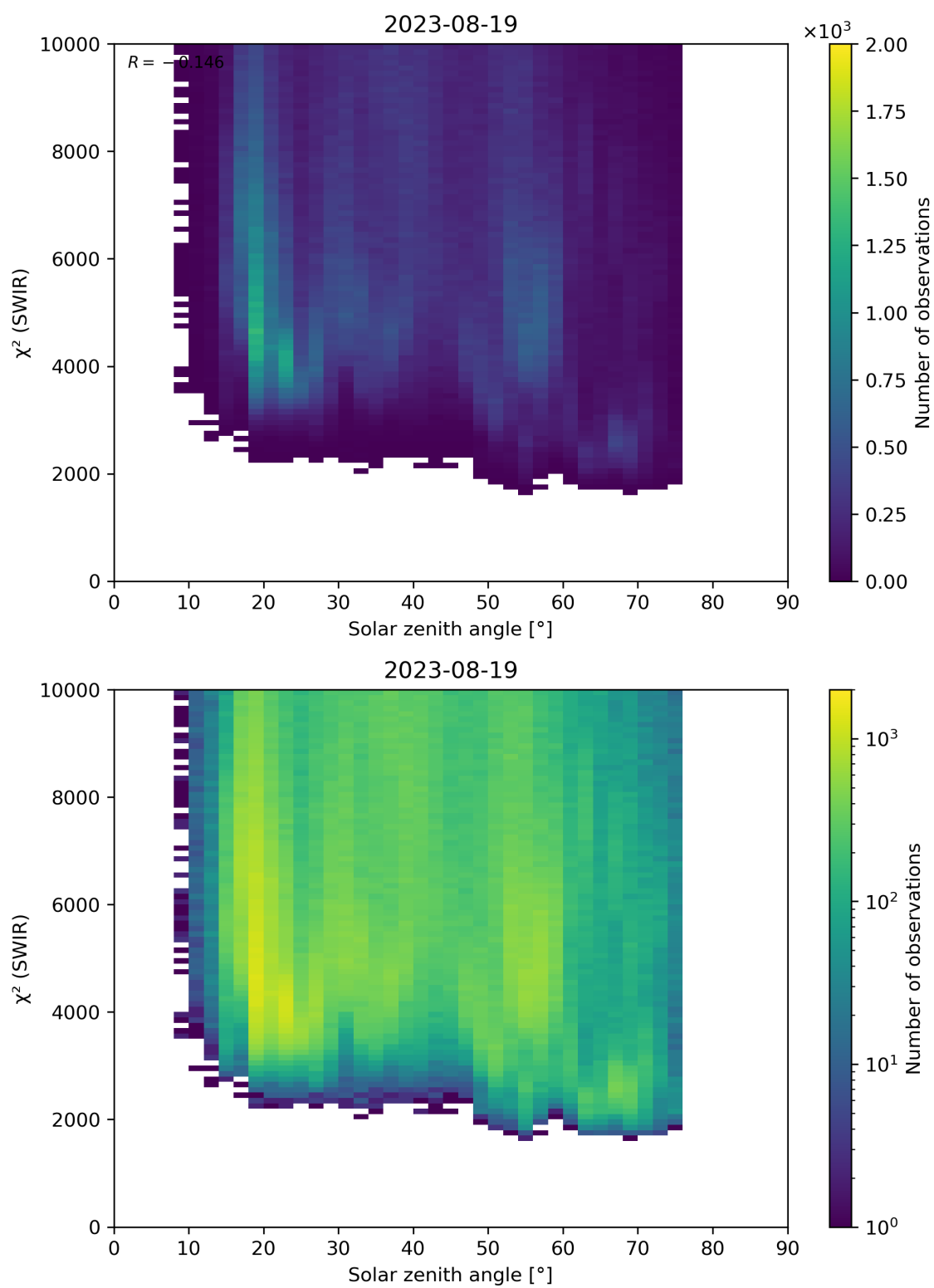
Figure 95: Scatter density plot of “Solar zenith angle” against “ \chi^2 (SWIR)” for 2023-08-18 to 2023-08-20.
