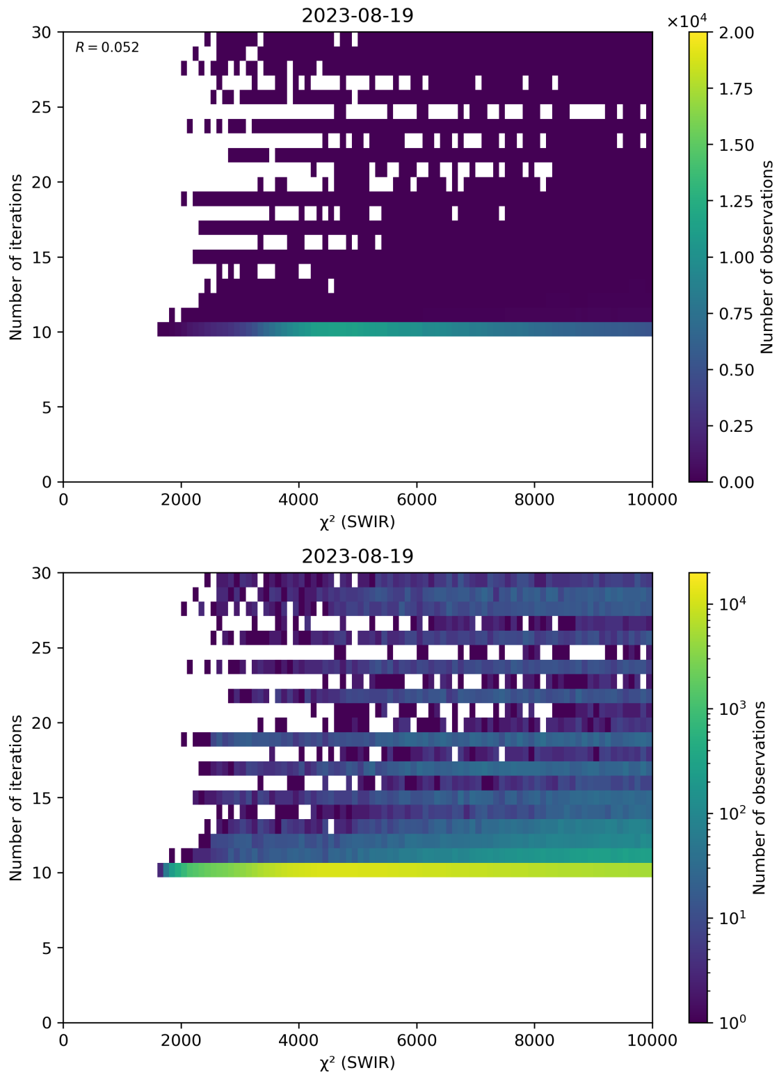
Figure 50: Scatter density plot of “ \chi^2 (SWIR)” against “Number of iterations” for 2023-08-18 to 2023-08-20.
