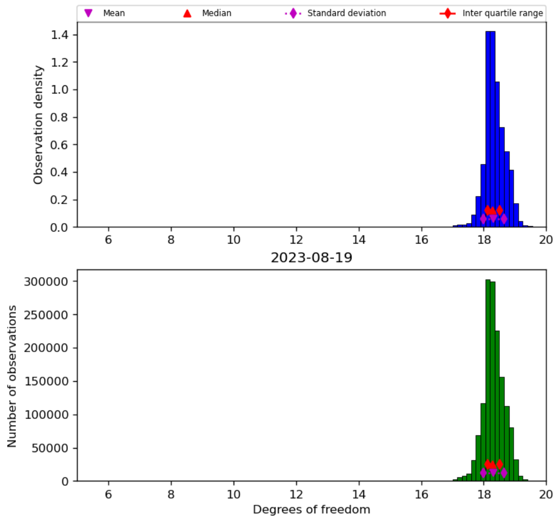
Figure 30: Histogram of “Degrees of freedom” for 2023-08-18 to 2023-08-20
