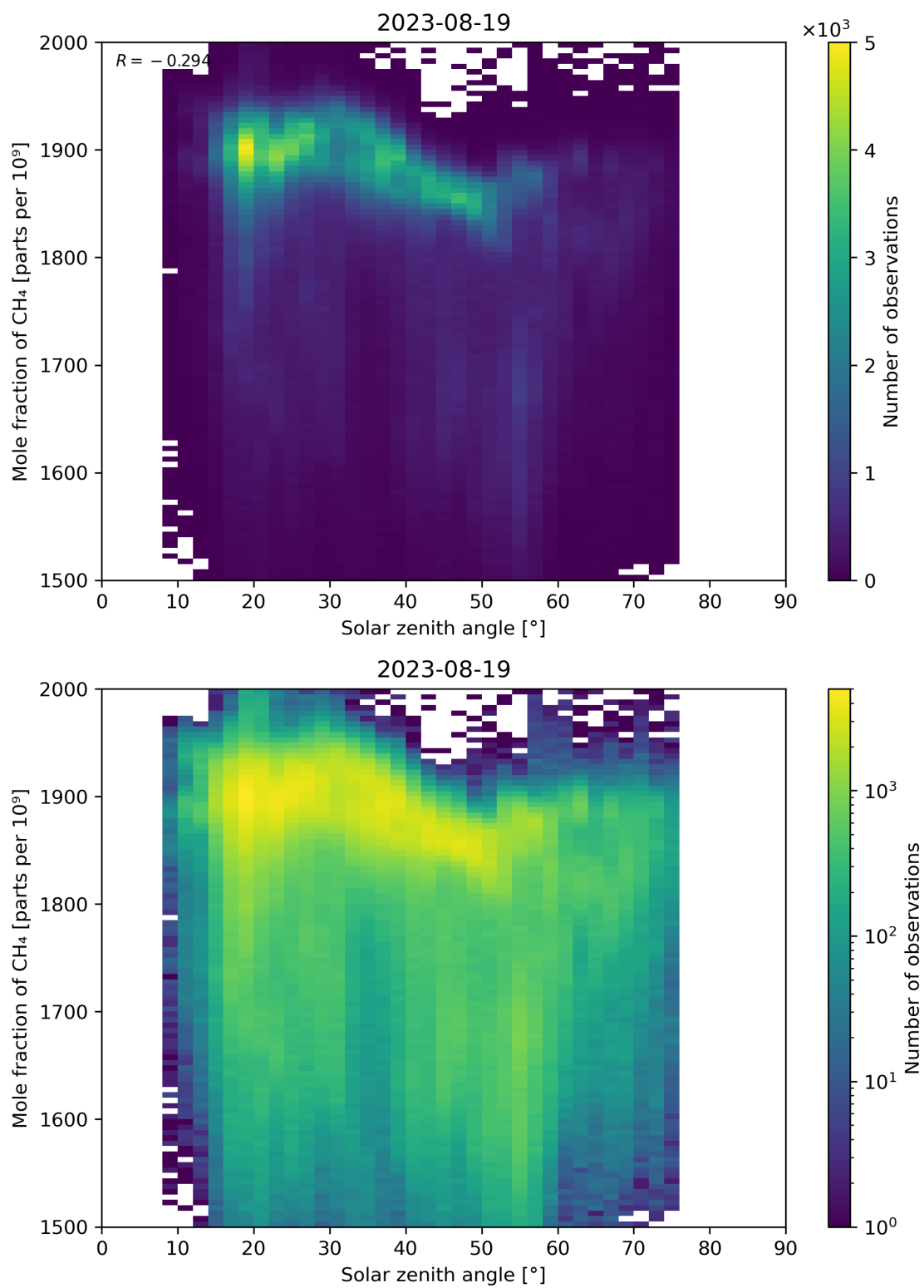
Figure 99: Scatter density plot of “Solar zenith angle” against “Mole fraction of CH 4 ” for 2023-08-18 to 2023-08-20.
