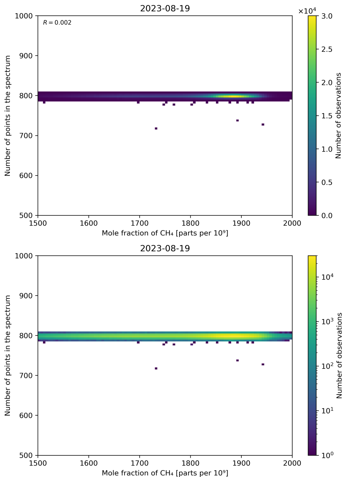
Figure 77: Scatter density plot of “Mole fraction of CH 4 ” against “Number of points in the spectrum” for 2023-08-18 to 2023-08-20.
