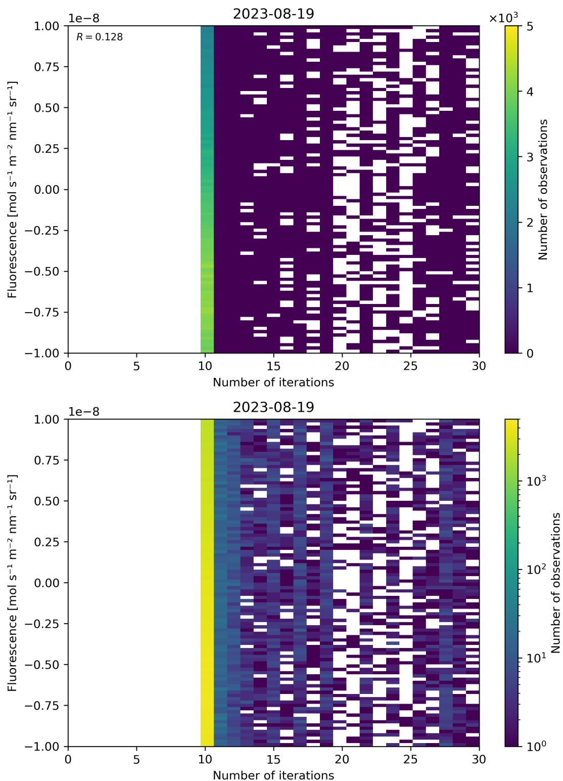
Figure 87: Scatter density plot of “Number of iterations” against “Fluorescence” for 2023-08-18 to 2023-08-20.
