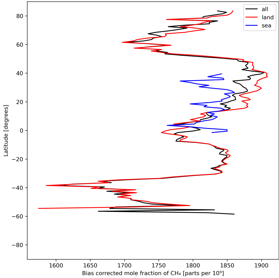
Figure 14: Zonal average of “Bias corrected mole fraction of CH 4 ” for 2023-08-18 to 2023-08-20.
