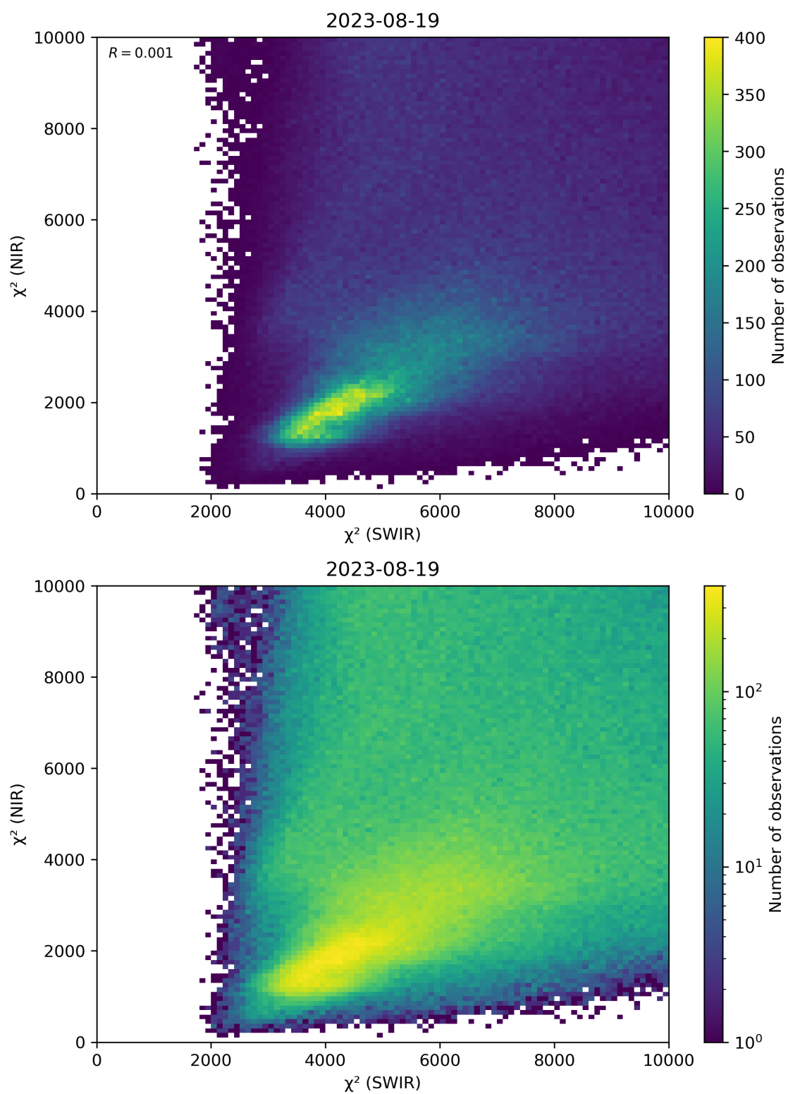
Figure 47: Scatter density plot of “ \chi^2 (SWIR)” against “ \chi^2 (NIR)” for 2023-08-18 to 2023-08-20.
