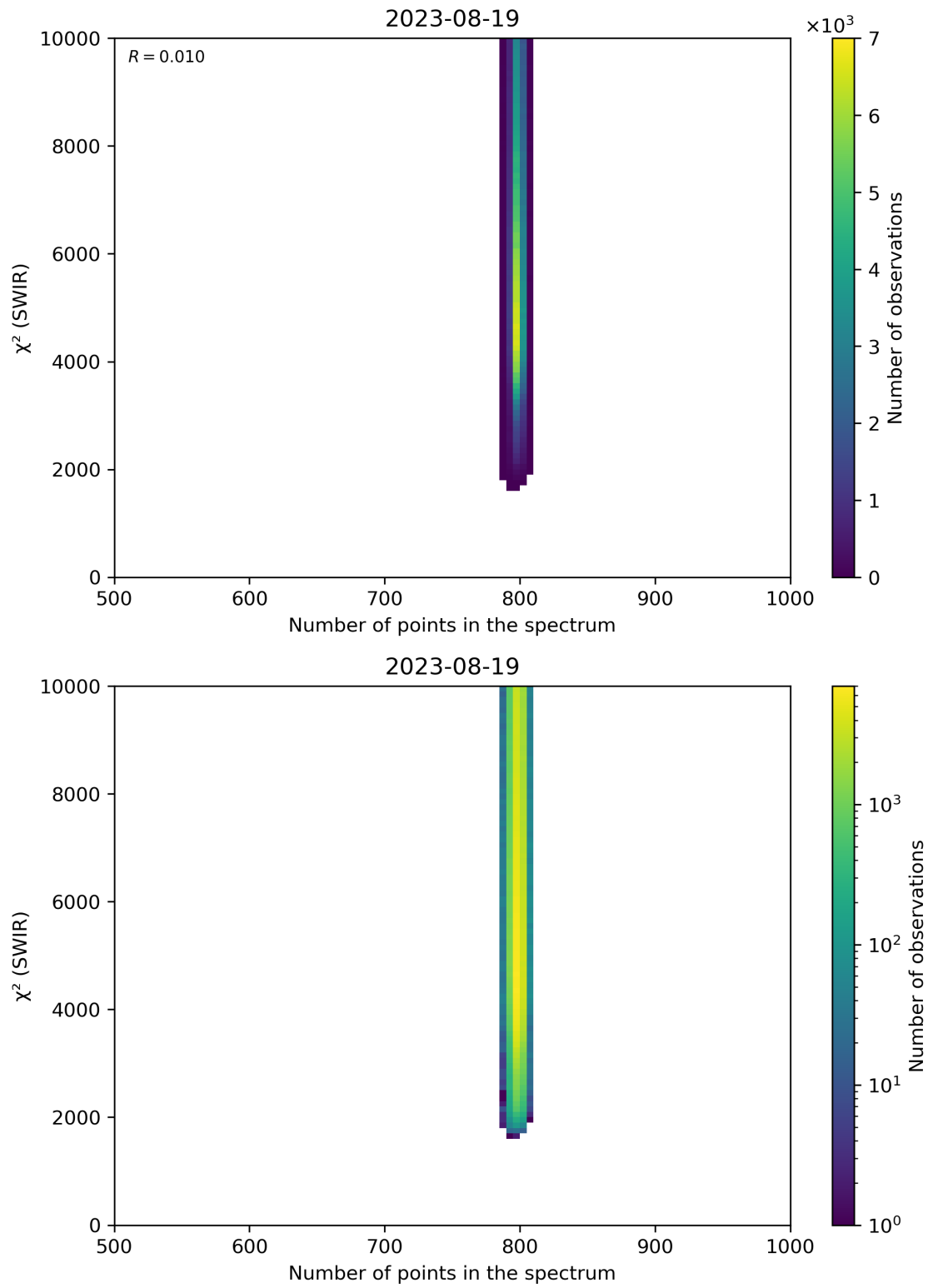
Figure 89: Scatter density plot of “Number of points in the spectrum” against “ \chi^2 (SWIR)” for 2023-08-18 to 2023-08-20.
