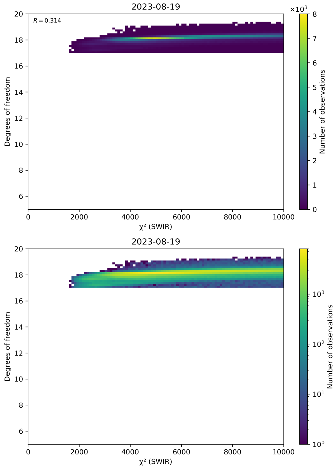
Figure 48: Scatter density plot of “ \chi^2 (SWIR)” against “Degrees of freedom” for 2023-08-18 to 2023-08-20.
