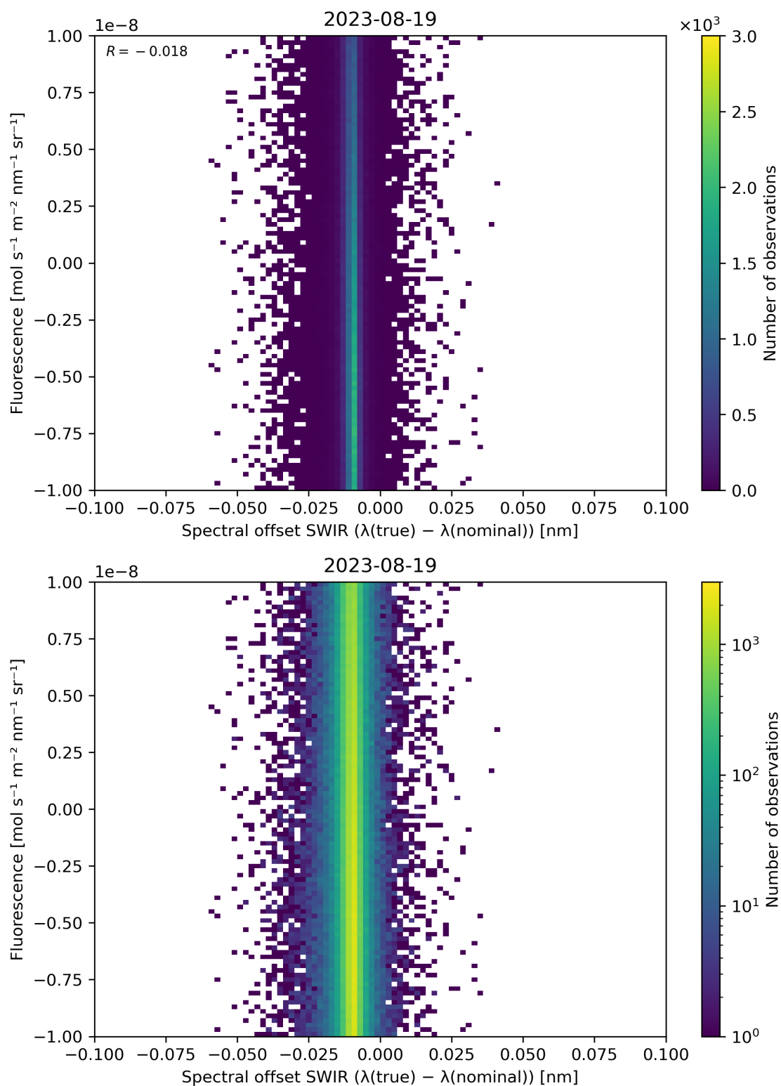
Figure 120: Scatter density plot of “Spectral offset SWIR ( \lambda(\text{true}) - \lambda(\text{nominal}) )” against “Fluorescence” for 2023-08-18 to 2023-08-20.
