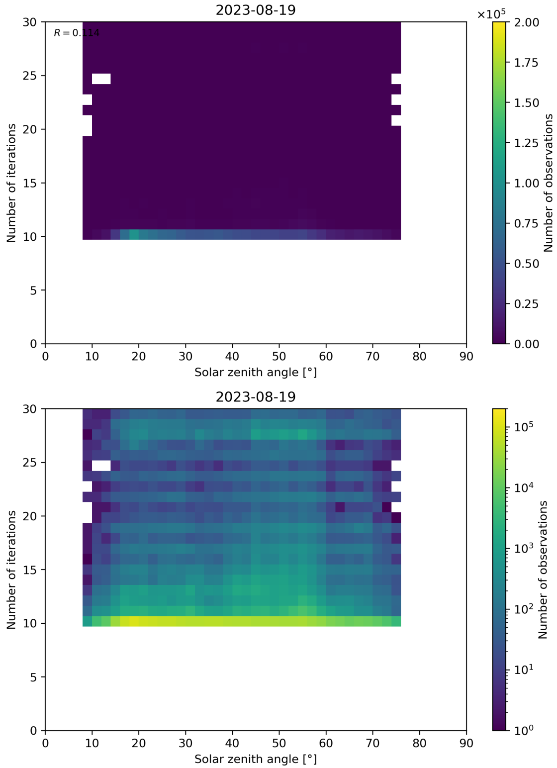
Figure 102: Scatter density plot of “Solar zenith angle” against “Number of iterations” for 2023-08-18 to 2023-08-20.
