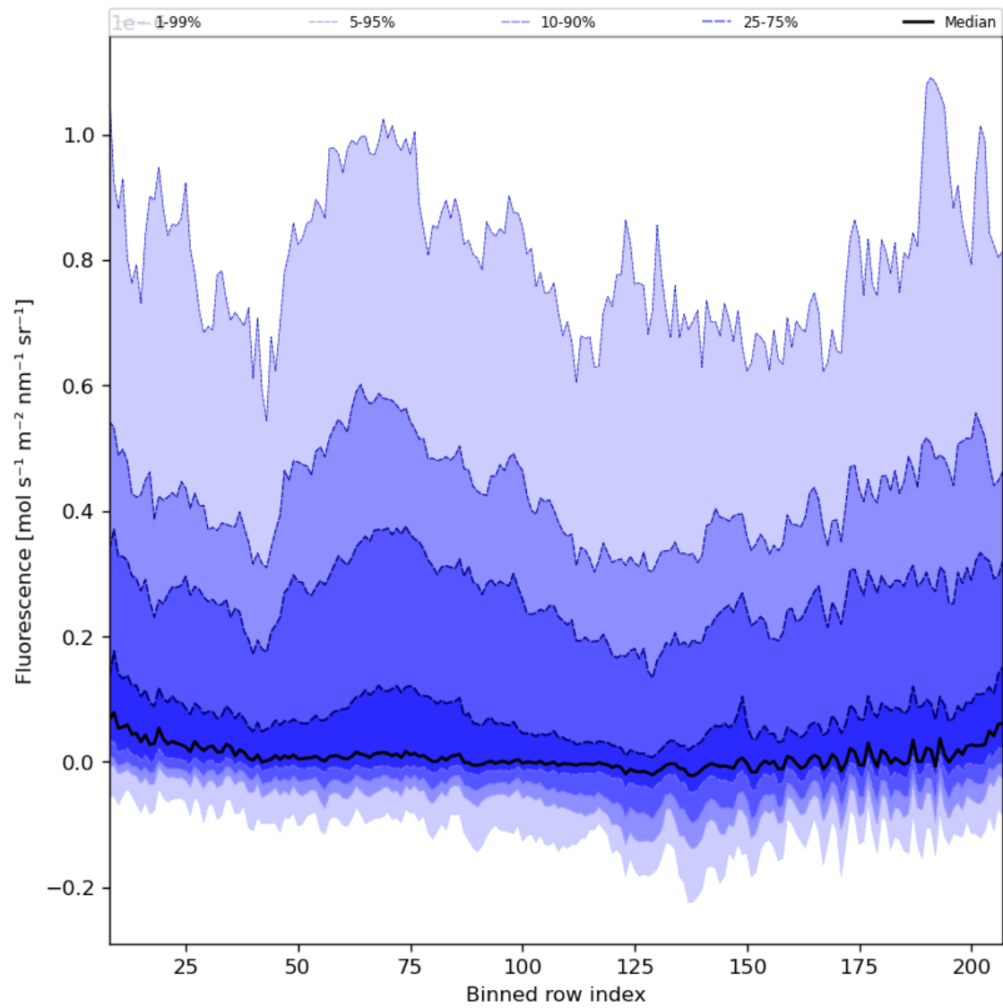
Figure 43: Along track statistics of “Fluorescence” for 2023-08-18 to 2023-08-20
