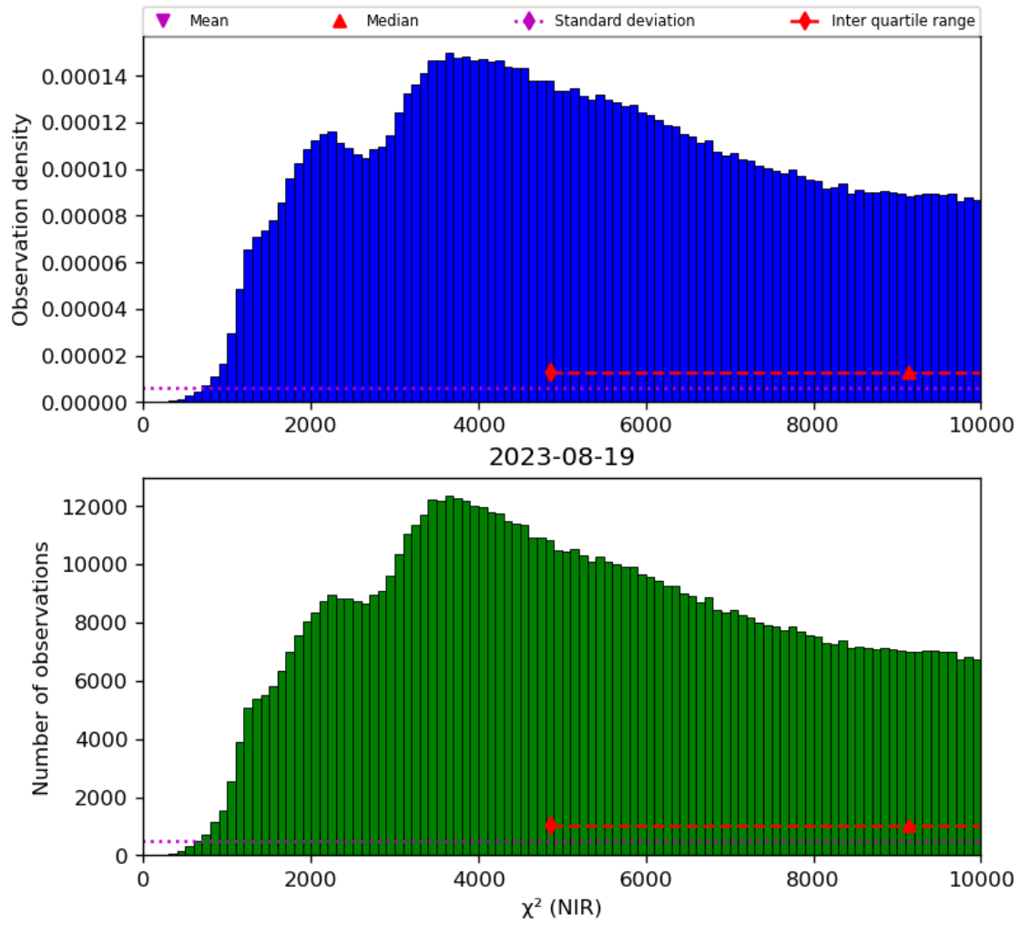
Figure 29: Histogram of “ \chi^2 (NIR)” for 2023-08-18 to 2023-08-20
