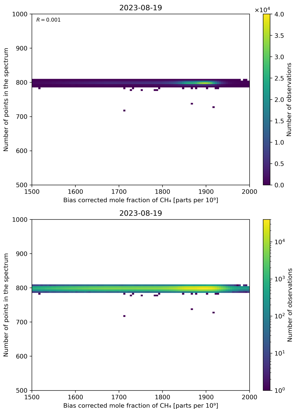
Figure 68: Scatter density plot of “Bias corrected mole fraction of CH 4 ” against “Number of points in the spectrum” for 2023-08-18 to 2023-08-20.
