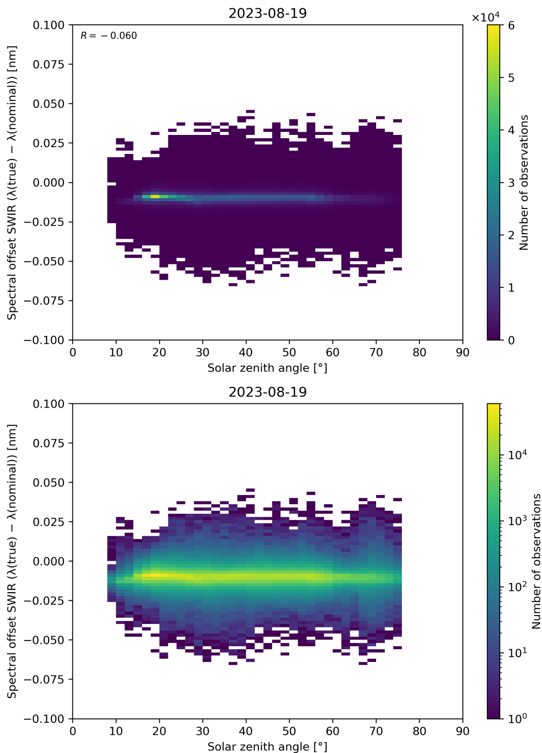
Figure 104: Scatter density plot of “Solar zenith angle” against “Spectral offset SWIR ( \lambda(\text{true}) - \lambda(\text{nominal}) )” for 2023-08-18 to 2023-08-20.
