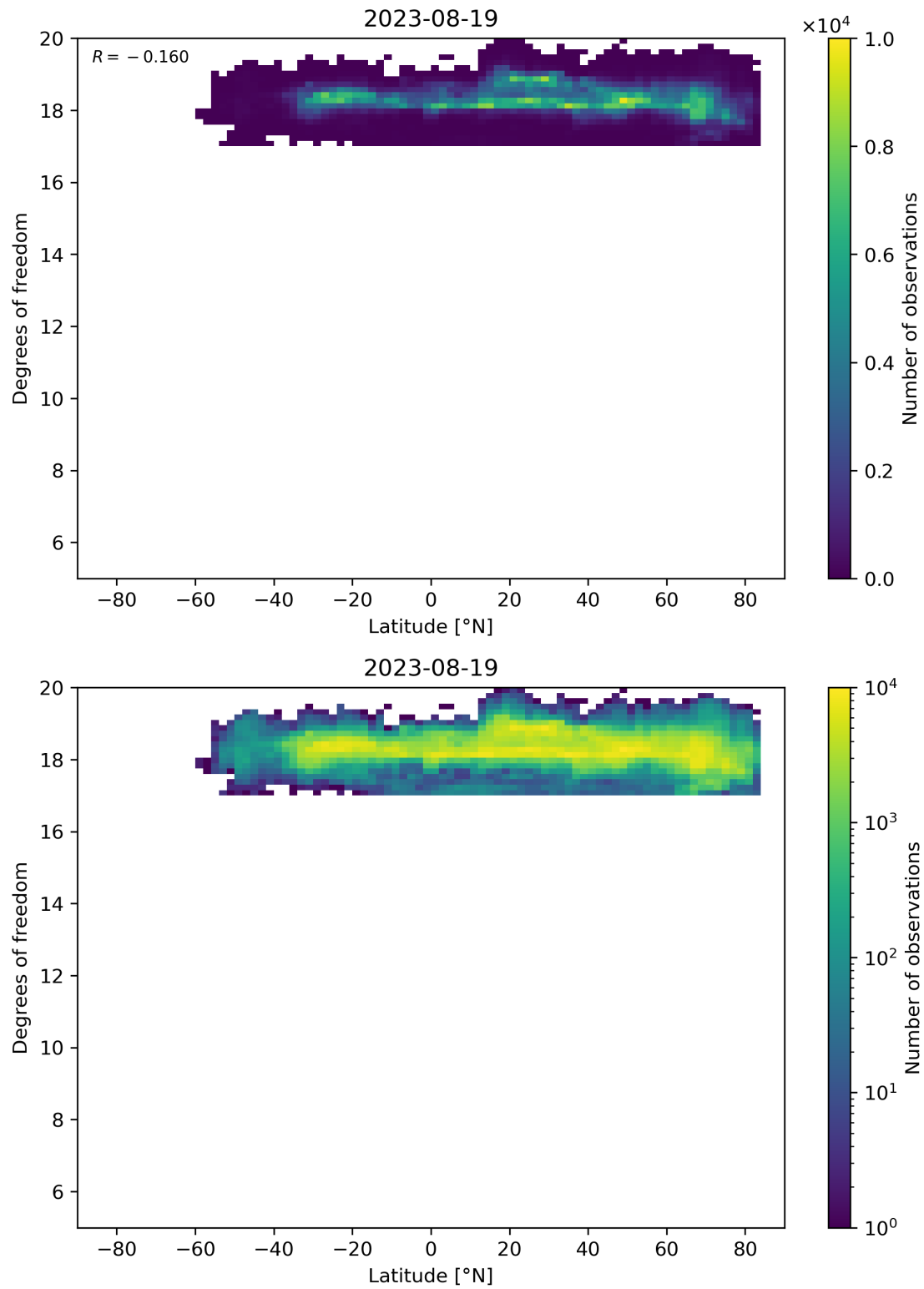
Figure 55: Scatter density plot of “Latitude” against “Degrees of freedom” for 2023-08-18 to 2023-08-20.
