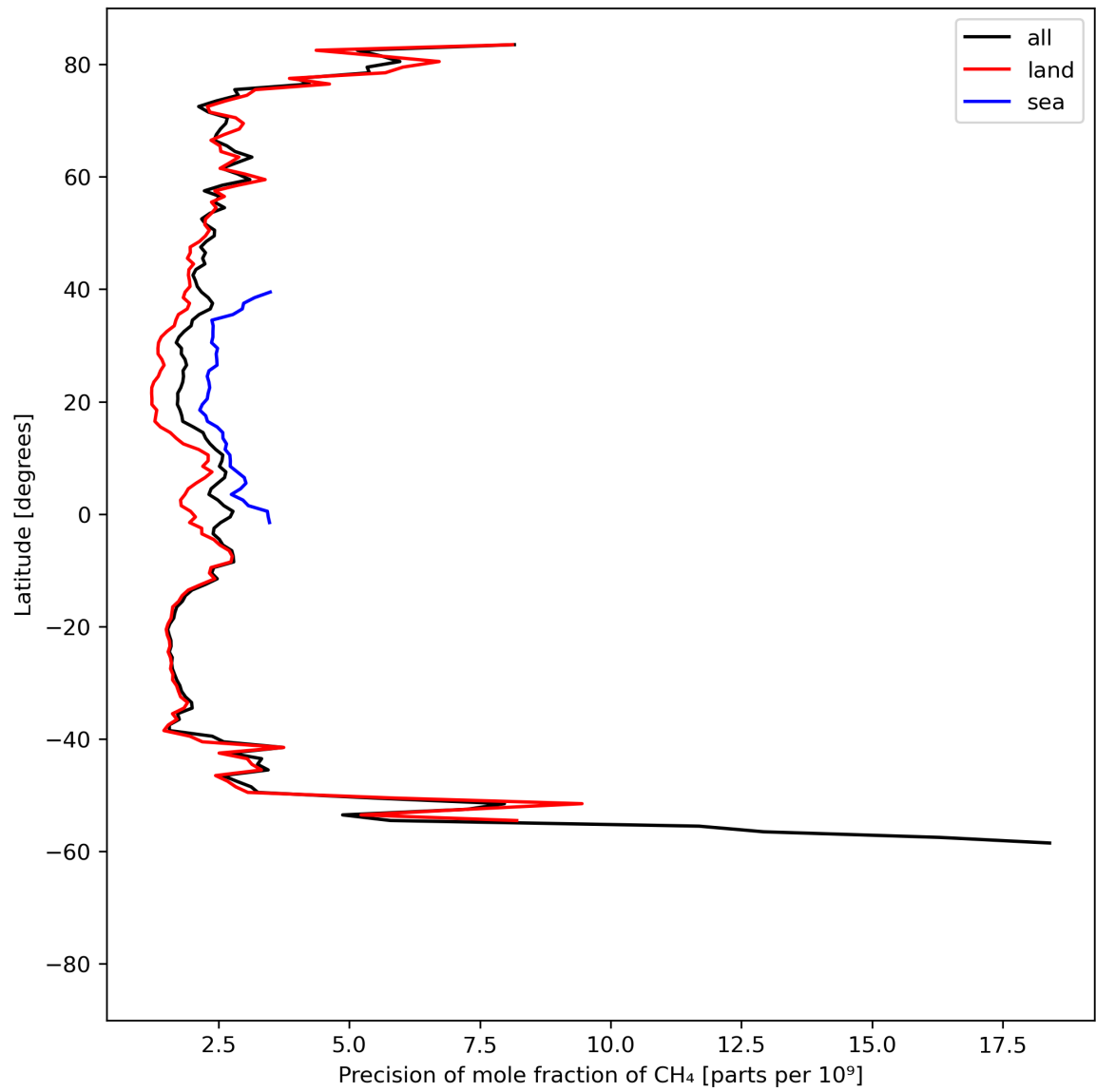
Figure 13: Zonal average of “Precision of mole fraction of CH 4 ” for 2023-08-18 to 2023-08-20.
