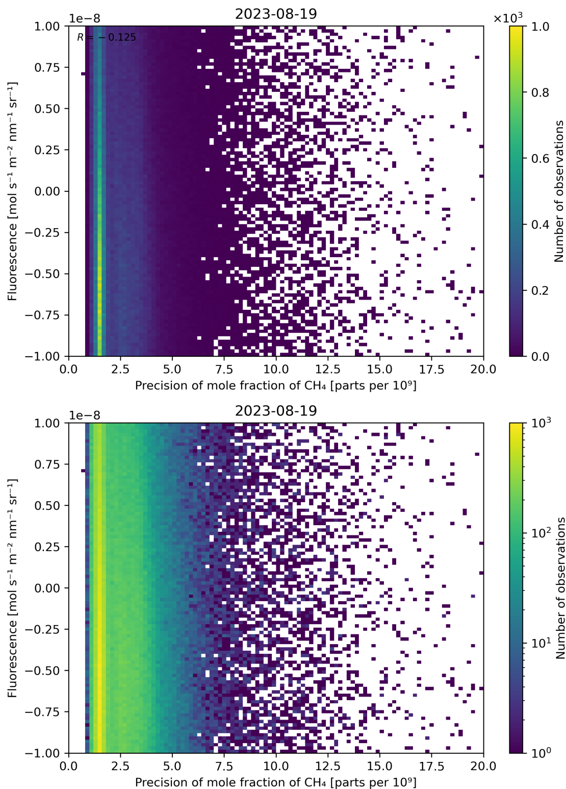
Figure 81: Scatter density plot of “Precision of mole fraction of \text{CH}_4 ” against “Fluorescence” for 2023-08-18 to 2023-08-20.
