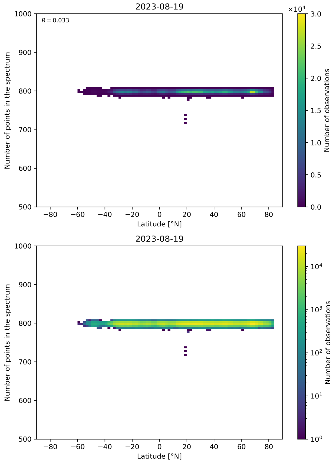
Figure 61: Scatter density plot of “Latitude” against “Number of points in the spectrum” for 2023-08-18 to 2023-08-20.
