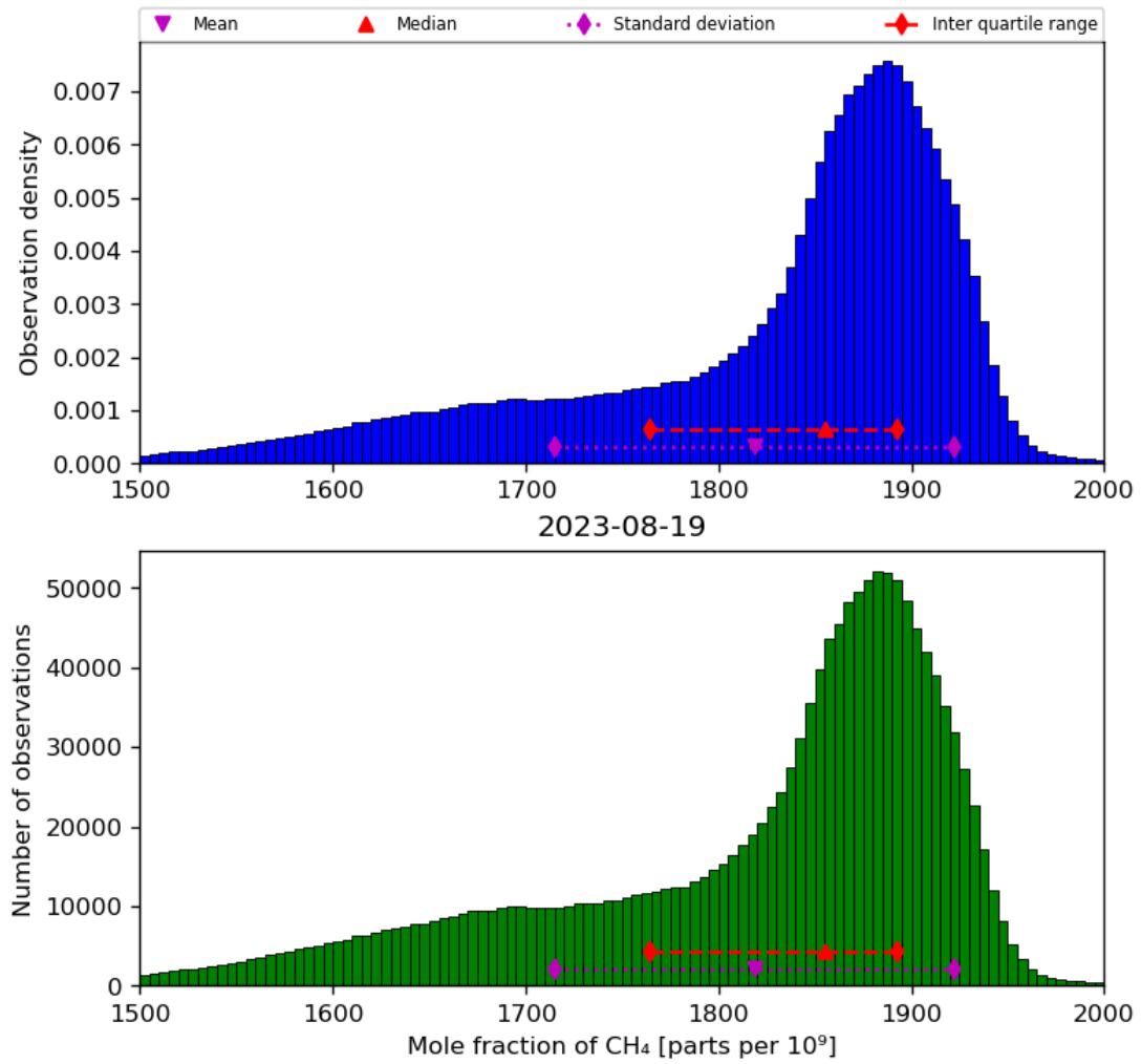
Figure 23: Histogram of "Mole fraction of CH 4 " for 2023-08-18 to 2023-08-20
