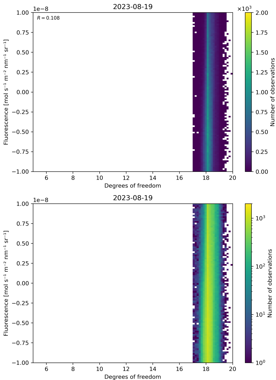
Figure 51: Scatter density plot of “Degrees of freedom” against “Fluorescence” for 2023-08-18 to 2023-08-20.
