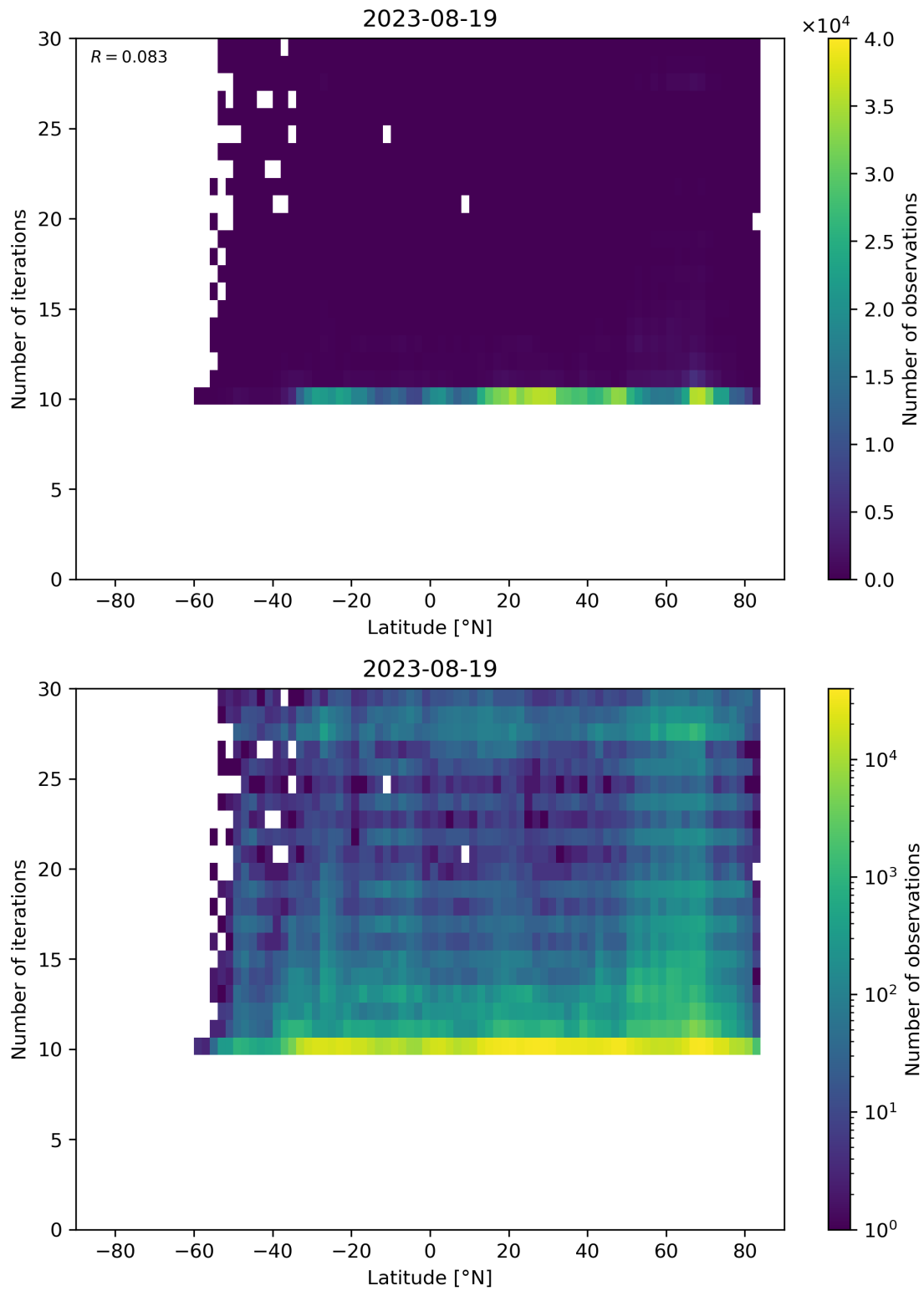
Figure 60: Scatter density plot of “Latitude” against “Number of iterations” for 2023-08-18 to 2023-08-20.
