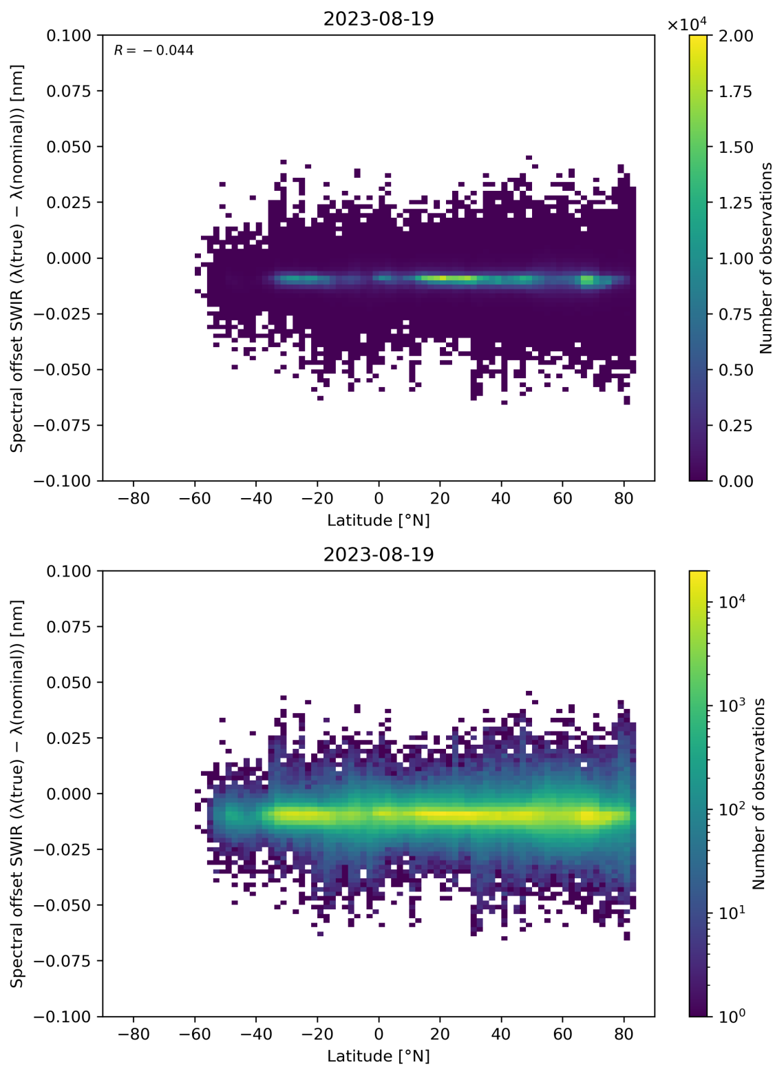
Figure 62: Scatter density plot of “Latitude” against “Spectral offset SWIR ( \lambda(\text{true}) - \lambda(\text{nominal}) )” for 2023-08-18 to 2023-08-20.
