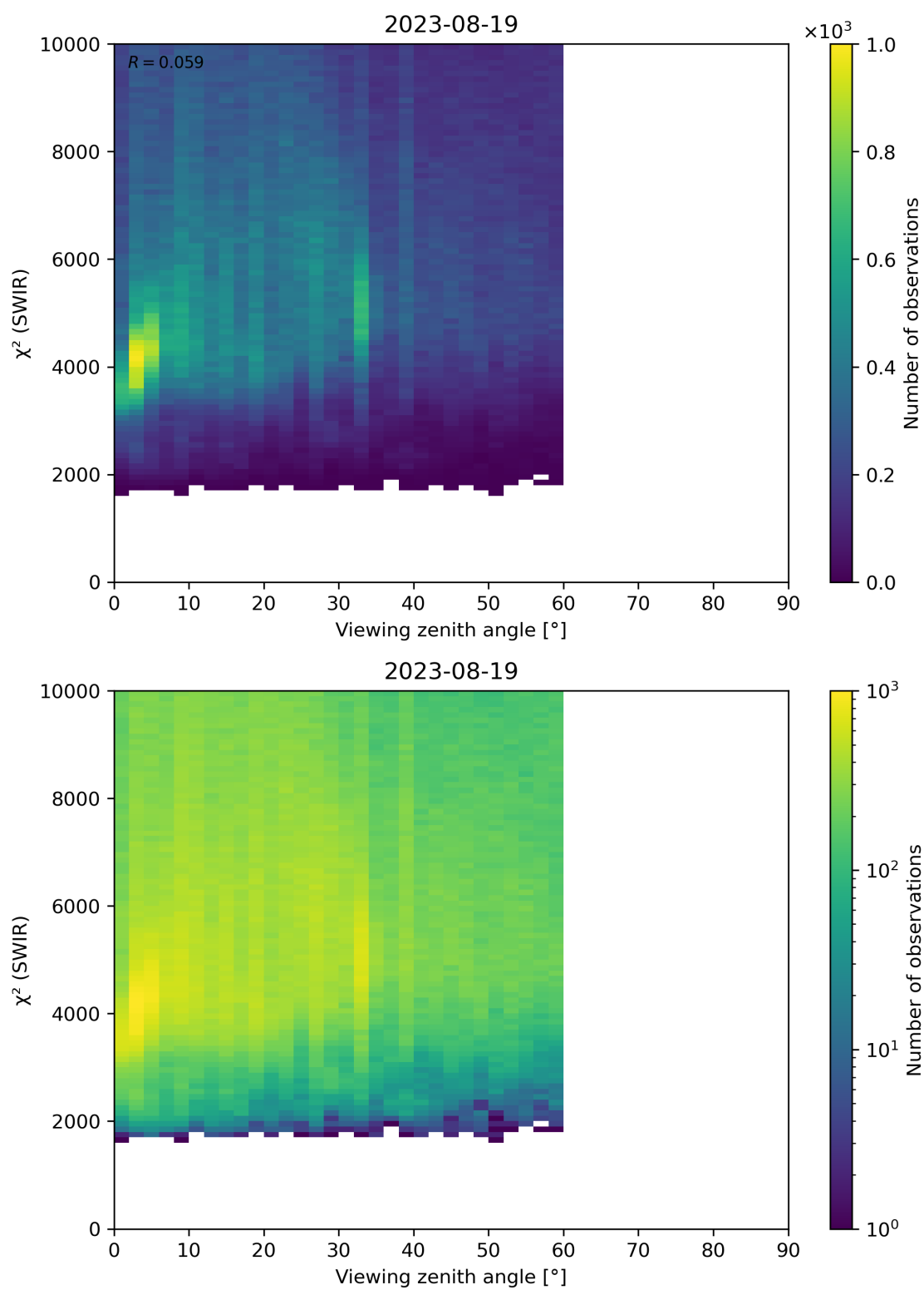
Figure 106: Scatter density plot of “Viewing zenith angle” against “ \chi^2 (SWIR)” for 2023-08-18 to 2023-08-20.
