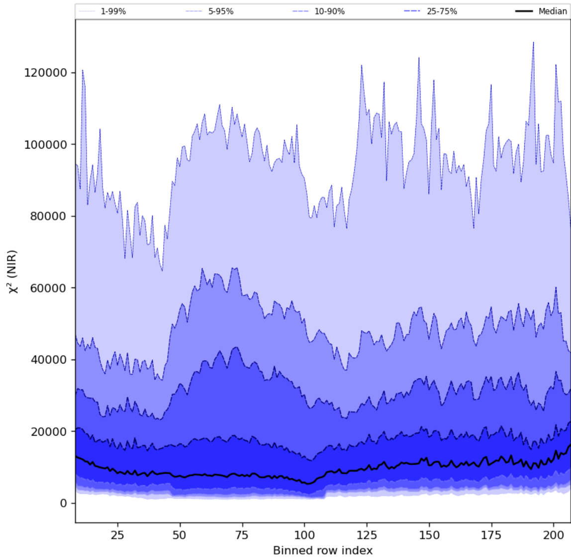
Figure 40: Along track statistics of “ \chi^2 (NIR)” for 2023-08-18 to 2023-08-20
