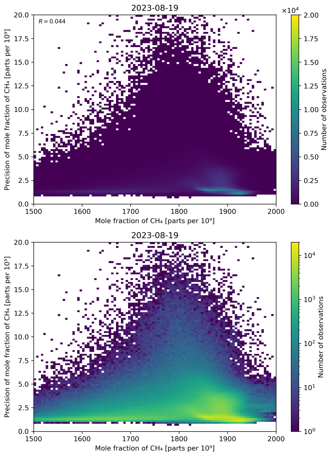
Figure 75: Scatter density plot of “Mole fraction of CH 4 ” against “Precision of mole fraction of CH 4 ” for 2023-08-18 to 2023-08-20.
