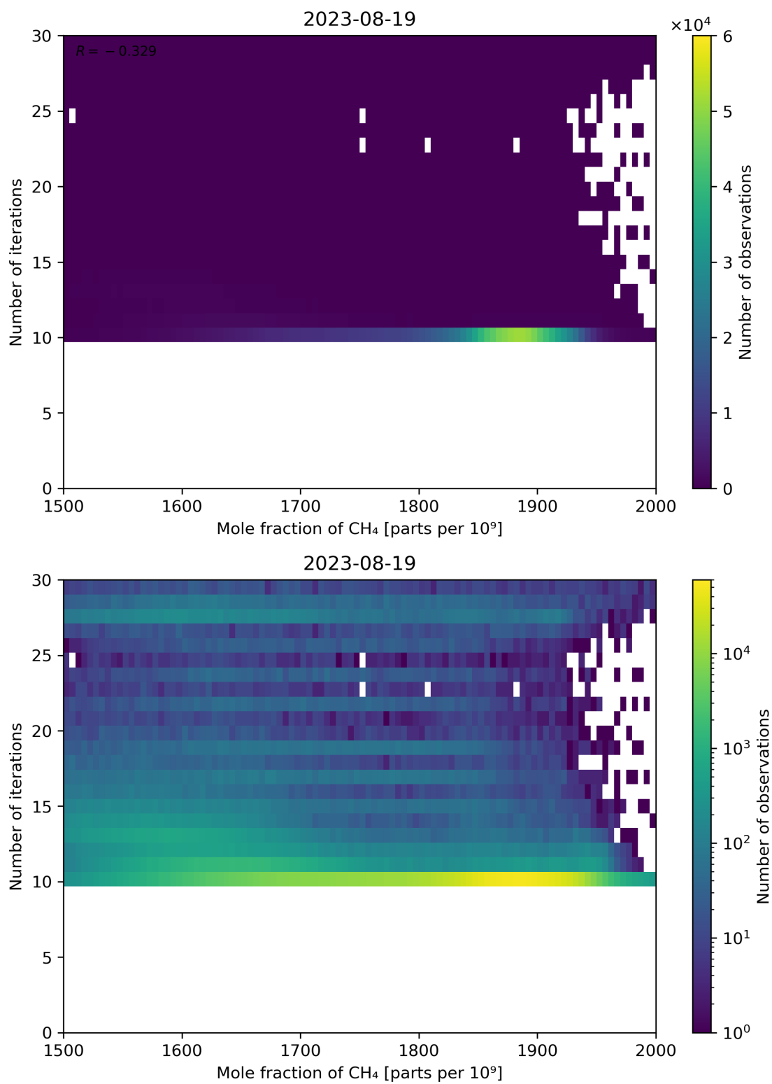
Figure 76: Scatter density plot of “Mole fraction of CH 4 ” against “Number of iterations” for 2023-08-18 to 2023-08-20.
