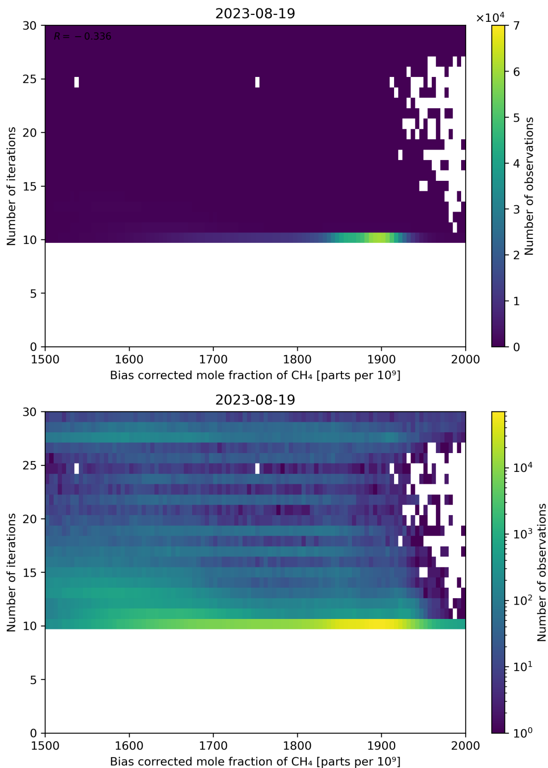
Figure 67: Scatter density plot of “Bias corrected mole fraction of CH 4 ” against “Number of iterations” for 2023-08-18 to 2023-08-20.
