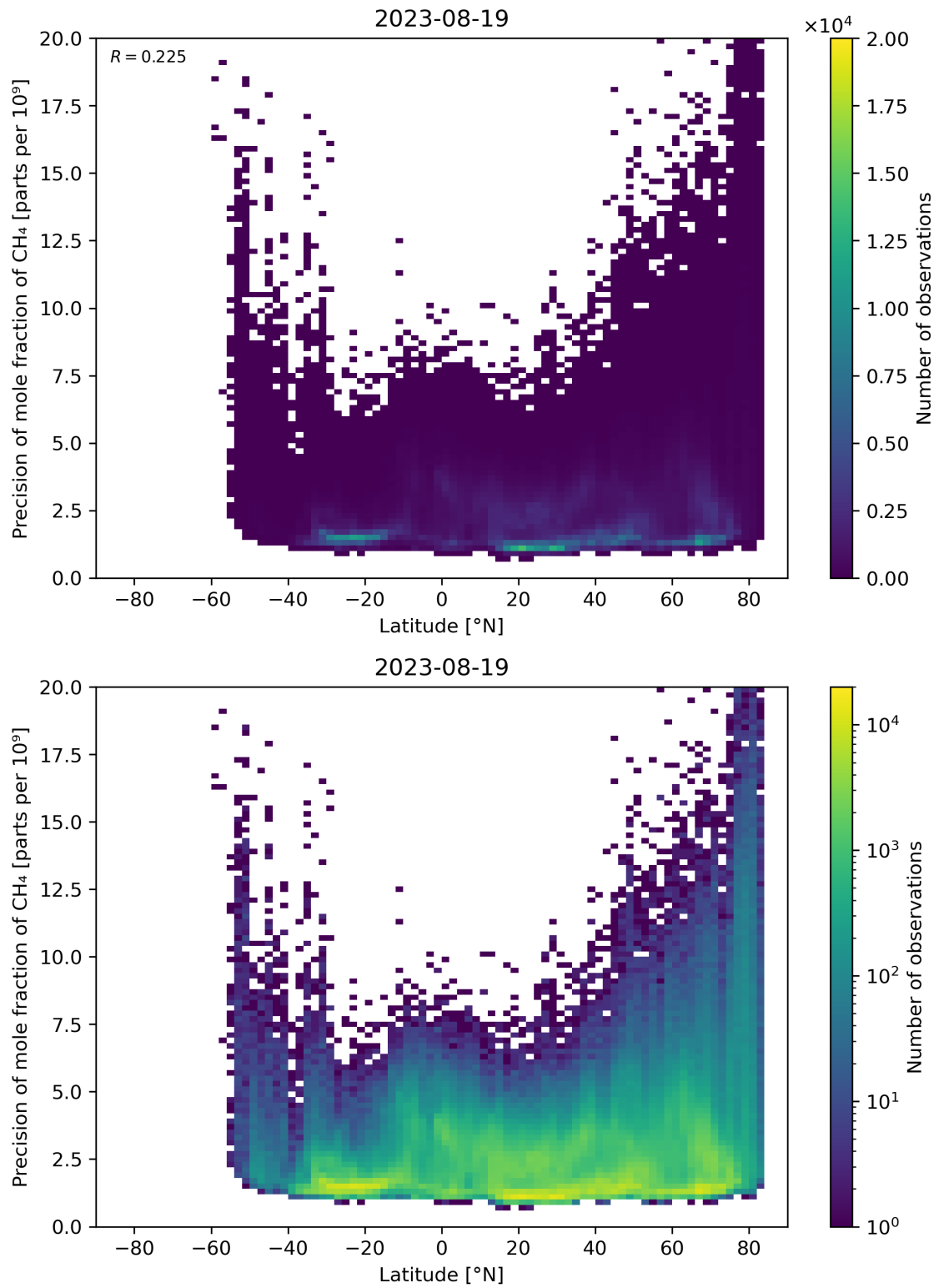
Figure 59: Scatter density plot of “Latitude” against “Precision of mole fraction of \text{CH}_4 ” for 2023-08-18 to 2023-08-20.
