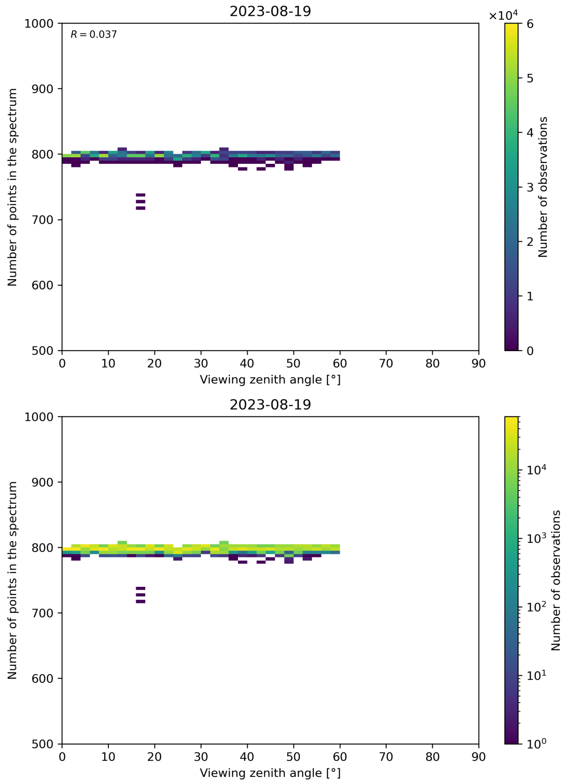
Figure 114: Scatter density plot of “Viewing zenith angle” against “Number of points in the spectrum” for 2023-08-18 to 2023-08-20.
