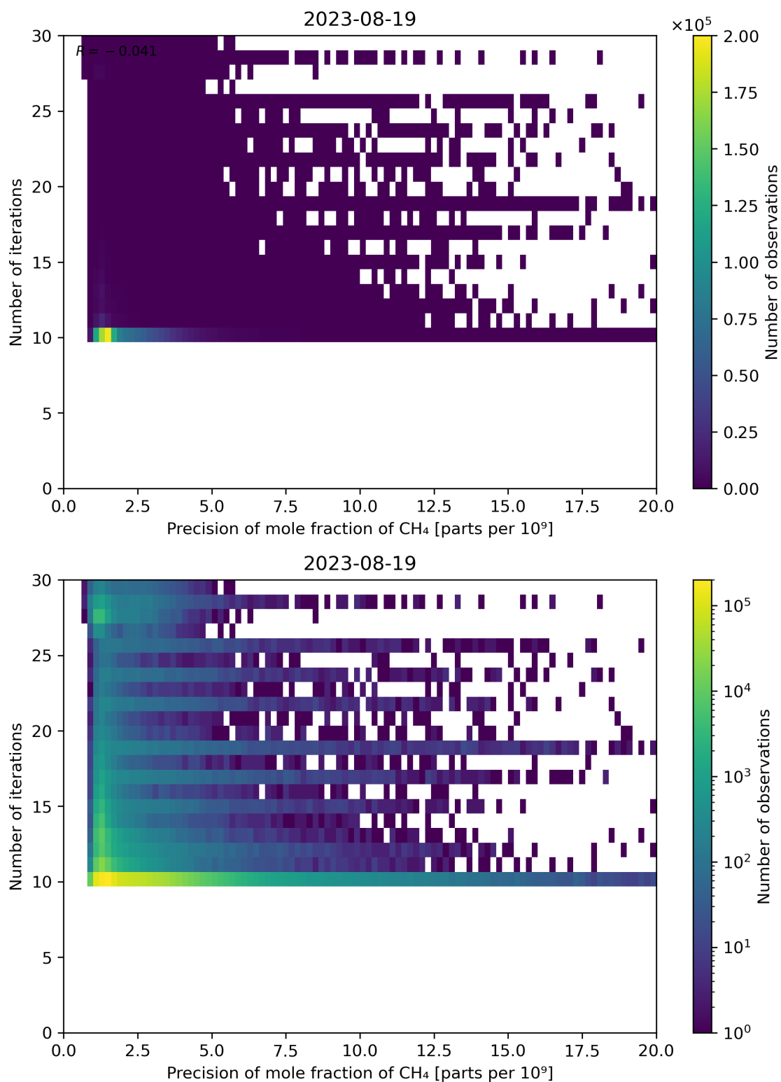
Figure 83: Scatter density plot of “Precision of mole fraction of CH 4 ” against “Number of iterations” for 2023-08-18 to 2023-08-20.
