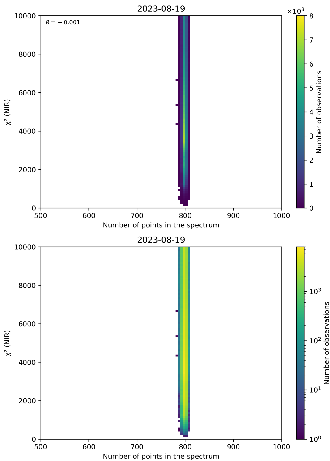
Figure 88: Scatter density plot of “Number of points in the spectrum” against “ \chi^2 (NIR)” for 2023-08-18 to 2023-08-20.
