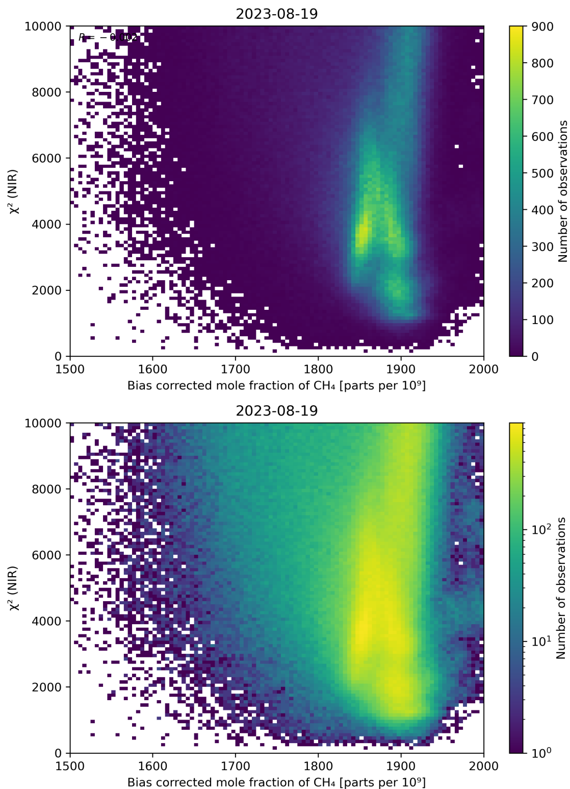
Figure 63: Scatter density plot of “Bias corrected mole fraction of CH 4 ” against “ \chi^2 (NIR)” for 2023-08-18 to 2023-08-20.
