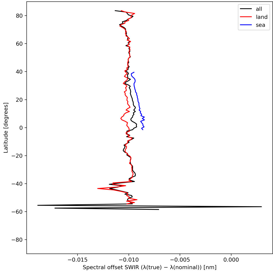
Figure 16: Zonal average of “Spectral offset SWIR ( \lambda(\text{true}) - \lambda(\text{nominal}) )” for 2023-08-18 to 2023-08-20.
