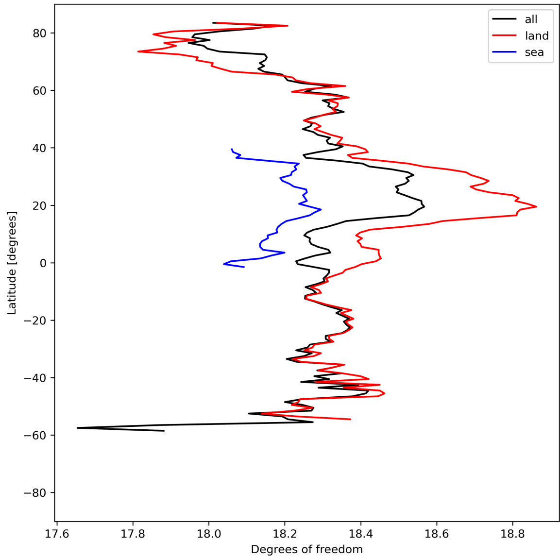
Figure 19: Zonal average of “Degrees of freedom” for 2023-08-18 to 2023-08-20.
