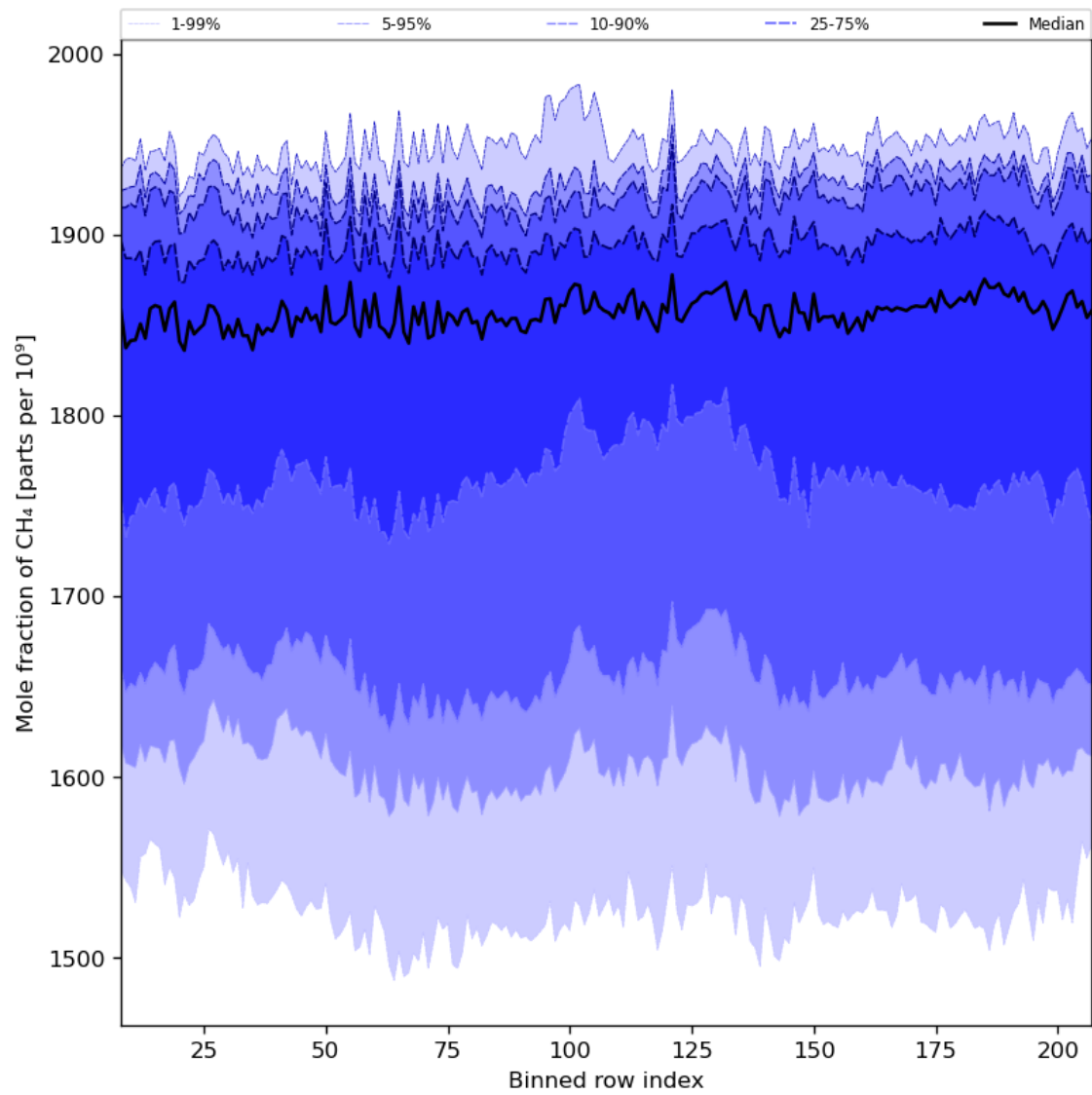
Figure 34: Along track statistics of “Mole fraction of CH 4 ” for 2023-08-18 to 2023-08-20
