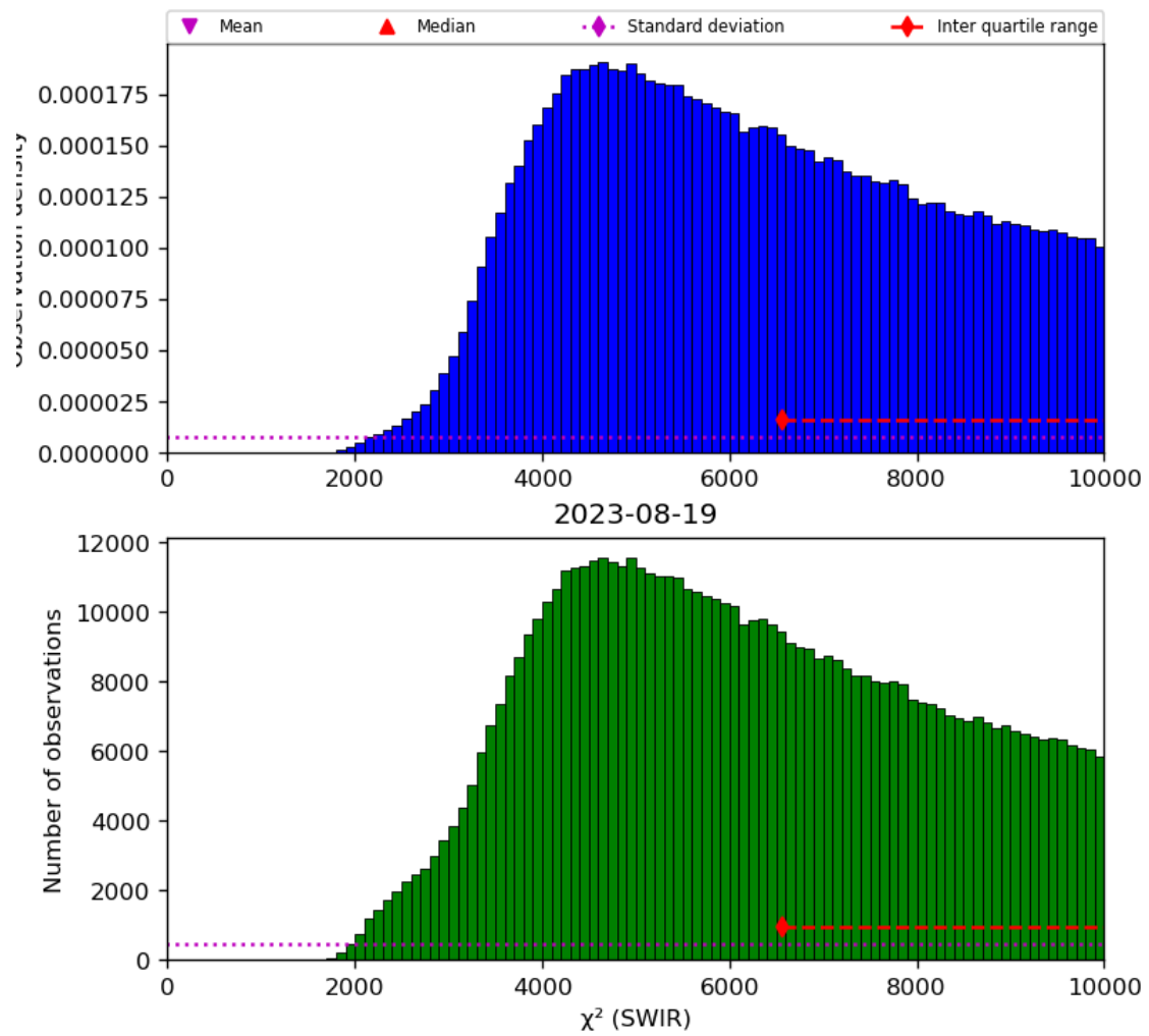
Figure 28: Histogram of “ \chi^2 (SWIR)” for 2023-08-18 to 2023-08-20
