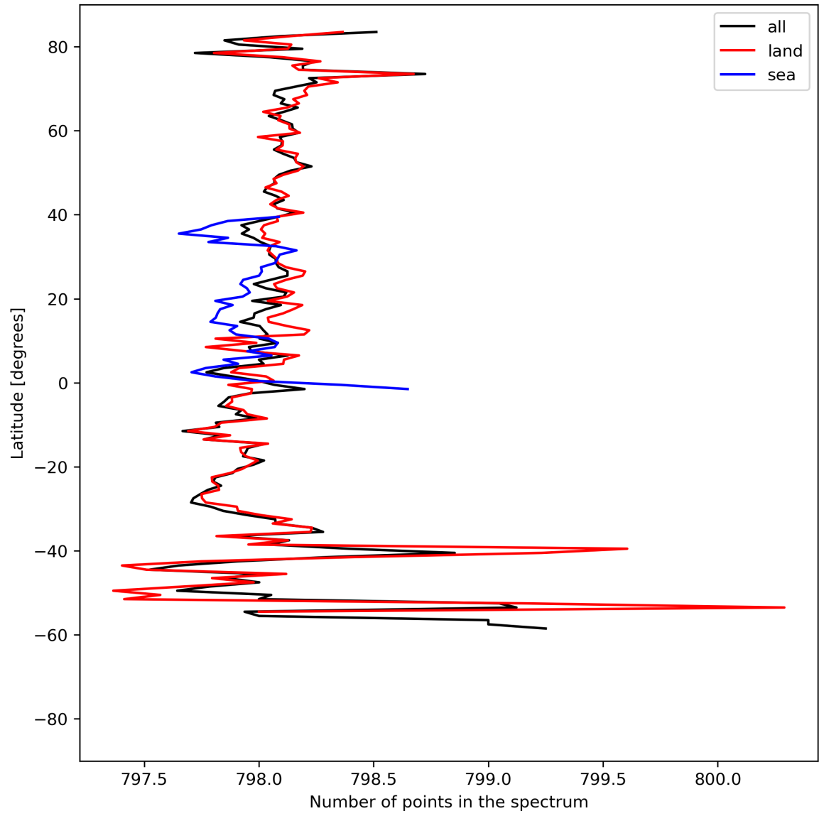
Figure 15: Zonal average of “Number of points in the spectrum” for 2023-08-18 to 2023-08-20.
