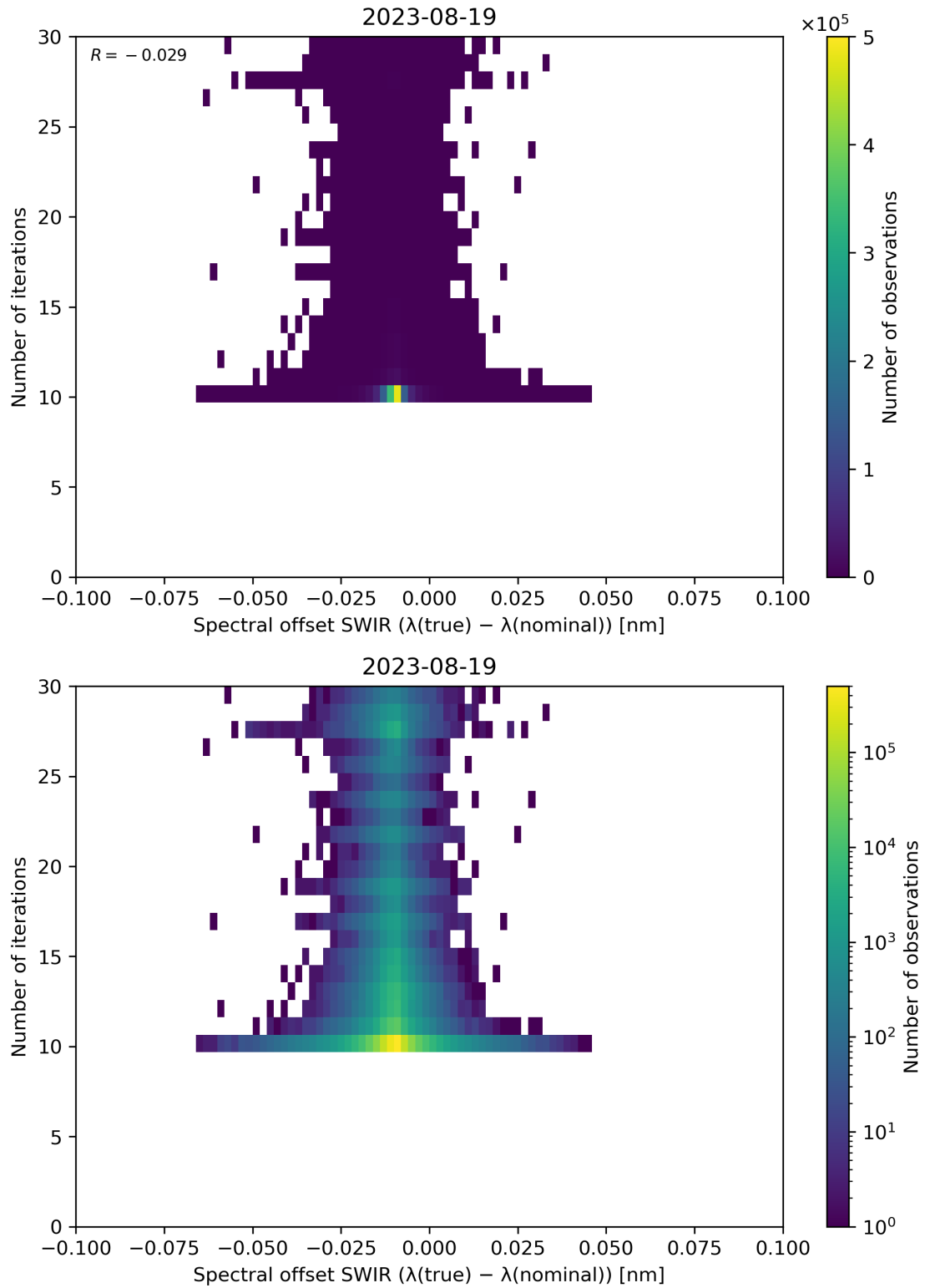
Figure 121: Scatter density plot of “Spectral offset SWIR ( \lambda(\text{true}) - \lambda(\text{nominal}) )” against “Number of iterations” for 2023-08-18 to 2023-08-20.
