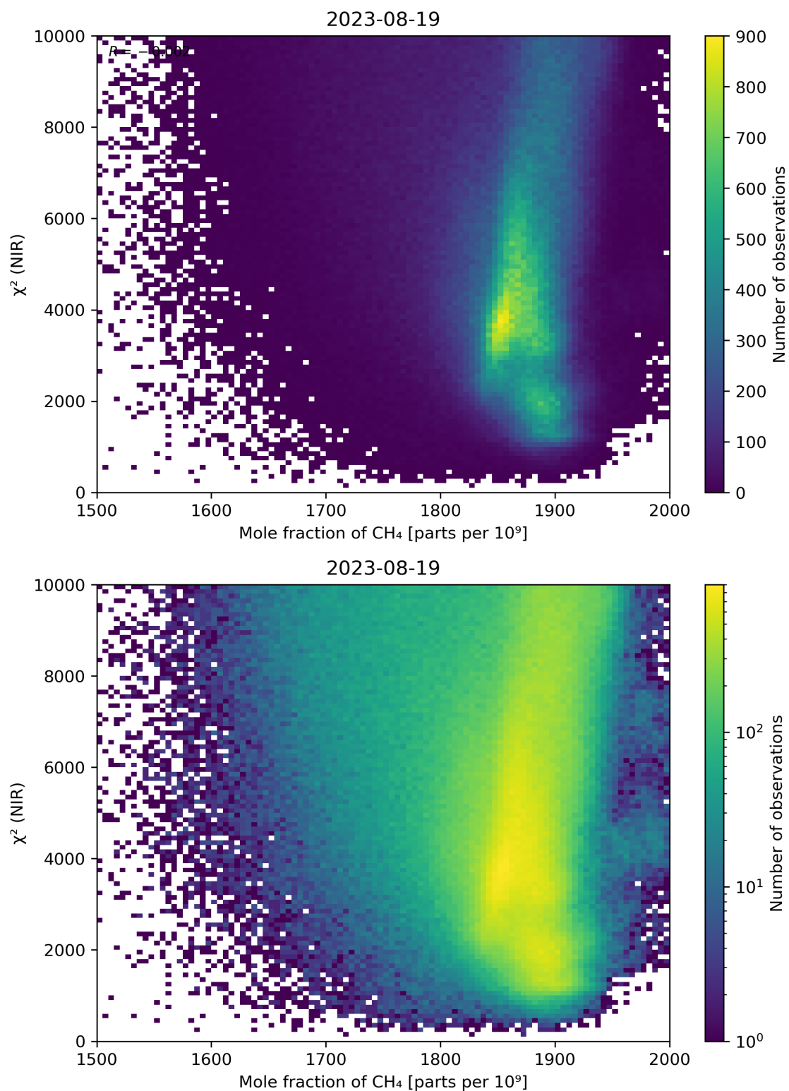
Figure 70: Scatter density plot of “Mole fraction of CH 4 ” against “ \chi^2 (NIR)” for 2023-08-18 to 2023-08-20.
