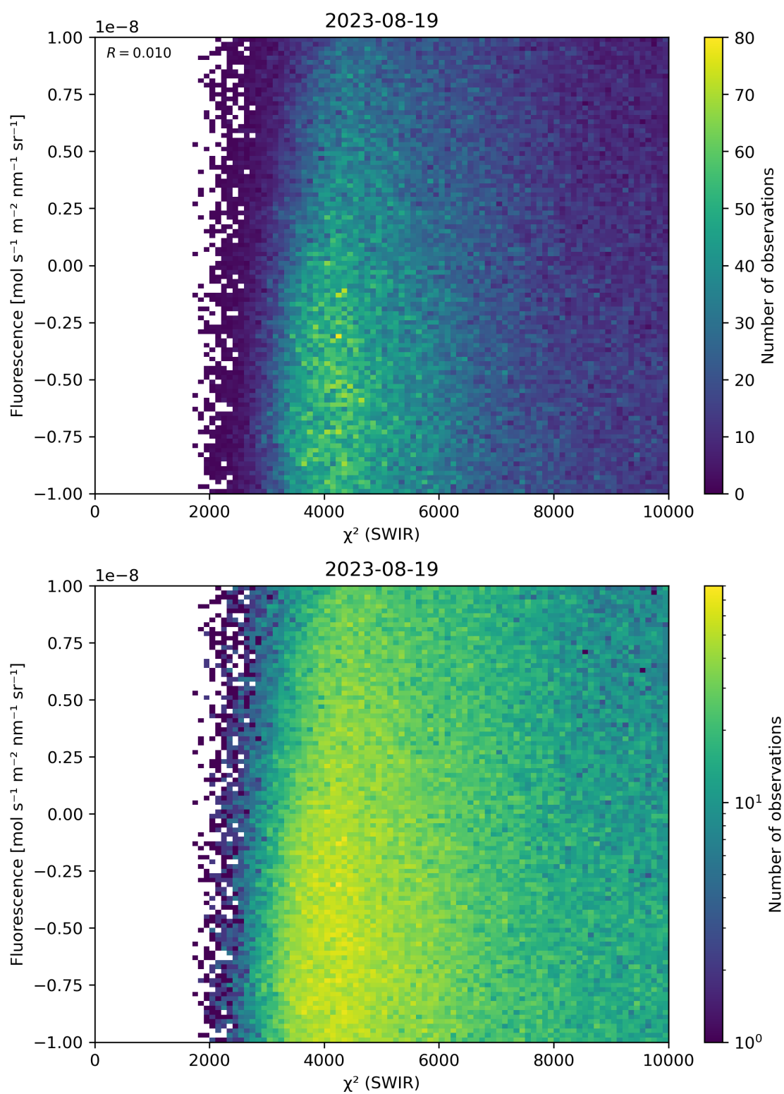
Figure 49: Scatter density plot of “ \chi^2 (SWIR)” against “Fluorescence” for 2023-08-18 to 2023-08-20.
