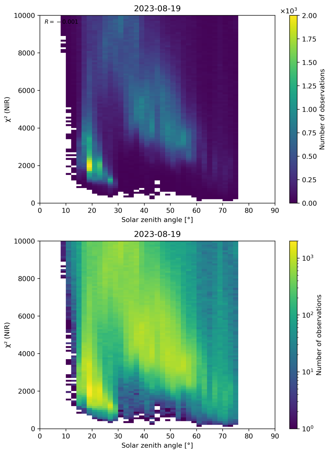
Figure 94: Scatter density plot of “Solar zenith angle” against “ \chi^2 (NIR)” for 2023-08-18 to 2023-08-20.
