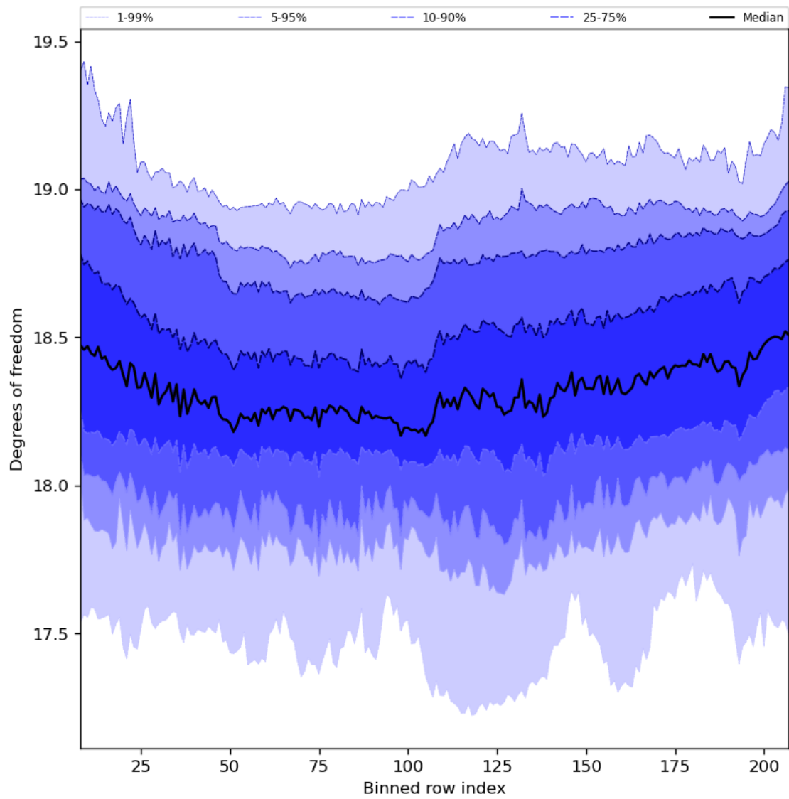
Figure 41: Along track statistics of “Degrees of freedom” for 2023-08-18 to 2023-08-20
