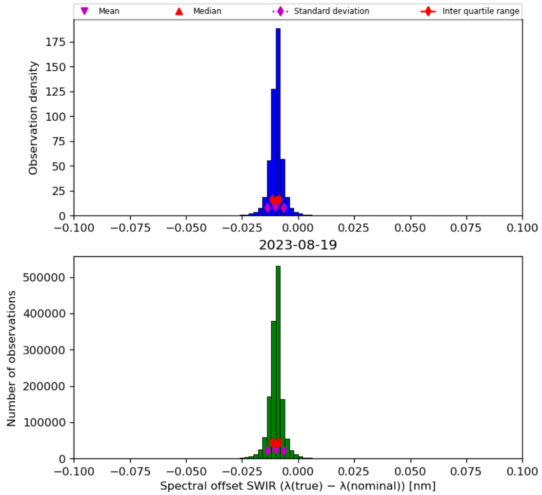
Figure 27: Histogram of “Spectral offset SWIR ( \lambda(\text{true}) - \lambda(\text{nominal}) )” for 2023-08-18 to 2023-08-20
