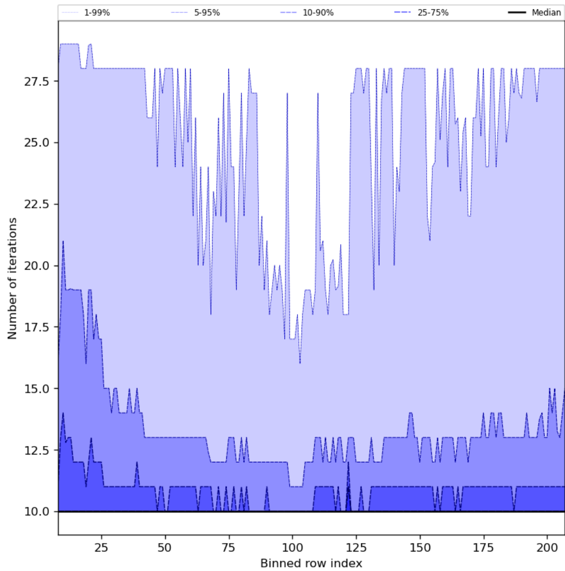
Figure 42: Along track statistics of “Number of iterations” for 2023-08-18 to 2023-08-20
