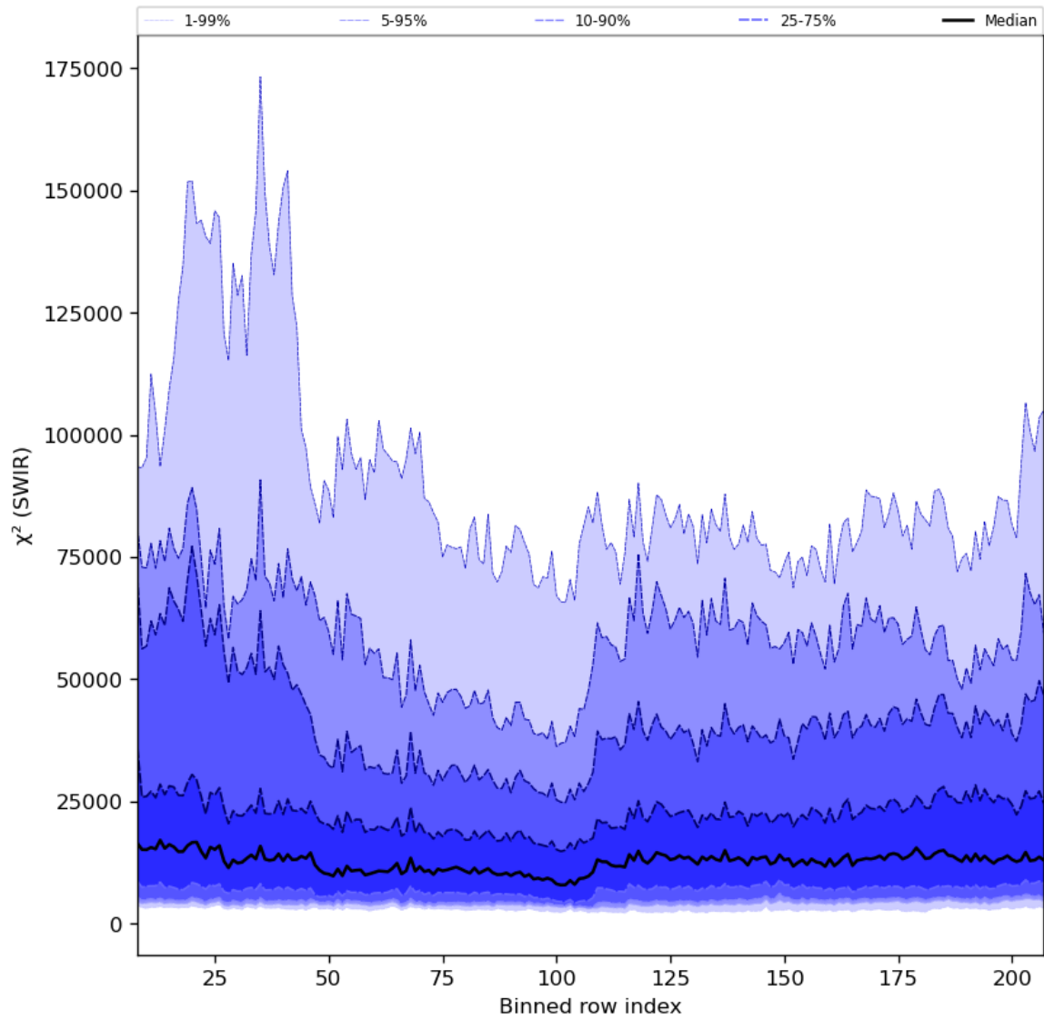
Figure 39: Along track statistics of " \chi^2 (SWIR)" for 2023-08-18 to 2023-08-20
