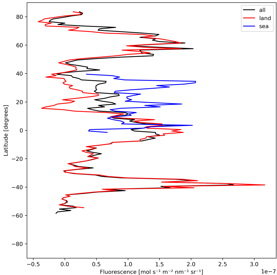
Figure 21: Zonal average of “Fluorescence” for 2023-08-18 to 2023-08-20.
