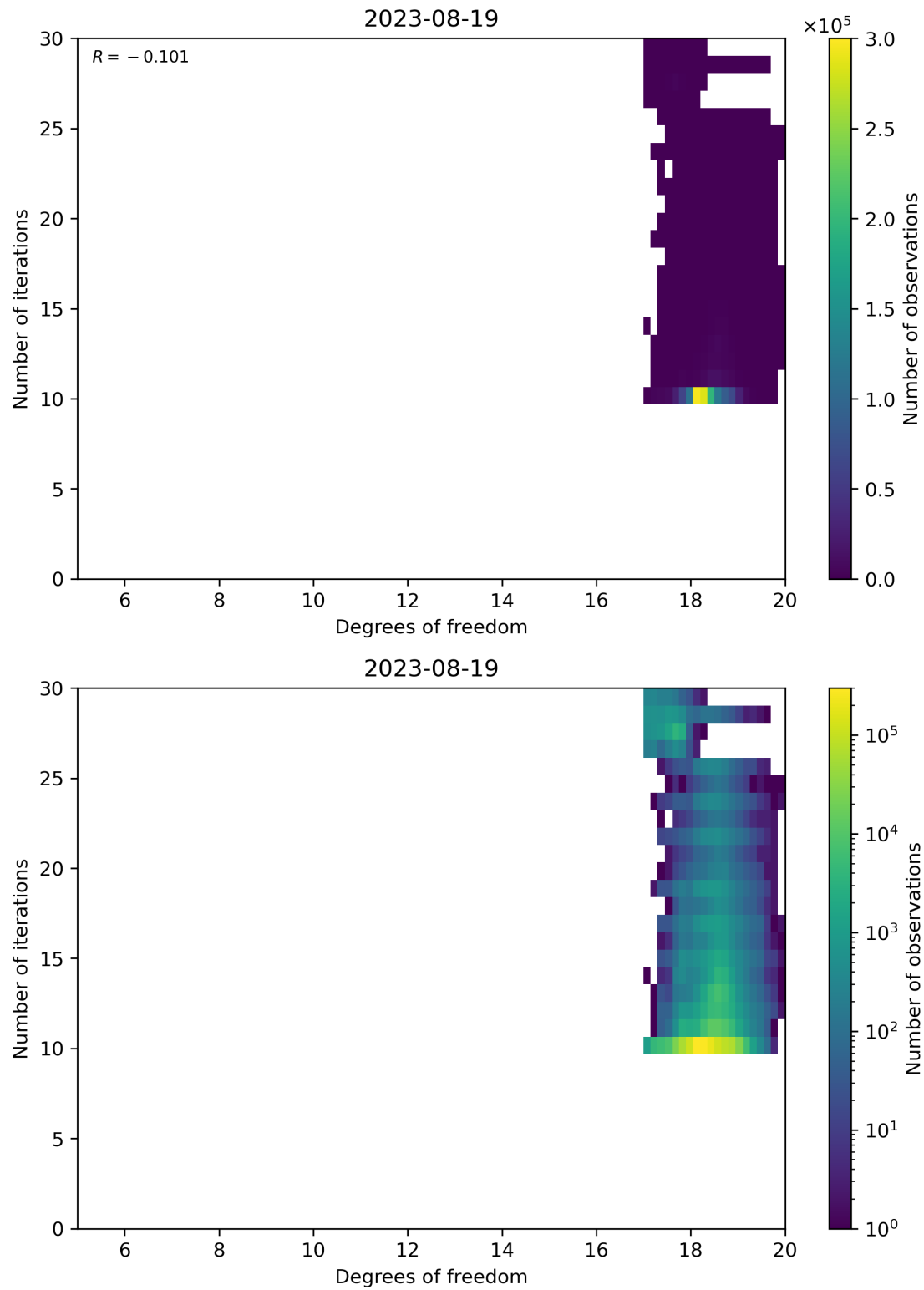
Figure 52: Scatter density plot of “Degrees of freedom” against “Number of iterations” for 2023-08-18 to 2023-08-20.
