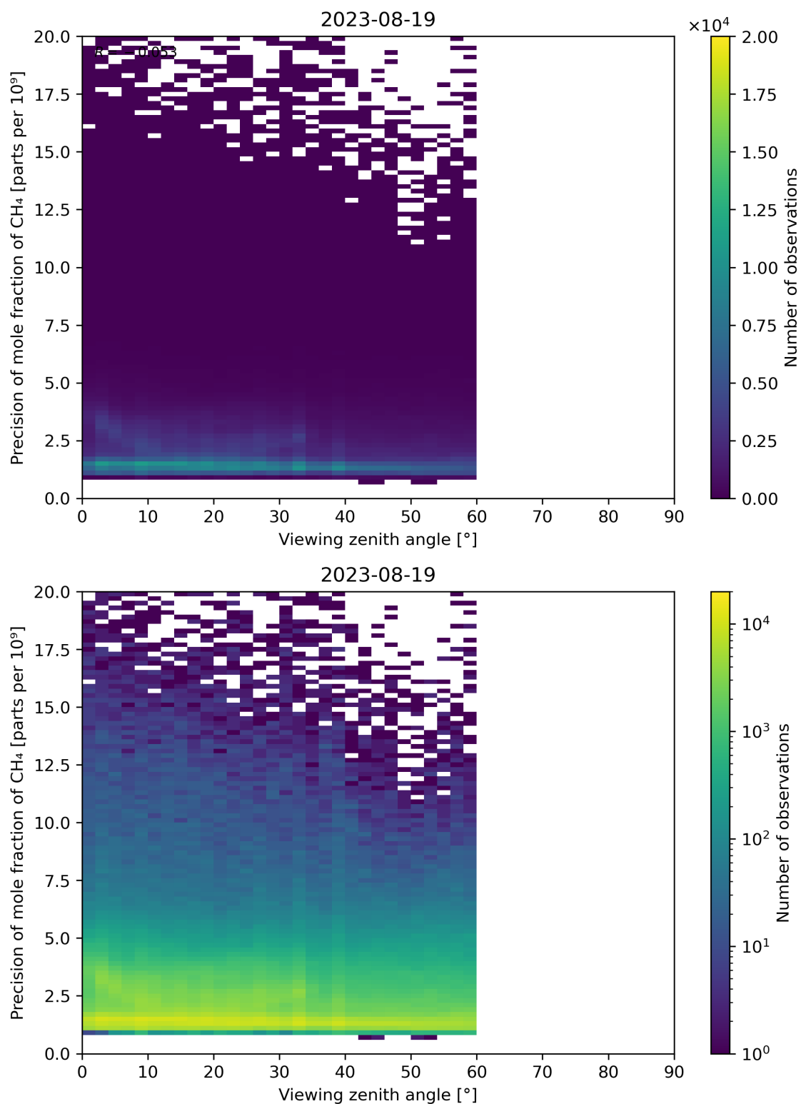
Figure 112: Scatter density plot of “Viewing zenith angle” against “Precision of mole fraction of CH 4 ” for 2023-08-18 to 2023-08-20.
