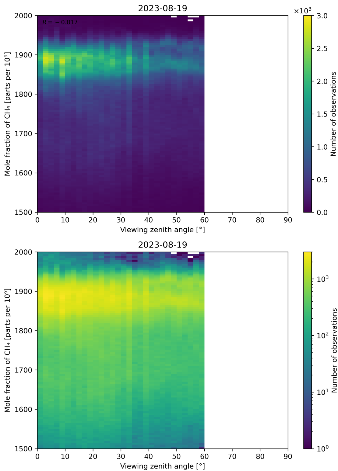
Figure 110: Scatter density plot of “Viewing zenith angle” against “Mole fraction of CH 4 ” for 2023-08-18 to 2023-08-20.
