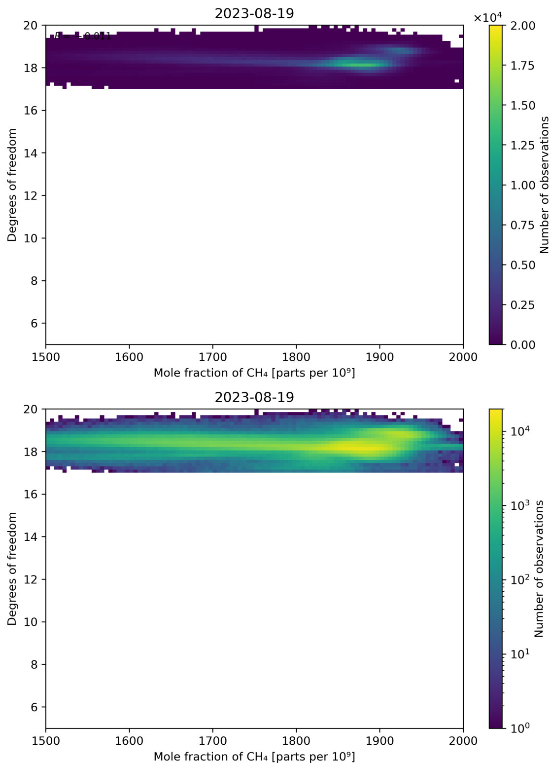
Figure 72: Scatter density plot of “Mole fraction of CH 4 ” against “Degrees of freedom” for 2023-08-18 to 2023-08-20.
