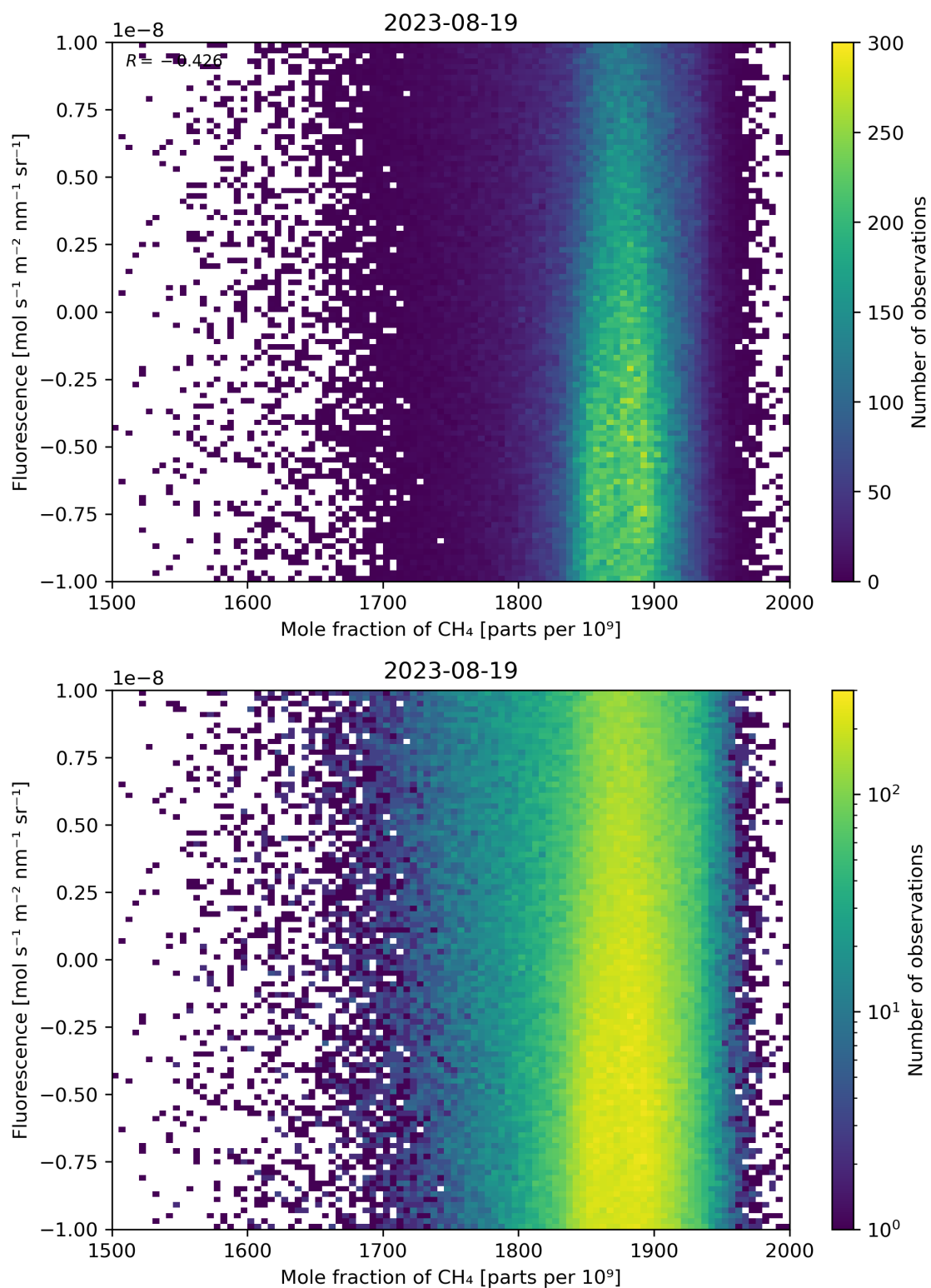
Figure 73: Scatter density plot of “Mole fraction of \text{CH}_4 ” against “Fluorescence” for 2023-08-18 to 2023-08-20.
