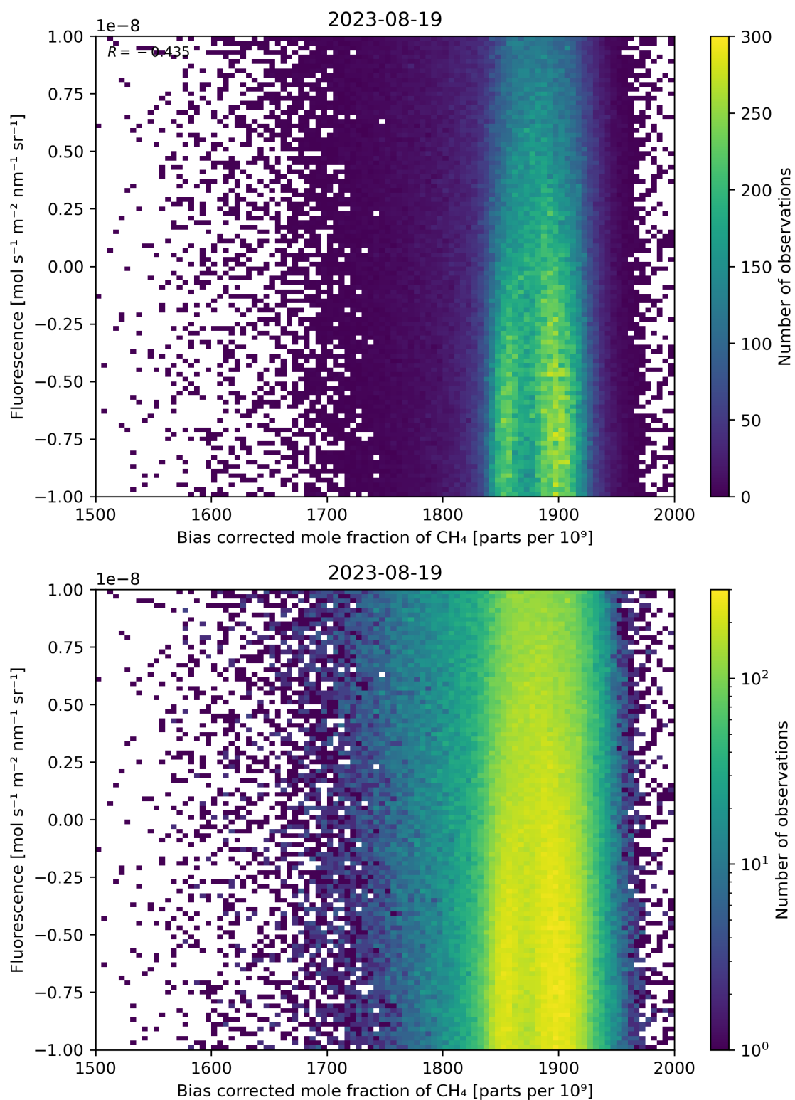
Figure 66: Scatter density plot of “Bias corrected mole fraction of CH 4 ” against “Fluorescence” for 2023-08-18 to 2023-08-20.
