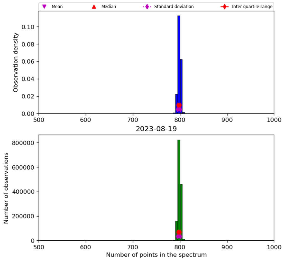
Figure 26: Histogram of “Number of points in the spectrum” for 2023-08-18 to 2023-08-20
