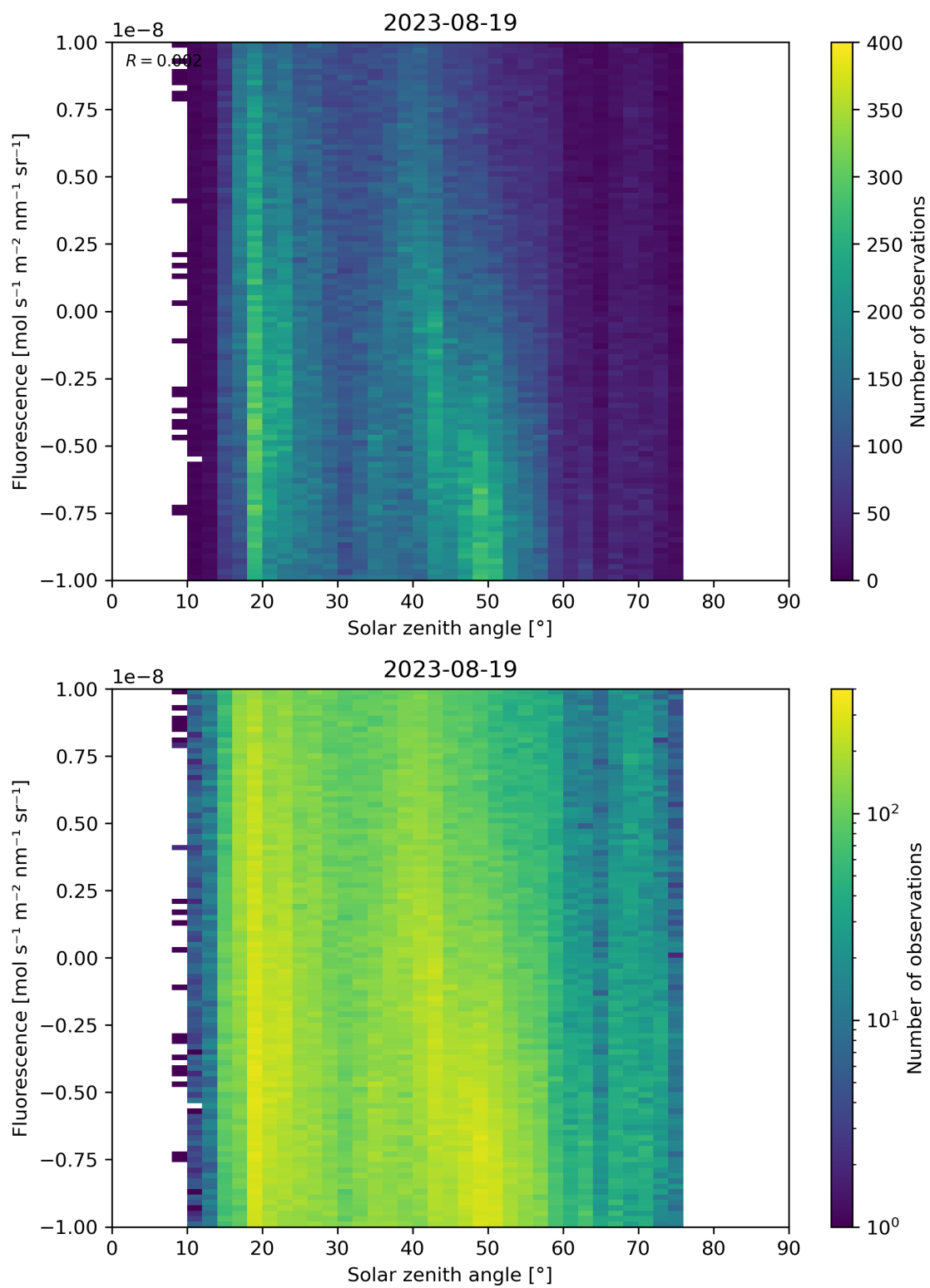
Figure 97: Scatter density plot of “Solar zenith angle” against “Fluorescence” for 2023-08-18 to 2023-08-20.
