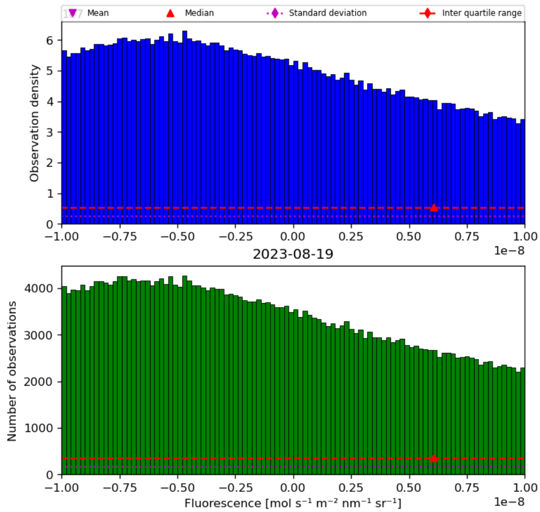
Figure 32: Histogram of “Fluorescence” for 2023-08-18 to 2023-08-20
