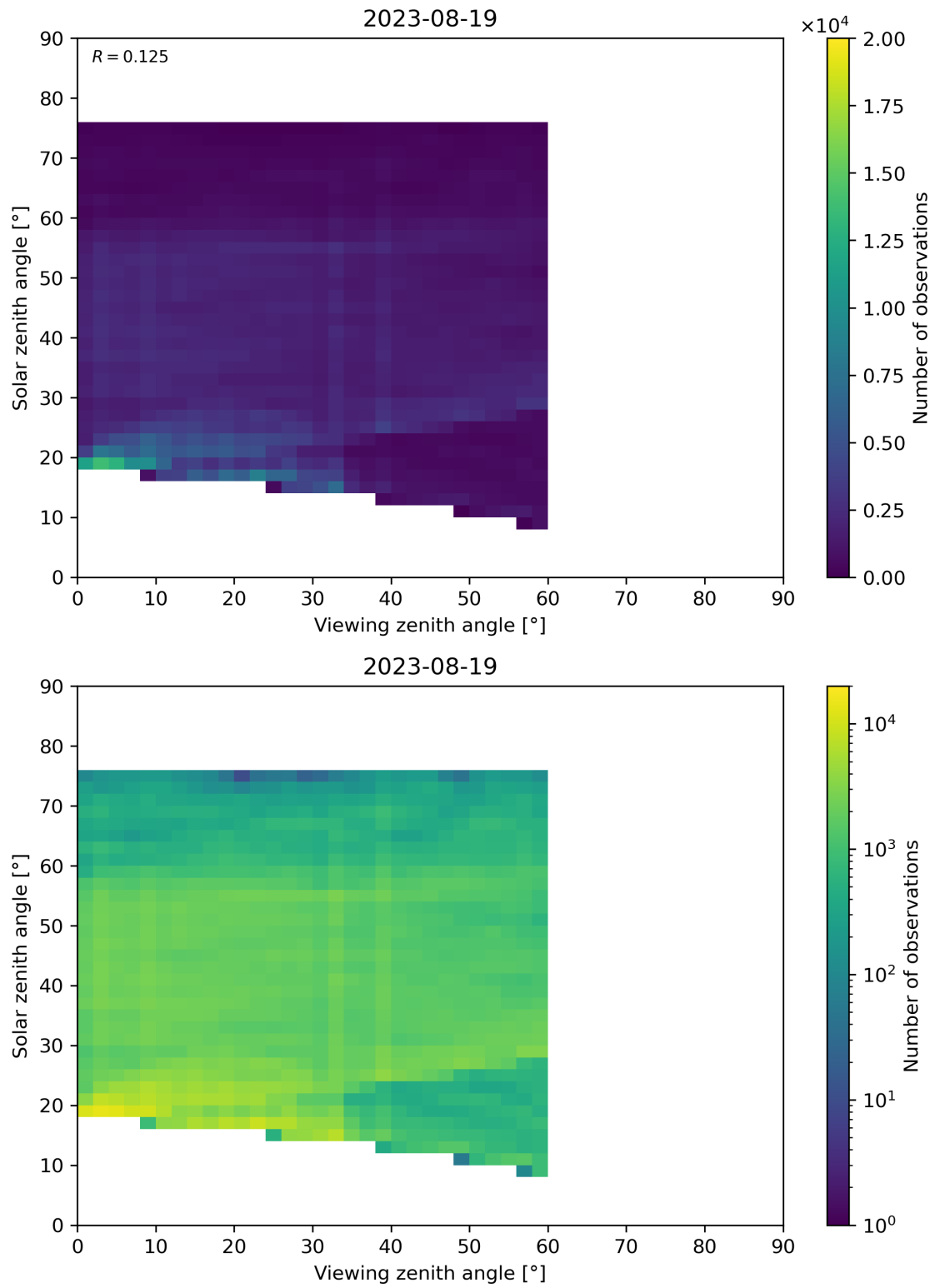
Figure 115: Scatter density plot of “Viewing zenith angle” against “Solar zenith angle” for 2023-08-18 to 2023-08-20.
