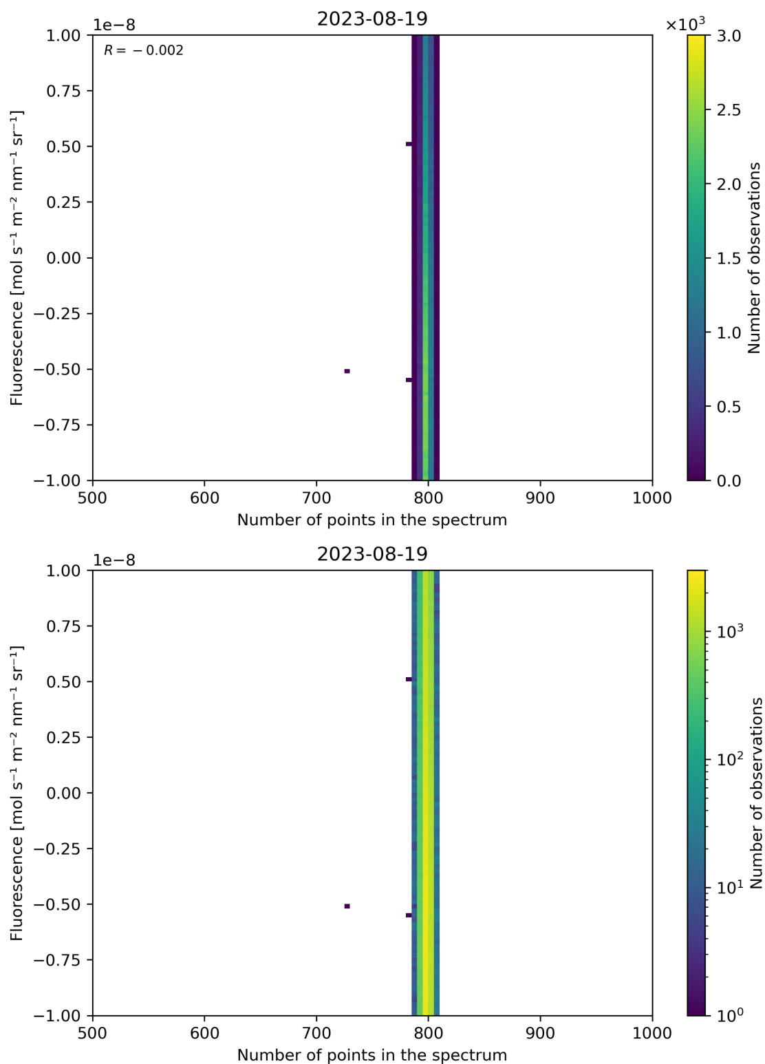
Figure 91: Scatter density plot of “Number of points in the spectrum” against “Fluorescence” for 2023-08-18 to 2023-08-20.
