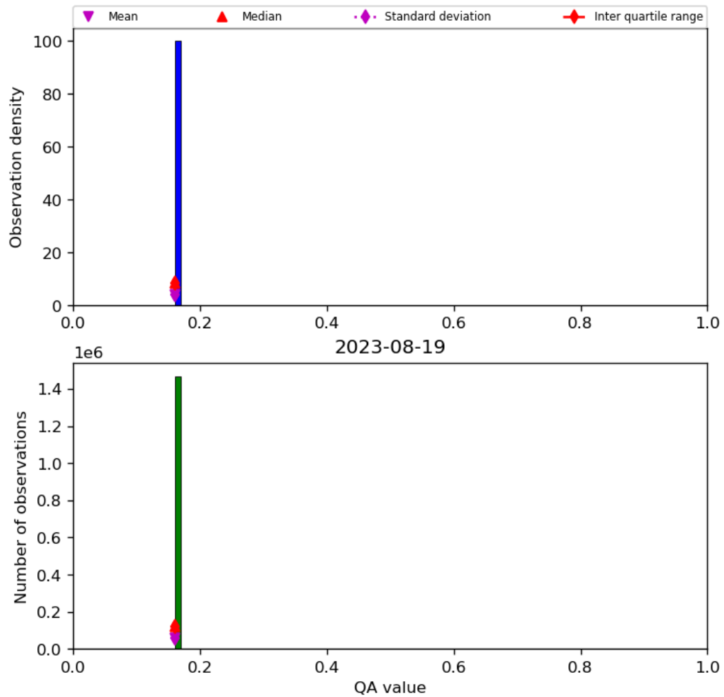
Figure 22: Histogram of “QA value” for 2023-08-18 to 2023-08-20
