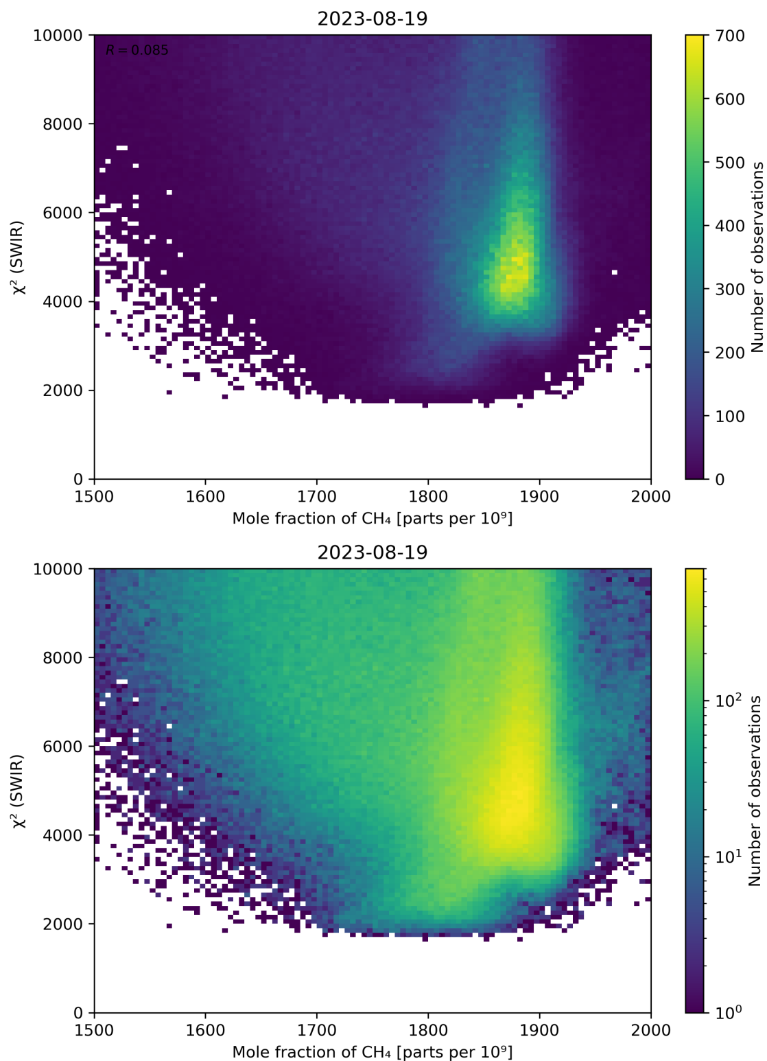
Figure 71: Scatter density plot of “Mole fraction of CH 4 ” against “ \chi^2 (SWIR)” for 2023-08-18 to 2023-08-20.
