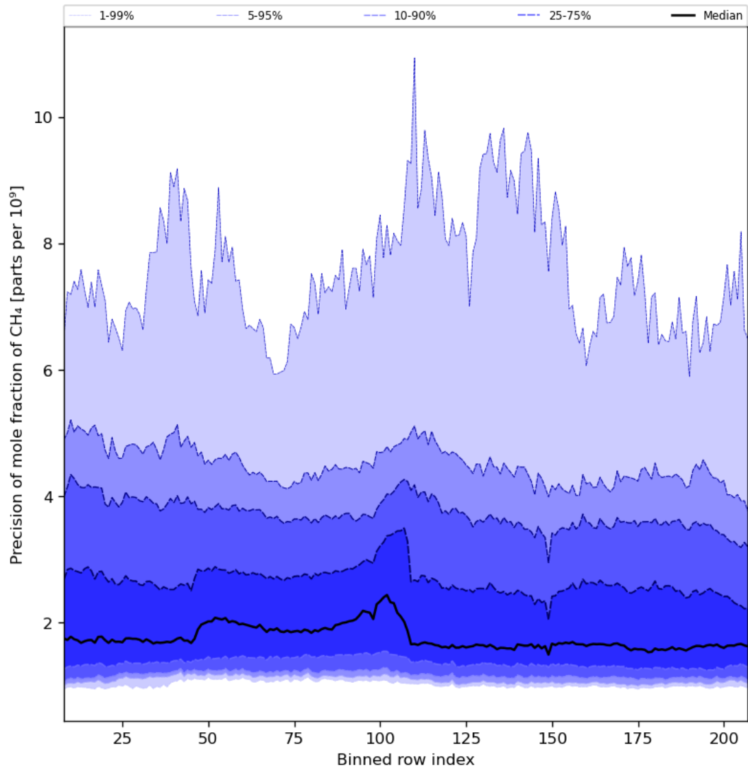
Figure 35: Along track statistics of “Precision of mole fraction of CH 4 ” for 2023-08-18 to 2023-08-20
