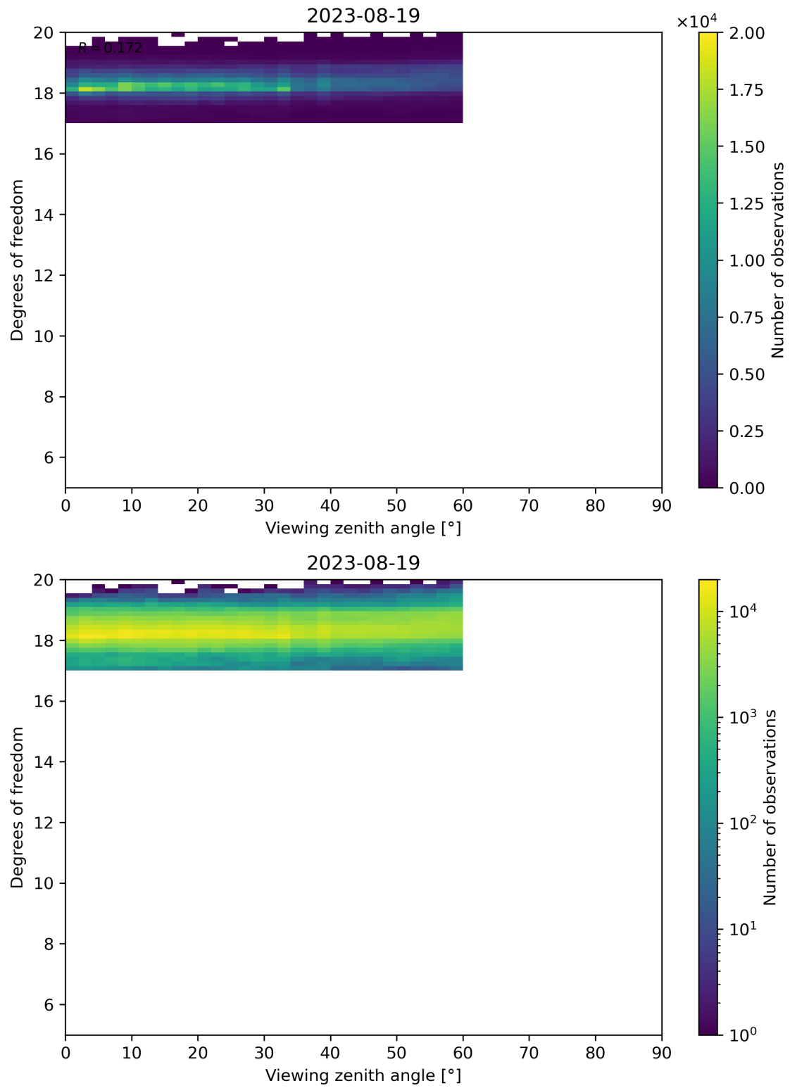
Figure 107: Scatter density plot of “Viewing zenith angle” against “Degrees of freedom” for 2023-08-18 to 2023-08-20.
