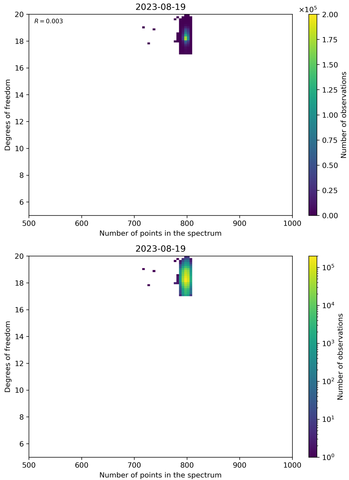
Figure 90: Scatter density plot of “Number of points in the spectrum” against “Degrees of freedom” for 2023-08-18 to 2023-08-20.
