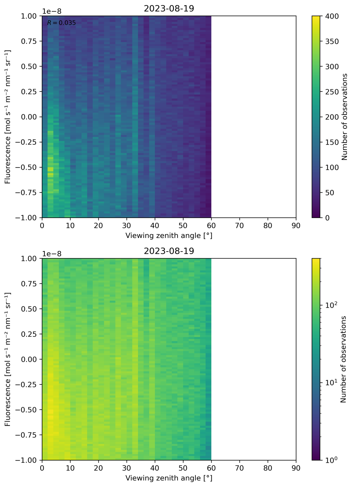
Figure 108: Scatter density plot of “Viewing zenith angle” against “Fluorescence” for 2023-08-18 to 2023-08-20.
