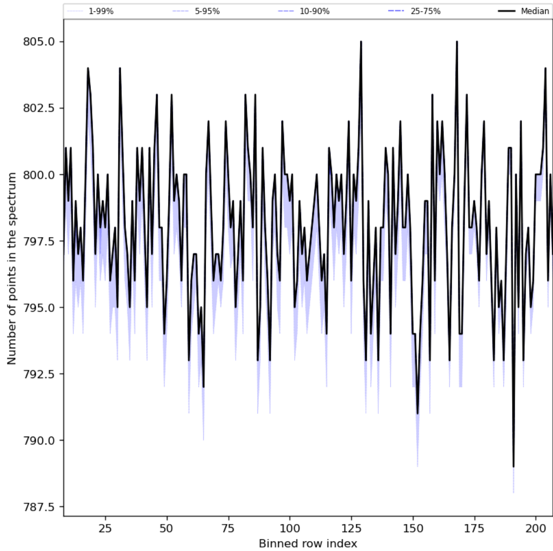
Figure 37: Along track statistics of “Number of points in the spectrum” for 2023-08-18 to 2023-08-20
