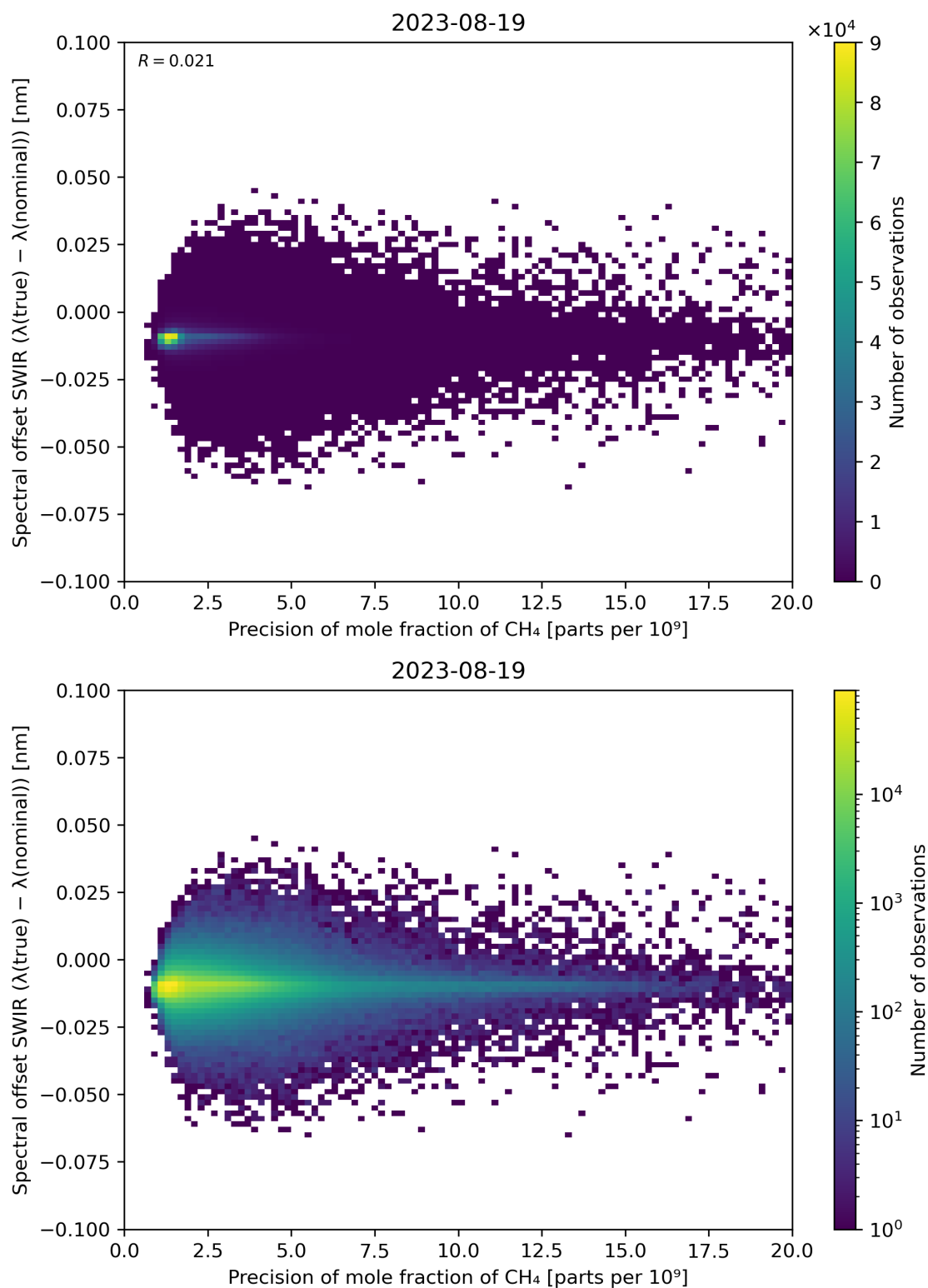
Figure 85: Scatter density plot of “Precision of mole fraction of \text{CH}_4 ” against “Spectral offset SWIR ( \lambda(\text{true}) - \lambda(\text{nominal}) )” for 2023-08-18 to 2023-08-20.
