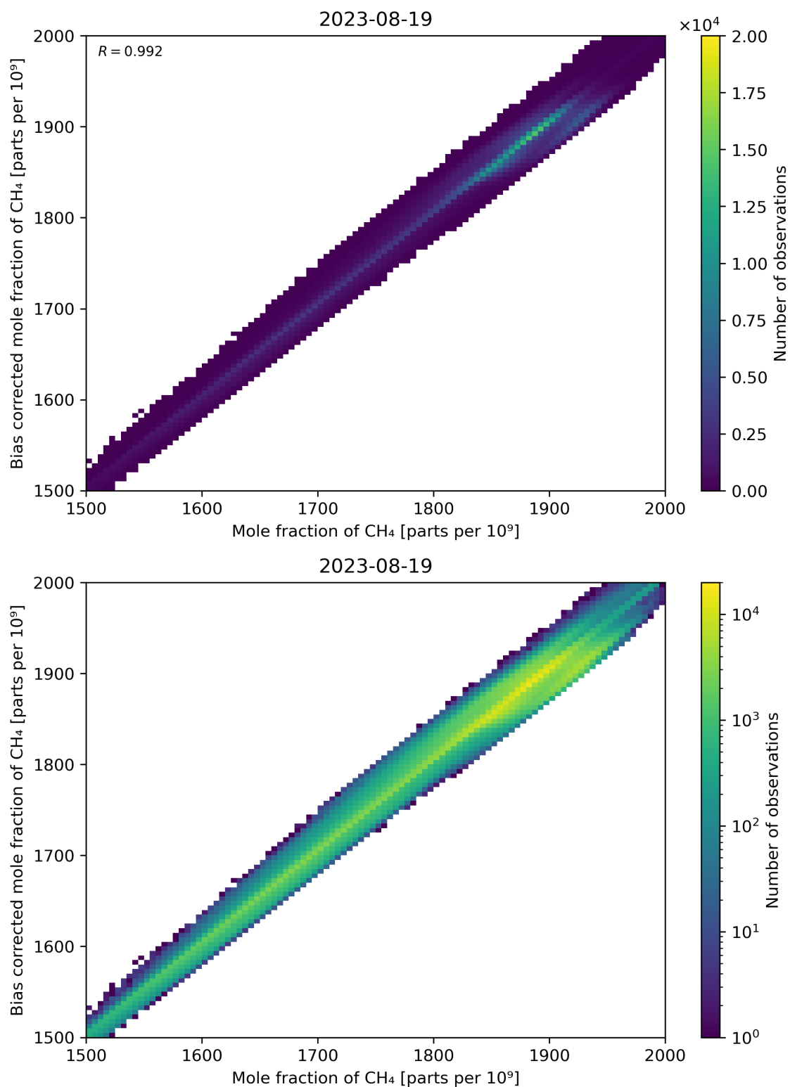
Figure 74: Scatter density plot of “Mole fraction of CH 4 ” against “Bias corrected mole fraction of CH 4 ” for 2023-08-18 to 2023-08-20.
