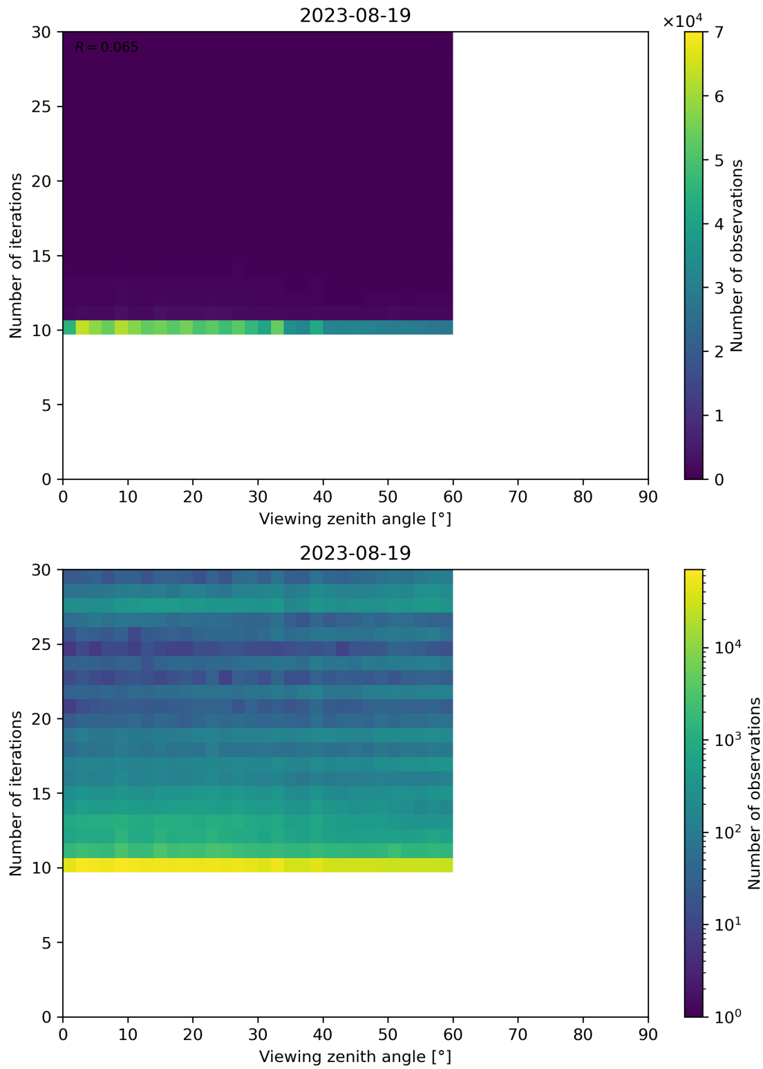
Figure 113: Scatter density plot of “Viewing zenith angle” against “Number of iterations” for 2023-08-18 to 2023-08-20.
