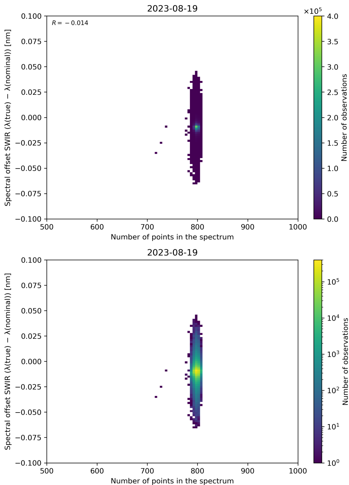
Figure 93: Scatter density plot of “Number of points in the spectrum” against “Spectral offset SWIR ( \lambda(\text{true}) - \lambda(\text{nominal}) )” for 2023-08-18 to 2023-08-20.
