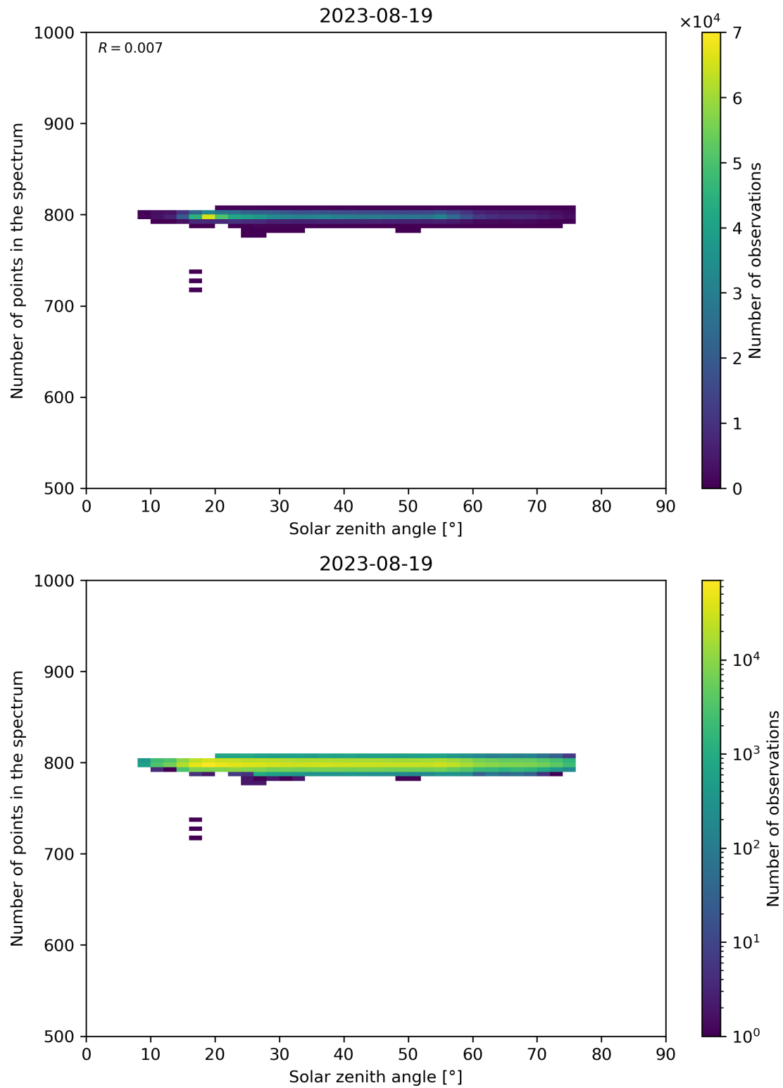
Figure 103: Scatter density plot of “Solar zenith angle” against “Number of points in the spectrum” for 2023-08-18 to 2023-08-20.
