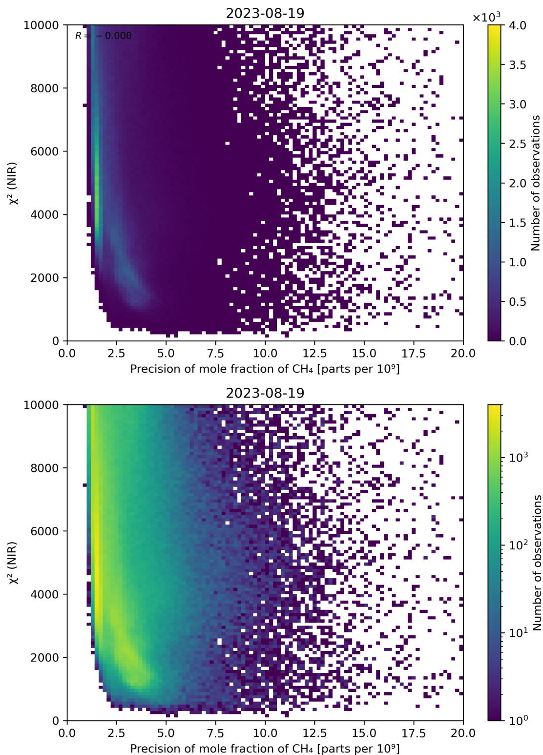
Figure 78: Scatter density plot of “Precision of mole fraction of CH 4 ” against “ \chi^2 (NIR)” for 2023-08-18 to 2023-08-20.
