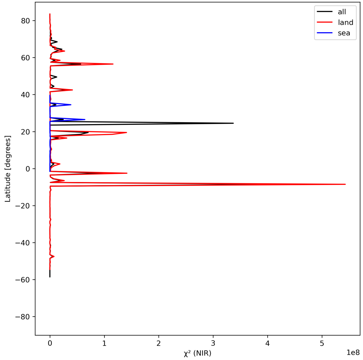
Figure 18: Zonal average of “ \chi^2 (NIR)” for 2023-08-18 to 2023-08-20.
