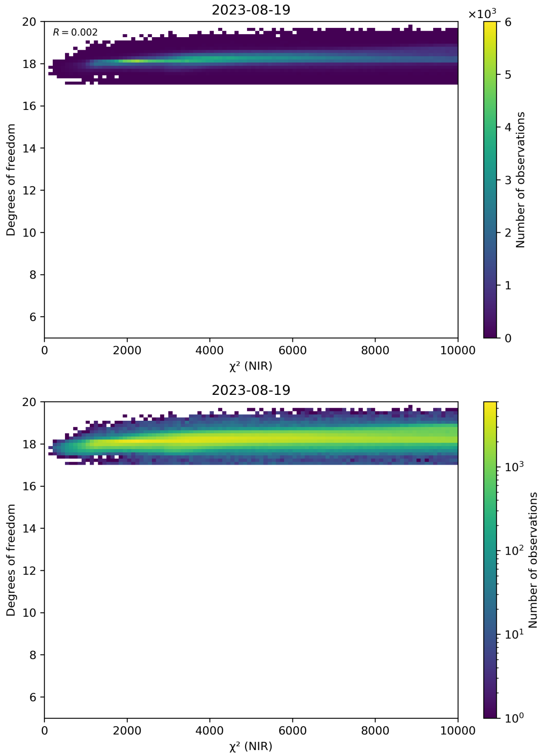
Figure 44: Scatter density plot of “ \chi^2 (NIR)” against “Degrees of freedom” for 2023-08-18 to 2023-08-20.
