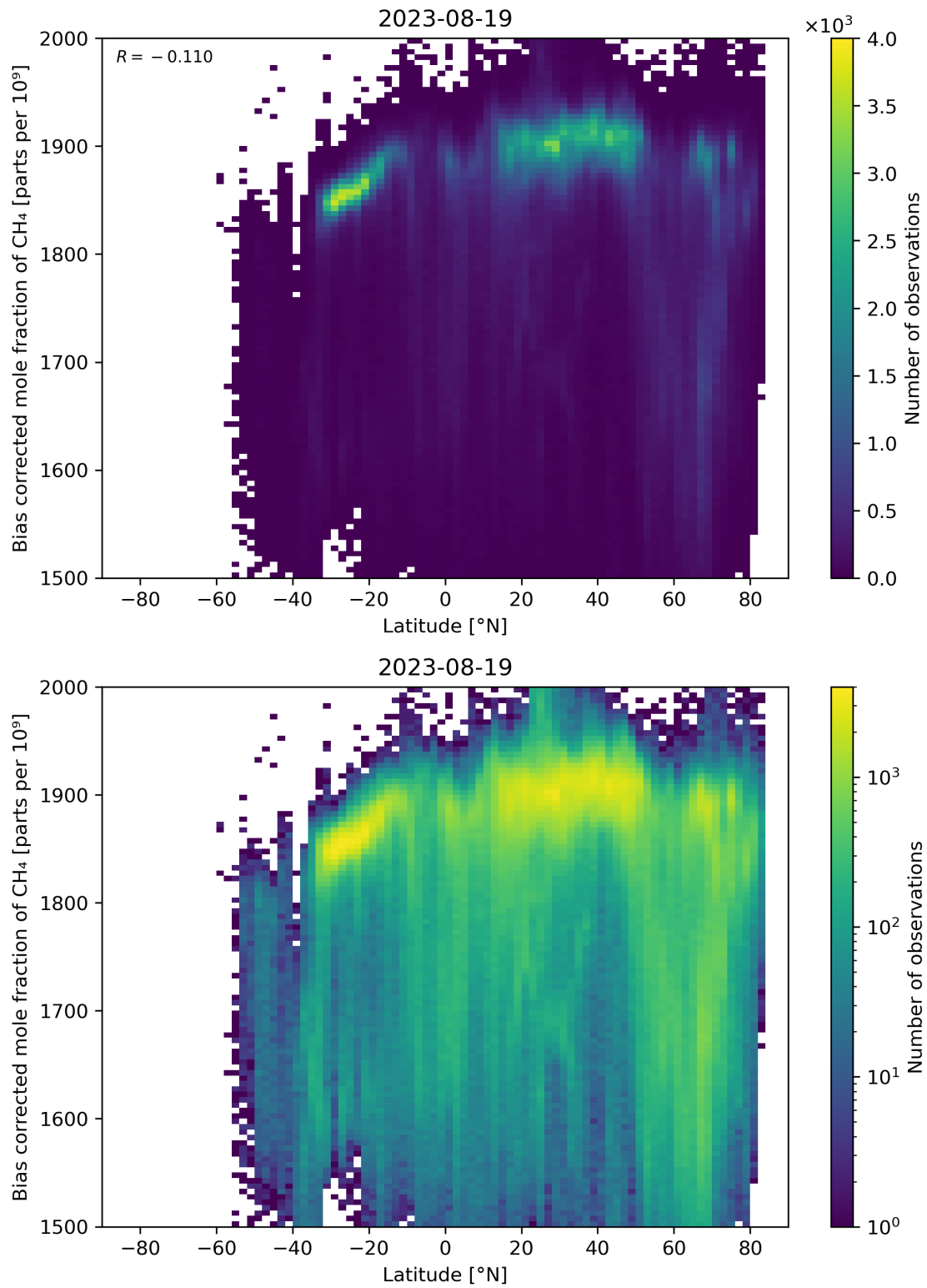
Figure 58: Scatter density plot of “Latitude” against “Bias corrected mole fraction of \text{CH}_4 ” for 2023-08-18 to 2023-08-20.
