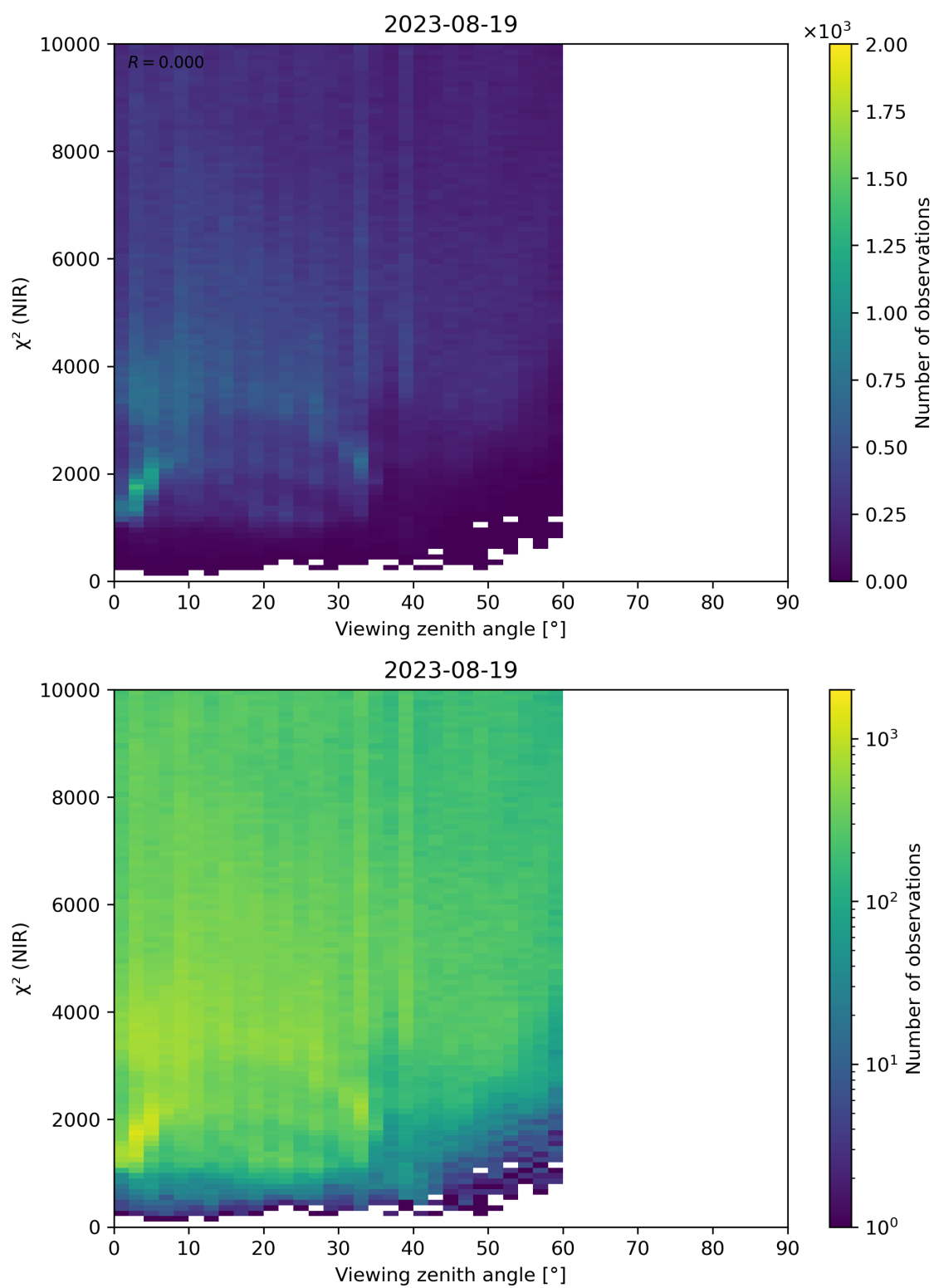
Figure 105: Scatter density plot of “Viewing zenith angle” against “ \chi^2 (NIR)” for 2023-08-18 to 2023-08-20.
