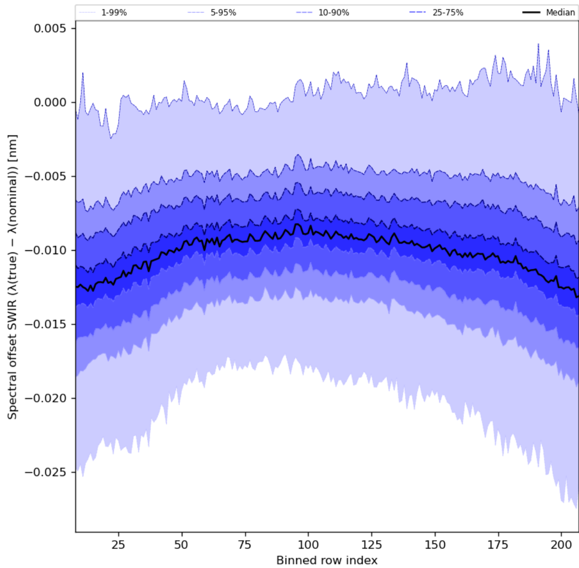
Figure 38: Along track statistics of “Spectral offset SWIR ( \lambda(\text{true}) - \lambda(\text{nominal}) )” for 2023-08-18 to 2023-08-20
