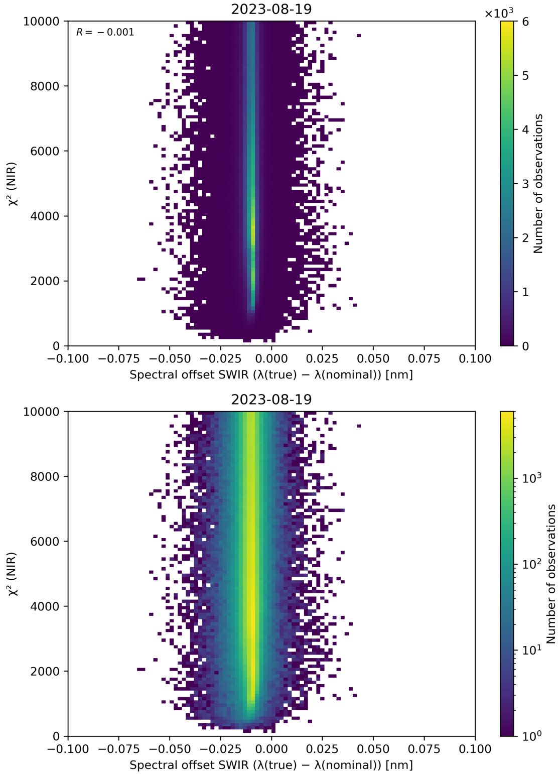
Figure 117: Scatter density plot of “Spectral offset SWIR ( \lambda(\text{true}) - \lambda(\text{nominal}) )” against “ \chi^2 (NIR)” for 2023-08-18 to 2023-08-20.
