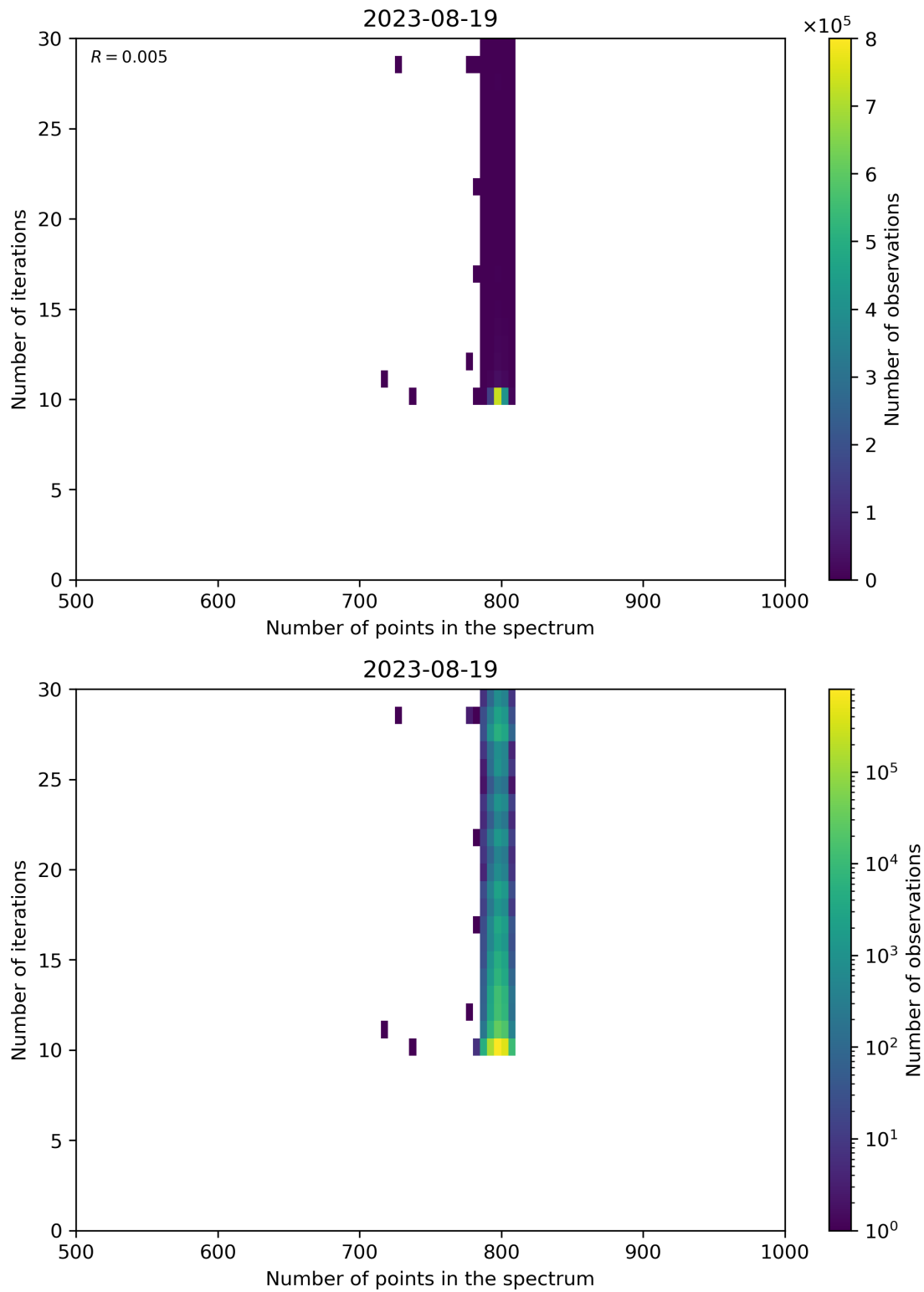
Figure 92: Scatter density plot of “Number of points in the spectrum” against “Number of iterations” for 2023-08-18 to 2023-08-20.
