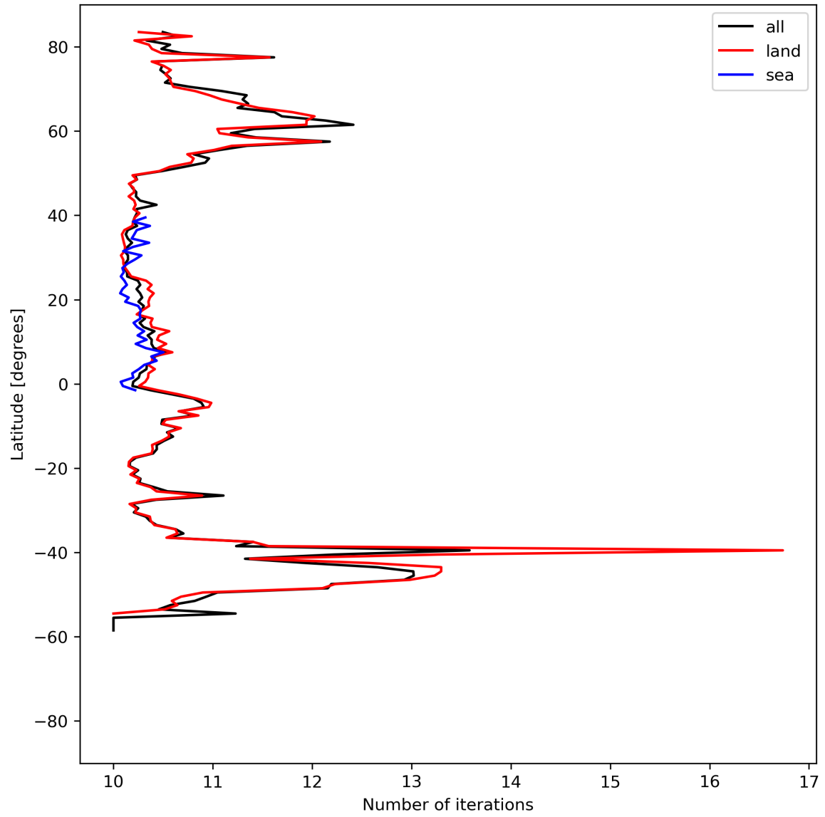
Figure 20: Zonal average of “Number of iterations” for 2023-08-18 to 2023-08-20.
