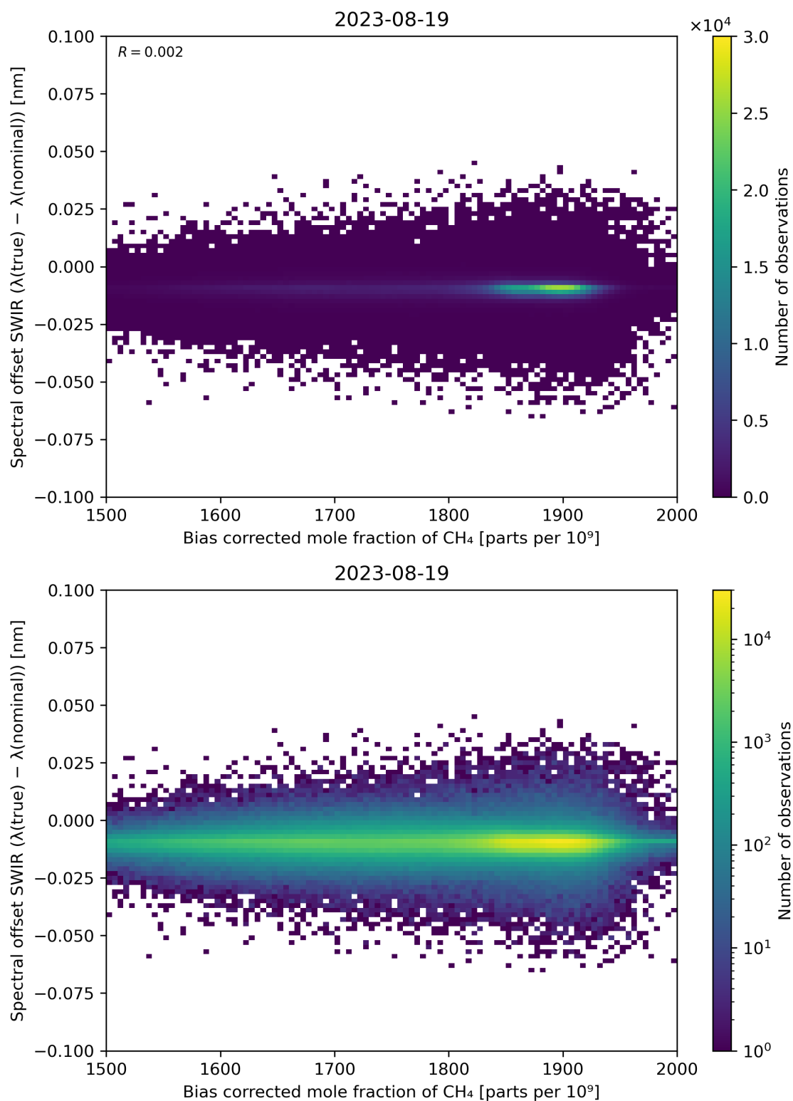
Figure 69: Scatter density plot of “Bias corrected mole fraction of \text{CH}_4 ” against “Spectral offset SWIR ( \lambda(\text{true}) - \lambda(\text{nominal}) )” for 2023-08-18 to 2023-08-20.
