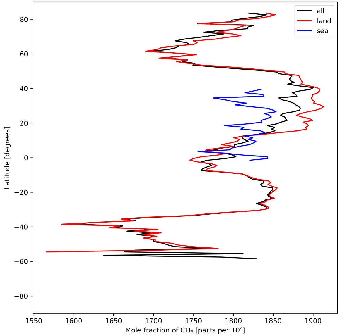
Figure 12: Zonal average of “Mole fraction of CH 4 ” for 2023-08-18 to 2023-08-20.
