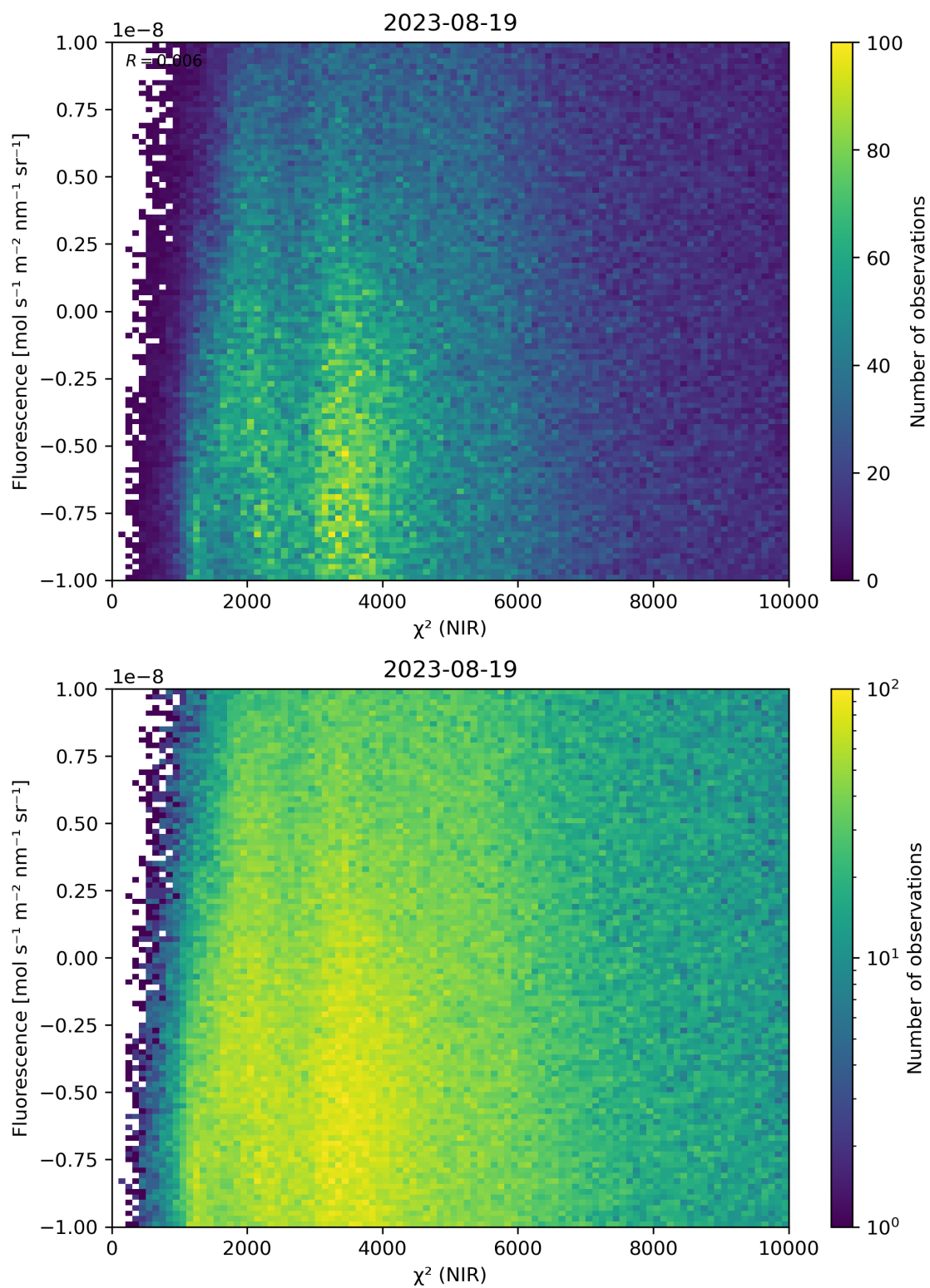
Figure 45: Scatter density plot of “ \chi^2 (NIR)” against “Fluorescence” for 2023-08-18 to 2023-08-20.
