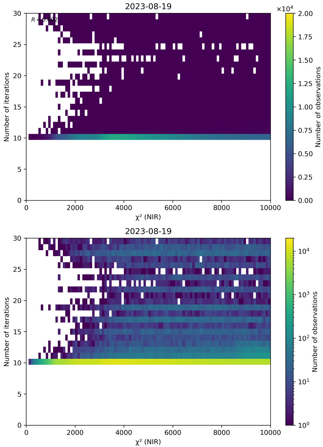
Figure 46: Scatter density plot of “ \chi^2 (NIR)” against “Number of iterations” for 2023-08-18 to 2023-08-20.
