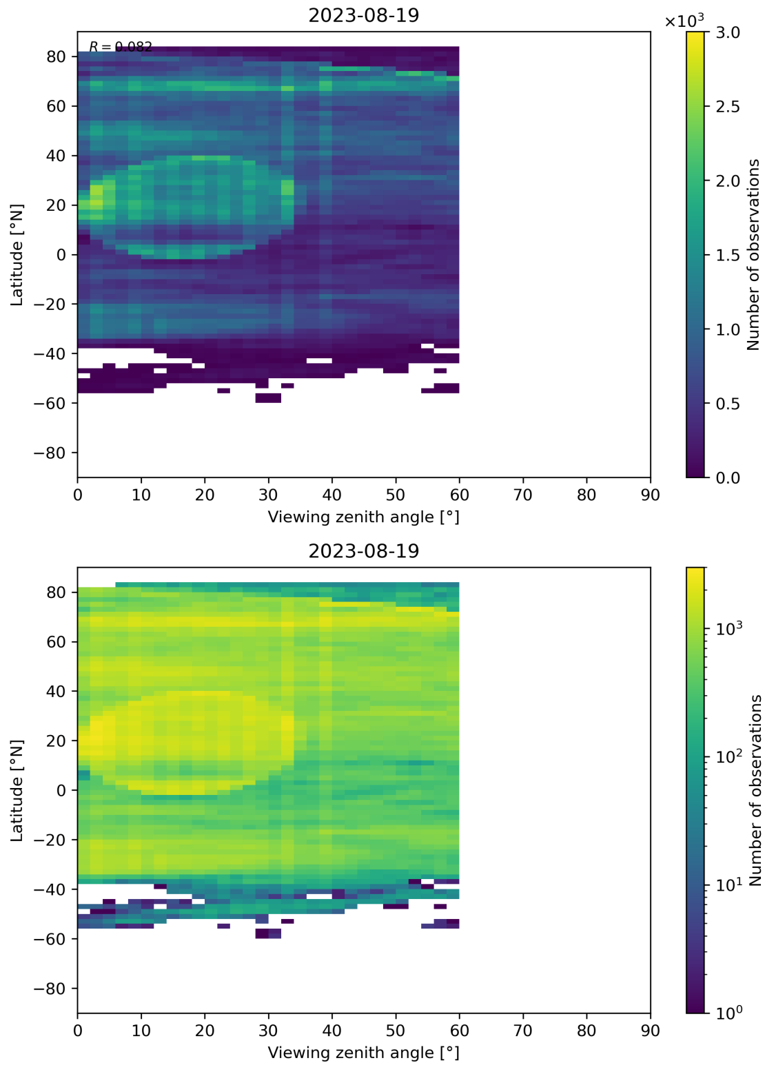
Figure 109: Scatter density plot of “Viewing zenith angle” against “Latitude” for 2023-08-18 to 2023-08-20.
