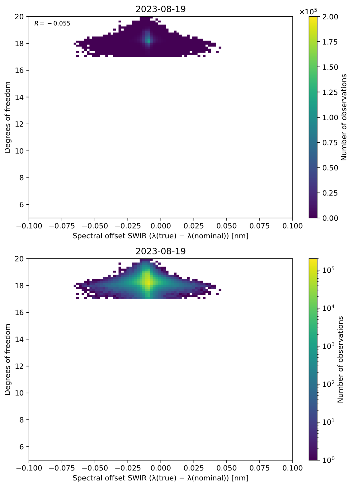
Figure 119: Scatter density plot of “Spectral offset SWIR ( \lambda(\text{true}) - \lambda(\text{nominal}) )” against “Degrees of freedom” for 2023-08-18 to 2023-08-20.
