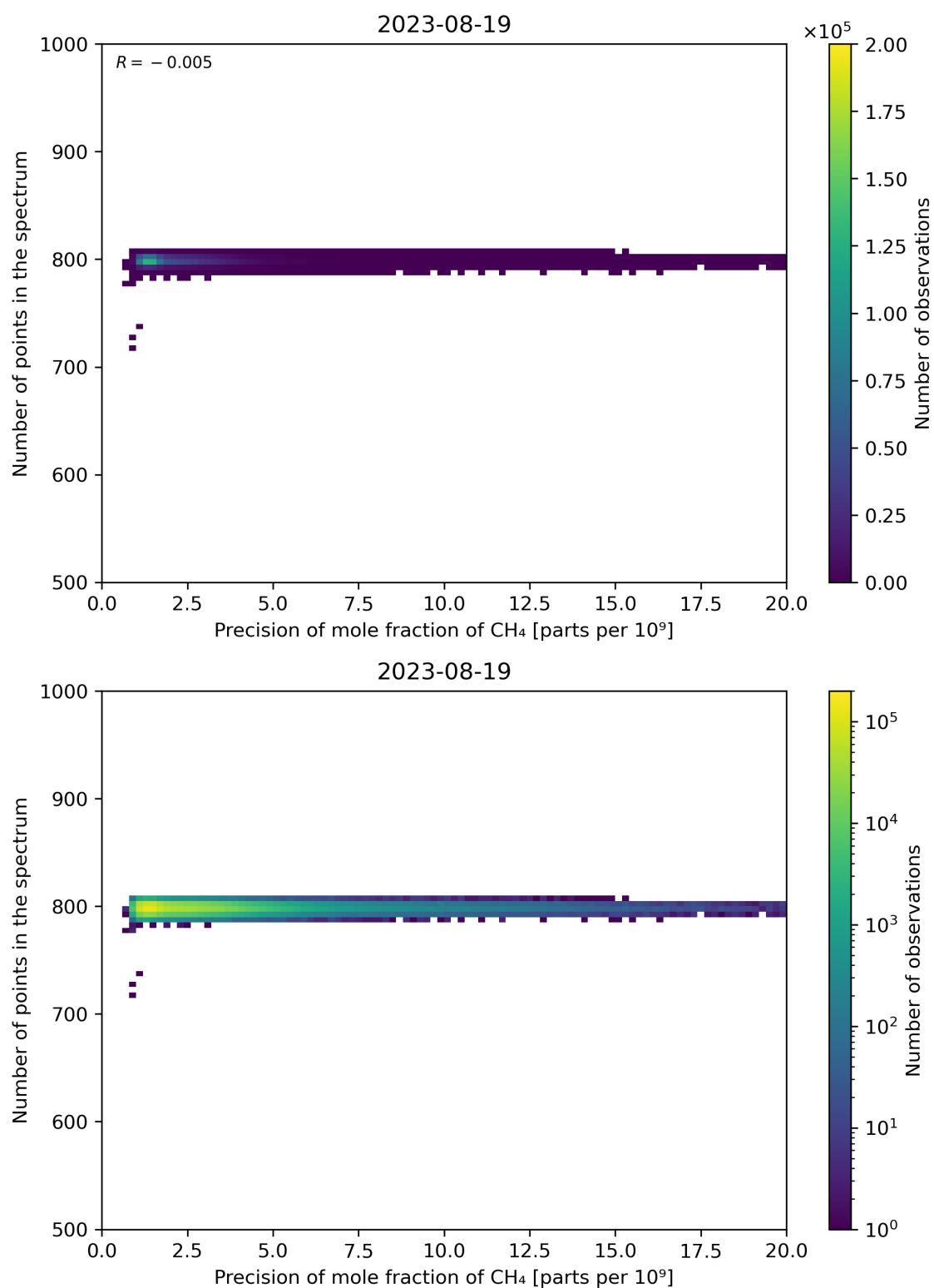
Figure 84: Scatter density plot of “Precision of mole fraction of CH 4 ” against “Number of points in the spectrum” for 2023-08-18 to 2023-08-20.
