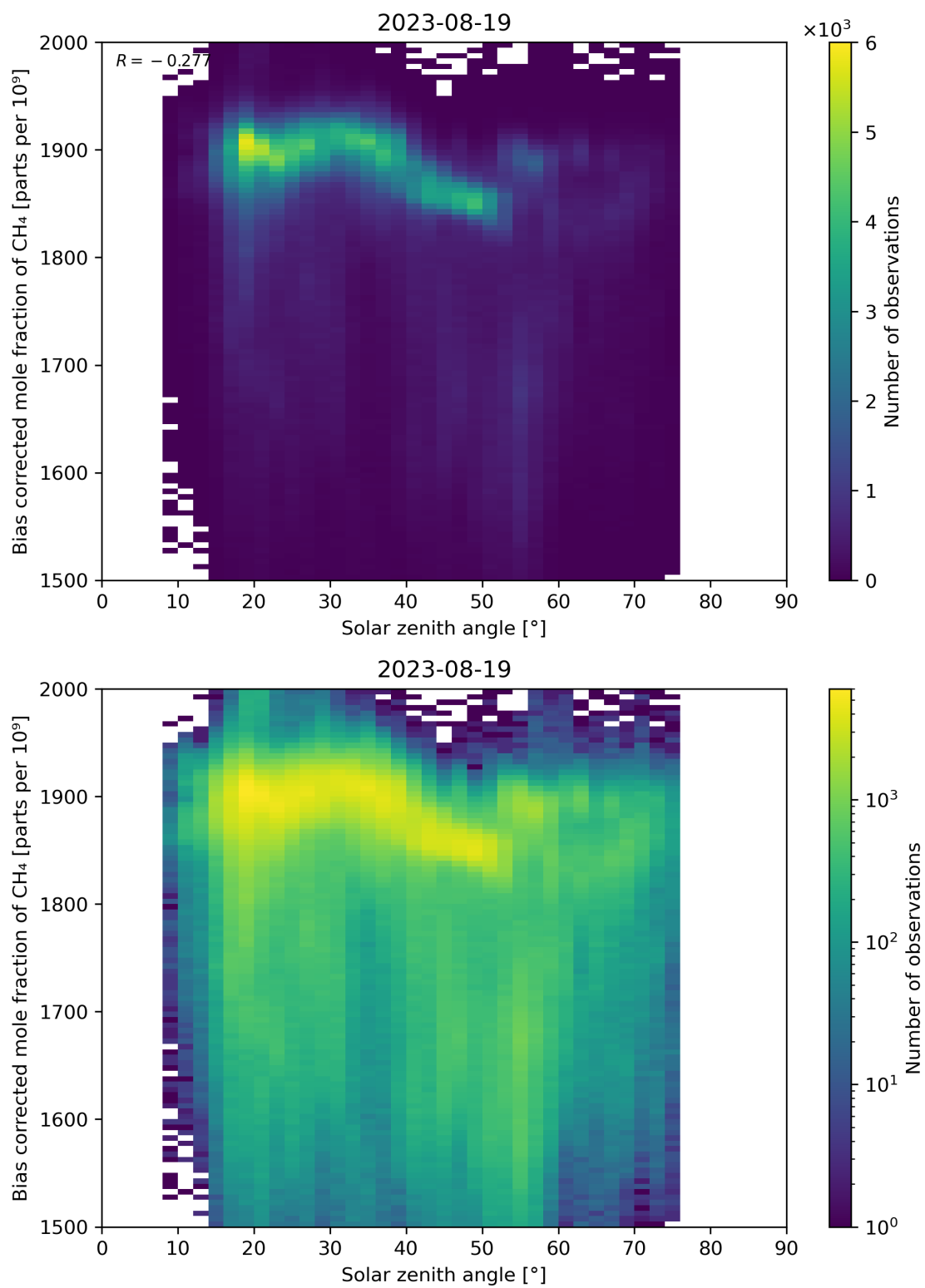
Figure 100: Scatter density plot of “Solar zenith angle” against “Bias corrected mole fraction of CH 4 ” for 2023-08-18 to 2023-08-20.
