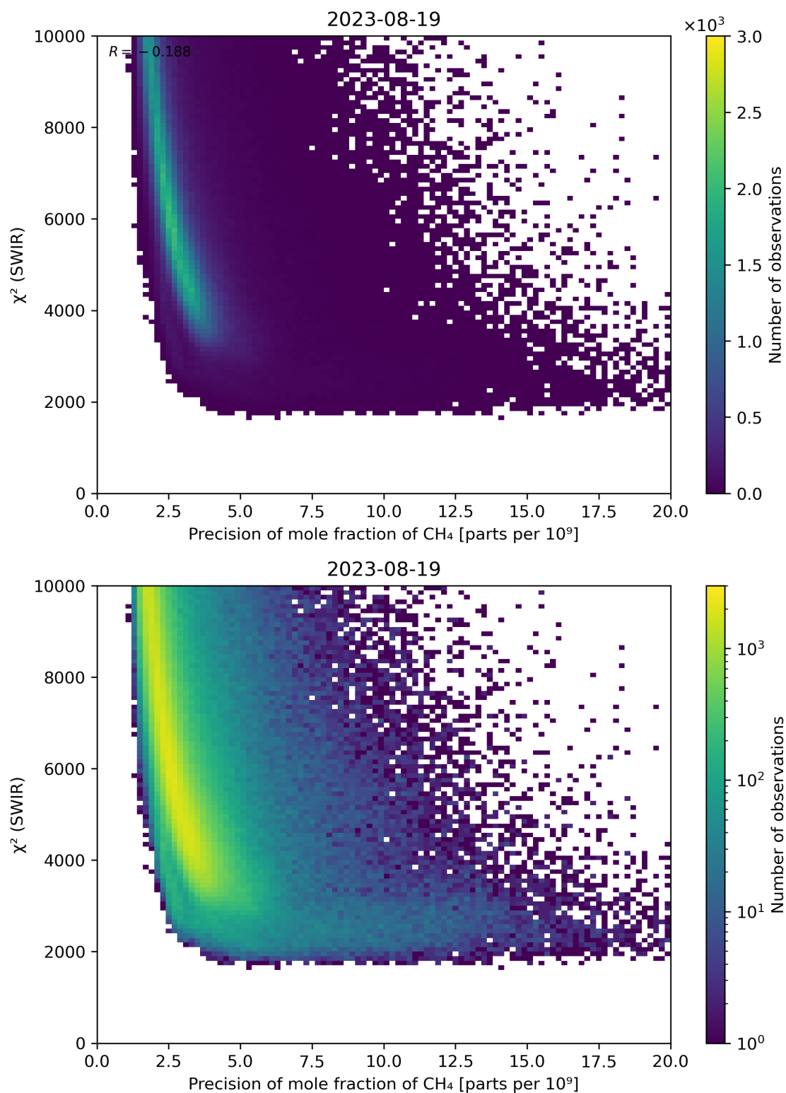
Figure 79: Scatter density plot of “Precision of mole fraction of \text{CH}_4 ” against “ \chi^2 (SWIR)” for 2023-08-18 to 2023-08-20.
