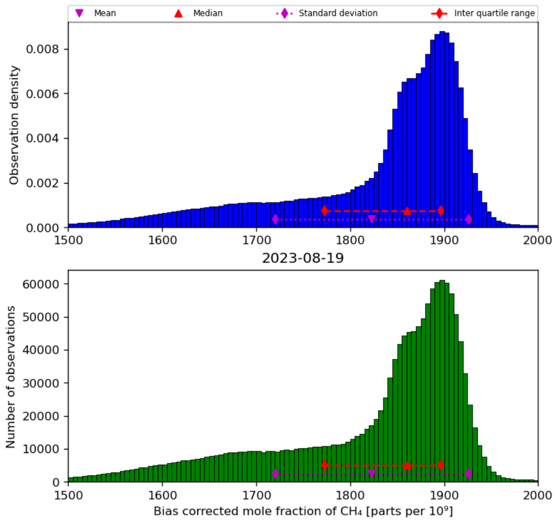
Figure 25: Histogram of “Bias corrected mole fraction of CH 4 ” for 2023-08-18 to 2023-08-20
