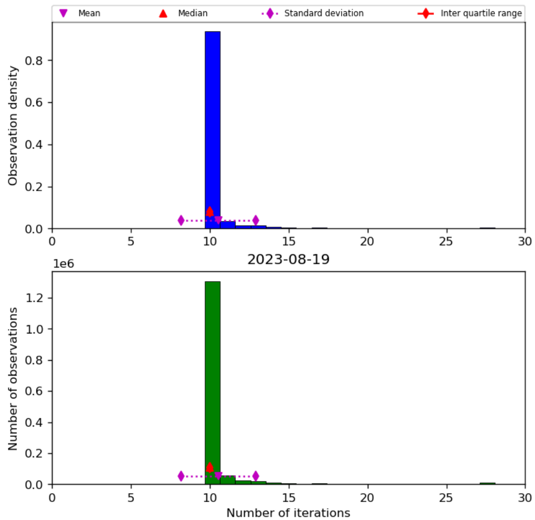
Figure 31: Histogram of “Number of iterations” for 2023-08-18 to 2023-08-20
