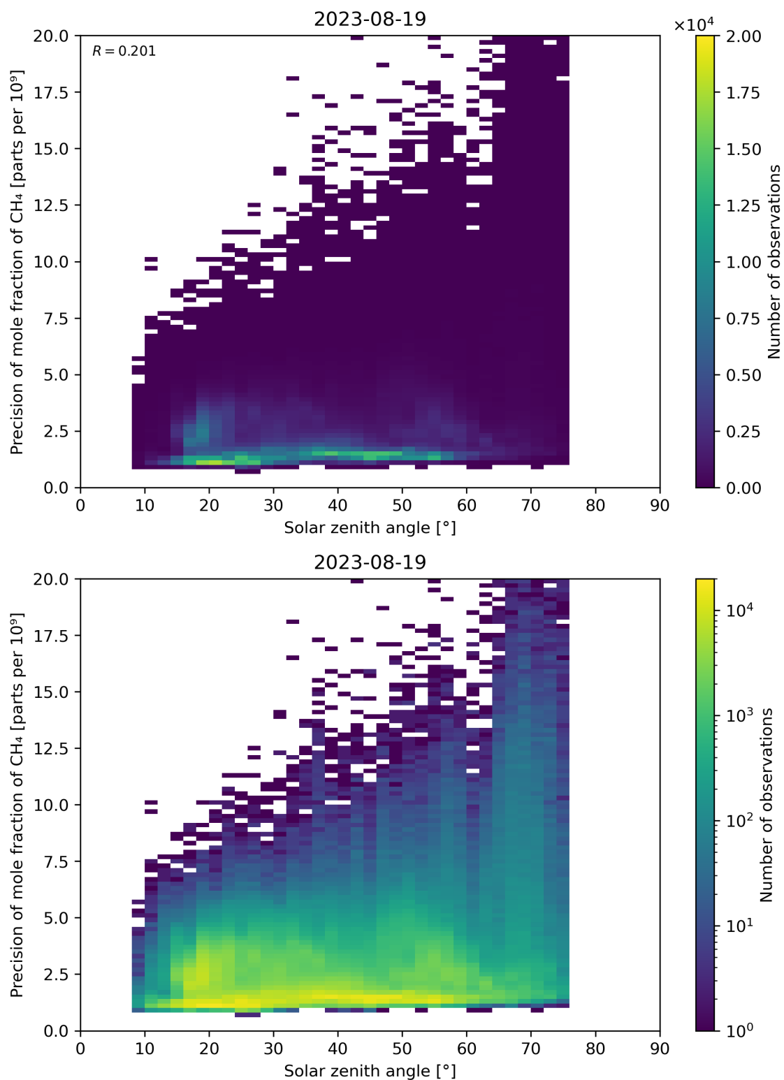
Figure 101: Scatter density plot of “Solar zenith angle” against “Precision of mole fraction of \text{CH}_4 ” for 2023-08-18 to 2023-08-20.
