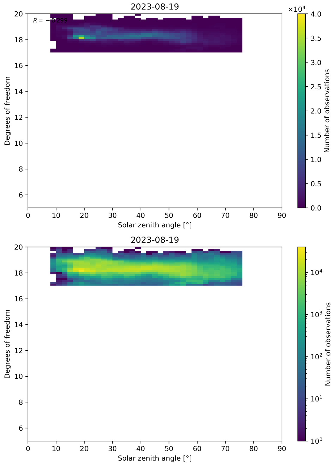
Figure 96: Scatter density plot of “Solar zenith angle” against “Degrees of freedom” for 2023-08-18 to 2023-08-20.
