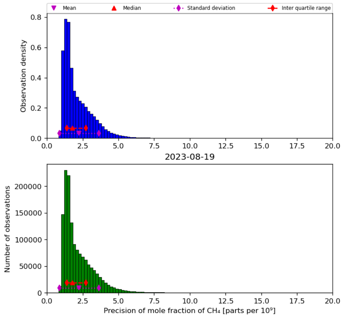
Figure 24: Histogram of “Precision of mole fraction of CH 4 ” for 2023-08-18 to 2023-08-20
