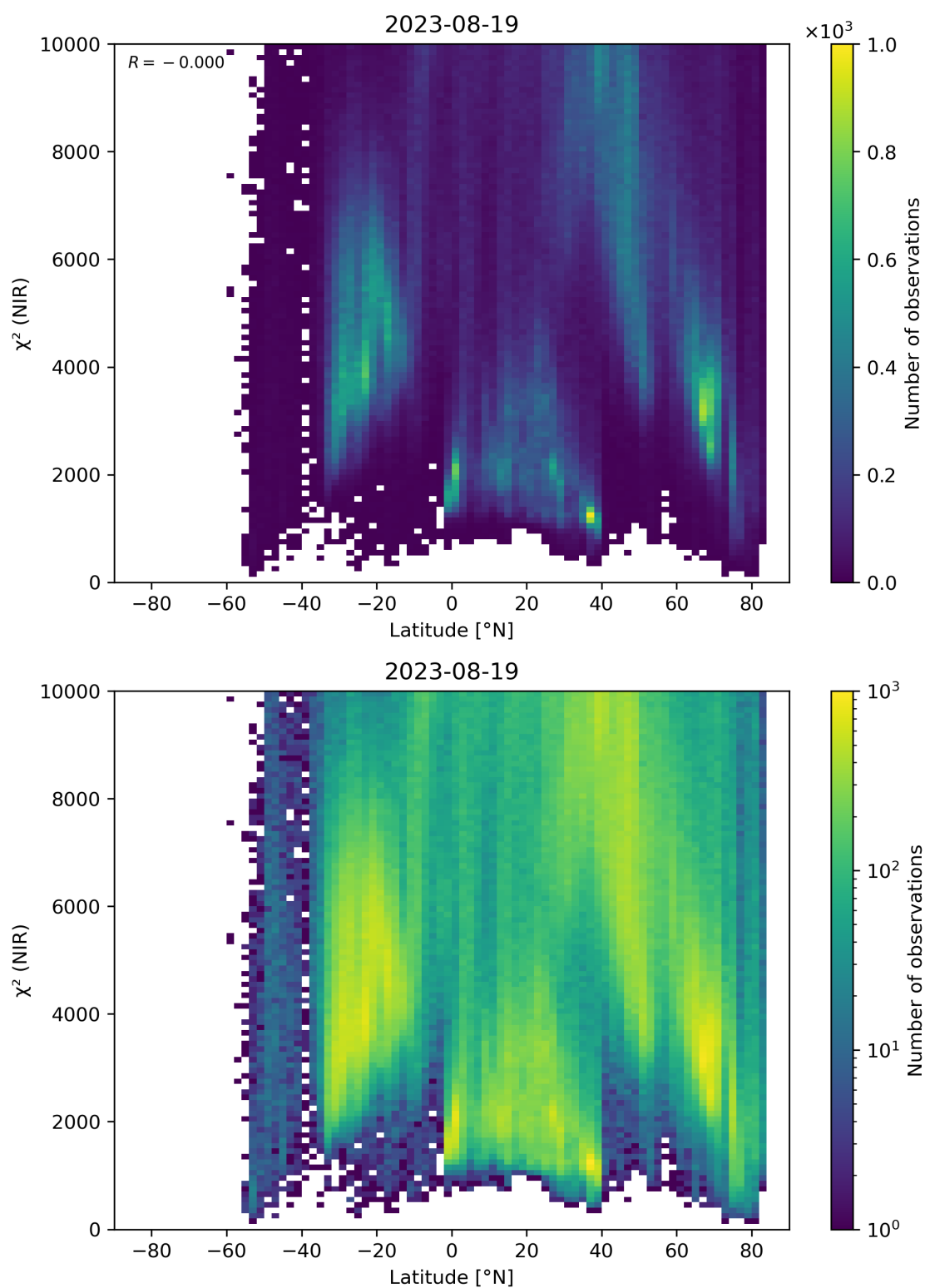
Figure 53: Scatter density plot of “Latitude” against “ \chi^2 (NIR)” for 2023-08-18 to 2023-08-20.
