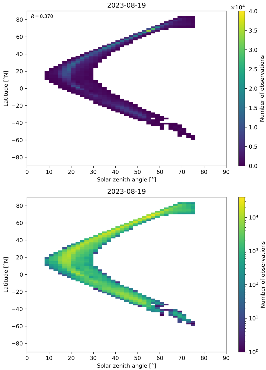
Figure 98: Scatter density plot of “Solar zenith angle” against “Latitude” for 2023-08-18 to 2023-08-20.
