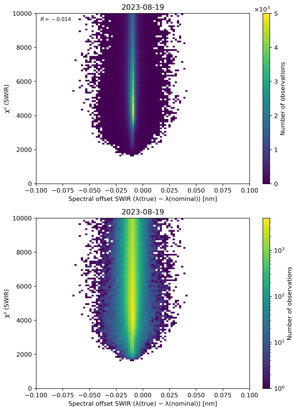
Figure 118: Scatter density plot of “Spectral offset SWIR ( \lambda(\text{true}) - \lambda(\text{nominal}) )” against “ \chi^2 (SWIR)” for 2023-08-18 to 2023-08-20.
