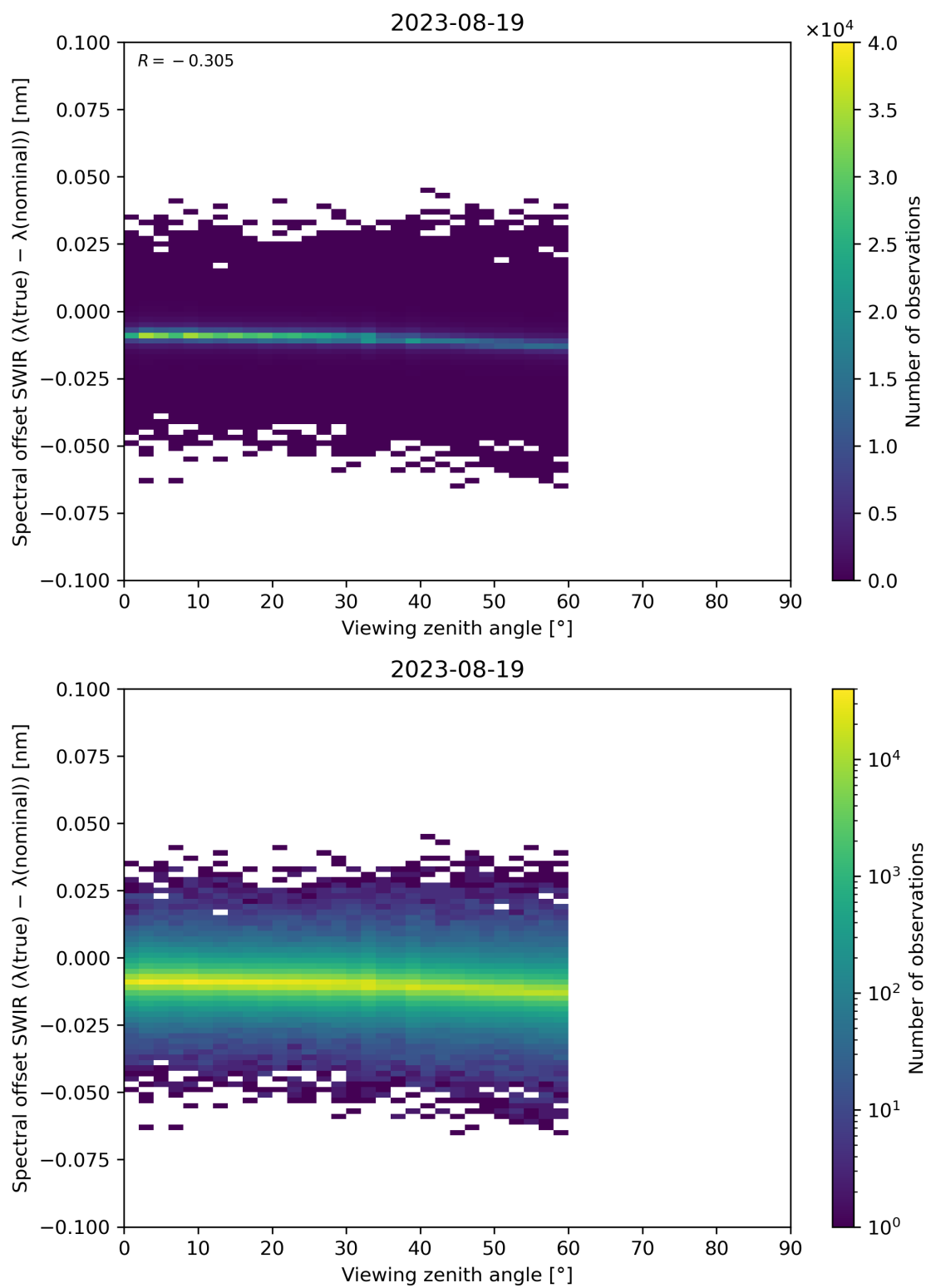
Figure 116: Scatter density plot of “Viewing zenith angle” against “Spectral offset SWIR ( \lambda(\text{true}) - \lambda(\text{nominal}) )” for 2023-08-18 to 2023-08-20.
