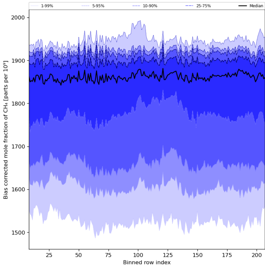
Figure 36: Along track statistics of “Bias corrected mole fraction of CH 4 ” for 2023-08-18 to 2023-08-20
