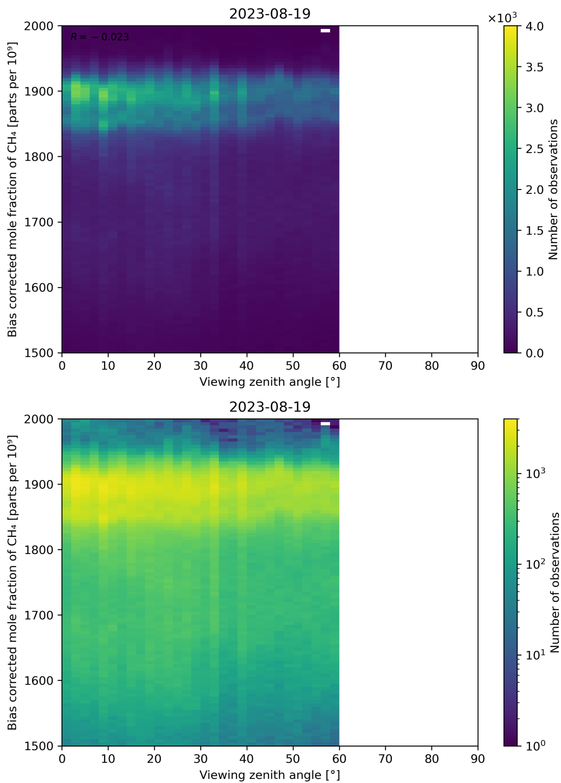
Figure 111: Scatter density plot of “Viewing zenith angle” against “Bias corrected mole fraction of CH 4 ” for 2023-08-18 to 2023-08-20.
