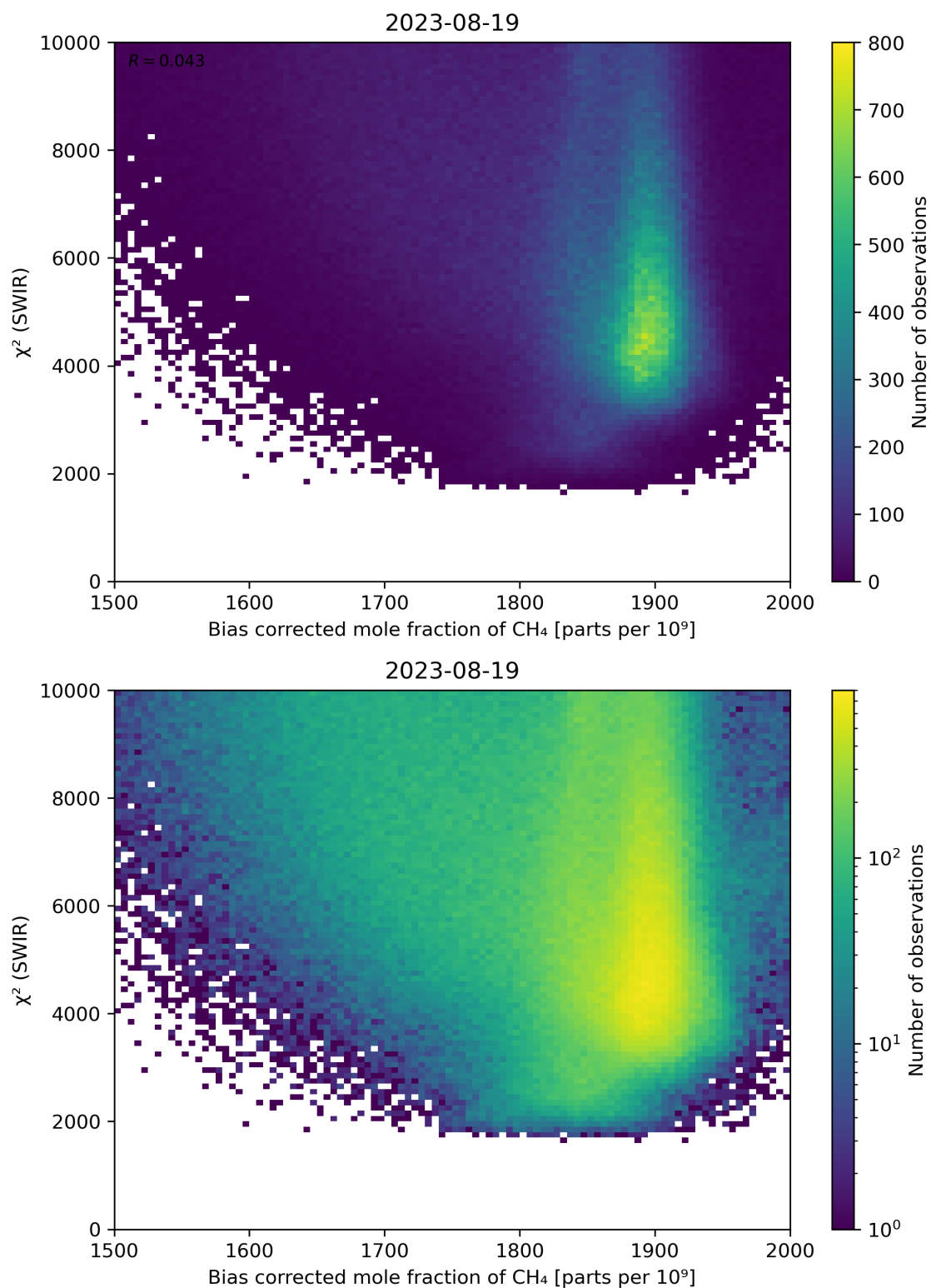
Figure 64: Scatter density plot of “Bias corrected mole fraction of \text{CH}_4 ” against “ \chi^2 (SWIR)” for 2023-08-18 to 2023-08-20.
