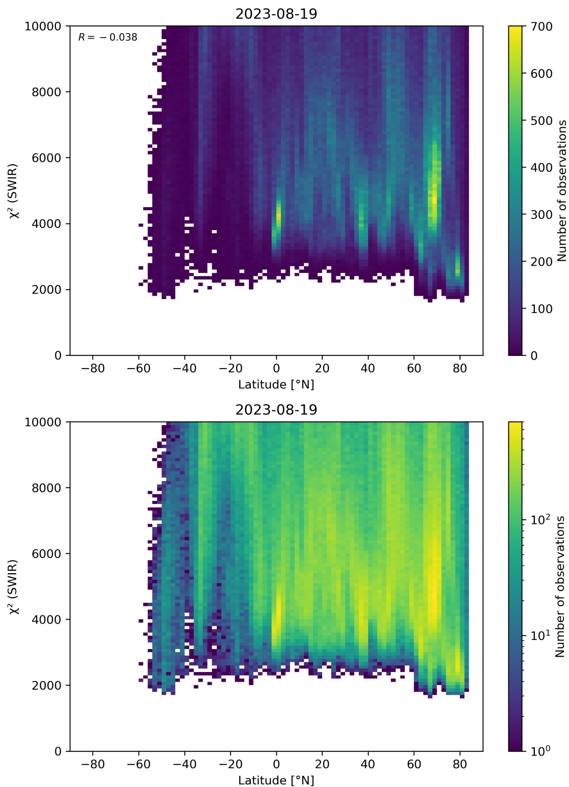
Figure 54: Scatter density plot of “Latitude” against “ \chi^2 (SWIR)” for 2023-08-18 to 2023-08-20.
