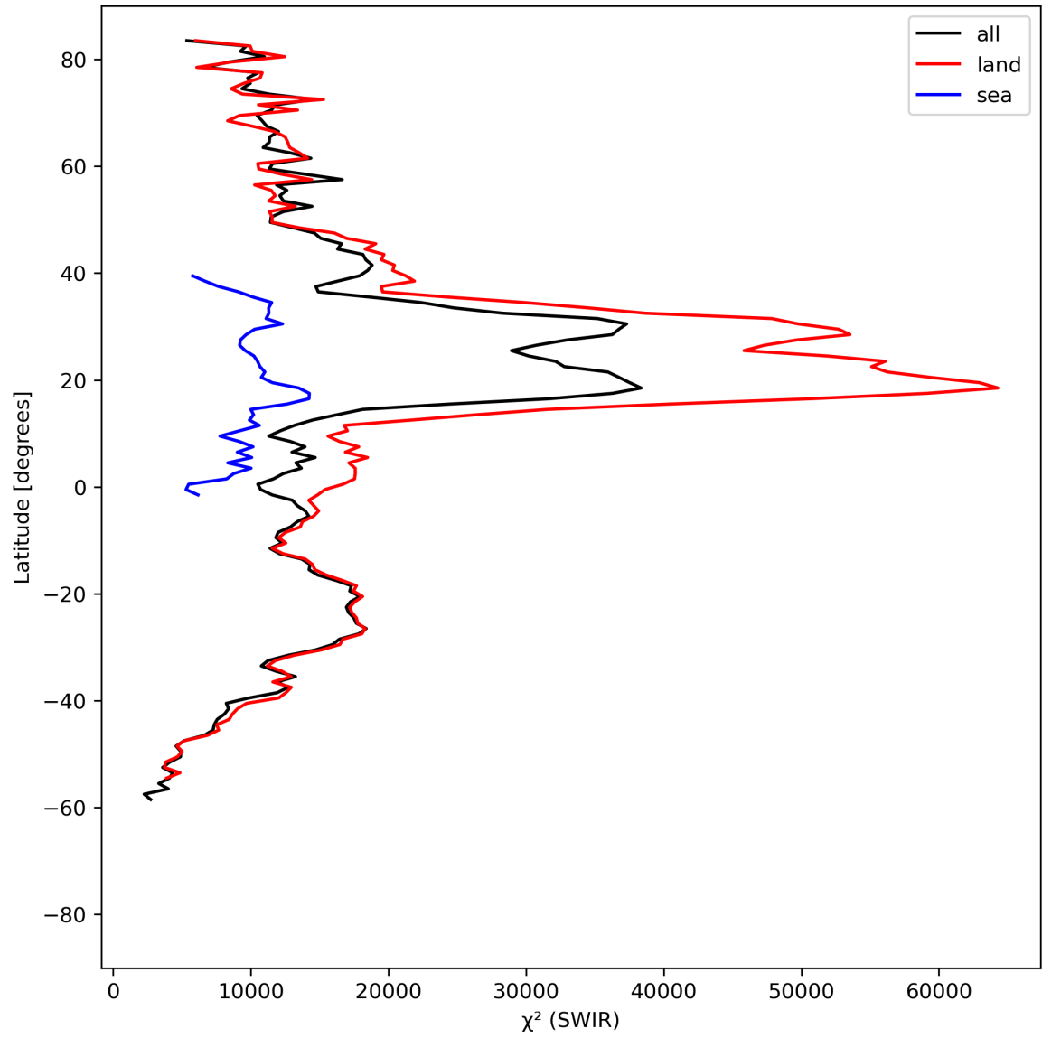
Figure 17: Zonal average of “ \chi^2 (SWIR)” for 2023-08-18 to 2023-08-20.
