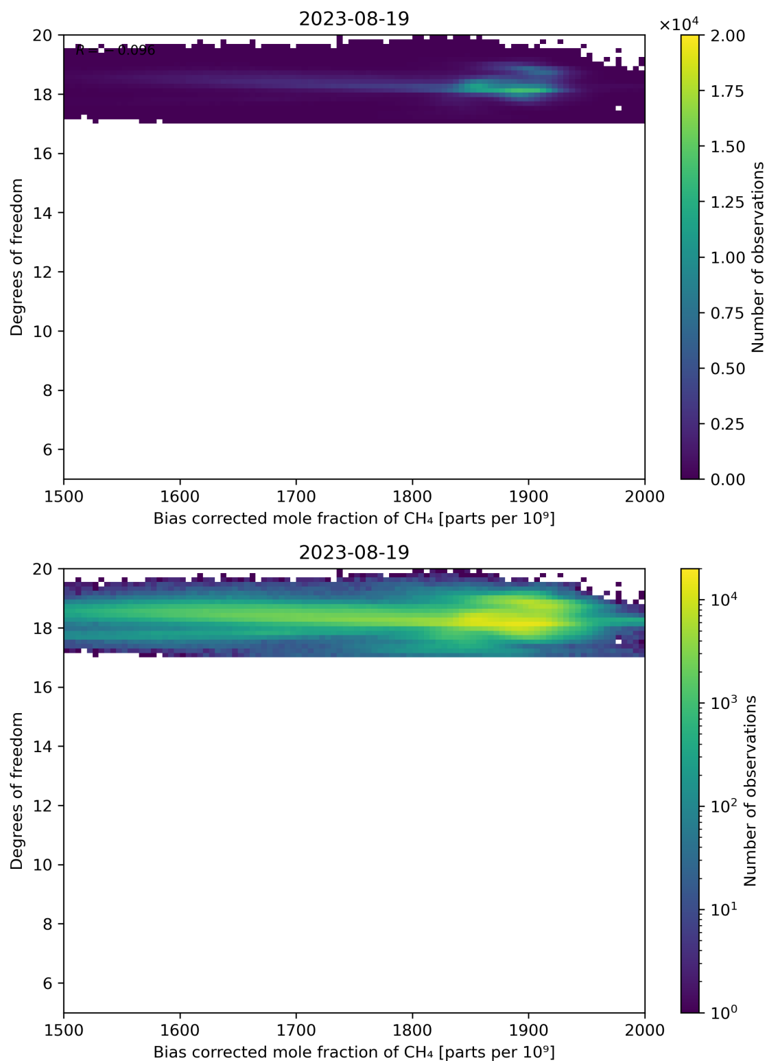
Figure 65: Scatter density plot of “Bias corrected mole fraction of CH 4 ” against “Degrees of freedom” for 2023-08-18 to 2023-08-20.
