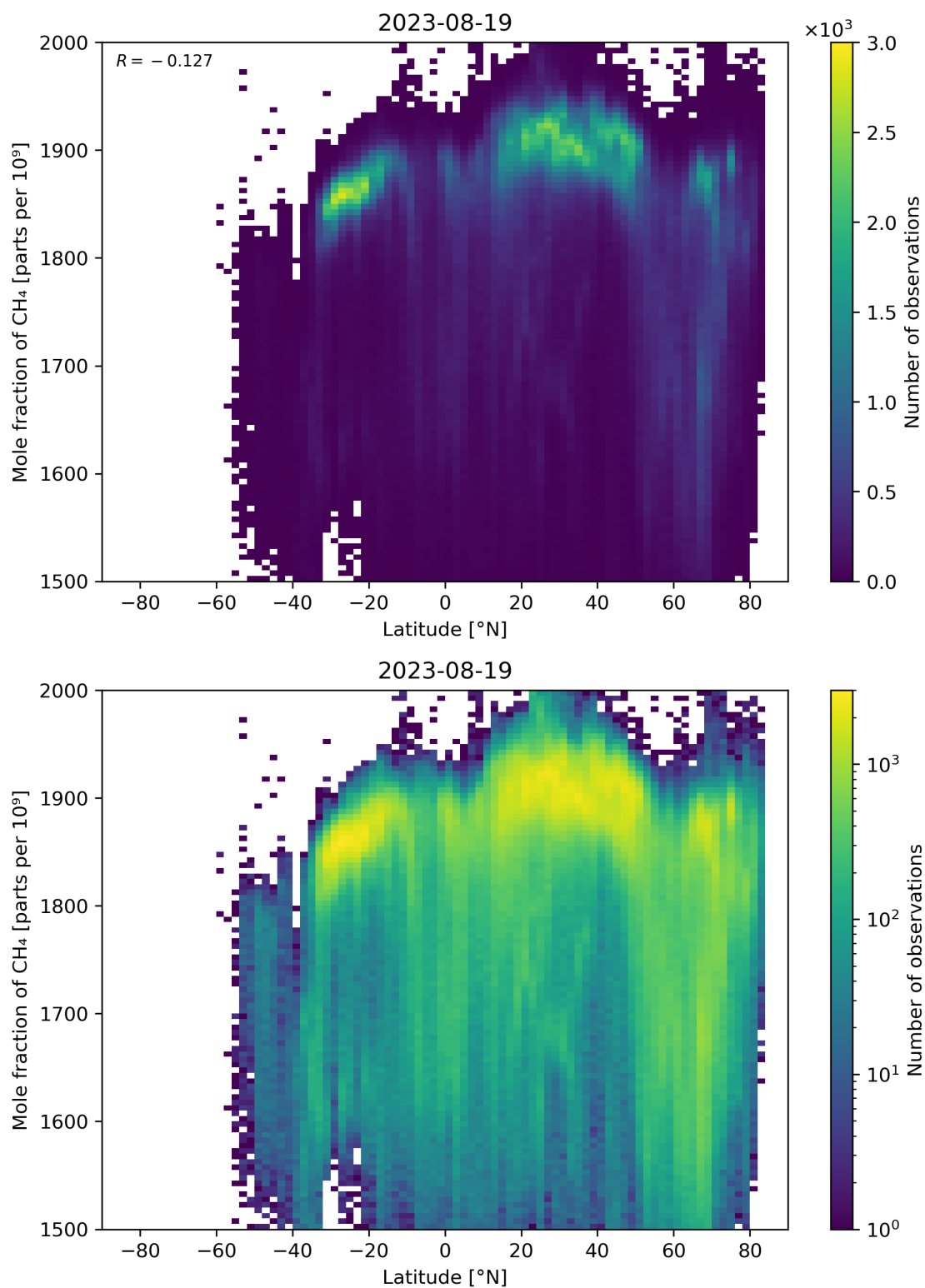
Figure 57: Scatter density plot of “Latitude” against “Mole fraction of CH 4 ” for 2023-08-18 to 2023-08-20.
