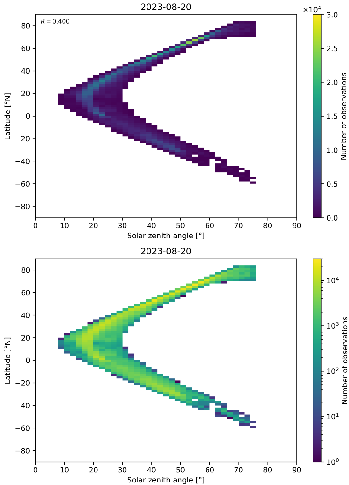
Figure 98: Scatter density plot of “Solar zenith angle” against “Latitude” for 2023-08-20 to 2023-08-21.
