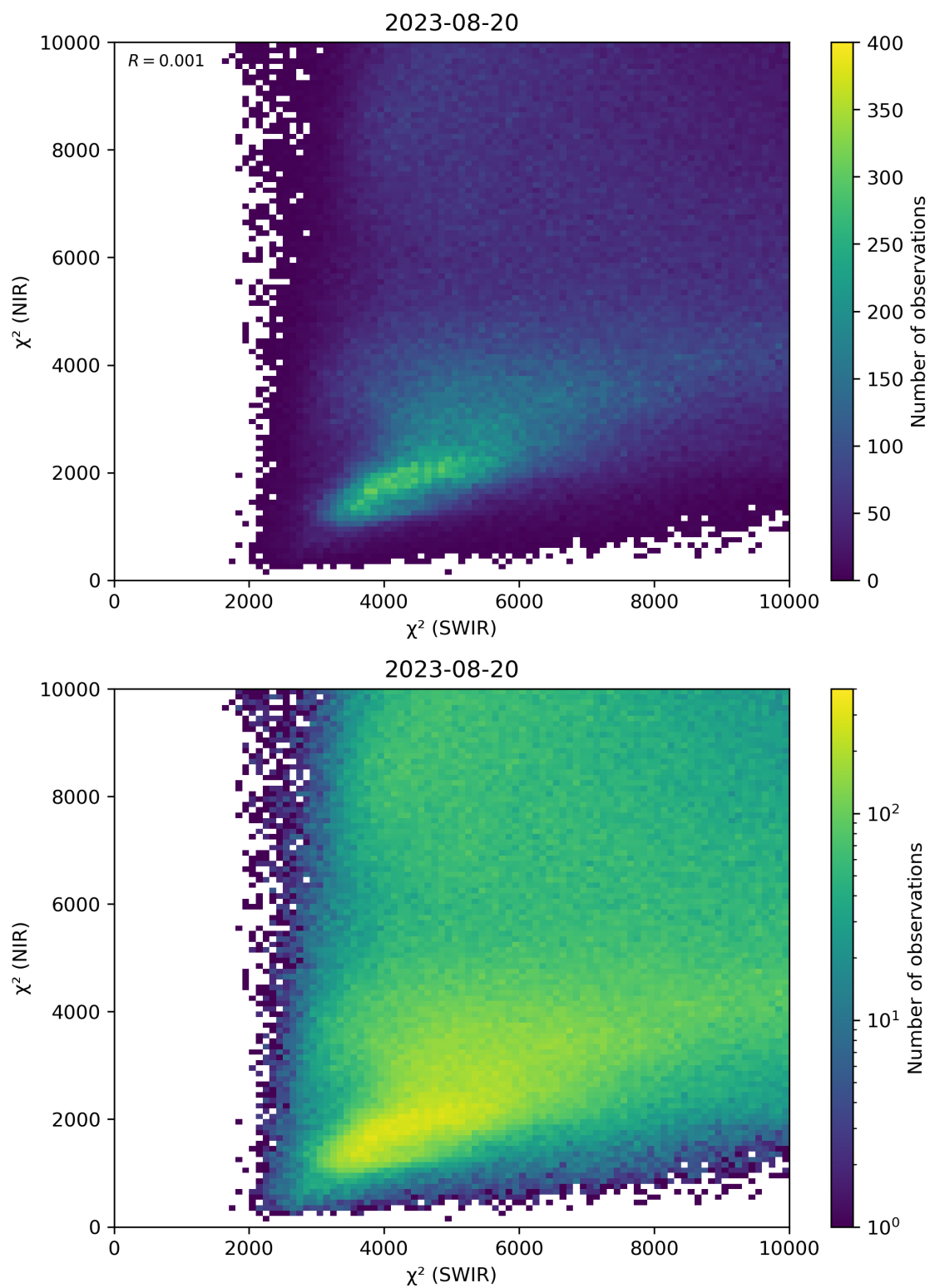
Figure 47: Scatter density plot of “ \chi^2 (SWIR)” against “ \chi^2 (NIR)” for 2023-08-20 to 2023-08-21.
