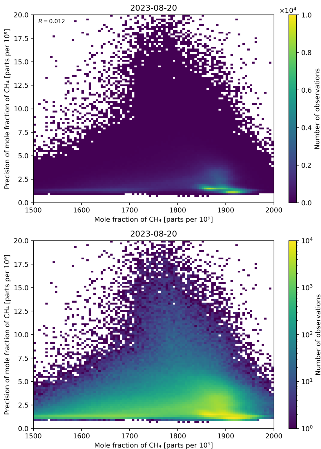
Figure 75: Scatter density plot of “Mole fraction of CH 4 ” against “Precision of mole fraction of CH 4 ” for 2023-08-20 to 2023-08-21.
