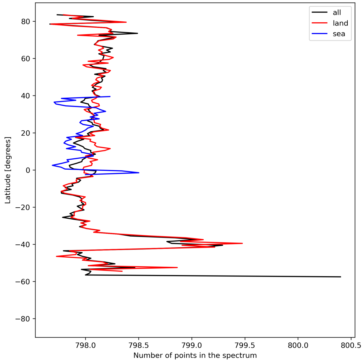
Figure 15: Zonal average of “Number of points in the spectrum” for 2023-08-20 to 2023-08-21.
