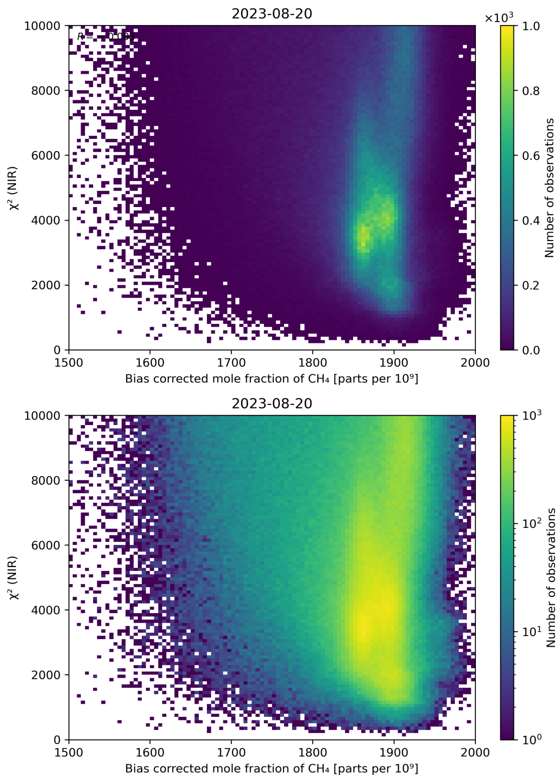
Figure 63: Scatter density plot of “Bias corrected mole fraction of CH 4 ” against “ \chi^2 (NIR)” for 2023-08-20 to 2023-08-21.
