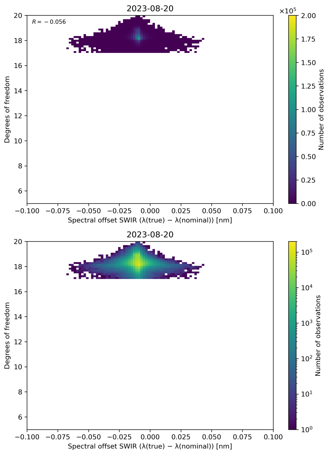
Figure 119: Scatter density plot of “Spectral offset SWIR ( \lambda(\text{true}) - \lambda(\text{nominal}) )” against “Degrees of freedom” for 2023-08-20 to 2023-08-21.
