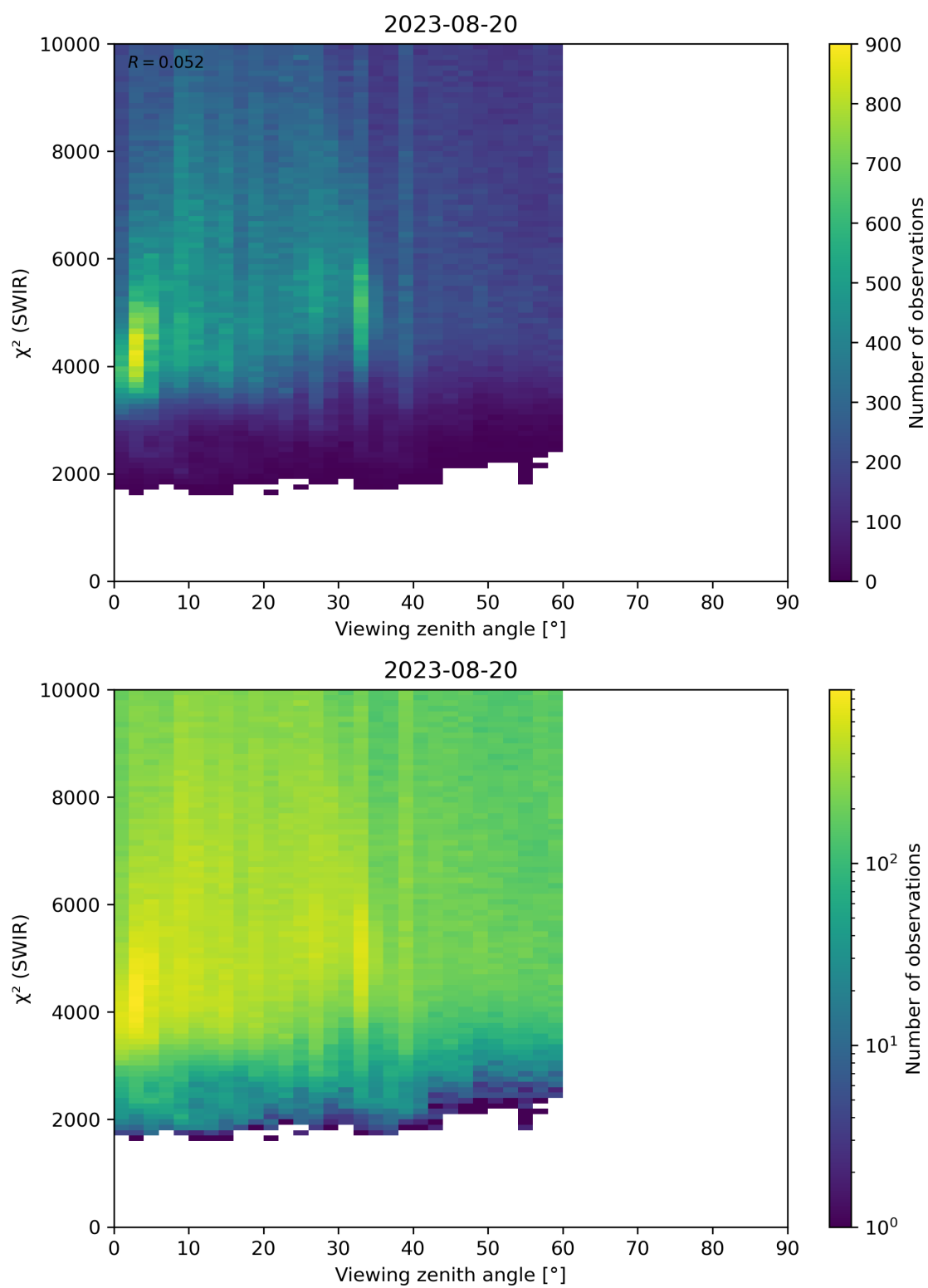
Figure 106: Scatter density plot of “Viewing zenith angle” against “ \chi^2 (SWIR)” for 2023-08-20 to 2023-08-21.
