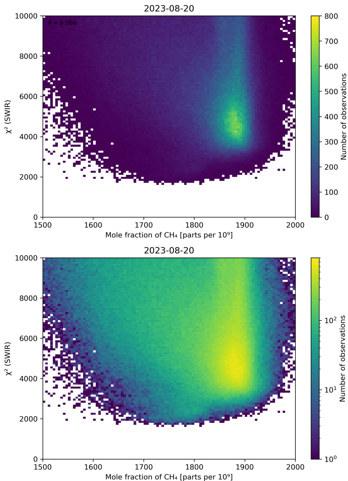
Figure 71: Scatter density plot of “Mole fraction of CH 4 ” against “ \chi^2 (SWIR)” for 2023-08-20 to 2023-08-21.
