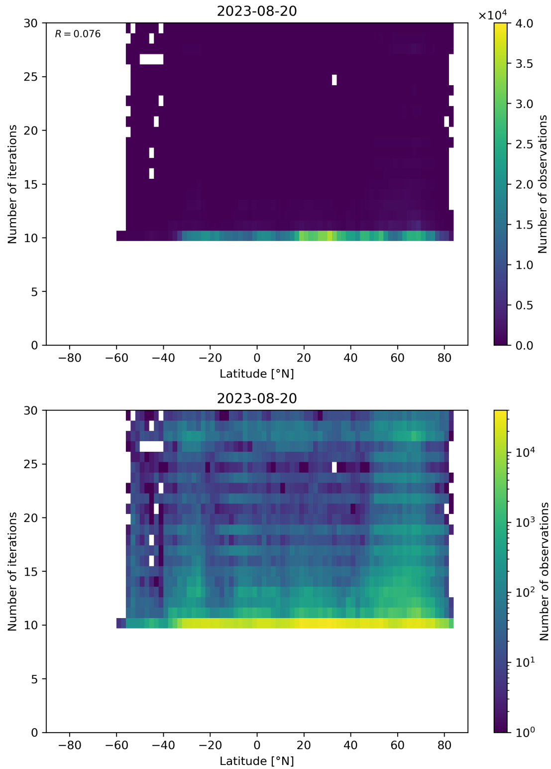
Figure 60: Scatter density plot of “Latitude” against “Number of iterations” for 2023-08-20 to 2023-08-21.
