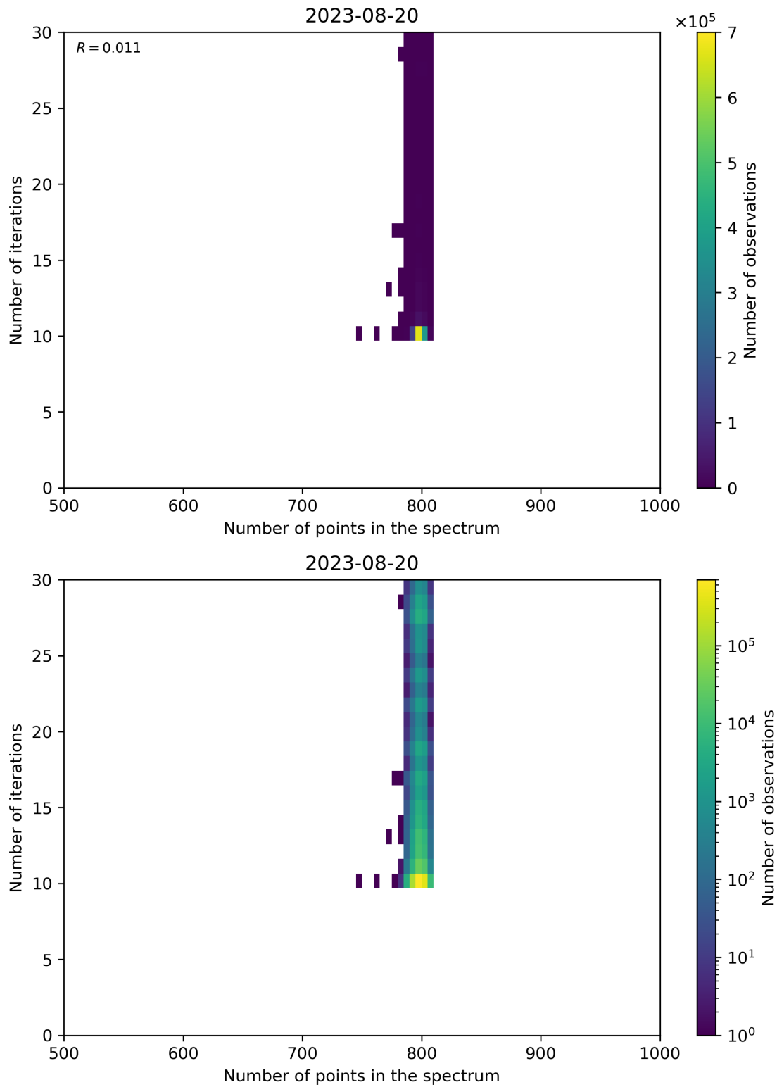
Figure 92: Scatter density plot of “Number of points in the spectrum” against “Number of iterations” for 2023-08-20 to 2023-08-21.
