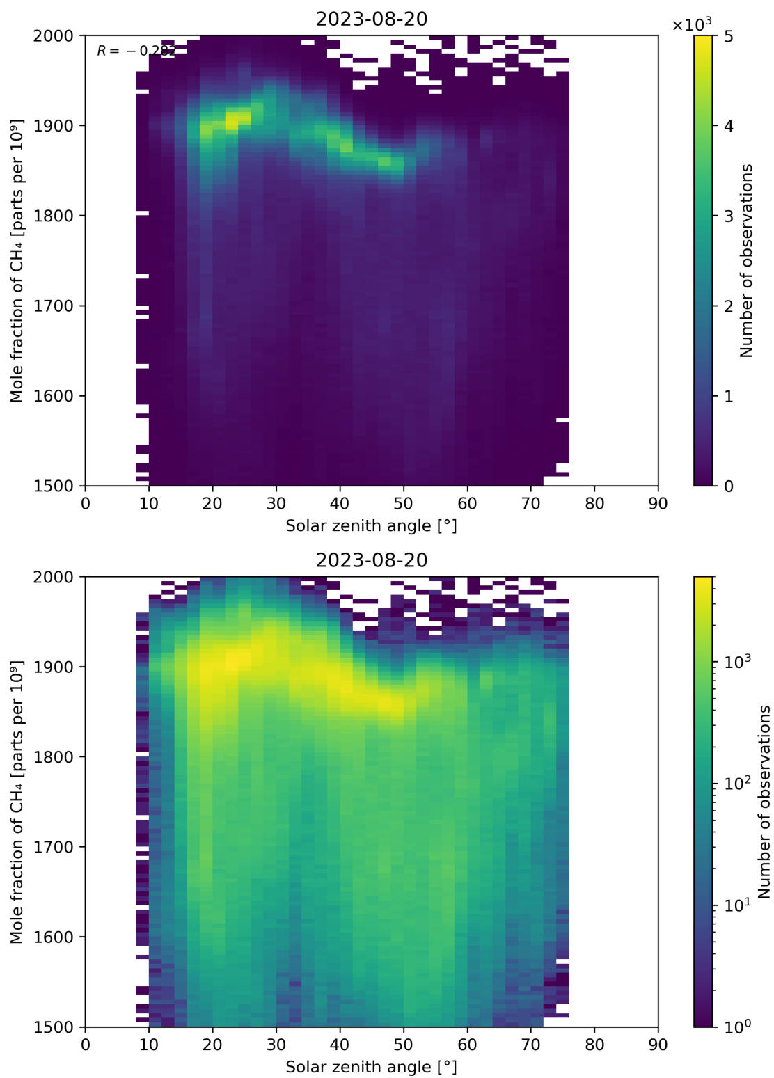
Figure 99: Scatter density plot of “Solar zenith angle” against “Mole fraction of \text{CH}_4 ” for 2023-08-20 to 2023-08-21.
