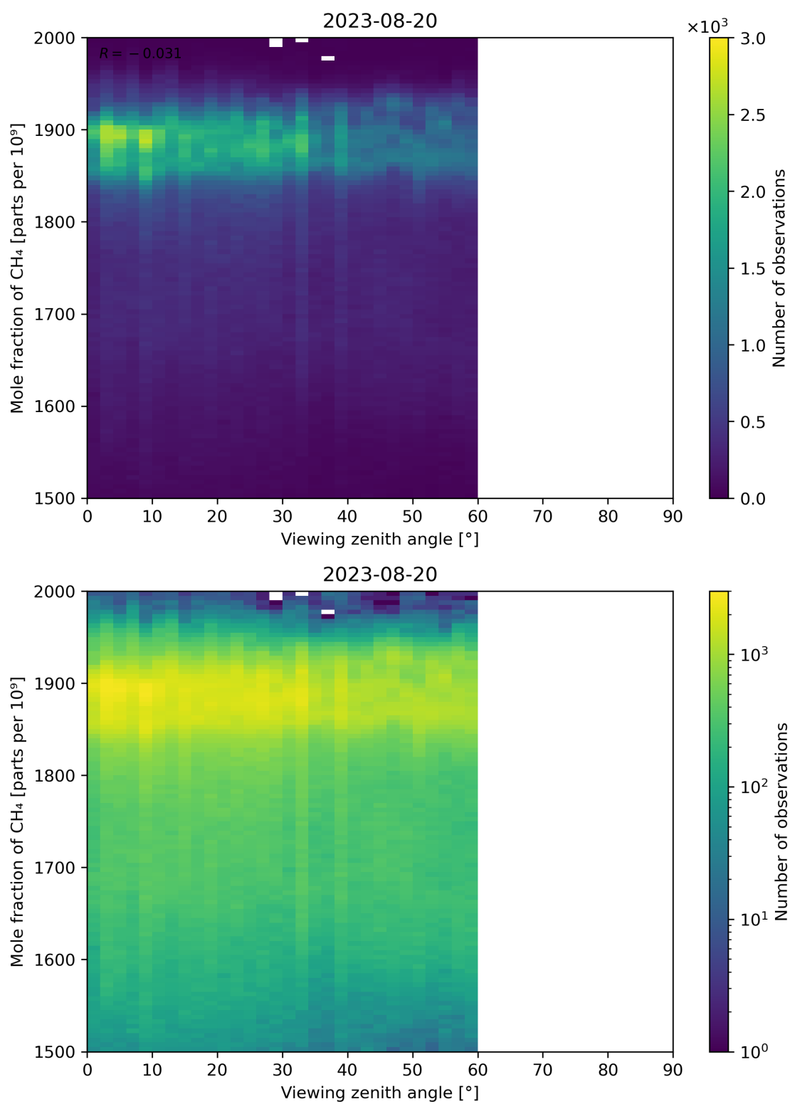
Figure 110: Scatter density plot of “Viewing zenith angle” against “Mole fraction of CH 4 ” for 2023-08-20 to 2023-08-21.
