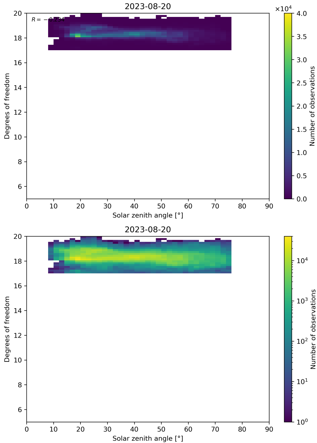
Figure 96: Scatter density plot of “Solar zenith angle” against “Degrees of freedom” for 2023-08-20 to 2023-08-21.
