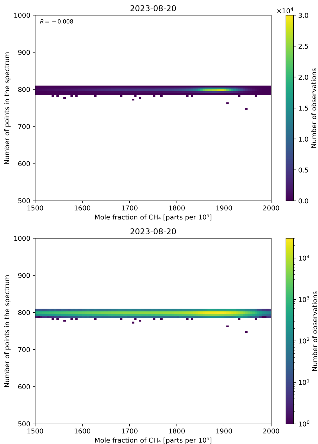
Figure 77: Scatter density plot of “Mole fraction of CH 4 ” against “Number of points in the spectrum” for 2023-08-20 to 2023-08-21.
