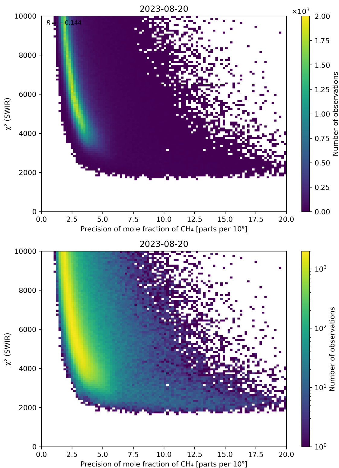
Figure 79: Scatter density plot of “Precision of mole fraction of \text{CH}_4 ” against “ \chi^2 (SWIR)” for 2023-08-20 to 2023-08-21.
