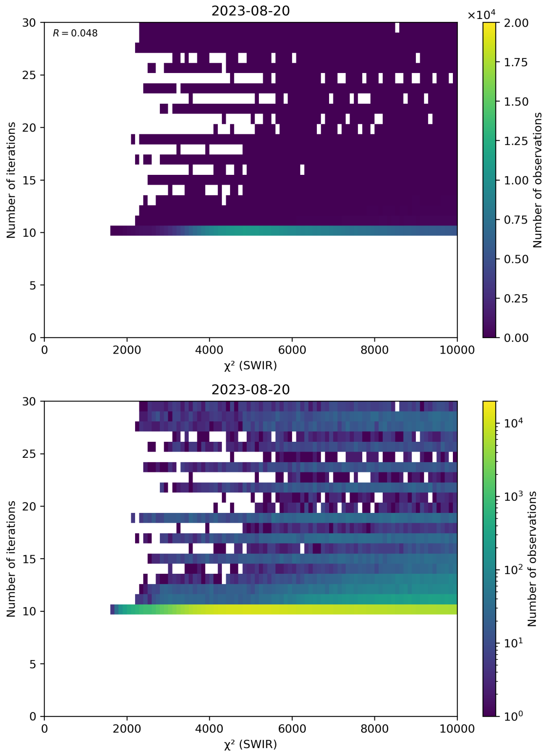
Figure 50: Scatter density plot of “ \chi^2 (SWIR)” against “Number of iterations” for 2023-08-20 to 2023-08-21.
