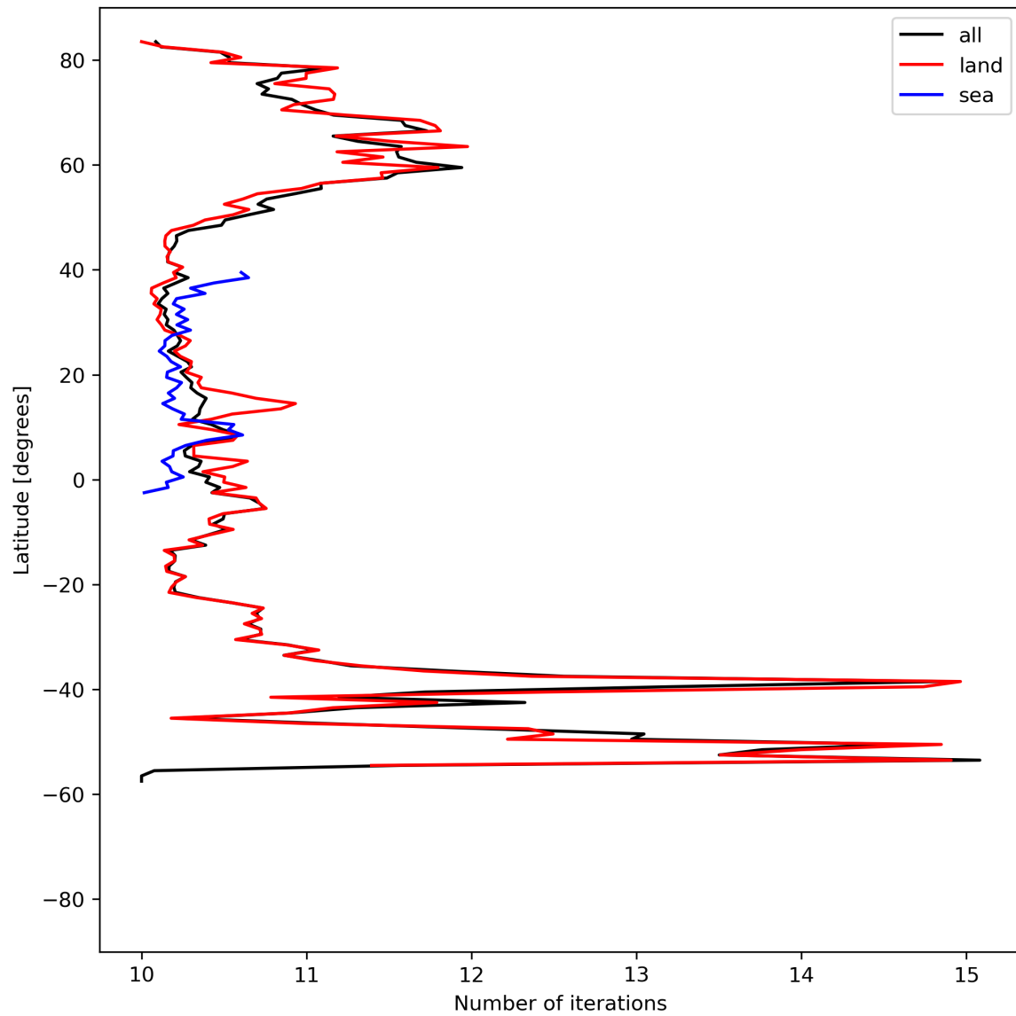
Figure 20: Zonal average of “Number of iterations” for 2023-08-20 to 2023-08-21.
