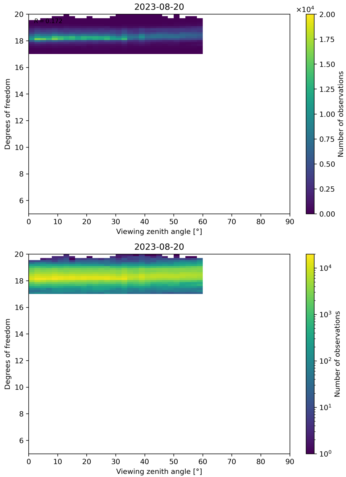
Figure 107: Scatter density plot of “Viewing zenith angle” against “Degrees of freedom” for 2023-08-20 to 2023-08-21.
