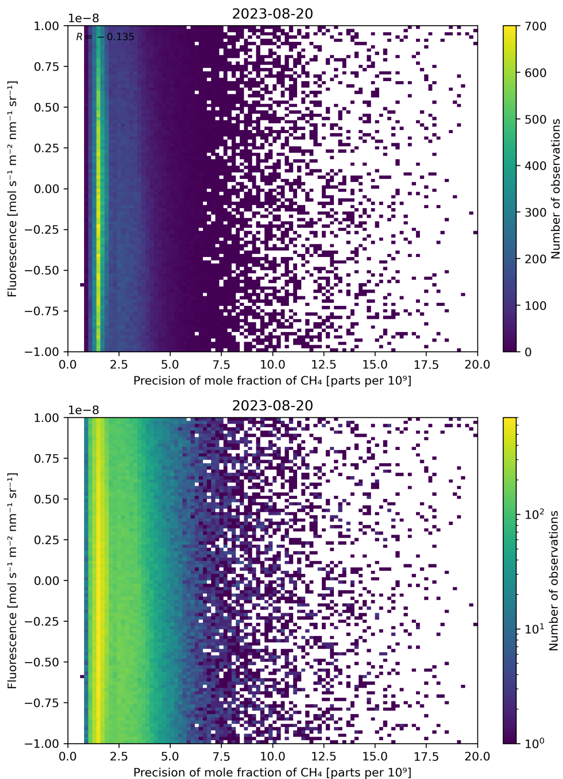
Figure 81: Scatter density plot of “Precision of mole fraction of \text{CH}_4 ” against “Fluorescence” for 2023-08-20 to 2023-08-21.
