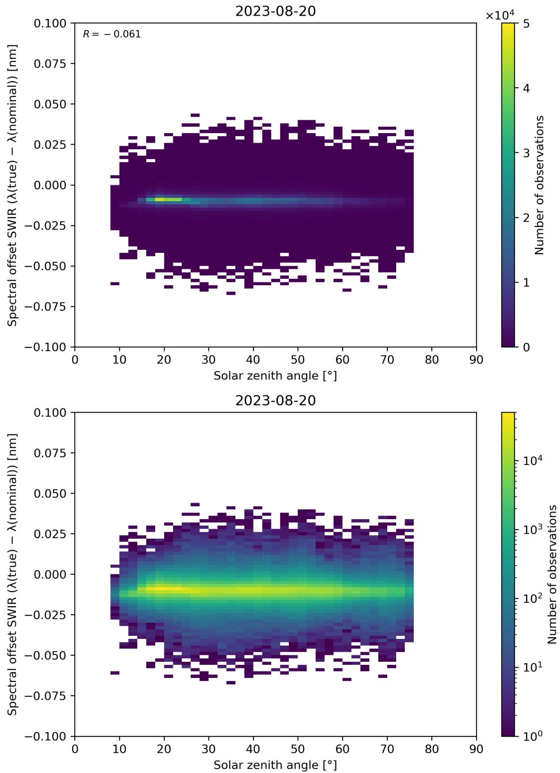
Figure 104: Scatter density plot of “Solar zenith angle” against “Spectral offset SWIR ( \lambda(\text{true}) - \lambda(\text{nominal}) )” for 2023-08-20 to 2023-08-21.
