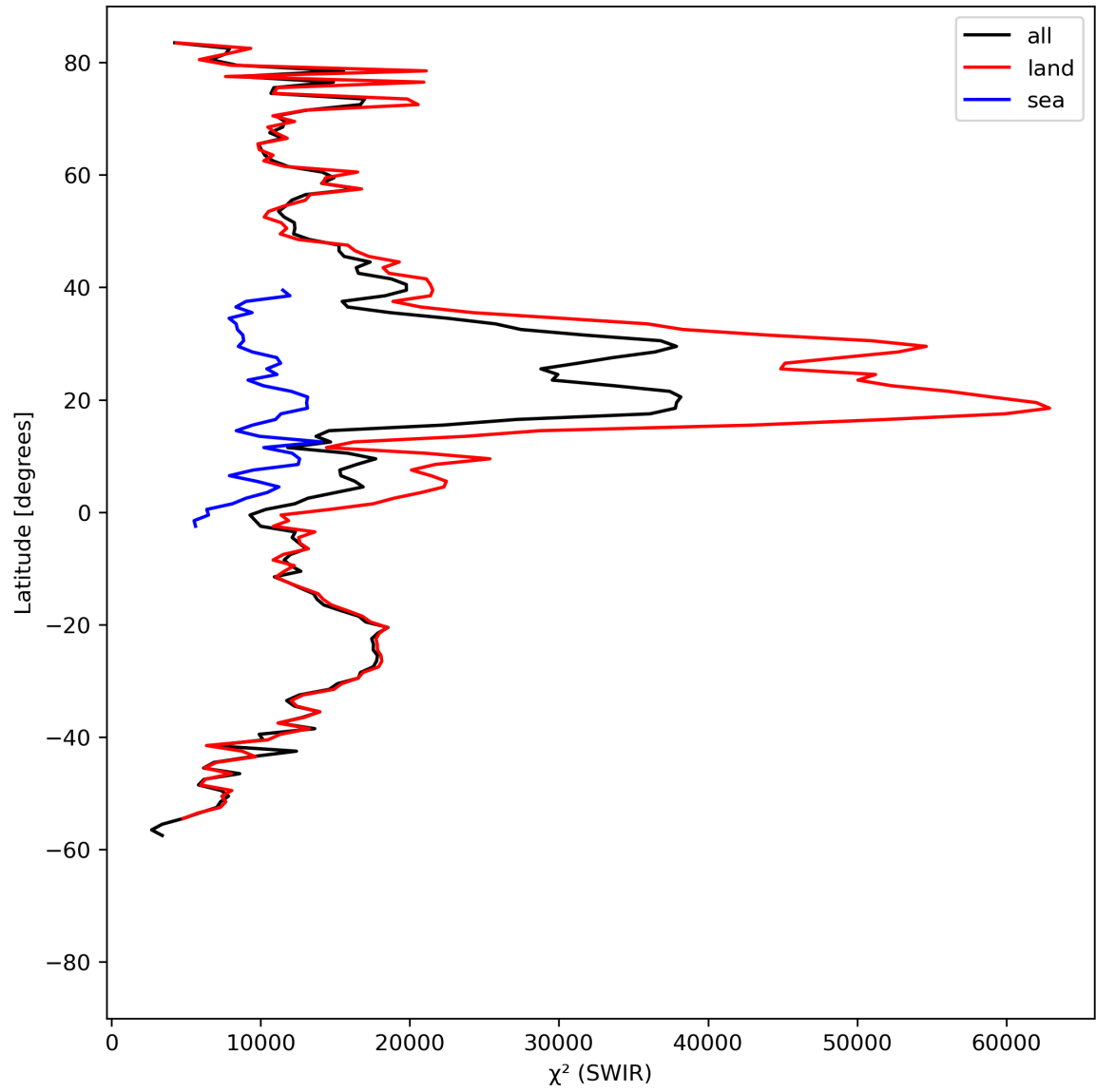
Figure 17: Zonal average of “ \chi^2 (SWIR)” for 2023-08-20 to 2023-08-21.
