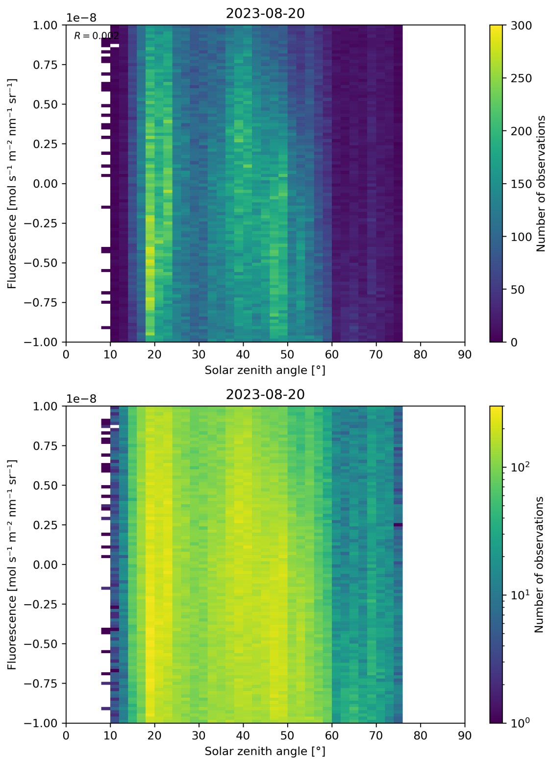
Figure 97: Scatter density plot of “Solar zenith angle” against “Fluorescence” for 2023-08-20 to 2023-08-21.
