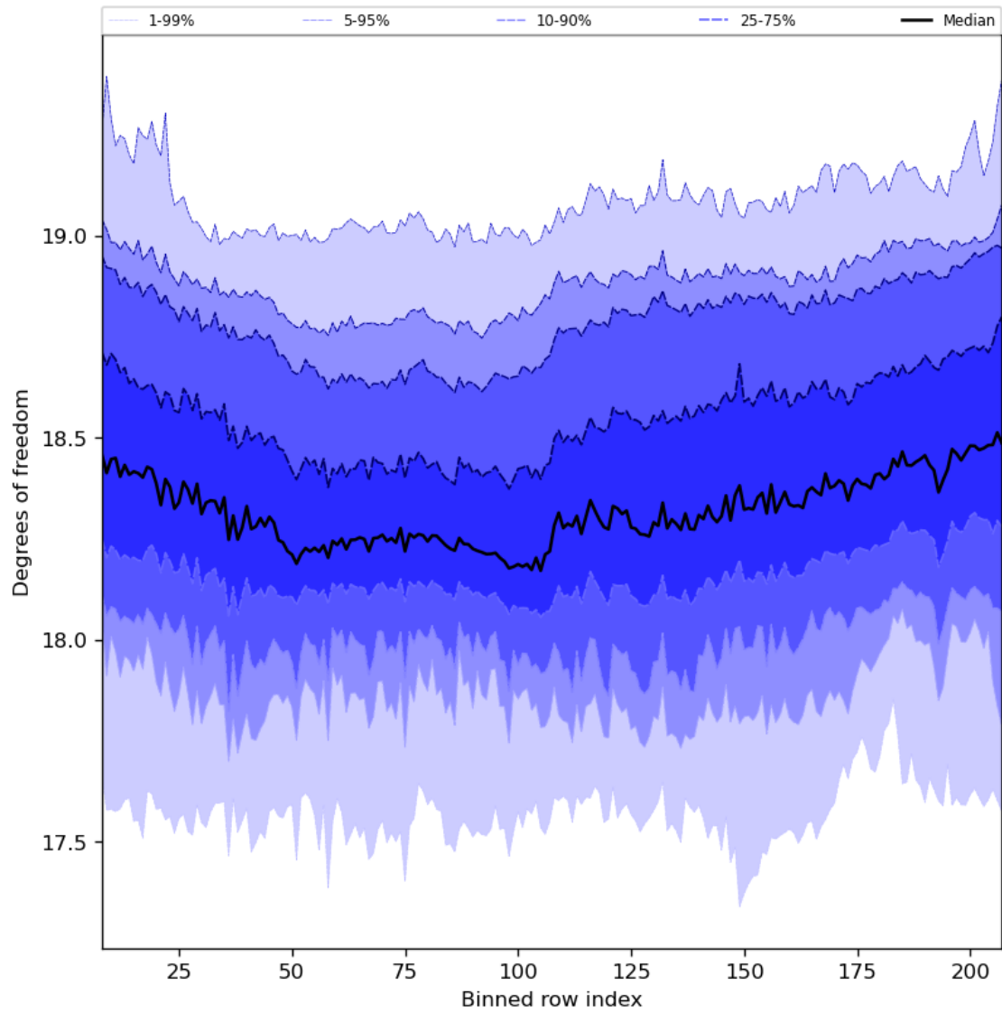
Figure 41: Along track statistics of “Degrees of freedom” for 2023-08-20 to 2023-08-21
