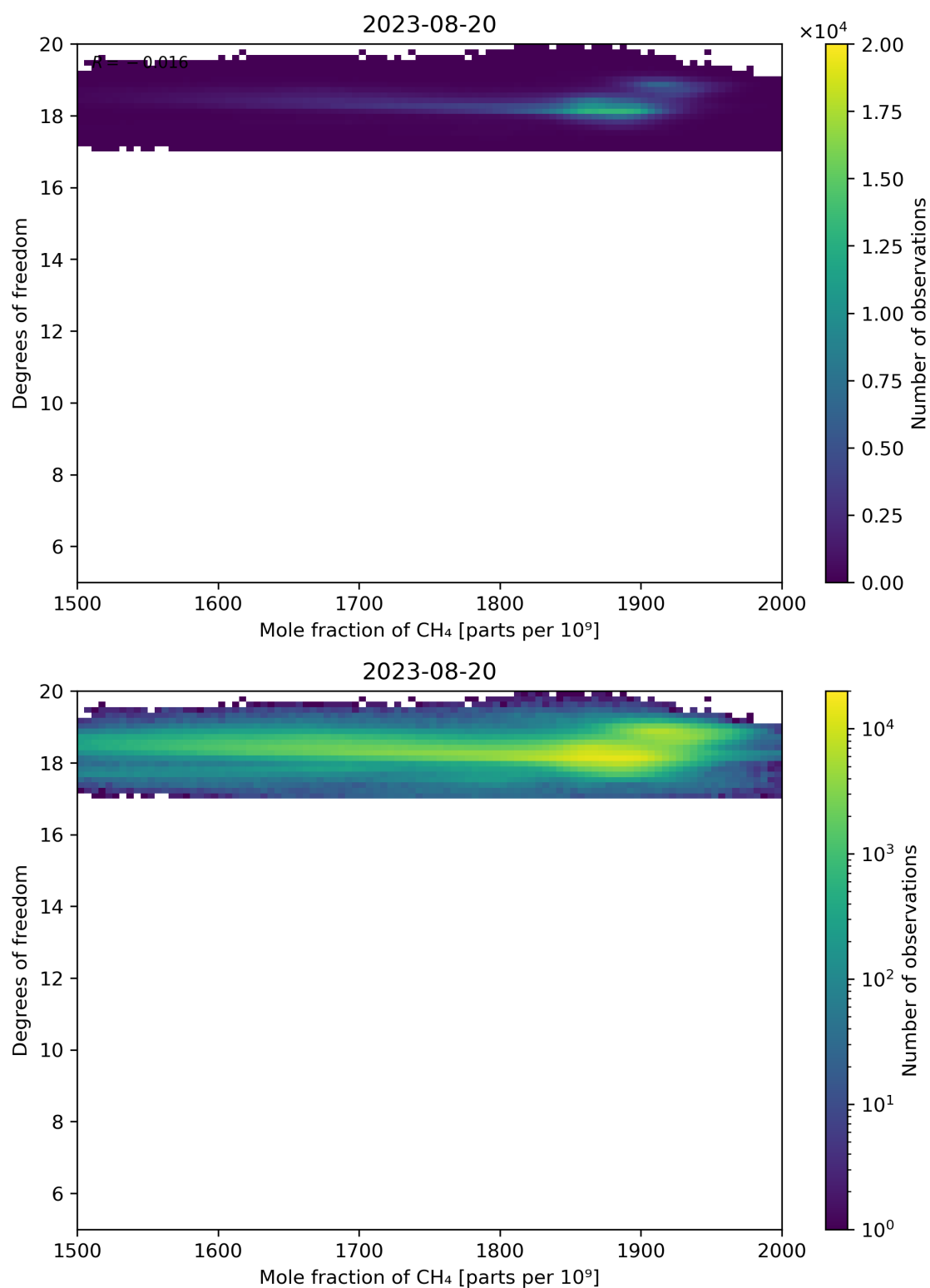
Figure 72: Scatter density plot of “Mole fraction of CH 4 ” against “Degrees of freedom” for 2023-08-20 to 2023-08-21.
