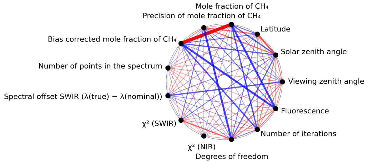
Figure 1: Map of correlation graph for 2023-08-20 to 2023-08-21.
