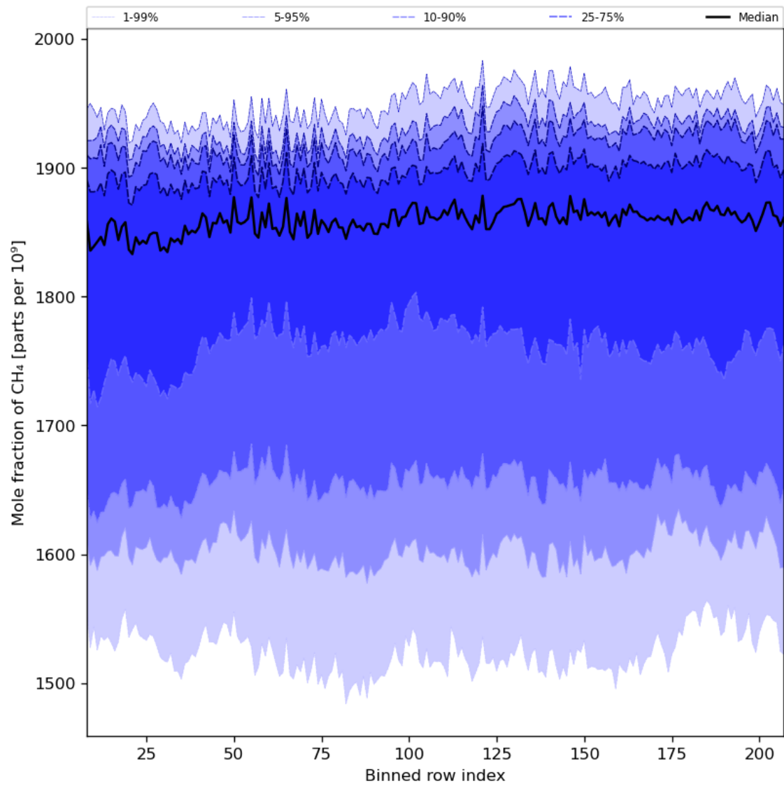
Figure 34: Along track statistics of “Mole fraction of CH 4 ” for 2023-08-20 to 2023-08-21
