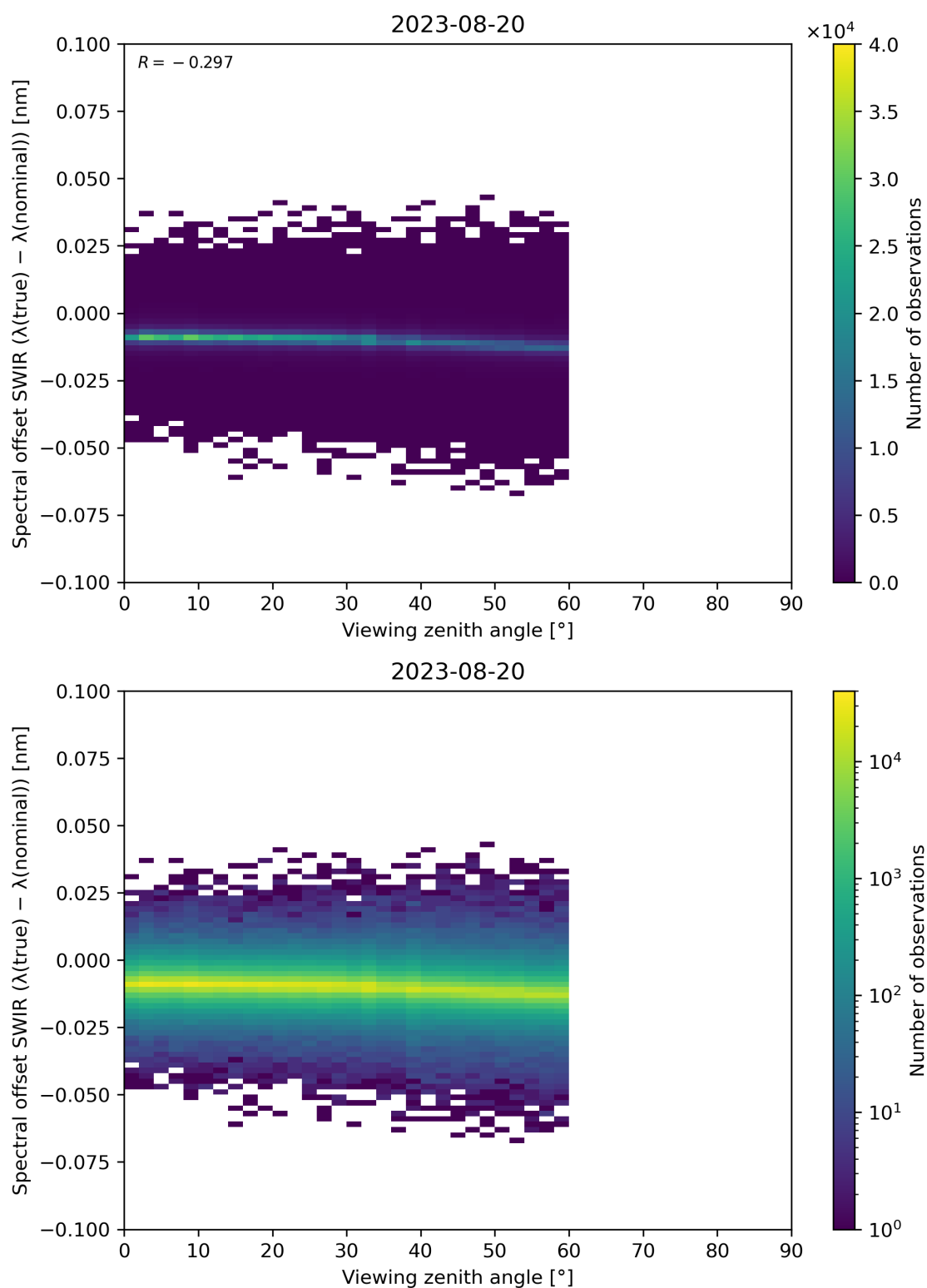
Figure 116: Scatter density plot of “Viewing zenith angle” against “Spectral offset SWIR ( \lambda(\text{true}) - \lambda(\text{nominal}) )” for 2023-08-20 to 2023-08-21.
