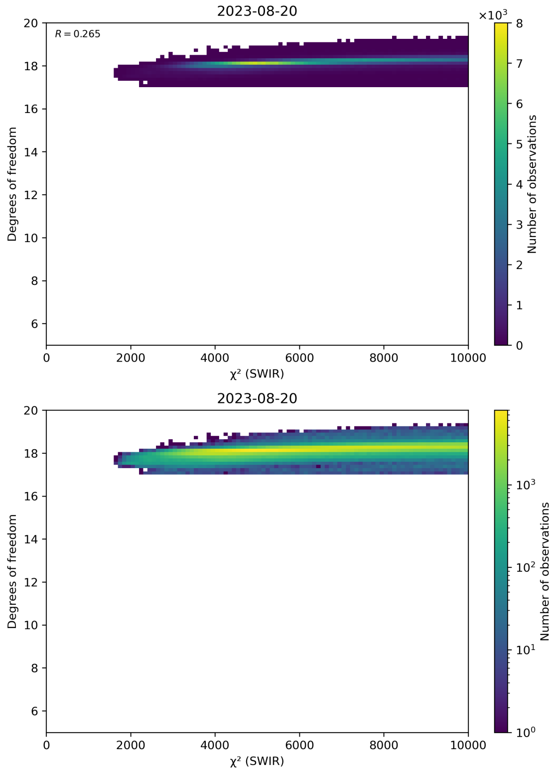
Figure 48: Scatter density plot of “ \chi^2 (SWIR)” against “Degrees of freedom” for 2023-08-20 to 2023-08-21.
