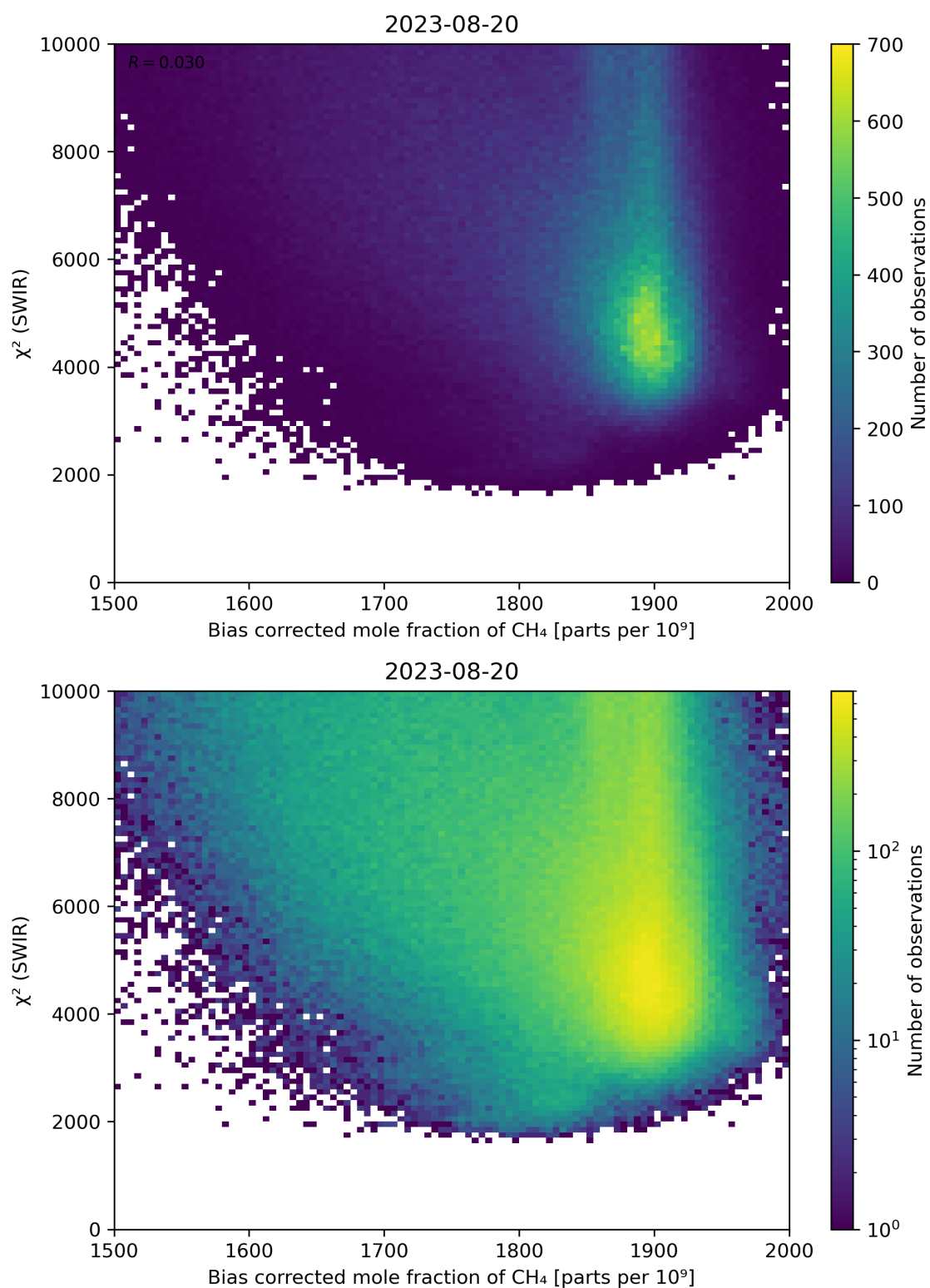
Figure 64: Scatter density plot of “Bias corrected mole fraction of CH 4 ” against “ \chi^2 (SWIR)” for 2023-08-20 to 2023-08-21.
