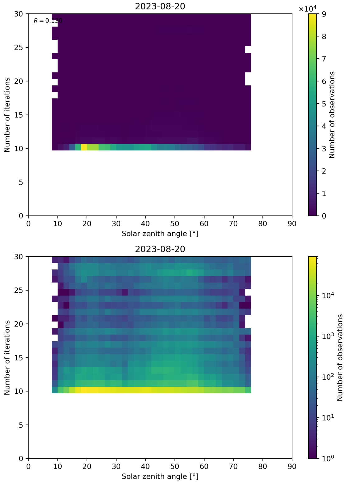
Figure 102: Scatter density plot of “Solar zenith angle” against “Number of iterations” for 2023-08-20 to 2023-08-21.
