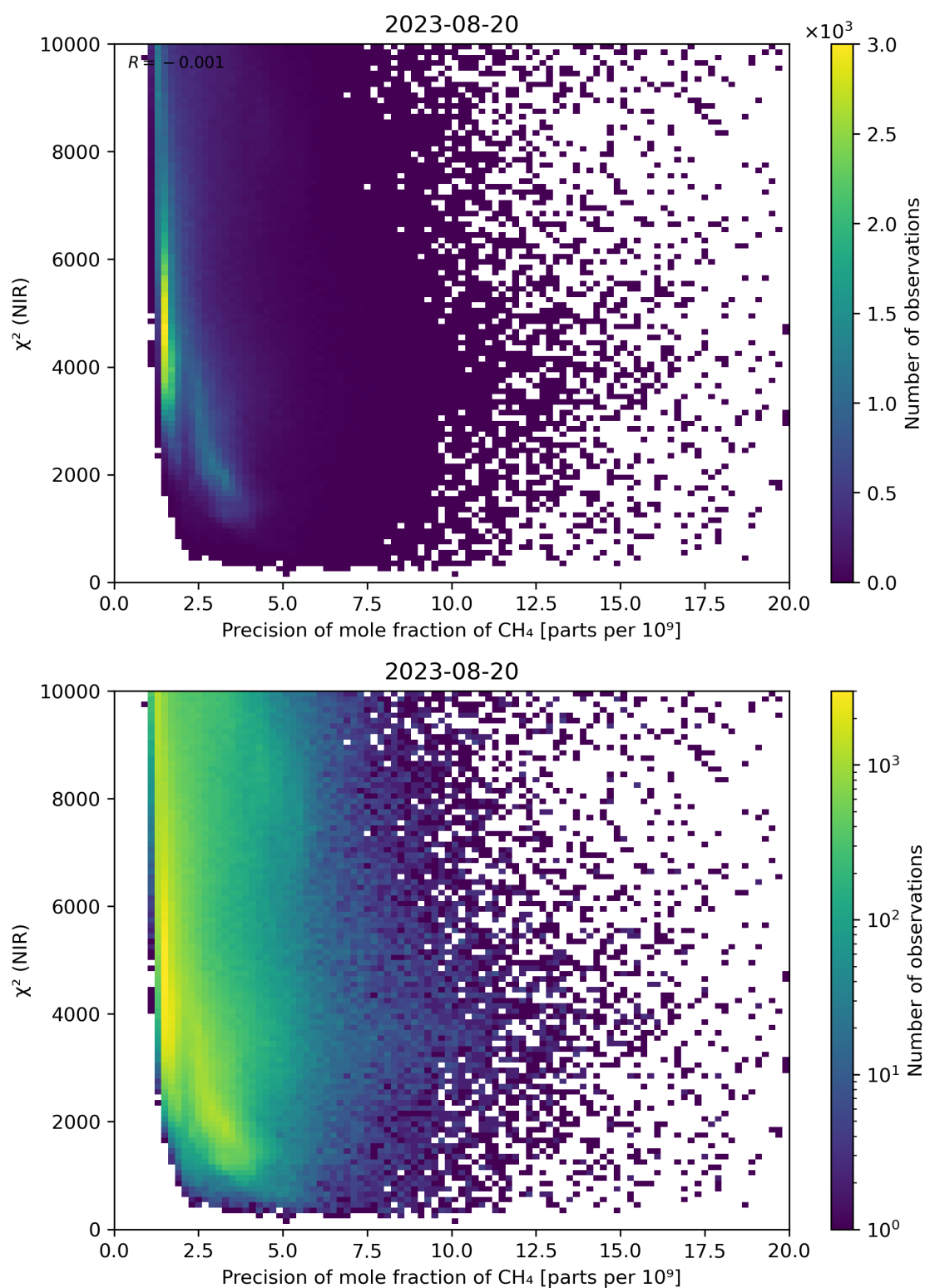
Figure 78: Scatter density plot of “Precision of mole fraction of CH 4 ” against “ \chi^2 (NIR)” for 2023-08-20 to 2023-08-21.
