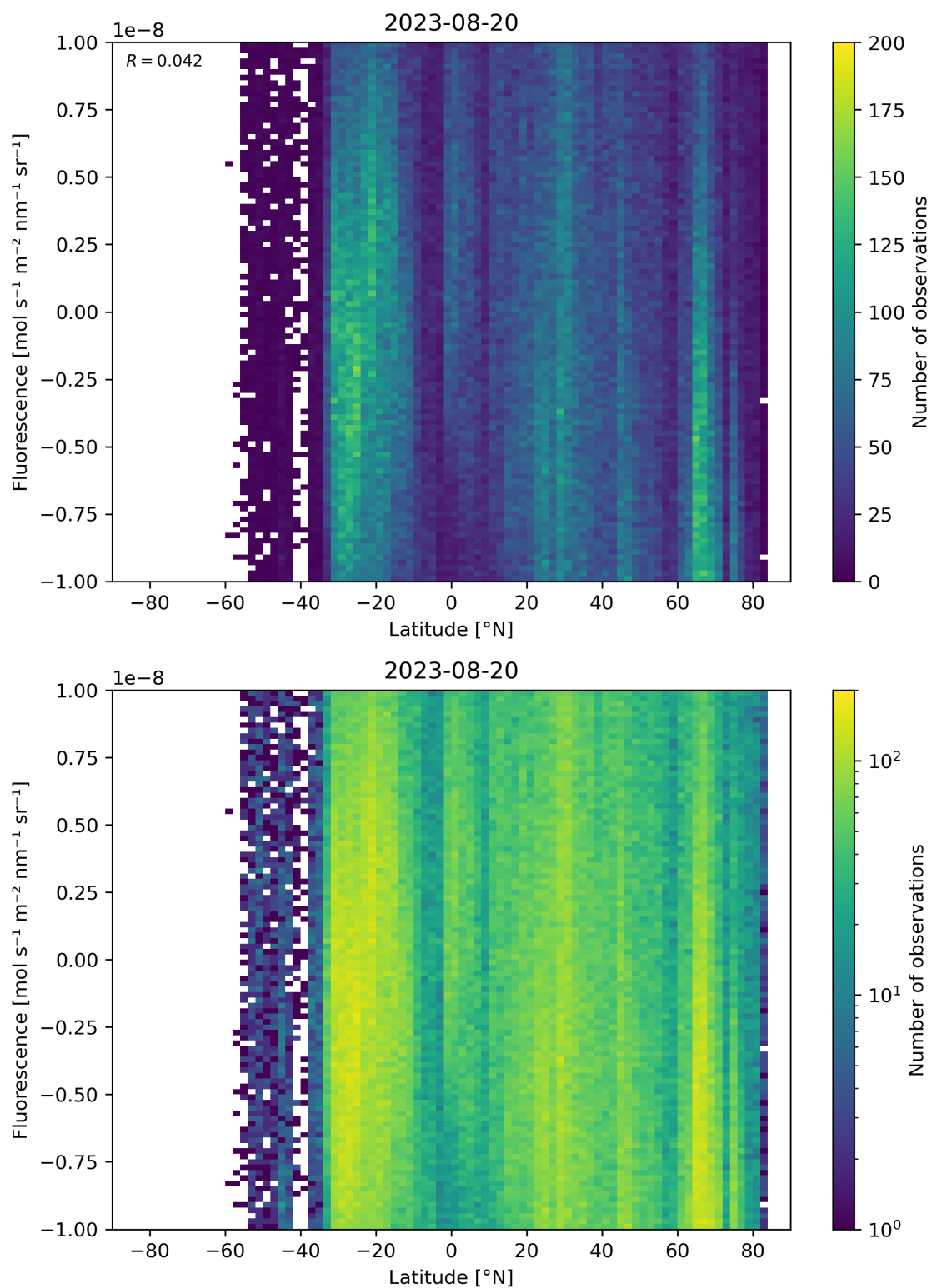
Figure 56: Scatter density plot of “Latitude” against “Fluorescence” for 2023-08-20 to 2023-08-21.
