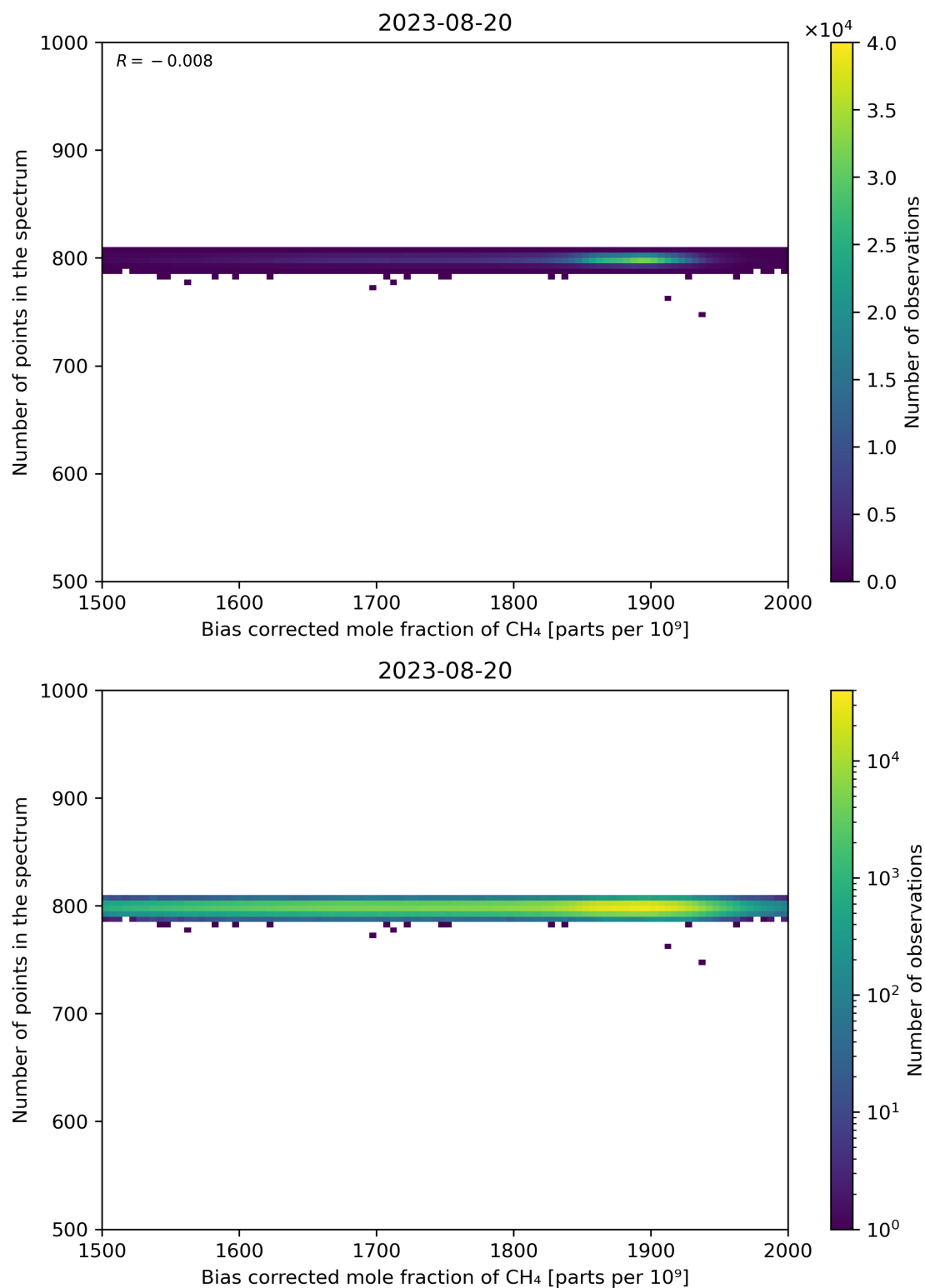
Figure 68: Scatter density plot of “Bias corrected mole fraction of CH 4 ” against “Number of points in the spectrum” for 2023-08-20 to 2023-08-21.
