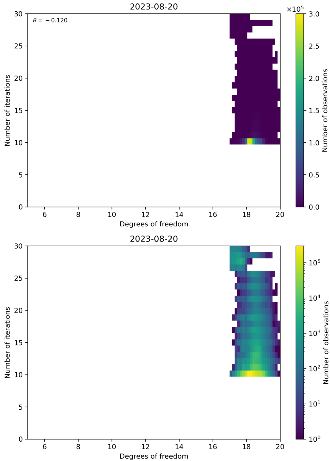
Figure 52: Scatter density plot of “Degrees of freedom” against “Number of iterations” for 2023-08-20 to 2023-08-21.
