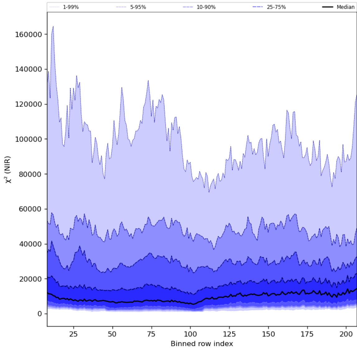
Figure 40: Along track statistics of “ \chi^2 (NIR)” for 2023-08-20 to 2023-08-21
