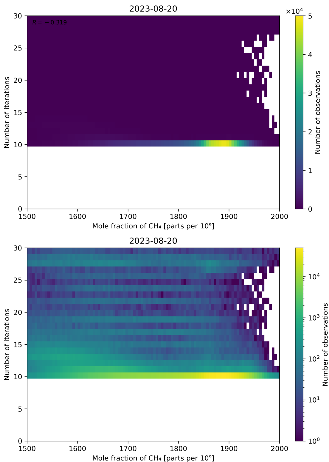
Figure 76: Scatter density plot of “Mole fraction of CH 4 ” against “Number of iterations” for 2023-08-20 to 2023-08-21.
