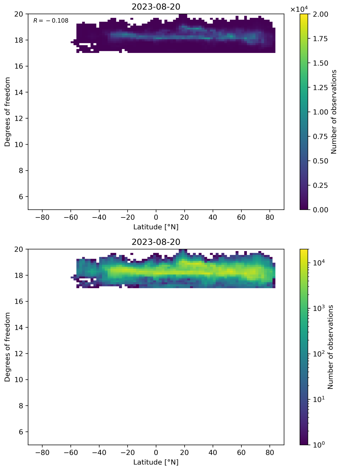
Figure 55: Scatter density plot of “Latitude” against “Degrees of freedom” for 2023-08-20 to 2023-08-21.
