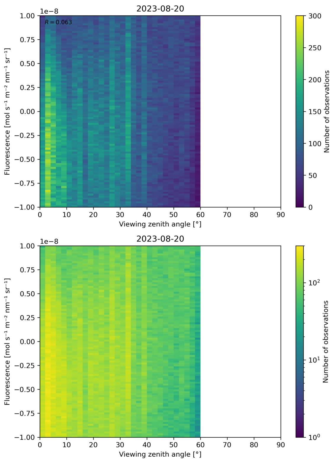
Figure 108: Scatter density plot of “Viewing zenith angle” against “Fluorescence” for 2023-08-20 to 2023-08-21.
