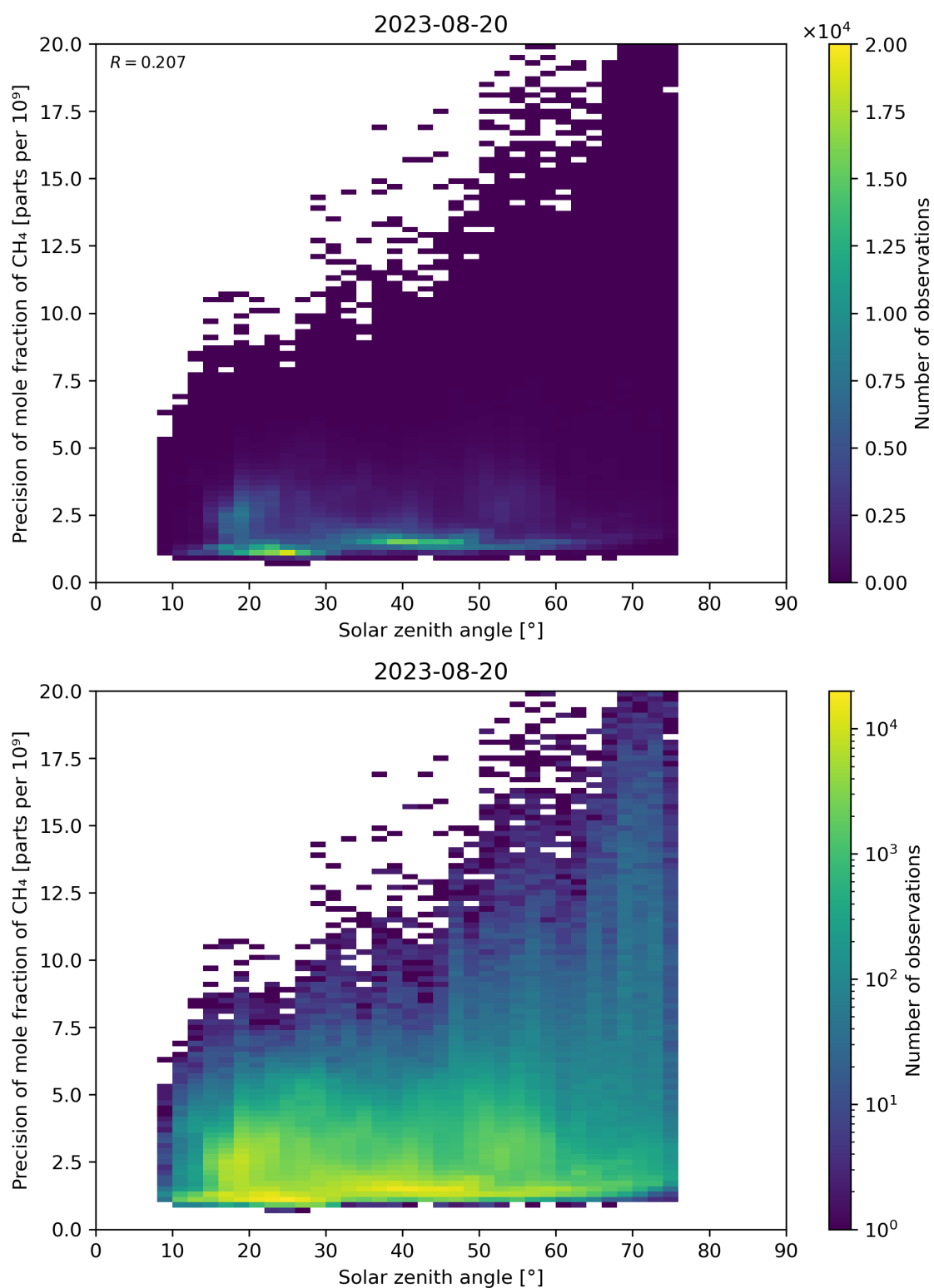
Figure 101: Scatter density plot of “Solar zenith angle” against “Precision of mole fraction of \text{CH}_4 ” for 2023-08-20 to 2023-08-21.
