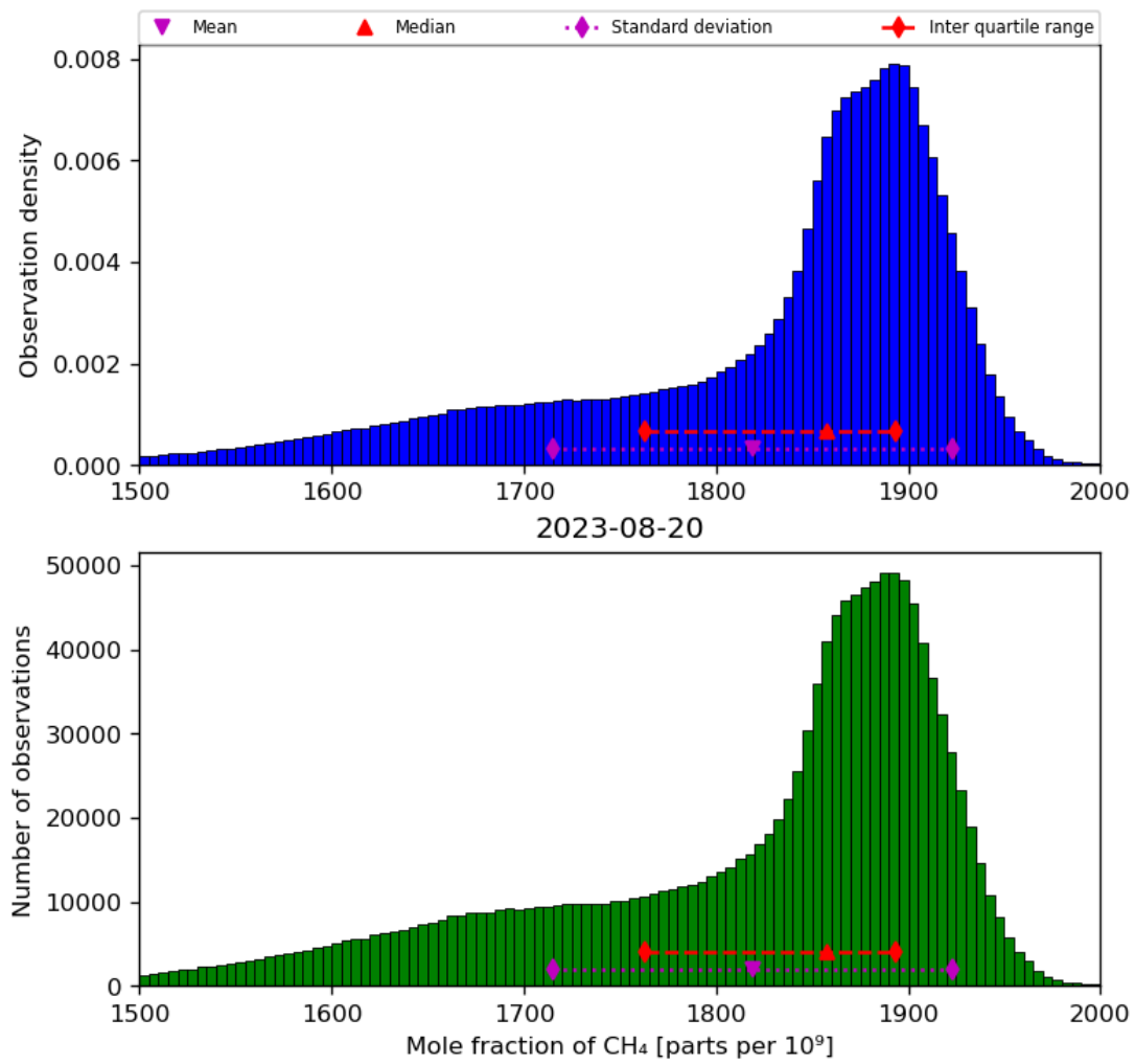
Figure 23: Histogram of “Mole fraction of CH 4 ” for 2023-08-20 to 2023-08-21
