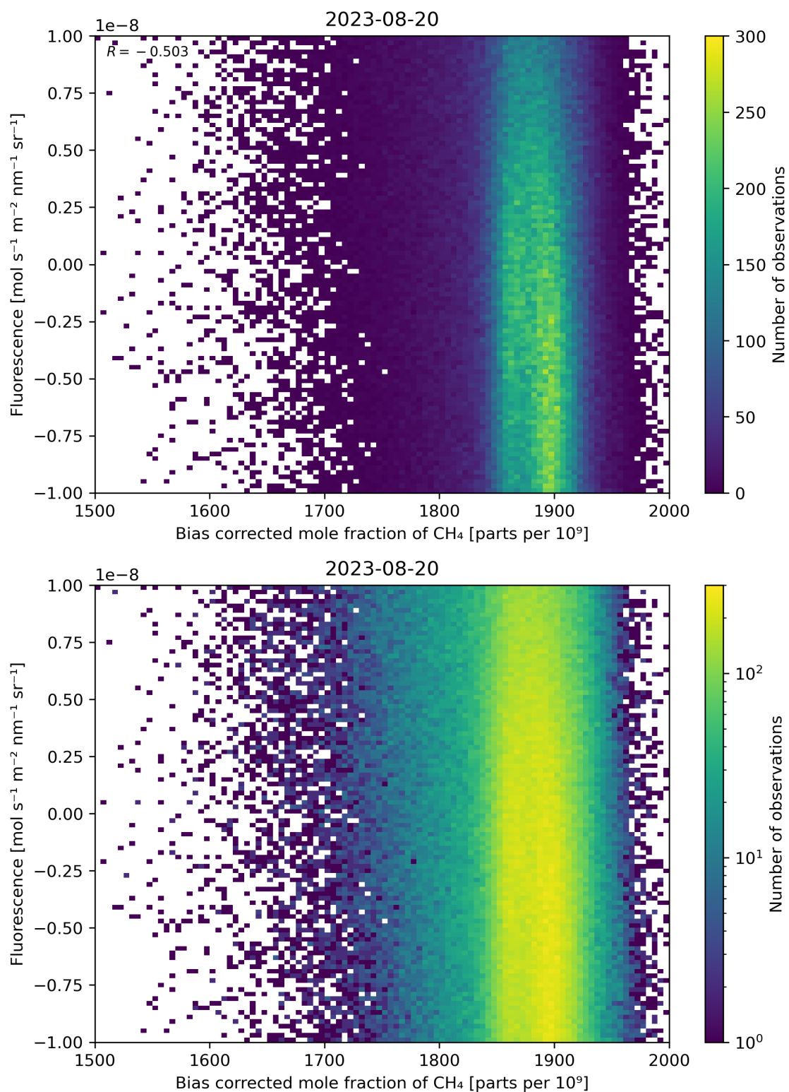
Figure 66: Scatter density plot of “Bias corrected mole fraction of \text{CH}_4 ” against “Fluorescence” for 2023-08-20 to 2023-08-21.
