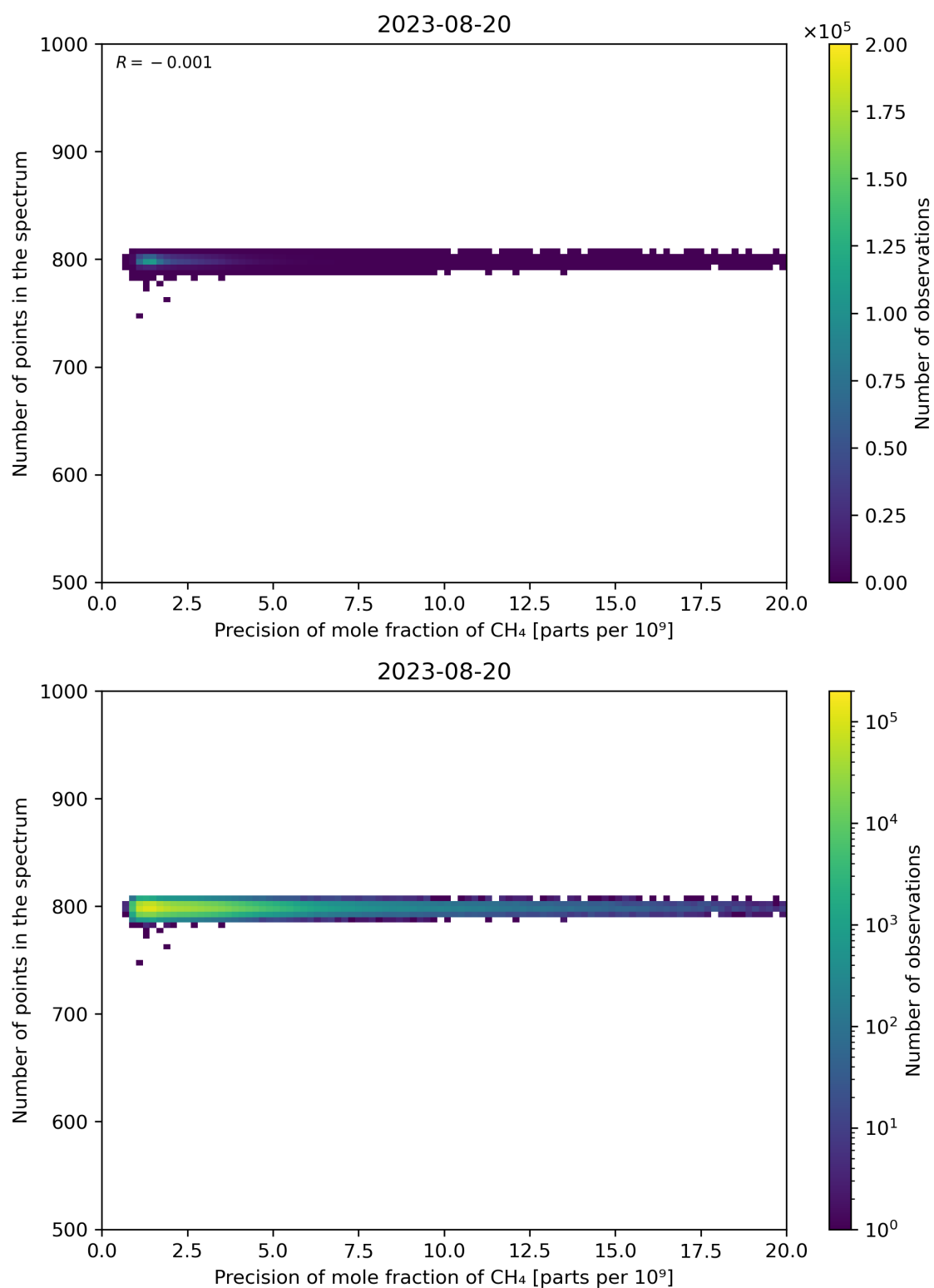
Figure 84: Scatter density plot of “Precision of mole fraction of CH 4 ” against “Number of points in the spectrum” for 2023-08-20 to 2023-08-21.
