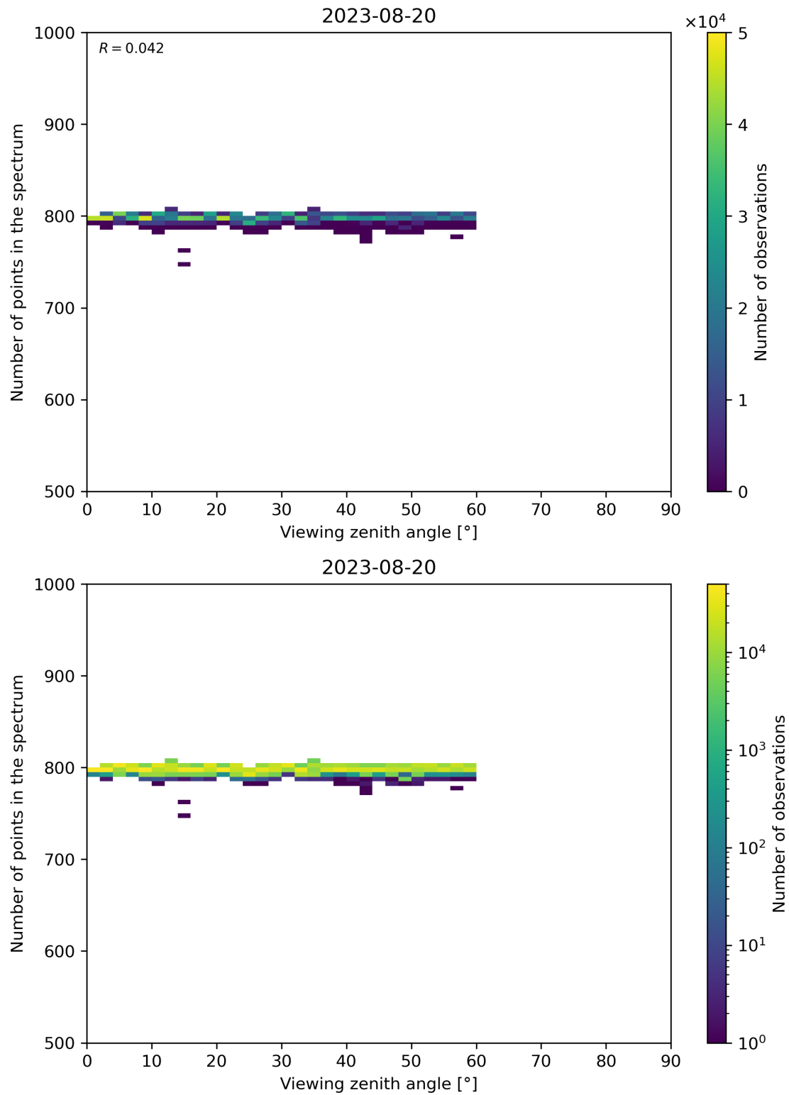
Figure 114: Scatter density plot of “Viewing zenith angle” against “Number of points in the spectrum” for 2023-08-20 to 2023-08-21.
