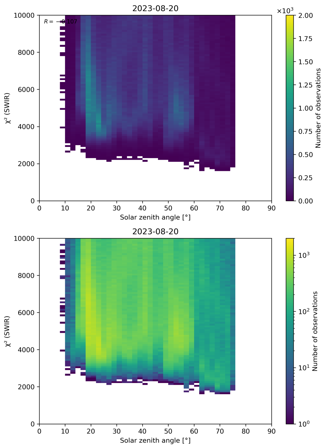
Figure 95: Scatter density plot of “Solar zenith angle” against “ \chi^2 (SWIR)” for 2023-08-20 to 2023-08-21.
