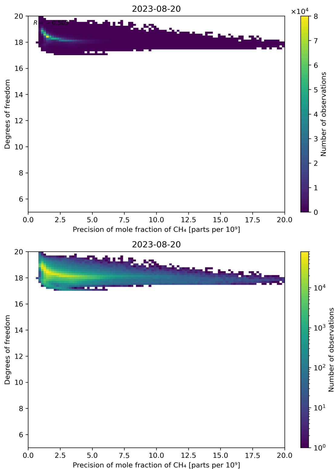
Figure 80: Scatter density plot of “Precision of mole fraction of CH 4 ” against “Degrees of freedom” for 2023-08-20 to 2023-08-21.
