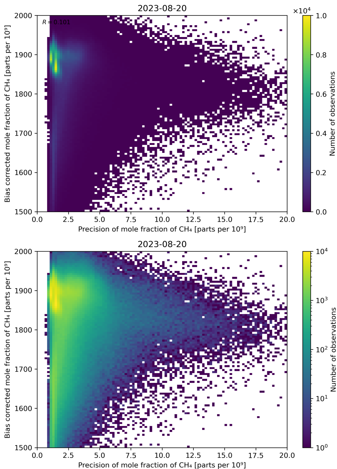
Figure 82: Scatter density plot of “Precision of mole fraction of CH 4 ” against “Bias corrected mole fraction of CH 4 ” for 2023-08-20 to 2023-08-21.
