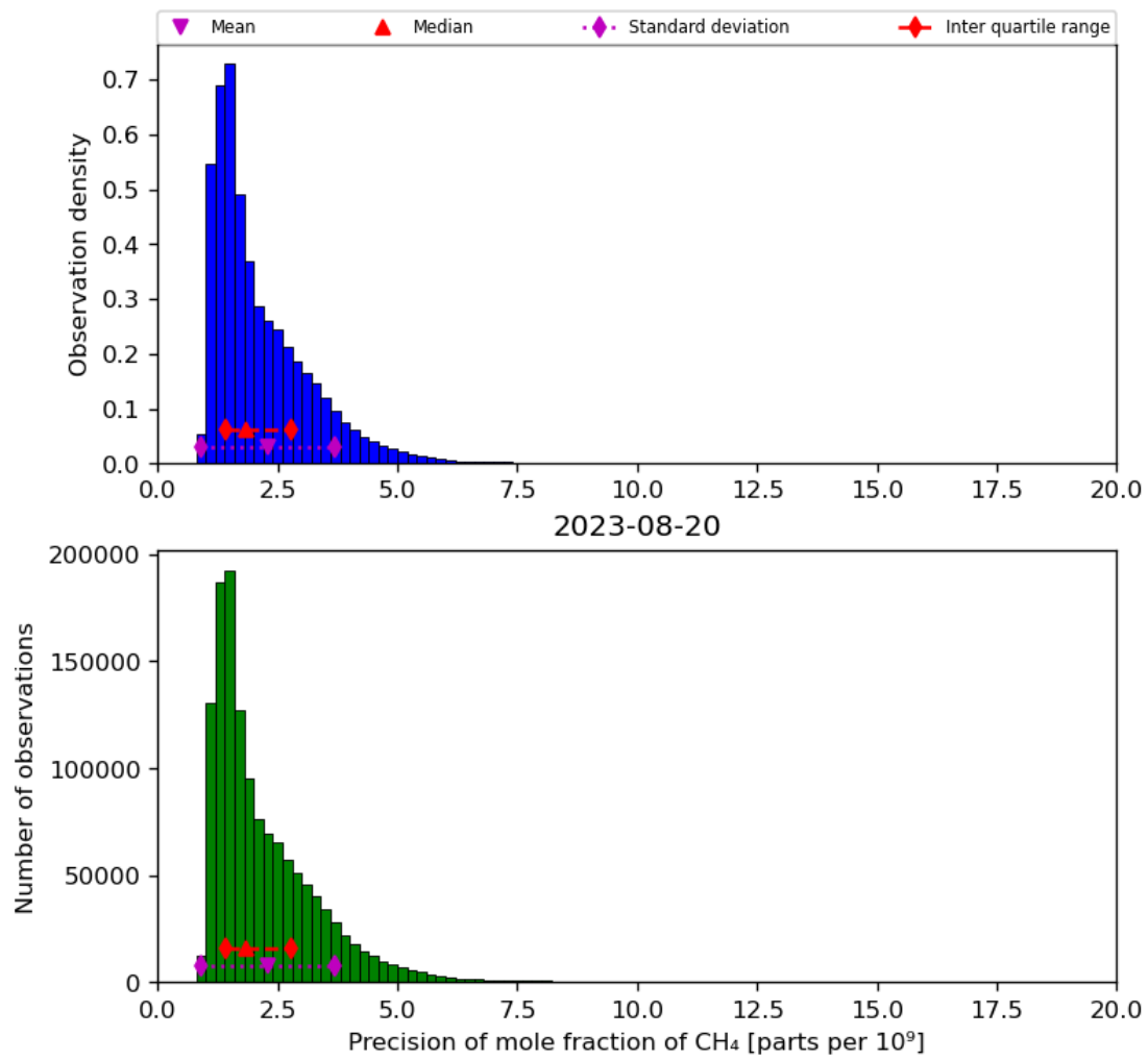
Figure 24: Histogram of “Precision of mole fraction of CH 4 ” for 2023-08-20 to 2023-08-21
