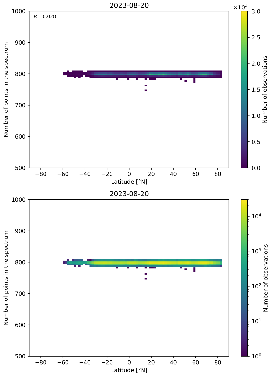
Figure 61: Scatter density plot of “Latitude” against “Number of points in the spectrum” for 2023-08-20 to 2023-08-21.
