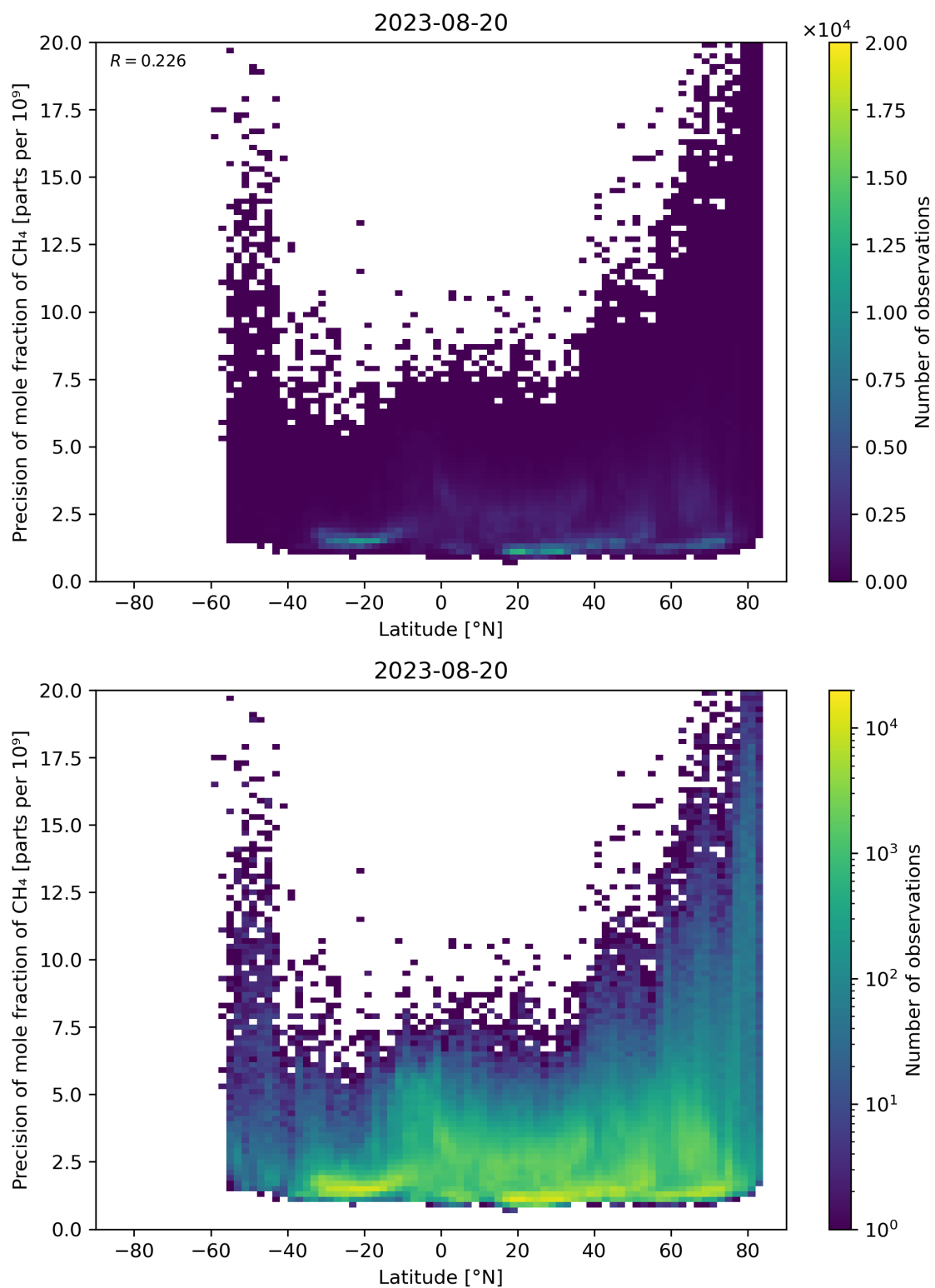
Figure 59: Scatter density plot of “Latitude” against “Precision of mole fraction of \text{CH}_4 ” for 2023-08-20 to 2023-08-21.
