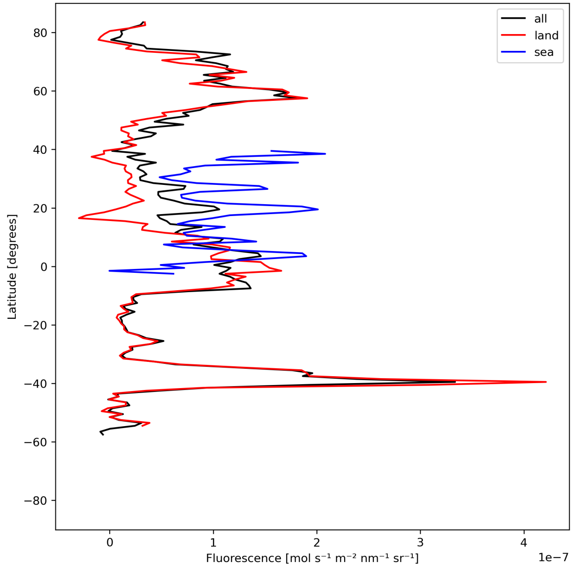
Figure 21: Zonal average of “Fluorescence” for 2023-08-20 to 2023-08-21.
