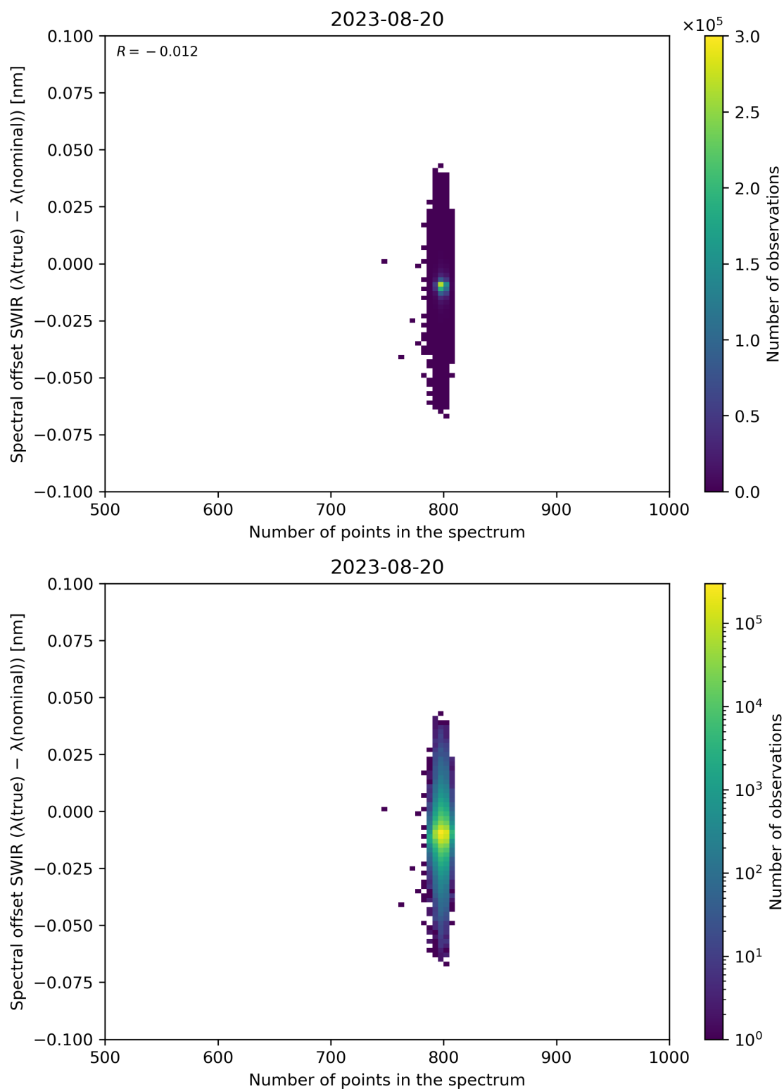
Figure 93: Scatter density plot of “Number of points in the spectrum” against “Spectral offset SWIR ( \lambda(\text{true}) - \lambda(\text{nominal}) )” for 2023-08-20 to 2023-08-21.
