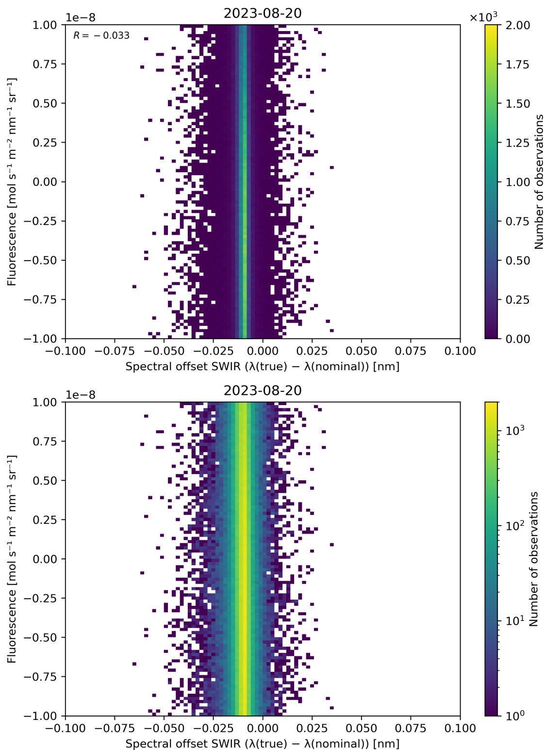
Figure 120: Scatter density plot of “Spectral offset SWIR ( \lambda(\text{true}) - \lambda(\text{nominal}) )” against “Fluorescence” for 2023-08-20 to 2023-08-21.
