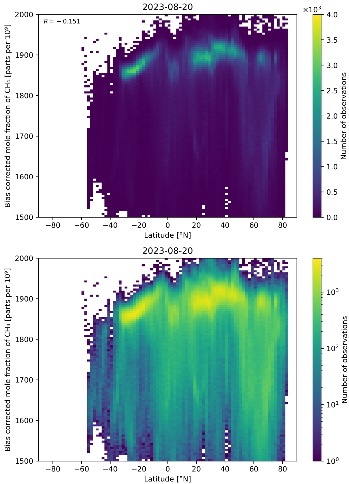
Figure 58: Scatter density plot of “Latitude” against “Bias corrected mole fraction of \text{CH}_4 ” for 2023-08-20 to 2023-08-21.
