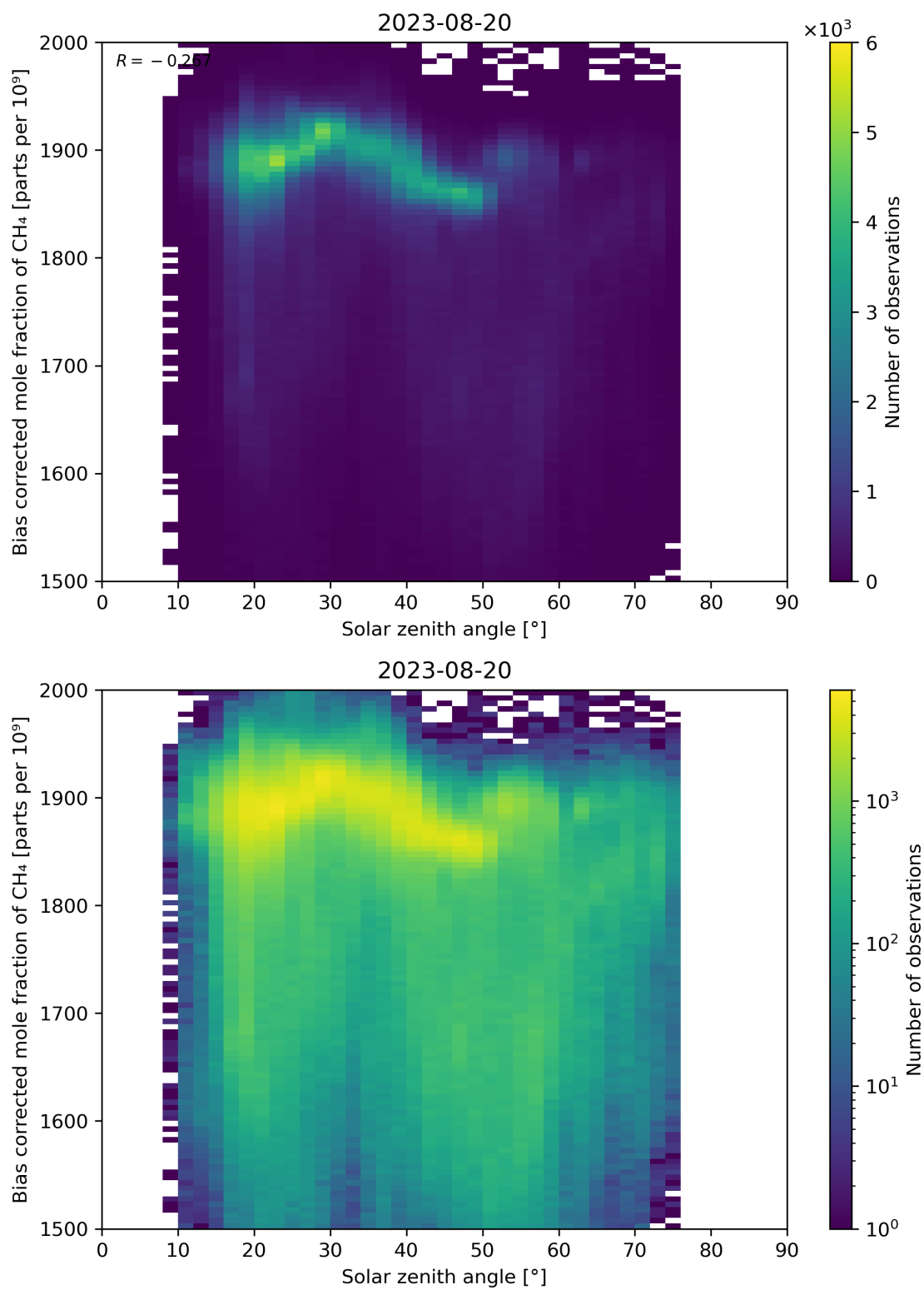
Figure 100: Scatter density plot of “Solar zenith angle” against “Bias corrected mole fraction of CH 4 ” for 2023-08-20 to 2023-08-21.
