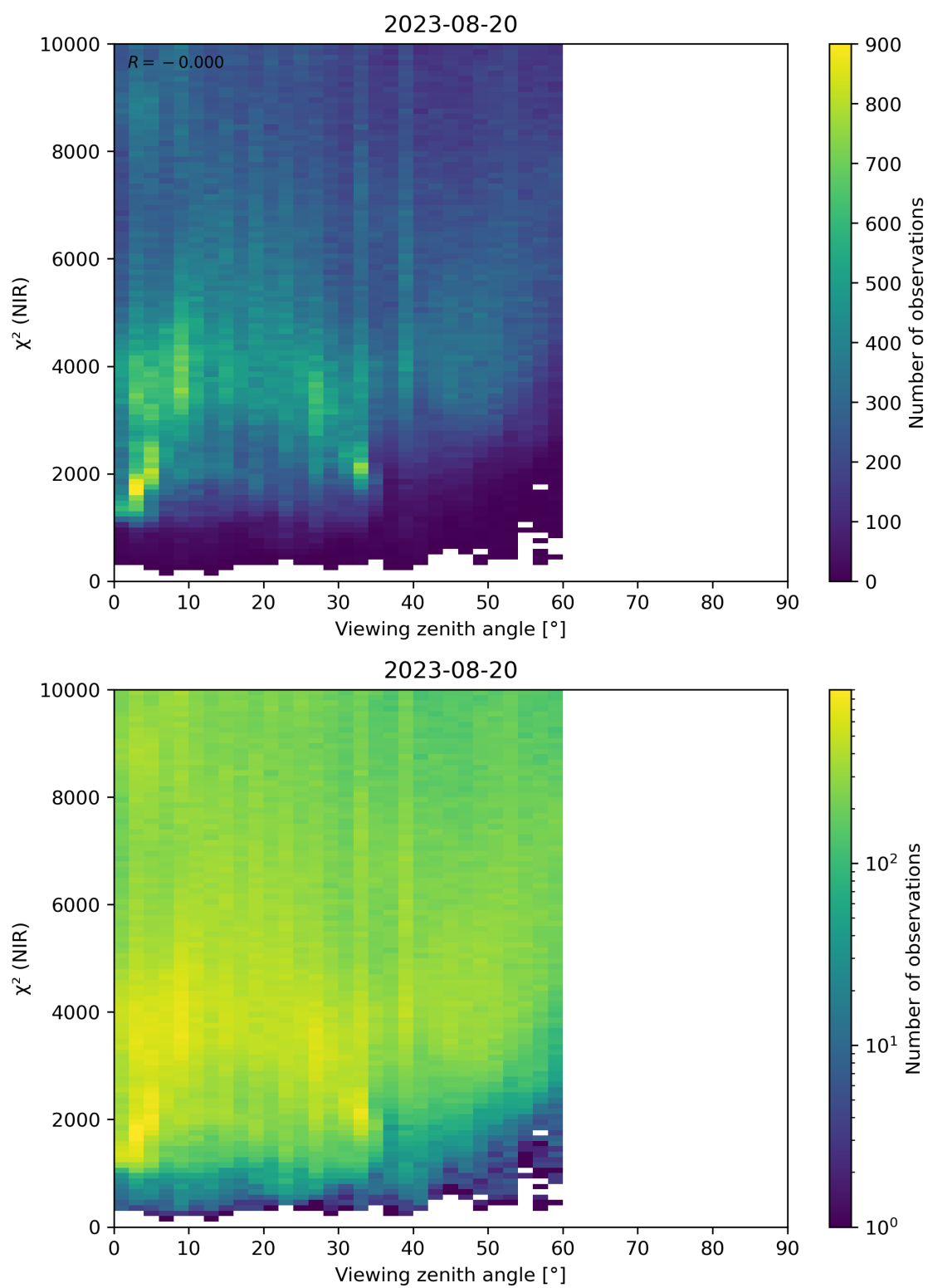
Figure 105: Scatter density plot of “Viewing zenith angle” against “ \chi^2 (NIR)” for 2023-08-20 to 2023-08-21.
