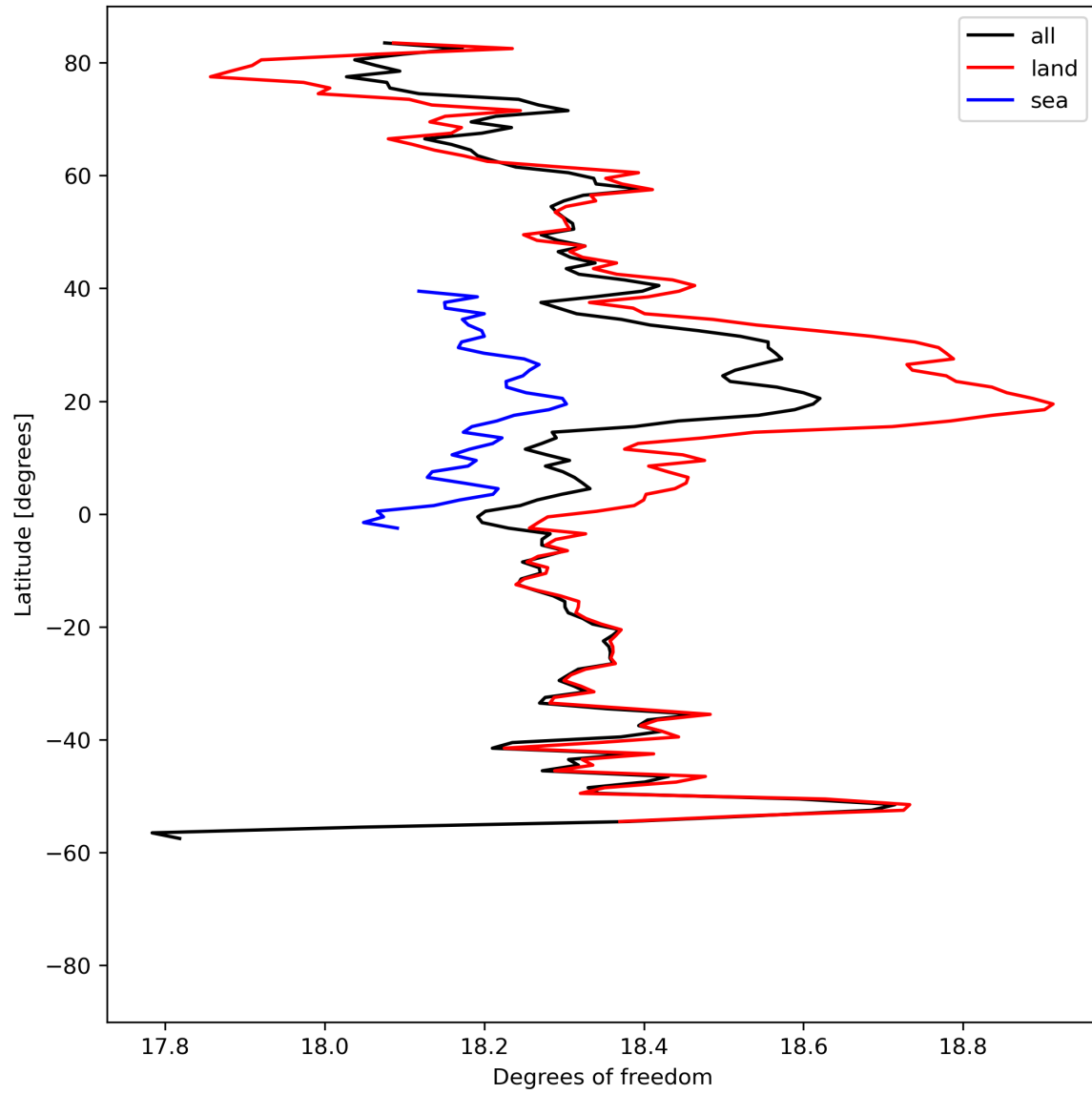
Figure 19: Zonal average of “Degrees of freedom” for 2023-08-20 to 2023-08-21.
