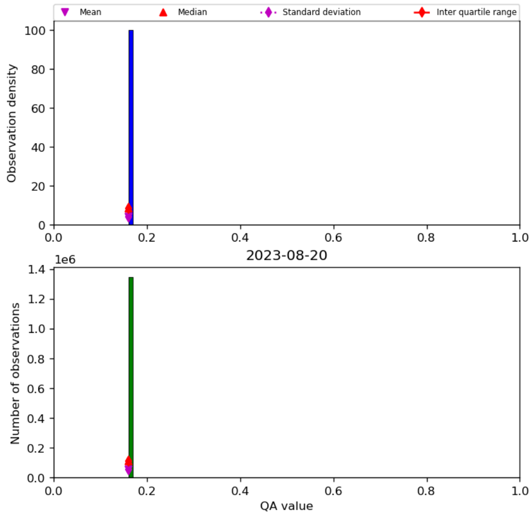
Figure 22: Histogram of “QA value” for 2023-08-20 to 2023-08-21
