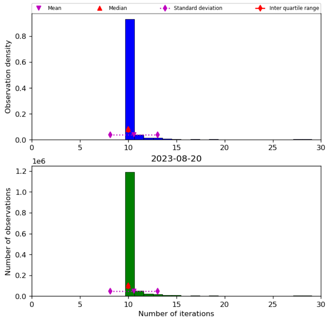
Figure 31: Histogram of “Number of iterations” for 2023-08-20 to 2023-08-21
