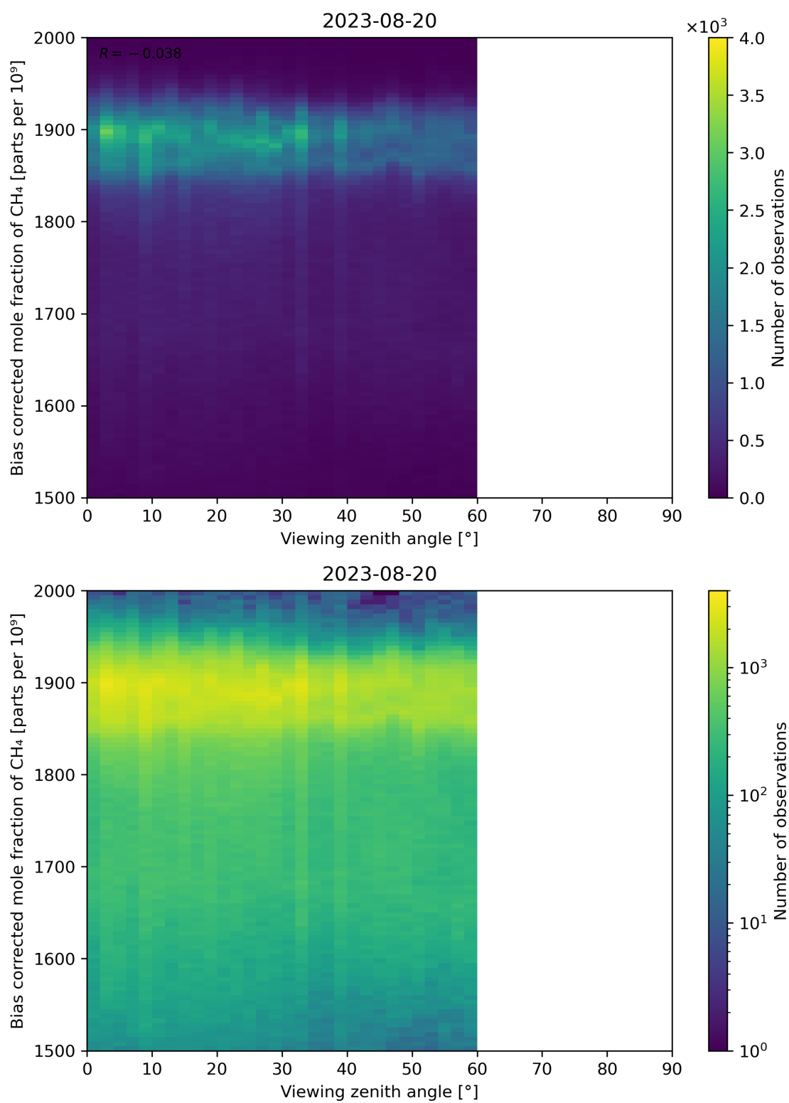
Figure 111: Scatter density plot of “Viewing zenith angle” against “Bias corrected mole fraction of CH 4 ” for 2023-08-20 to 2023-08-21.
