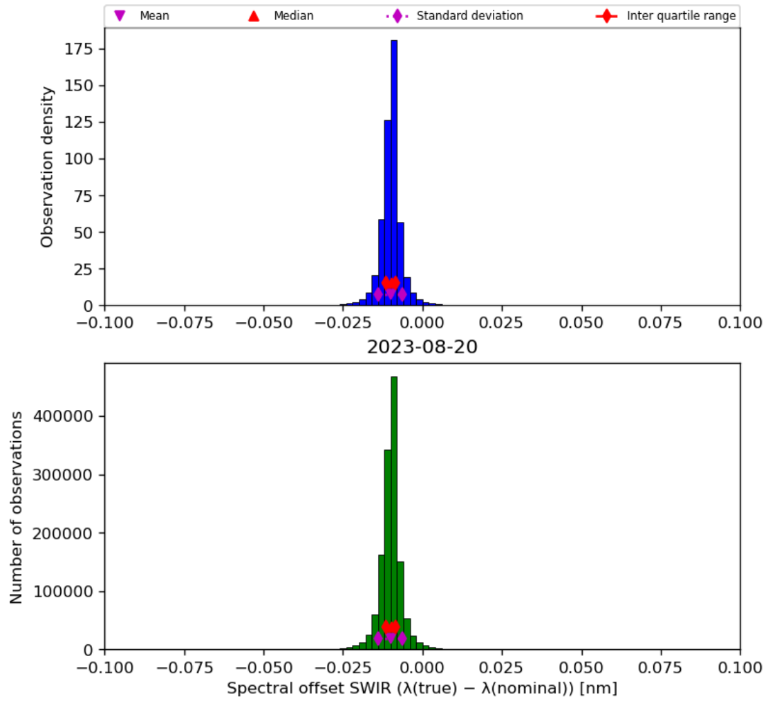
Figure 27: Histogram of “Spectral offset SWIR ( \lambda(\text{true}) - \lambda(\text{nominal}) )” for 2023-08-20 to 2023-08-21
