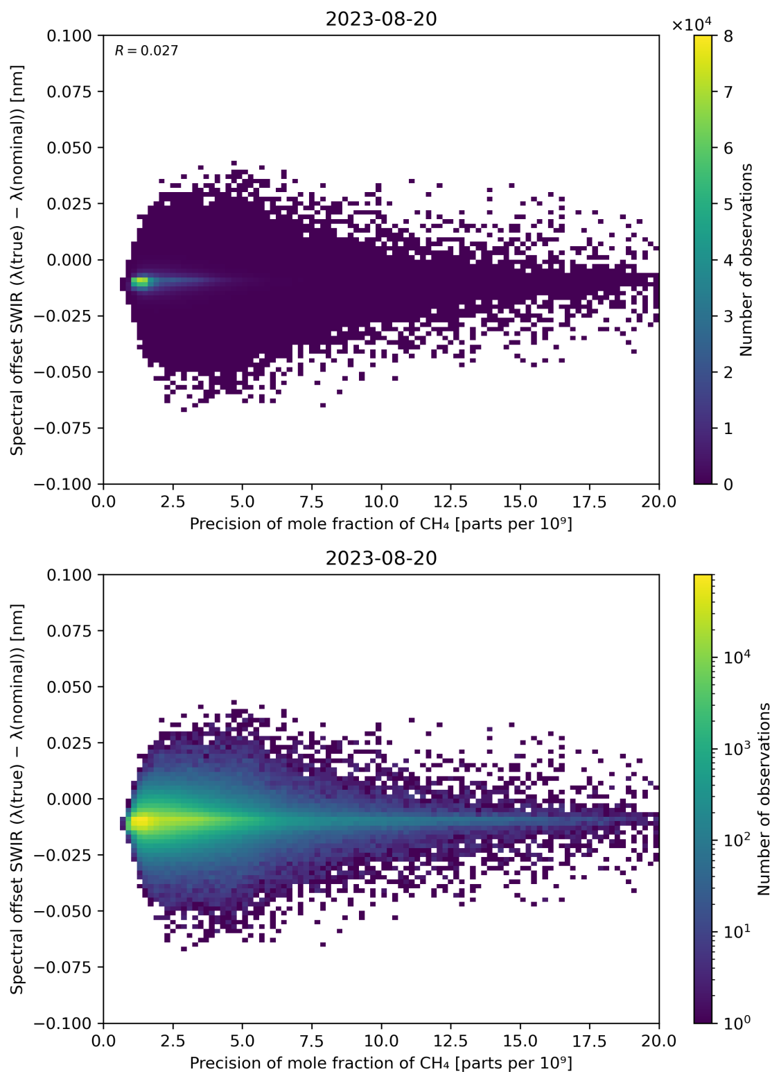
Figure 85: Scatter density plot of “Precision of mole fraction of CH 4 ” against “Spectral offset SWIR ( \lambda(\text{true}) - \lambda(\text{nominal}) )” for 2023-08-20 to 2023-08-21.
