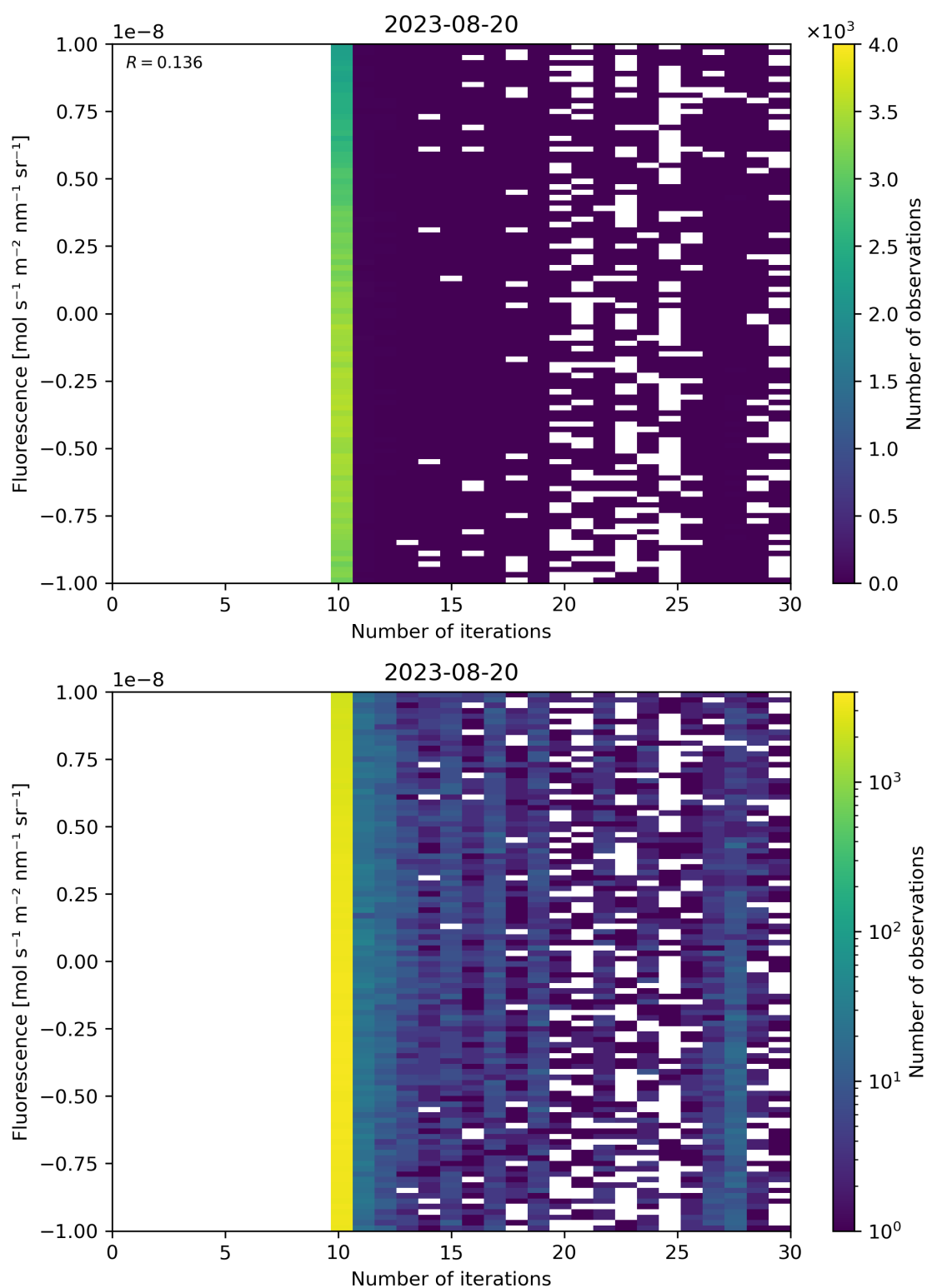
Figure 87: Scatter density plot of “Number of iterations” against “Fluorescence” for 2023-08-20 to 2023-08-21.
