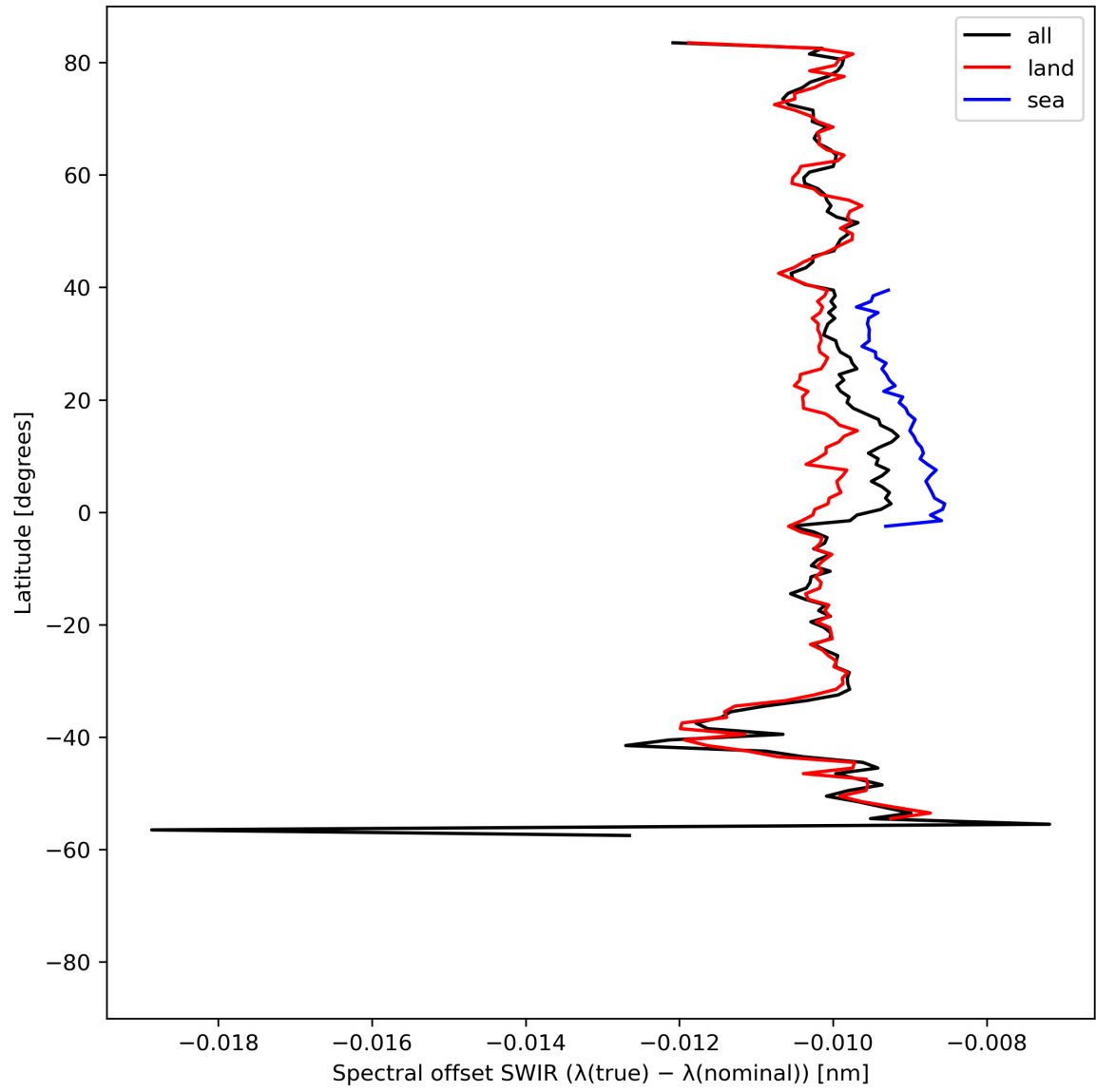
Figure 16: Zonal average of “Spectral offset SWIR ( \lambda(\text{true}) - \lambda(\text{nominal}) )” for 2023-08-20 to 2023-08-21.
