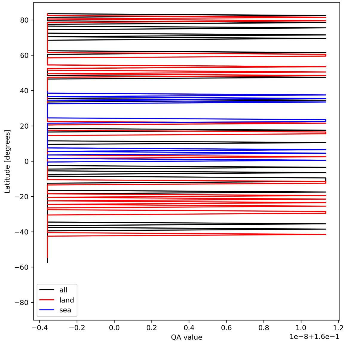
Figure 11: Zonal average of “QA value” for 2023-08-20 to 2023-08-21.
