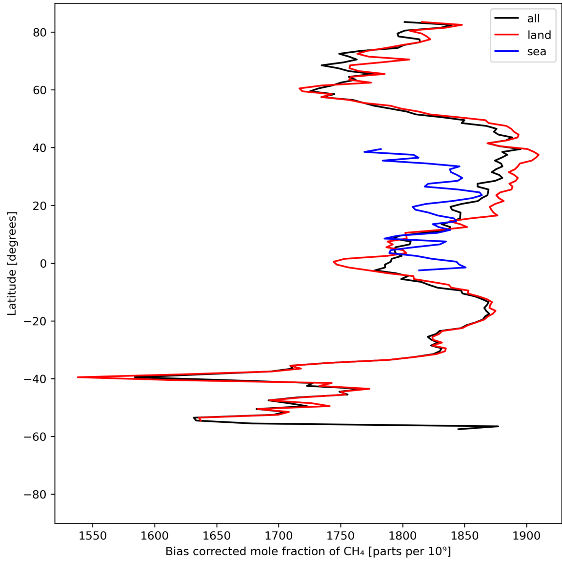
Figure 14: Zonal average of “Bias corrected mole fraction of CH 4 ” for 2023-08-20 to 2023-08-21.
