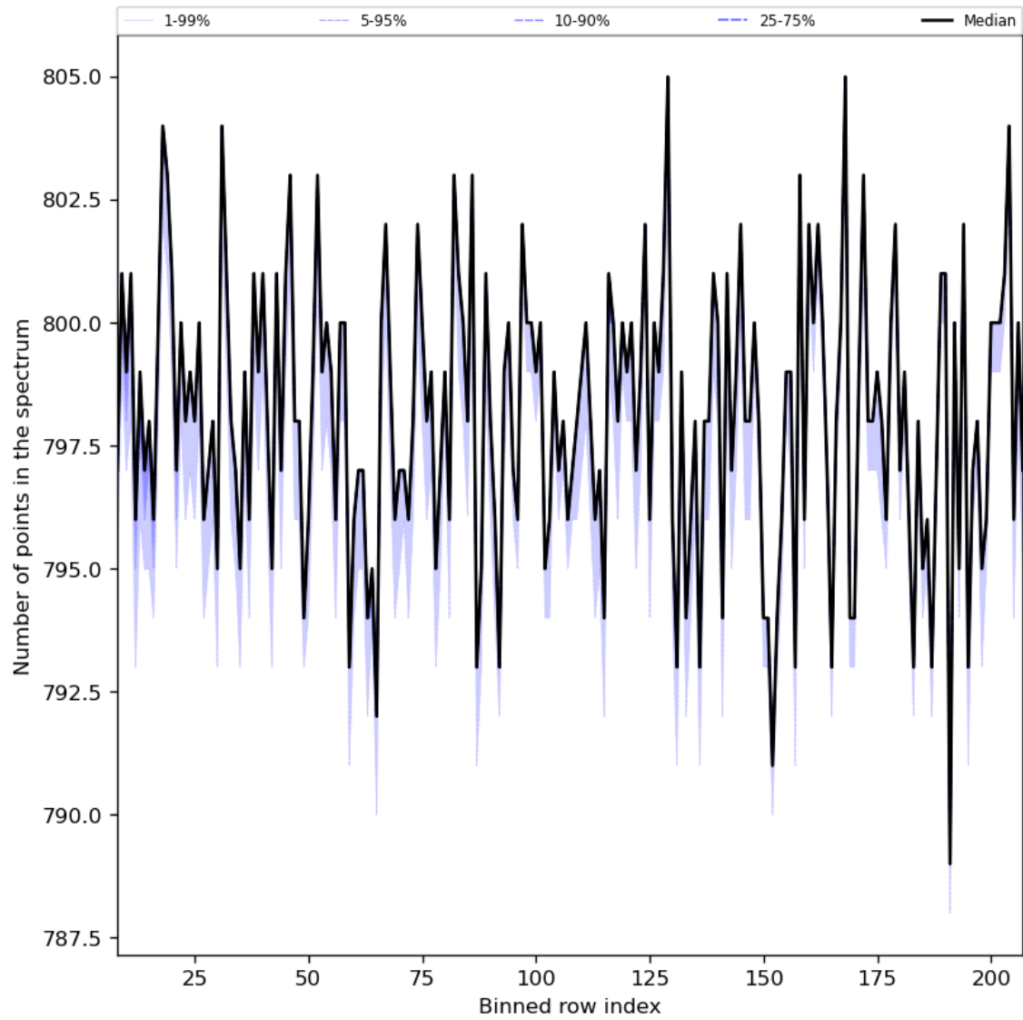
Figure 37: Along track statistics of “Number of points in the spectrum” for 2023-08-20 to 2023-08-21
