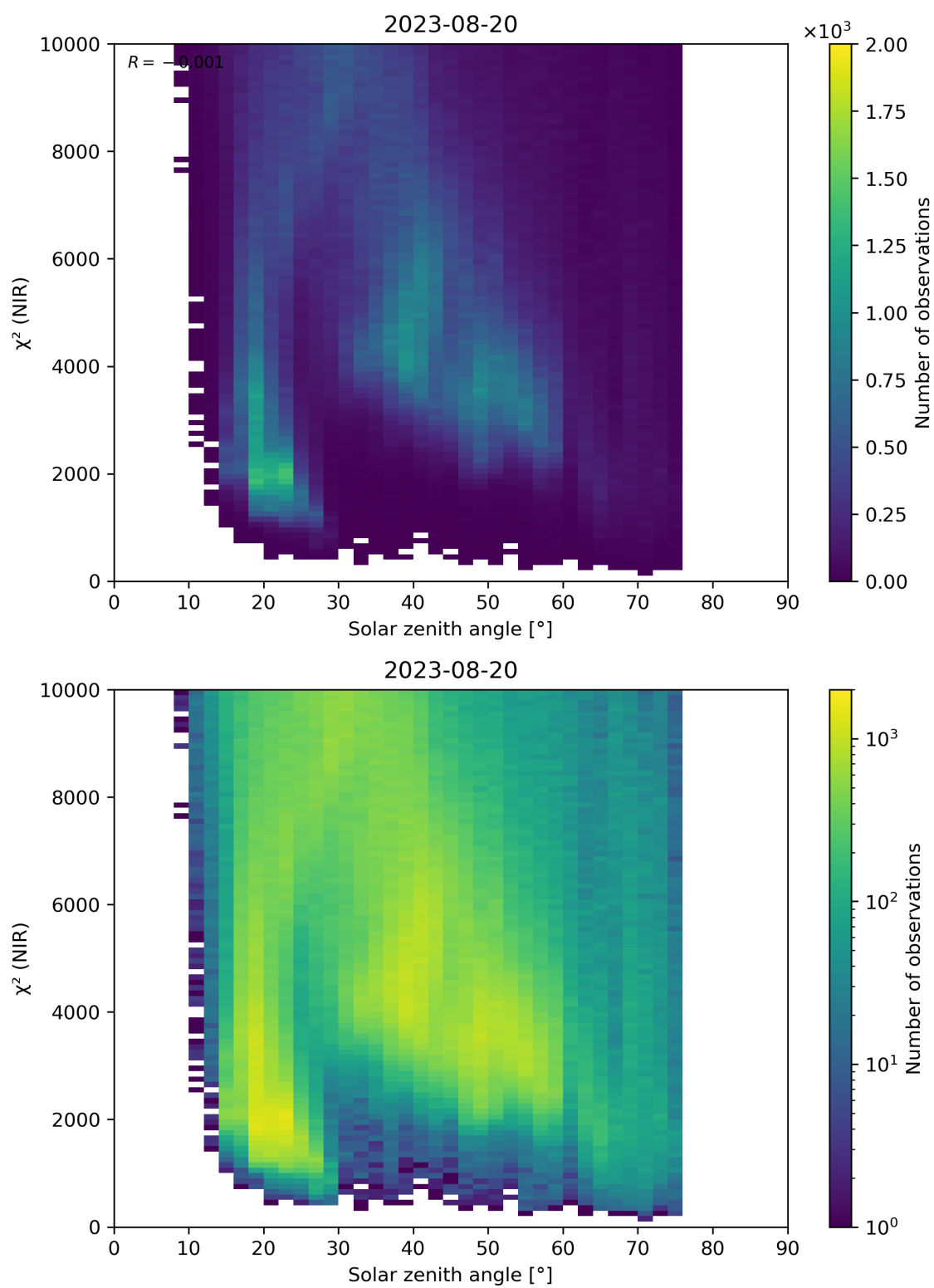
Figure 94: Scatter density plot of “Solar zenith angle” against “ \chi^2 (NIR)” for 2023-08-20 to 2023-08-21.
