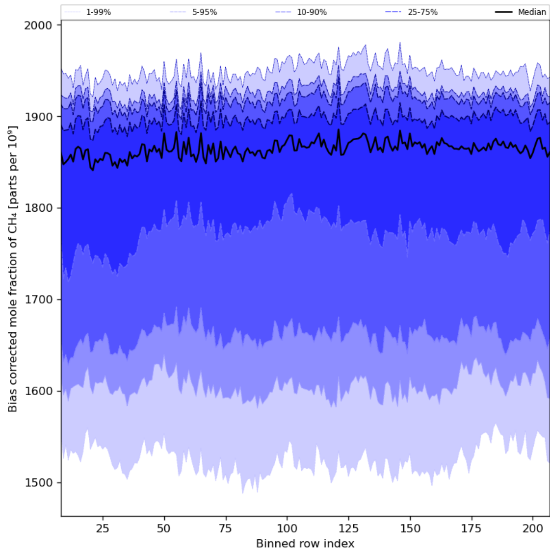
Figure 36: Along track statistics of “Bias corrected mole fraction of CH 4 ” for 2023-08-20 to 2023-08-21
