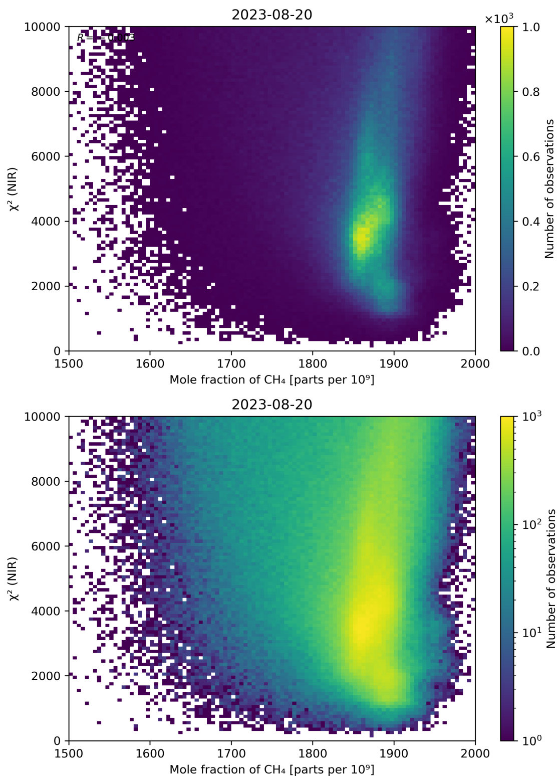
Figure 70: Scatter density plot of “Mole fraction of \text{CH}_4 ” against “ \chi^2 (NIR)” for 2023-08-20 to 2023-08-21.
