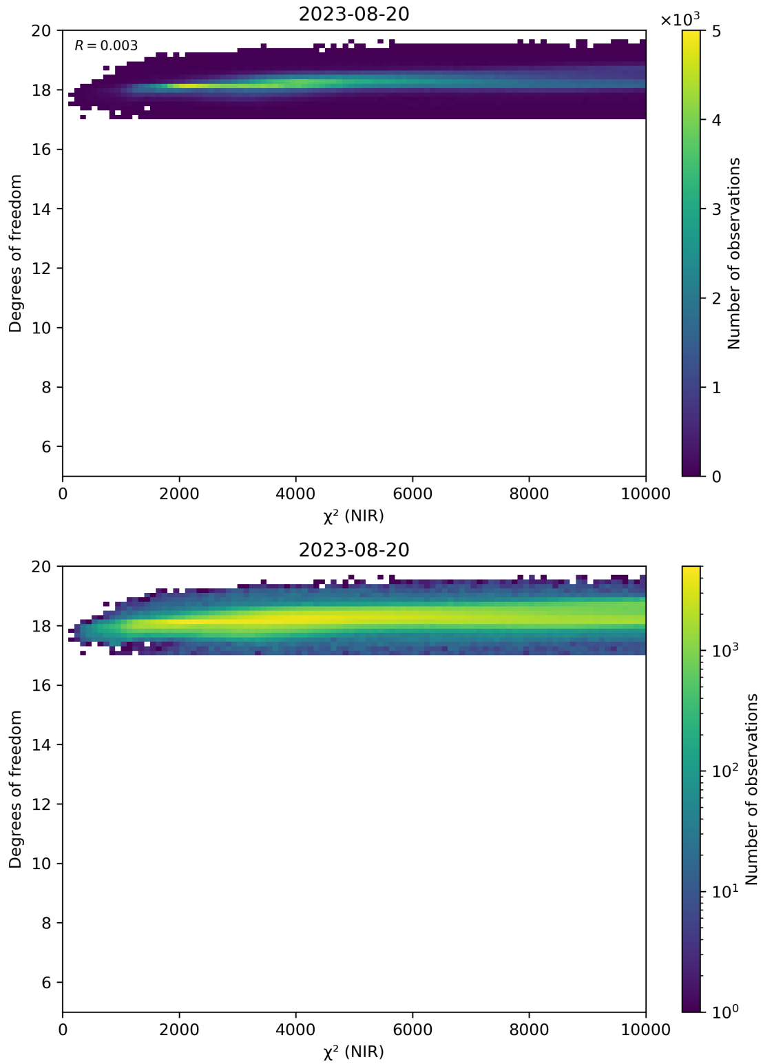
Figure 44: Scatter density plot of “ \chi^2 (NIR)” against “Degrees of freedom” for 2023-08-20 to 2023-08-21.
