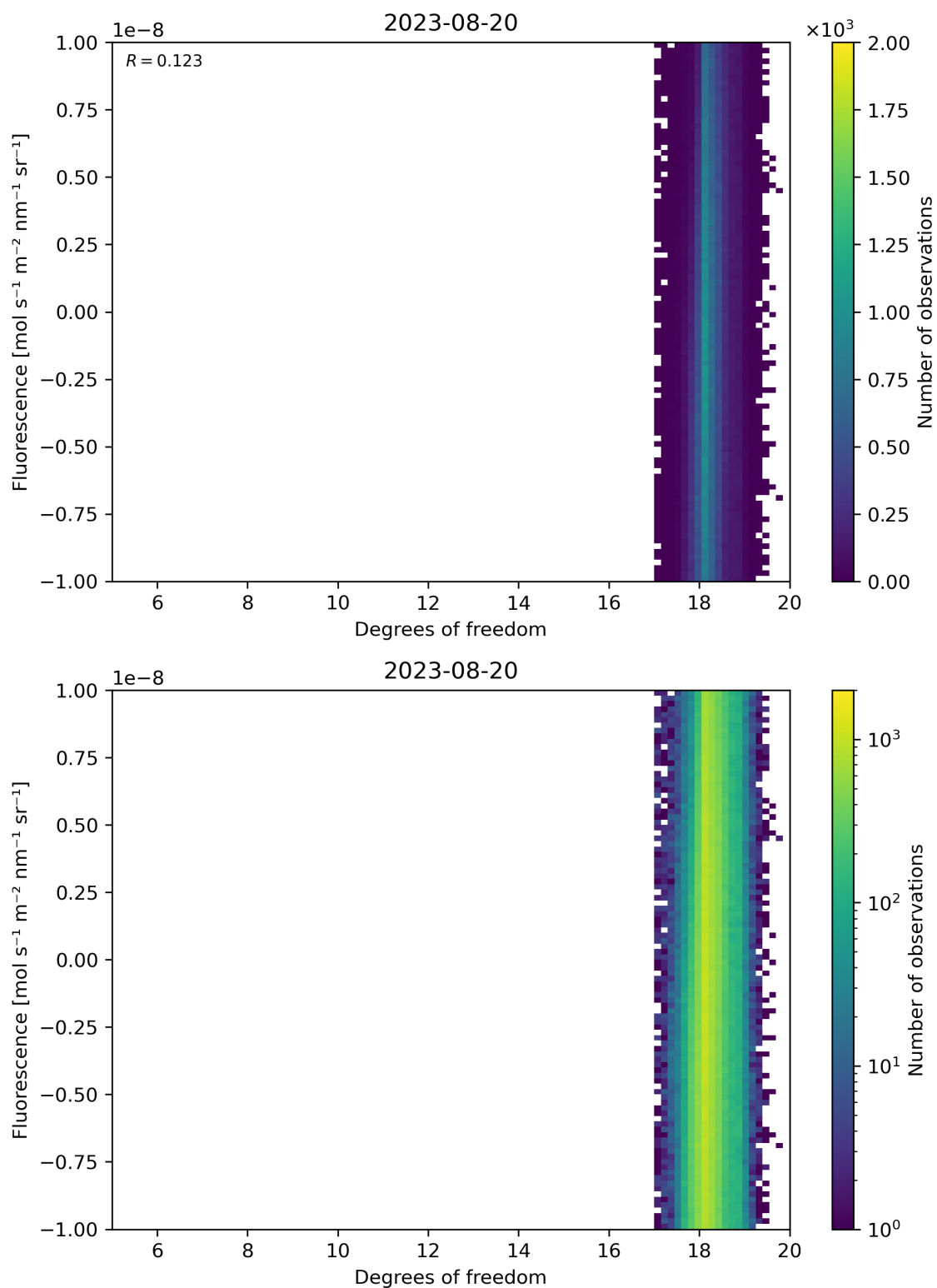
Figure 51: Scatter density plot of “Degrees of freedom” against “Fluorescence” for 2023-08-20 to 2023-08-21.
