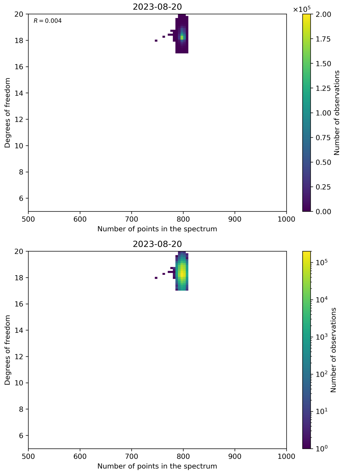
Figure 90: Scatter density plot of “Number of points in the spectrum” against “Degrees of freedom” for 2023-08-20 to 2023-08-21.
