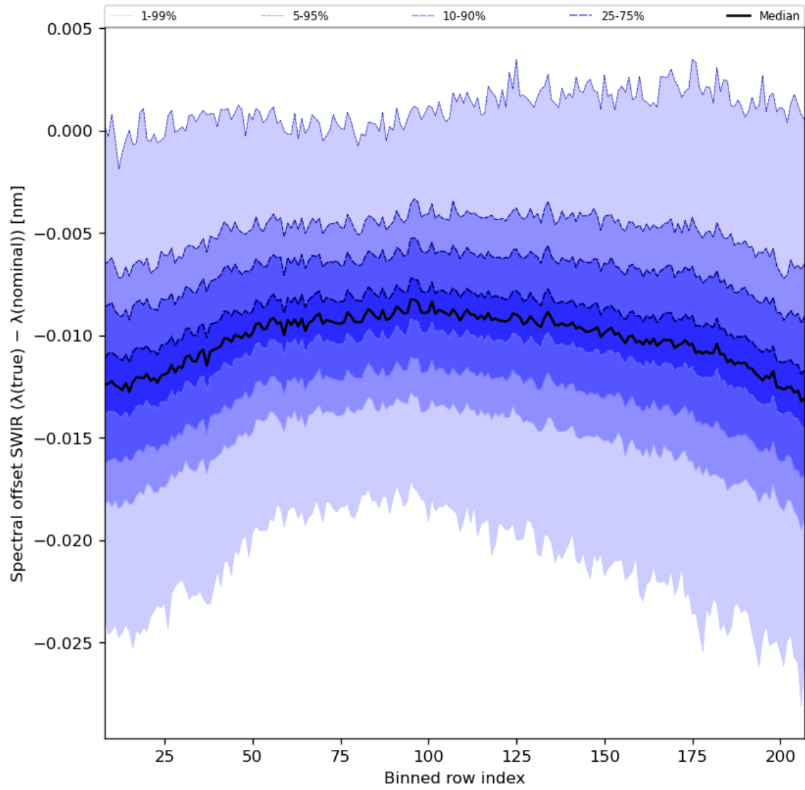
Figure 38: Along track statistics of “Spectral offset SWIR ( \lambda(\text{true}) - \lambda(\text{nominal}) )” for 2023-08-20 to 2023-08-21
