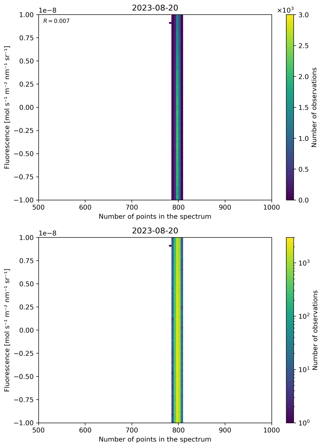
Figure 91: Scatter density plot of “Number of points in the spectrum” against “Fluorescence” for 2023-08-20 to 2023-08-21.
