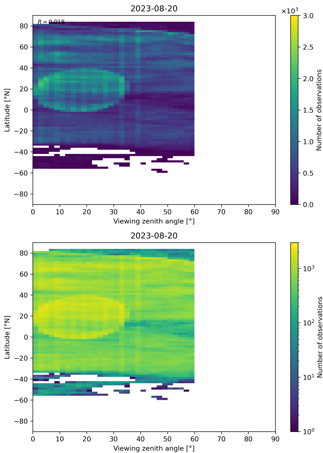
Figure 109: Scatter density plot of “Viewing zenith angle” against “Latitude” for 2023-08-20 to 2023-08-21.
