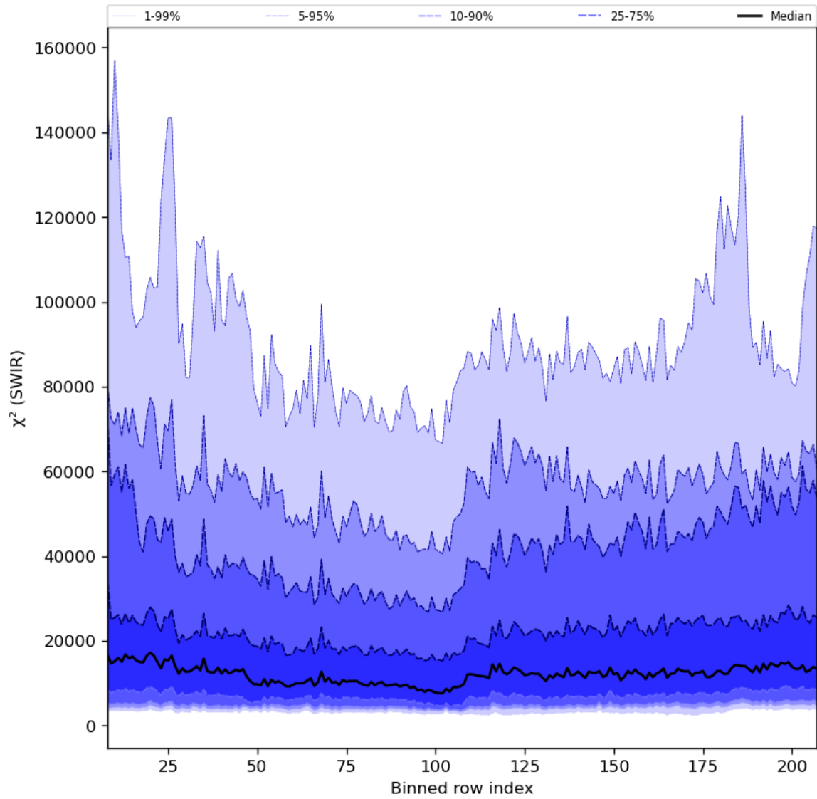
Figure 39: Along track statistics of “ \chi^2 (SWIR)” for 2023-08-20 to 2023-08-21
