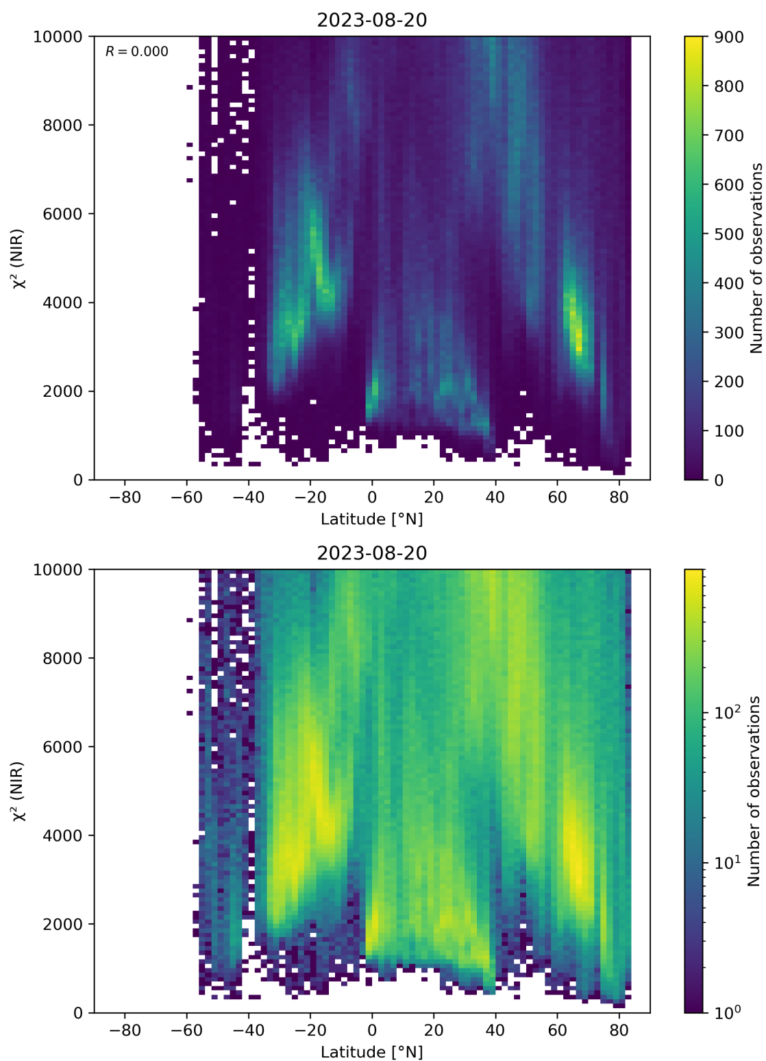
Figure 53: Scatter density plot of “Latitude” against “ \chi^2 (NIR)” for 2023-08-20 to 2023-08-21.
