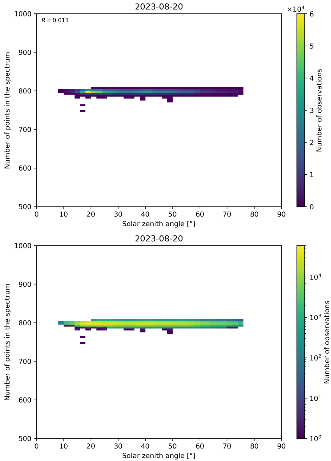
Figure 103: Scatter density plot of “Solar zenith angle” against “Number of points in the spectrum” for 2023-08-20 to 2023-08-21.
