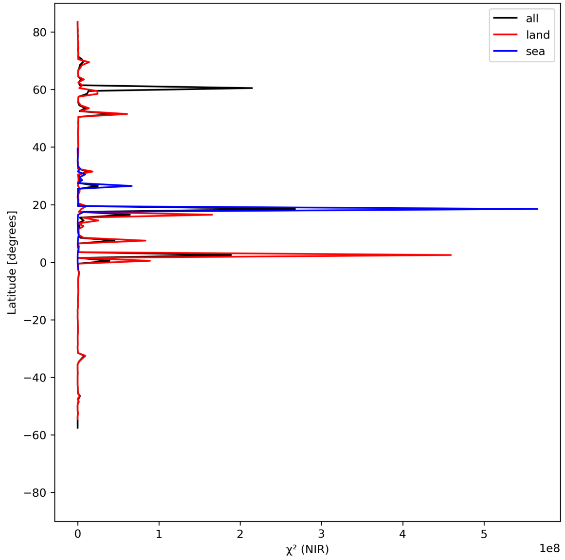
Figure 18: Zonal average of “ \chi^2 (NIR)” for 2023-08-20 to 2023-08-21.
