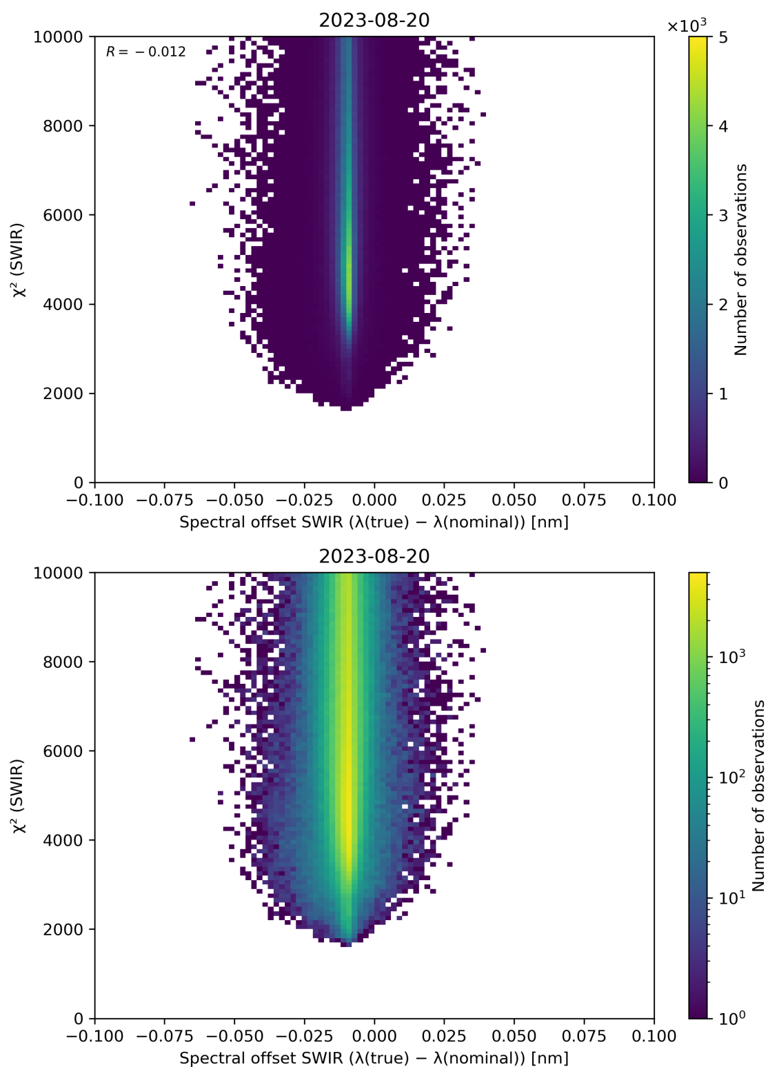
Figure 118: Scatter density plot of “Spectral offset SWIR ( \lambda(\text{true}) - \lambda(\text{nominal}) )” against “ \chi^2 (SWIR)” for 2023-08-20 to 2023-08-21.
