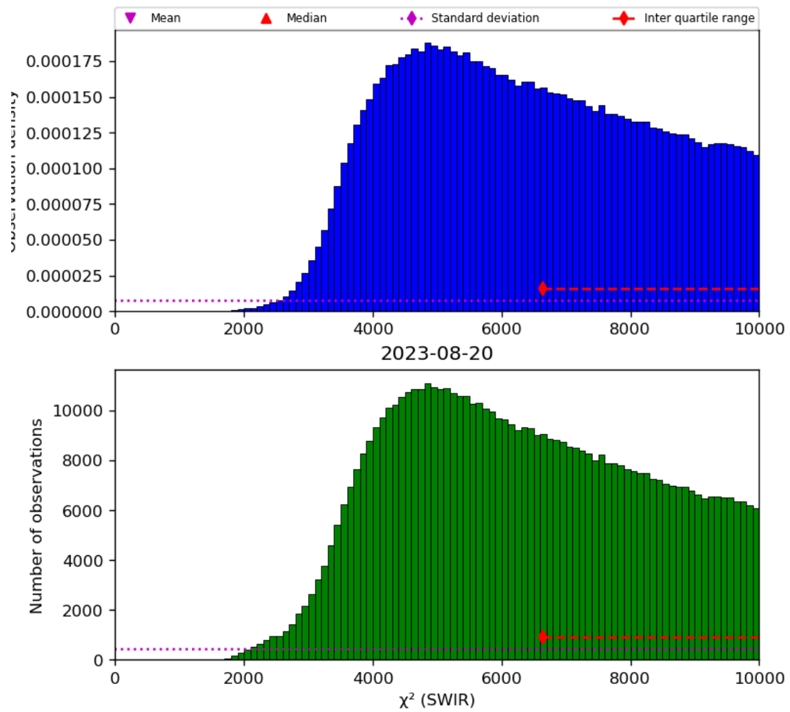
Figure 28: Histogram of “ \chi^2 (SWIR)” for 2023-08-20 to 2023-08-21
