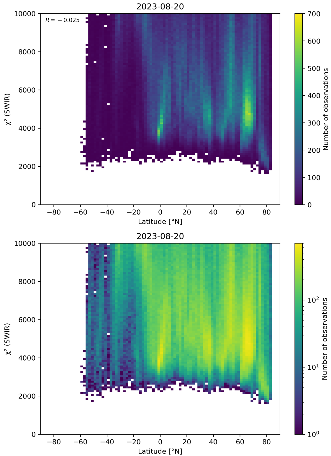
Figure 54: Scatter density plot of “Latitude” against “ \chi^2 (SWIR)” for 2023-08-20 to 2023-08-21.
