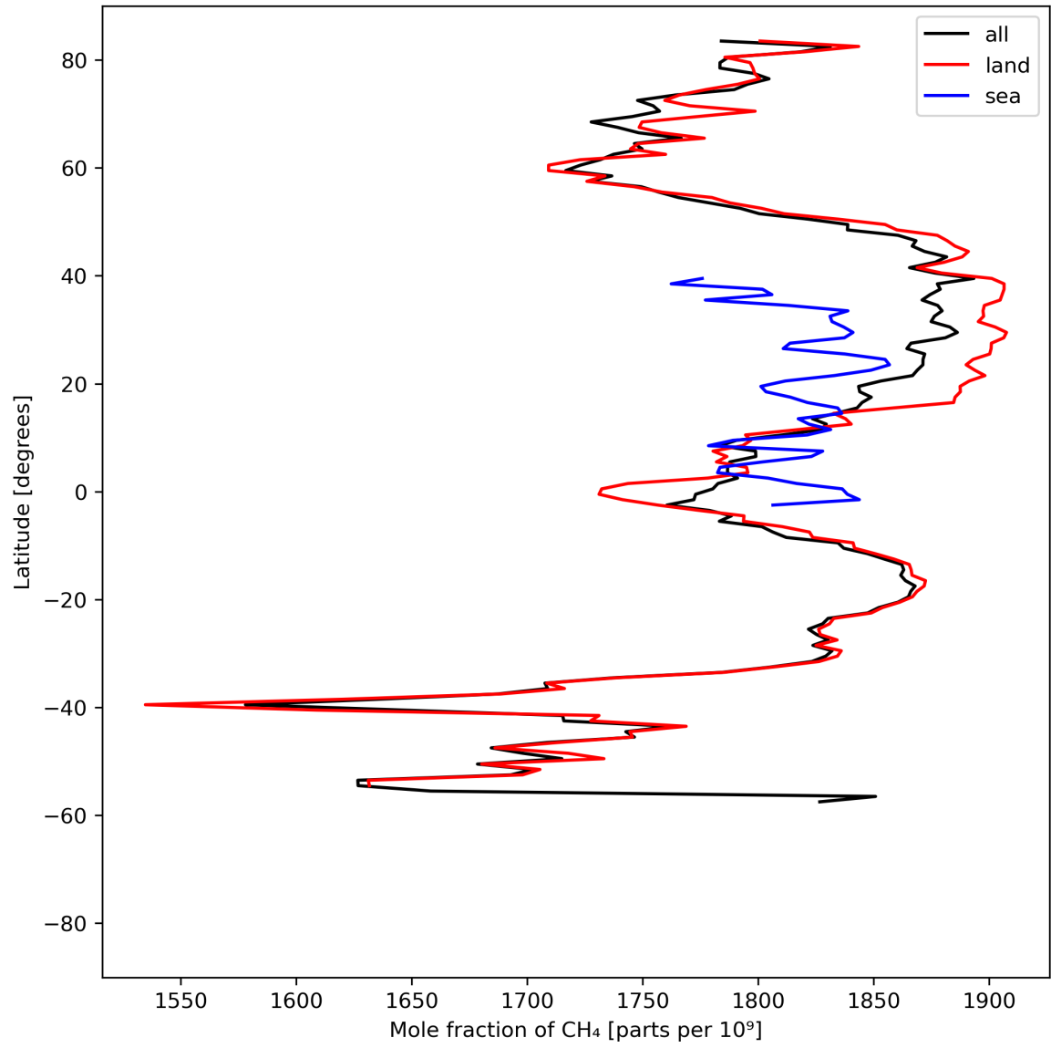
Figure 12: Zonal average of “Mole fraction of \text{CH}_4 ” for 2023-08-20 to 2023-08-21.
