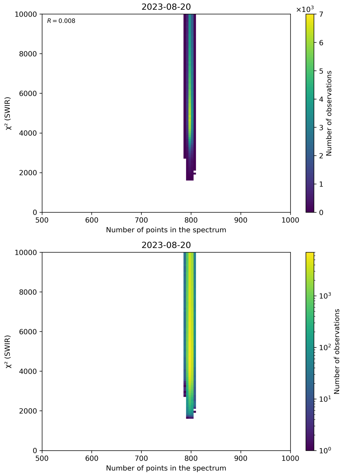
Figure 89: Scatter density plot of “Number of points in the spectrum” against “ \chi^2 (SWIR)” for 2023-08-20 to 2023-08-21.
