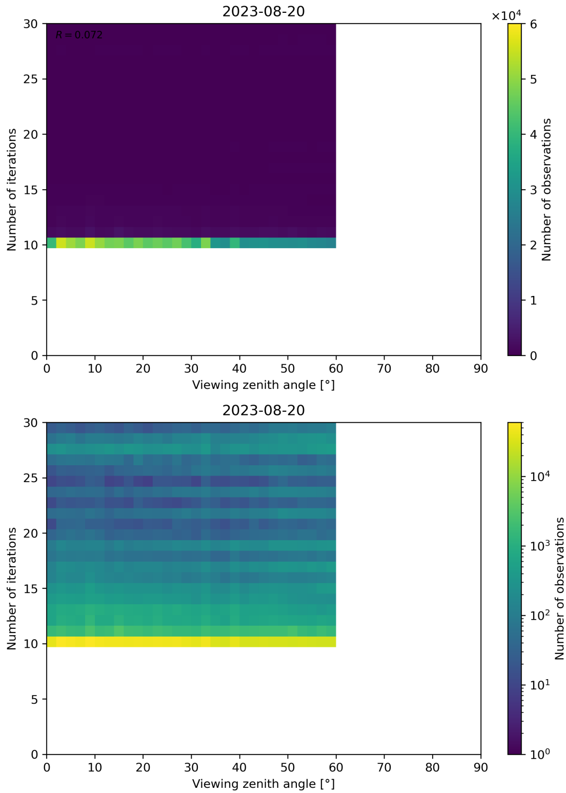
Figure 113: Scatter density plot of “Viewing zenith angle” against “Number of iterations” for 2023-08-20 to 2023-08-21.
