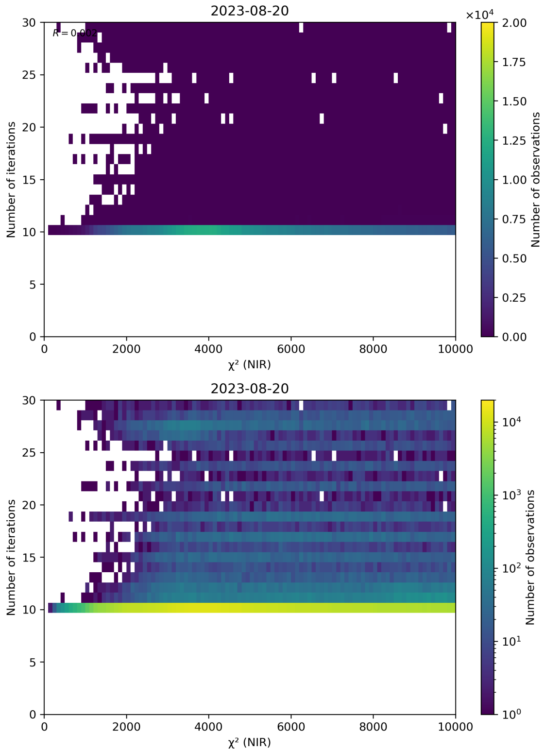
Figure 46: Scatter density plot of “ \chi^2 (NIR)” against “Number of iterations” for 2023-08-20 to 2023-08-21.
