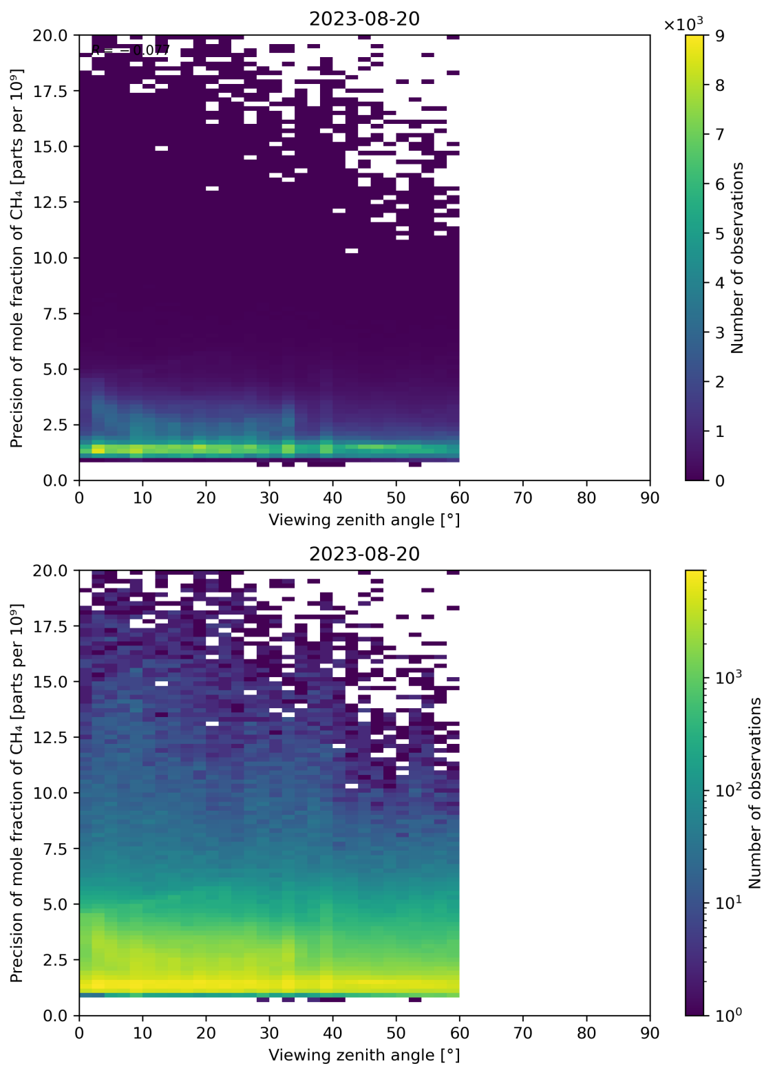
Figure 112: Scatter density plot of “Viewing zenith angle” against “Precision of mole fraction of CH 4 ” for 2023-08-20 to 2023-08-21.
