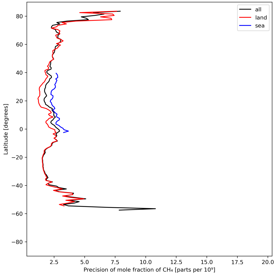
Figure 13: Zonal average of “Precision of mole fraction of \text{CH}_4 ” for 2023-08-20 to 2023-08-21.
