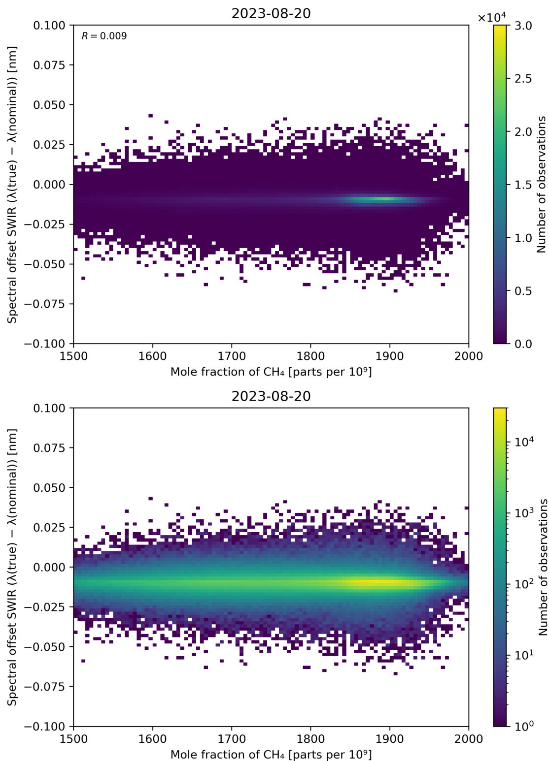
Figure 86: Scatter density plot of “Mole fraction of CH 4 ” against “Spectral offset SWIR ( \lambda(\text{true}) - \lambda(\text{nominal}) )” for 2023-08-20 to 2023-08-21.
