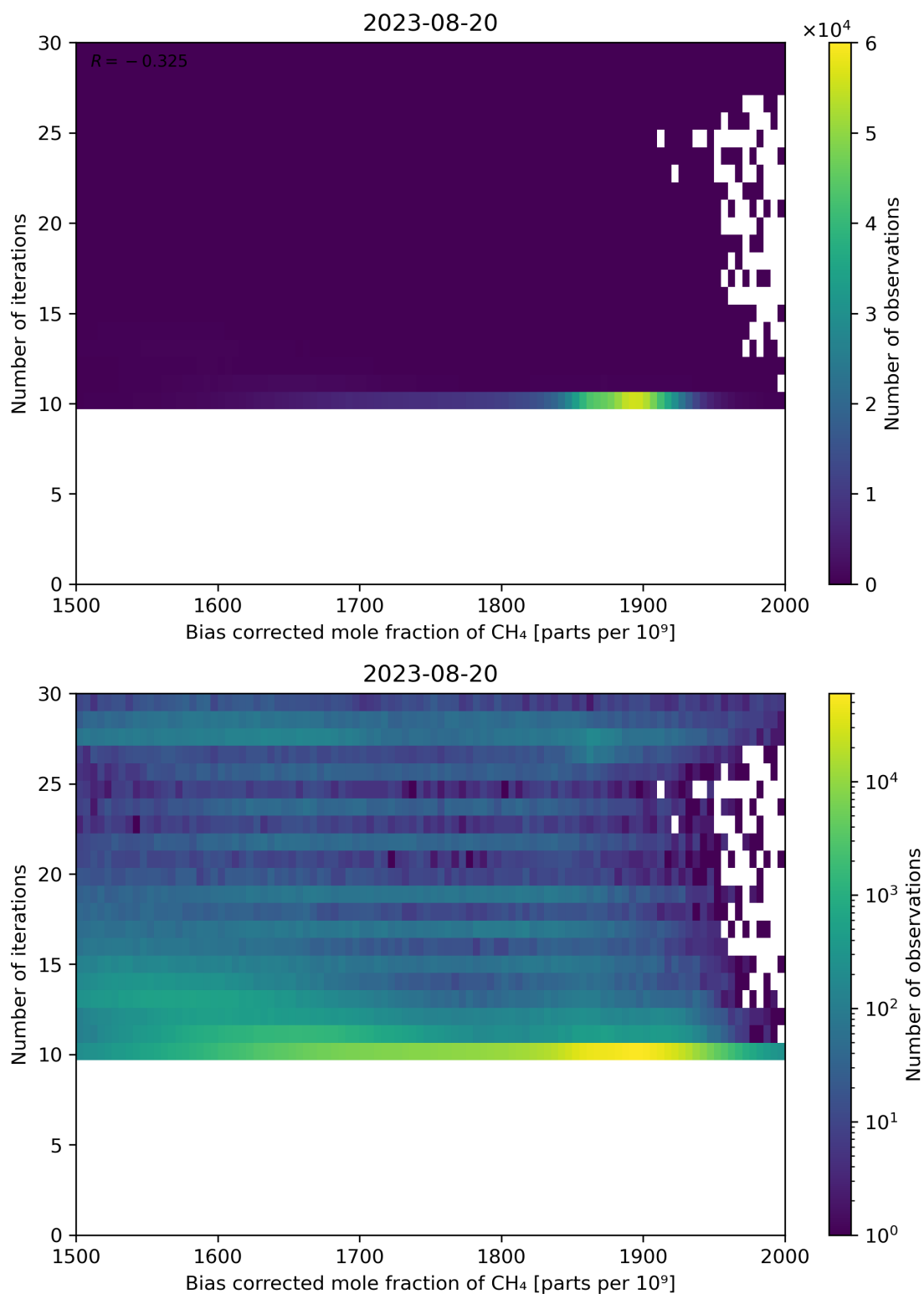
Figure 67: Scatter density plot of “Bias corrected mole fraction of CH 4 ” against “Number of iterations” for 2023-08-20 to 2023-08-21.
