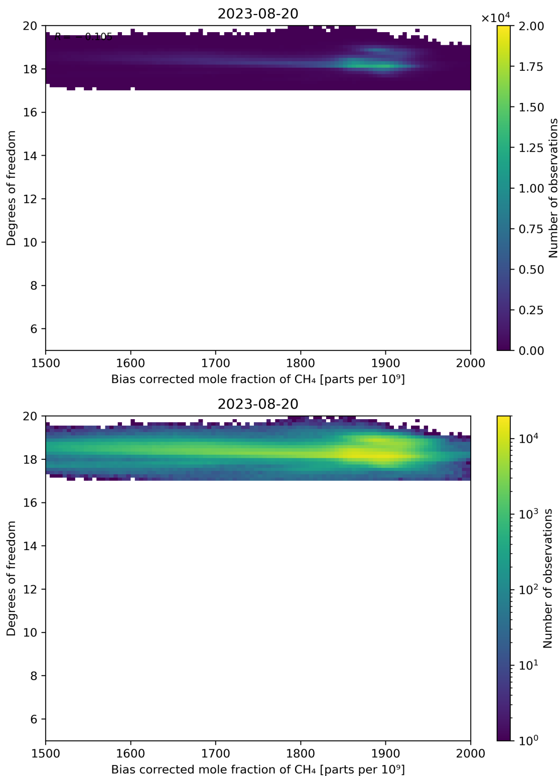
Figure 65: Scatter density plot of “Bias corrected mole fraction of CH 4 ” against “Degrees of freedom” for 2023-08-20 to 2023-08-21.
