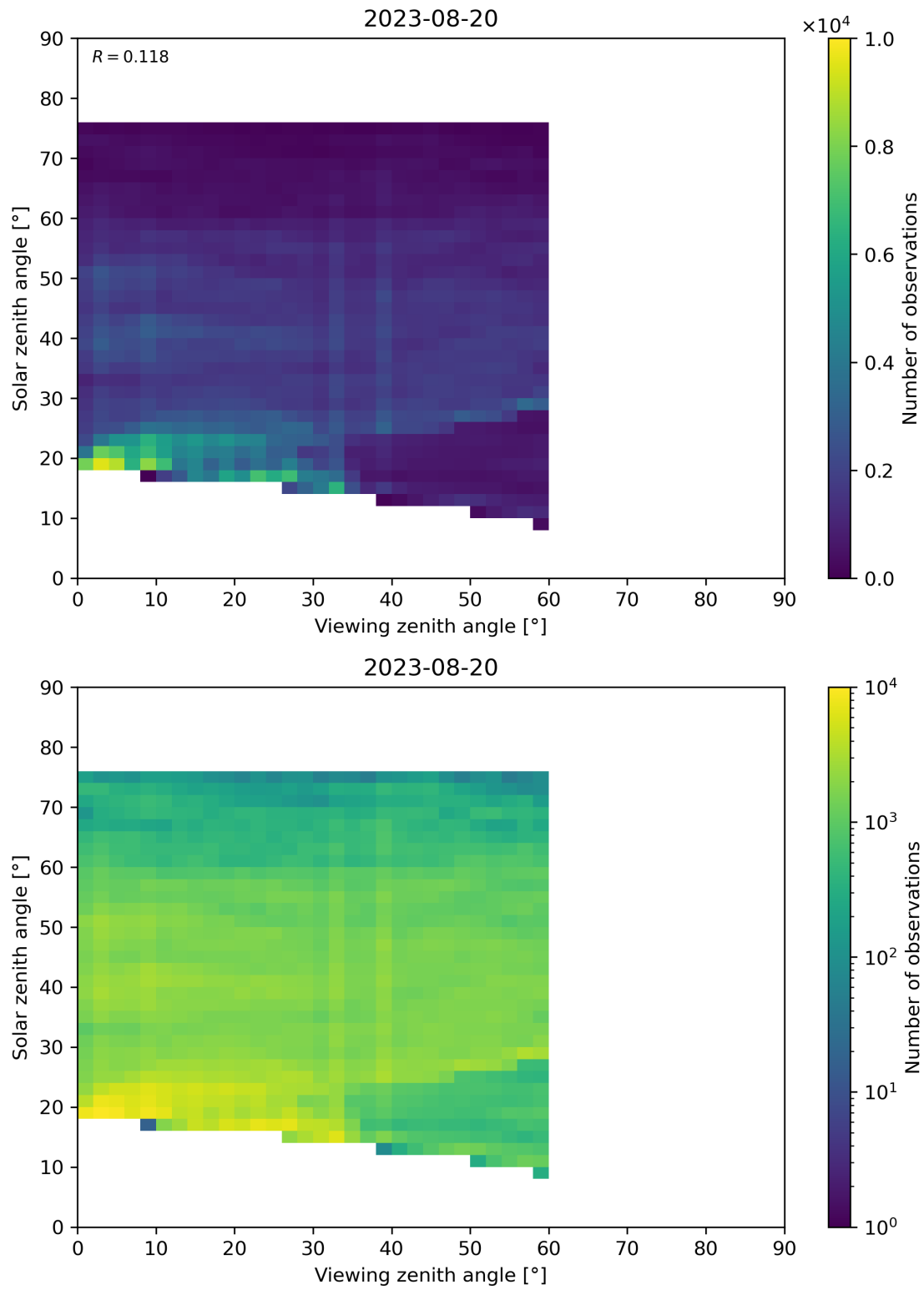
Figure 115: Scatter density plot of “Viewing zenith angle” against “Solar zenith angle” for 2023-08-20 to 2023-08-21.
