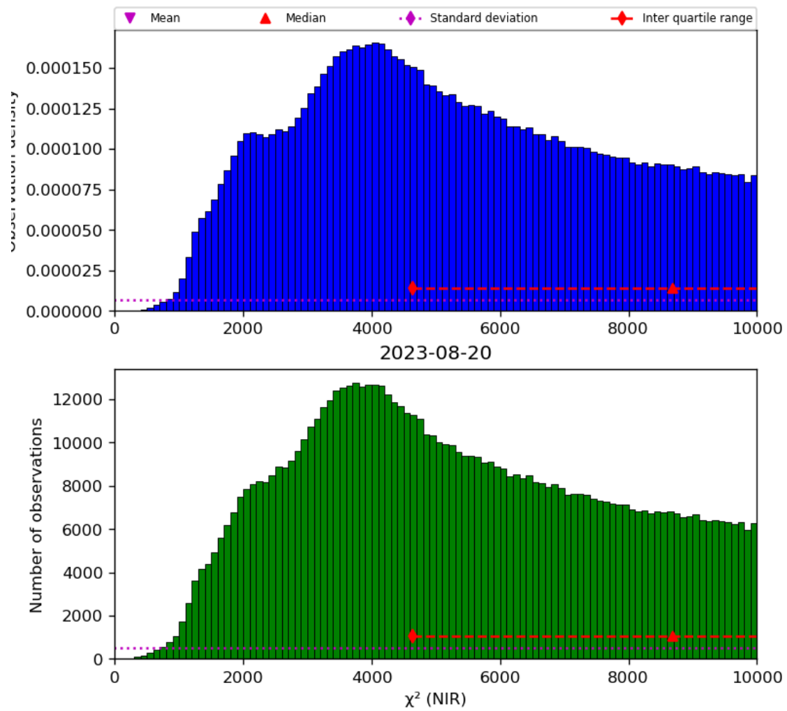
Figure 29: Histogram of “ \chi^2 (NIR)” for 2023-08-20 to 2023-08-21
