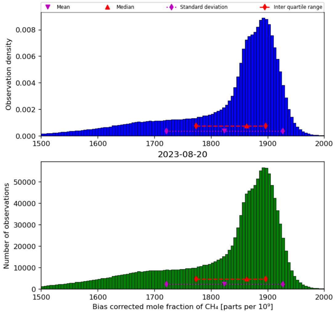
Figure 25: Histogram of “Bias corrected mole fraction of CH 4 ” for 2023-08-20 to 2023-08-21
