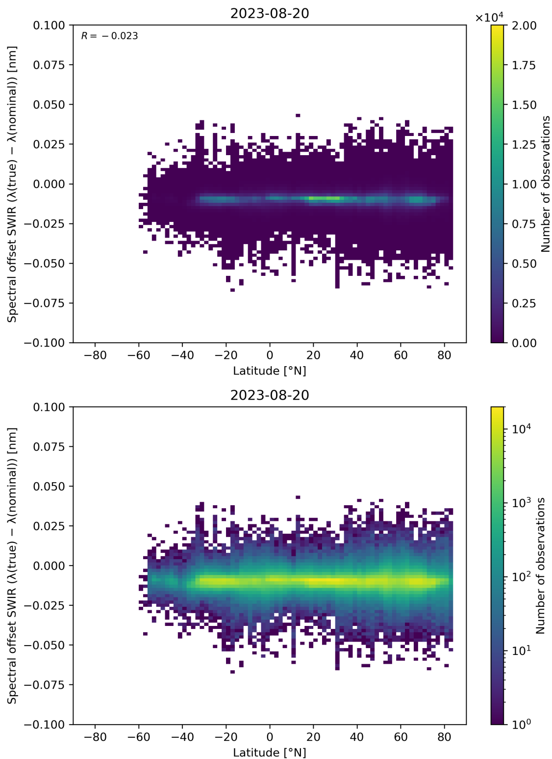
Figure 62: Scatter density plot of “Latitude” against “Spectral offset SWIR ( \lambda(\text{true}) - \lambda(\text{nominal}) )” for 2023-08-20 to 2023-08-21.
