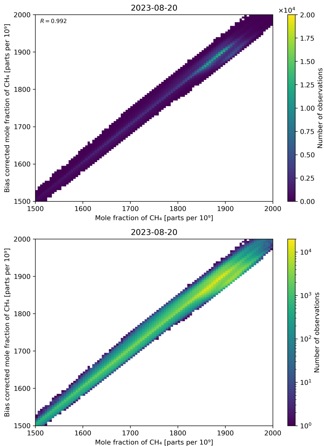
Figure 74: Scatter density plot of “Mole fraction of CH 4 ” against “Bias corrected mole fraction of CH 4 ” for 2023-08-20 to 2023-08-21.
