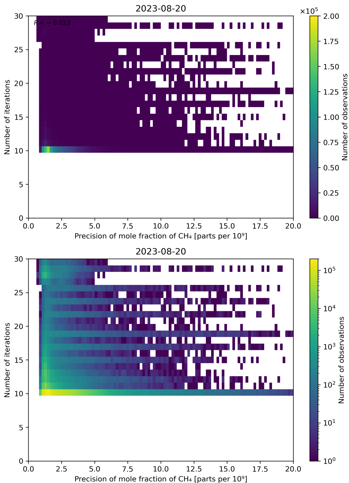
Figure 83: Scatter density plot of “Precision of mole fraction of CH 4 ” against “Number of iterations” for 2023-08-20 to 2023-08-21.
