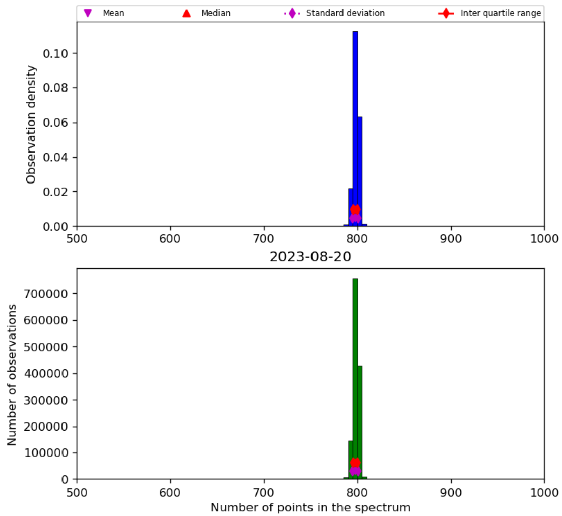
Figure 26: Histogram of “Number of points in the spectrum” for 2023-08-20 to 2023-08-21
