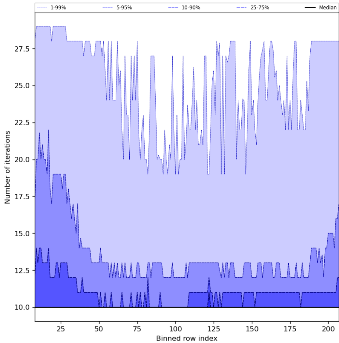
Figure 42: Along track statistics of “Number of iterations” for 2023-08-20 to 2023-08-21
