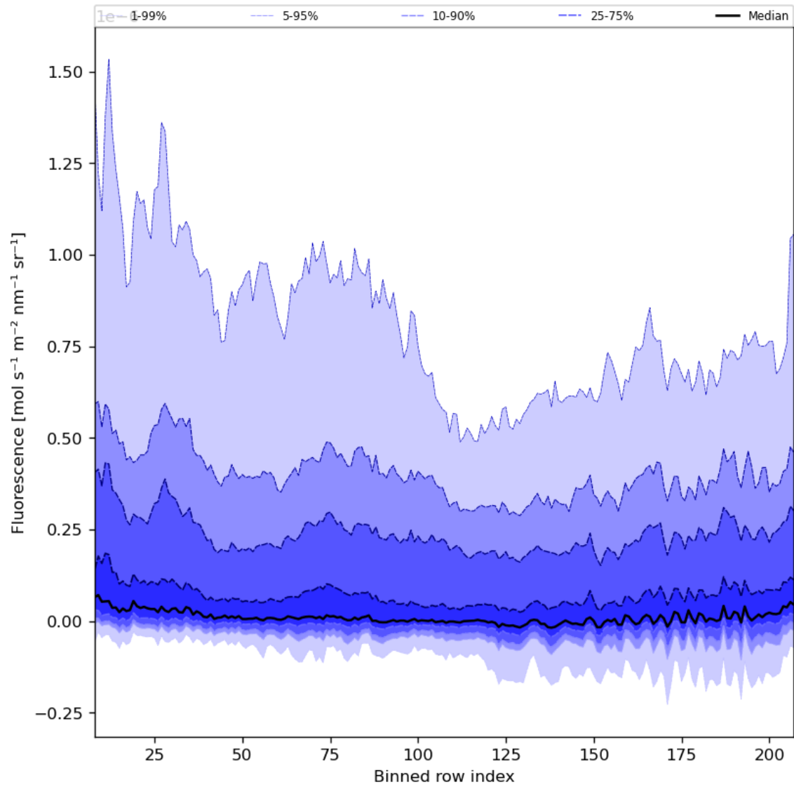
Figure 43: Along track statistics of “Fluorescence” for 2023-08-20 to 2023-08-21
