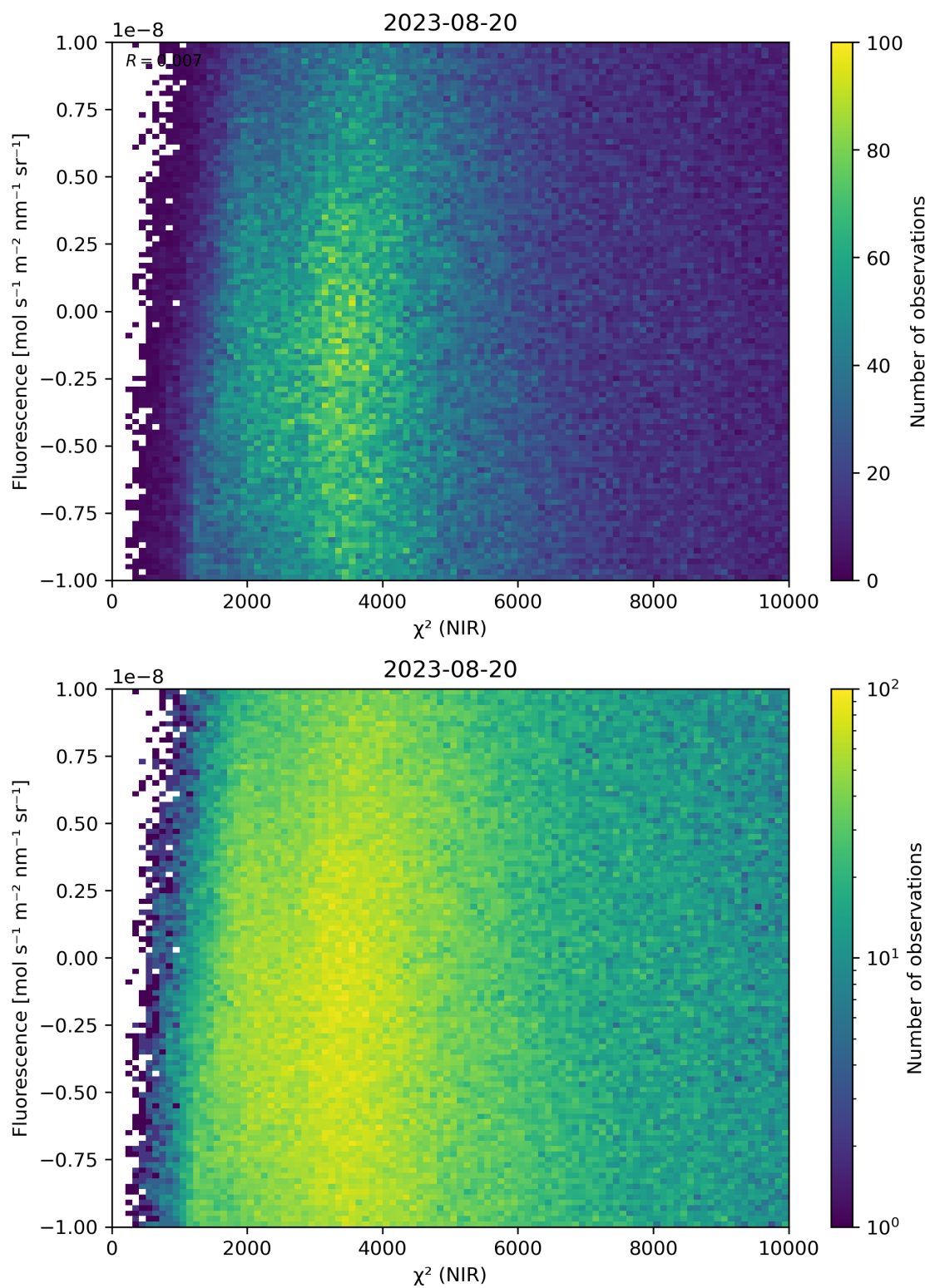
Figure 45: Scatter density plot of “ \chi^2 (NIR)” against “Fluorescence” for 2023-08-20 to 2023-08-21.
