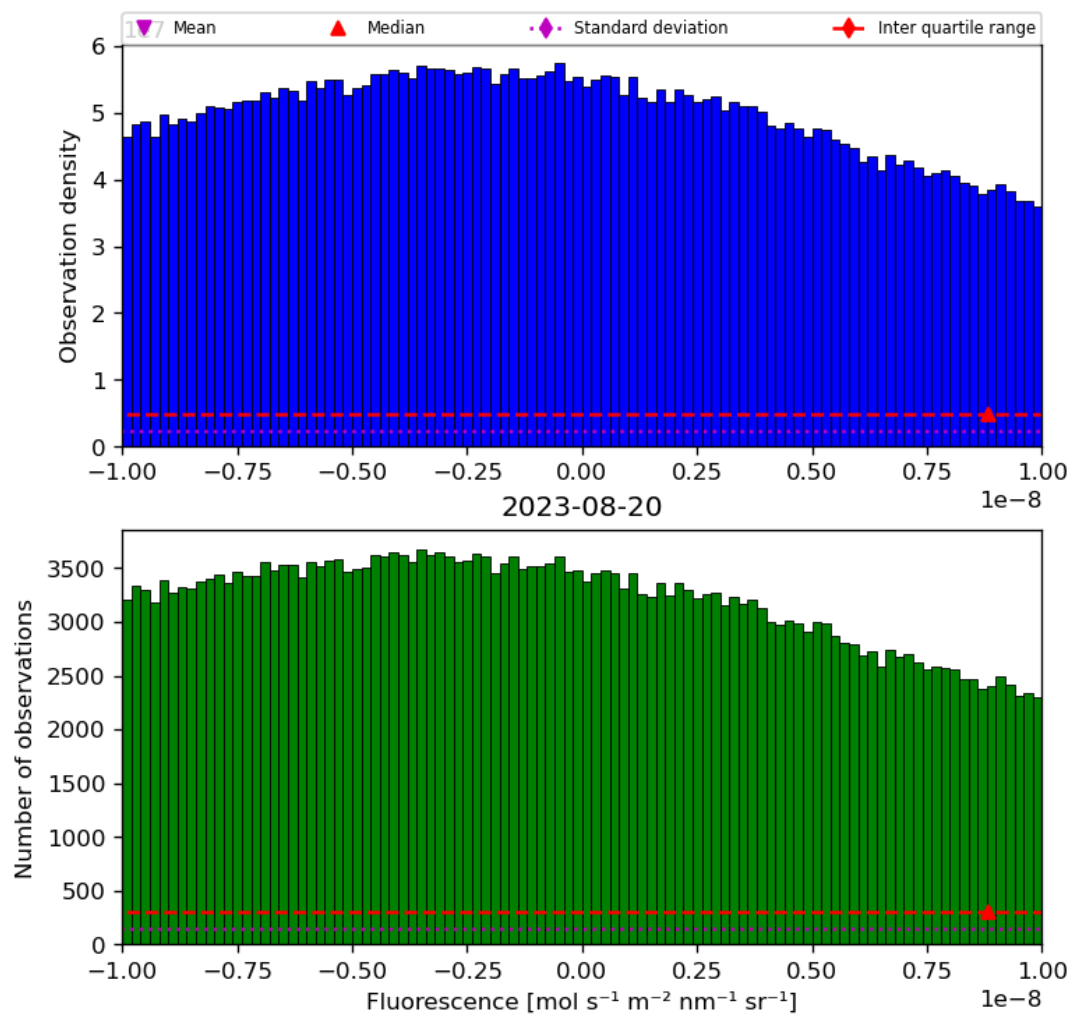
Figure 32: Histogram of “Fluorescence” for 2023-08-20 to 2023-08-21
