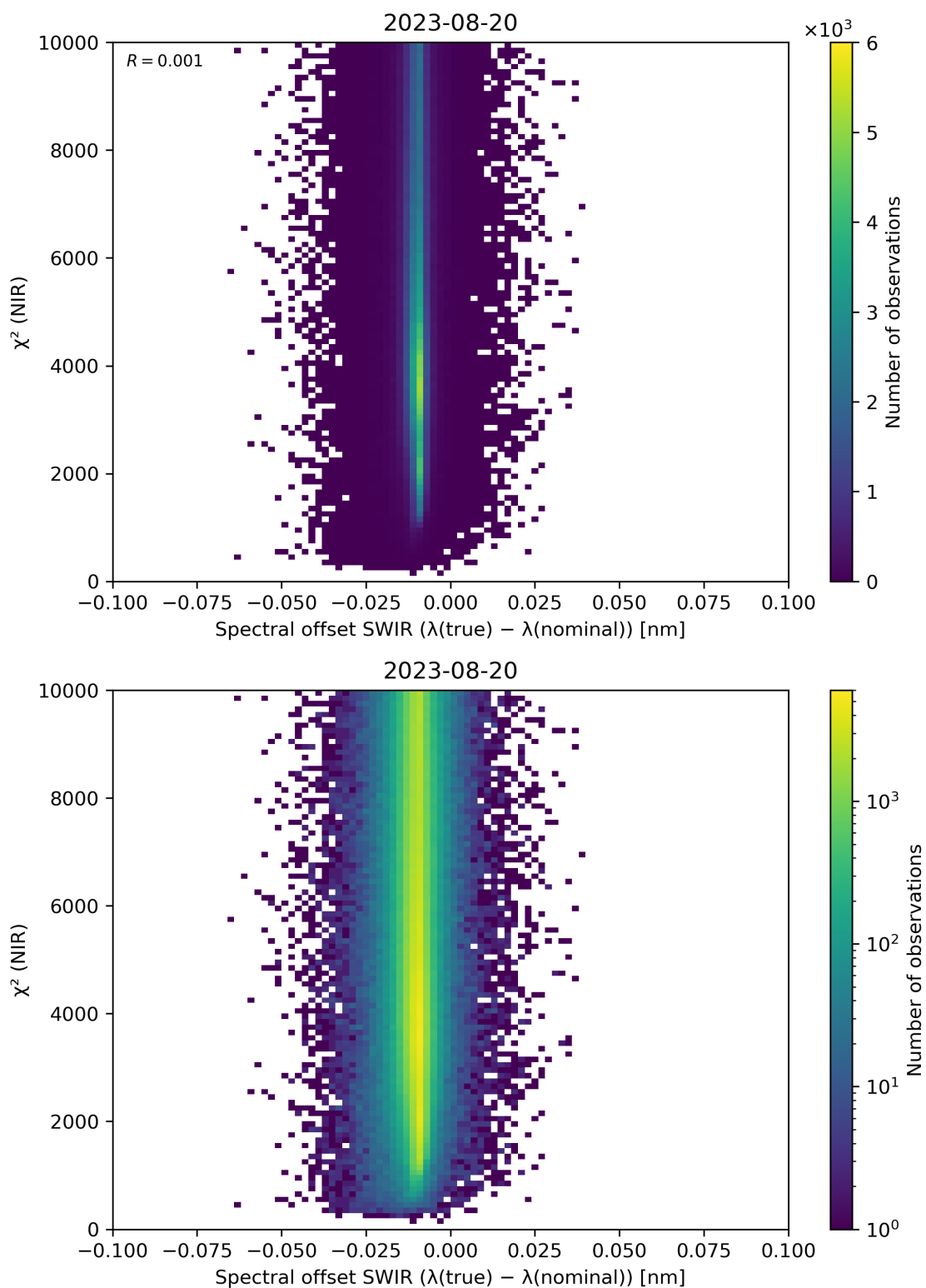
Figure 117: Scatter density plot of “Spectral offset SWIR ( \lambda(\text{true}) - \lambda(\text{nominal}) )” against “ \chi^2 (NIR)” for 2023-08-20 to 2023-08-21.
