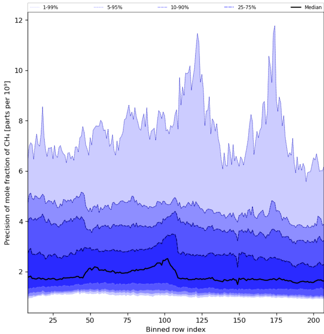
Figure 35: Along track statistics of “Precision of mole fraction of CH 4 ” for 2023-08-20 to 2023-08-21
