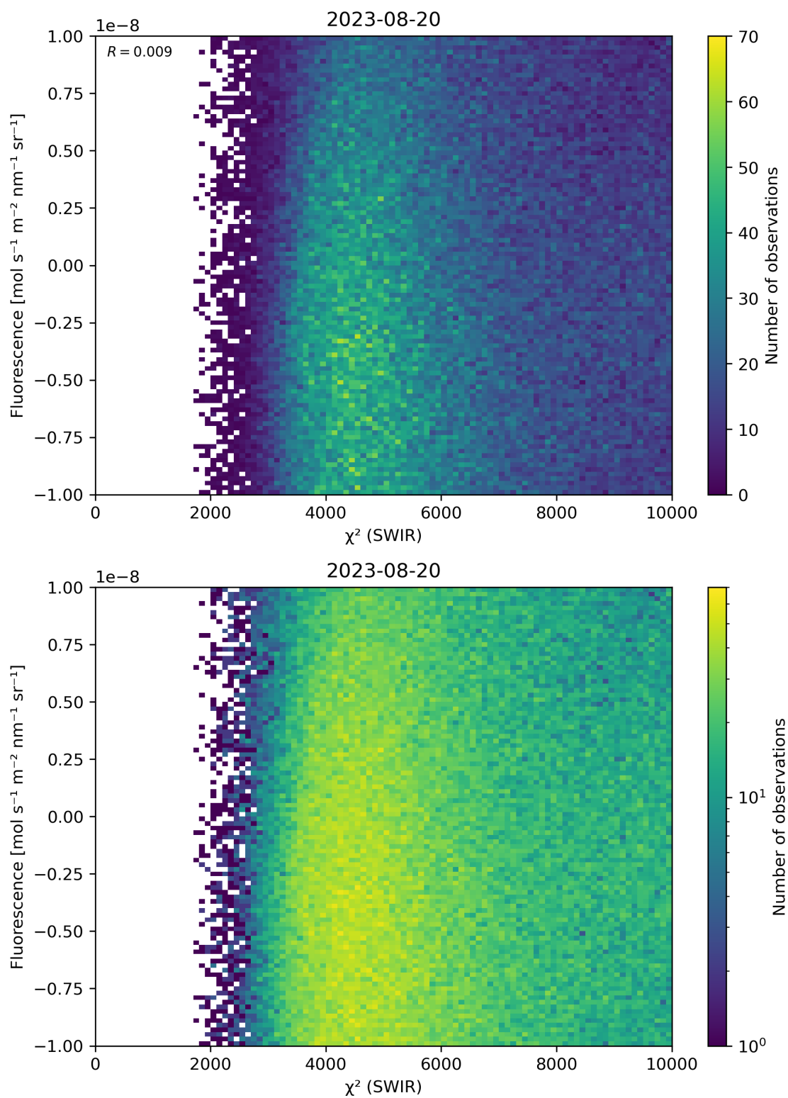
Figure 49: Scatter density plot of “ \chi^2 (SWIR)” against “Fluorescence” for 2023-08-20 to 2023-08-21.
