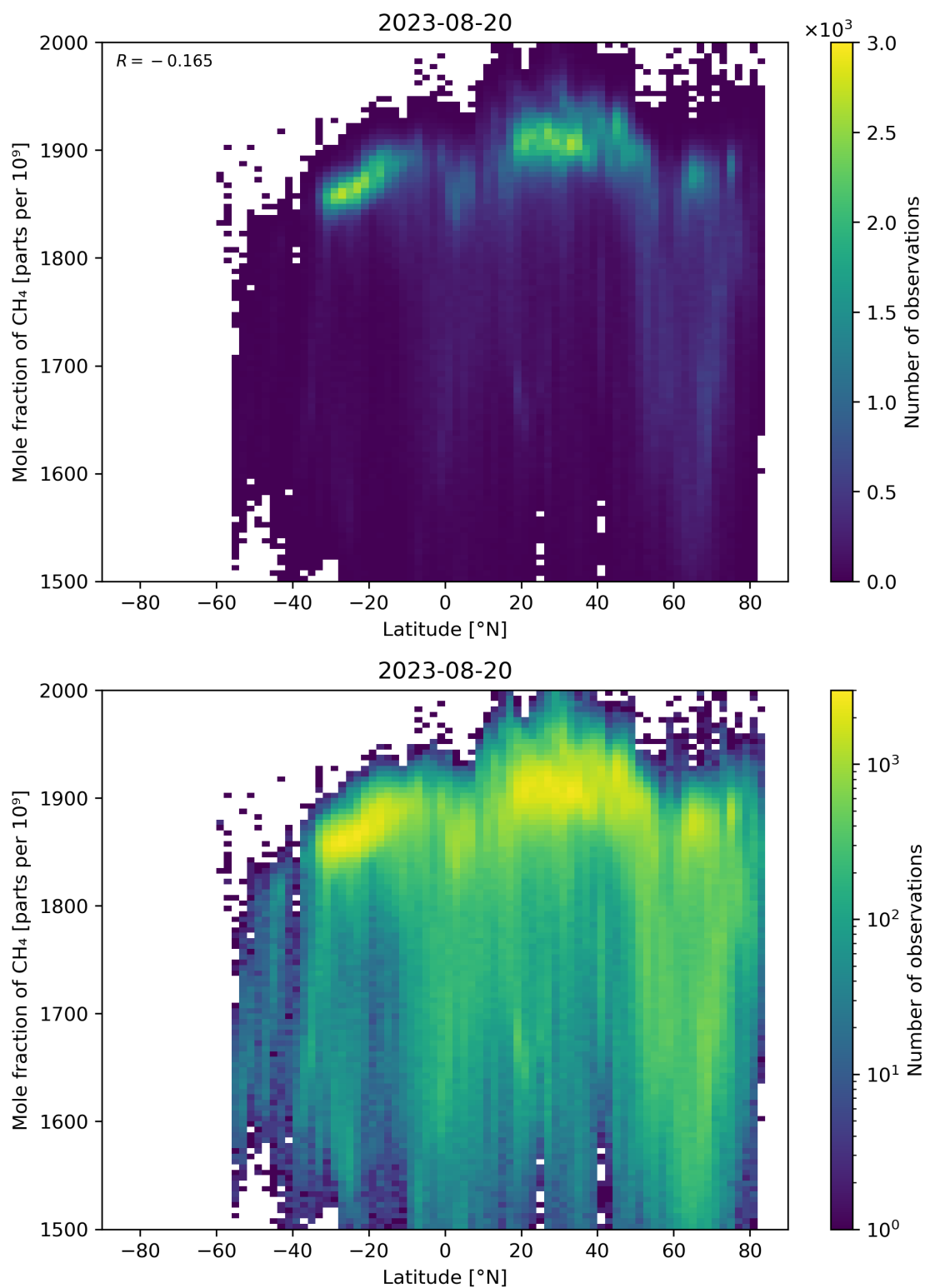
Figure 57: Scatter density plot of “Latitude” against “Mole fraction of CH 4 ” for 2023-08-20 to 2023-08-21.
