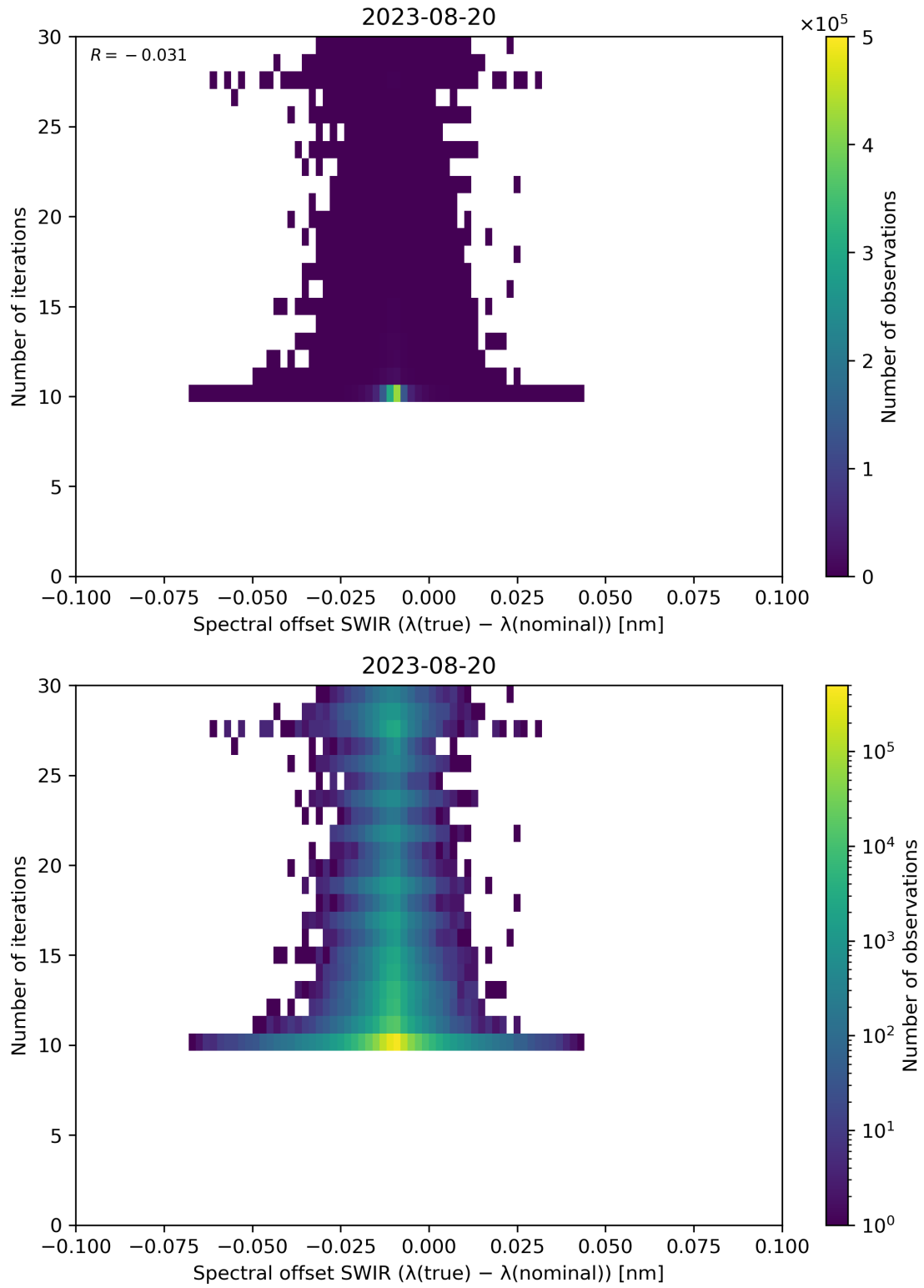
Figure 121: Scatter density plot of “Spectral offset SWIR ( \lambda(\text{true}) - \lambda(\text{nominal}) )” against “Number of iterations” for 2023-08-20 to 2023-08-21.
