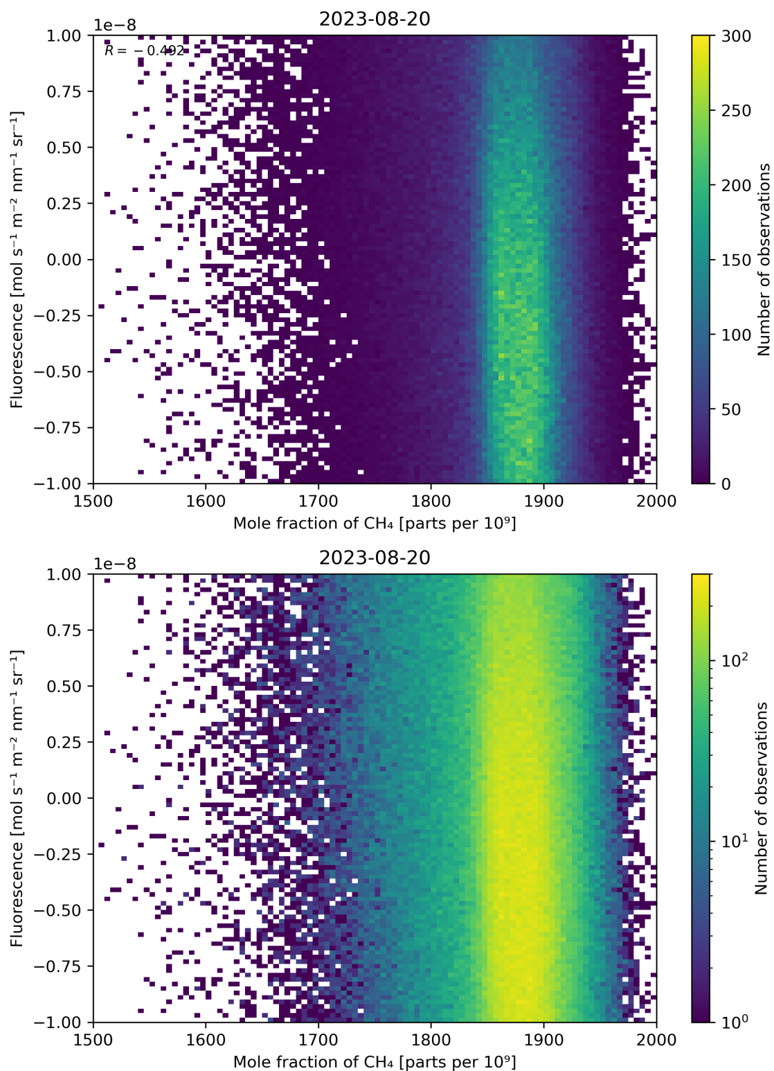
Figure 73: Scatter density plot of “Mole fraction of \text{CH}_4 ” against “Fluorescence” for 2023-08-20 to 2023-08-21.
