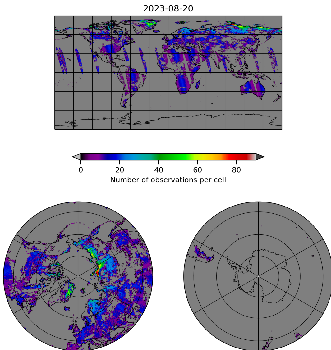
Figure 10: Map of the number of observations for 2023-08-20 to 2023-08-21
