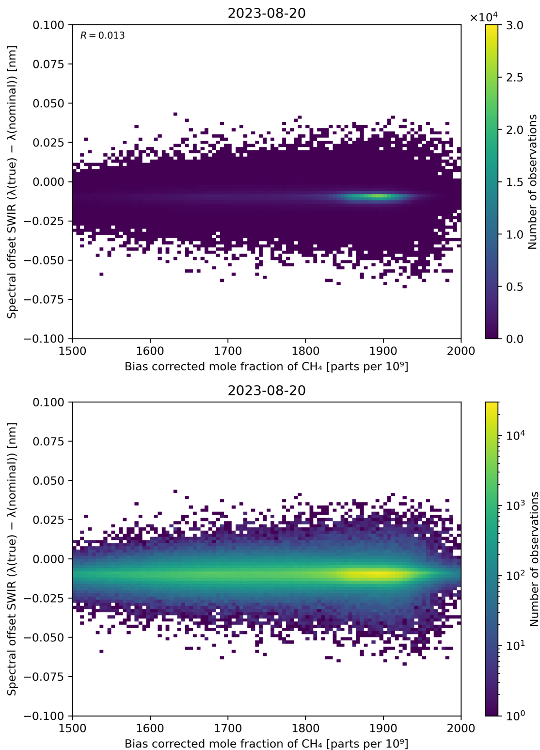
Figure 69: Scatter density plot of “Bias corrected mole fraction of \text{CH}_4 ” against “Spectral offset SWIR ( \lambda(\text{true}) - \lambda(\text{nominal}) )” for 2023-08-20 to 2023-08-21.
