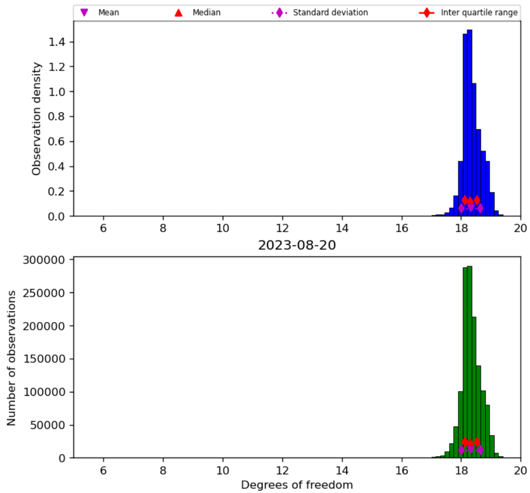
Figure 30: Histogram of “Degrees of freedom” for 2023-08-20 to 2023-08-21
