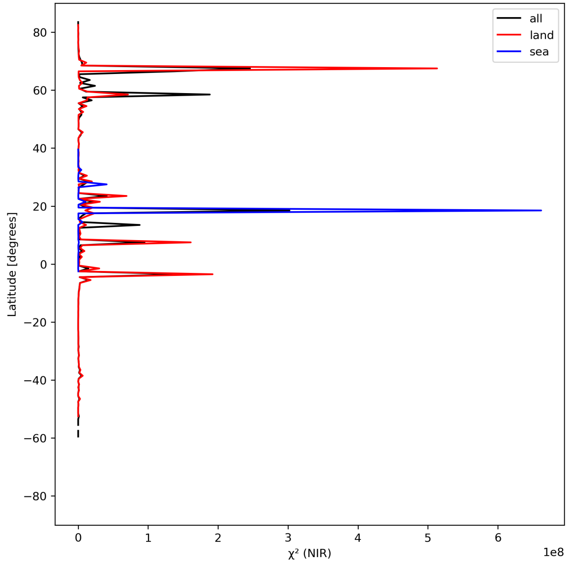
Figure 18: Zonal average of “ \chi^2 (NIR)” for 2023-08-20 to 2023-08-22.
