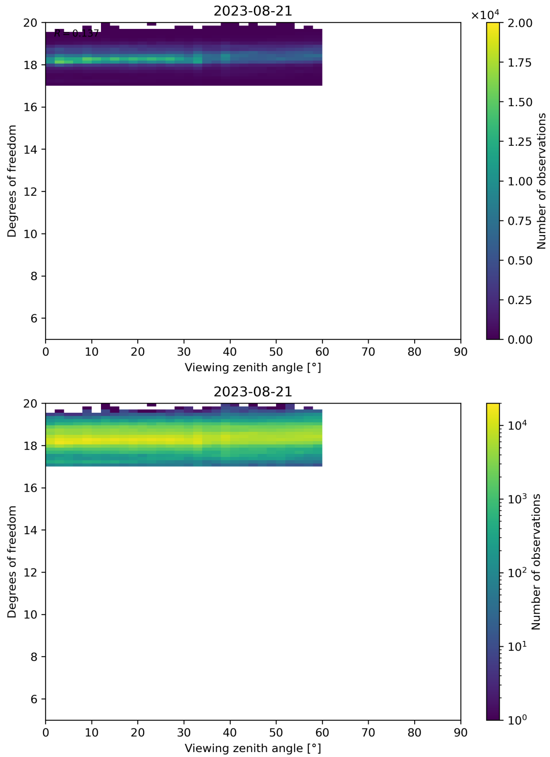
Figure 107: Scatter density plot of “Viewing zenith angle” against “Degrees of freedom” for 2023-08-20 to 2023-08-22.
