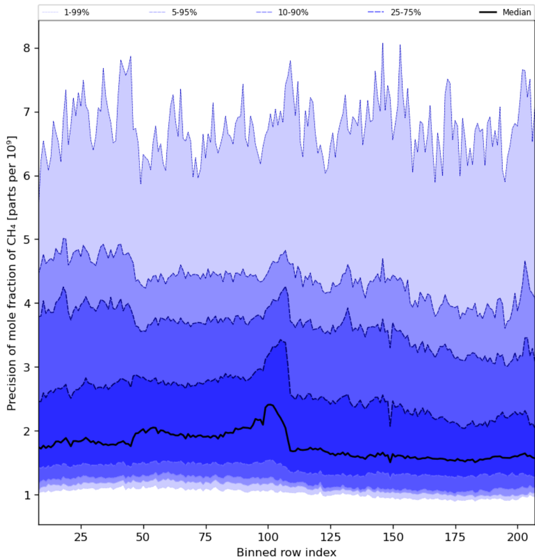
Figure 35: Along track statistics of “Precision of mole fraction of CH 4 ” for 2023-08-20 to 2023-08-22
