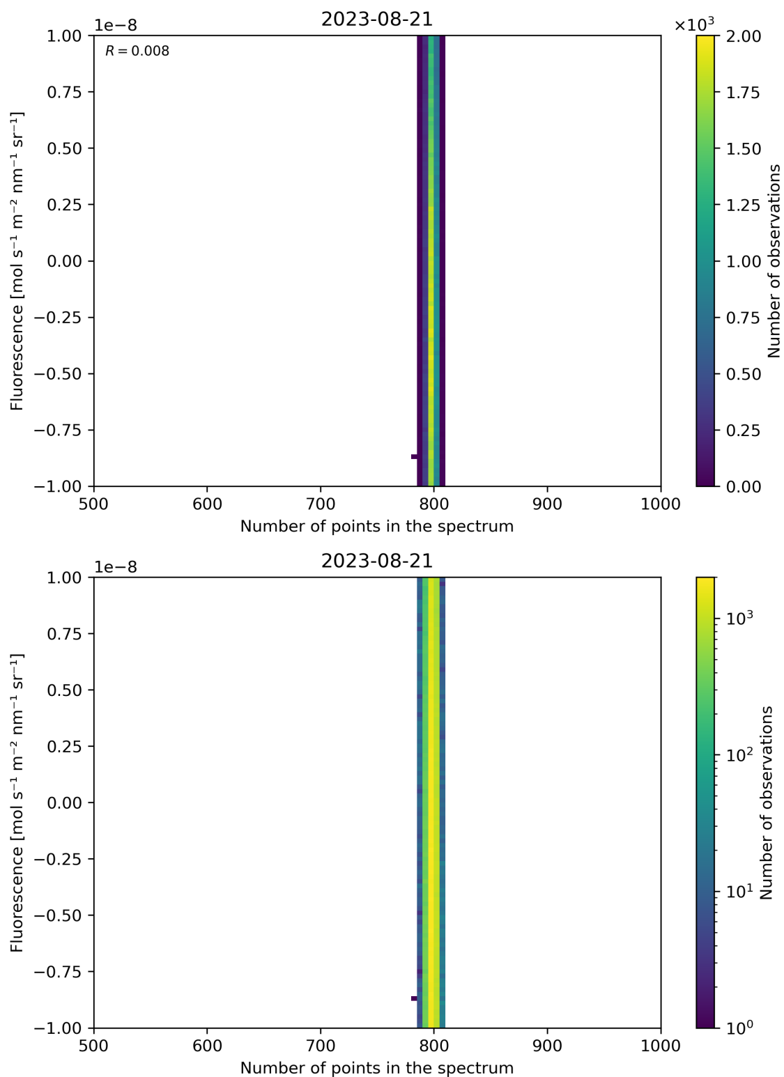
Figure 91: Scatter density plot of “Number of points in the spectrum” against “Fluorescence” for 2023-08-20 to 2023-08-22.
