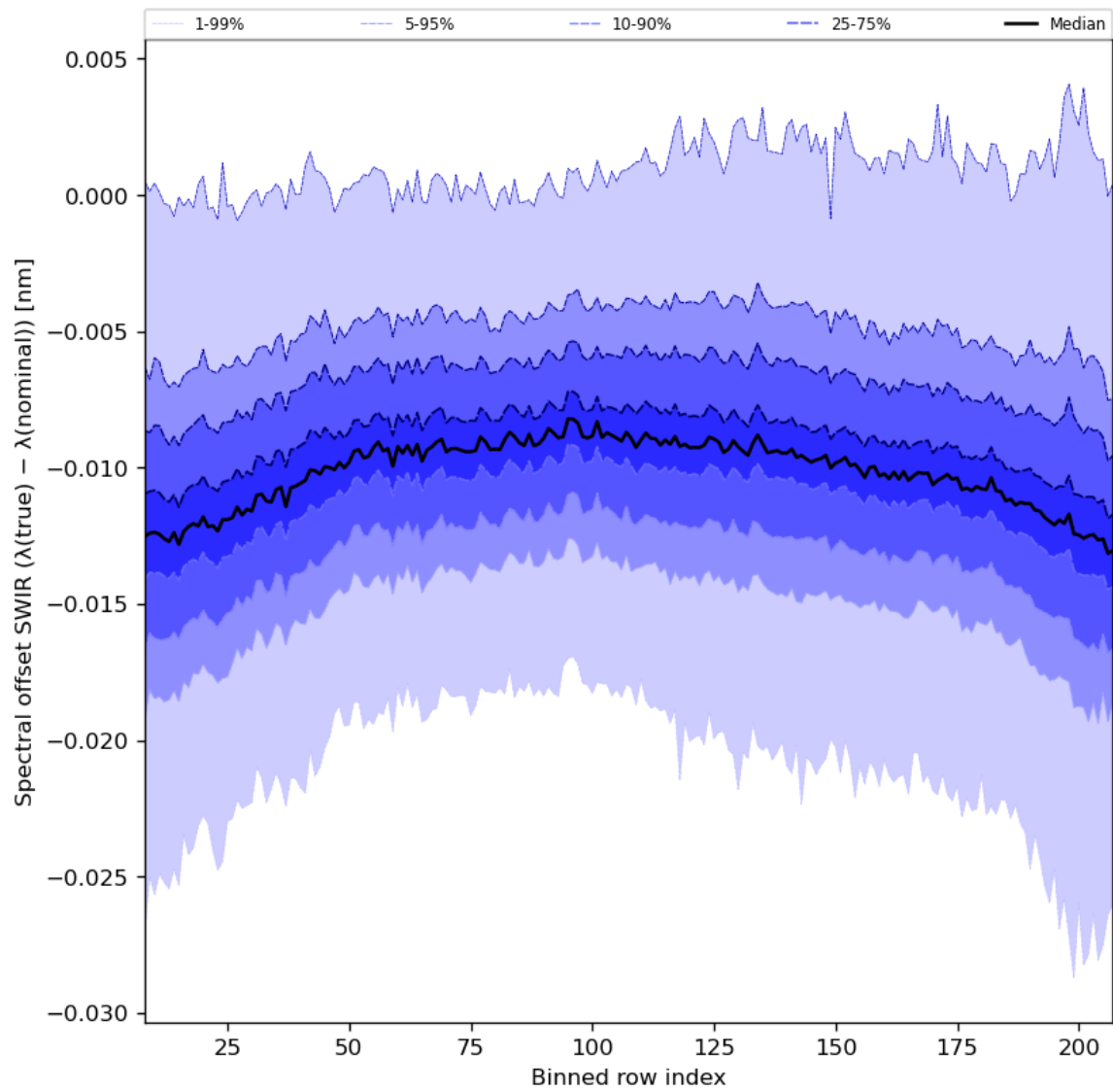
Figure 38: Along track statistics of “Spectral offset SWIR ( \lambda(\text{true}) - \lambda(\text{nominal}) )” for 2023-08-20 to 2023-08-22
