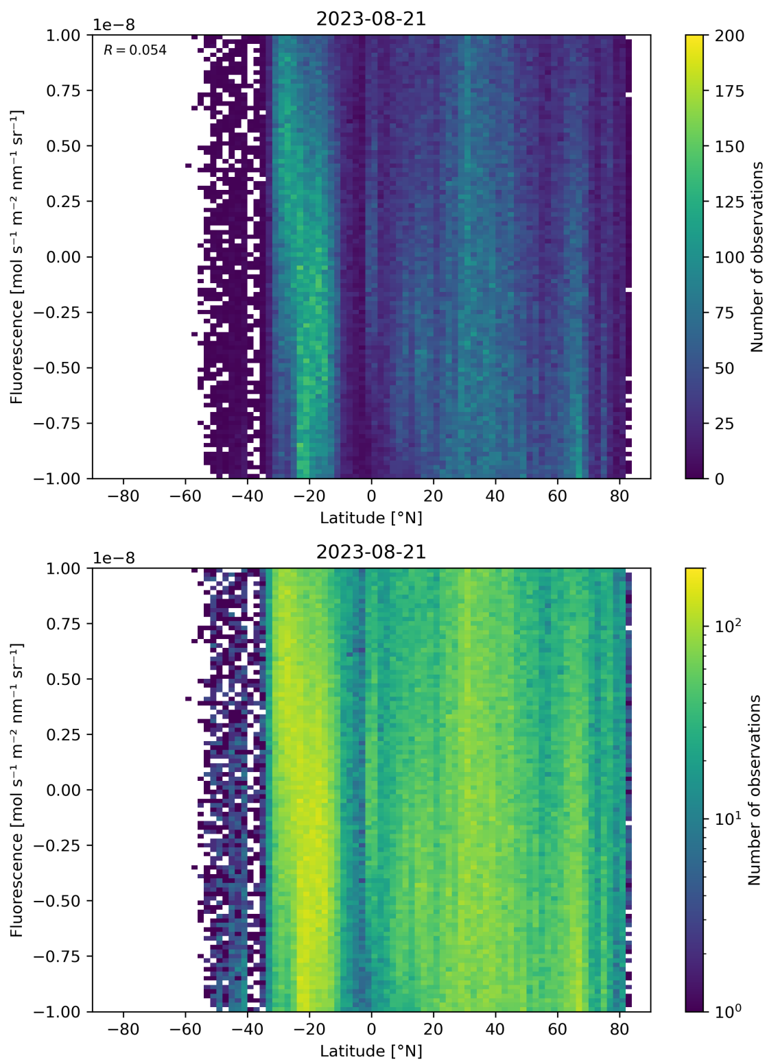
Figure 56: Scatter density plot of “Latitude” against “Fluorescence” for 2023-08-20 to 2023-08-22.
