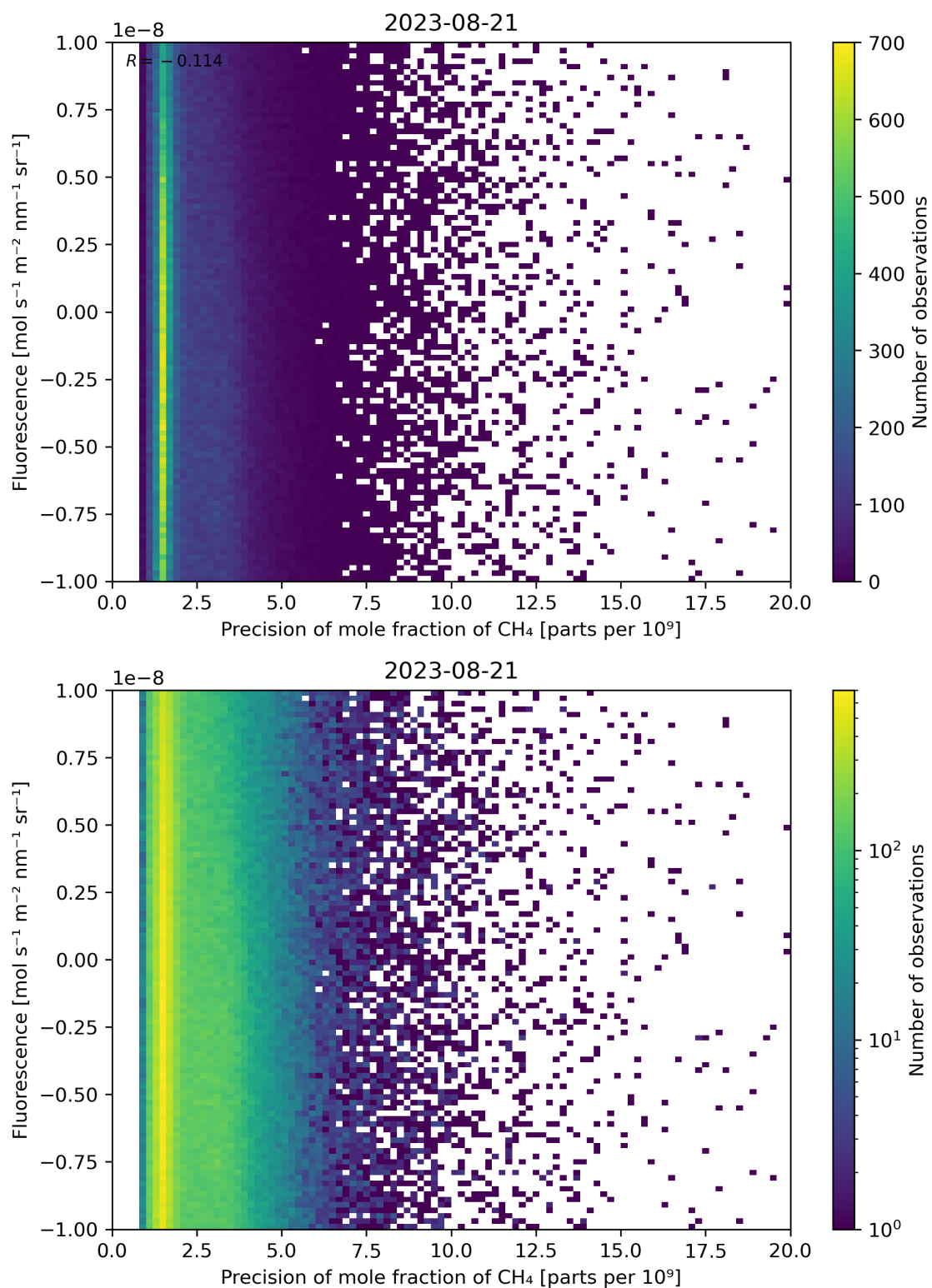
Figure 81: Scatter density plot of “Precision of mole fraction of \text{CH}_4 ” against “Fluorescence” for 2023-08-20 to 2023-08-22.
