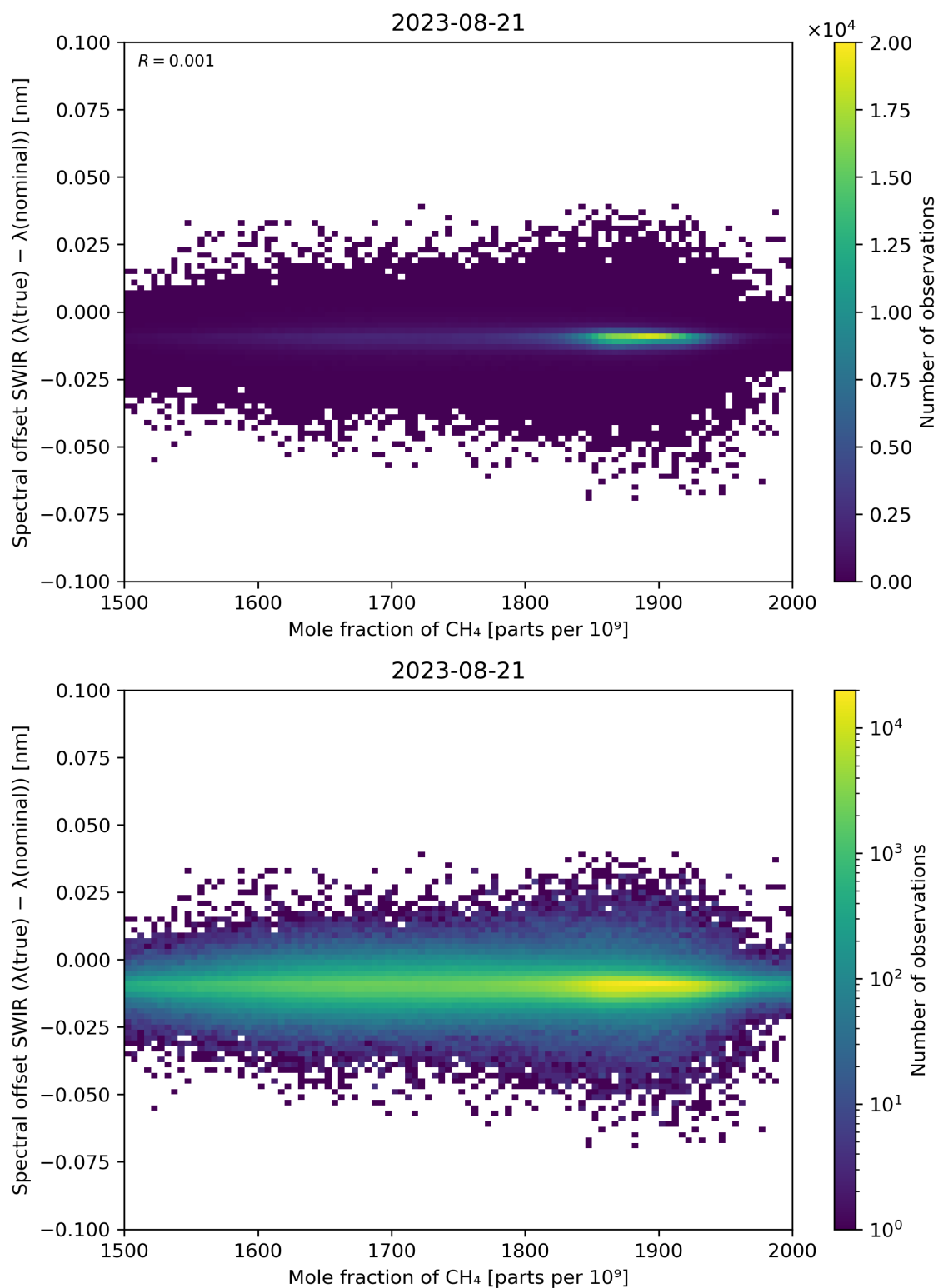
Figure 86: Scatter density plot of “Mole fraction of CH 4 ” against “Spectral offset SWIR ( \lambda(\text{true}) - \lambda(\text{nominal}) )” for 2023-08-20 to 2023-08-22.
