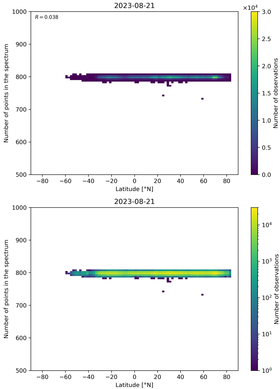
Figure 61: Scatter density plot of “Latitude” against “Number of points in the spectrum” for 2023-08-20 to 2023-08-22.
