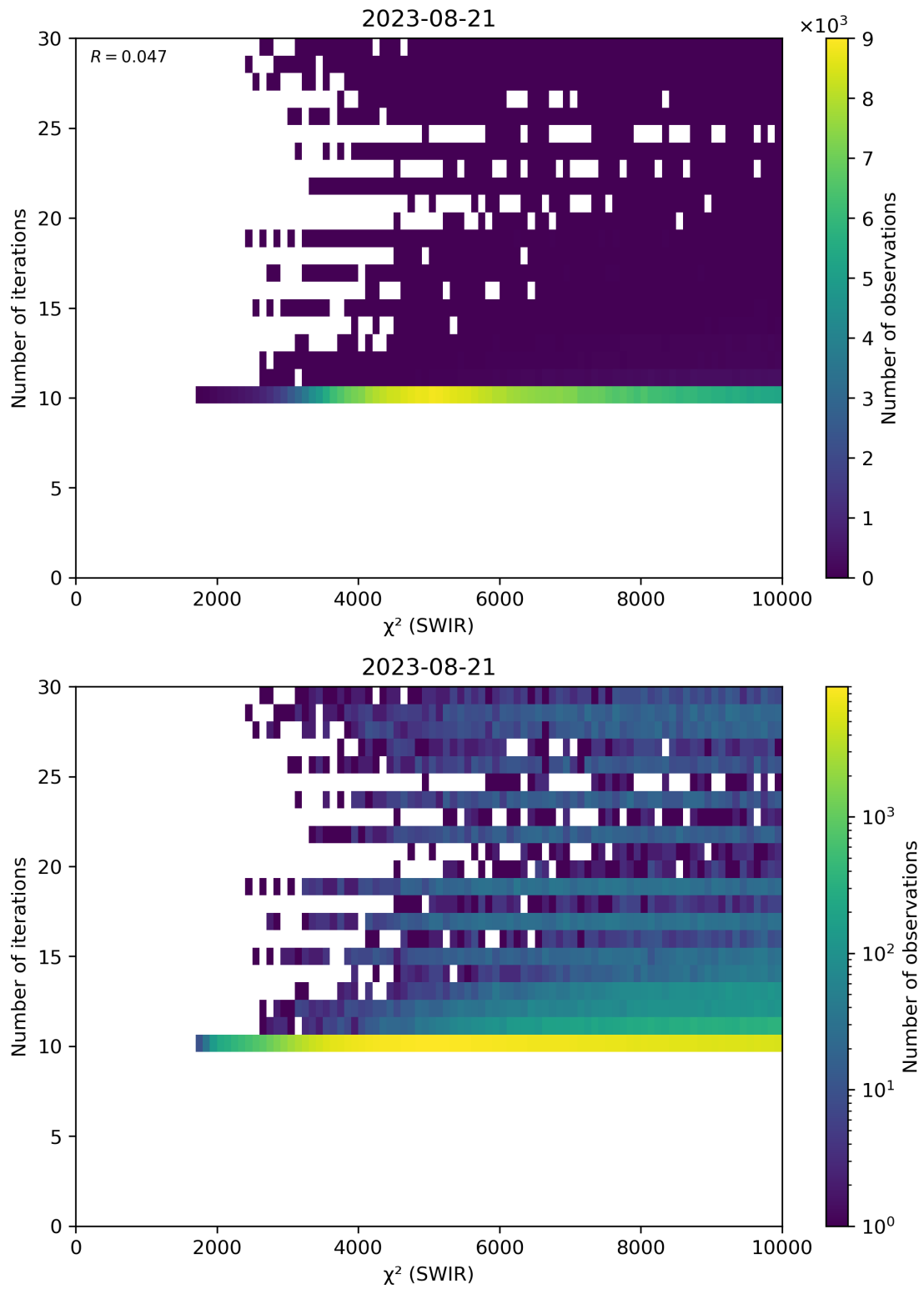
Figure 50: Scatter density plot of “ \chi^2 (SWIR)” against “Number of iterations” for 2023-08-20 to 2023-08-22.
