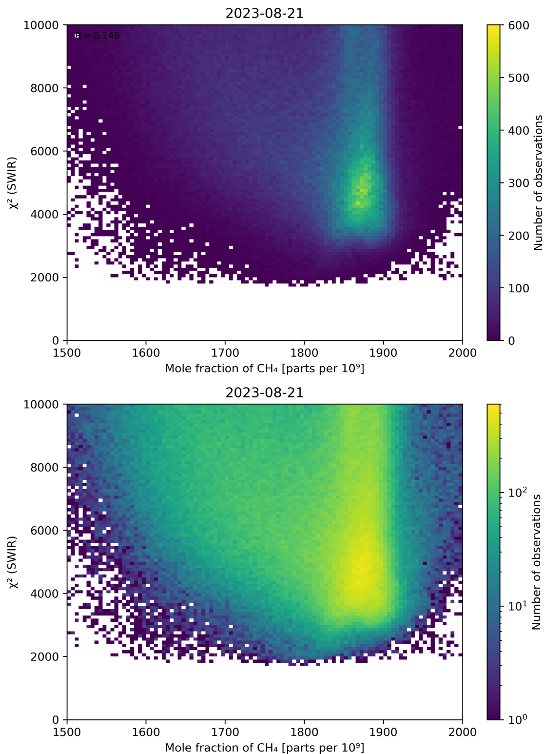
Figure 71: Scatter density plot of “Mole fraction of CH 4 ” against “ \chi^2 (SWIR)” for 2023-08-20 to 2023-08-22.
