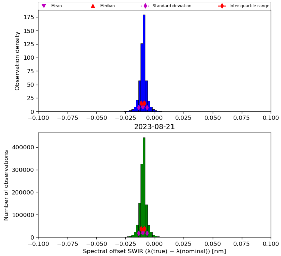
Figure 27: Histogram of “Spectral offset SWIR ( \lambda(\text{true}) - \lambda(\text{nominal}) )” for 2023-08-20 to 2023-08-22
