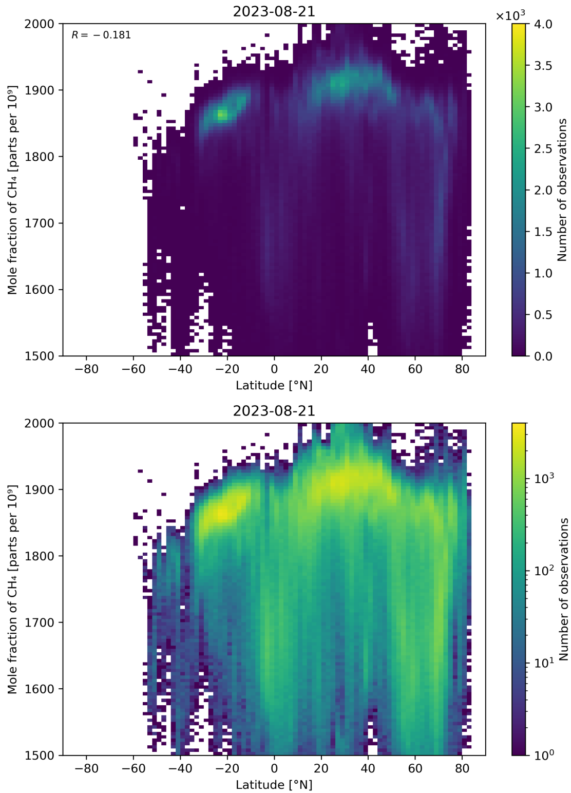
Figure 57: Scatter density plot of “Latitude” against “Mole fraction of CH 4 ” for 2023-08-20 to 2023-08-22.
