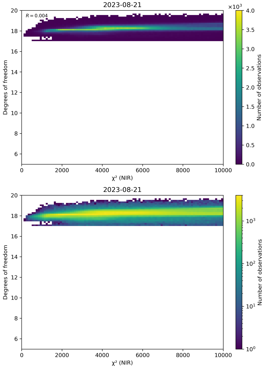
Figure 44: Scatter density plot of “ \chi^2 (NIR)” against “Degrees of freedom” for 2023-08-20 to 2023-08-22.
