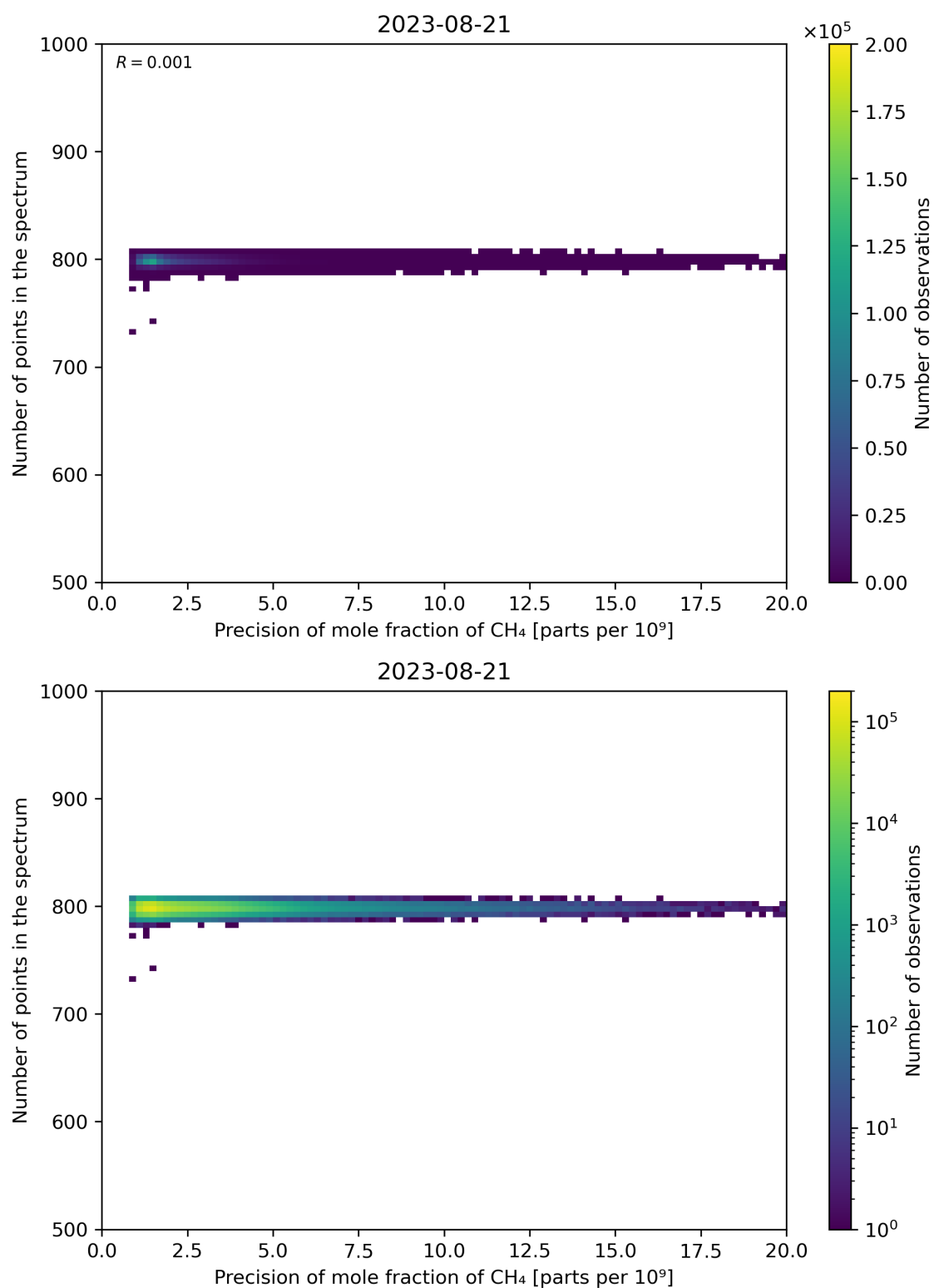
Figure 84: Scatter density plot of “Precision of mole fraction of \text{CH}_4 ” against “Number of points in the spectrum” for 2023-08-20 to 2023-08-22.
