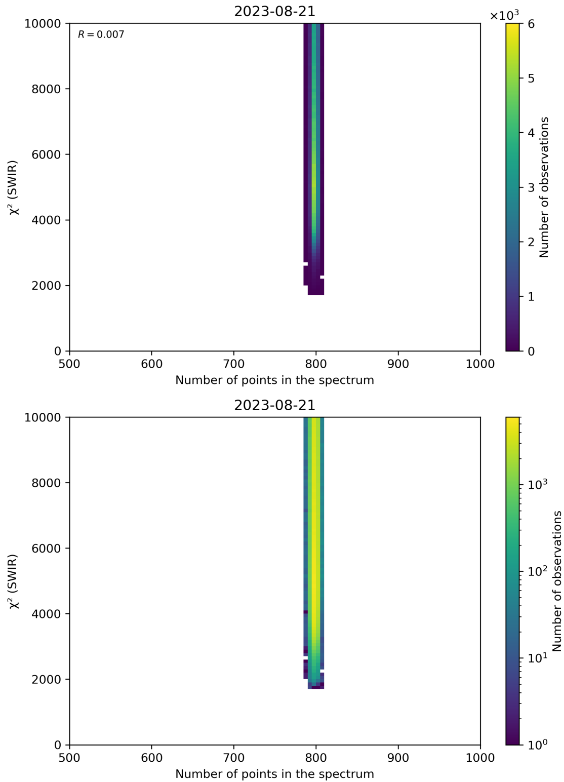
Figure 89: Scatter density plot of “Number of points in the spectrum” against “ \chi^2 (SWIR)” for 2023-08-20 to 2023-08-22.
