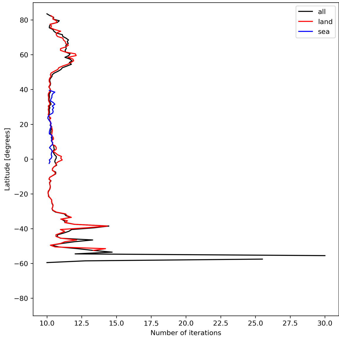
Figure 20: Zonal average of “Number of iterations” for 2023-08-20 to 2023-08-22.
