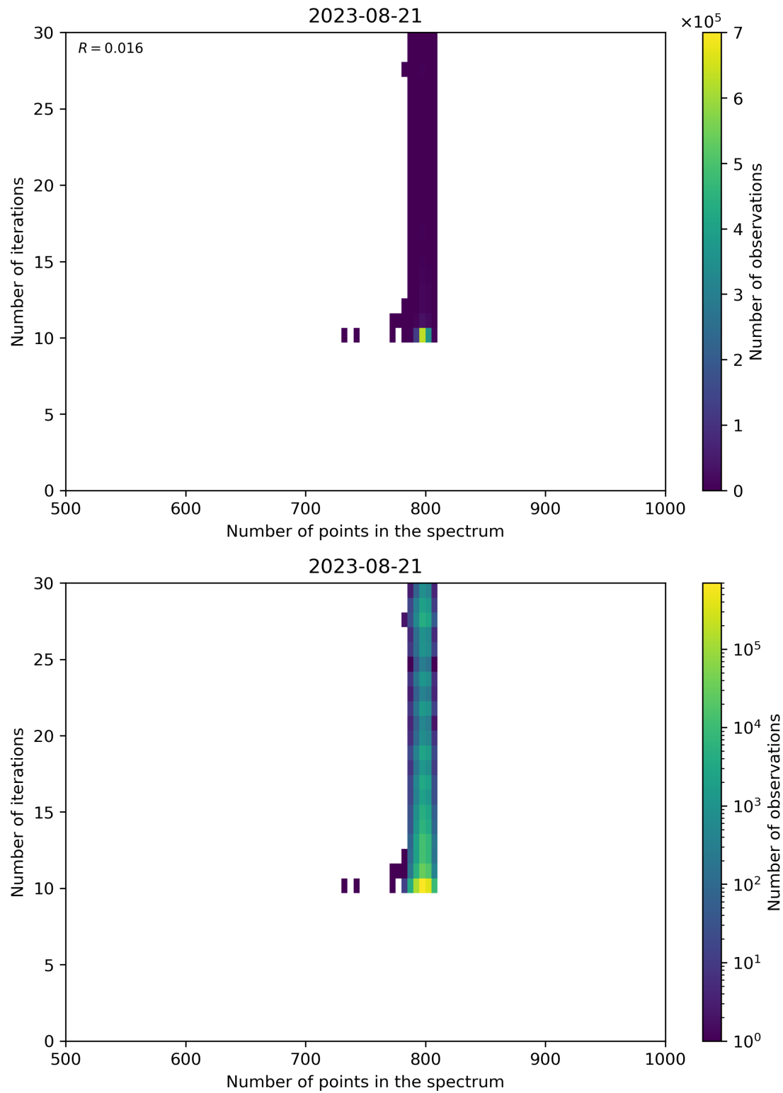
Figure 92: Scatter density plot of “Number of points in the spectrum” against “Number of iterations” for 2023-08-20 to 2023-08-22.
