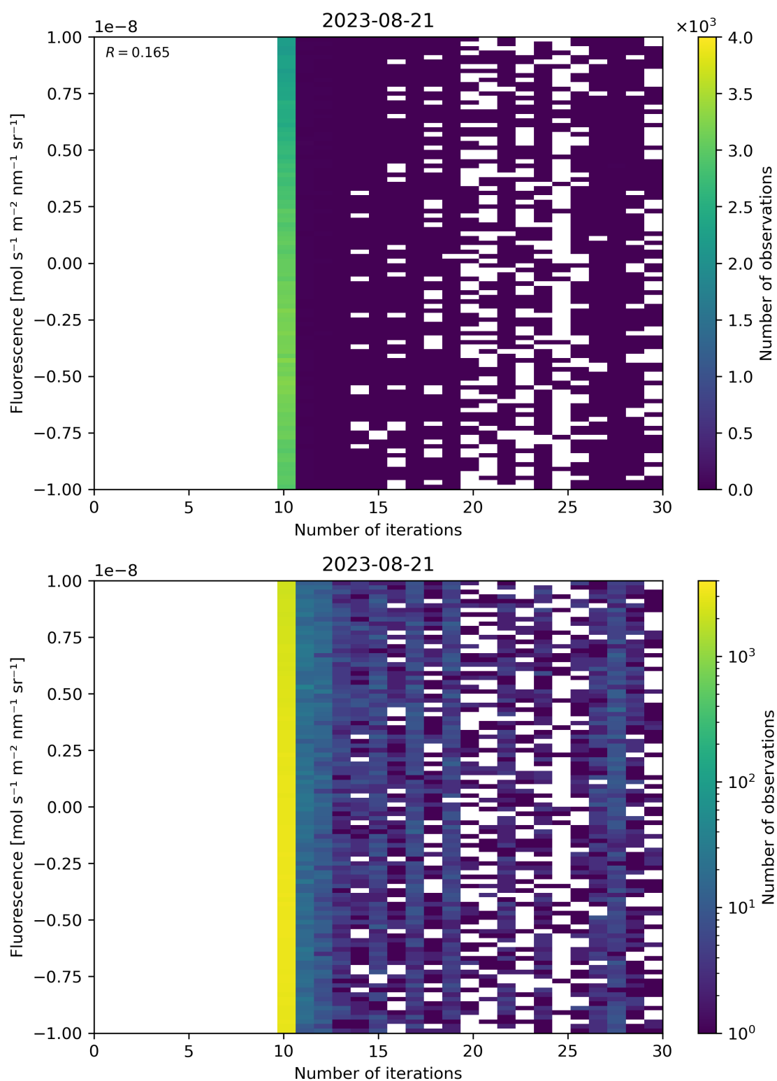
Figure 87: Scatter density plot of “Number of iterations” against “Fluorescence” for 2023-08-20 to 2023-08-22.
