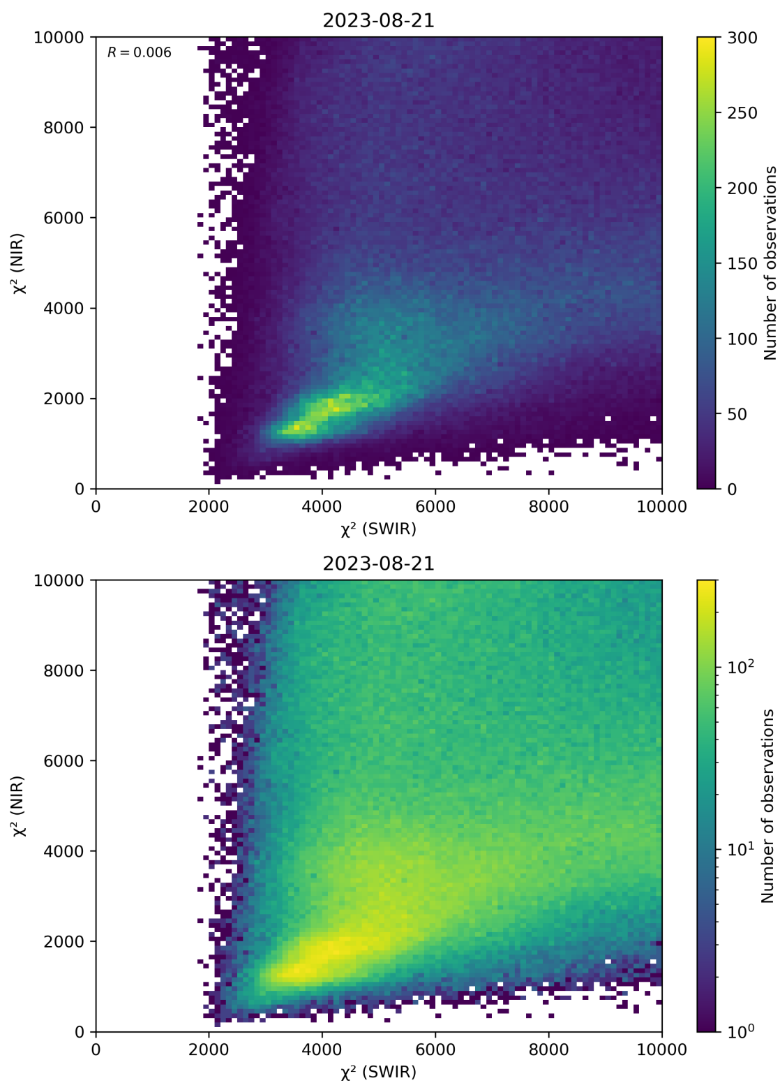
Figure 47: Scatter density plot of “ \chi^2 (SWIR)” against “ \chi^2 (NIR)” for 2023-08-20 to 2023-08-22.
