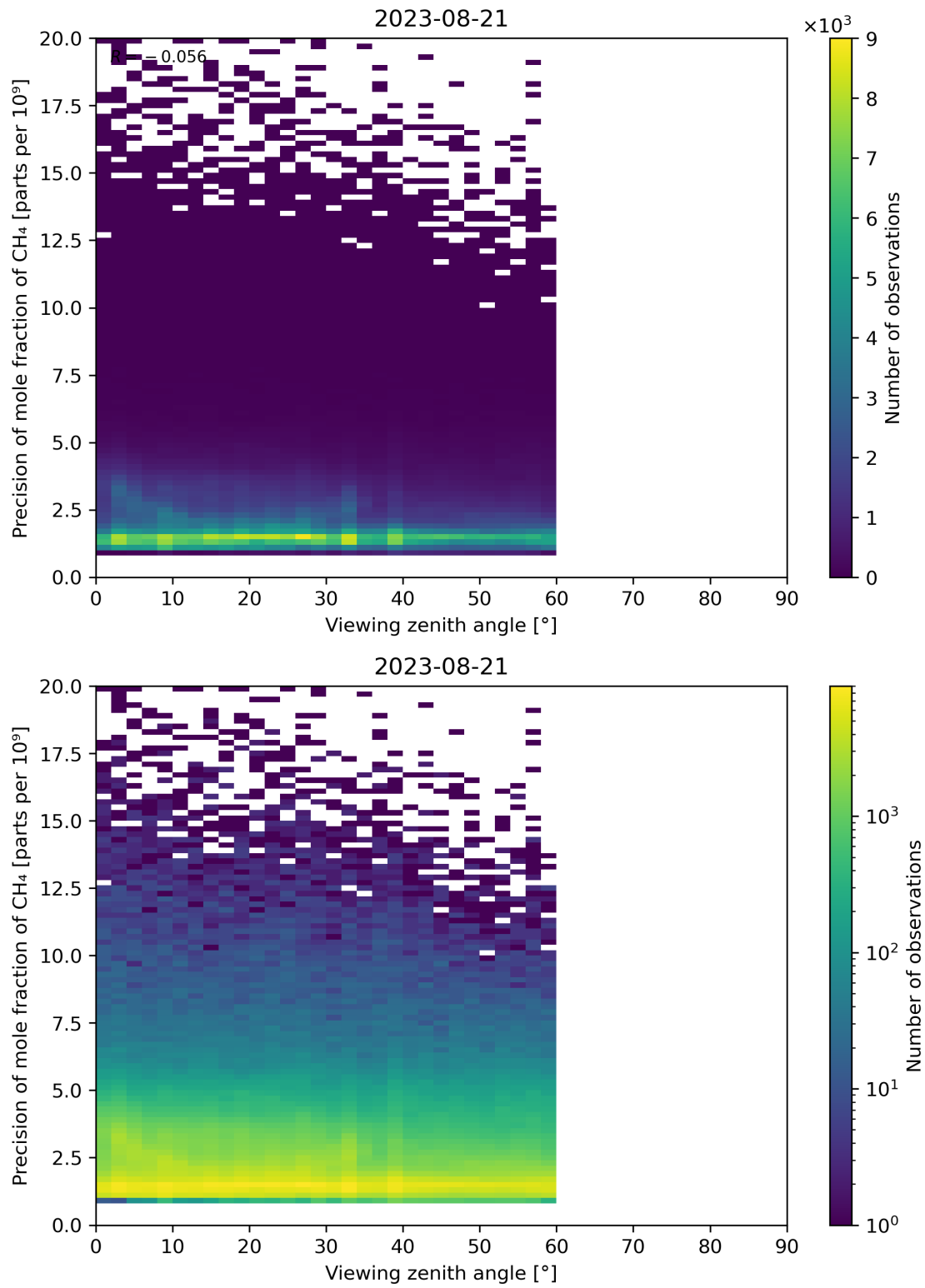
Figure 112: Scatter density plot of “Viewing zenith angle” against “Precision of mole fraction of CH 4 ” for 2023-08-20 to 2023-08-22.
