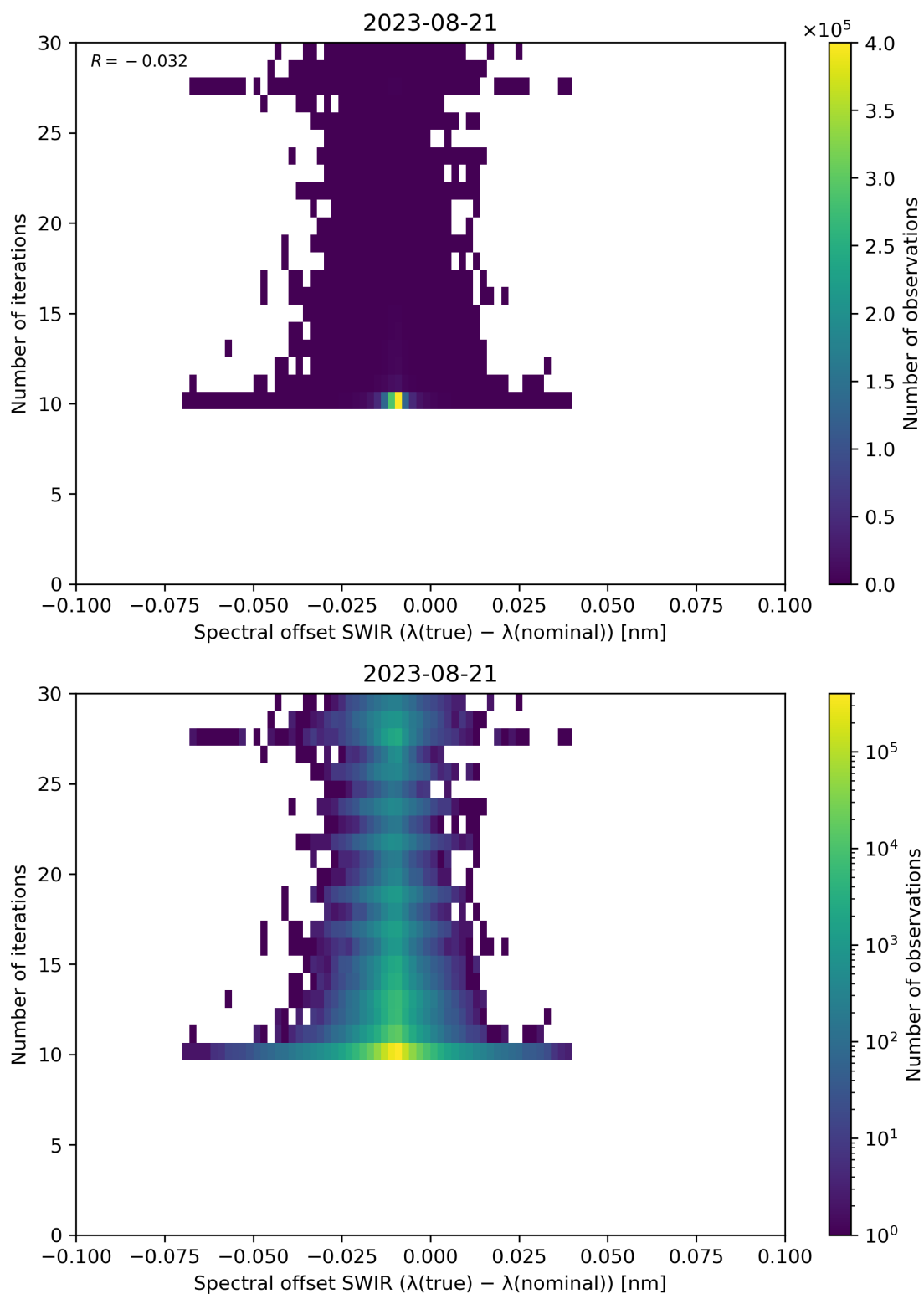
Figure 121: Scatter density plot of “Spectral offset SWIR ( \lambda(\text{true}) - \lambda(\text{nominal}) )” against “Number of iterations” for 2023-08-20 to 2023-08-22.
