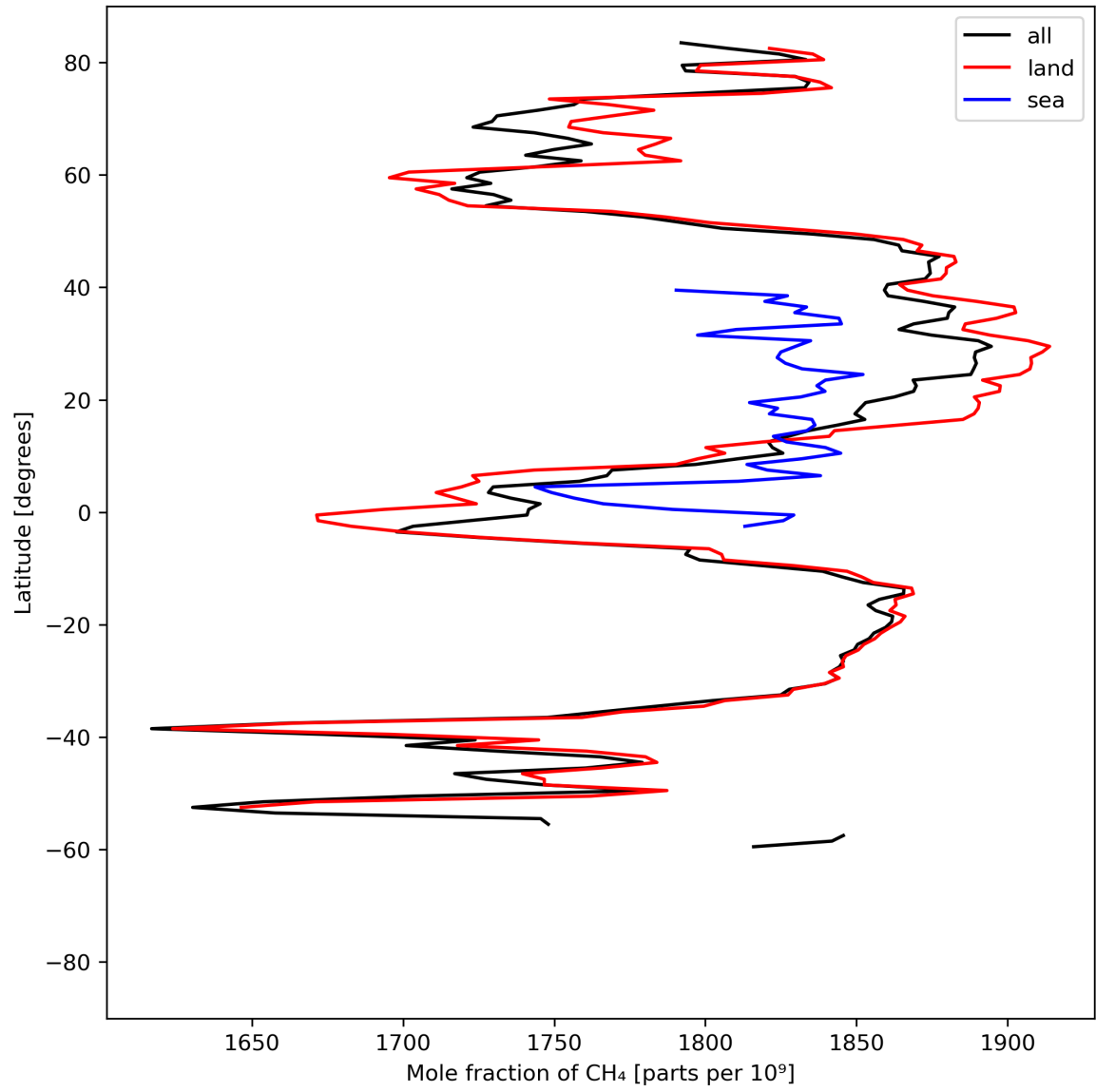
Figure 12: Zonal average of “Mole fraction of \text{CH}_4 ” for 2023-08-20 to 2023-08-22.
