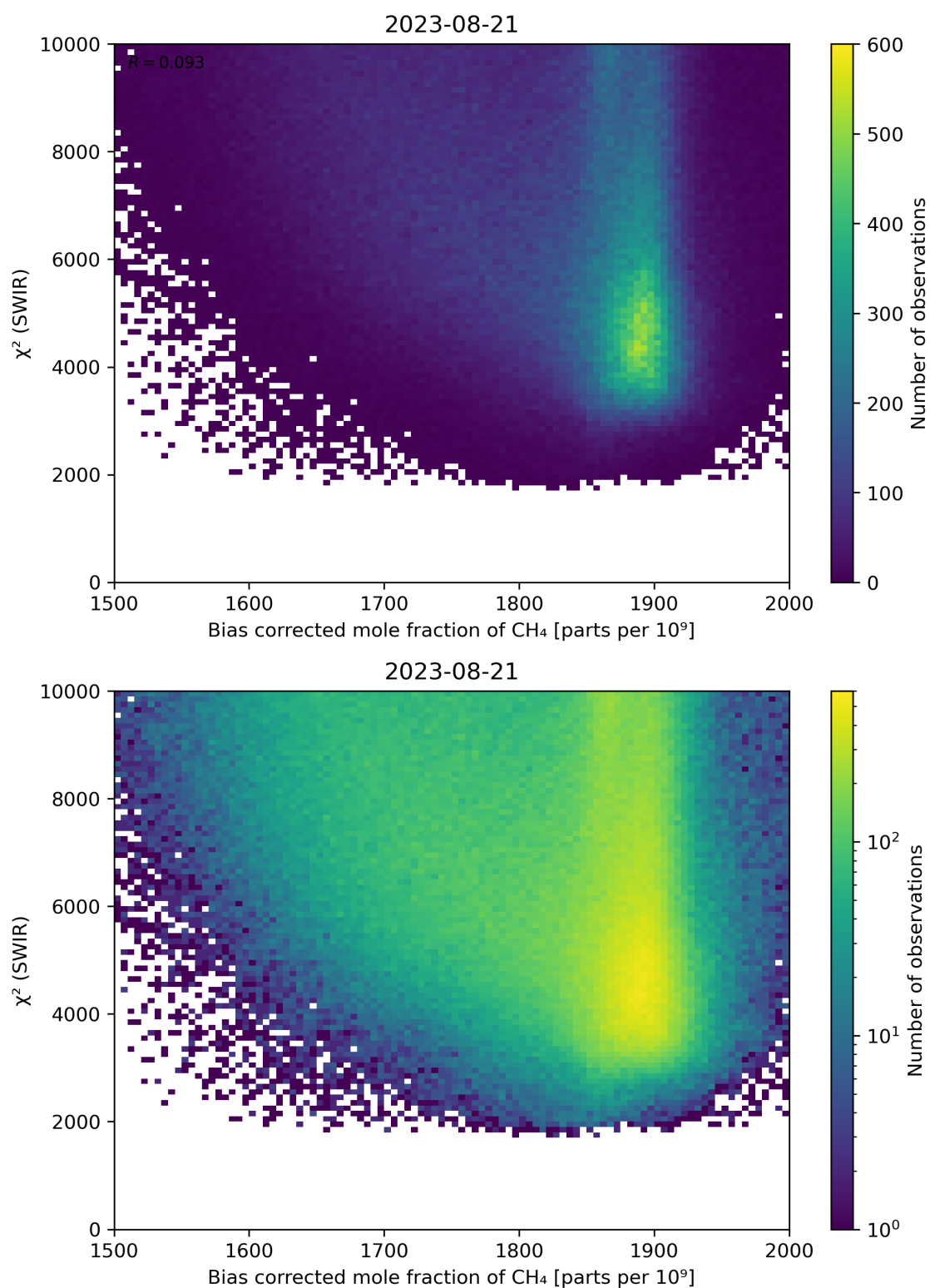
Figure 64: Scatter density plot of “Bias corrected mole fraction of \text{CH}_4 ” against “ \chi^2 (SWIR)” for 2023-08-20 to 2023-08-22.
