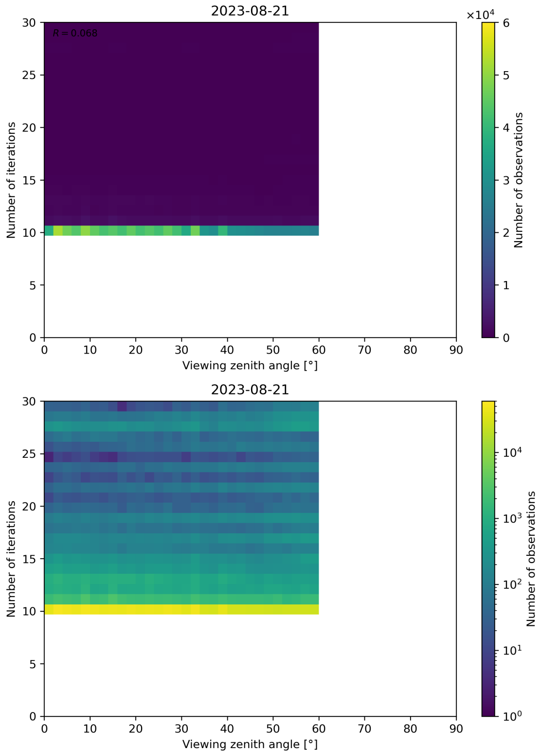
Figure 113: Scatter density plot of “Viewing zenith angle” against “Number of iterations” for 2023-08-20 to 2023-08-22.
