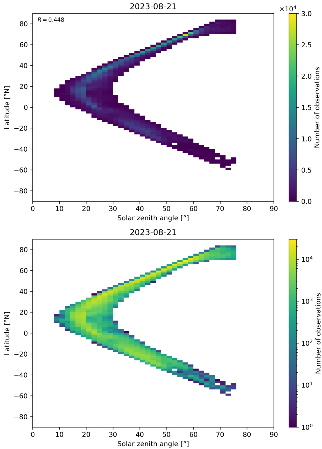
Figure 98: Scatter density plot of “Solar zenith angle” against “Latitude” for 2023-08-20 to 2023-08-22.
