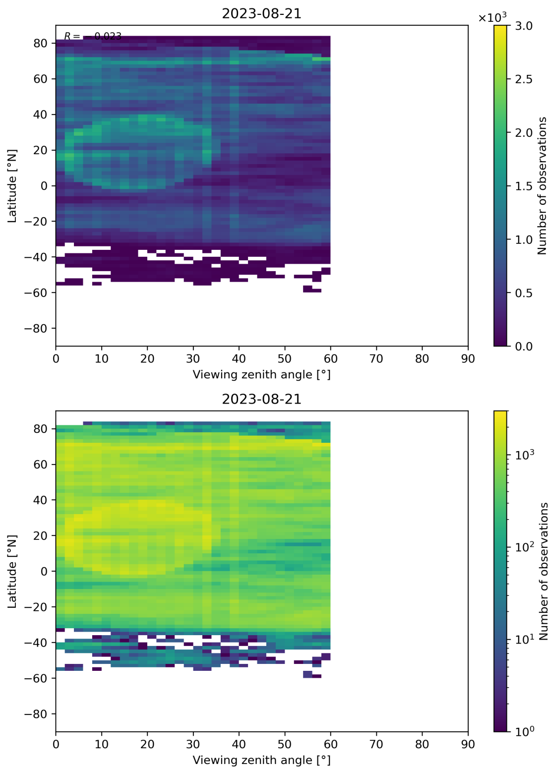
Figure 109: Scatter density plot of “Viewing zenith angle” against “Latitude” for 2023-08-20 to 2023-08-22.
