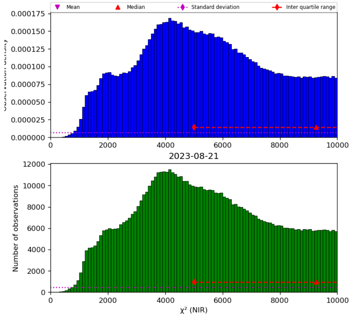
Figure 29: Histogram of “ \chi^2 (NIR)” for 2023-08-20 to 2023-08-22
