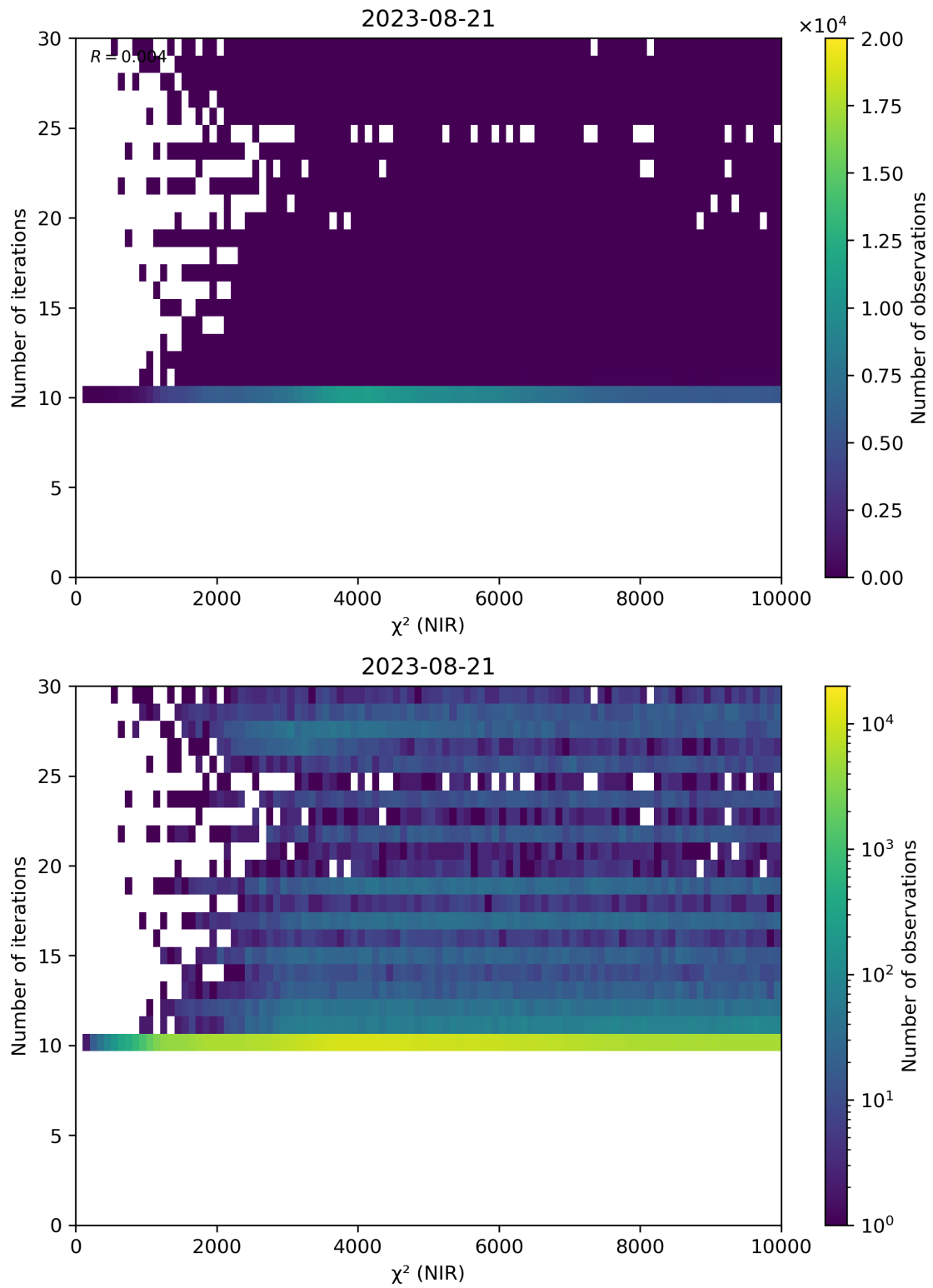
Figure 46: Scatter density plot of “ \chi^2 (NIR)” against “Number of iterations” for 2023-08-20 to 2023-08-22.
