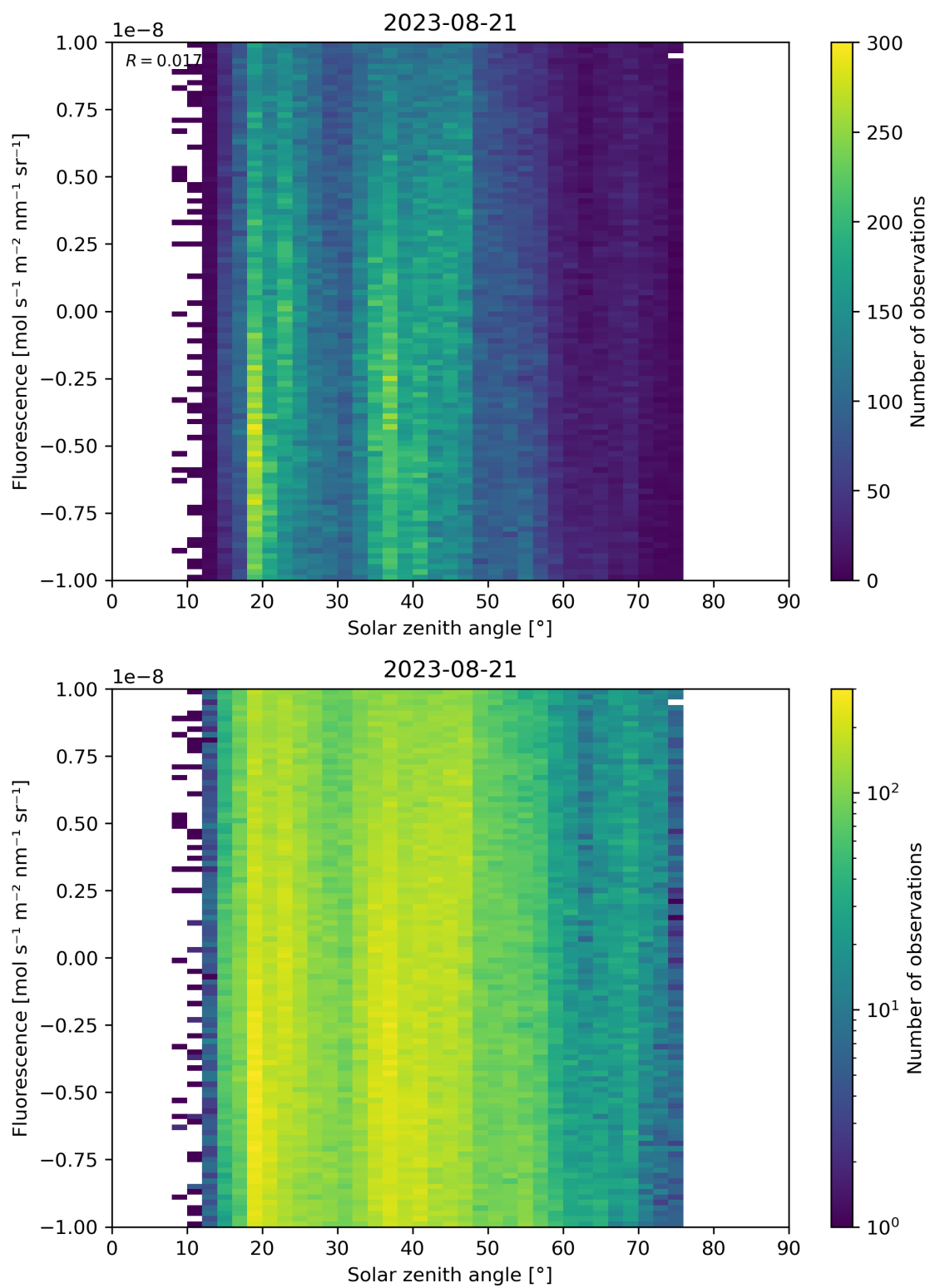
Figure 97: Scatter density plot of “Solar zenith angle” against “Fluorescence” for 2023-08-20 to 2023-08-22.
