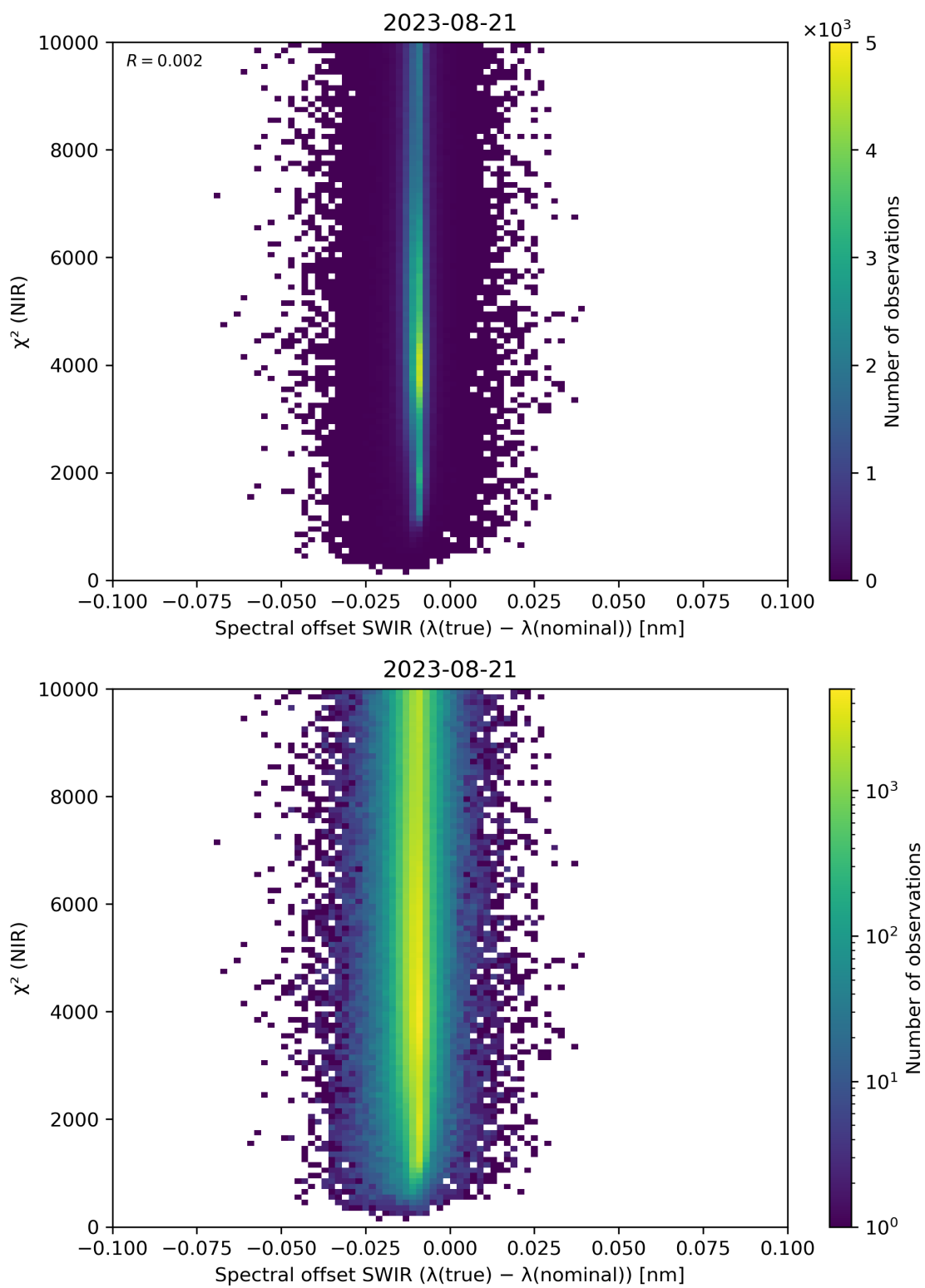
Figure 117: Scatter density plot of “Spectral offset SWIR ( \lambda(\text{true}) - \lambda(\text{nominal}) )” against “ \chi^2 (NIR)” for 2023-08-20 to 2023-08-22.
