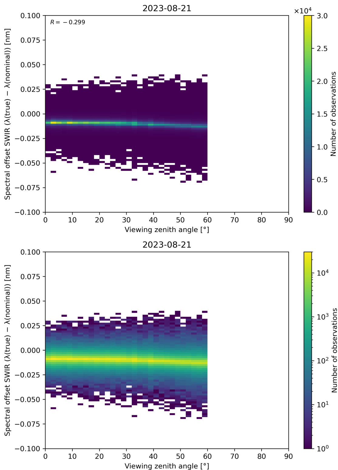
Figure 116: Scatter density plot of “Viewing zenith angle” against “Spectral offset SWIR ( \lambda(\text{true}) - \lambda(\text{nominal}) )” for 2023-08-20 to 2023-08-22.
