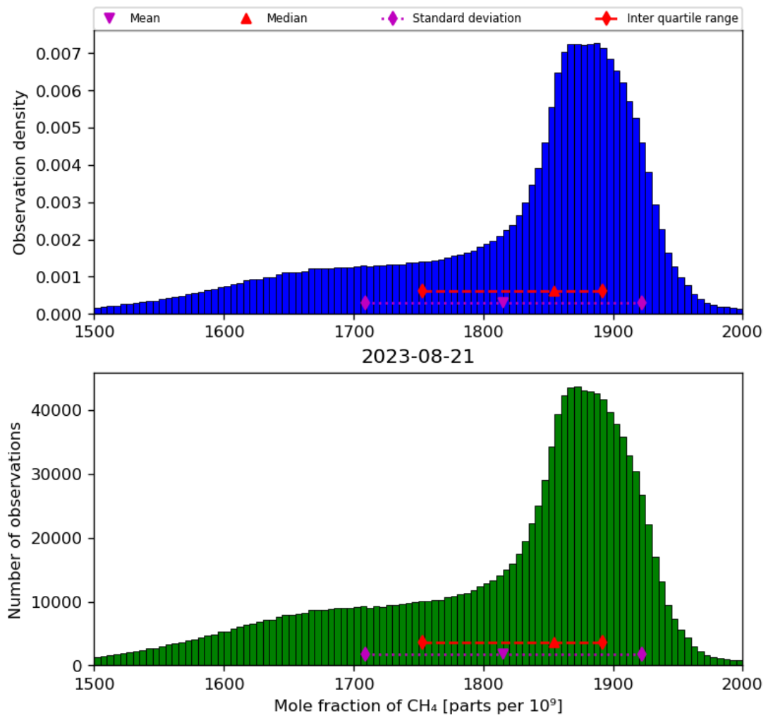
Figure 23: Histogram of “Mole fraction of CH 4 ” for 2023-08-20 to 2023-08-22
