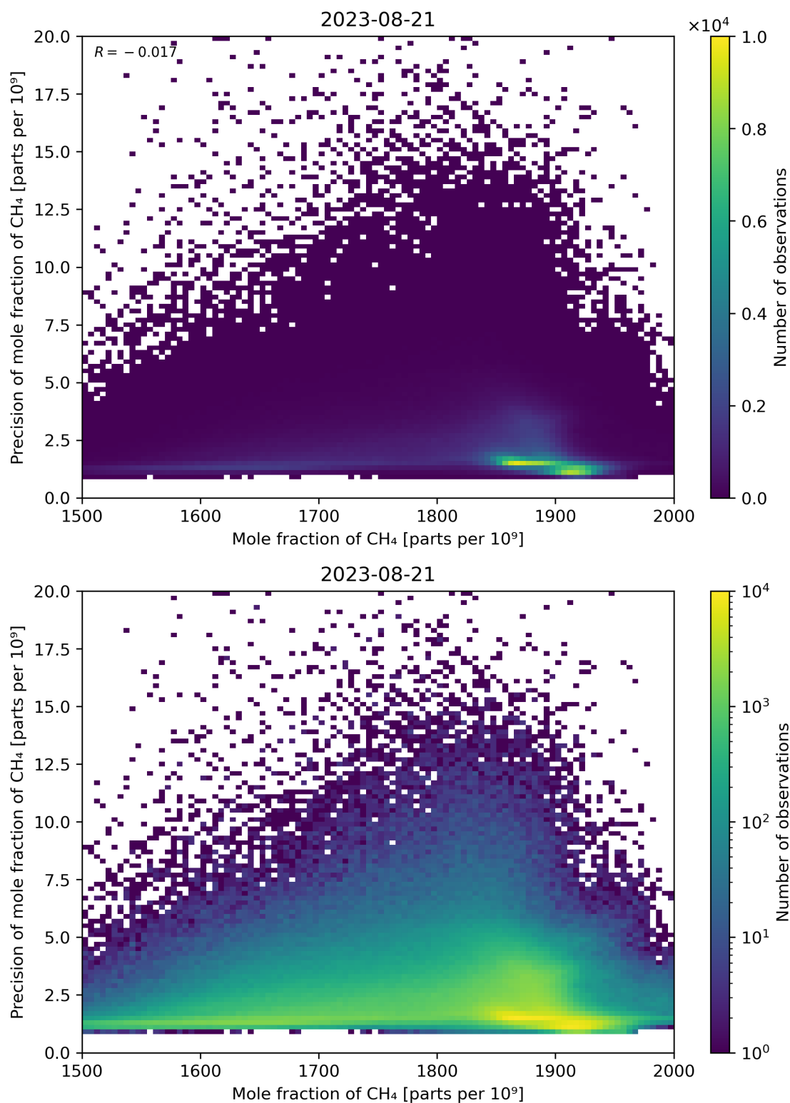
Figure 75: Scatter density plot of “Mole fraction of CH 4 ” against “Precision of mole fraction of CH 4 ” for 2023-08-20 to 2023-08-22.
