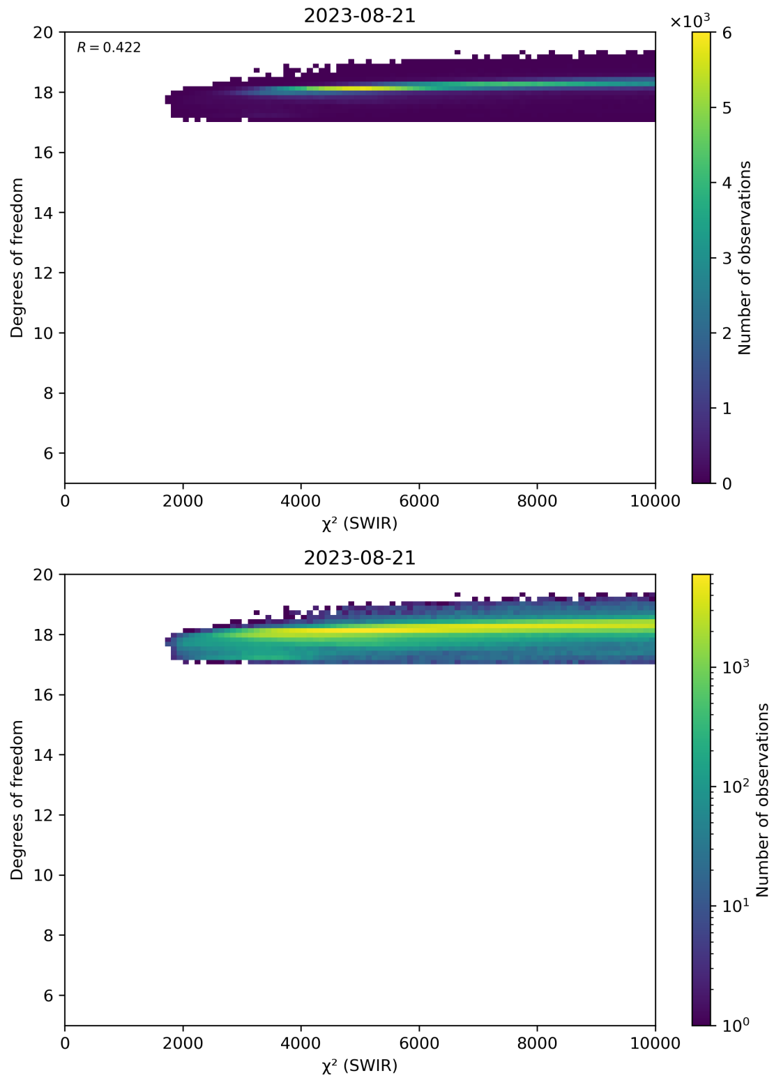
Figure 48: Scatter density plot of “ \chi^2 (SWIR)” against “Degrees of freedom” for 2023-08-20 to 2023-08-22.
