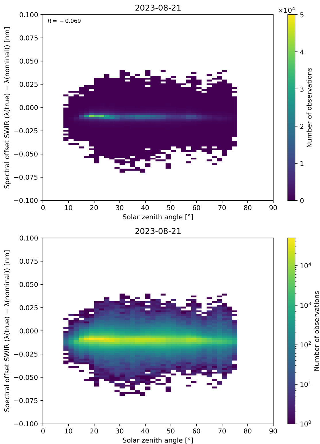
Figure 104: Scatter density plot of “Solar zenith angle” against “Spectral offset SWIR ( \lambda(\text{true}) - \lambda(\text{nominal}) )” for 2023-08-20 to 2023-08-22.
