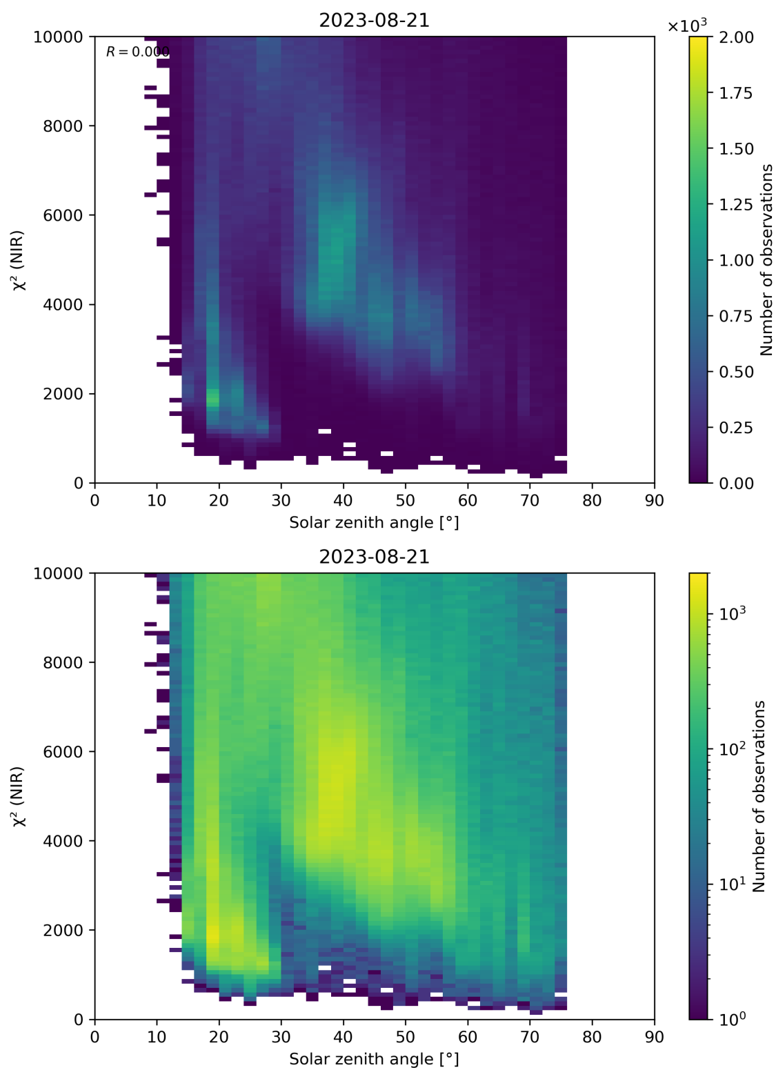
Figure 94: Scatter density plot of “Solar zenith angle” against “ \chi^2 (NIR)” for 2023-08-20 to 2023-08-22.
