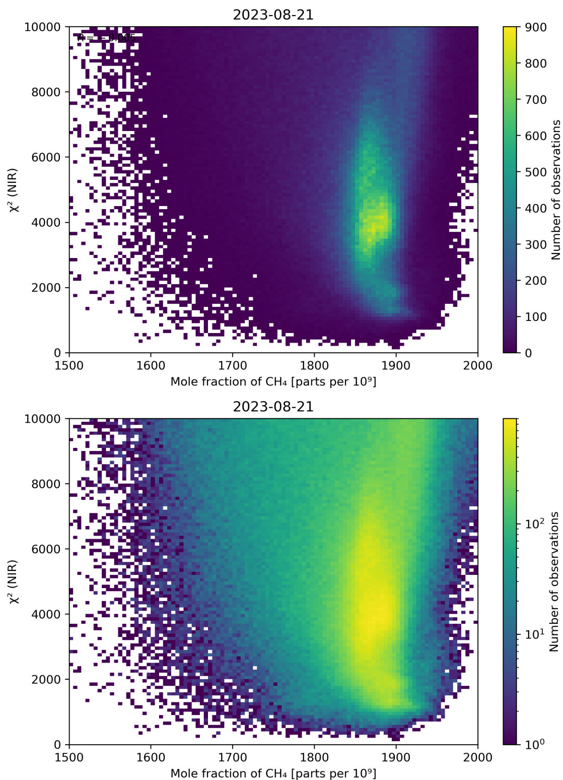
Figure 70: Scatter density plot of “Mole fraction of CH 4 ” against “ \chi^2 (NIR)” for 2023-08-20 to 2023-08-22.
