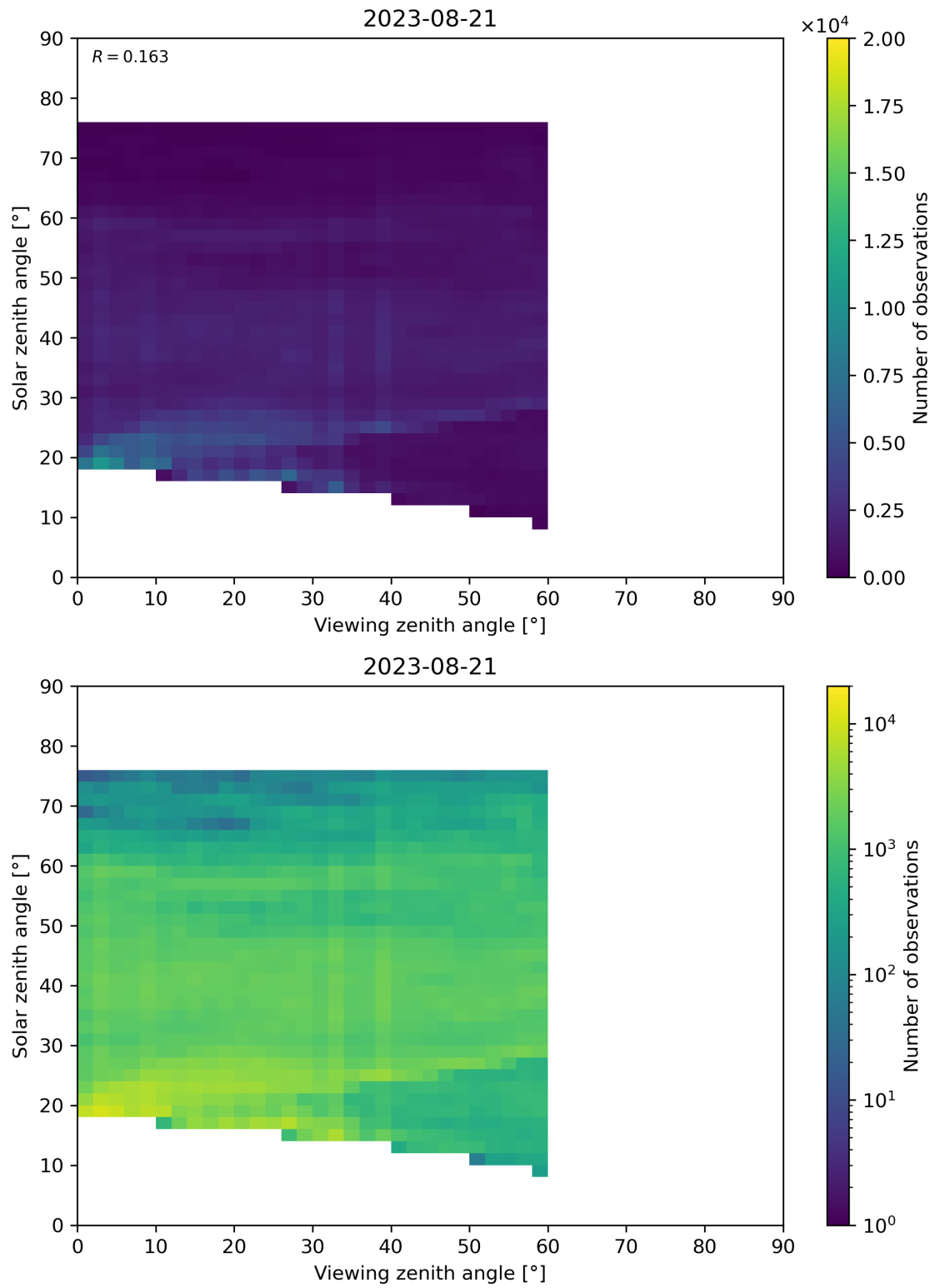
Figure 115: Scatter density plot of “Viewing zenith angle” against “Solar zenith angle” for 2023-08-20 to 2023-08-22.
