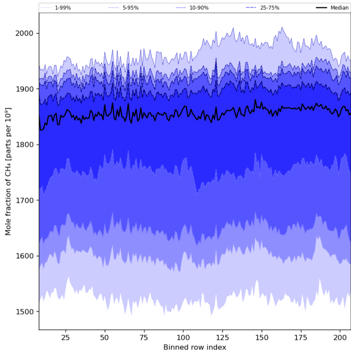
Figure 34: Along track statistics of “Mole fraction of CH 4 ” for 2023-08-20 to 2023-08-22
