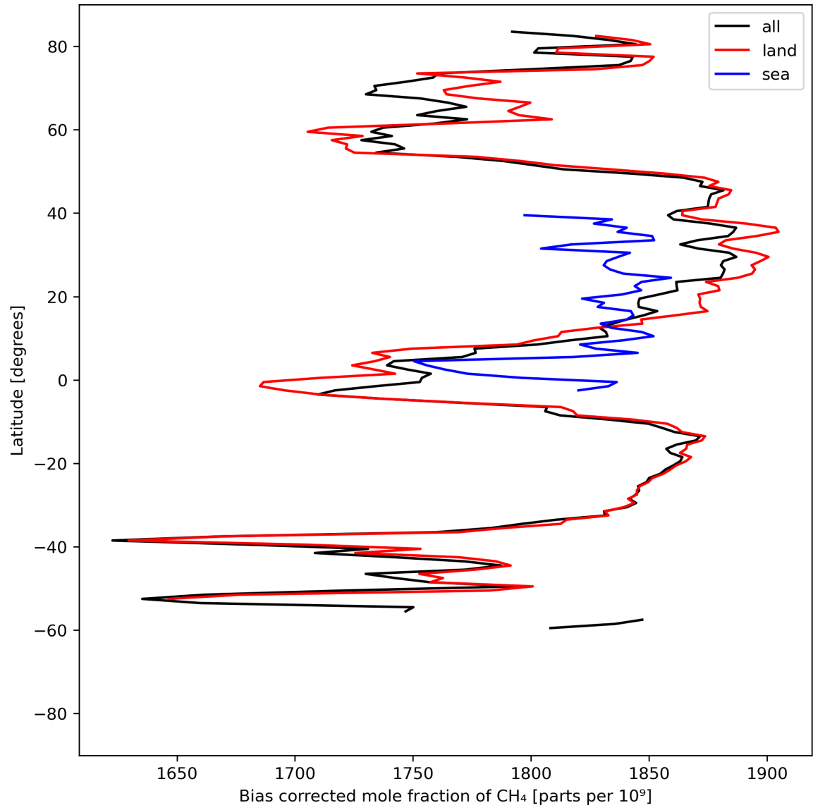
Figure 14: Zonal average of “Bias corrected mole fraction of \text{CH}_4 ” for 2023-08-20 to 2023-08-22.
