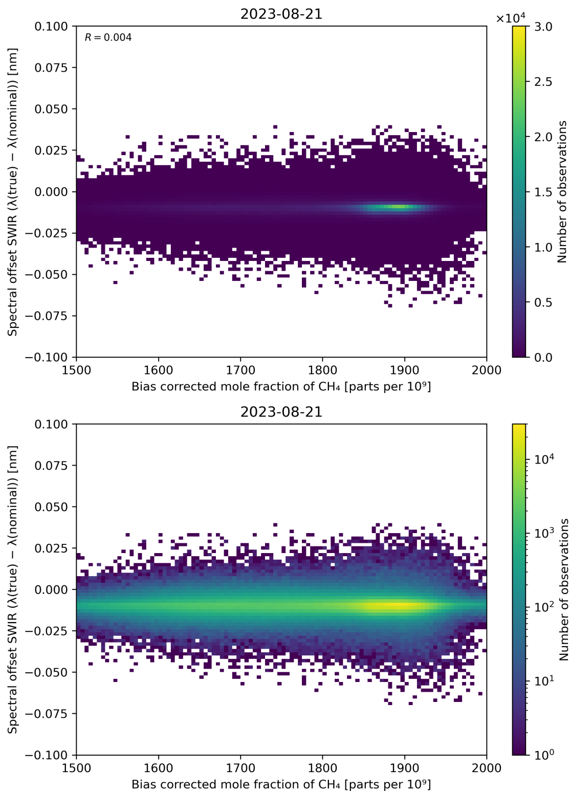
Figure 69: Scatter density plot of “Bias corrected mole fraction of \text{CH}_4 ” against “Spectral offset SWIR ( \lambda(\text{true}) - \lambda(\text{nominal}) )” for 2023-08-20 to 2023-08-22.
