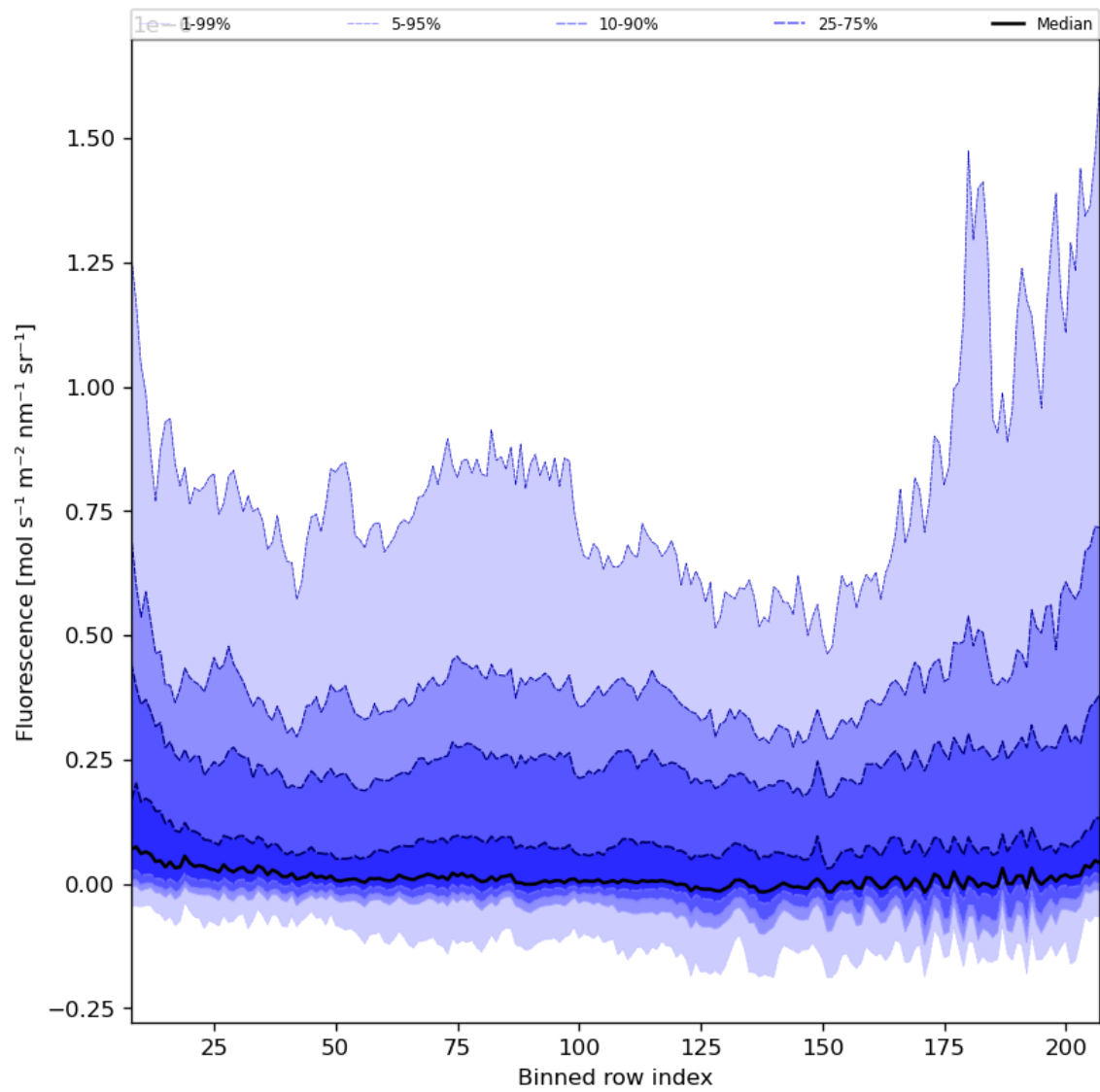
Figure 43: Along track statistics of “Fluorescence” for 2023-08-20 to 2023-08-22
