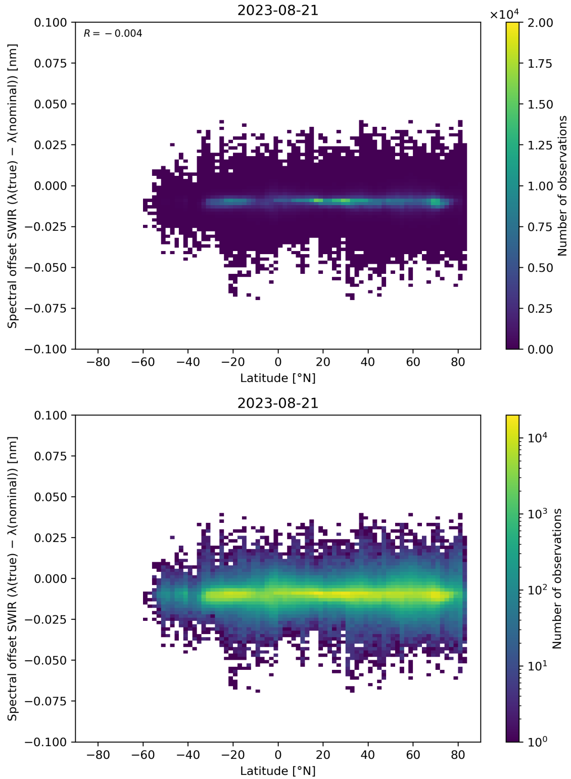
Figure 62: Scatter density plot of “Latitude” against “Spectral offset SWIR ( \lambda(\text{true}) - \lambda(\text{nominal}) )” for 2023-08-20 to 2023-08-22.
