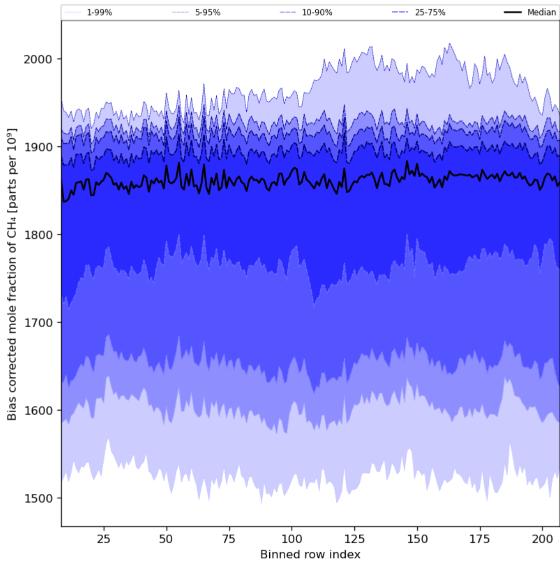
Figure 36: Along track statistics of “Bias corrected mole fraction of CH 4 ” for 2023-08-20 to 2023-08-22
