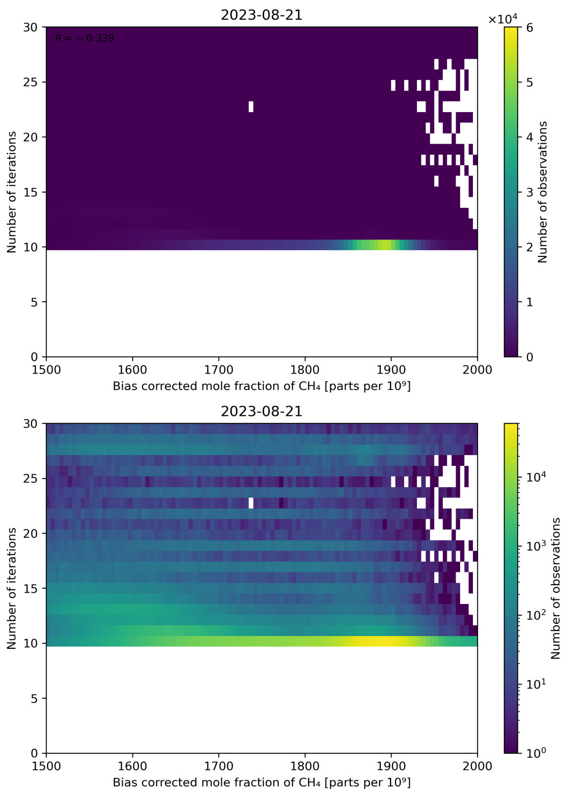
Figure 67: Scatter density plot of “Bias corrected mole fraction of CH 4 ” against “Number of iterations” for 2023-08-20 to 2023-08-22.
