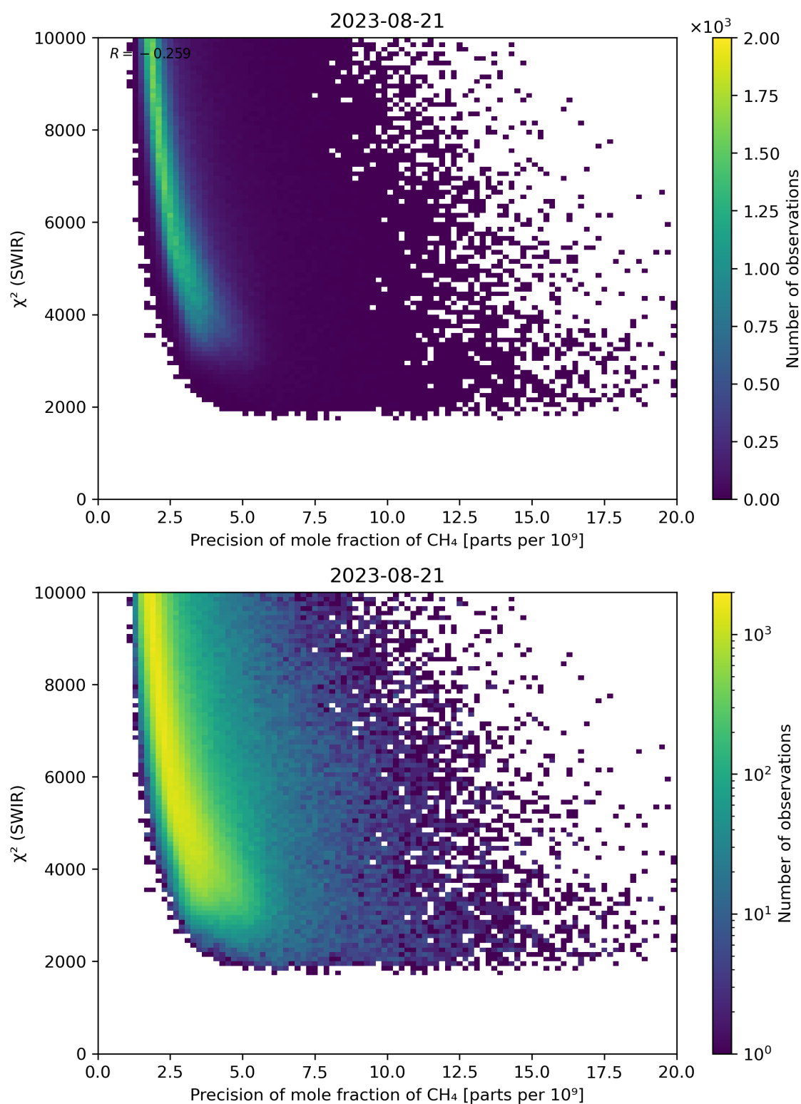
Figure 79: Scatter density plot of “Precision of mole fraction of \text{CH}_4 ” against “ \chi^2 (SWIR)” for 2023-08-20 to 2023-08-22.
