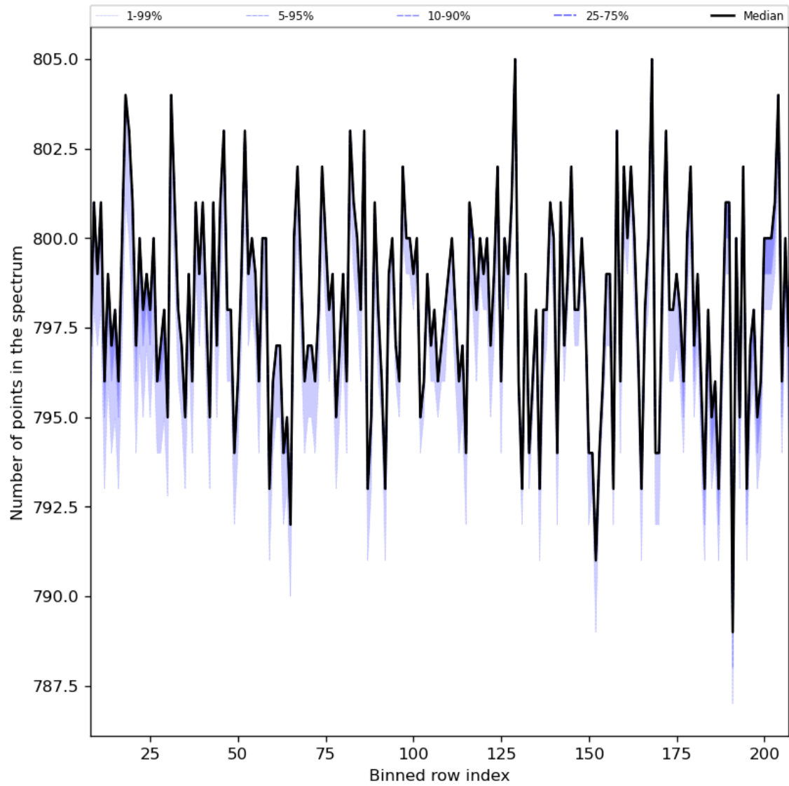
Figure 37: Along track statistics of “Number of points in the spectrum” for 2023-08-20 to 2023-08-22
