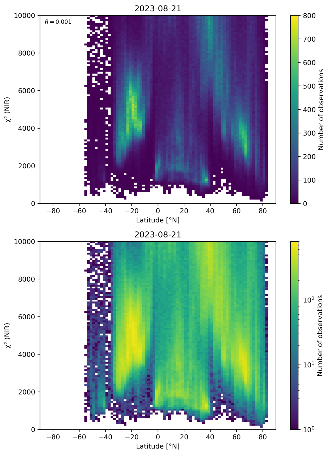
Figure 53: Scatter density plot of “Latitude” against “ \chi^2 (NIR)” for 2023-08-20 to 2023-08-22.
