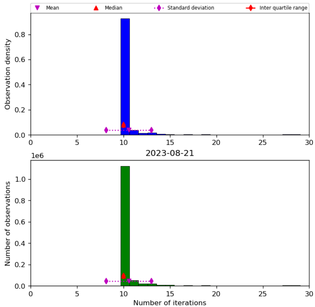
Figure 31: Histogram of “Number of iterations” for 2023-08-20 to 2023-08-22
