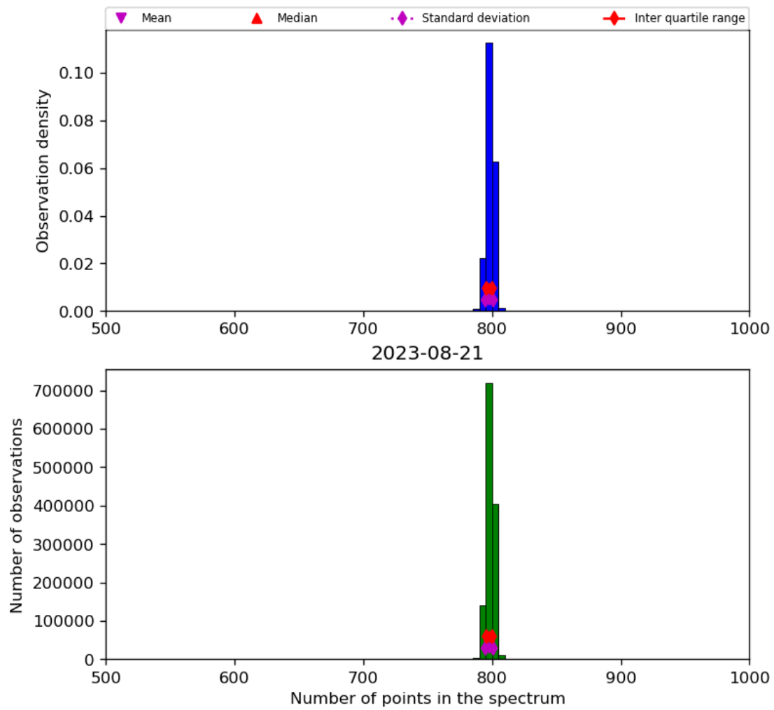
Figure 26: Histogram of “Number of points in the spectrum” for 2023-08-20 to 2023-08-22
