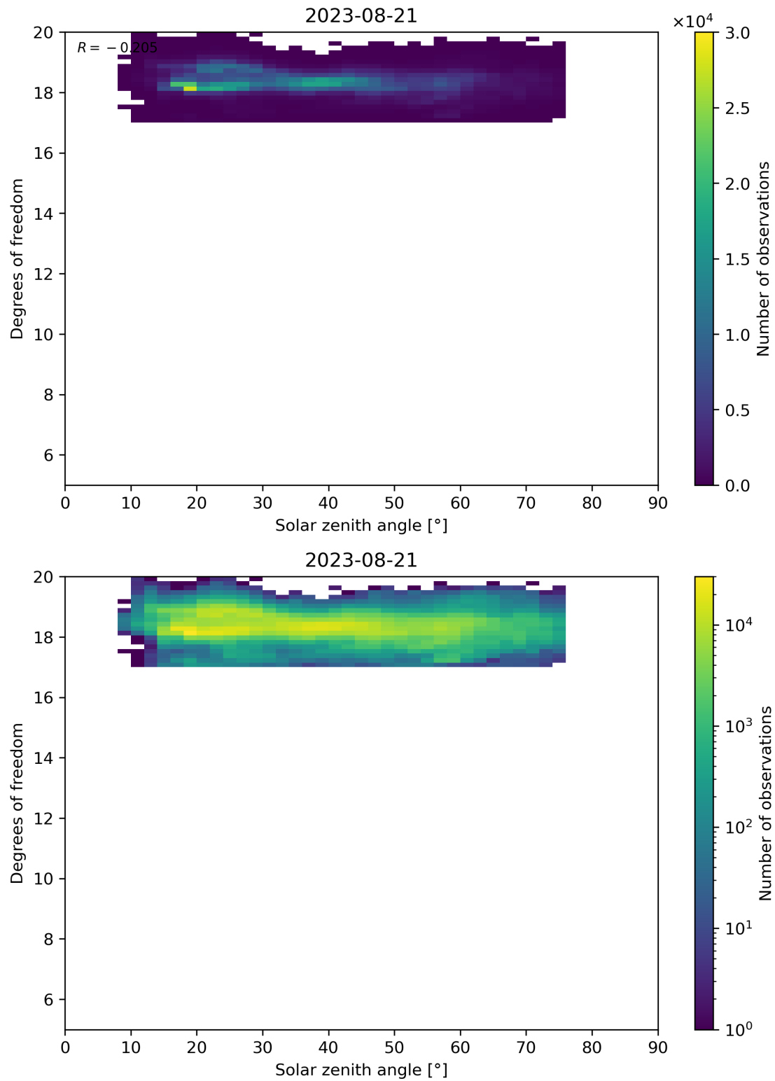
Figure 96: Scatter density plot of “Solar zenith angle” against “Degrees of freedom” for 2023-08-20 to 2023-08-22.
