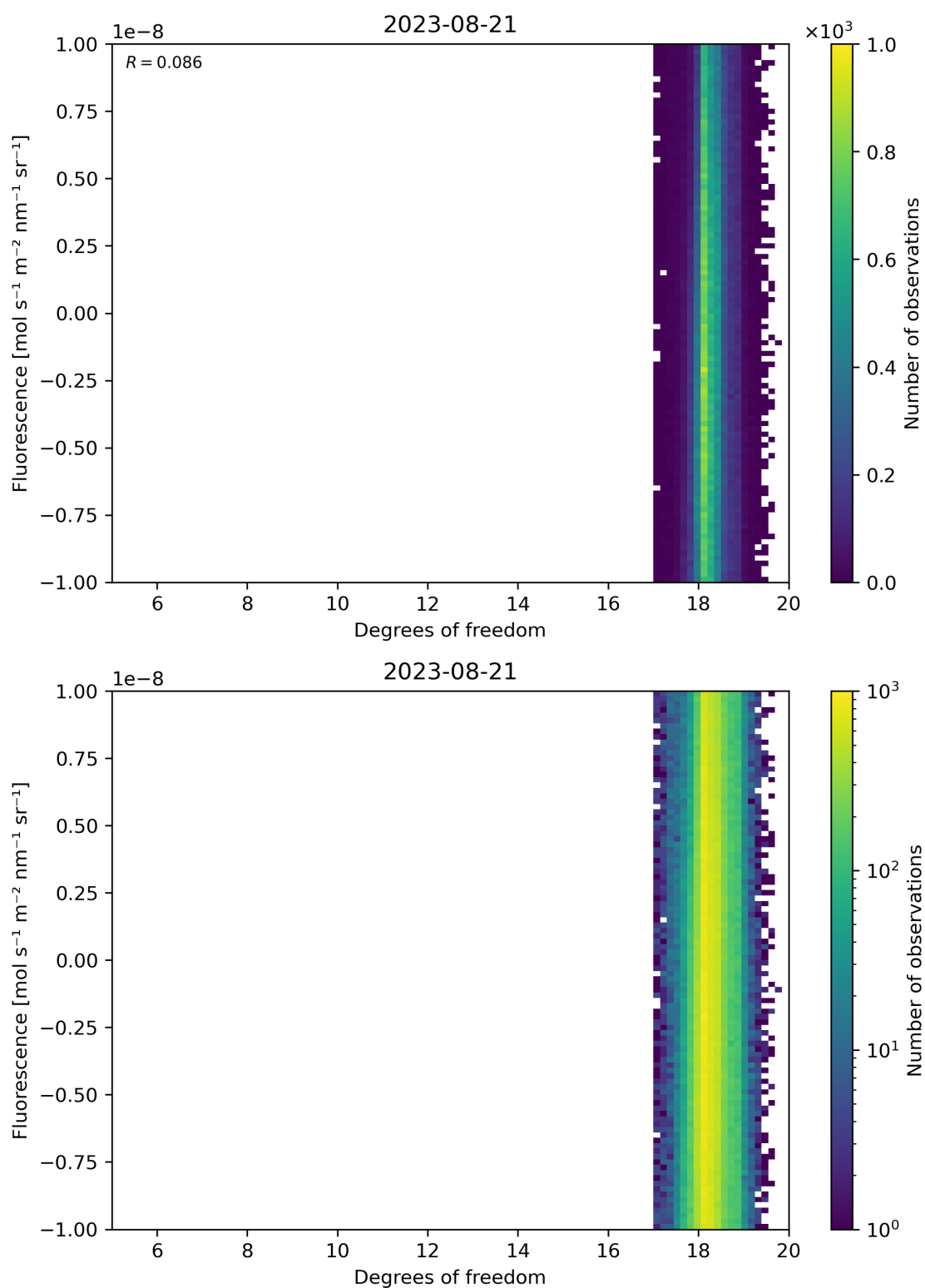
Figure 51: Scatter density plot of “Degrees of freedom” against “Fluorescence” for 2023-08-20 to 2023-08-22.
