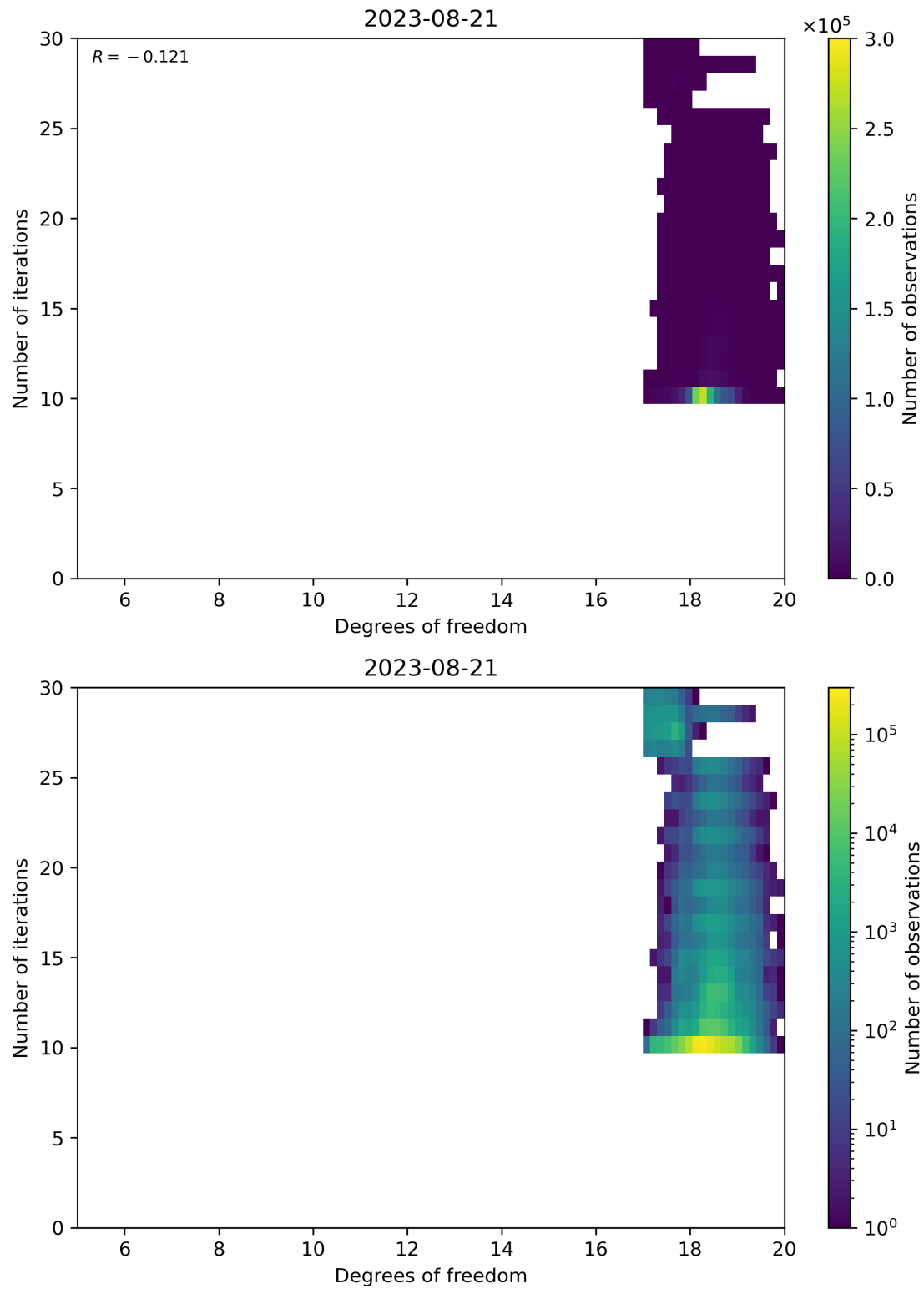
Figure 52: Scatter density plot of “Degrees of freedom” against “Number of iterations” for 2023-08-20 to 2023-08-22.
