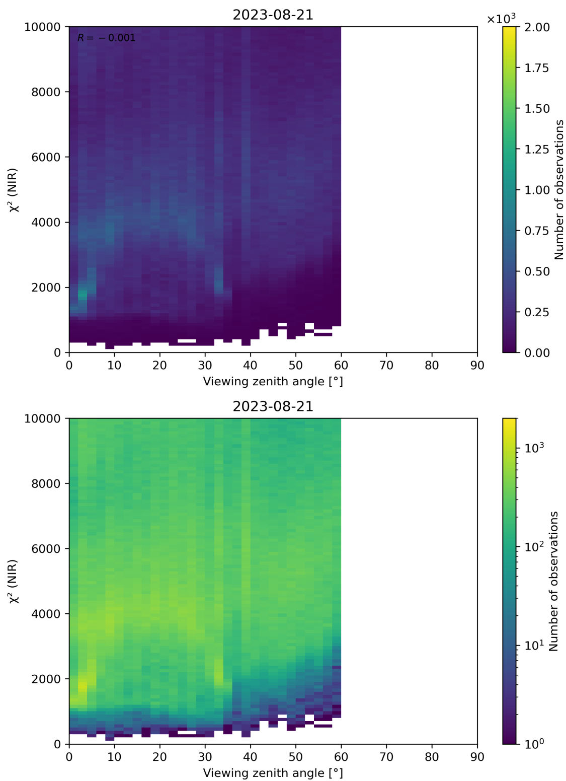
Figure 105: Scatter density plot of “Viewing zenith angle” against “ \chi^2 (NIR)” for 2023-08-20 to 2023-08-22.
