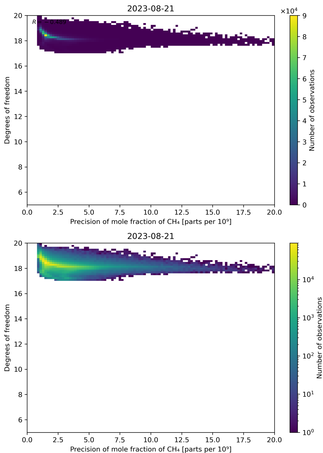
Figure 80: Scatter density plot of “Precision of mole fraction of CH 4 ” against “Degrees of freedom” for 2023-08-20 to 2023-08-22.
