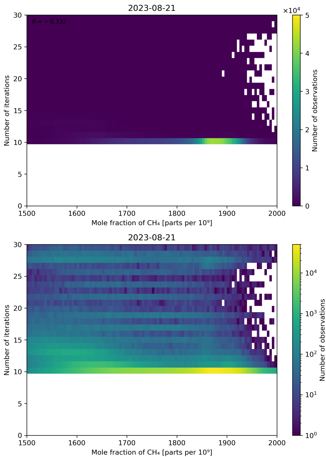
Figure 76: Scatter density plot of “Mole fraction of CH 4 ” against “Number of iterations” for 2023-08-20 to 2023-08-22.
