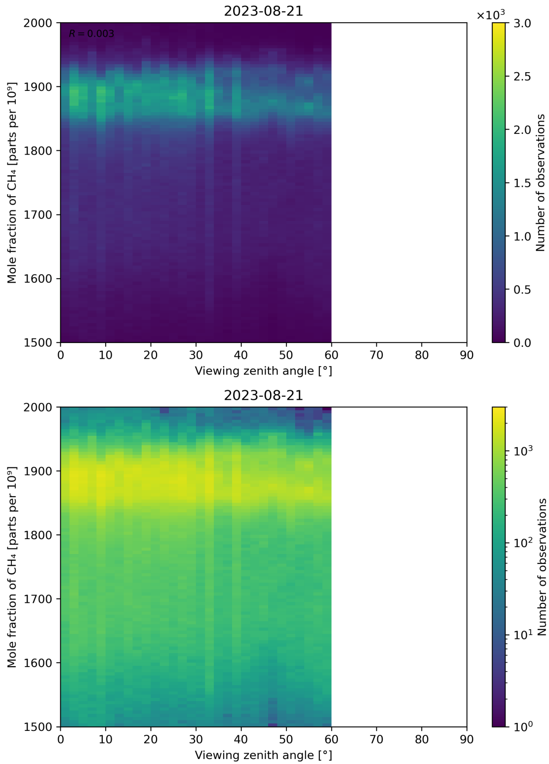
Figure 110: Scatter density plot of “Viewing zenith angle” against “Mole fraction of CH 4 ” for 2023-08-20 to 2023-08-22.
