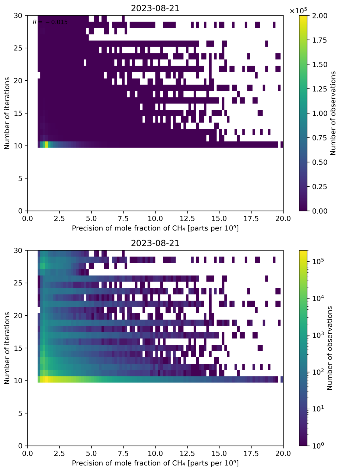
Figure 83: Scatter density plot of “Precision of mole fraction of CH 4 ” against “Number of iterations” for 2023-08-20 to 2023-08-22.
