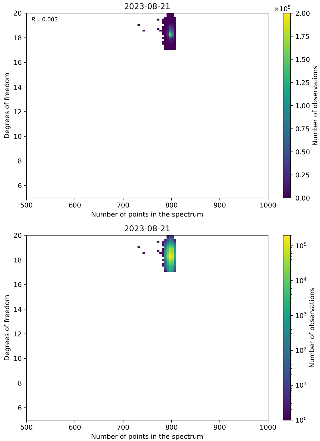
Figure 90: Scatter density plot of “Number of points in the spectrum” against “Degrees of freedom” for 2023-08-20 to 2023-08-22.
