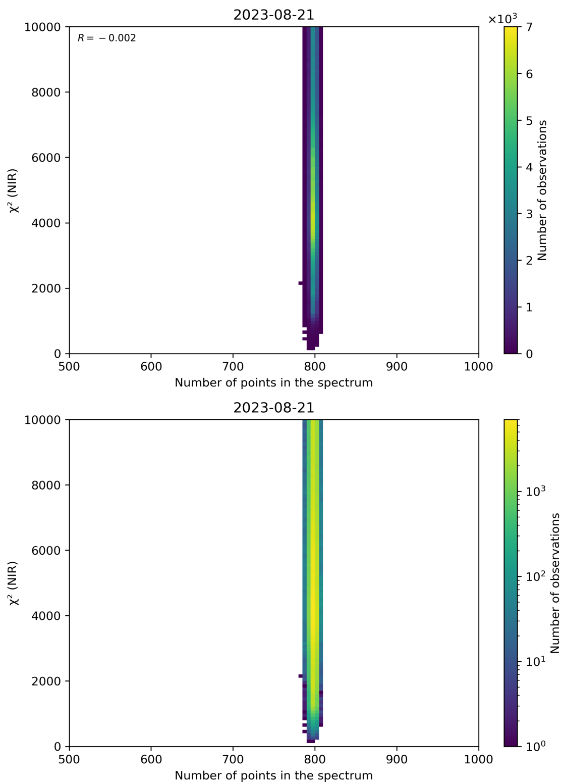
Figure 88: Scatter density plot of “Number of points in the spectrum” against “ \chi^2 (NIR)” for 2023-08-20 to 2023-08-22.
