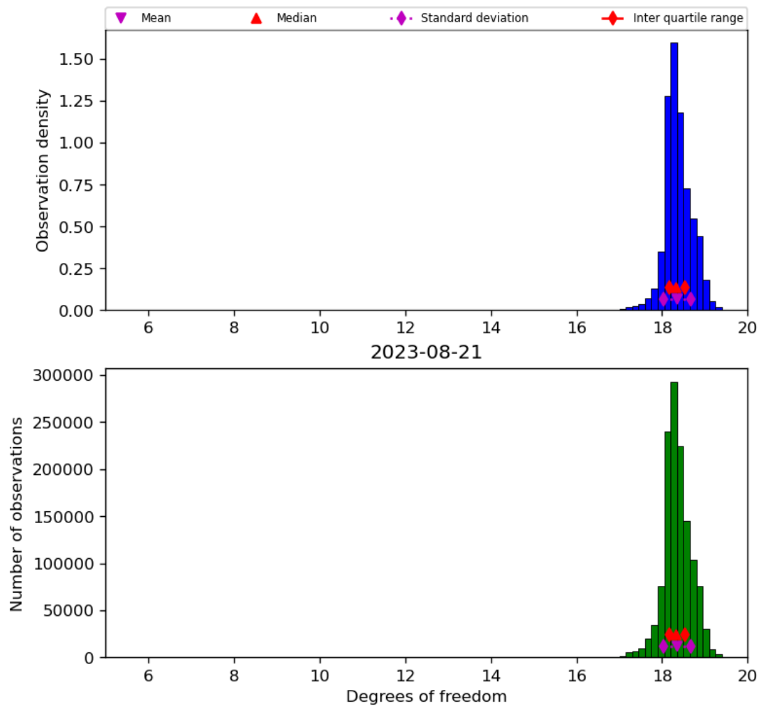
Figure 30: Histogram of “Degrees of freedom” for 2023-08-20 to 2023-08-22
