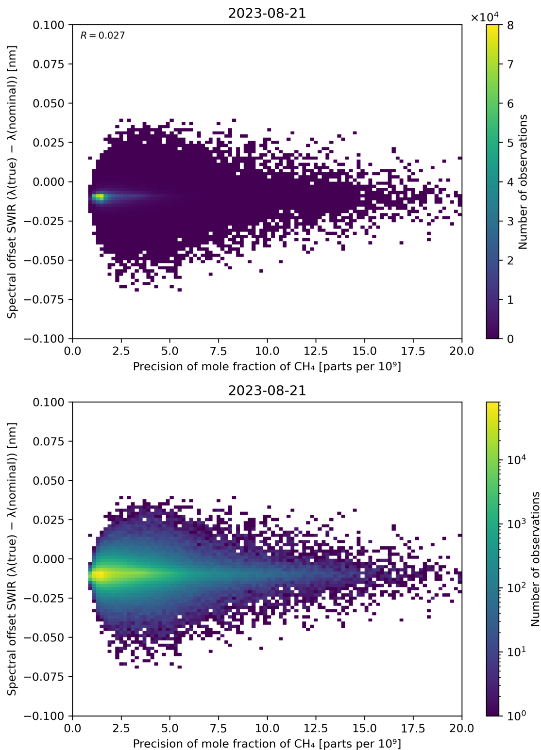
Figure 85: Scatter density plot of “Precision of mole fraction of \text{CH}_4 ” against “Spectral offset SWIR ( \lambda(\text{true}) - \lambda(\text{nominal}) )” for 2023-08-20 to 2023-08-22.
