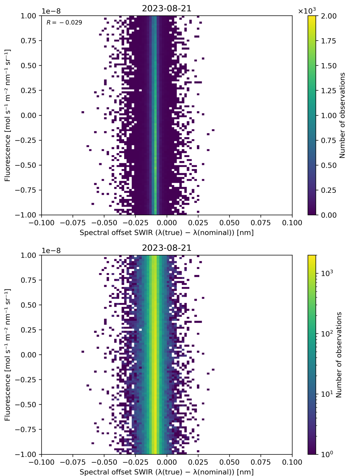
Figure 120: Scatter density plot of “Spectral offset SWIR ( \lambda(\text{true}) - \lambda(\text{nominal}) )” against “Fluorescence” for 2023-08-20 to 2023-08-22.
