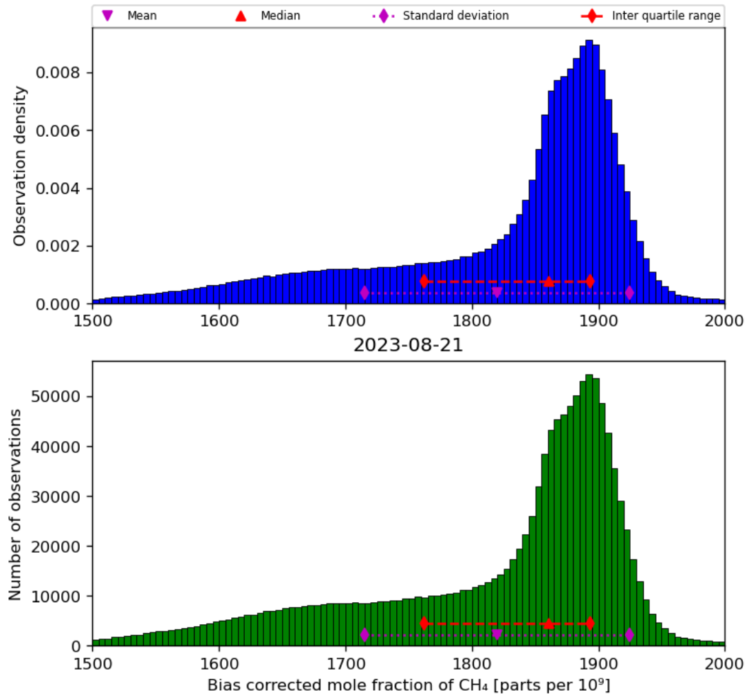
Figure 25: Histogram of “Bias corrected mole fraction of CH 4 ” for 2023-08-20 to 2023-08-22
