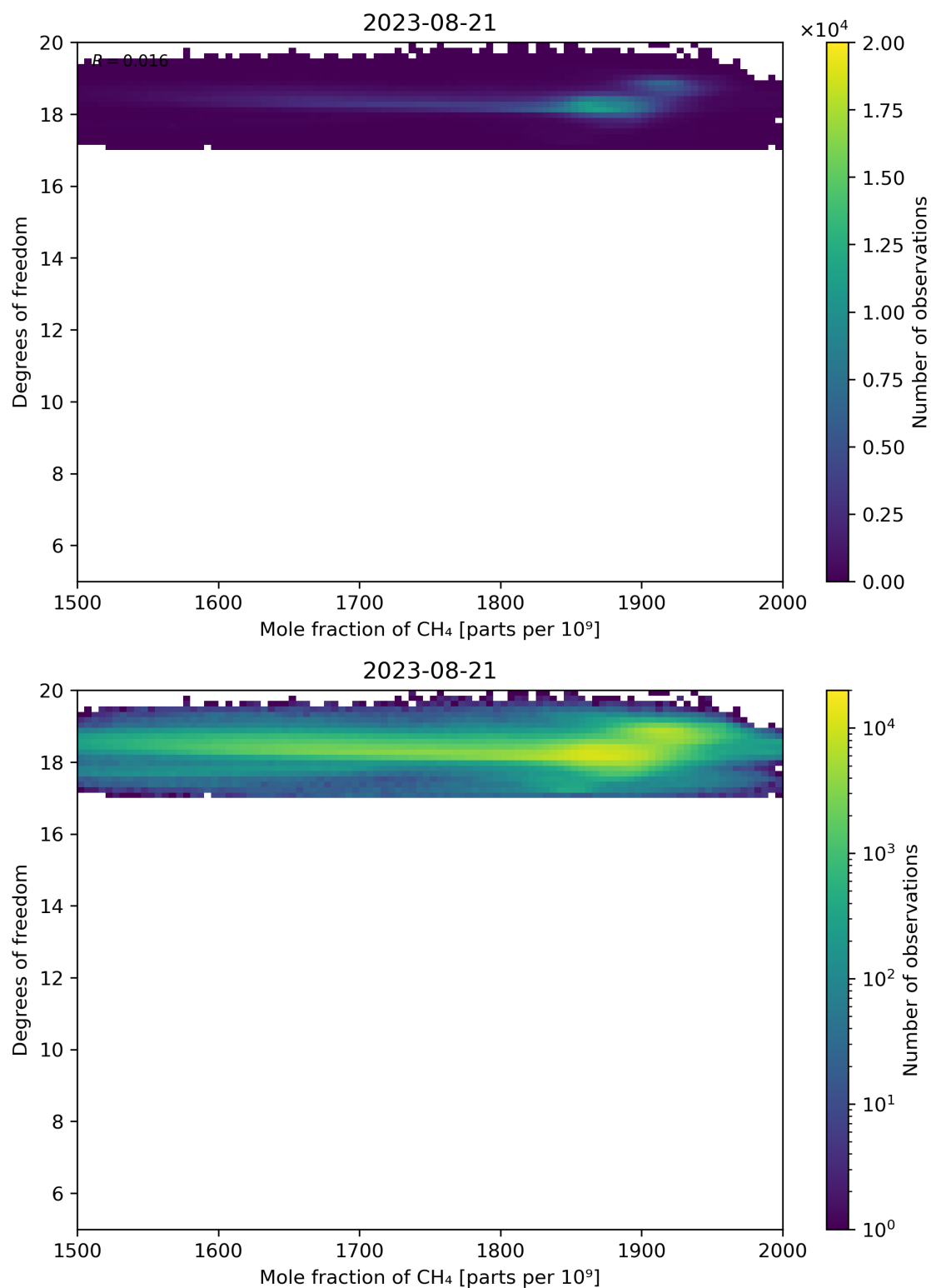
Figure 72: Scatter density plot of “Mole fraction of CH 4 ” against “Degrees of freedom” for 2023-08-20 to 2023-08-22.
