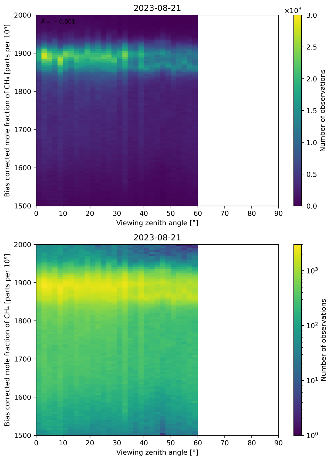
Figure 111: Scatter density plot of “Viewing zenith angle” against “Bias corrected mole fraction of CH 4 ” for 2023-08-20 to 2023-08-22.
