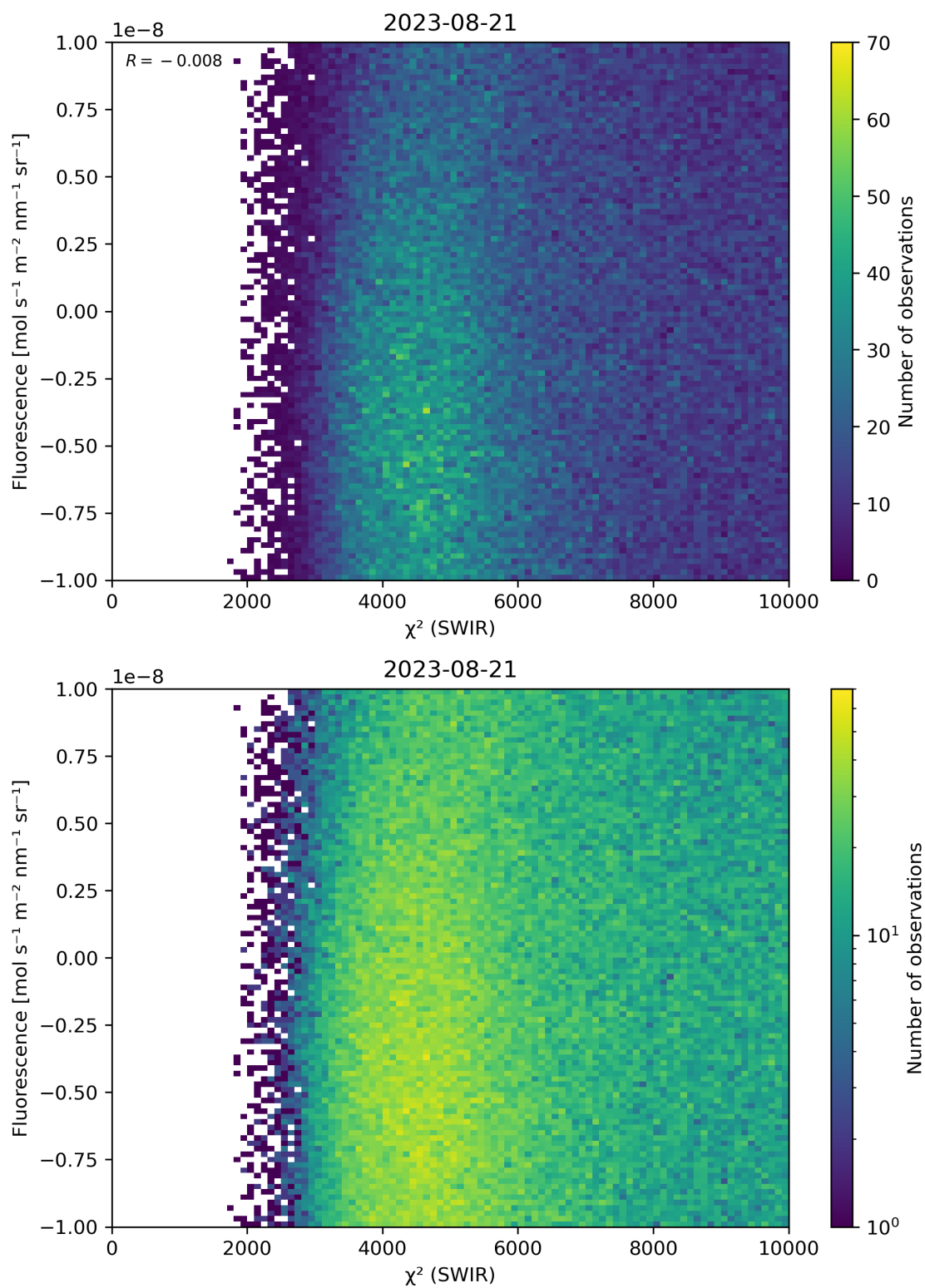
Figure 49: Scatter density plot of “ \chi^2 (SWIR)” against “Fluorescence” for 2023-08-20 to 2023-08-22.
