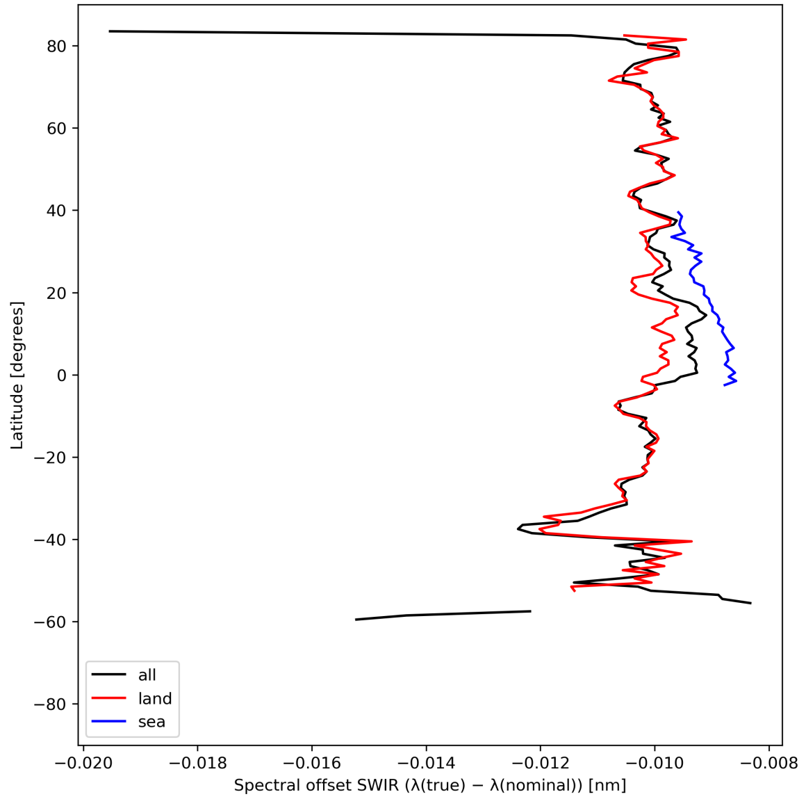
Figure 16: Zonal average of “Spectral offset SWIR ( \lambda(\text{true}) - \lambda(\text{nominal}) )” for 2023-08-20 to 2023-08-22.
