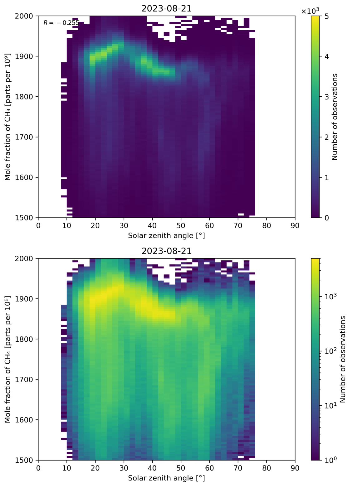
Figure 99: Scatter density plot of “Solar zenith angle” against “Mole fraction of CH 4 ” for 2023-08-20 to 2023-08-22.
