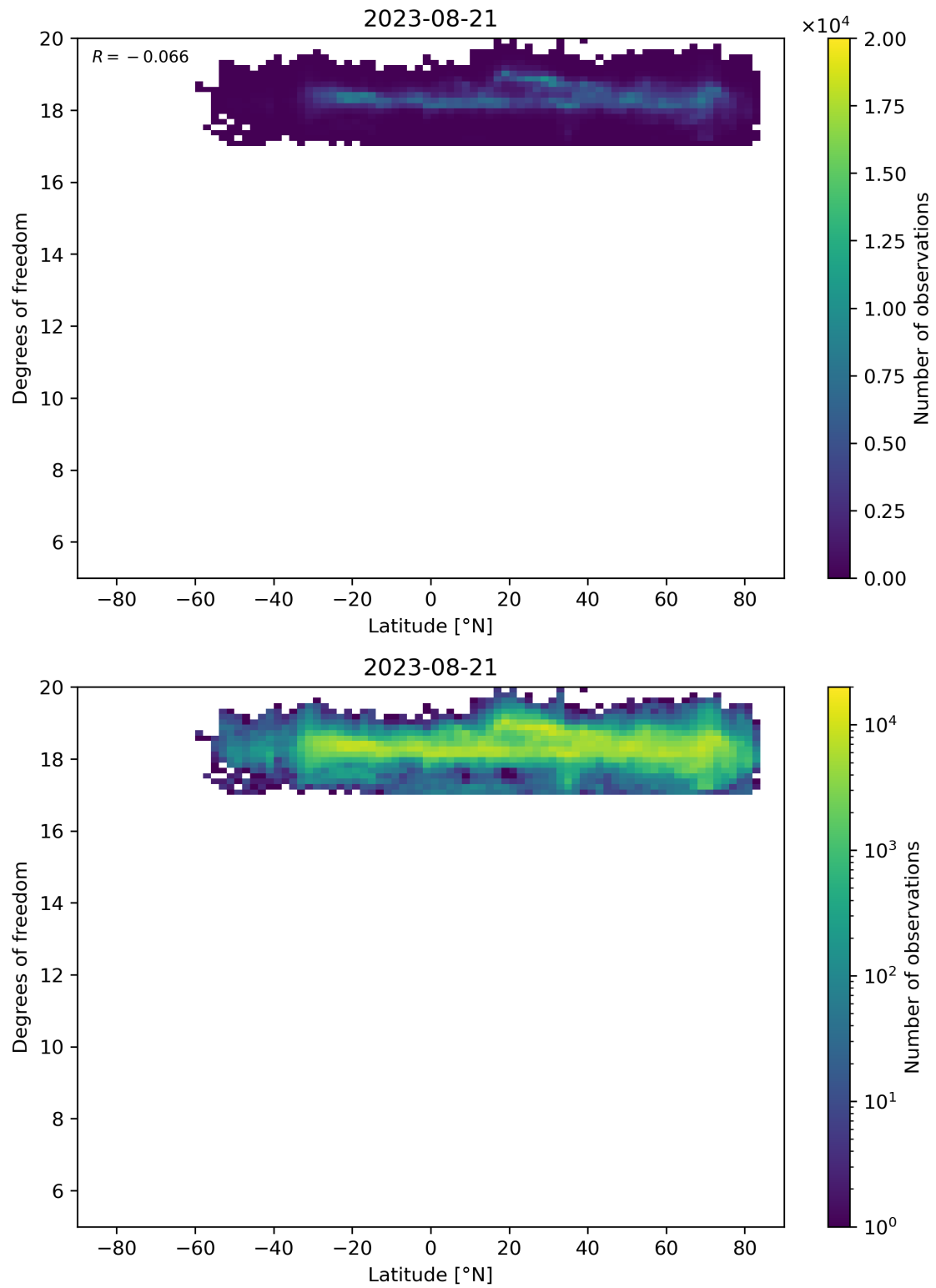
Figure 55: Scatter density plot of “Latitude” against “Degrees of freedom” for 2023-08-20 to 2023-08-22.
