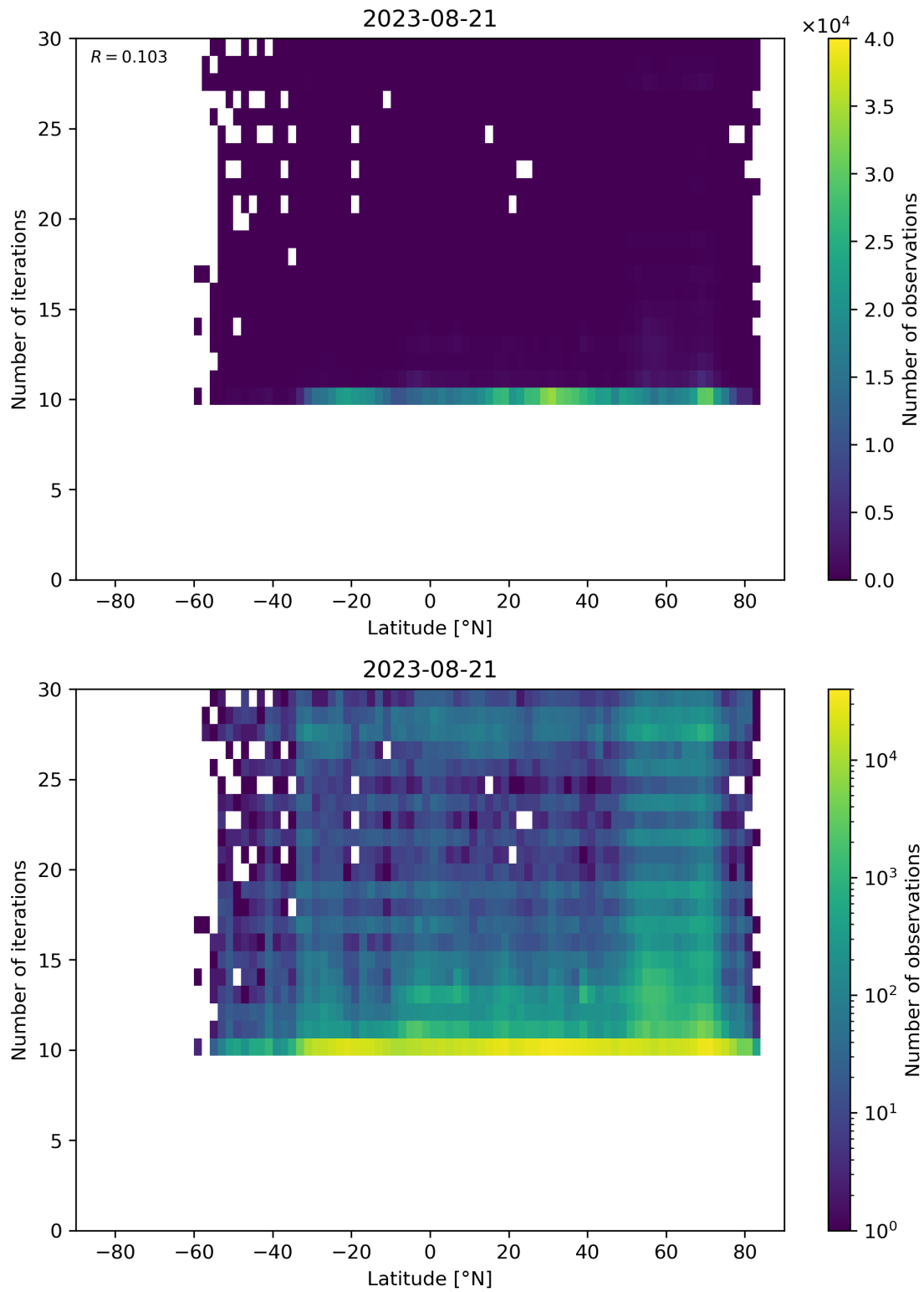
Figure 60: Scatter density plot of “Latitude” against “Number of iterations” for 2023-08-20 to 2023-08-22.
