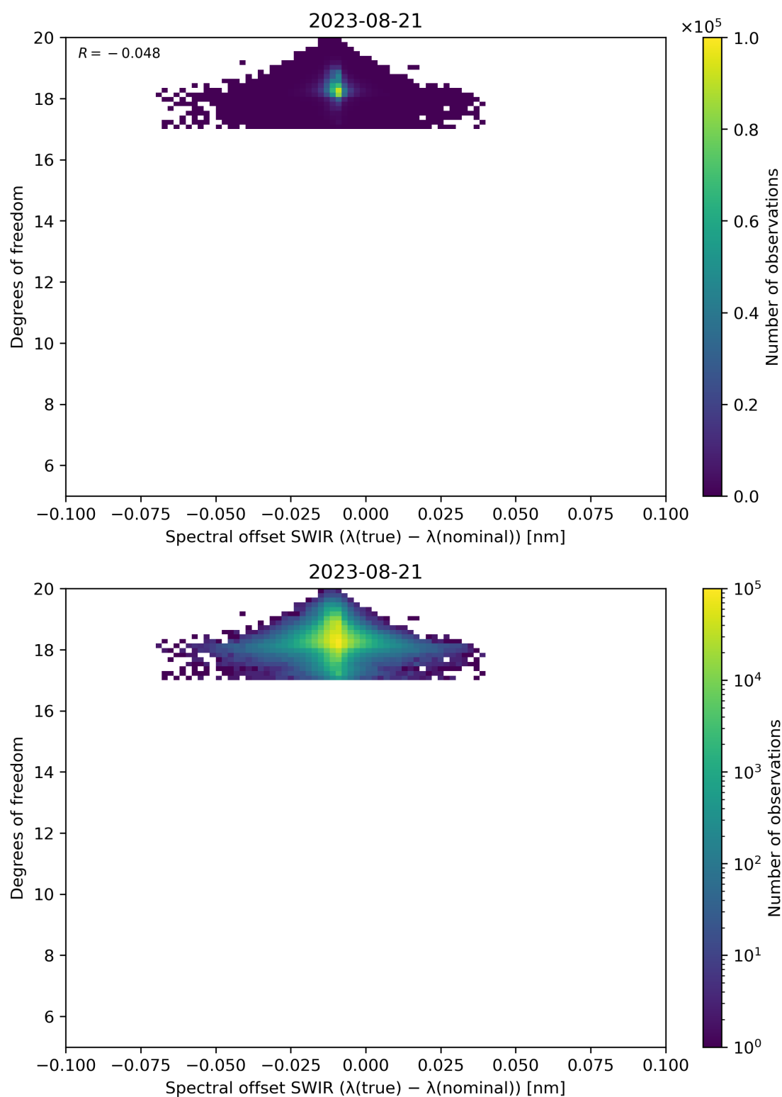
Figure 119: Scatter density plot of “Spectral offset SWIR ( \lambda(\text{true}) - \lambda(\text{nominal}) )” against “Degrees of freedom” for 2023-08-20 to 2023-08-22.
