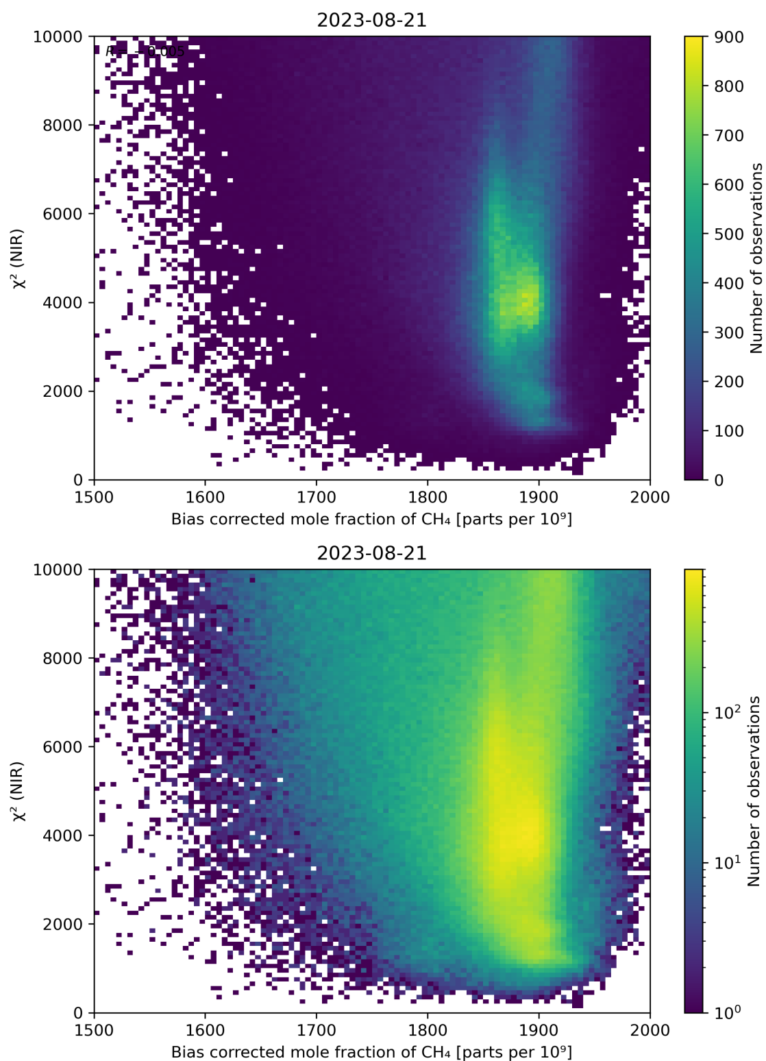
Figure 63: Scatter density plot of “Bias corrected mole fraction of CH 4 ” against “ \chi^2 (NIR)” for 2023-08-20 to 2023-08-22.
