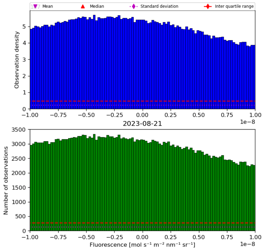
Figure 32: Histogram of “Fluorescence” for 2023-08-20 to 2023-08-22
