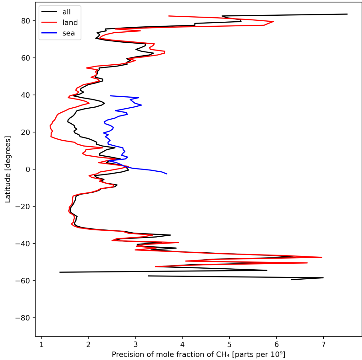
Figure 13: Zonal average of “Precision of mole fraction of CH 4 ” for 2023-08-20 to 2023-08-22.
