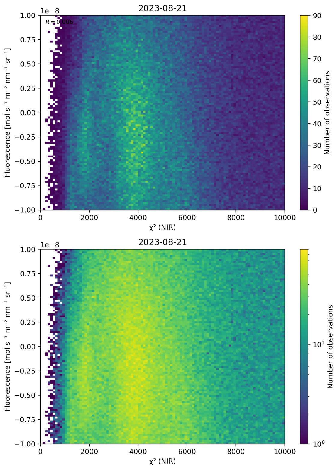
Figure 45: Scatter density plot of “ \chi^2 (NIR)” against “Fluorescence” for 2023-08-20 to 2023-08-22.
