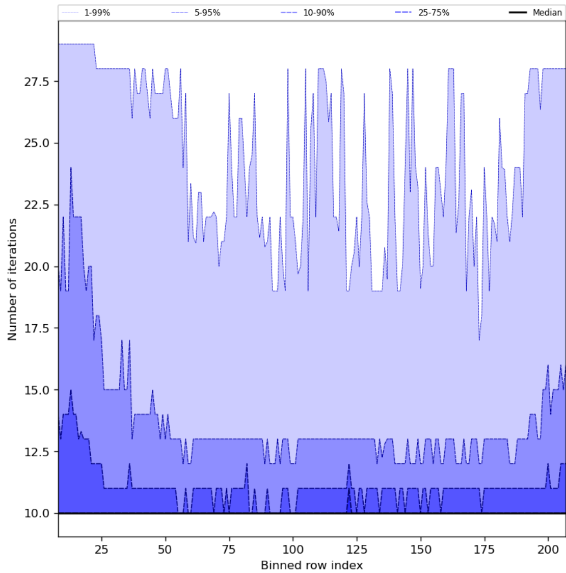
Figure 42: Along track statistics of “Number of iterations” for 2023-08-20 to 2023-08-22
