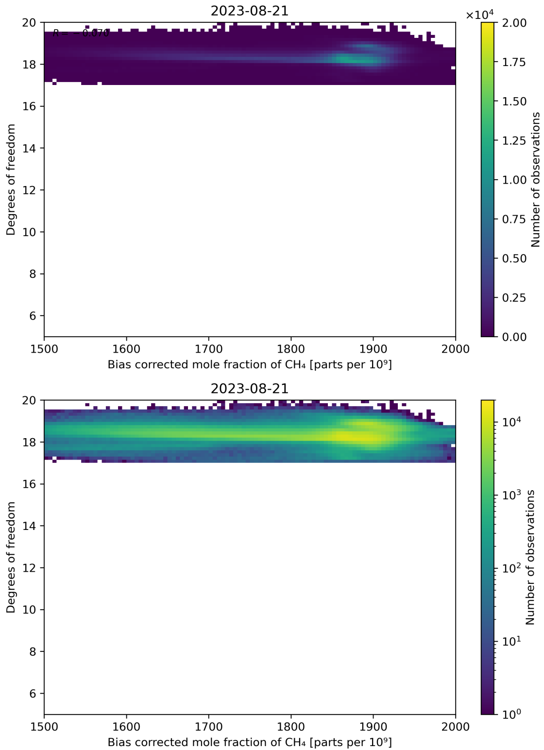
Figure 65: Scatter density plot of “Bias corrected mole fraction of CH 4 ” against “Degrees of freedom” for 2023-08-20 to 2023-08-22.
