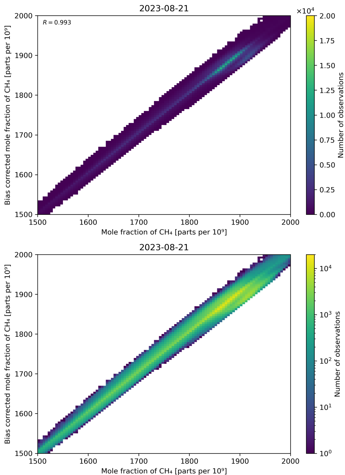
Figure 74: Scatter density plot of “Mole fraction of CH 4 ” against “Bias corrected mole fraction of CH 4 ” for 2023-08-20 to 2023-08-22.
