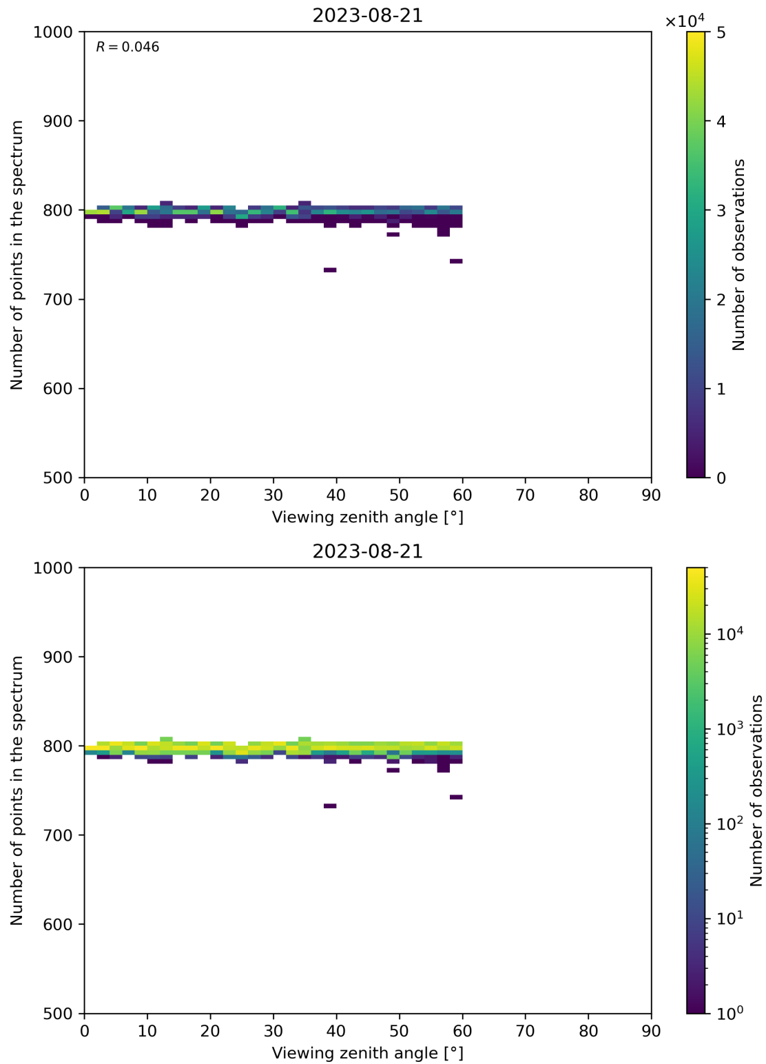
Figure 114: Scatter density plot of “Viewing zenith angle” against “Number of points in the spectrum” for 2023-08-20 to 2023-08-22.
