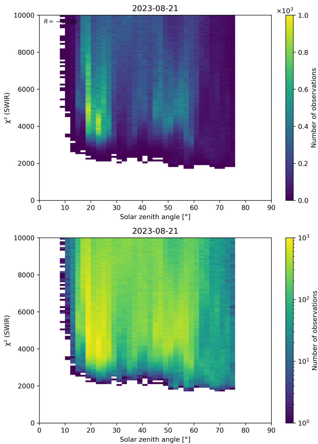
Figure 95: Scatter density plot of “Solar zenith angle” against “ \chi^2 (SWIR)” for 2023-08-20 to 2023-08-22.
