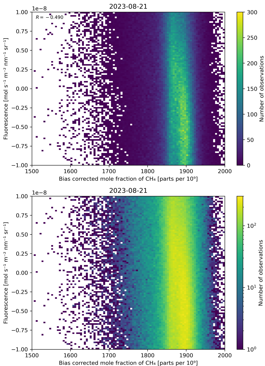
Figure 66: Scatter density plot of “Bias corrected mole fraction of \text{CH}_4 ” against “Fluorescence” for 2023-08-20 to 2023-08-22.
