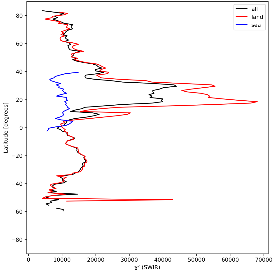
Figure 17: Zonal average of “ \chi^2 (SWIR)” for 2023-08-20 to 2023-08-22.
