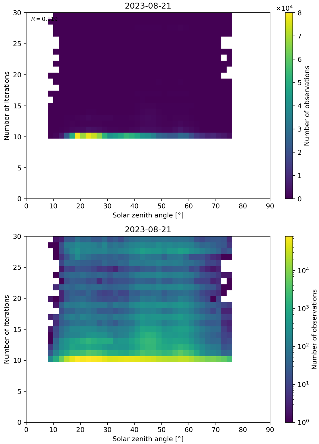
Figure 102: Scatter density plot of “Solar zenith angle” against “Number of iterations” for 2023-08-20 to 2023-08-22.
