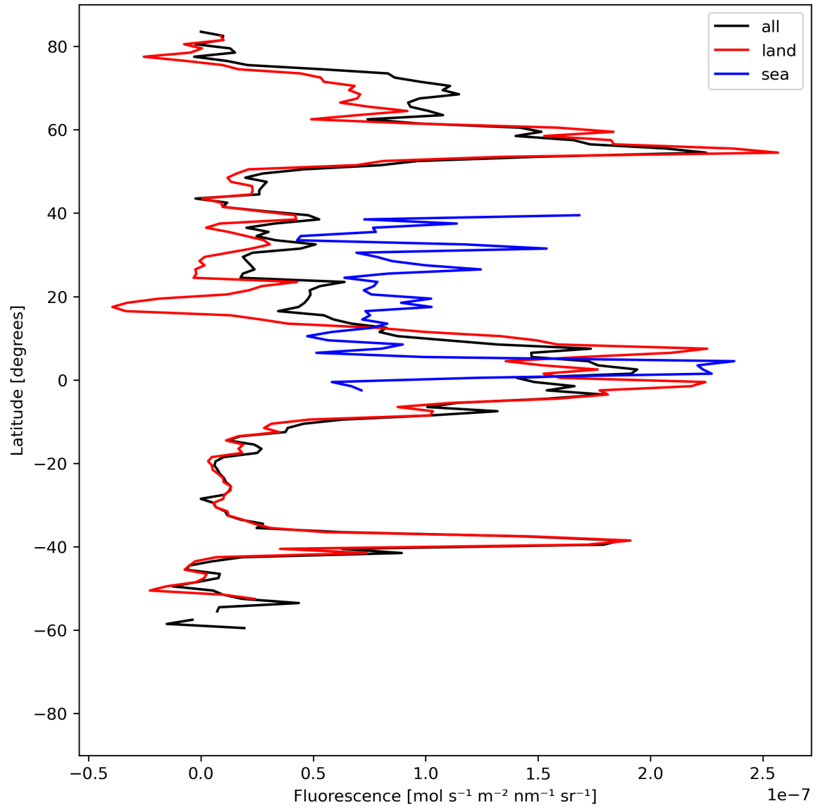
Figure 21: Zonal average of “Fluorescence” for 2023-08-20 to 2023-08-22.
