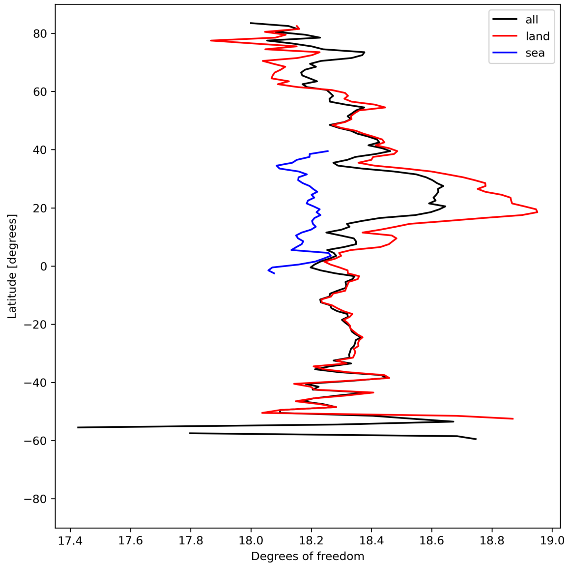
Figure 19: Zonal average of “Degrees of freedom” for 2023-08-20 to 2023-08-22.
