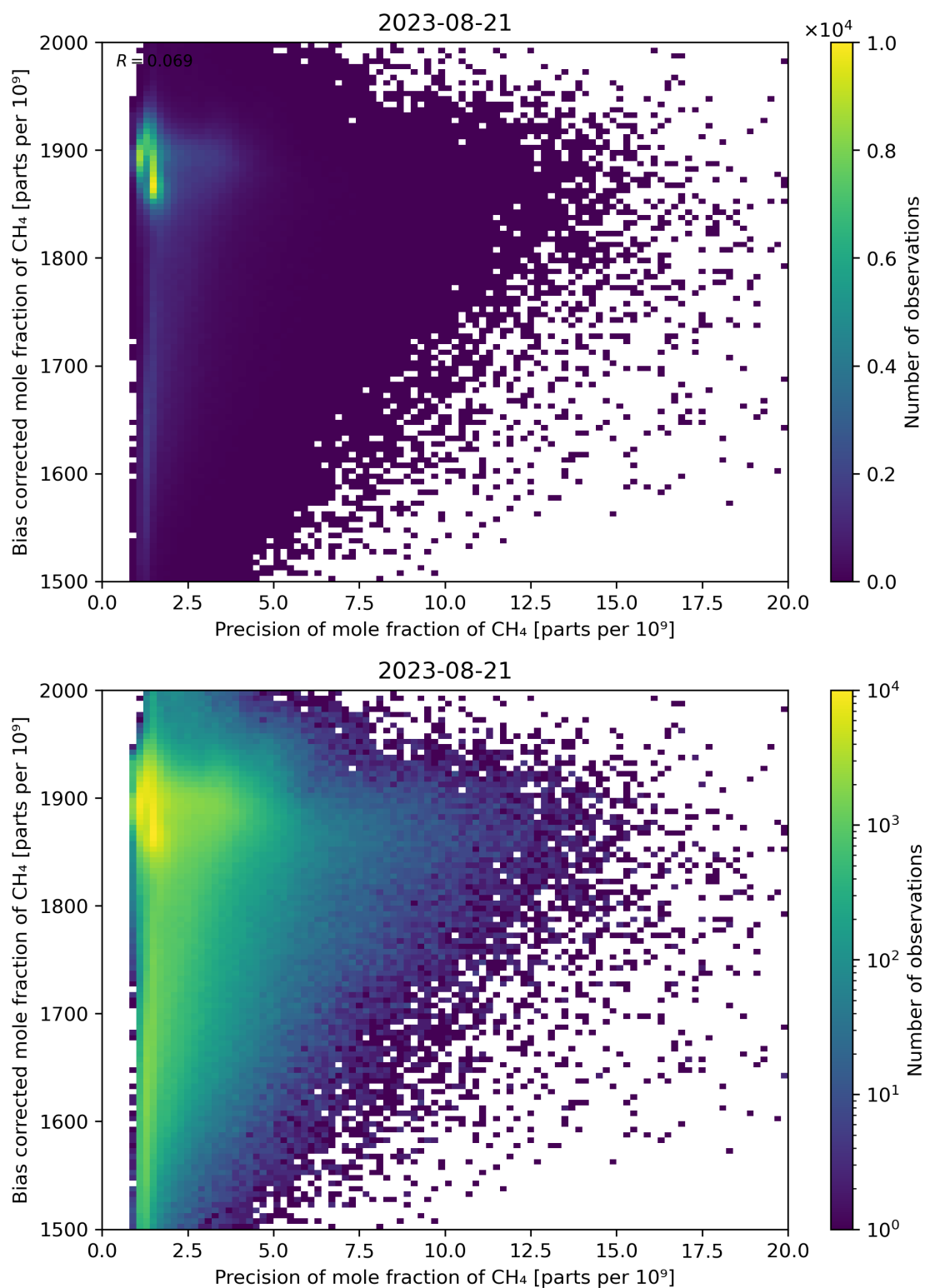
Figure 82: Scatter density plot of “Precision of mole fraction of CH 4 ” against “Bias corrected mole fraction of CH 4 ” for 2023-08-20 to 2023-08-22.
