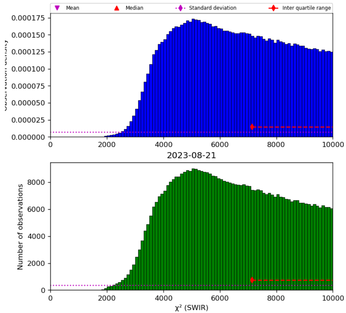
Figure 28: Histogram of “ \chi^2 (SWIR)” for 2023-08-20 to 2023-08-22
