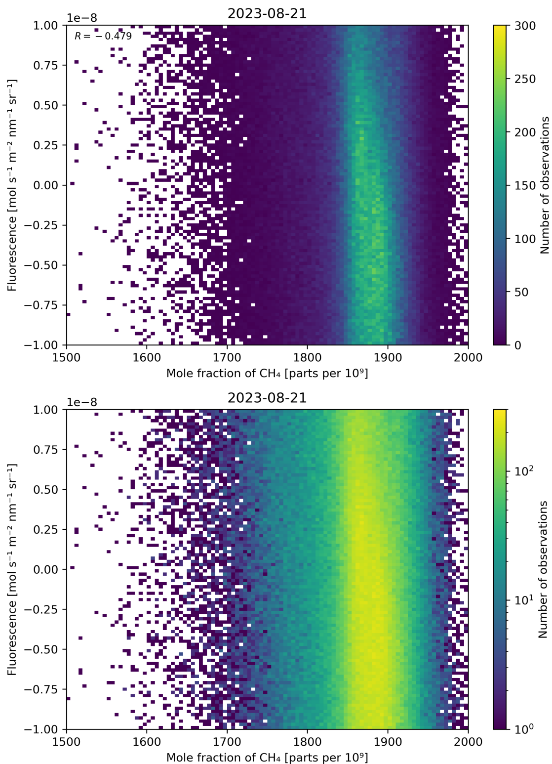
Figure 73: Scatter density plot of “Mole fraction of \text{CH}_4 ” against “Fluorescence” for 2023-08-20 to 2023-08-22.
