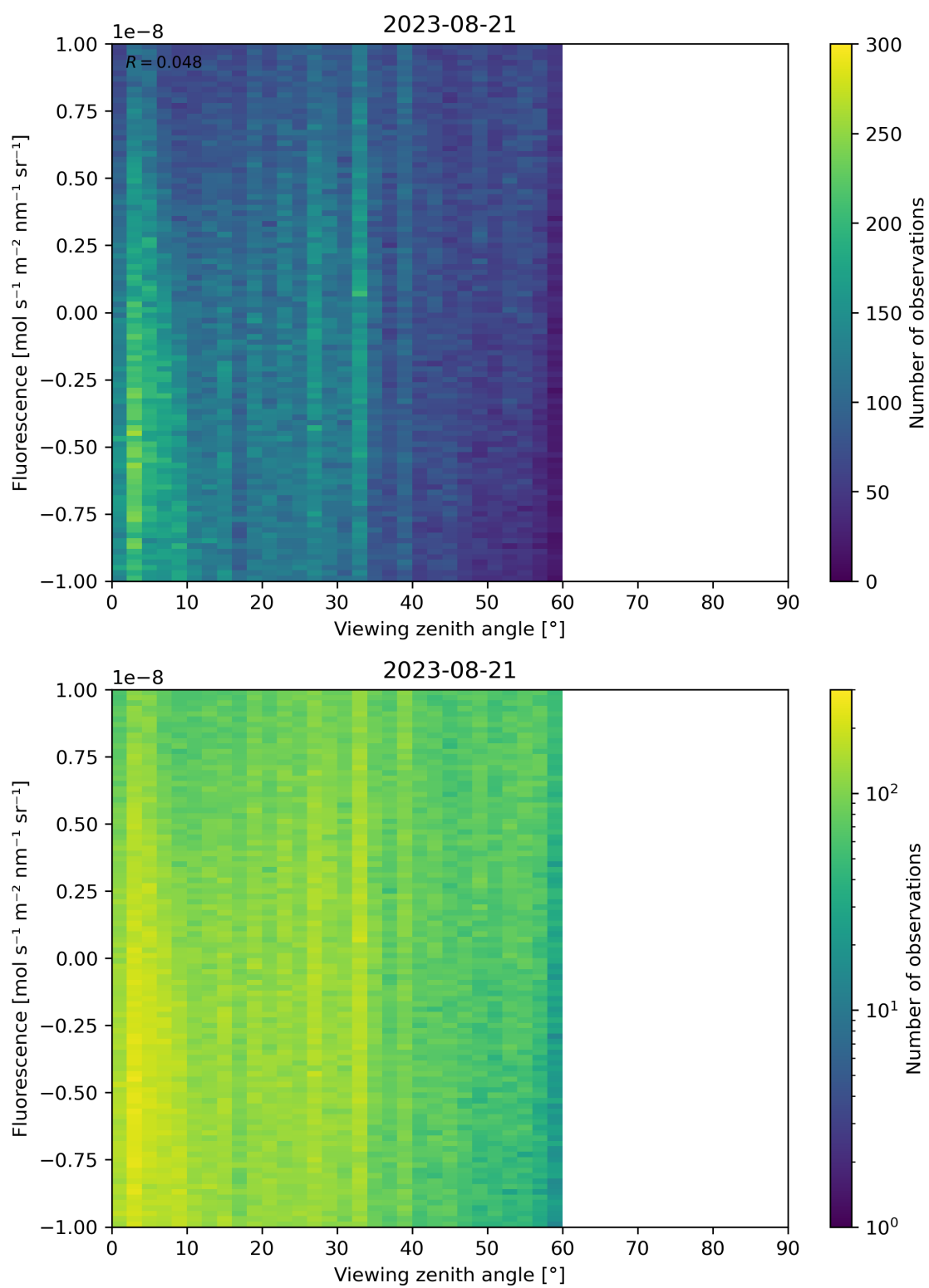
Figure 108: Scatter density plot of “Viewing zenith angle” against “Fluorescence” for 2023-08-20 to 2023-08-22.
