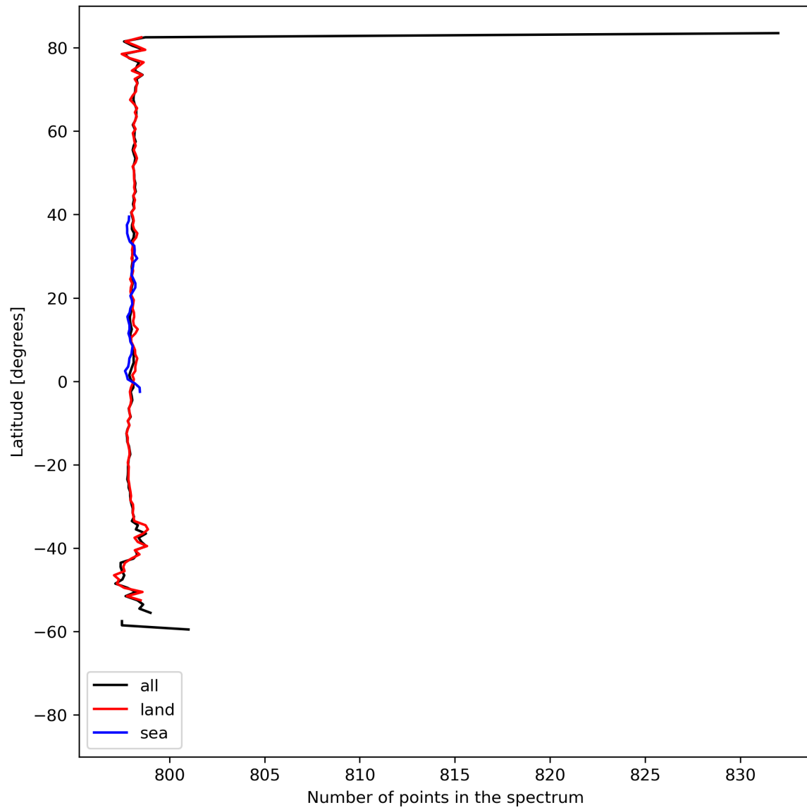
Figure 15: Zonal average of “Number of points in the spectrum” for 2023-08-20 to 2023-08-22.
