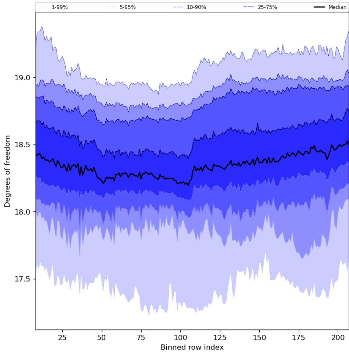
Figure 41: Along track statistics of “Degrees of freedom” for 2023-08-20 to 2023-08-22
