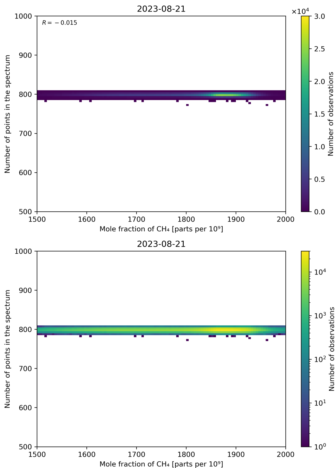
Figure 77: Scatter density plot of “Mole fraction of CH 4 ” against “Number of points in the spectrum” for 2023-08-20 to 2023-08-22.
