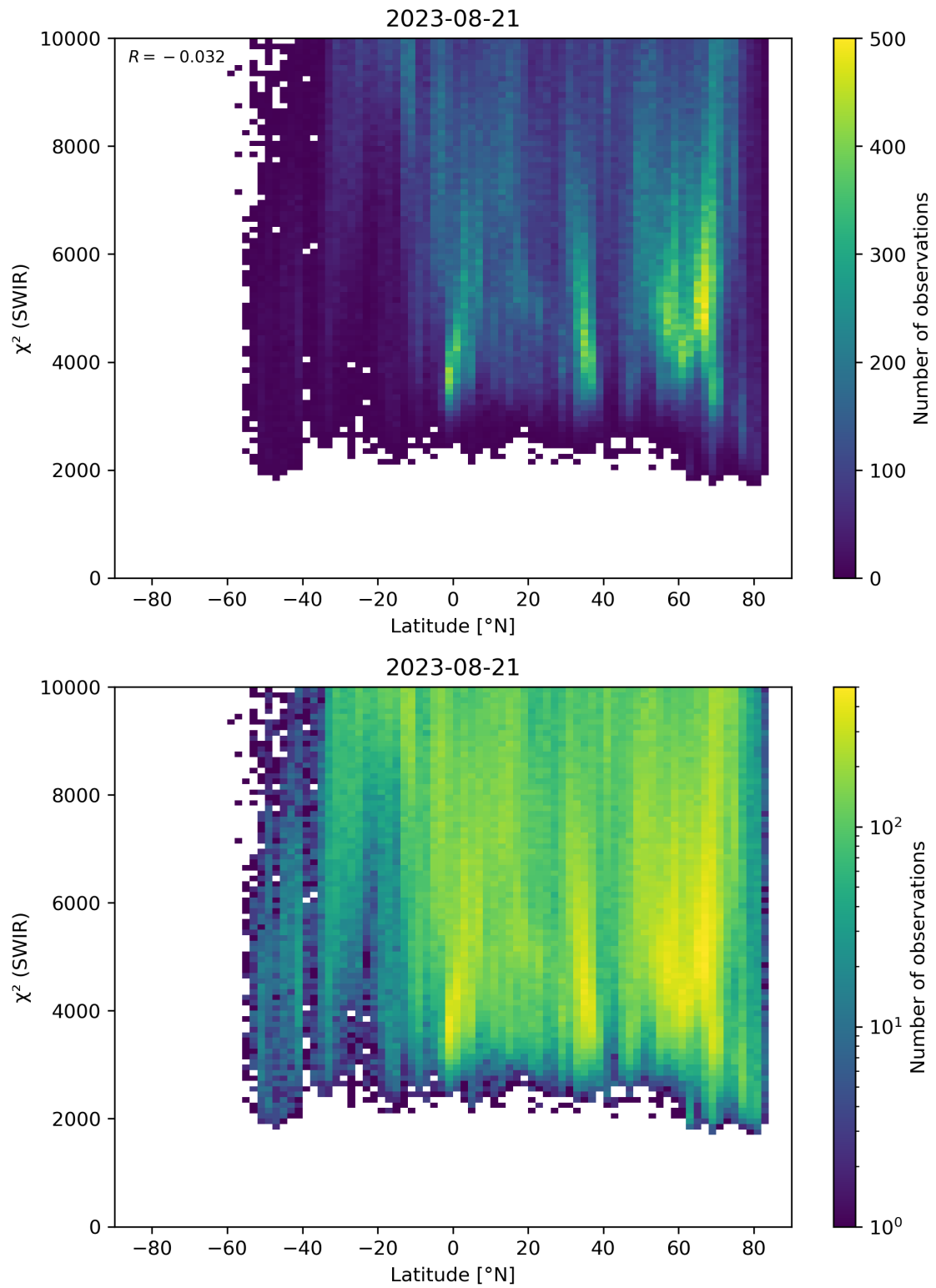
Figure 54: Scatter density plot of “Latitude” against “ \chi^2 (SWIR)” for 2023-08-20 to 2023-08-22.
