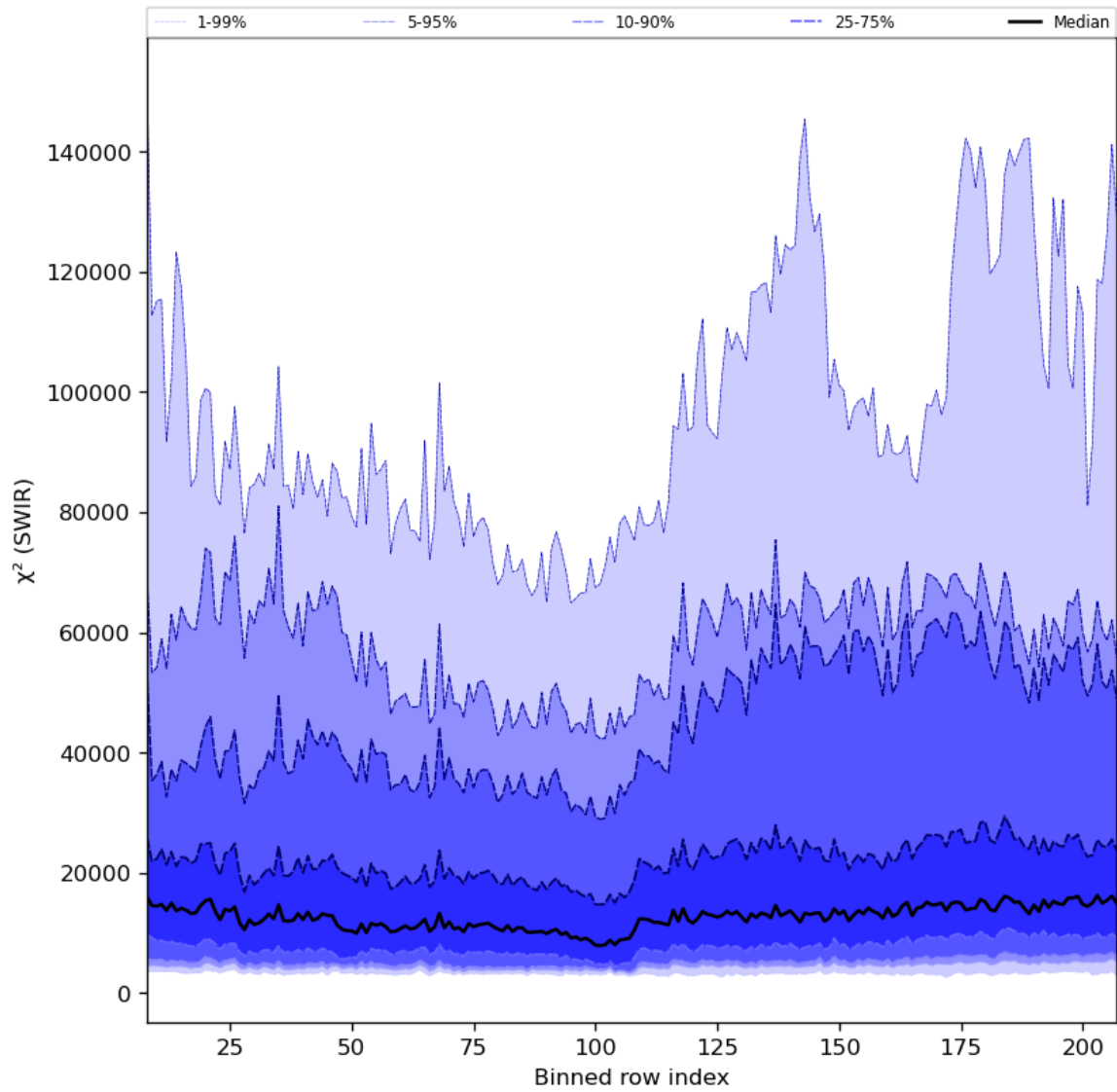
Figure 39: Along track statistics of “ \chi^2 (SWIR)” for 2023-08-20 to 2023-08-22
