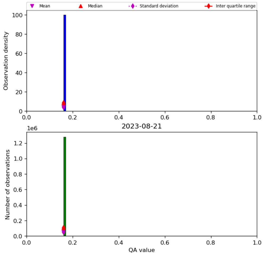
Figure 22: Histogram of “QA value” for 2023-08-20 to 2023-08-22
