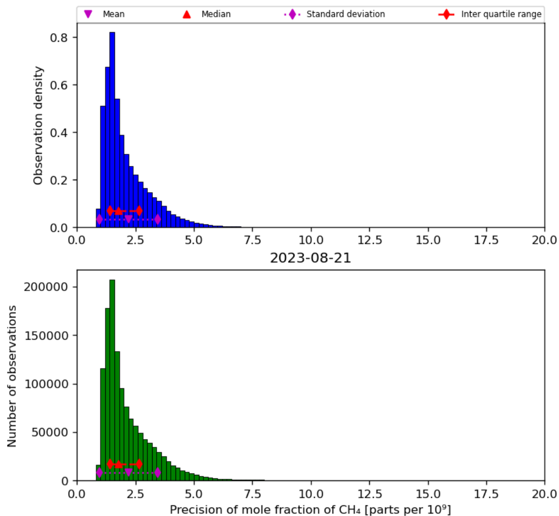
Figure 24: Histogram of “Precision of mole fraction of CH 4 ” for 2023-08-20 to 2023-08-22
