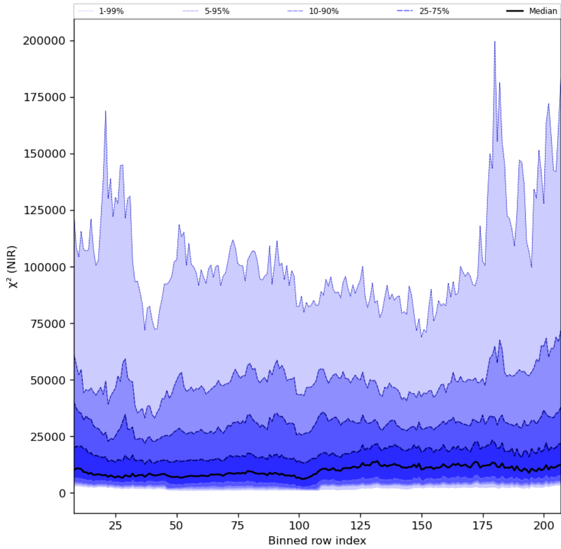
Figure 40: Along track statistics of “ \chi^2 (NIR)” for 2023-08-20 to 2023-08-22
