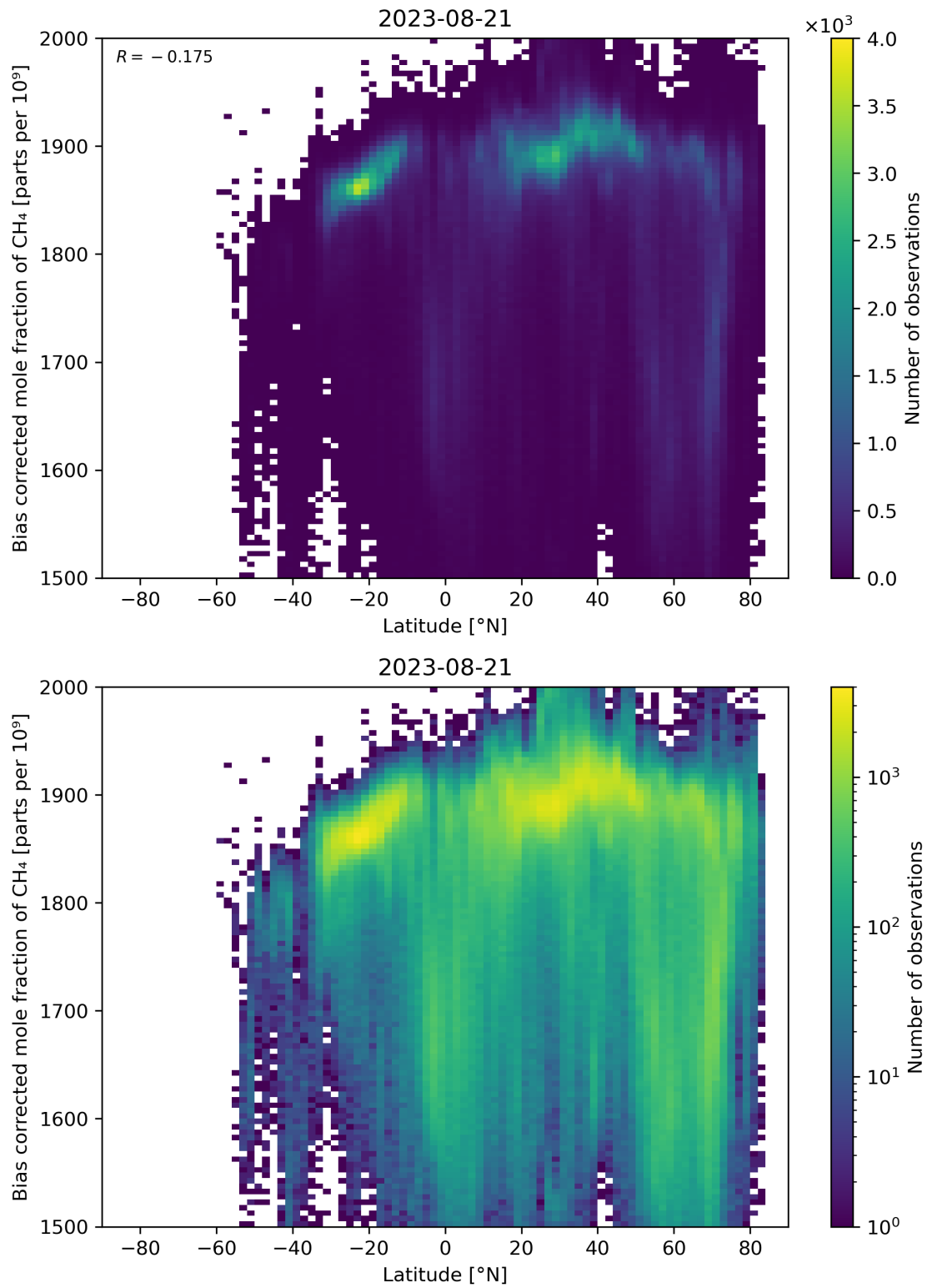
Figure 58: Scatter density plot of “Latitude” against “Bias corrected mole fraction of \text{CH}_4 ” for 2023-08-20 to 2023-08-22.
