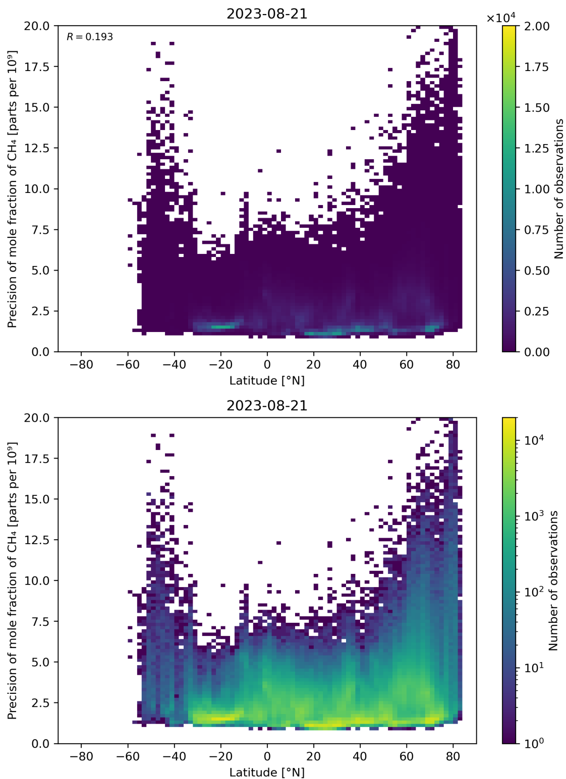
Figure 59: Scatter density plot of “Latitude” against “Precision of mole fraction of \text{CH}_4 ” for 2023-08-20 to 2023-08-22.
