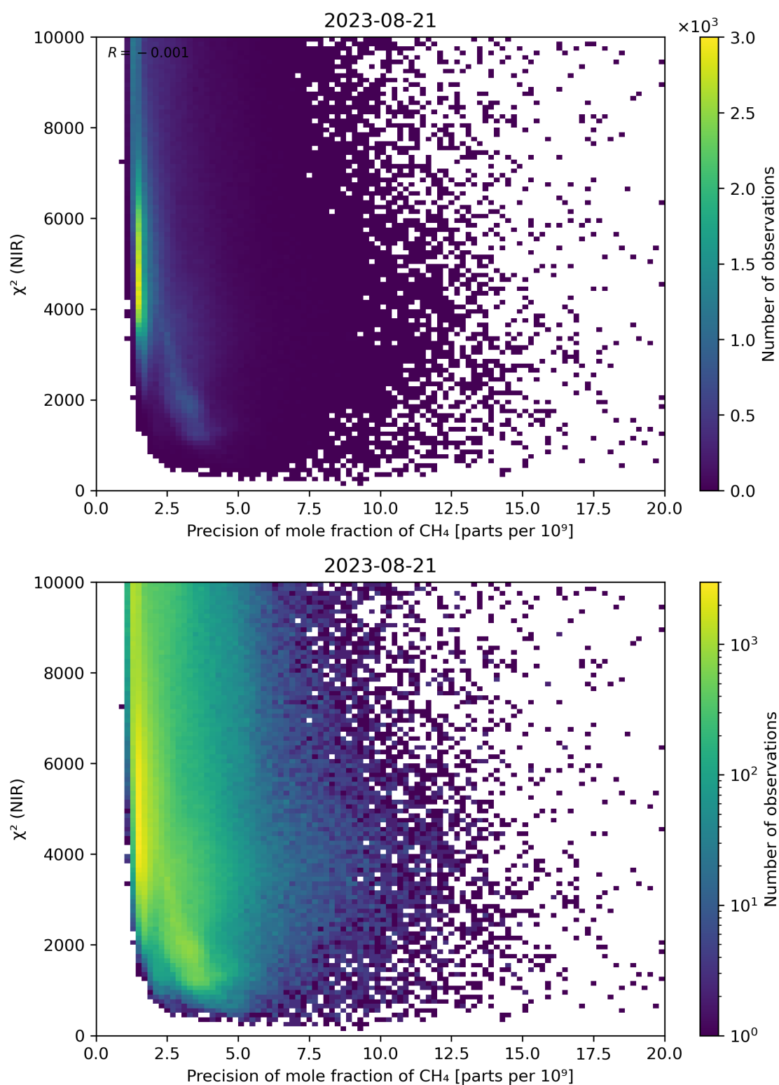
Figure 78: Scatter density plot of “Precision of mole fraction of CH 4 ” against “ \chi^2 (NIR)” for 2023-08-20 to 2023-08-22.
