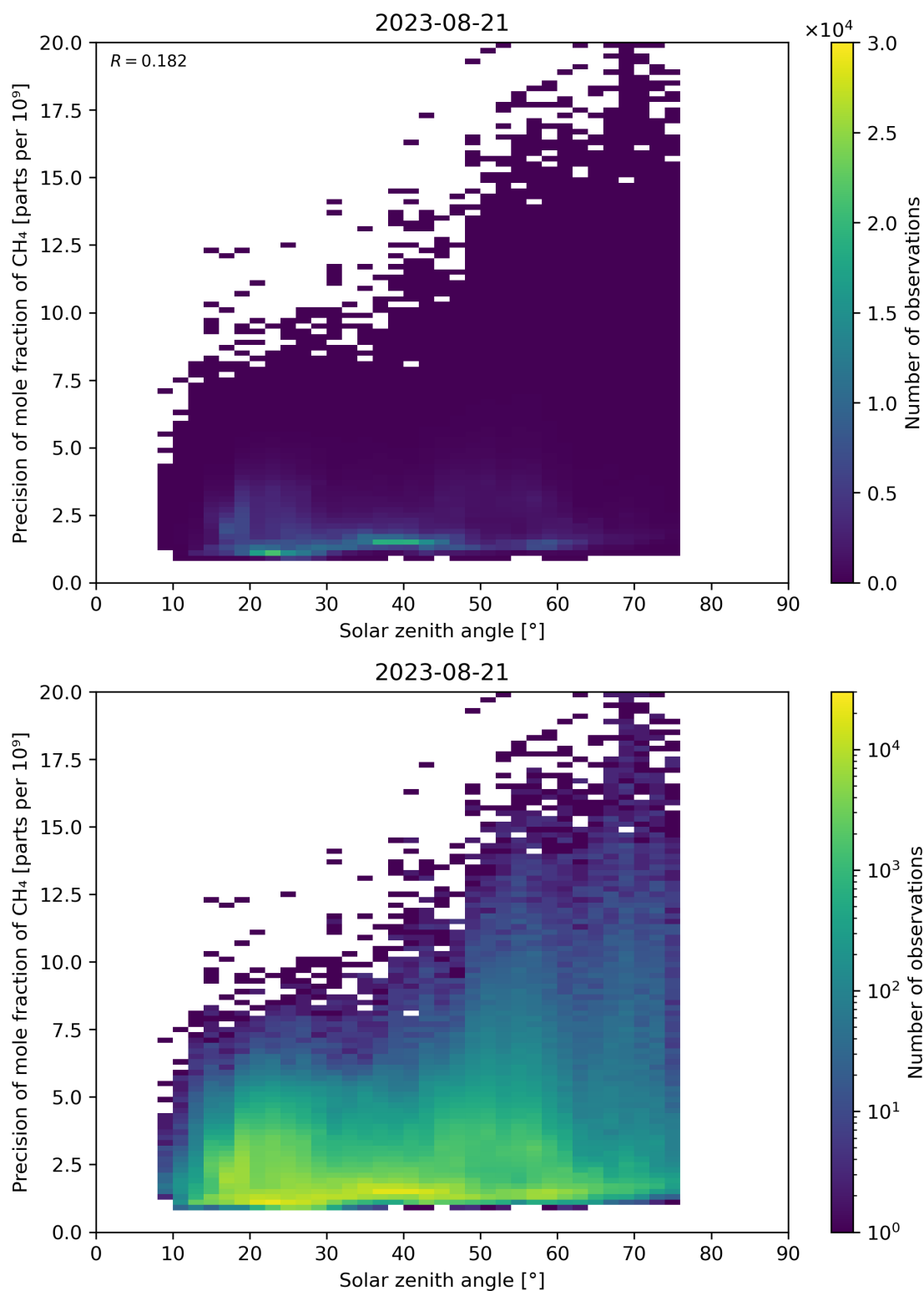
Figure 101: Scatter density plot of “Solar zenith angle” against “Precision of mole fraction of CH 4 ” for 2023-08-20 to 2023-08-22.
