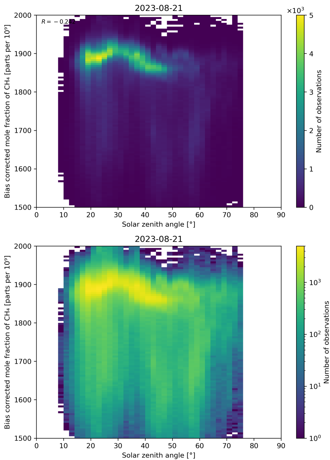
Figure 100: Scatter density plot of “Solar zenith angle” against “Bias corrected mole fraction of CH 4 ” for 2023-08-20 to 2023-08-22.
