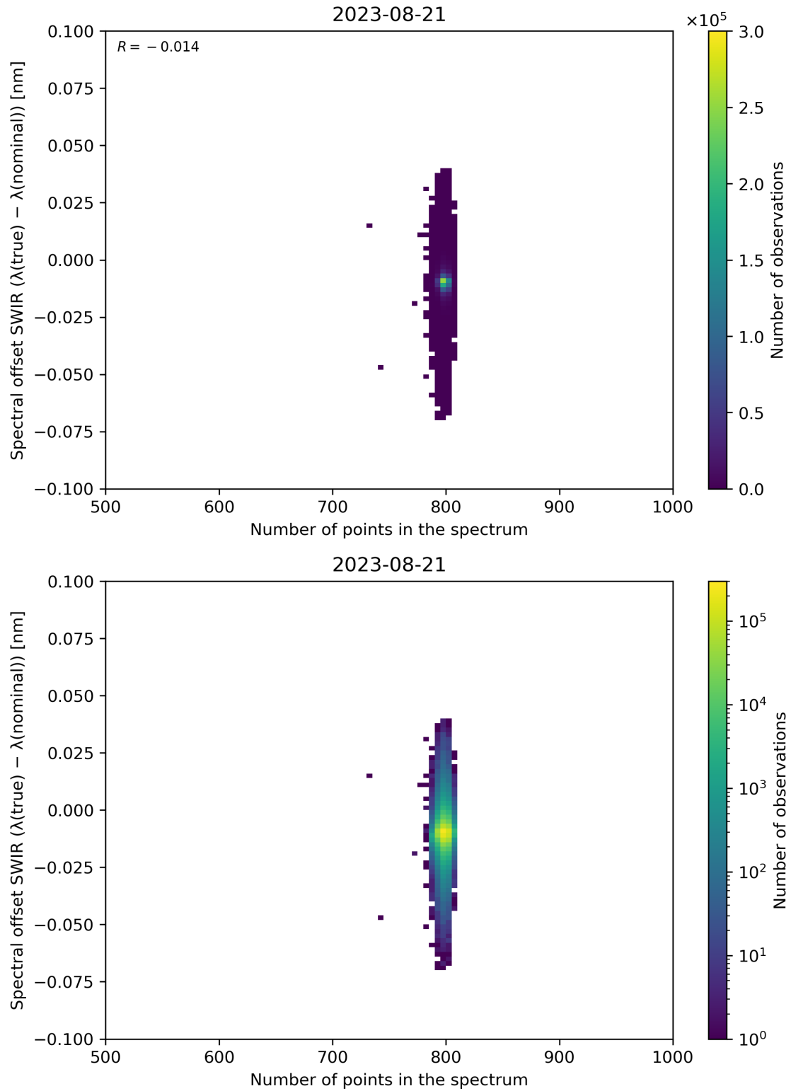
Figure 93: Scatter density plot of “Number of points in the spectrum” against “Spectral offset SWIR ( \lambda(\text{true}) - \lambda(\text{nominal}) )” for 2023-08-20 to 2023-08-22.
