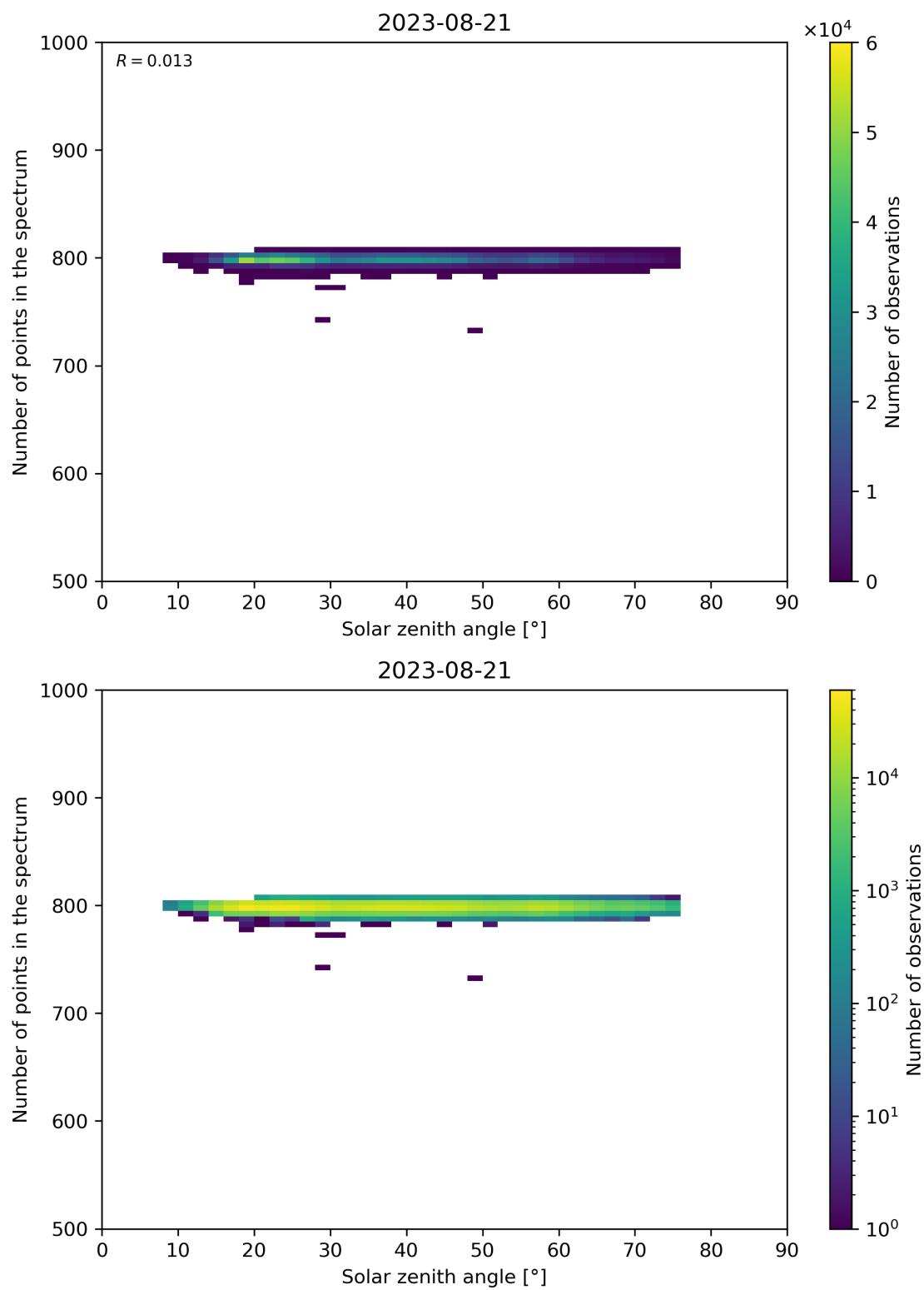
Figure 103: Scatter density plot of “Solar zenith angle” against “Number of points in the spectrum” for 2023-08-20 to 2023-08-22.
