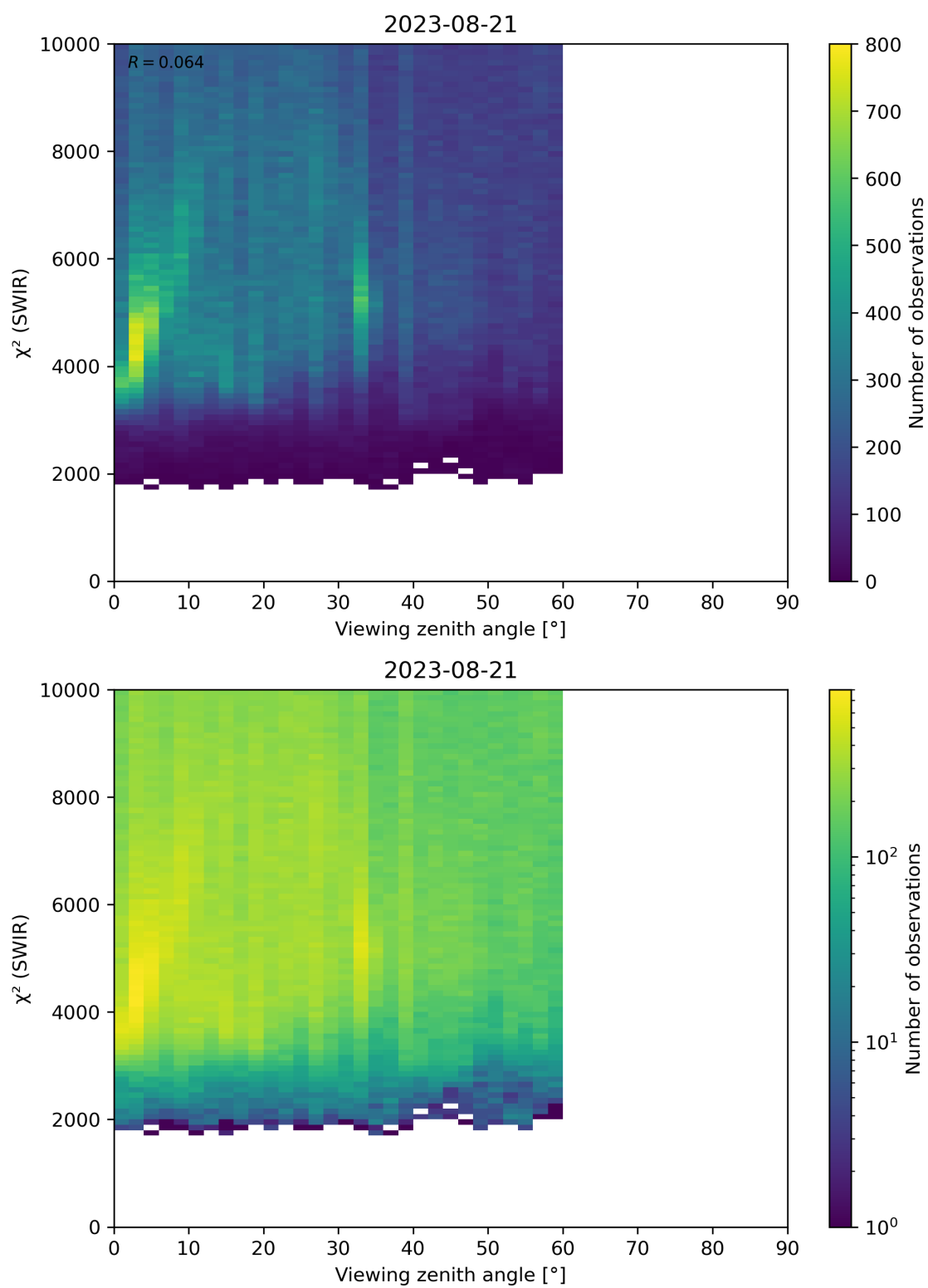
Figure 106: Scatter density plot of “Viewing zenith angle” against “ \chi^2 (SWIR)” for 2023-08-20 to 2023-08-22.
