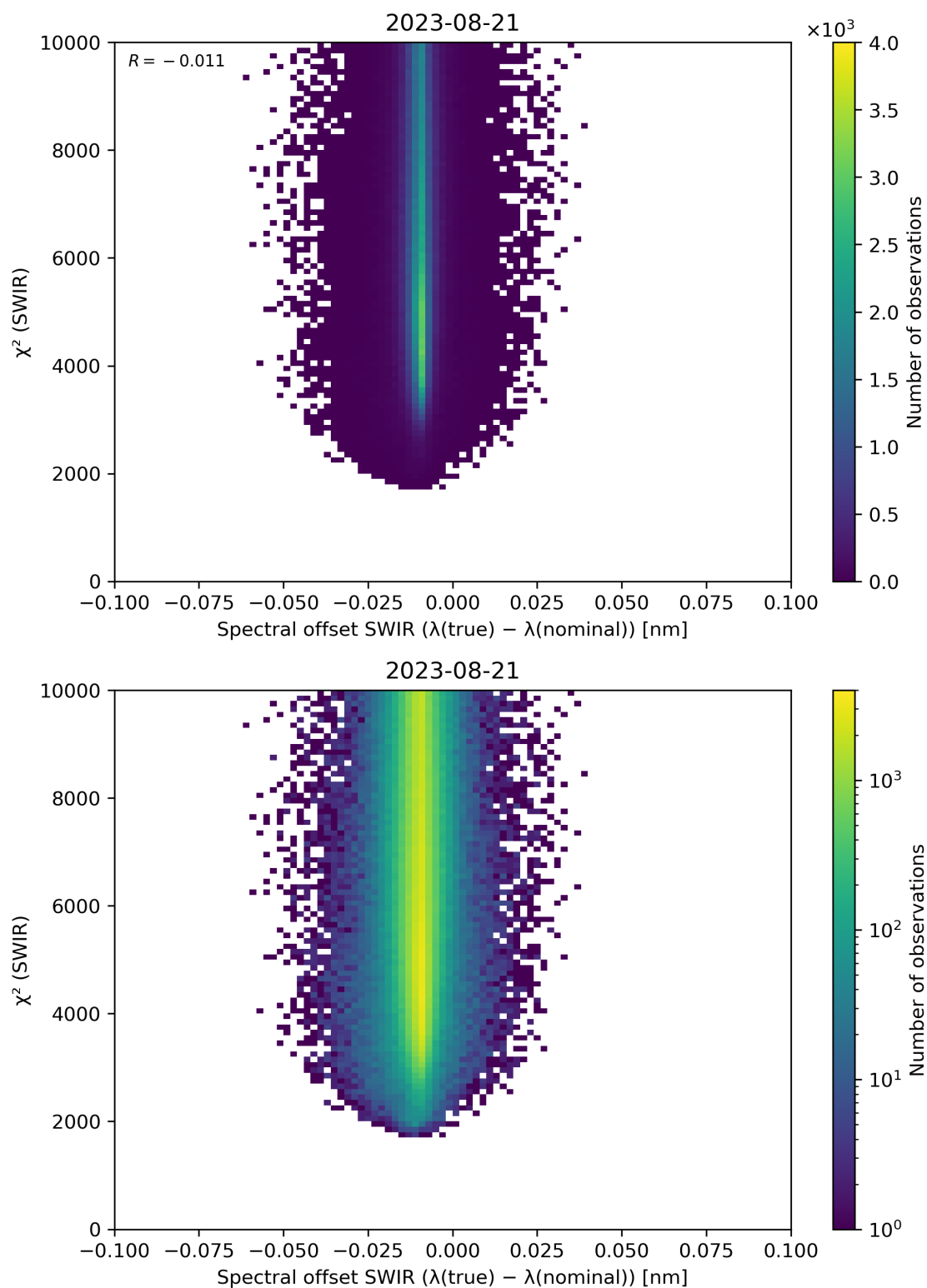
Figure 118: Scatter density plot of “Spectral offset SWIR ( \lambda(\text{true}) - \lambda(\text{nominal}) )” against “ \chi^2 (SWIR)” for 2023-08-20 to 2023-08-22.
