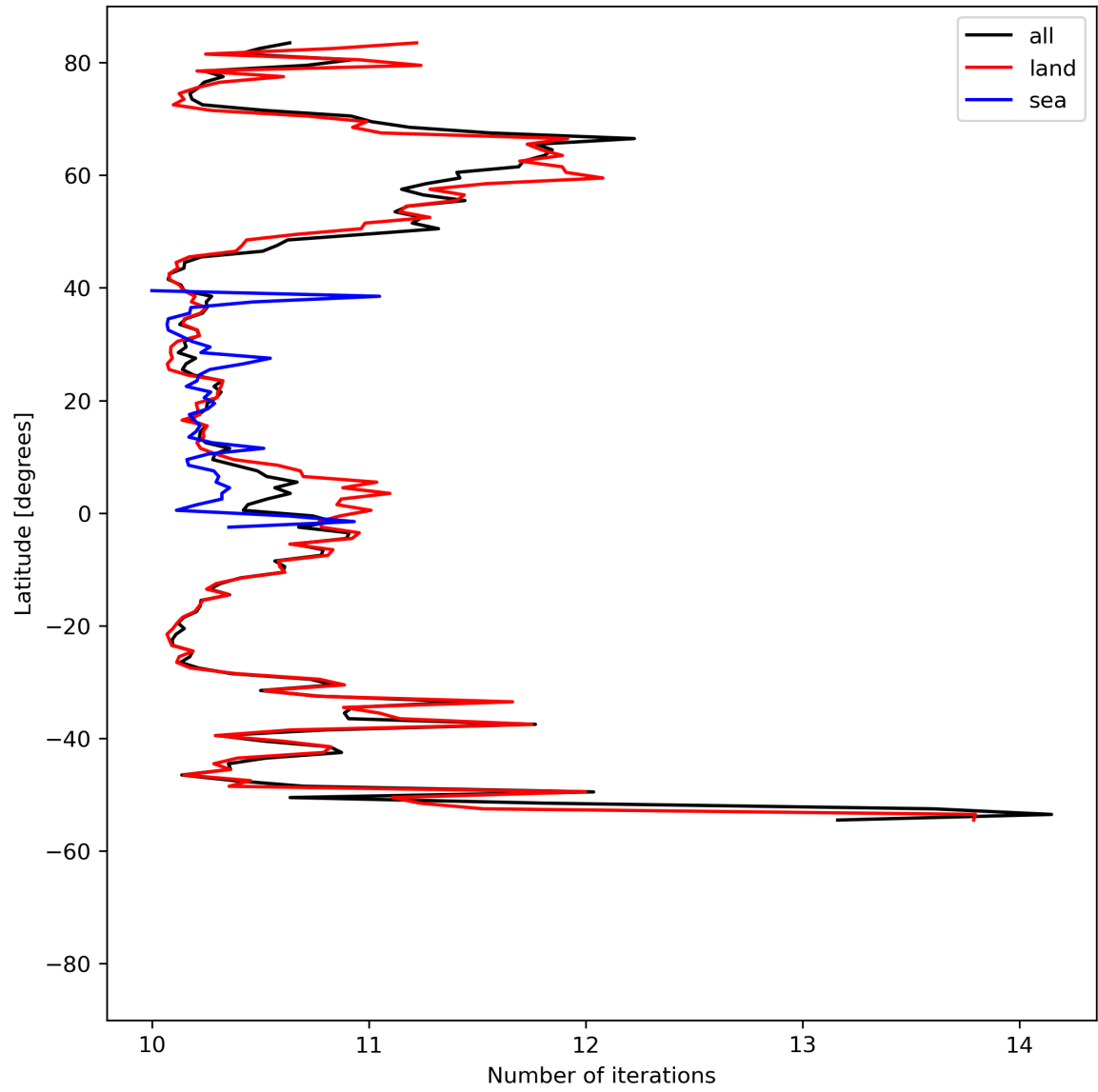
Figure 20: Zonal average of “Number of iterations” for 2023-08-21 to 2023-08-23.
