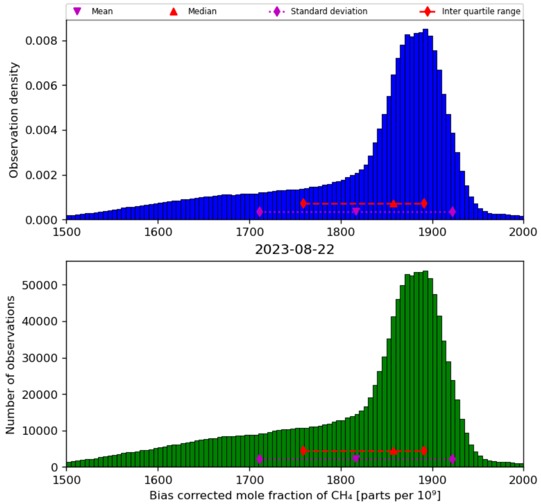
Figure 25: Histogram of “Bias corrected mole fraction of CH 4 ” for 2023-08-21 to 2023-08-23
