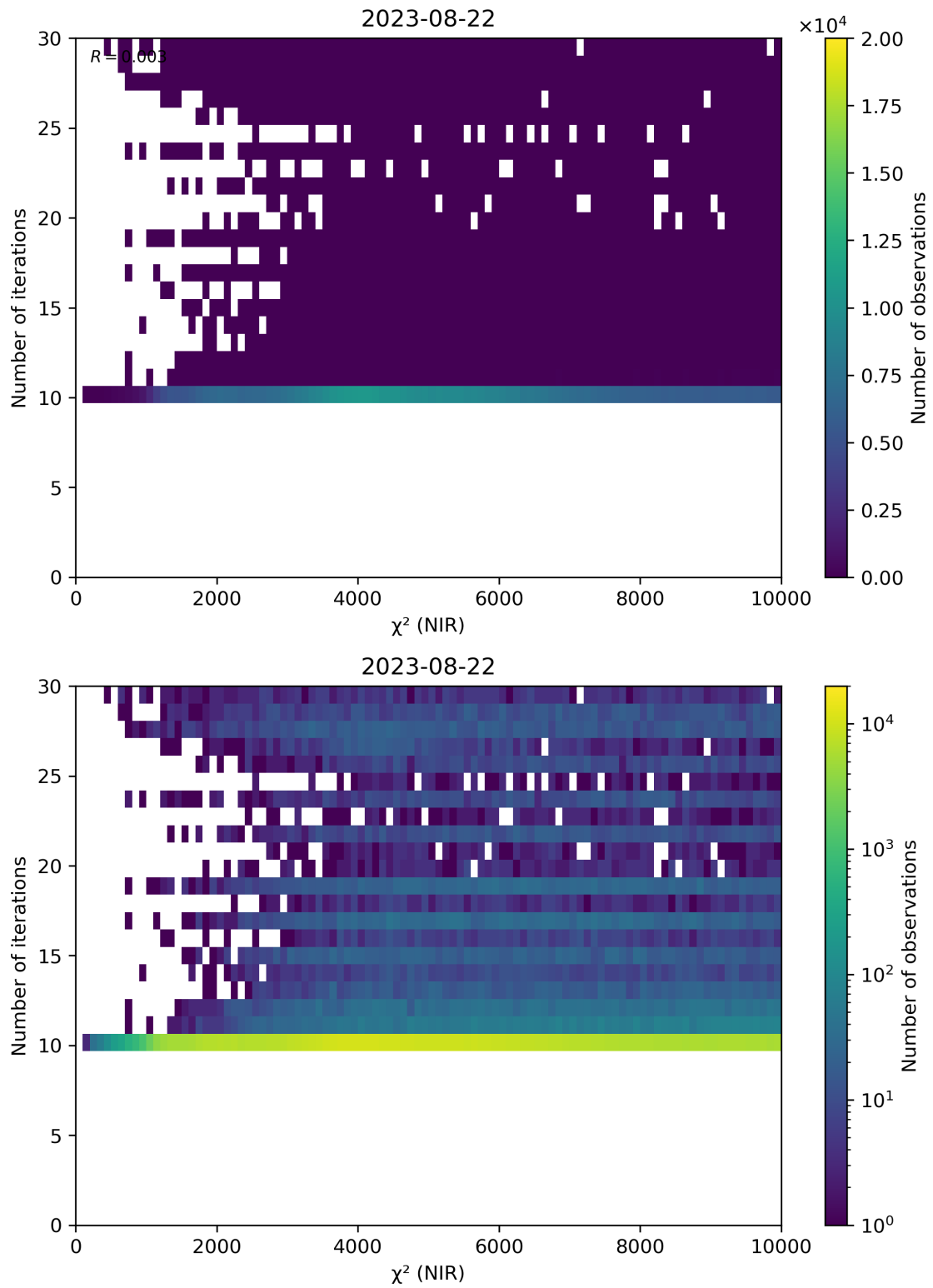
Figure 46: Scatter density plot of “ \chi^2 (NIR)” against “Number of iterations” for 2023-08-21 to 2023-08-23.
