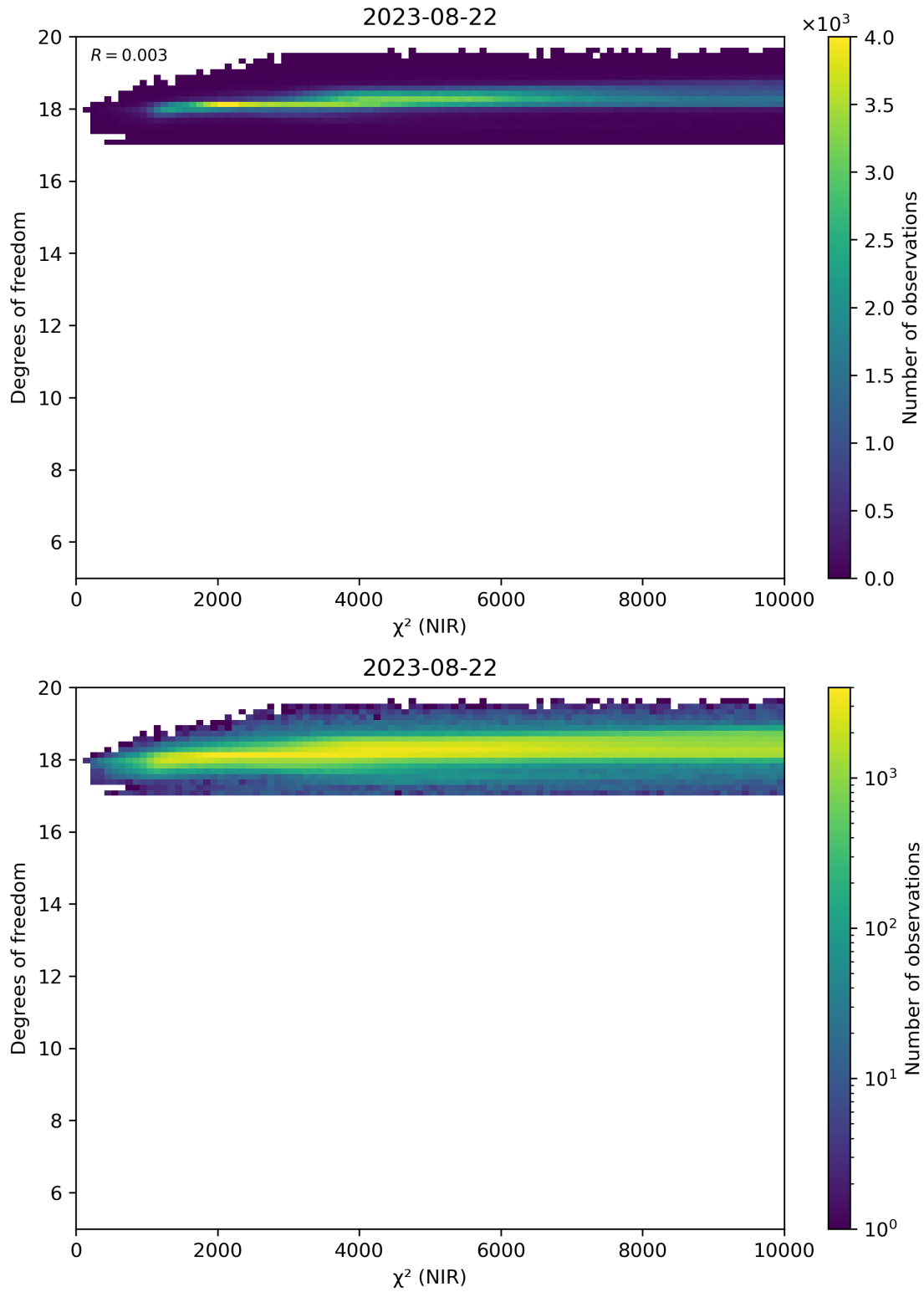
Figure 44: Scatter density plot of “ \chi^2 (NIR)” against “Degrees of freedom” for 2023-08-21 to 2023-08-23.
