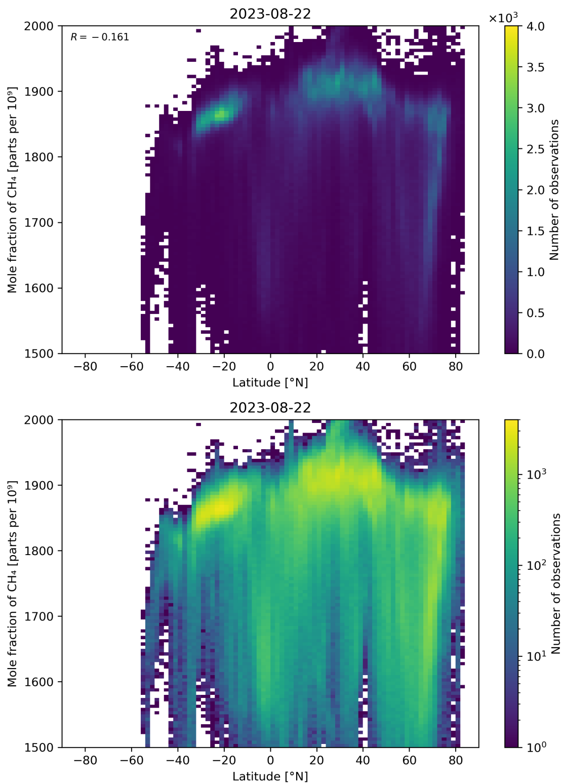
Figure 57: Scatter density plot of “Latitude” against “Mole fraction of \text{CH}_4 ” for 2023-08-21 to 2023-08-23.
