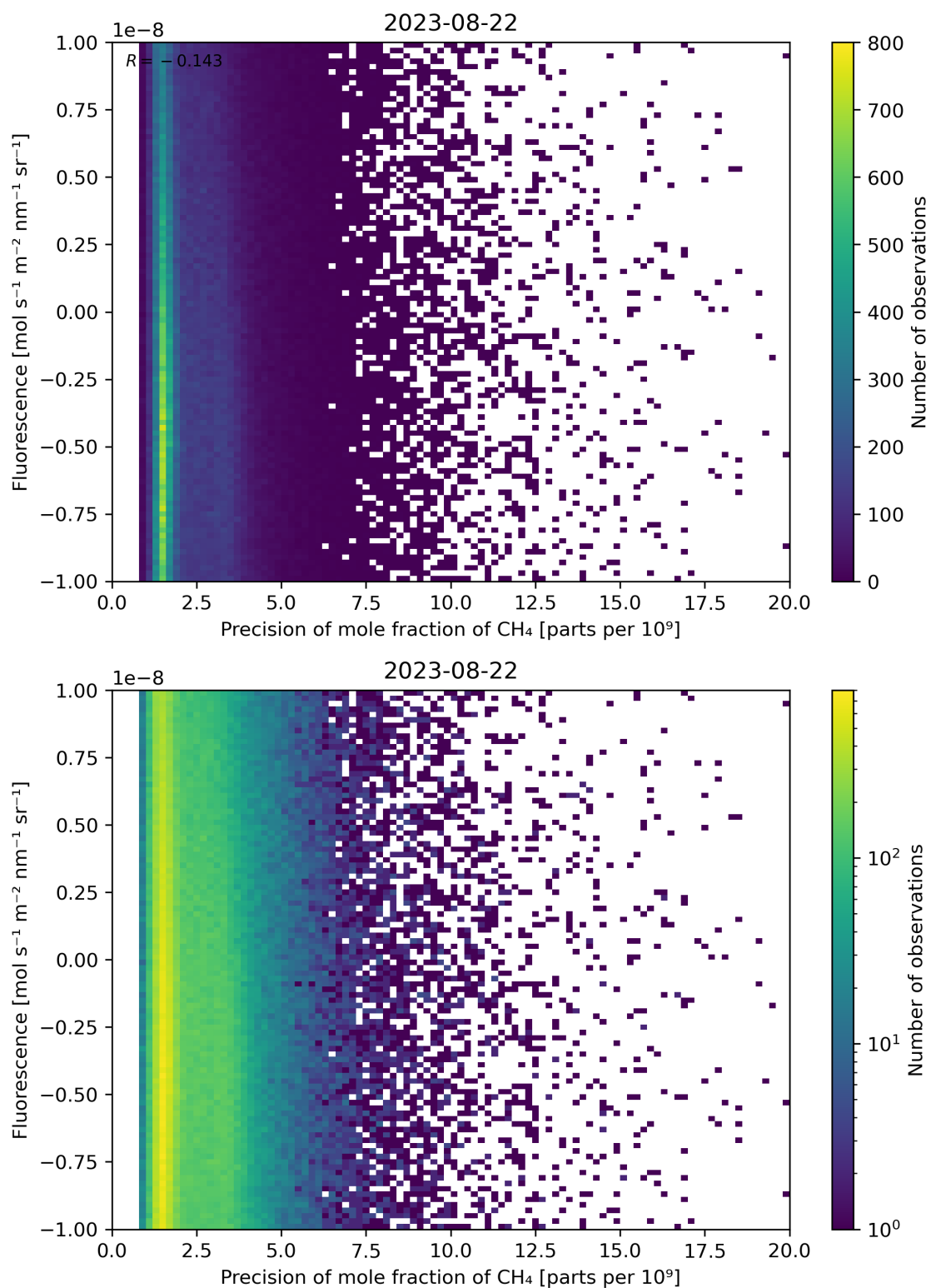
Figure 81: Scatter density plot of “Precision of mole fraction of \text{CH}_4 ” against “Fluorescence” for 2023-08-21 to 2023-08-23.
