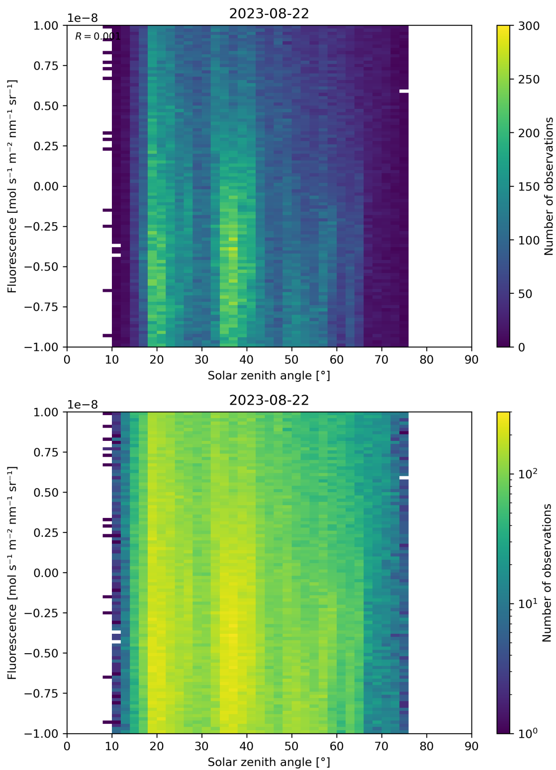
Figure 97: Scatter density plot of “Solar zenith angle” against “Fluorescence” for 2023-08-21 to 2023-08-23.
