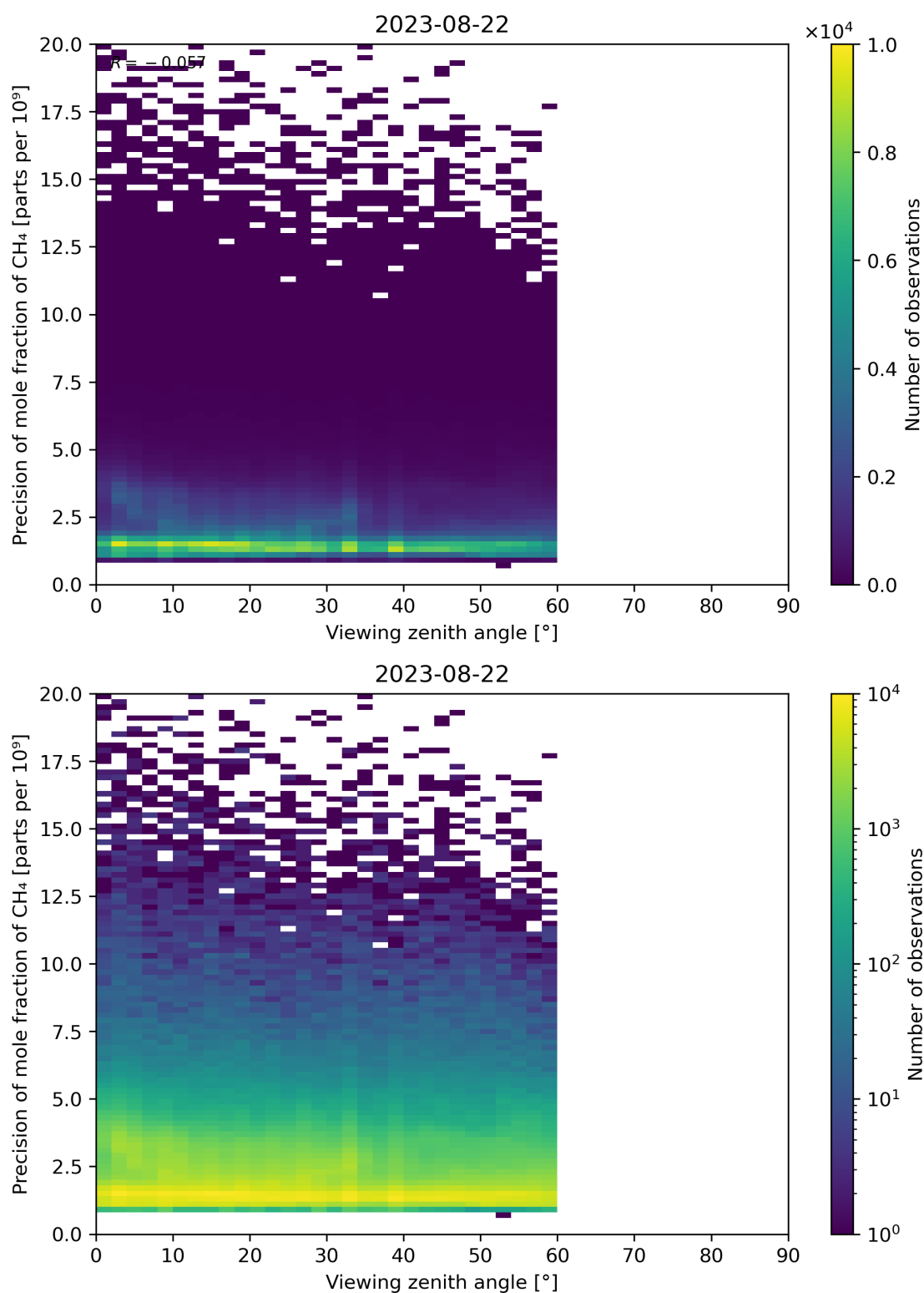
Figure 112: Scatter density plot of “Viewing zenith angle” against “Precision of mole fraction of CH 4 ” for 2023-08-21 to 2023-08-23.
