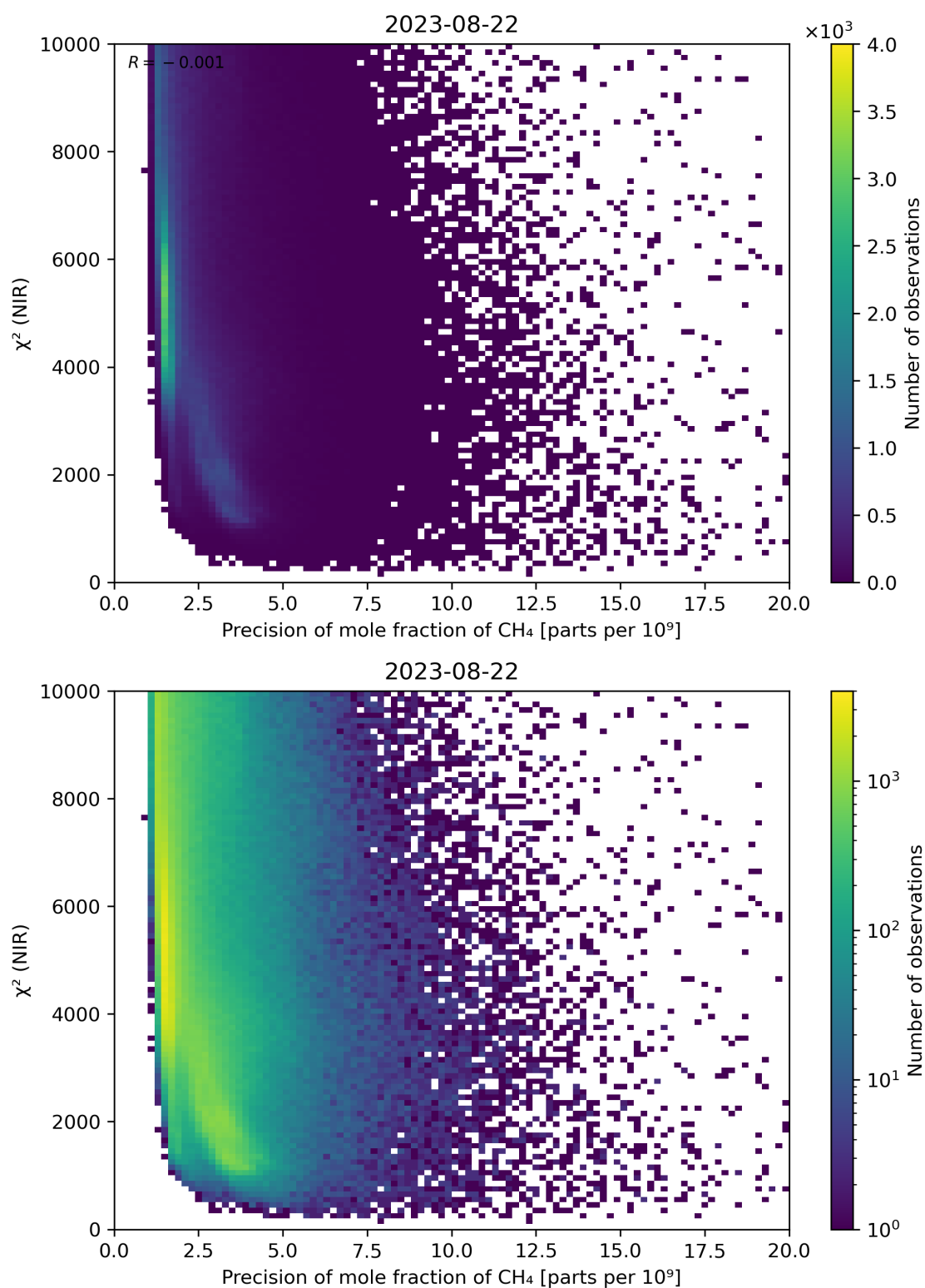
Figure 78: Scatter density plot of “Precision of mole fraction of CH 4 ” against “ \chi^2 (NIR)” for 2023-08-21 to 2023-08-23.
