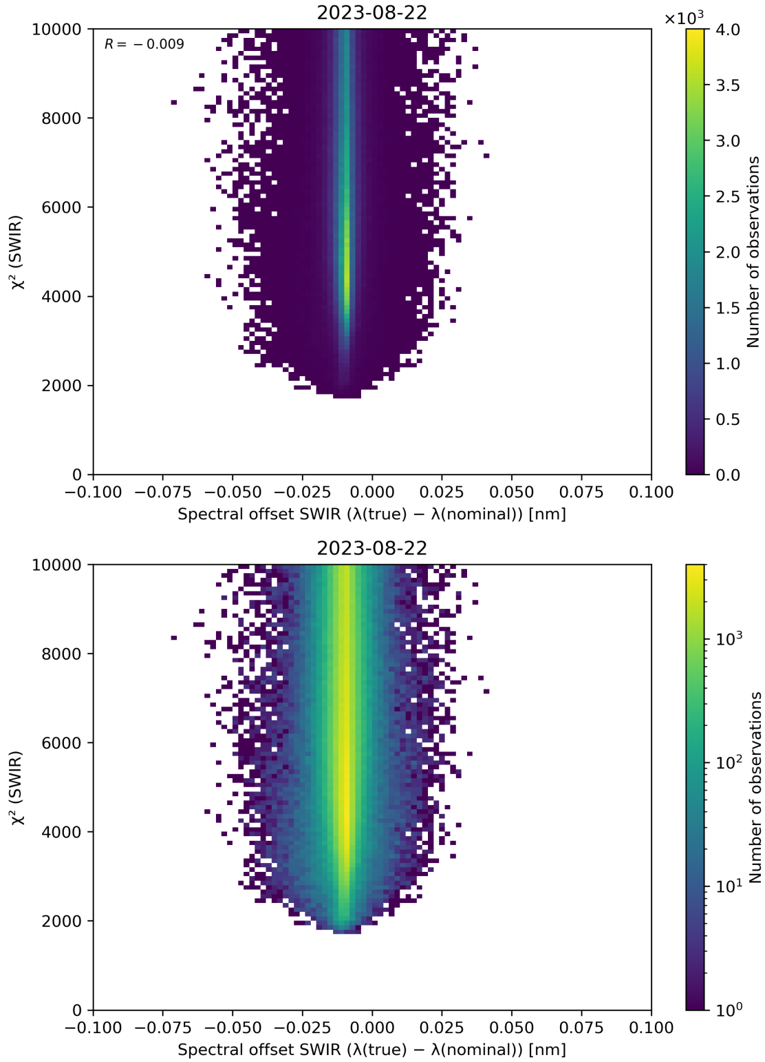
Figure 118: Scatter density plot of “Spectral offset SWIR ( \lambda(\text{true}) - \lambda(\text{nominal}) )” against “ \chi^2 (SWIR)” for 2023-08-21 to 2023-08-23.
