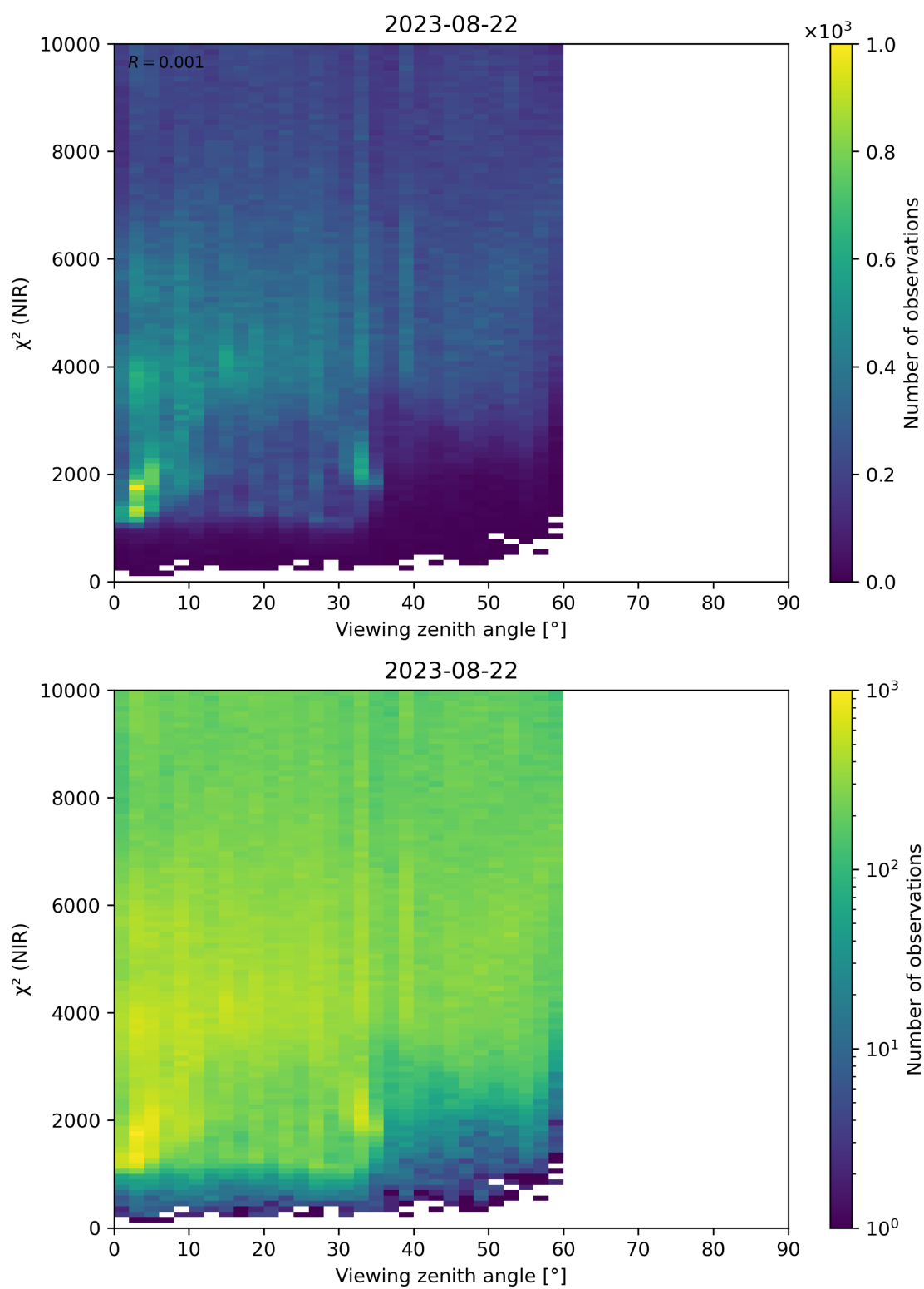
Figure 105: Scatter density plot of “Viewing zenith angle” against “ \chi^2 (NIR)” for 2023-08-21 to 2023-08-23.
