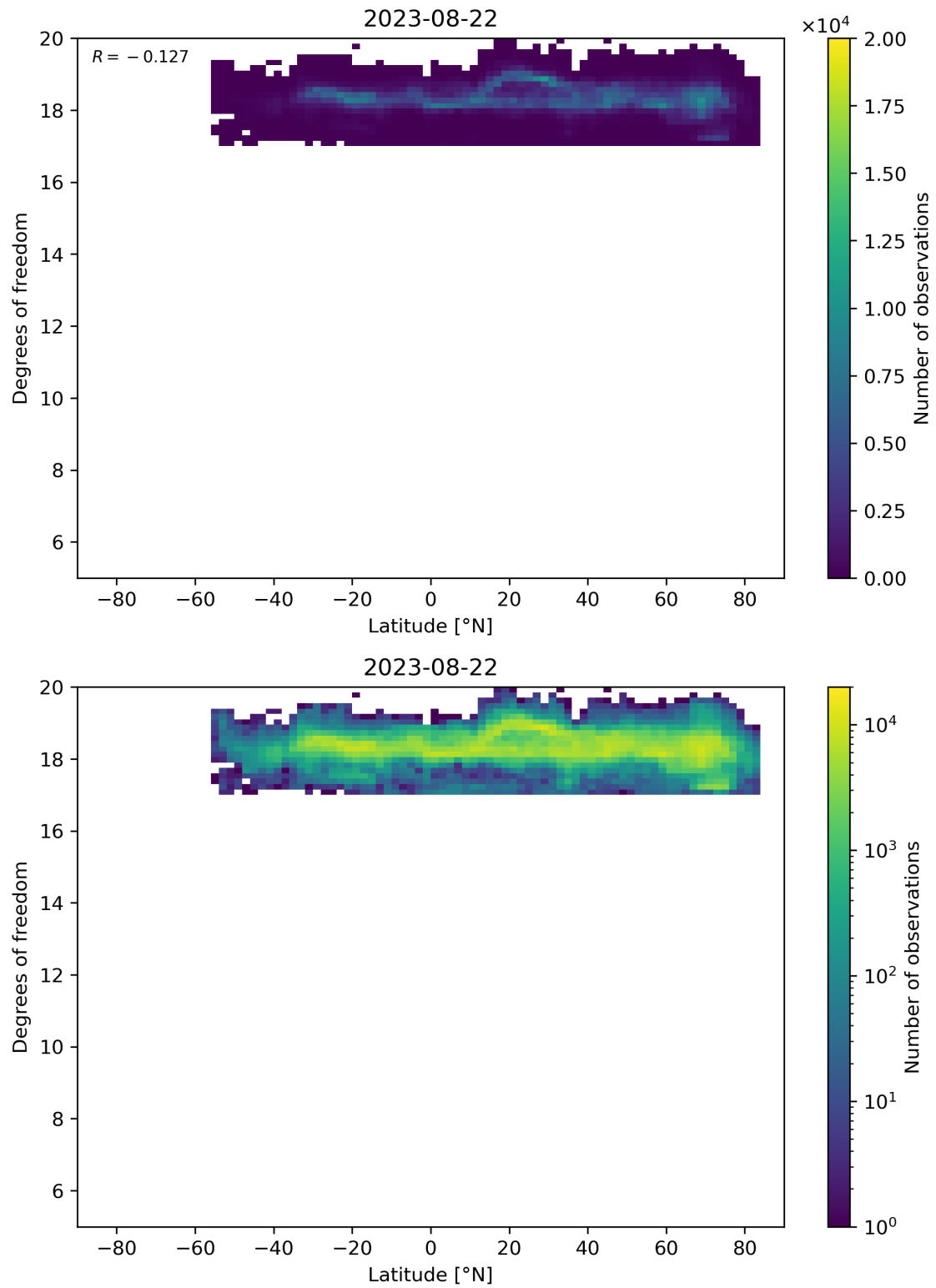
Figure 55: Scatter density plot of “Latitude” against “Degrees of freedom” for 2023-08-21 to 2023-08-23.
