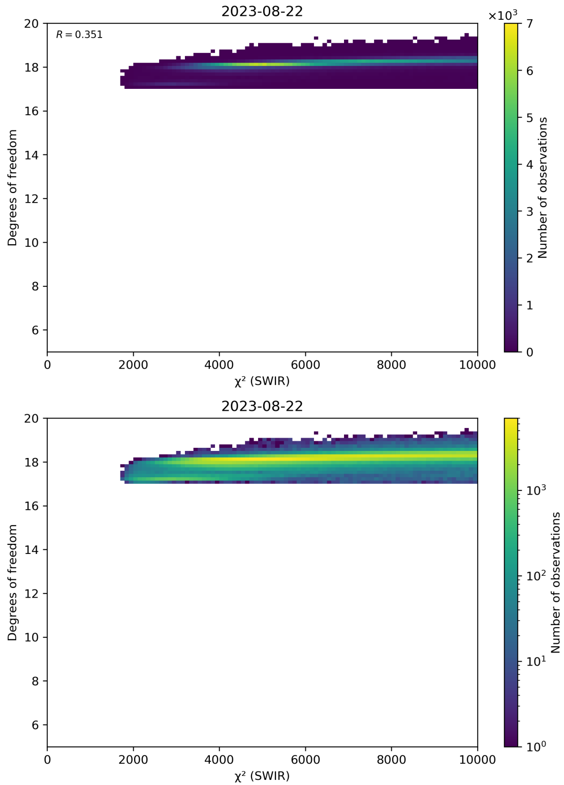
Figure 48: Scatter density plot of “ \chi^2 (SWIR)” against “Degrees of freedom” for 2023-08-21 to 2023-08-23.
