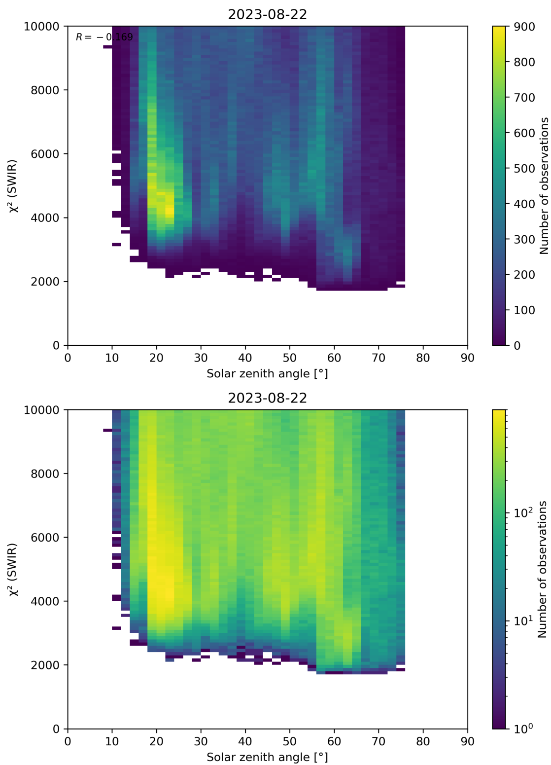
Figure 95: Scatter density plot of “Solar zenith angle” against “ \chi^2 (SWIR)” for 2023-08-21 to 2023-08-23.
