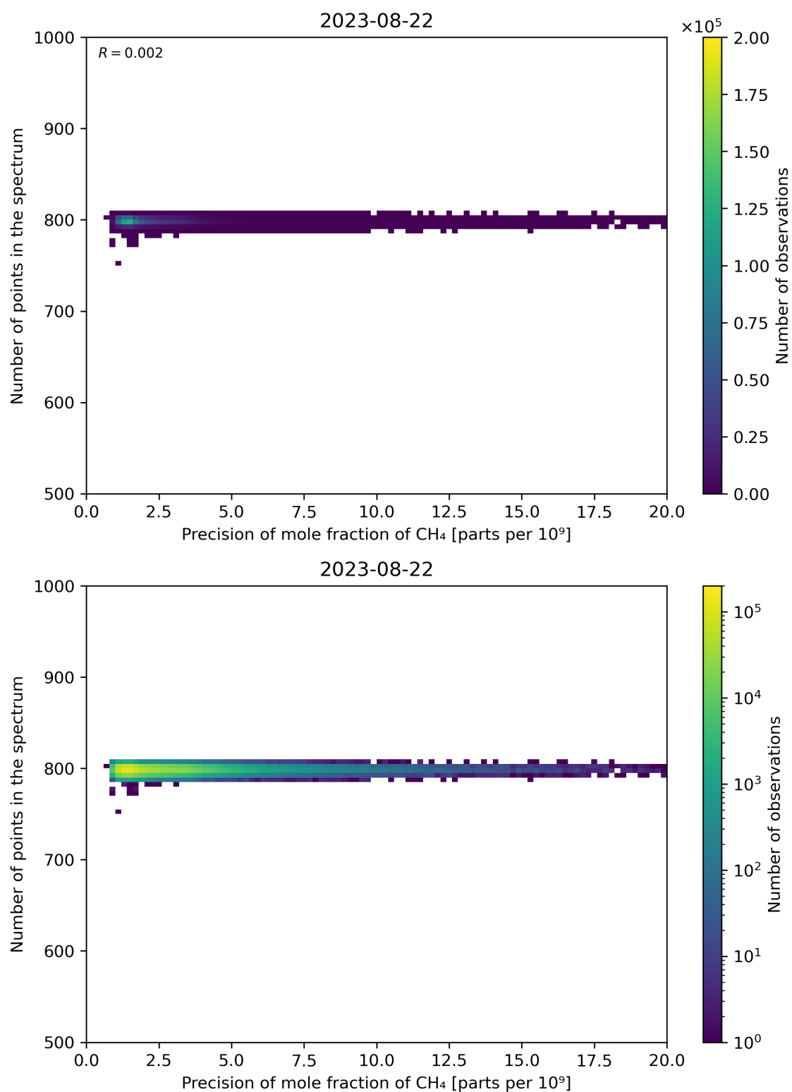
Figure 84: Scatter density plot of “Precision of mole fraction of CH 4 ” against “Number of points in the spectrum” for 2023-08-21 to 2023-08-23.
