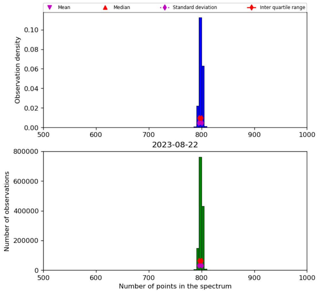
Figure 26: Histogram of “Number of points in the spectrum” for 2023-08-21 to 2023-08-23
