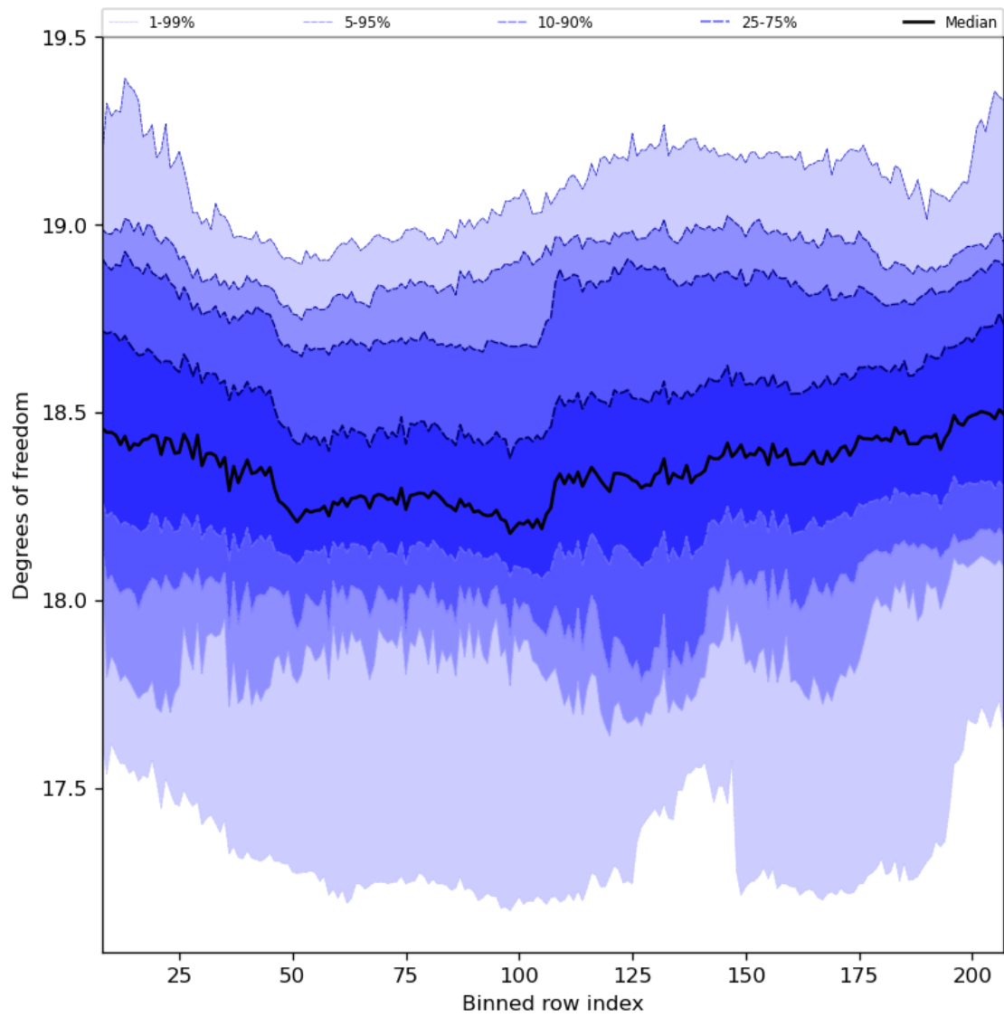
Figure 41: Along track statistics of “Degrees of freedom” for 2023-08-21 to 2023-08-23
