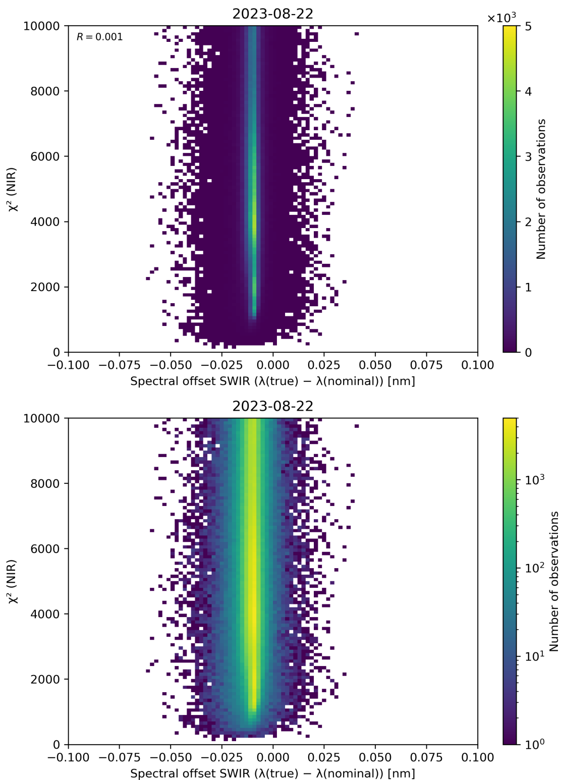
Figure 117: Scatter density plot of “Spectral offset SWIR ( \lambda(\text{true}) - \lambda(\text{nominal}) )” against “ \chi^2 (NIR)” for 2023-08-21 to 2023-08-23.
