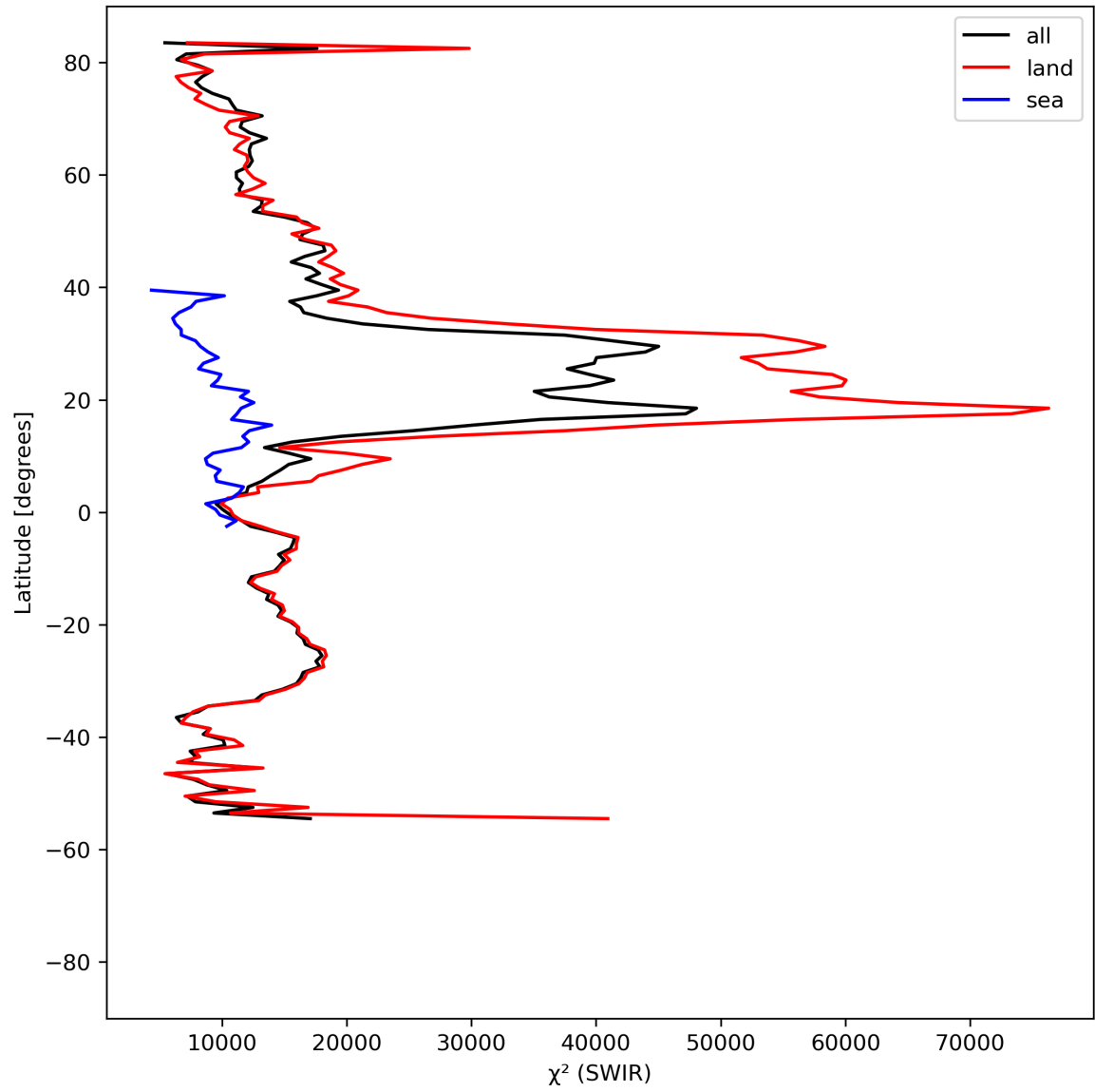
Figure 17: Zonal average of “ \chi^2 (SWIR)” for 2023-08-21 to 2023-08-23.
