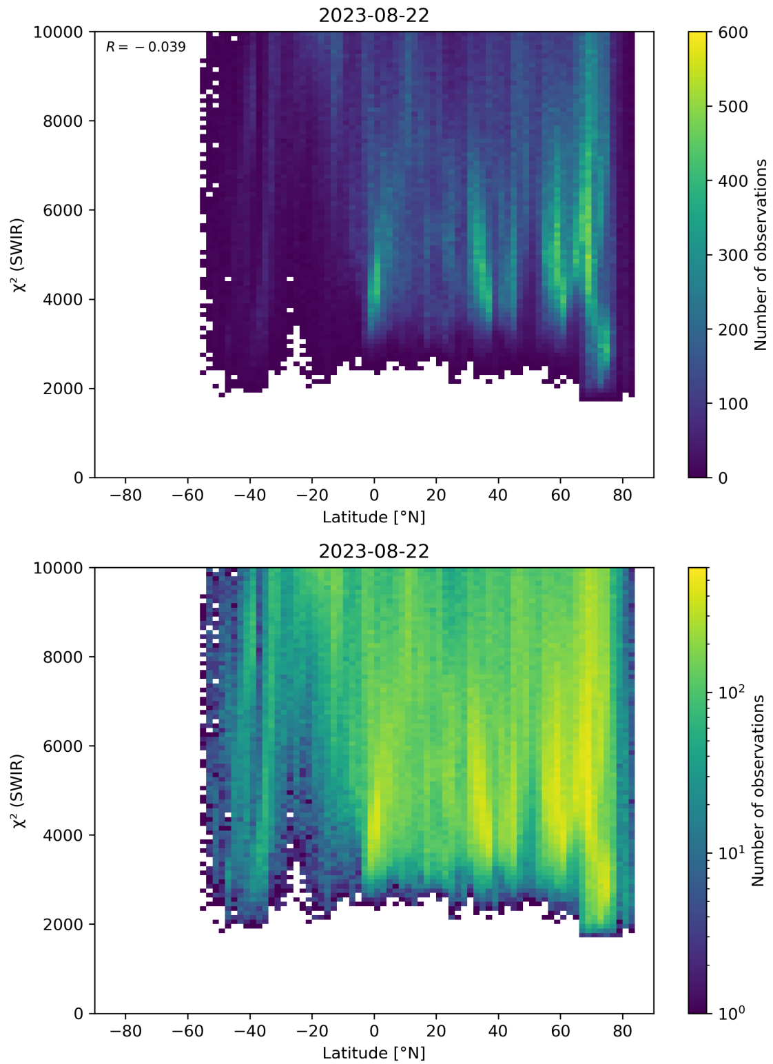
Figure 54: Scatter density plot of “Latitude” against “ \chi^2 (SWIR)” for 2023-08-21 to 2023-08-23.
