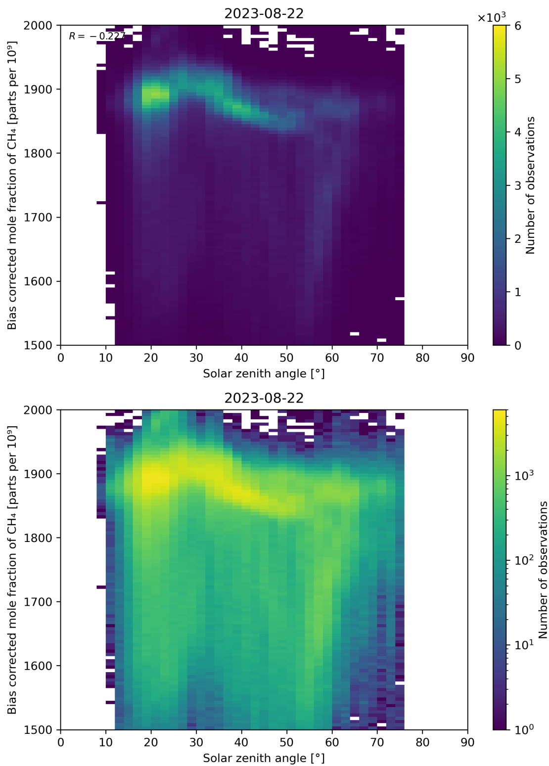
Figure 100: Scatter density plot of “Solar zenith angle” against “Bias corrected mole fraction of CH 4 ” for 2023-08-21 to 2023-08-23.
