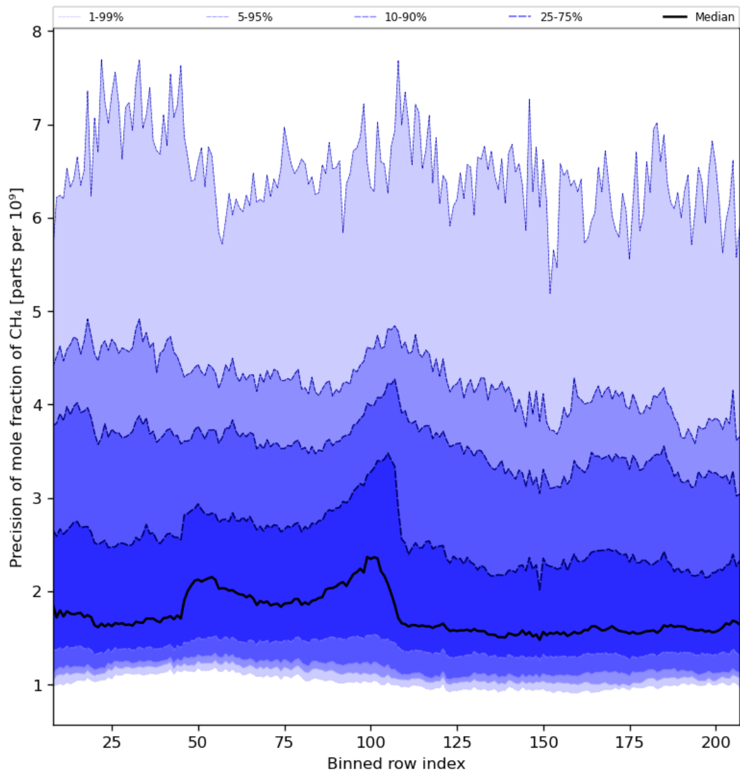
Figure 35: Along track statistics of “Precision of mole fraction of CH 4 ” for 2023-08-21 to 2023-08-23
