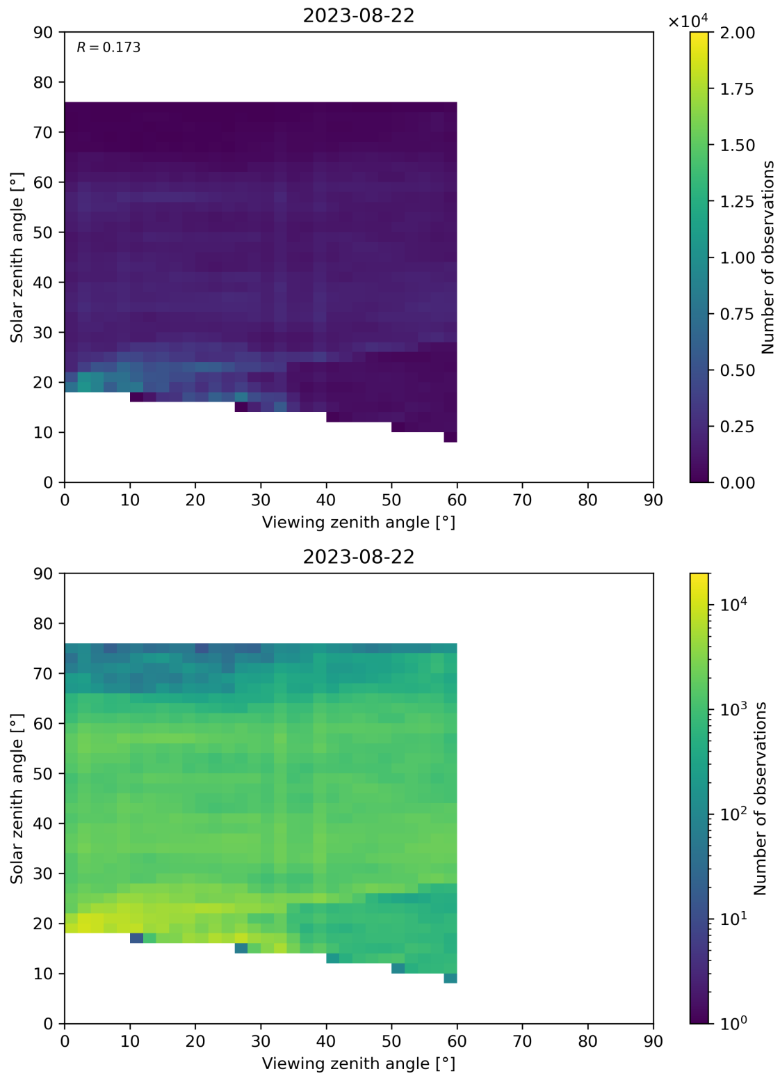
Figure 115: Scatter density plot of “Viewing zenith angle” against “Solar zenith angle” for 2023-08-21 to 2023-08-23.
