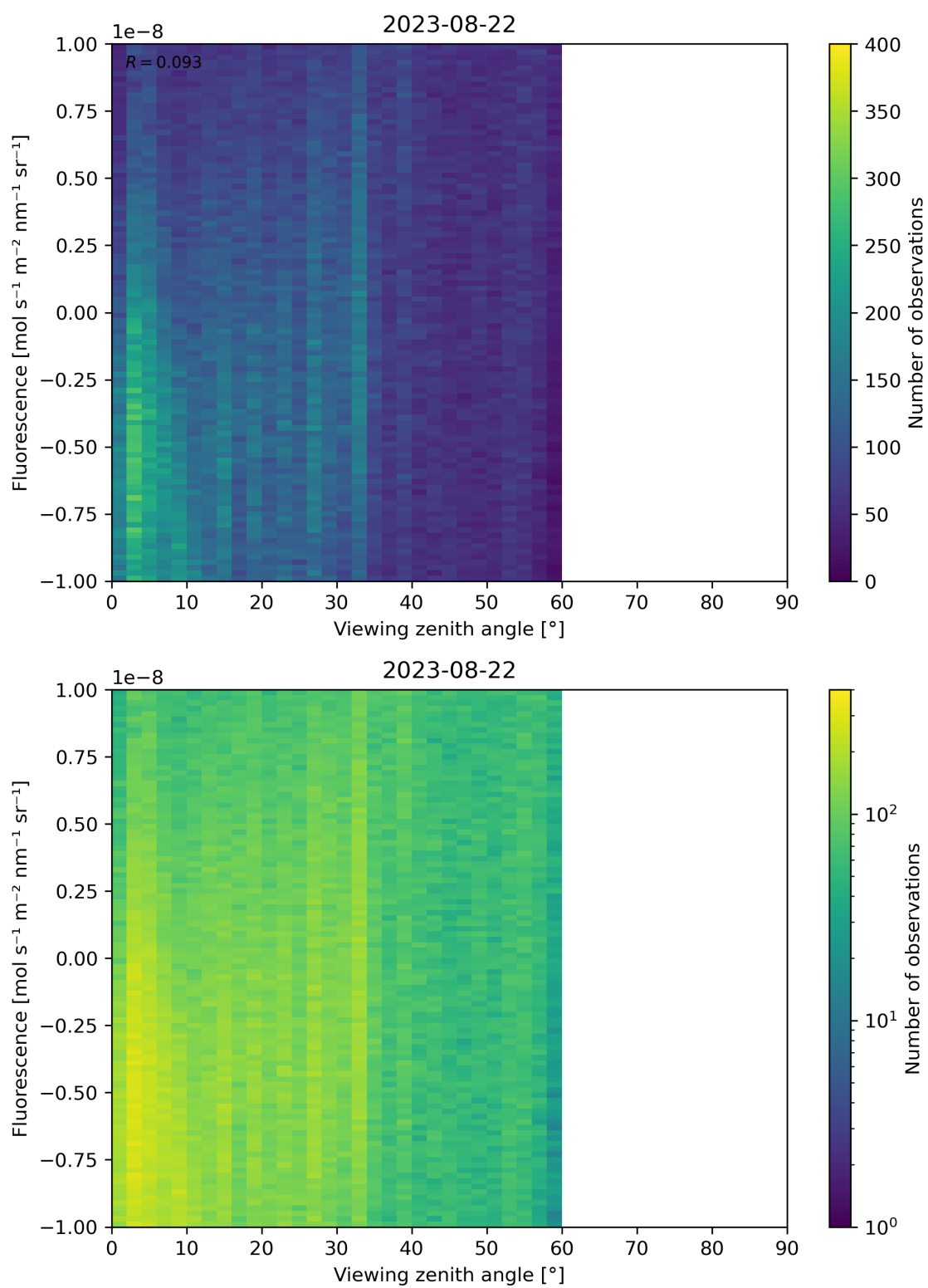
Figure 108: Scatter density plot of “Viewing zenith angle” against “Fluorescence” for 2023-08-21 to 2023-08-23.
