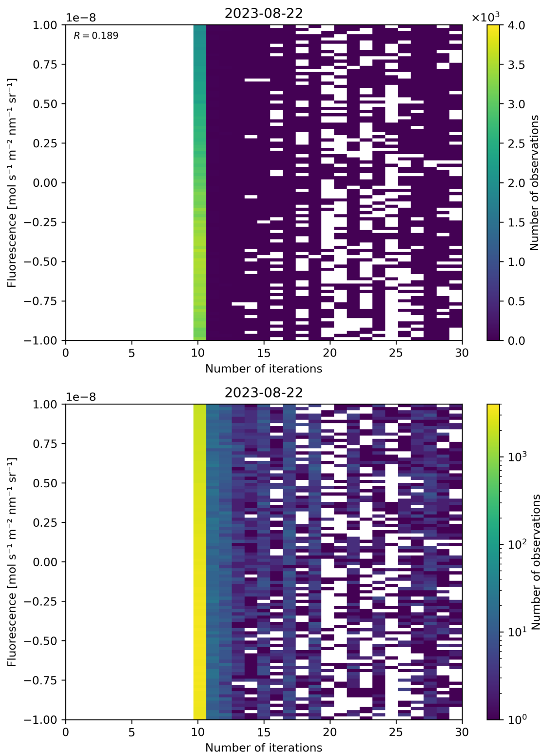
Figure 87: Scatter density plot of “Number of iterations” against “Fluorescence” for 2023-08-21 to 2023-08-23.
