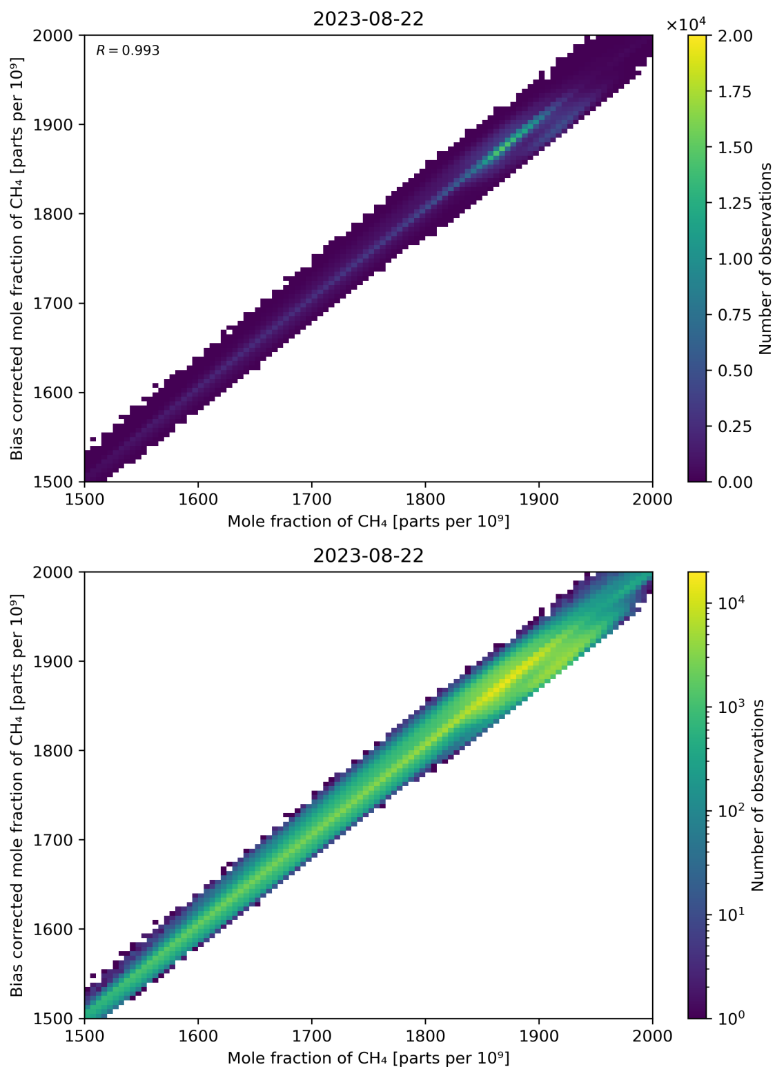
Figure 74: Scatter density plot of “Mole fraction of CH 4 ” against “Bias corrected mole fraction of CH 4 ” for 2023-08-21 to 2023-08-23.
