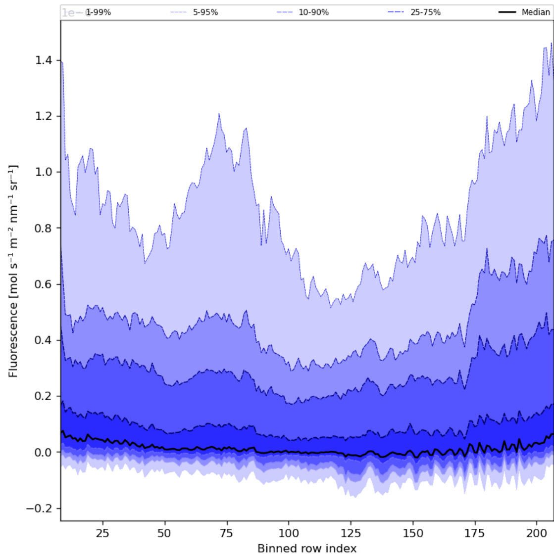
Figure 43: Along track statistics of “Fluorescence” for 2023-08-21 to 2023-08-23
