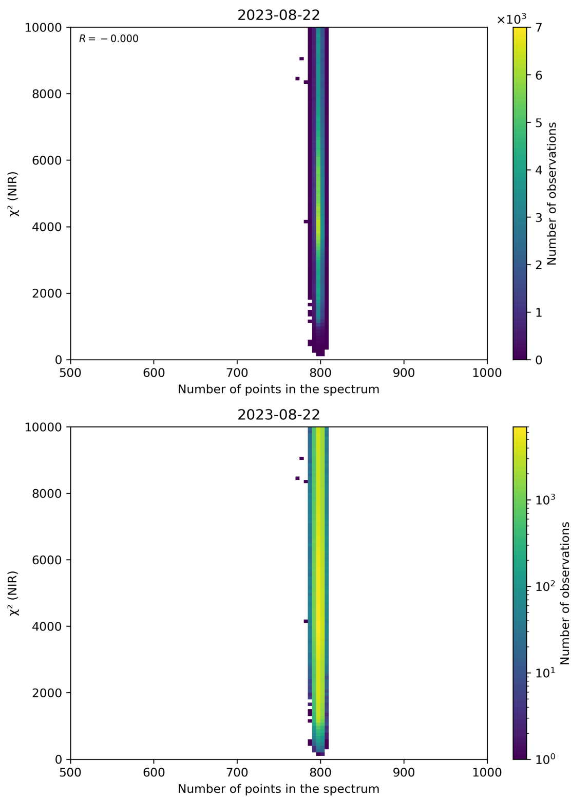
Figure 88: Scatter density plot of “Number of points in the spectrum” against “ \chi^2 (NIR)” for 2023-08-21 to 2023-08-23.
