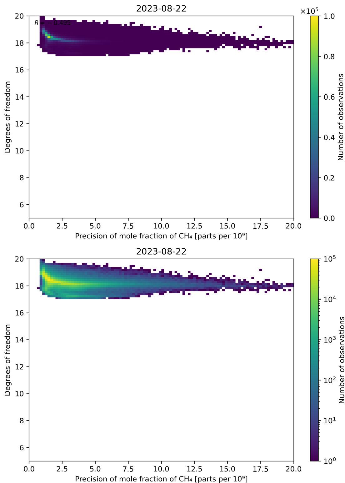
Figure 80: Scatter density plot of “Precision of mole fraction of CH 4 ” against “Degrees of freedom” for 2023-08-21 to 2023-08-23.
