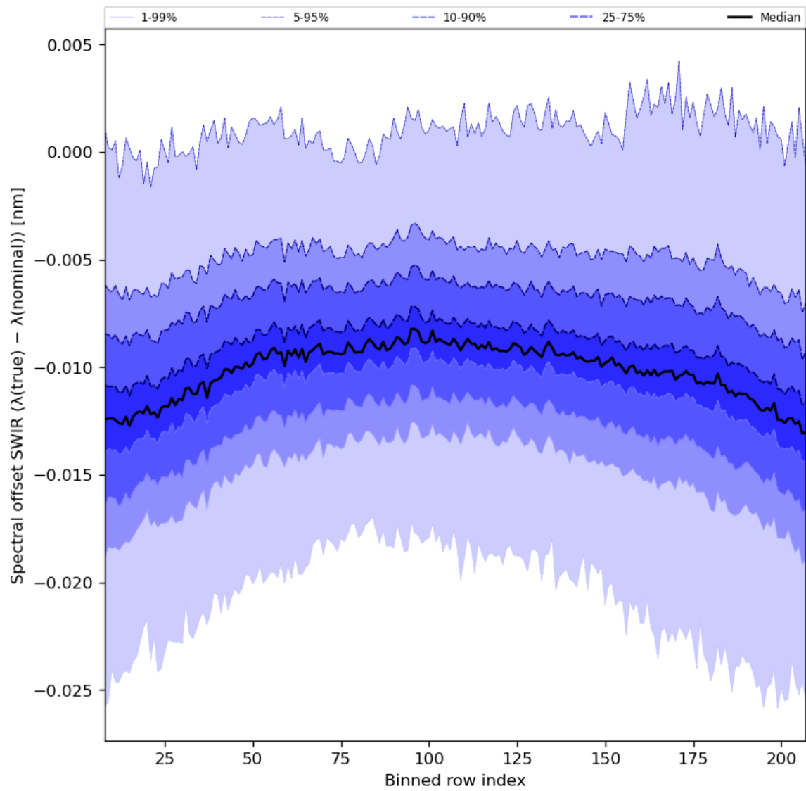
Figure 38: Along track statistics of “Spectral offset SWIR ( \lambda(\text{true}) - \lambda(\text{nominal}) )” for 2023-08-21 to 2023-08-23
