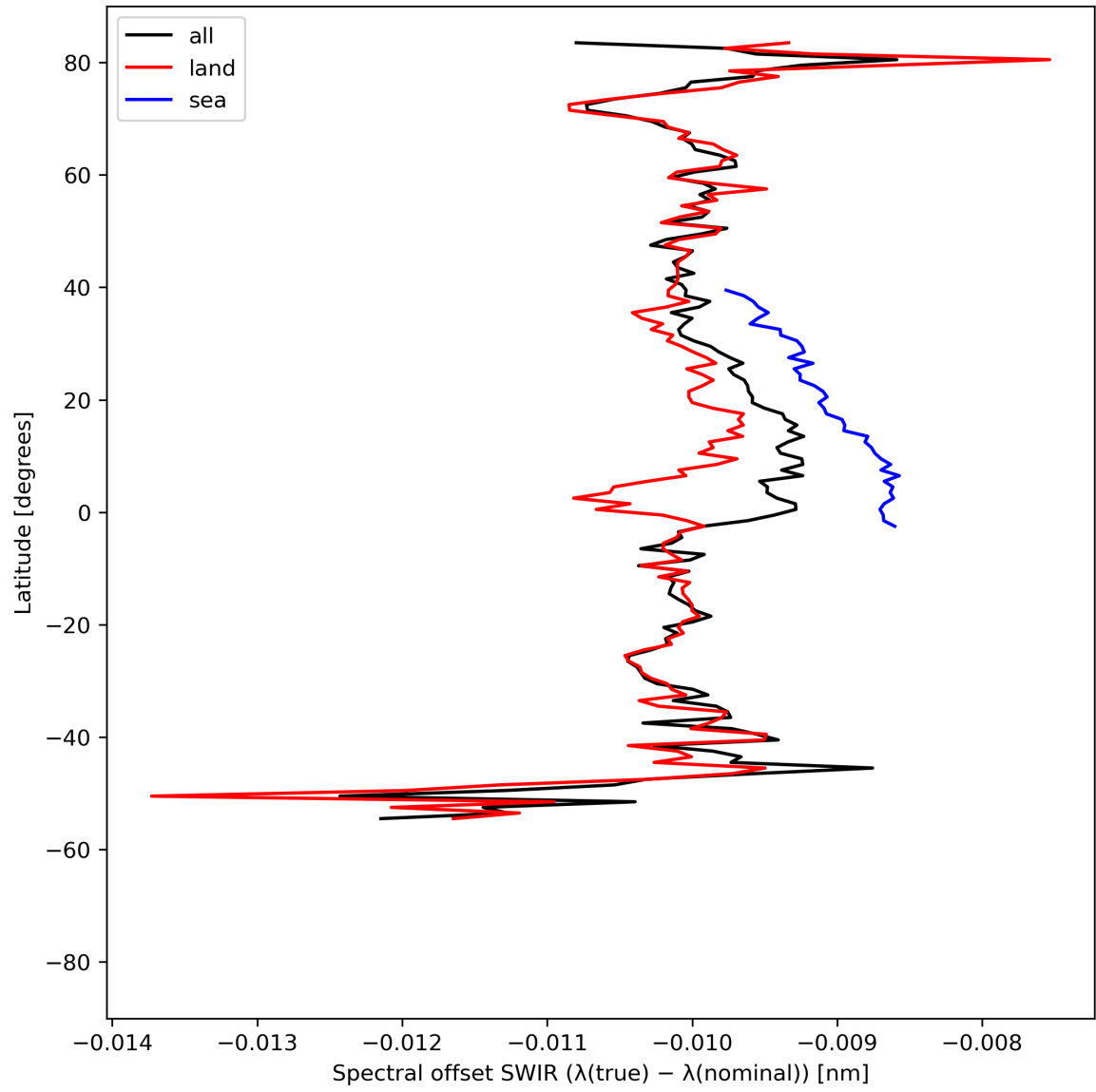
Figure 16: Zonal average of “Spectral offset SWIR ( \lambda(\text{true}) - \lambda(\text{nominal}) )” for 2023-08-21 to 2023-08-23.
