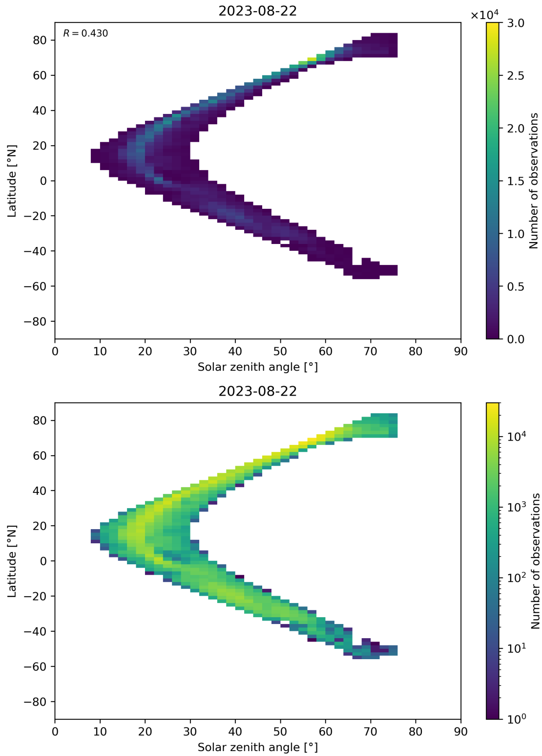
Figure 98: Scatter density plot of “Solar zenith angle” against “Latitude” for 2023-08-21 to 2023-08-23.
