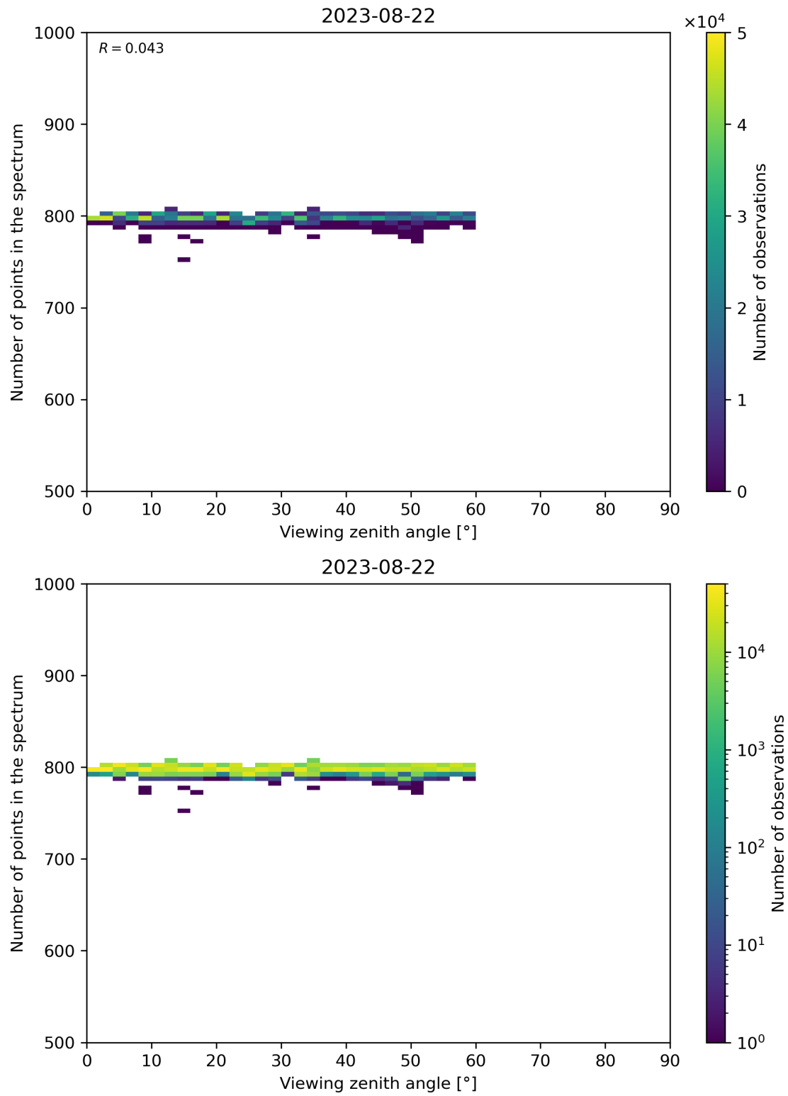
Figure 114: Scatter density plot of “Viewing zenith angle” against “Number of points in the spectrum” for 2023-08-21 to 2023-08-23.
