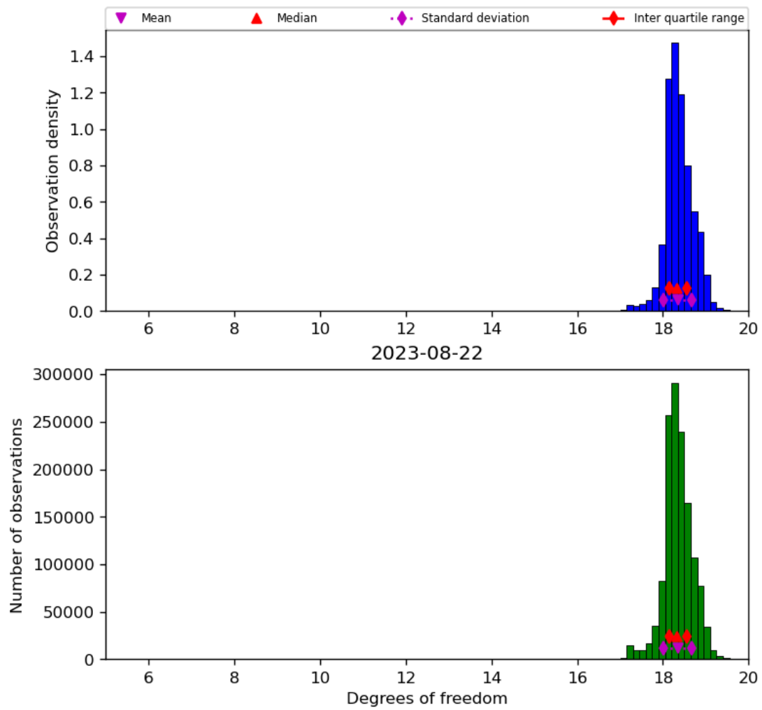
Figure 30: Histogram of “Degrees of freedom” for 2023-08-21 to 2023-08-23
