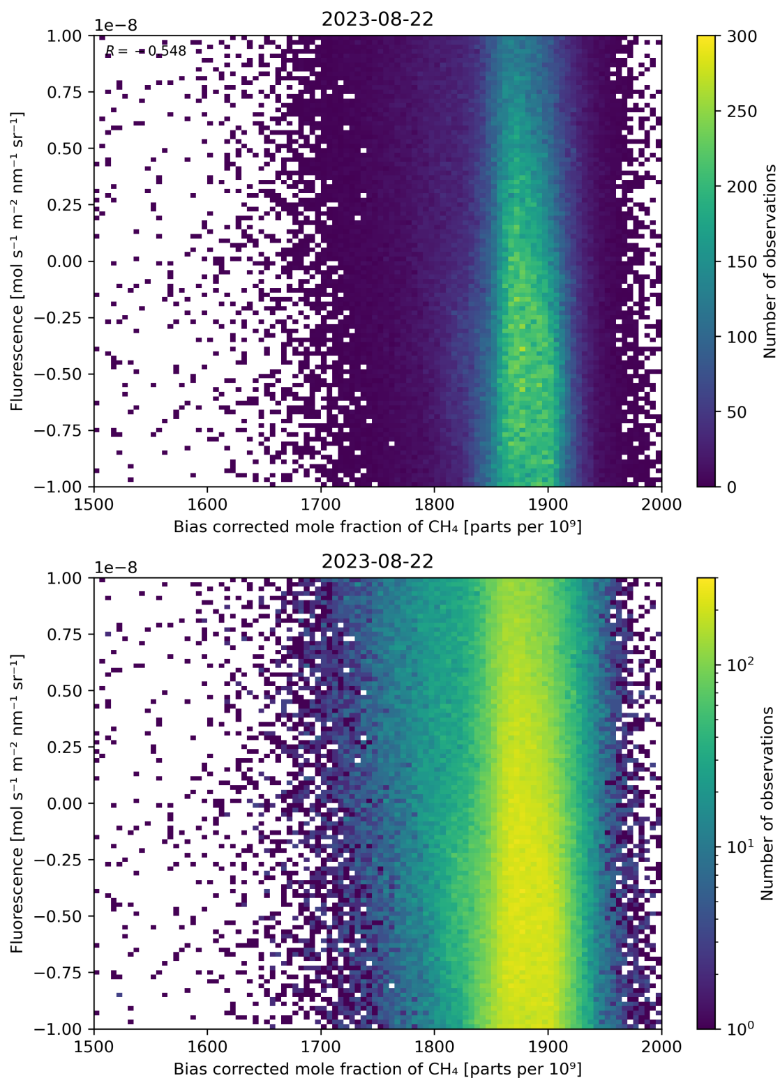
Figure 66: Scatter density plot of “Bias corrected mole fraction of \text{CH}_4 ” against “Fluorescence” for 2023-08-21 to 2023-08-23.
