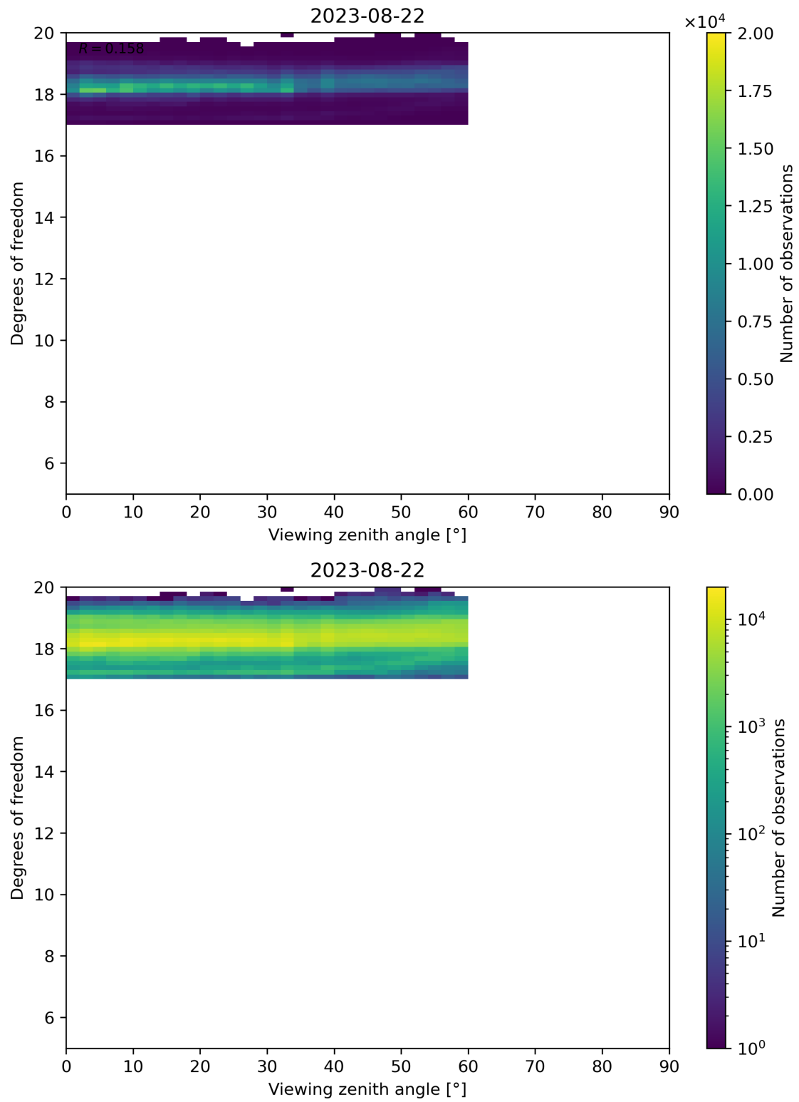
Figure 107: Scatter density plot of “Viewing zenith angle” against “Degrees of freedom” for 2023-08-21 to 2023-08-23.
