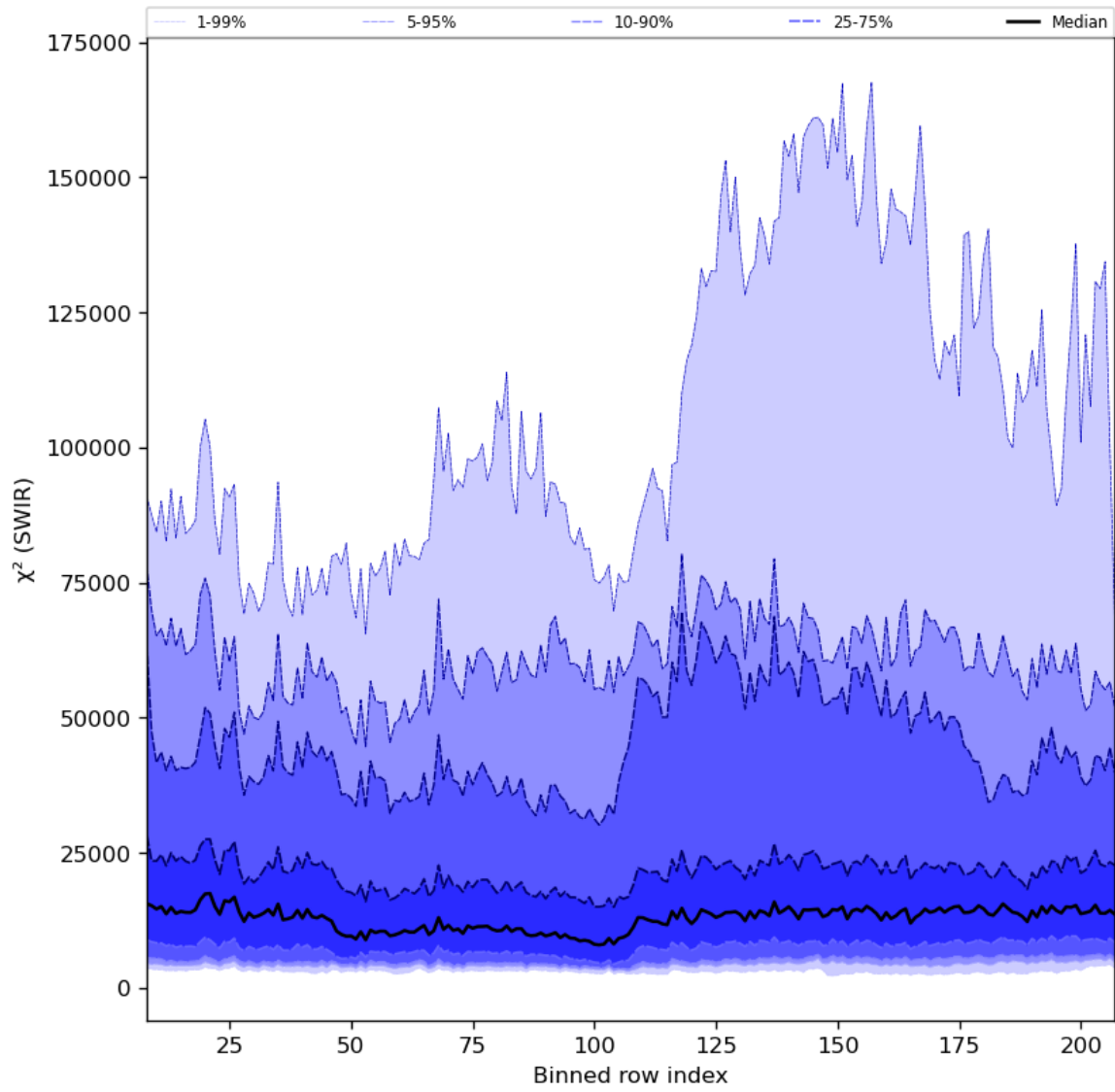
Figure 39: Along track statistics of " \chi^2 (SWIR)" for 2023-08-21 to 2023-08-23
