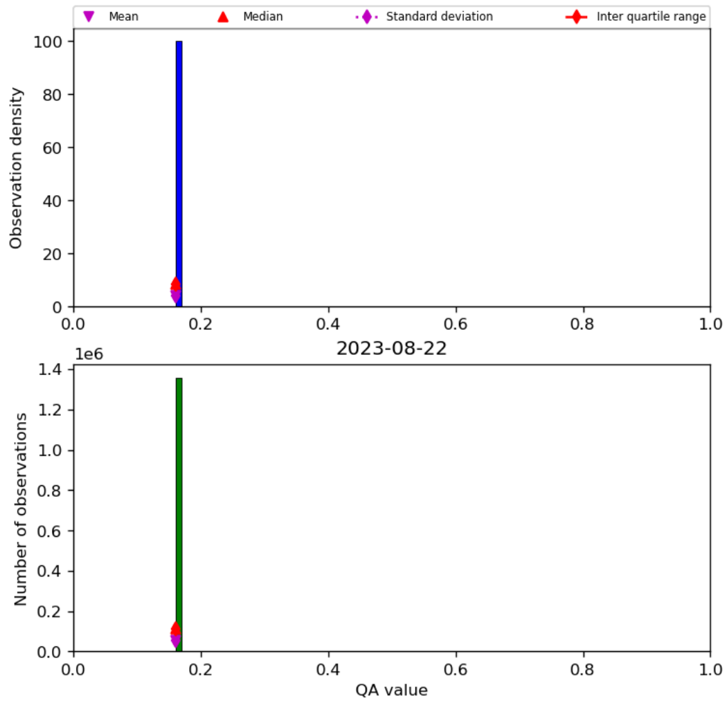
Figure 22: Histogram of “QA value” for 2023-08-21 to 2023-08-23
