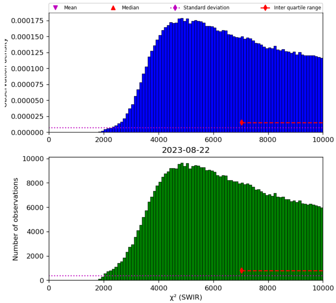
Figure 28: Histogram of " \chi^2 (SWIR)" for 2023-08-21 to 2023-08-23
