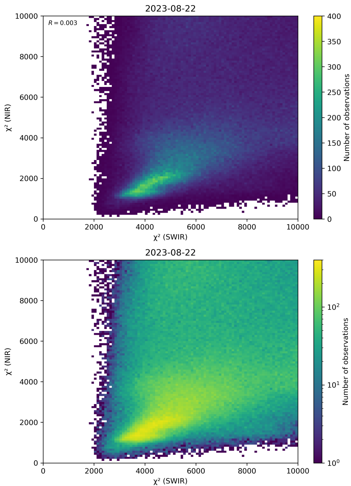
Figure 47: Scatter density plot of “ \chi^2 (SWIR)” against “ \chi^2 (NIR)” for 2023-08-21 to 2023-08-23.
