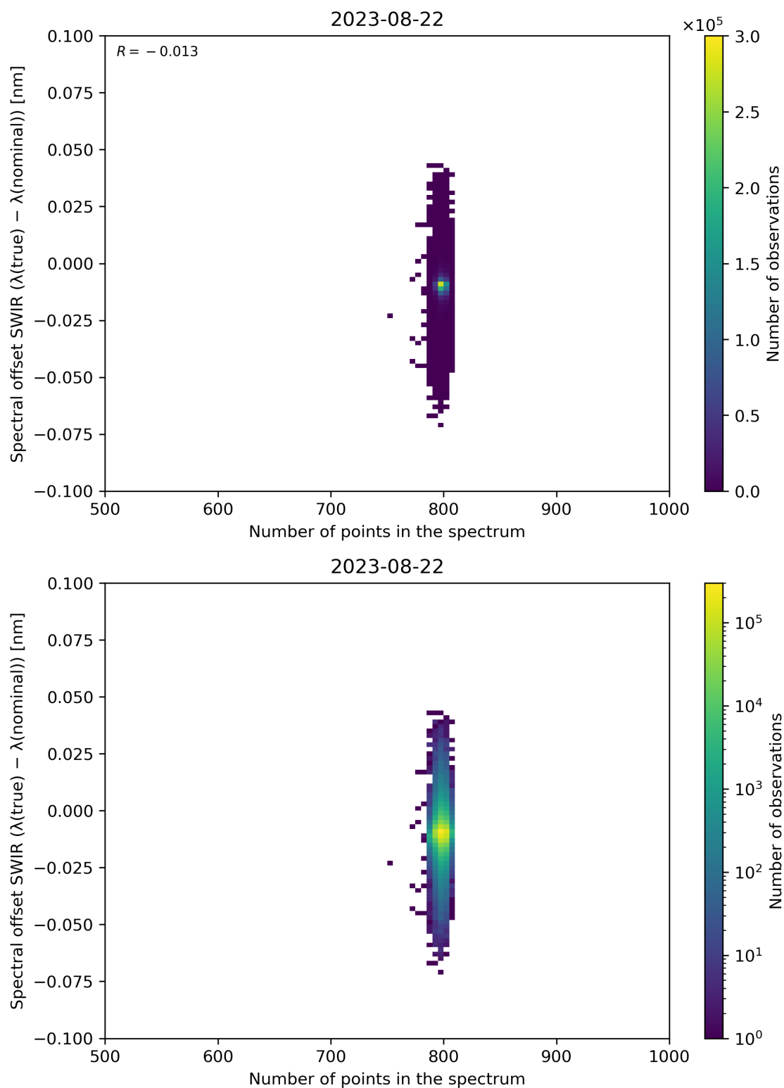
Figure 93: Scatter density plot of “Number of points in the spectrum” against “Spectral offset SWIR ( \lambda(\text{true}) - \lambda(\text{nominal}) )” for 2023-08-21 to 2023-08-23.
