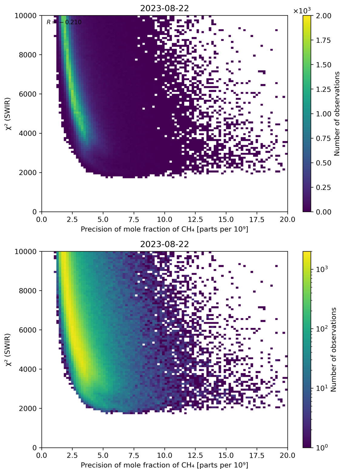
Figure 79: Scatter density plot of “Precision of mole fraction of \text{CH}_4 ” against “ \chi^2 (SWIR)” for 2023-08-21 to 2023-08-23.
