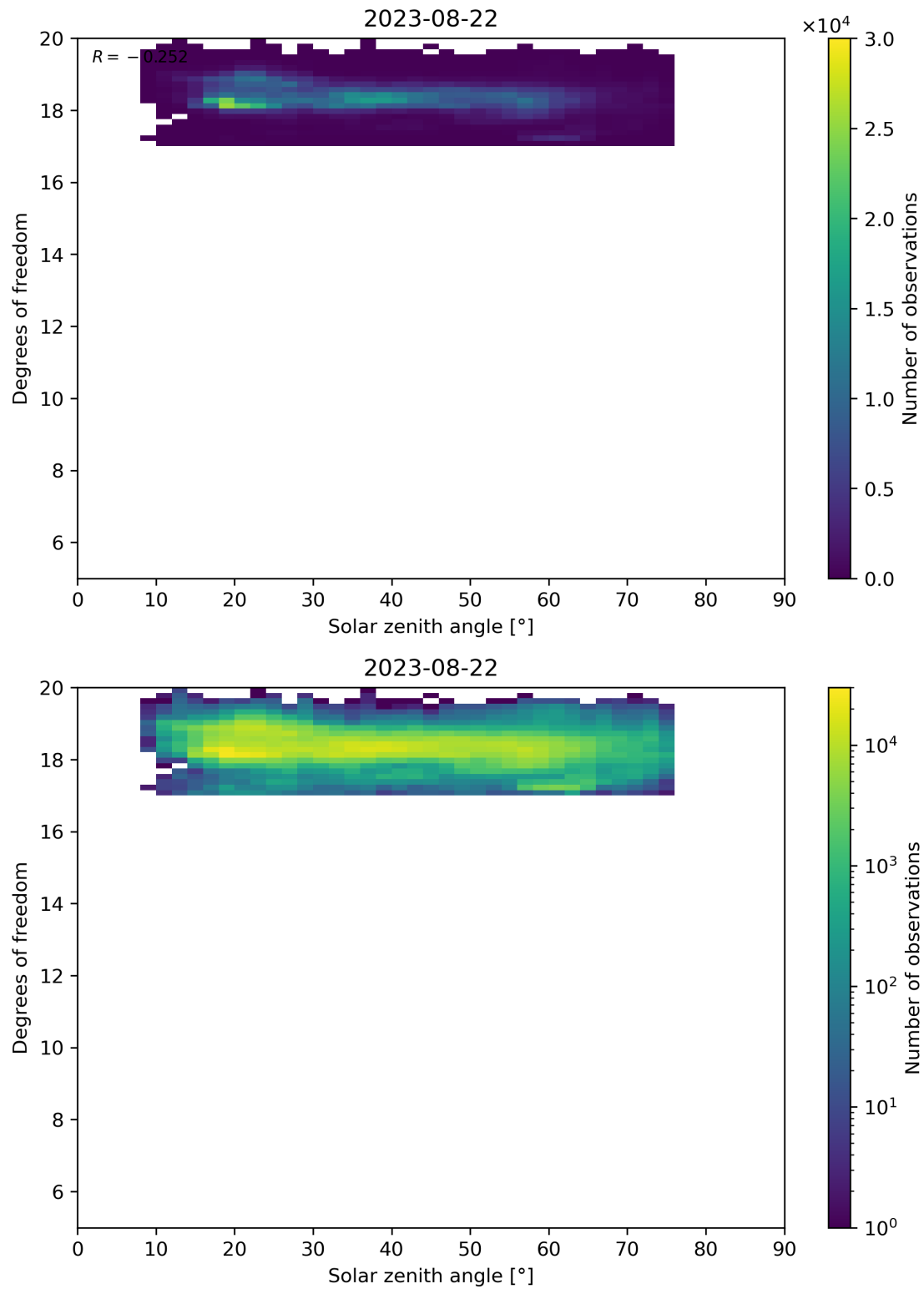
Figure 96: Scatter density plot of “Solar zenith angle” against “Degrees of freedom” for 2023-08-21 to 2023-08-23.
