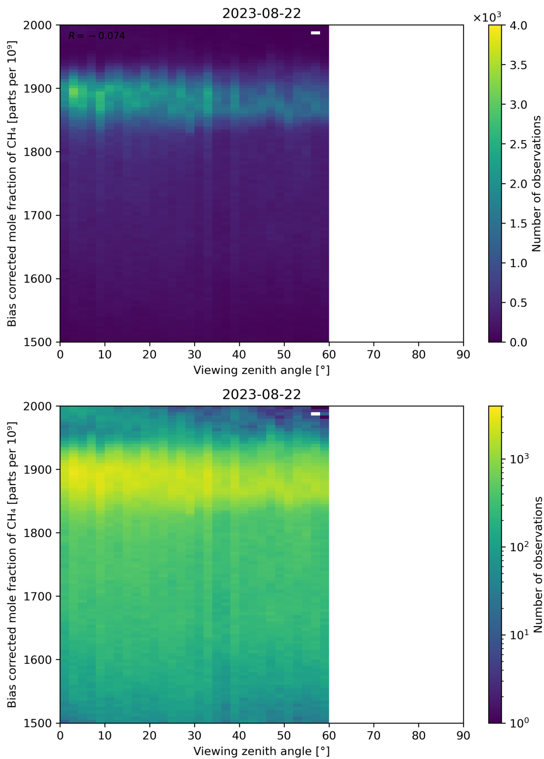
Figure 111: Scatter density plot of “Viewing zenith angle” against “Bias corrected mole fraction of CH 4 ” for 2023-08-21 to 2023-08-23.
