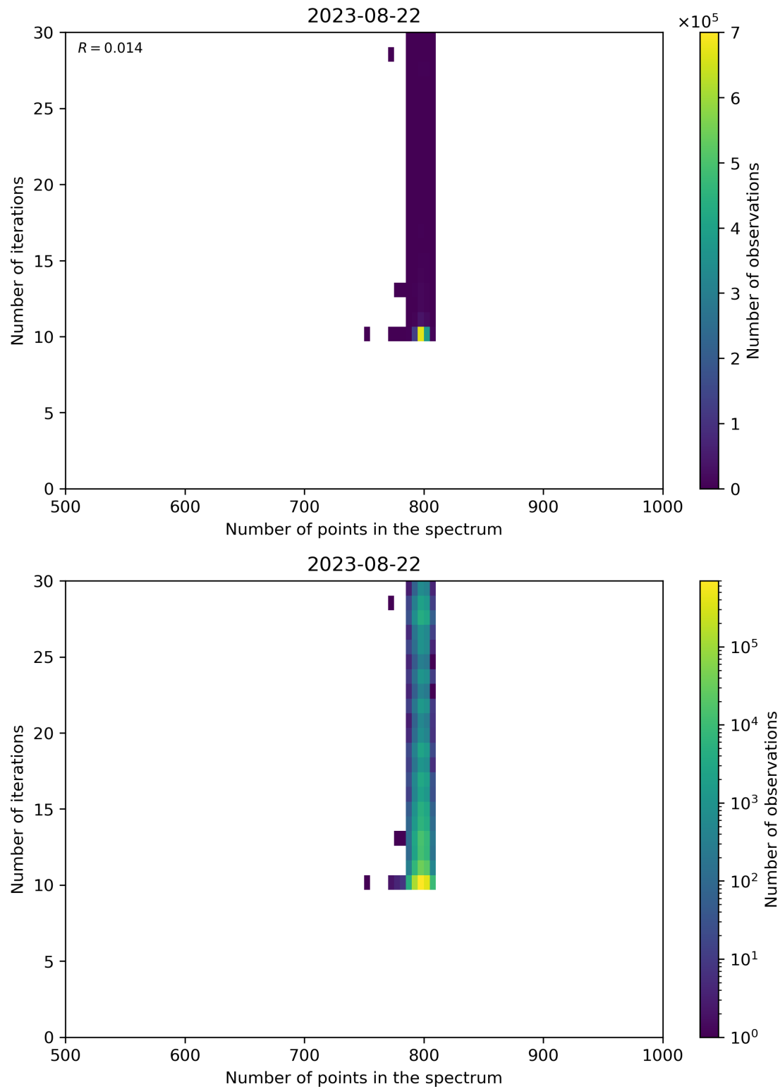
Figure 92: Scatter density plot of “Number of points in the spectrum” against “Number of iterations” for 2023-08-21 to 2023-08-23.
