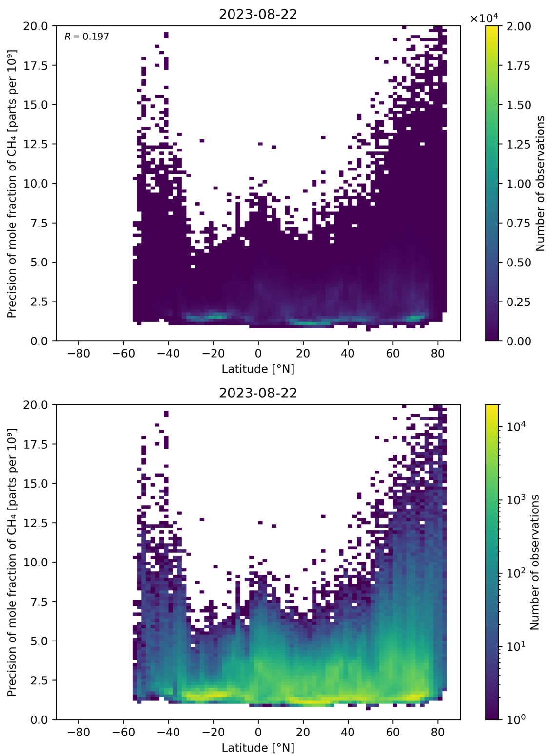
Figure 59: Scatter density plot of “Latitude” against “Precision of mole fraction of \text{CH}_4 ” for 2023-08-21 to 2023-08-23.
