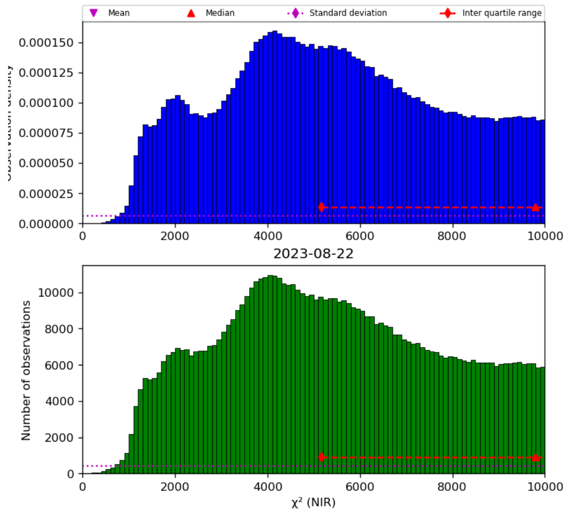
Figure 29: Histogram of “ \chi^2 (NIR)” for 2023-08-21 to 2023-08-23
