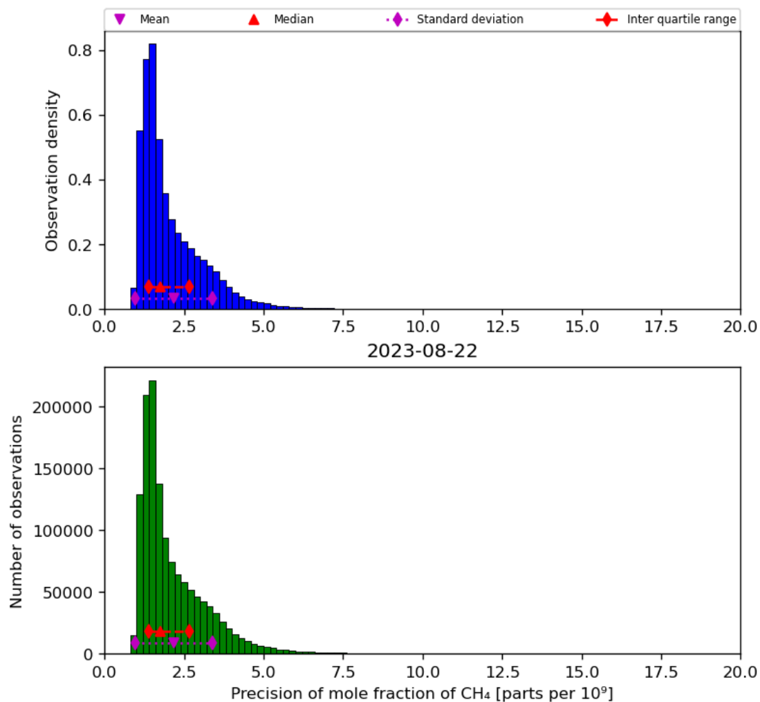
Figure 24: Histogram of “Precision of mole fraction of CH 4 ” for 2023-08-21 to 2023-08-23
