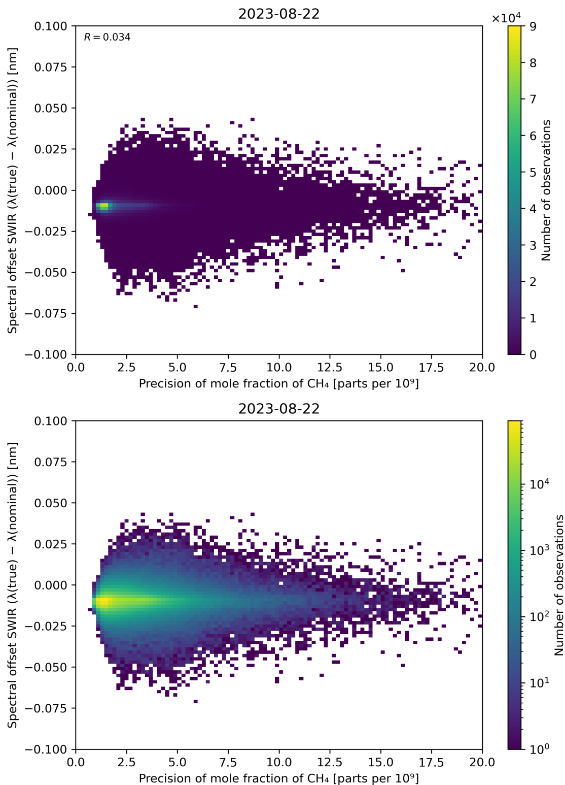
Figure 85: Scatter density plot of “Precision of mole fraction of \text{CH}_4 ” against “Spectral offset SWIR ( \lambda(\text{true}) - \lambda(\text{nominal}) )” for 2023-08-21 to 2023-08-23.
