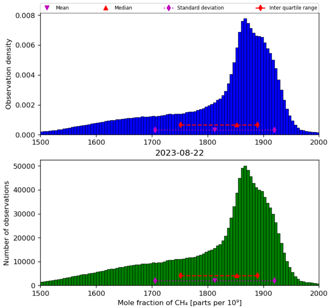
Figure 23: Histogram of “Mole fraction of CH 4 ” for 2023-08-21 to 2023-08-23
