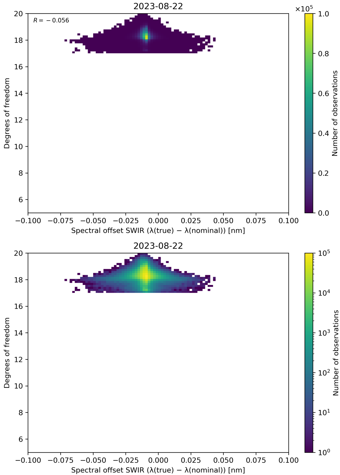
Figure 119: Scatter density plot of “Spectral offset SWIR ( \lambda(\text{true}) - \lambda(\text{nominal}) )” against “Degrees of freedom” for 2023-08-21 to 2023-08-23.
