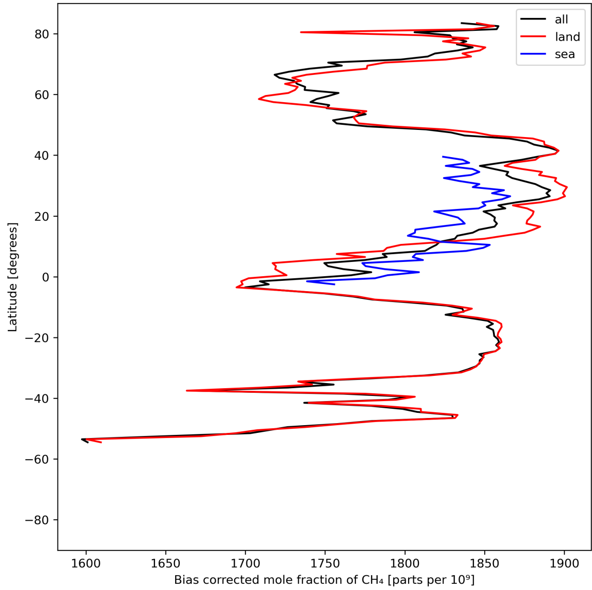
Figure 14: Zonal average of “Bias corrected mole fraction of CH 4 ” for 2023-08-21 to 2023-08-23.
