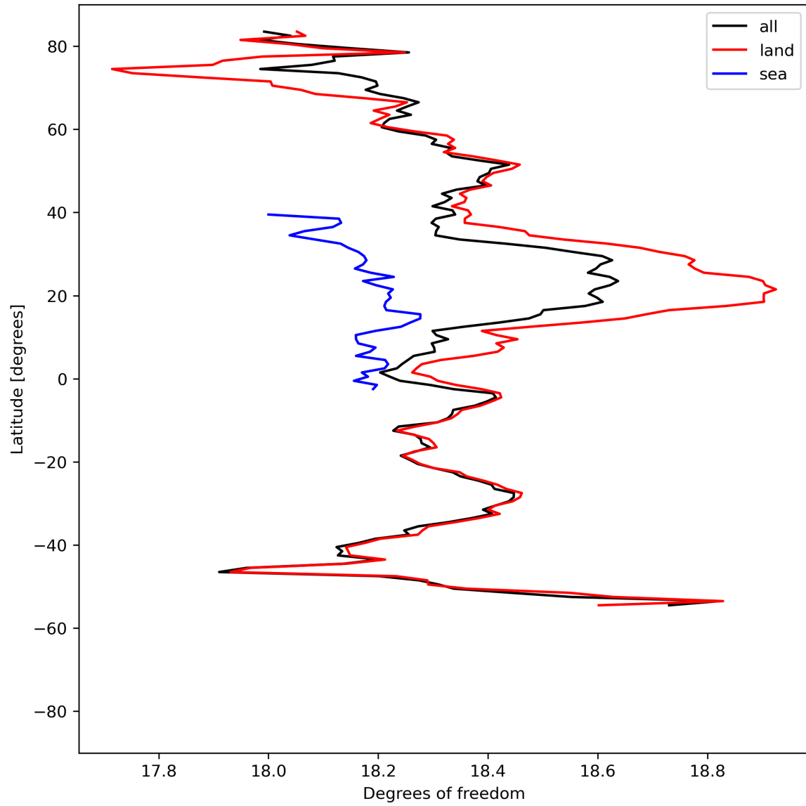
Figure 19: Zonal average of “Degrees of freedom” for 2023-08-21 to 2023-08-23.
