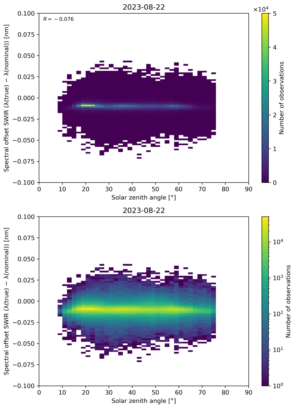
Figure 104: Scatter density plot of “Solar zenith angle” against “Spectral offset SWIR ( \lambda(\text{true}) - \lambda(\text{nominal}) )” for 2023-08-21 to 2023-08-23.
