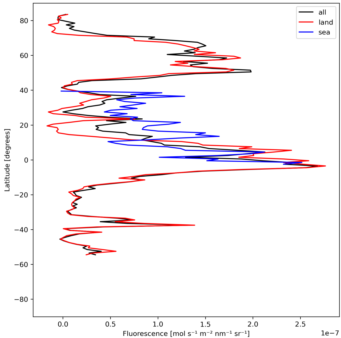
Figure 21: Zonal average of “Fluorescence” for 2023-08-21 to 2023-08-23.
