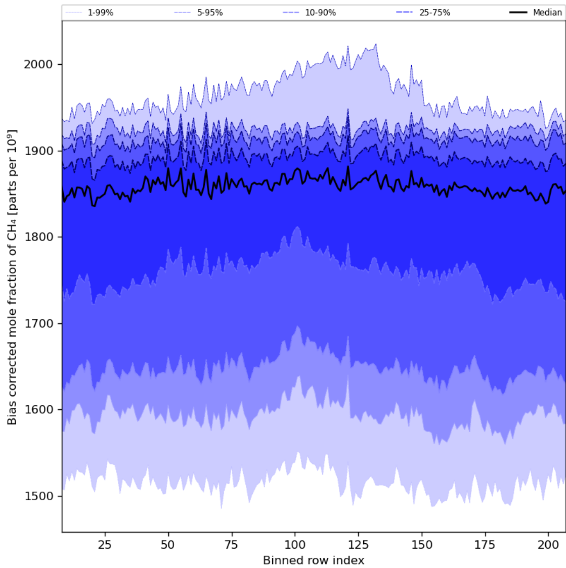
Figure 36: Along track statistics of “Bias corrected mole fraction of CH 4 ” for 2023-08-21 to 2023-08-23
