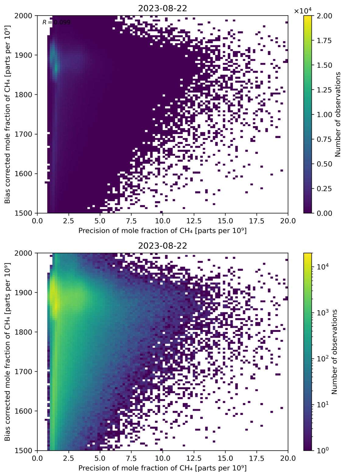
Figure 82: Scatter density plot of “Precision of mole fraction of \text{CH}_4 ” against “Bias corrected mole fraction of \text{CH}_4 ” for 2023-08-21 to 2023-08-23.
