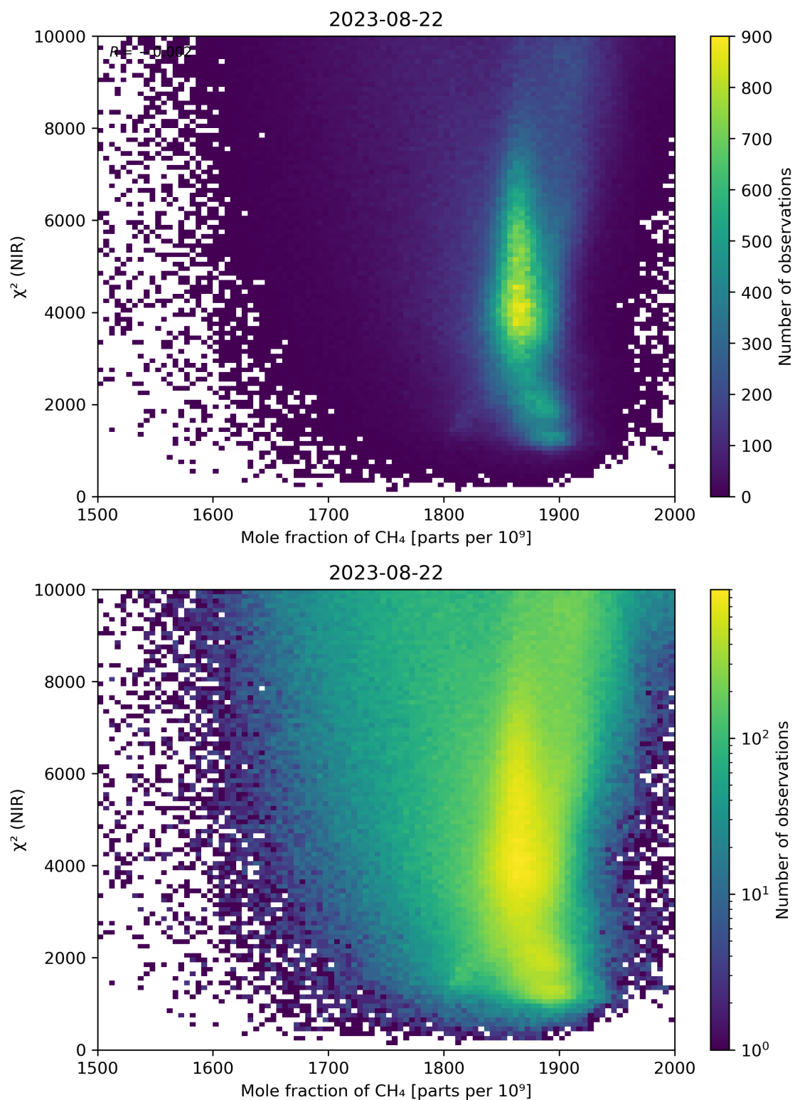
Figure 70: Scatter density plot of “Mole fraction of CH 4 ” against “ \chi^2 (NIR)” for 2023-08-21 to 2023-08-23.
