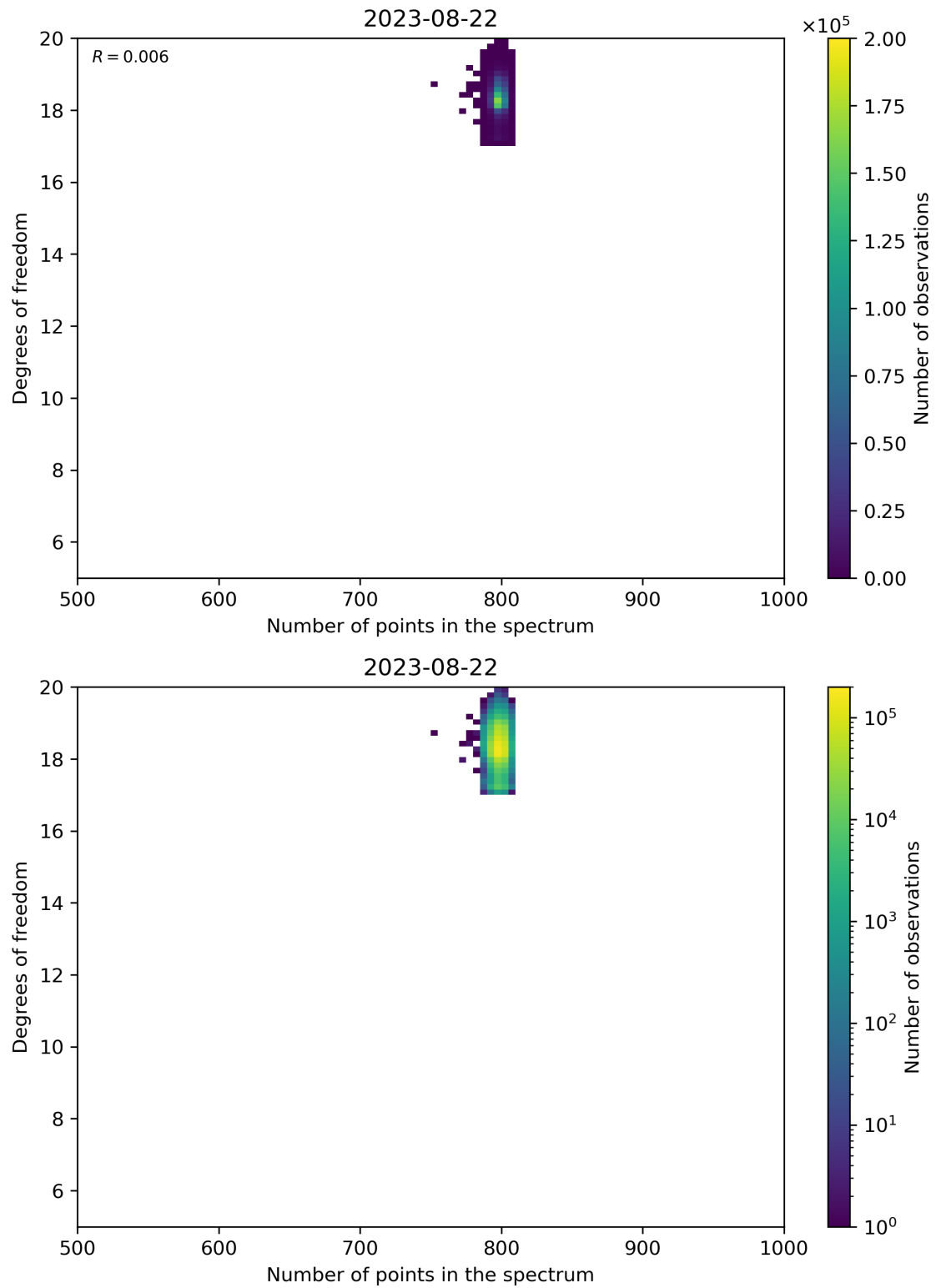
Figure 90: Scatter density plot of “Number of points in the spectrum” against “Degrees of freedom” for 2023-08-21 to 2023-08-23.
