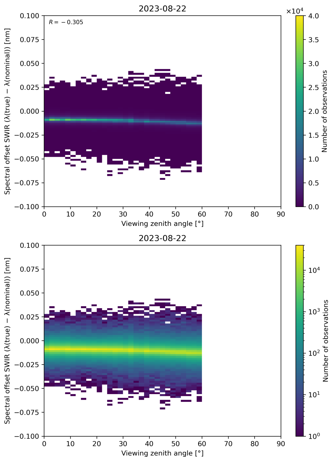
Figure 116: Scatter density plot of “Viewing zenith angle” against “Spectral offset SWIR ( \lambda(\text{true}) - \lambda(\text{nominal}) )” for 2023-08-21 to 2023-08-23.
