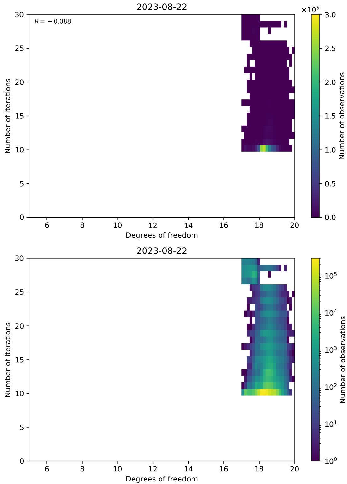
Figure 52: Scatter density plot of “Degrees of freedom” against “Number of iterations” for 2023-08-21 to 2023-08-23.
