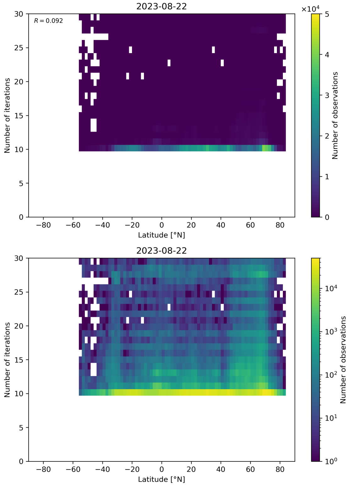
Figure 60: Scatter density plot of “Latitude” against “Number of iterations” for 2023-08-21 to 2023-08-23.
