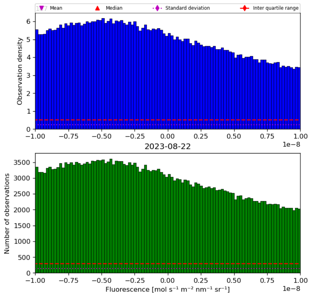
Figure 32: Histogram of “Fluorescence” for 2023-08-21 to 2023-08-23
