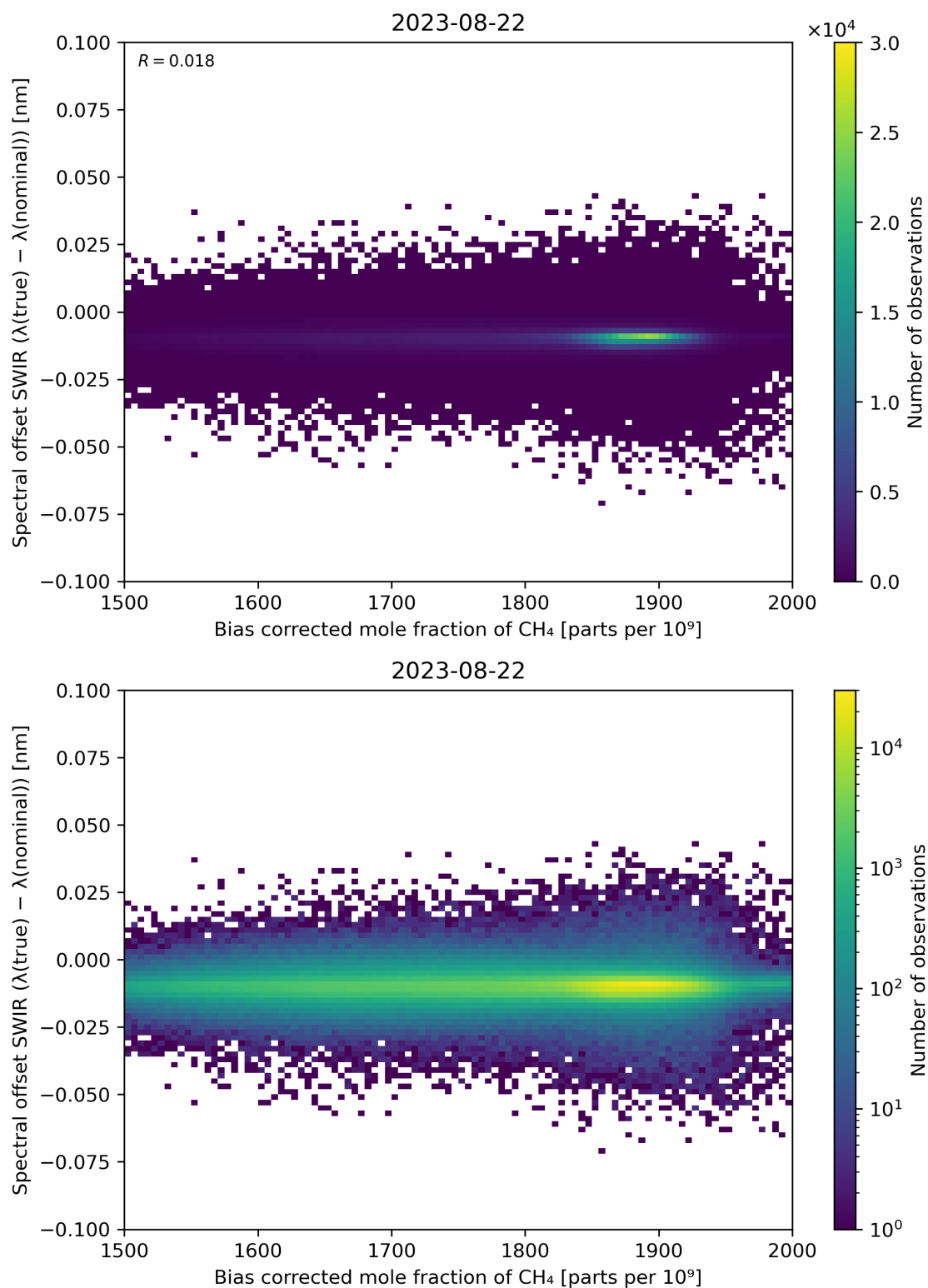
Figure 69: Scatter density plot of “Bias corrected mole fraction of \text{CH}_4 ” against “Spectral offset SWIR ( \lambda(\text{true}) - \lambda(\text{nominal}) )” for 2023-08-21 to 2023-08-23.
