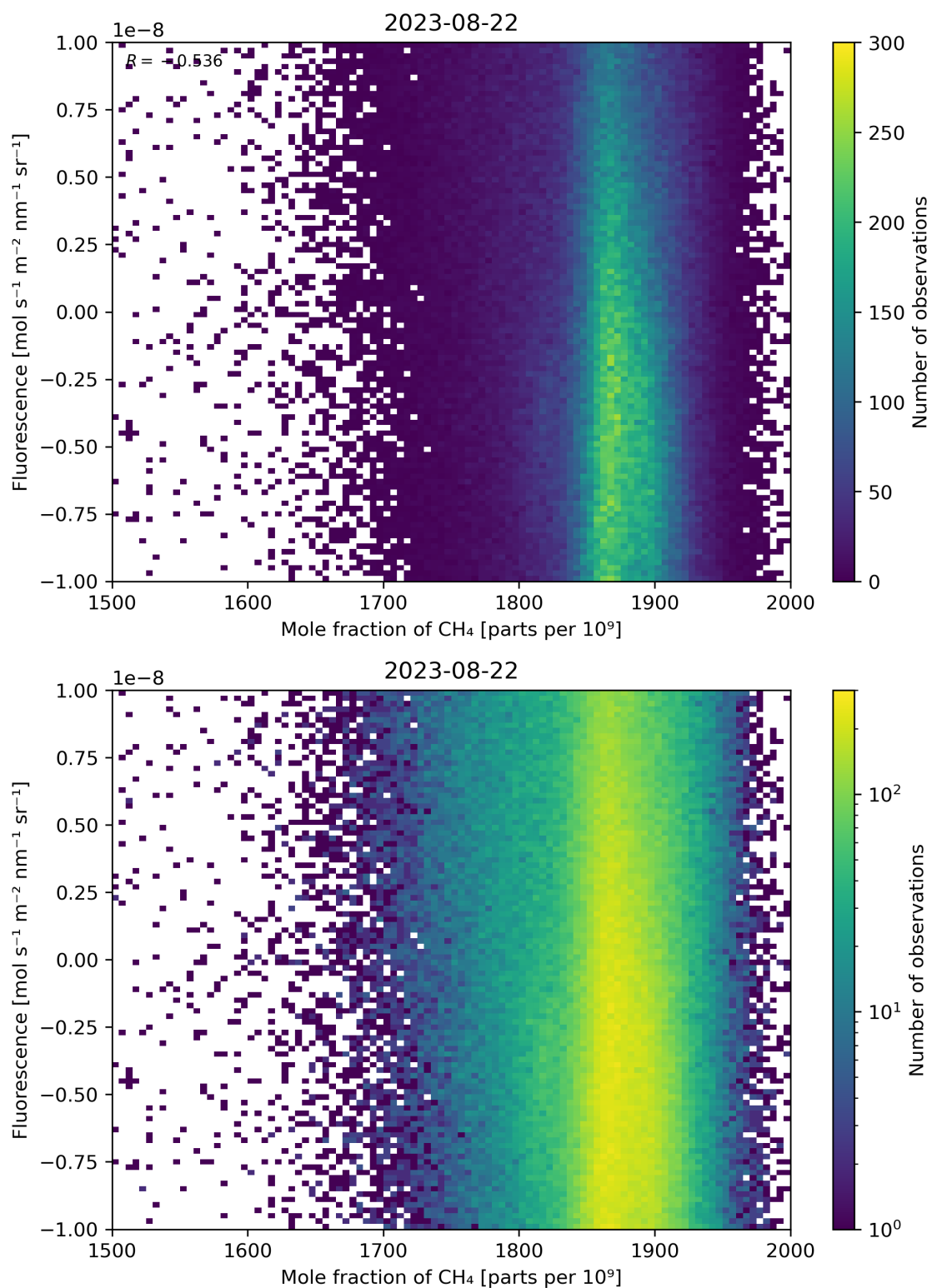
Figure 73: Scatter density plot of “Mole fraction of \text{CH}_4 ” against “Fluorescence” for 2023-08-21 to 2023-08-23.
