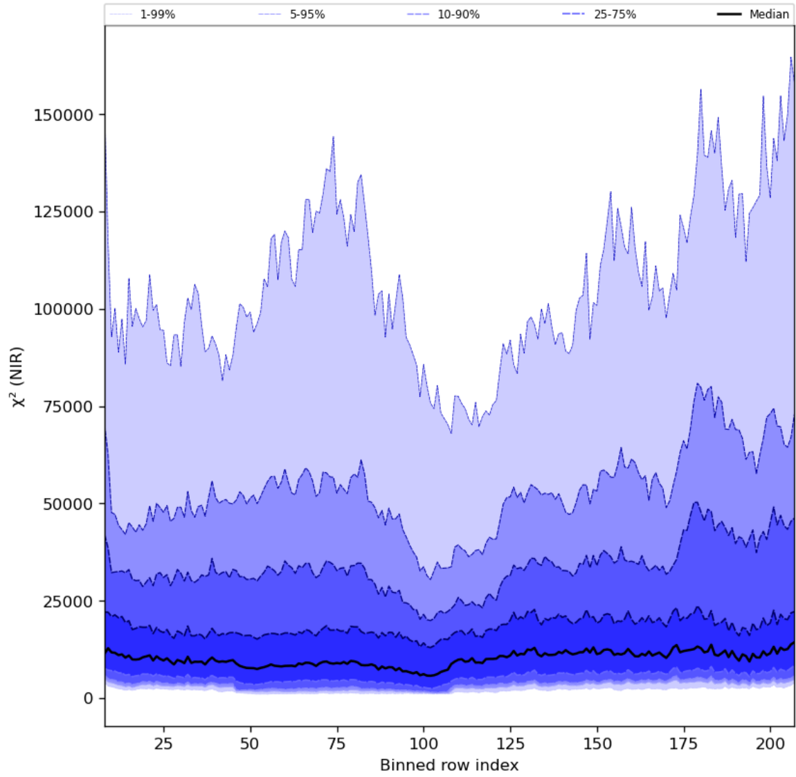
Figure 40: Along track statistics of “ \chi^2 (NIR)” for 2023-08-21 to 2023-08-23
