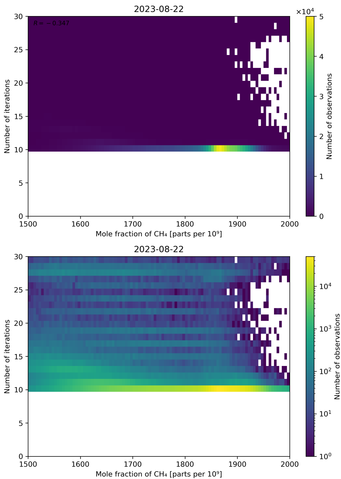
Figure 76: Scatter density plot of “Mole fraction of CH 4 ” against “Number of iterations” for 2023-08-21 to 2023-08-23.
