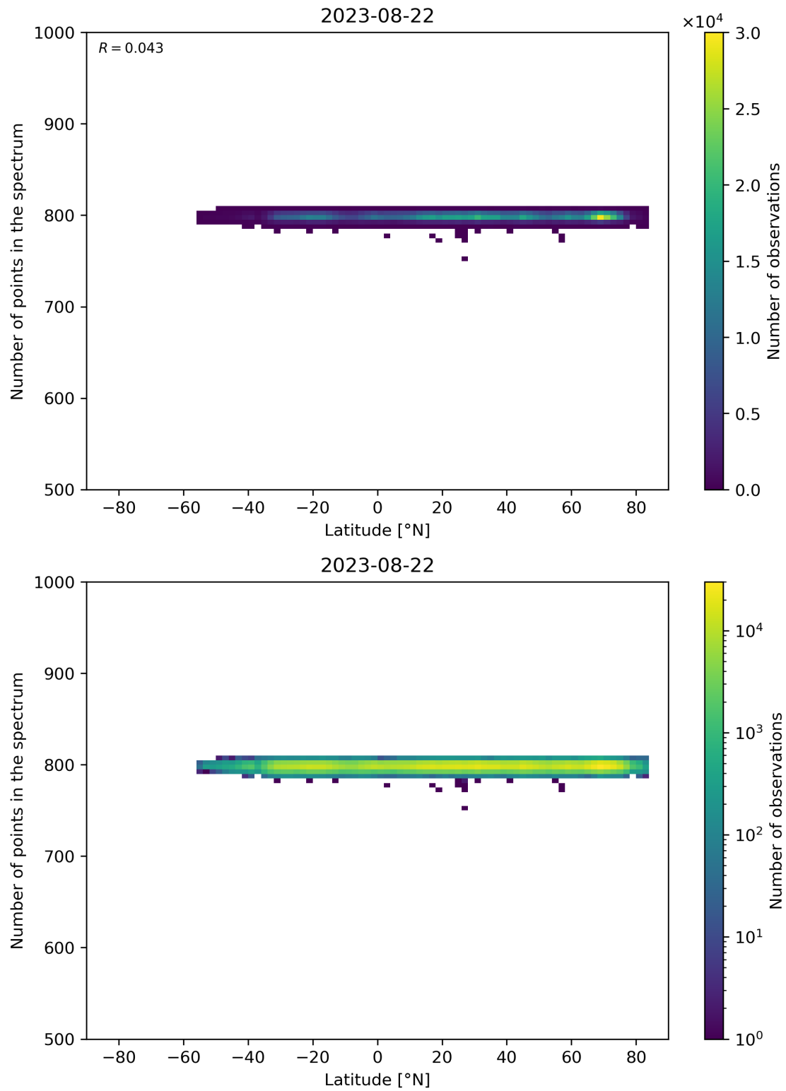
Figure 61: Scatter density plot of “Latitude” against “Number of points in the spectrum” for 2023-08-21 to 2023-08-23.
