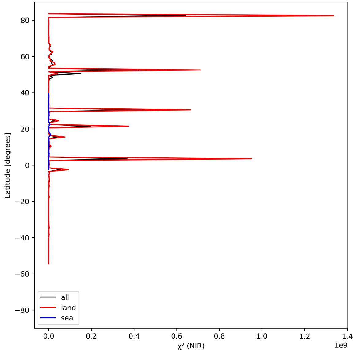
Figure 18: Zonal average of “ \chi^2 (NIR)” for 2023-08-21 to 2023-08-23.
