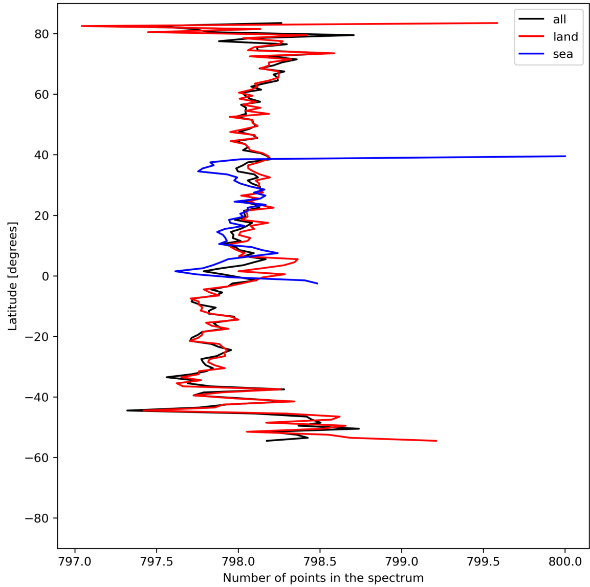
Figure 15: Zonal average of “Number of points in the spectrum” for 2023-08-21 to 2023-08-23.
