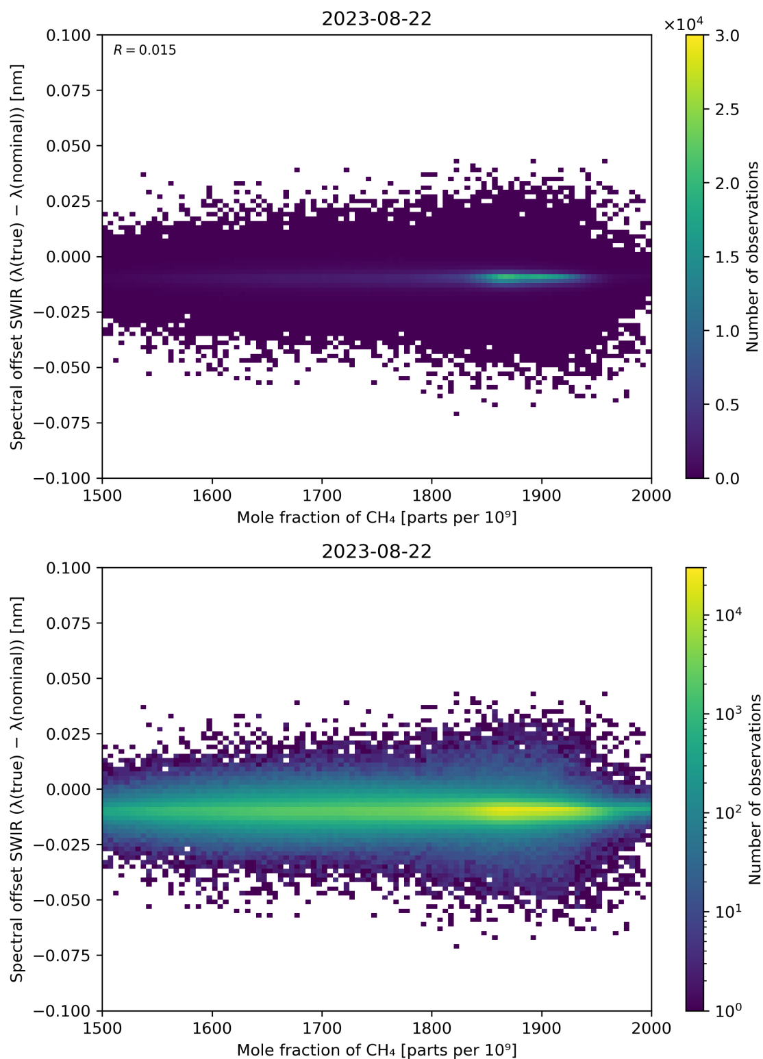
Figure 86: Scatter density plot of “Mole fraction of CH 4 ” against “Spectral offset SWIR ( \lambda(\text{true}) - \lambda(\text{nominal}) )” for 2023-08-21 to 2023-08-23.
