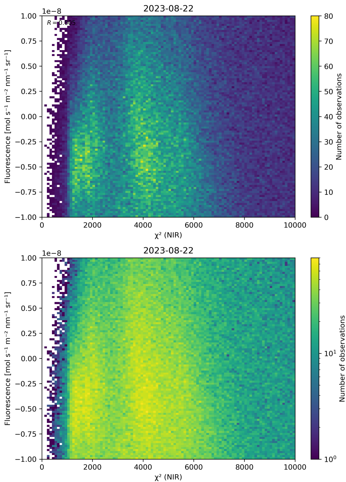
Figure 45: Scatter density plot of “ \chi^2 (NIR)” against “Fluorescence” for 2023-08-21 to 2023-08-23.
