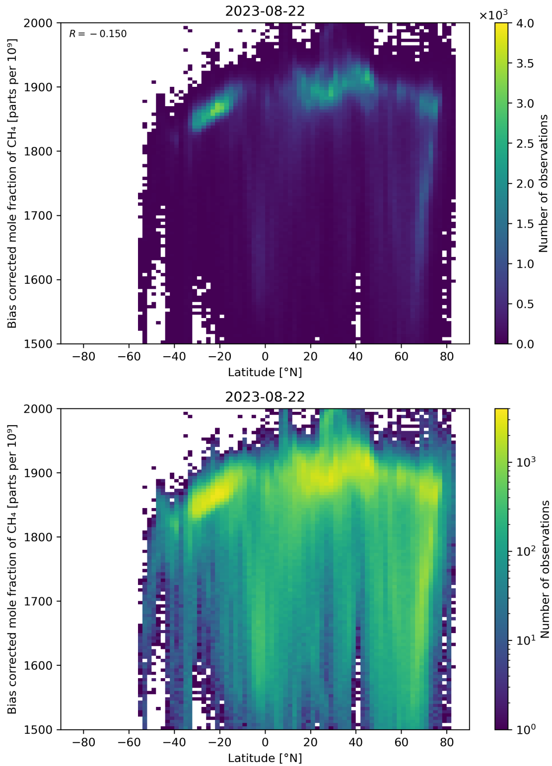
Figure 58: Scatter density plot of “Latitude” against “Bias corrected mole fraction of CH 4 ” for 2023-08-21 to 2023-08-23.
