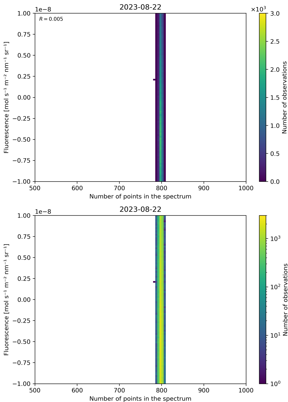
Figure 91: Scatter density plot of “Number of points in the spectrum” against “Fluorescence” for 2023-08-21 to 2023-08-23.
