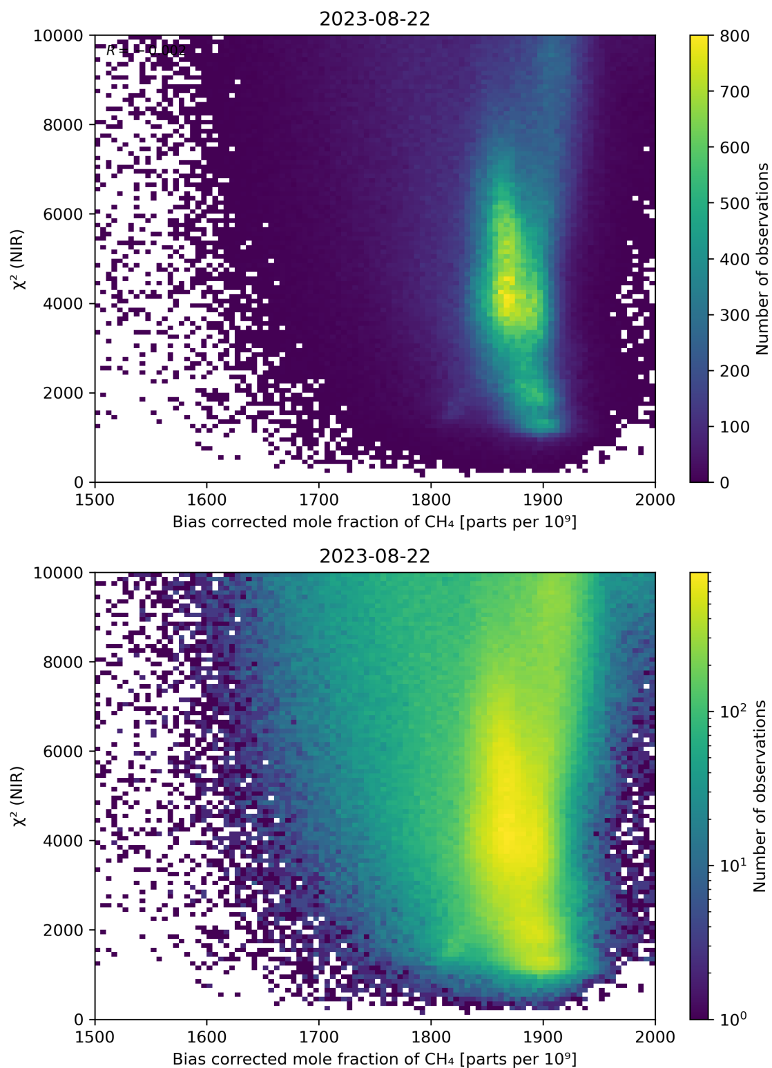
Figure 63: Scatter density plot of “Bias corrected mole fraction of CH 4 ” against “ \chi^2 (NIR)” for 2023-08-21 to 2023-08-23.
