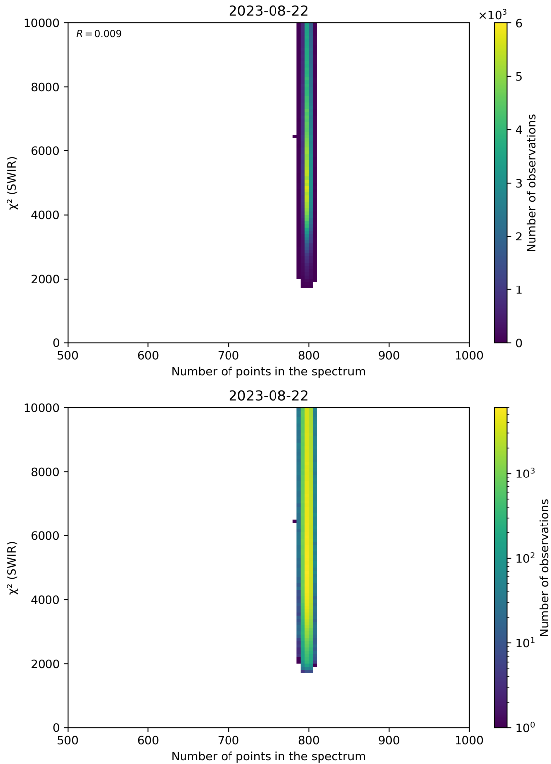
Figure 89: Scatter density plot of “Number of points in the spectrum” against “ \chi^2 (SWIR)” for 2023-08-21 to 2023-08-23.
