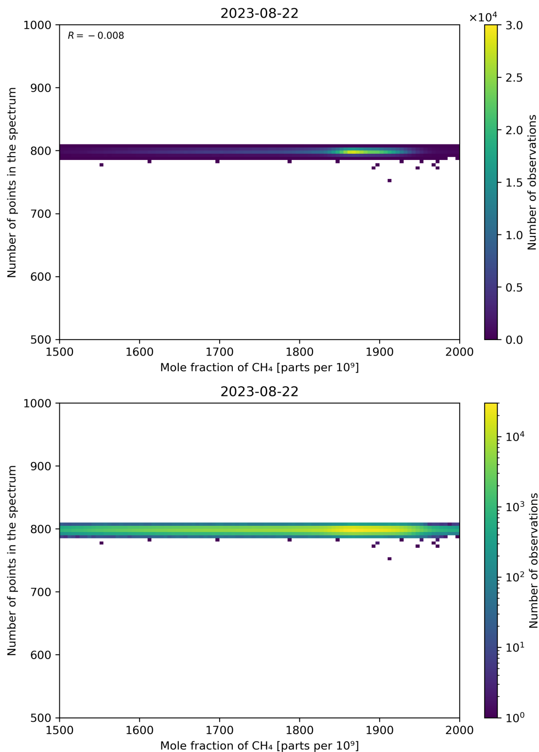
Figure 77: Scatter density plot of “Mole fraction of CH 4 ” against “Number of points in the spectrum” for 2023-08-21 to 2023-08-23.
