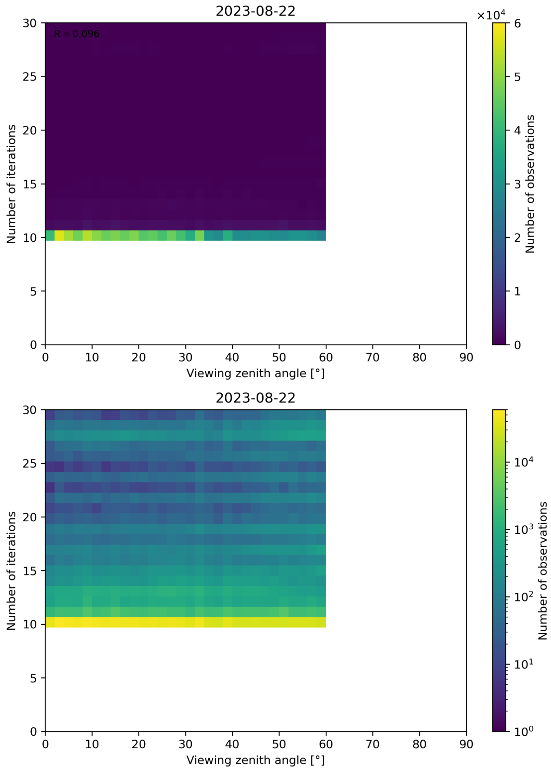
Figure 113: Scatter density plot of “Viewing zenith angle” against “Number of iterations” for 2023-08-21 to 2023-08-23.
