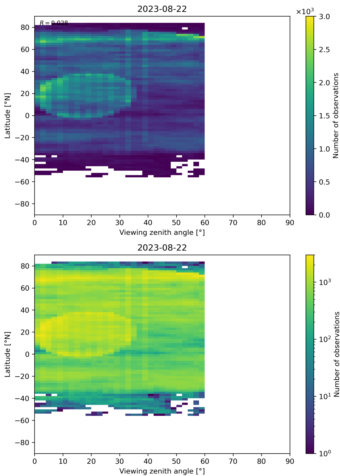
Figure 109: Scatter density plot of “Viewing zenith angle” against “Latitude” for 2023-08-21 to 2023-08-23.
