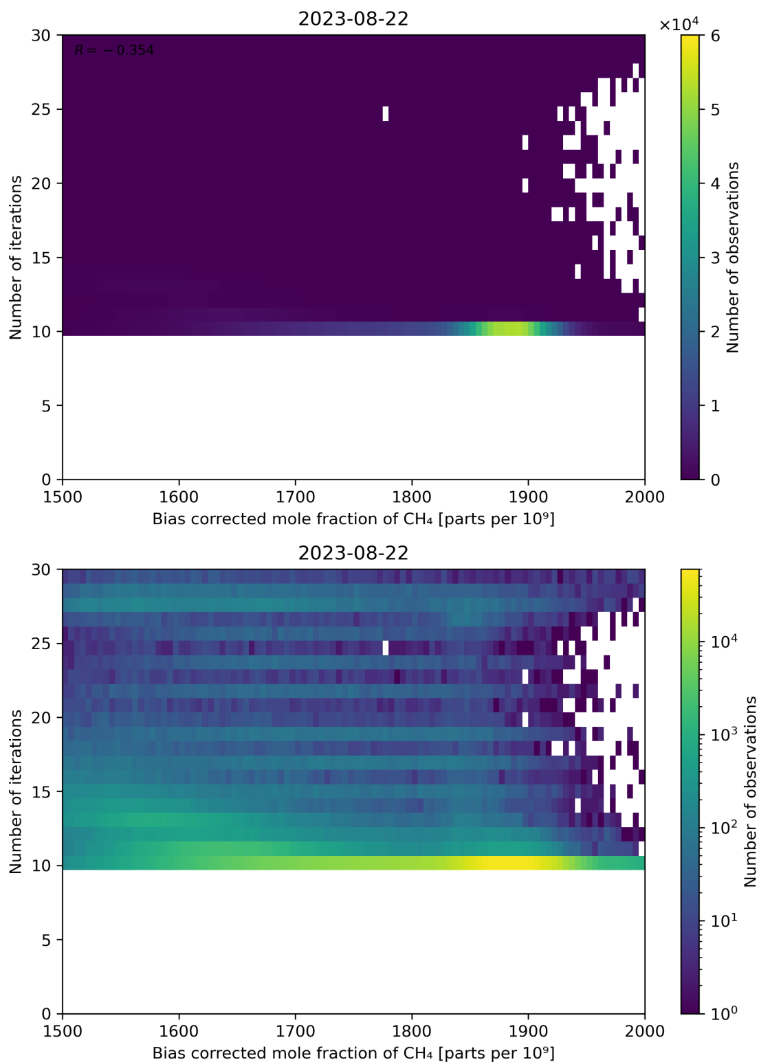
Figure 67: Scatter density plot of “Bias corrected mole fraction of CH 4 ” against “Number of iterations” for 2023-08-21 to 2023-08-23.
