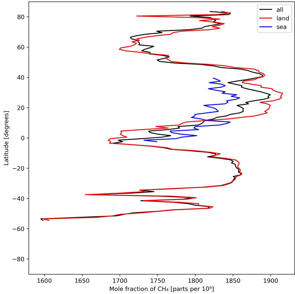
Figure 12: Zonal average of “Mole fraction of \text{CH}_4 ” for 2023-08-21 to 2023-08-23.
