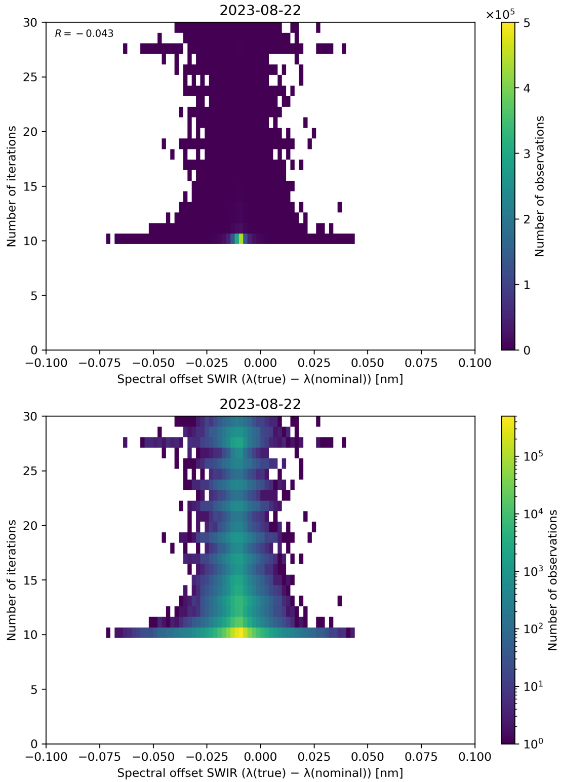
Figure 121: Scatter density plot of “Spectral offset SWIR ( \lambda(\text{true}) - \lambda(\text{nominal}) )” against “Number of iterations” for 2023-08-21 to 2023-08-23.
