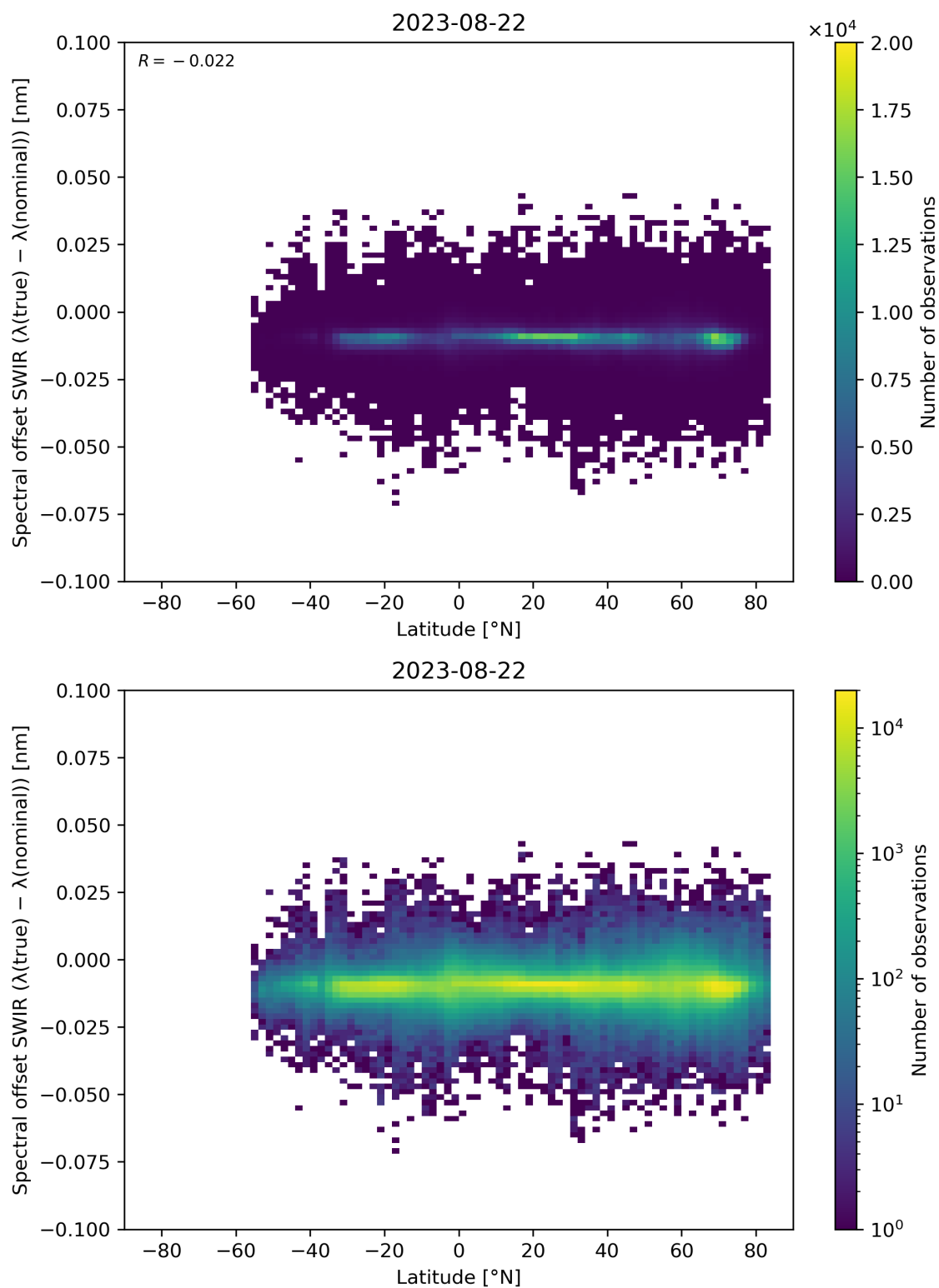
Figure 62: Scatter density plot of “Latitude” against “Spectral offset SWIR ( \lambda(\text{true}) - \lambda(\text{nominal}) )” for 2023-08-21 to 2023-08-23.
