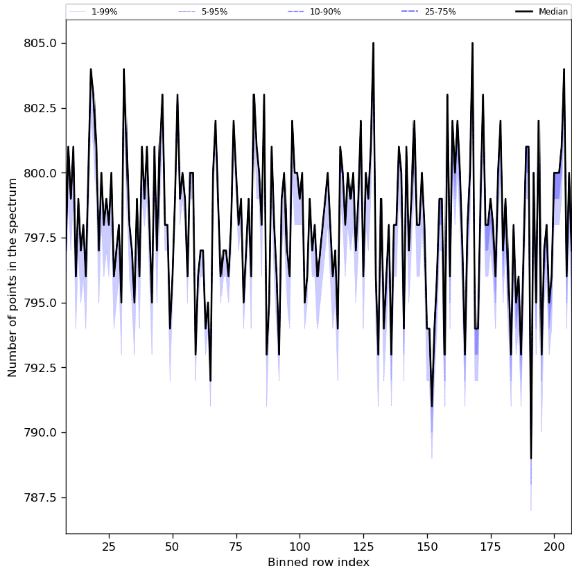
Figure 37: Along track statistics of “Number of points in the spectrum” for 2023-08-21 to 2023-08-23
