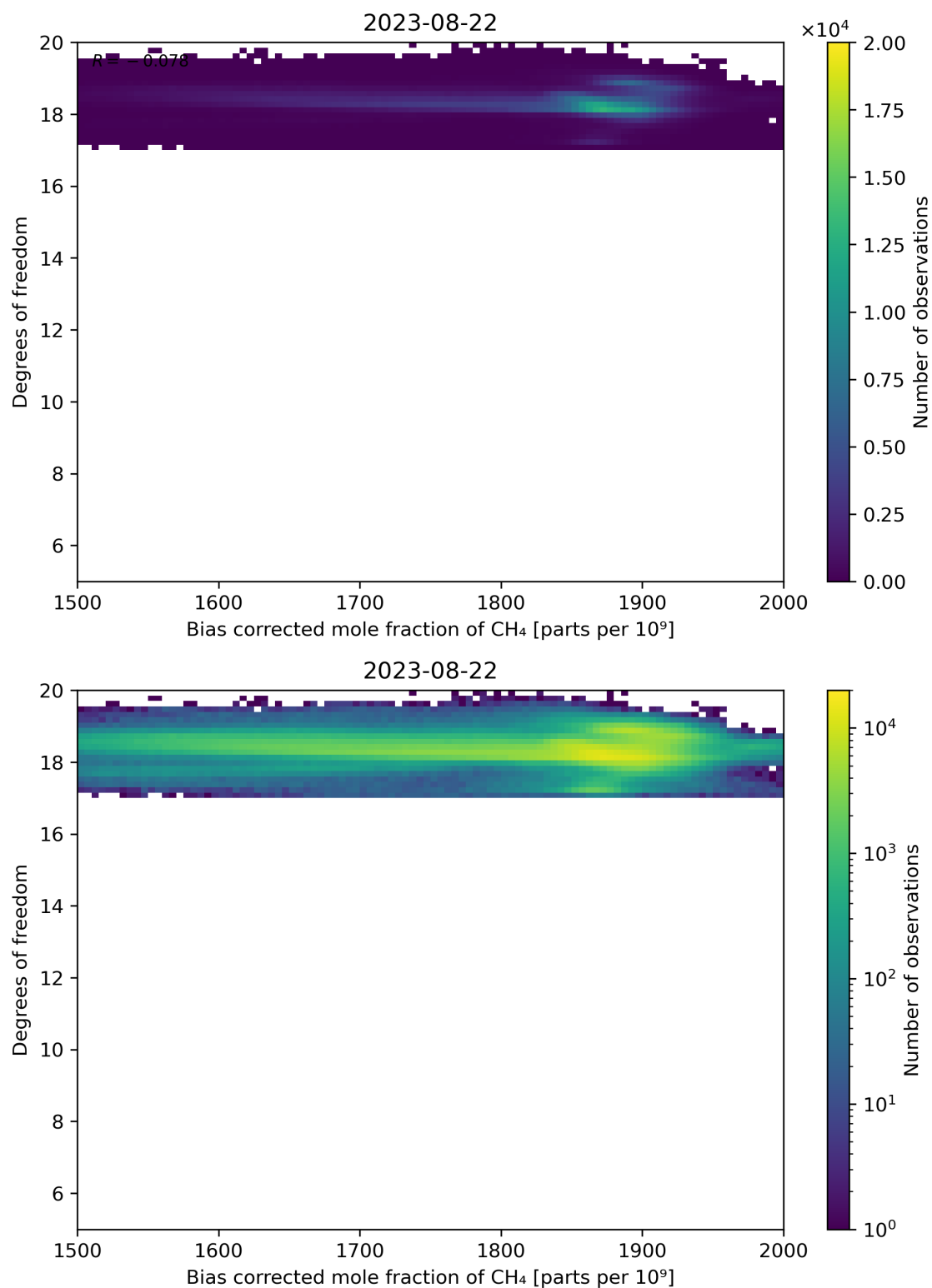
Figure 65: Scatter density plot of “Bias corrected mole fraction of CH 4 ” against “Degrees of freedom” for 2023-08-21 to 2023-08-23.
