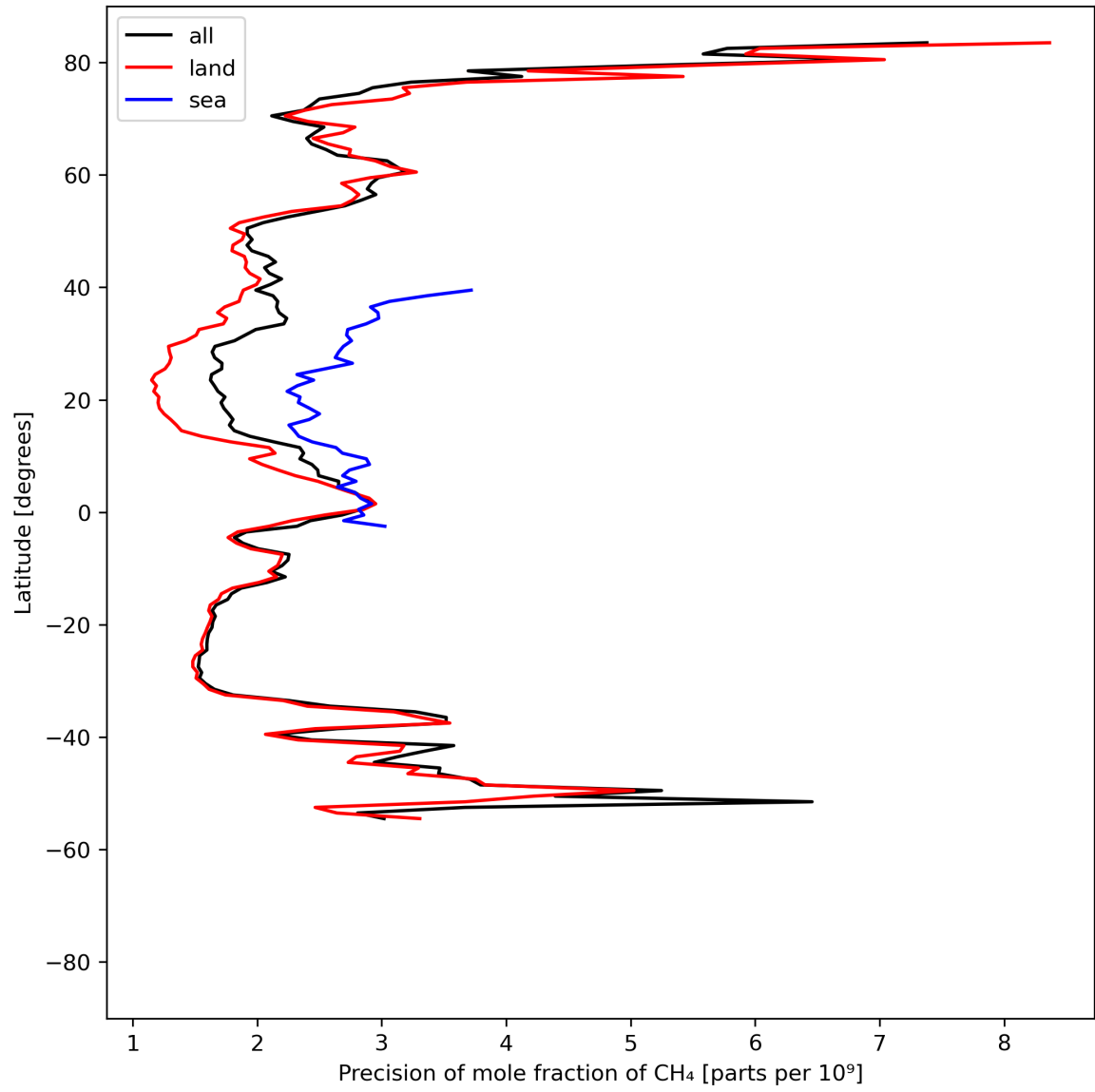
Figure 13: Zonal average of “Precision of mole fraction of CH 4 ” for 2023-08-21 to 2023-08-23.
