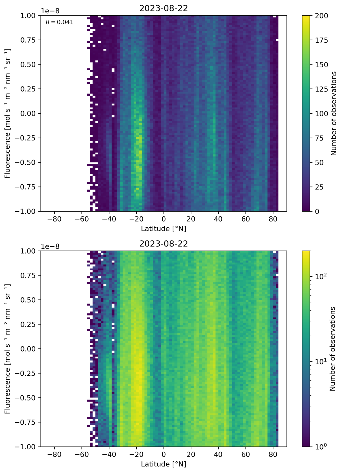
Figure 56: Scatter density plot of “Latitude” against “Fluorescence” for 2023-08-21 to 2023-08-23.
