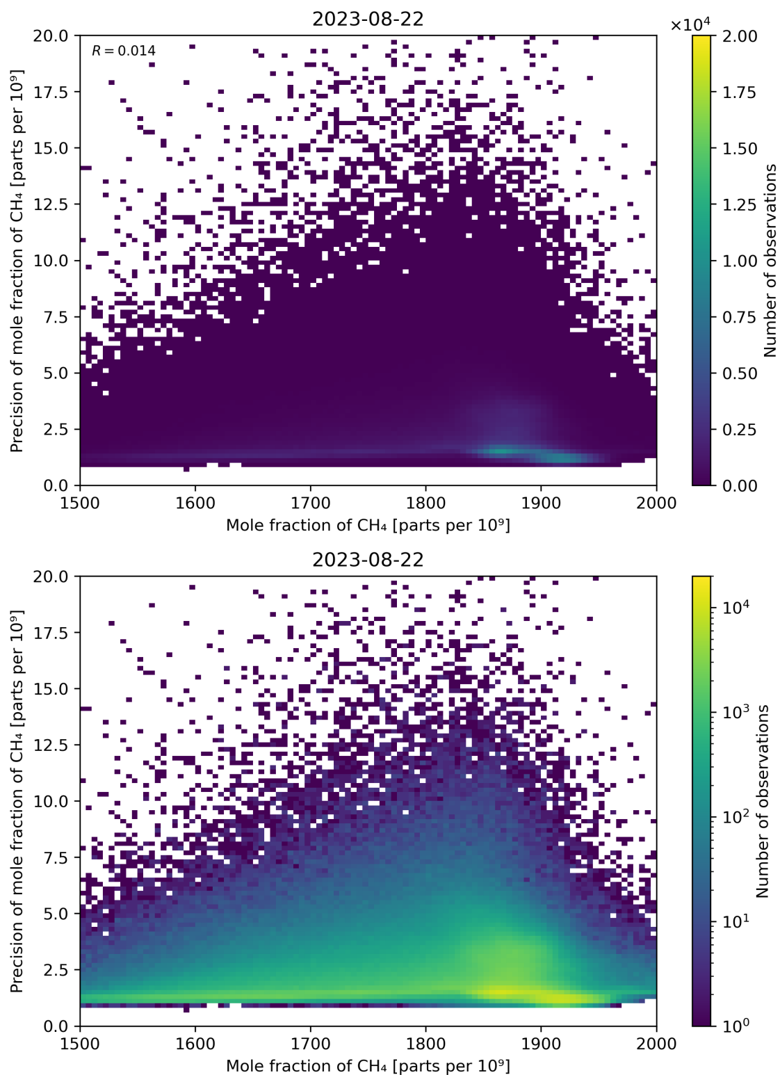
Figure 75: Scatter density plot of “Mole fraction of CH 4 ” against “Precision of mole fraction of CH 4 ” for 2023-08-21 to 2023-08-23.
