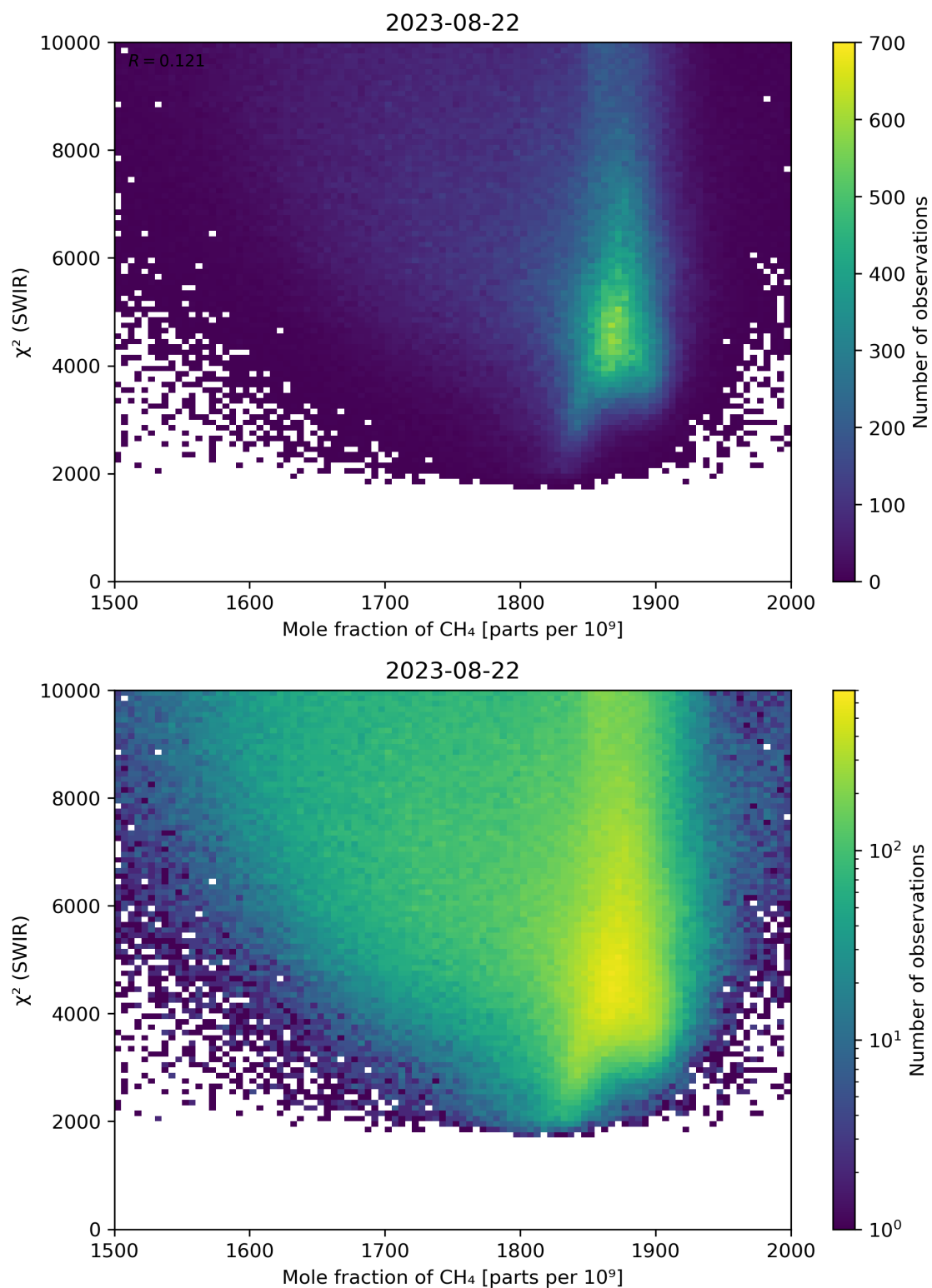
Figure 71: Scatter density plot of “Mole fraction of \text{CH}_4 ” against “ \chi^2 (SWIR)” for 2023-08-21 to 2023-08-23.
