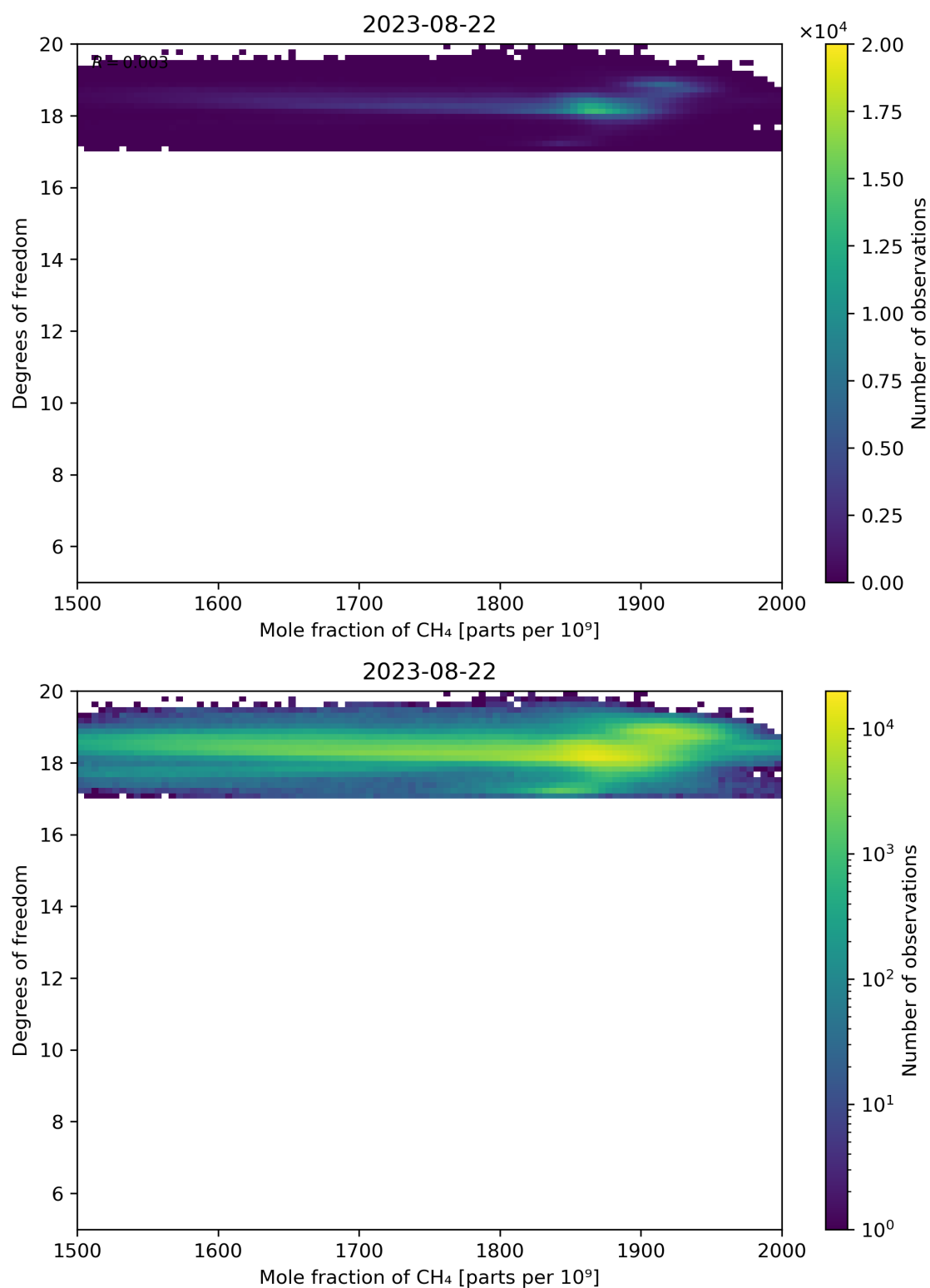
Figure 72: Scatter density plot of “Mole fraction of CH 4 ” against “Degrees of freedom” for 2023-08-21 to 2023-08-23.
