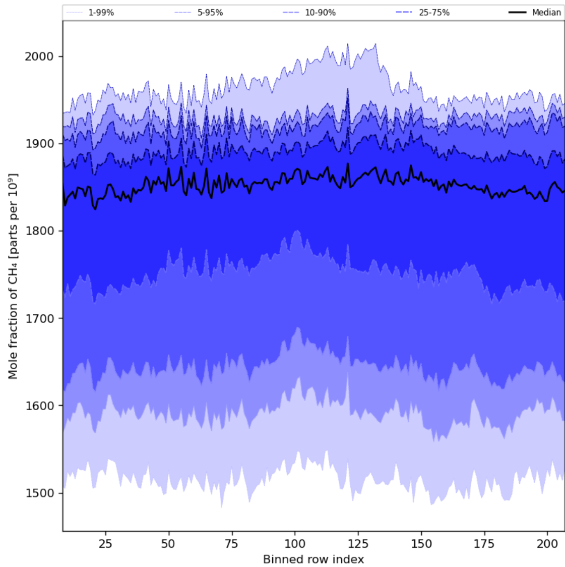
Figure 34: Along track statistics of “Mole fraction of CH 4 ” for 2023-08-21 to 2023-08-23
