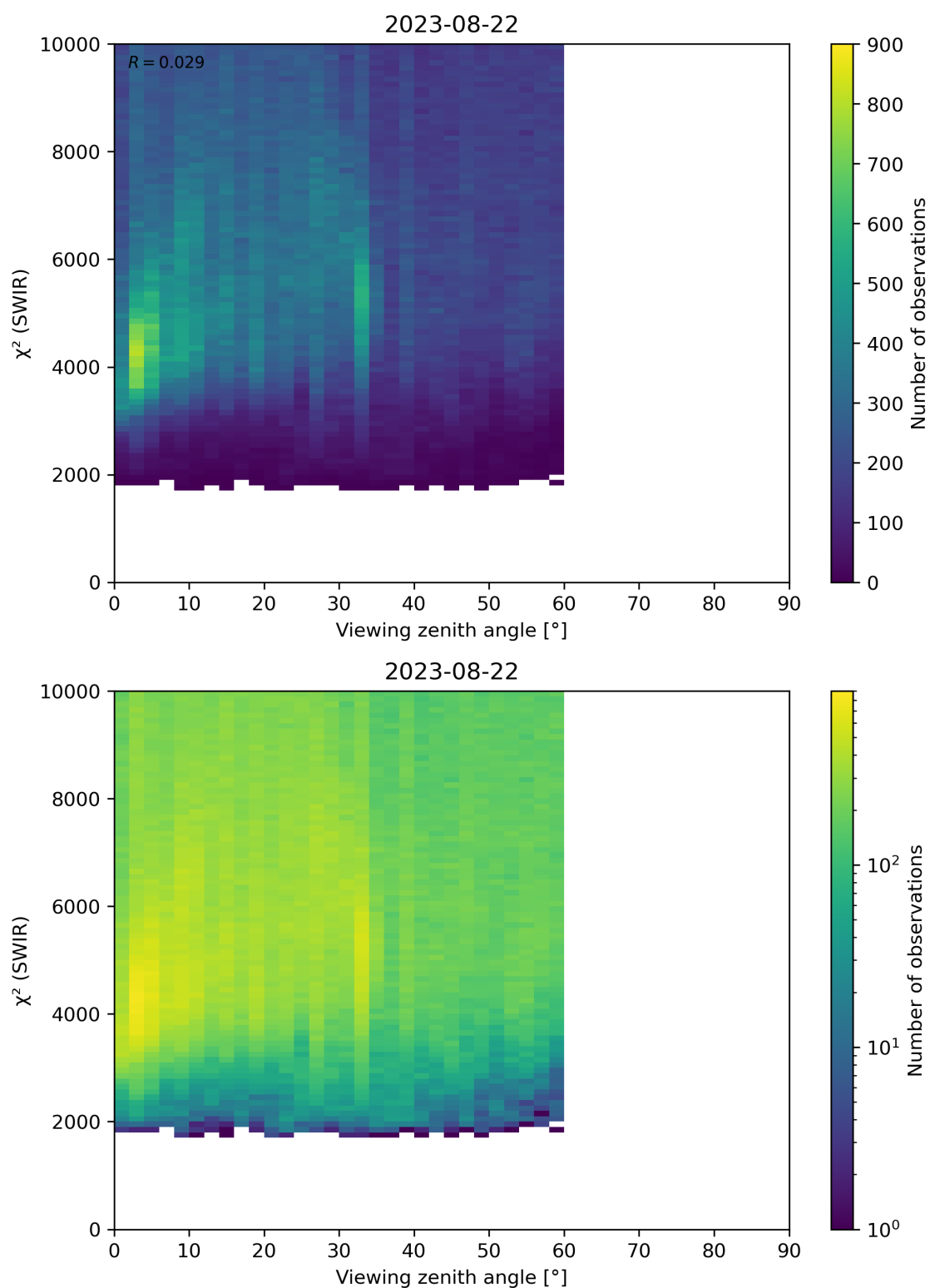
Figure 106: Scatter density plot of “Viewing zenith angle” against “ \chi^2 (SWIR)” for 2023-08-21 to 2023-08-23.
