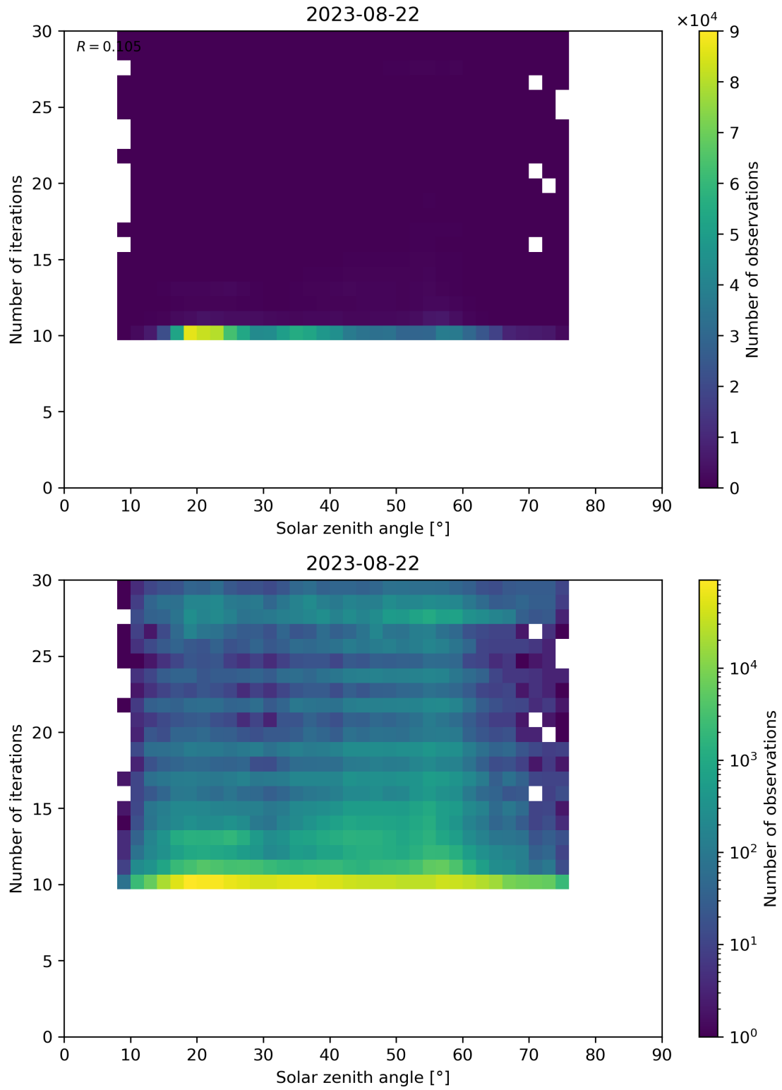
Figure 102: Scatter density plot of “Solar zenith angle” against “Number of iterations” for 2023-08-21 to 2023-08-23.
