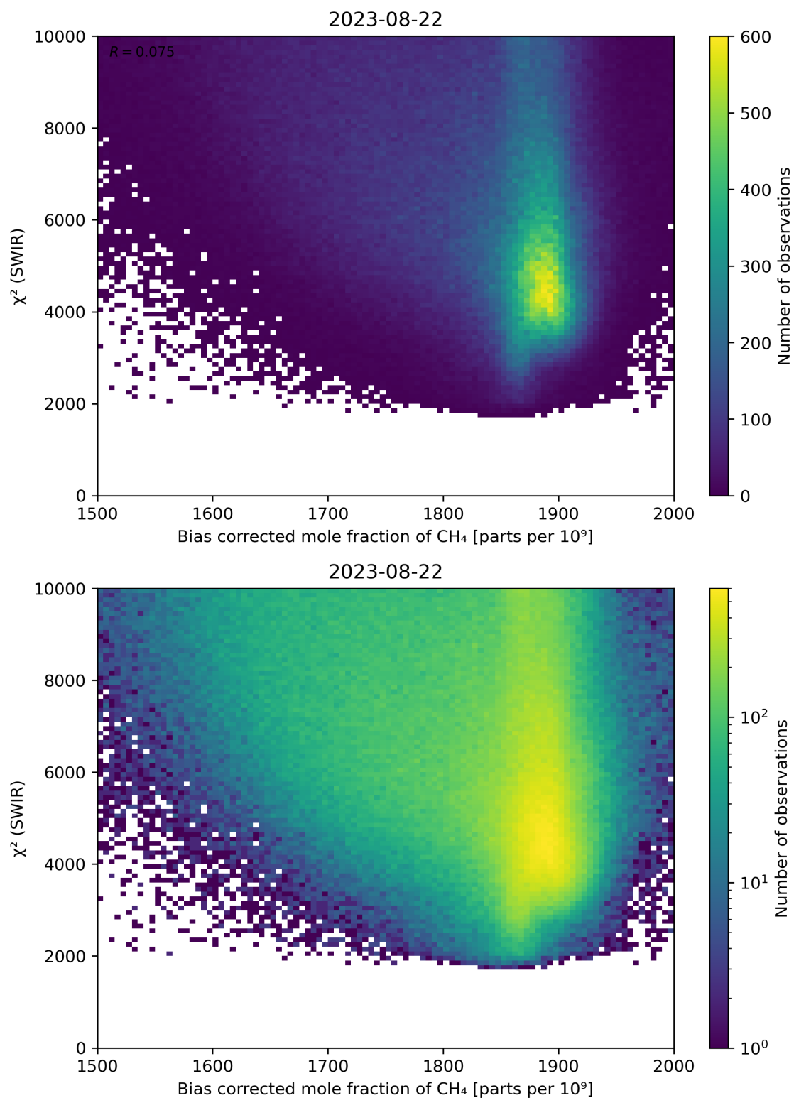
Figure 64: Scatter density plot of “Bias corrected mole fraction of \text{CH}_4 ” against “ \chi^2 (SWIR)” for 2023-08-21 to 2023-08-23.
