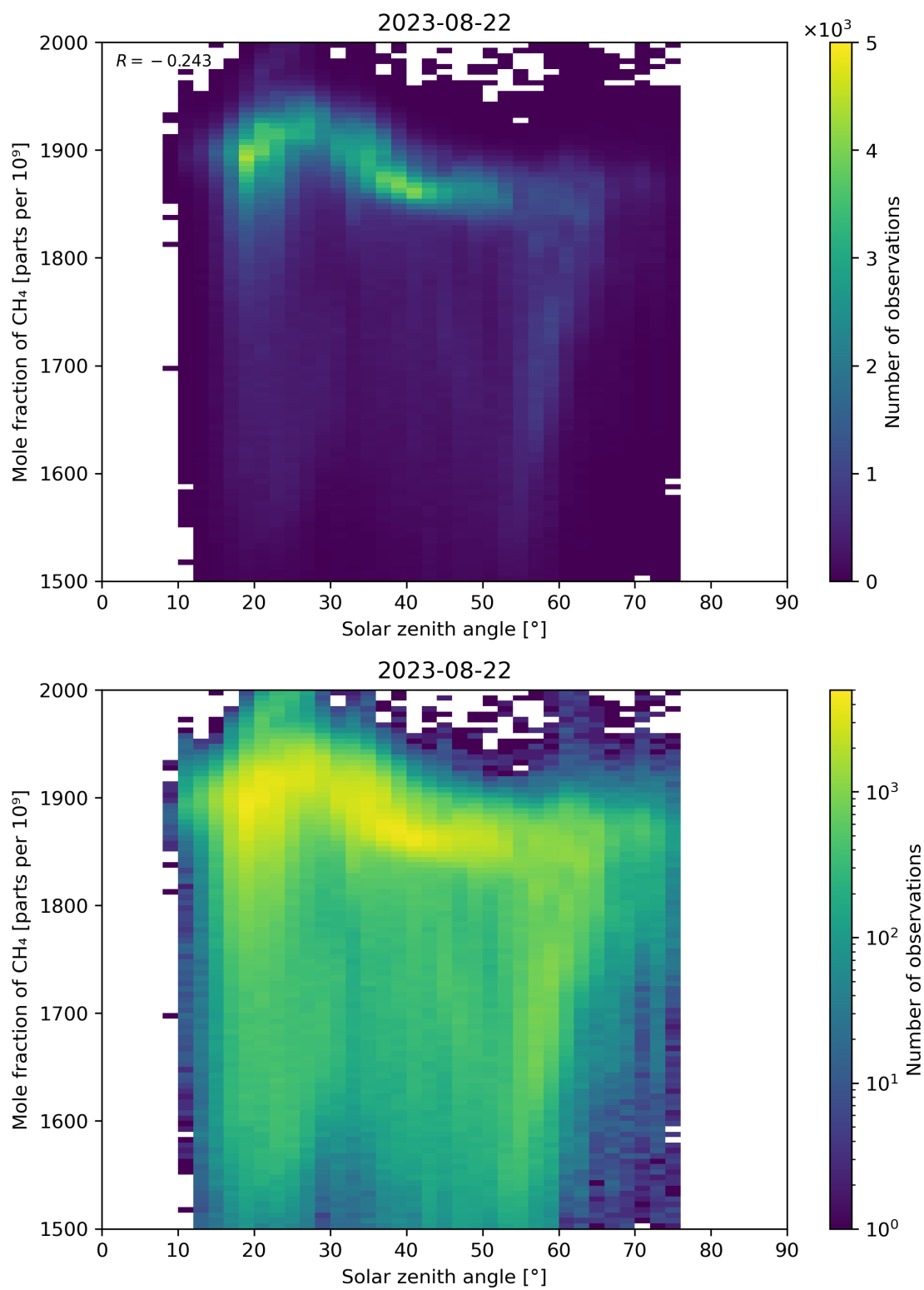
Figure 99: Scatter density plot of “Solar zenith angle” against “Mole fraction of CH 4 ” for 2023-08-21 to 2023-08-23.
