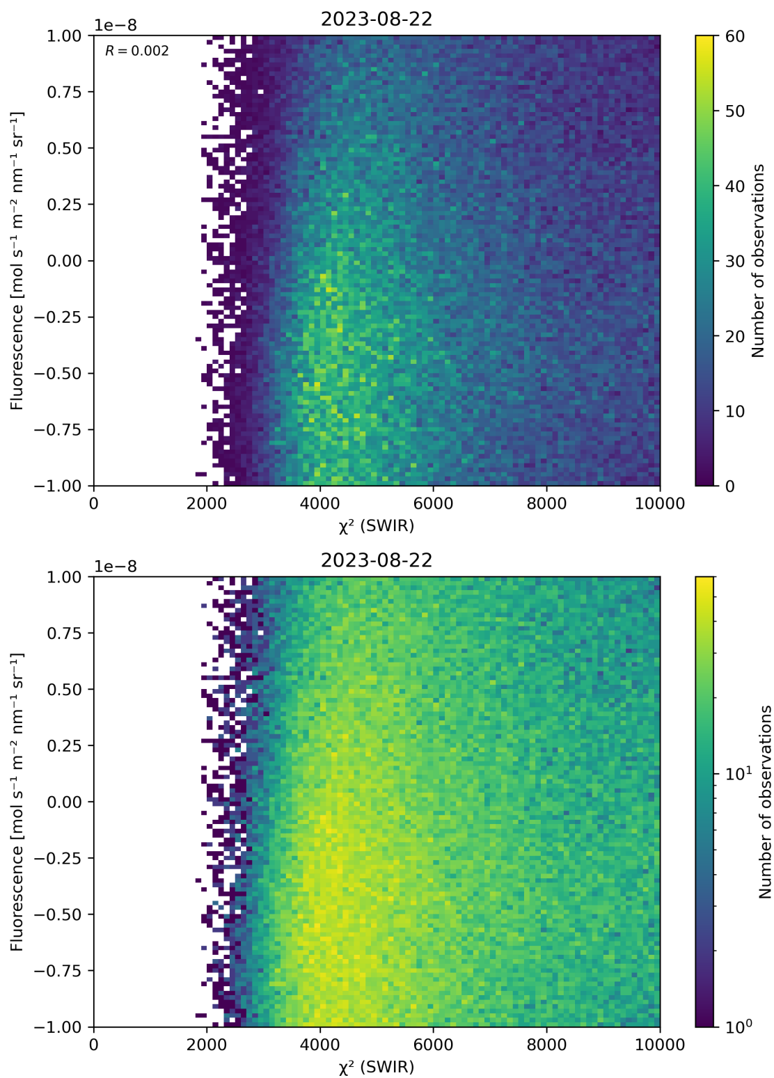
Figure 49: Scatter density plot of “ \chi^2 (SWIR)” against “Fluorescence” for 2023-08-21 to 2023-08-23.
