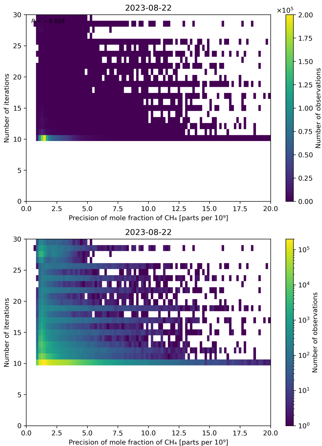
Figure 83: Scatter density plot of “Precision of mole fraction of CH 4 ” against “Number of iterations” for 2023-08-21 to 2023-08-23.
