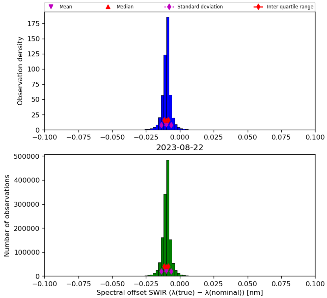
Figure 27: Histogram of “Spectral offset SWIR ( \lambda(\text{true}) - \lambda(\text{nominal}) )” for 2023-08-21 to 2023-08-23
