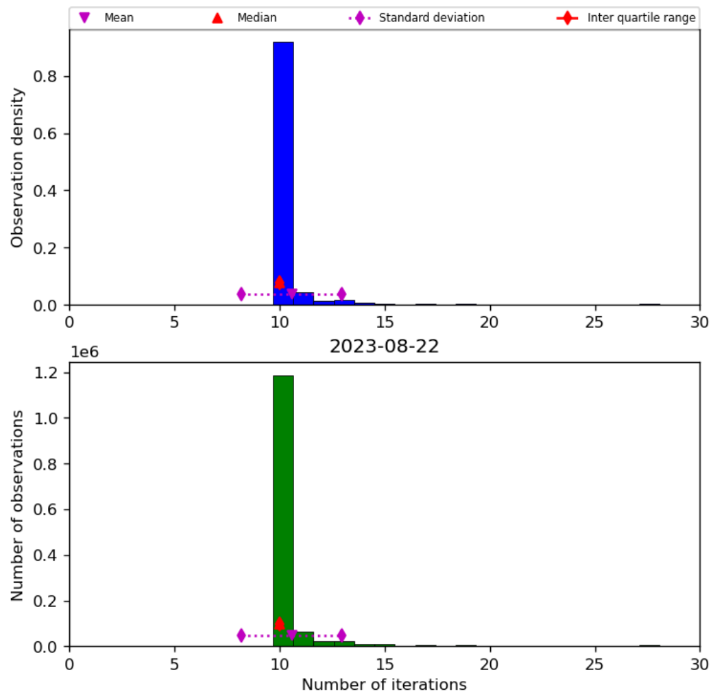
Figure 31: Histogram of “Number of iterations” for 2023-08-21 to 2023-08-23
