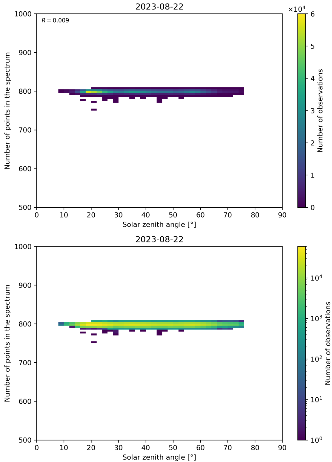
Figure 103: Scatter density plot of “Solar zenith angle” against “Number of points in the spectrum” for 2023-08-21 to 2023-08-23.
