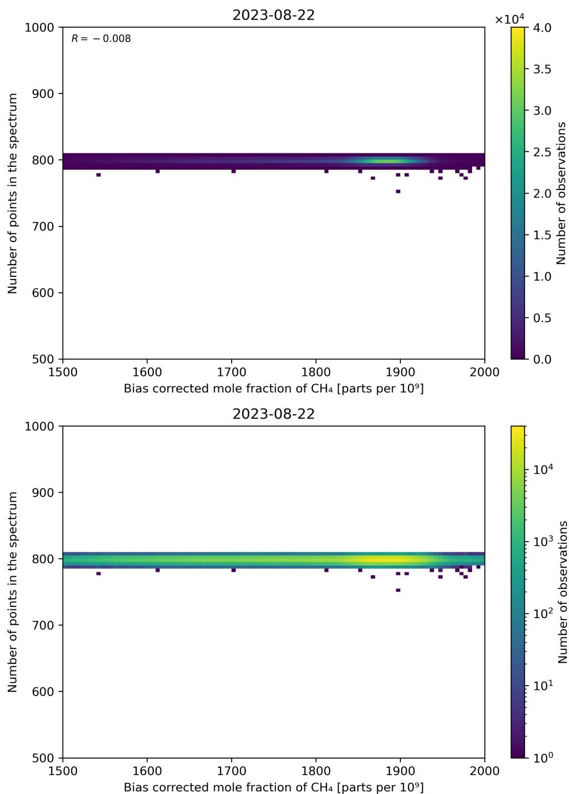
Figure 68: Scatter density plot of “Bias corrected mole fraction of CH 4 ” against “Number of points in the spectrum” for 2023-08-21 to 2023-08-23.
