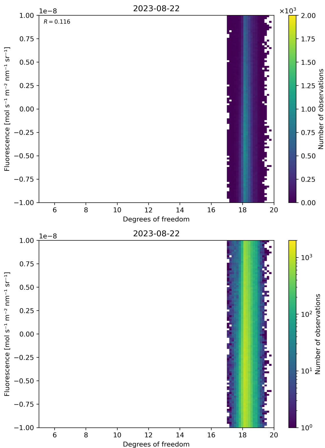
Figure 51: Scatter density plot of “Degrees of freedom” against “Fluorescence” for 2023-08-21 to 2023-08-23.
