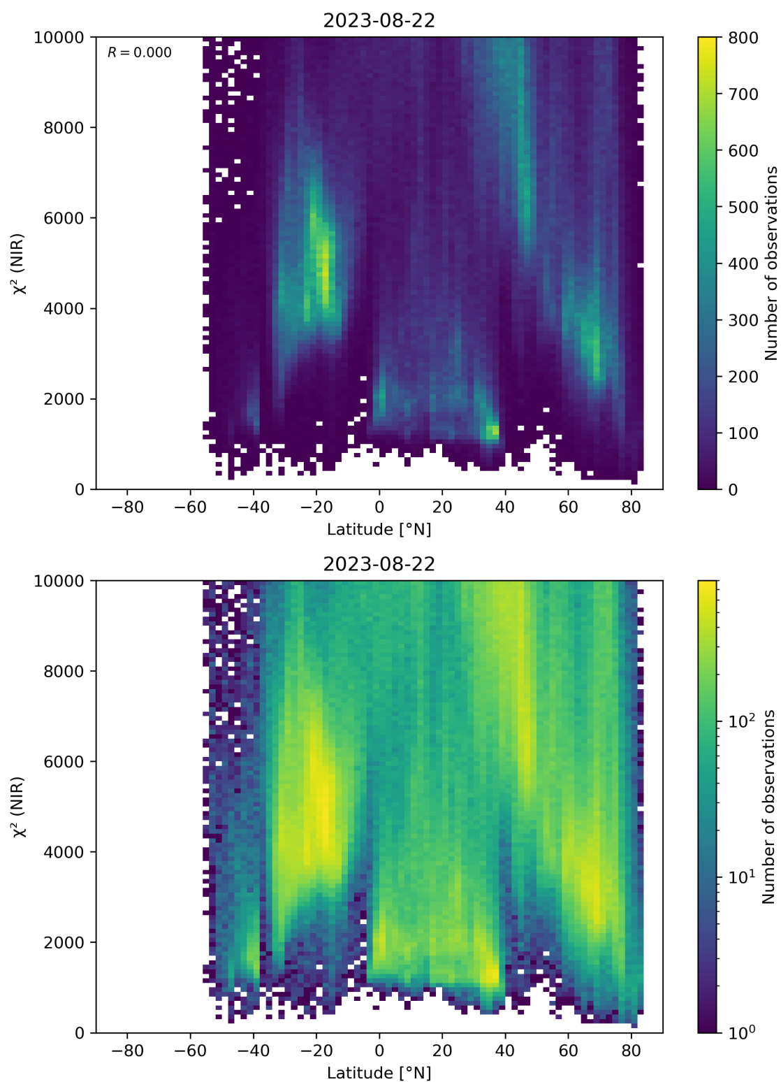
Figure 53: Scatter density plot of “Latitude” against “ \chi^2 (NIR)” for 2023-08-21 to 2023-08-23.
