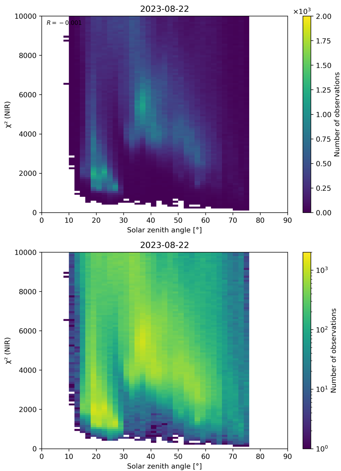
Figure 94: Scatter density plot of “Solar zenith angle” against “ \chi^2 (NIR)” for 2023-08-21 to 2023-08-23.
