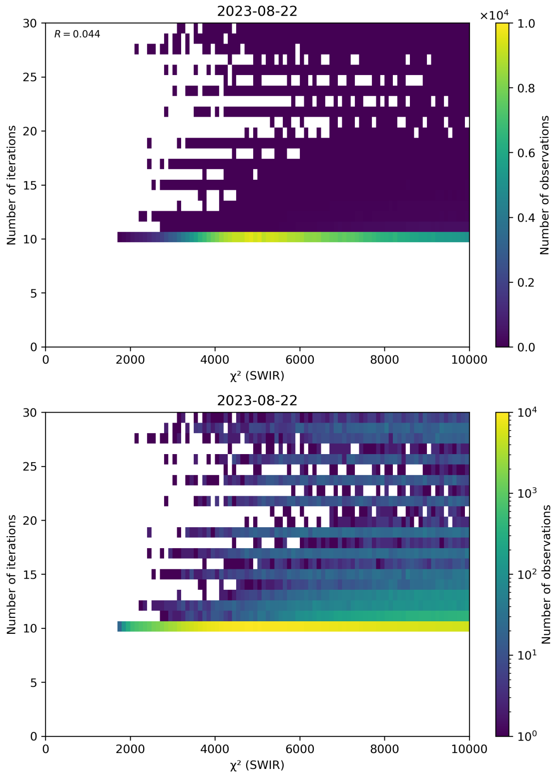
Figure 50: Scatter density plot of “ \chi^2 (SWIR)” against “Number of iterations” for 2023-08-21 to 2023-08-23.
