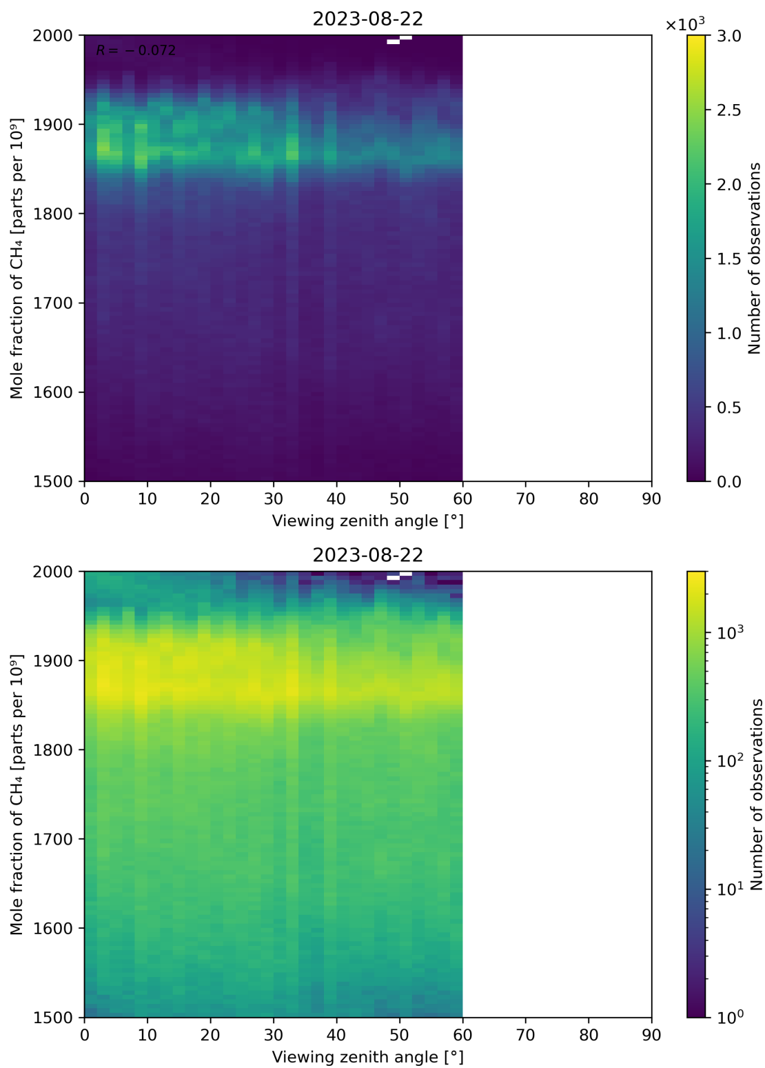
Figure 110: Scatter density plot of “Viewing zenith angle” against “Mole fraction of CH 4 ” for 2023-08-21 to 2023-08-23.
