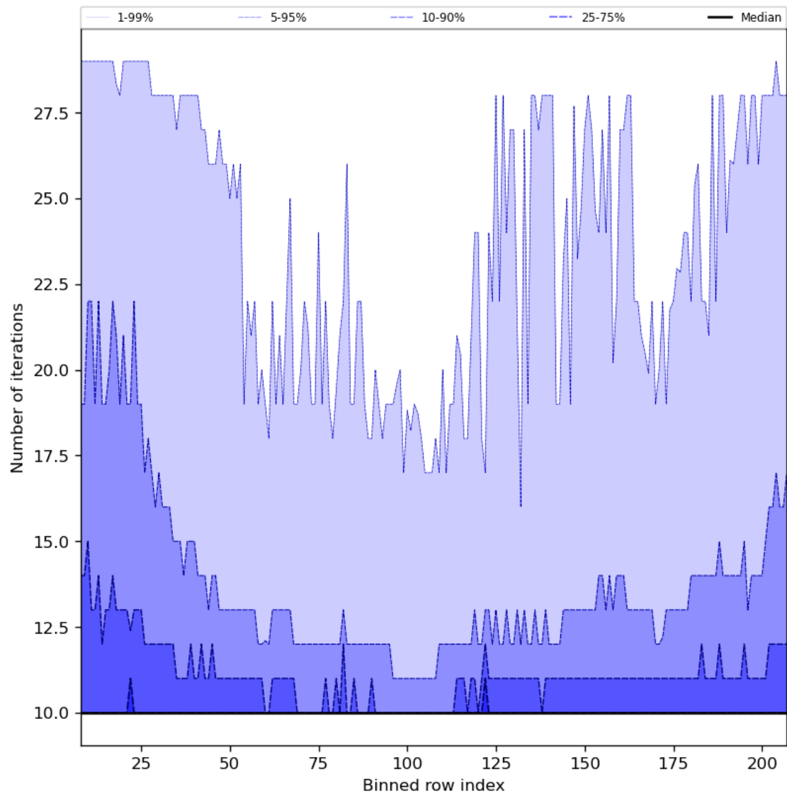
Figure 42: Along track statistics of “Number of iterations” for 2023-08-21 to 2023-08-23
