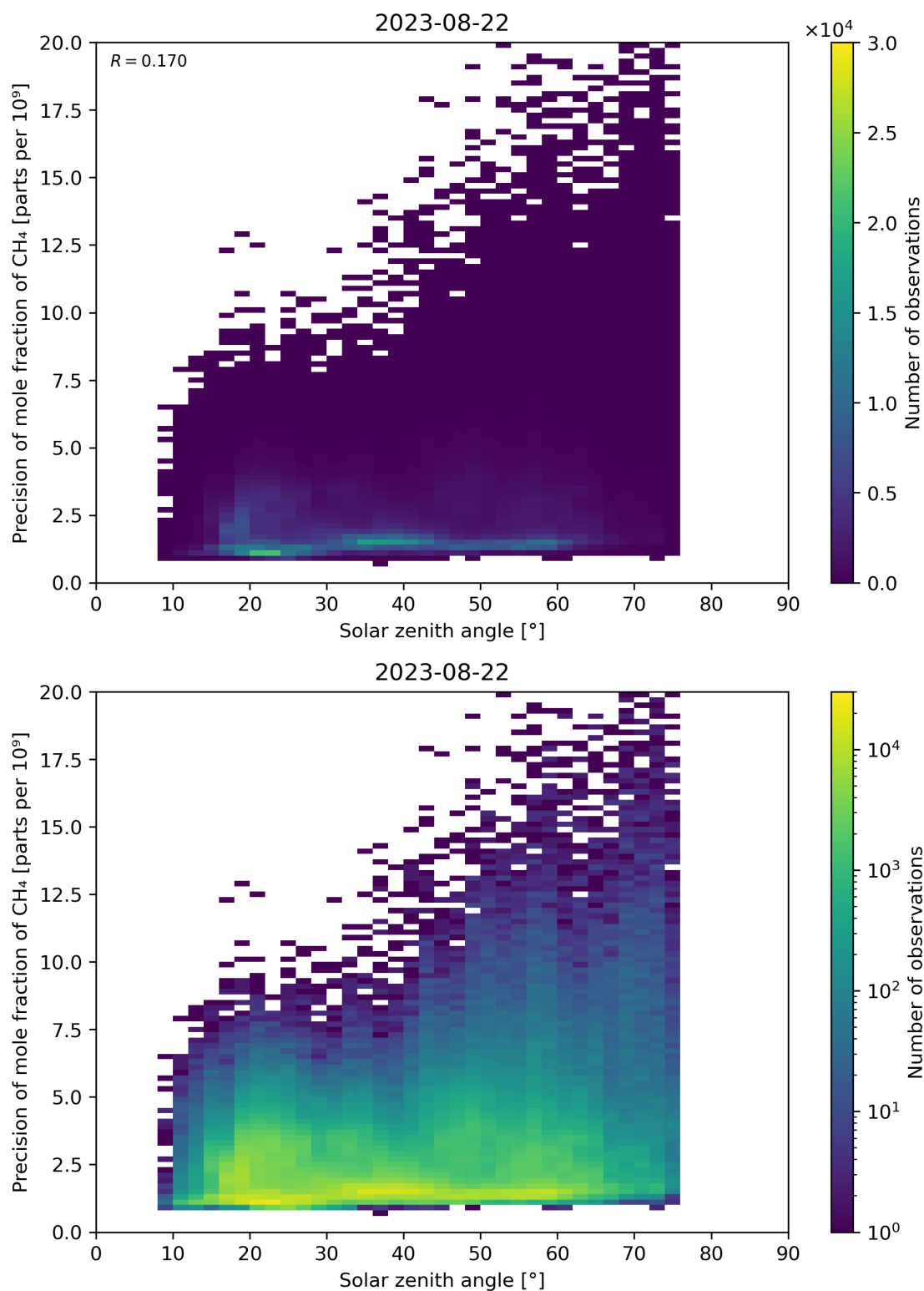
Figure 101: Scatter density plot of “Solar zenith angle” against “Precision of mole fraction of CH 4 ” for 2023-08-21 to 2023-08-23.
