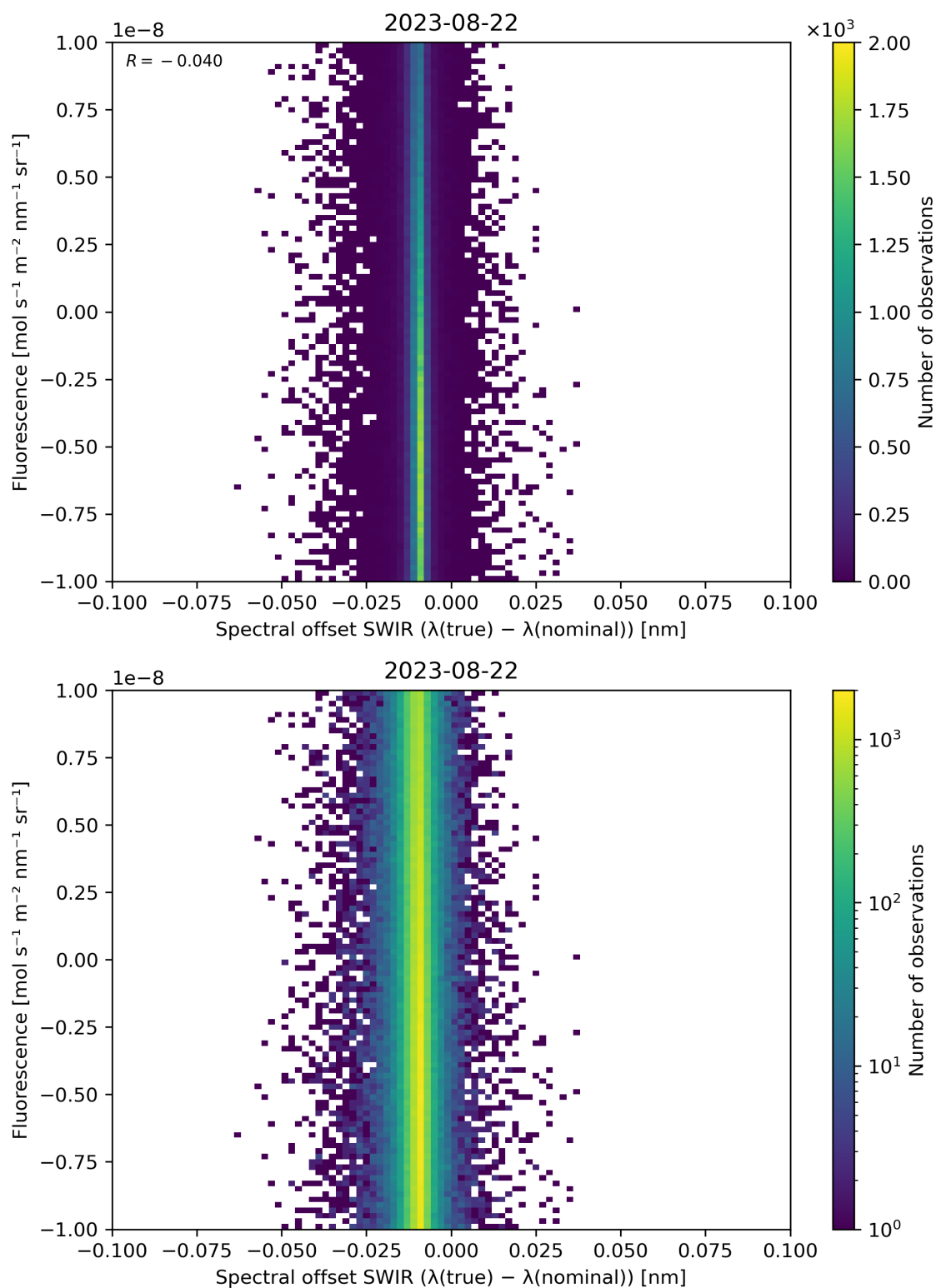
Figure 120: Scatter density plot of “Spectral offset SWIR ( \lambda(\text{true}) - \lambda(\text{nominal}) )” against “Fluorescence” for 2023-08-21 to 2023-08-23.
