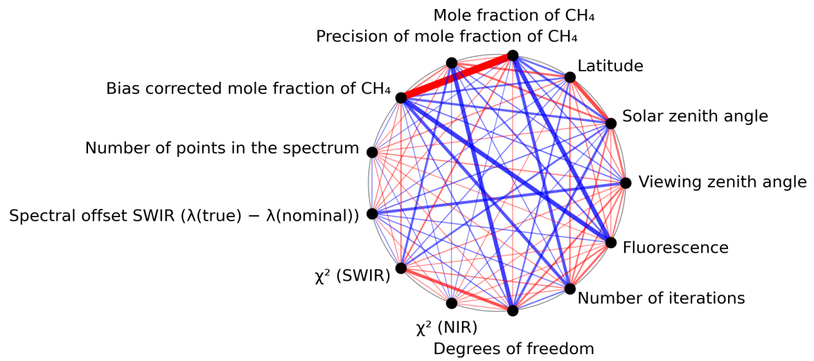
Figure 1: Map of correlation graph for 2023-08-21 to 2023-08-23.
