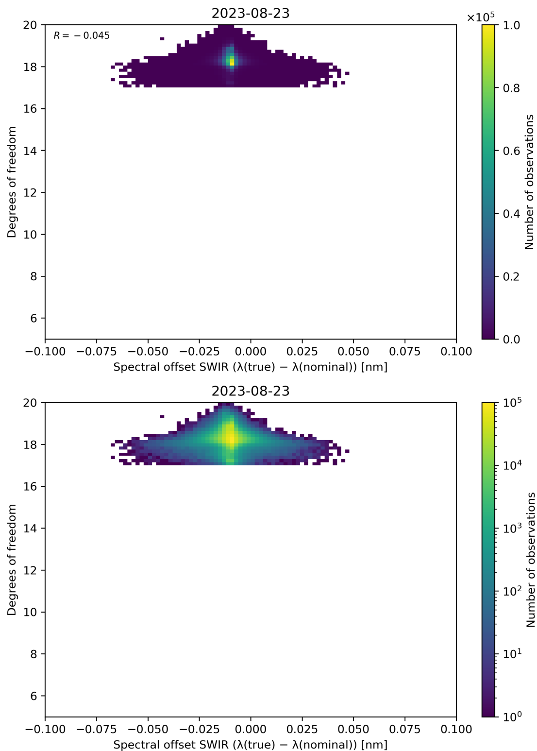
Figure 119: Scatter density plot of “Spectral offset SWIR ( \lambda(\text{true}) - \lambda(\text{nominal}) )” against “Degrees of freedom” for 2023-08-22 to 2023-08-24.
