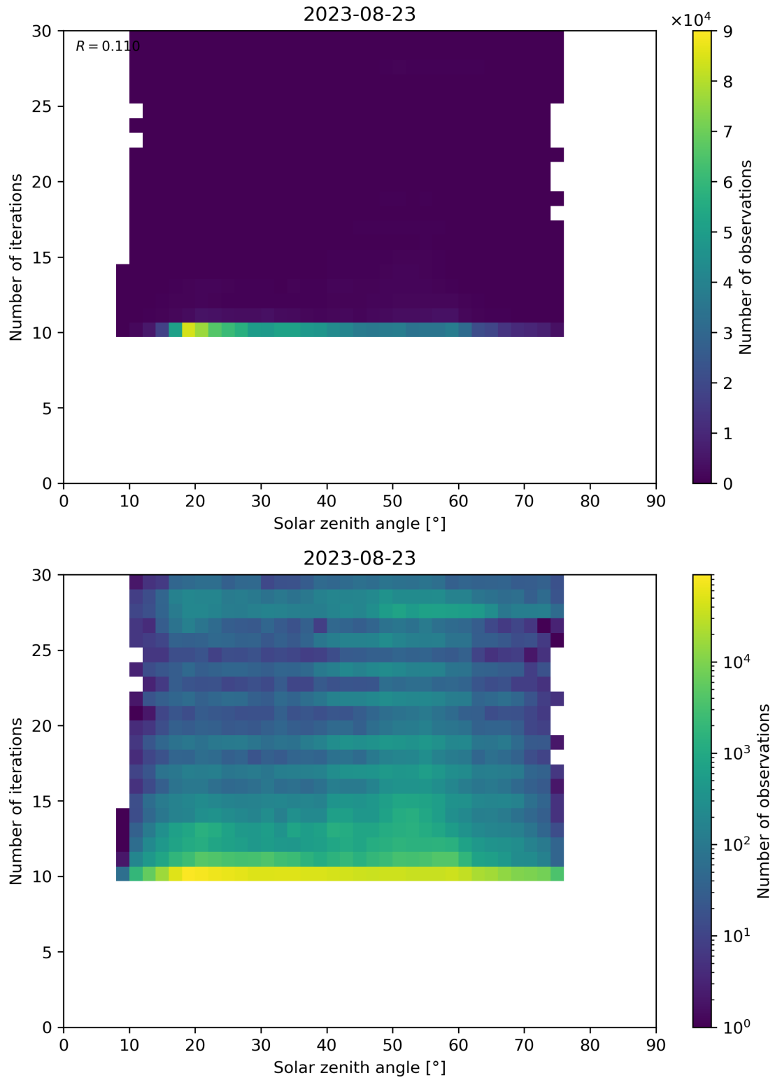
Figure 102: Scatter density plot of “Solar zenith angle” against “Number of iterations” for 2023-08-22 to 2023-08-24.
