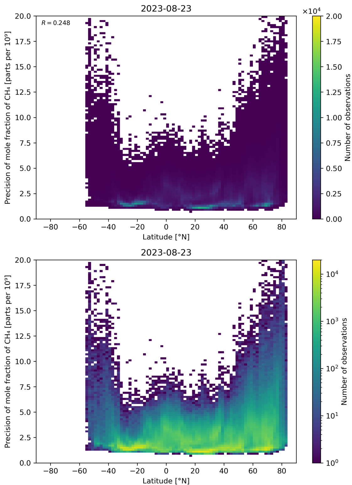
Figure 59: Scatter density plot of “Latitude” against “Precision of mole fraction of CH 4 ” for 2023-08-22 to 2023-08-24.
