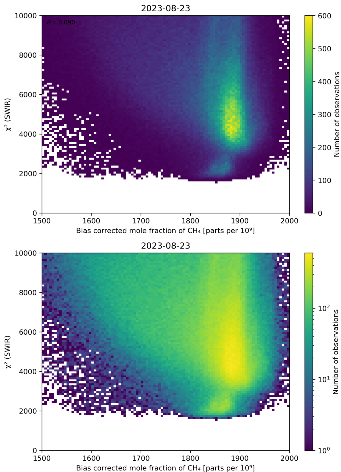
Figure 64: Scatter density plot of “Bias corrected mole fraction of \text{CH}_4 ” against “ \chi^2 (SWIR)” for 2023-08-22 to 2023-08-24.
