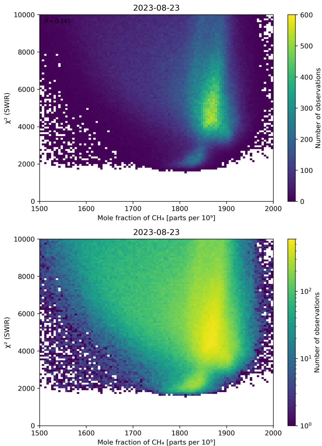
Figure 71: Scatter density plot of “Mole fraction of \text{CH}_4 ” against “ \chi^2 (SWIR)” for 2023-08-22 to 2023-08-24.
