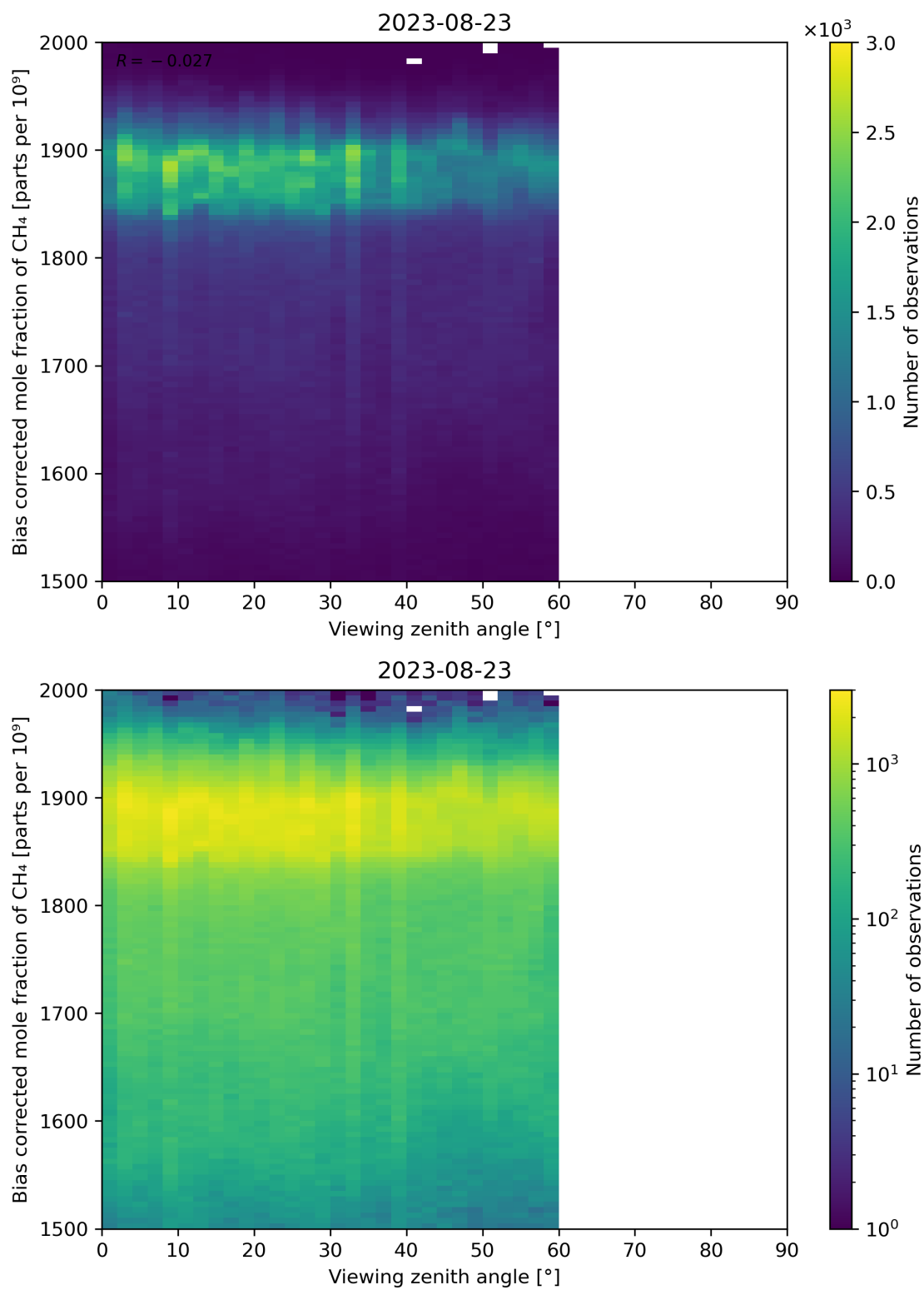
Figure 111: Scatter density plot of “Viewing zenith angle” against “Bias corrected mole fraction of CH 4 ” for 2023-08-22 to 2023-08-24.
