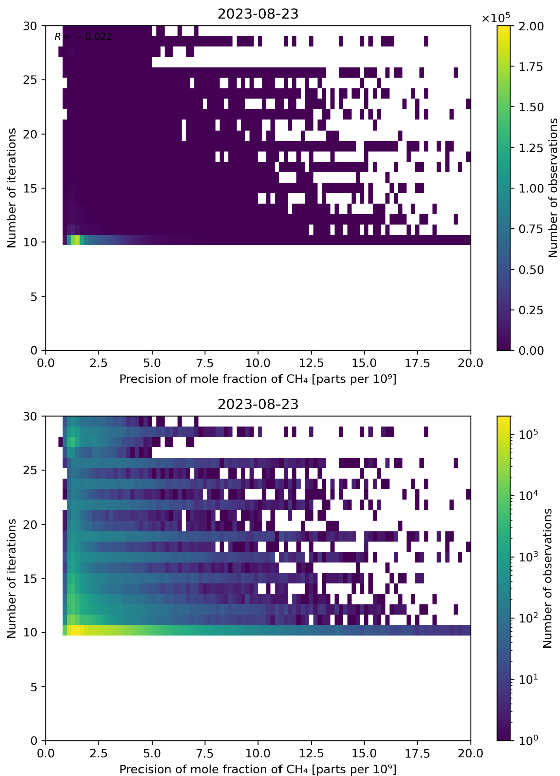
Figure 83: Scatter density plot of “Precision of mole fraction of CH 4 ” against “Number of iterations” for 2023-08-22 to 2023-08-24.
