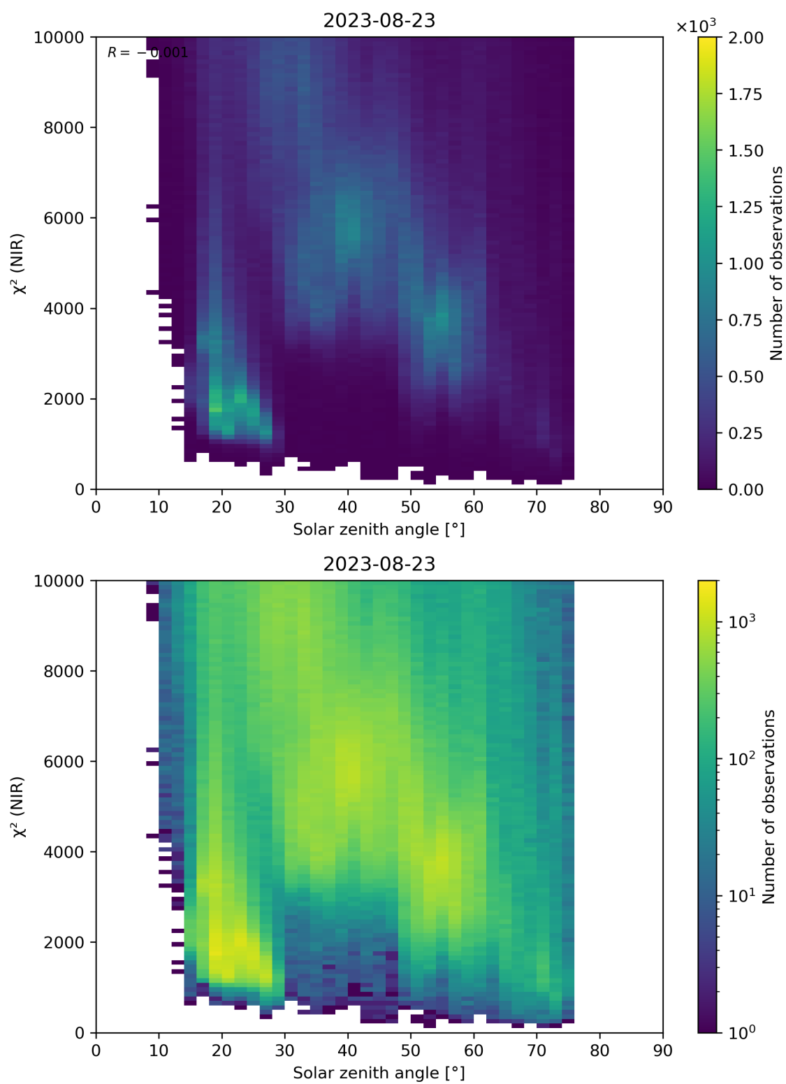
Figure 94: Scatter density plot of “Solar zenith angle” against “ \chi^2 (NIR)” for 2023-08-22 to 2023-08-24.
