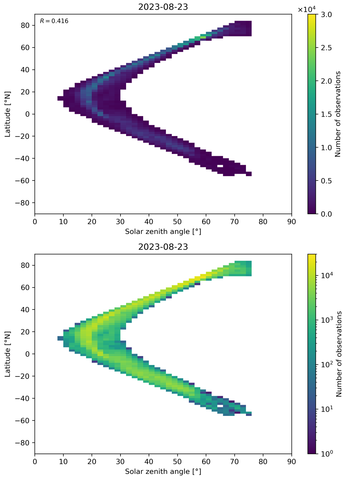
Figure 98: Scatter density plot of “Solar zenith angle” against “Latitude” for 2023-08-22 to 2023-08-24.
