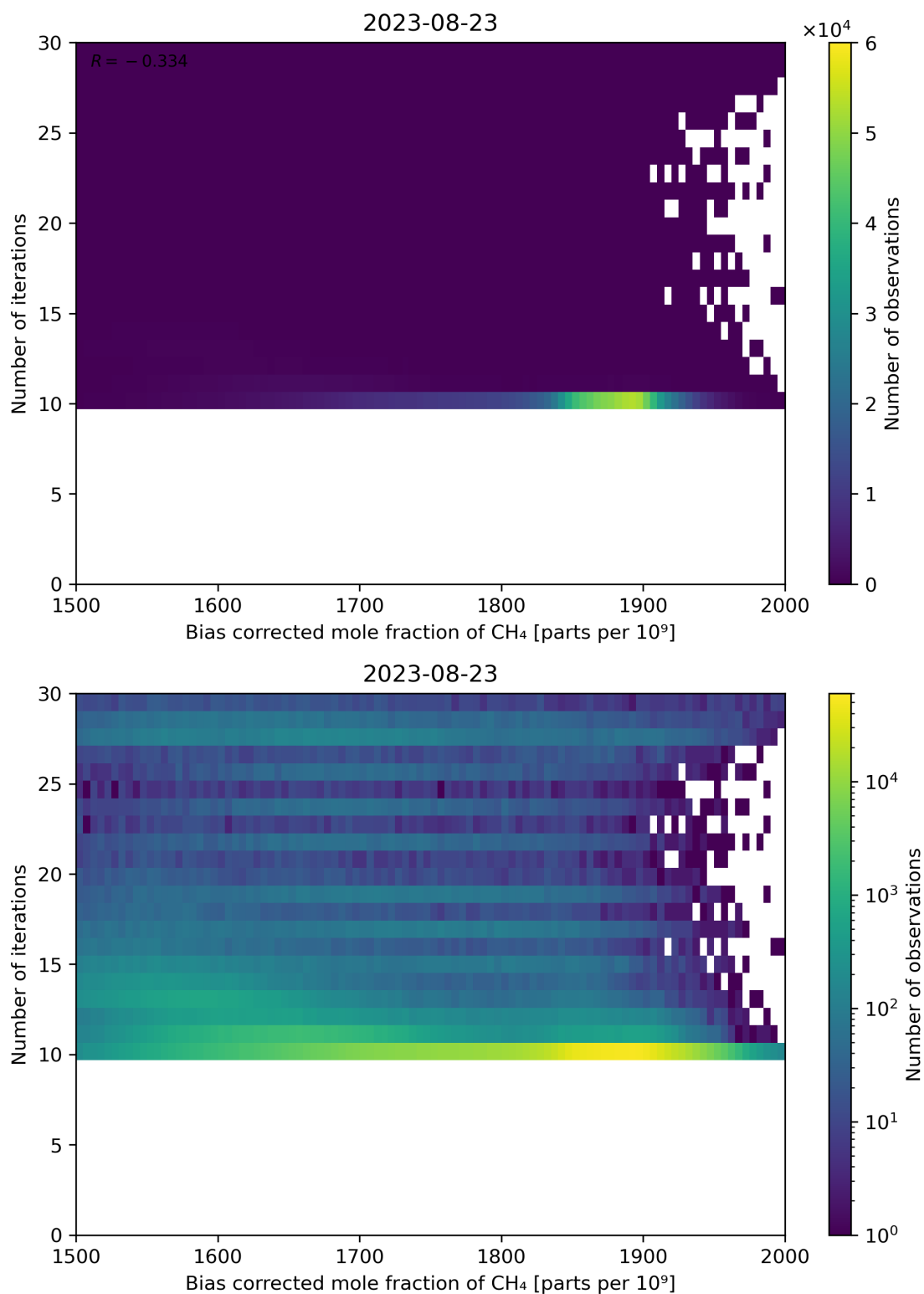
Figure 67: Scatter density plot of “Bias corrected mole fraction of CH 4 ” against “Number of iterations” for 2023-08-22 to 2023-08-24.
