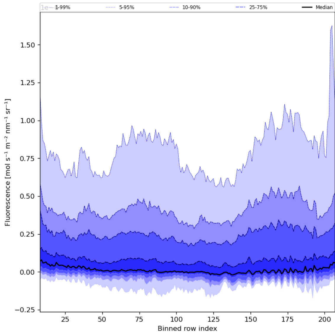
Figure 43: Along track statistics of “Fluorescence” for 2023-08-22 to 2023-08-24
