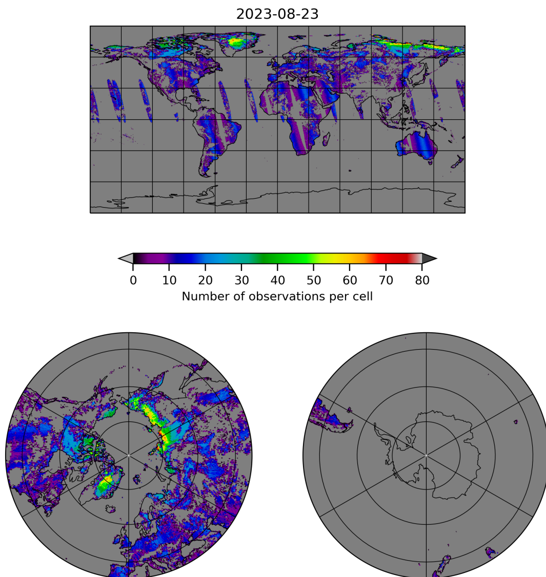
Figure 10: Map of the number of observations for 2023-08-22 to 2023-08-24
