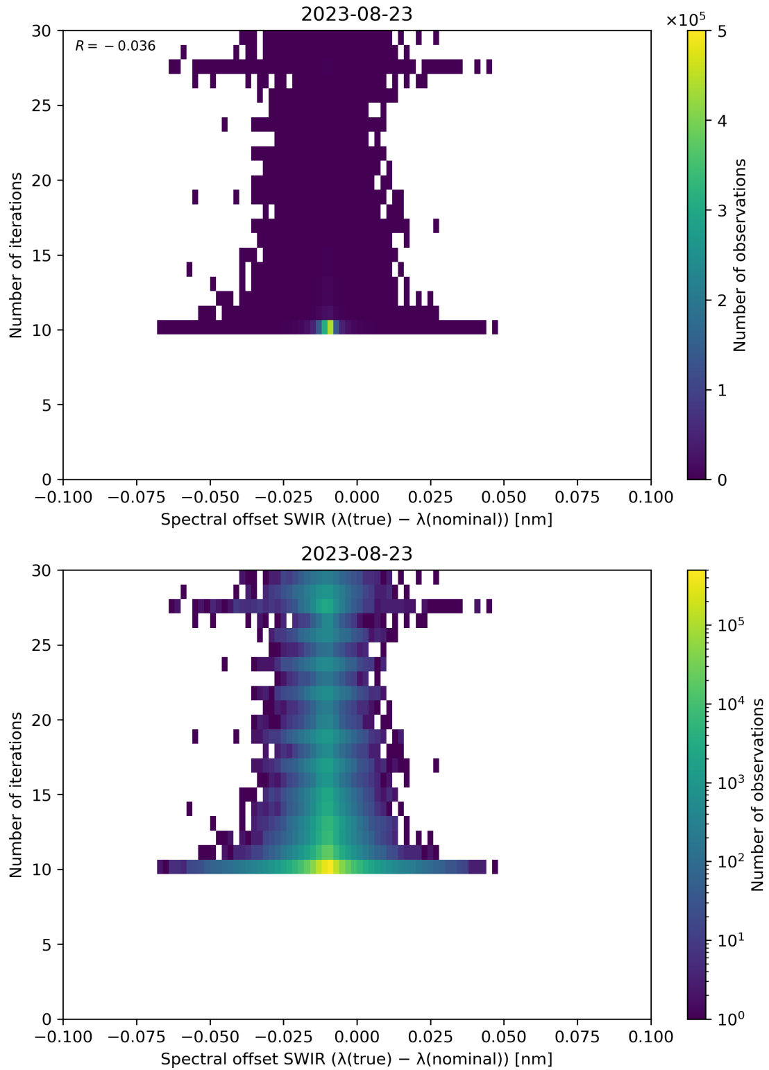
Figure 121: Scatter density plot of “Spectral offset SWIR ( \lambda(\text{true}) - \lambda(\text{nominal}) )” against “Number of iterations” for 2023-08-22 to 2023-08-24.
