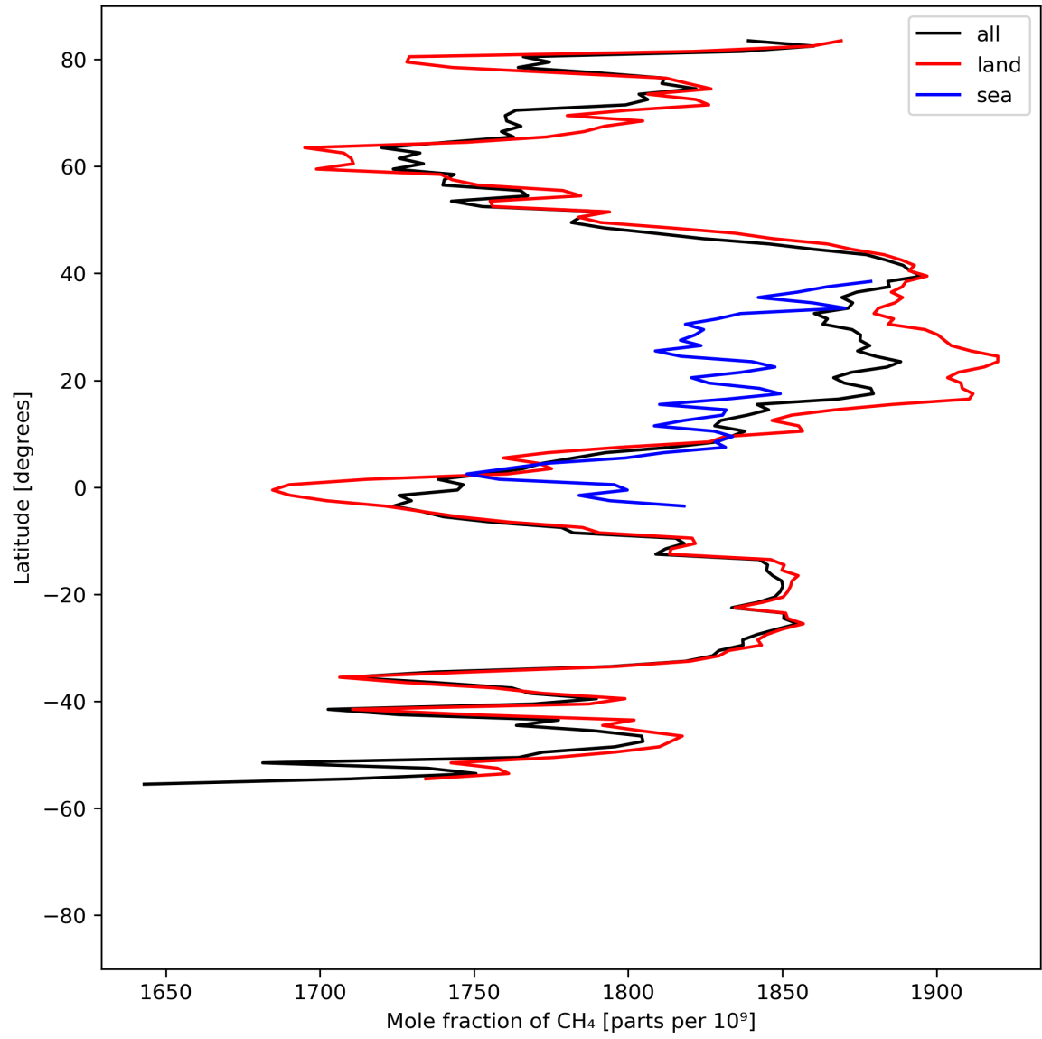
Figure 12: Zonal average of “Mole fraction of \text{CH}_4 ” for 2023-08-22 to 2023-08-24.
