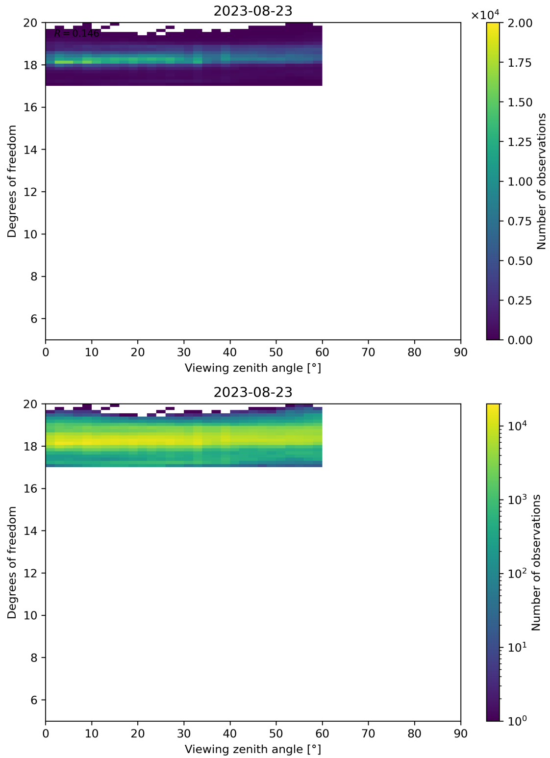
Figure 107: Scatter density plot of “Viewing zenith angle” against “Degrees of freedom” for 2023-08-22 to 2023-08-24.
