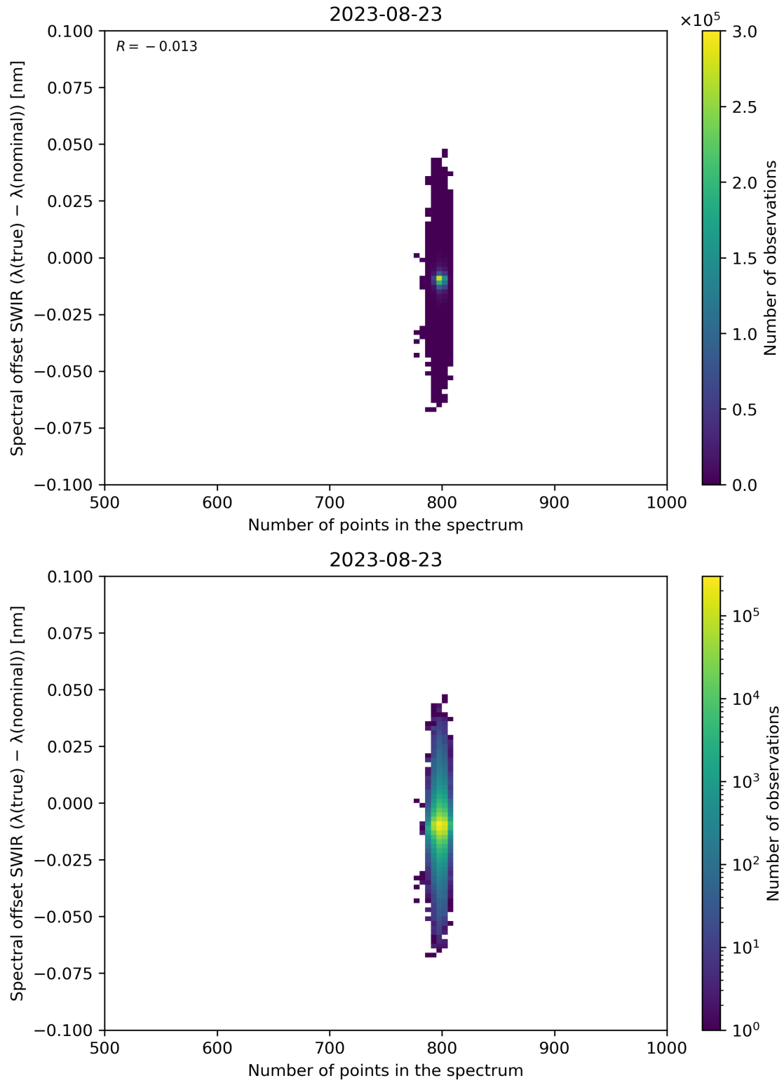
Figure 93: Scatter density plot of “Number of points in the spectrum” against “Spectral offset SWIR ( \lambda(\text{true}) - \lambda(\text{nominal}) )” for 2023-08-22 to 2023-08-24.
