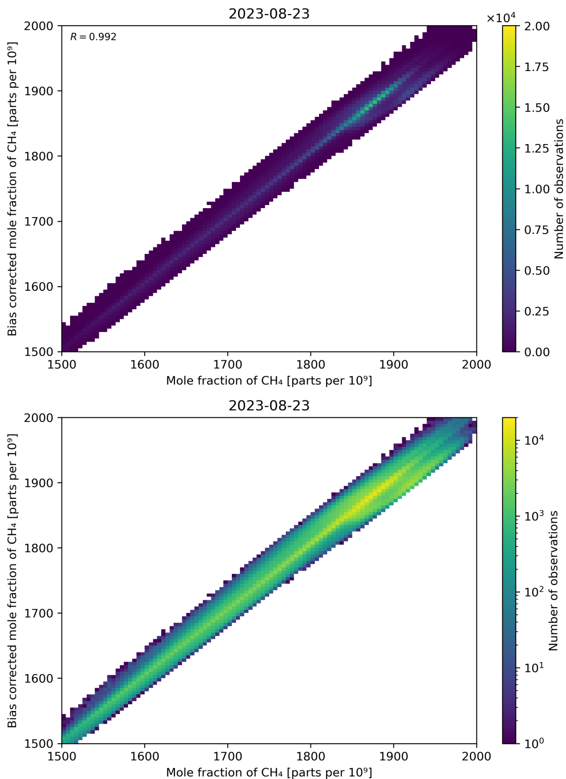
Figure 74: Scatter density plot of “Mole fraction of CH 4 ” against “Bias corrected mole fraction of CH 4 ” for 2023-08-22 to 2023-08-24.
