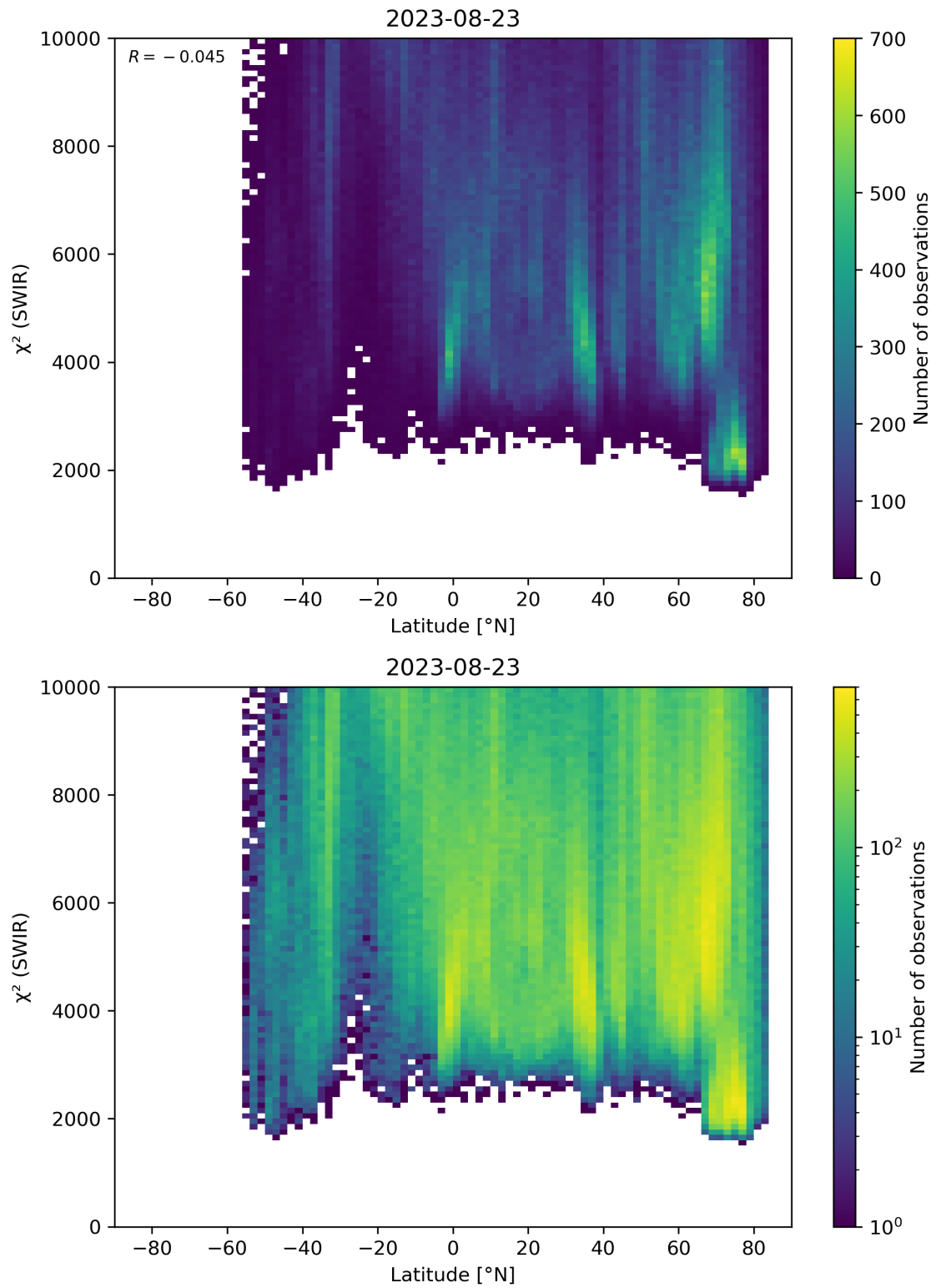
Figure 54: Scatter density plot of “Latitude” against “ \chi^2 (SWIR)” for 2023-08-22 to 2023-08-24.
