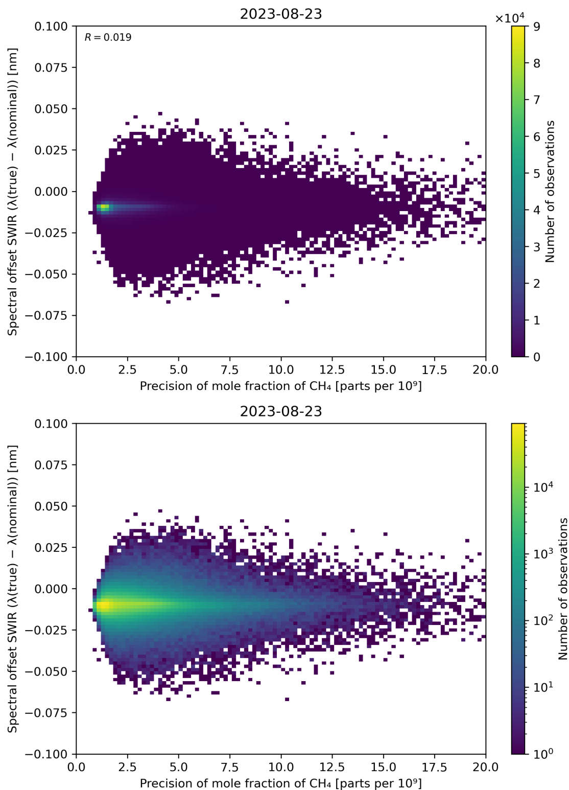
Figure 85: Scatter density plot of “Precision of mole fraction of CH 4 ” against “Spectral offset SWIR ( \lambda(\text{true}) - \lambda(\text{nominal}) )” for 2023-08-22 to 2023-08-24.
