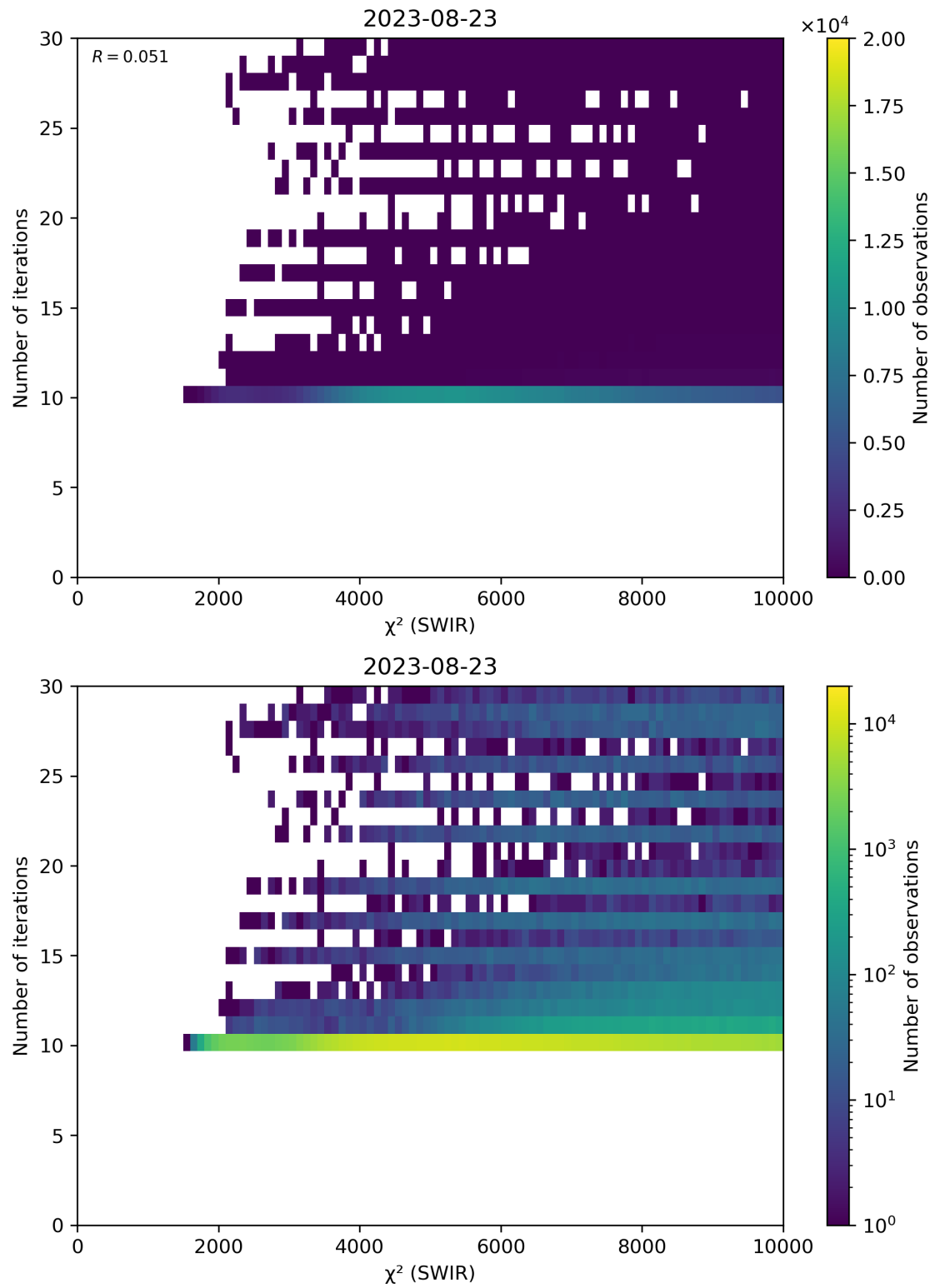
Figure 50: Scatter density plot of “ \chi^2 (SWIR)” against “Number of iterations” for 2023-08-22 to 2023-08-24.
