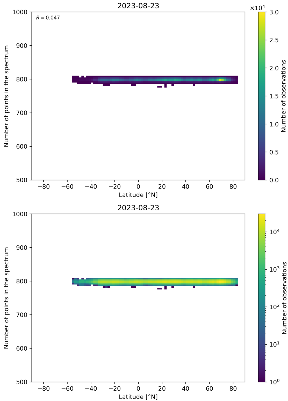
Figure 61: Scatter density plot of “Latitude” against “Number of points in the spectrum” for 2023-08-22 to 2023-08-24.
