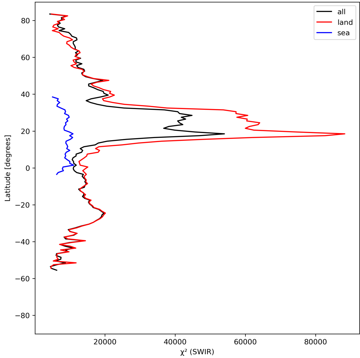
Figure 17: Zonal average of “ \chi^2 (SWIR)” for 2023-08-22 to 2023-08-24.
