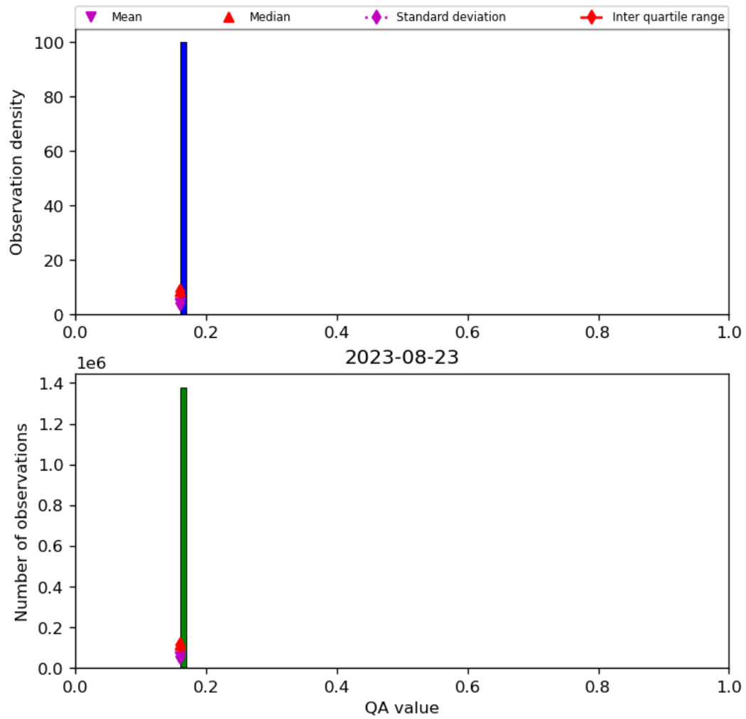
Figure 22: Histogram of “QA value” for 2023-08-22 to 2023-08-24
