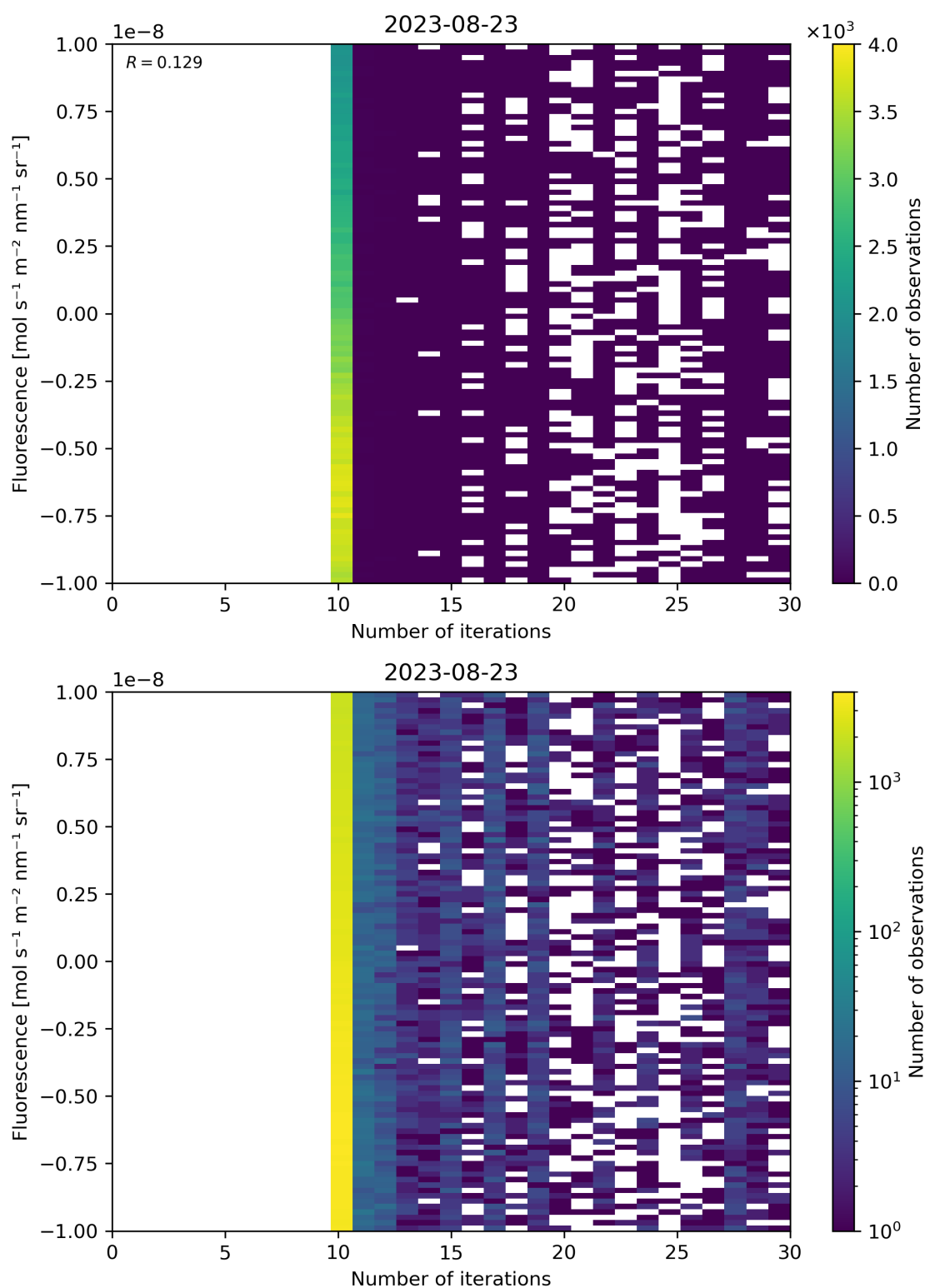
Figure 87: Scatter density plot of “Number of iterations” against “Fluorescence” for 2023-08-22 to 2023-08-24.
