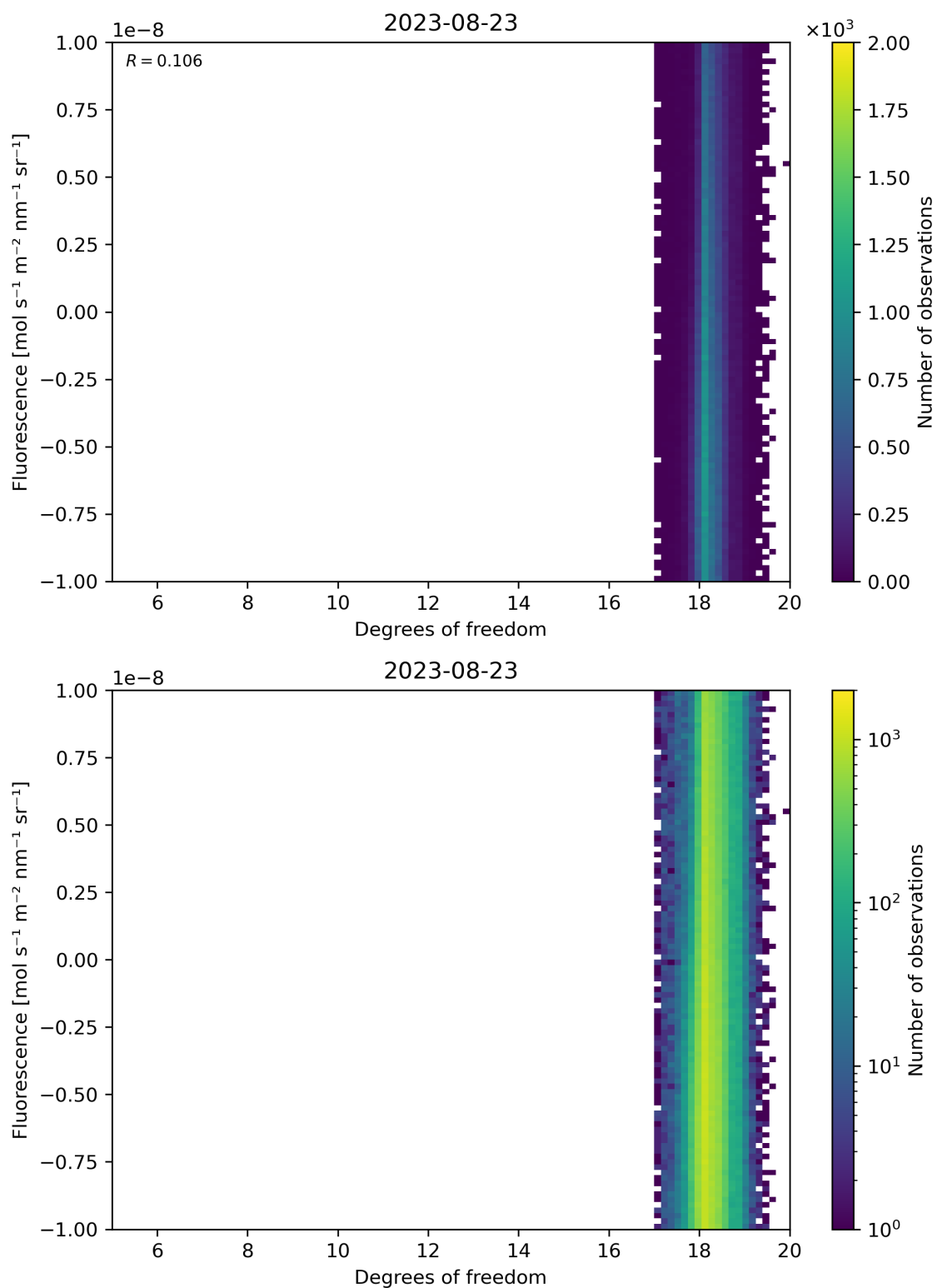
Figure 51: Scatter density plot of “Degrees of freedom” against “Fluorescence” for 2023-08-22 to 2023-08-24.
