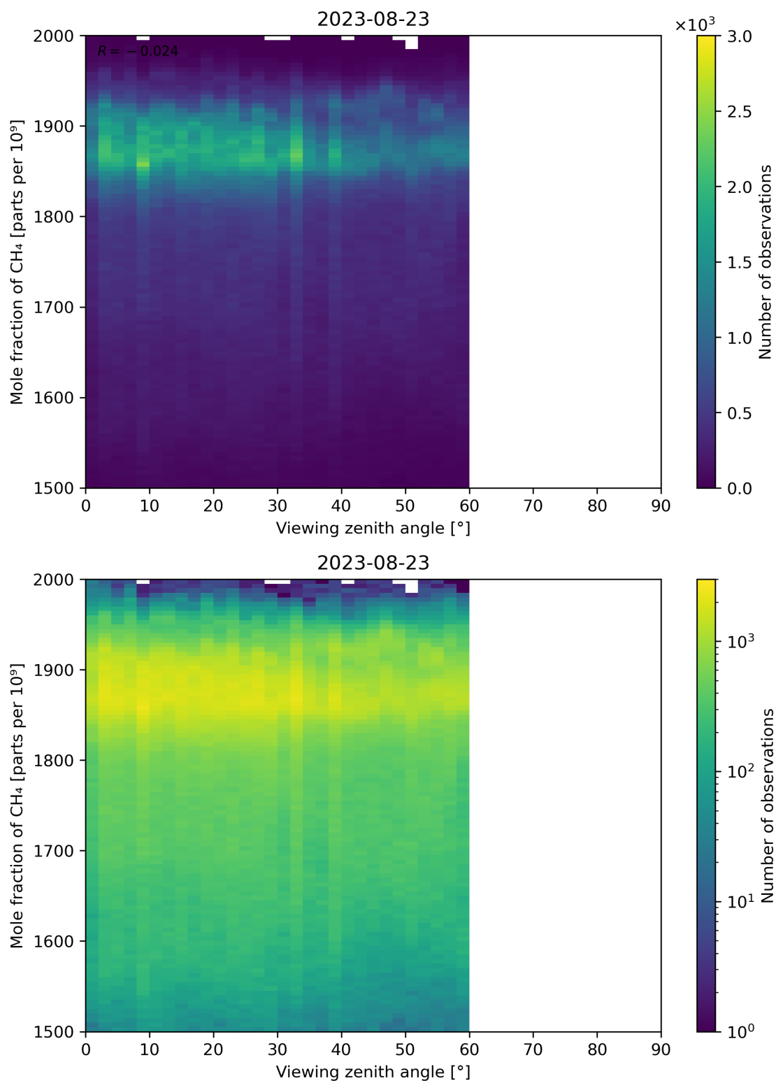
Figure 110: Scatter density plot of “Viewing zenith angle” against “Mole fraction of CH 4 ” for 2023-08-22 to 2023-08-24.
