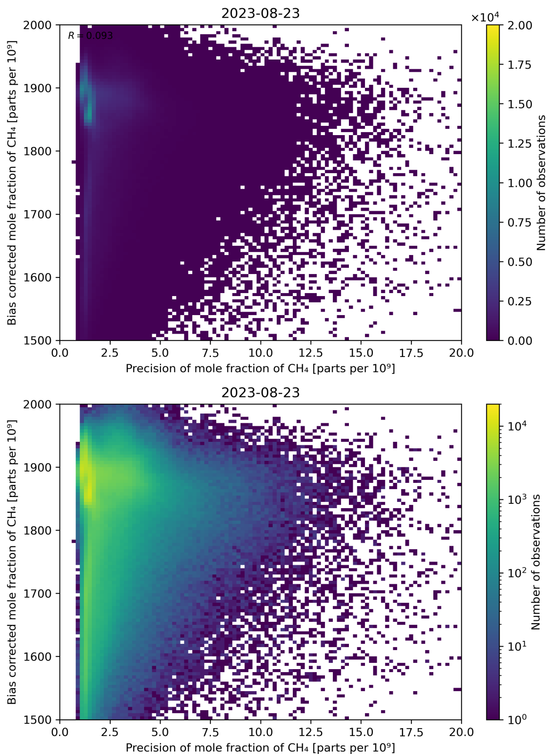
Figure 82: Scatter density plot of “Precision of mole fraction of \text{CH}_4 ” against “Bias corrected mole fraction of \text{CH}_4 ” for 2023-08-22 to 2023-08-24.
