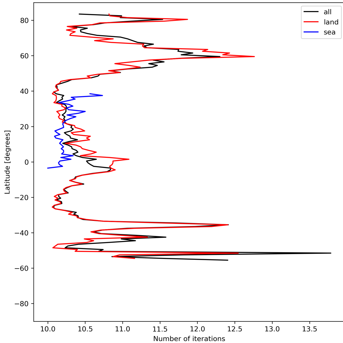
Figure 20: Zonal average of “Number of iterations” for 2023-08-22 to 2023-08-24.
