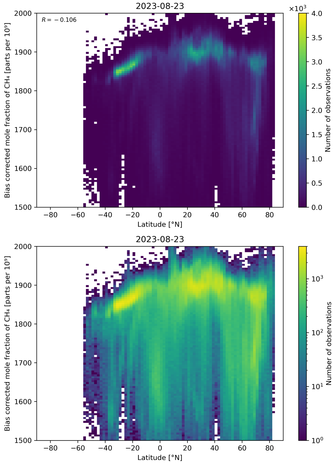
Figure 58: Scatter density plot of “Latitude” against “Bias corrected mole fraction of \text{CH}_4 ” for 2023-08-22 to 2023-08-24.
