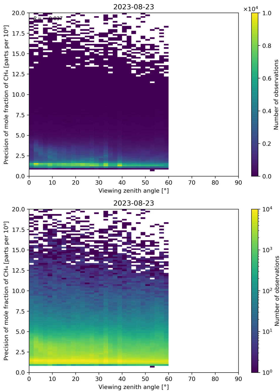
Figure 112: Scatter density plot of “Viewing zenith angle” against “Precision of mole fraction of CH 4 ” for 2023-08-22 to 2023-08-24.
