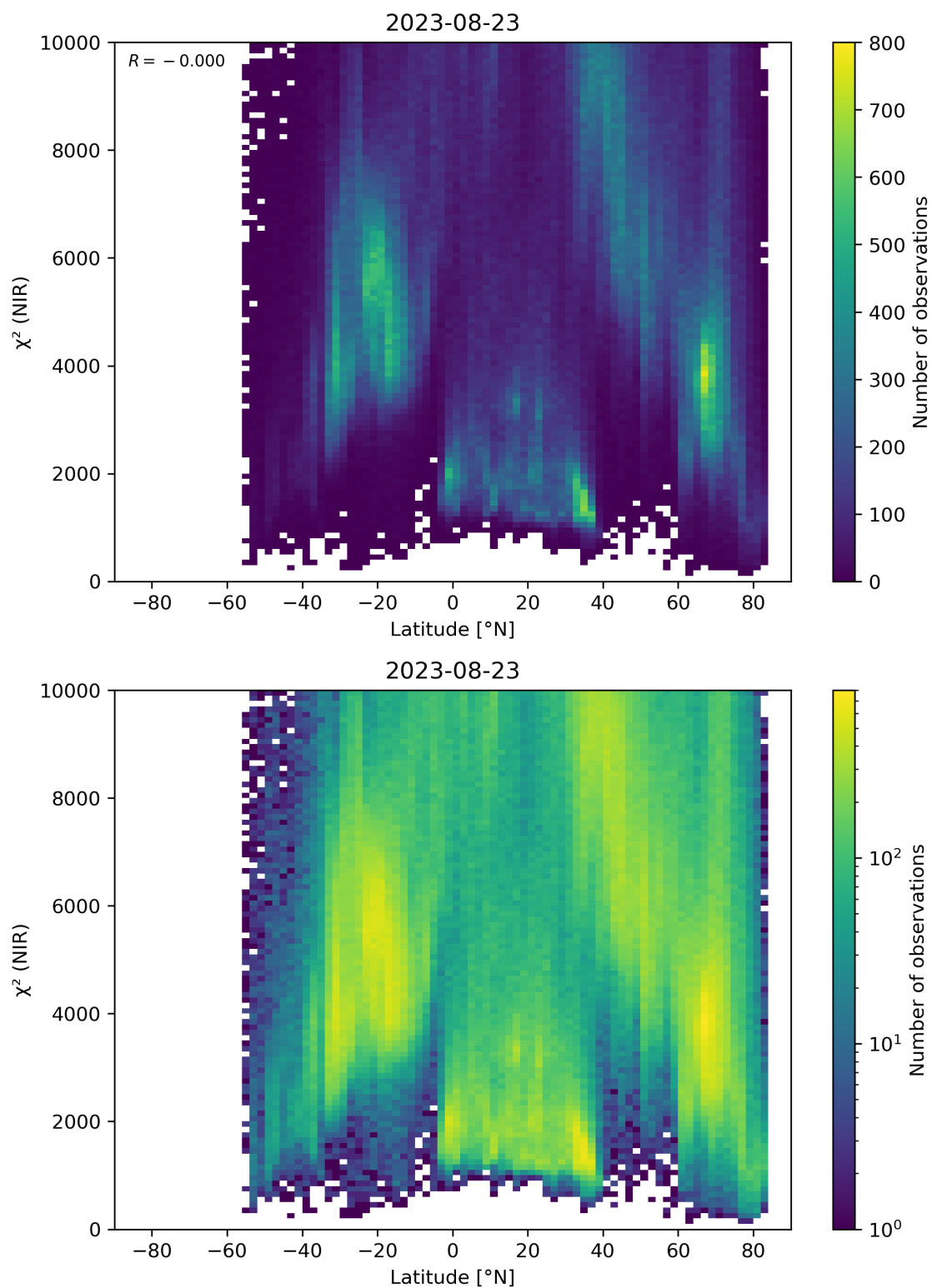
Figure 53: Scatter density plot of “Latitude” against “ \chi^2 (NIR)” for 2023-08-22 to 2023-08-24.
