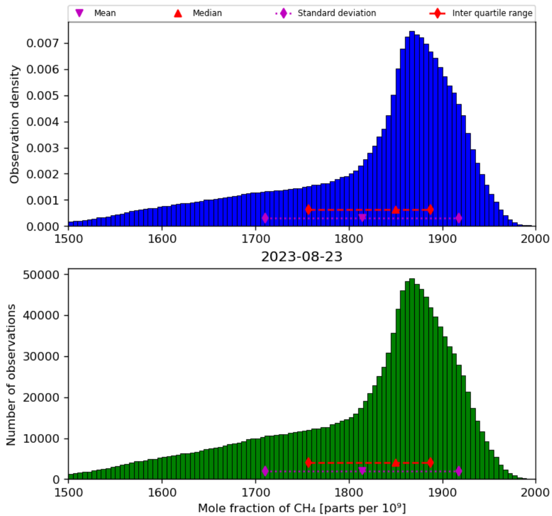
Figure 23: Histogram of “Mole fraction of CH 4 ” for 2023-08-22 to 2023-08-24
