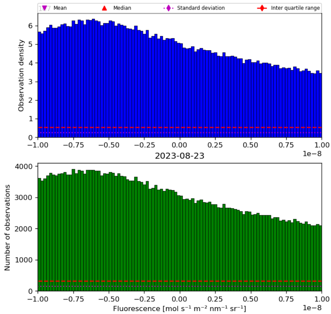
Figure 32: Histogram of “Fluorescence” for 2023-08-22 to 2023-08-24
