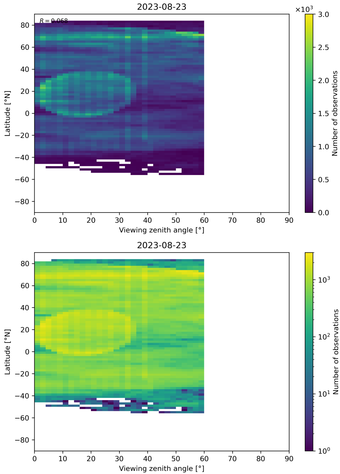
Figure 109: Scatter density plot of “Viewing zenith angle” against “Latitude” for 2023-08-22 to 2023-08-24.
