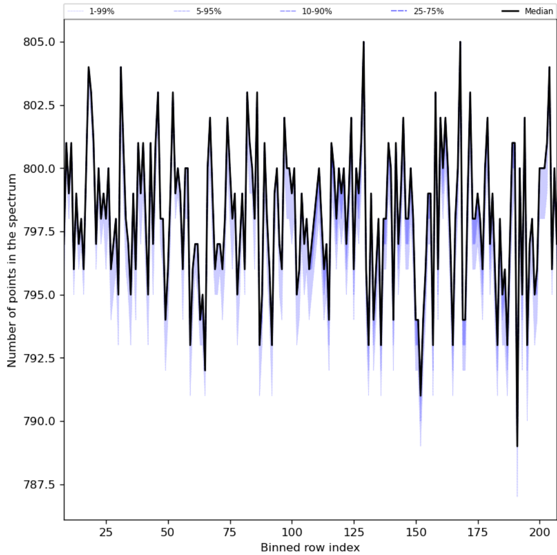
Figure 37: Along track statistics of “Number of points in the spectrum” for 2023-08-22 to 2023-08-24
