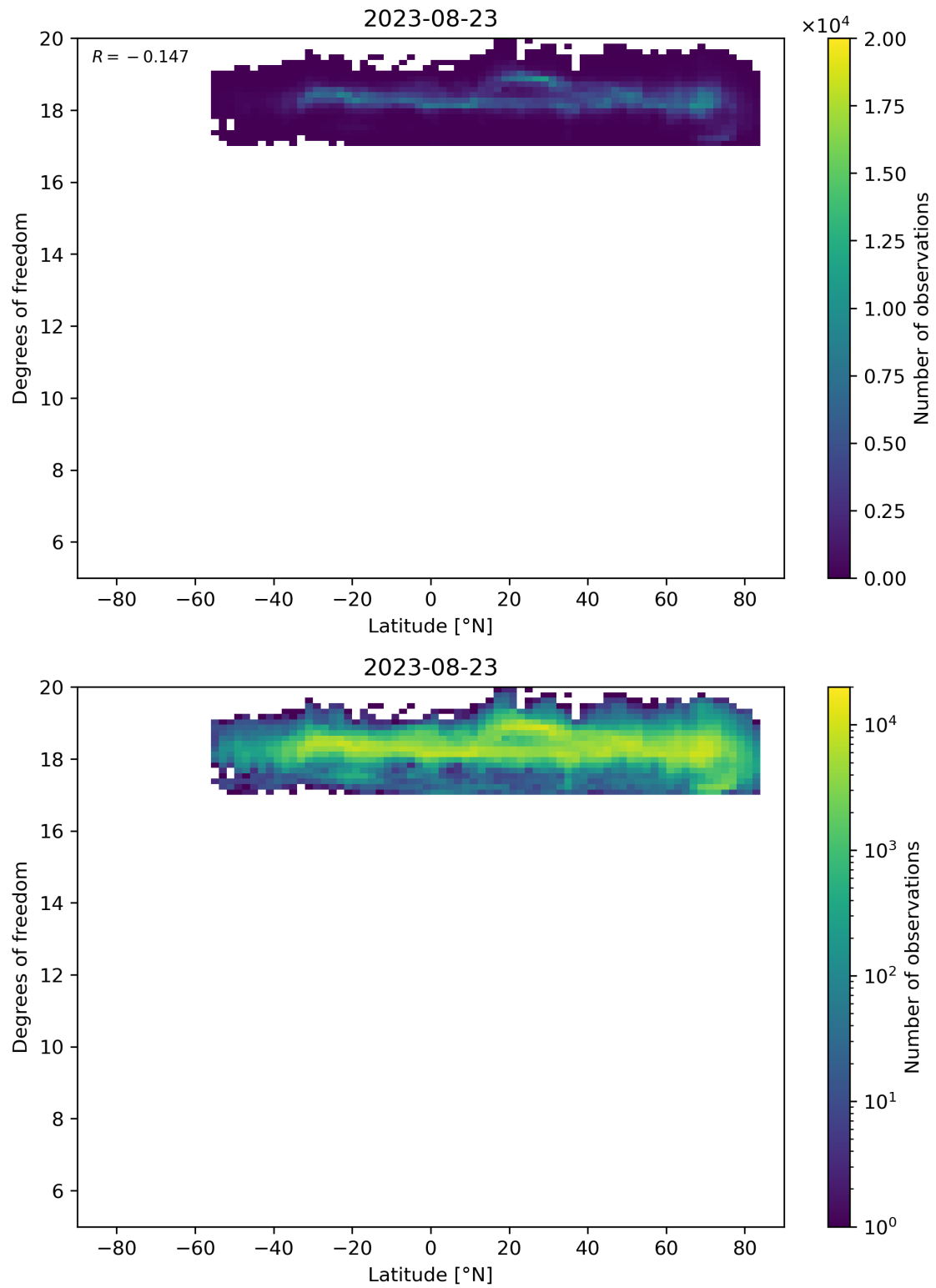
Figure 55: Scatter density plot of “Latitude” against “Degrees of freedom” for 2023-08-22 to 2023-08-24.
