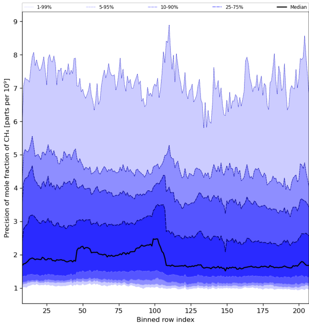
Figure 35: Along track statistics of “Precision of mole fraction of CH 4 ” for 2023-08-22 to 2023-08-24
