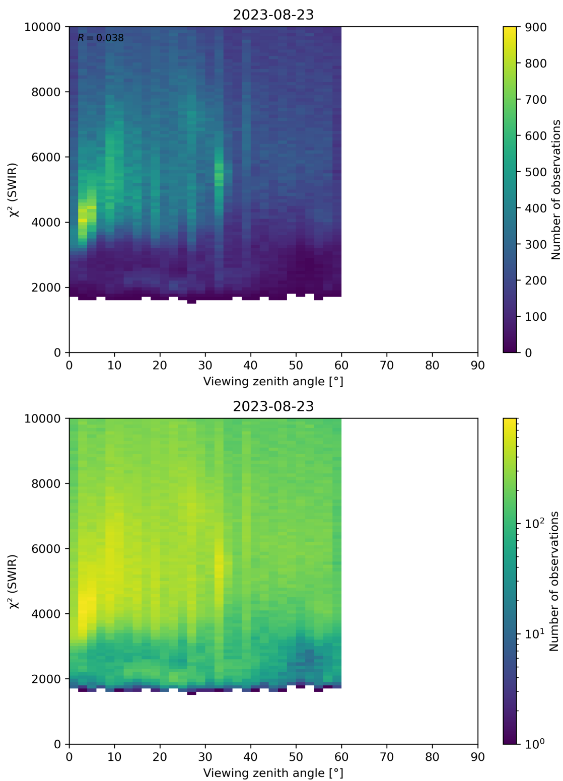
Figure 106: Scatter density plot of “Viewing zenith angle” against “ \chi^2 (SWIR)” for 2023-08-22 to 2023-08-24.
