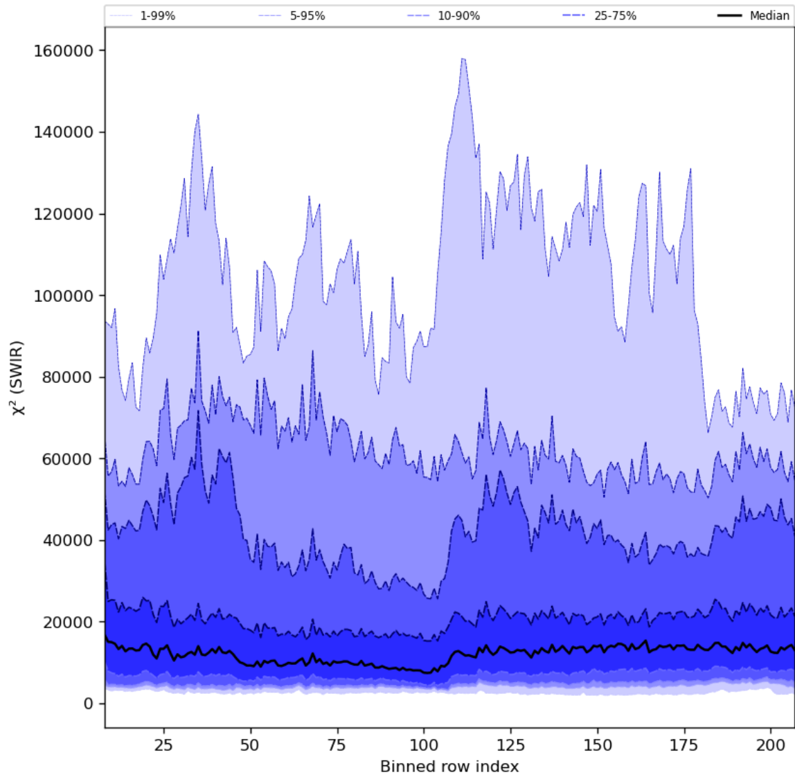
Figure 39: Along track statistics of “ \chi^2 (SWIR)” for 2023-08-22 to 2023-08-24
