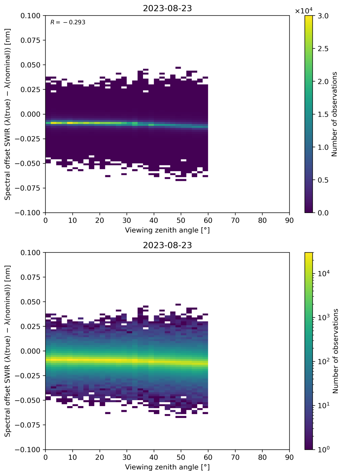
Figure 116: Scatter density plot of “Viewing zenith angle” against “Spectral offset SWIR ( \lambda(\text{true}) - \lambda(\text{nominal}) )” for 2023-08-22 to 2023-08-24.
