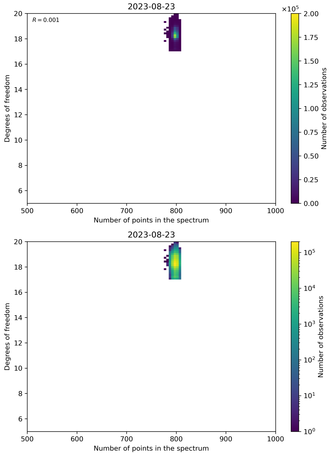
Figure 90: Scatter density plot of “Number of points in the spectrum” against “Degrees of freedom” for 2023-08-22 to 2023-08-24.
