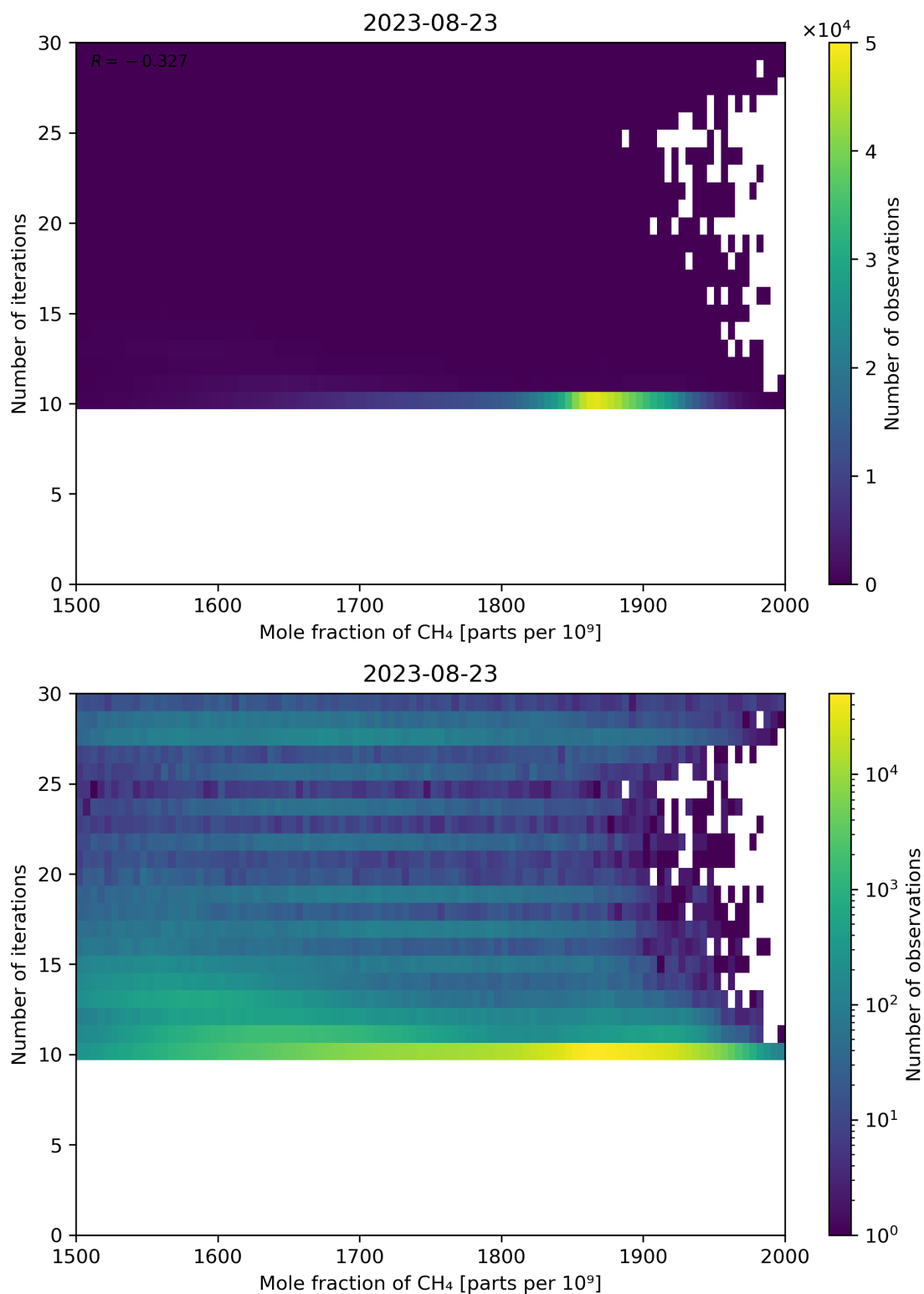
Figure 76: Scatter density plot of “Mole fraction of CH 4 ” against “Number of iterations” for 2023-08-22 to 2023-08-24.
