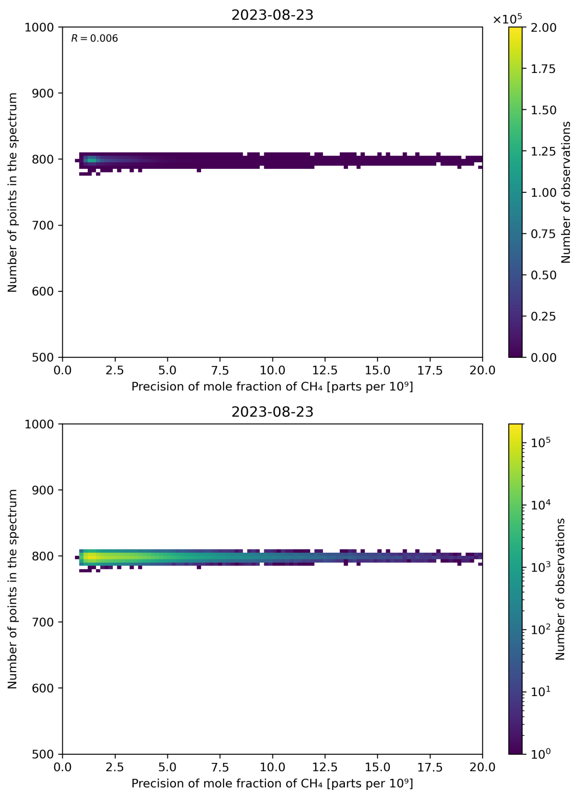
Figure 84: Scatter density plot of “Precision of mole fraction of CH 4 ” against “Number of points in the spectrum” for 2023-08-22 to 2023-08-24.
