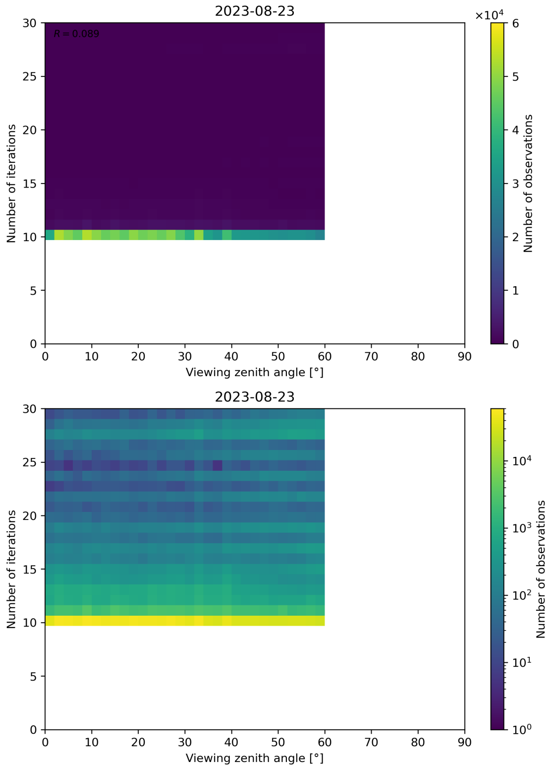
Figure 113: Scatter density plot of “Viewing zenith angle” against “Number of iterations” for 2023-08-22 to 2023-08-24.
