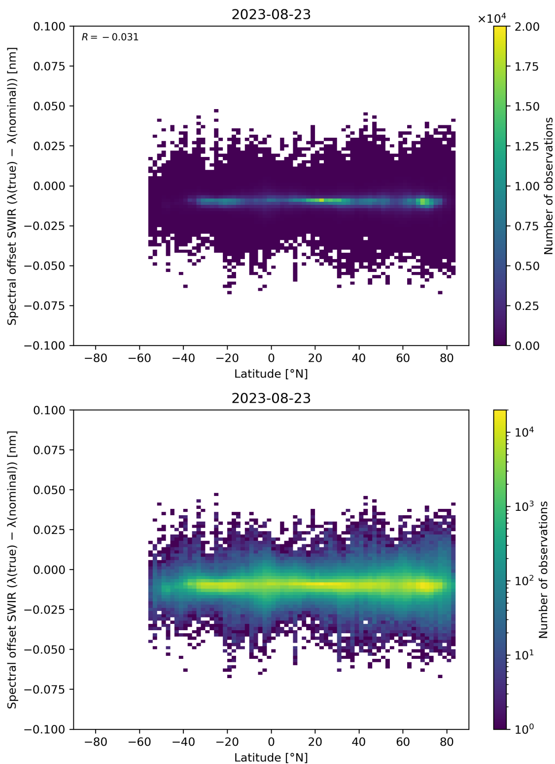
Figure 62: Scatter density plot of “Latitude” against “Spectral offset SWIR ( \lambda(\text{true}) - \lambda(\text{nominal}) )” for 2023-08-22 to 2023-08-24.
