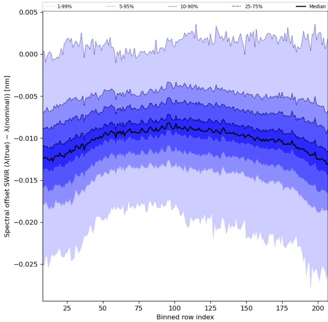
Figure 38: Along track statistics of “Spectral offset SWIR ( \lambda(\text{true}) - \lambda(\text{nominal}) )” for 2023-08-22 to 2023-08-24
