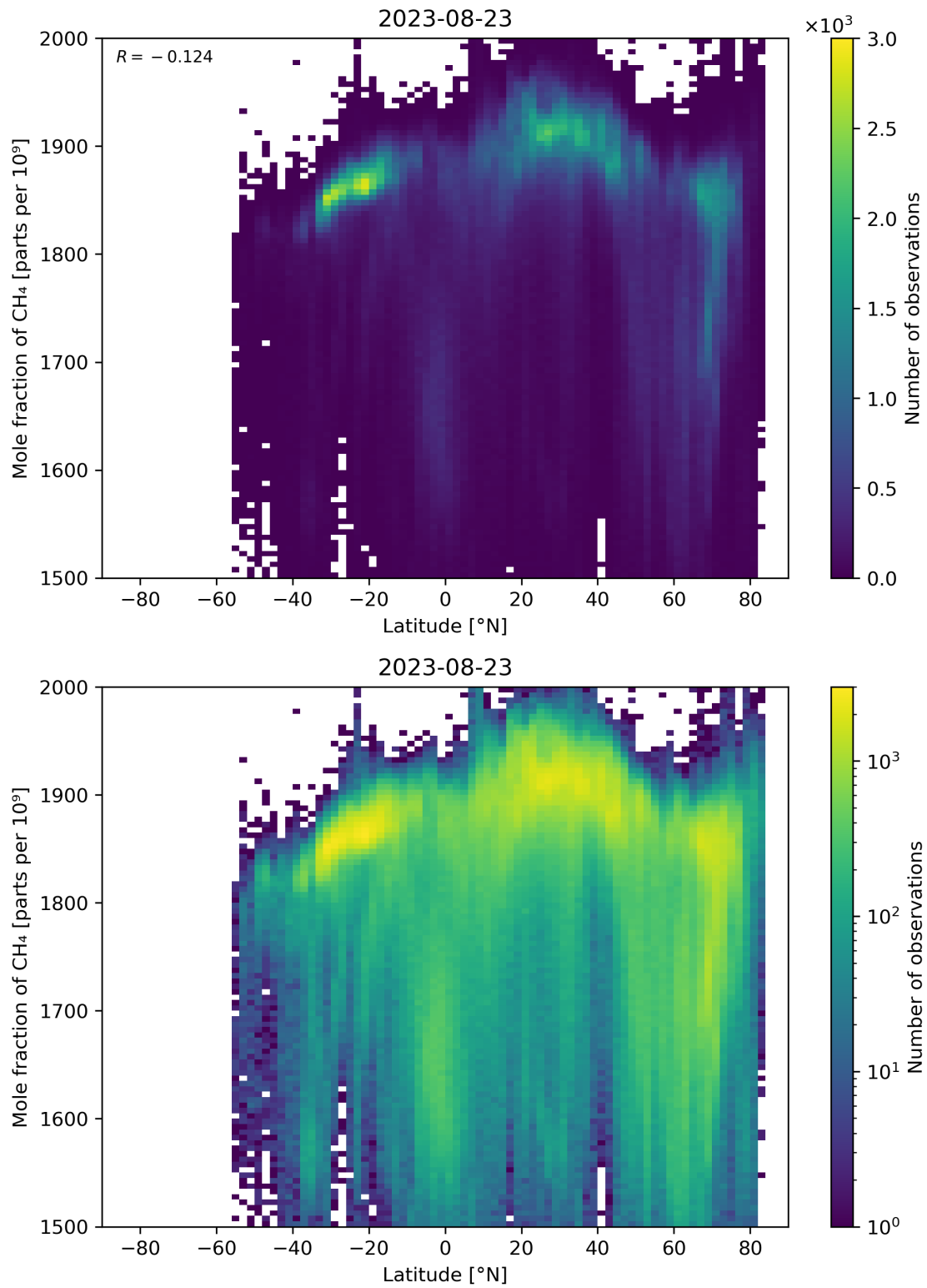
Figure 57: Scatter density plot of “Latitude” against “Mole fraction of CH 4 ” for 2023-08-22 to 2023-08-24.
