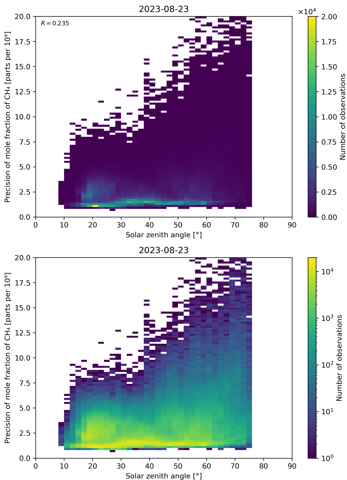
Figure 101: Scatter density plot of “Solar zenith angle” against “Precision of mole fraction of \text{CH}_4 ” for 2023-08-22 to 2023-08-24.
