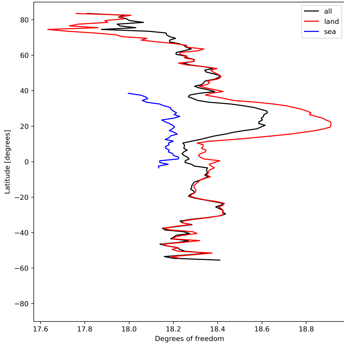
Figure 19: Zonal average of “Degrees of freedom” for 2023-08-22 to 2023-08-24.
