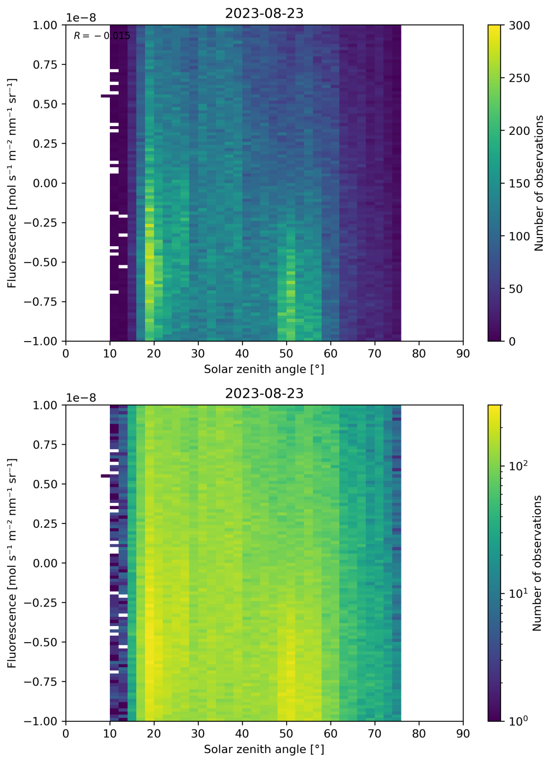
Figure 97: Scatter density plot of “Solar zenith angle” against “Fluorescence” for 2023-08-22 to 2023-08-24.
