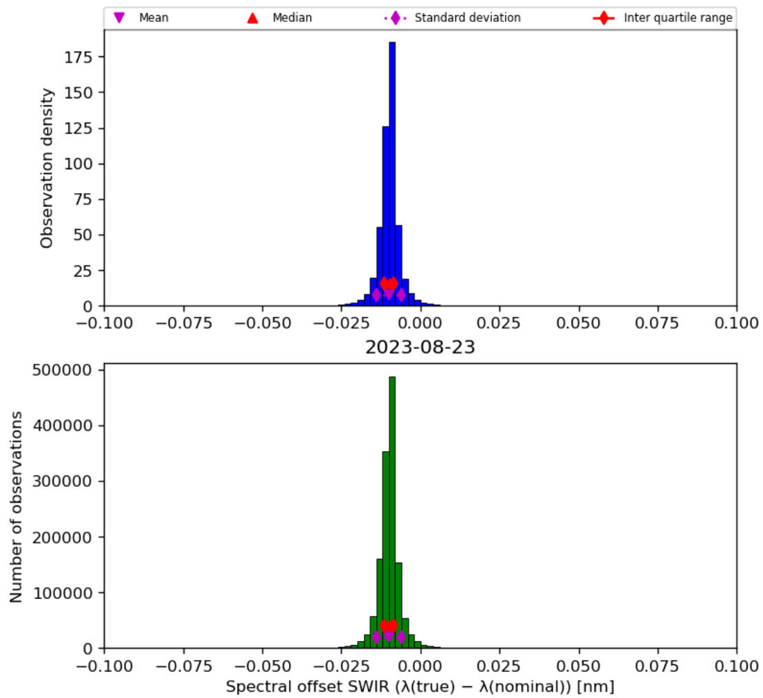
Figure 27: Histogram of “Spectral offset SWIR ( \lambda(\text{true}) - \lambda(\text{nominal}) )” for 2023-08-22 to 2023-08-24
