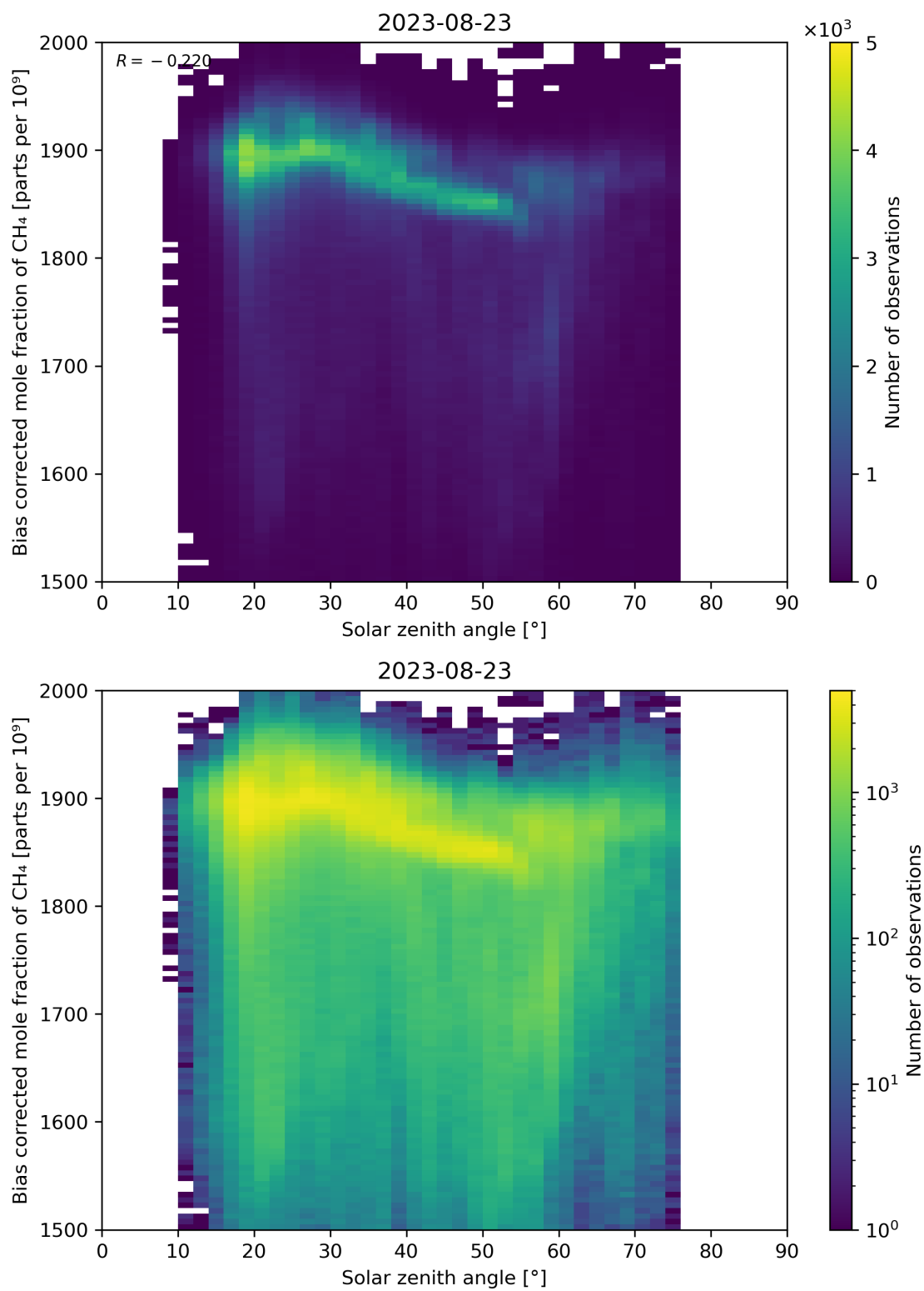
Figure 100: Scatter density plot of “Solar zenith angle” against “Bias corrected mole fraction of \text{CH}_4 ” for 2023-08-22 to 2023-08-24.
