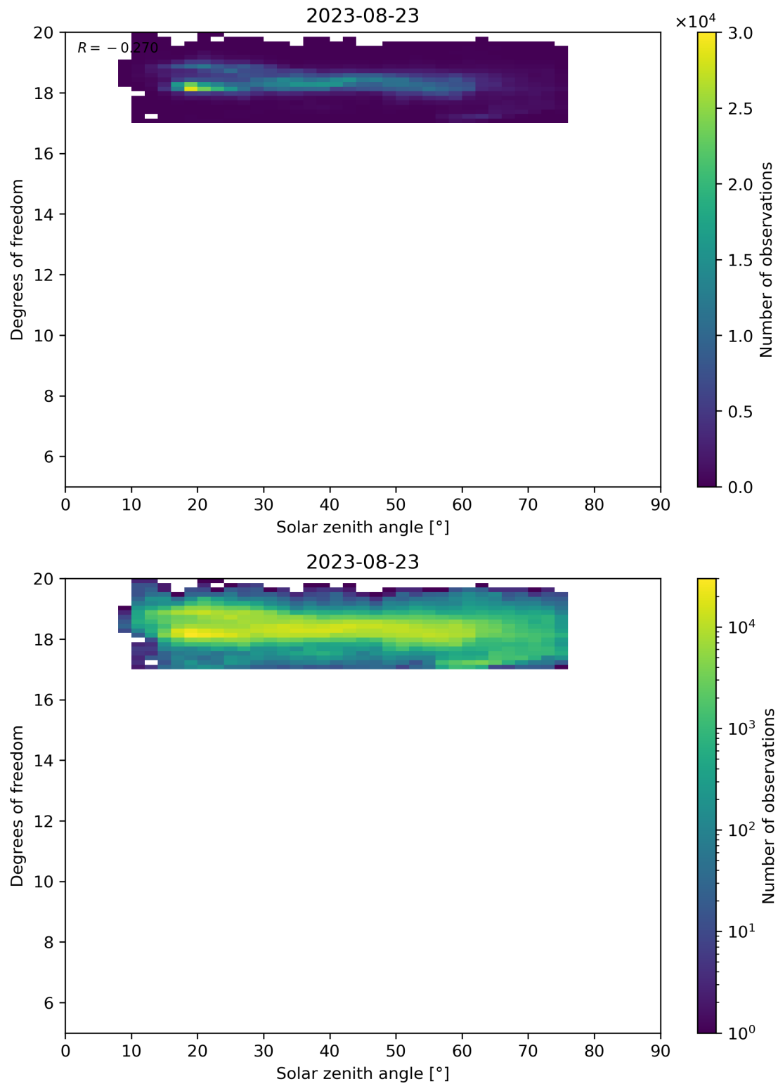
Figure 96: Scatter density plot of “Solar zenith angle” against “Degrees of freedom” for 2023-08-22 to 2023-08-24.
