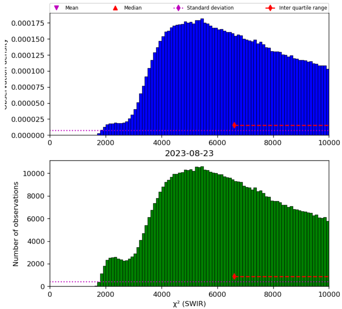
Figure 28: Histogram of “ \chi^2 (SWIR)” for 2023-08-22 to 2023-08-24
