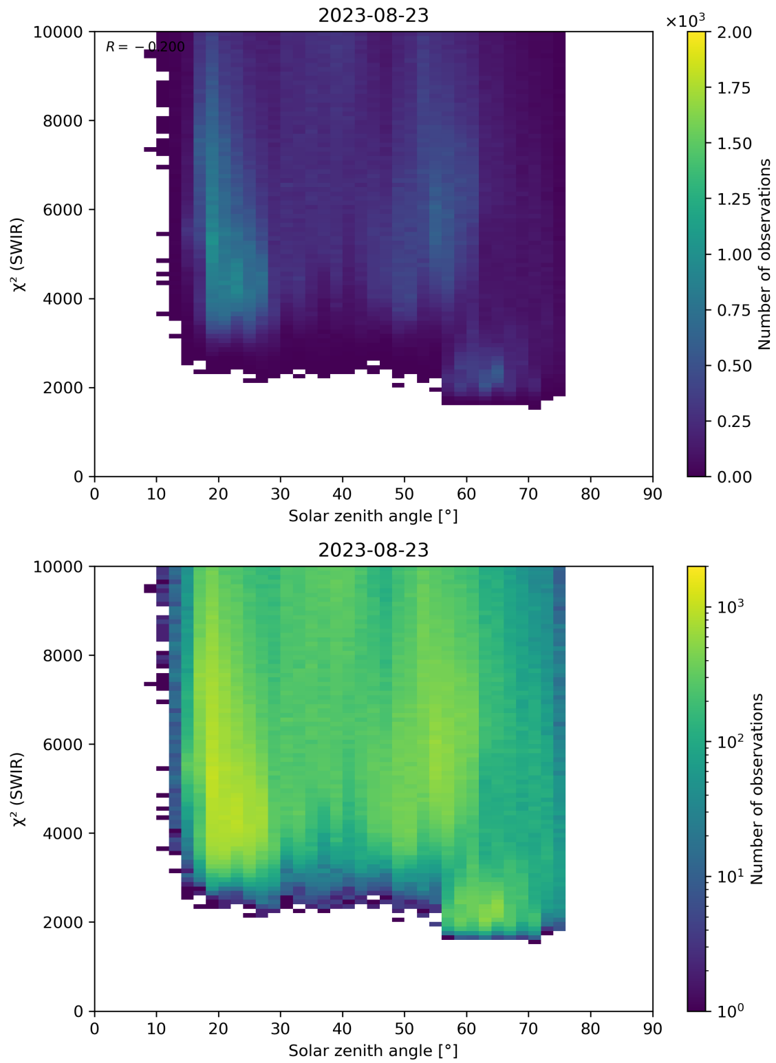
Figure 95: Scatter density plot of “Solar zenith angle” against “ \chi^2 (SWIR)” for 2023-08-22 to 2023-08-24.
