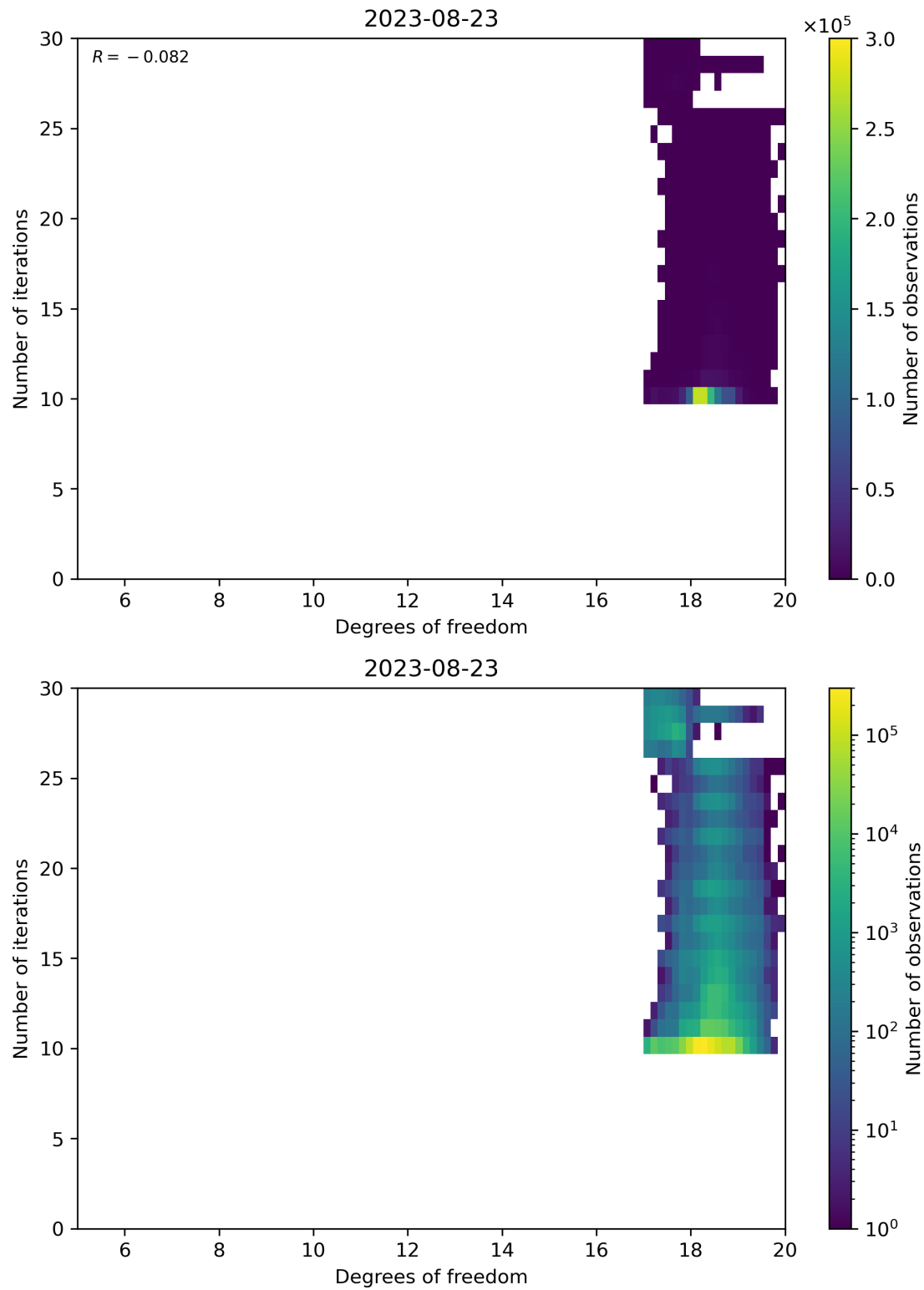
Figure 52: Scatter density plot of “Degrees of freedom” against “Number of iterations” for 2023-08-22 to 2023-08-24.
