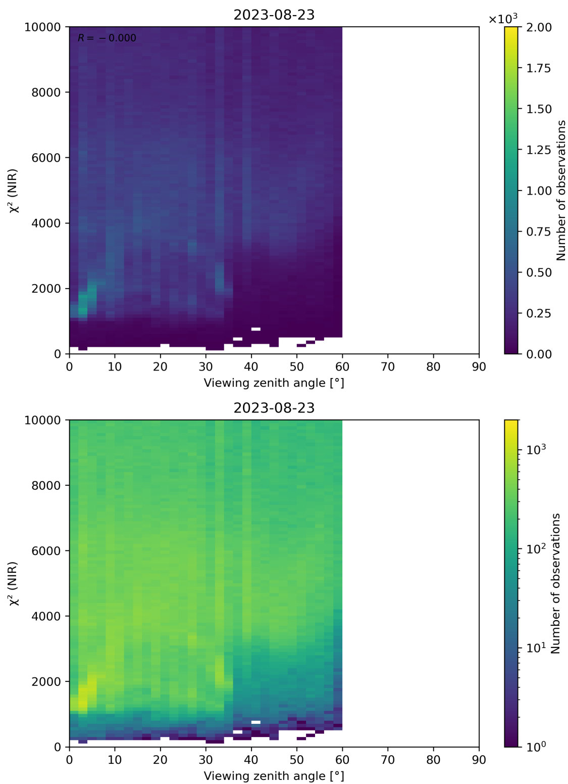
Figure 105: Scatter density plot of “Viewing zenith angle” against “ \chi^2 (NIR)” for 2023-08-22 to 2023-08-24.
