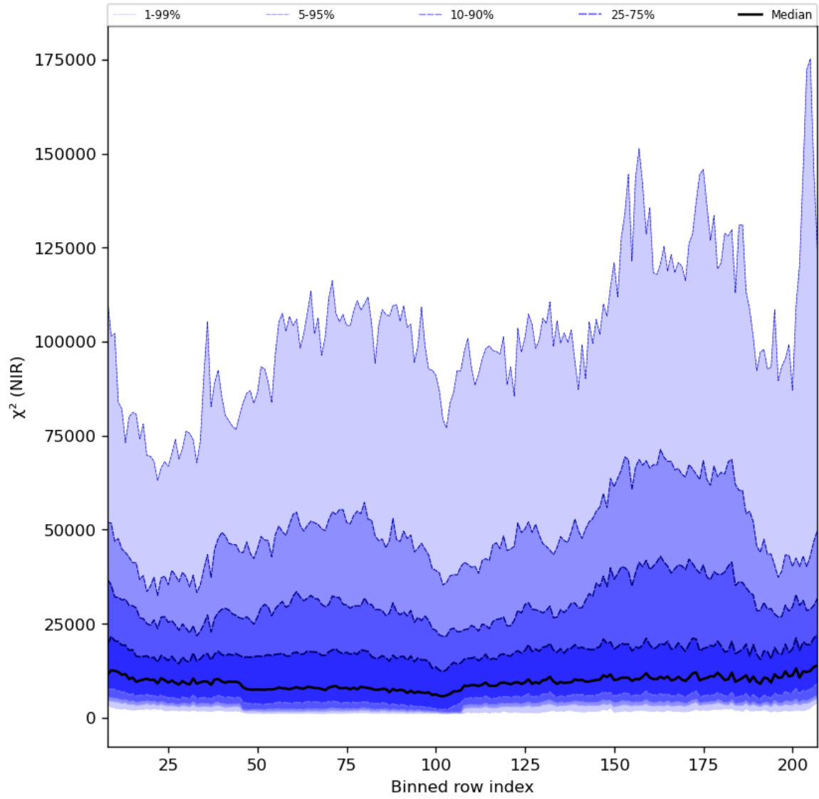
Figure 40: Along track statistics of “ \chi^2 (NIR)” for 2023-08-22 to 2023-08-24
