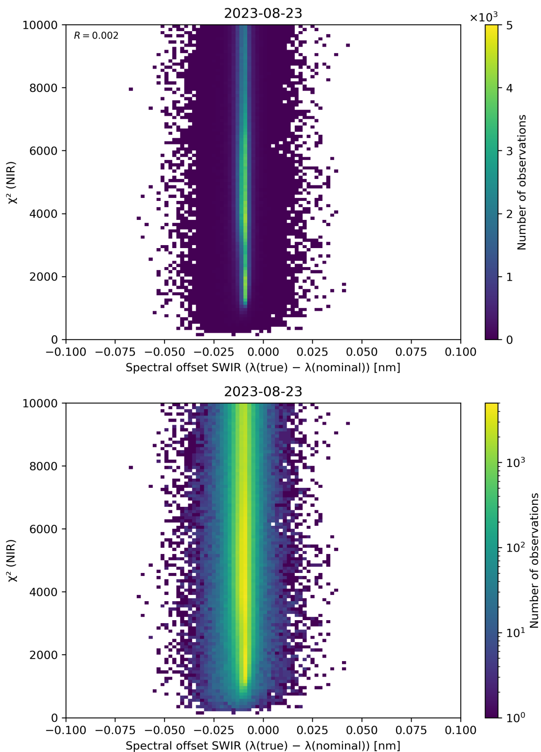
Figure 117: Scatter density plot of “Spectral offset SWIR ( \lambda(\text{true}) - \lambda(\text{nominal}) )” against “ \chi^2 (NIR)” for 2023-08-22 to 2023-08-24.
