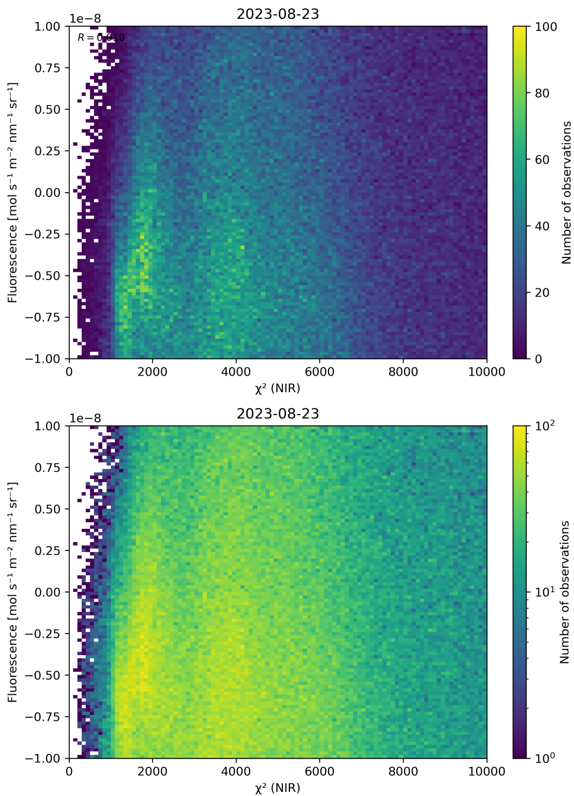
Figure 45: Scatter density plot of “ \chi^2 (NIR)” against “Fluorescence” for 2023-08-22 to 2023-08-24.
