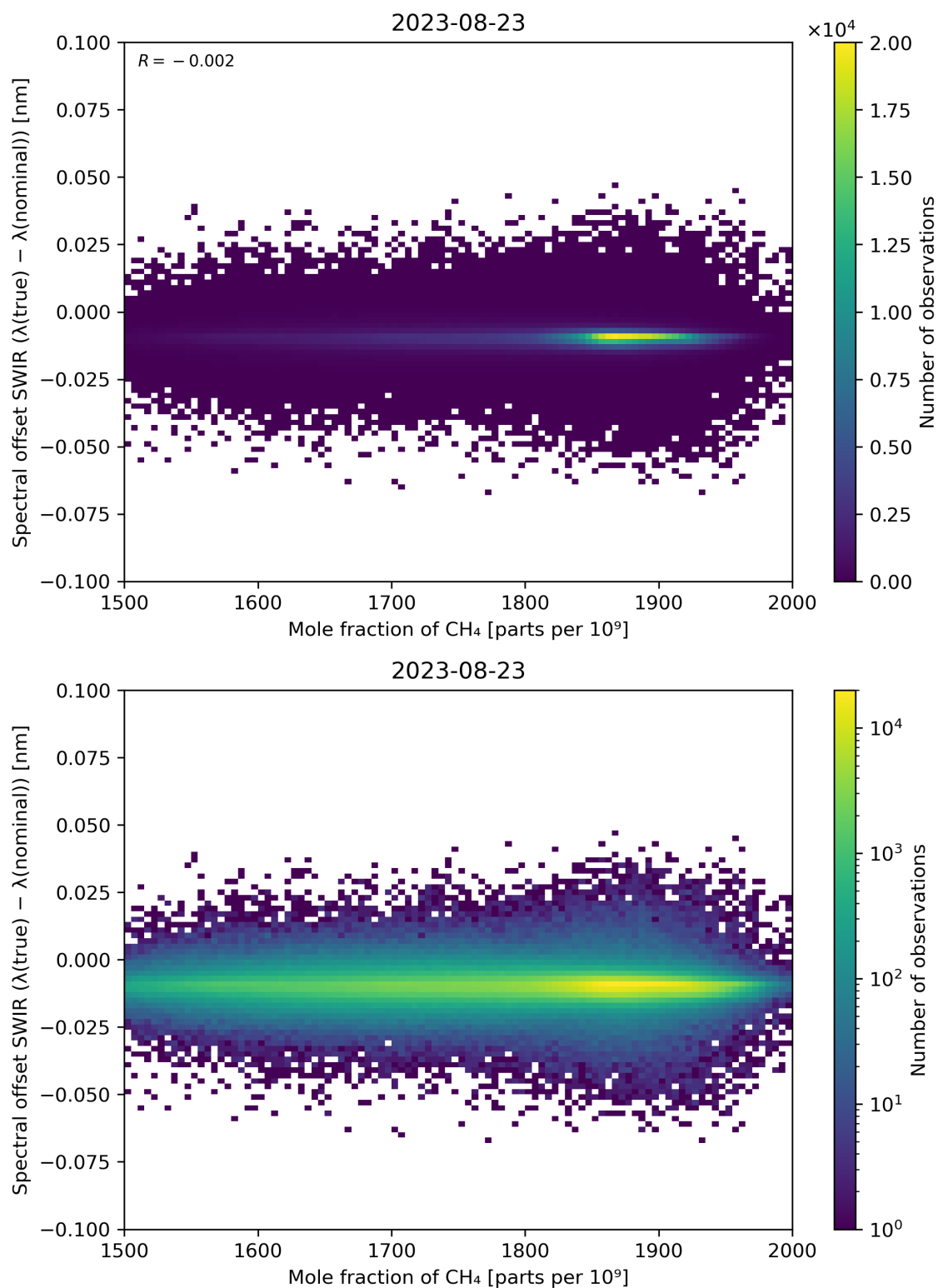
Figure 86: Scatter density plot of “Mole fraction of CH 4 ” against “Spectral offset SWIR ( \lambda(\text{true}) - \lambda(\text{nominal}) )” for 2023-08-22 to 2023-08-24.
