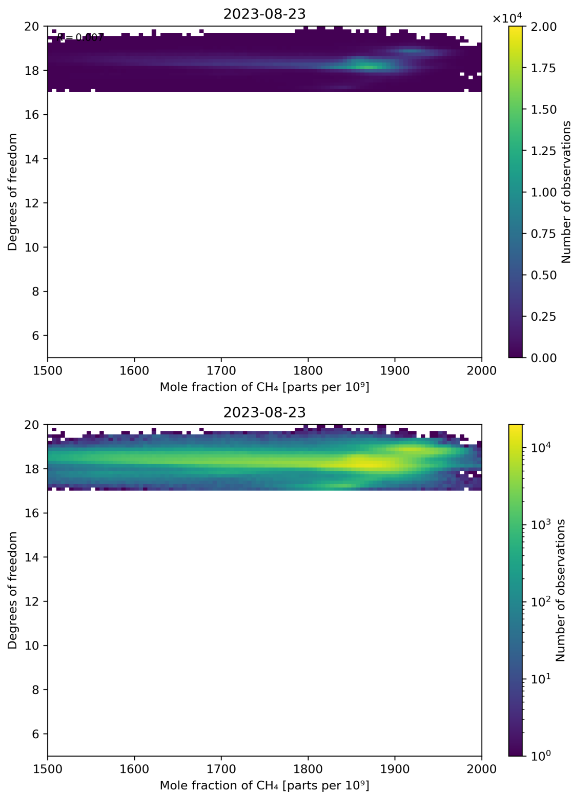
Figure 72: Scatter density plot of “Mole fraction of CH 4 ” against “Degrees of freedom” for 2023-08-22 to 2023-08-24.
