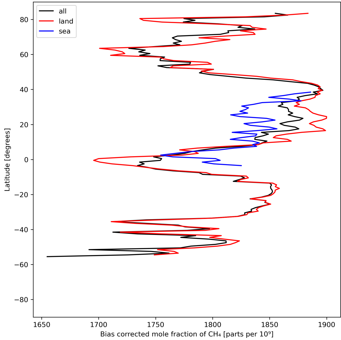
Figure 14: Zonal average of “Bias corrected mole fraction of CH 4 ” for 2023-08-22 to 2023-08-24.
