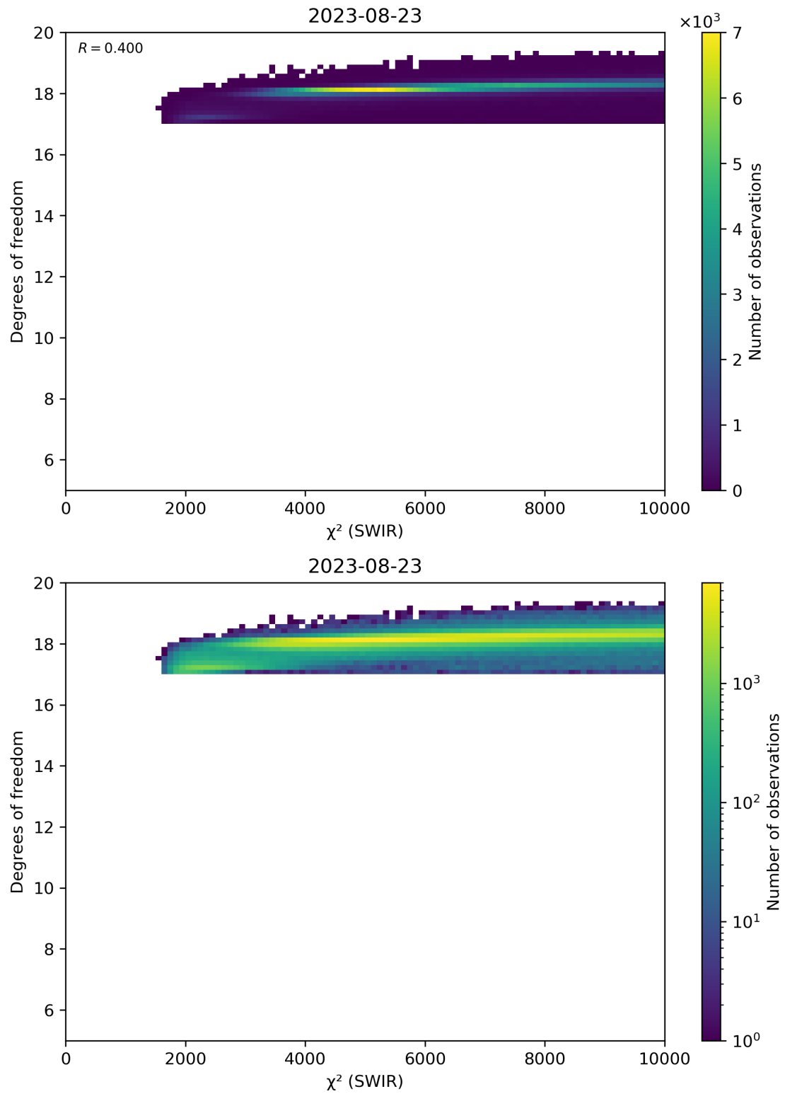
Figure 48: Scatter density plot of “ \chi^2 (SWIR)” against “Degrees of freedom” for 2023-08-22 to 2023-08-24.
