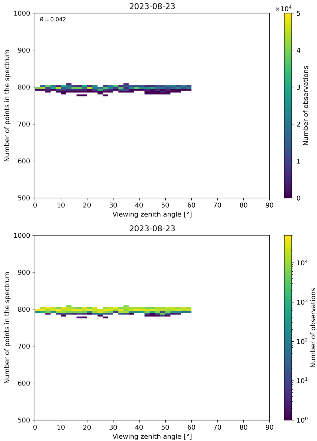
Figure 114: Scatter density plot of “Viewing zenith angle” against “Number of points in the spectrum” for 2023-08-22 to 2023-08-24.
