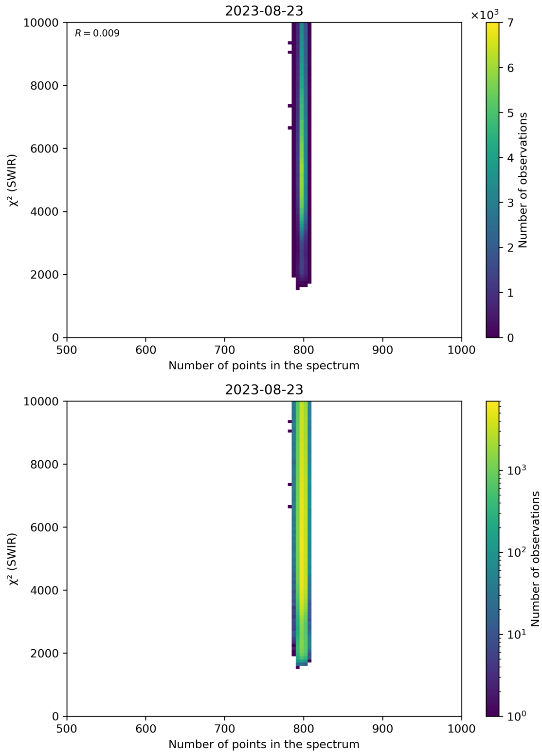
Figure 89: Scatter density plot of “Number of points in the spectrum” against “ \chi^2 (SWIR)” for 2023-08-22 to 2023-08-24.
