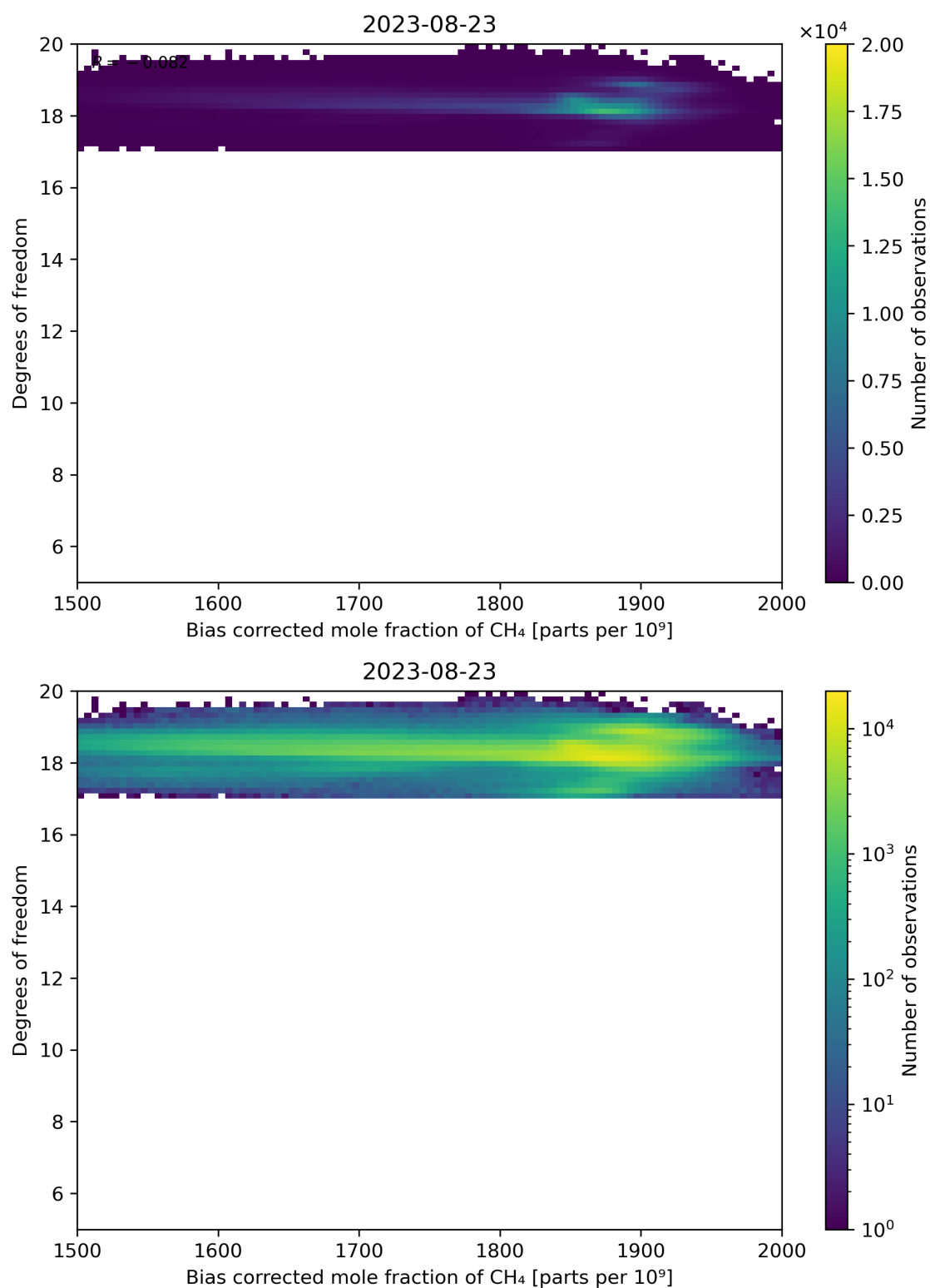
Figure 65: Scatter density plot of “Bias corrected mole fraction of CH 4 ” against “Degrees of freedom” for 2023-08-22 to 2023-08-24.
