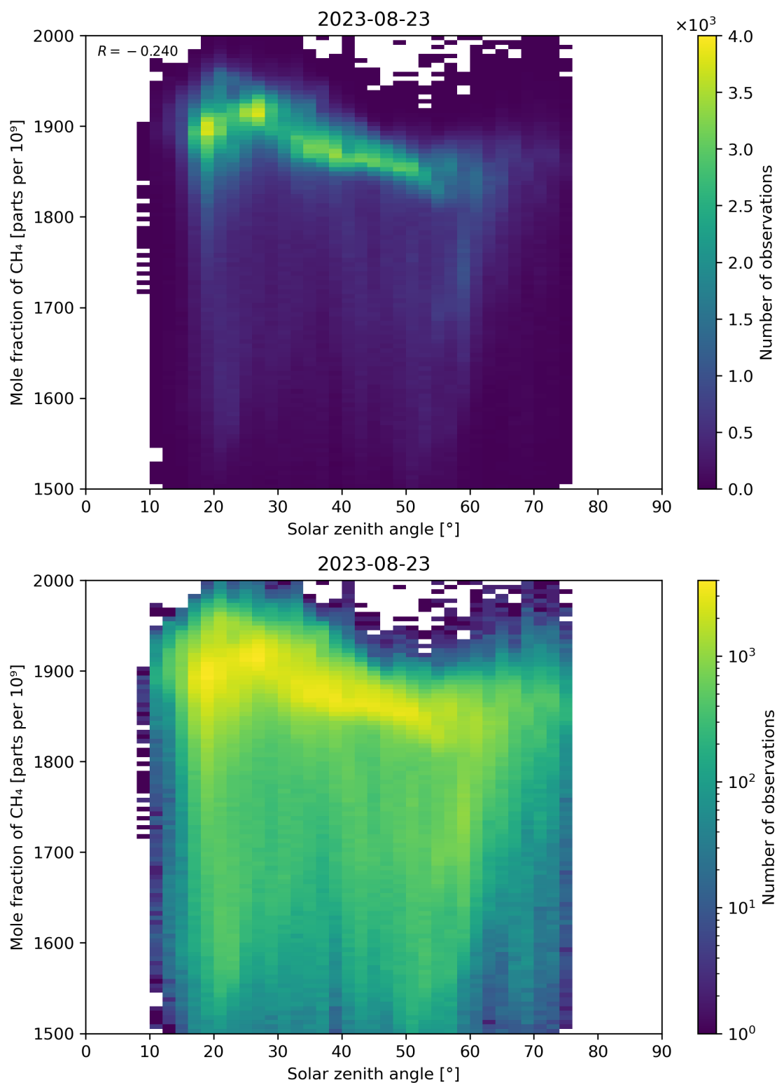
Figure 99: Scatter density plot of “Solar zenith angle” against “Mole fraction of CH 4 ” for 2023-08-22 to 2023-08-24.
