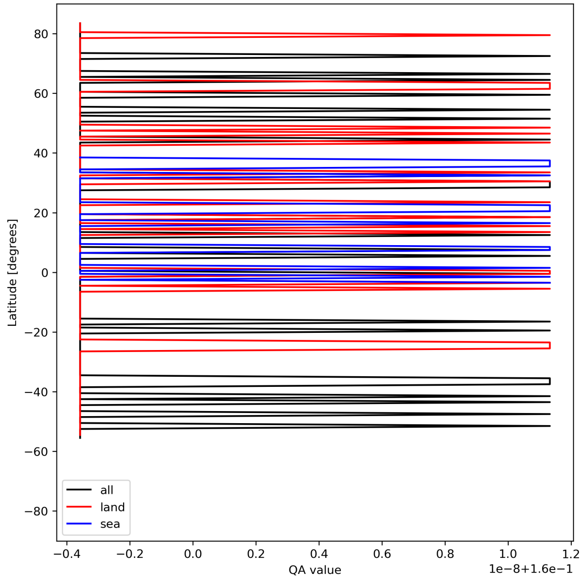
Figure 11: Zonal average of “QA value” for 2023-08-22 to 2023-08-24.
