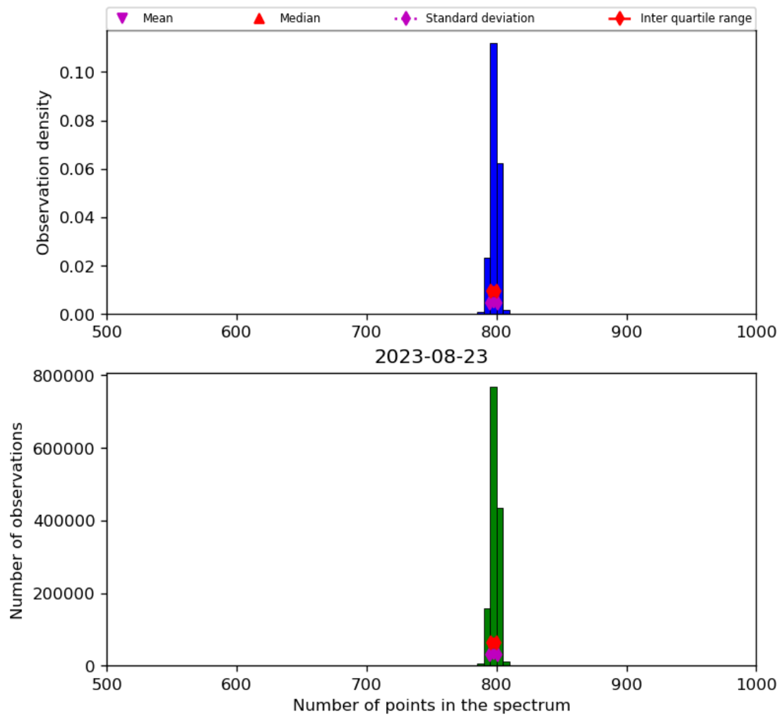
Figure 26: Histogram of “Number of points in the spectrum” for 2023-08-22 to 2023-08-24
