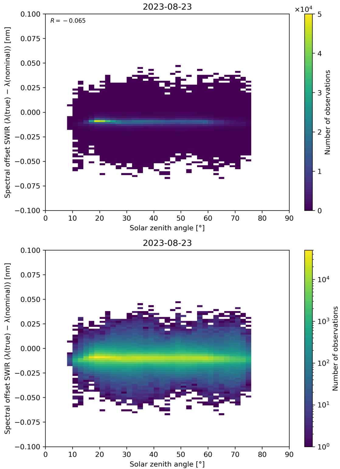
Figure 104: Scatter density plot of “Solar zenith angle” against “Spectral offset SWIR ( \lambda(\text{true}) - \lambda(\text{nominal}) )” for 2023-08-22 to 2023-08-24.
