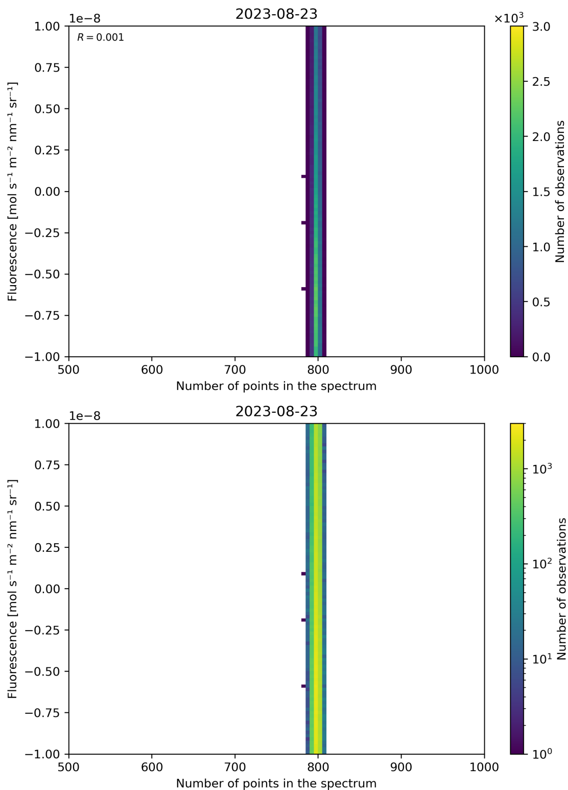
Figure 91: Scatter density plot of “Number of points in the spectrum” against “Fluorescence” for 2023-08-22 to 2023-08-24.
