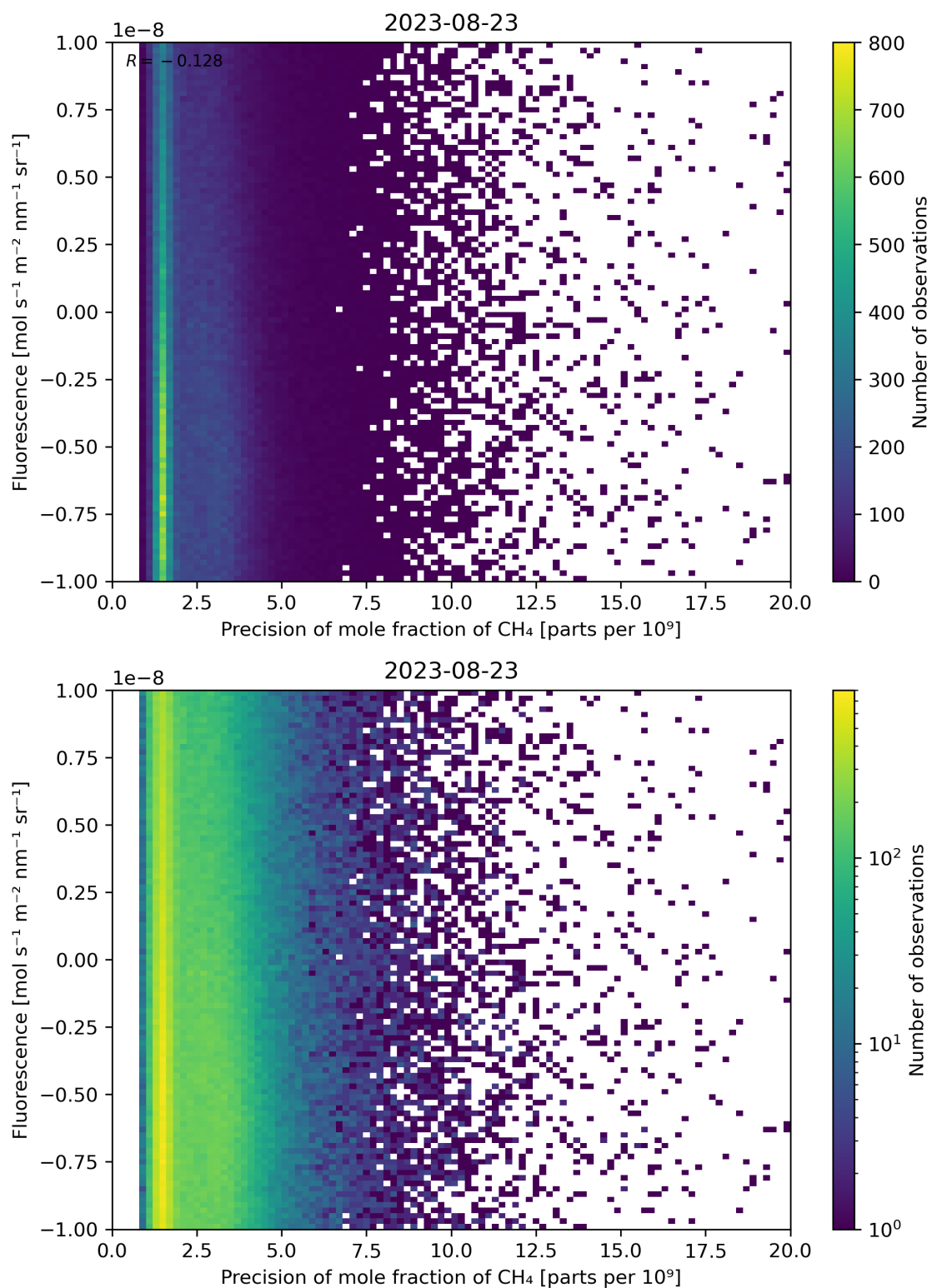
Figure 81: Scatter density plot of “Precision of mole fraction of \text{CH}_4 ” against “Fluorescence” for 2023-08-22 to 2023-08-24.
