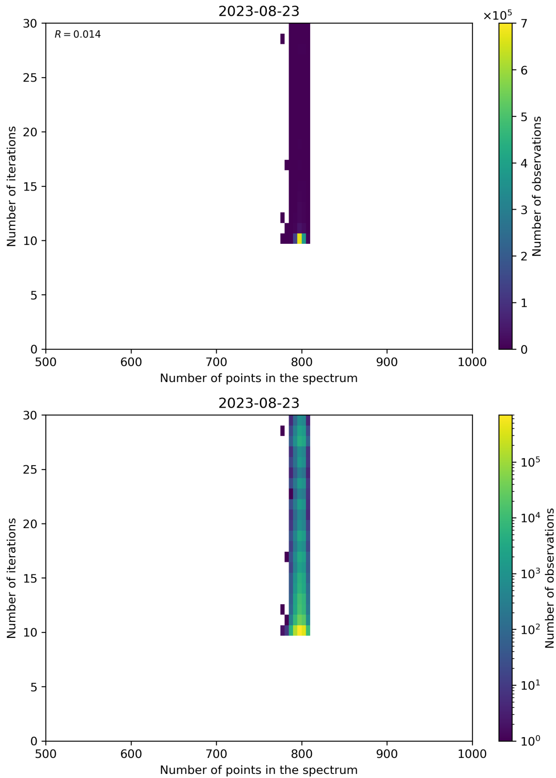
Figure 92: Scatter density plot of “Number of points in the spectrum” against “Number of iterations” for 2023-08-22 to 2023-08-24.
