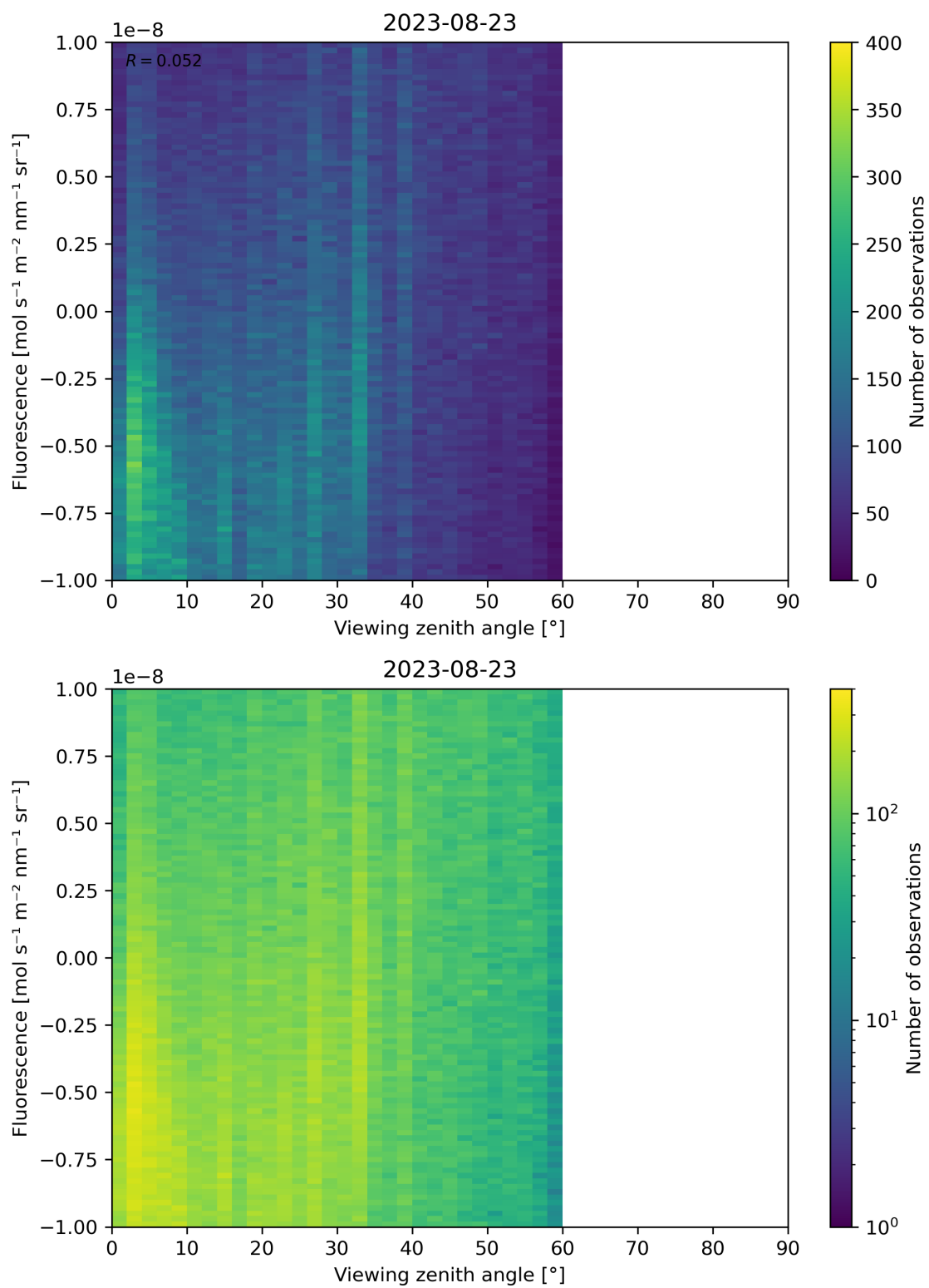
Figure 108: Scatter density plot of “Viewing zenith angle” against “Fluorescence” for 2023-08-22 to 2023-08-24.
