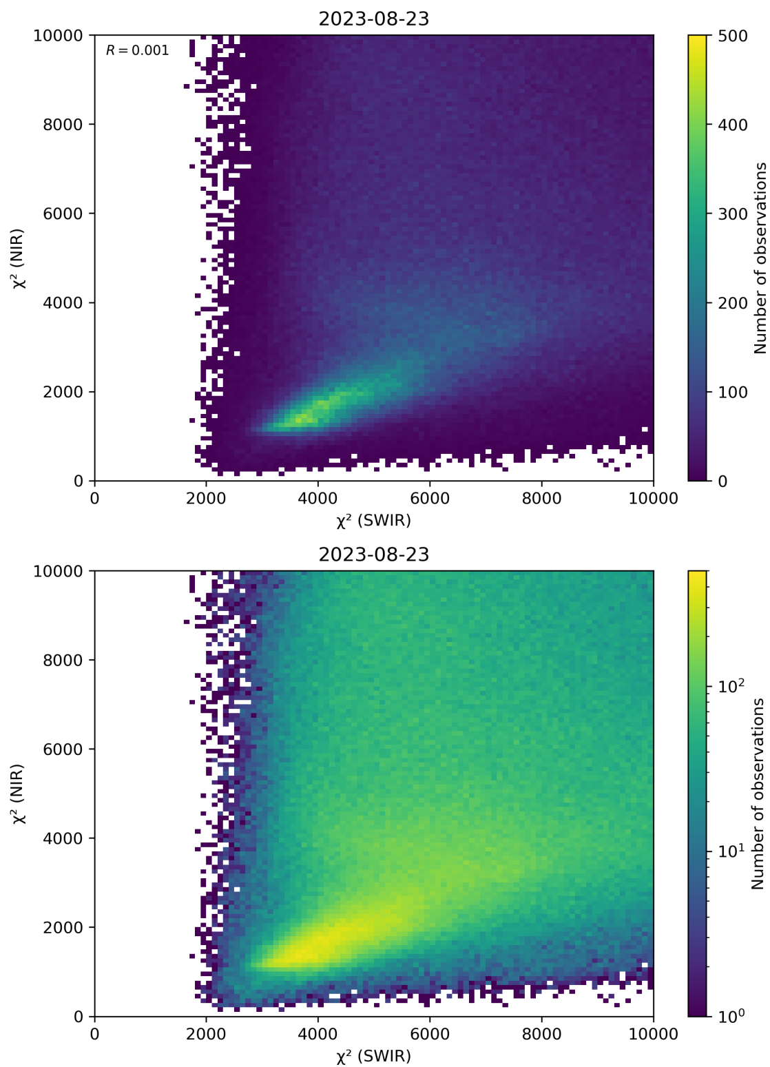
Figure 47: Scatter density plot of “ \chi^2 (SWIR)” against “ \chi^2 (NIR)” for 2023-08-22 to 2023-08-24.
