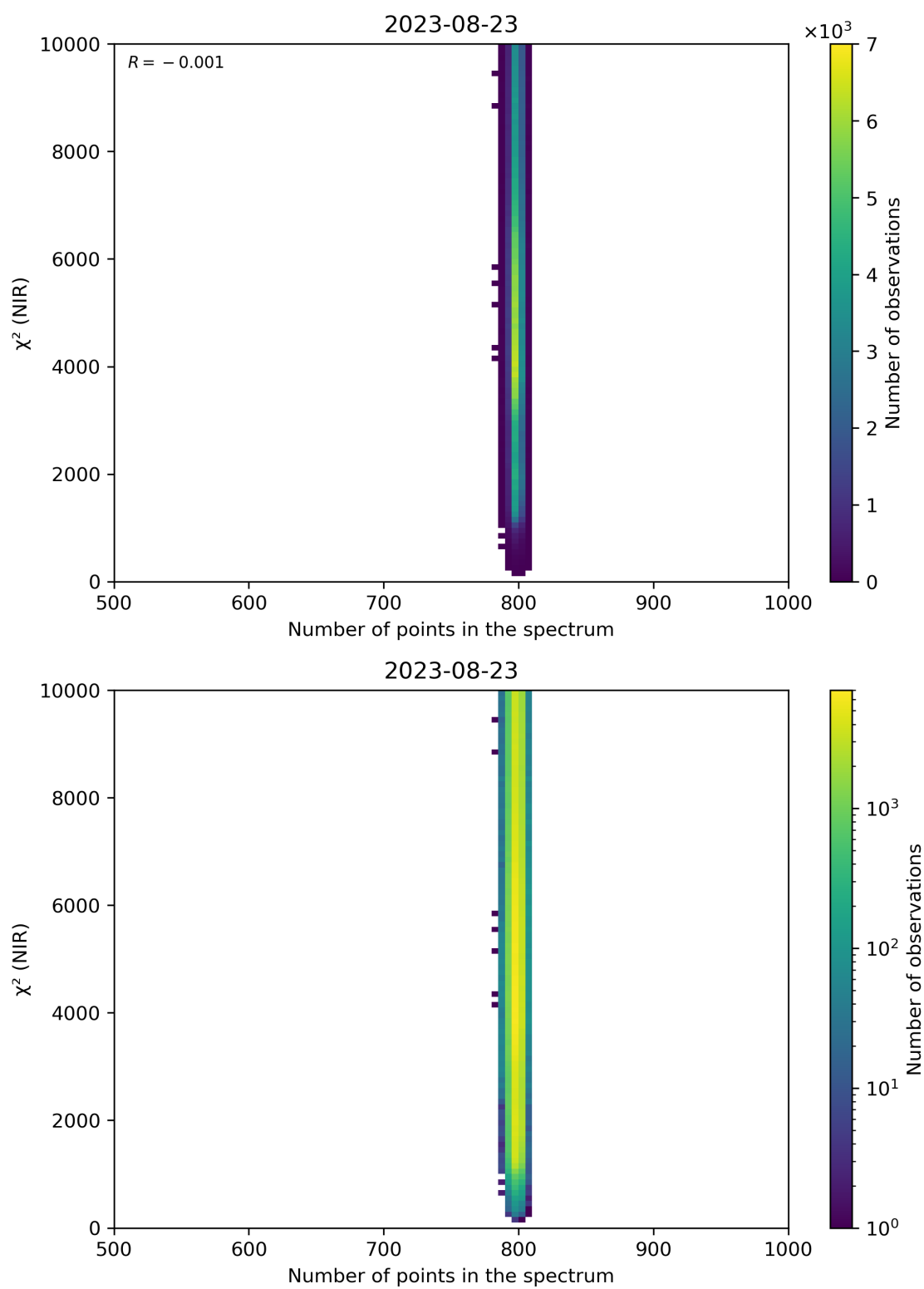
Figure 88: Scatter density plot of “Number of points in the spectrum” against “ \chi^2 (NIR)” for 2023-08-22 to 2023-08-24.
