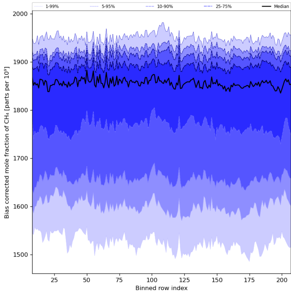
Figure 36: Along track statistics of “Bias corrected mole fraction of CH 4 ” for 2023-08-22 to 2023-08-24
