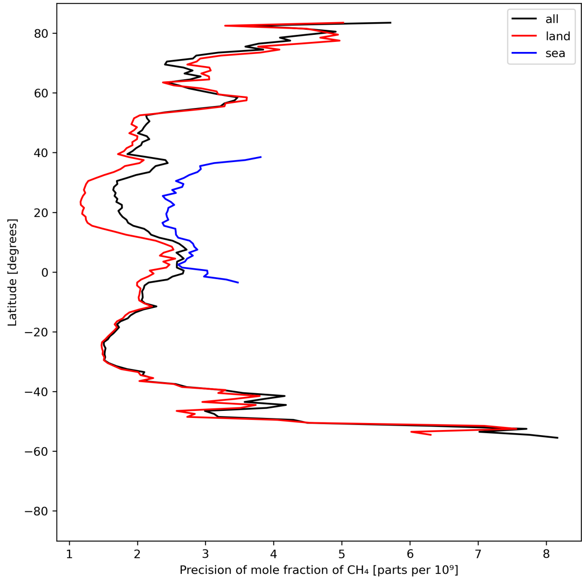
Figure 13: Zonal average of “Precision of mole fraction of CH 4 ” for 2023-08-22 to 2023-08-24.
