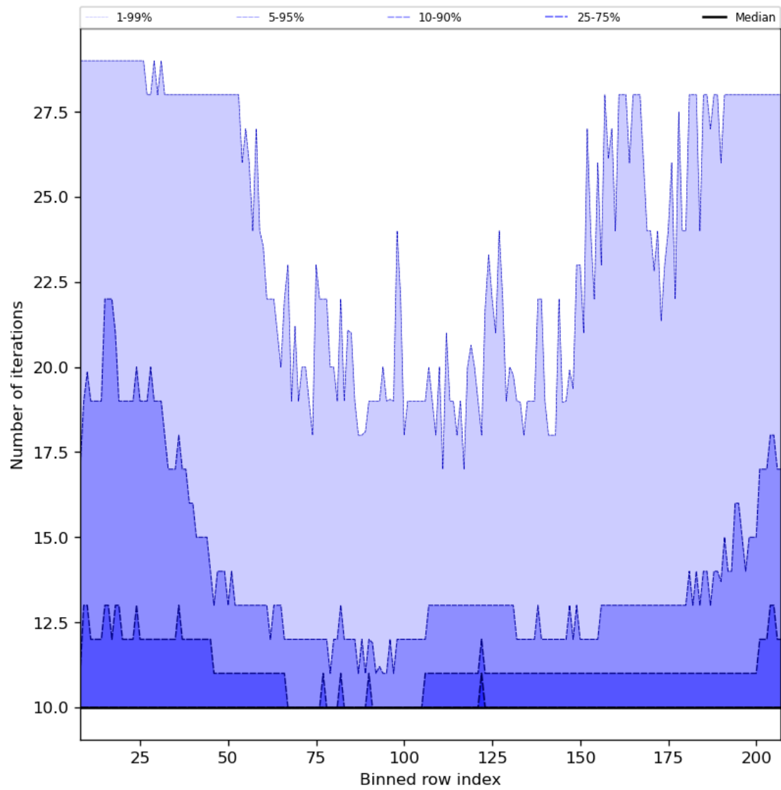
Figure 42: Along track statistics of “Number of iterations” for 2023-08-22 to 2023-08-24
