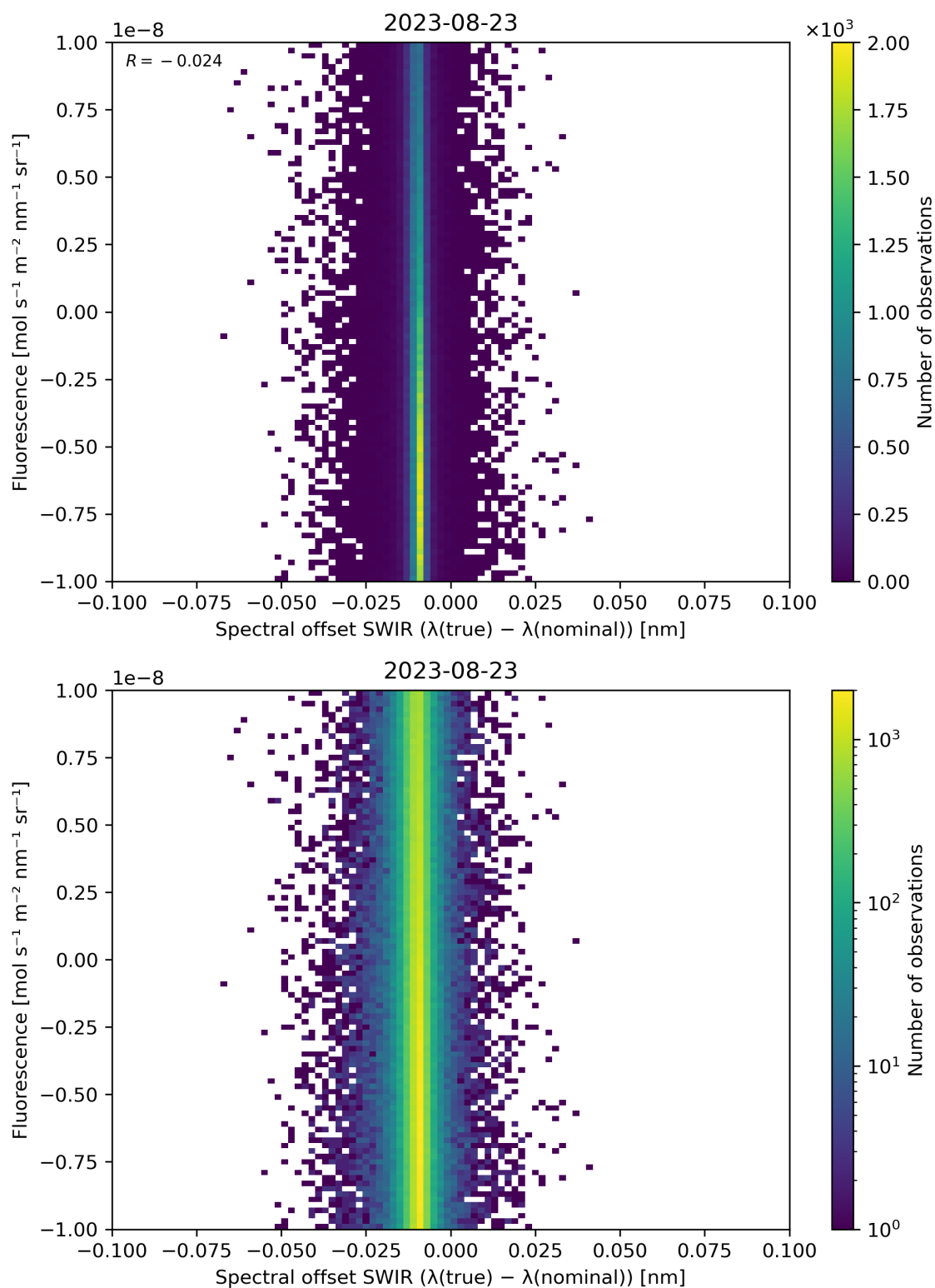
Figure 120: Scatter density plot of “Spectral offset SWIR ( \lambda(\text{true}) - \lambda(\text{nominal}) )” against “Fluorescence” for 2023-08-22 to 2023-08-24.
