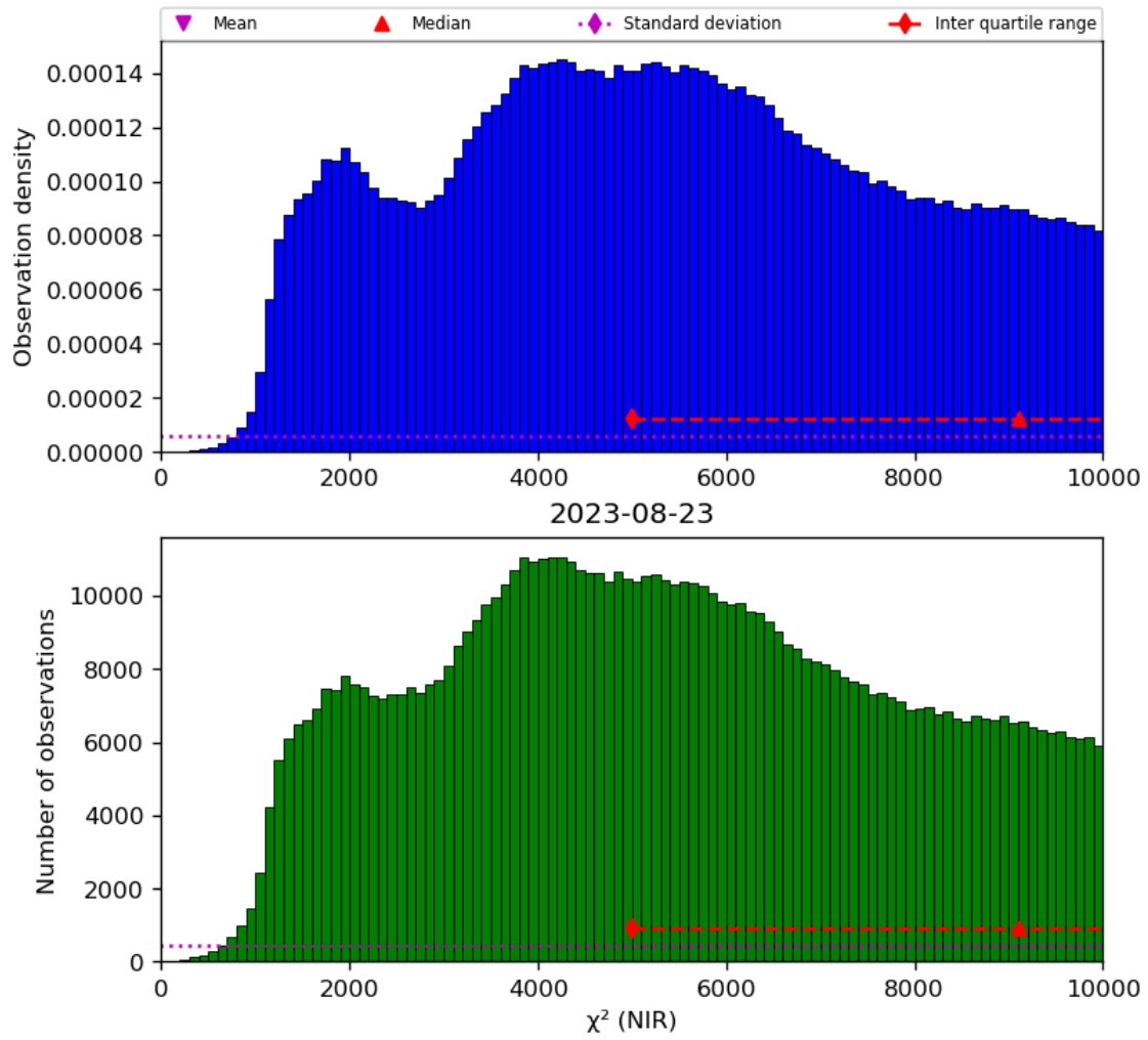
Figure 29: Histogram of “ \chi^2 (NIR)” for 2023-08-22 to 2023-08-24
