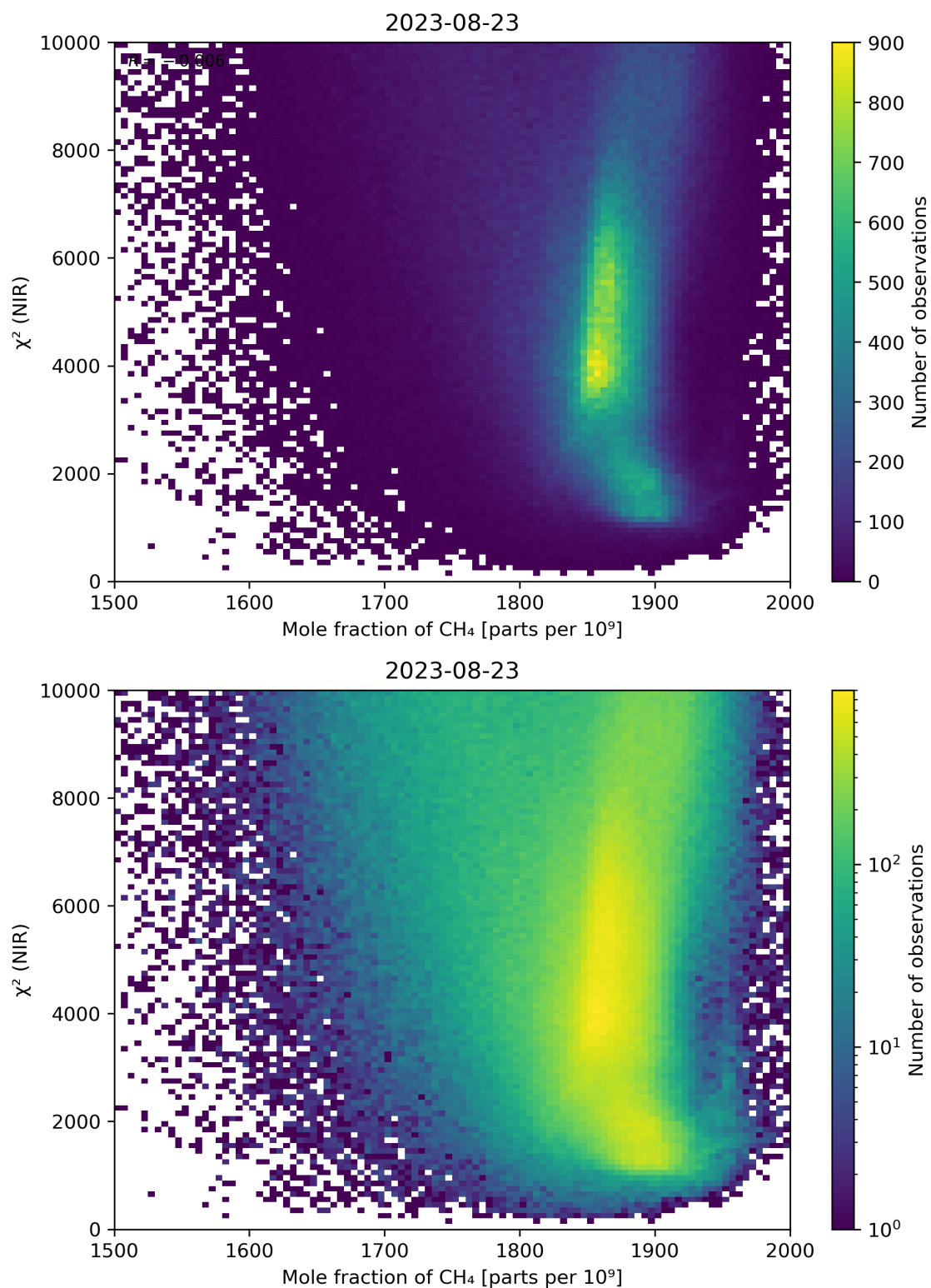
Figure 70: Scatter density plot of “Mole fraction of \text{CH}_4 ” against “ \chi^2 (NIR)” for 2023-08-22 to 2023-08-24.
