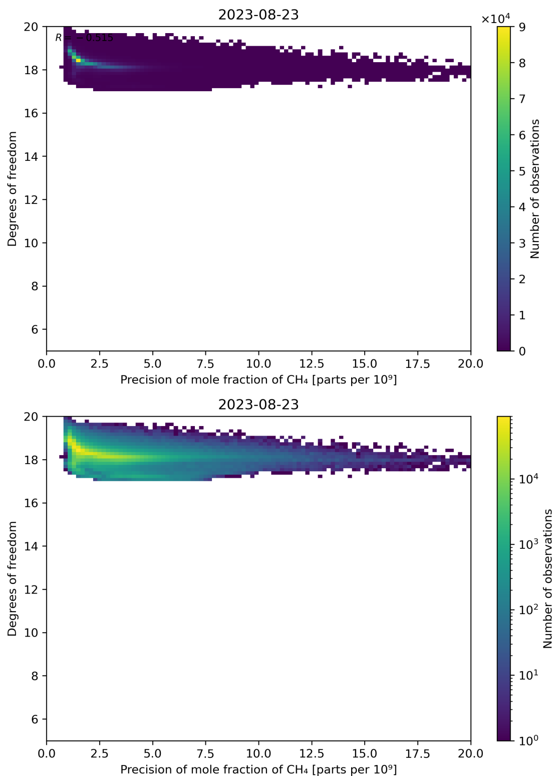
Figure 80: Scatter density plot of “Precision of mole fraction of CH 4 ” against “Degrees of freedom” for 2023-08-22 to 2023-08-24.
