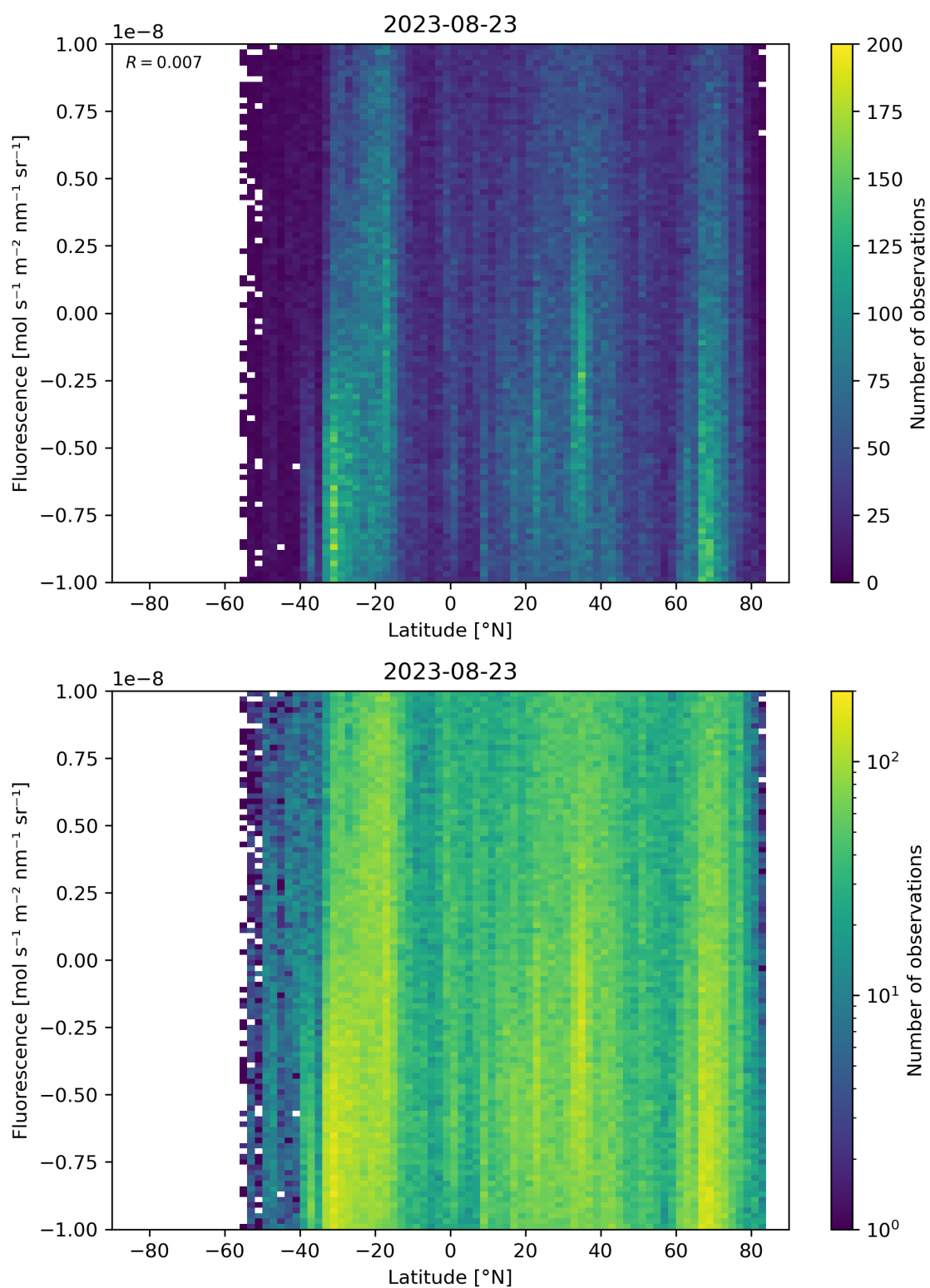
Figure 56: Scatter density plot of “Latitude” against “Fluorescence” for 2023-08-22 to 2023-08-24.
