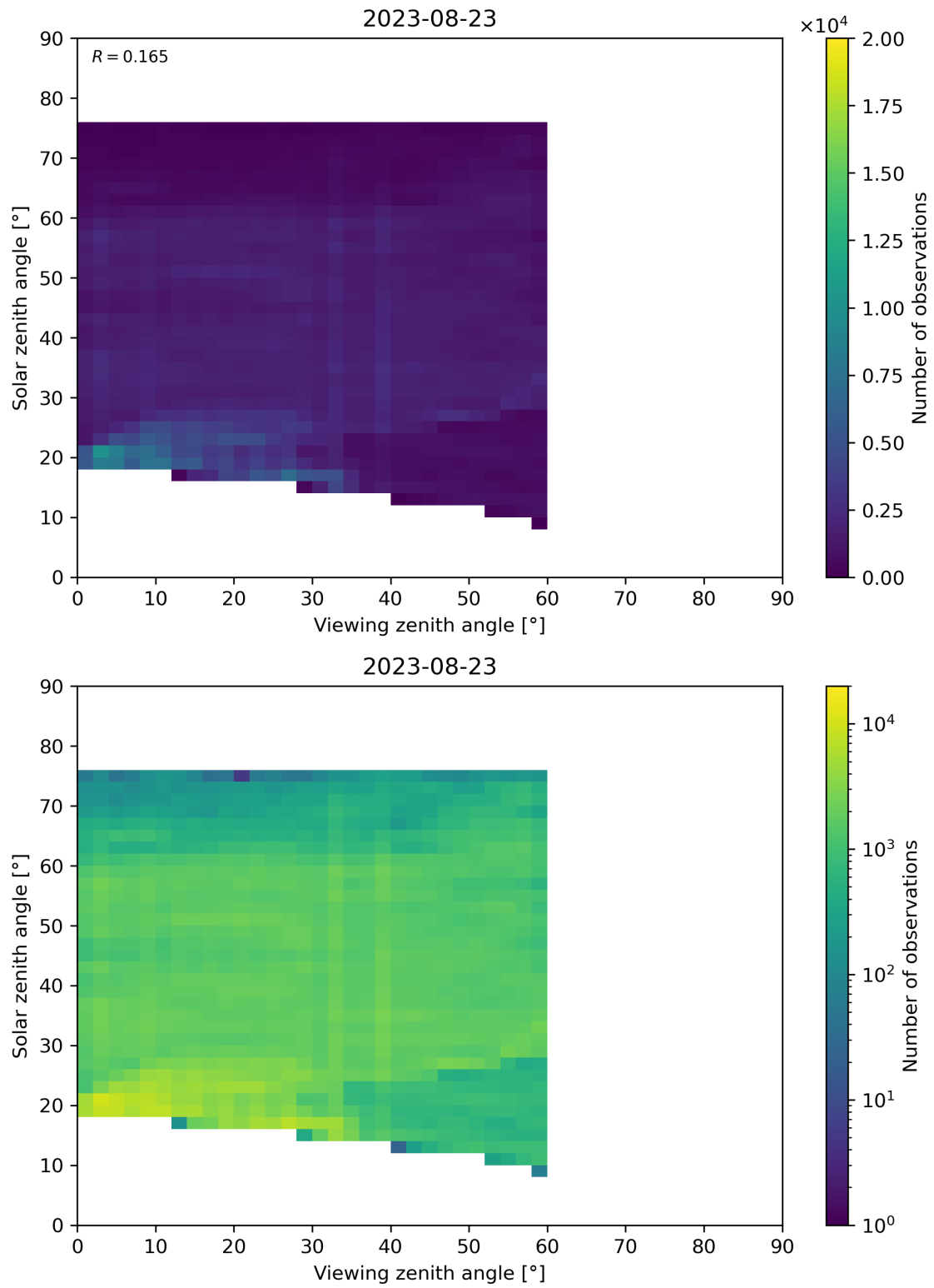
Figure 115: Scatter density plot of “Viewing zenith angle” against “Solar zenith angle” for 2023-08-22 to 2023-08-24.
