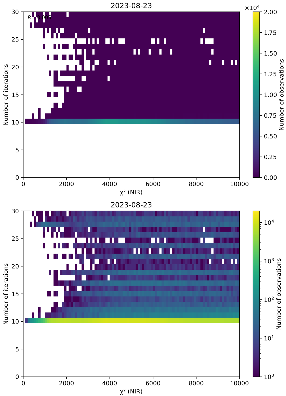
Figure 46: Scatter density plot of “ \chi^2 (NIR)” against “Number of iterations” for 2023-08-22 to 2023-08-24.
