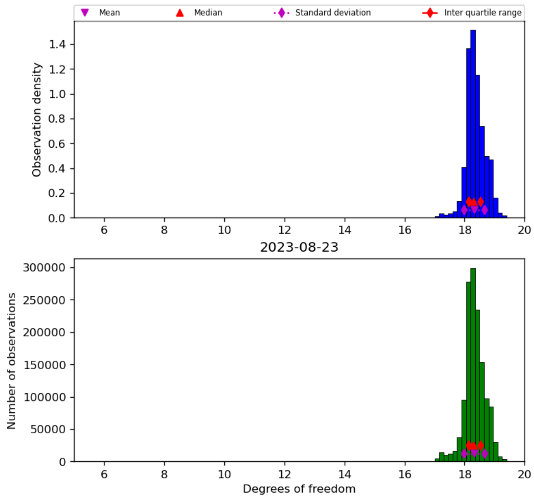
Figure 30: Histogram of “Degrees of freedom” for 2023-08-22 to 2023-08-24
