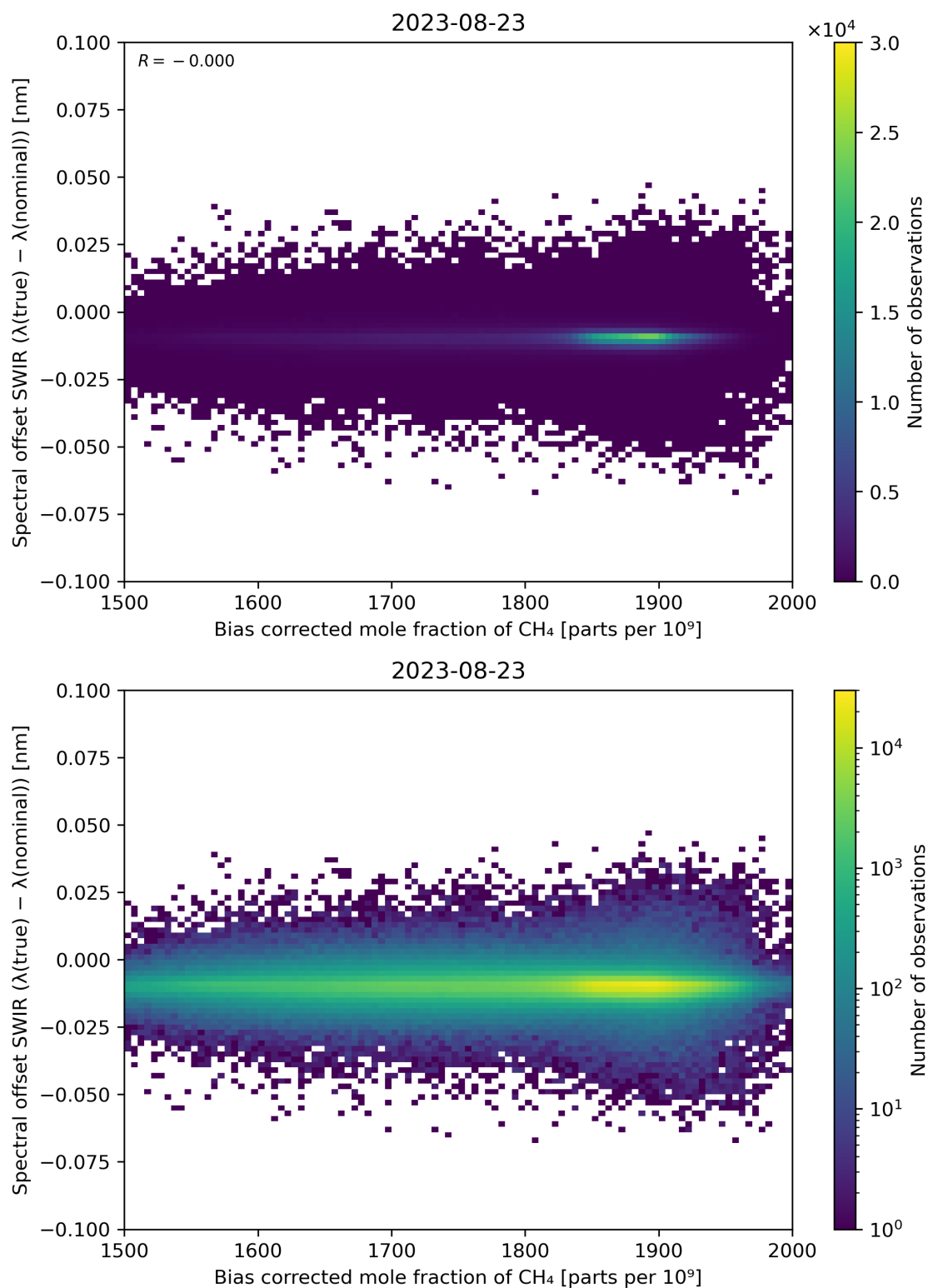
Figure 69: Scatter density plot of “Bias corrected mole fraction of \text{CH}_4 ” against “Spectral offset SWIR ( \lambda(\text{true}) - \lambda(\text{nominal}) )” for 2023-08-22 to 2023-08-24.
