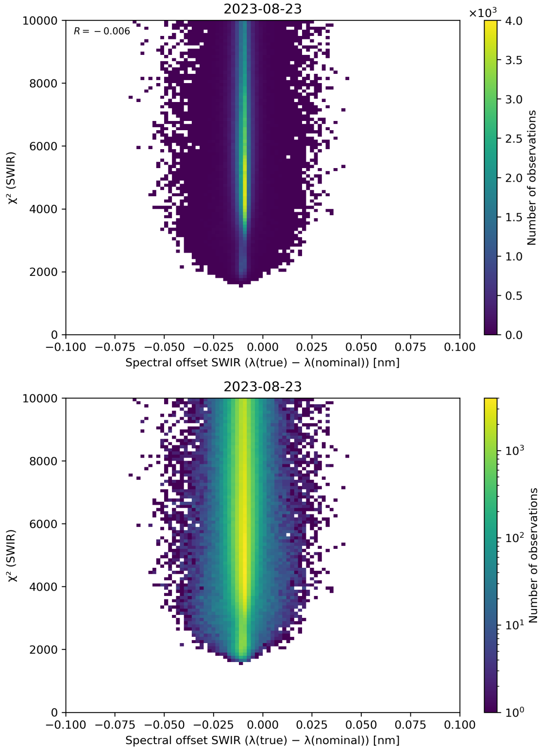
Figure 118: Scatter density plot of “Spectral offset SWIR ( \lambda(\text{true}) - \lambda(\text{nominal}) )” against “ \chi^2 (SWIR)” for 2023-08-22 to 2023-08-24.
