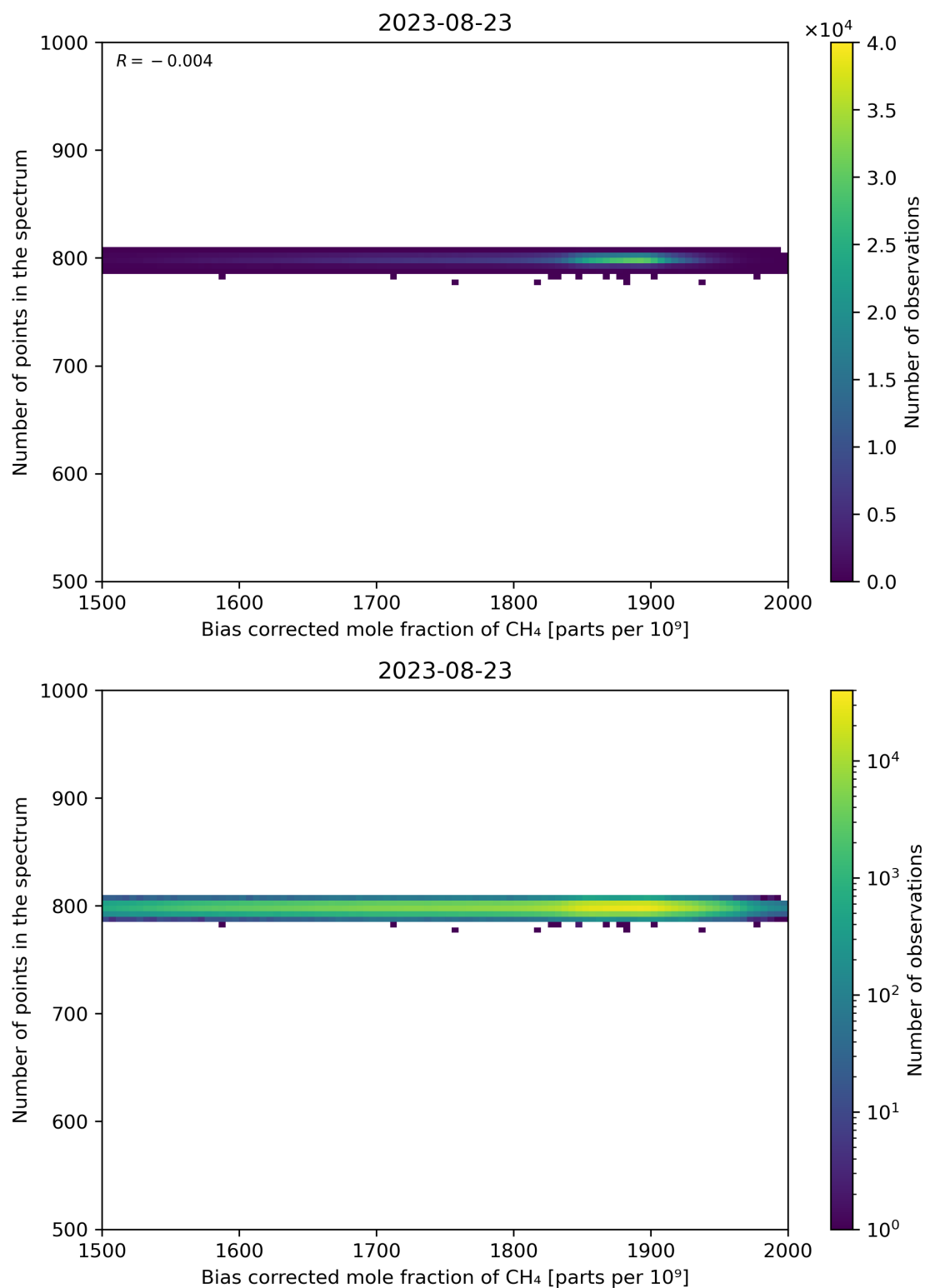
Figure 68: Scatter density plot of “Bias corrected mole fraction of CH 4 ” against “Number of points in the spectrum” for 2023-08-22 to 2023-08-24.
