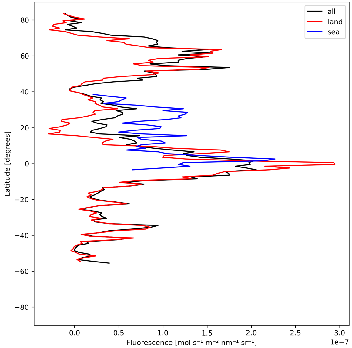
Figure 21: Zonal average of “Fluorescence” for 2023-08-22 to 2023-08-24.
