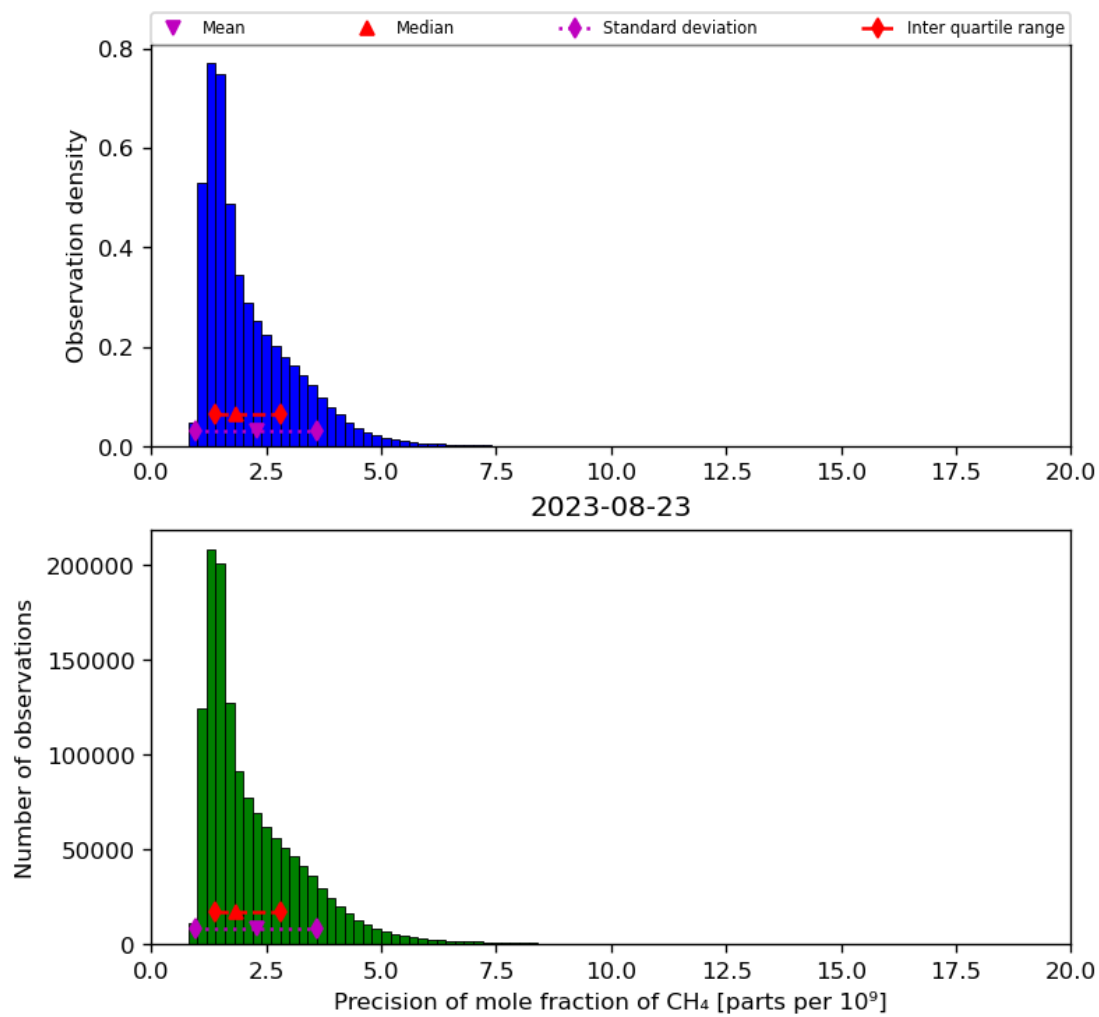
Figure 24: Histogram of “Precision of mole fraction of CH 4 ” for 2023-08-22 to 2023-08-24
