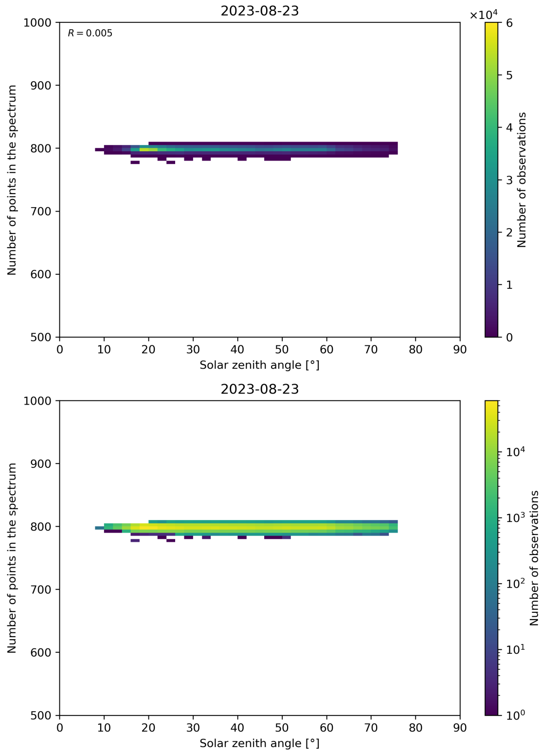
Figure 103: Scatter density plot of “Solar zenith angle” against “Number of points in the spectrum” for 2023-08-22 to 2023-08-24.
