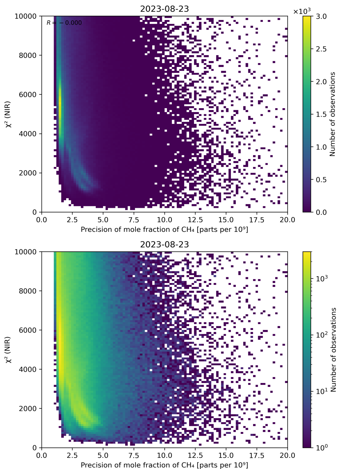
Figure 78: Scatter density plot of “Precision of mole fraction of CH 4 ” against “ \chi^2 (NIR)” for 2023-08-22 to 2023-08-24.
