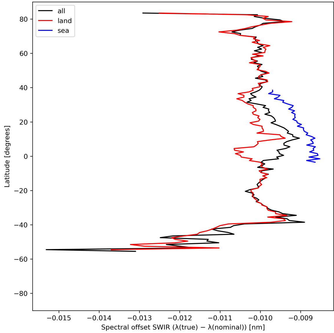
Figure 16: Zonal average of “Spectral offset SWIR ( \lambda(\text{true}) - \lambda(\text{nominal}) )” for 2023-08-22 to 2023-08-24.
