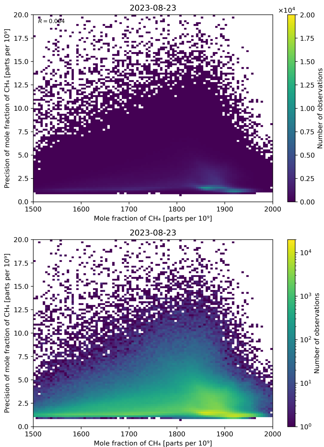
Figure 75: Scatter density plot of “Mole fraction of CH 4 ” against “Precision of mole fraction of CH 4 ” for 2023-08-22 to 2023-08-24.
