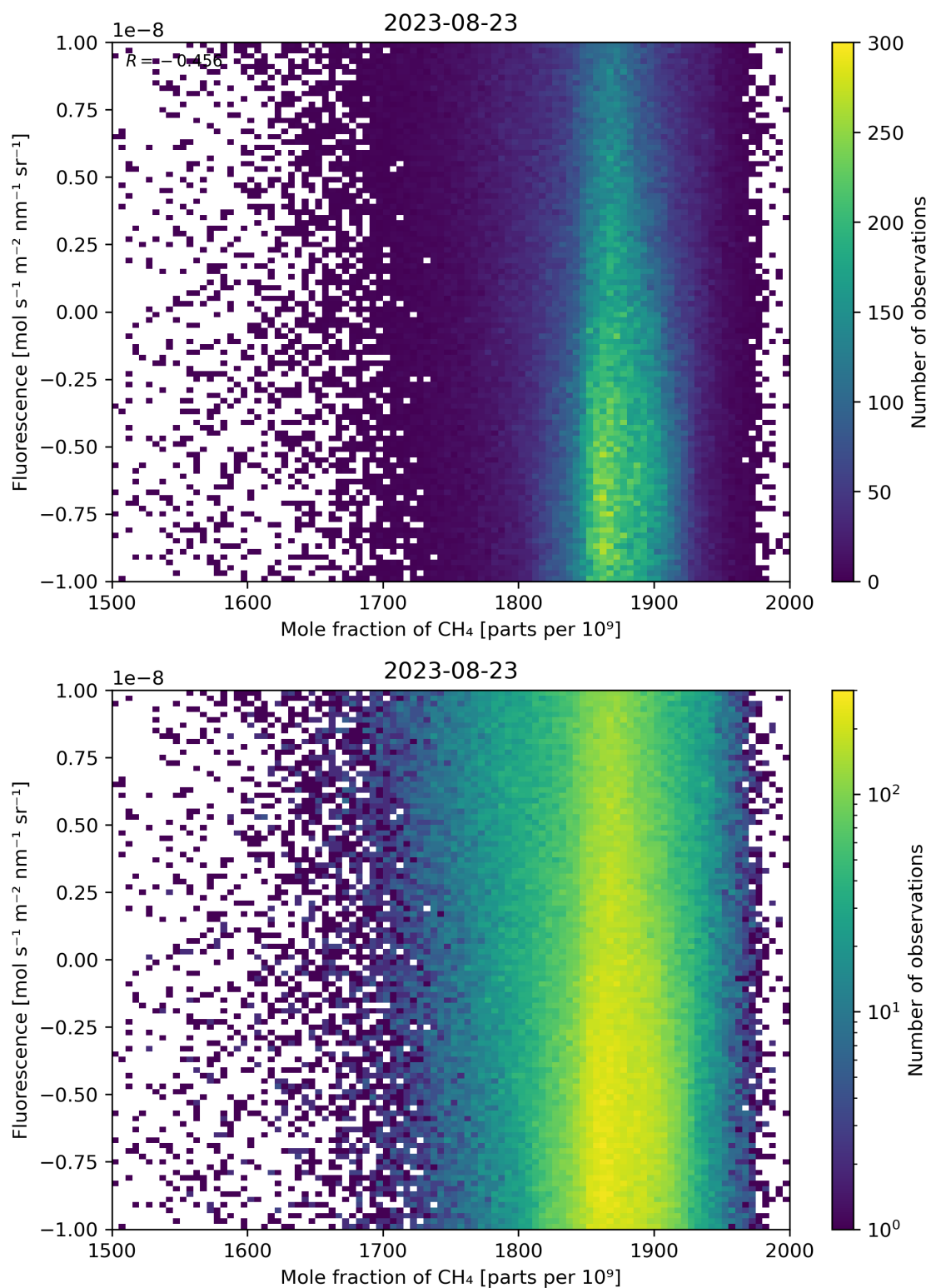
Figure 73: Scatter density plot of “Mole fraction of \text{CH}_4 ” against “Fluorescence” for 2023-08-22 to 2023-08-24.
