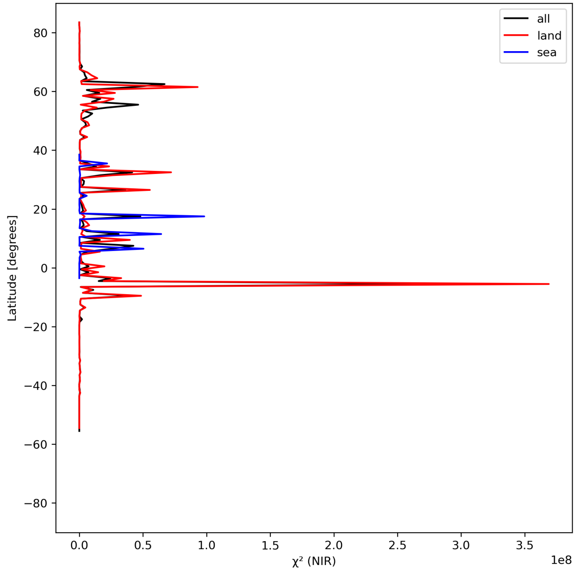
Figure 18: Zonal average of “ \chi^2 (NIR)” for 2023-08-22 to 2023-08-24.
