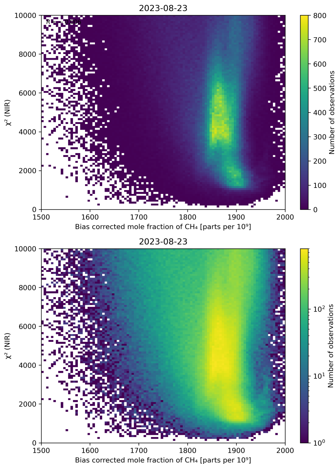
Figure 63: Scatter density plot of “Bias corrected mole fraction of \text{CH}_4 ” against “ \chi^2 (NIR)” for 2023-08-22 to 2023-08-24.
