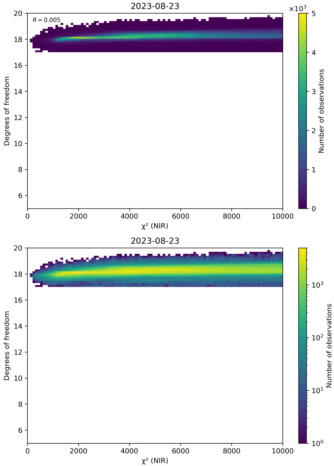
Figure 44: Scatter density plot of “ \chi^2 (NIR)” against “Degrees of freedom” for 2023-08-22 to 2023-08-24.
