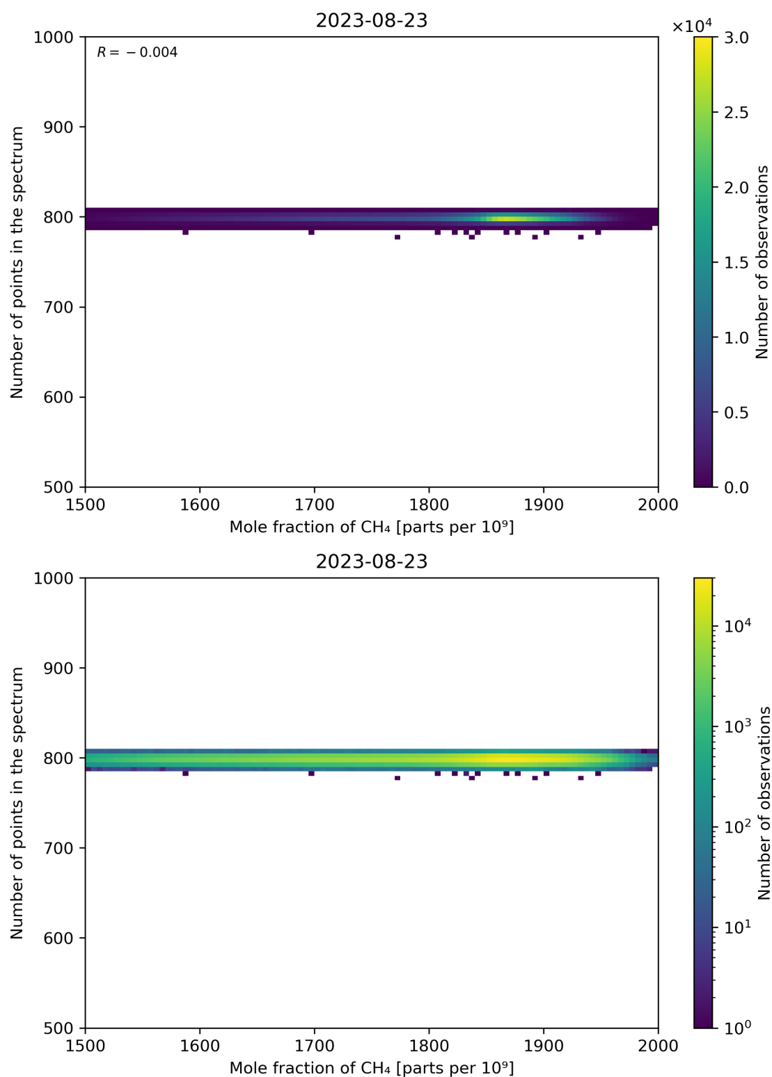
Figure 77: Scatter density plot of “Mole fraction of CH 4 ” against “Number of points in the spectrum” for 2023-08-22 to 2023-08-24.
