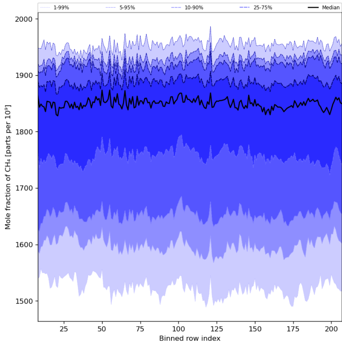
Figure 34: Along track statistics of “Mole fraction of CH 4 ” for 2023-08-22 to 2023-08-24
