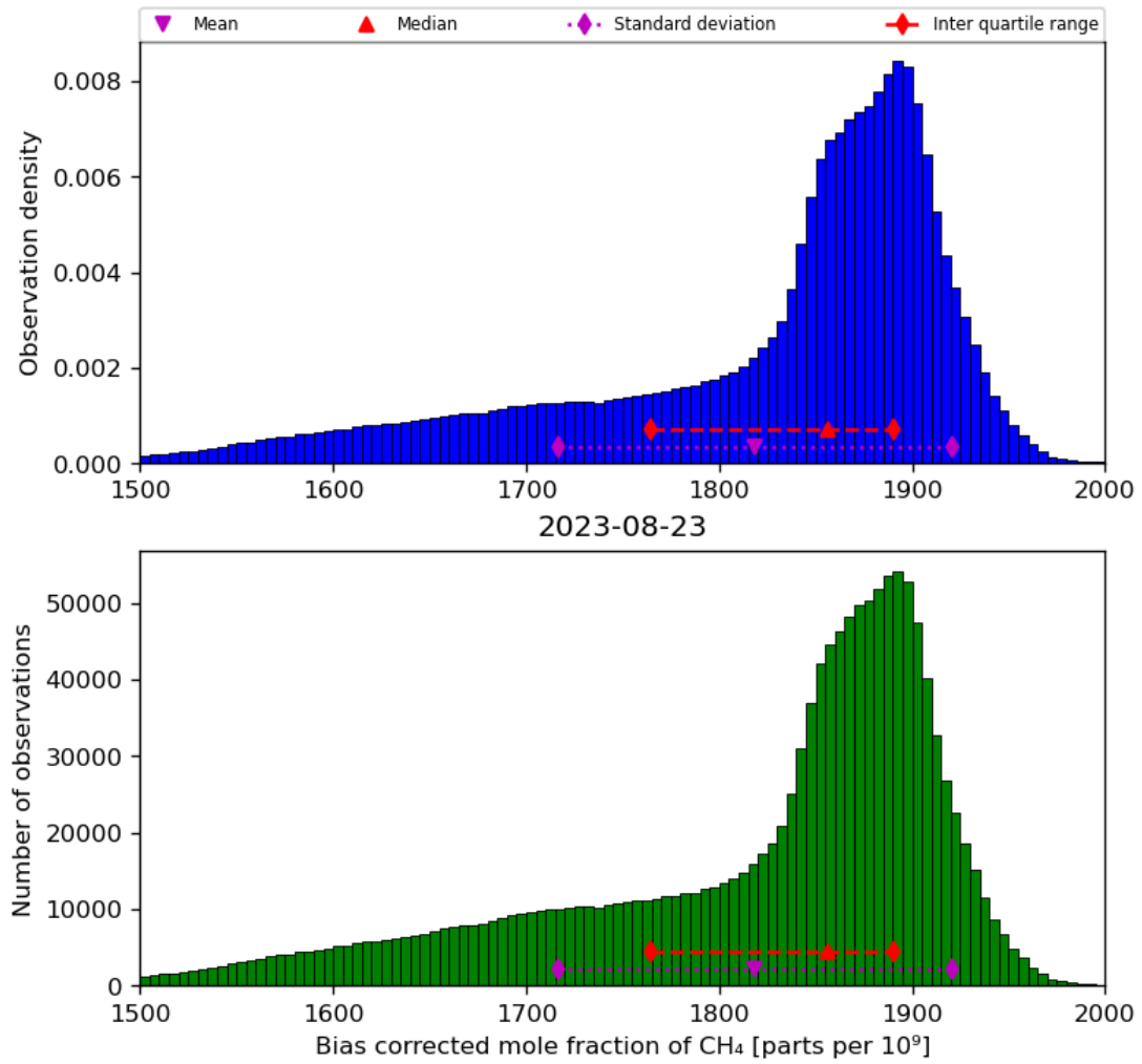
Figure 25: Histogram of “Bias corrected mole fraction of CH 4 ” for 2023-08-22 to 2023-08-24
