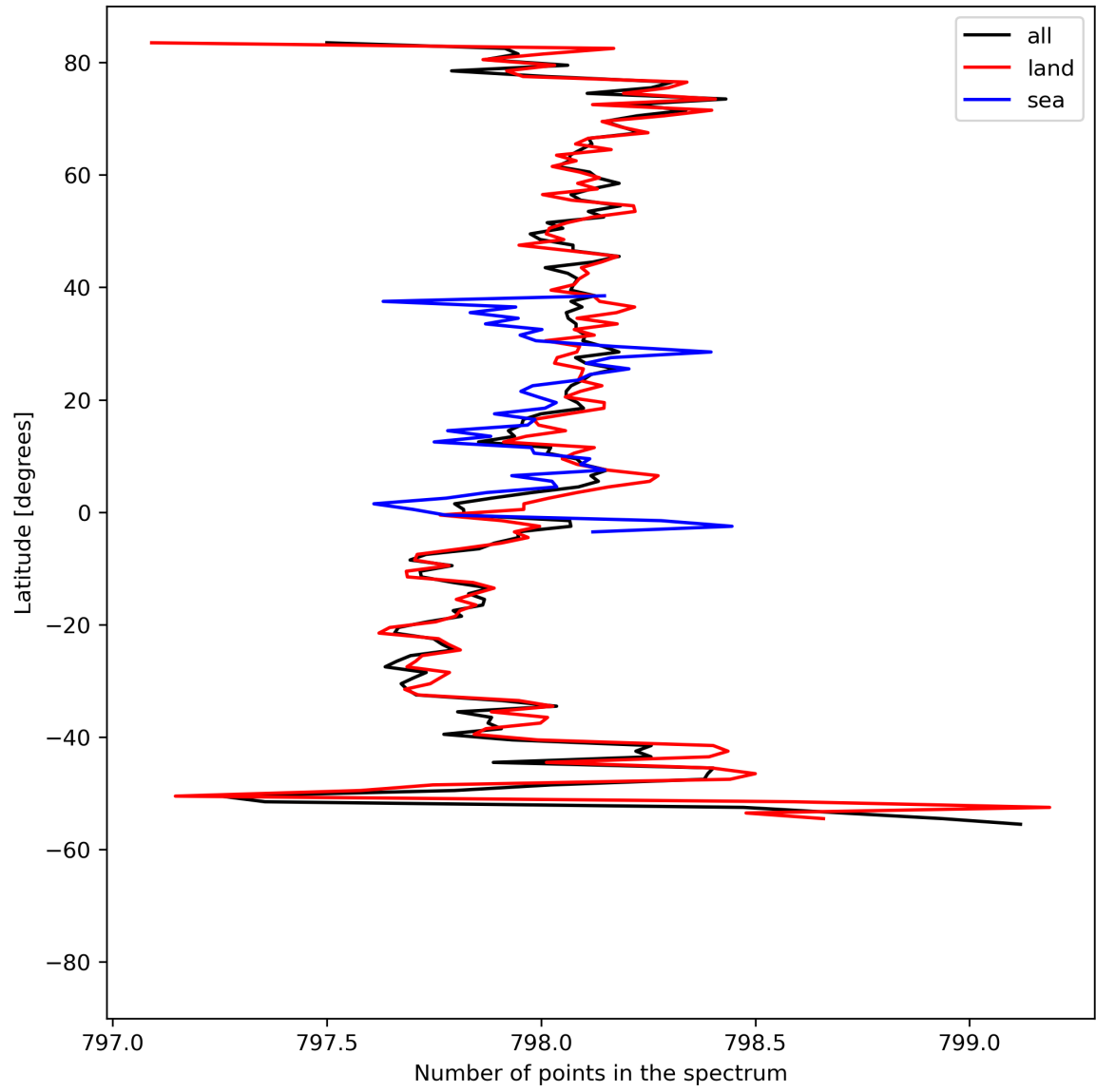
Figure 15: Zonal average of “Number of points in the spectrum” for 2023-08-22 to 2023-08-24.
