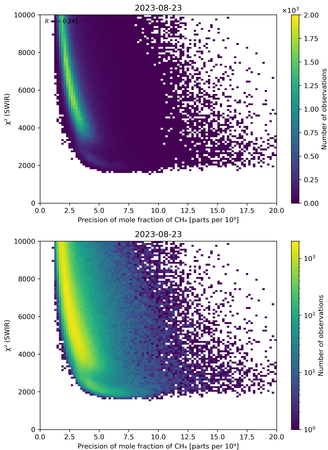
Figure 79: Scatter density plot of “Precision of mole fraction of CH 4 ” against “ \chi^2 (SWIR)” for 2023-08-22 to 2023-08-24.
