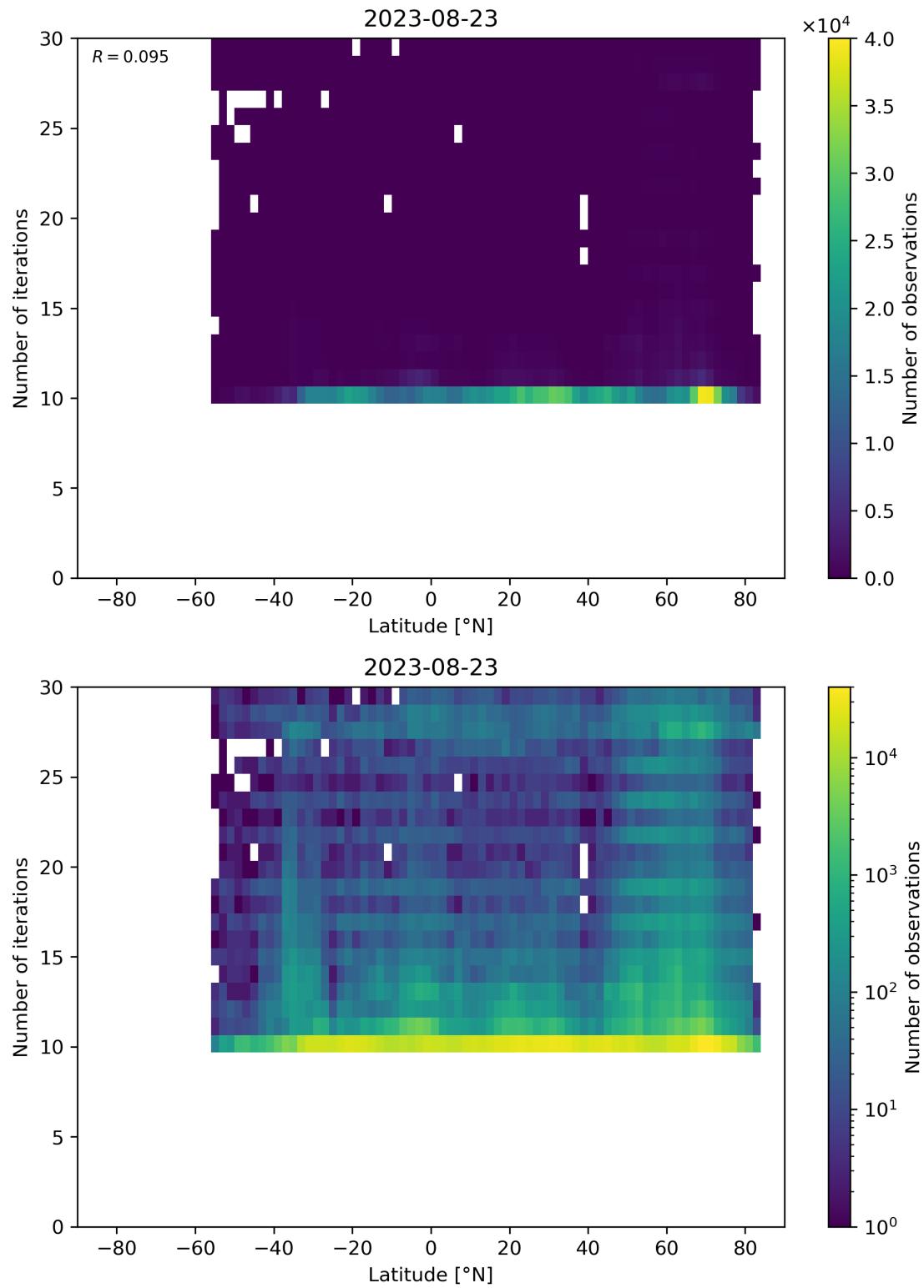
Figure 60: Scatter density plot of “Latitude” against “Number of iterations” for 2023-08-22 to 2023-08-24.
