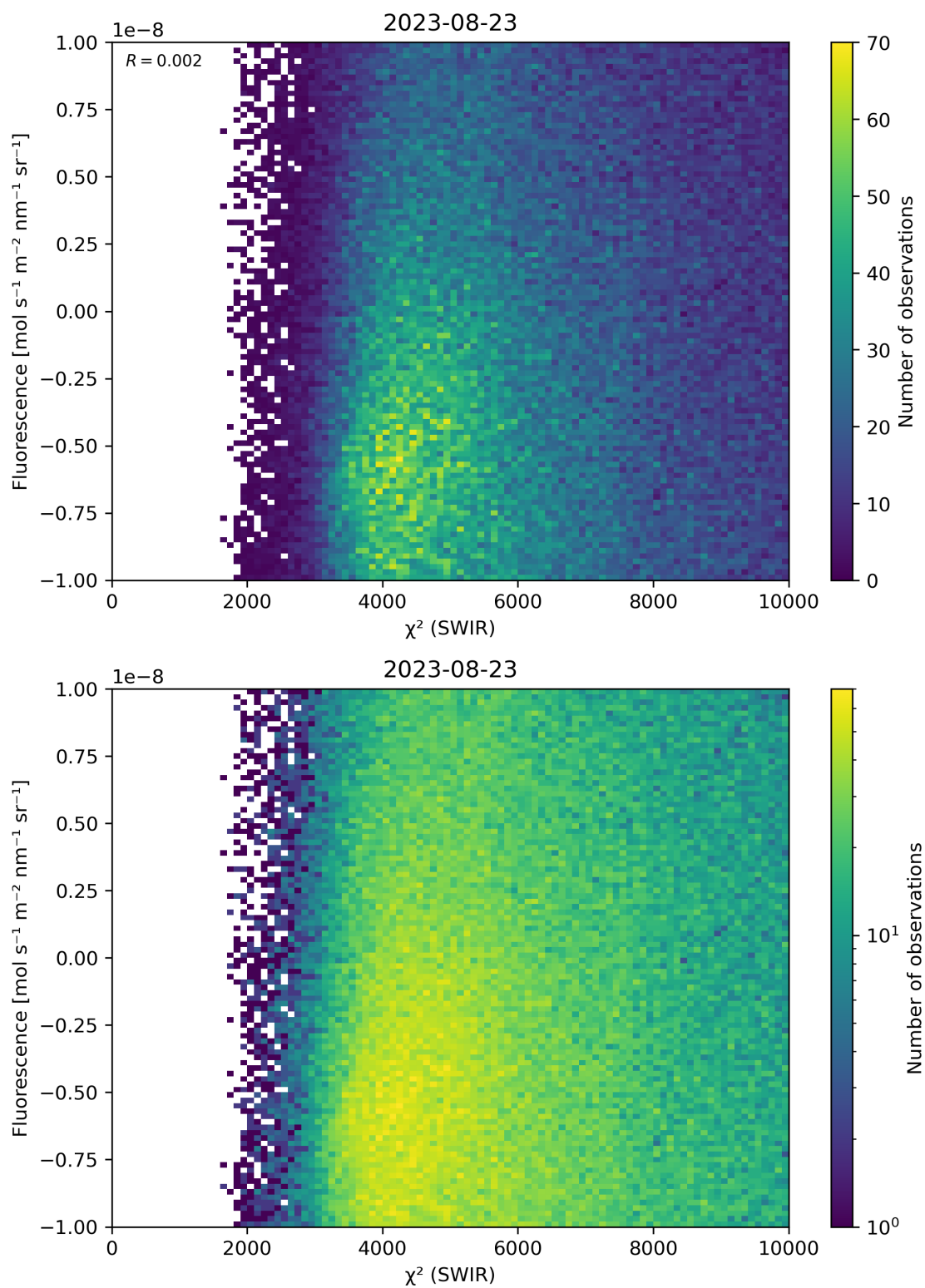
Figure 49: Scatter density plot of “ \chi^2 (SWIR)” against “Fluorescence” for 2023-08-22 to 2023-08-24.
