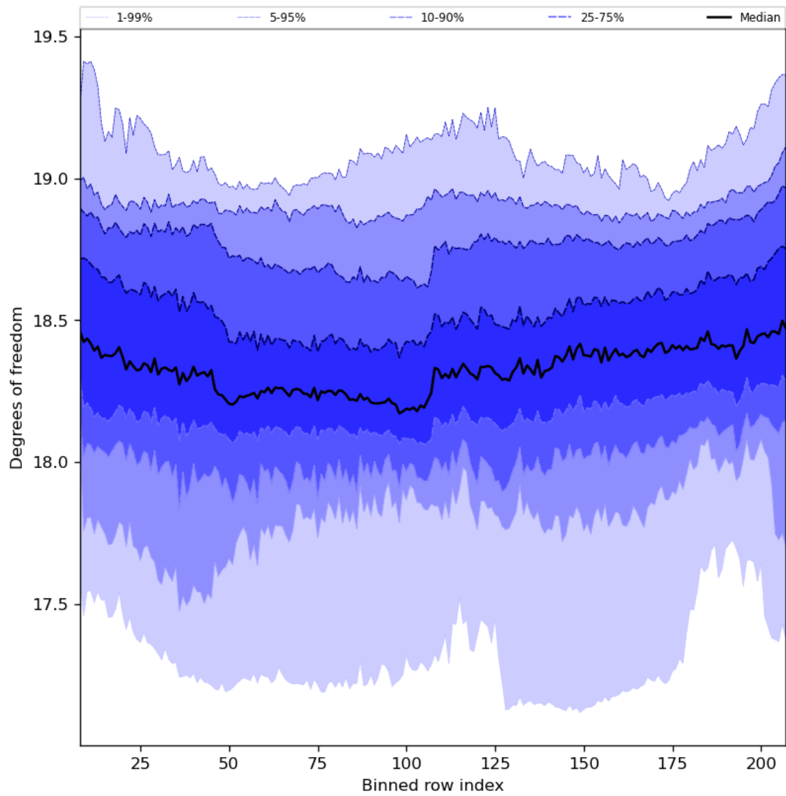
Figure 41: Along track statistics of “Degrees of freedom” for 2023-08-22 to 2023-08-24
