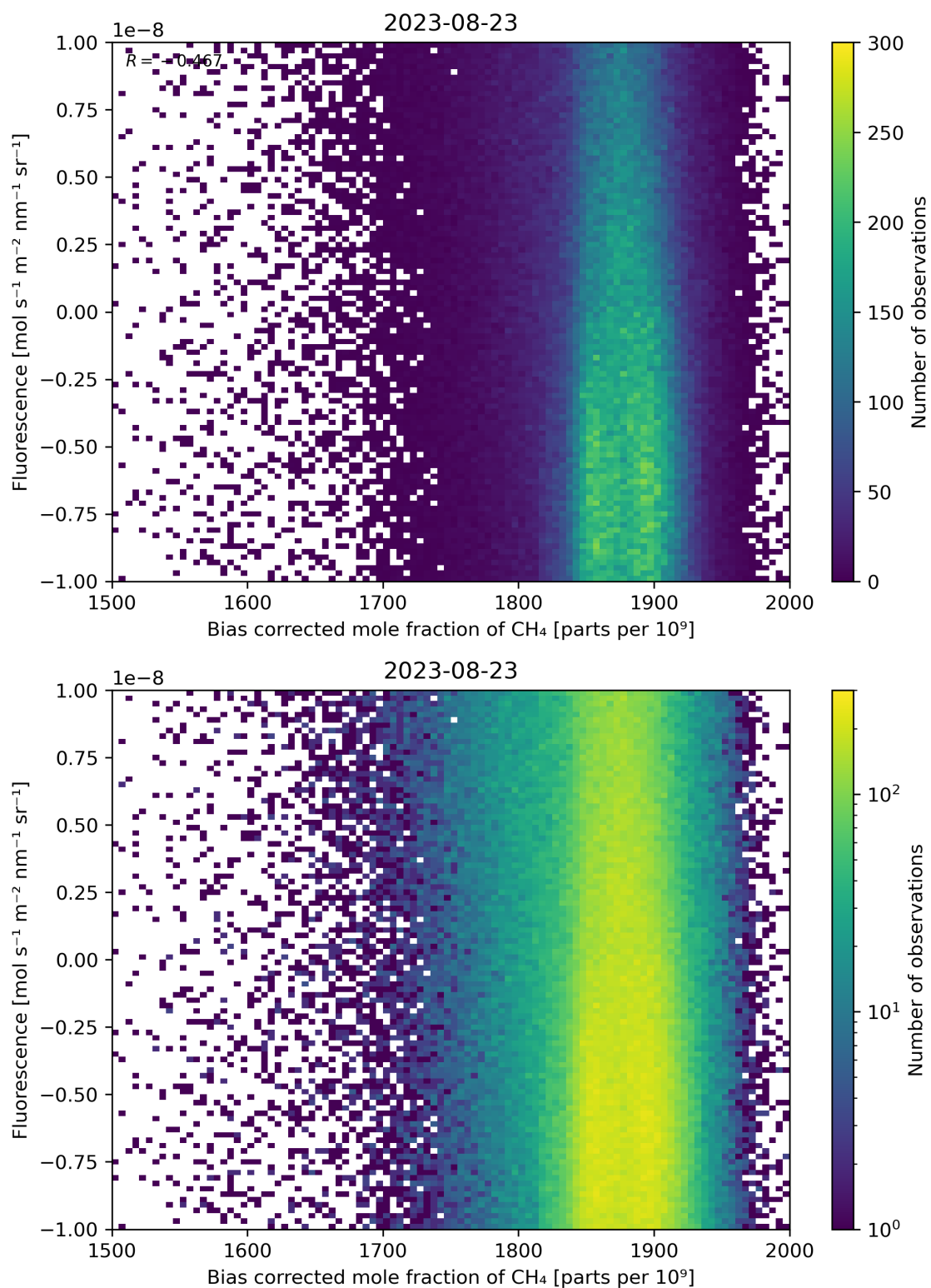
Figure 66: Scatter density plot of “Bias corrected mole fraction of \text{CH}_4 ” against “Fluorescence” for 2023-08-22 to 2023-08-24.
