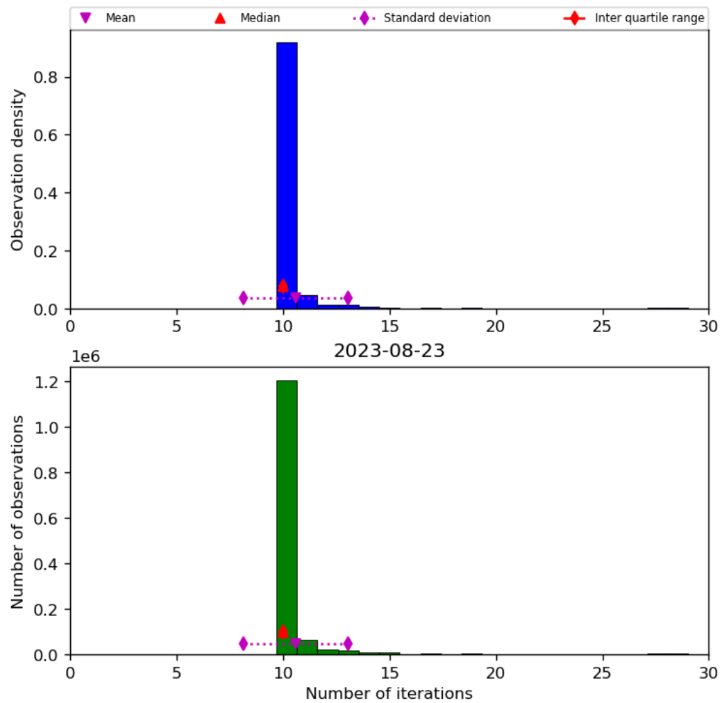
Figure 31: Histogram of “Number of iterations” for 2023-08-22 to 2023-08-24
