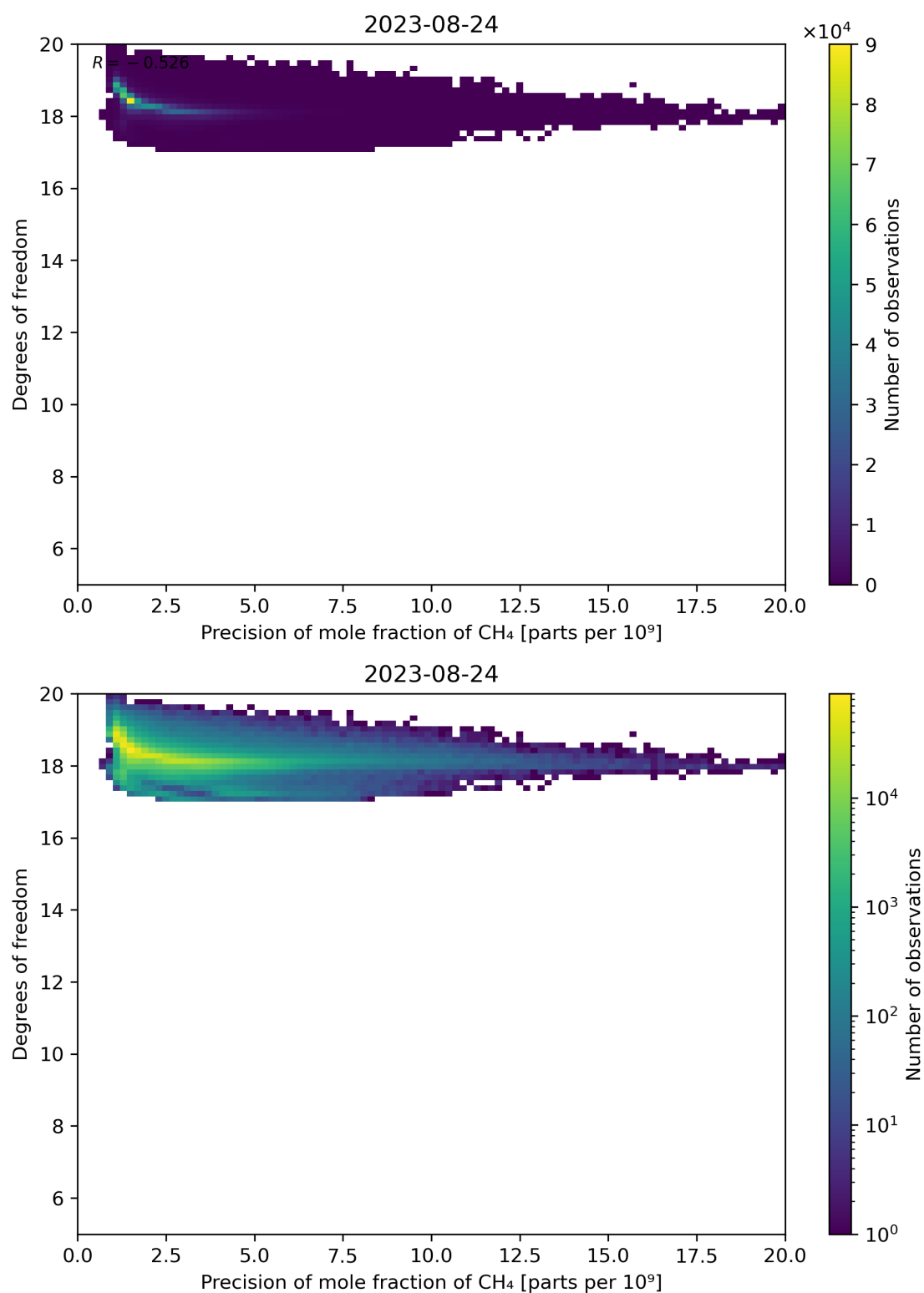
Figure 80: Scatter density plot of “Precision of mole fraction of CH 4 ” against “Degrees of freedom” for 2023-08-23 to 2023-08-25.
