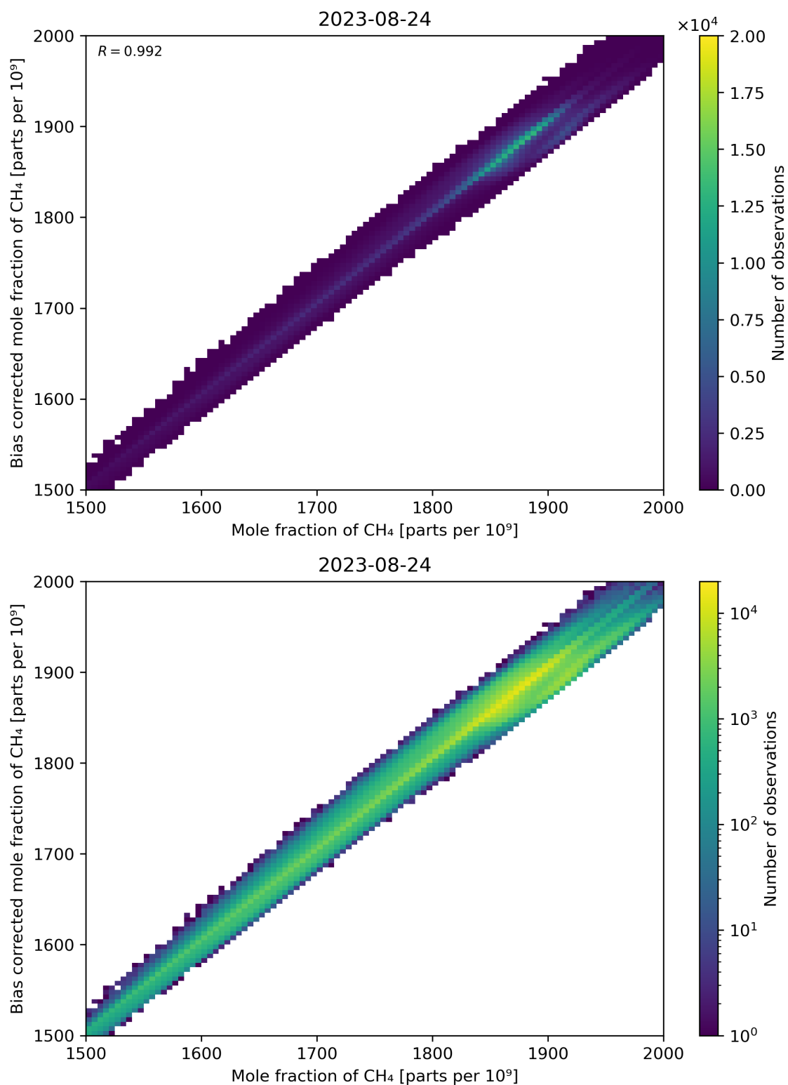
Figure 74: Scatter density plot of “Mole fraction of CH 4 ” against “Bias corrected mole fraction of CH 4 ” for 2023-08-23 to 2023-08-25.
