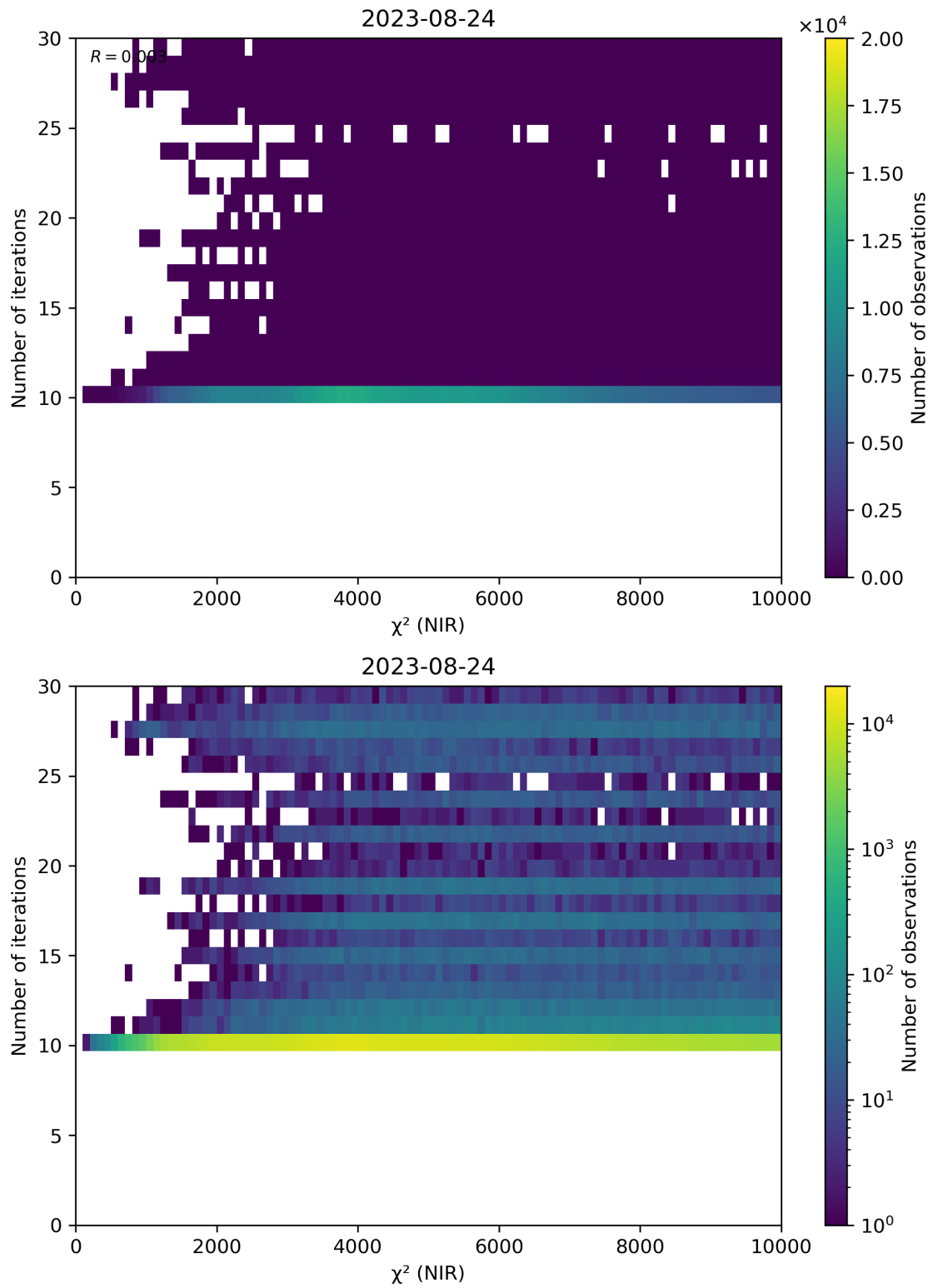
Figure 46: Scatter density plot of “ \chi^2 (NIR)” against “Number of iterations” for 2023-08-23 to 2023-08-25.
