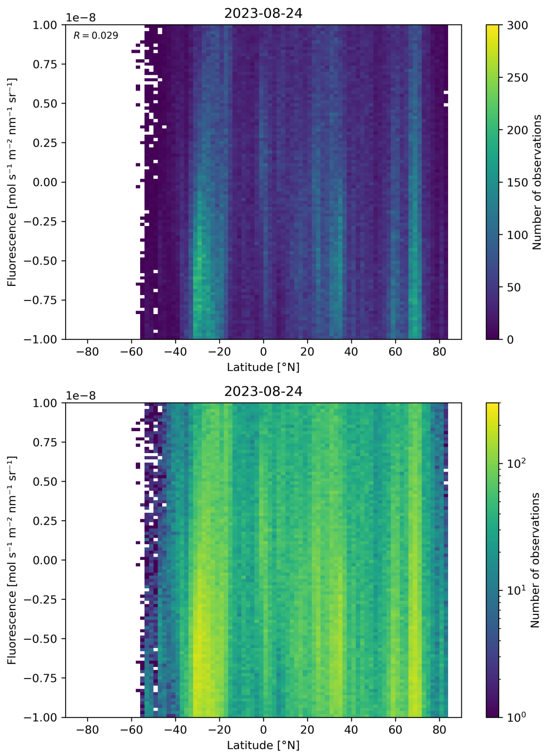
Figure 56: Scatter density plot of “Latitude” against “Fluorescence” for 2023-08-23 to 2023-08-25.
