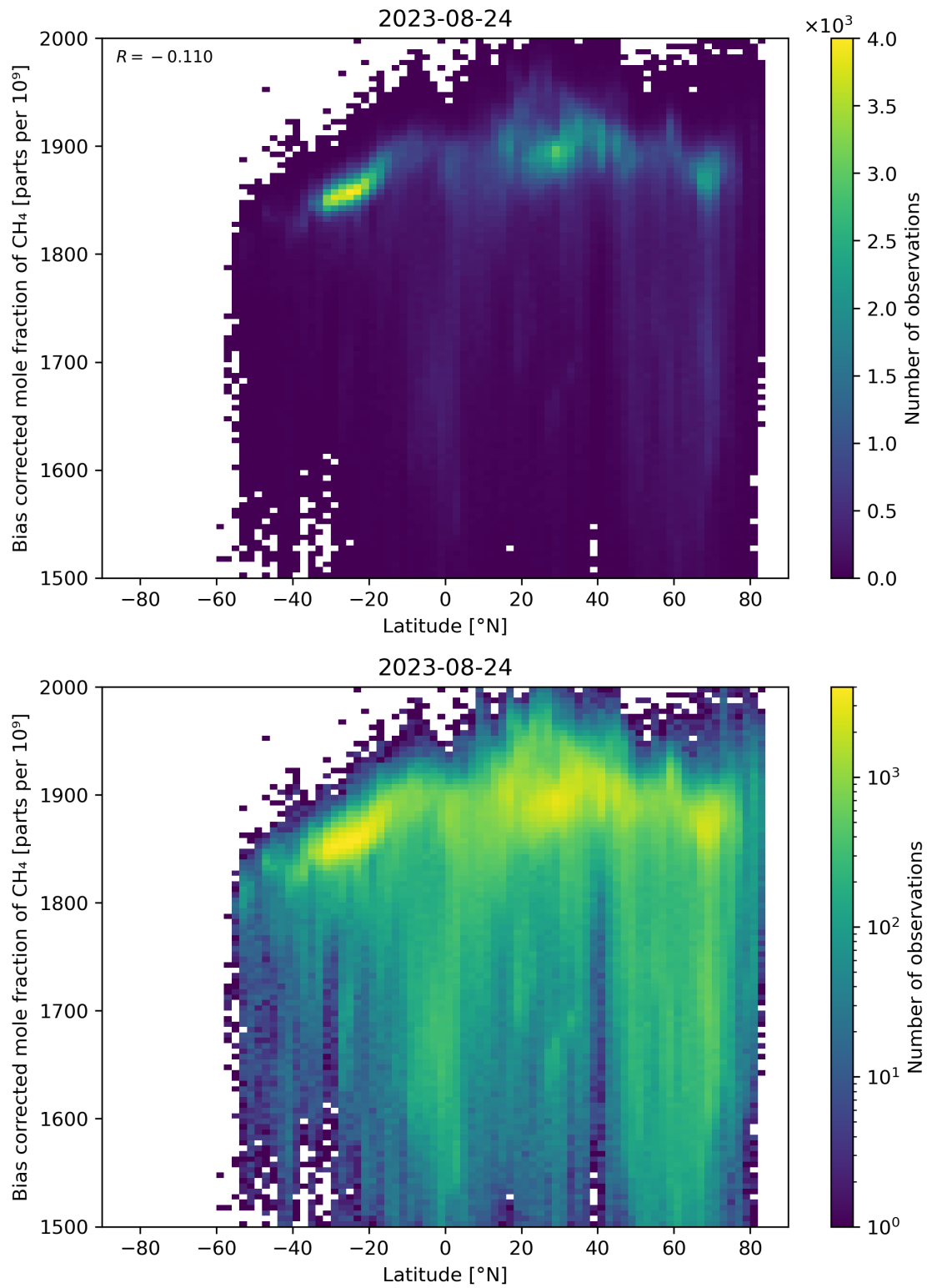
Figure 58: Scatter density plot of “Latitude” against “Bias corrected mole fraction of \text{CH}_4 ” for 2023-08-23 to 2023-08-25.
