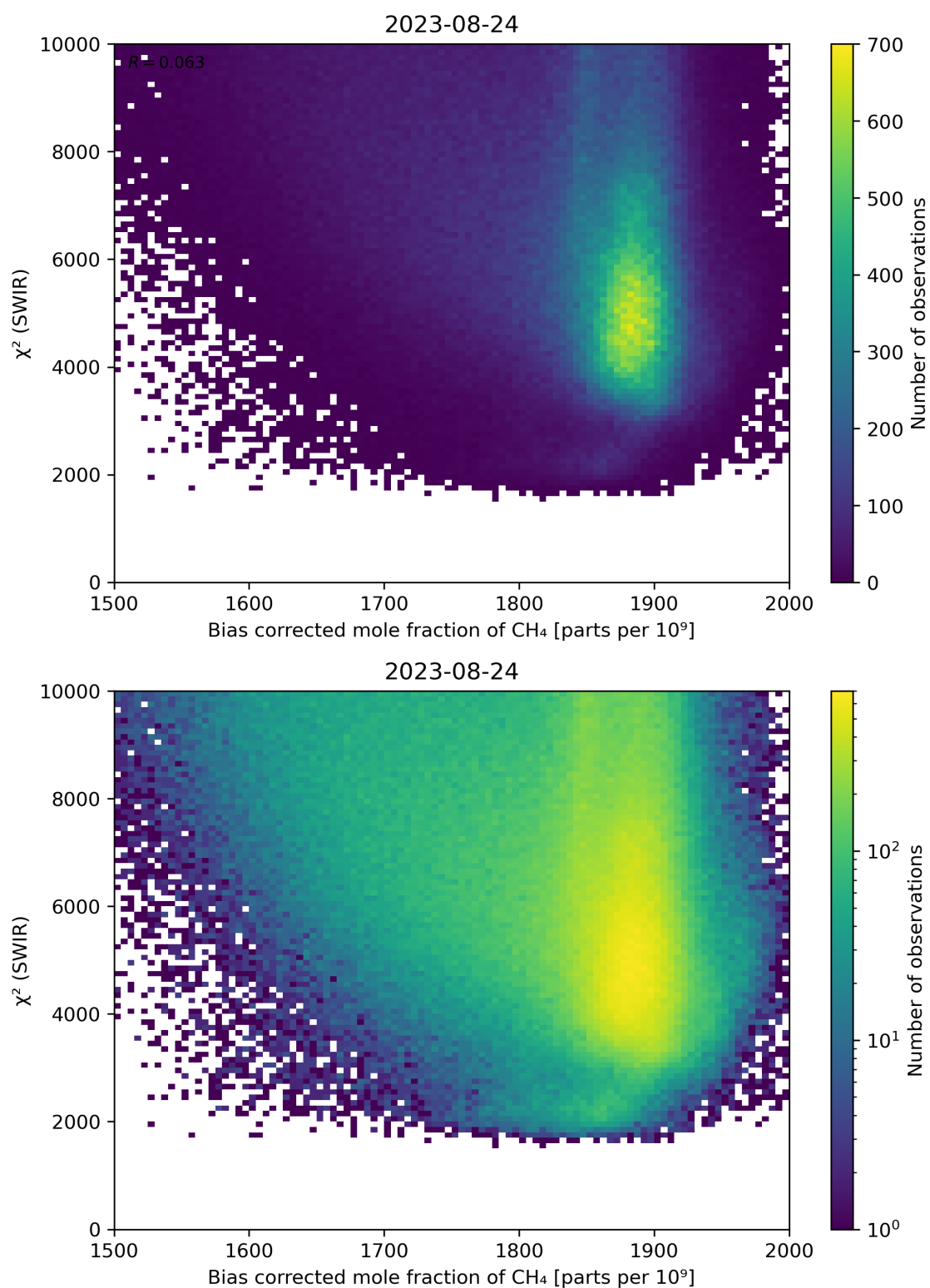
Figure 64: Scatter density plot of “Bias corrected mole fraction of CH 4 ” against “ \chi^2 (SWIR)” for 2023-08-23 to 2023-08-25.
