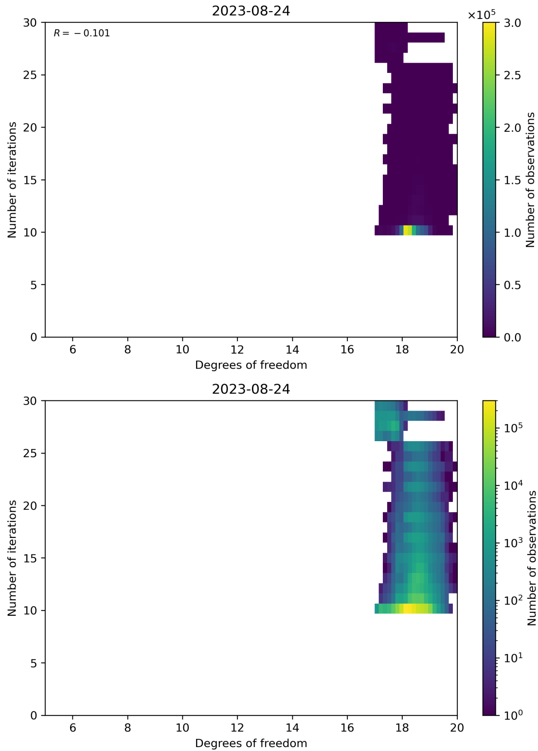
Figure 52: Scatter density plot of “Degrees of freedom” against “Number of iterations” for 2023-08-23 to 2023-08-25.
