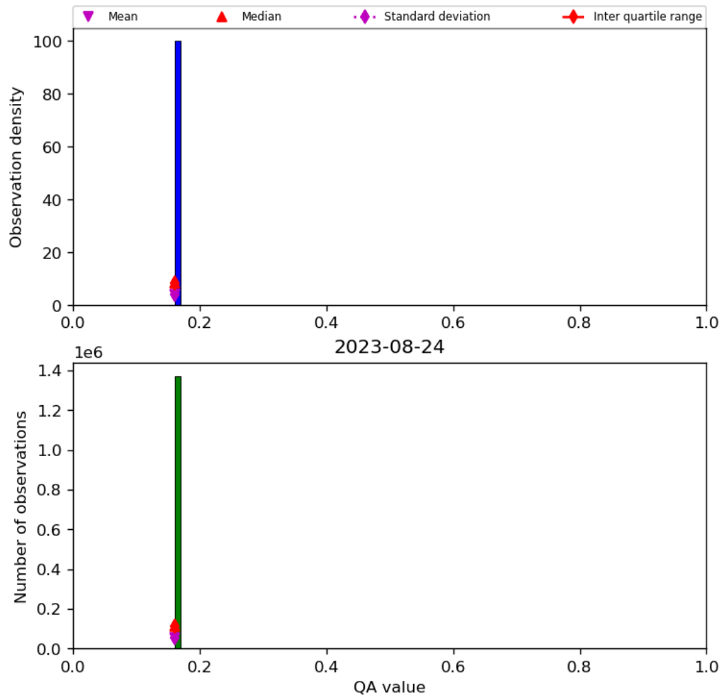
Figure 22: Histogram of “QA value” for 2023-08-23 to 2023-08-25
