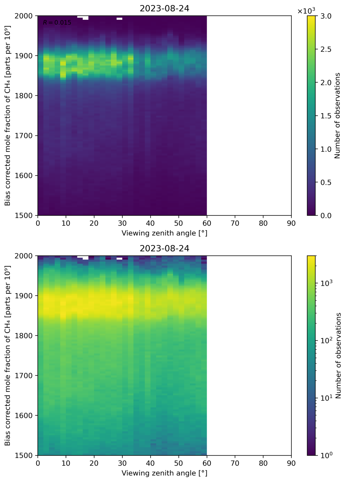
Figure 111: Scatter density plot of “Viewing zenith angle” against “Bias corrected mole fraction of CH 4 ” for 2023-08-23 to 2023-08-25.
