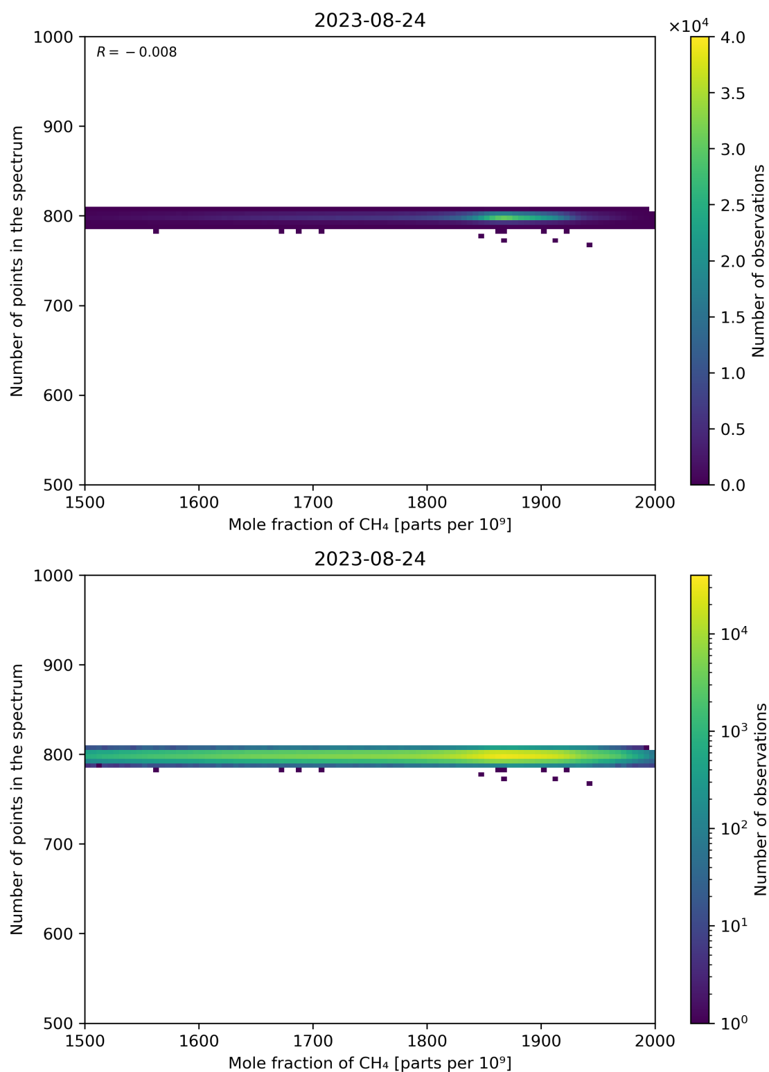
Figure 77: Scatter density plot of “Mole fraction of CH 4 ” against “Number of points in the spectrum” for 2023-08-23 to 2023-08-25.
