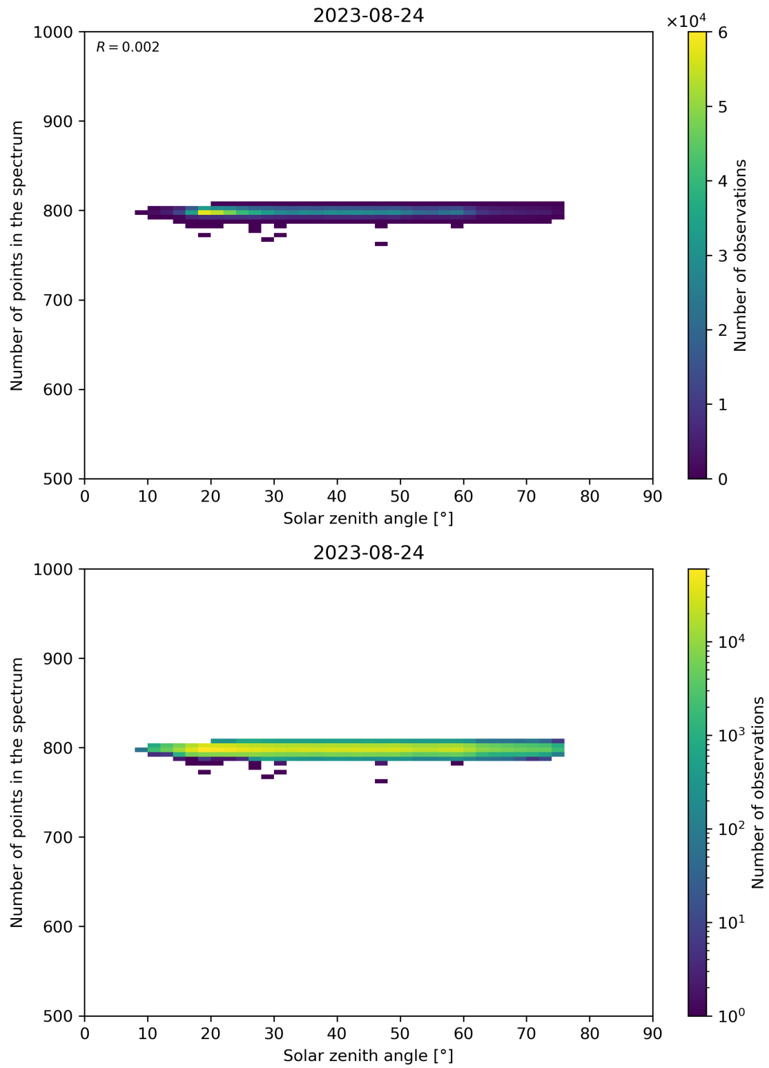
Figure 103: Scatter density plot of “Solar zenith angle” against “Number of points in the spectrum” for 2023-08-23 to 2023-08-25.
