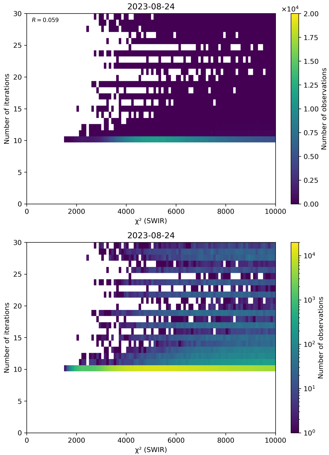
Figure 50: Scatter density plot of “ \chi^2 (SWIR)” against “Number of iterations” for 2023-08-23 to 2023-08-25.
