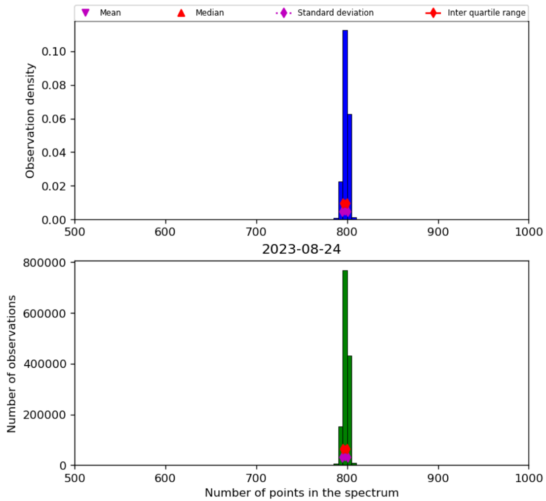
Figure 26: Histogram of “Number of points in the spectrum” for 2023-08-23 to 2023-08-25
