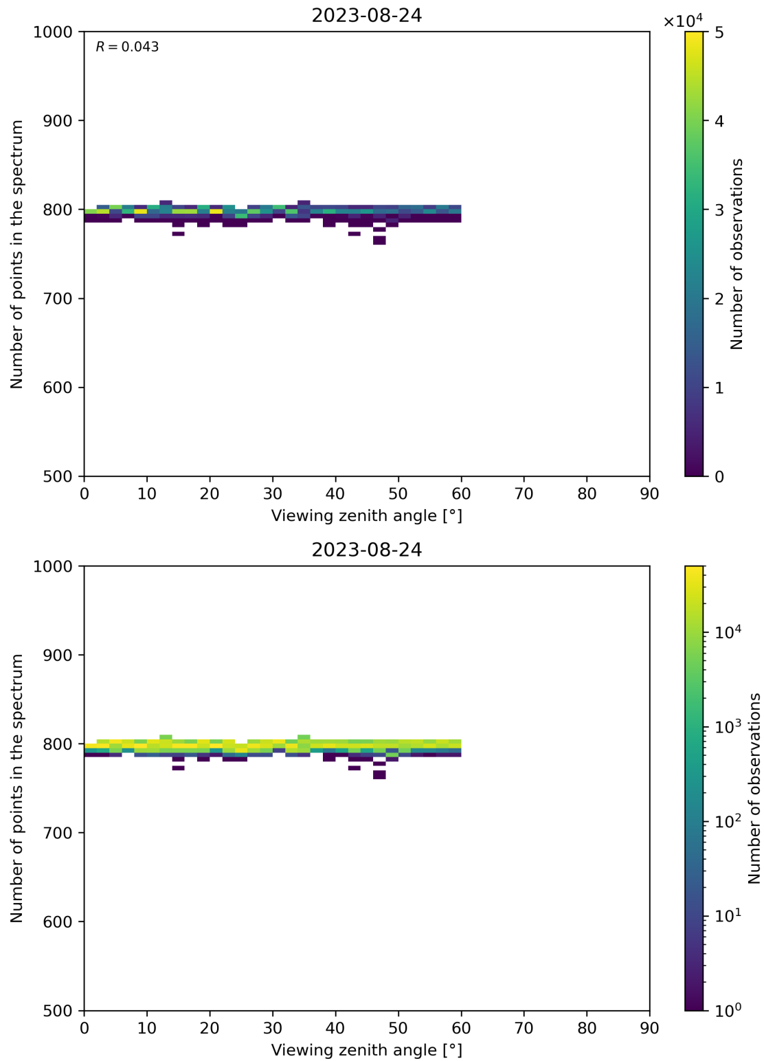
Figure 114: Scatter density plot of “Viewing zenith angle” against “Number of points in the spectrum” for 2023-08-23 to 2023-08-25.
