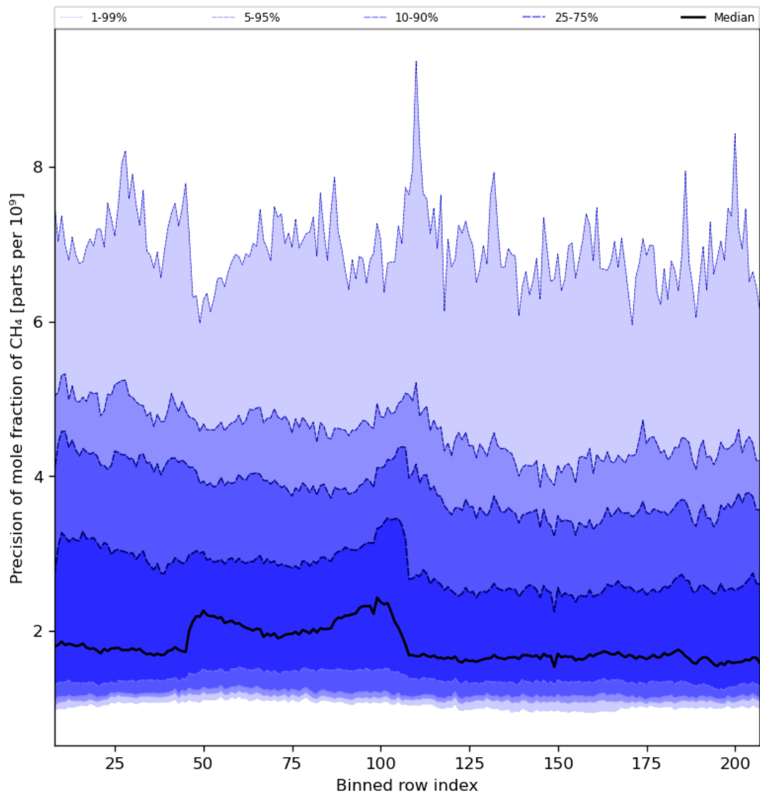
Figure 35: Along track statistics of “Precision of mole fraction of CH 4 ” for 2023-08-23 to 2023-08-25
