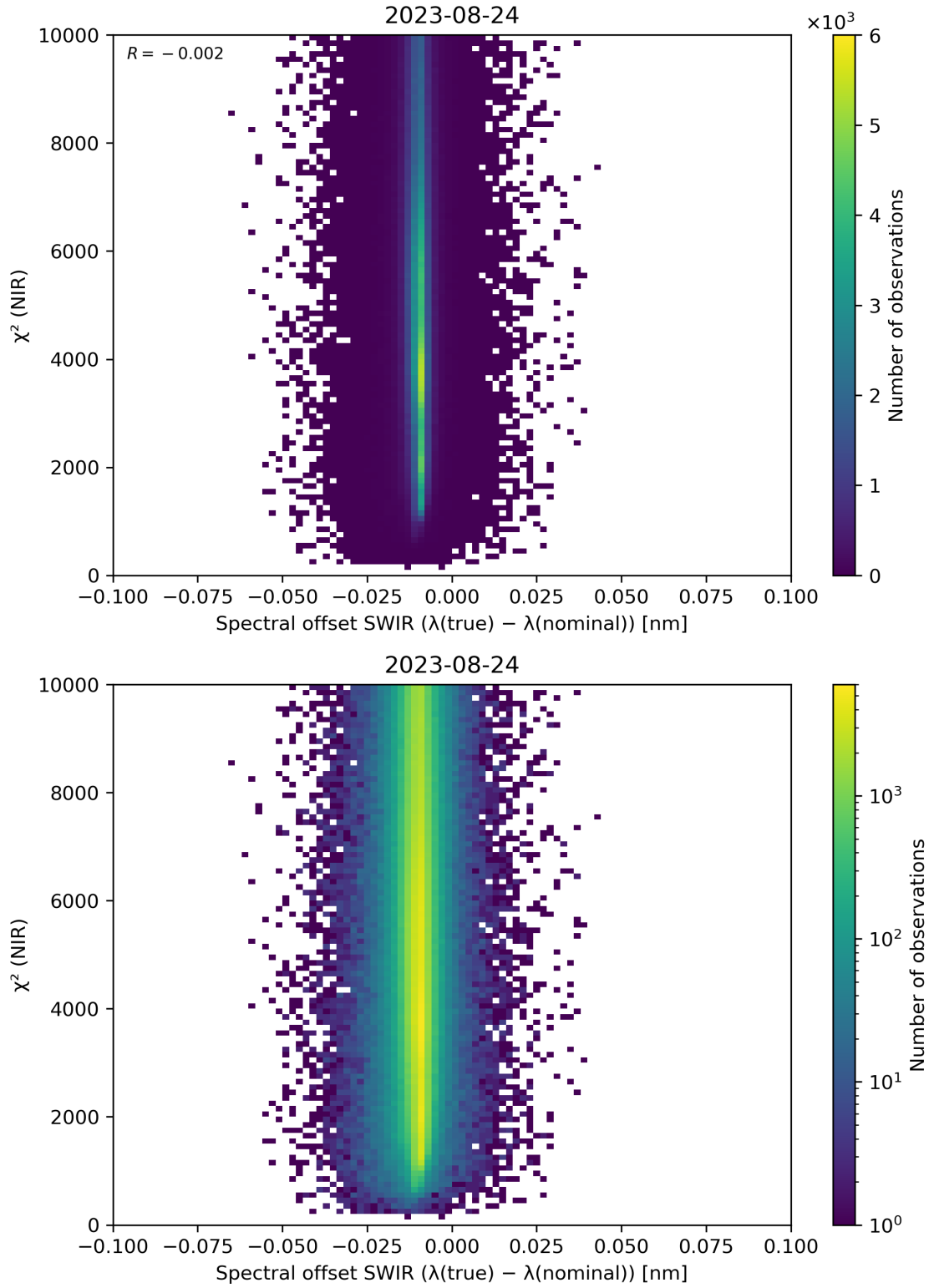
Figure 117: Scatter density plot of “Spectral offset SWIR ( \lambda(\text{true}) - \lambda(\text{nominal}) )” against “ \chi^2 (NIR)” for 2023-08-23 to 2023-08-25.
