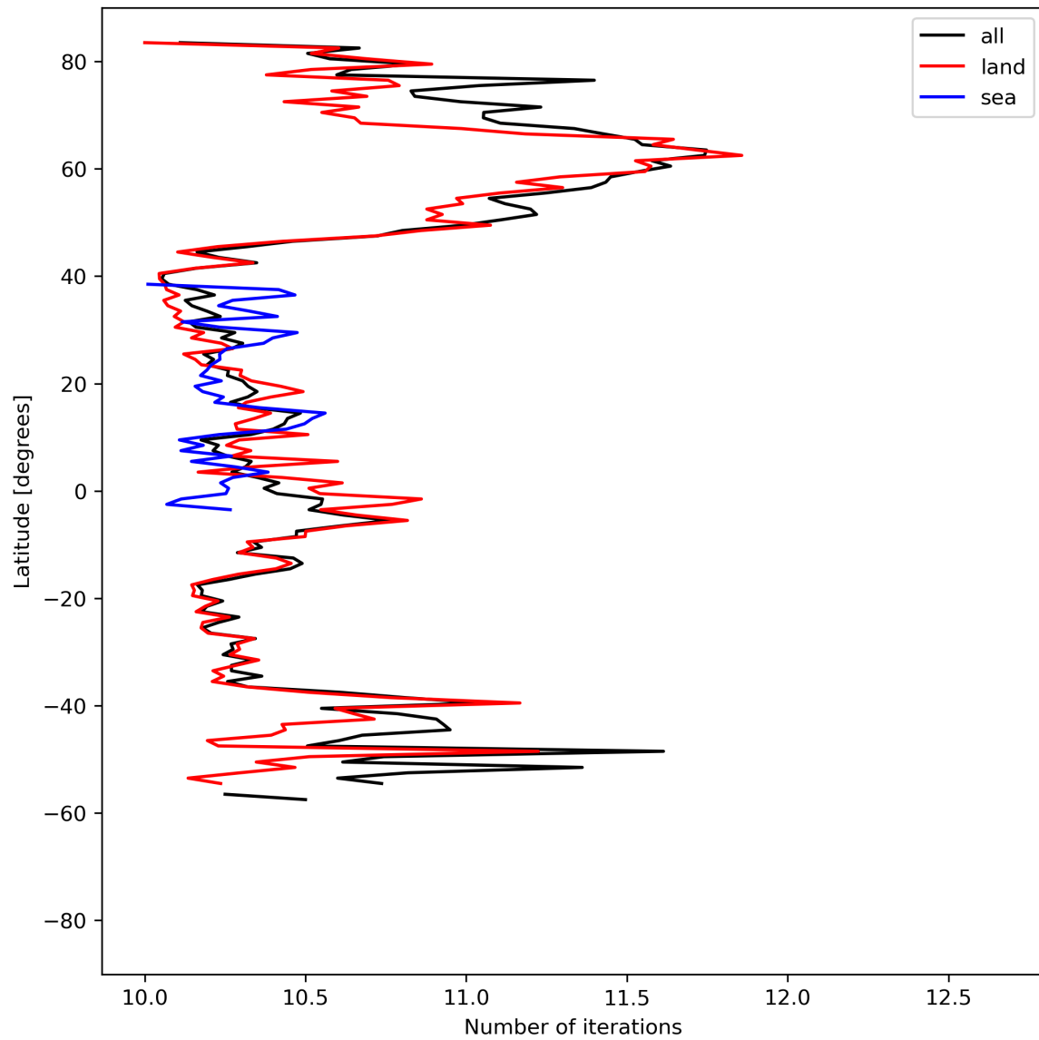
Figure 20: Zonal average of “Number of iterations” for 2023-08-23 to 2023-08-25.
