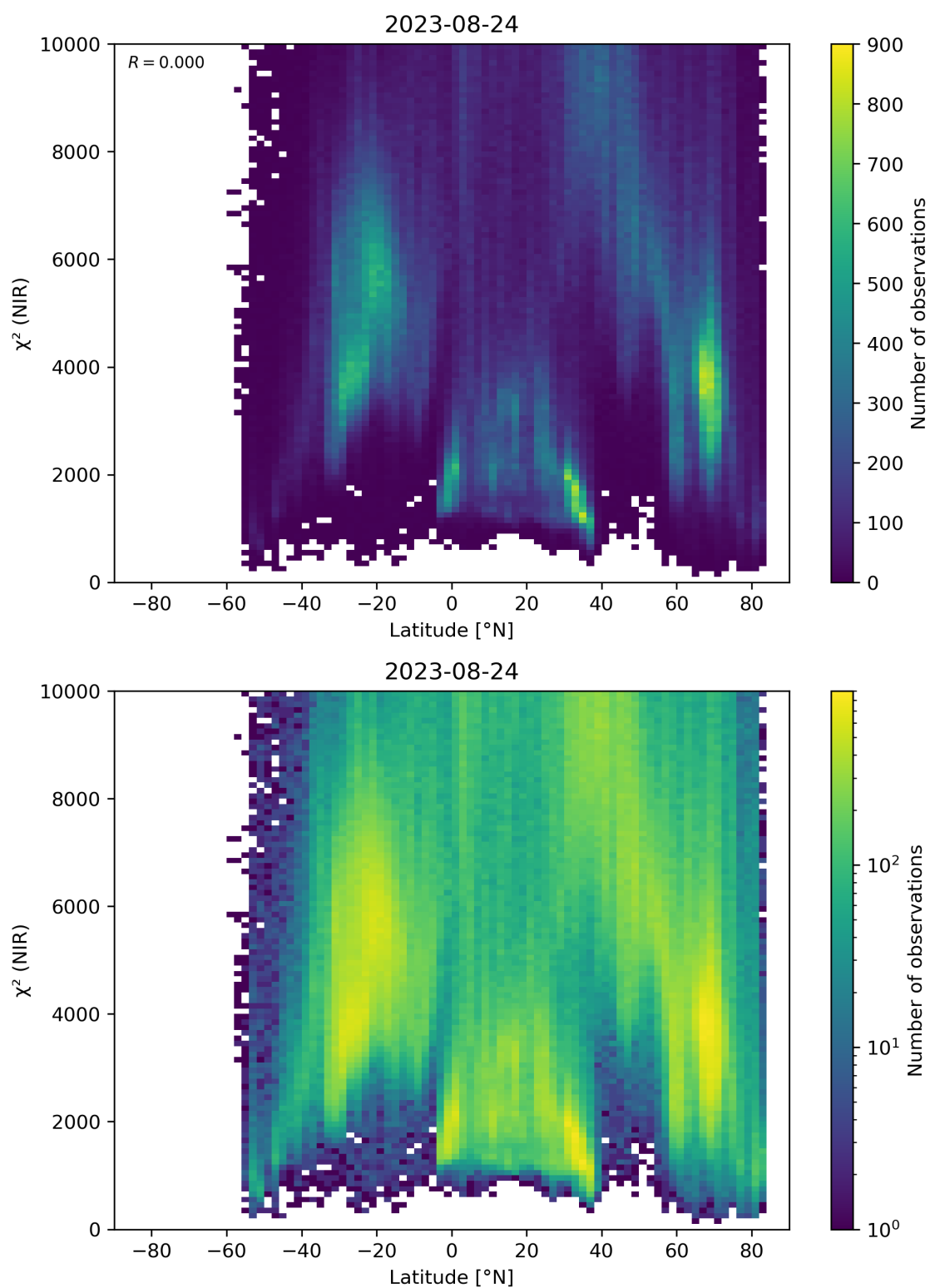
Figure 53: Scatter density plot of “Latitude” against “ \chi^2 (NIR)” for 2023-08-23 to 2023-08-25.
