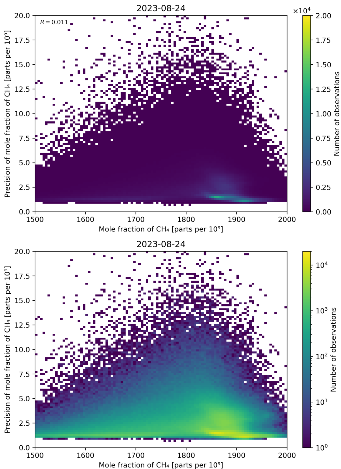
Figure 75: Scatter density plot of “Mole fraction of CH 4 ” against “Precision of mole fraction of CH 4 ” for 2023-08-23 to 2023-08-25.
