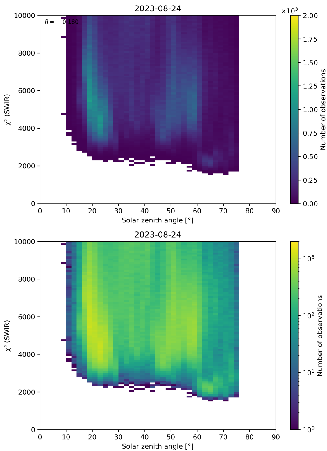
Figure 95: Scatter density plot of “Solar zenith angle” against “ \chi^2 (SWIR)” for 2023-08-23 to 2023-08-25.
