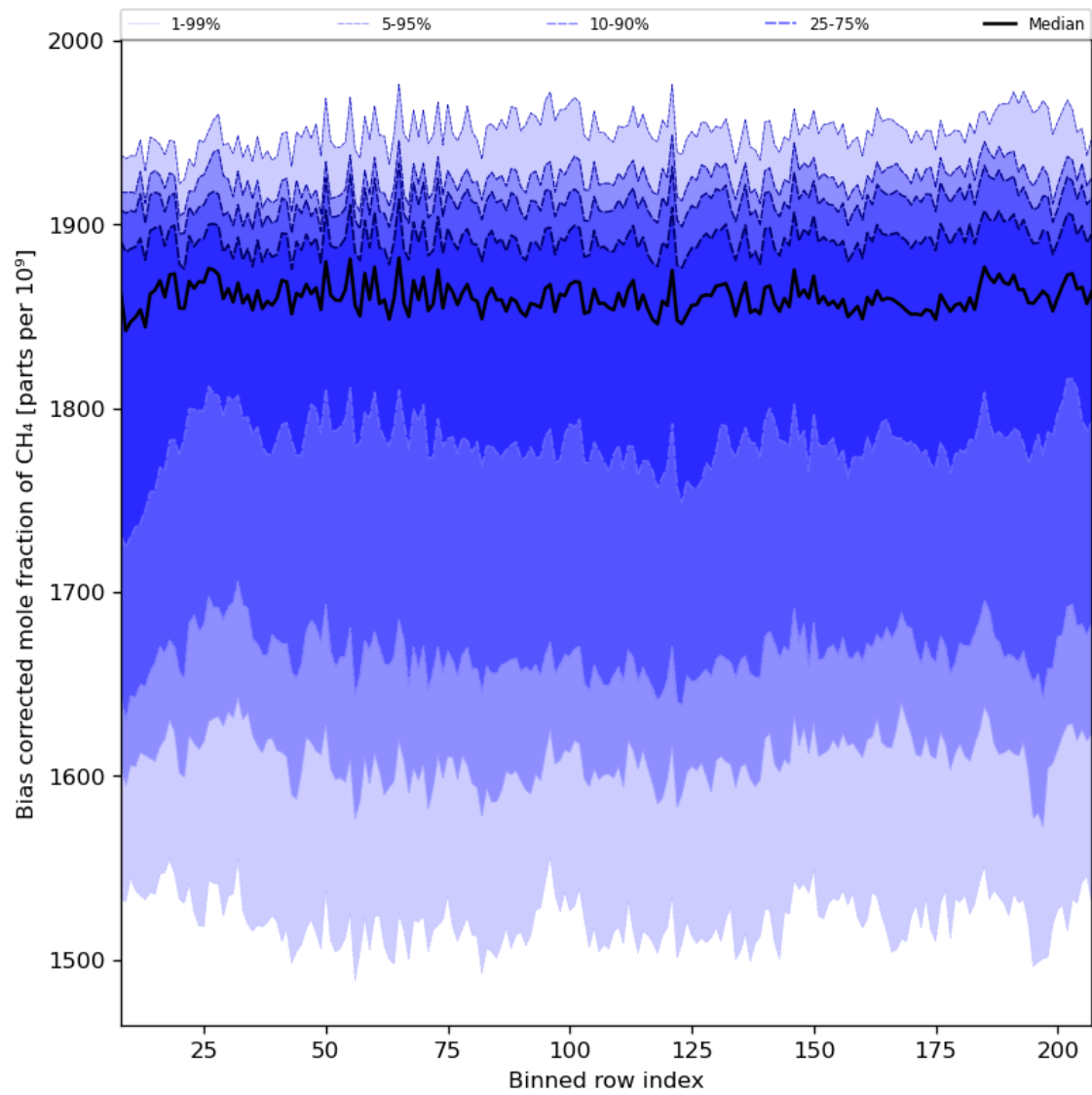
Figure 36: Along track statistics of “Bias corrected mole fraction of CH 4 ” for 2023-08-23 to 2023-08-25
