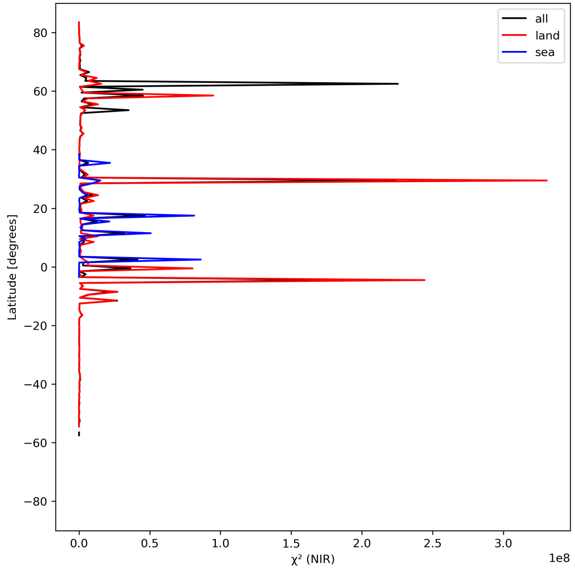
Figure 18: Zonal average of “ \chi^2 (NIR)” for 2023-08-23 to 2023-08-25.
