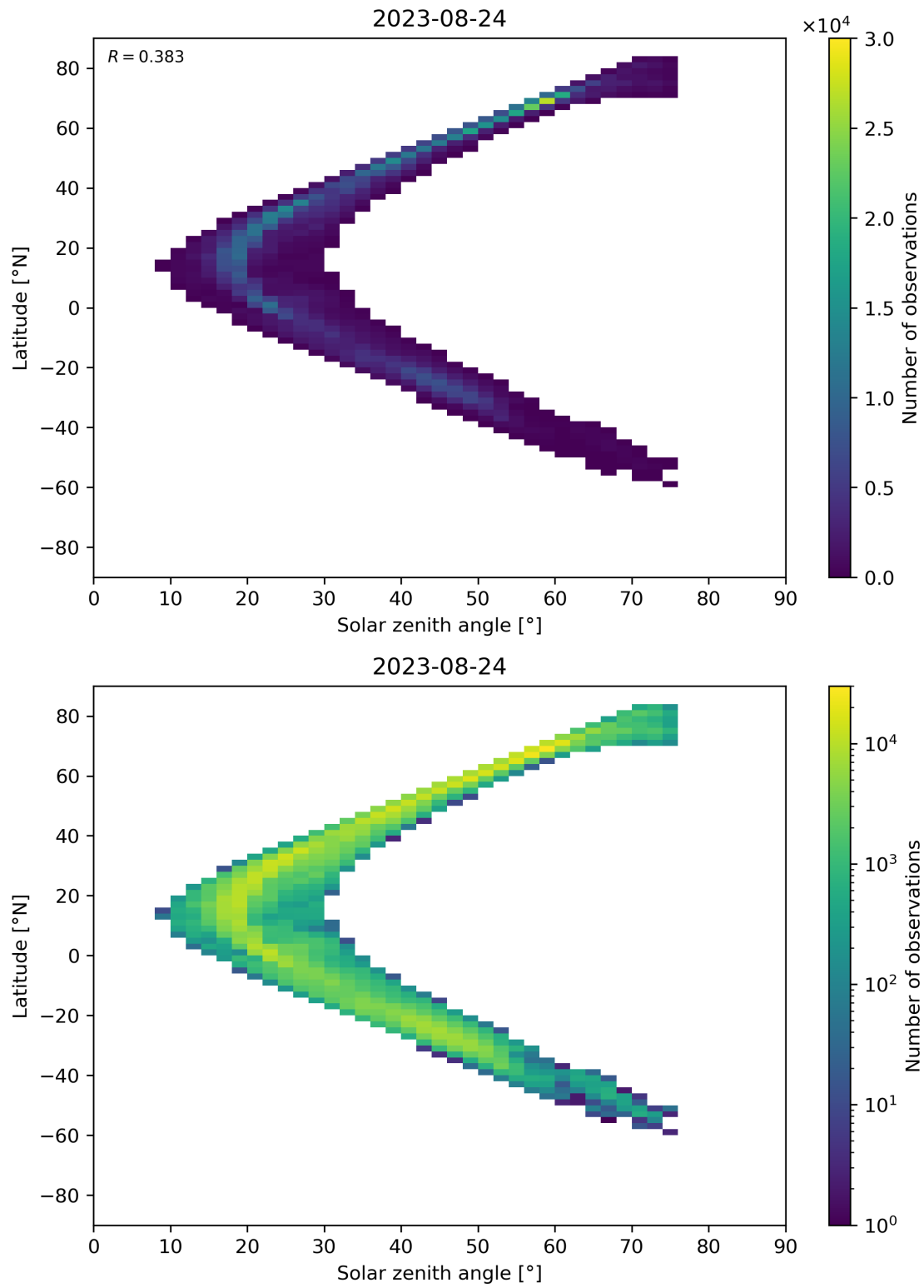
Figure 98: Scatter density plot of “Solar zenith angle” against “Latitude” for 2023-08-23 to 2023-08-25.
