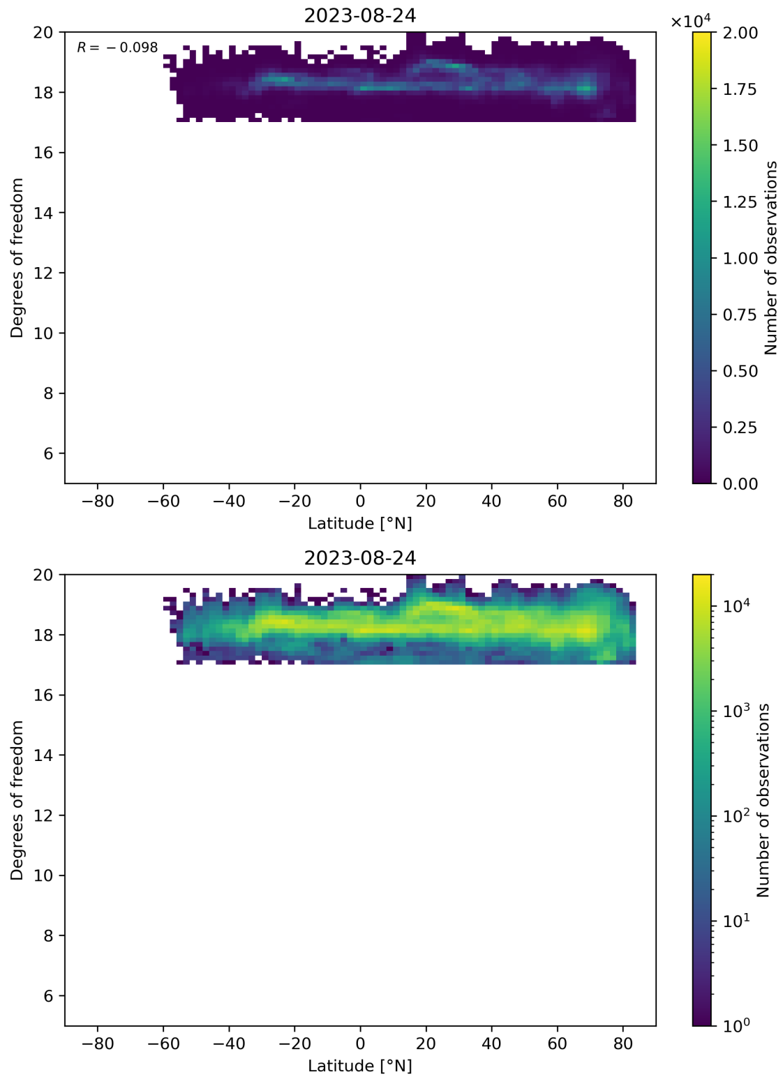
Figure 55: Scatter density plot of “Latitude” against “Degrees of freedom” for 2023-08-23 to 2023-08-25.
