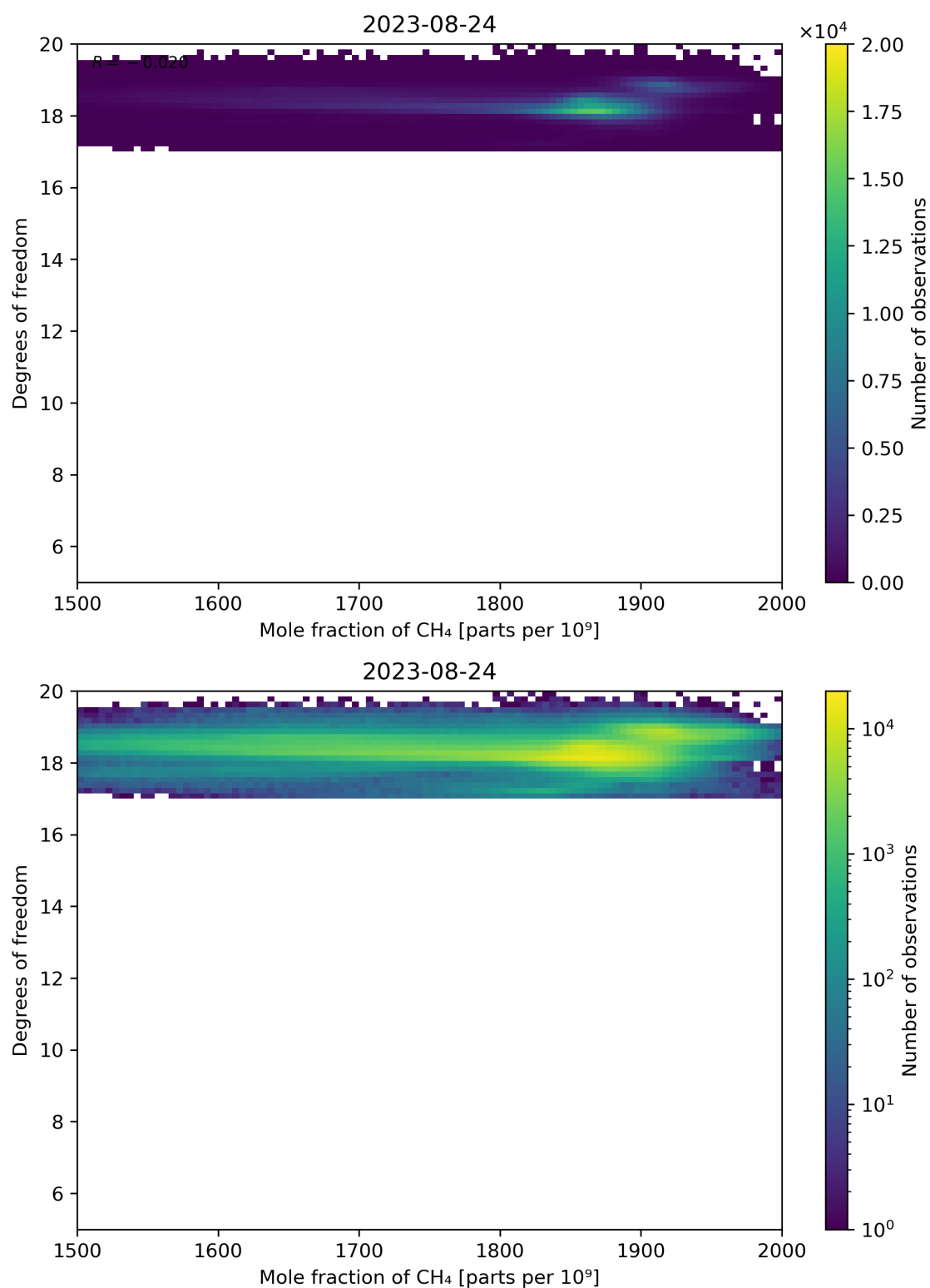
Figure 72: Scatter density plot of “Mole fraction of CH 4 ” against “Degrees of freedom” for 2023-08-23 to 2023-08-25.
