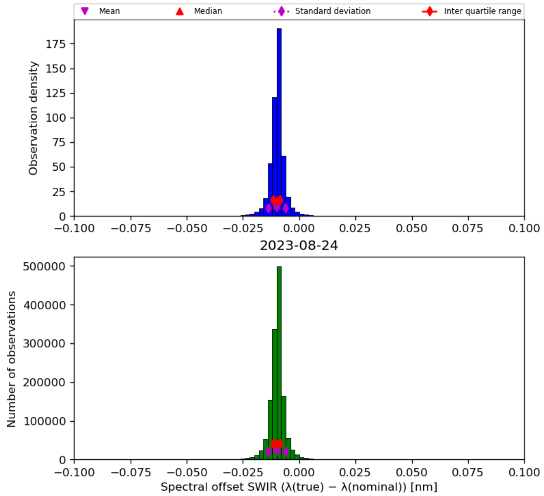
Figure 27: Histogram of “Spectral offset SWIR ( \lambda(\text{true}) - \lambda(\text{nominal}) )” for 2023-08-23 to 2023-08-25
