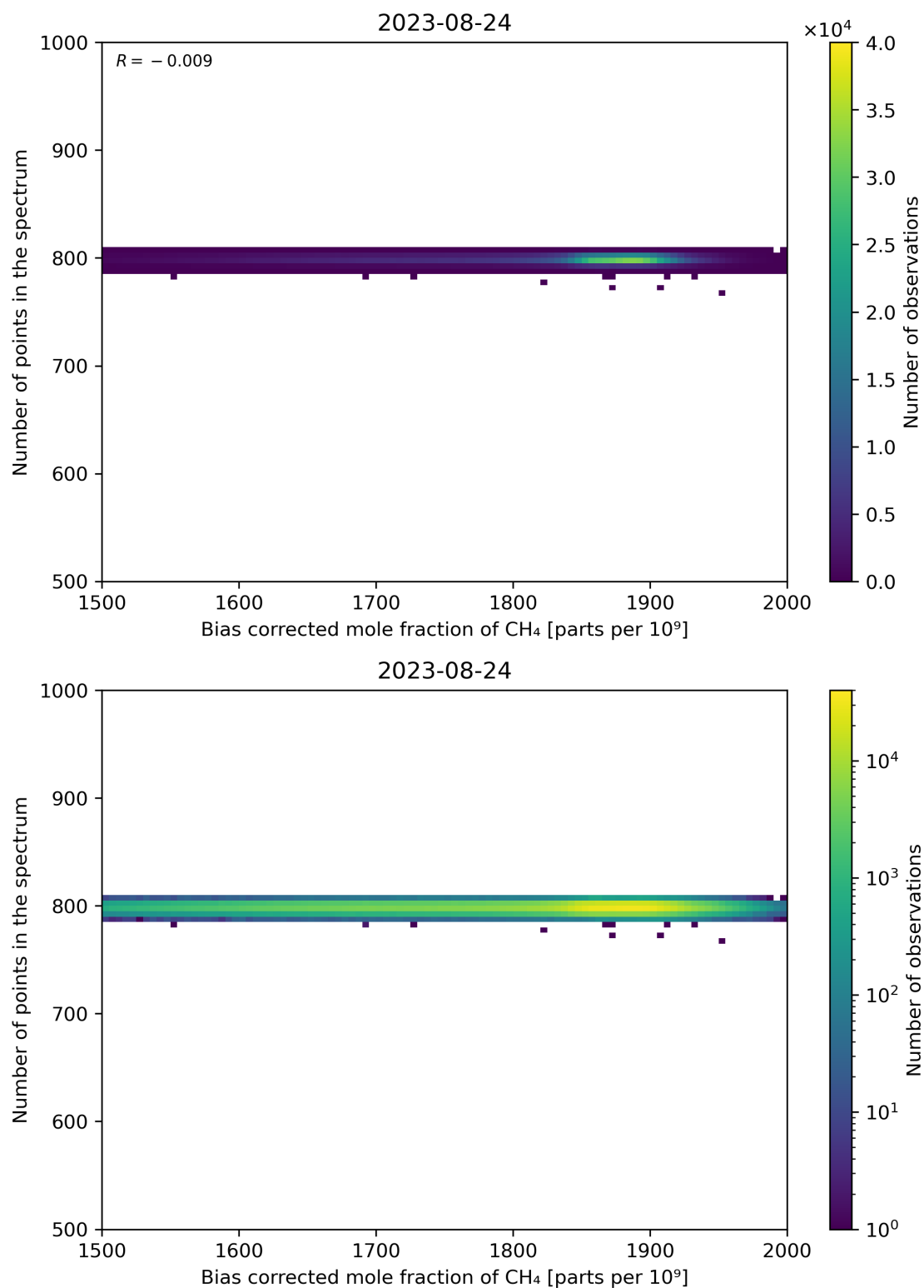
Figure 68: Scatter density plot of “Bias corrected mole fraction of CH 4 ” against “Number of points in the spectrum” for 2023-08-23 to 2023-08-25.
