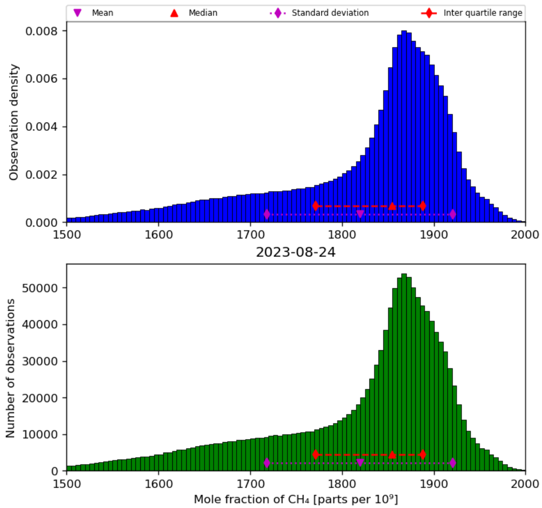
Figure 23: Histogram of “Mole fraction of CH 4 ” for 2023-08-23 to 2023-08-25
