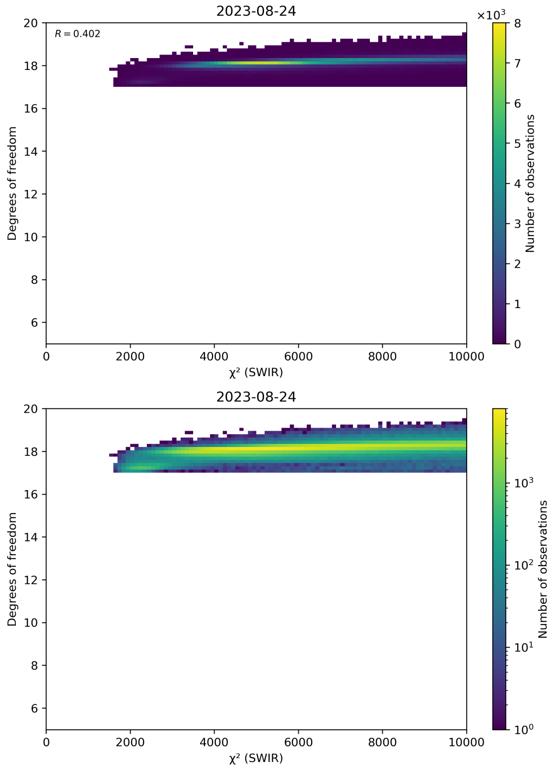
Figure 48: Scatter density plot of “ \chi^2 (SWIR)” against “Degrees of freedom” for 2023-08-23 to 2023-08-25.
