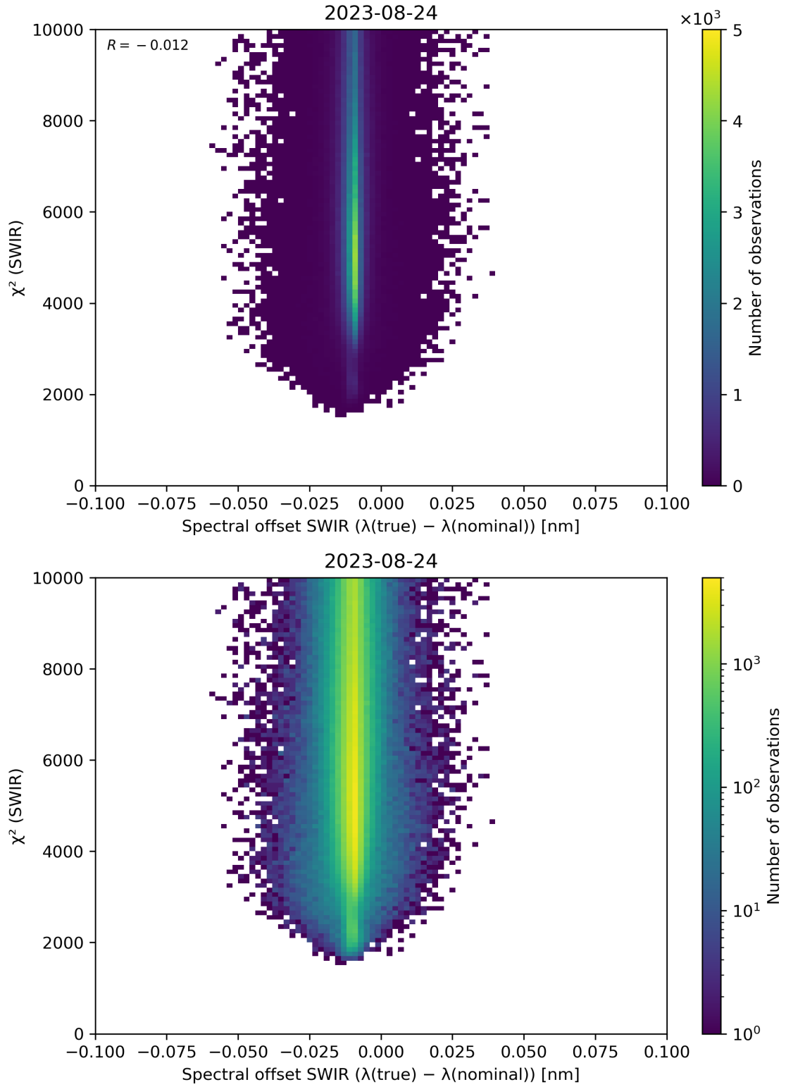
Figure 118: Scatter density plot of “Spectral offset SWIR ( \lambda(\text{true}) - \lambda(\text{nominal}) )” against “ \chi^2 (SWIR)” for 2023-08-23 to 2023-08-25.
