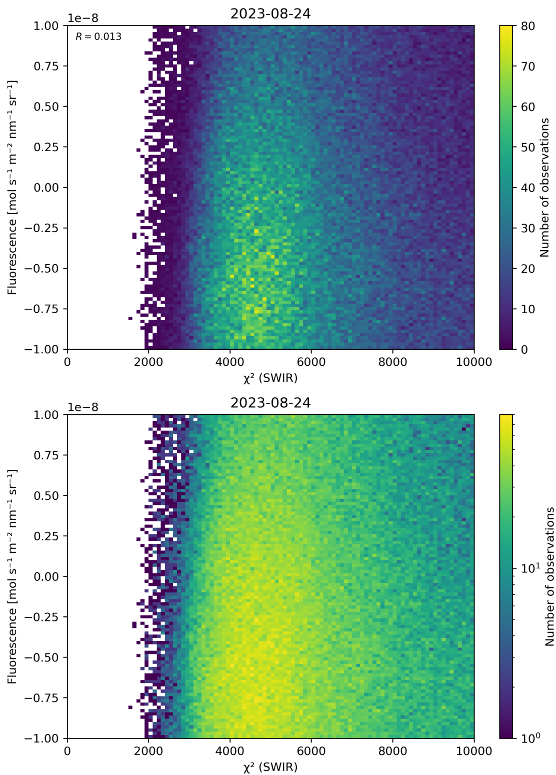
Figure 49: Scatter density plot of “ \chi^2 (SWIR)” against “Fluorescence” for 2023-08-23 to 2023-08-25.
