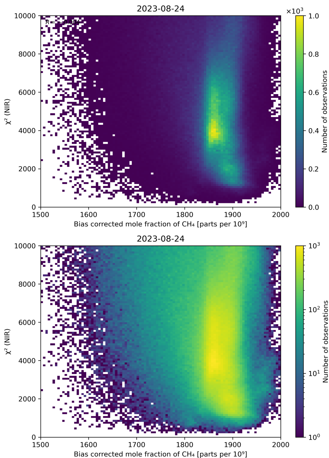
Figure 63: Scatter density plot of “Bias corrected mole fraction of \text{CH}_4 ” against “ \chi^2 (NIR)” for 2023-08-23 to 2023-08-25.
