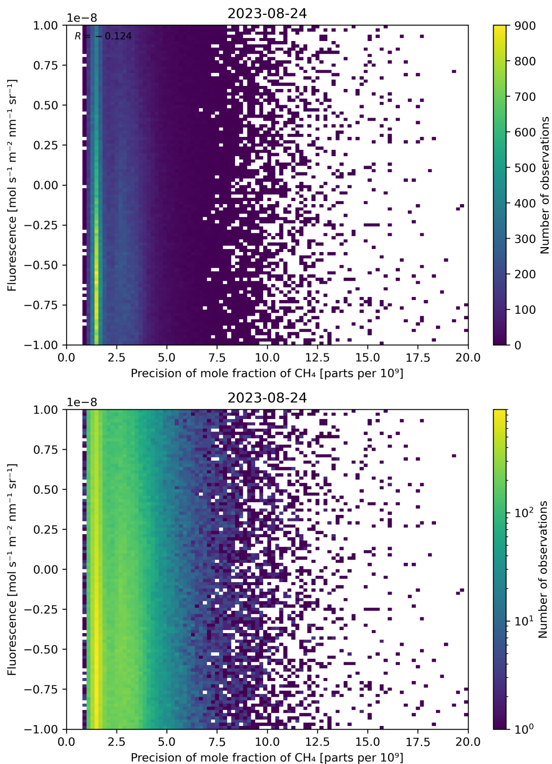
Figure 81: Scatter density plot of “Precision of mole fraction of \text{CH}_4 ” against “Fluorescence” for 2023-08-23 to 2023-08-25.
