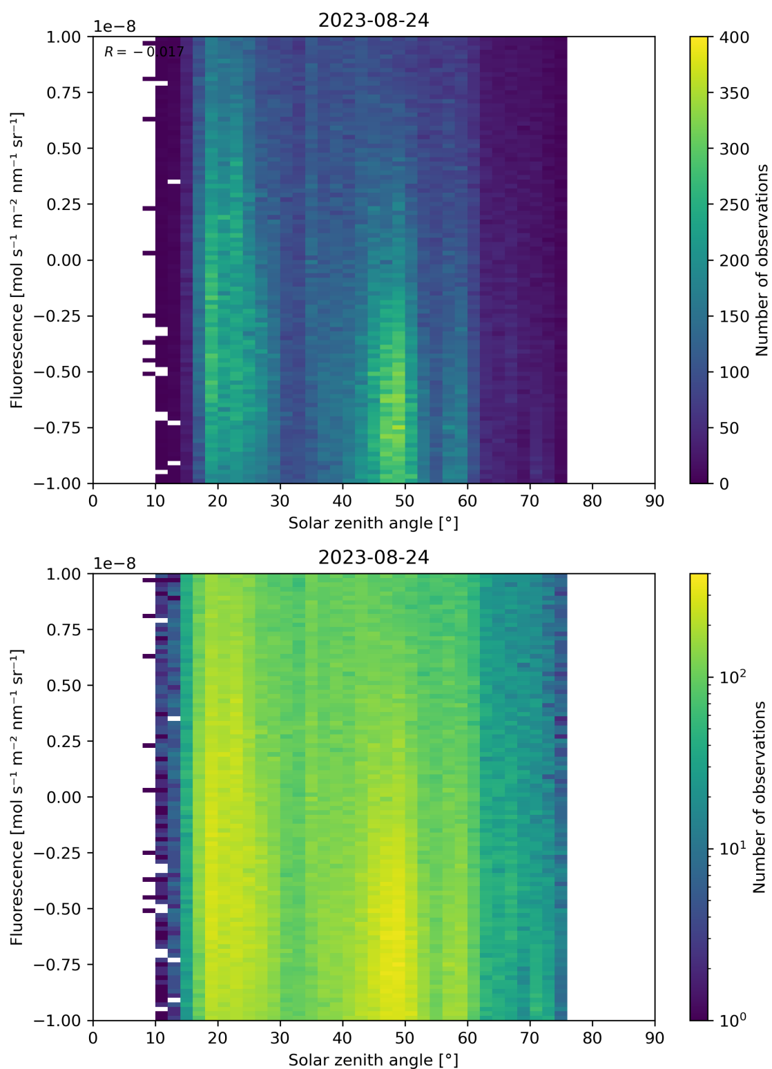
Figure 97: Scatter density plot of “Solar zenith angle” against “Fluorescence” for 2023-08-23 to 2023-08-25.
