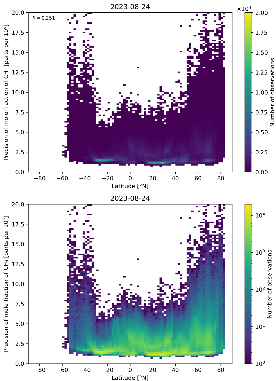
Figure 59: Scatter density plot of “Latitude” against “Precision of mole fraction of CH 4 ” for 2023-08-23 to 2023-08-25.
