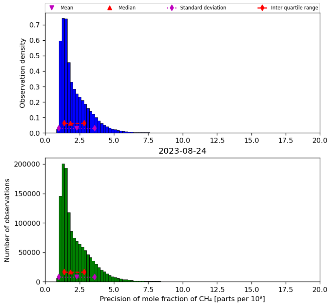
Figure 24: Histogram of “Precision of mole fraction of CH 4 ” for 2023-08-23 to 2023-08-25
