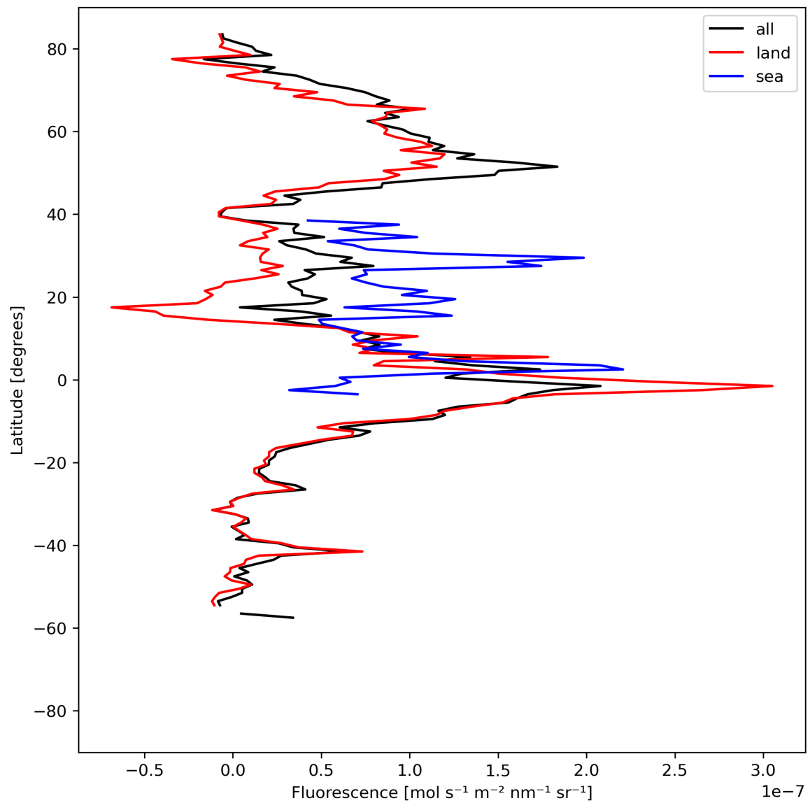
Figure 21: Zonal average of “Fluorescence” for 2023-08-23 to 2023-08-25.
