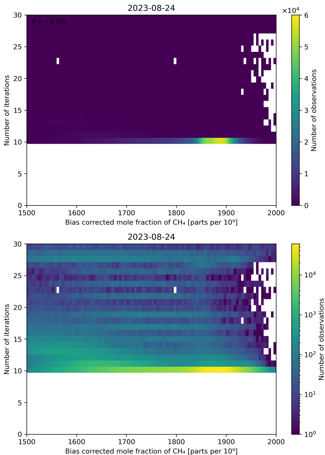
Figure 67: Scatter density plot of “Bias corrected mole fraction of CH 4 ” against “Number of iterations” for 2023-08-23 to 2023-08-25.
