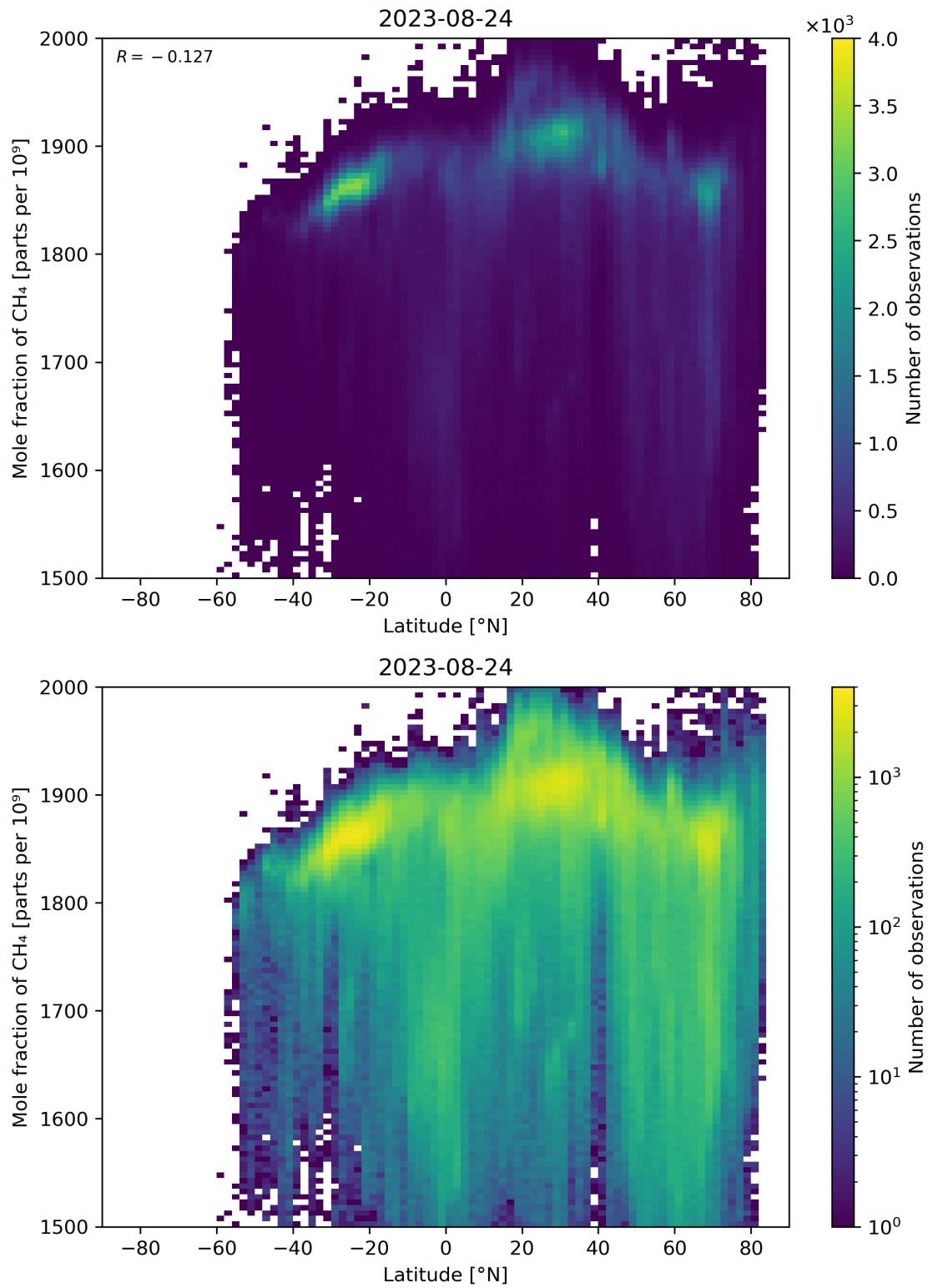
Figure 57: Scatter density plot of “Latitude” against “Mole fraction of CH 4 ” for 2023-08-23 to 2023-08-25.
