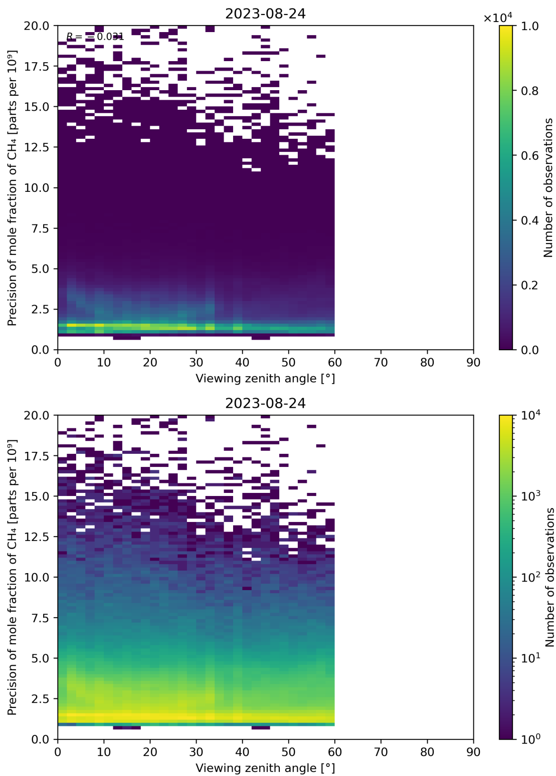
Figure 112: Scatter density plot of “Viewing zenith angle” against “Precision of mole fraction of CH 4 ” for 2023-08-23 to 2023-08-25.
