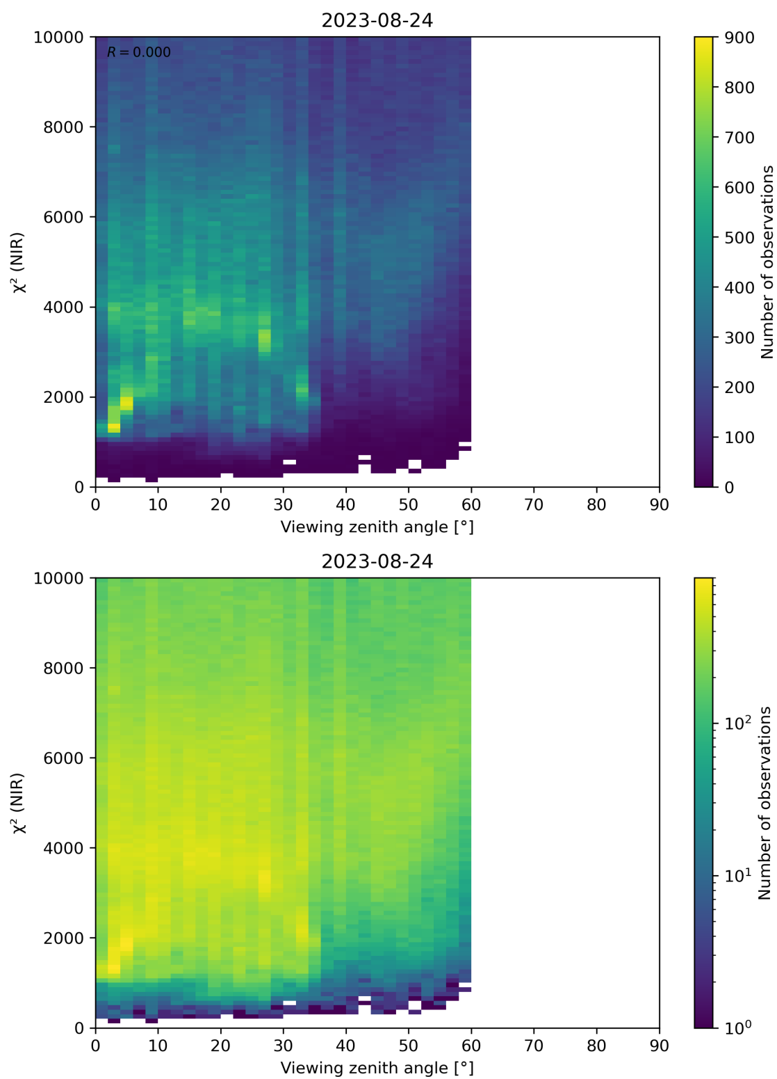
Figure 105: Scatter density plot of “Viewing zenith angle” against “ \chi^2 (NIR)” for 2023-08-23 to 2023-08-25.
