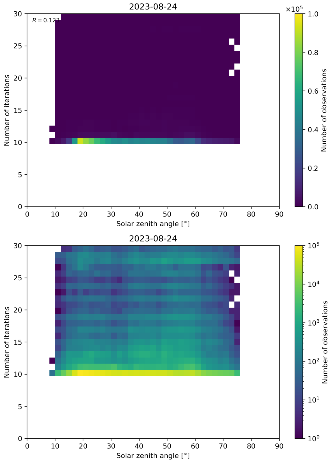
Figure 102: Scatter density plot of “Solar zenith angle” against “Number of iterations” for 2023-08-23 to 2023-08-25.
