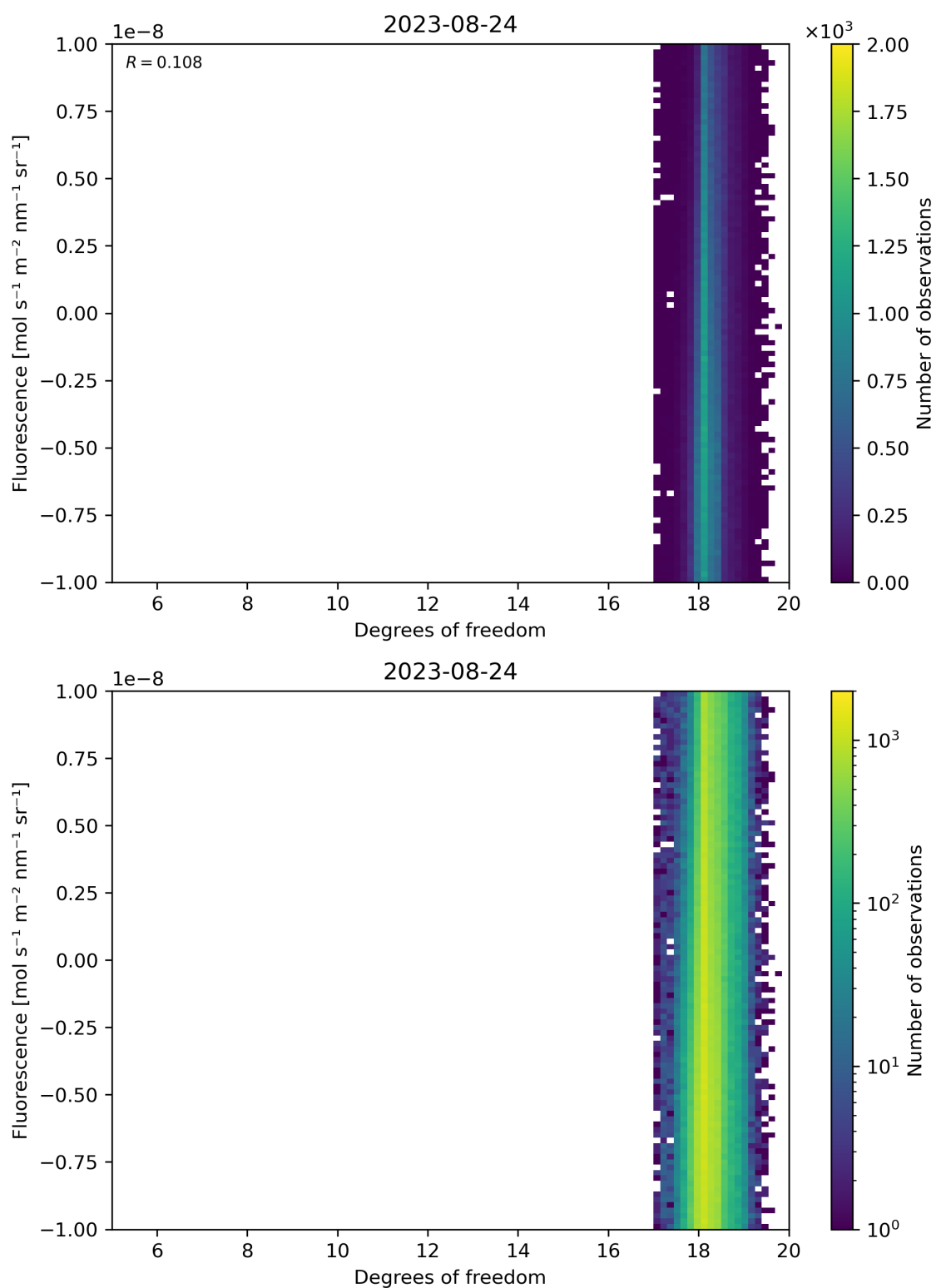
Figure 51: Scatter density plot of “Degrees of freedom” against “Fluorescence” for 2023-08-23 to 2023-08-25.
