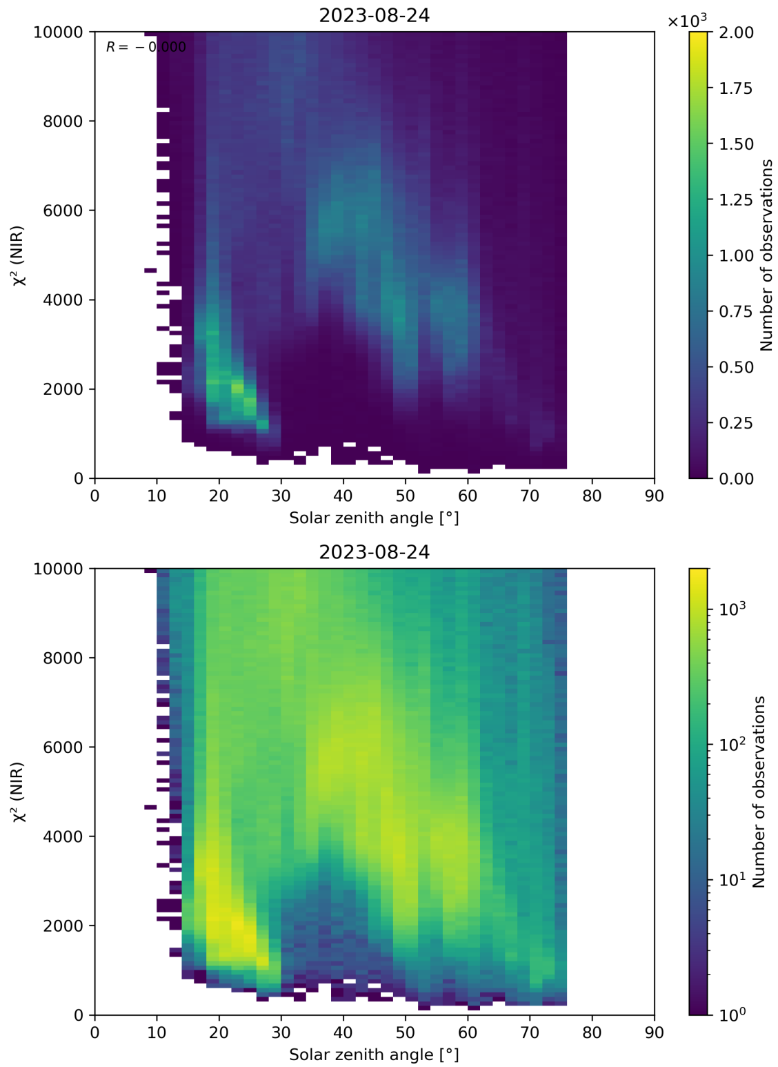
Figure 94: Scatter density plot of “Solar zenith angle” against “ \chi^2 (NIR)” for 2023-08-23 to 2023-08-25.
