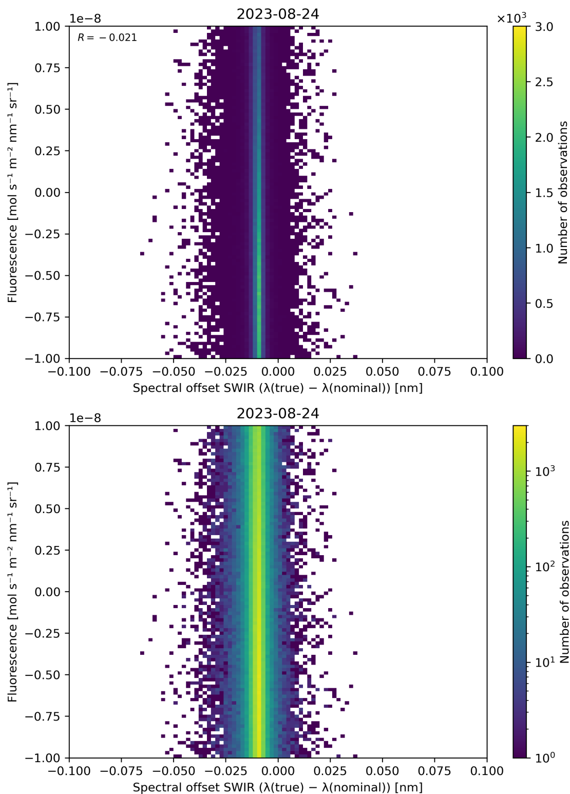
Figure 120: Scatter density plot of “Spectral offset SWIR ( \lambda(\text{true}) - \lambda(\text{nominal}) )” against “Fluorescence” for 2023-08-23 to 2023-08-25.
