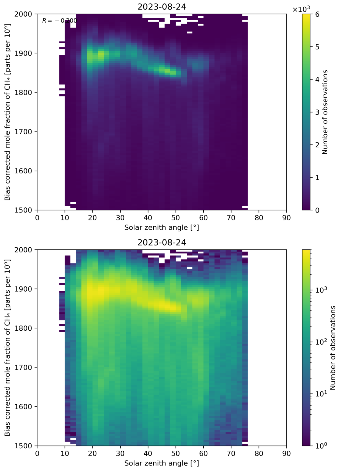
Figure 100: Scatter density plot of “Solar zenith angle” against “Bias corrected mole fraction of CH 4 ” for 2023-08-23 to 2023-08-25.
