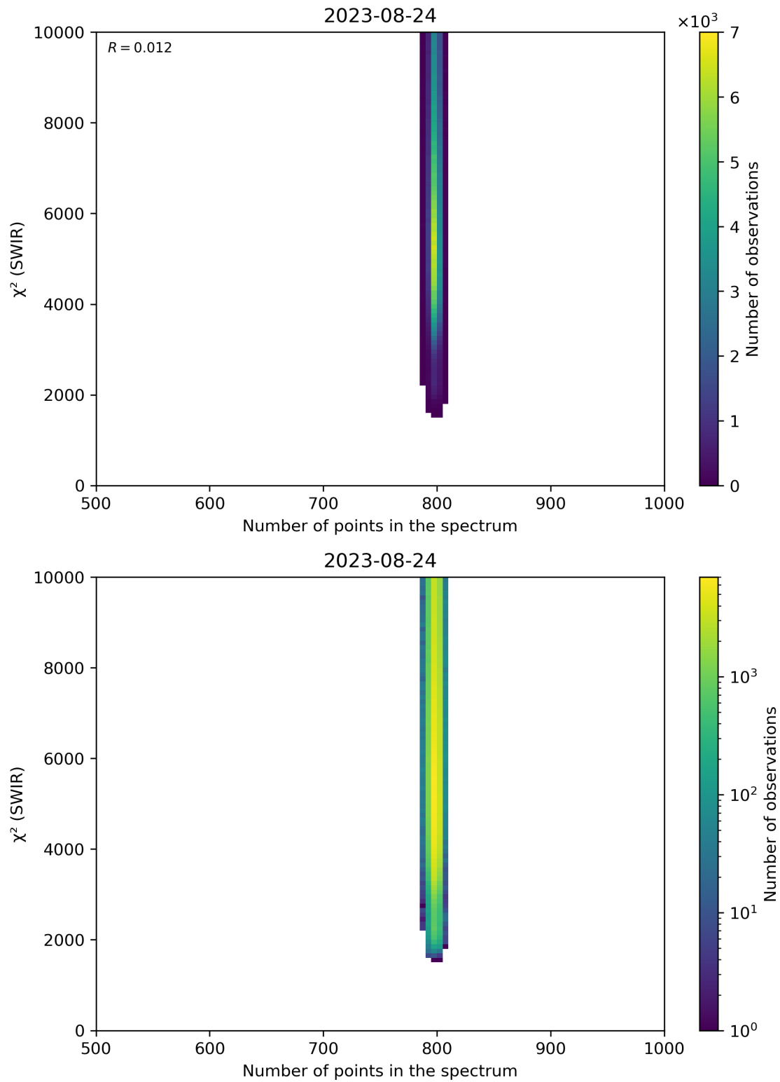
Figure 89: Scatter density plot of “Number of points in the spectrum” against “ \chi^2 (SWIR)” for 2023-08-23 to 2023-08-25.
