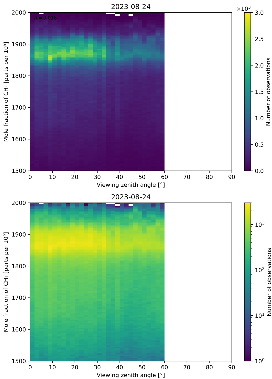
Figure 110: Scatter density plot of “Viewing zenith angle” against “Mole fraction of CH 4 ” for 2023-08-23 to 2023-08-25.
