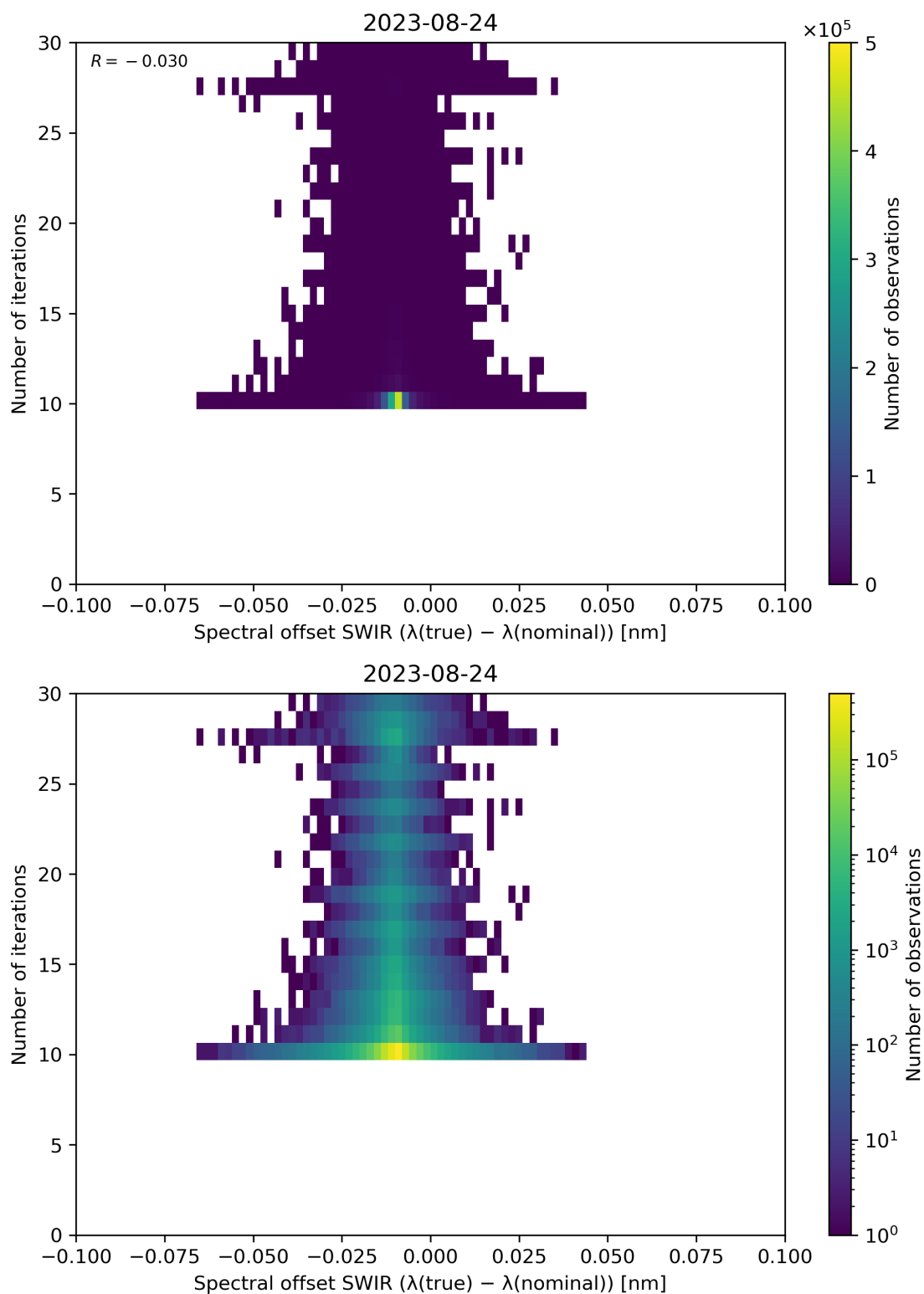
Figure 121: Scatter density plot of “Spectral offset SWIR ( \lambda(\text{true}) - \lambda(\text{nominal}) )” against “Number of iterations” for 2023-08-23 to 2023-08-25.
