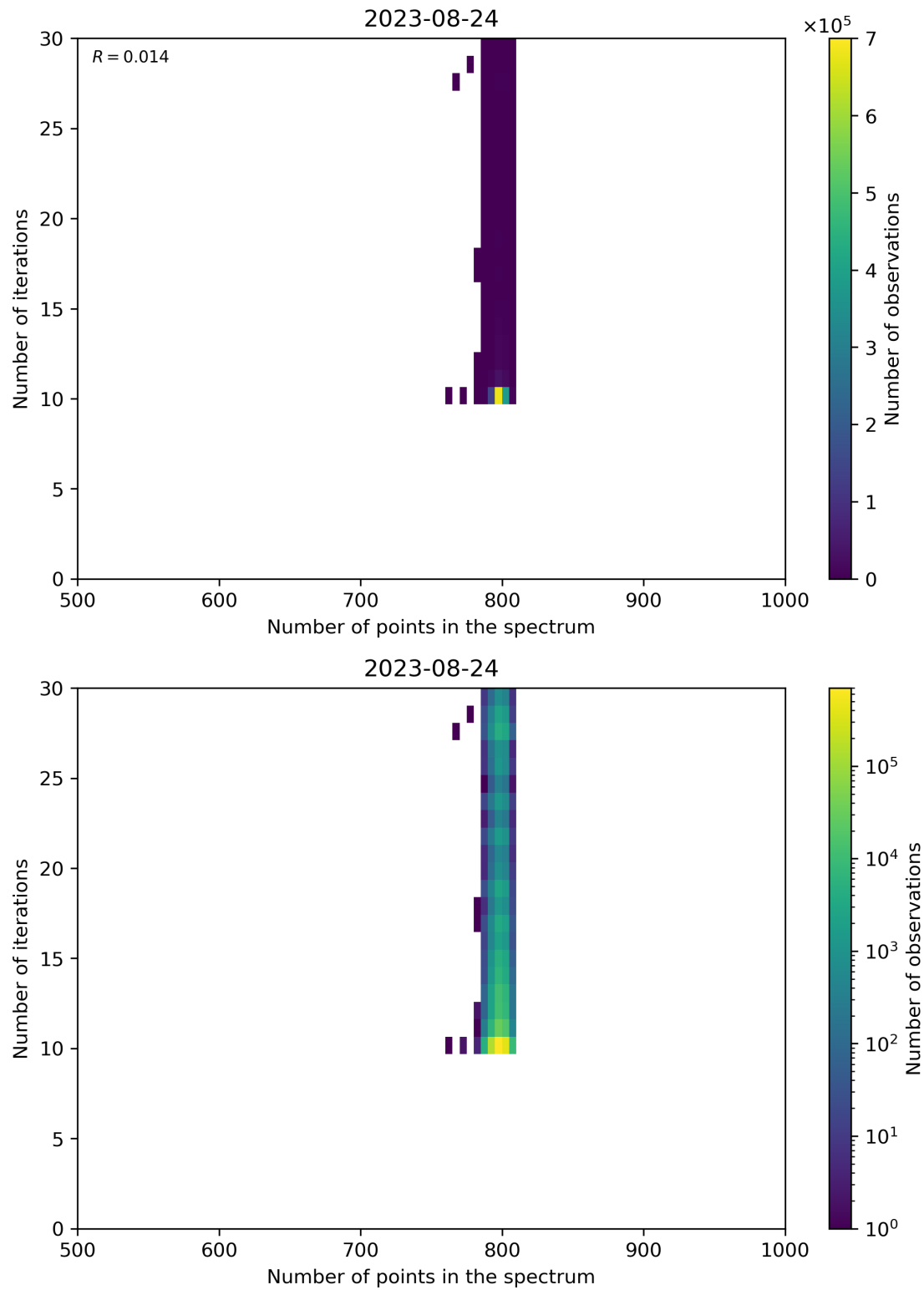
Figure 92: Scatter density plot of “Number of points in the spectrum” against “Number of iterations” for 2023-08-23 to 2023-08-25.
