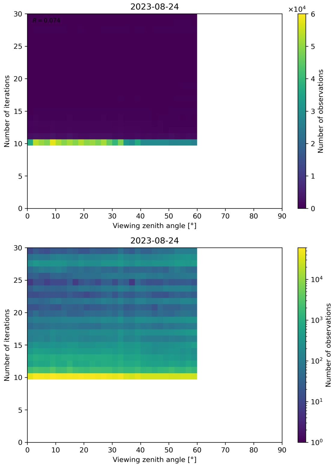
Figure 113: Scatter density plot of “Viewing zenith angle” against “Number of iterations” for 2023-08-23 to 2023-08-25.
