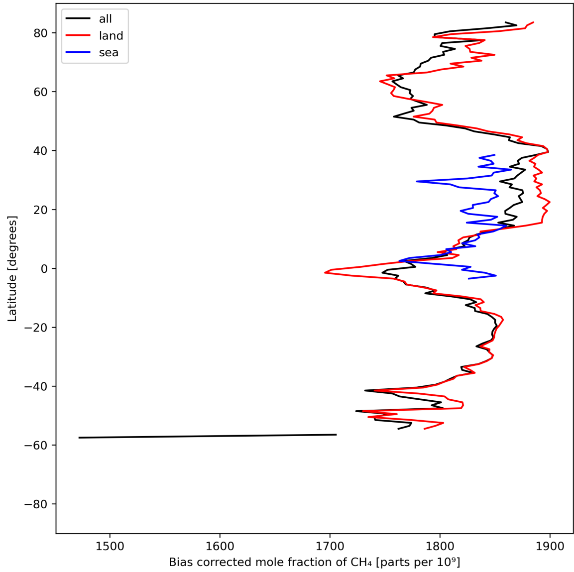
Figure 14: Zonal average of “Bias corrected mole fraction of CH 4 ” for 2023-08-23 to 2023-08-25.
