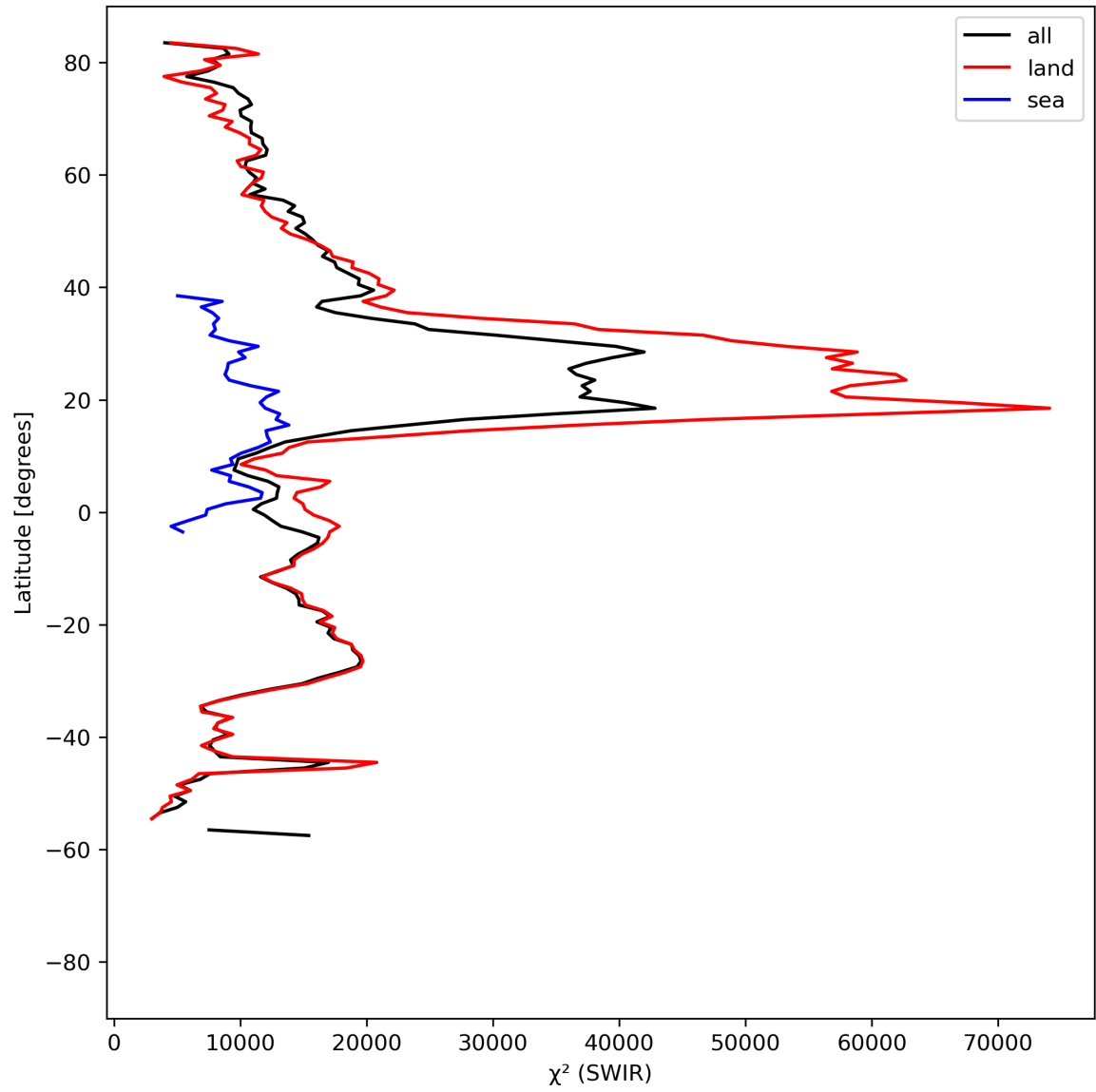
Figure 17: Zonal average of “ \chi^2 (SWIR)” for 2023-08-23 to 2023-08-25.
