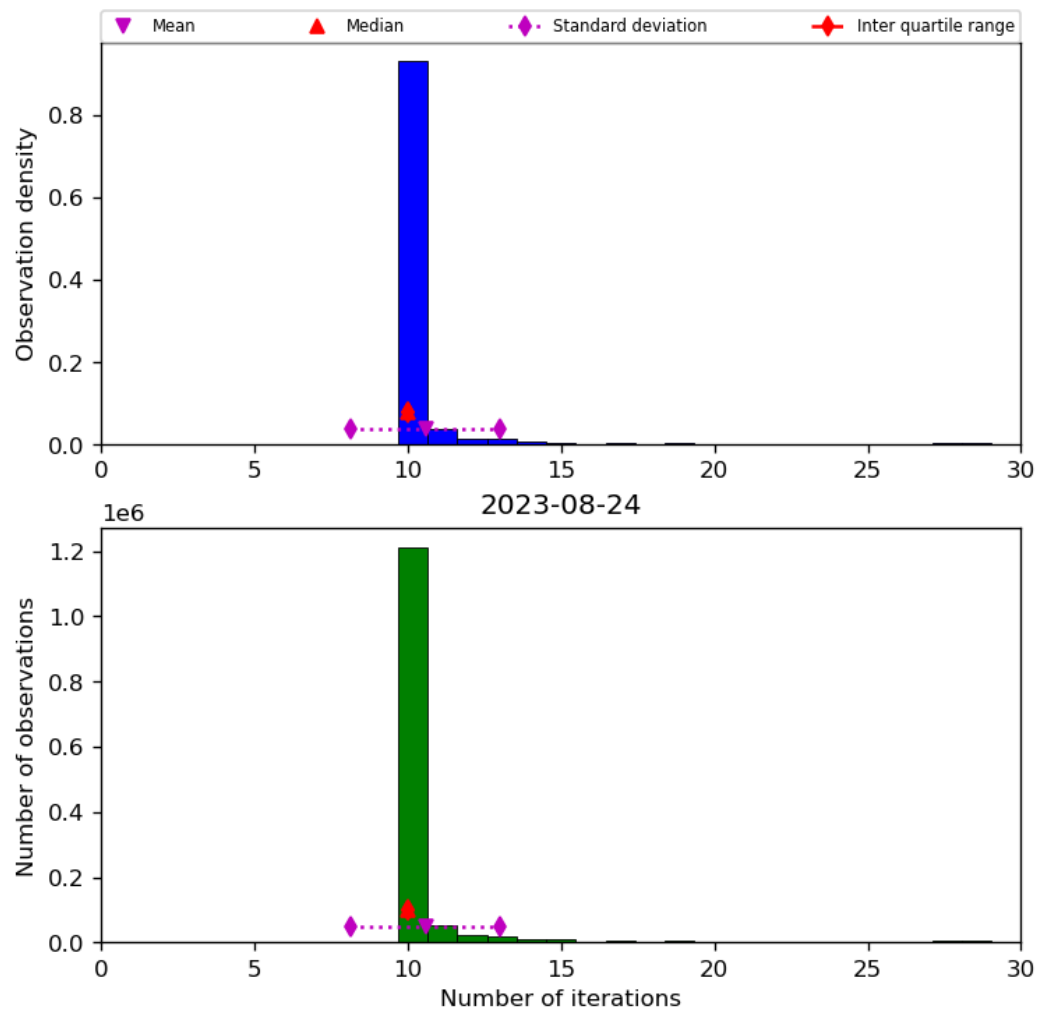
Figure 31: Histogram of “Number of iterations” for 2023-08-23 to 2023-08-25
