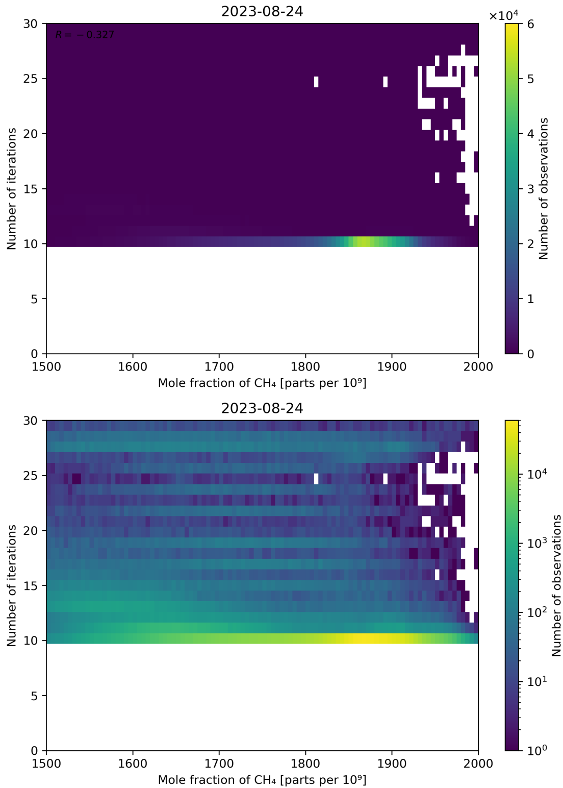
Figure 76: Scatter density plot of “Mole fraction of CH 4 ” against “Number of iterations” for 2023-08-23 to 2023-08-25.
