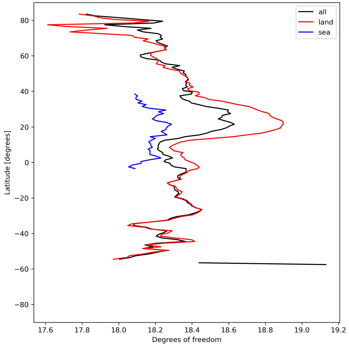
Figure 19: Zonal average of “Degrees of freedom” for 2023-08-23 to 2023-08-25.
