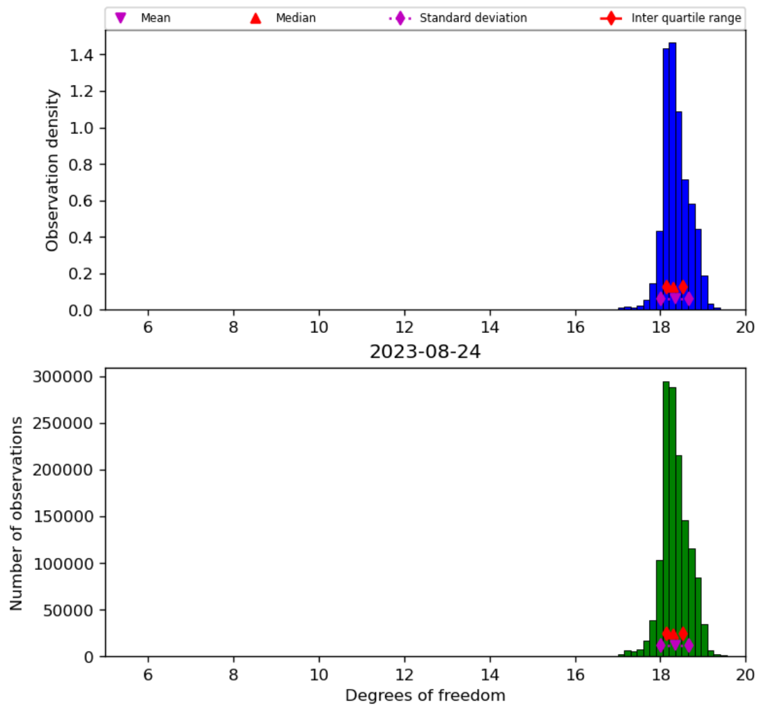
Figure 30: Histogram of “Degrees of freedom” for 2023-08-23 to 2023-08-25
