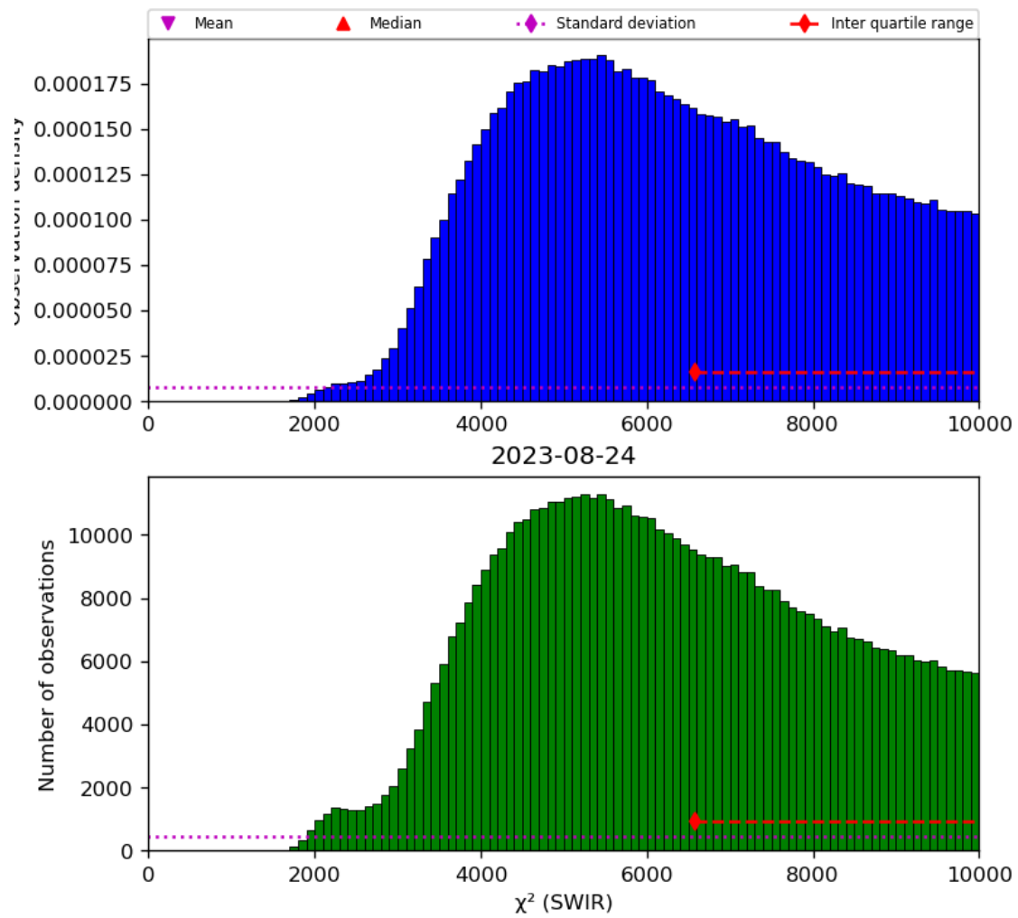
Figure 28: Histogram of “ \chi^2 (SWIR)” for 2023-08-23 to 2023-08-25
