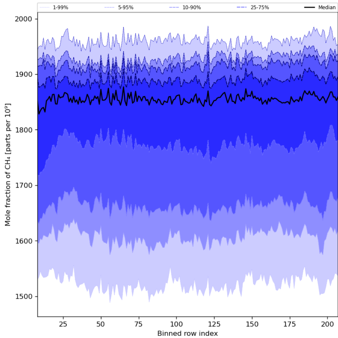
Figure 34: Along track statistics of “Mole fraction of CH 4 ” for 2023-08-23 to 2023-08-25
