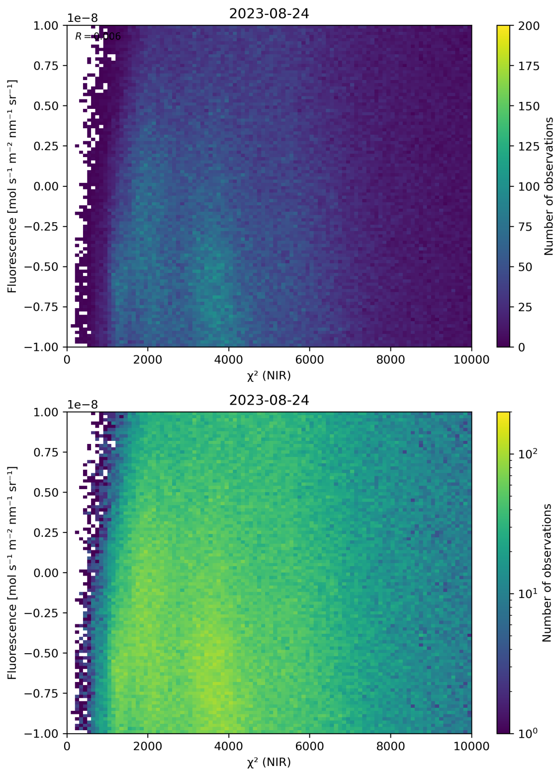
Figure 45: Scatter density plot of “ \chi^2 (NIR)” against “Fluorescence” for 2023-08-23 to 2023-08-25.
