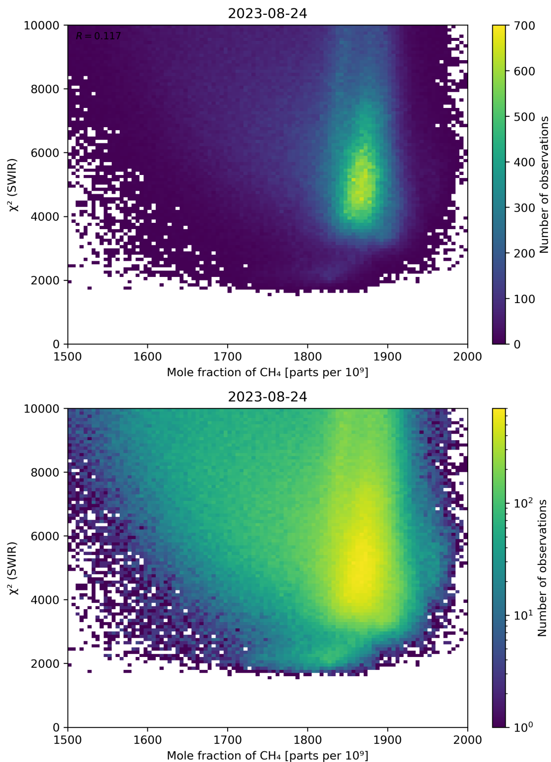
Figure 71: Scatter density plot of “Mole fraction of CH 4 ” against “ \chi^2 (SWIR)” for 2023-08-23 to 2023-08-25.
