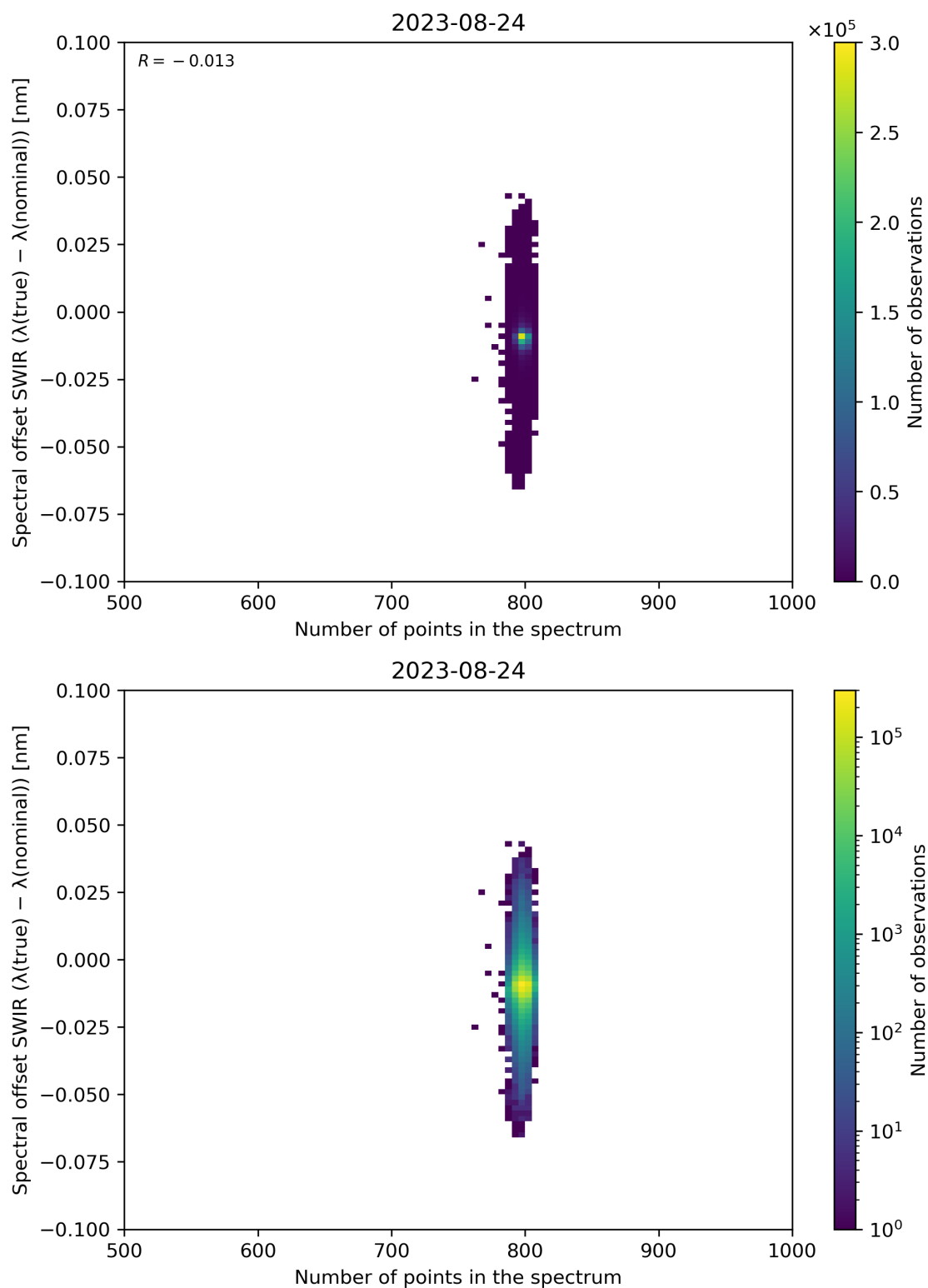
Figure 93: Scatter density plot of “Number of points in the spectrum” against “Spectral offset SWIR ( \lambda(\text{true}) - \lambda(\text{nominal}) )” for 2023-08-23 to 2023-08-25.
