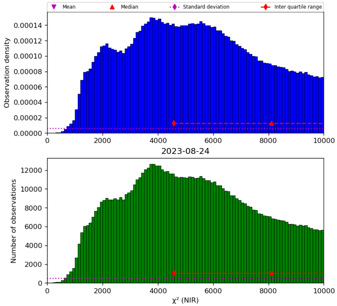
Figure 29: Histogram of " \chi^2 (NIR)" for 2023-08-23 to 2023-08-25
