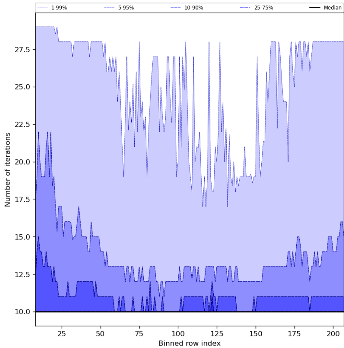
Figure 42: Along track statistics of “Number of iterations” for 2023-08-23 to 2023-08-25
