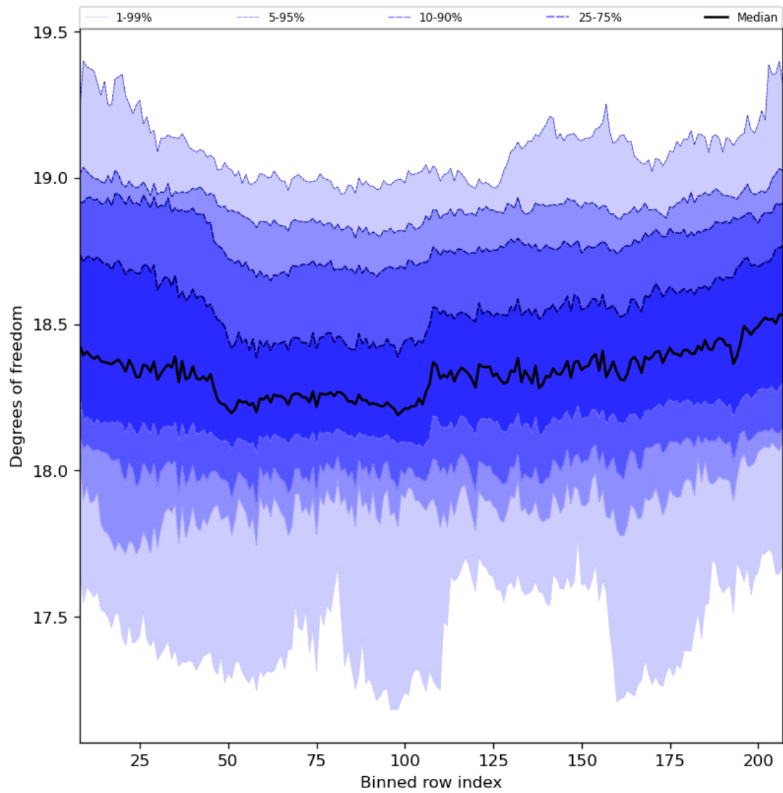
Figure 41: Along track statistics of “Degrees of freedom” for 2023-08-23 to 2023-08-25
