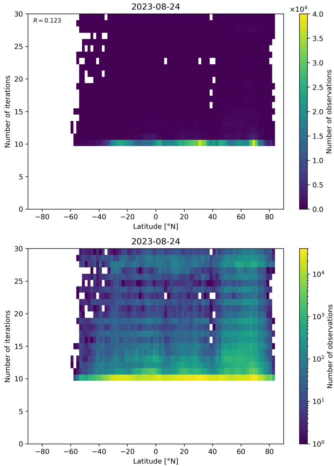
Figure 60: Scatter density plot of “Latitude” against “Number of iterations” for 2023-08-23 to 2023-08-25.
