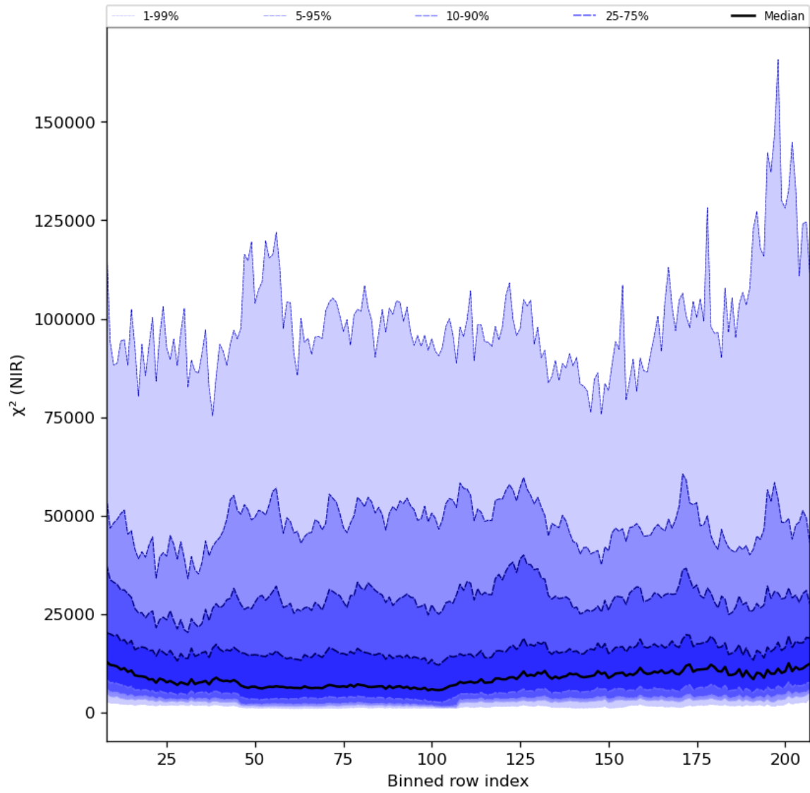
Figure 40: Along track statistics of " \chi^2 (NIR)" for 2023-08-23 to 2023-08-25
