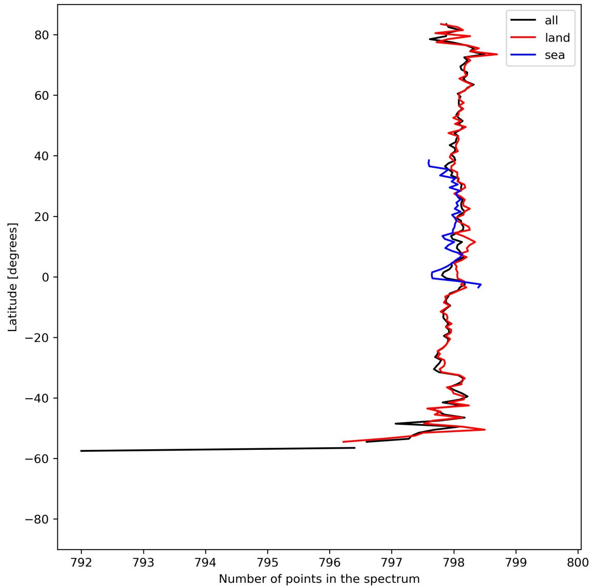
Figure 15: Zonal average of “Number of points in the spectrum” for 2023-08-23 to 2023-08-25.
