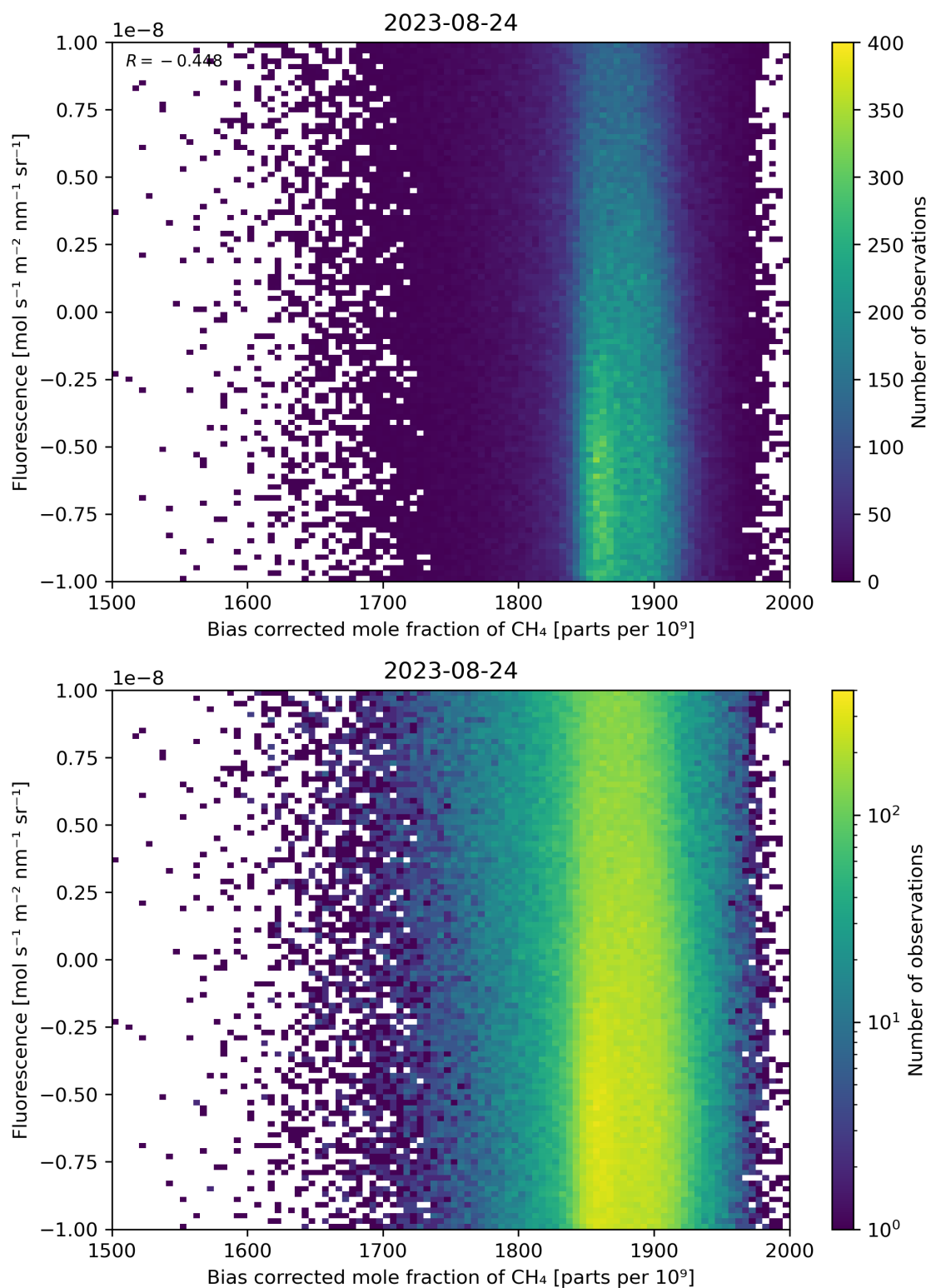
Figure 66: Scatter density plot of “Bias corrected mole fraction of \text{CH}_4 ” against “Fluorescence” for 2023-08-23 to 2023-08-25.
