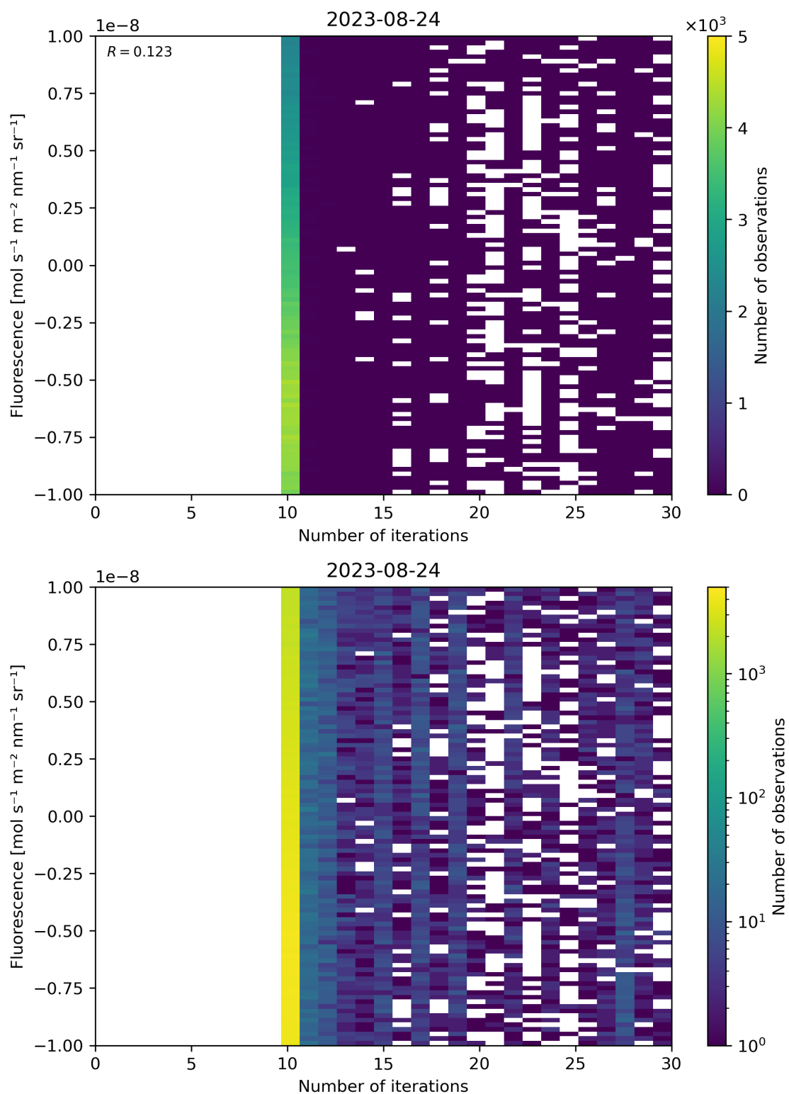
Figure 87: Scatter density plot of “Number of iterations” against “Fluorescence” for 2023-08-23 to 2023-08-25.
