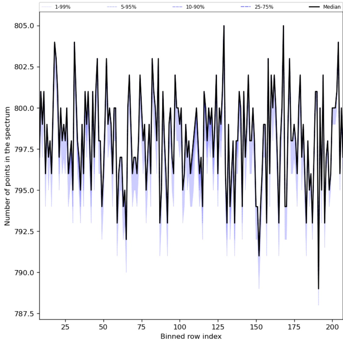
Figure 37: Along track statistics of “Number of points in the spectrum” for 2023-08-23 to 2023-08-25
