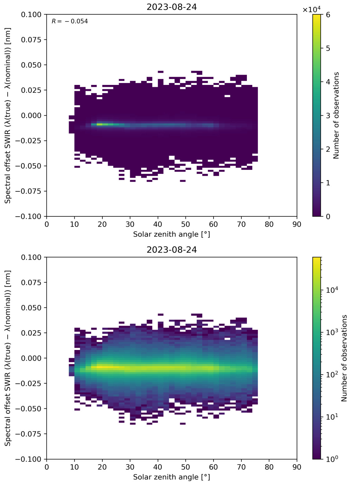
Figure 104: Scatter density plot of “Solar zenith angle” against “Spectral offset SWIR ( \lambda(\text{true}) - \lambda(\text{nominal}) )” for 2023-08-23 to 2023-08-25.
