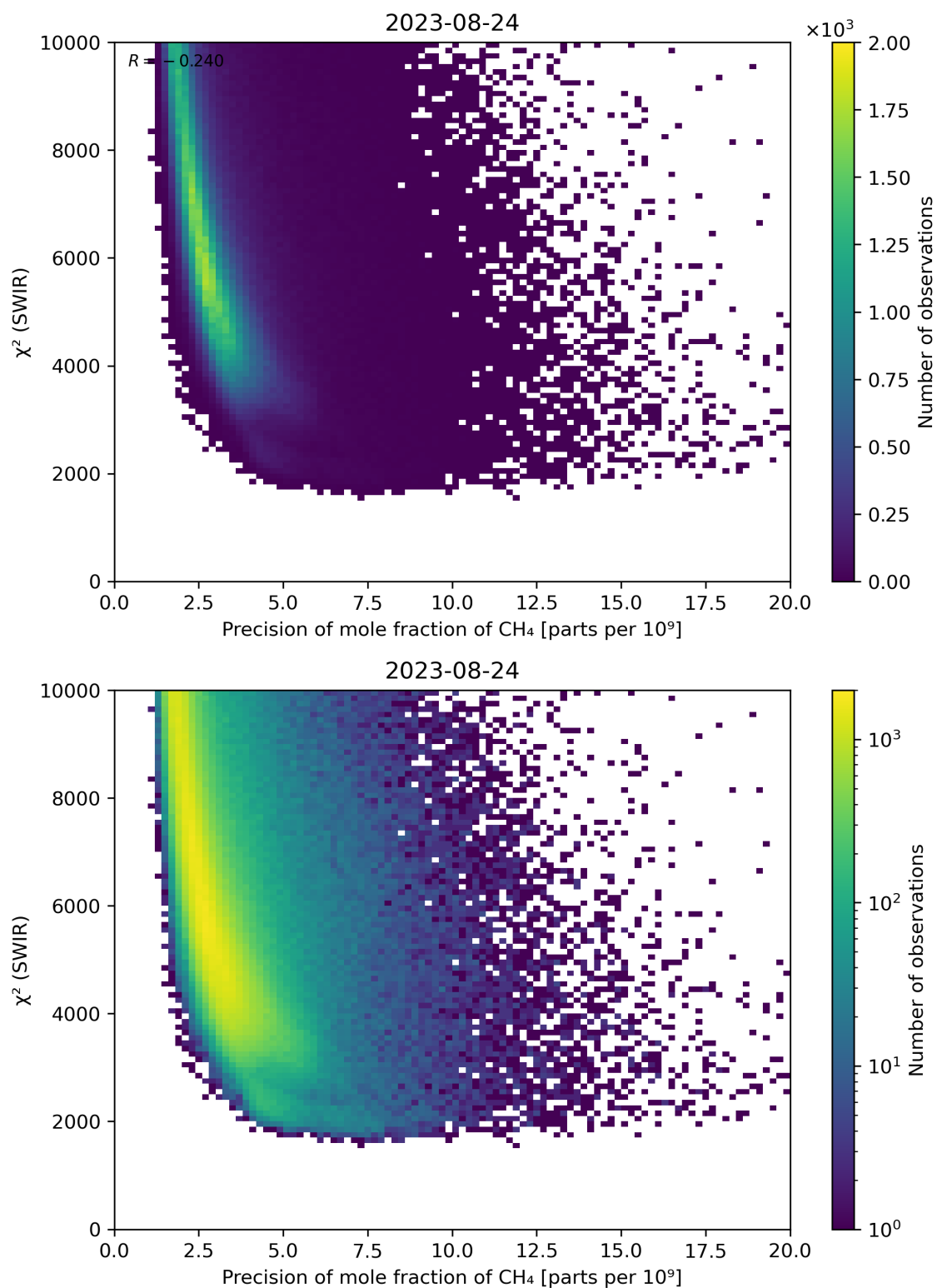
Figure 79: Scatter density plot of “Precision of mole fraction of CH 4 ” against “ \chi^2 (SWIR)” for 2023-08-23 to 2023-08-25.
