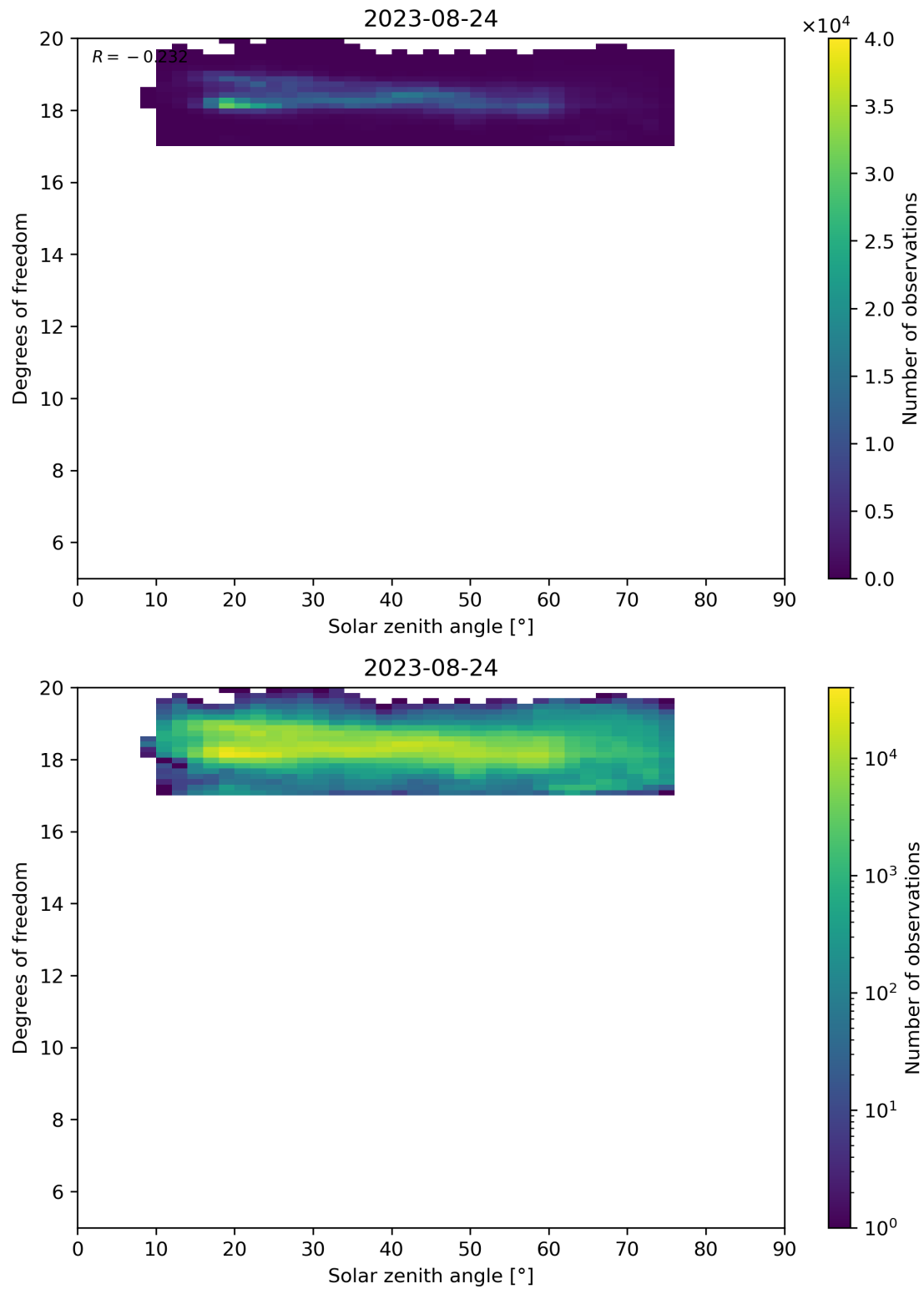
Figure 96: Scatter density plot of “Solar zenith angle” against “Degrees of freedom” for 2023-08-23 to 2023-08-25.
