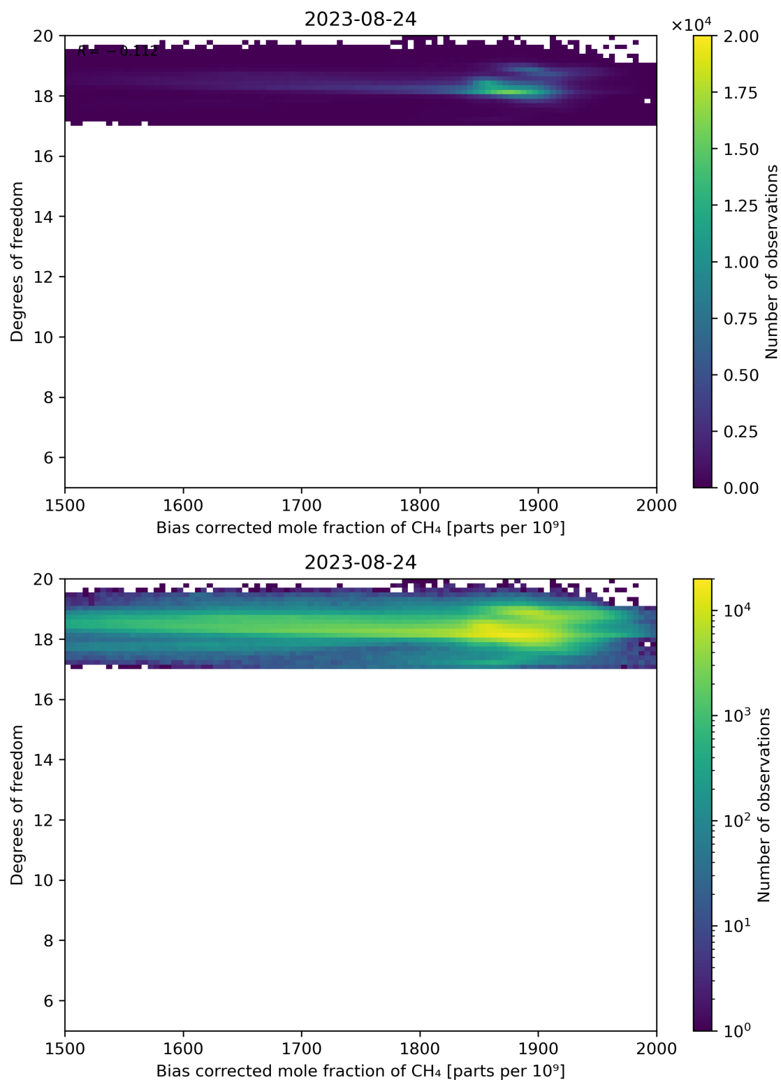
Figure 65: Scatter density plot of “Bias corrected mole fraction of CH 4 ” against “Degrees of freedom” for 2023-08-23 to 2023-08-25.
