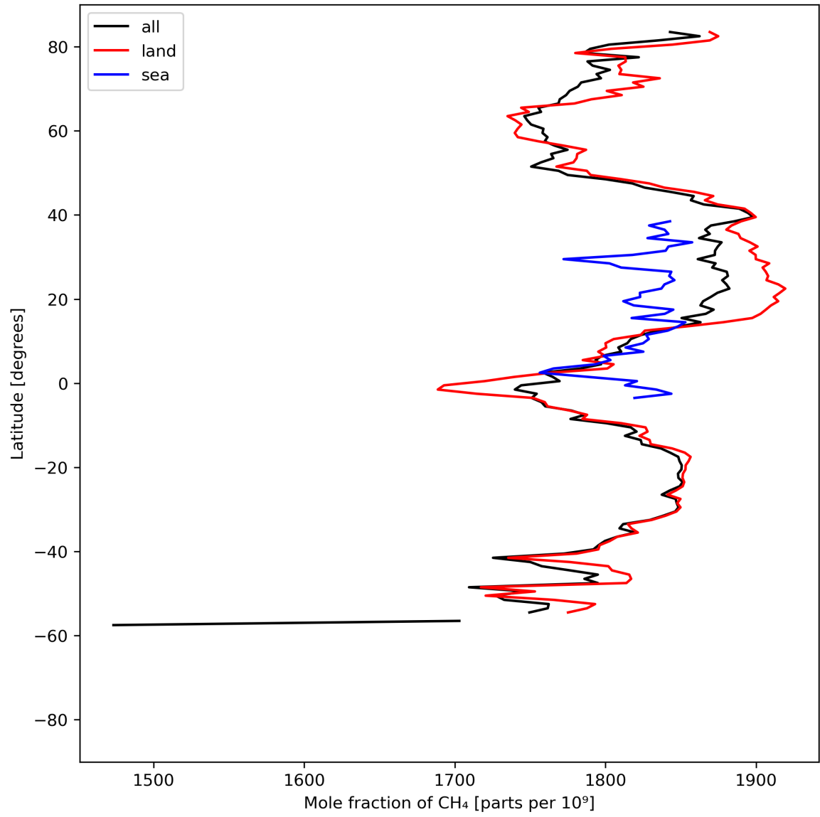
Figure 12: Zonal average of “Mole fraction of \text{CH}_4 ” for 2023-08-23 to 2023-08-25.
