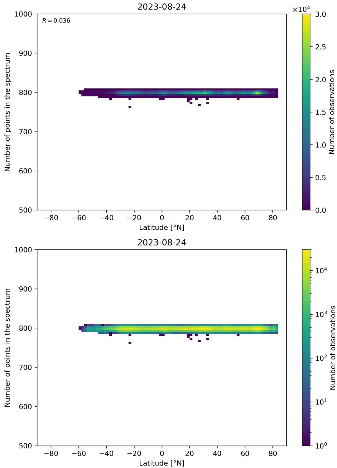
Figure 61: Scatter density plot of “Latitude” against “Number of points in the spectrum” for 2023-08-23 to 2023-08-25.
