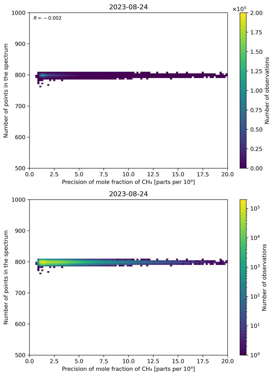
Figure 84: Scatter density plot of “Precision of mole fraction of CH 4 ” against “Number of points in the spectrum” for 2023-08-23 to 2023-08-25.
