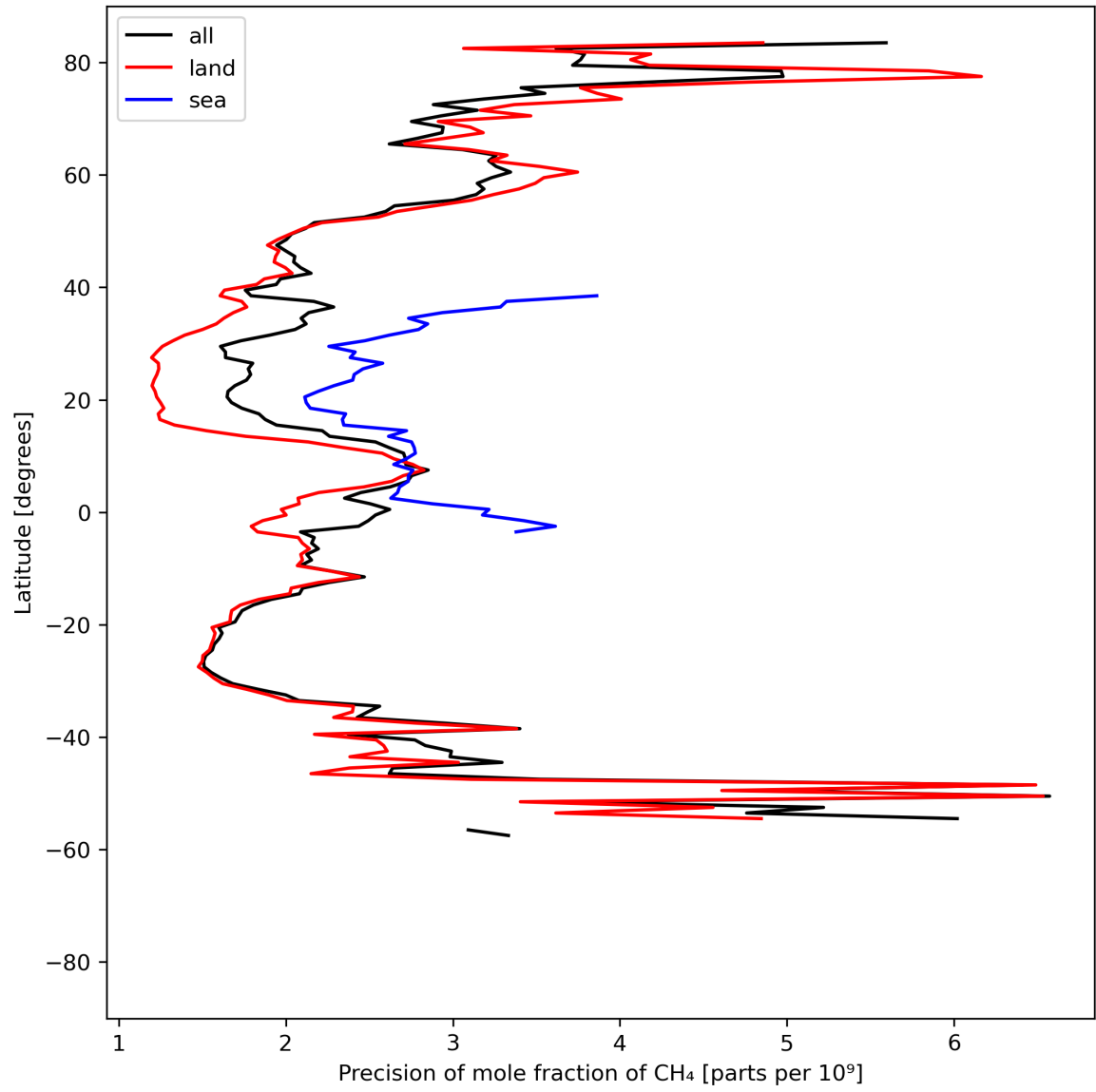
Figure 13: Zonal average of “Precision of mole fraction of CH 4 ” for 2023-08-23 to 2023-08-25.
