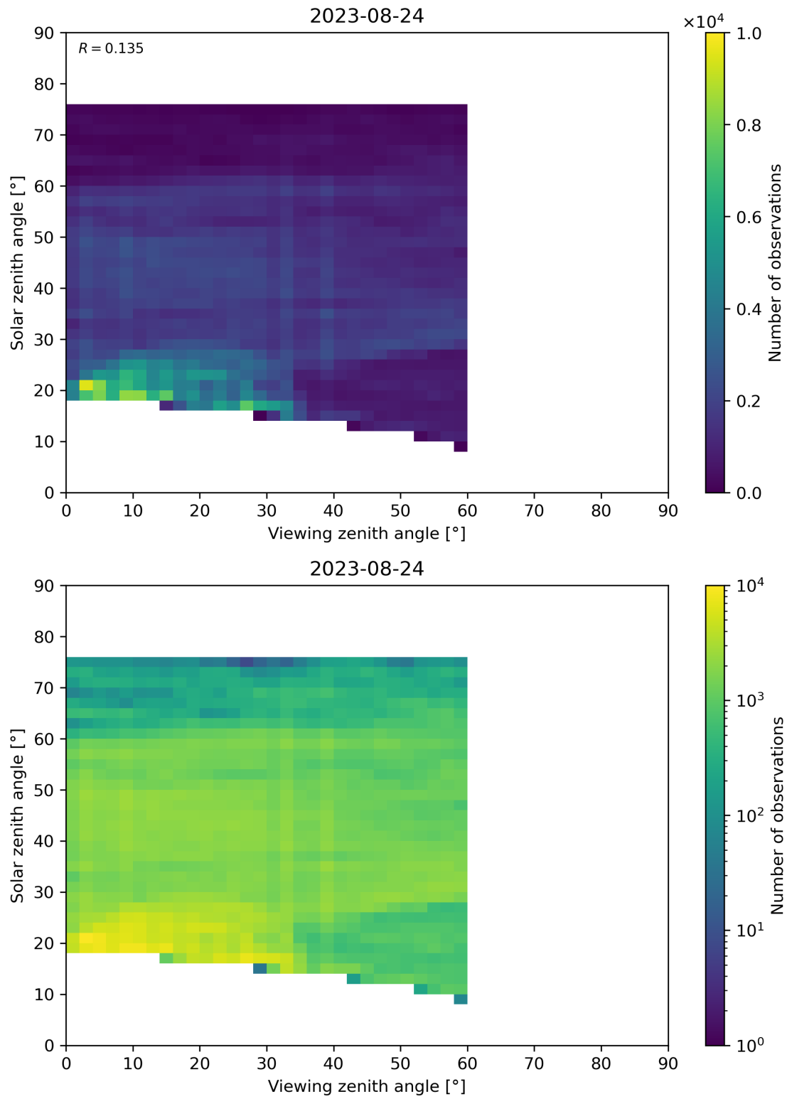
Figure 115: Scatter density plot of “Viewing zenith angle” against “Solar zenith angle” for 2023-08-23 to 2023-08-25.
