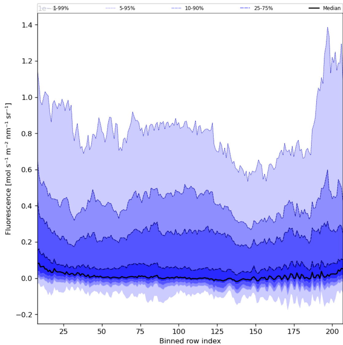
Figure 43: Along track statistics of “Fluorescence” for 2023-08-23 to 2023-08-25
