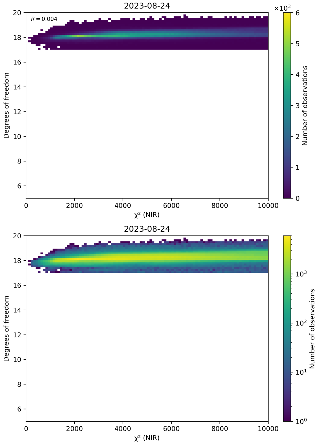
Figure 44: Scatter density plot of “ \chi^2 (NIR)” against “Degrees of freedom” for 2023-08-23 to 2023-08-25.
