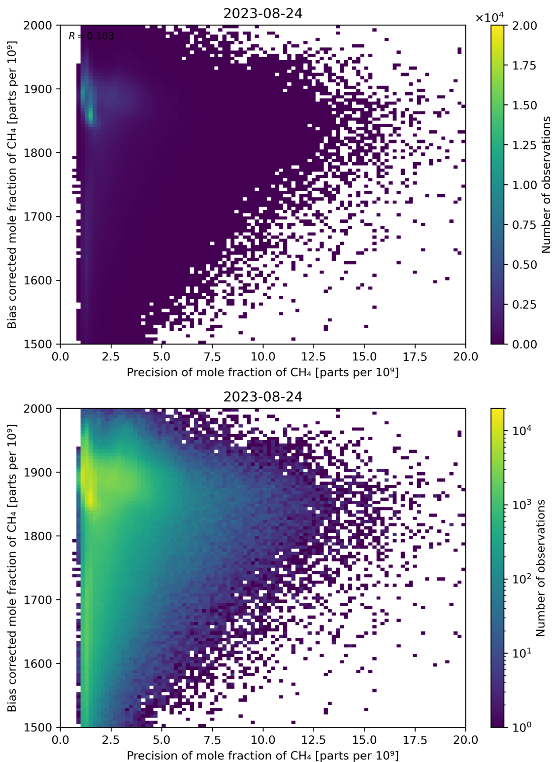
Figure 82: Scatter density plot of “Precision of mole fraction of \text{CH}_4 ” against “Bias corrected mole fraction of \text{CH}_4 ” for 2023-08-23 to 2023-08-25.
