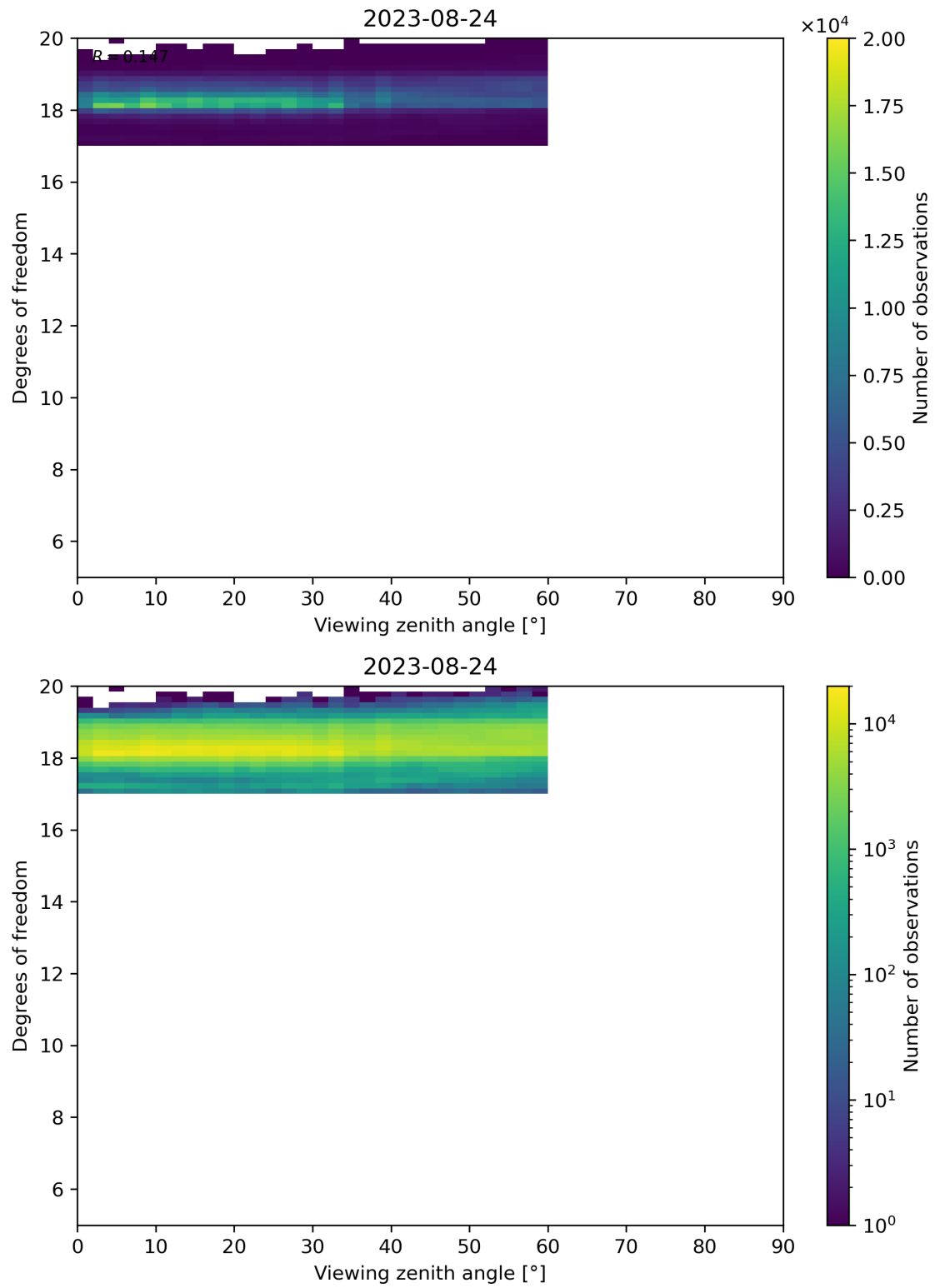
Figure 107: Scatter density plot of “Viewing zenith angle” against “Degrees of freedom” for 2023-08-23 to 2023-08-25.
