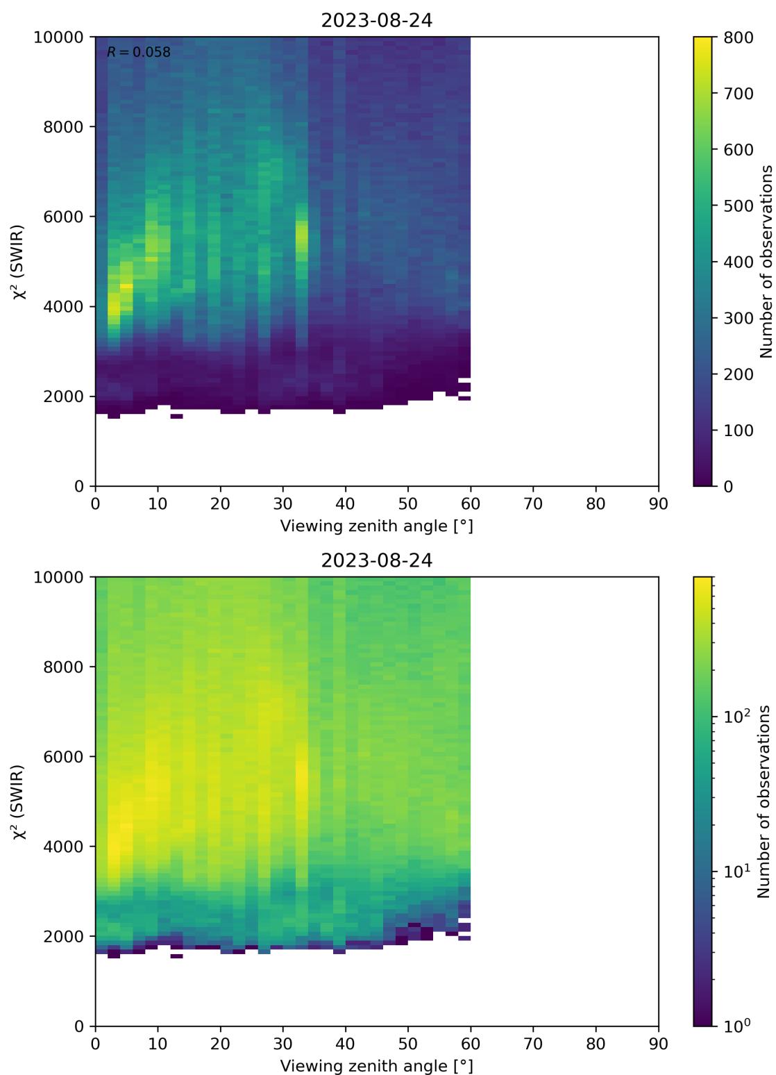
Figure 106: Scatter density plot of “Viewing zenith angle” against “ \chi^2 (SWIR)” for 2023-08-23 to 2023-08-25.
