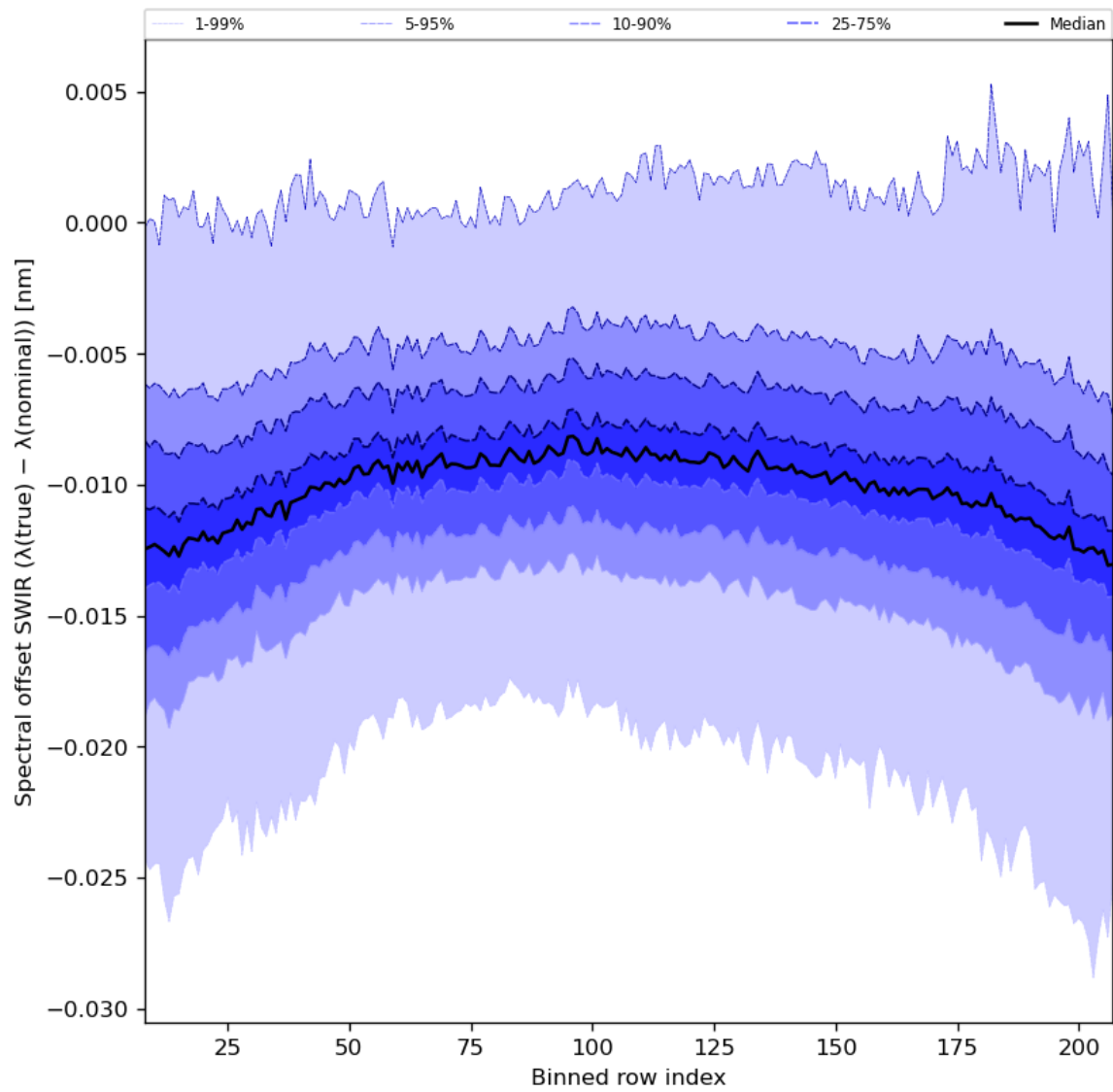
Figure 38: Along track statistics of “Spectral offset SWIR ( \lambda(\text{true}) - \lambda(\text{nominal}) )” for 2023-08-23 to 2023-08-25
