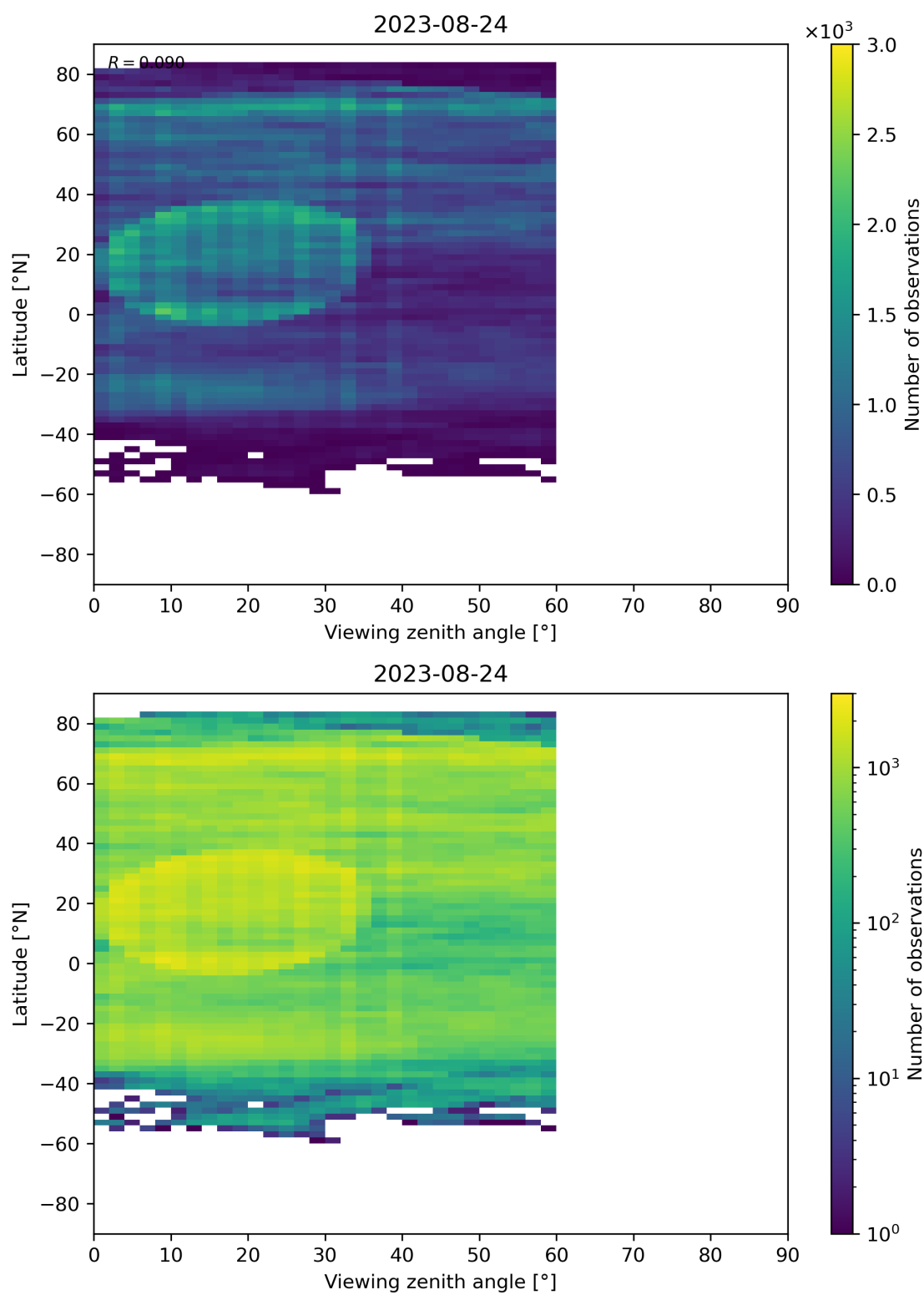
Figure 109: Scatter density plot of “Viewing zenith angle” against “Latitude” for 2023-08-23 to 2023-08-25.
