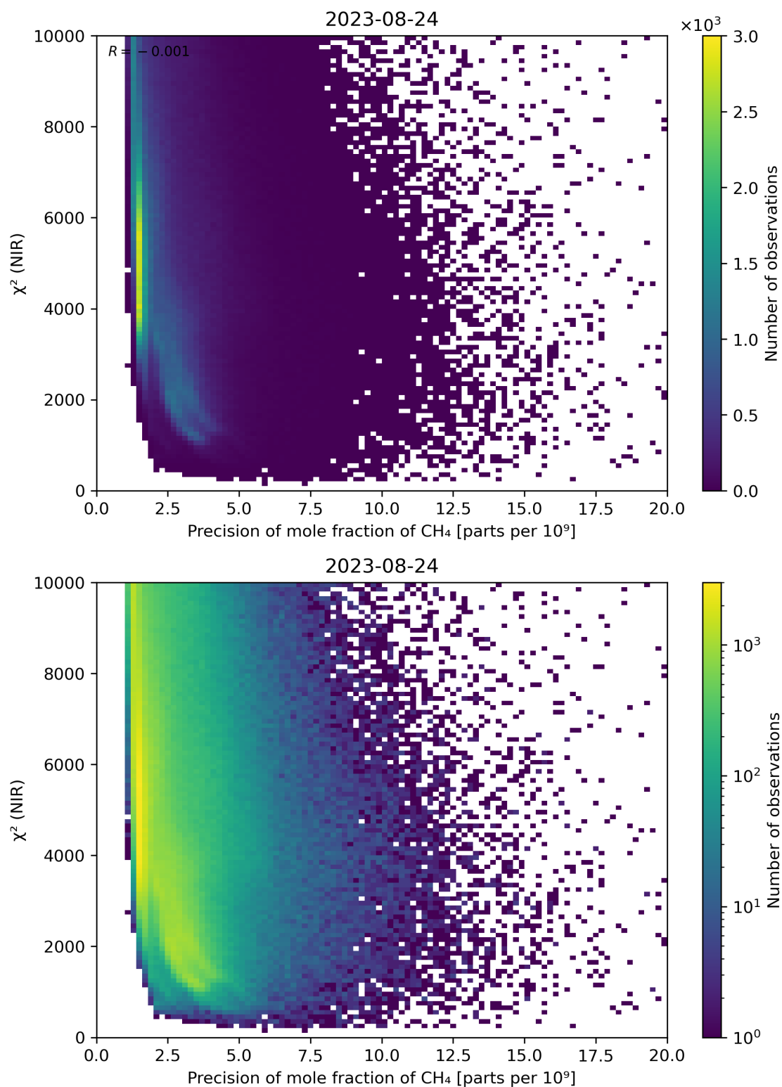
Figure 78: Scatter density plot of “Precision of mole fraction of CH 4 ” against “ \chi^2 (NIR)” for 2023-08-23 to 2023-08-25.
