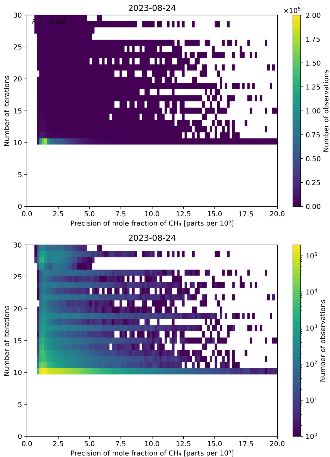
Figure 83: Scatter density plot of “Precision of mole fraction of CH 4 ” against “Number of iterations” for 2023-08-23 to 2023-08-25.
