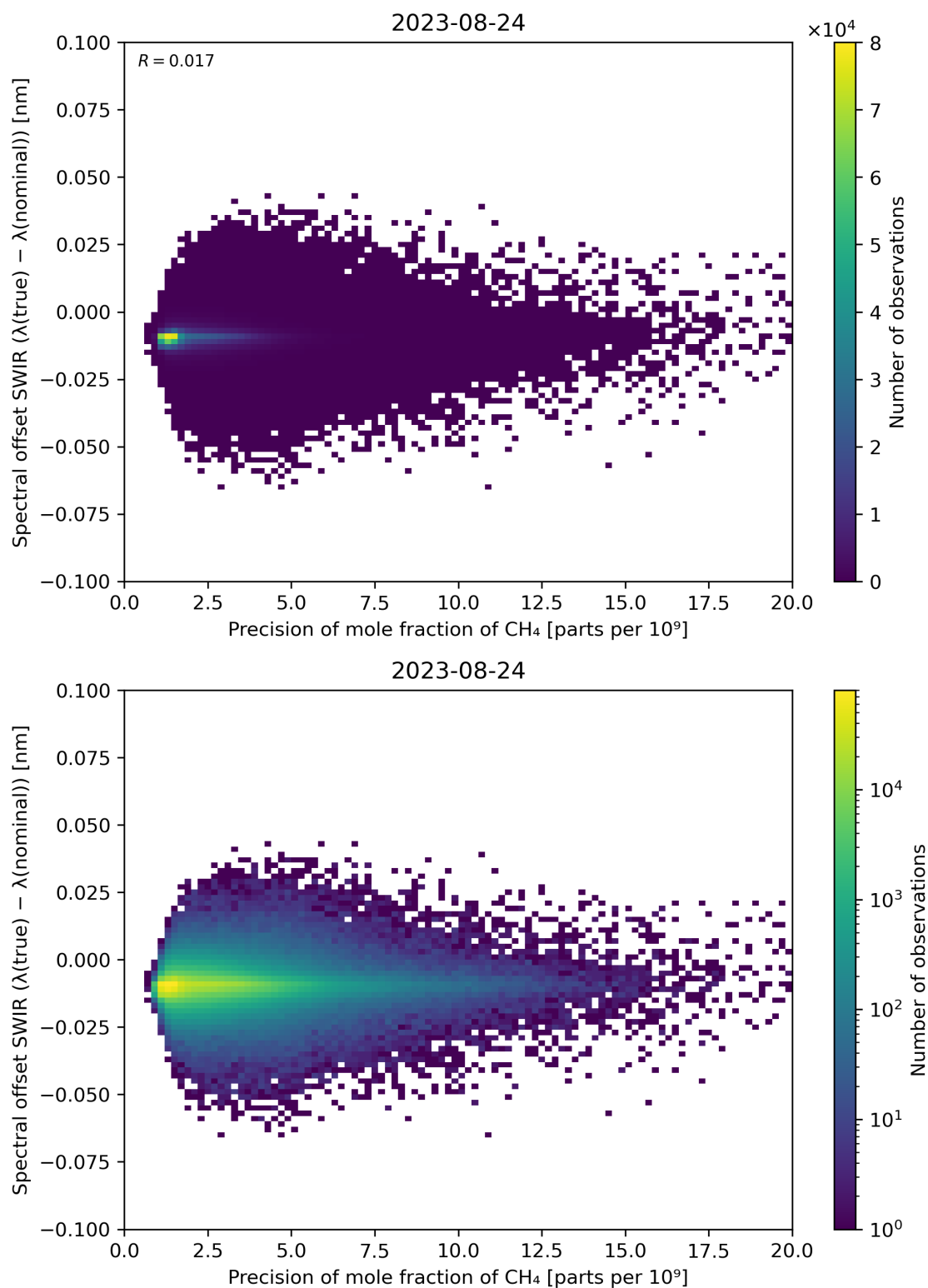
Figure 85: Scatter density plot of “Precision of mole fraction of CH 4 ” against “Spectral offset SWIR ( \lambda(\text{true}) - \lambda(\text{nominal}) )” for 2023-08-23 to 2023-08-25.
