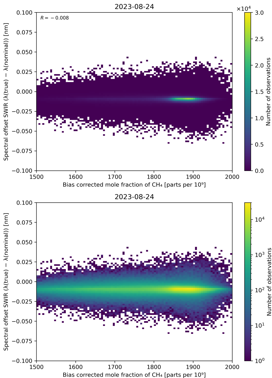
Figure 69: Scatter density plot of “Bias corrected mole fraction of \text{CH}_4 ” against “Spectral offset SWIR ( \lambda(\text{true}) - \lambda(\text{nominal}) )” for 2023-08-23 to 2023-08-25.
