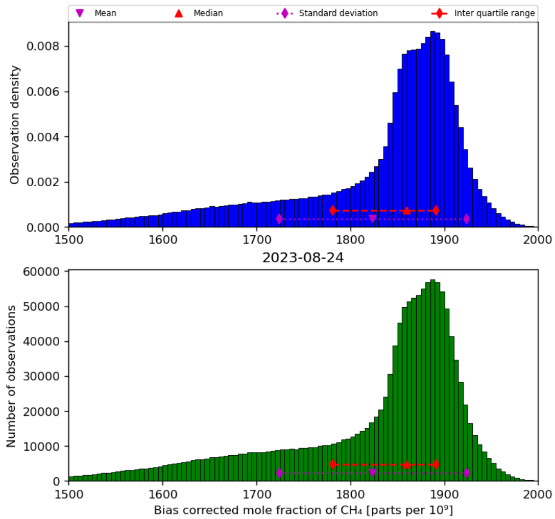
Figure 25: Histogram of “Bias corrected mole fraction of CH 4 ” for 2023-08-23 to 2023-08-25
