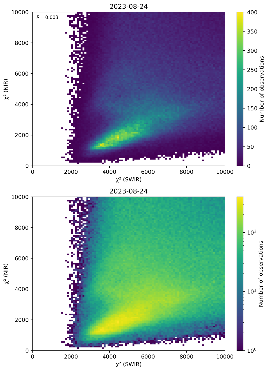
Figure 47: Scatter density plot of “ \chi^2 (SWIR)” against “ \chi^2 (NIR)” for 2023-08-23 to 2023-08-25.
