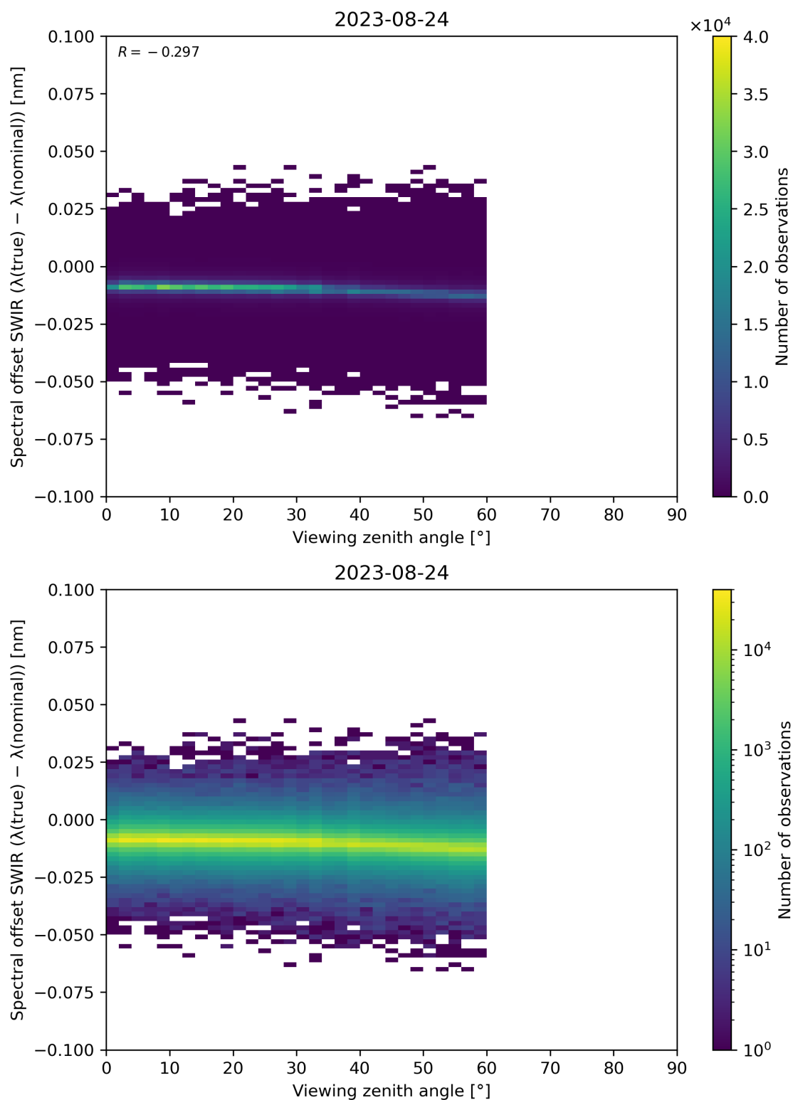
Figure 116: Scatter density plot of “Viewing zenith angle” against “Spectral offset SWIR ( \lambda(\text{true}) - \lambda(\text{nominal}) )” for 2023-08-23 to 2023-08-25.
