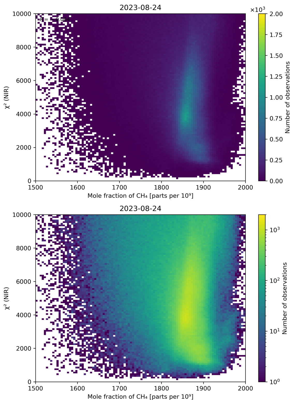
Figure 70: Scatter density plot of “Mole fraction of \text{CH}_4 ” against “ \chi^2 (NIR)” for 2023-08-23 to 2023-08-25.
