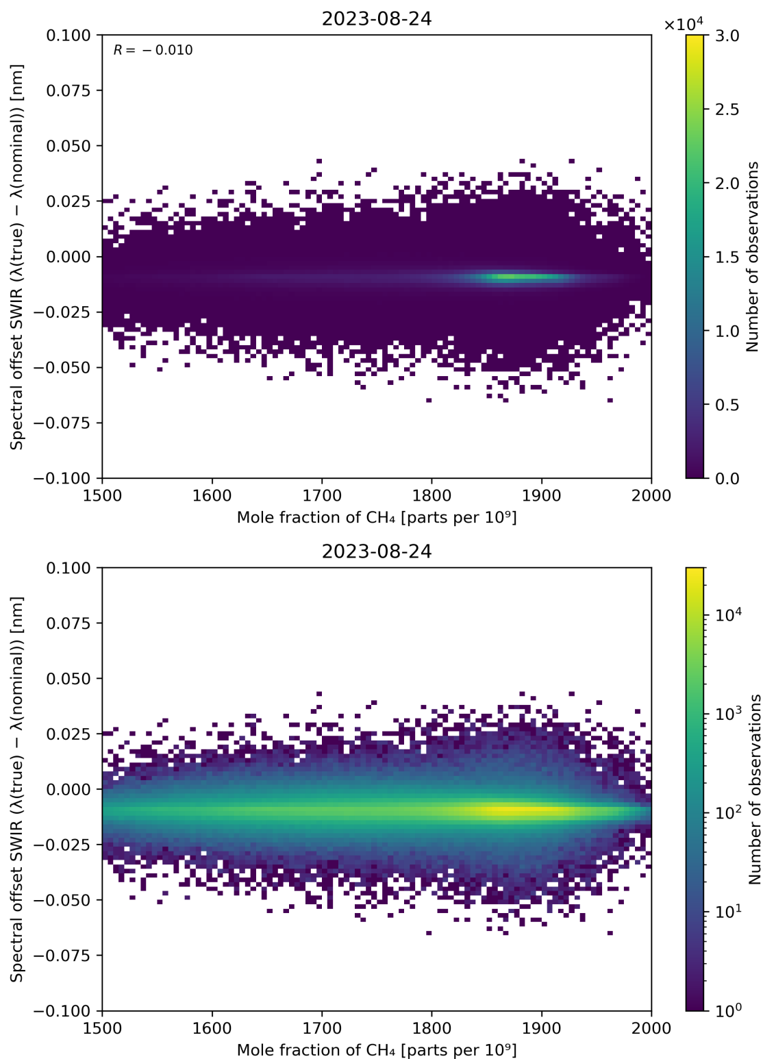
Figure 86: Scatter density plot of “Mole fraction of CH 4 ” against “Spectral offset SWIR ( \lambda(\text{true}) - \lambda(\text{nominal}) )” for 2023-08-23 to 2023-08-25.
