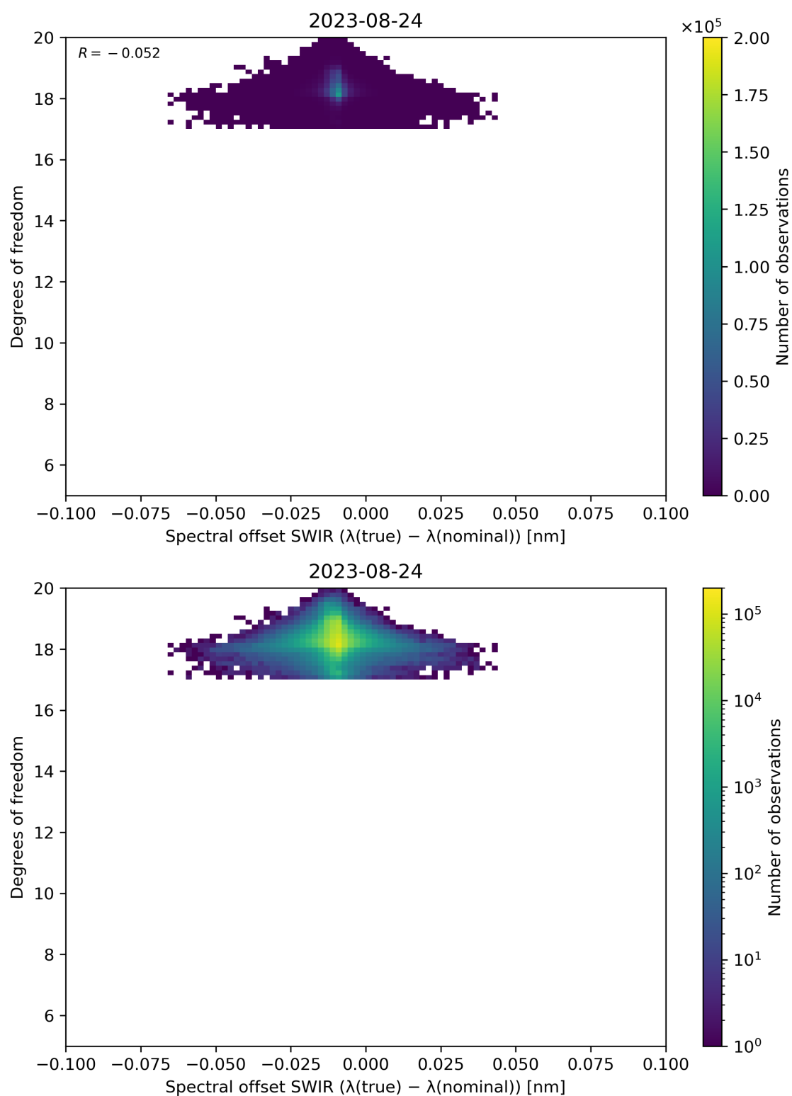
Figure 119: Scatter density plot of “Spectral offset SWIR ( \lambda(\text{true}) - \lambda(\text{nominal}) )” against “Degrees of freedom” for 2023-08-23 to 2023-08-25.
