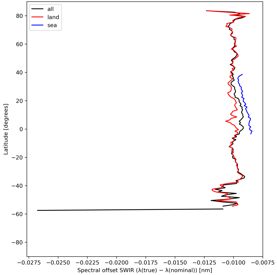
Figure 16: Zonal average of “Spectral offset SWIR ( \lambda(\text{true}) - \lambda(\text{nominal}) )” for 2023-08-23 to 2023-08-25.
