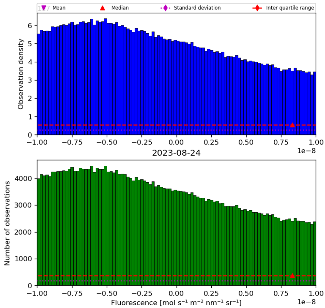
Figure 32: Histogram of “Fluorescence” for 2023-08-23 to 2023-08-25
