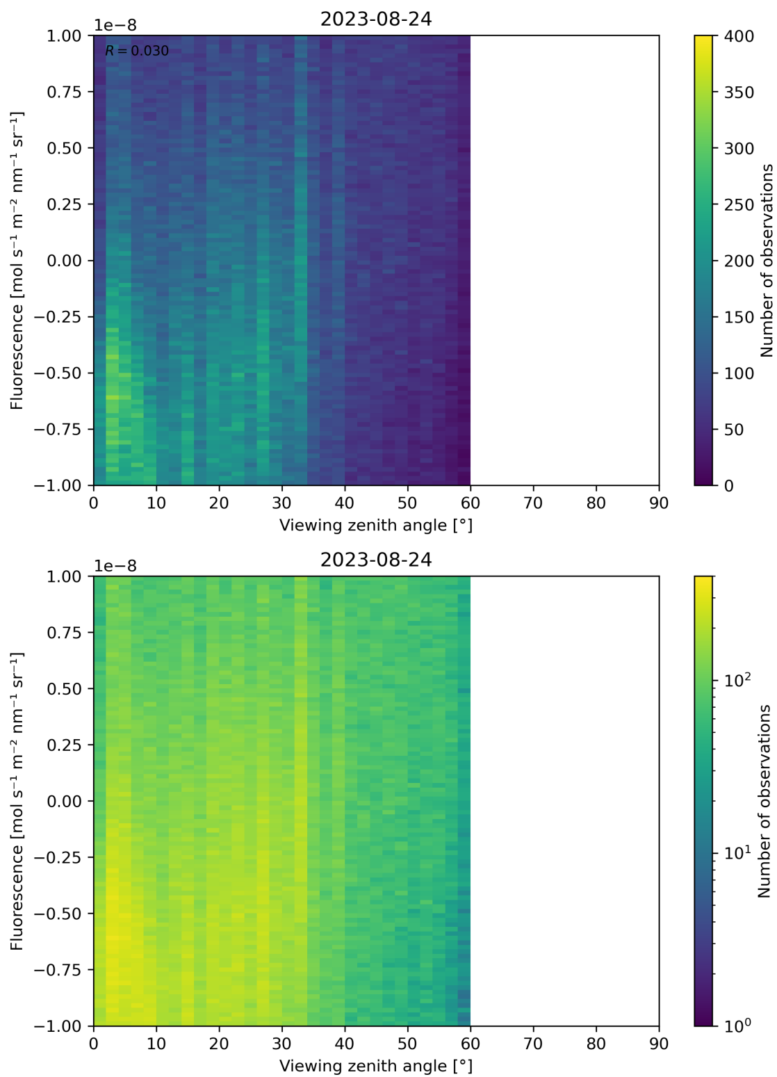
Figure 108: Scatter density plot of “Viewing zenith angle” against “Fluorescence” for 2023-08-23 to 2023-08-25.
