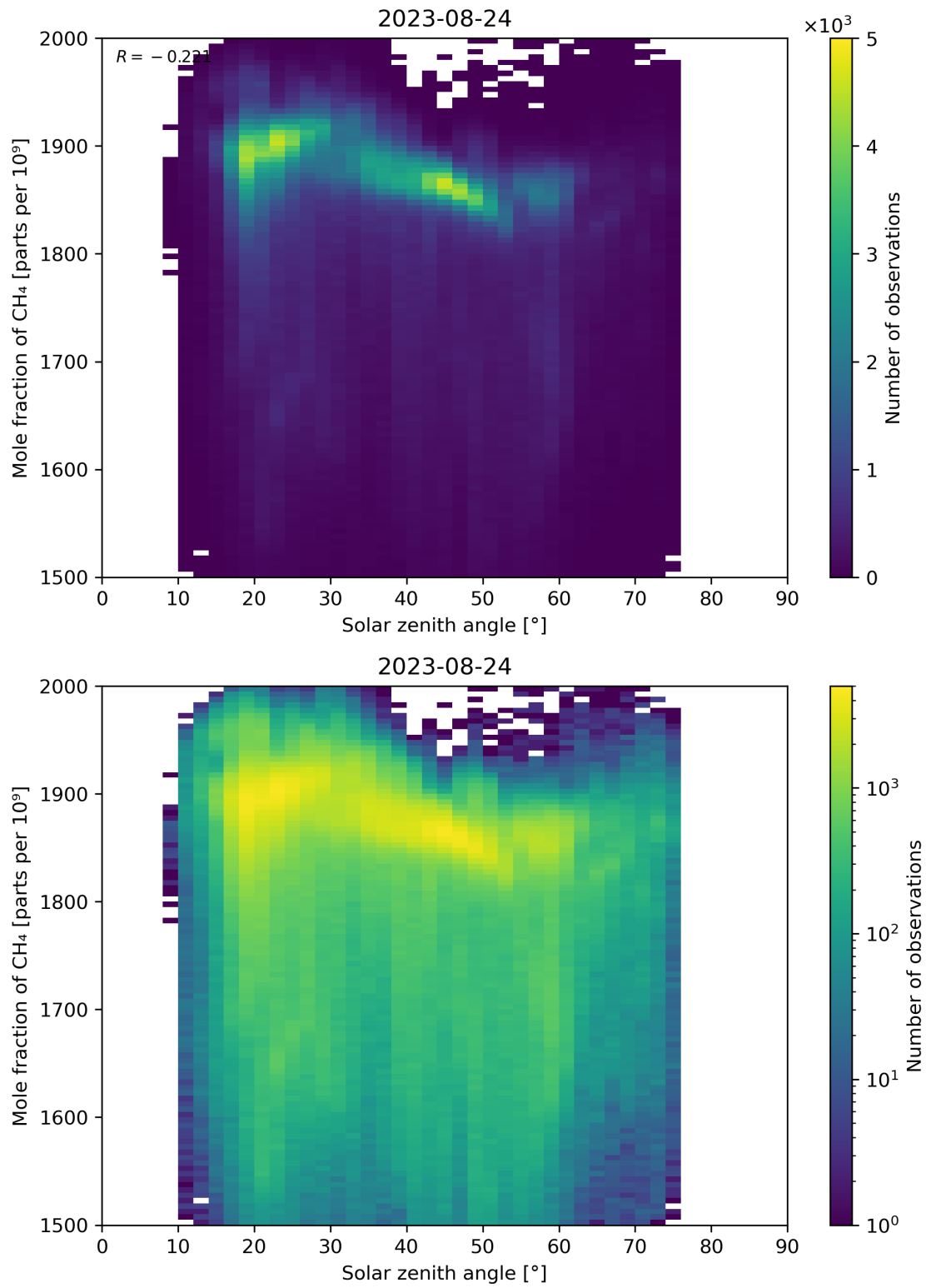
Figure 99: Scatter density plot of “Solar zenith angle” against “Mole fraction of CH 4 ” for 2023-08-23 to 2023-08-25.
