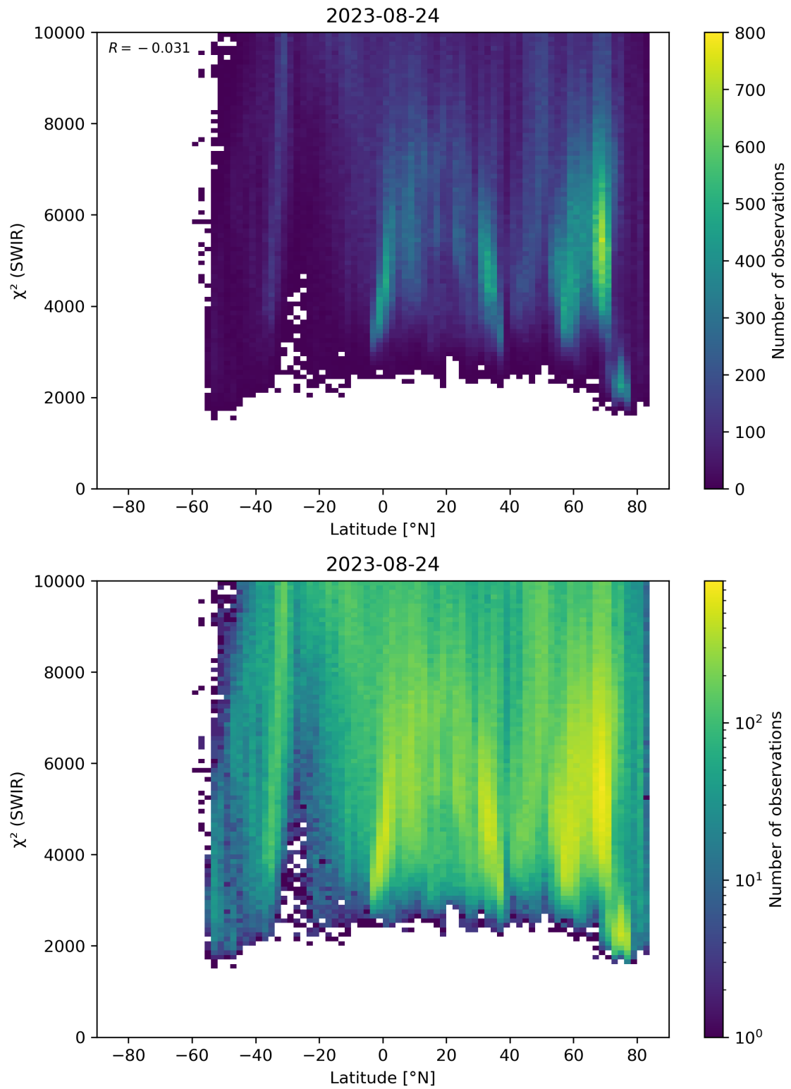
Figure 54: Scatter density plot of “Latitude” against “ \chi^2 (SWIR)” for 2023-08-23 to 2023-08-25.
