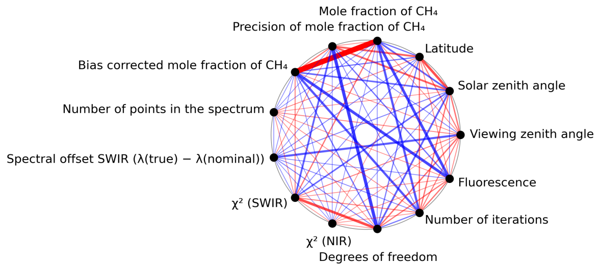
Figure 1: Map of correlation graph for 2023-08-23 to 2023-08-25.
