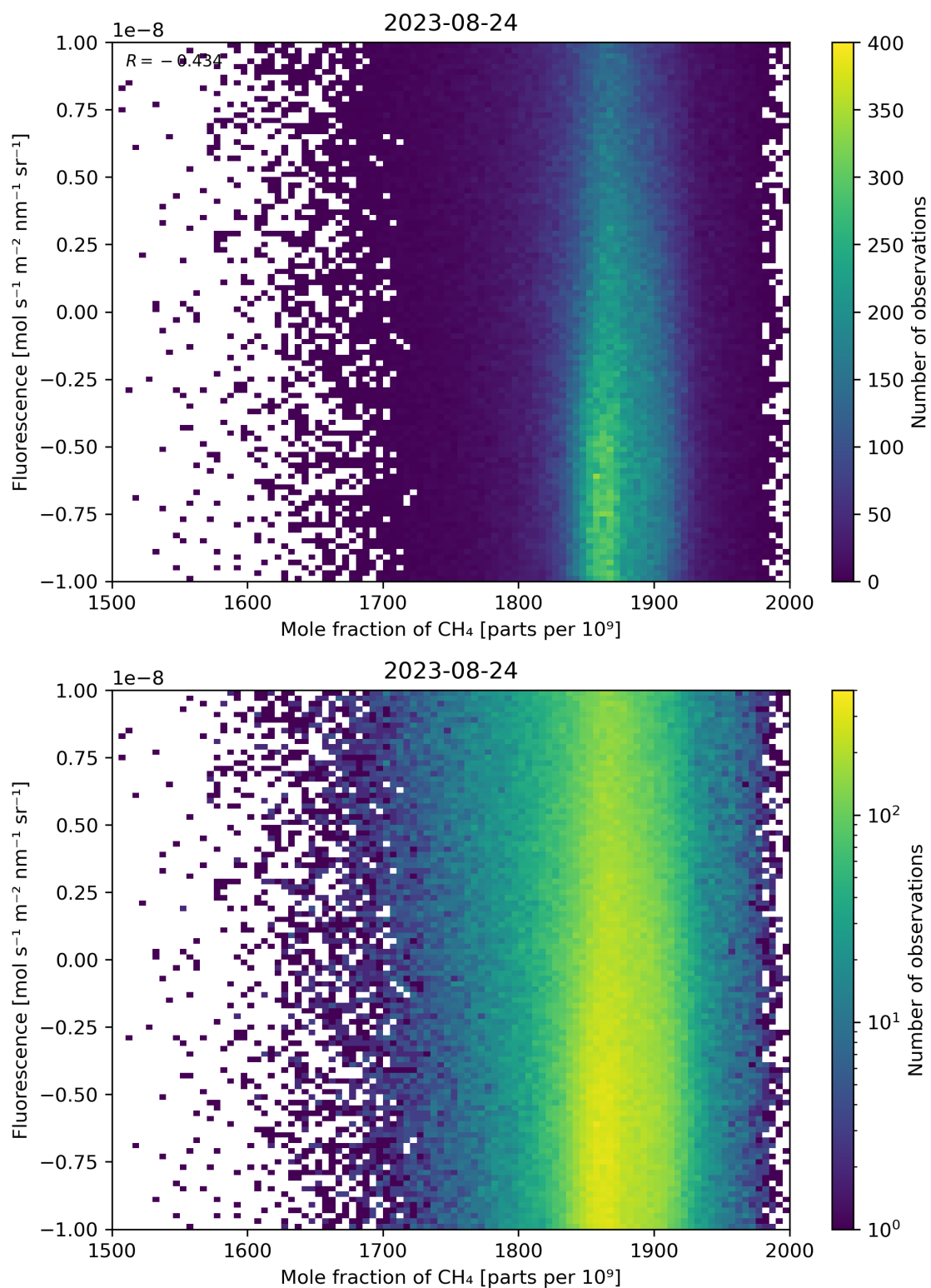
Figure 73: Scatter density plot of “Mole fraction of \text{CH}_4 ” against “Fluorescence” for 2023-08-23 to 2023-08-25.
