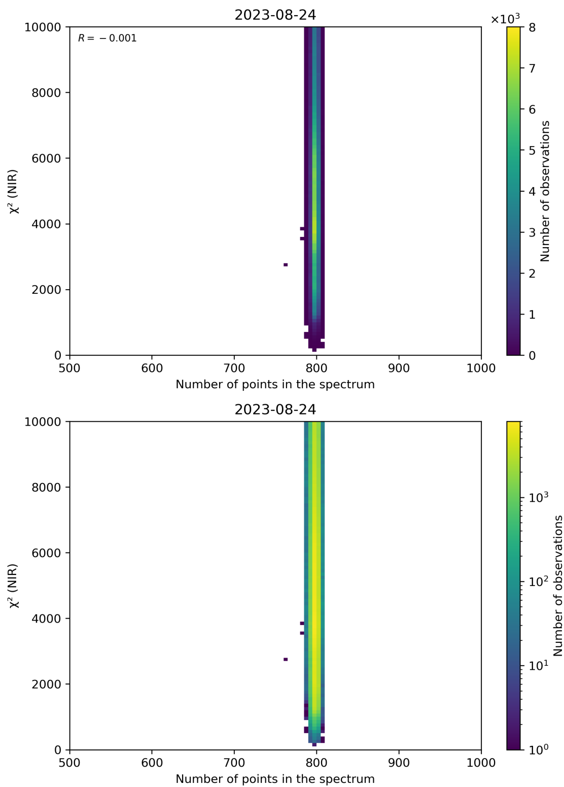
Figure 88: Scatter density plot of “Number of points in the spectrum” against “ \chi^2 (NIR)” for 2023-08-23 to 2023-08-25.
