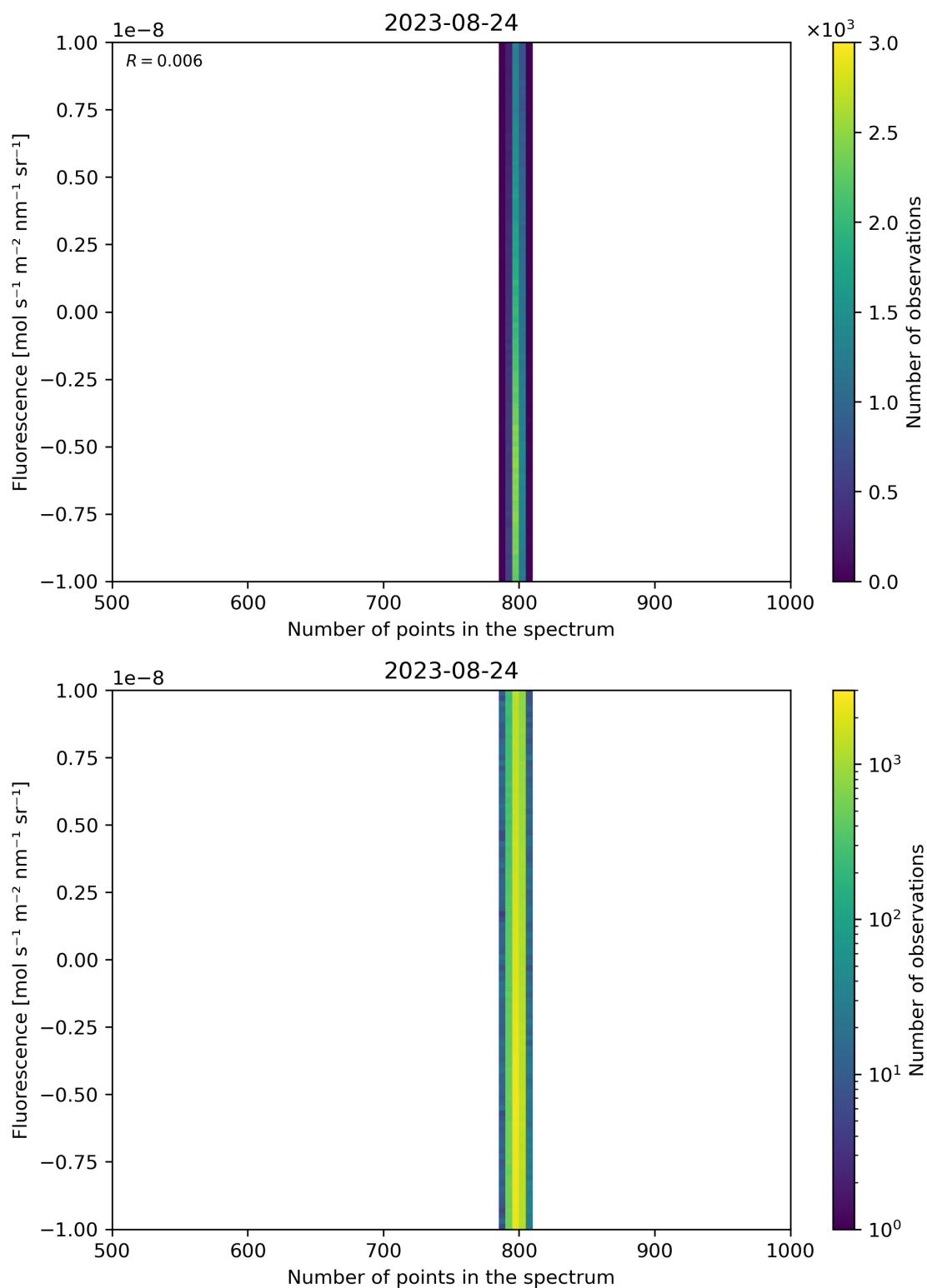
Figure 91: Scatter density plot of “Number of points in the spectrum” against “Fluorescence” for 2023-08-23 to 2023-08-25.
