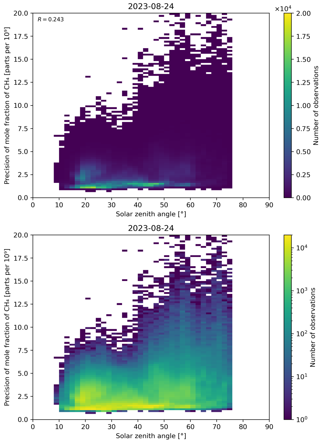
Figure 101: Scatter density plot of “Solar zenith angle” against “Precision of mole fraction of \text{CH}_4 ” for 2023-08-23 to 2023-08-25.
