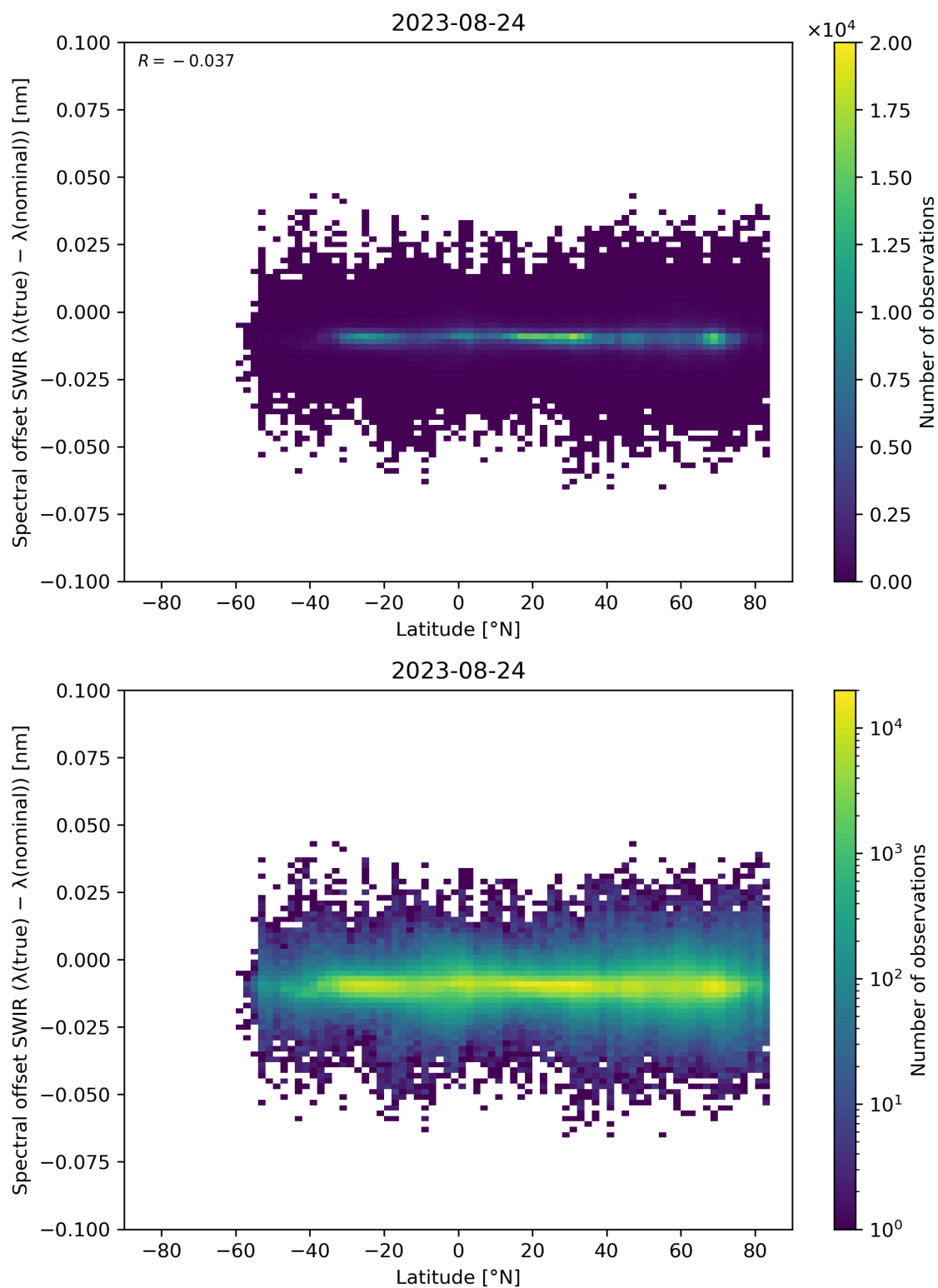
Figure 62: Scatter density plot of “Latitude” against “Spectral offset SWIR ( \lambda(\text{true}) - \lambda(\text{nominal}) )” for 2023-08-23 to 2023-08-25.
