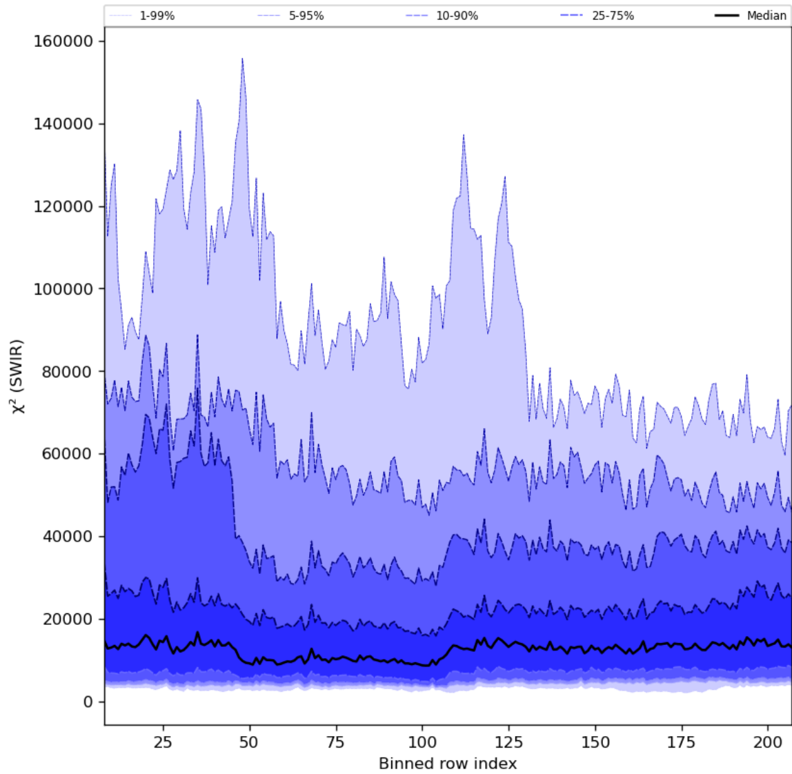
Figure 39: Along track statistics of " \chi^2 (SWIR)" for 2023-08-23 to 2023-08-25
