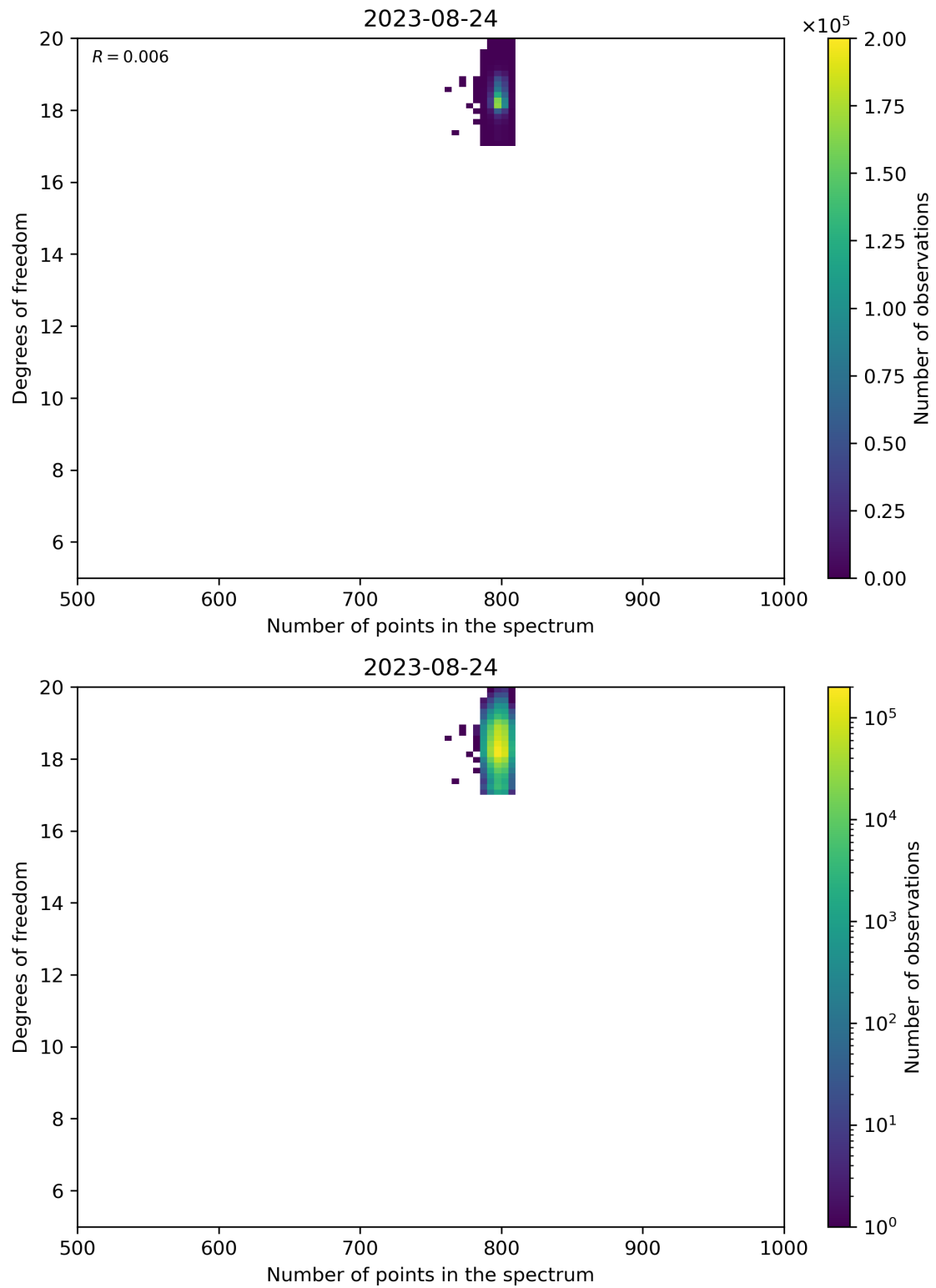
Figure 90: Scatter density plot of “Number of points in the spectrum” against “Degrees of freedom” for 2023-08-23 to 2023-08-25.
