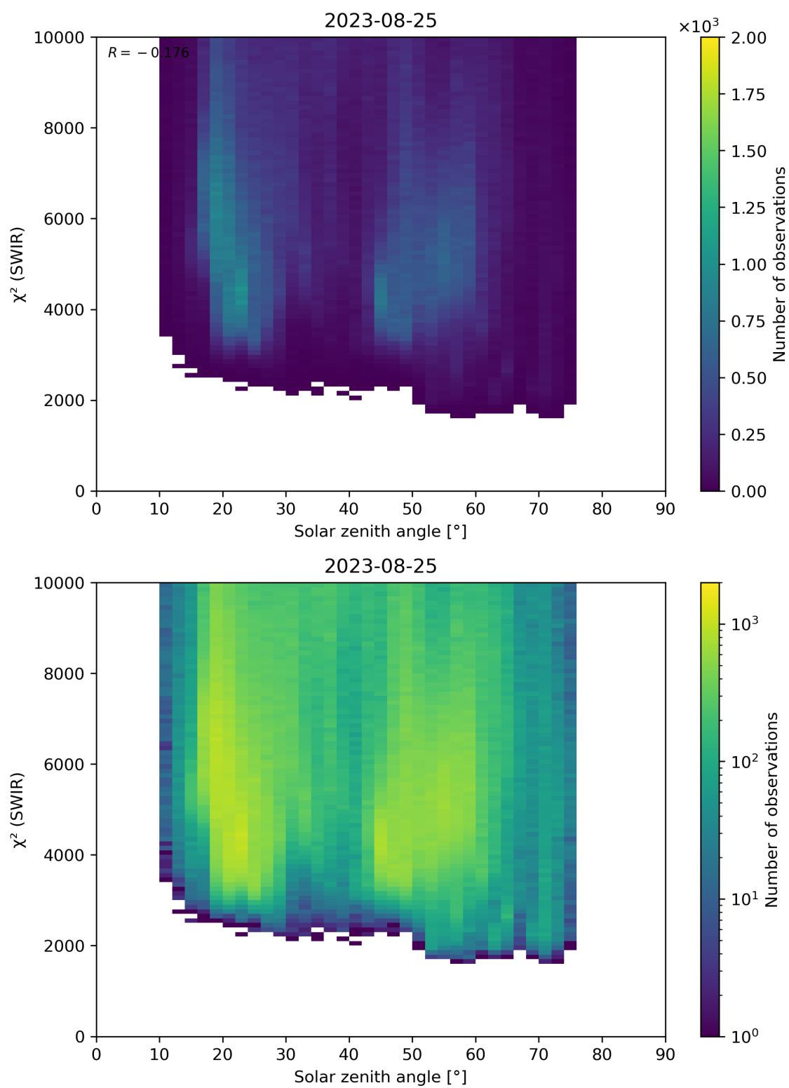
Figure 95: Scatter density plot of “Solar zenith angle” against “ \chi^2 (SWIR)” for 2023-08-25 to 2023-08-26.
