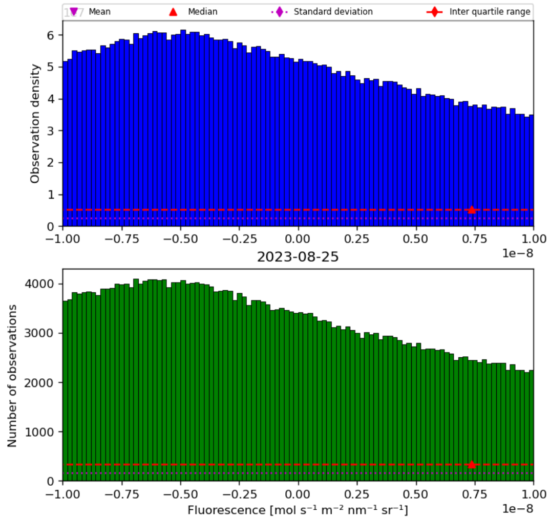
Figure 32: Histogram of “Fluorescence” for 2023-08-25 to 2023-08-26
