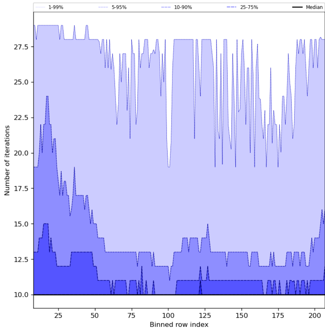
Figure 42: Along track statistics of “Number of iterations” for 2023-08-25 to 2023-08-26
