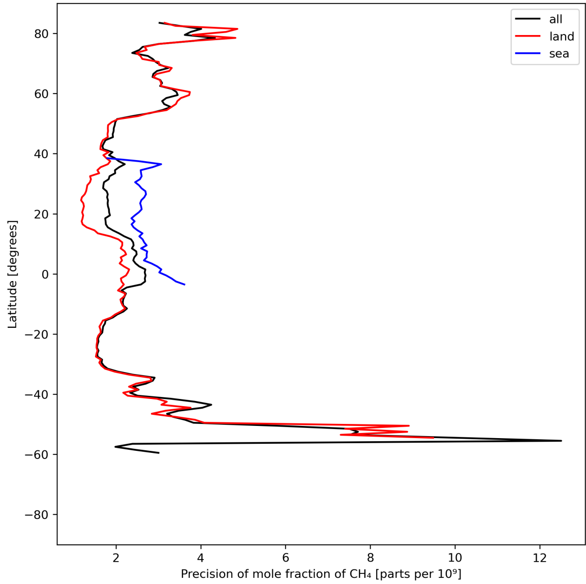
Figure 13: Zonal average of “Precision of mole fraction of \text{CH}_4 ” for 2023-08-25 to 2023-08-26.
