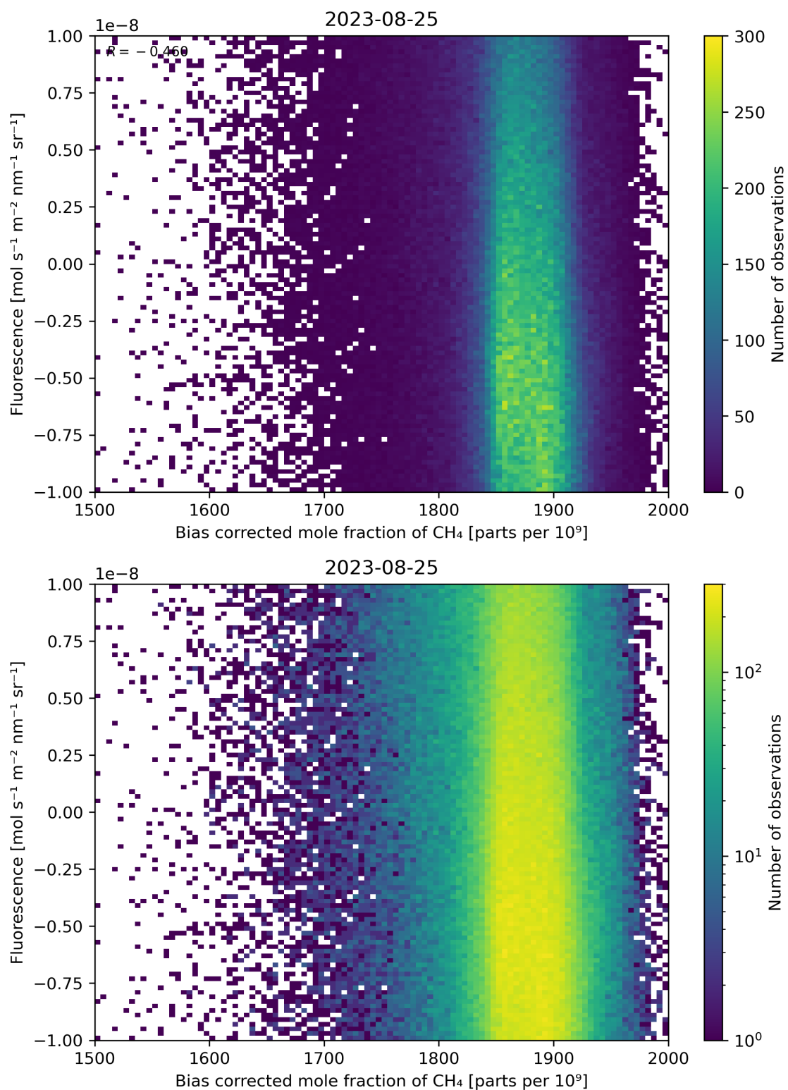
Figure 66: Scatter density plot of “Bias corrected mole fraction of \text{CH}_4 ” against “Fluorescence” for 2023-08-25 to 2023-08-26.
