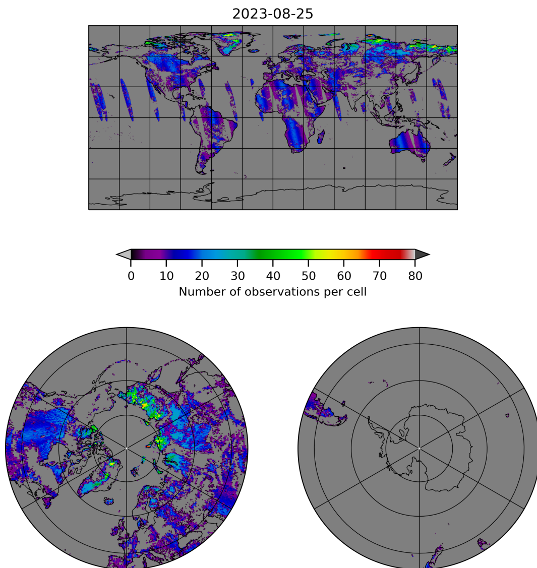
Figure 10: Map of the number of observations for 2023-08-25 to 2023-08-26
