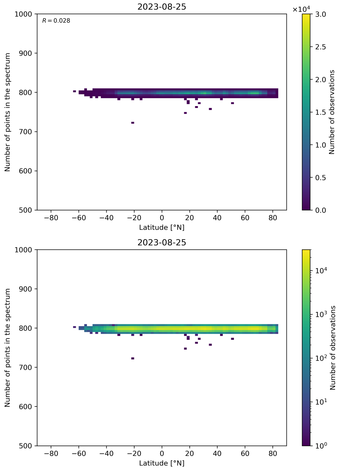
Figure 61: Scatter density plot of “Latitude” against “Number of points in the spectrum” for 2023-08-25 to 2023-08-26.
