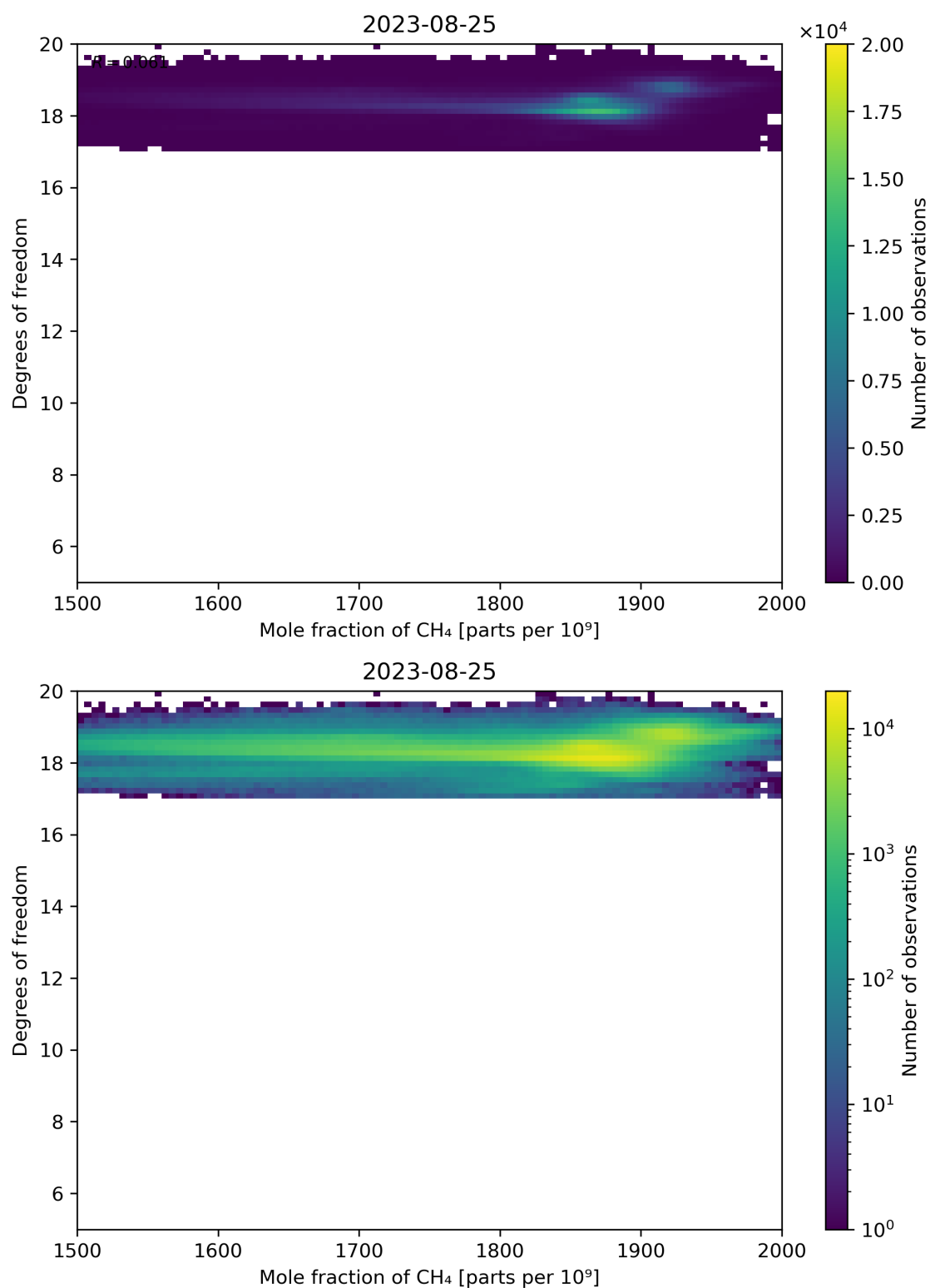
Figure 72: Scatter density plot of “Mole fraction of CH 4 ” against “Degrees of freedom” for 2023-08-25 to 2023-08-26.
