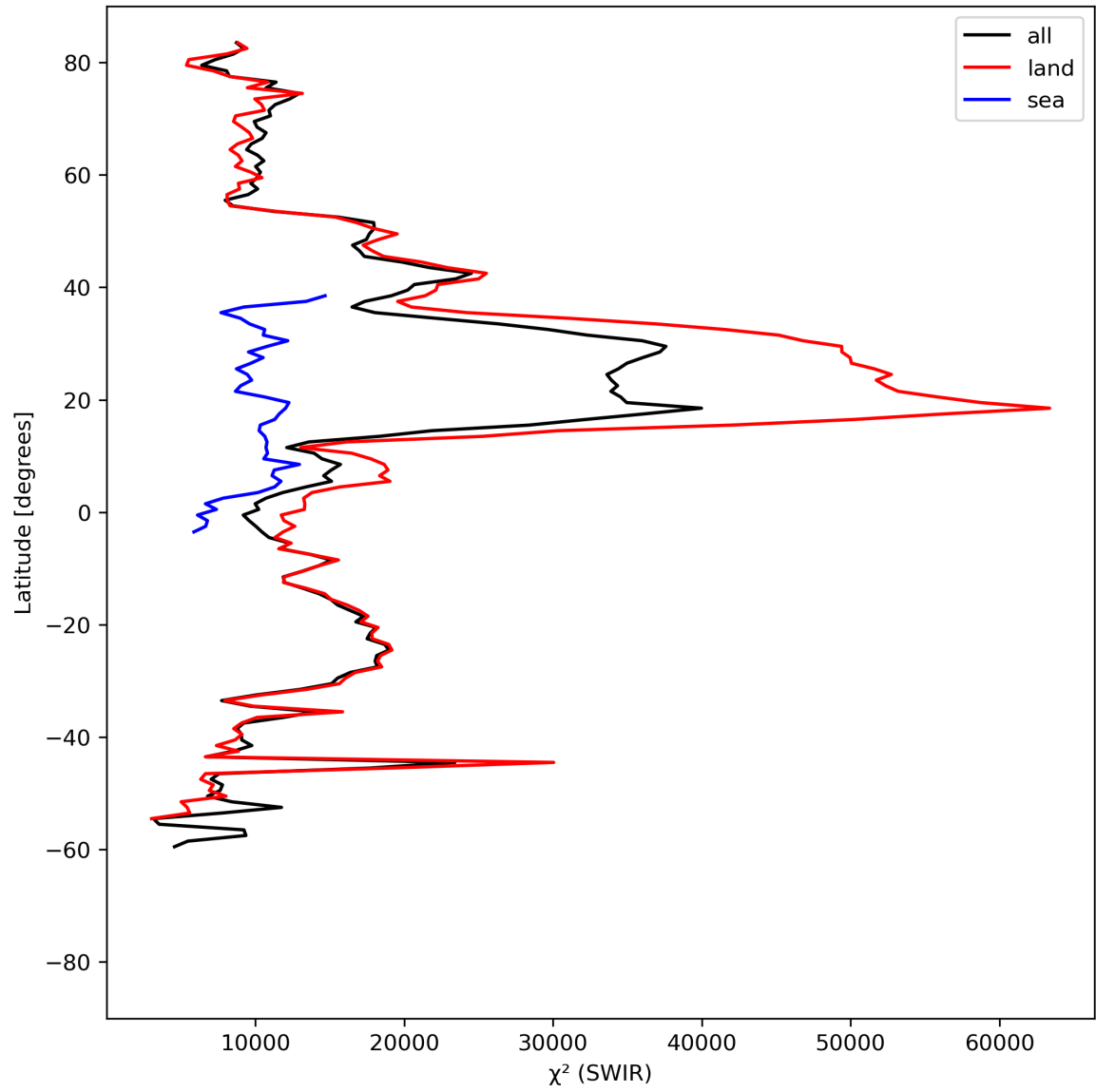
Figure 17: Zonal average of “ \chi^2 (SWIR)” for 2023-08-25 to 2023-08-26.
