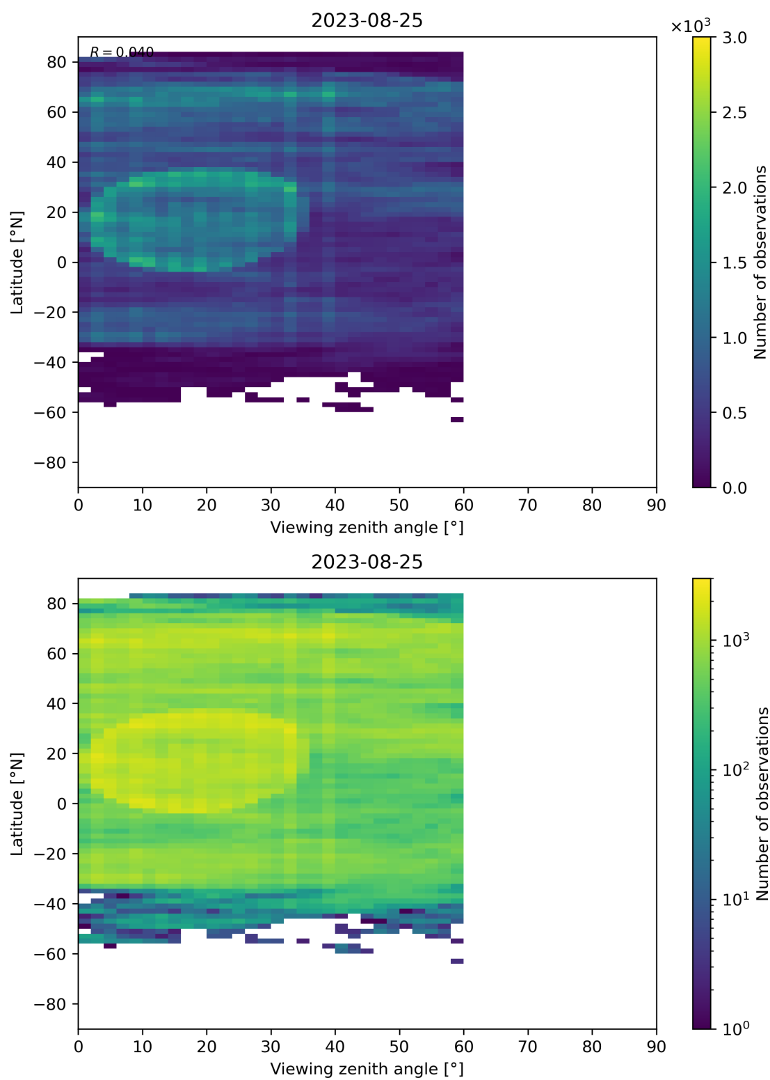
Figure 109: Scatter density plot of “Viewing zenith angle” against “Latitude” for 2023-08-25 to 2023-08-26.
