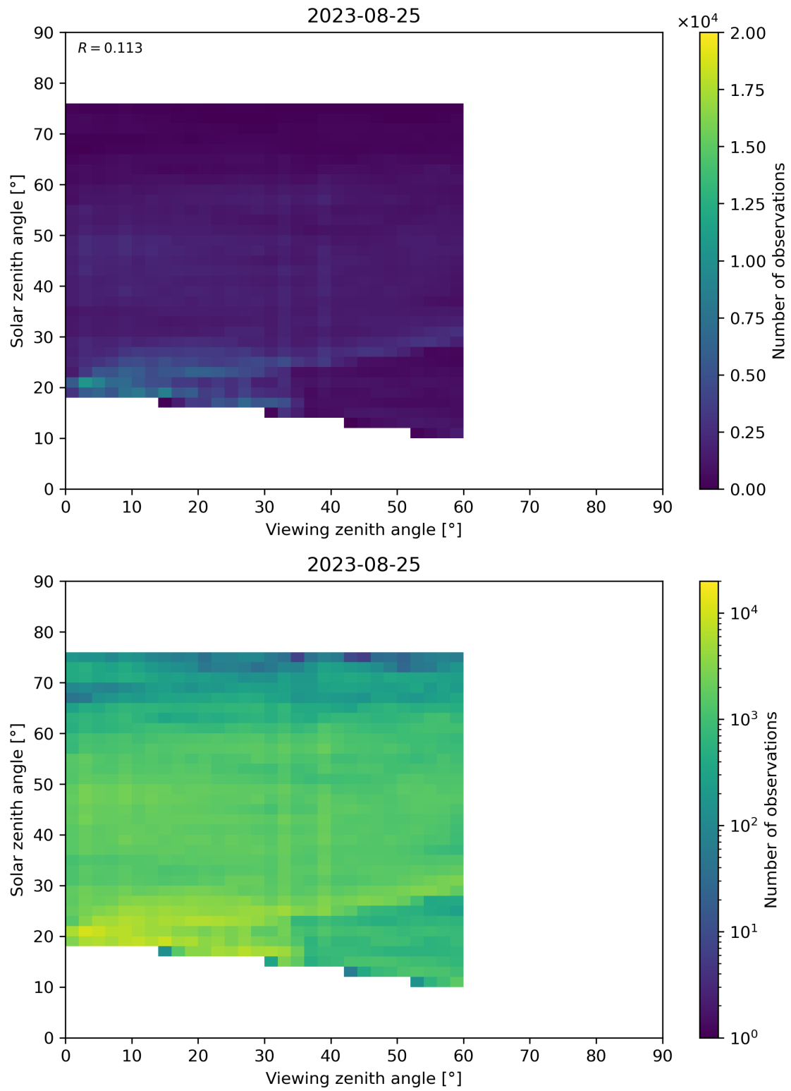
Figure 115: Scatter density plot of “Viewing zenith angle” against “Solar zenith angle” for 2023-08-25 to 2023-08-26.
