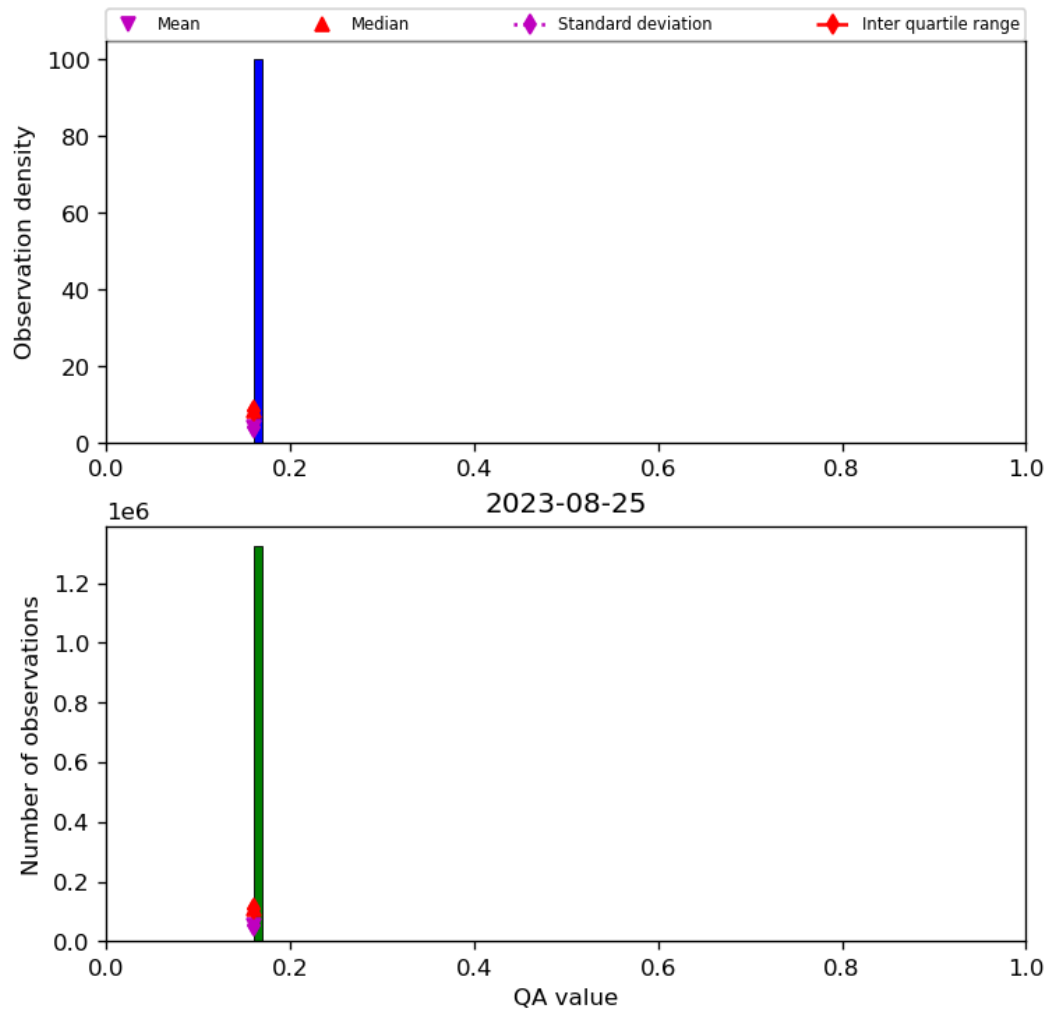
Figure 22: Histogram of “QA value” for 2023-08-25 to 2023-08-26
