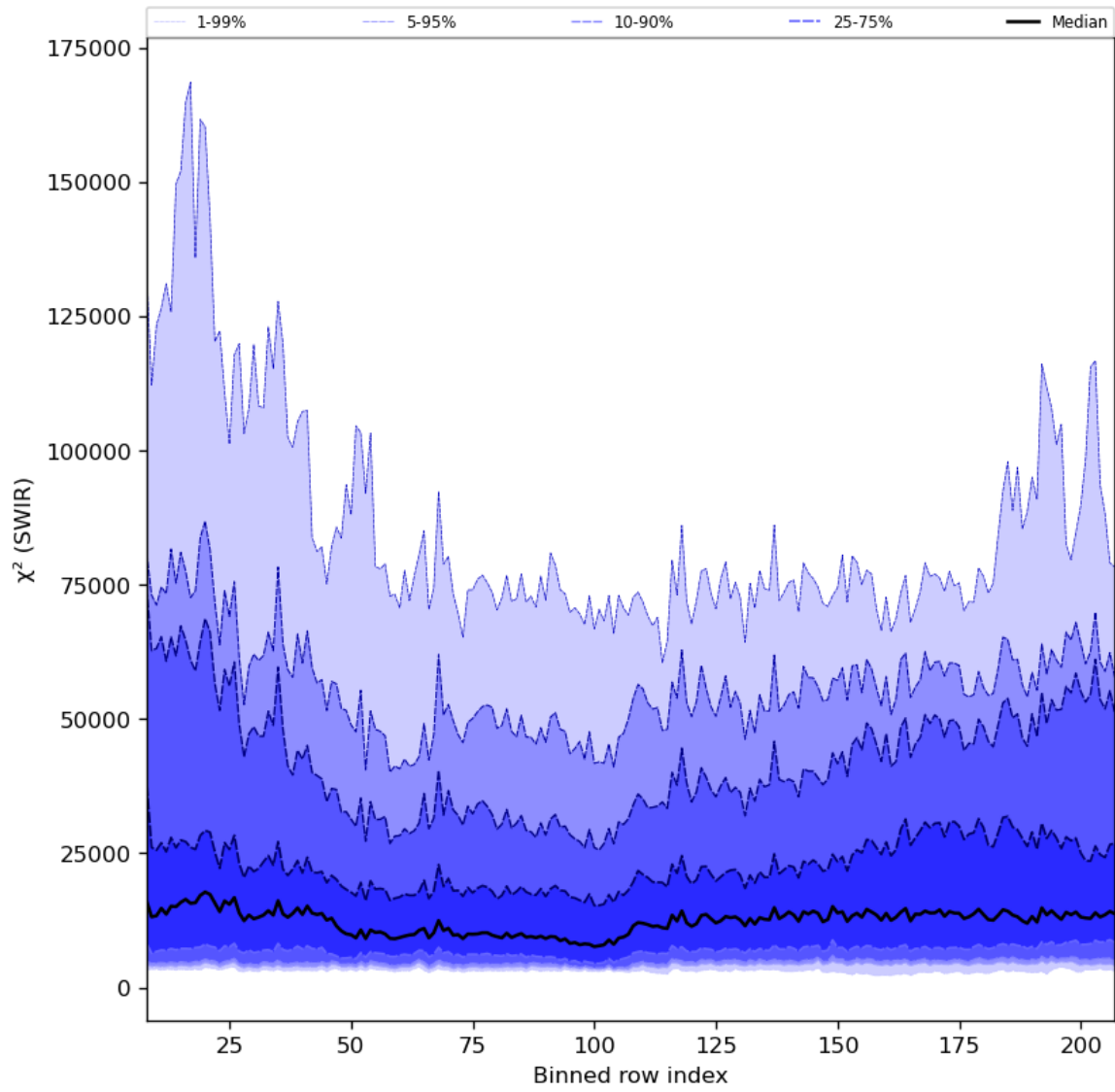
Figure 39: Along track statistics of “ \chi^2 (SWIR)” for 2023-08-25 to 2023-08-26
