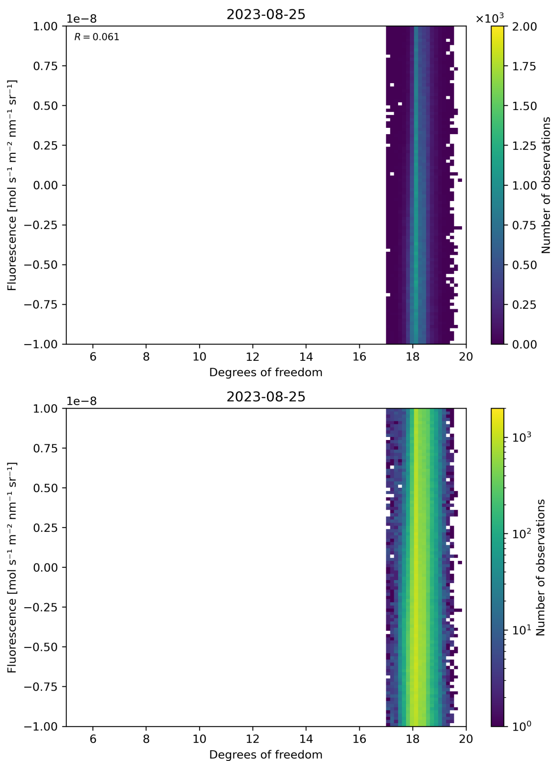
Figure 51: Scatter density plot of “Degrees of freedom” against “Fluorescence” for 2023-08-25 to 2023-08-26.
