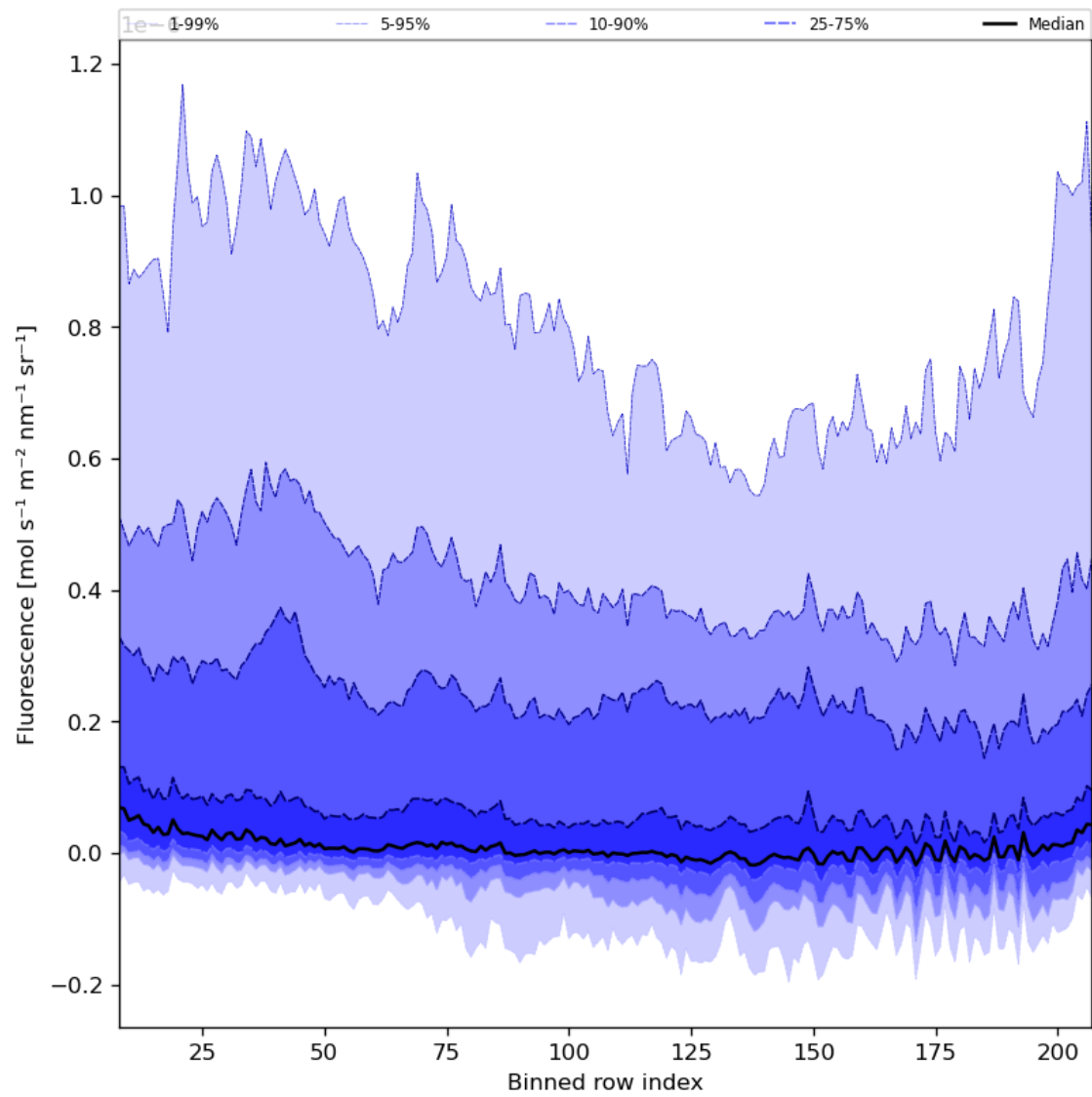
Figure 43: Along track statistics of “Fluorescence” for 2023-08-25 to 2023-08-26
