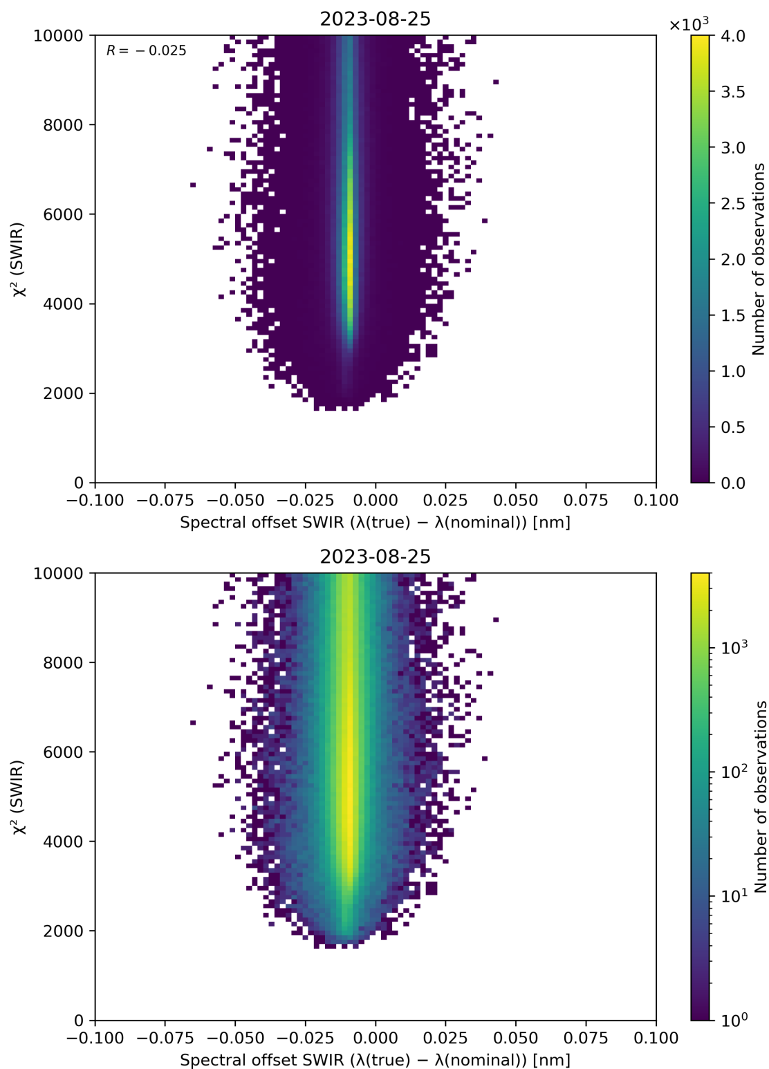
Figure 118: Scatter density plot of “Spectral offset SWIR ( \lambda(\text{true}) - \lambda(\text{nominal}) )” against “ \chi^2 (SWIR)” for 2023-08-25 to 2023-08-26.
