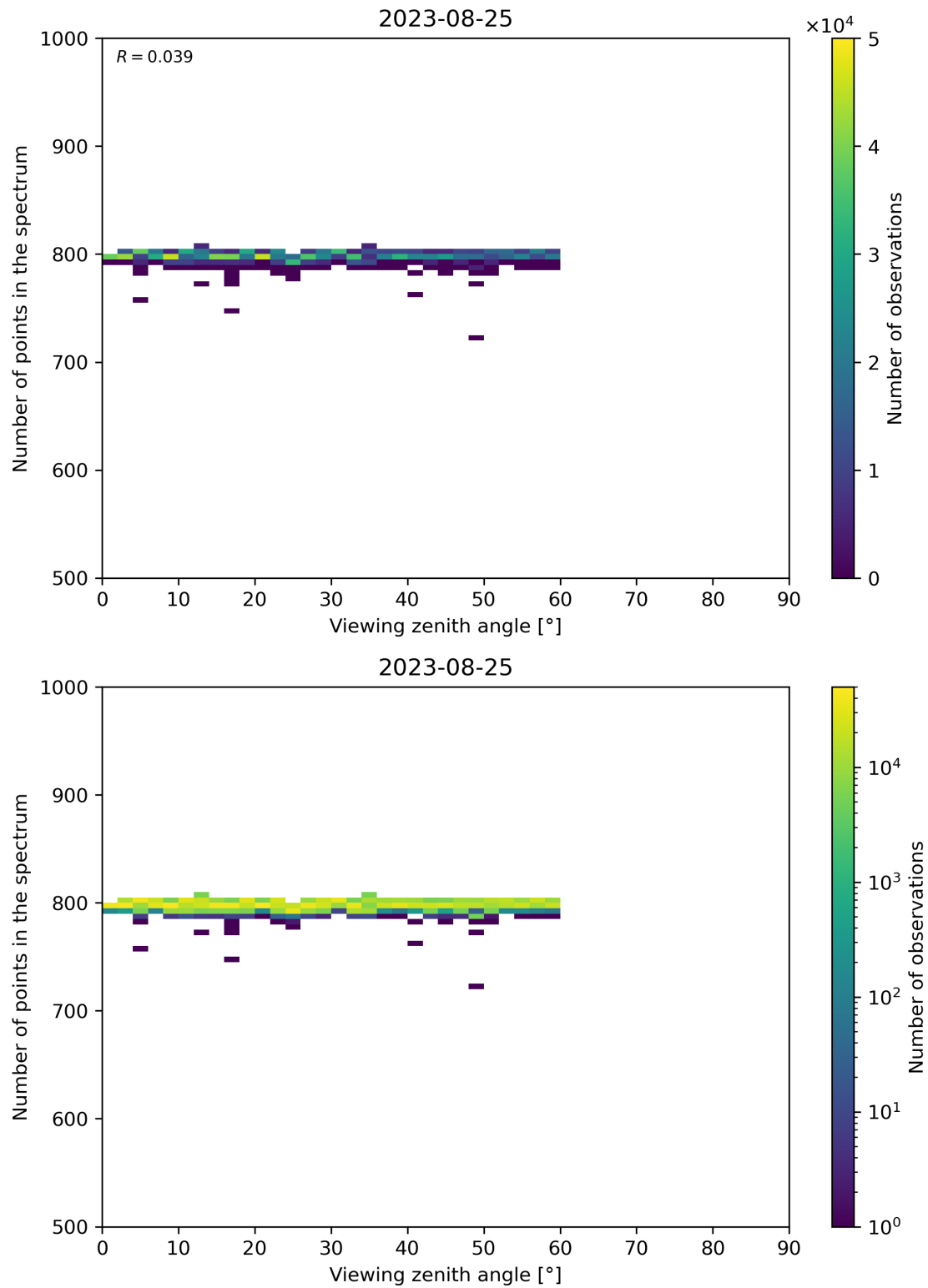
Figure 114: Scatter density plot of “Viewing zenith angle” against “Number of points in the spectrum” for 2023-08-25 to 2023-08-26.
