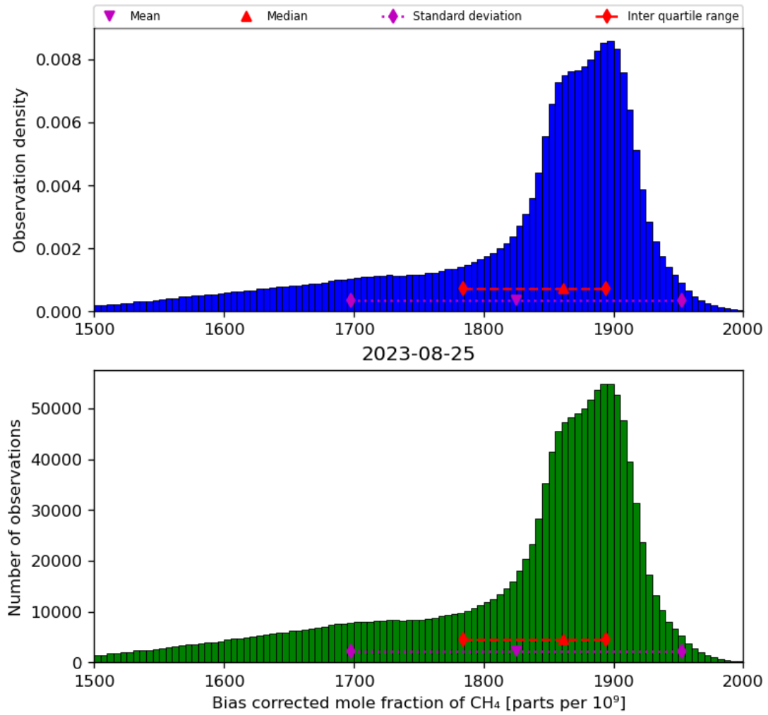
Figure 25: Histogram of “Bias corrected mole fraction of CH 4 ” for 2023-08-25 to 2023-08-26
