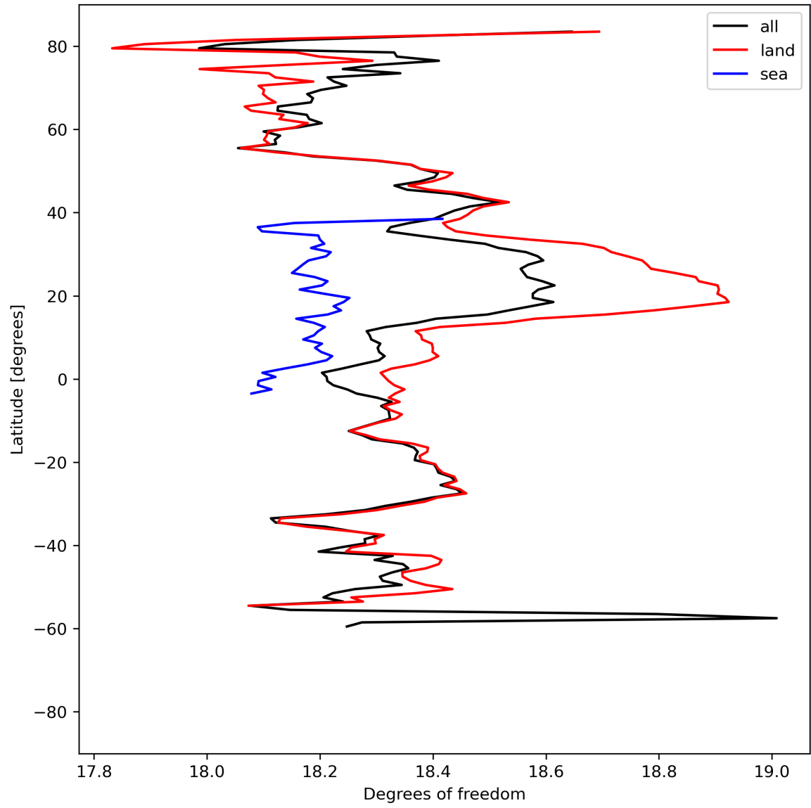
Figure 19: Zonal average of “Degrees of freedom” for 2023-08-25 to 2023-08-26.
