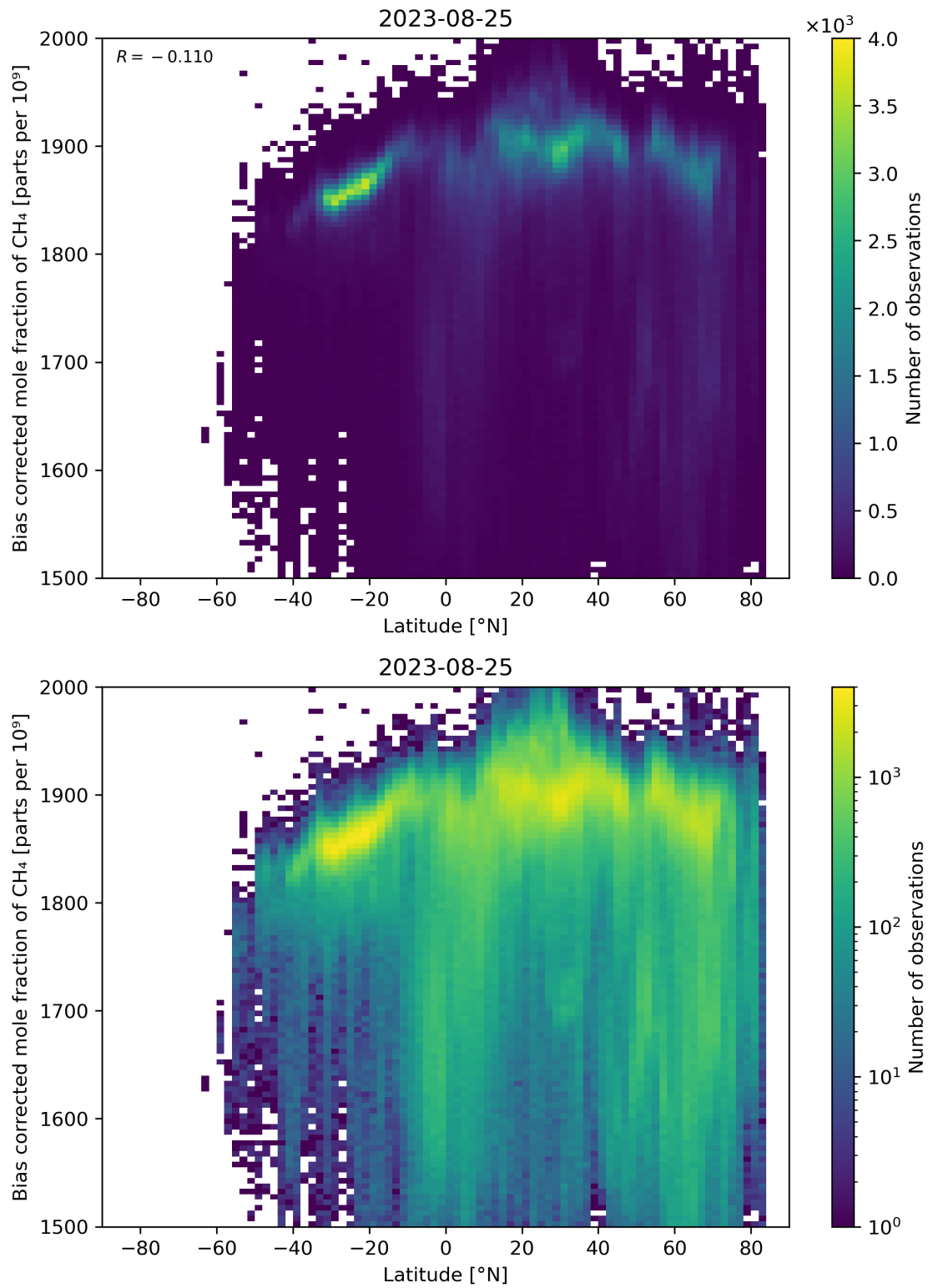
Figure 58: Scatter density plot of “Latitude” against “Bias corrected mole fraction of \text{CH}_4 ” for 2023-08-25 to 2023-08-26.
