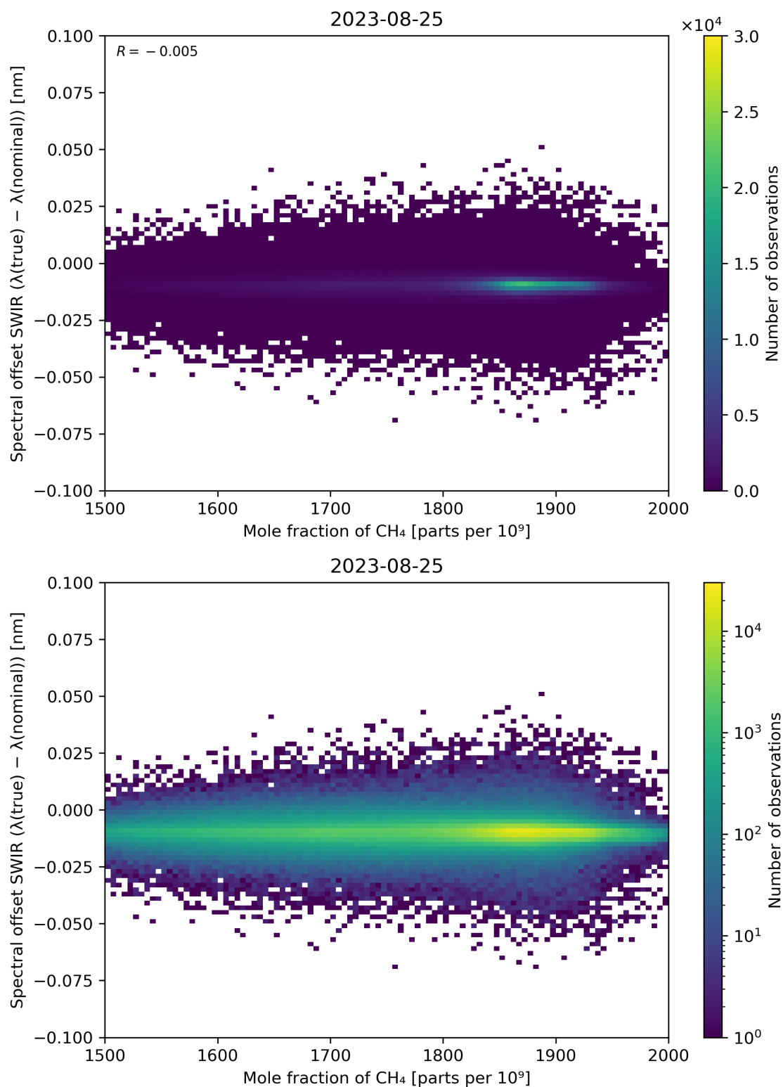
Figure 86: Scatter density plot of “Mole fraction of CH 4 ” against “Spectral offset SWIR ( \lambda(\text{true}) - \lambda(\text{nominal}) )” for 2023-08-25 to 2023-08-26.
