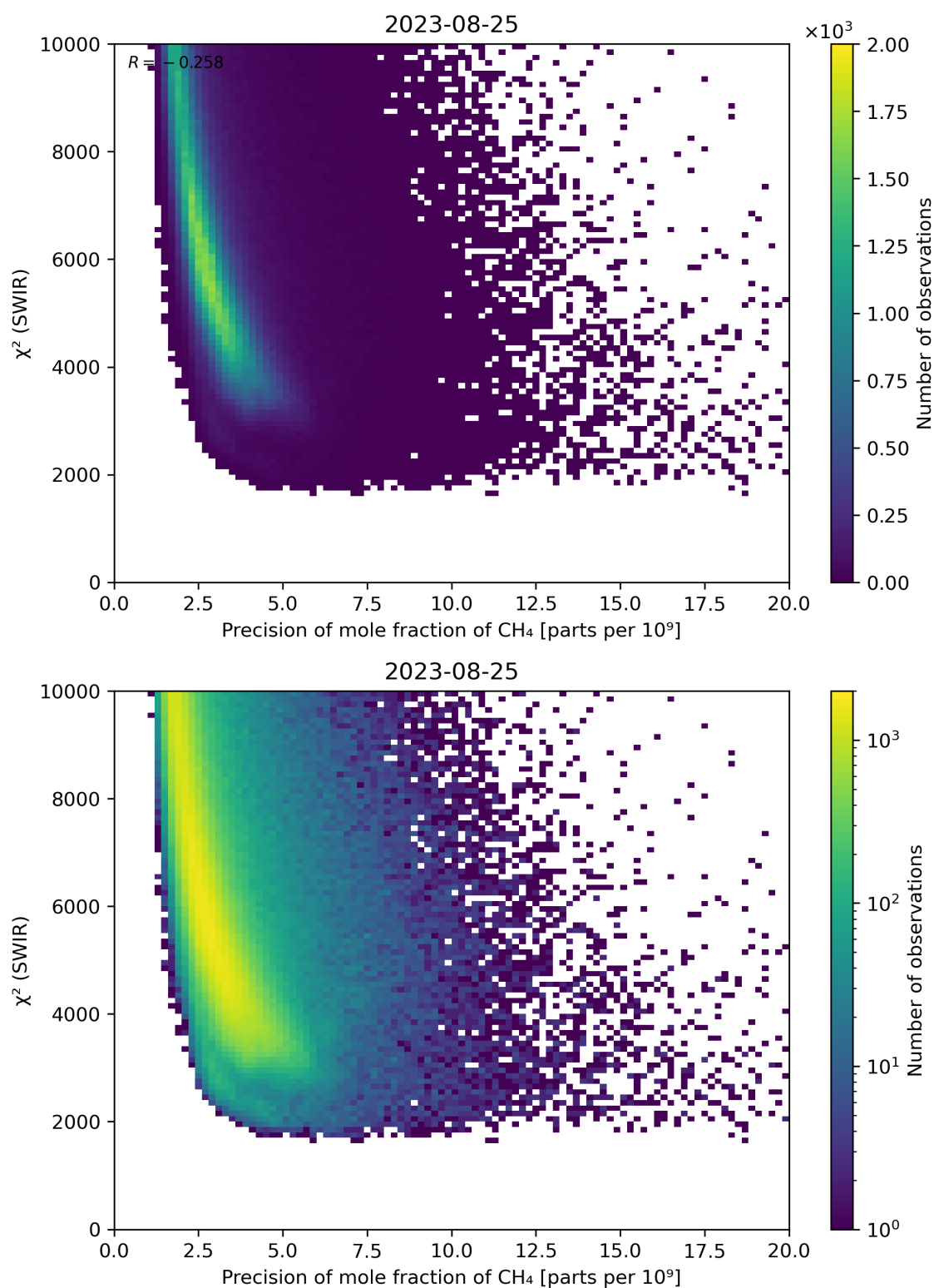
Figure 79: Scatter density plot of “Precision of mole fraction of \text{CH}_4 ” against “ \chi^2 (SWIR)” for 2023-08-25 to 2023-08-26.
