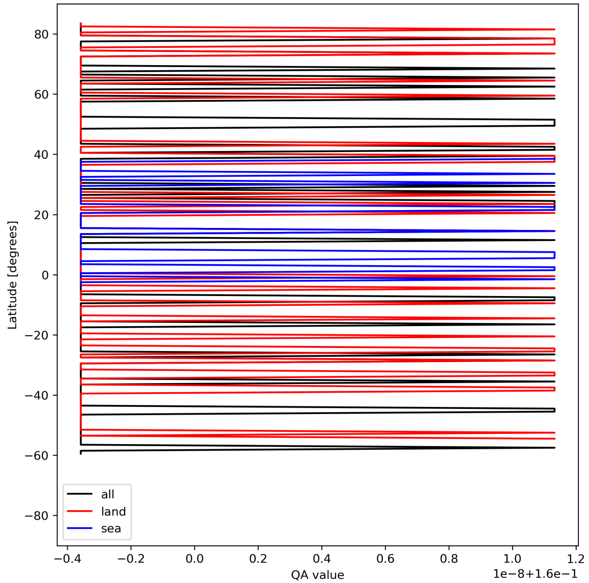
Figure 11: Zonal average of “QA value” for 2023-08-25 to 2023-08-26.
