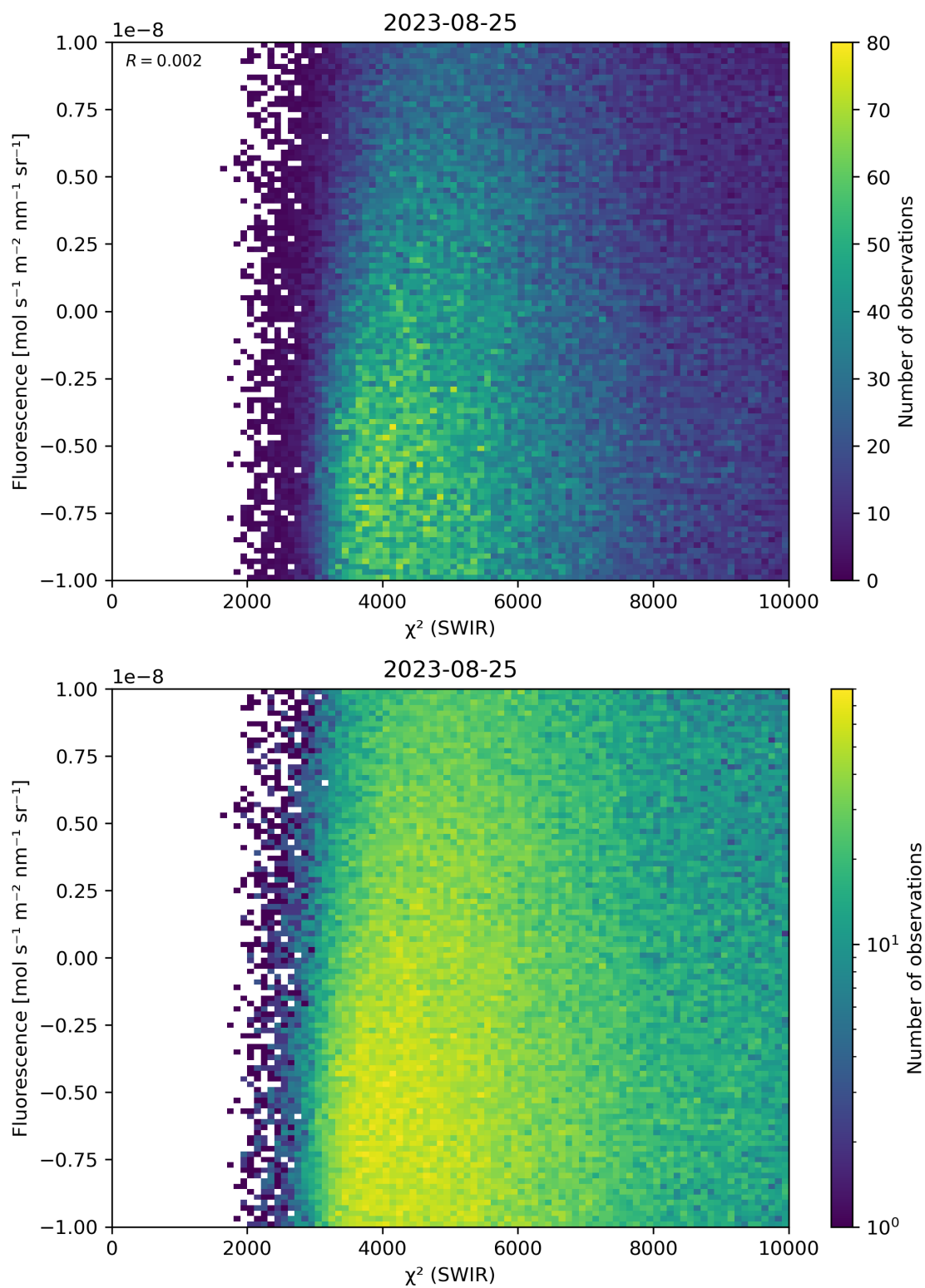
Figure 49: Scatter density plot of “ \chi^2 (SWIR)” against “Fluorescence” for 2023-08-25 to 2023-08-26.
