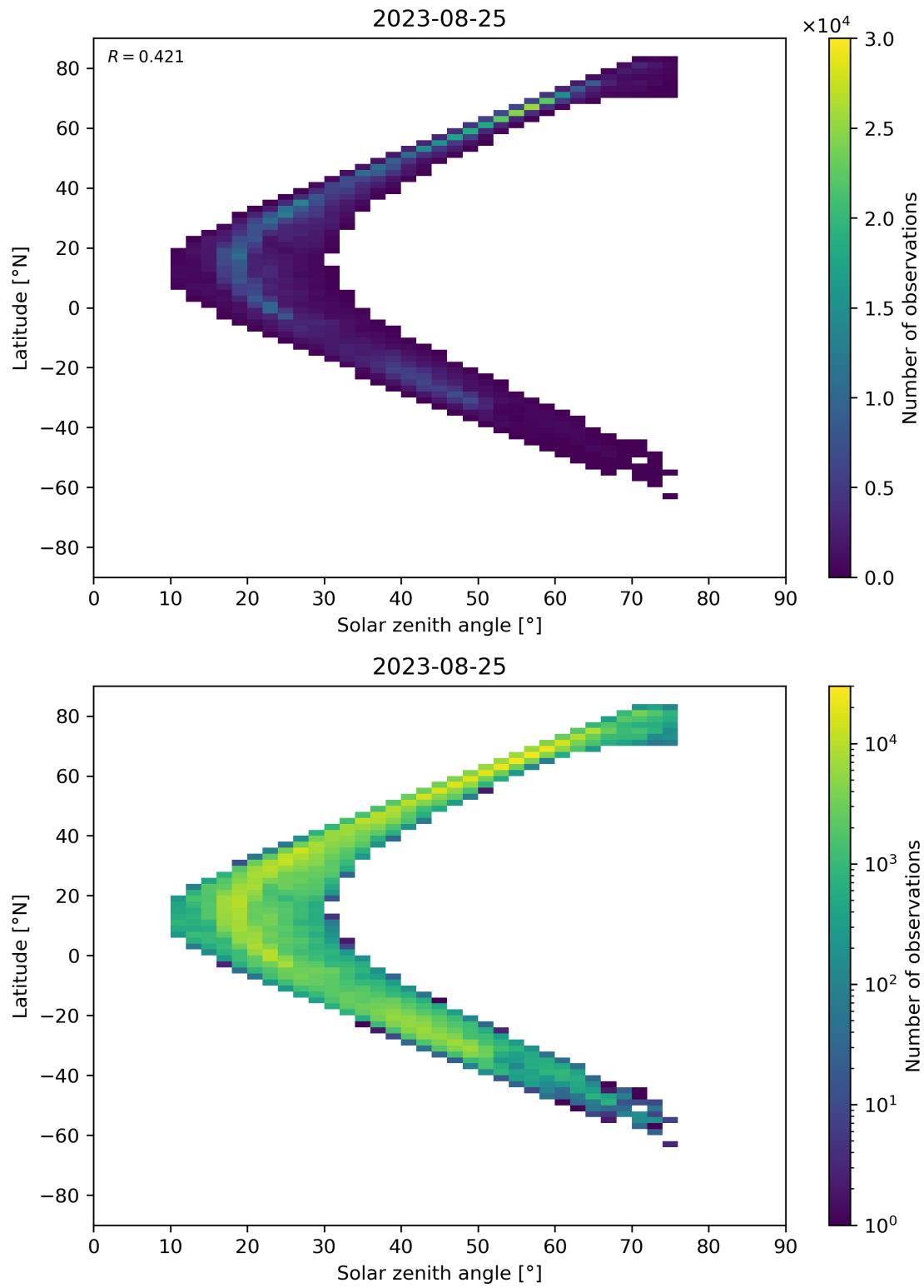
Figure 98: Scatter density plot of “Solar zenith angle” against “Latitude” for 2023-08-25 to 2023-08-26.
