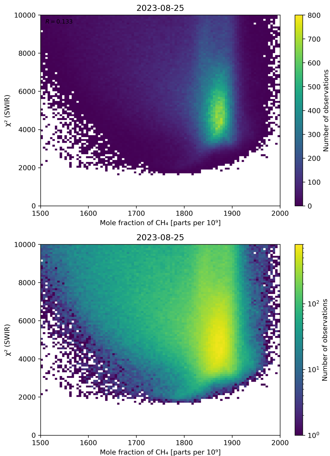
Figure 71: Scatter density plot of “Mole fraction of \text{CH}_4 ” against “ \chi^2 (SWIR)” for 2023-08-25 to 2023-08-26.
