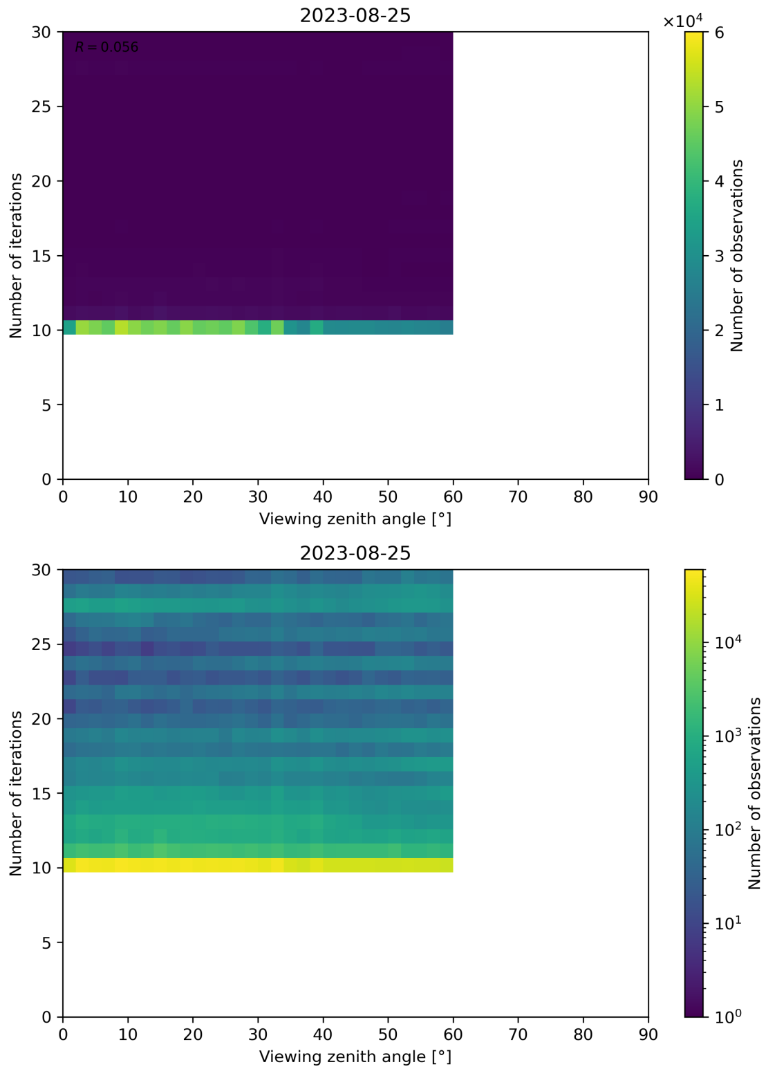
Figure 113: Scatter density plot of “Viewing zenith angle” against “Number of iterations” for 2023-08-25 to 2023-08-26.
