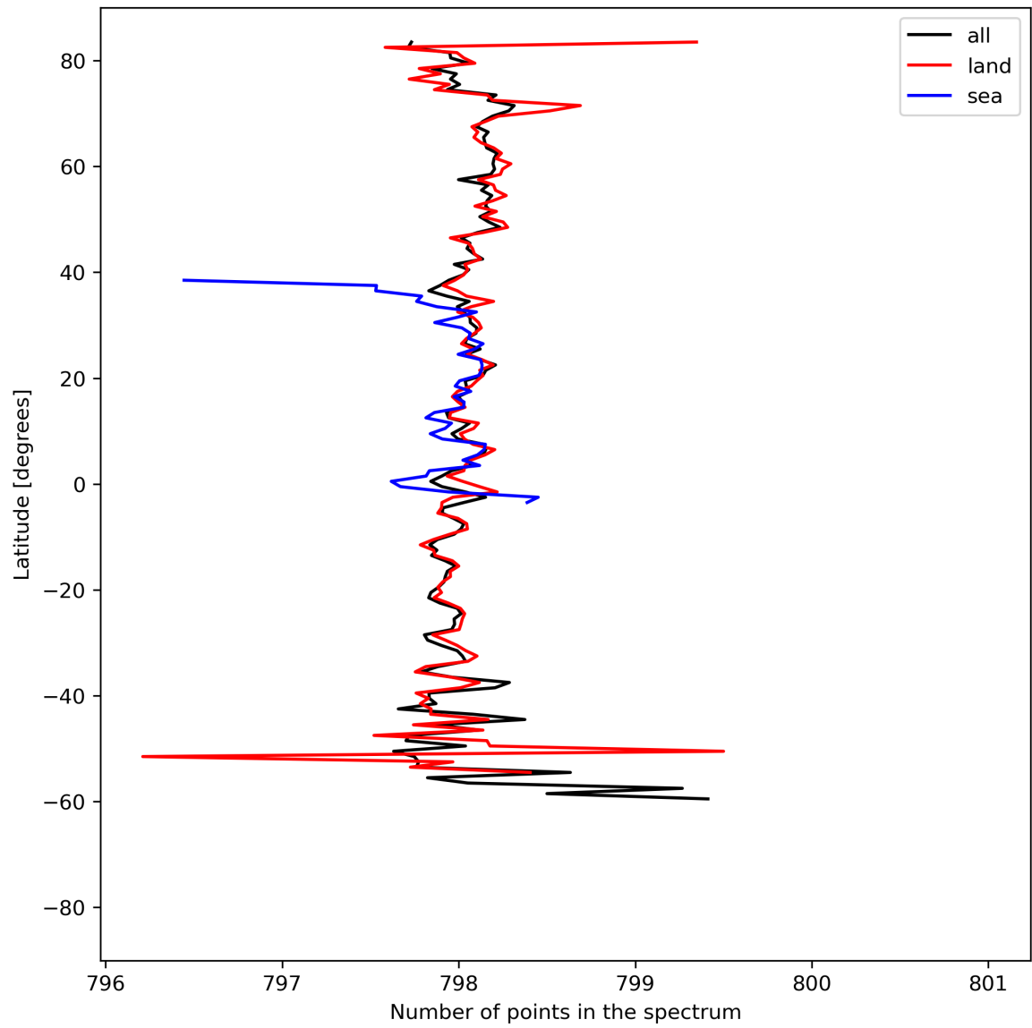
Figure 15: Zonal average of “Number of points in the spectrum” for 2023-08-25 to 2023-08-26.
