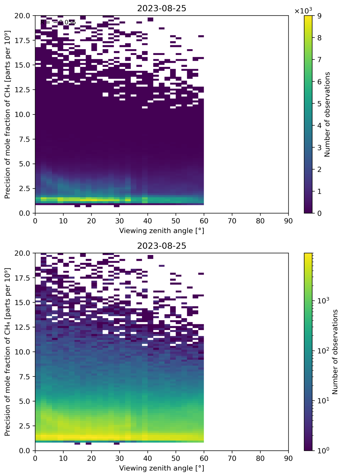
Figure 112: Scatter density plot of “Viewing zenith angle” against “Precision of mole fraction of CH 4 ” for 2023-08-25 to 2023-08-26.
