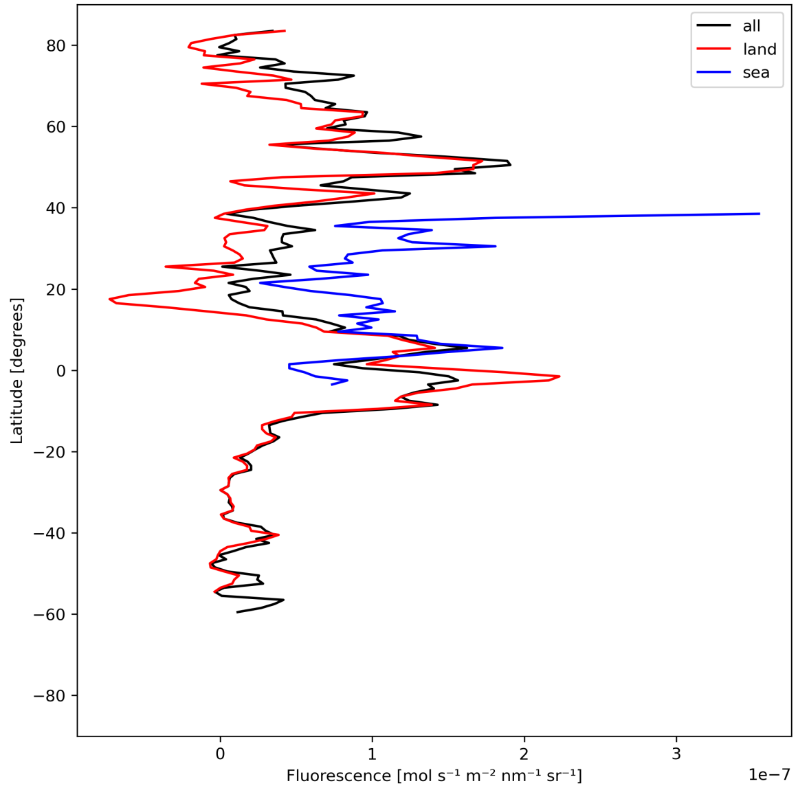
Figure 21: Zonal average of “Fluorescence” for 2023-08-25 to 2023-08-26.
