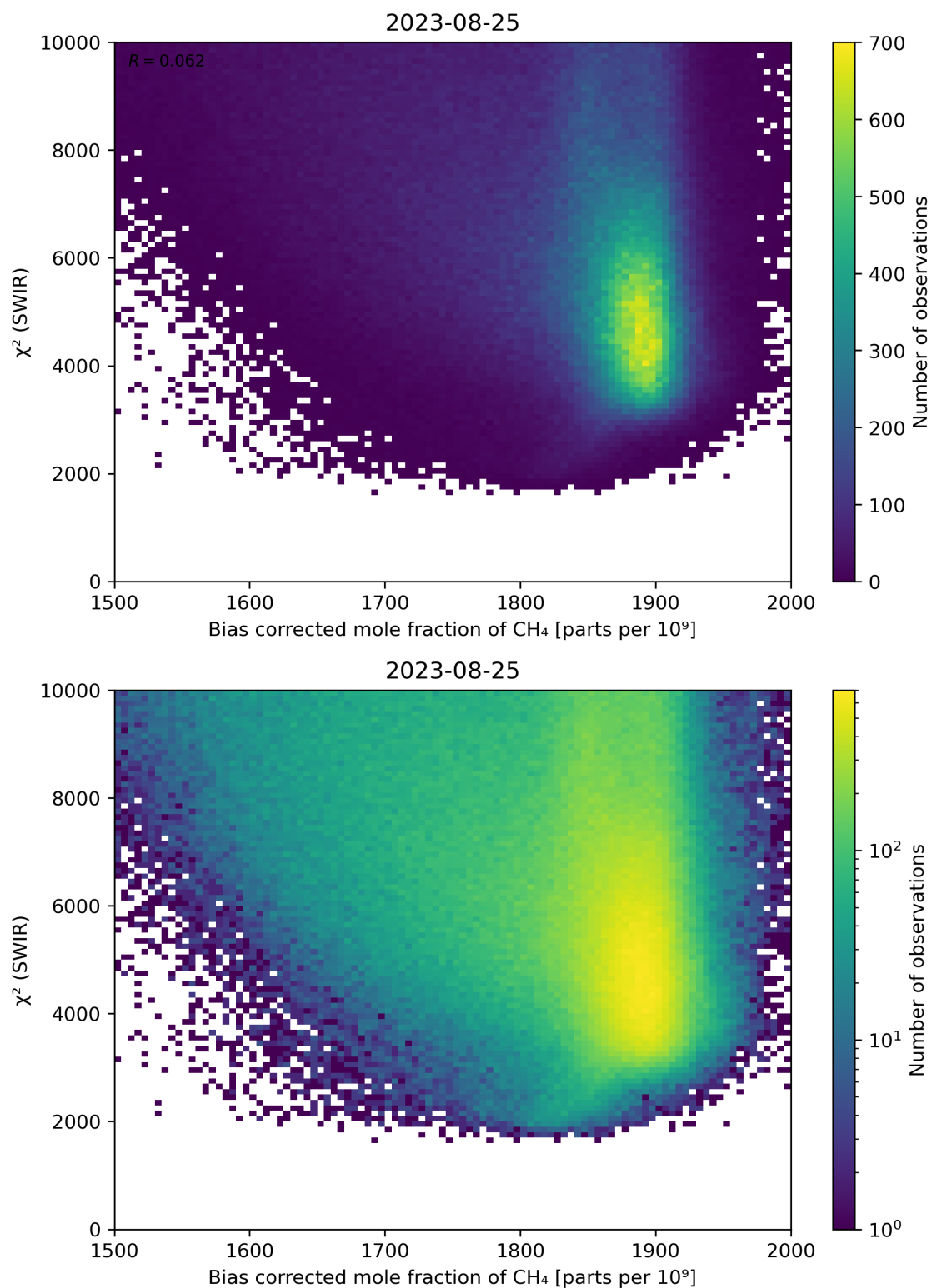
Figure 64: Scatter density plot of “Bias corrected mole fraction of CH 4 ” against “ \chi^2 (SWIR)” for 2023-08-25 to 2023-08-26.
