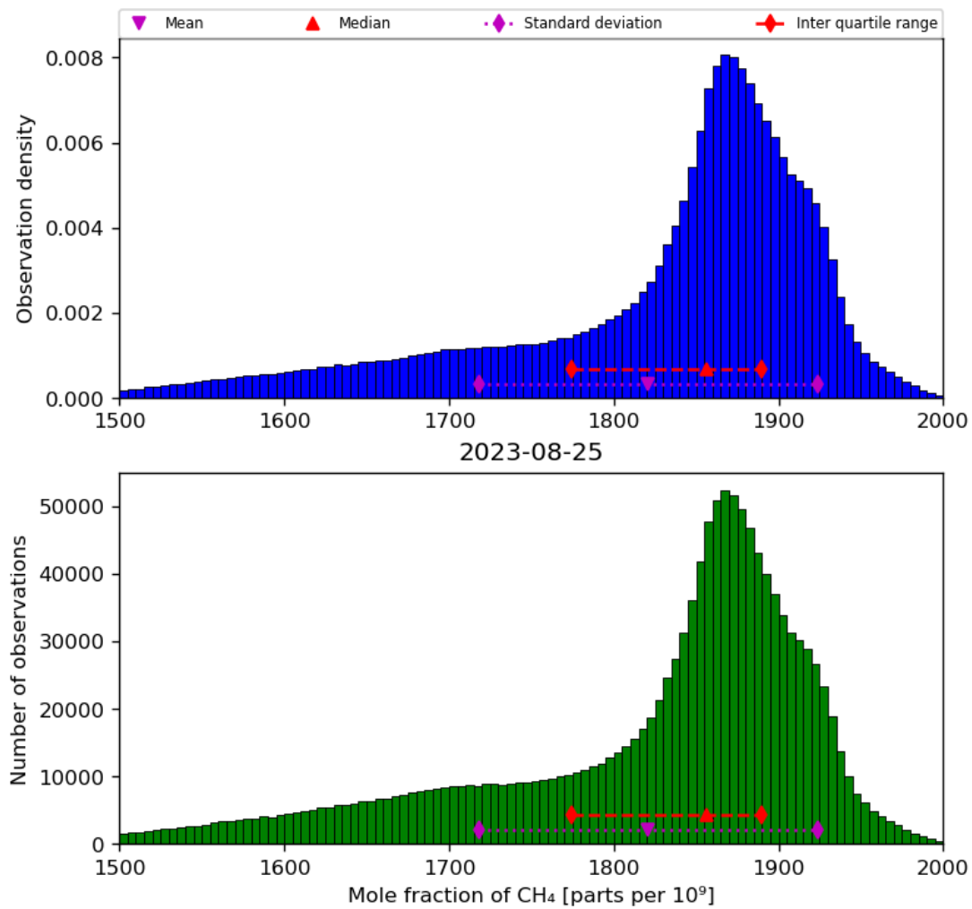
Figure 23: Histogram of “Mole fraction of CH 4 ” for 2023-08-25 to 2023-08-26
