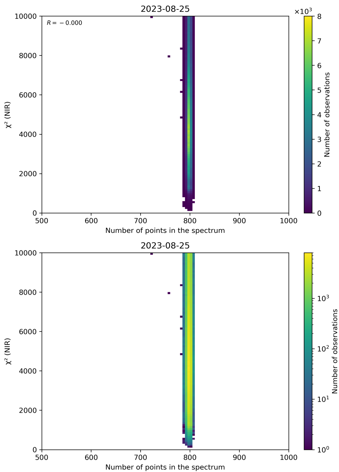
Figure 88: Scatter density plot of “Number of points in the spectrum” against “ \chi^2 (NIR)” for 2023-08-25 to 2023-08-26.
