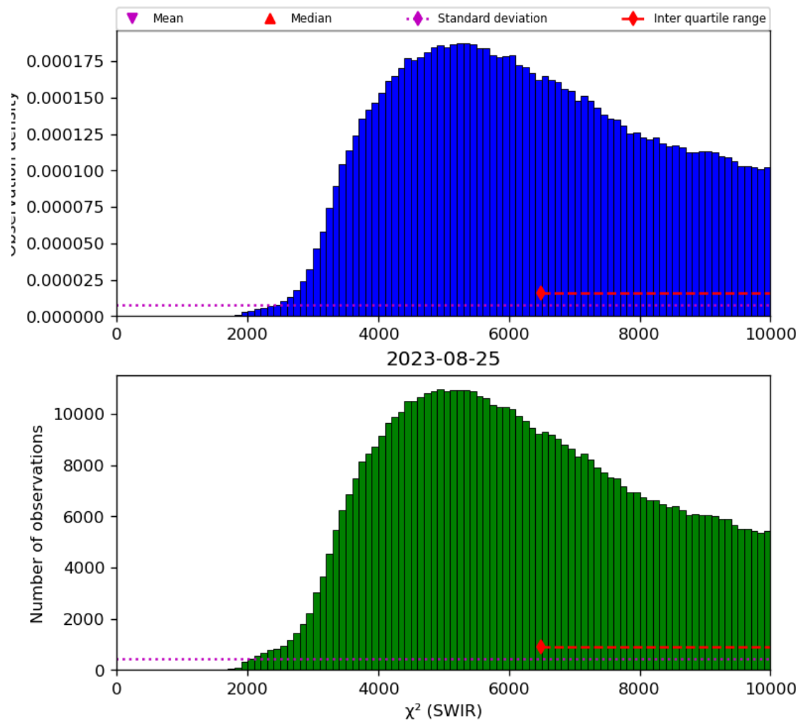
Figure 28: Histogram of “ \chi^2 (SWIR)” for 2023-08-25 to 2023-08-26
