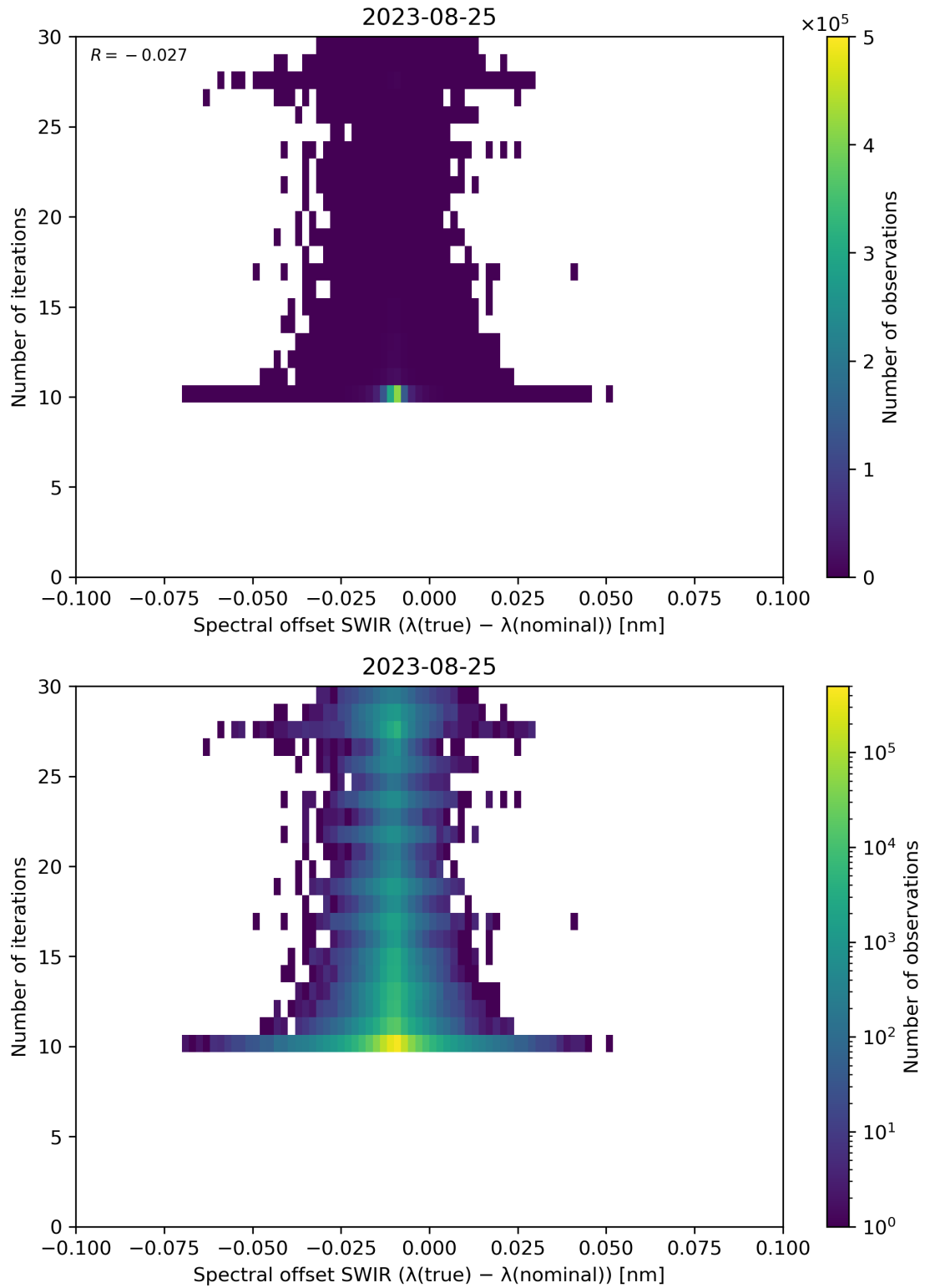
Figure 121: Scatter density plot of “Spectral offset SWIR ( \lambda(\text{true}) - \lambda(\text{nominal}) )” against “Number of iterations” for 2023-08-25 to 2023-08-26.
