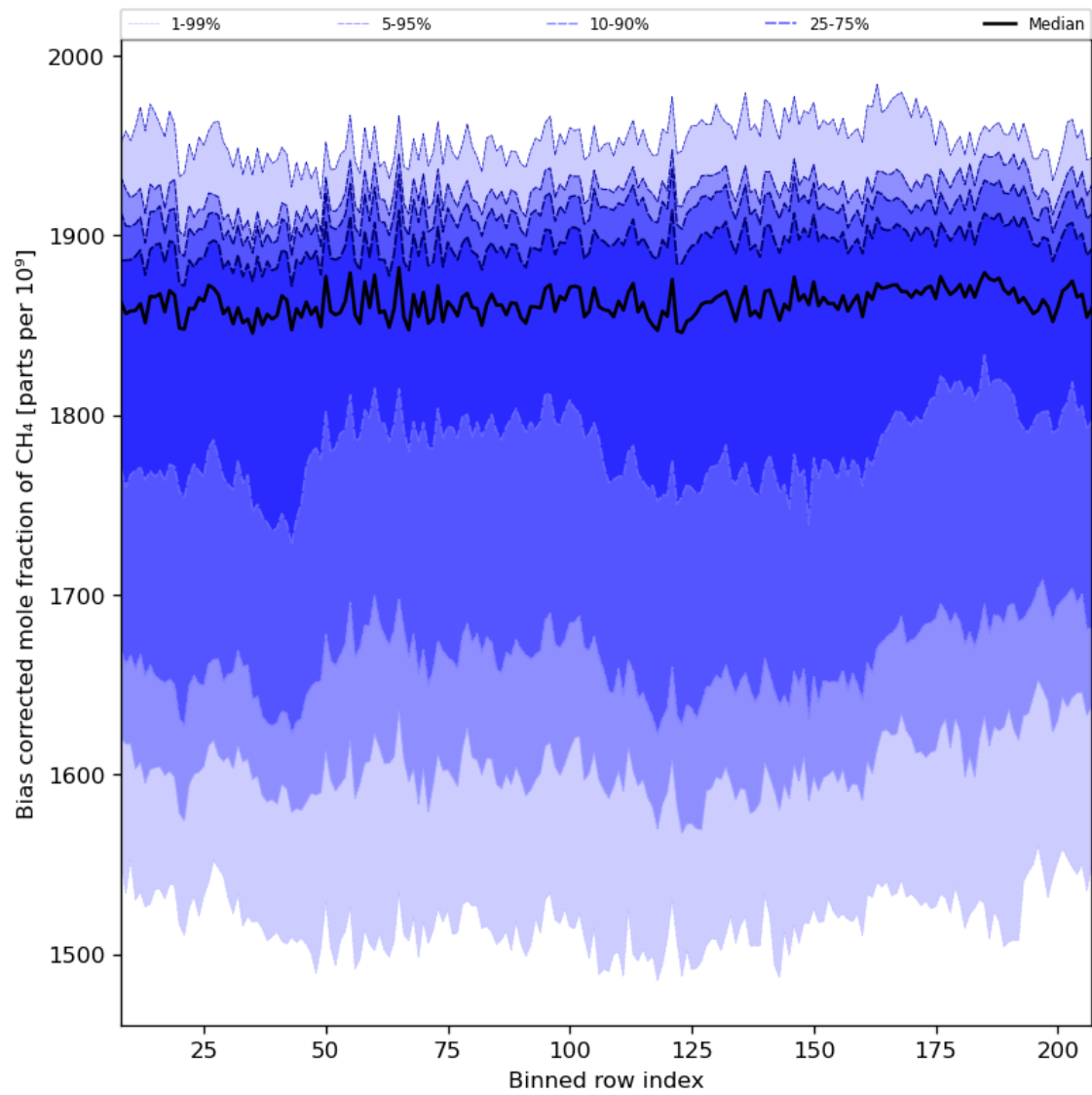
Figure 36: Along track statistics of “Bias corrected mole fraction of CH 4 ” for 2023-08-25 to 2023-08-26
