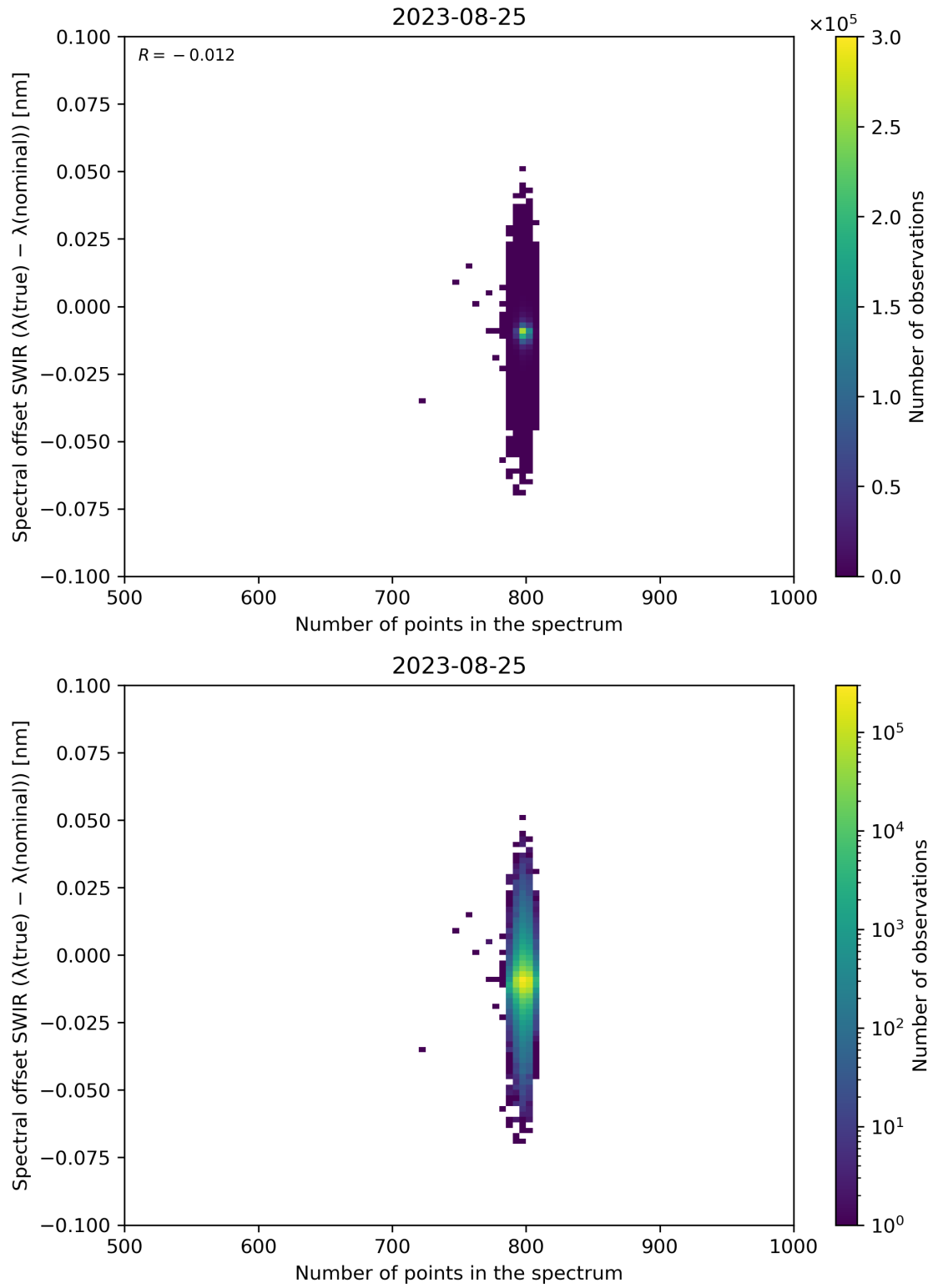
Figure 93: Scatter density plot of “Number of points in the spectrum” against “Spectral offset SWIR ( \lambda(\text{true}) - \lambda(\text{nominal}) )” for 2023-08-25 to 2023-08-26.
