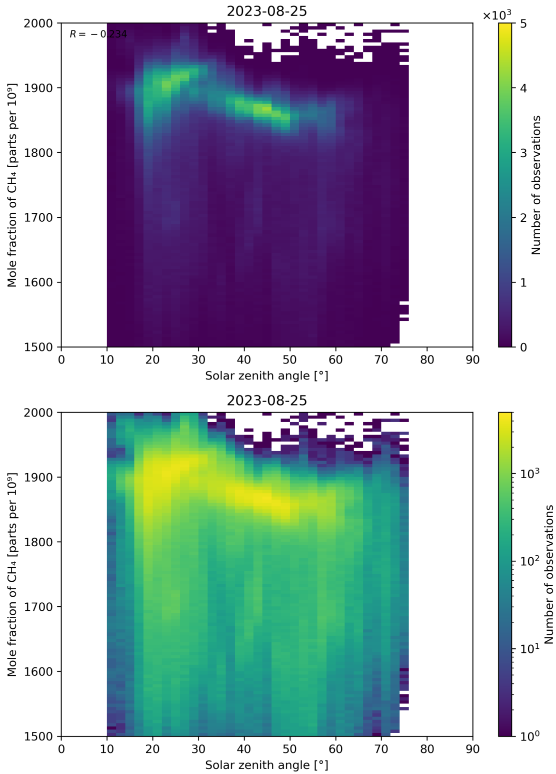
Figure 99: Scatter density plot of “Solar zenith angle” against “Mole fraction of CH 4 ” for 2023-08-25 to 2023-08-26.
