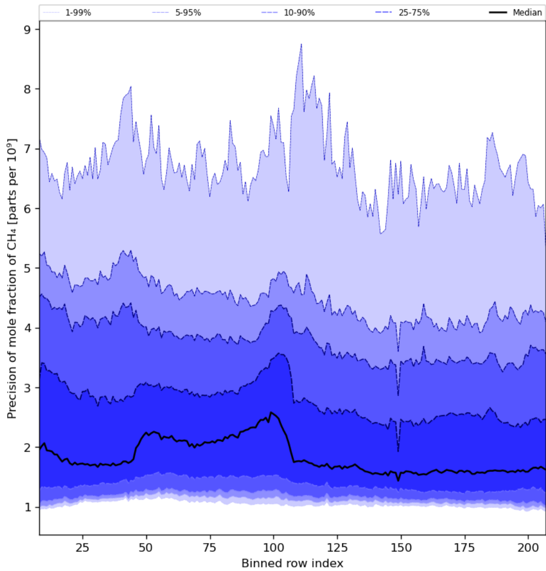
Figure 35: Along track statistics of “Precision of mole fraction of CH 4 ” for 2023-08-25 to 2023-08-26
