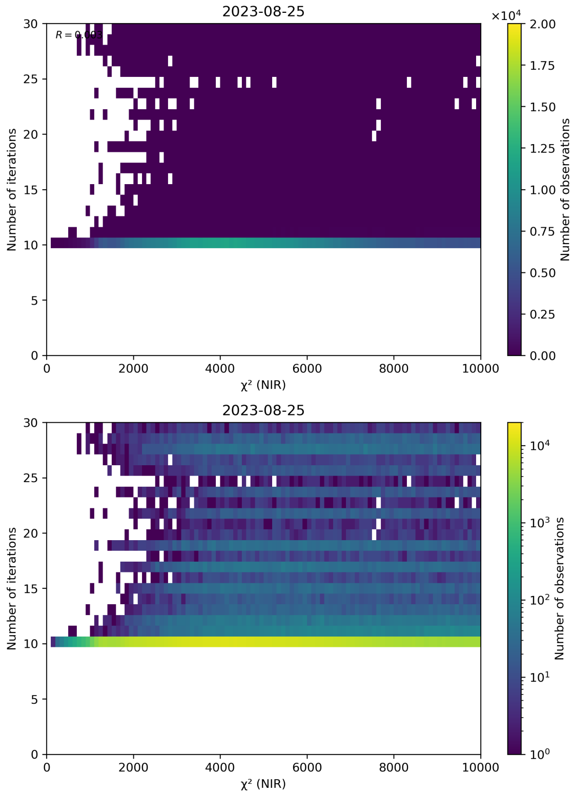
Figure 46: Scatter density plot of “ \chi^2 (NIR)” against “Number of iterations” for 2023-08-25 to 2023-08-26.
