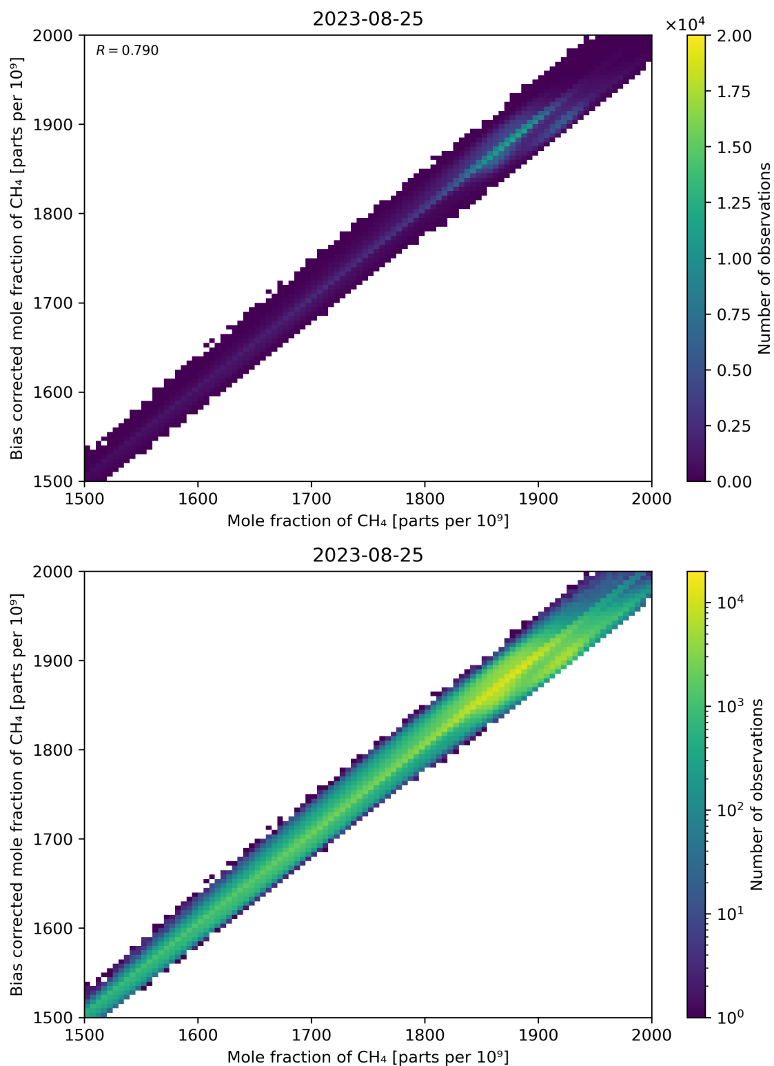
Figure 74: Scatter density plot of “Mole fraction of CH 4 ” against “Bias corrected mole fraction of CH 4 ” for 2023-08-25 to 2023-08-26.
