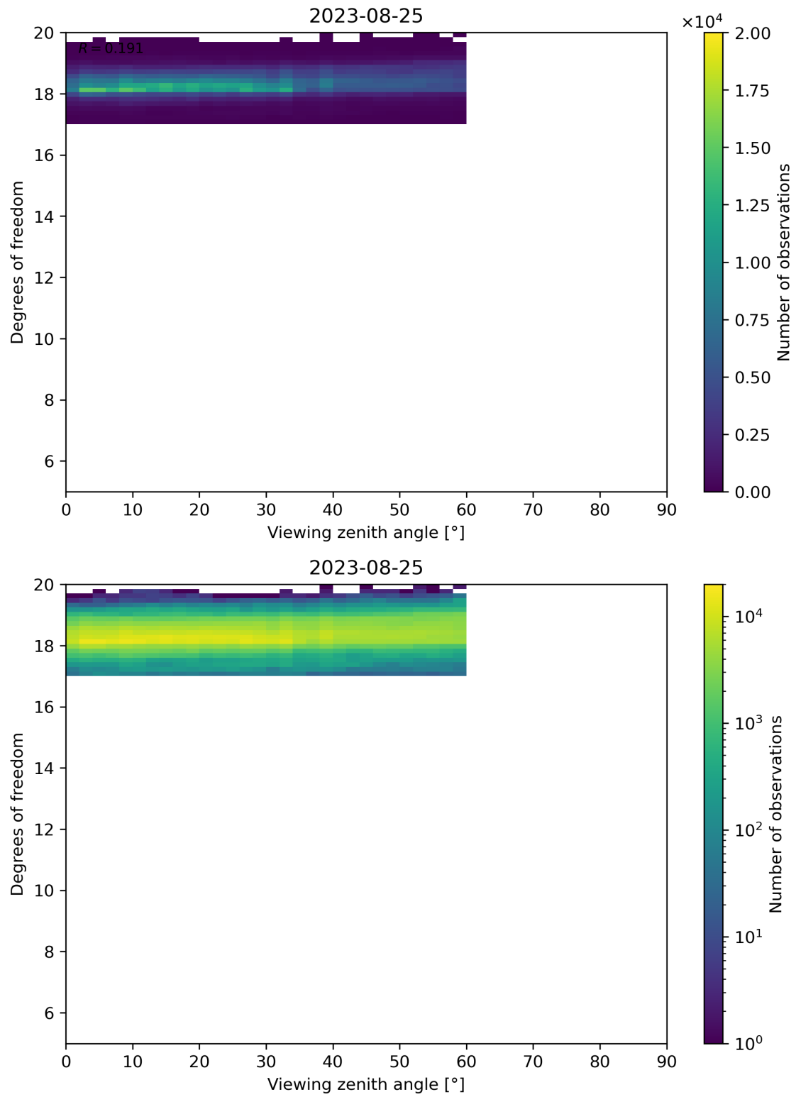
Figure 107: Scatter density plot of “Viewing zenith angle” against “Degrees of freedom” for 2023-08-25 to 2023-08-26.
