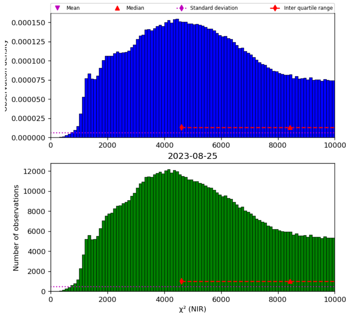
Figure 29: Histogram of “ \chi^2 (NIR)” for 2023-08-25 to 2023-08-26
