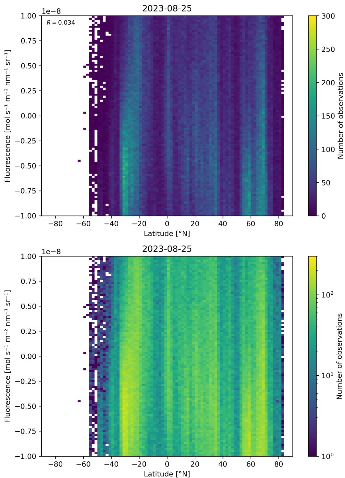
Figure 56: Scatter density plot of “Latitude” against “Fluorescence” for 2023-08-25 to 2023-08-26.
