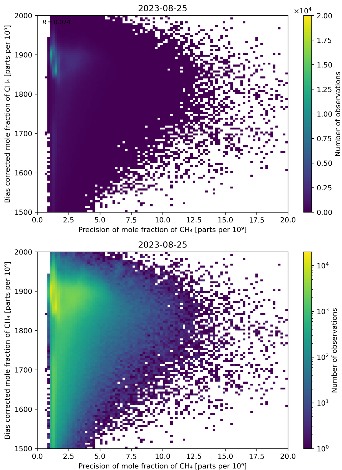
Figure 82: Scatter density plot of “Precision of mole fraction of \text{CH}_4 ” against “Bias corrected mole fraction of \text{CH}_4 ” for 2023-08-25 to 2023-08-26.
