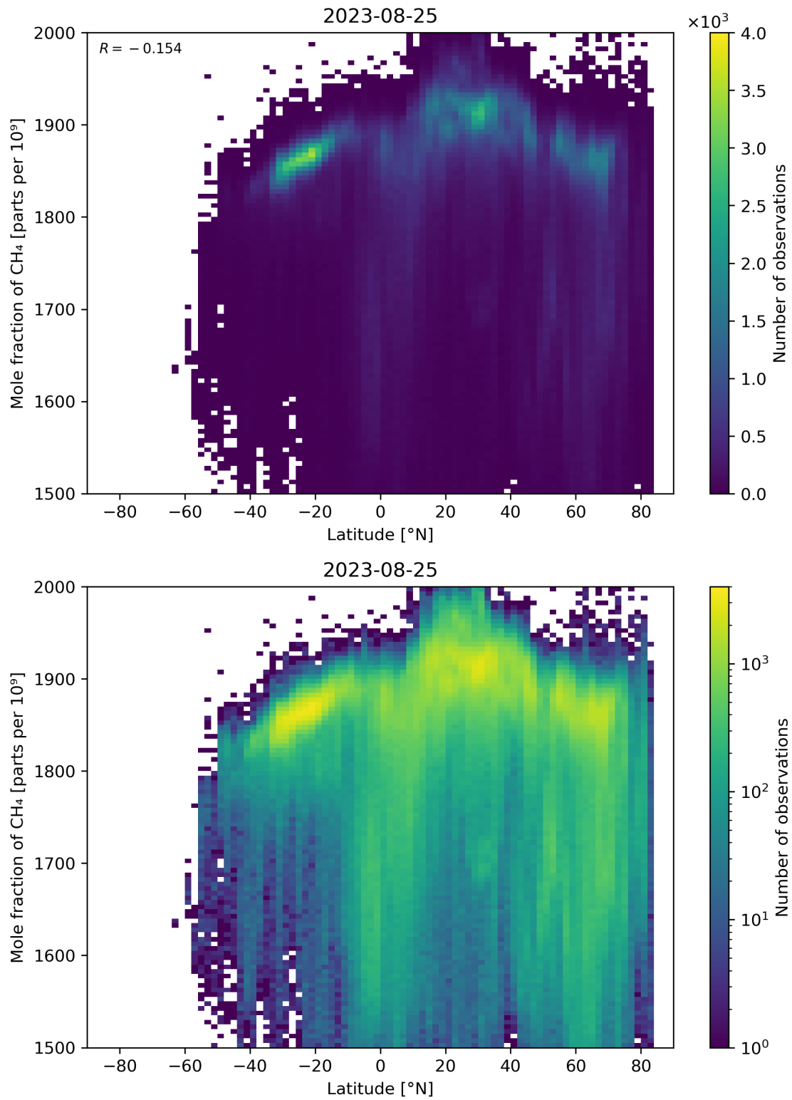
Figure 57: Scatter density plot of “Latitude” against “Mole fraction of CH 4 ” for 2023-08-25 to 2023-08-26.
