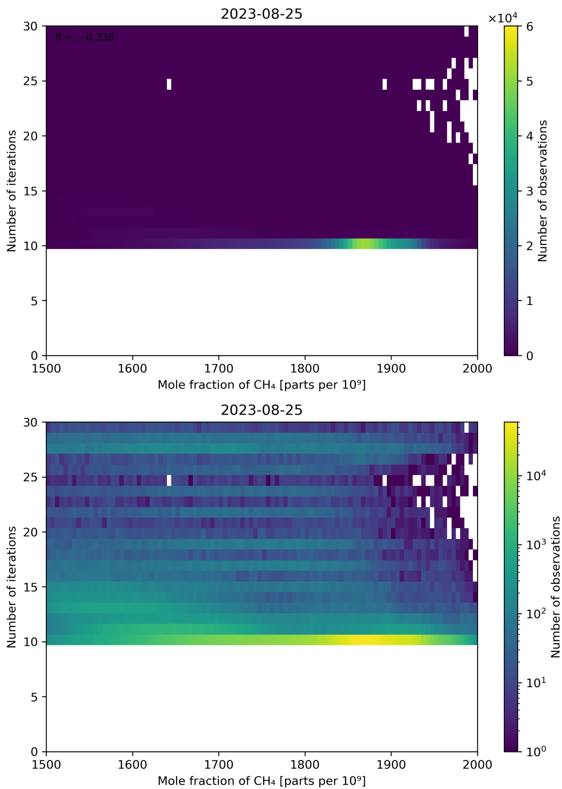
Figure 76: Scatter density plot of “Mole fraction of CH 4 ” against “Number of iterations” for 2023-08-25 to 2023-08-26.
