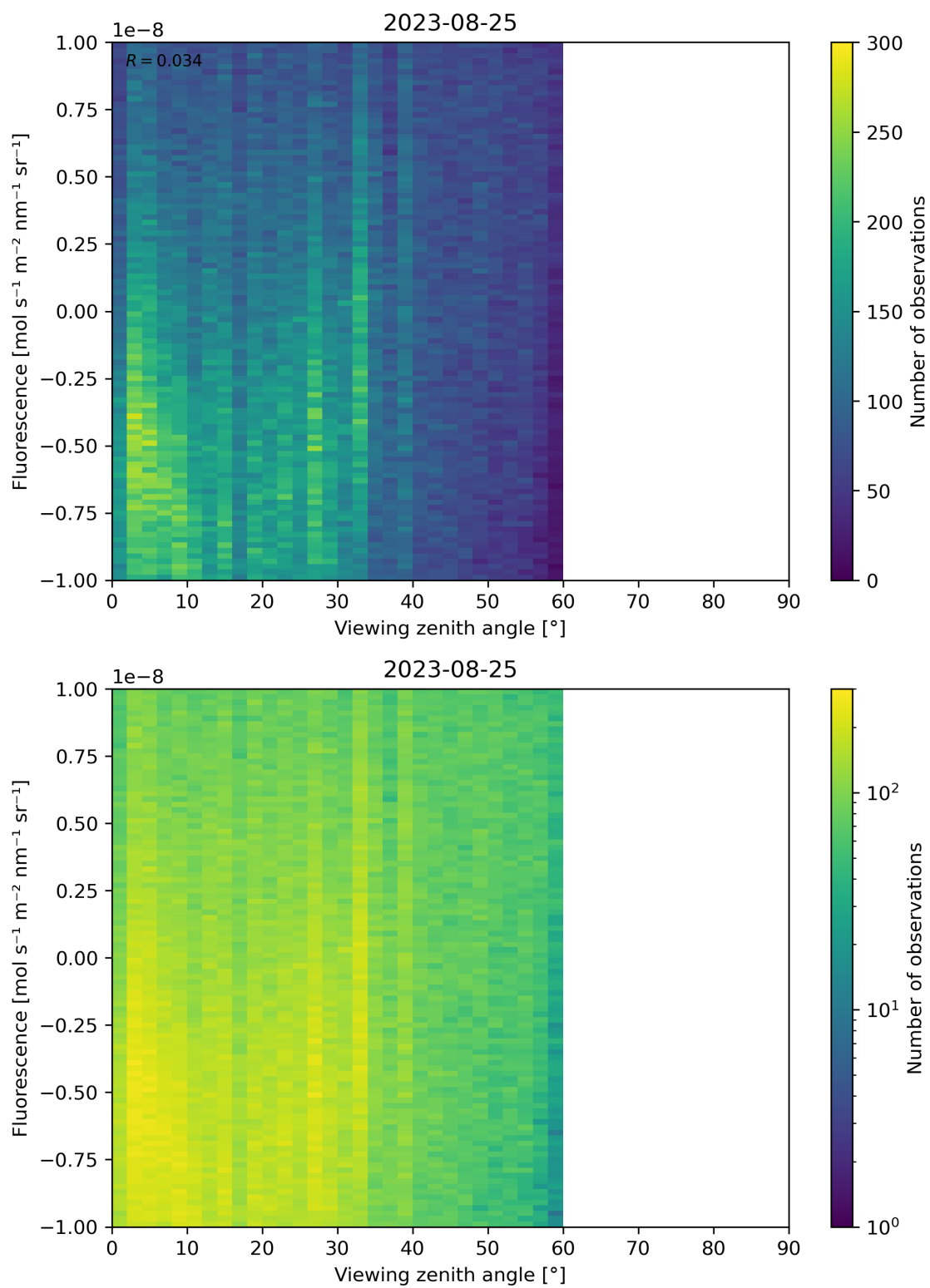
Figure 108: Scatter density plot of “Viewing zenith angle” against “Fluorescence” for 2023-08-25 to 2023-08-26.
