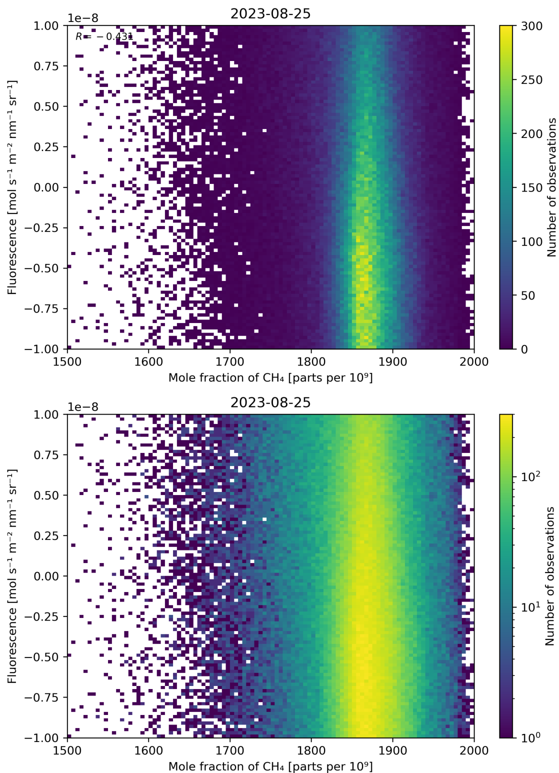
Figure 73: Scatter density plot of “Mole fraction of \text{CH}_4 ” against “Fluorescence” for 2023-08-25 to 2023-08-26.
