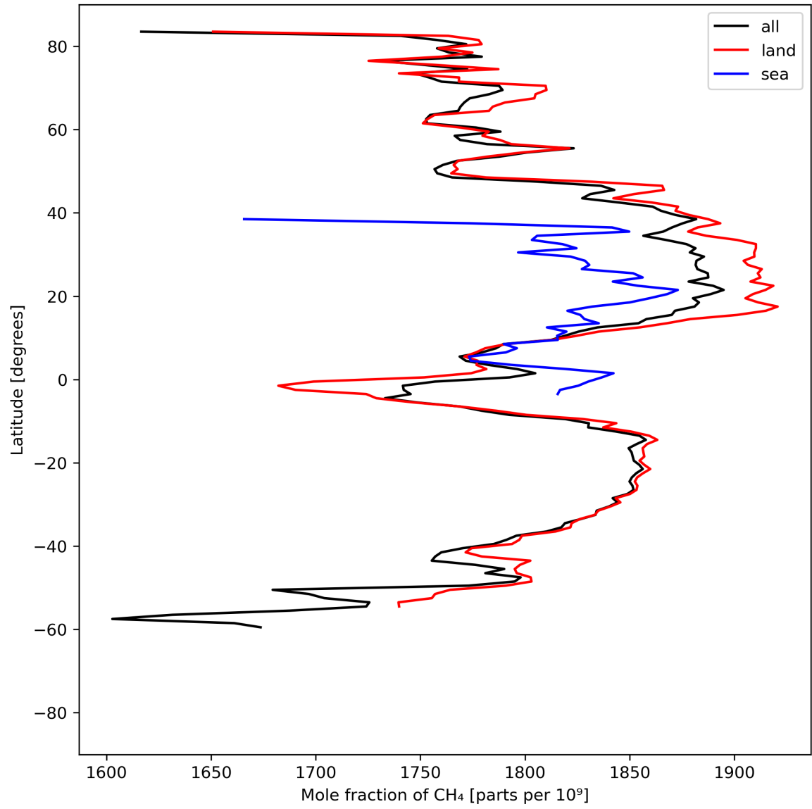
Figure 12: Zonal average of “Mole fraction of CH 4 ” for 2023-08-25 to 2023-08-26.
