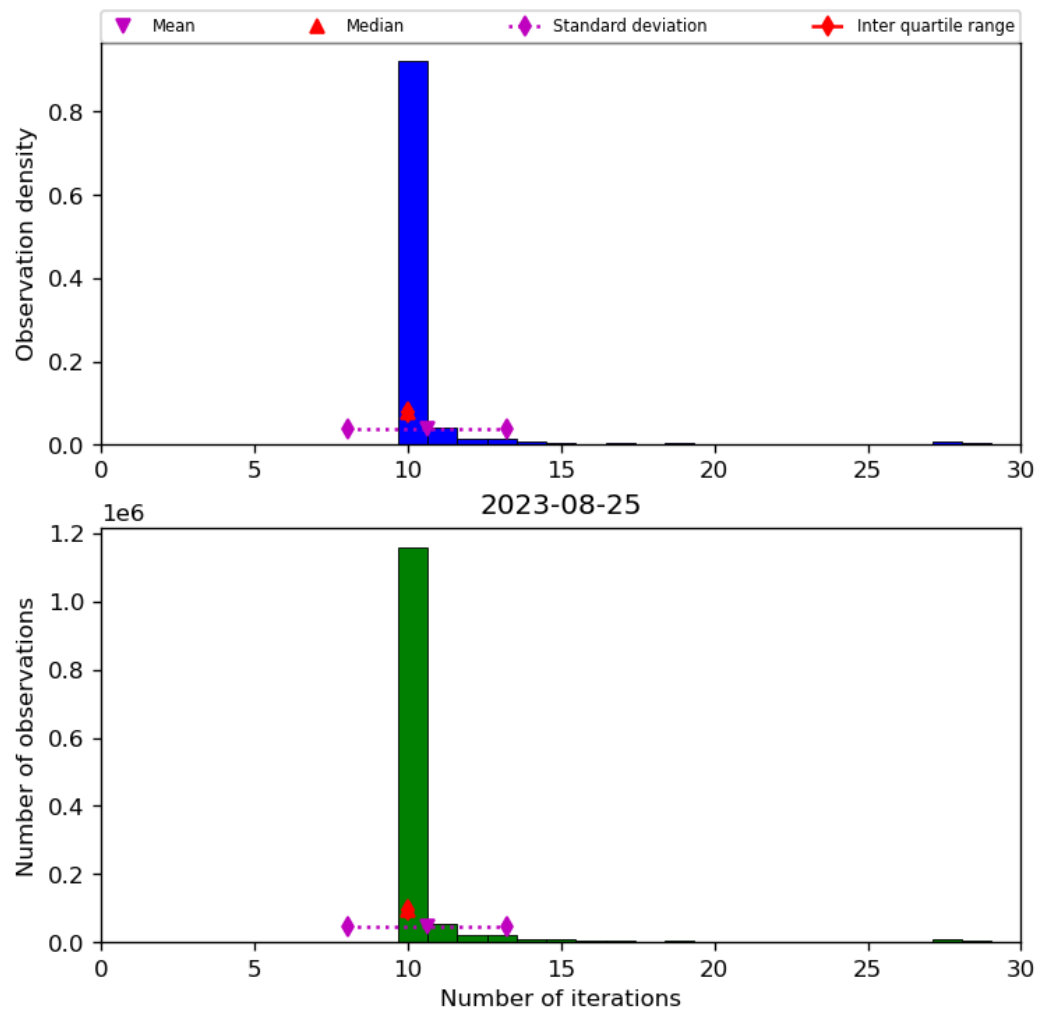
Figure 31: Histogram of “Number of iterations” for 2023-08-25 to 2023-08-26
