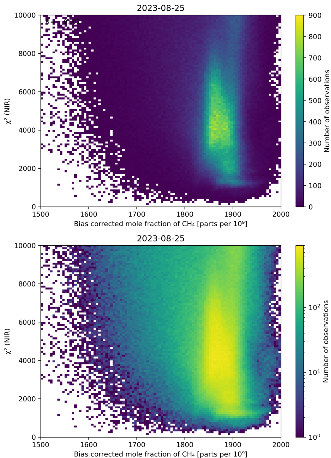
Figure 63: Scatter density plot of “Bias corrected mole fraction of CH 4 ” against “ \chi^2 (NIR)” for 2023-08-25 to 2023-08-26.
