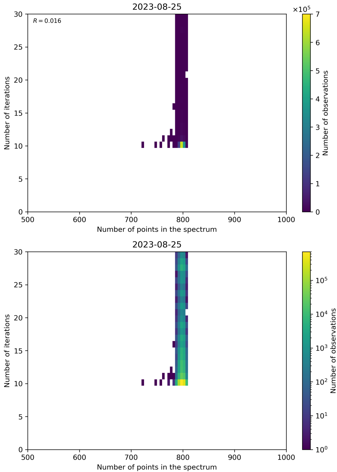
Figure 92: Scatter density plot of “Number of points in the spectrum” against “Number of iterations” for 2023-08-25 to 2023-08-26.
