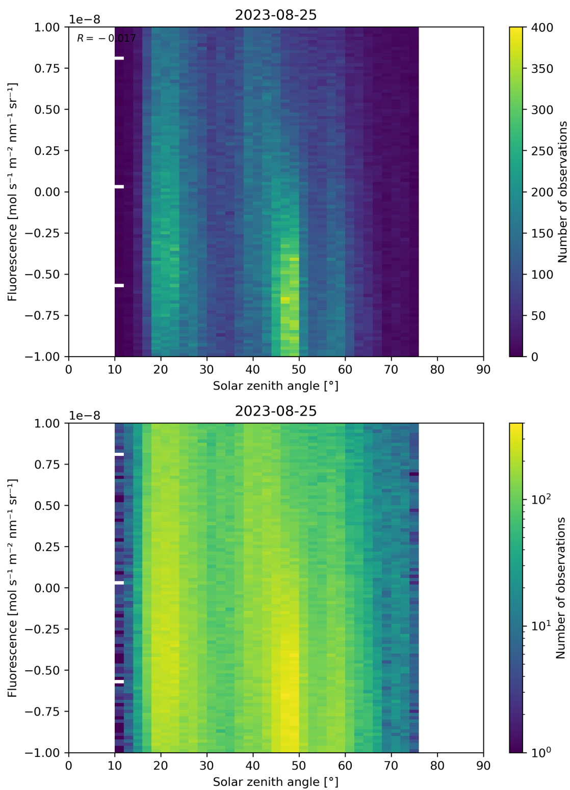
Figure 97: Scatter density plot of “Solar zenith angle” against “Fluorescence” for 2023-08-25 to 2023-08-26.
