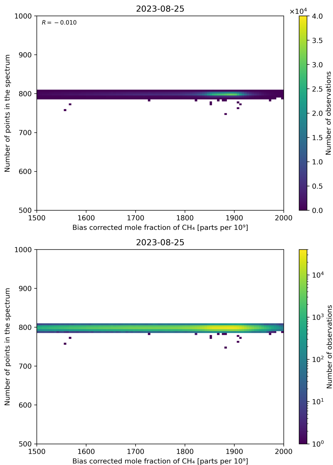
Figure 68: Scatter density plot of “Bias corrected mole fraction of CH 4 ” against “Number of points in the spectrum” for 2023-08-25 to 2023-08-26.
