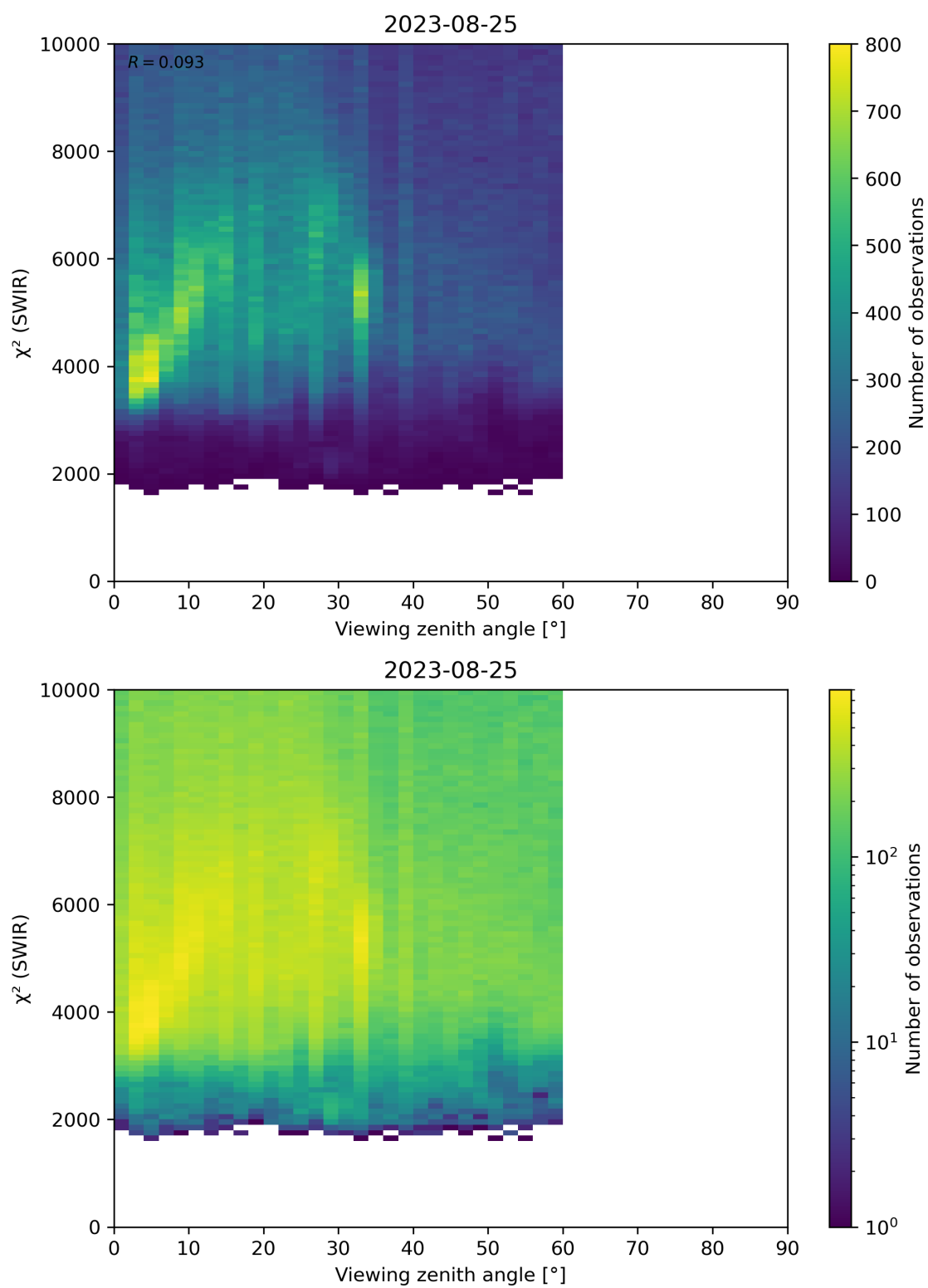
Figure 106: Scatter density plot of “Viewing zenith angle” against “ \chi^2 (SWIR)” for 2023-08-25 to 2023-08-26.
