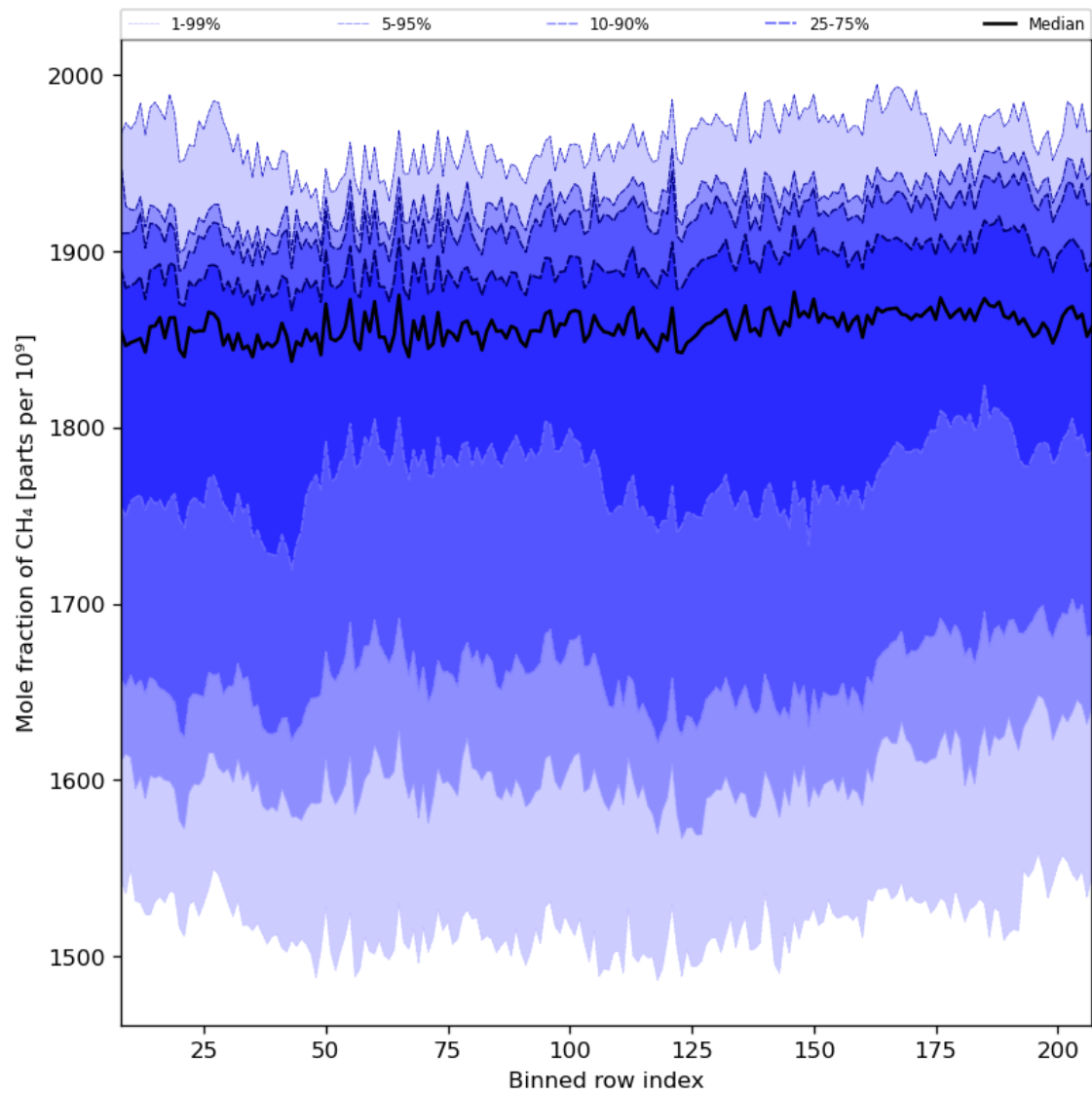
Figure 34: Along track statistics of “Mole fraction of CH 4 ” for 2023-08-25 to 2023-08-26
