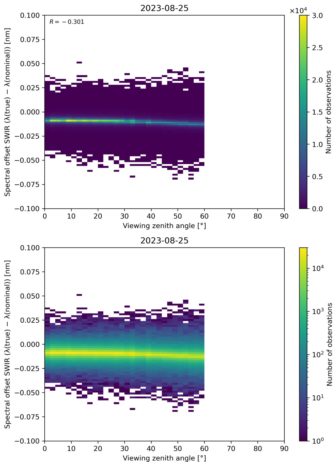
Figure 116: Scatter density plot of “Viewing zenith angle” against “Spectral offset SWIR ( \lambda(\text{true}) - \lambda(\text{nominal}) )” for 2023-08-25 to 2023-08-26.
