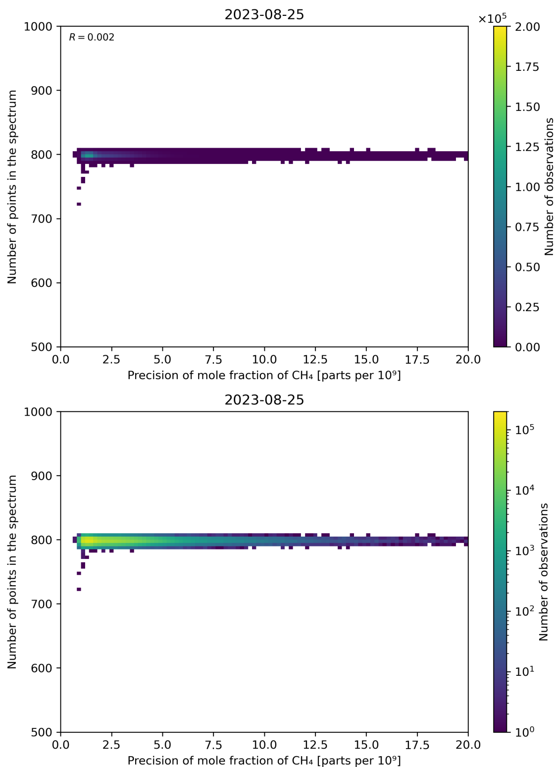
Figure 84: Scatter density plot of “Precision of mole fraction of CH 4 ” against “Number of points in the spectrum” for 2023-08-25 to 2023-08-26.
