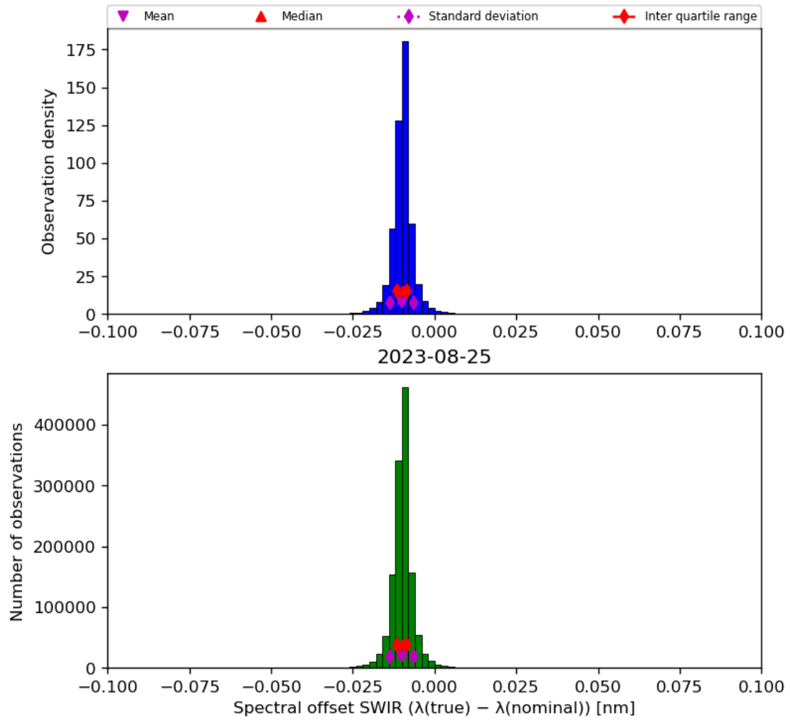
Figure 27: Histogram of “Spectral offset SWIR ( \lambda(\text{true}) - \lambda(\text{nominal}) )” for 2023-08-25 to 2023-08-26
