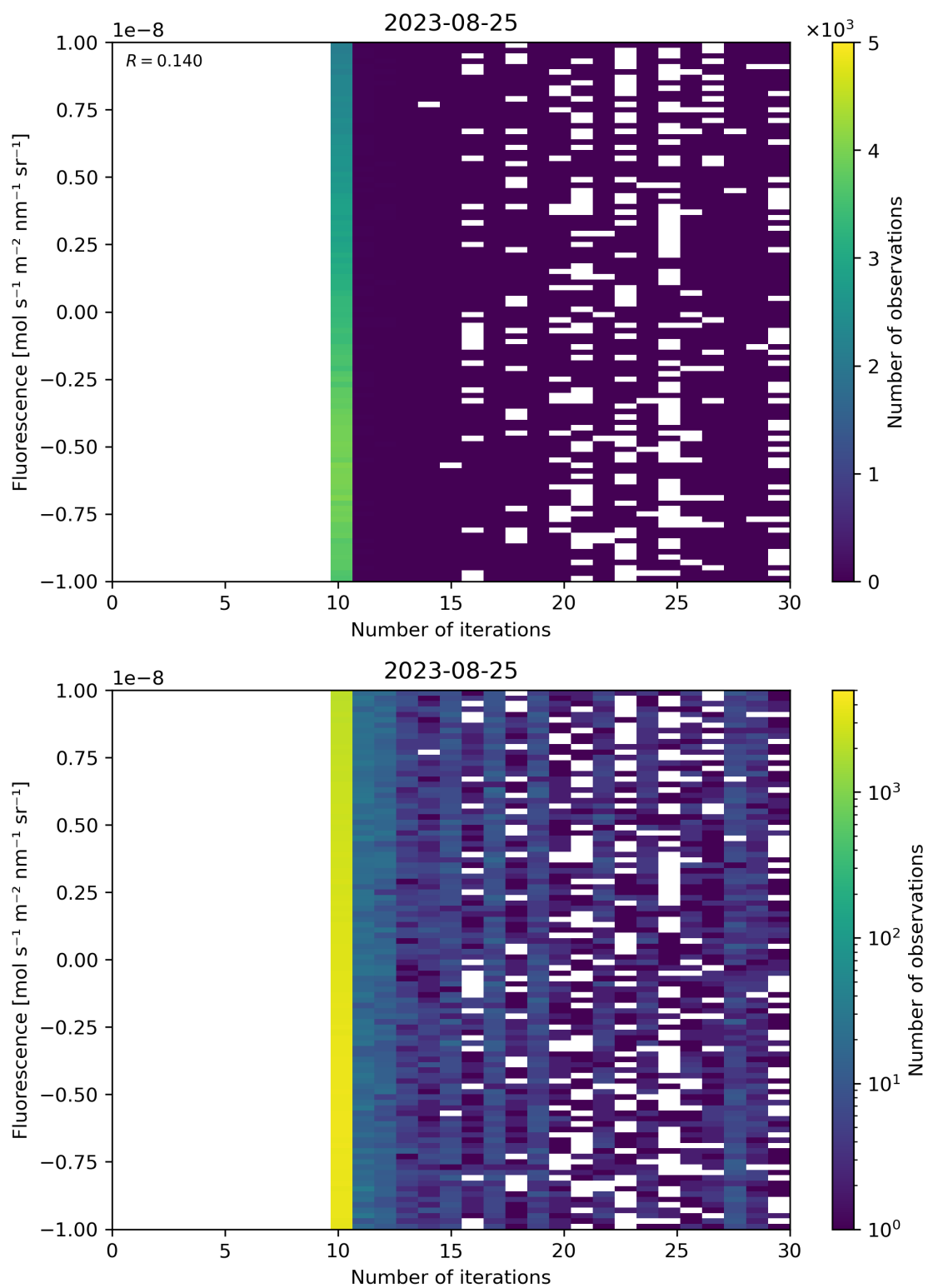
Figure 87: Scatter density plot of “Number of iterations” against “Fluorescence” for 2023-08-25 to 2023-08-26.
