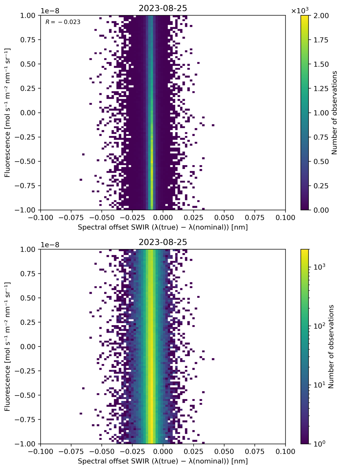
Figure 120: Scatter density plot of “Spectral offset SWIR ( \lambda(\text{true}) - \lambda(\text{nominal}) )” against “Fluorescence” for 2023-08-25 to 2023-08-26.
