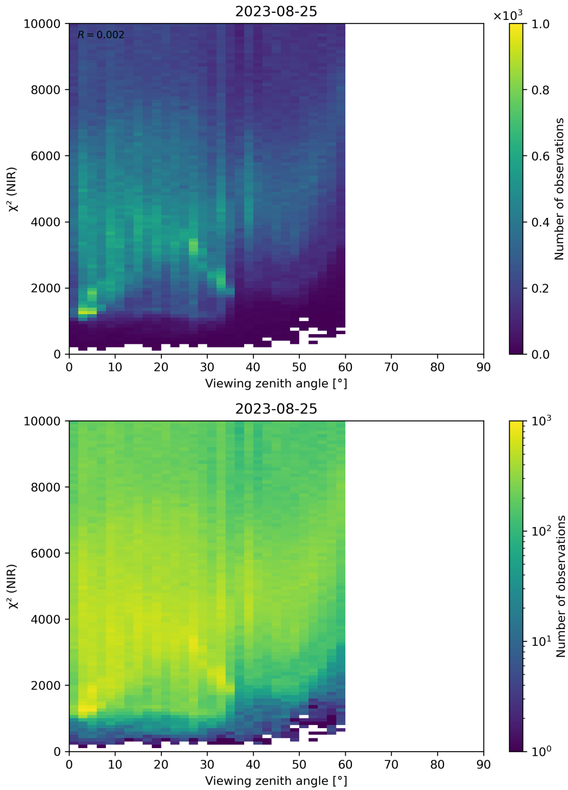
Figure 105: Scatter density plot of “Viewing zenith angle” against “ \chi^2 (NIR)” for 2023-08-25 to 2023-08-26.
