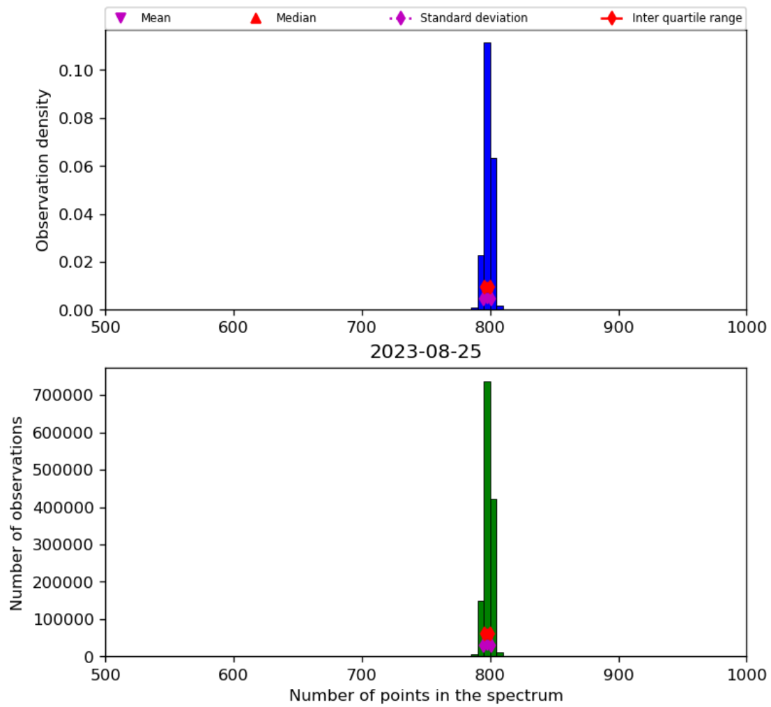
Figure 26: Histogram of “Number of points in the spectrum” for 2023-08-25 to 2023-08-26
