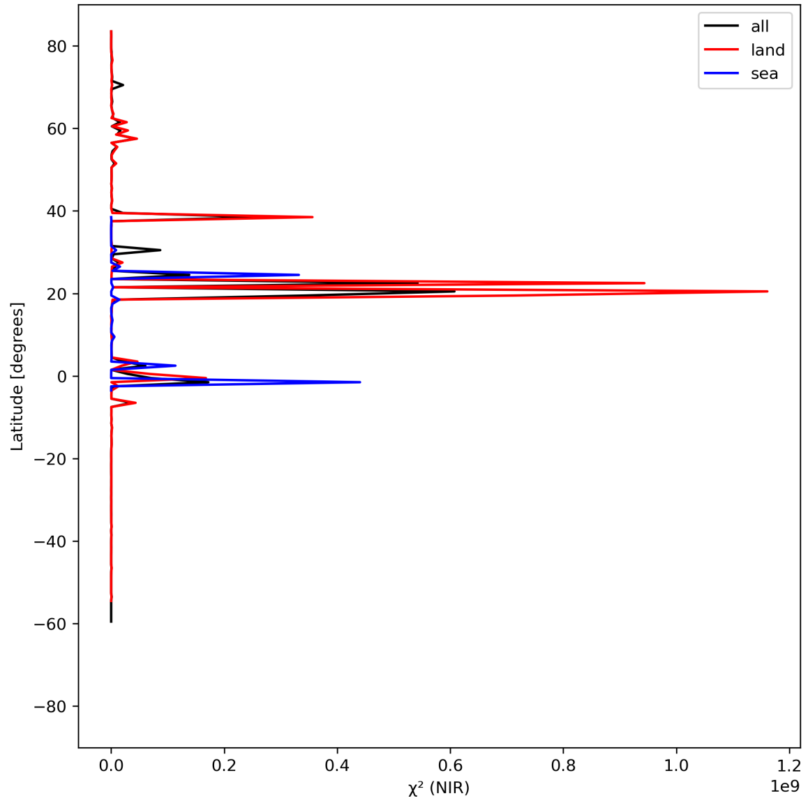
Figure 18: Zonal average of “ \chi^2 (NIR)” for 2023-08-25 to 2023-08-26.
