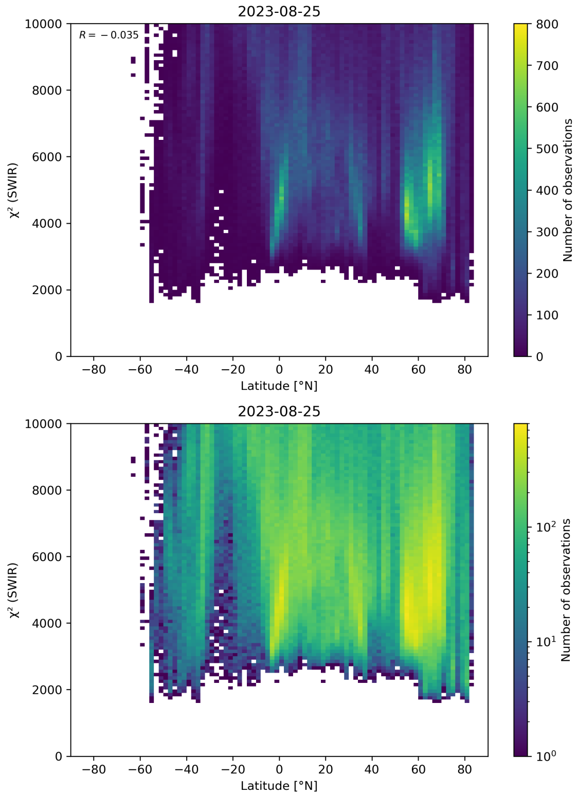
Figure 54: Scatter density plot of “Latitude” against “ \chi^2 (SWIR)” for 2023-08-25 to 2023-08-26.
