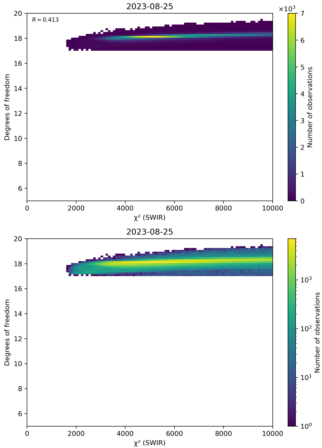
Figure 48: Scatter density plot of “ \chi^2 (SWIR)” against “Degrees of freedom” for 2023-08-25 to 2023-08-26.
