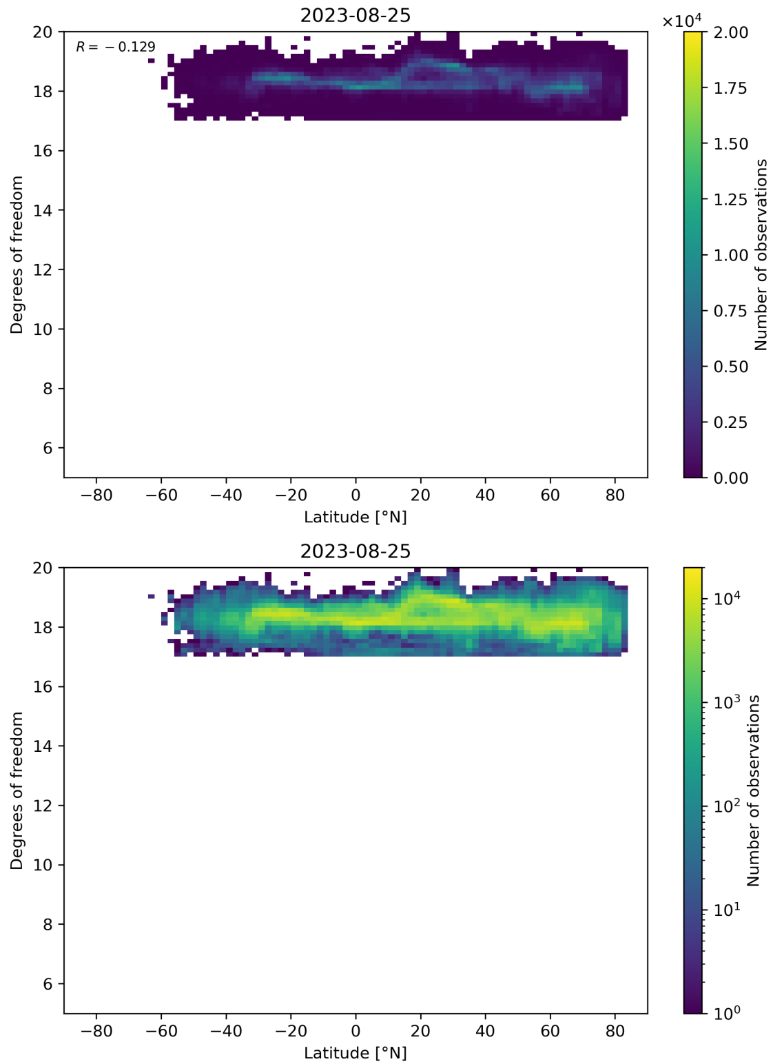
Figure 55: Scatter density plot of “Latitude” against “Degrees of freedom” for 2023-08-25 to 2023-08-26.
