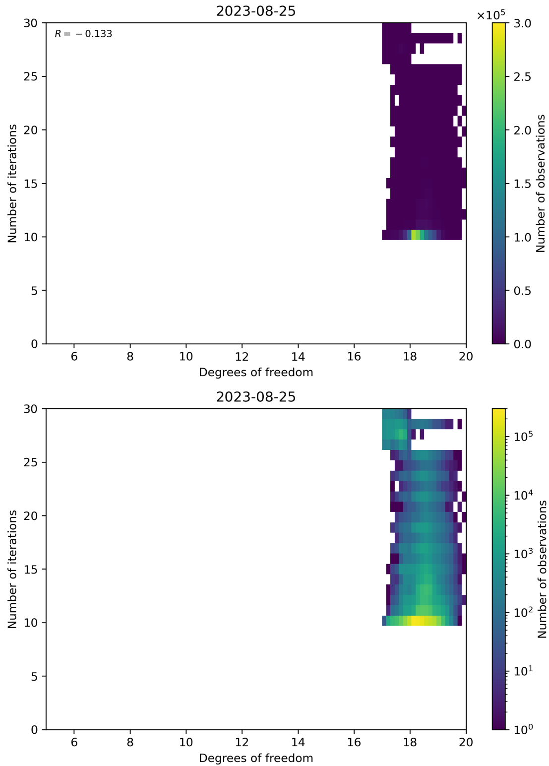
Figure 52: Scatter density plot of “Degrees of freedom” against “Number of iterations” for 2023-08-25 to 2023-08-26.
