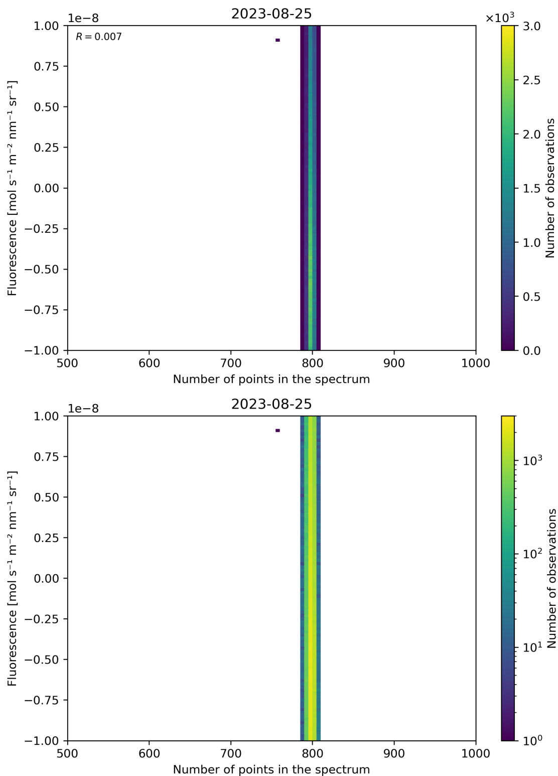
Figure 91: Scatter density plot of “Number of points in the spectrum” against “Fluorescence” for 2023-08-25 to 2023-08-26.
