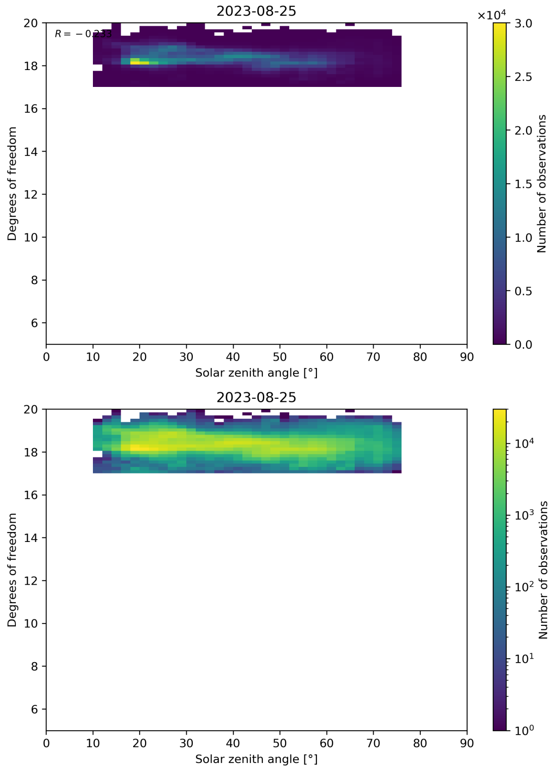
Figure 96: Scatter density plot of “Solar zenith angle” against “Degrees of freedom” for 2023-08-25 to 2023-08-26.
