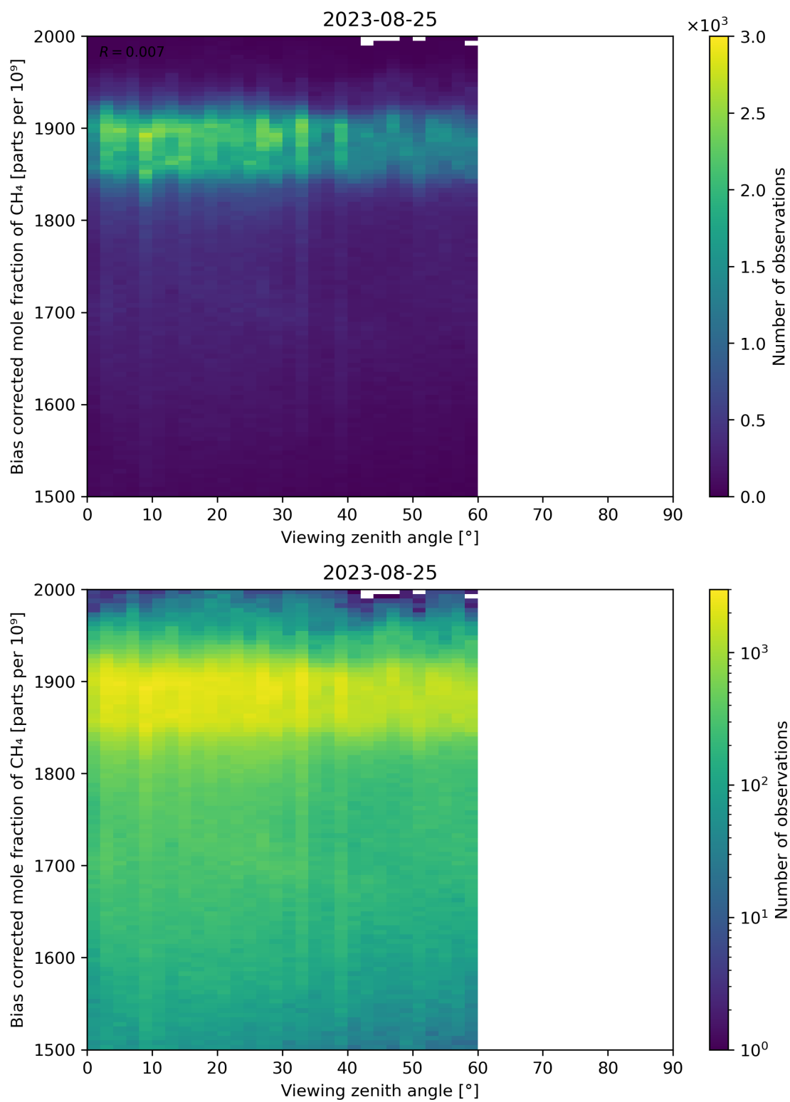
Figure 111: Scatter density plot of “Viewing zenith angle” against “Bias corrected mole fraction of CH 4 ” for 2023-08-25 to 2023-08-26.
