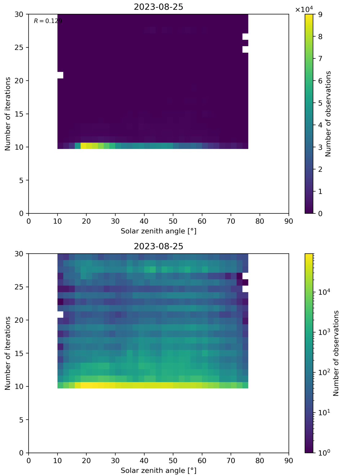
Figure 102: Scatter density plot of “Solar zenith angle” against “Number of iterations” for 2023-08-25 to 2023-08-26.
