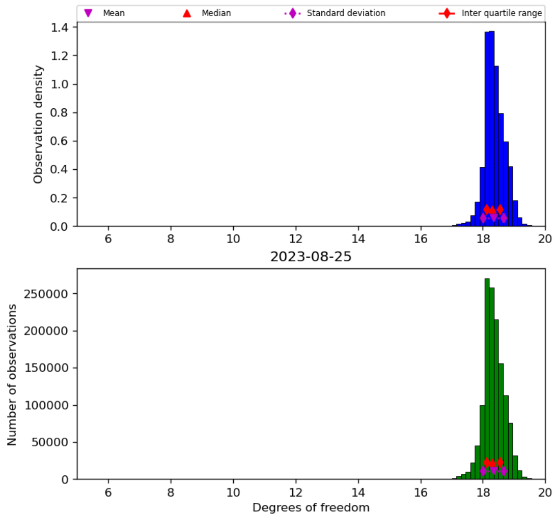
Figure 30: Histogram of “Degrees of freedom” for 2023-08-25 to 2023-08-26
