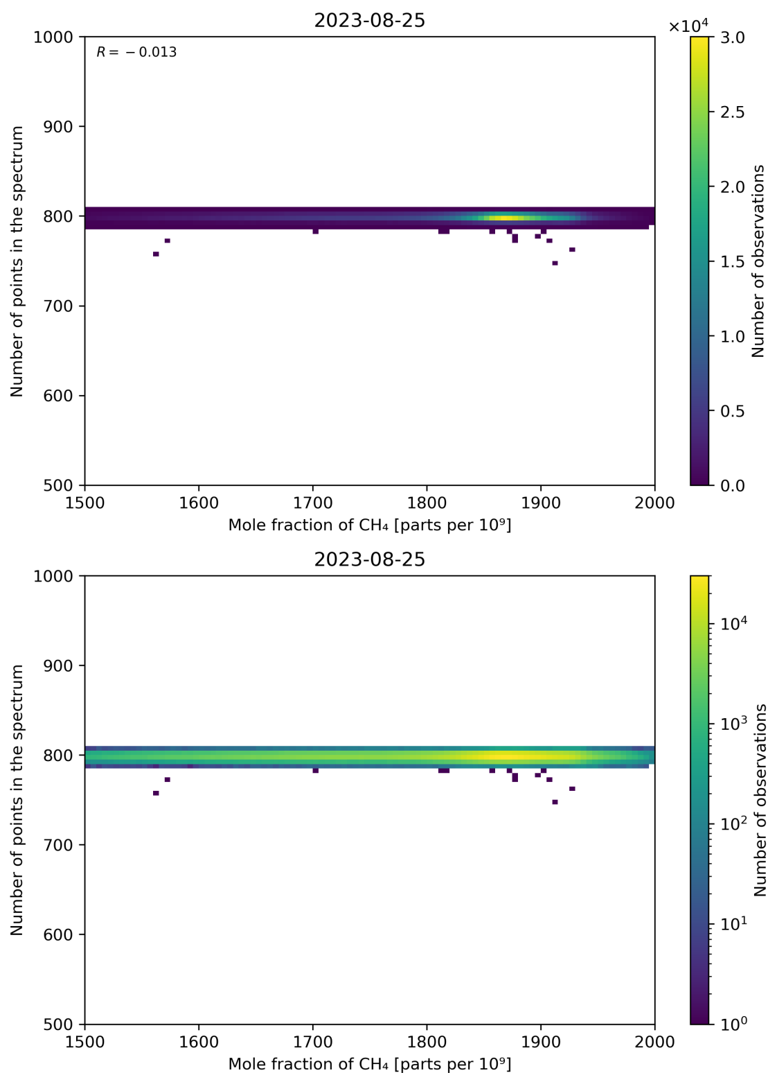
Figure 77: Scatter density plot of “Mole fraction of CH 4 ” against “Number of points in the spectrum” for 2023-08-25 to 2023-08-26.
