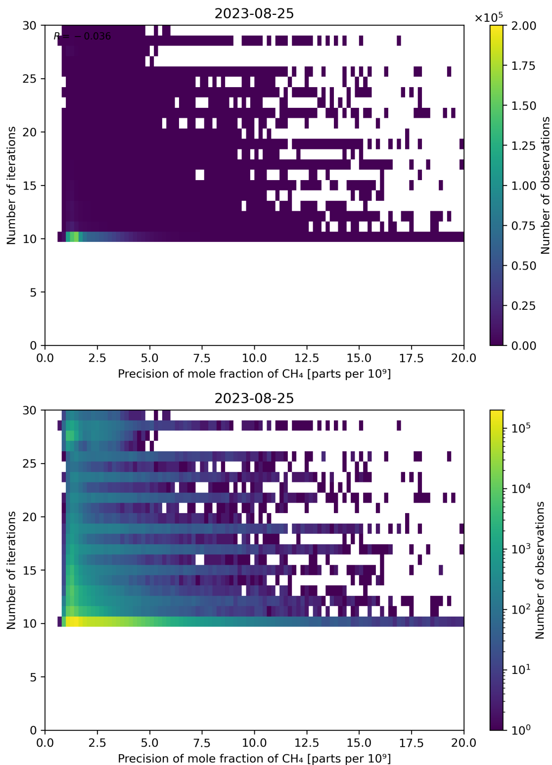
Figure 83: Scatter density plot of “Precision of mole fraction of CH 4 ” against “Number of iterations” for 2023-08-25 to 2023-08-26.
