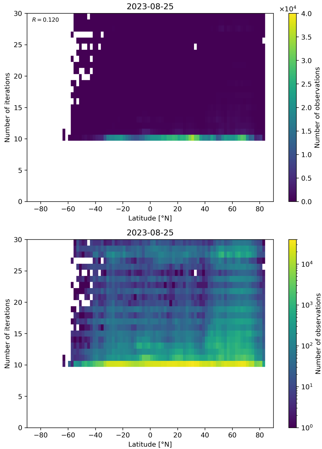
Figure 60: Scatter density plot of “Latitude” against “Number of iterations” for 2023-08-25 to 2023-08-26.
