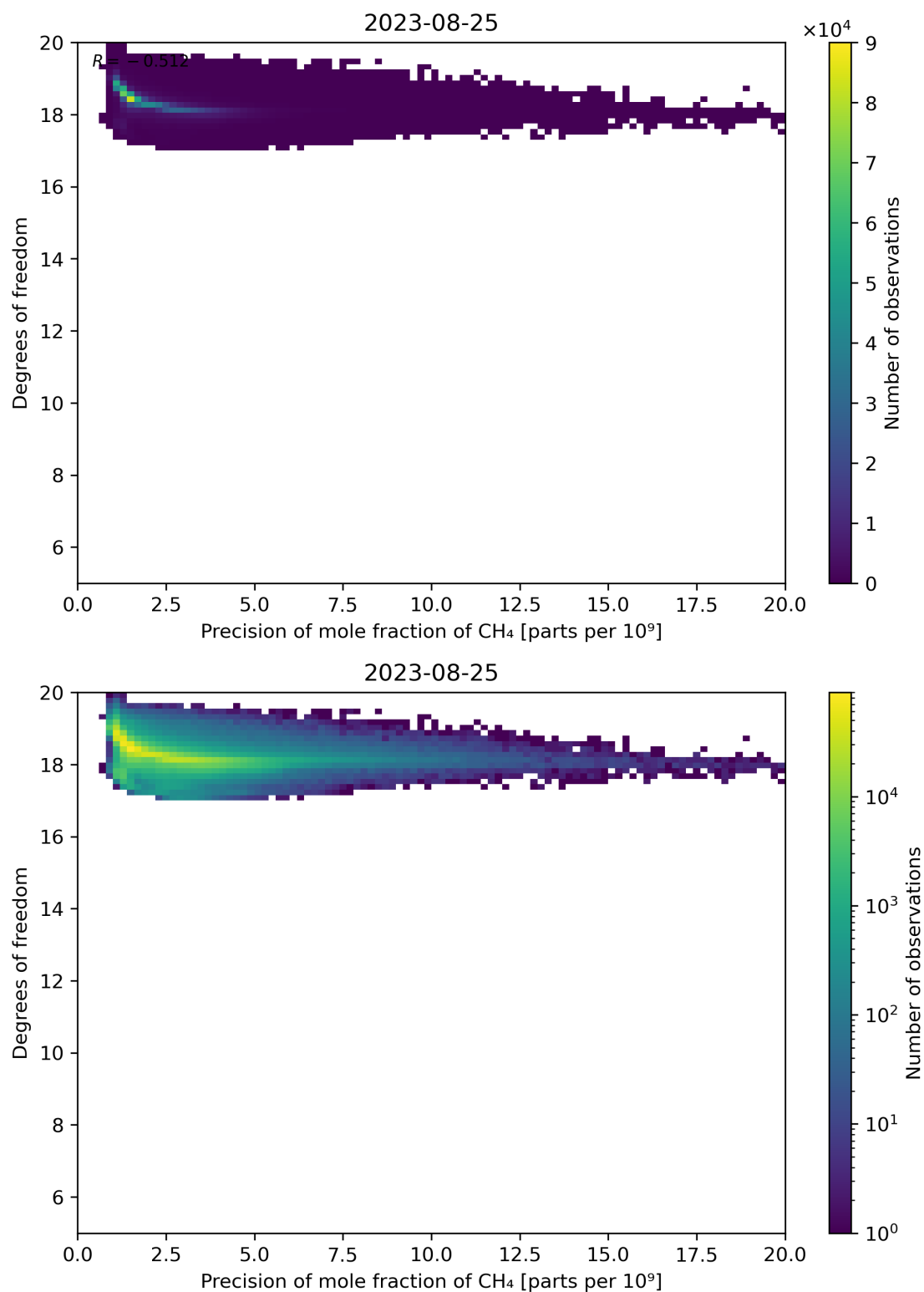
Figure 80: Scatter density plot of “Precision of mole fraction of CH 4 ” against “Degrees of freedom” for 2023-08-25 to 2023-08-26.
