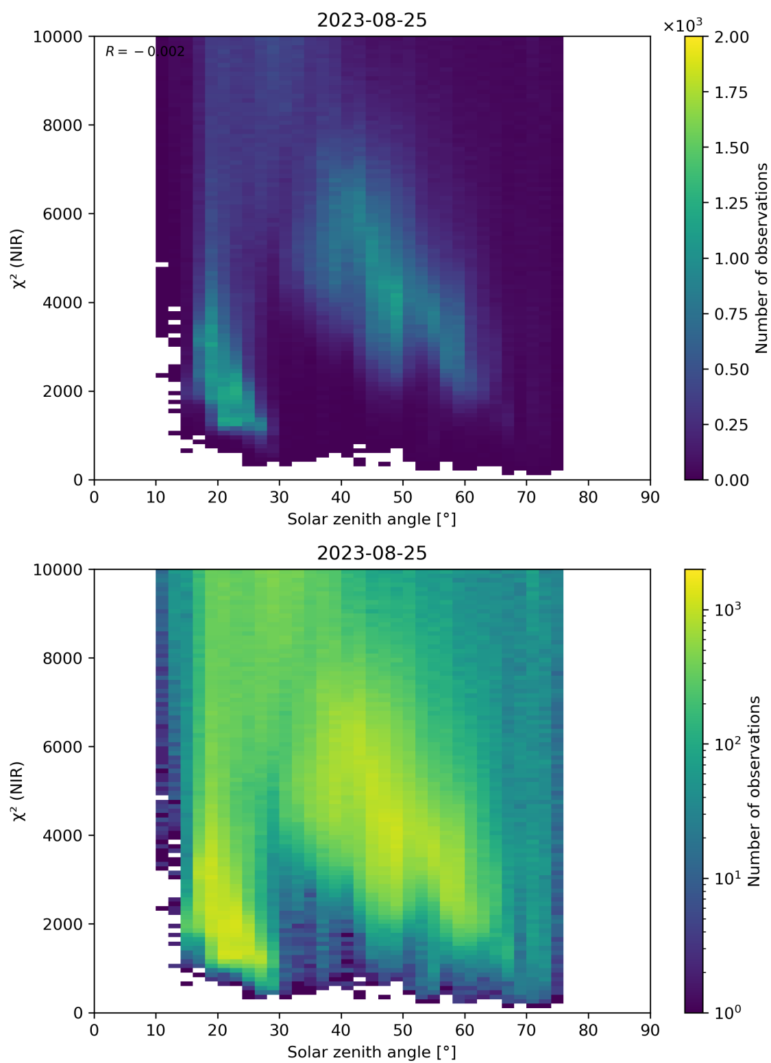
Figure 94: Scatter density plot of “Solar zenith angle” against “ \chi^2 (NIR)” for 2023-08-25 to 2023-08-26.
