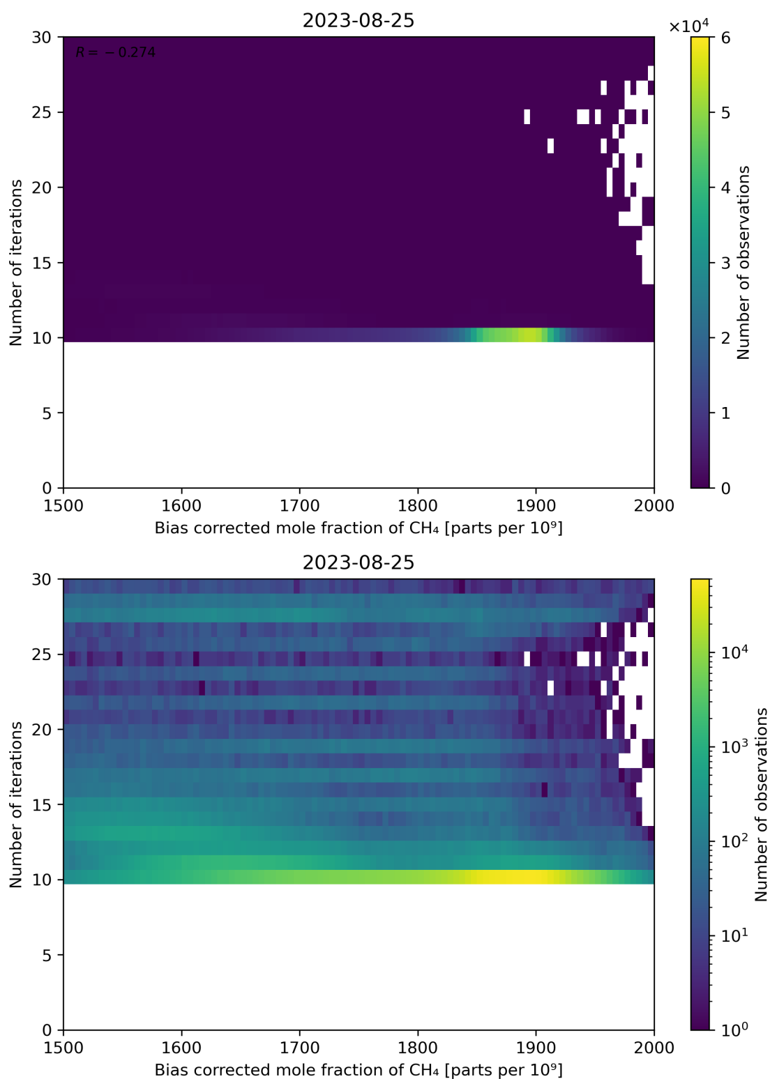
Figure 67: Scatter density plot of “Bias corrected mole fraction of CH 4 ” against “Number of iterations” for 2023-08-25 to 2023-08-26.
