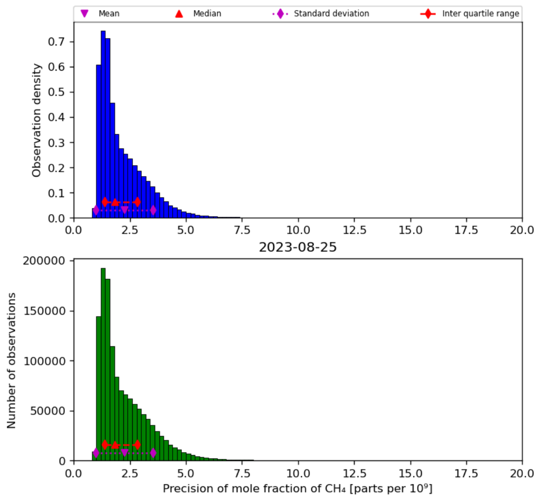
Figure 24: Histogram of “Precision of mole fraction of CH 4 ” for 2023-08-25 to 2023-08-26
