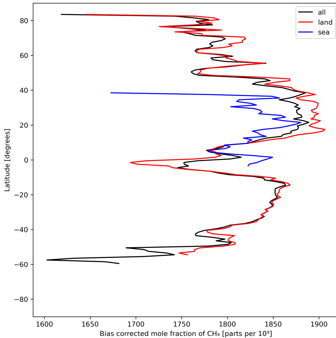
Figure 14: Zonal average of “Bias corrected mole fraction of CH 4 ” for 2023-08-25 to 2023-08-26.
