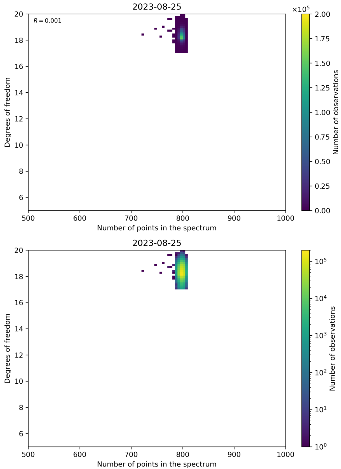
Figure 90: Scatter density plot of “Number of points in the spectrum” against “Degrees of freedom” for 2023-08-25 to 2023-08-26.
