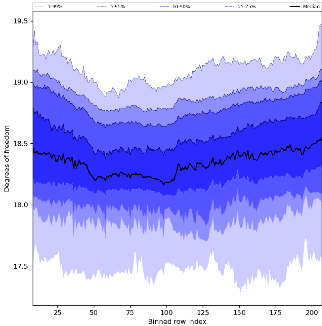
Figure 41: Along track statistics of “Degrees of freedom” for 2023-08-25 to 2023-08-26
