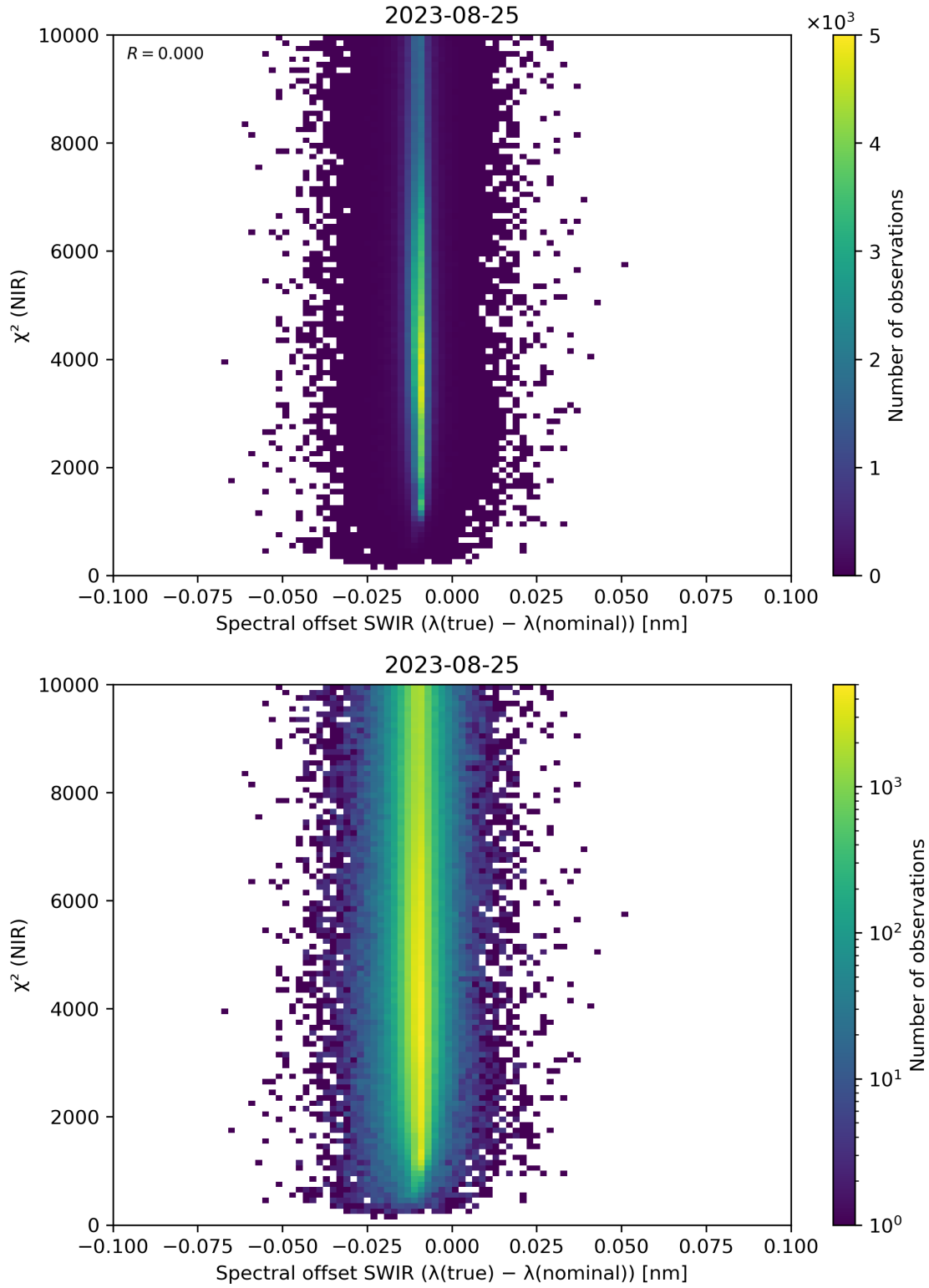
Figure 117: Scatter density plot of “Spectral offset SWIR ( \lambda(\text{true}) - \lambda(\text{nominal}) )” against “ \chi^2 (NIR)” for 2023-08-25 to 2023-08-26.
