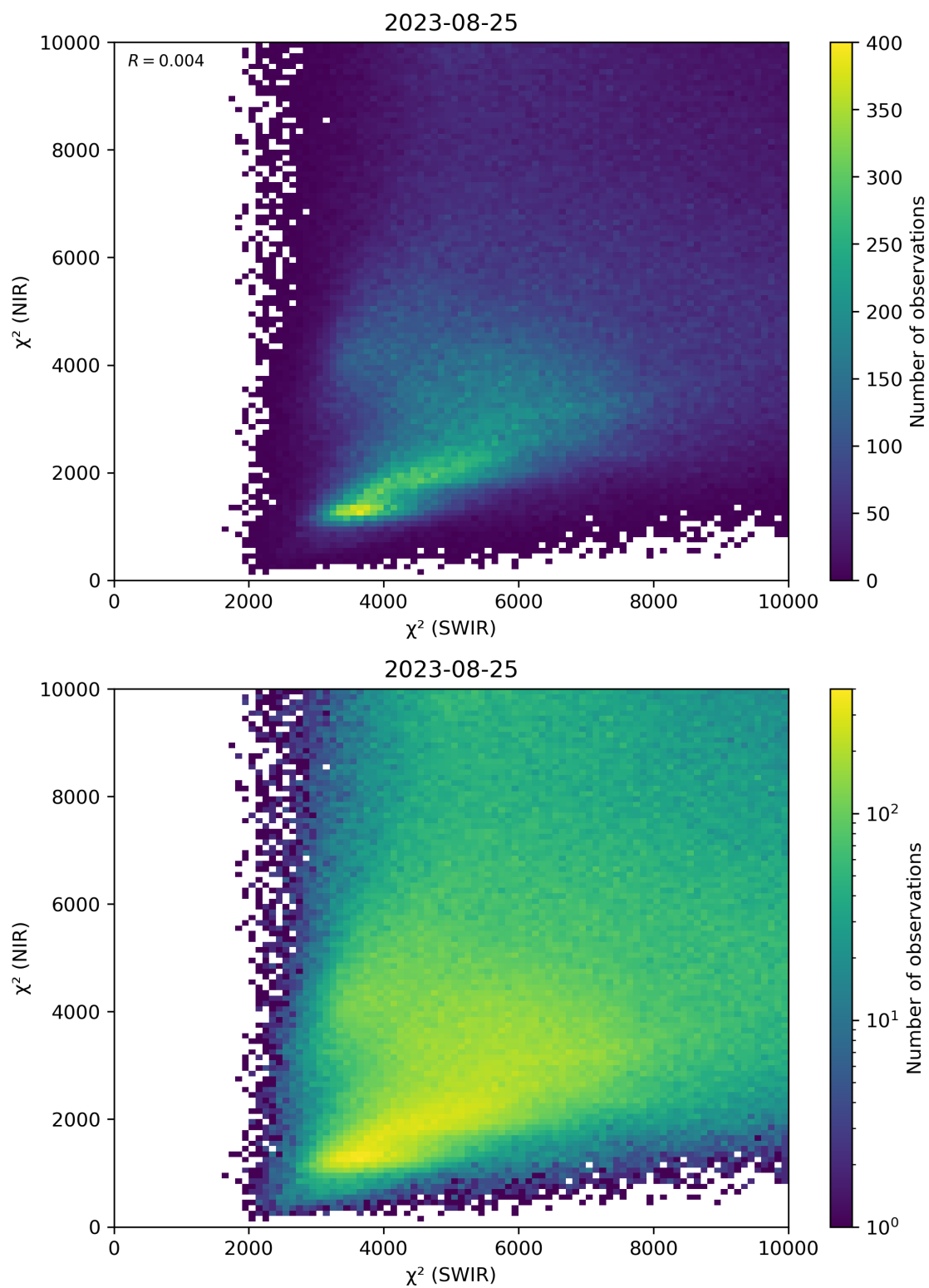
Figure 47: Scatter density plot of “ \chi^2 (SWIR)” against “ \chi^2 (NIR)” for 2023-08-25 to 2023-08-26.
