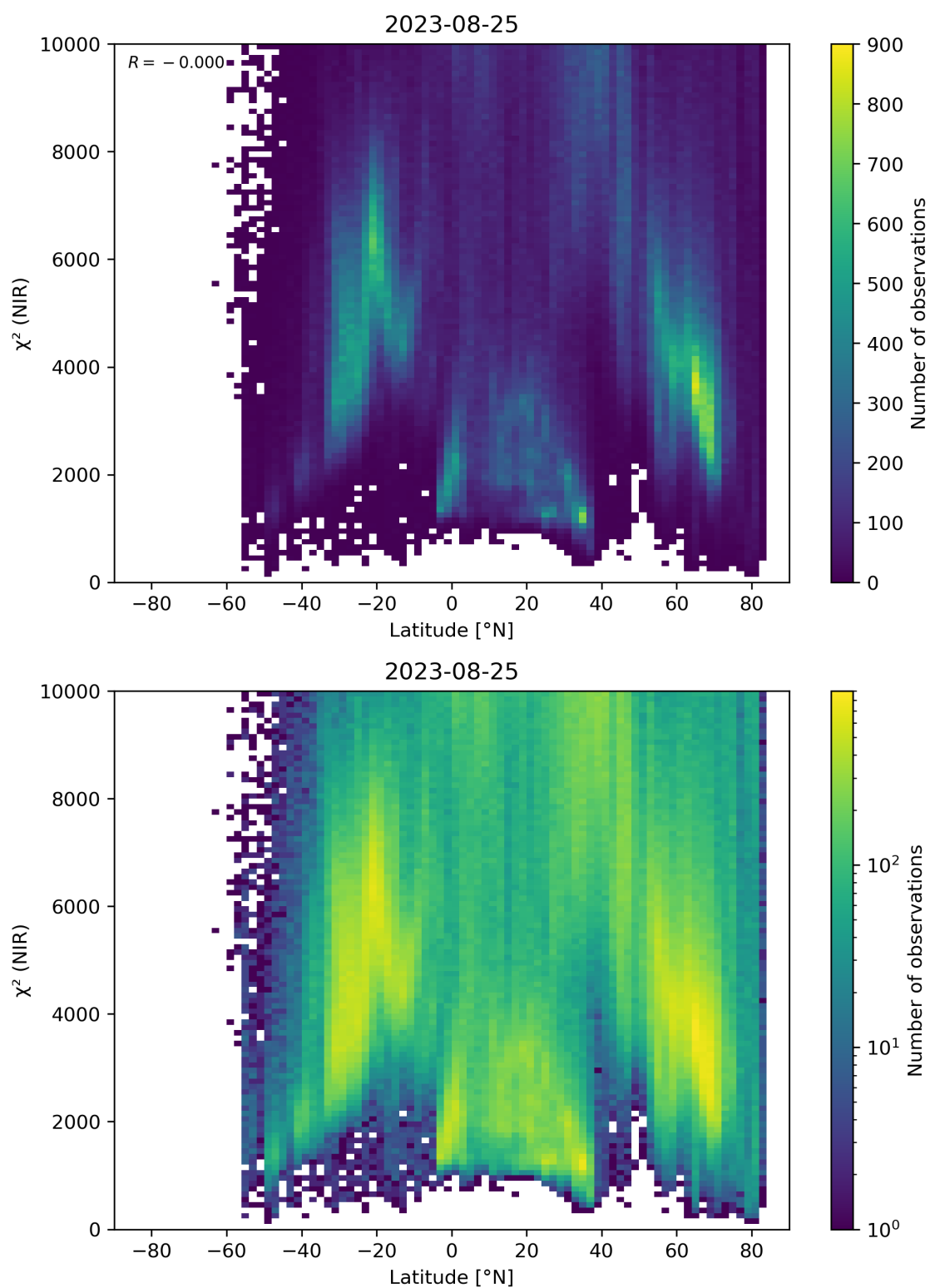
Figure 53: Scatter density plot of “Latitude” against “ \chi^2 (NIR)” for 2023-08-25 to 2023-08-26.
