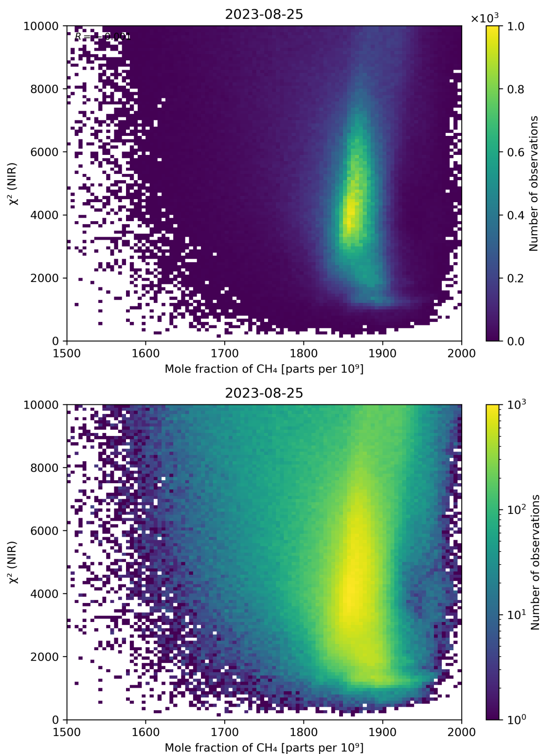
Figure 70: Scatter density plot of “Mole fraction of \text{CH}_4 ” against “ \chi^2 (NIR)” for 2023-08-25 to 2023-08-26.
