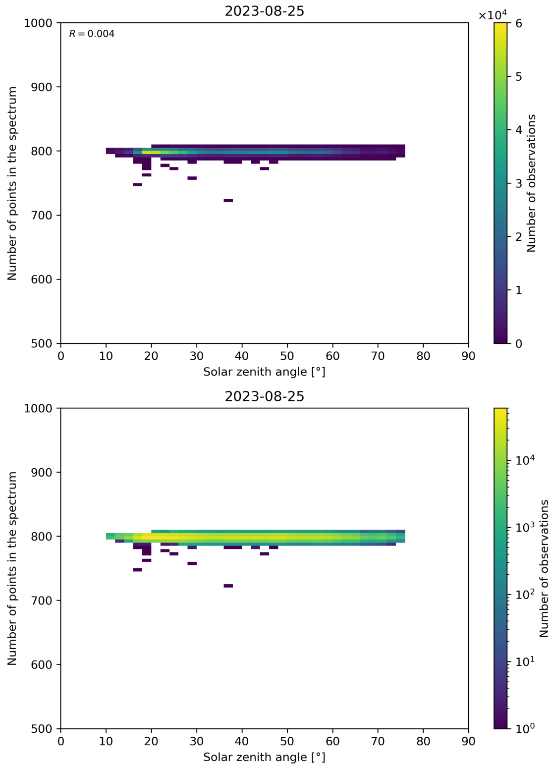
Figure 103: Scatter density plot of “Solar zenith angle” against “Number of points in the spectrum” for 2023-08-25 to 2023-08-26.
