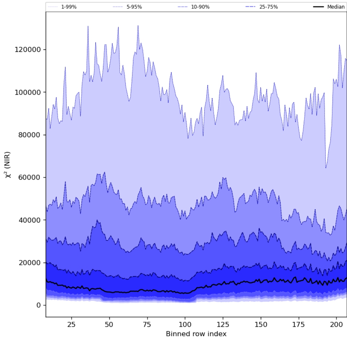
Figure 40: Along track statistics of " \chi^2 (NIR)" for 2023-08-25 to 2023-08-26
