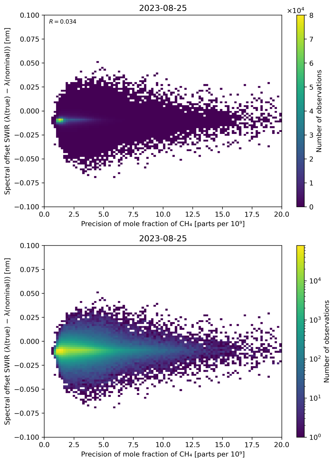
Figure 85: Scatter density plot of “Precision of mole fraction of CH 4 ” against “Spectral offset SWIR ( \lambda(\text{true}) - \lambda(\text{nominal}) )” for 2023-08-25 to 2023-08-26.
