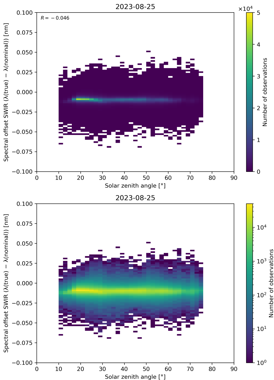
Figure 104: Scatter density plot of “Solar zenith angle” against “Spectral offset SWIR ( \lambda(\text{true}) - \lambda(\text{nominal}) )” for 2023-08-25 to 2023-08-26.
