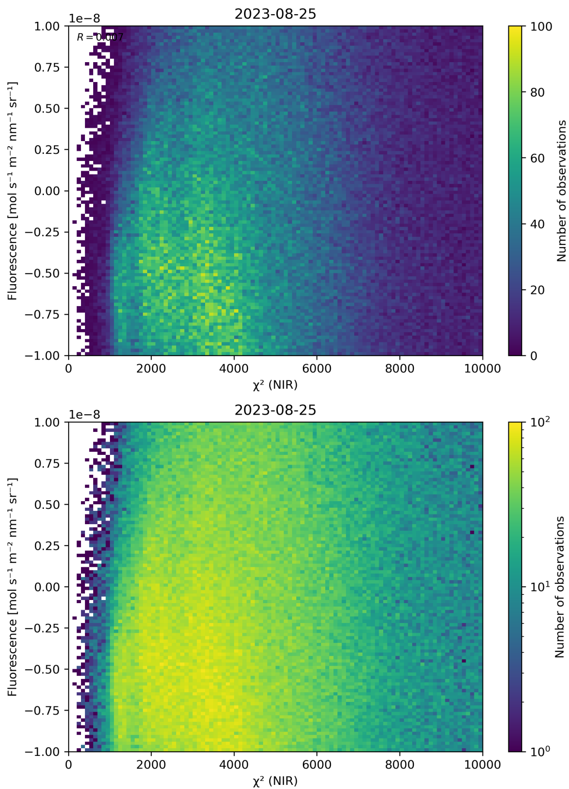
Figure 45: Scatter density plot of “ \chi^2 (NIR)” against “Fluorescence” for 2023-08-25 to 2023-08-26.
