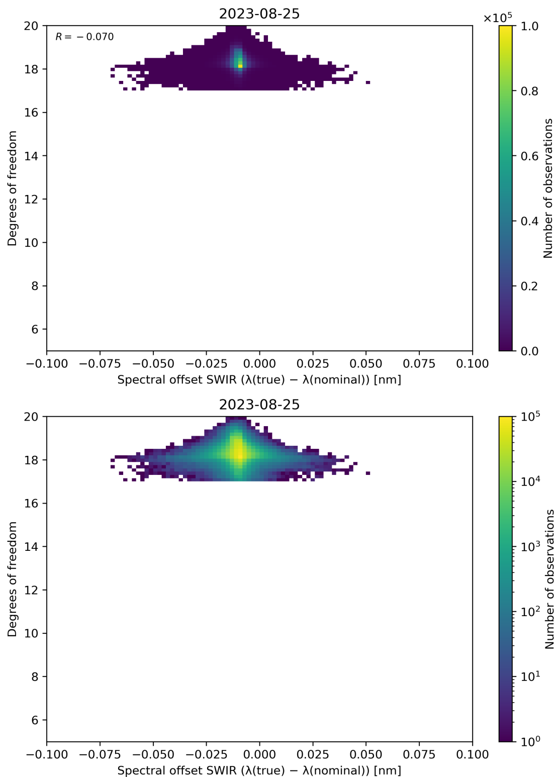
Figure 119: Scatter density plot of “Spectral offset SWIR ( \lambda(\text{true}) - \lambda(\text{nominal}) )” against “Degrees of freedom” for 2023-08-25 to 2023-08-26.
