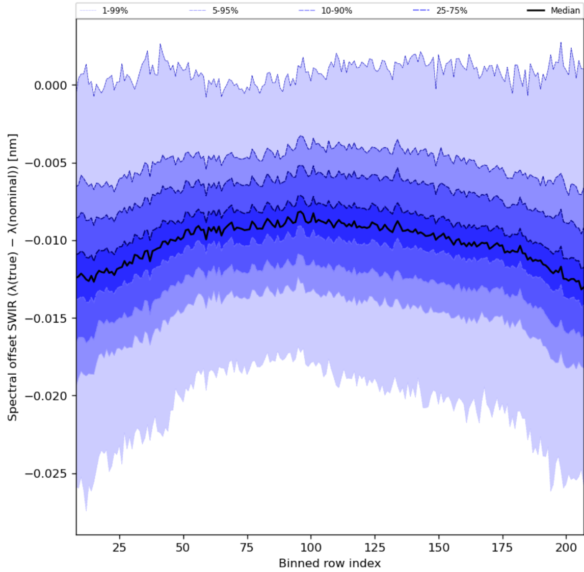
Figure 38: Along track statistics of “Spectral offset SWIR ( \lambda(\text{true}) - \lambda(\text{nominal}) )” for 2023-08-25 to 2023-08-26
