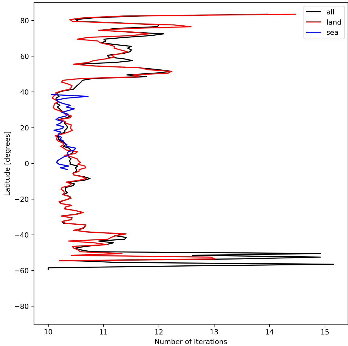
Figure 20: Zonal average of “Number of iterations” for 2023-08-25 to 2023-08-26.
