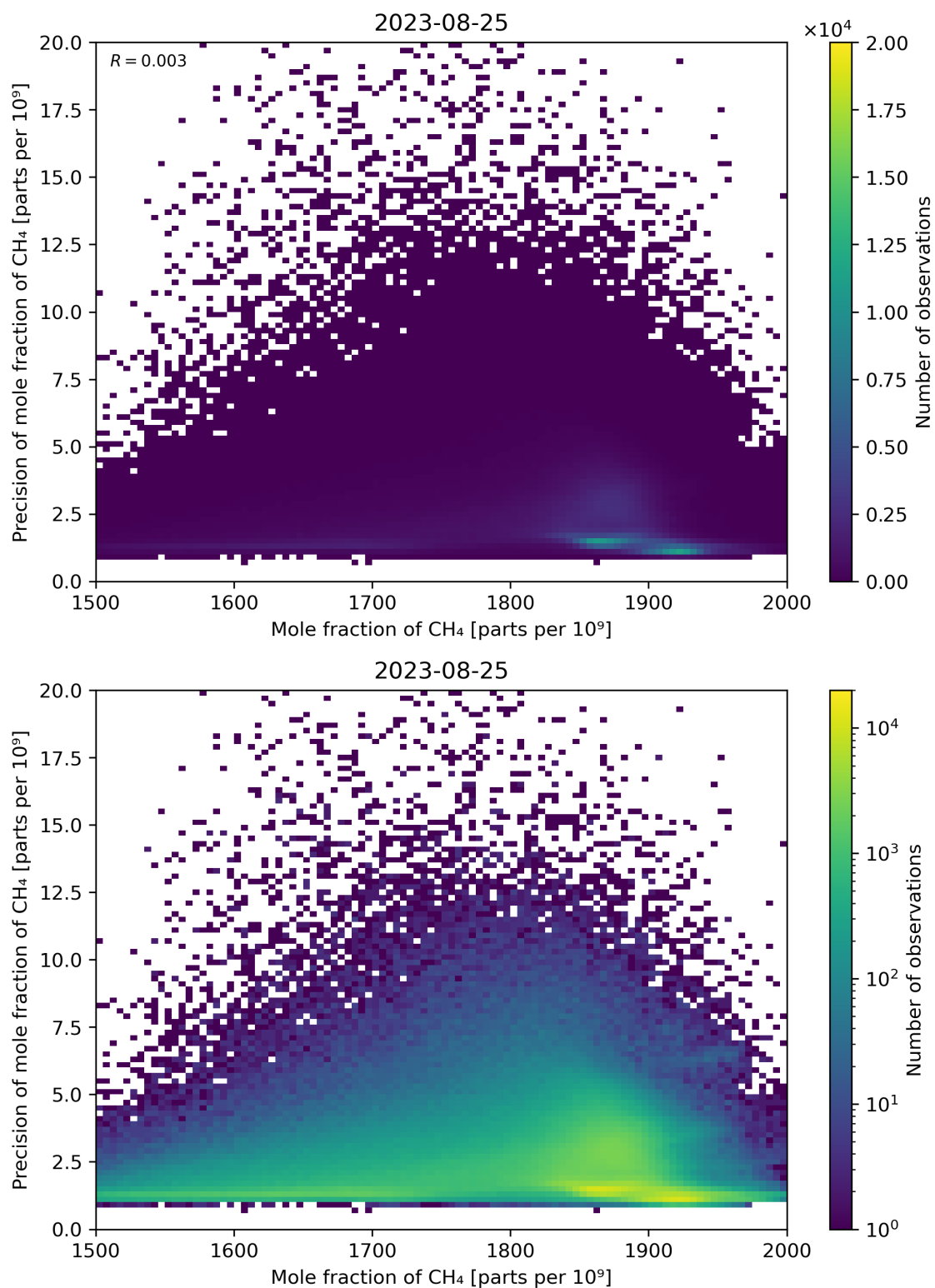
Figure 75: Scatter density plot of “Mole fraction of CH 4 ” against “Precision of mole fraction of CH 4 ” for 2023-08-25 to 2023-08-26.
