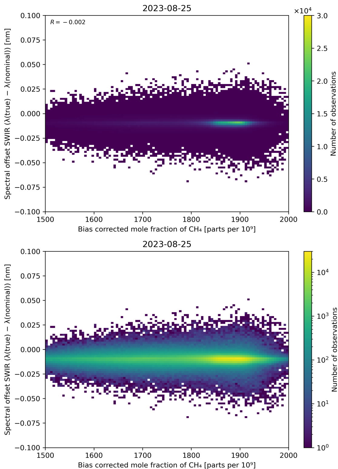
Figure 69: Scatter density plot of “Bias corrected mole fraction of \text{CH}_4 ” against “Spectral offset SWIR ( \lambda(\text{true}) - \lambda(\text{nominal}) )” for 2023-08-25 to 2023-08-26.
