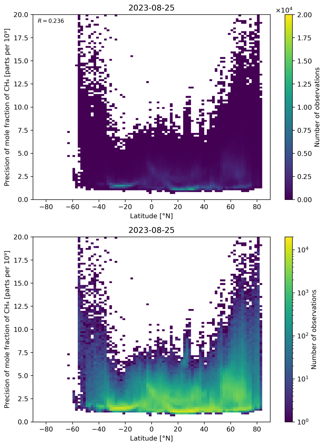
Figure 59: Scatter density plot of “Latitude” against “Precision of mole fraction of \text{CH}_4 ” for 2023-08-25 to 2023-08-26.
