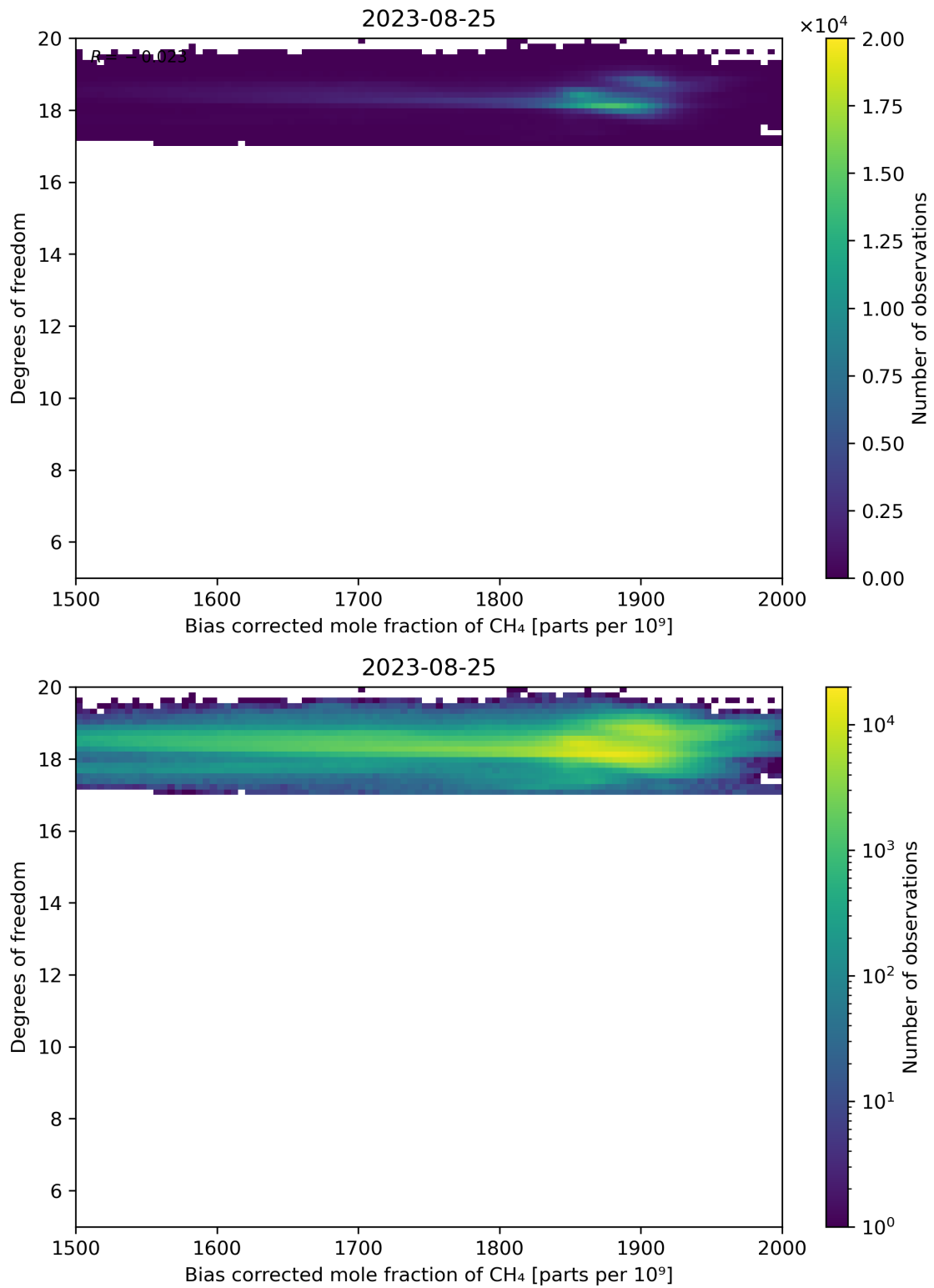
Figure 65: Scatter density plot of “Bias corrected mole fraction of CH 4 ” against “Degrees of freedom” for 2023-08-25 to 2023-08-26.
