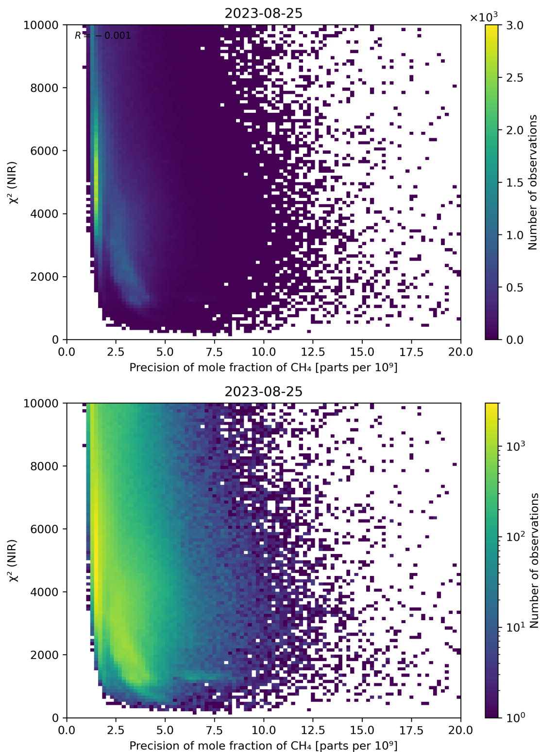
Figure 78: Scatter density plot of “Precision of mole fraction of CH 4 ” against “ \chi^2 (NIR)” for 2023-08-25 to 2023-08-26.
