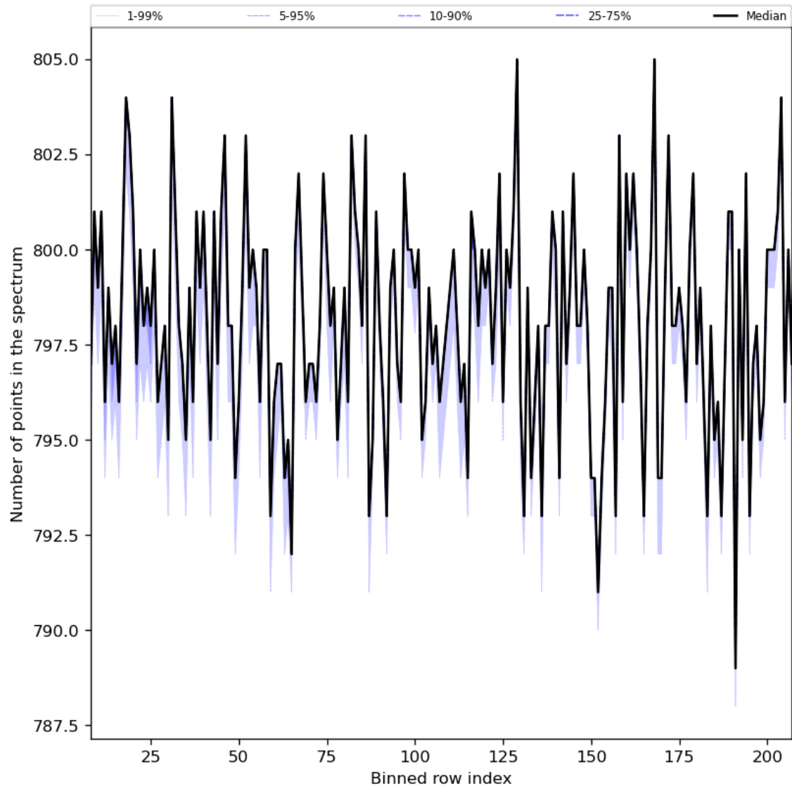
Figure 37: Along track statistics of “Number of points in the spectrum” for 2023-08-25 to 2023-08-26
