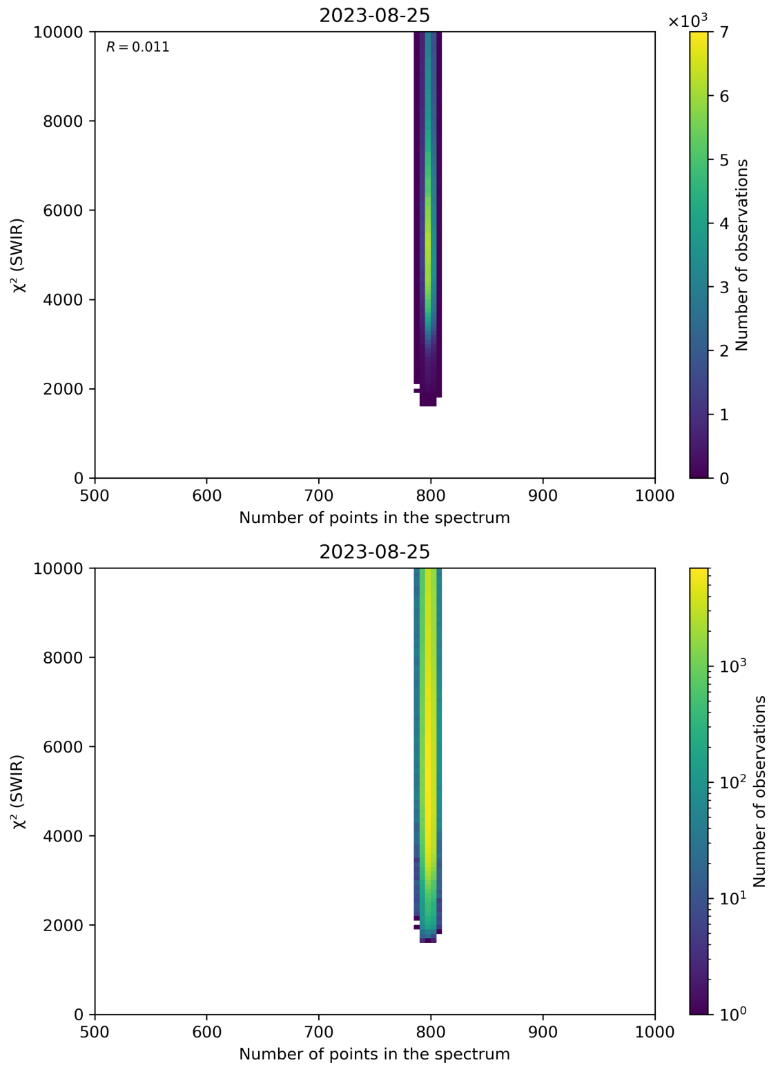
Figure 89: Scatter density plot of “Number of points in the spectrum” against “ \chi^2 (SWIR)” for 2023-08-25 to 2023-08-26.
