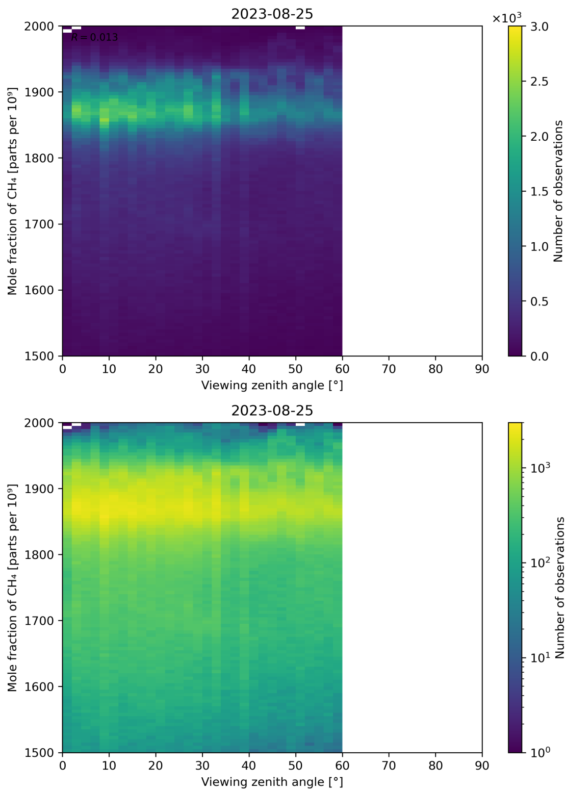
Figure 110: Scatter density plot of “Viewing zenith angle” against “Mole fraction of CH 4 ” for 2023-08-25 to 2023-08-26.
