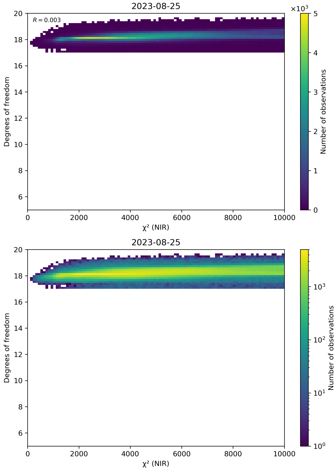
Figure 44: Scatter density plot of “ \chi^2 (NIR)” against “Degrees of freedom” for 2023-08-25 to 2023-08-26.
