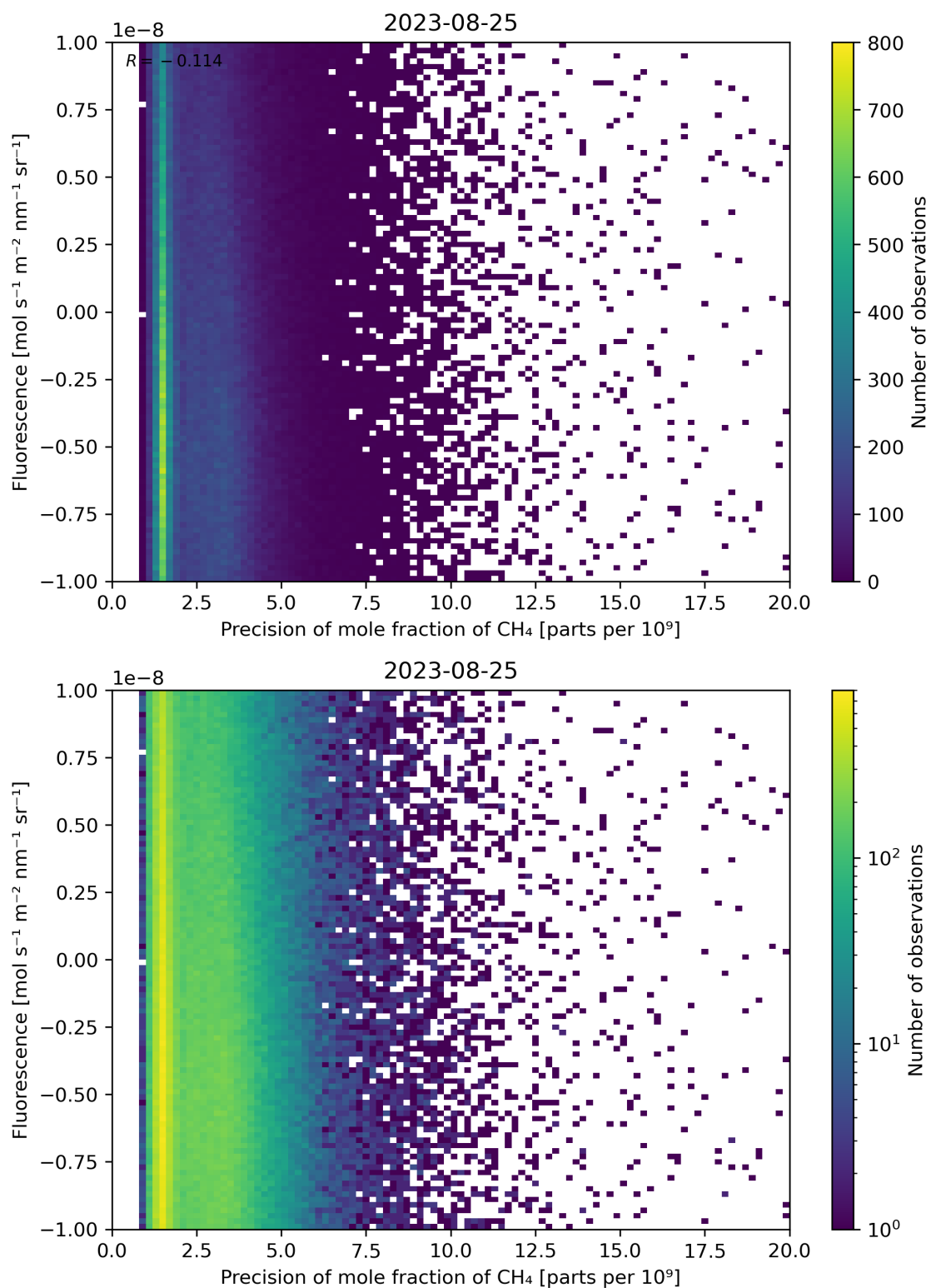
Figure 81: Scatter density plot of “Precision of mole fraction of \text{CH}_4 ” against “Fluorescence” for 2023-08-25 to 2023-08-26.
