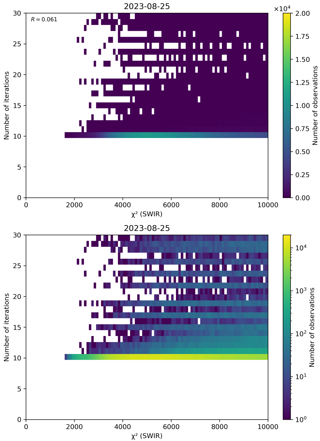
Figure 50: Scatter density plot of “ \chi^2 (SWIR)” against “Number of iterations” for 2023-08-25 to 2023-08-26.
