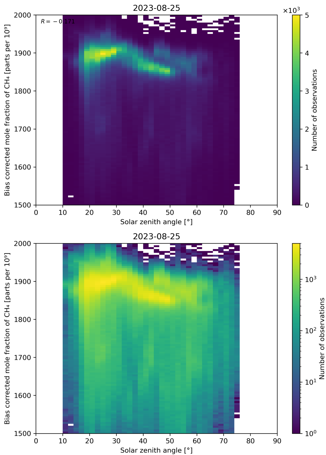
Figure 100: Scatter density plot of “Solar zenith angle” against “Bias corrected mole fraction of CH 4 ” for 2023-08-25 to 2023-08-26.
