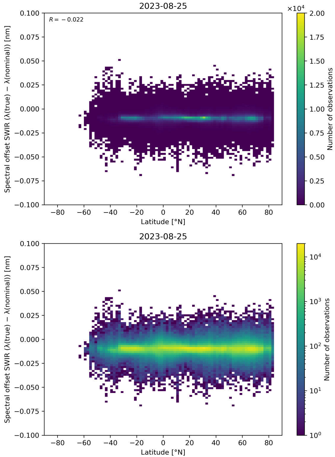
Figure 62: Scatter density plot of “Latitude” against “Spectral offset SWIR ( \lambda(\text{true}) - \lambda(\text{nominal}) )” for 2023-08-25 to 2023-08-26.
