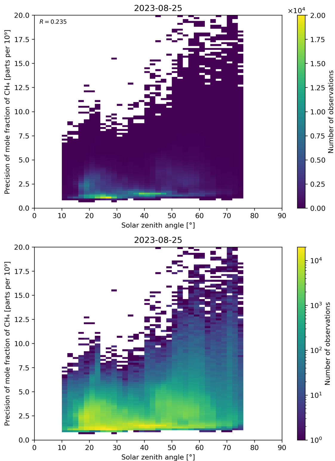
Figure 101: Scatter density plot of “Solar zenith angle” against “Precision of mole fraction of CH 4 ” for 2023-08-25 to 2023-08-26.
