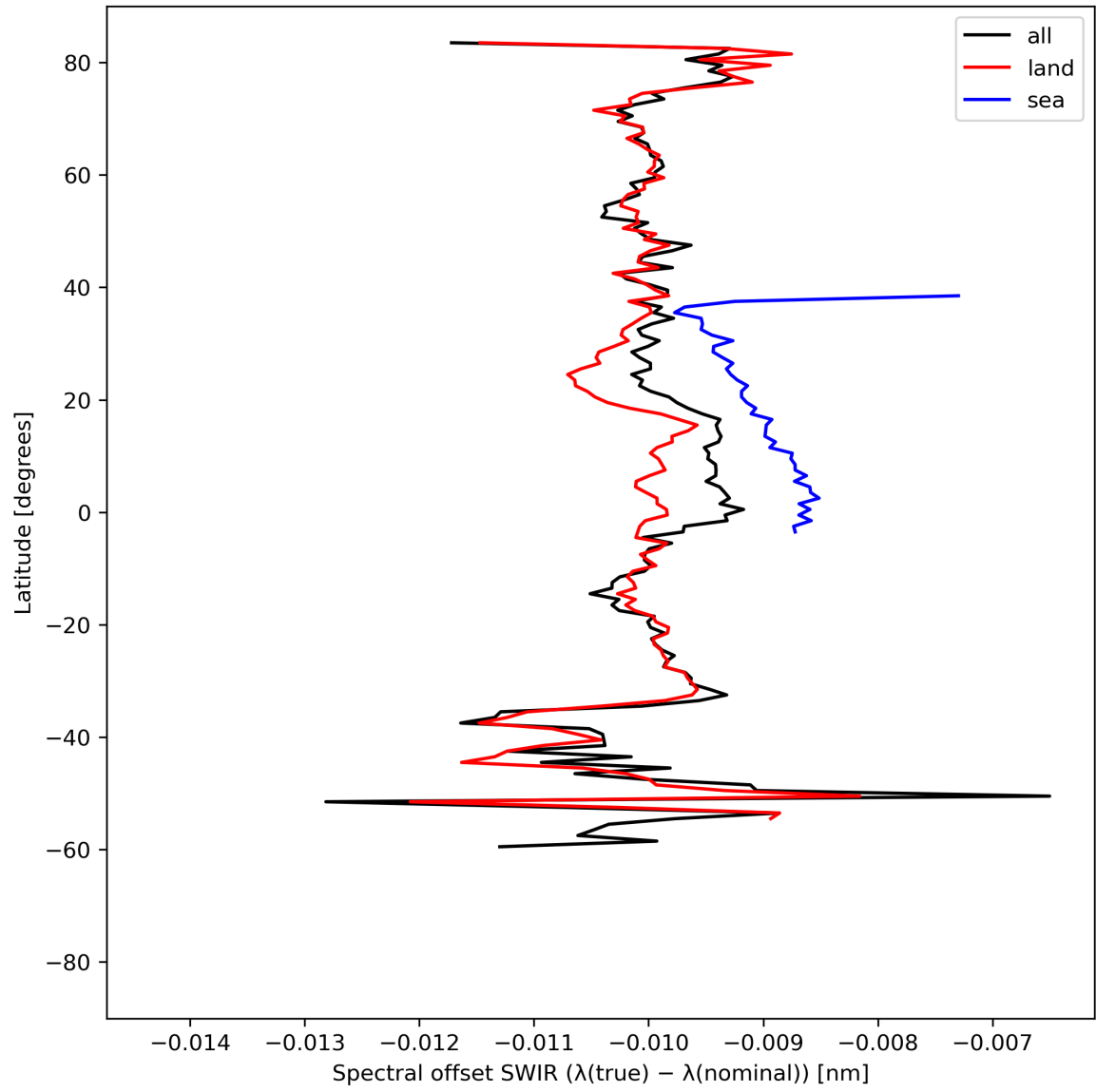
Figure 16: Zonal average of “Spectral offset SWIR ( \lambda(\text{true}) - \lambda(\text{nominal}) )” for 2023-08-25 to 2023-08-26.
