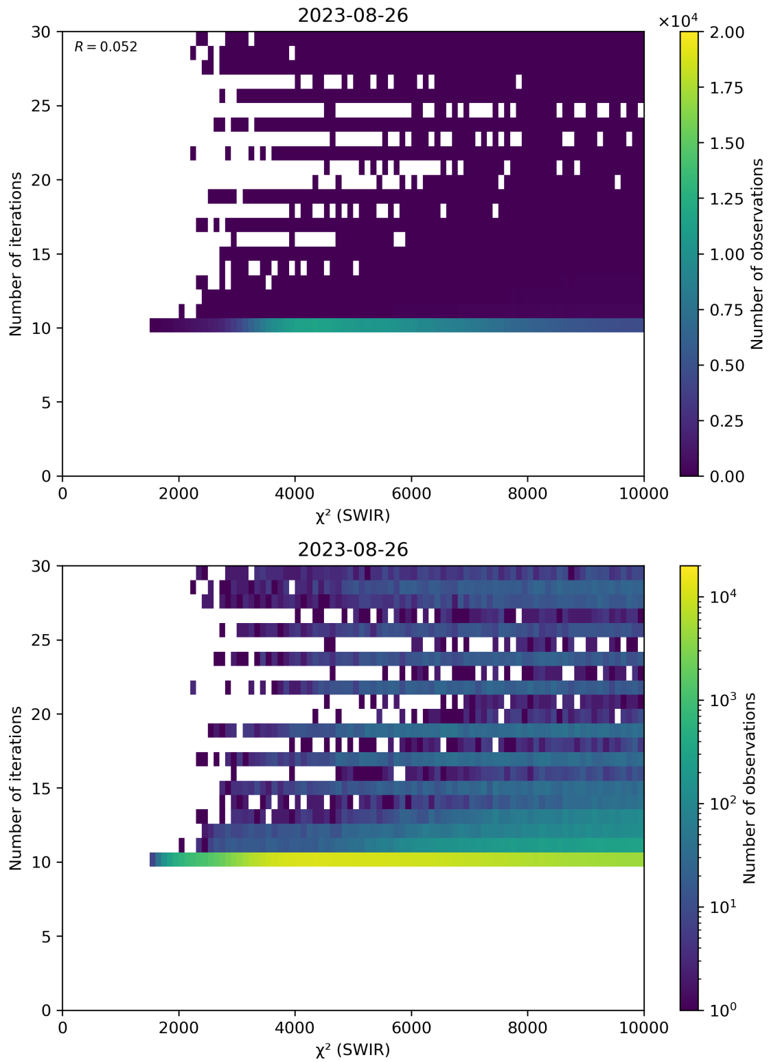
Figure 50: Scatter density plot of “ \chi^2 (SWIR)” against “Number of iterations” for 2023-08-25 to 2023-08-27.
