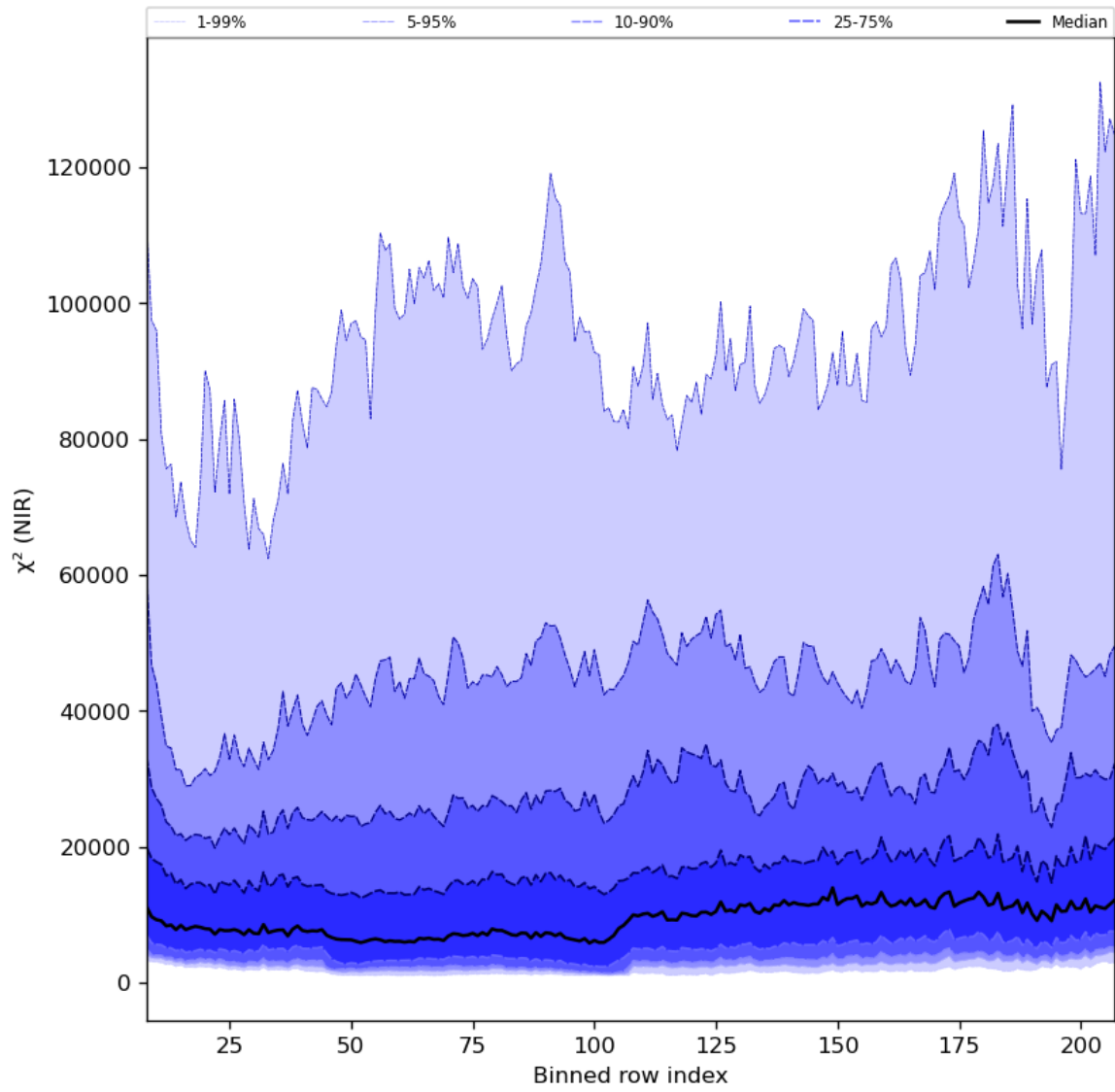
Figure 40: Along track statistics of " \chi^2 (NIR)" for 2023-08-25 to 2023-08-27
