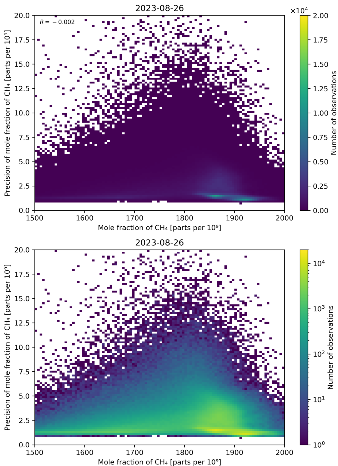
Figure 75: Scatter density plot of “Mole fraction of CH 4 ” against “Precision of mole fraction of CH 4 ” for 2023-08-25 to 2023-08-27.
