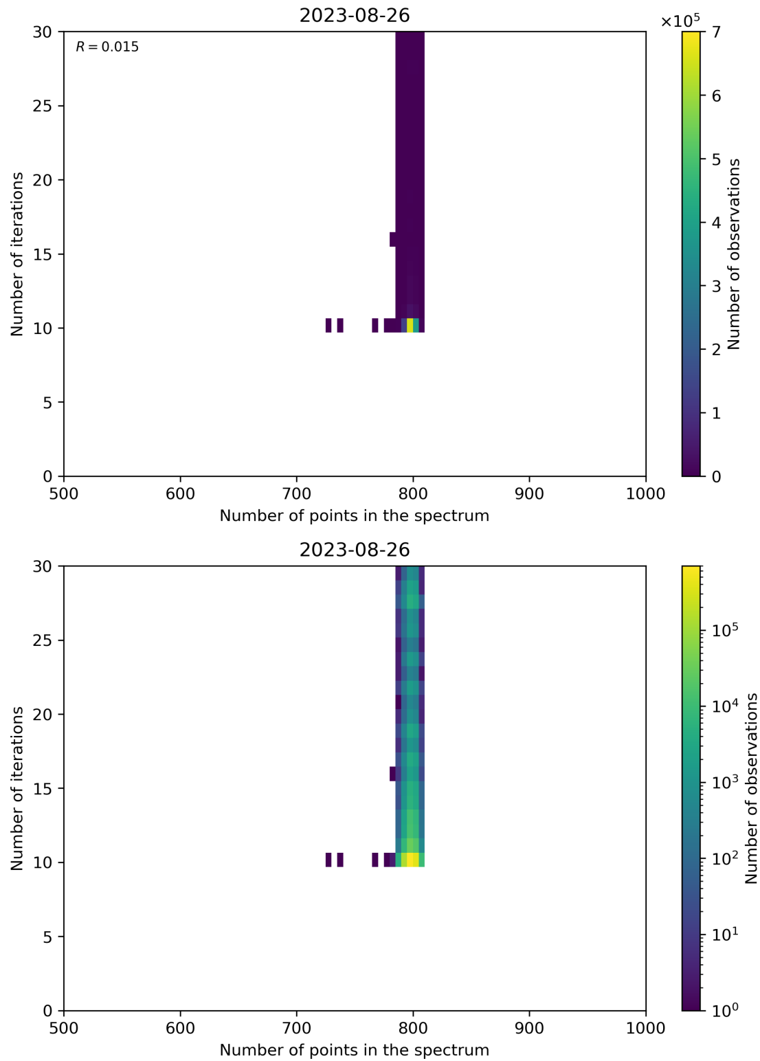
Figure 92: Scatter density plot of “Number of points in the spectrum” against “Number of iterations” for 2023-08-25 to 2023-08-27.
