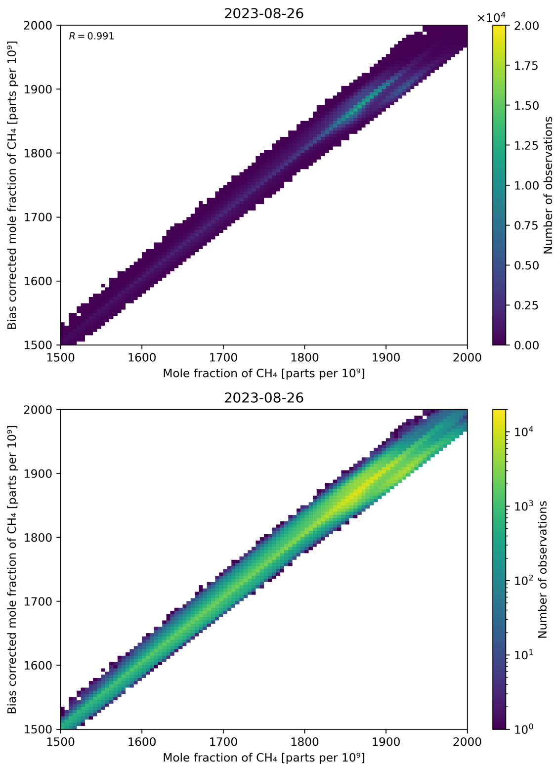
Figure 74: Scatter density plot of “Mole fraction of CH 4 ” against “Bias corrected mole fraction of CH 4 ” for 2023-08-25 to 2023-08-27.
