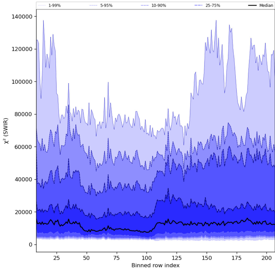
Figure 39: Along track statistics of “ \chi^2 (SWIR)” for 2023-08-25 to 2023-08-27
