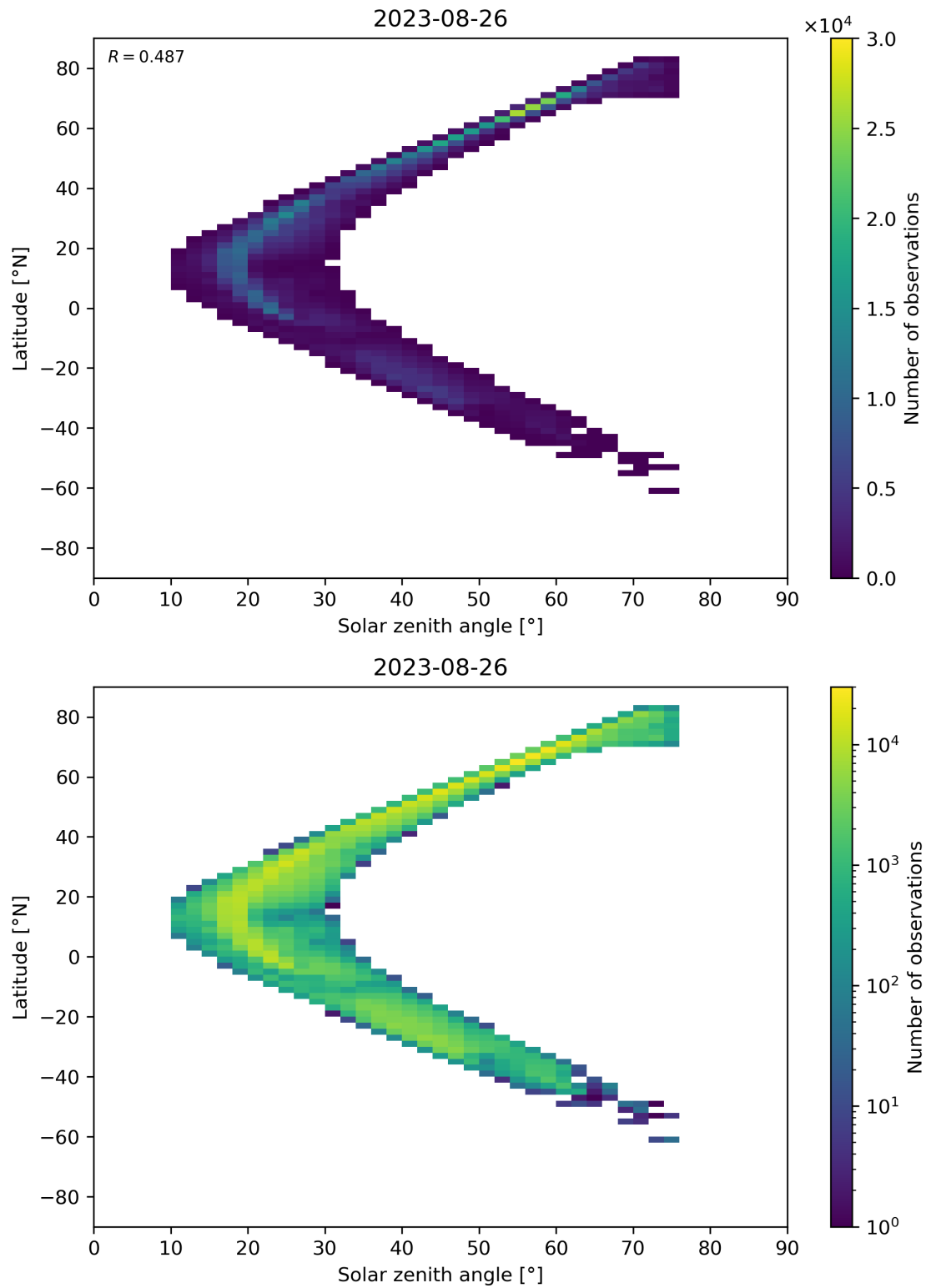
Figure 98: Scatter density plot of “Solar zenith angle” against “Latitude” for 2023-08-25 to 2023-08-27.
