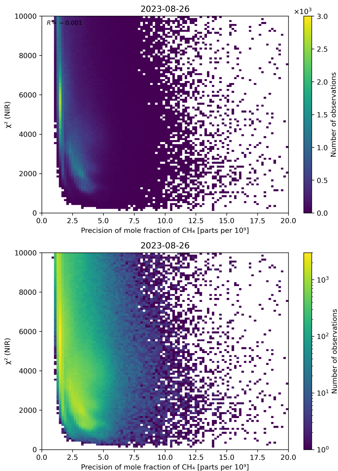
Figure 78: Scatter density plot of “Precision of mole fraction of CH 4 ” against “ \chi^2 (NIR)” for 2023-08-25 to 2023-08-27.
