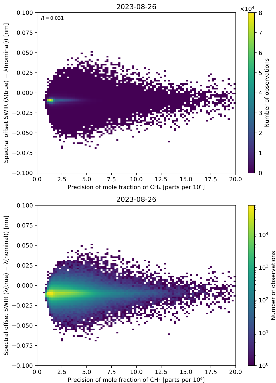
Figure 85: Scatter density plot of “Precision of mole fraction of CH 4 ” against “Spectral offset SWIR ( \lambda(\text{true}) - \lambda(\text{nominal}) )” for 2023-08-25 to 2023-08-27.
