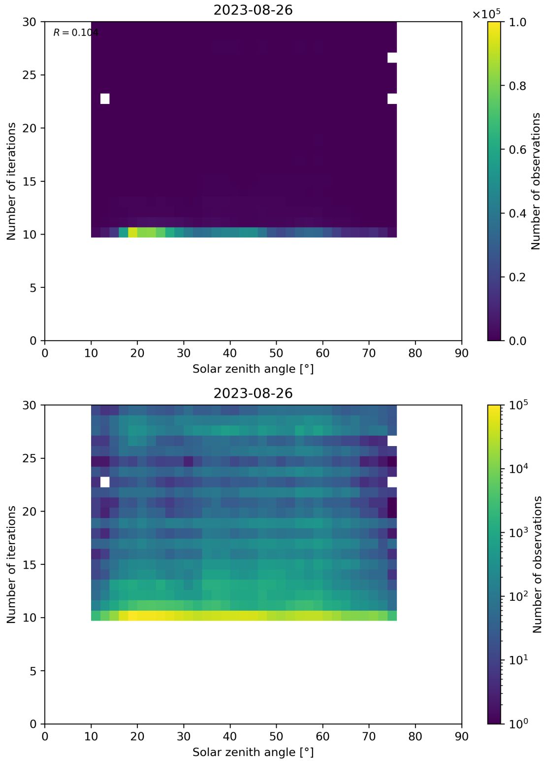
Figure 102: Scatter density plot of “Solar zenith angle” against “Number of iterations” for 2023-08-25 to 2023-08-27.
