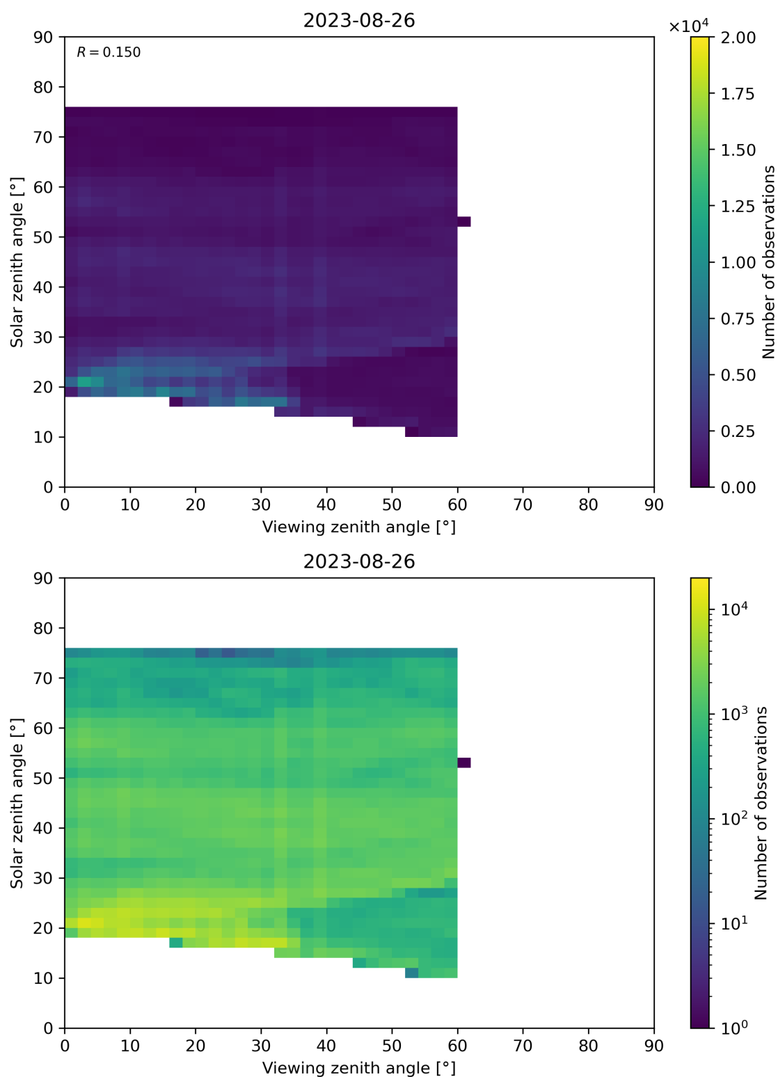
Figure 115: Scatter density plot of “Viewing zenith angle” against “Solar zenith angle” for 2023-08-25 to 2023-08-27.
