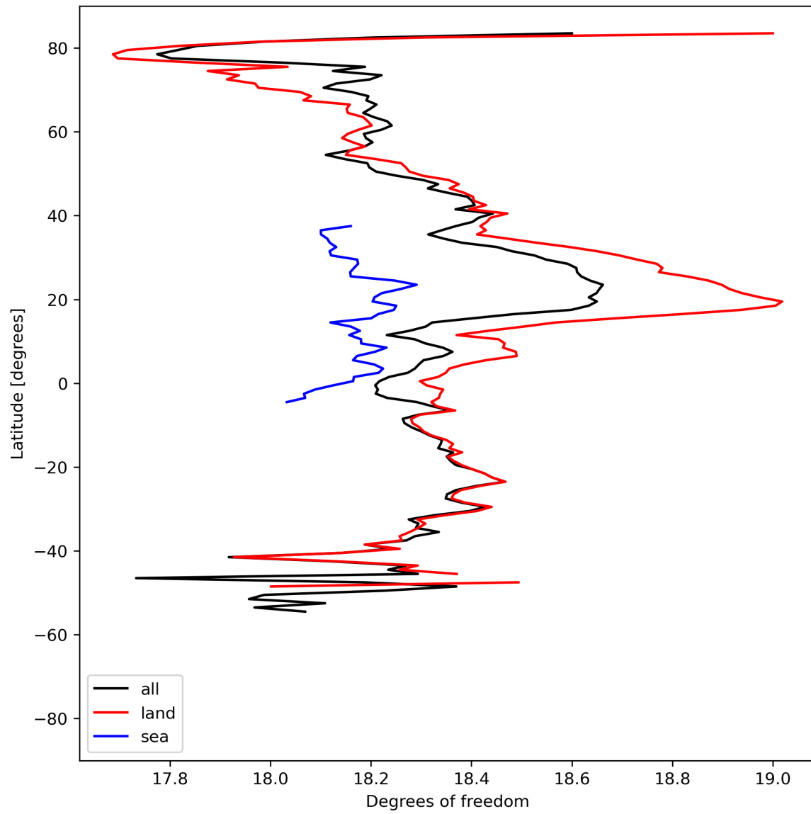
Figure 19: Zonal average of “Degrees of freedom” for 2023-08-25 to 2023-08-27.
