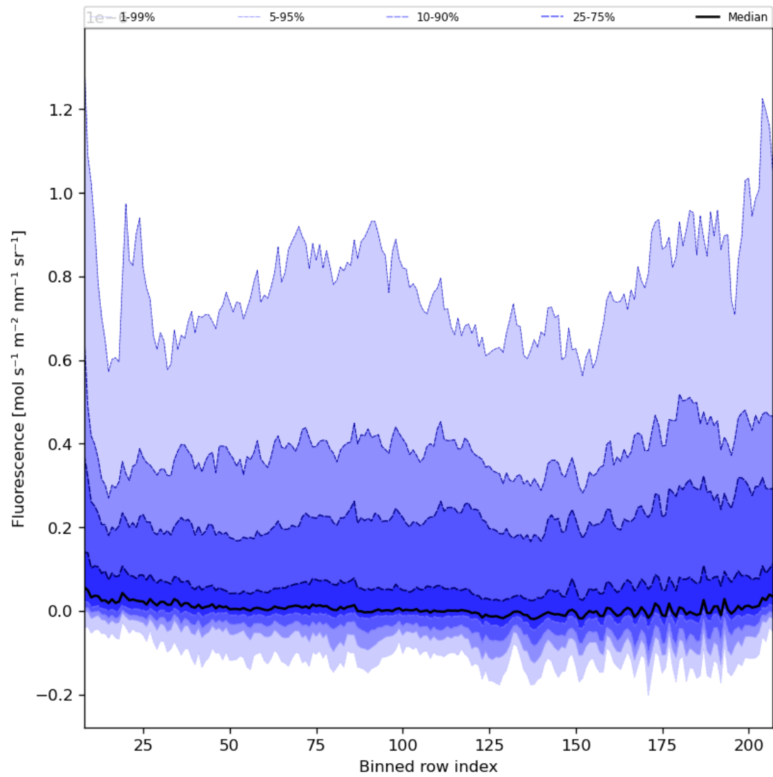
Figure 43: Along track statistics of “Fluorescence” for 2023-08-25 to 2023-08-27
