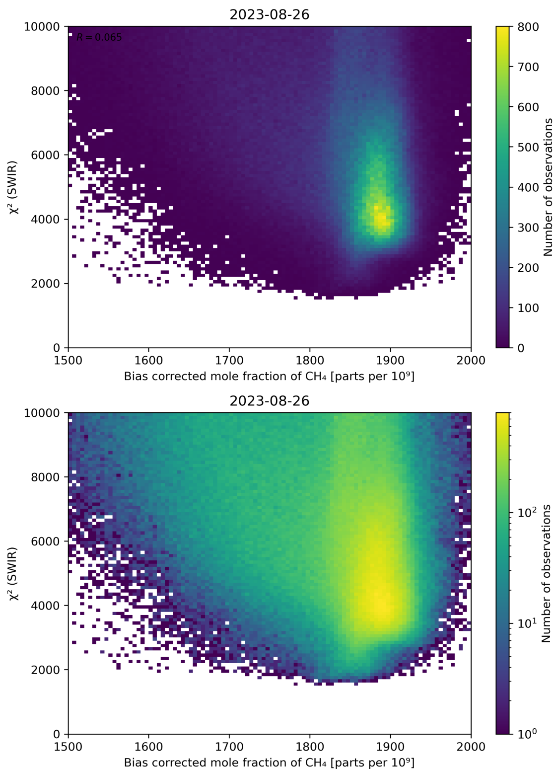
Figure 64: Scatter density plot of “Bias corrected mole fraction of CH 4 ” against “ \chi^2 (SWIR)” for 2023-08-25 to 2023-08-27.
