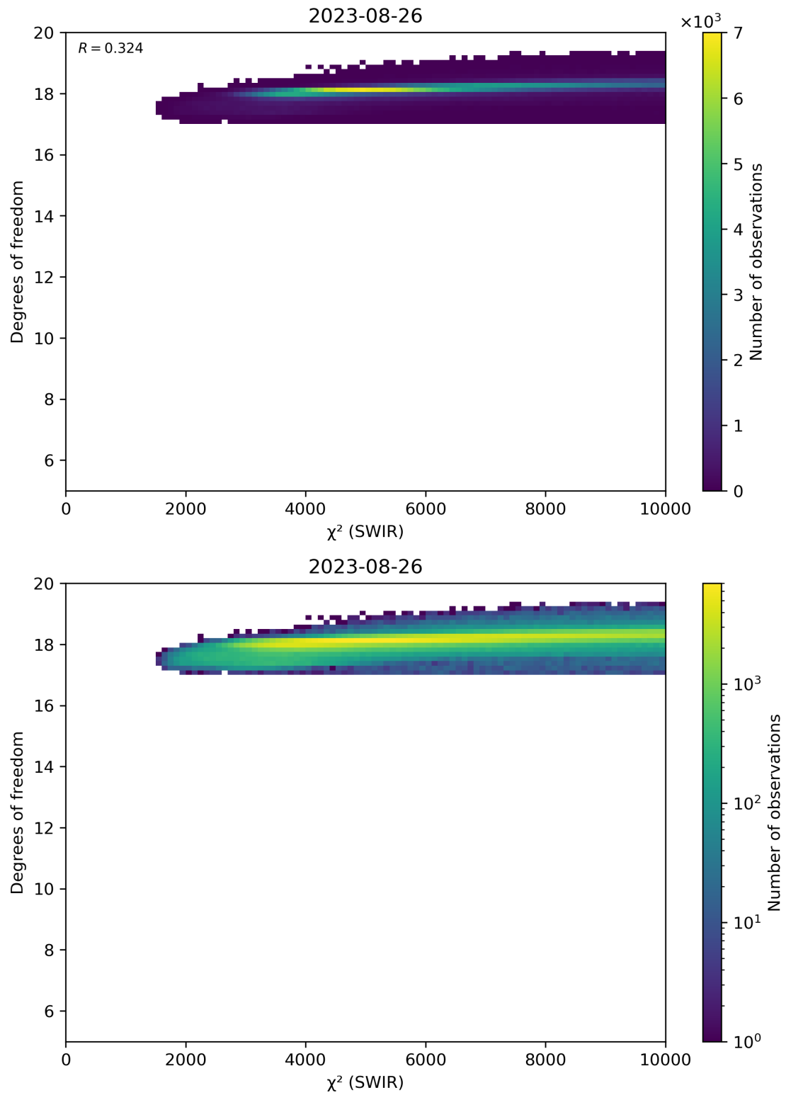
Figure 48: Scatter density plot of “ \chi^2 (SWIR)” against “Degrees of freedom” for 2023-08-25 to 2023-08-27.
