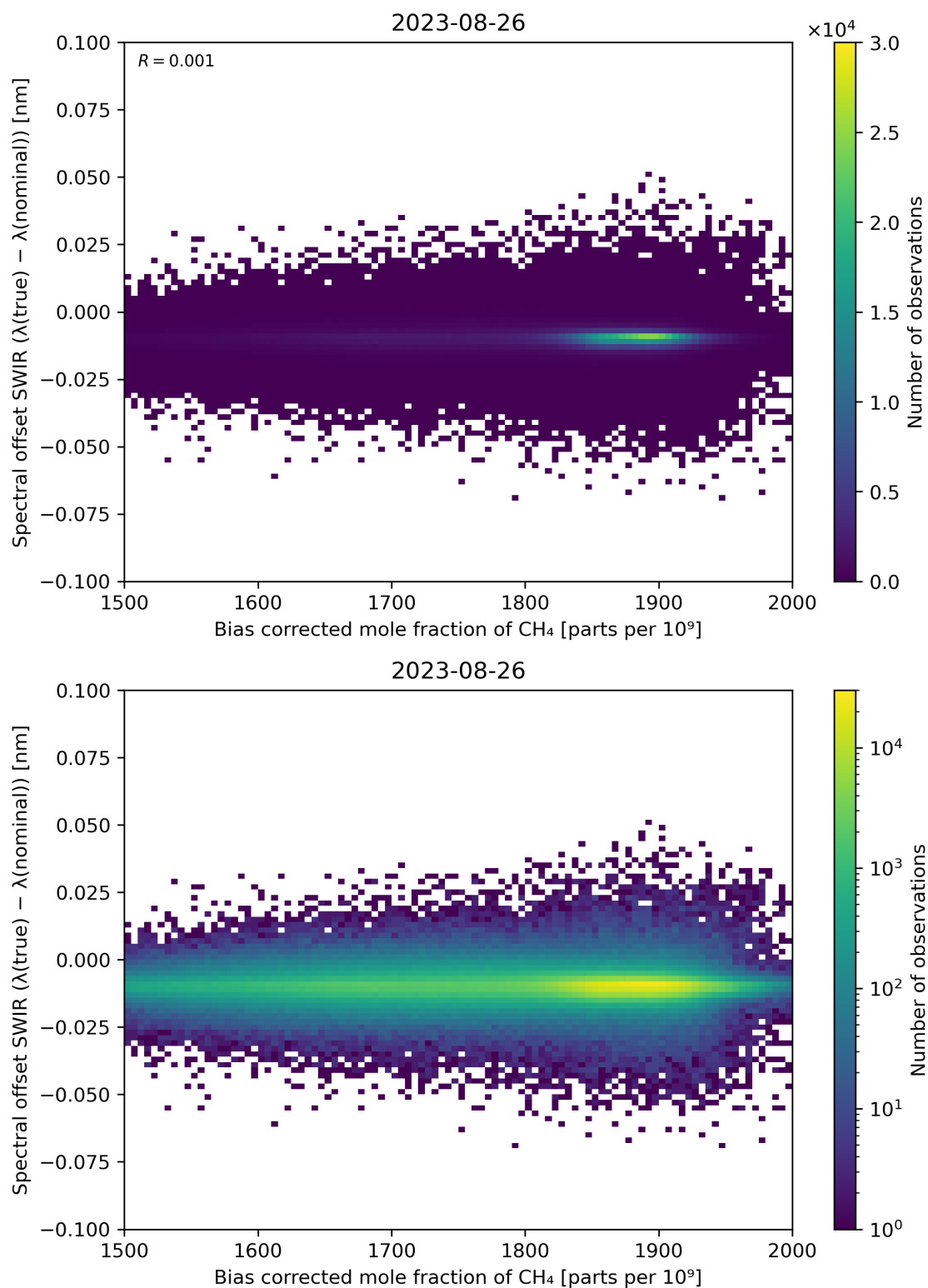
Figure 69: Scatter density plot of “Bias corrected mole fraction of \text{CH}_4 ” against “Spectral offset SWIR ( \lambda(\text{true}) - \lambda(\text{nominal}) )” for 2023-08-25 to 2023-08-27.
