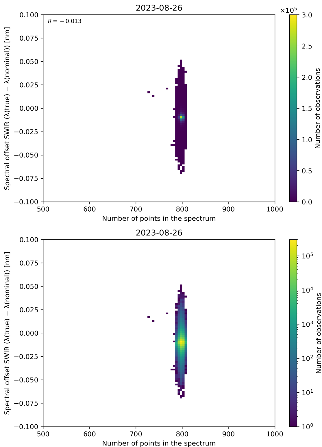
Figure 93: Scatter density plot of “Number of points in the spectrum” against “Spectral offset SWIR ( \lambda(\text{true}) - \lambda(\text{nominal}) )” for 2023-08-25 to 2023-08-27.
