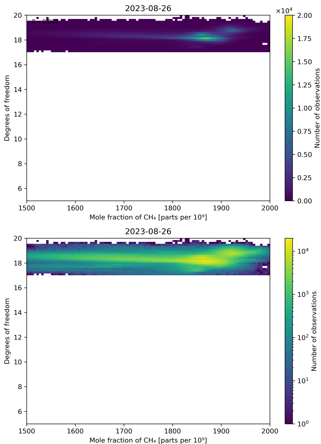
Figure 72: Scatter density plot of “Mole fraction of CH 4 ” against “Degrees of freedom” for 2023-08-25 to 2023-08-27.
