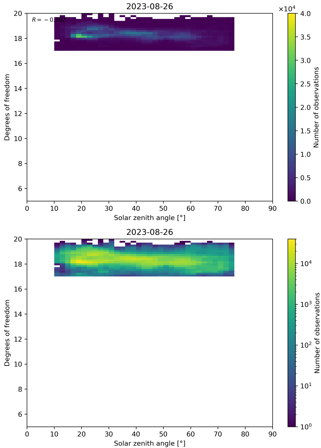
Figure 96: Scatter density plot of “Solar zenith angle” against “Degrees of freedom” for 2023-08-25 to 2023-08-27.
