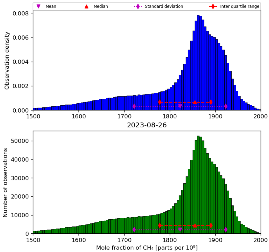
Figure 23: Histogram of “Mole fraction of CH 4 ” for 2023-08-25 to 2023-08-27
