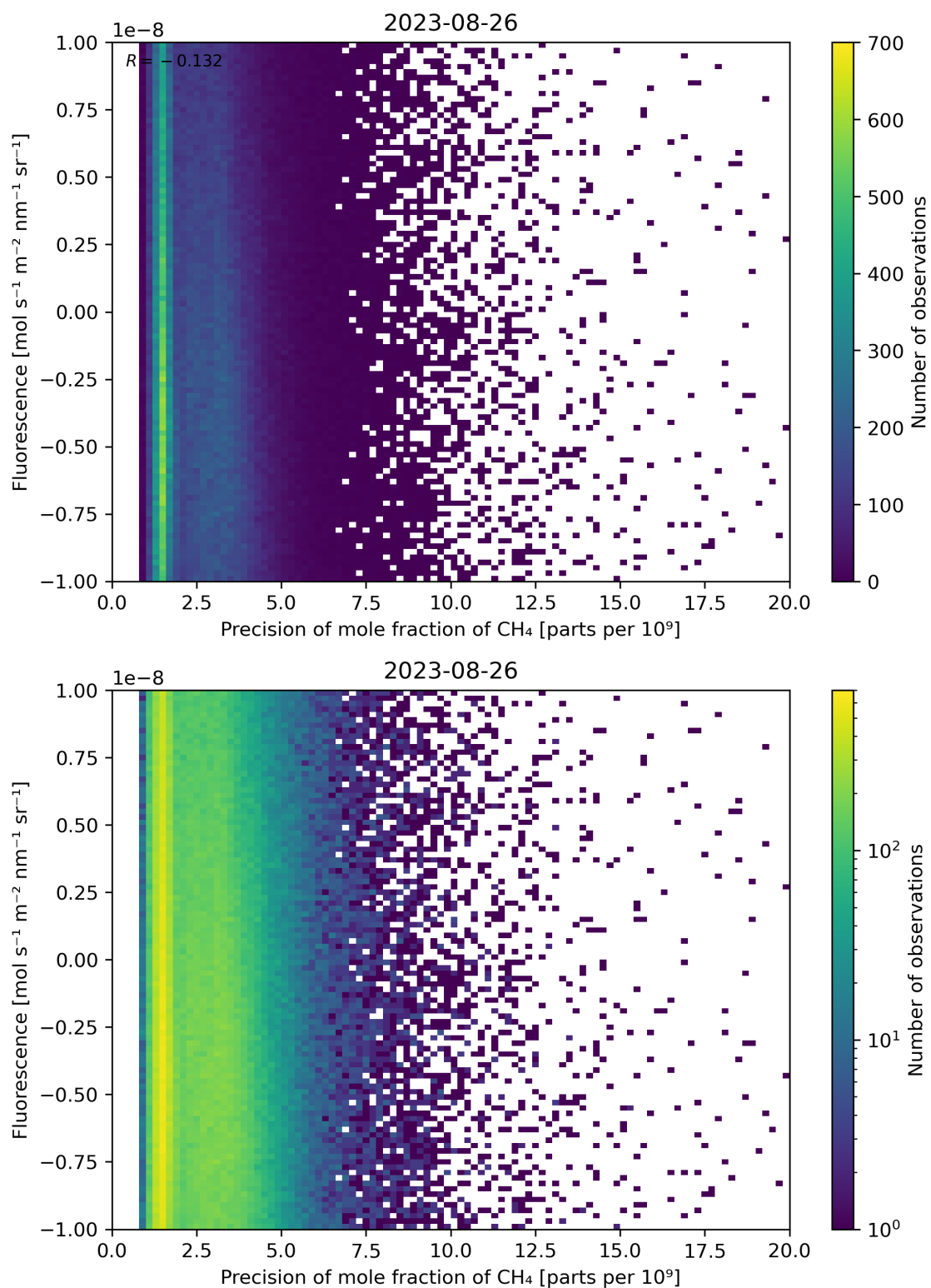
Figure 81: Scatter density plot of “Precision of mole fraction of \text{CH}_4 ” against “Fluorescence” for 2023-08-25 to 2023-08-27.
