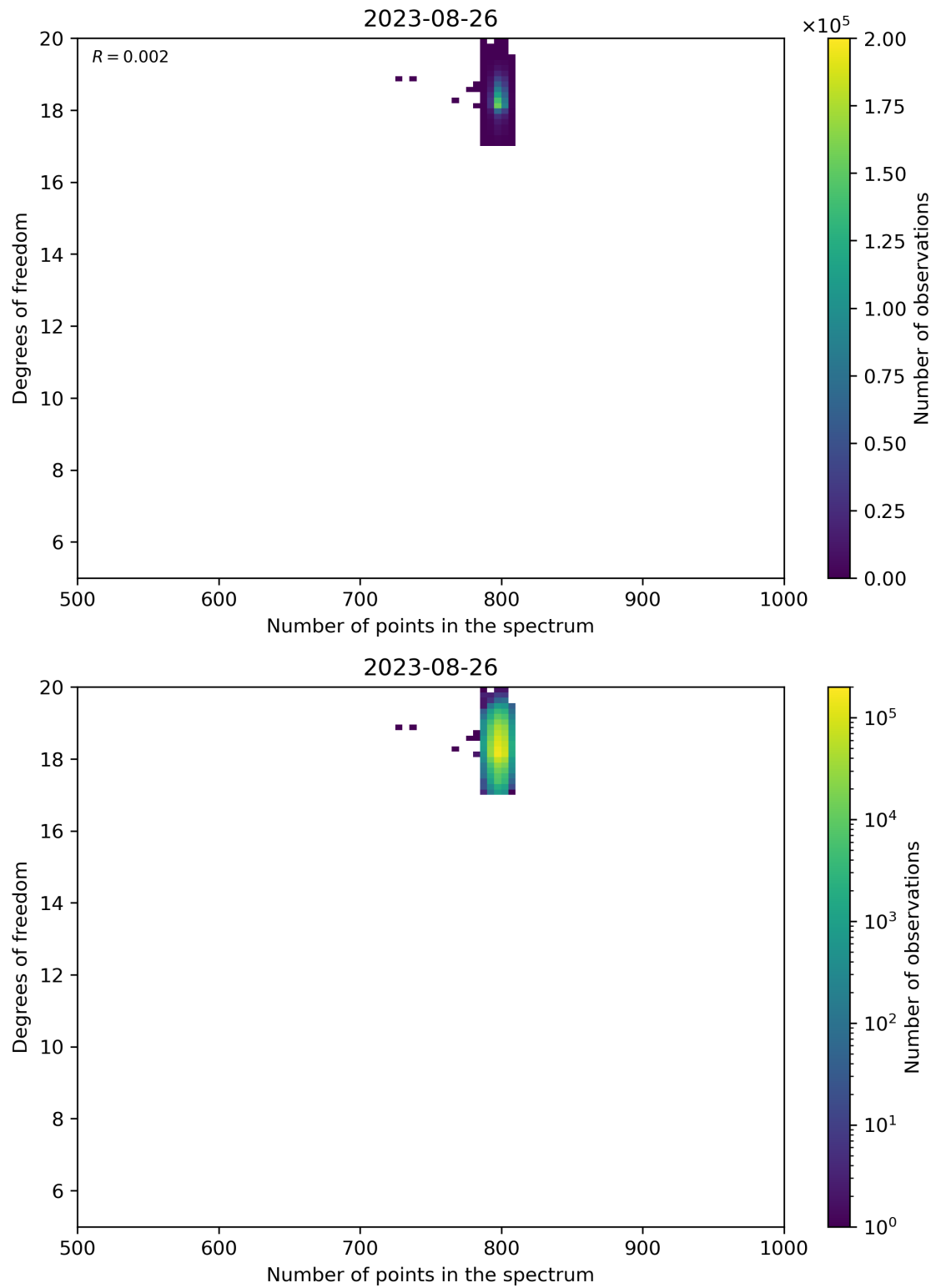
Figure 90: Scatter density plot of “Number of points in the spectrum” against “Degrees of freedom” for 2023-08-25 to 2023-08-27.
