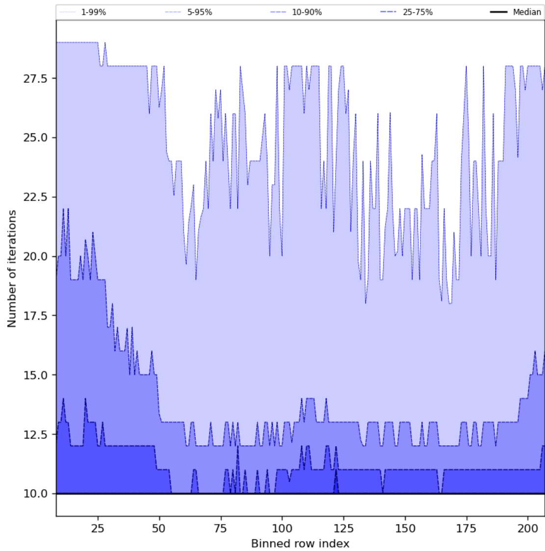
Figure 42: Along track statistics of “Number of iterations” for 2023-08-25 to 2023-08-27
