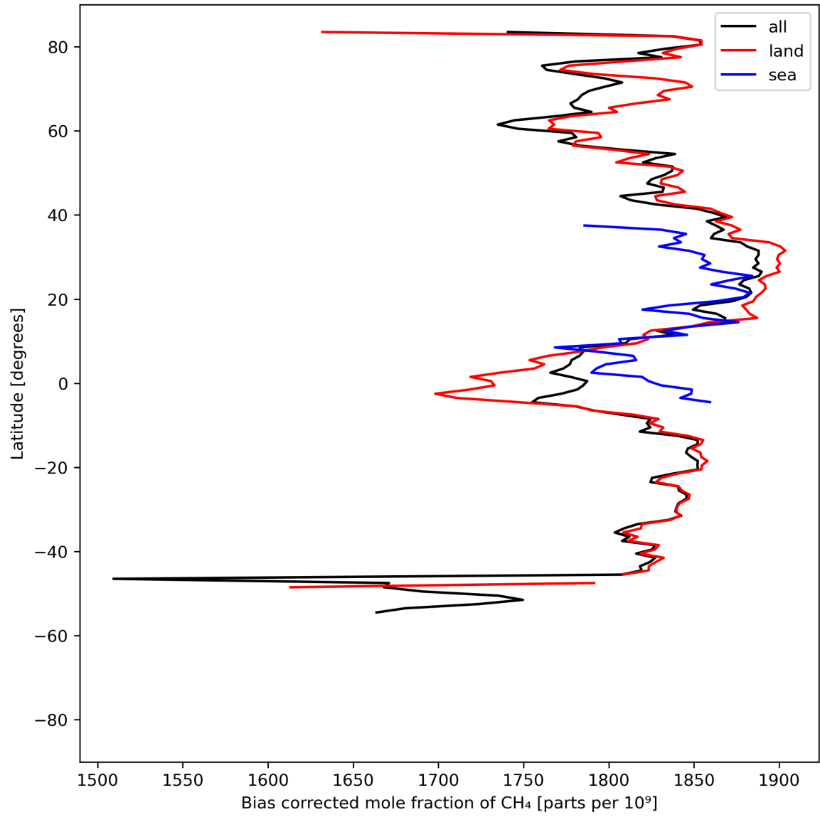
Figure 14: Zonal average of “Bias corrected mole fraction of \text{CH}_4 ” for 2023-08-25 to 2023-08-27.
