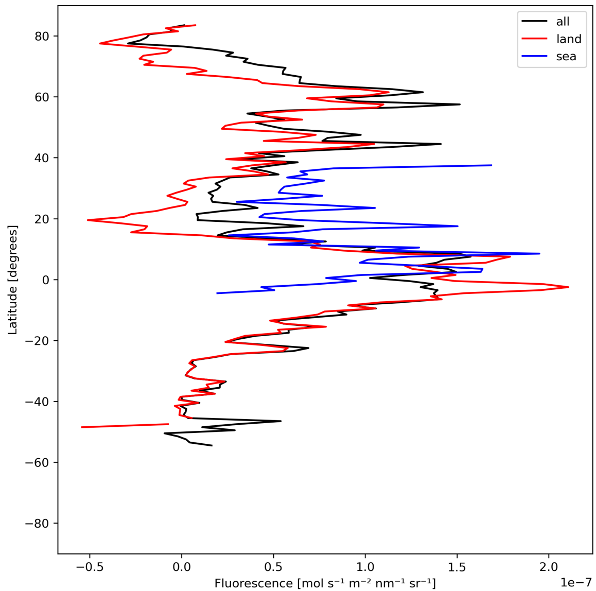
Figure 21: Zonal average of “Fluorescence” for 2023-08-25 to 2023-08-27.
