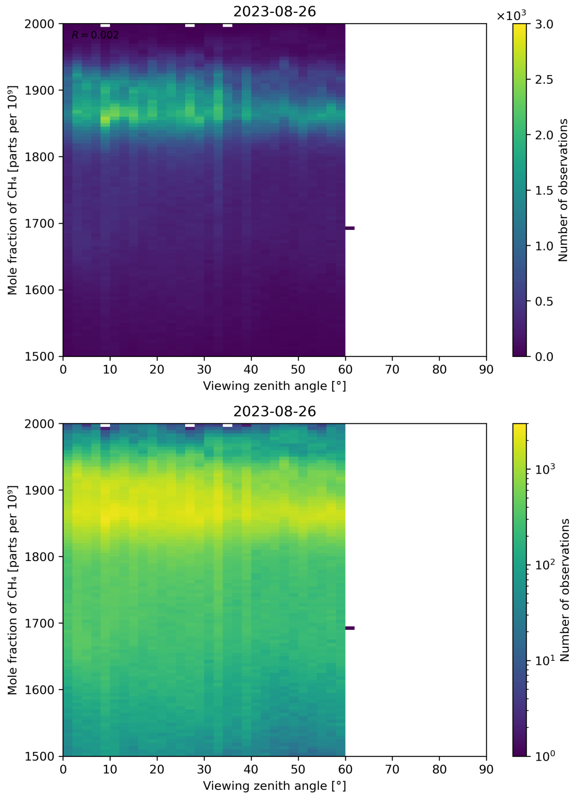
Figure 110: Scatter density plot of “Viewing zenith angle” against “Mole fraction of CH 4 ” for 2023-08-25 to 2023-08-27.
