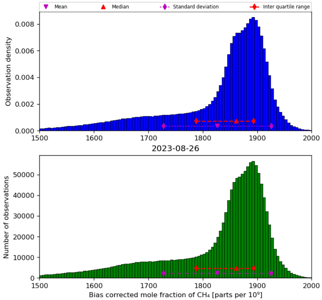
Figure 25: Histogram of “Bias corrected mole fraction of CH 4 ” for 2023-08-25 to 2023-08-27
