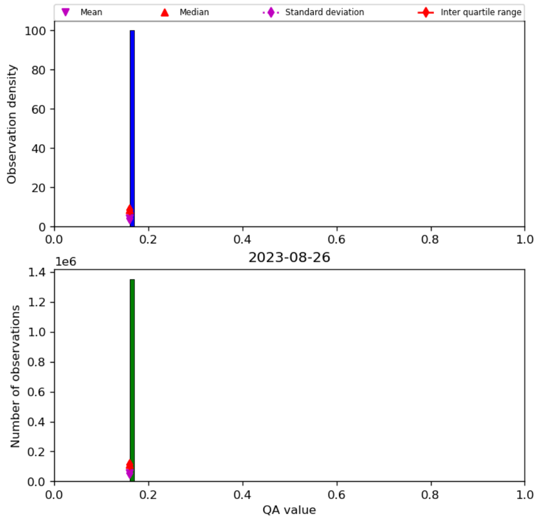
Figure 22: Histogram of “QA value” for 2023-08-25 to 2023-08-27
