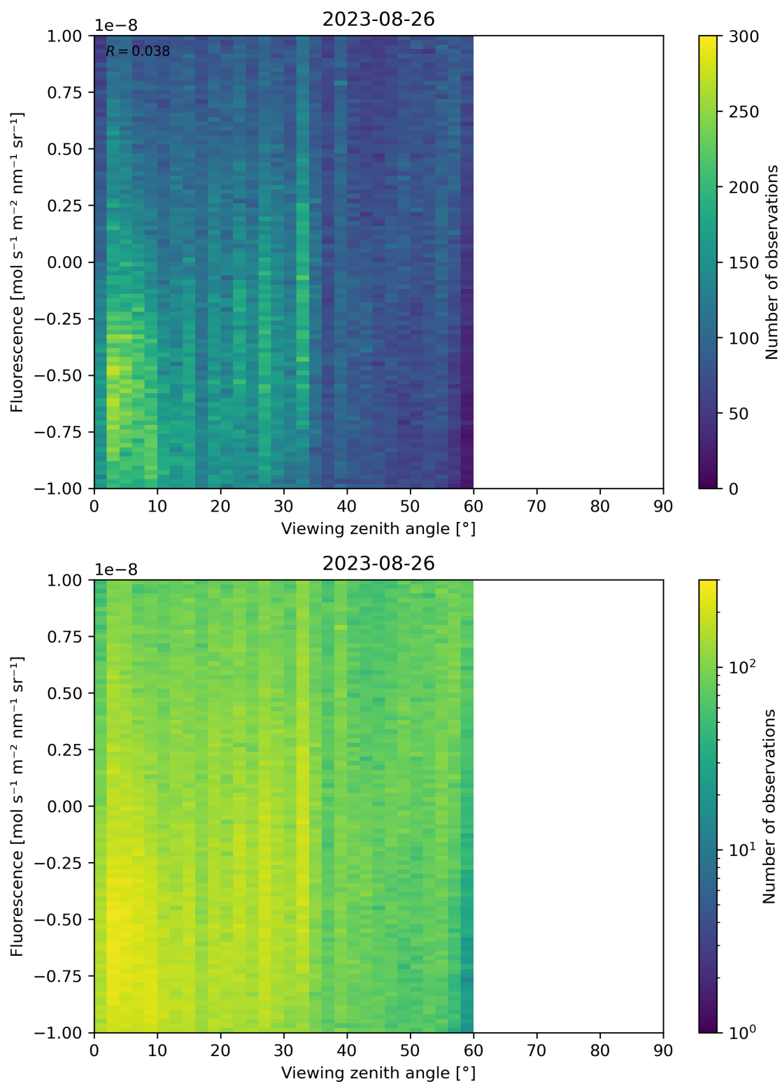
Figure 108: Scatter density plot of “Viewing zenith angle” against “Fluorescence” for 2023-08-25 to 2023-08-27.
