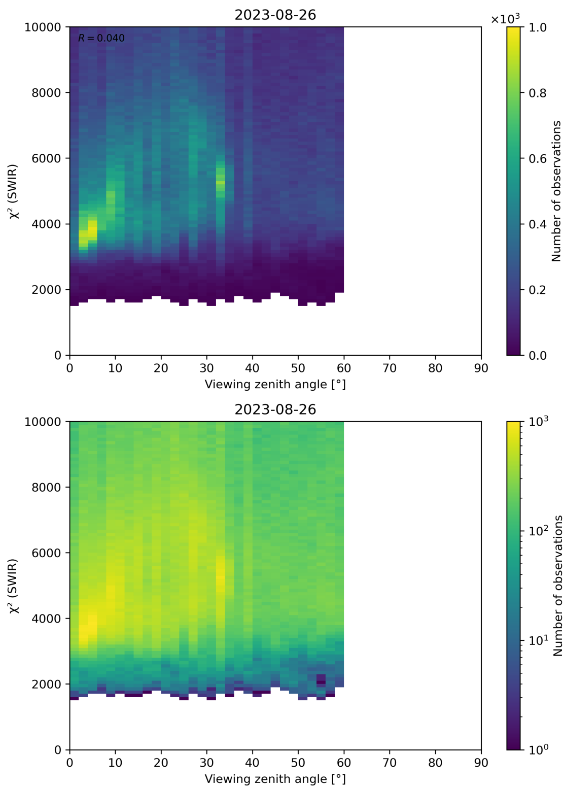
Figure 106: Scatter density plot of “Viewing zenith angle” against “ \chi^2 (SWIR)” for 2023-08-25 to 2023-08-27.
