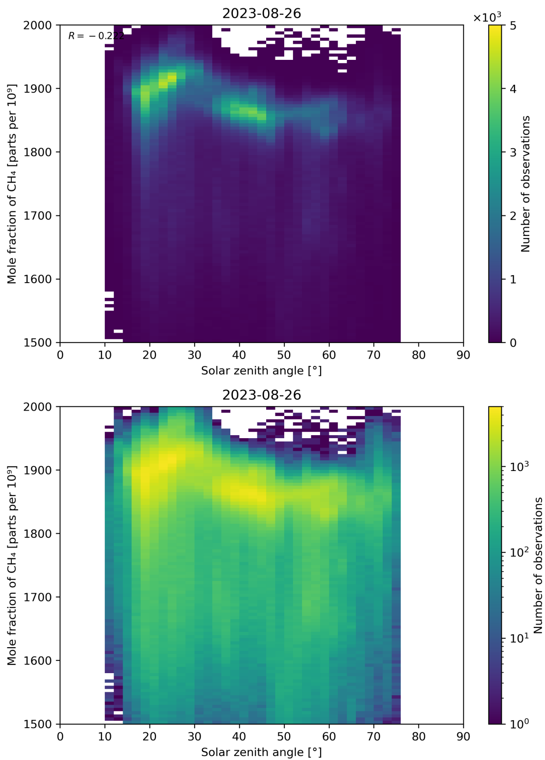
Figure 99: Scatter density plot of “Solar zenith angle” against “Mole fraction of CH 4 ” for 2023-08-25 to 2023-08-27.
