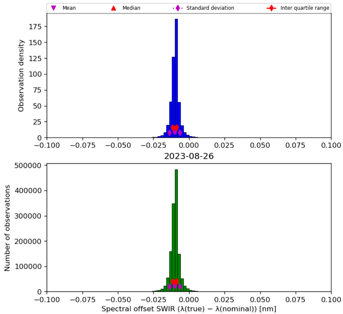
Figure 27: Histogram of “Spectral offset SWIR ( \lambda(\text{true}) - \lambda(\text{nominal}) )” for 2023-08-25 to 2023-08-27
