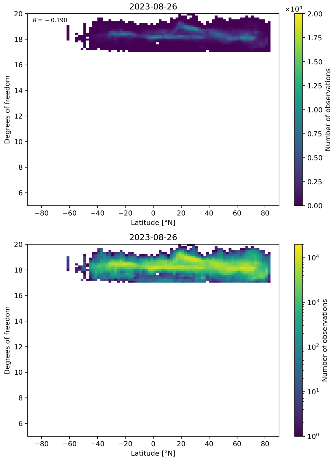
Figure 55: Scatter density plot of “Latitude” against “Degrees of freedom” for 2023-08-25 to 2023-08-27.
