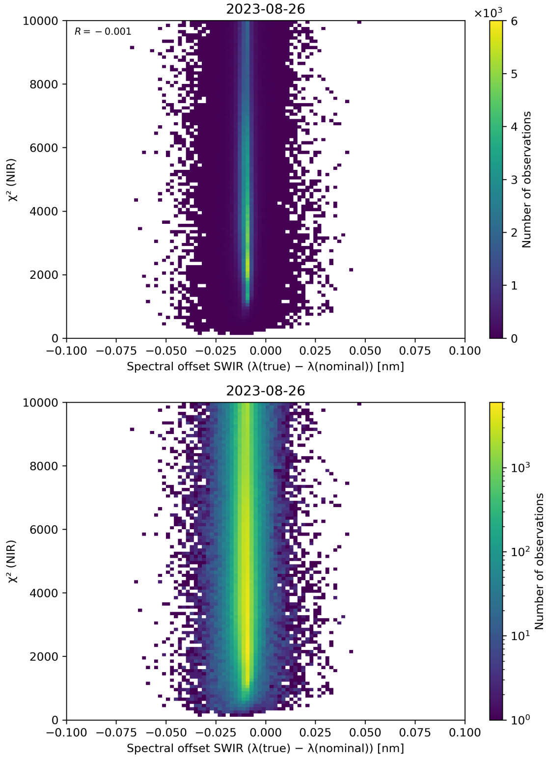
Figure 117: Scatter density plot of “Spectral offset SWIR ( \lambda(\text{true}) - \lambda(\text{nominal}) )” against “ \chi^2 (NIR)” for 2023-08-25 to 2023-08-27.
