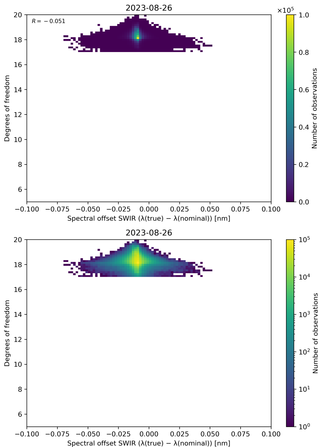
Figure 119: Scatter density plot of “Spectral offset SWIR ( \lambda(\text{true}) - \lambda(\text{nominal}) )” against “Degrees of freedom” for 2023-08-25 to 2023-08-27.
