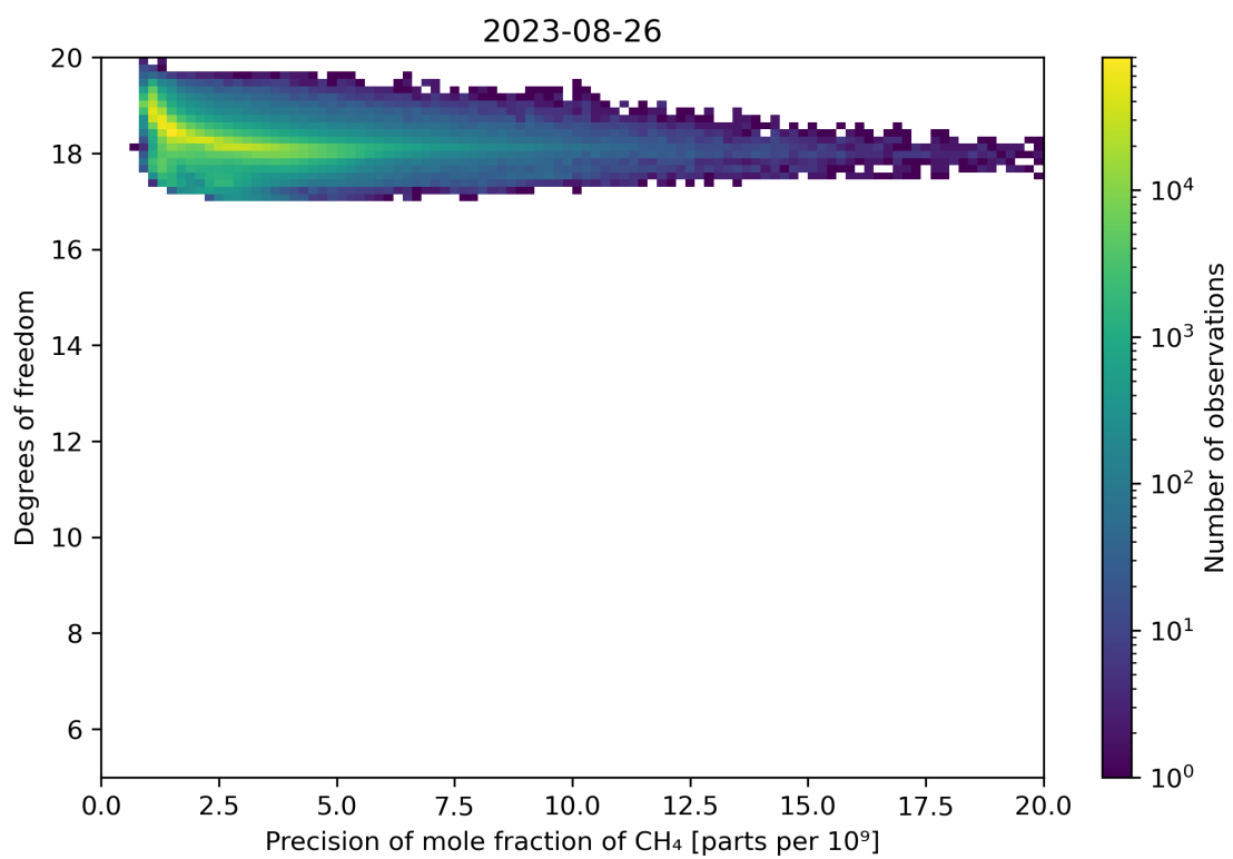
Figure 80: Scatter density plot of “Precision of mole fraction of CH 4 ” against “Degrees of freedom” for 2023-08-25 to 2023-08-27.
