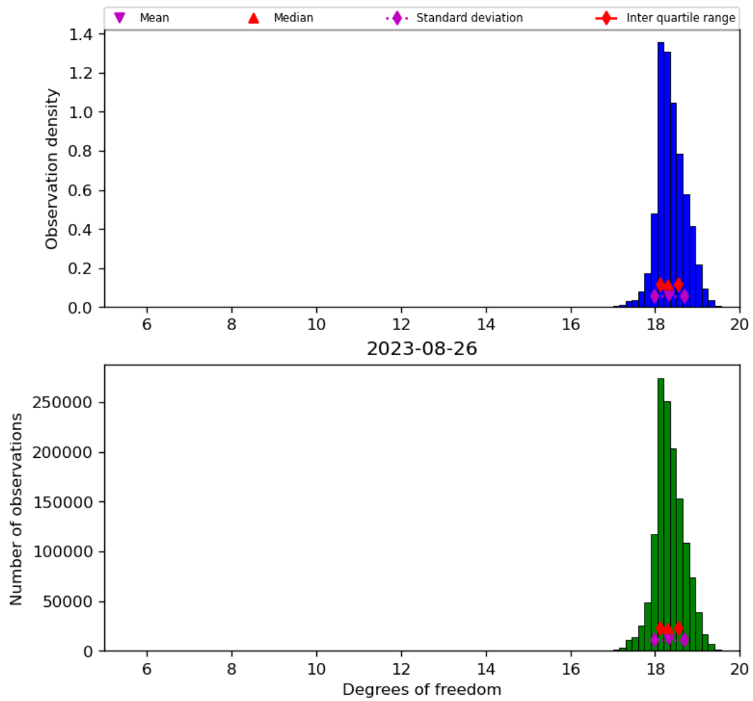
Figure 30: Histogram of “Degrees of freedom” for 2023-08-25 to 2023-08-27
