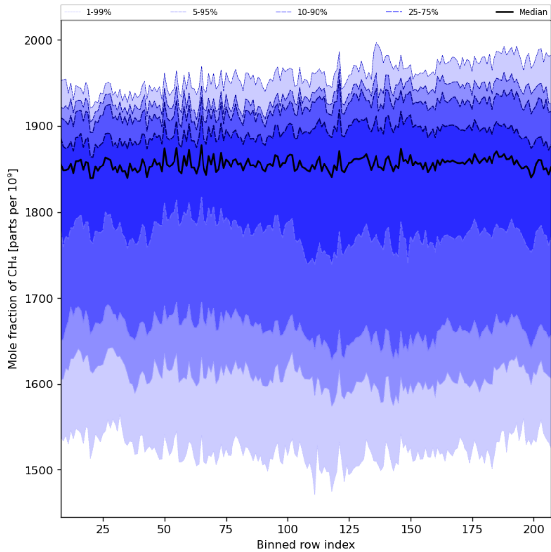
Figure 34: Along track statistics of “Mole fraction of CH 4 ” for 2023-08-25 to 2023-08-27
