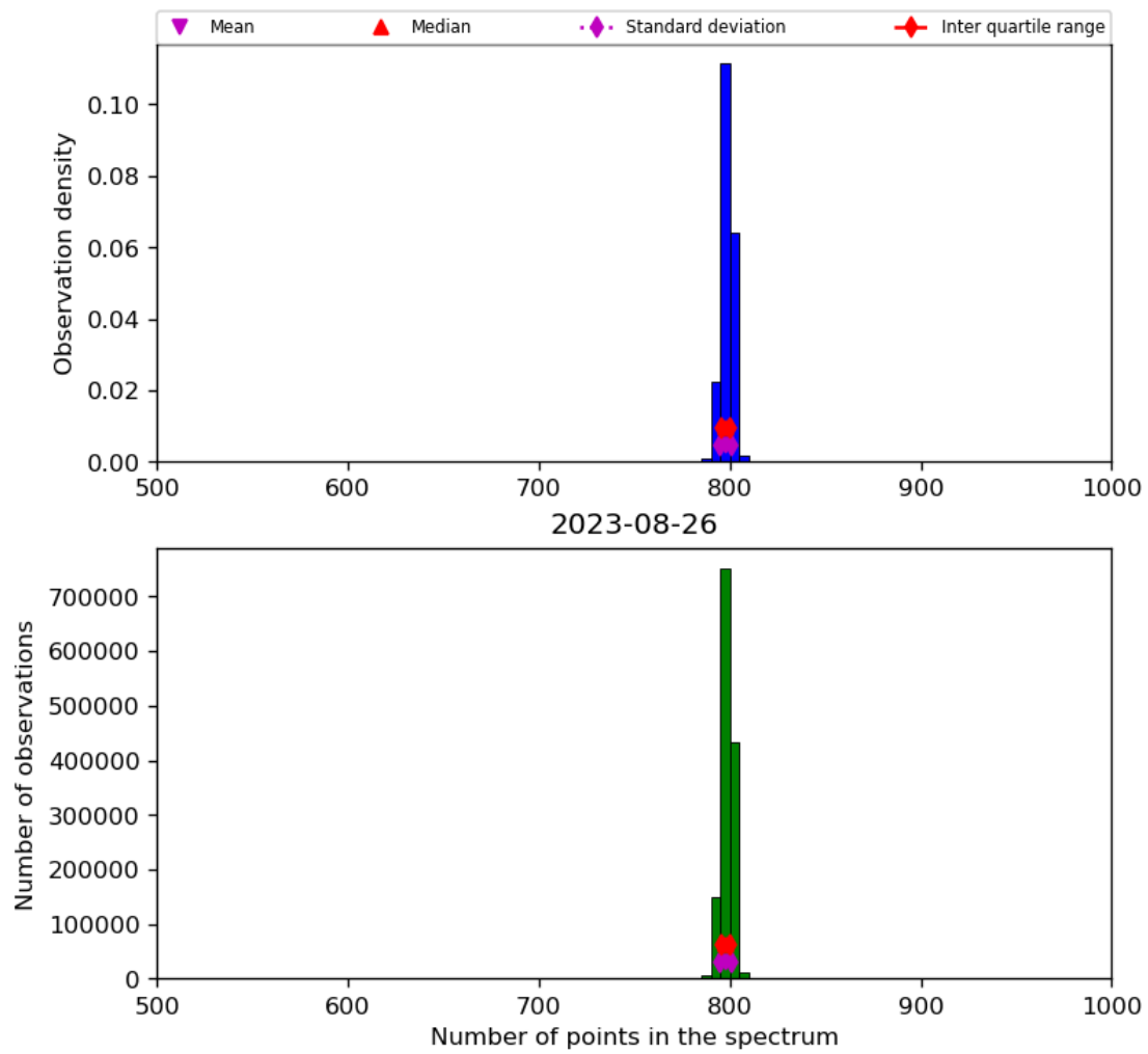
Figure 26: Histogram of “Number of points in the spectrum” for 2023-08-25 to 2023-08-27
