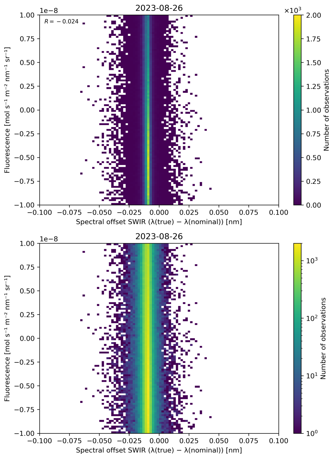
Figure 120: Scatter density plot of “Spectral offset SWIR ( \lambda(\text{true}) - \lambda(\text{nominal}) )” against “Fluorescence” for 2023-08-25 to 2023-08-27.
