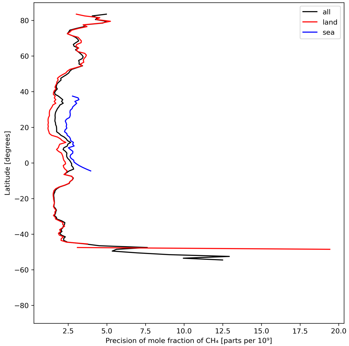
Figure 13: Zonal average of “Precision of mole fraction of CH 4 ” for 2023-08-25 to 2023-08-27.
