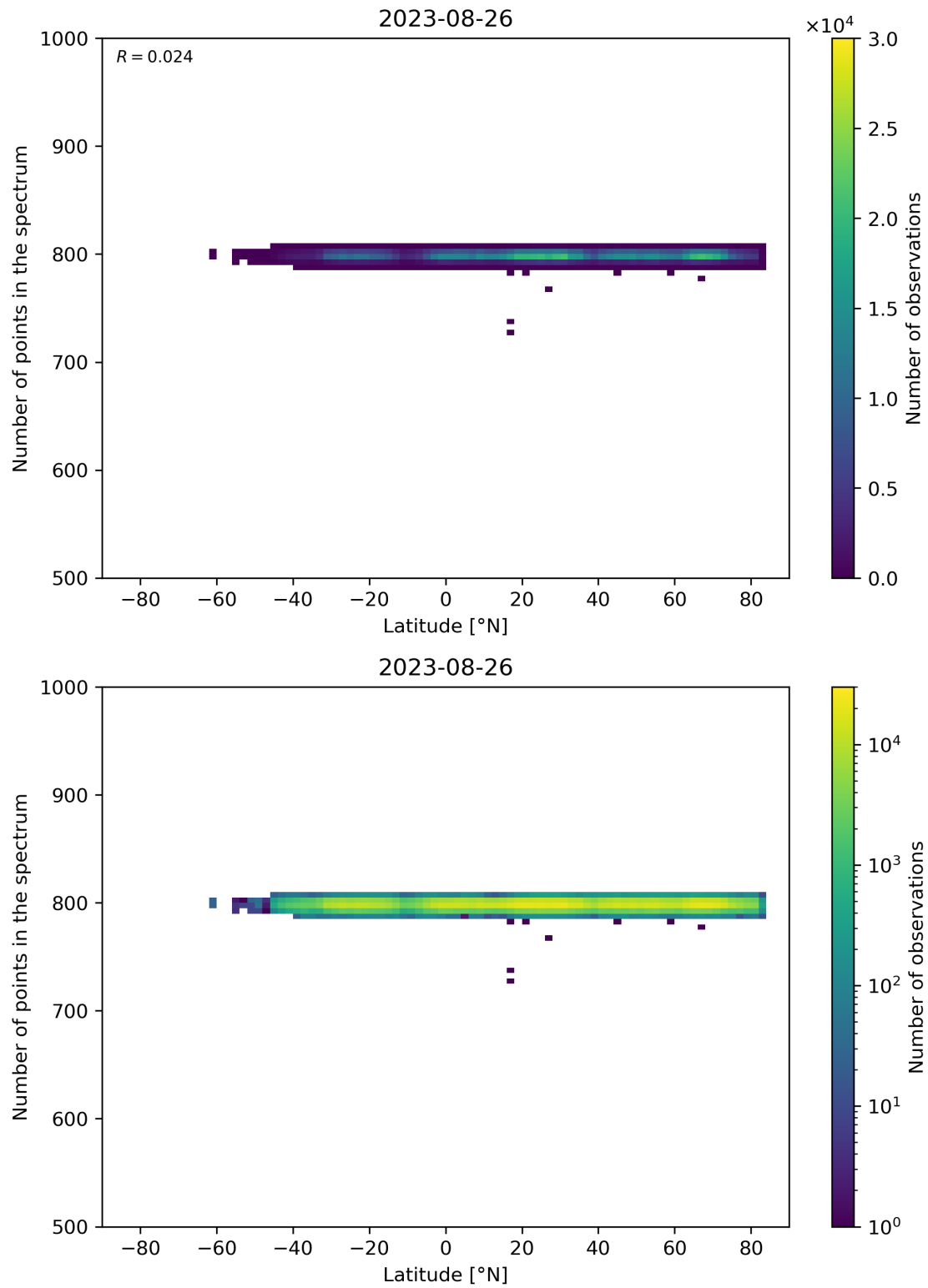
Figure 61: Scatter density plot of “Latitude” against “Number of points in the spectrum” for 2023-08-25 to 2023-08-27.
