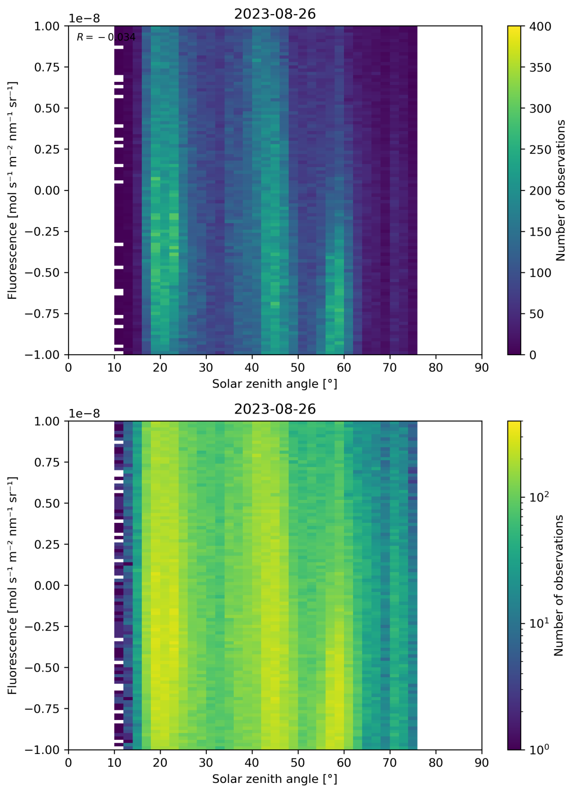
Figure 97: Scatter density plot of “Solar zenith angle” against “Fluorescence” for 2023-08-25 to 2023-08-27.
