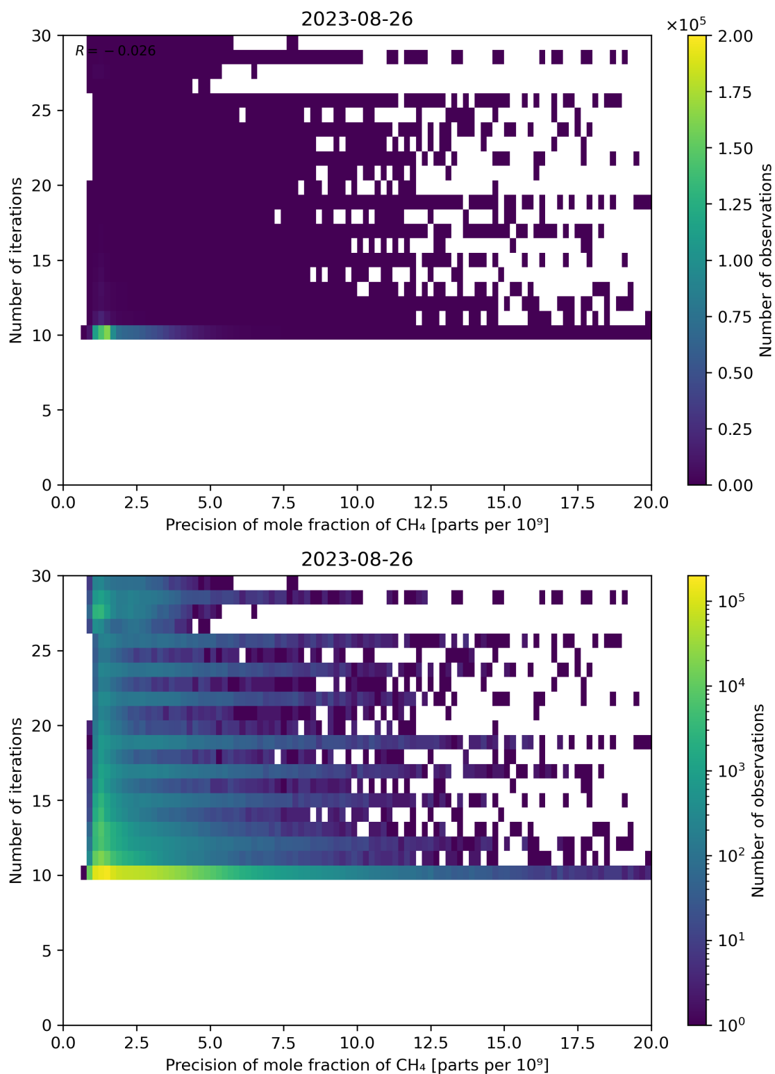
Figure 83: Scatter density plot of “Precision of mole fraction of CH 4 ” against “Number of iterations” for 2023-08-25 to 2023-08-27.
