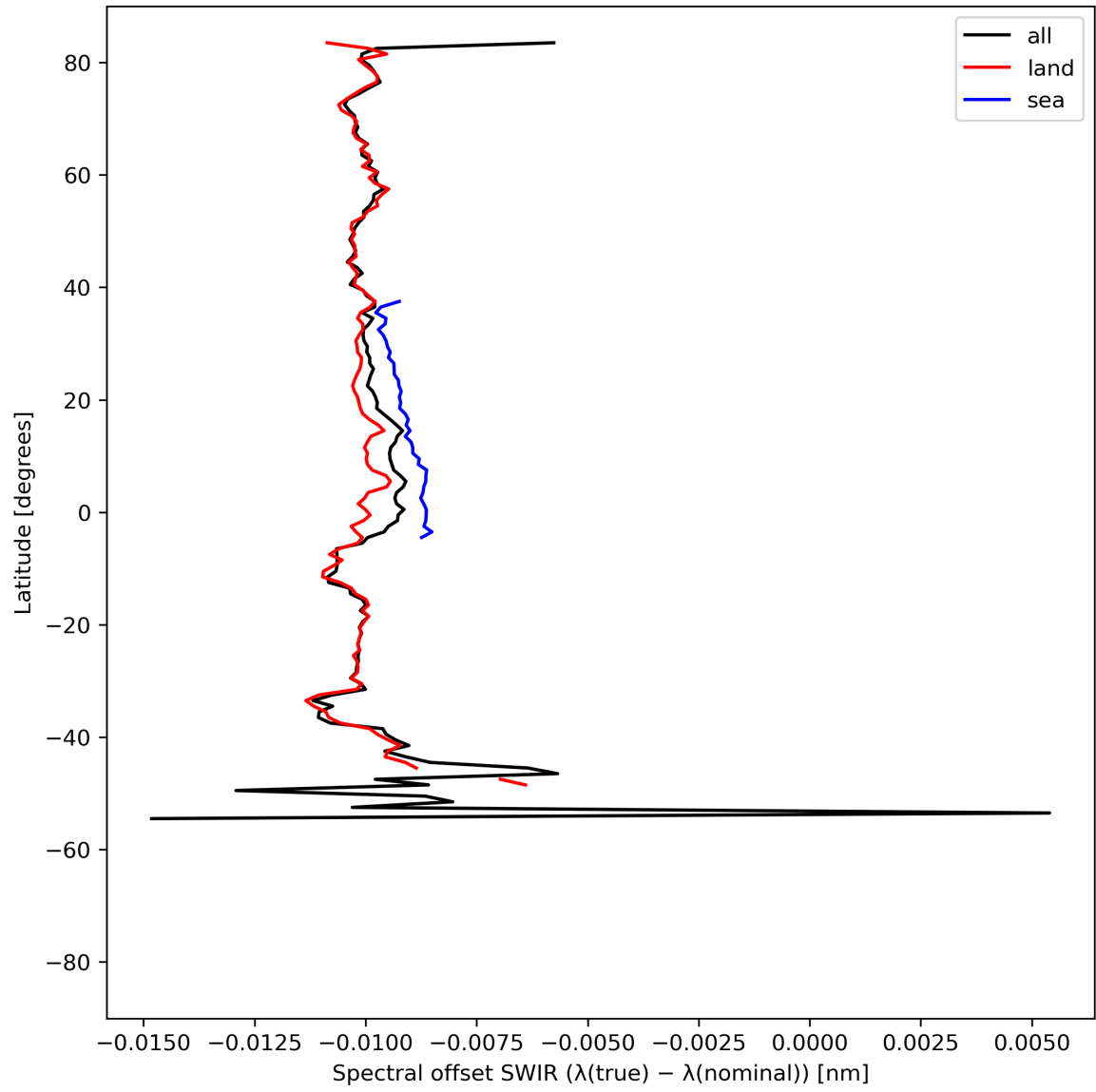
Figure 16: Zonal average of “Spectral offset SWIR ( \lambda(\text{true}) - \lambda(\text{nominal}) )” for 2023-08-25 to 2023-08-27.
