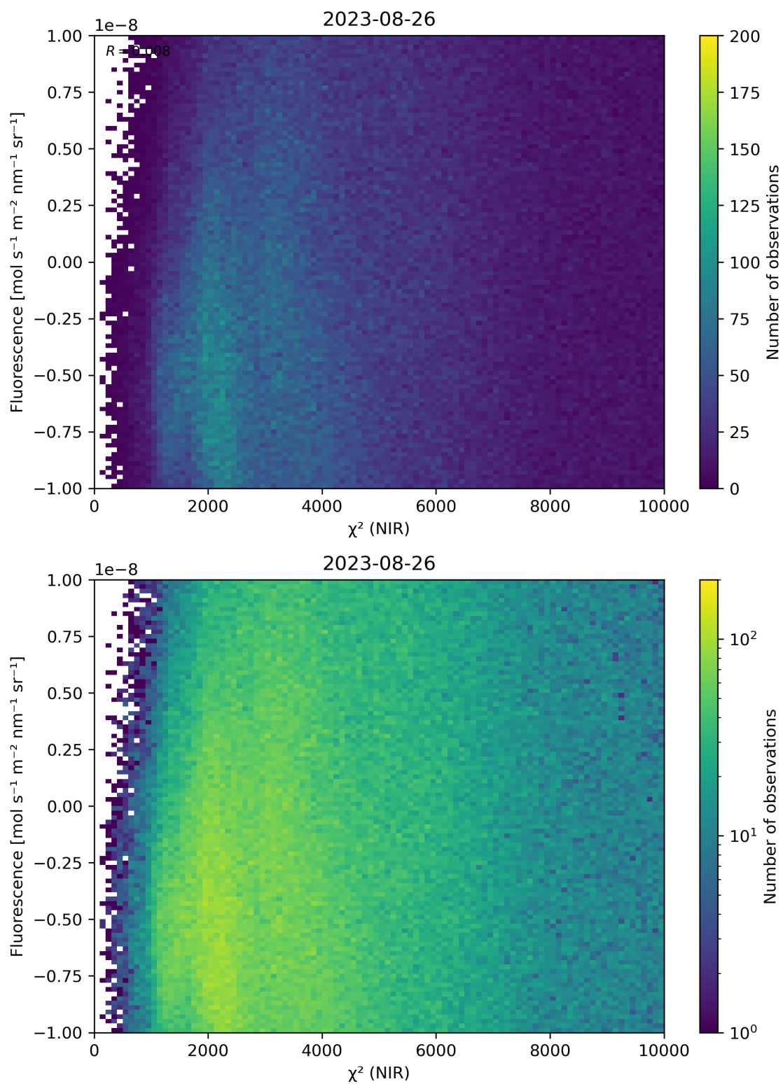
Figure 45: Scatter density plot of “ \chi^2 (NIR)” against “Fluorescence” for 2023-08-25 to 2023-08-27.
