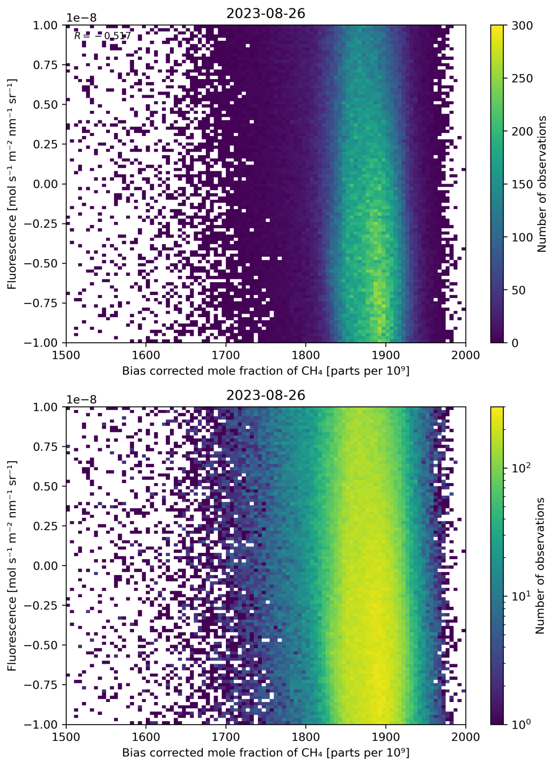
Figure 66: Scatter density plot of “Bias corrected mole fraction of \text{CH}_4 ” against “Fluorescence” for 2023-08-25 to 2023-08-27.
