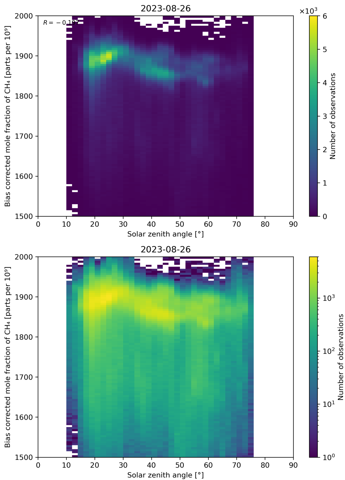
Figure 100: Scatter density plot of “Solar zenith angle” against “Bias corrected mole fraction of CH 4 ” for 2023-08-25 to 2023-08-27.
