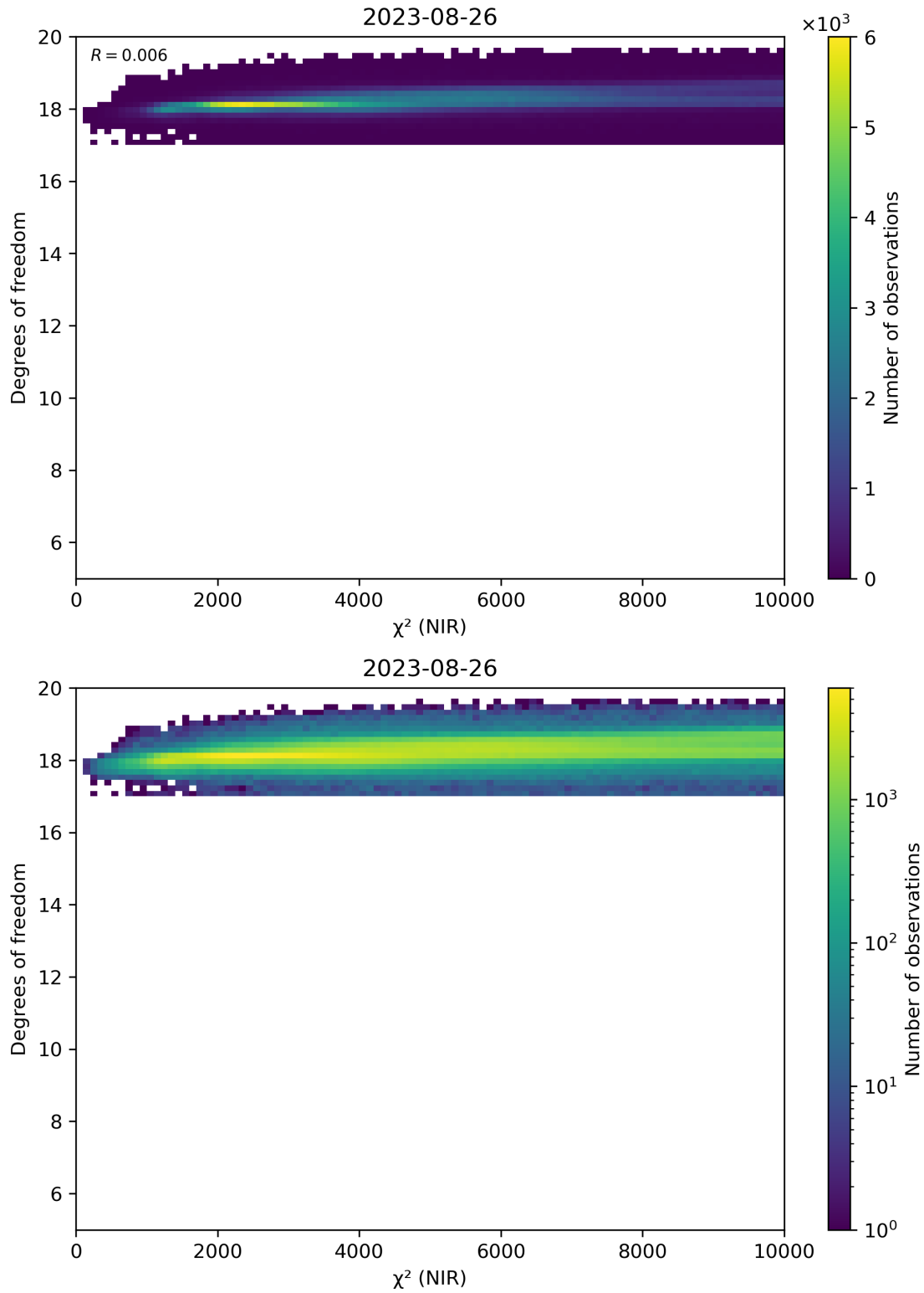
Figure 44: Scatter density plot of “ \chi^2 (NIR)” against “Degrees of freedom” for 2023-08-25 to 2023-08-27.
