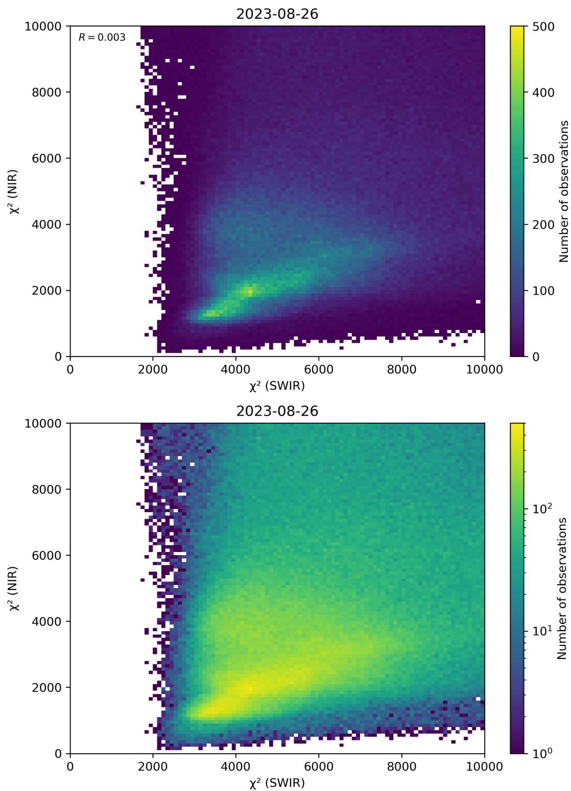
Figure 47: Scatter density plot of “ \chi^2 (SWIR)” against “ \chi^2 (NIR)” for 2023-08-25 to 2023-08-27.
