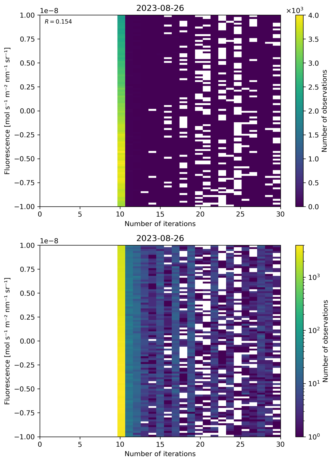
Figure 87: Scatter density plot of “Number of iterations” against “Fluorescence” for 2023-08-25 to 2023-08-27.
