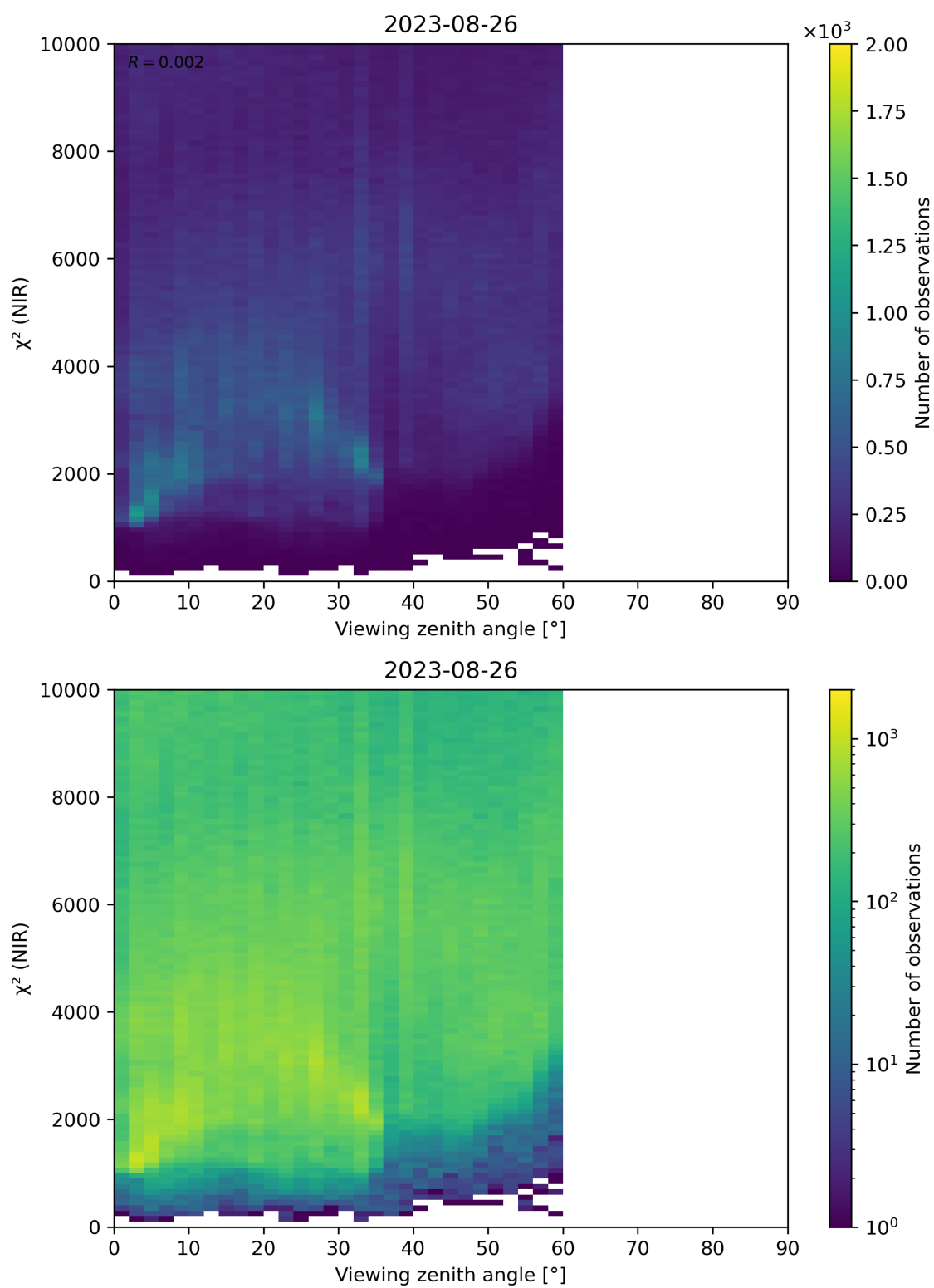
Figure 105: Scatter density plot of “Viewing zenith angle” against “ \chi^2 (NIR)” for 2023-08-25 to 2023-08-27.
