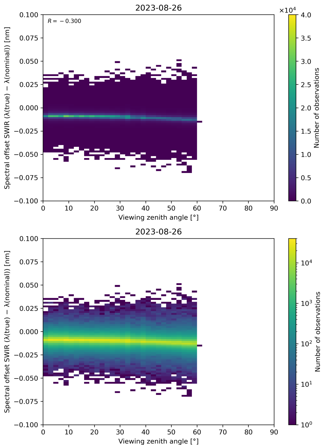
Figure 116: Scatter density plot of “Viewing zenith angle” against “Spectral offset SWIR ( \lambda(\text{true}) - \lambda(\text{nominal}) )” for 2023-08-25 to 2023-08-27.
