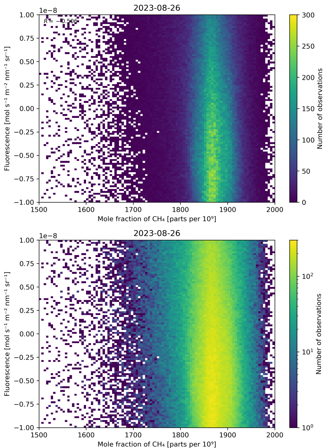
Figure 73: Scatter density plot of “Mole fraction of \text{CH}_4 ” against “Fluorescence” for 2023-08-25 to 2023-08-27.
