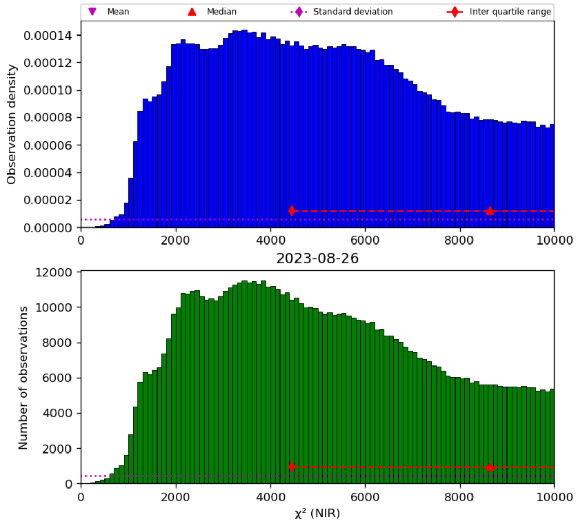
Figure 29: Histogram of " \chi^2 (NIR)" for 2023-08-25 to 2023-08-27
