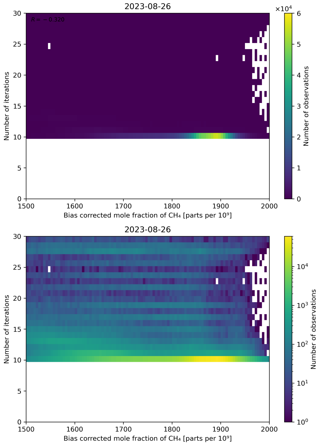
Figure 67: Scatter density plot of “Bias corrected mole fraction of CH 4 ” against “Number of iterations” for 2023-08-25 to 2023-08-27.
