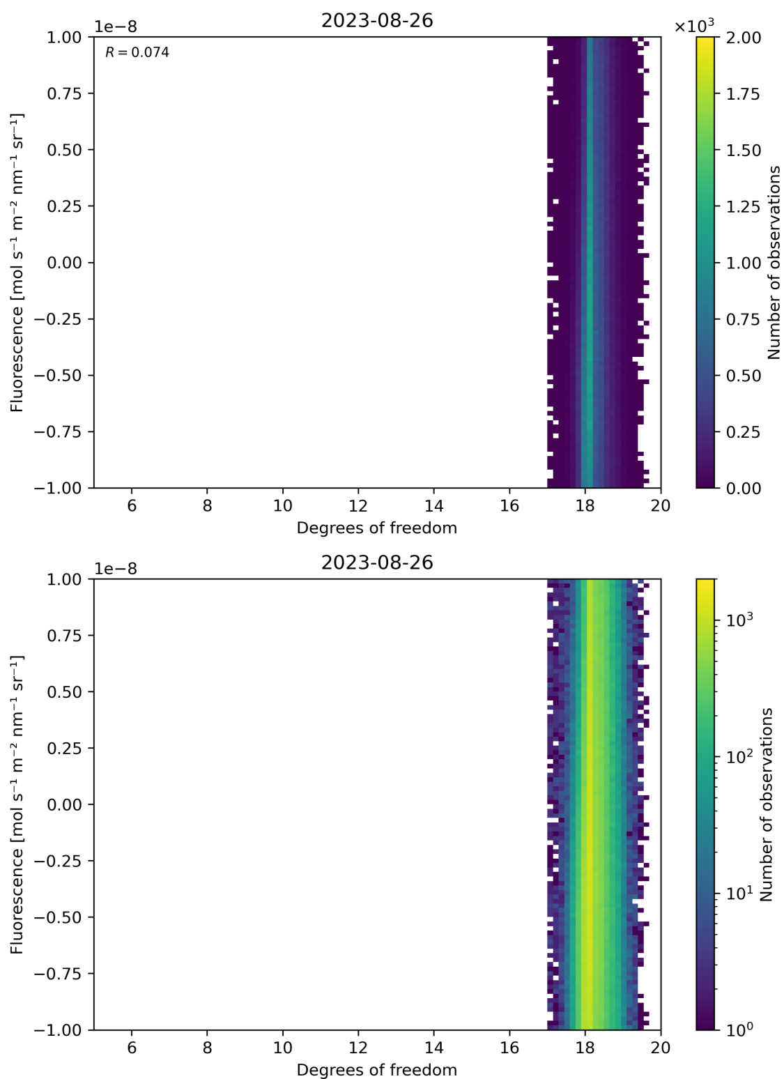
Figure 51: Scatter density plot of “Degrees of freedom” against “Fluorescence” for 2023-08-25 to 2023-08-27.
