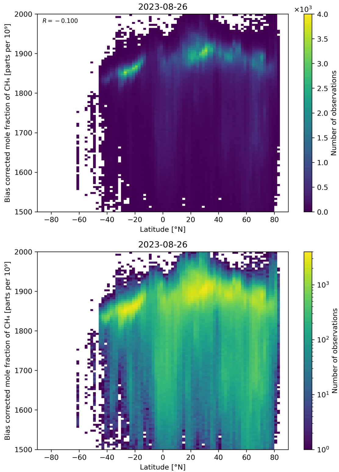
Figure 58: Scatter density plot of “Latitude” against “Bias corrected mole fraction of \text{CH}_4 ” for 2023-08-25 to 2023-08-27.
