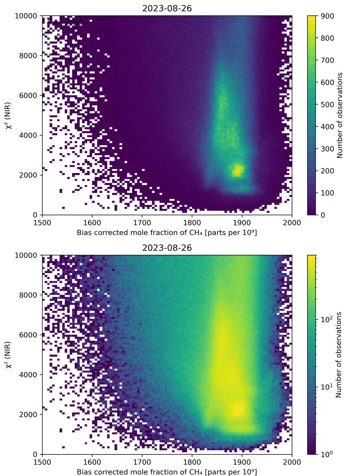
Figure 63: Scatter density plot of “Bias corrected mole fraction of \text{CH}_4 ” against “ \chi^2 (NIR)” for 2023-08-25 to 2023-08-27.
