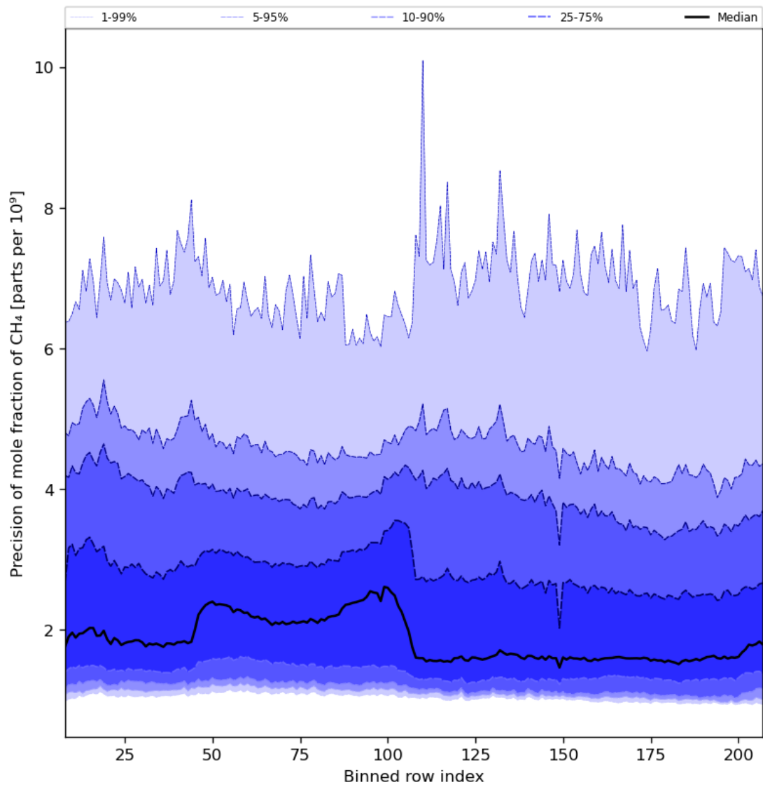
Figure 35: Along track statistics of “Precision of mole fraction of CH 4 ” for 2023-08-25 to 2023-08-27
