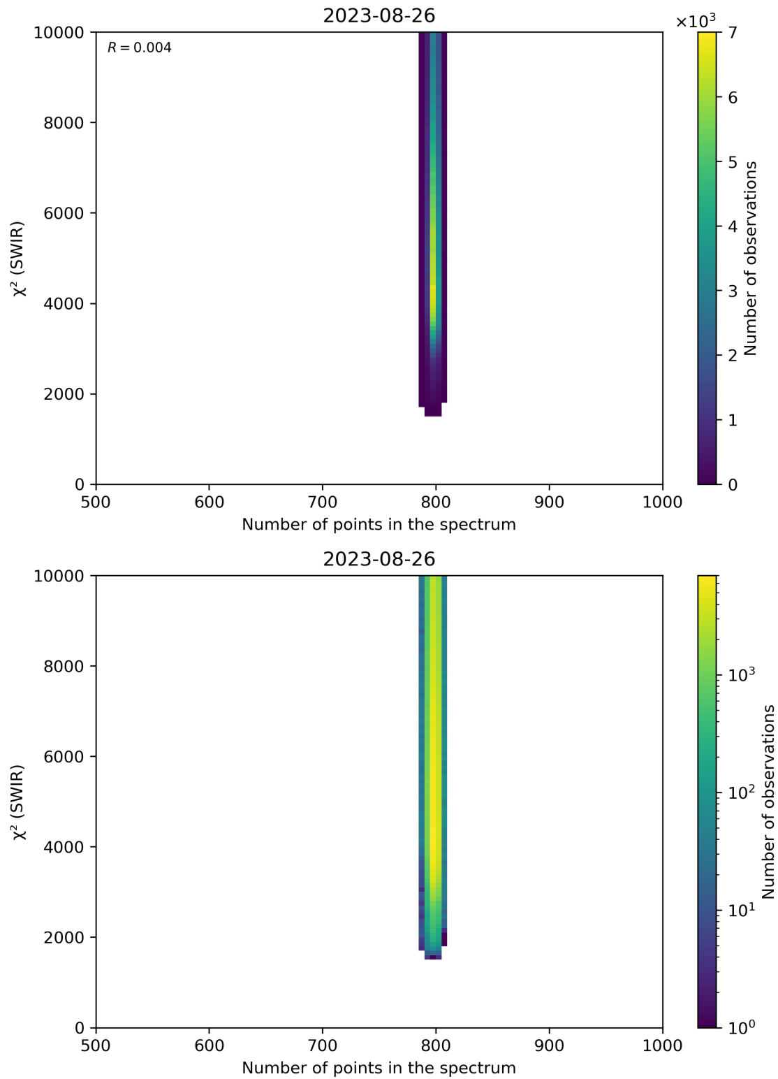
Figure 89: Scatter density plot of “Number of points in the spectrum” against “ \chi^2 (SWIR)” for 2023-08-25 to 2023-08-27.
