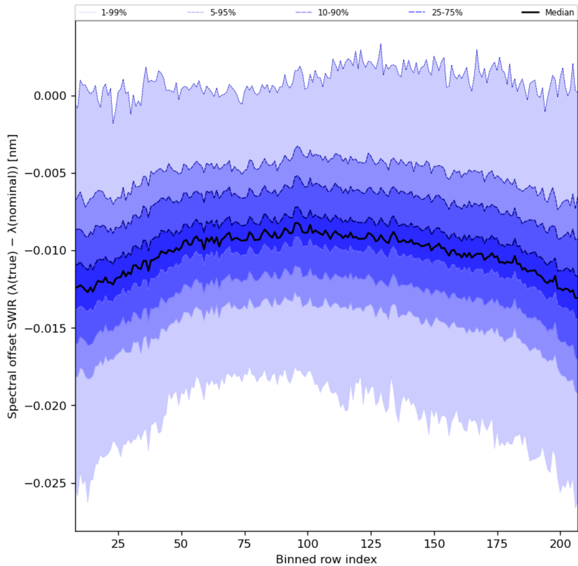
Figure 38: Along track statistics of “Spectral offset SWIR ( \lambda(\text{true}) - \lambda(\text{nominal}) )” for 2023-08-25 to 2023-08-27
