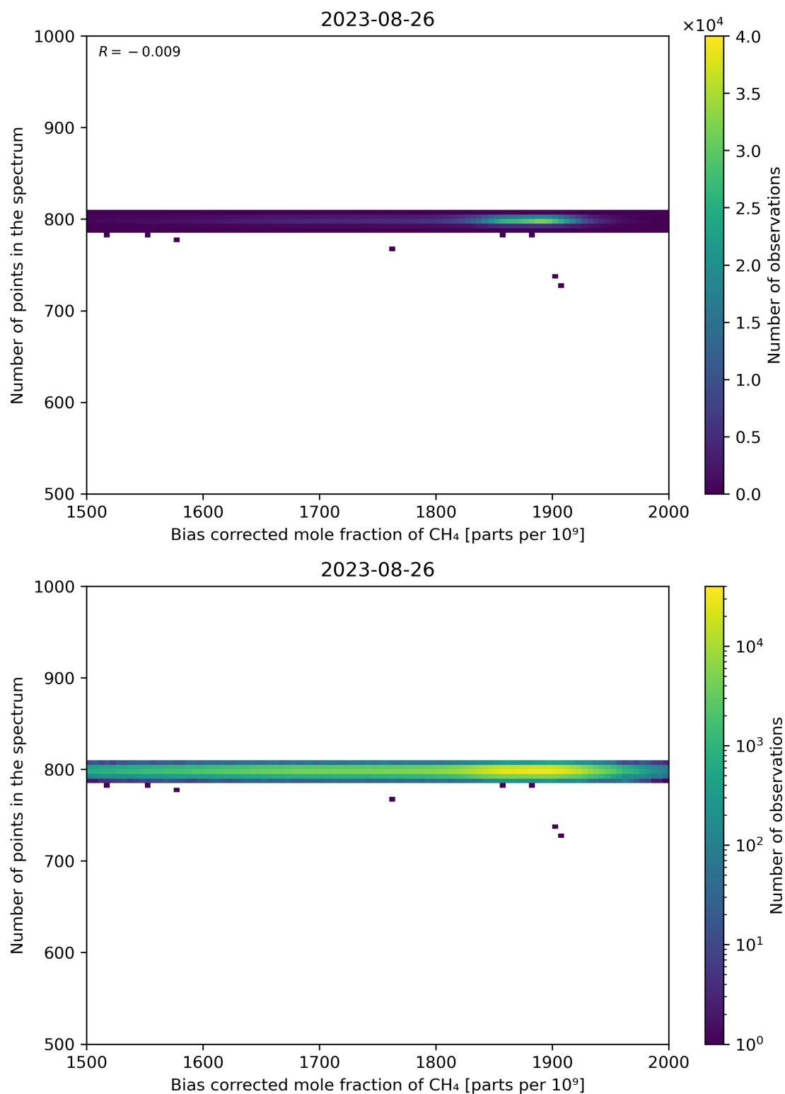
Figure 68: Scatter density plot of “Bias corrected mole fraction of CH 4 ” against “Number of points in the spectrum” for 2023-08-25 to 2023-08-27.
