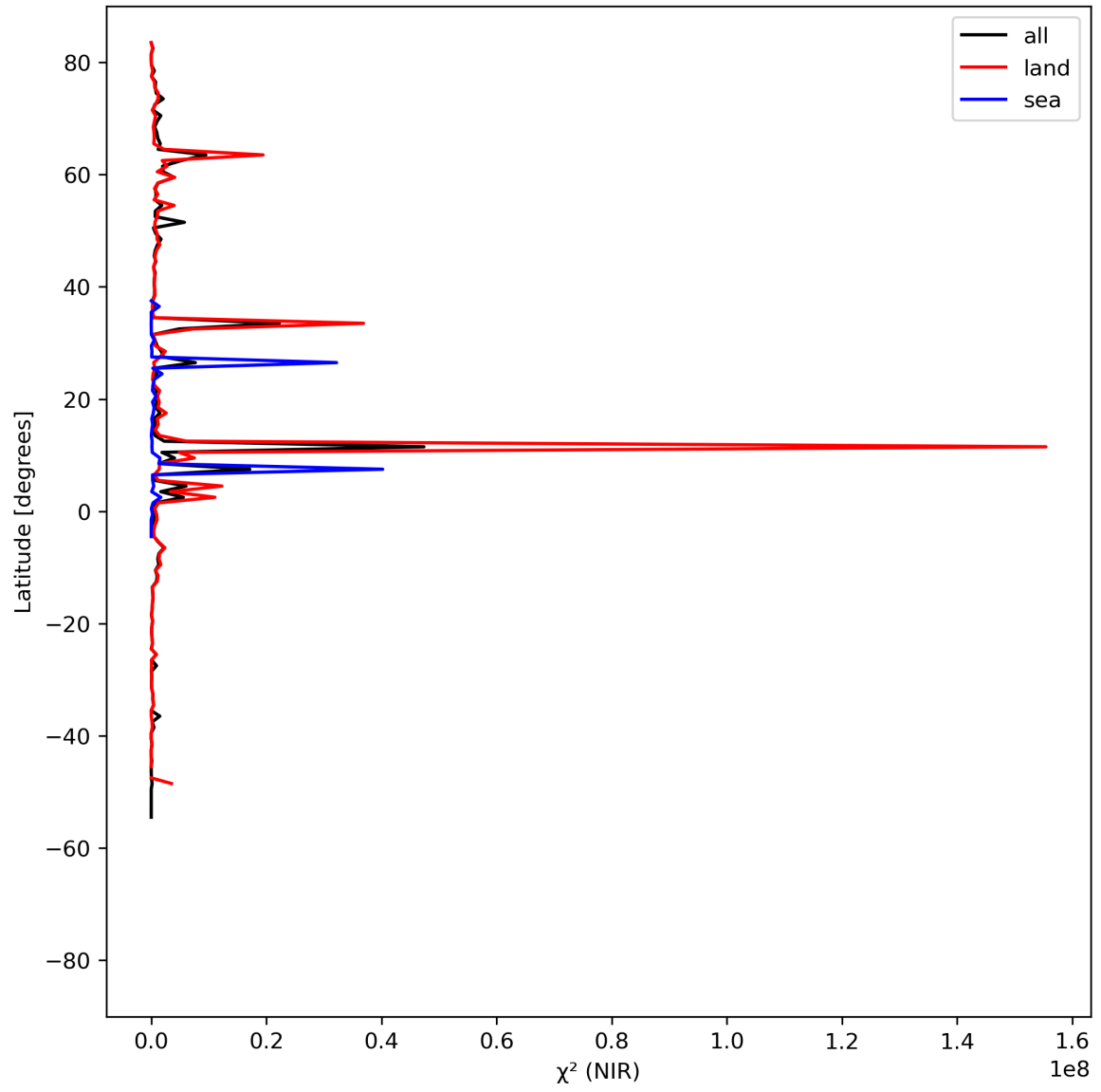
Figure 18: Zonal average of “ \chi^2 (NIR)” for 2023-08-25 to 2023-08-27.
