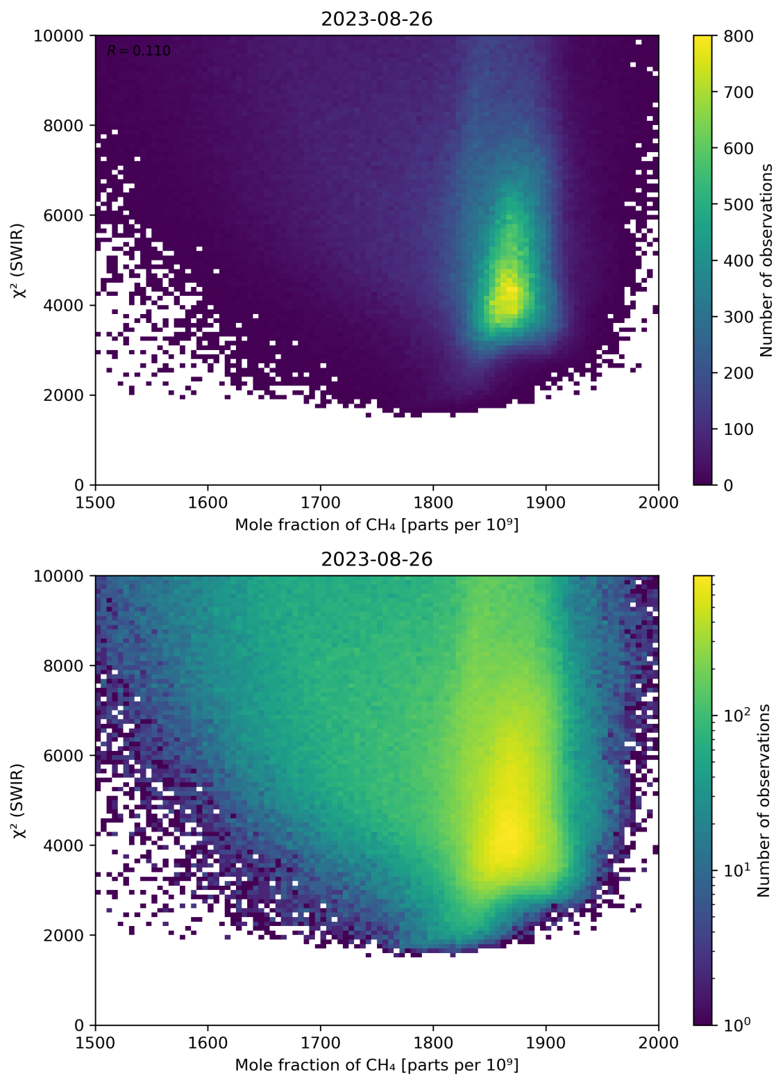
Figure 71: Scatter density plot of “Mole fraction of CH 4 ” against “ \chi^2 (SWIR)” for 2023-08-25 to 2023-08-27.
