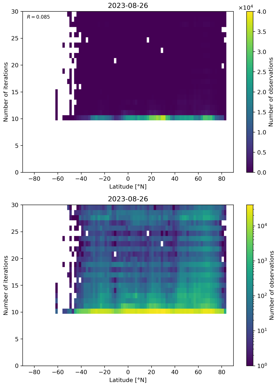
Figure 60: Scatter density plot of “Latitude” against “Number of iterations” for 2023-08-25 to 2023-08-27.
