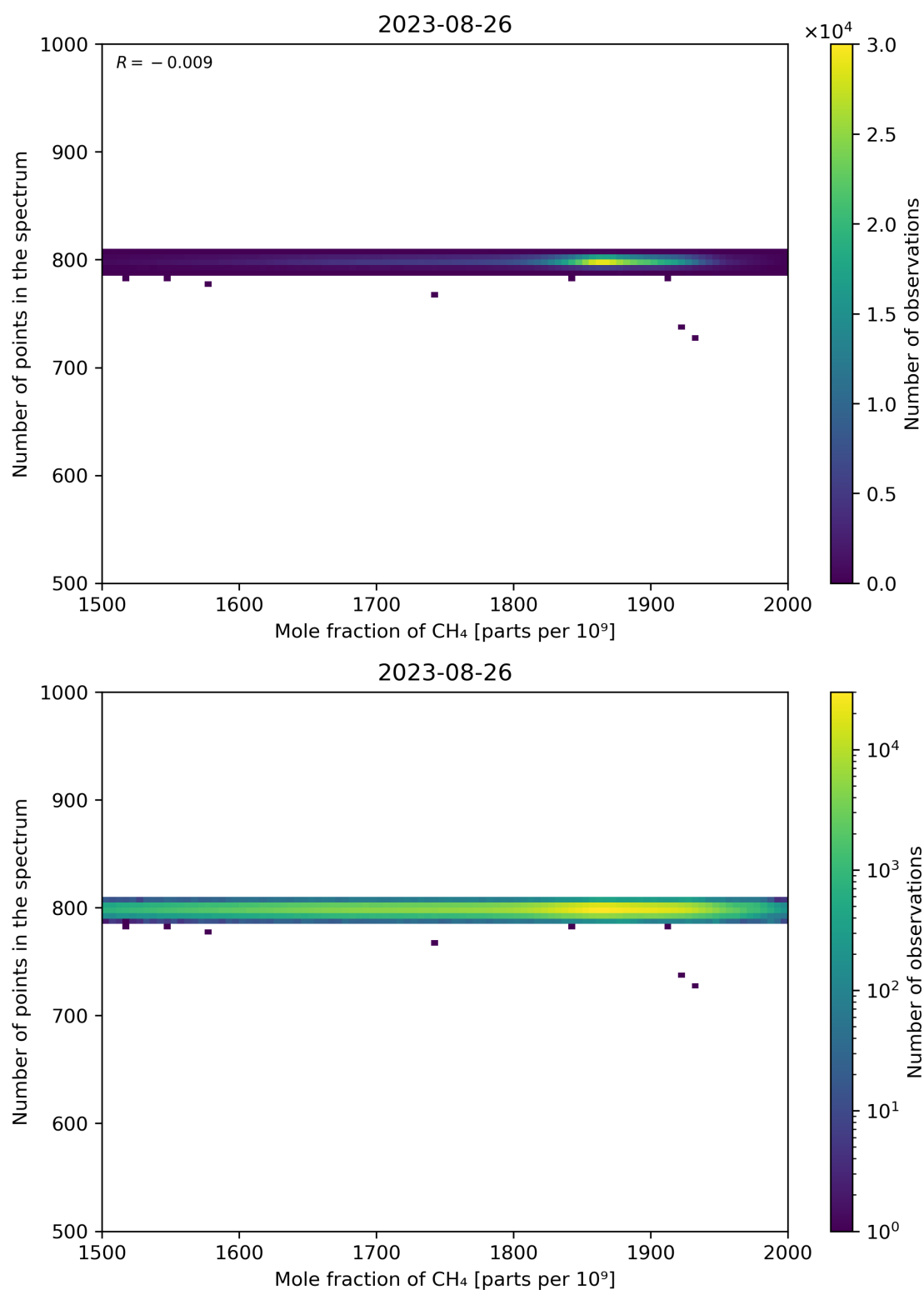
Figure 77: Scatter density plot of “Mole fraction of CH 4 ” against “Number of points in the spectrum” for 2023-08-25 to 2023-08-27.
