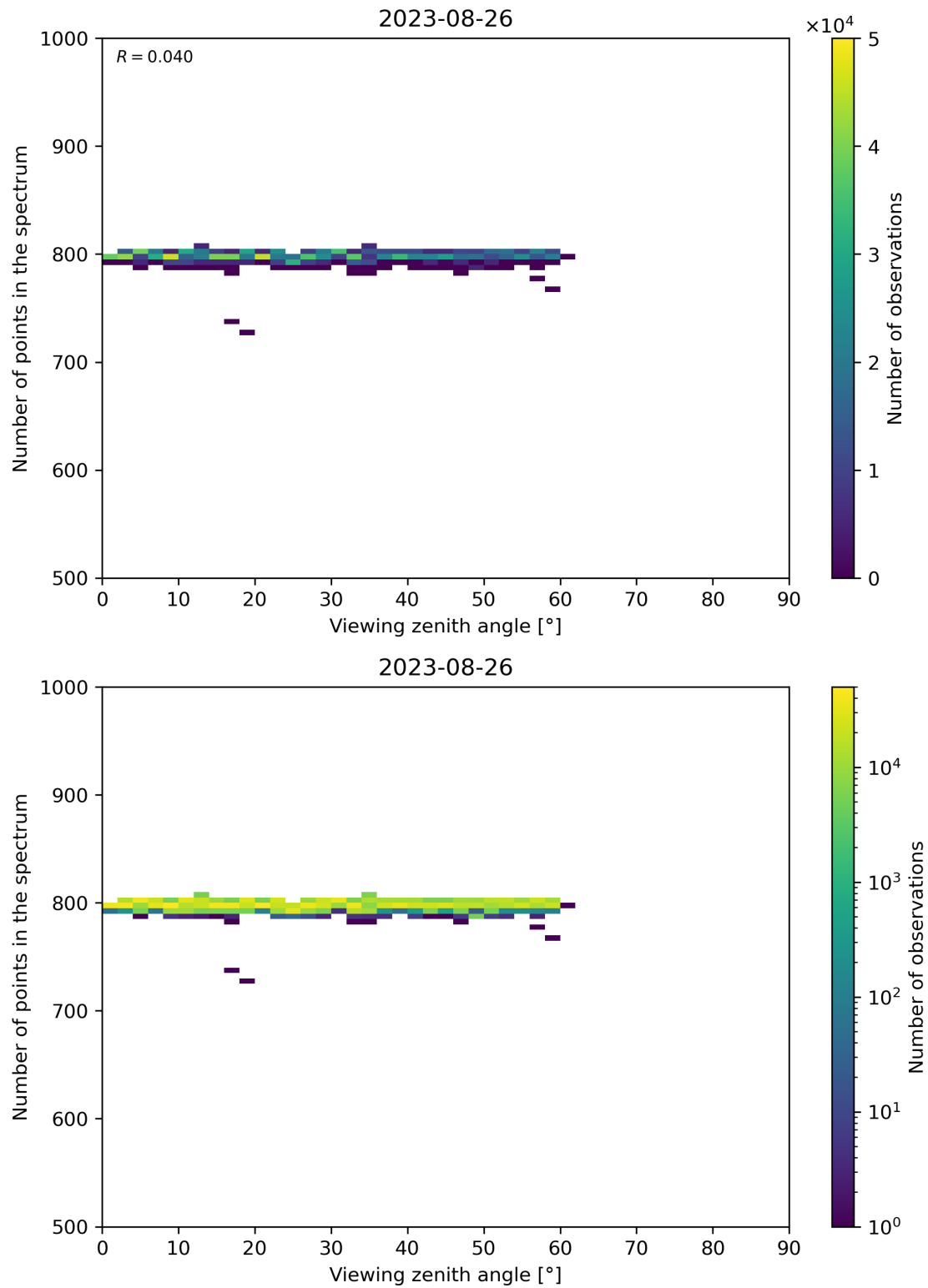
Figure 114: Scatter density plot of “Viewing zenith angle” against “Number of points in the spectrum” for 2023-08-25 to 2023-08-27.
