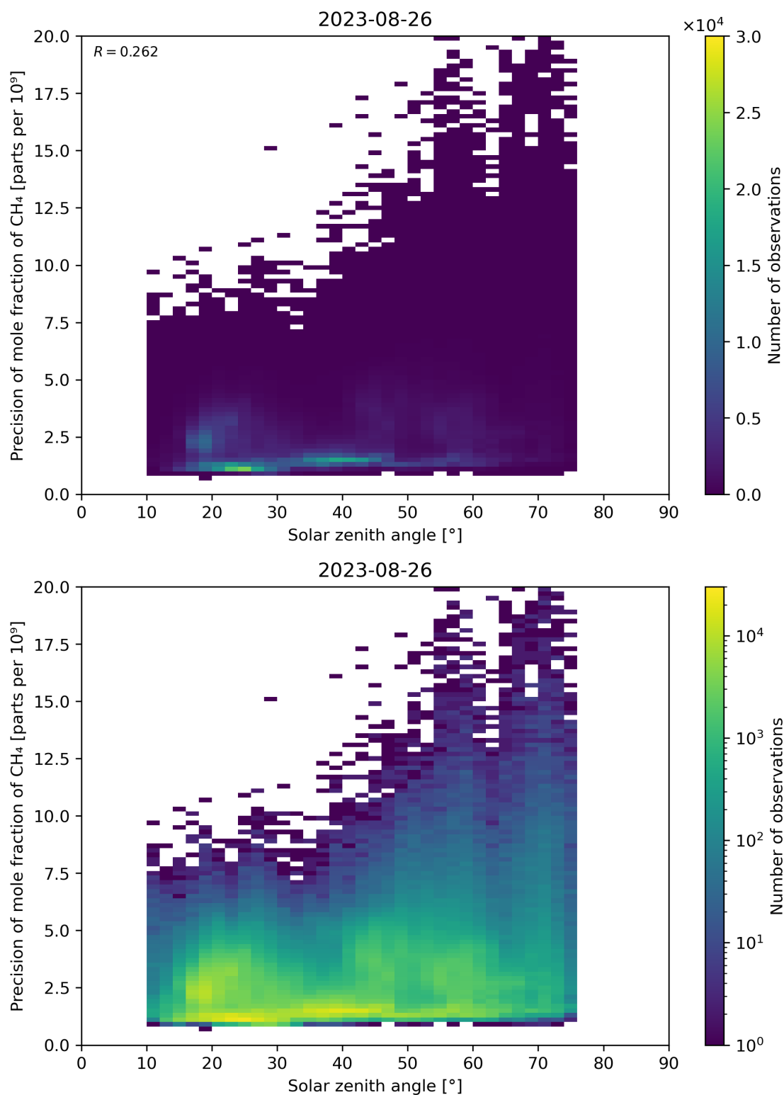
Figure 101: Scatter density plot of “Solar zenith angle” against “Precision of mole fraction of CH 4 ” for 2023-08-25 to 2023-08-27.
