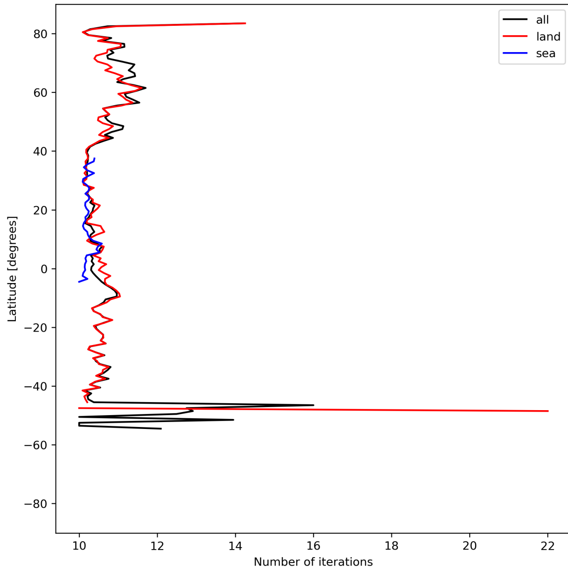
Figure 20: Zonal average of “Number of iterations” for 2023-08-25 to 2023-08-27.
