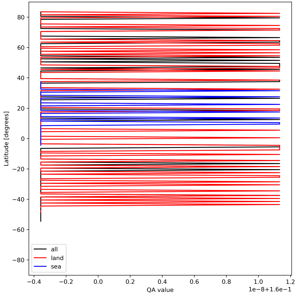
Figure 11: Zonal average of “QA value” for 2023-08-25 to 2023-08-27.
