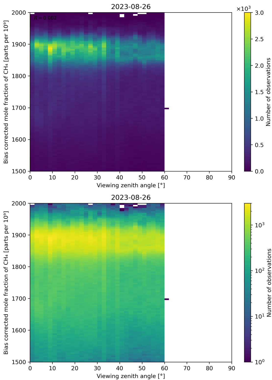
Figure 111: Scatter density plot of “Viewing zenith angle” against “Bias corrected mole fraction of CH 4 ” for 2023-08-25 to 2023-08-27.
