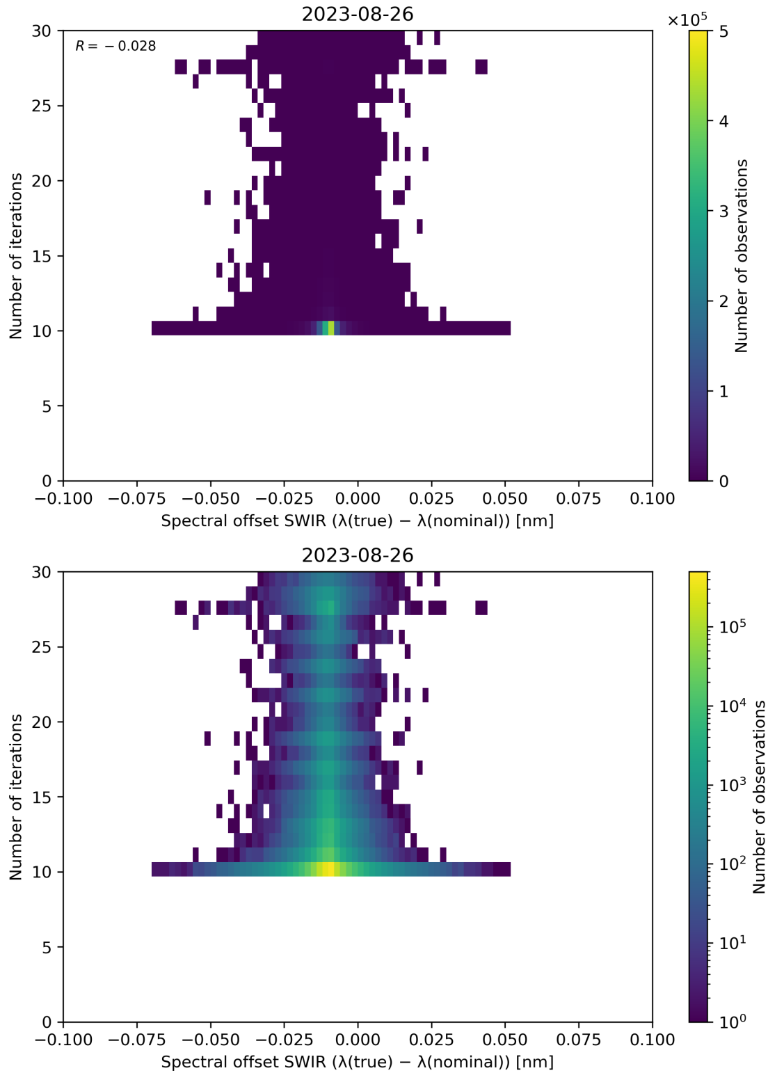
Figure 121: Scatter density plot of “Spectral offset SWIR ( \lambda(\text{true}) - \lambda(\text{nominal}) )” against “Number of iterations” for 2023-08-25 to 2023-08-27.
