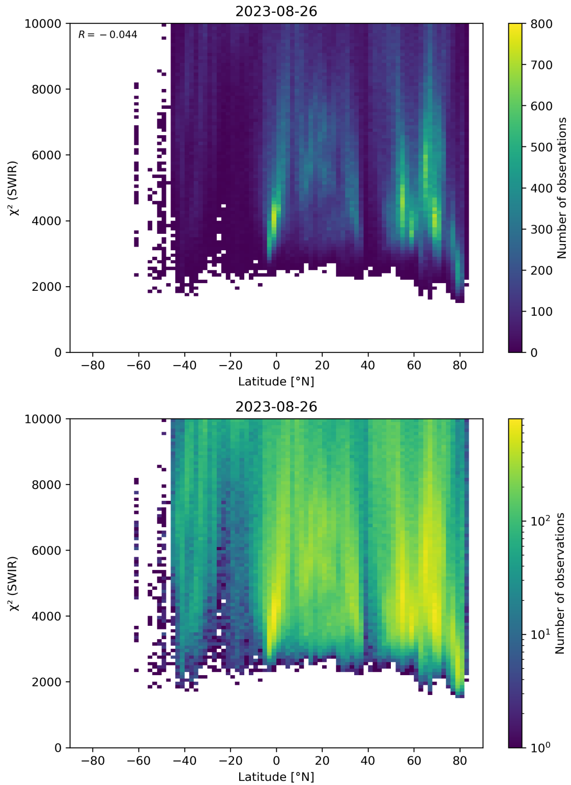
Figure 54: Scatter density plot of “Latitude” against “ \chi^2 (SWIR)” for 2023-08-25 to 2023-08-27.
