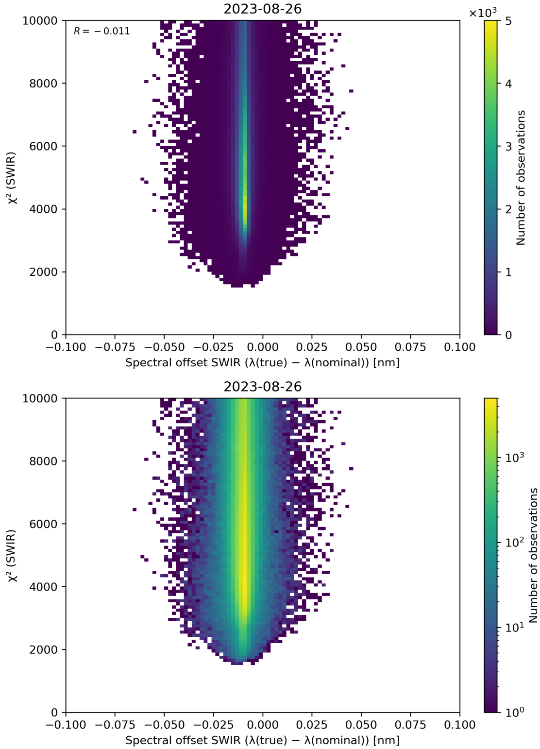
Figure 118: Scatter density plot of “Spectral offset SWIR ( \lambda(\text{true}) - \lambda(\text{nominal}) )” against “ \chi^2 (SWIR)” for 2023-08-25 to 2023-08-27.
