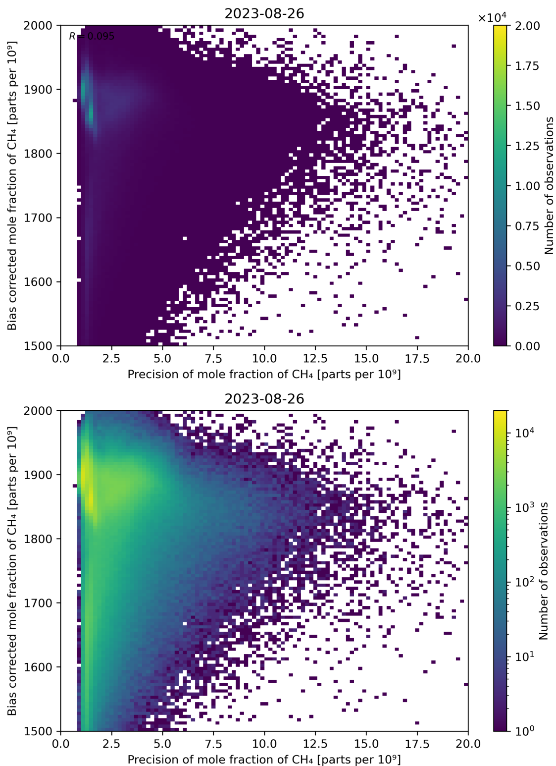
Figure 82: Scatter density plot of “Precision of mole fraction of CH 4 ” against “Bias corrected mole fraction of CH 4 ” for 2023-08-25 to 2023-08-27.
