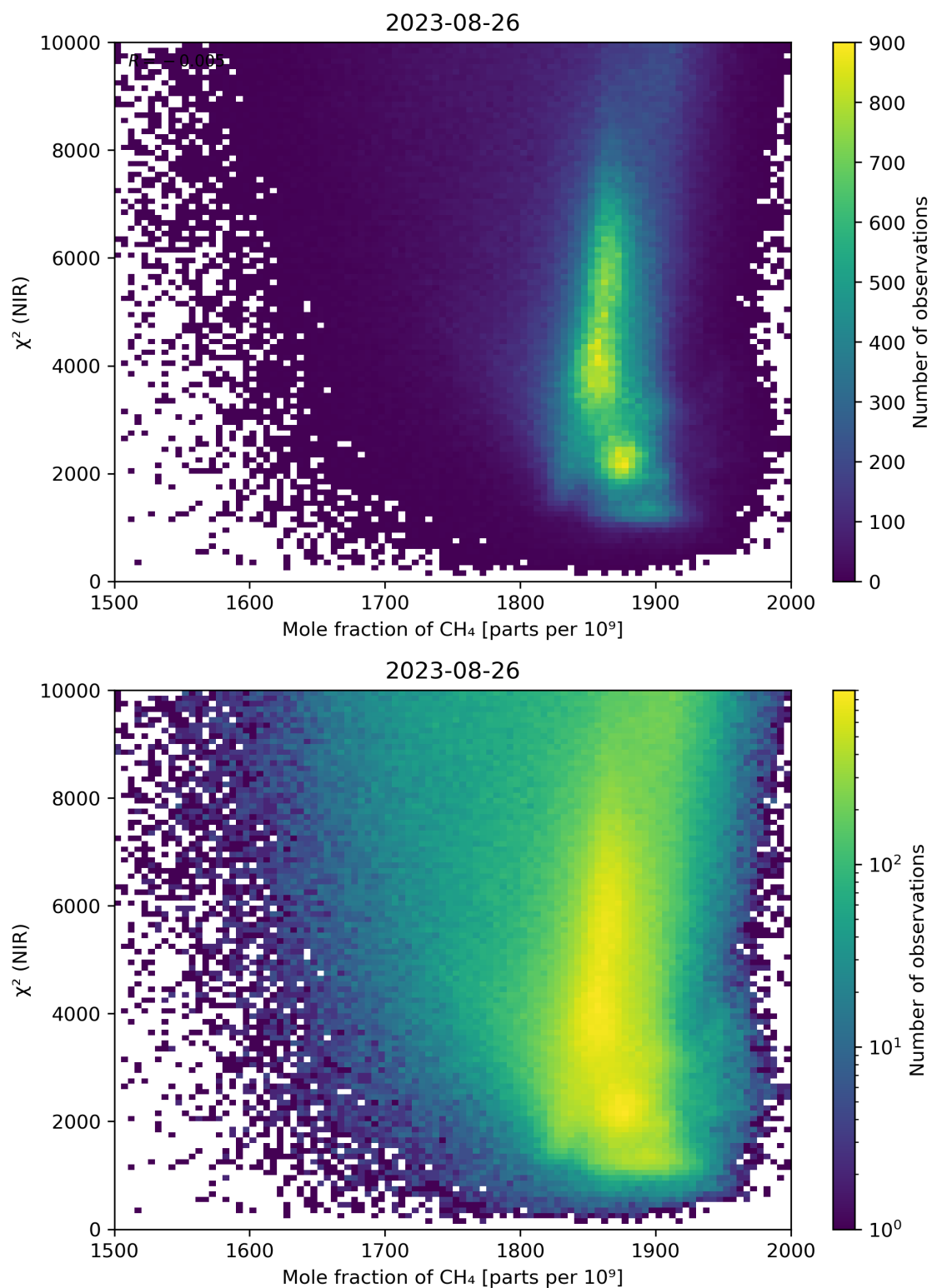
Figure 70: Scatter density plot of “Mole fraction of CH 4 ” against “ \chi^2 (NIR)” for 2023-08-25 to 2023-08-27.
