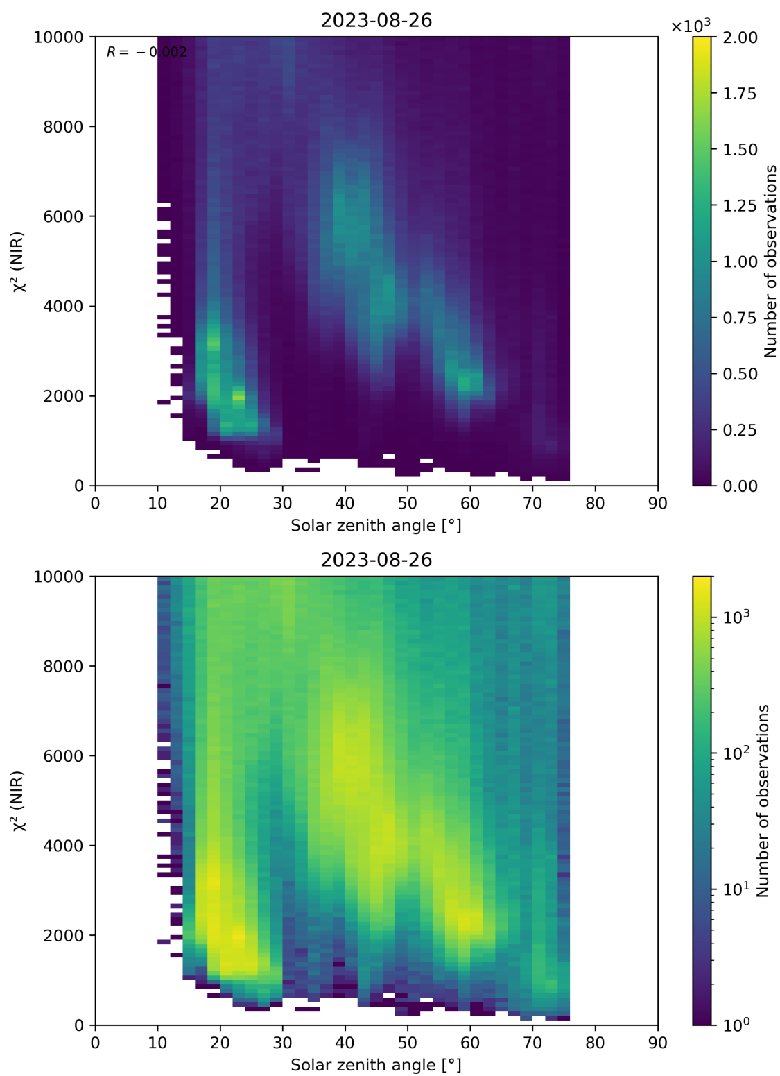
Figure 94: Scatter density plot of “Solar zenith angle” against “ \chi^2 (NIR)” for 2023-08-25 to 2023-08-27.
