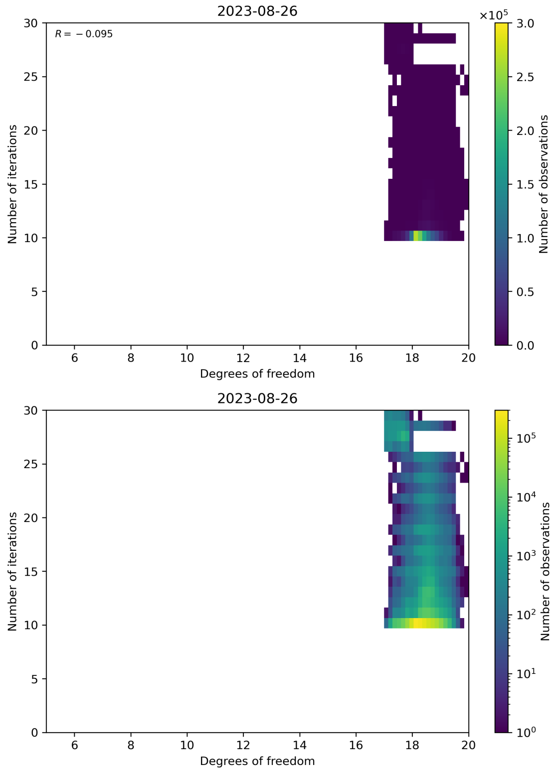
Figure 52: Scatter density plot of “Degrees of freedom” against “Number of iterations” for 2023-08-25 to 2023-08-27.
