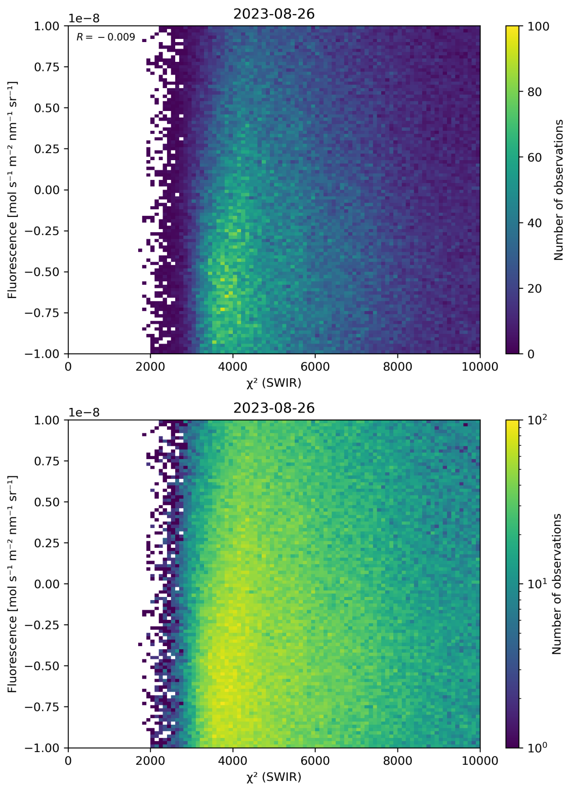
Figure 49: Scatter density plot of “ \chi^2 (SWIR)” against “Fluorescence” for 2023-08-25 to 2023-08-27.
