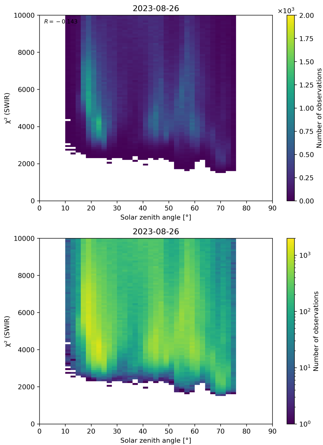
Figure 95: Scatter density plot of “Solar zenith angle” against “ \chi^2 (SWIR)” for 2023-08-25 to 2023-08-27.
