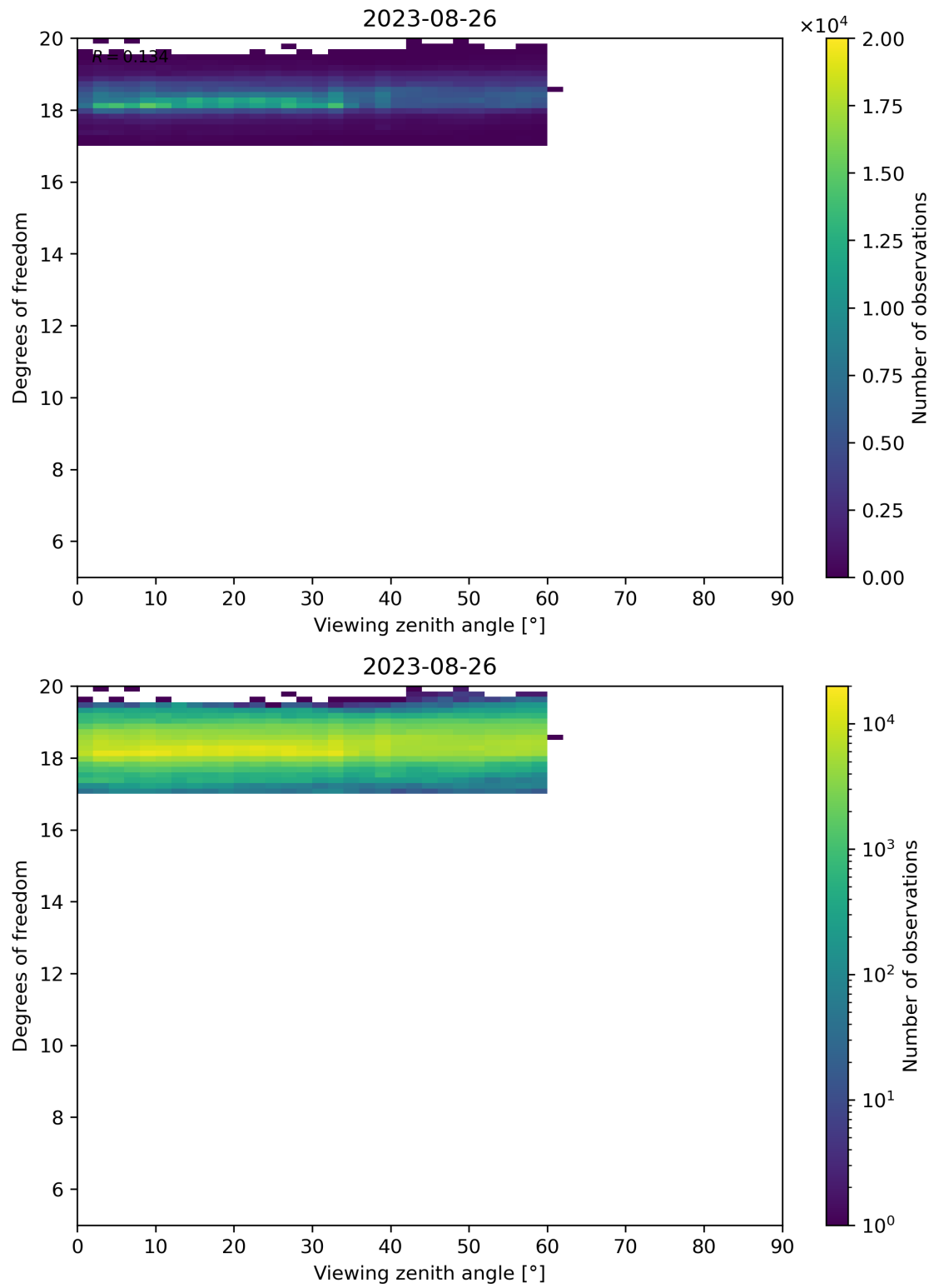
Figure 107: Scatter density plot of “Viewing zenith angle” against “Degrees of freedom” for 2023-08-25 to 2023-08-27.
