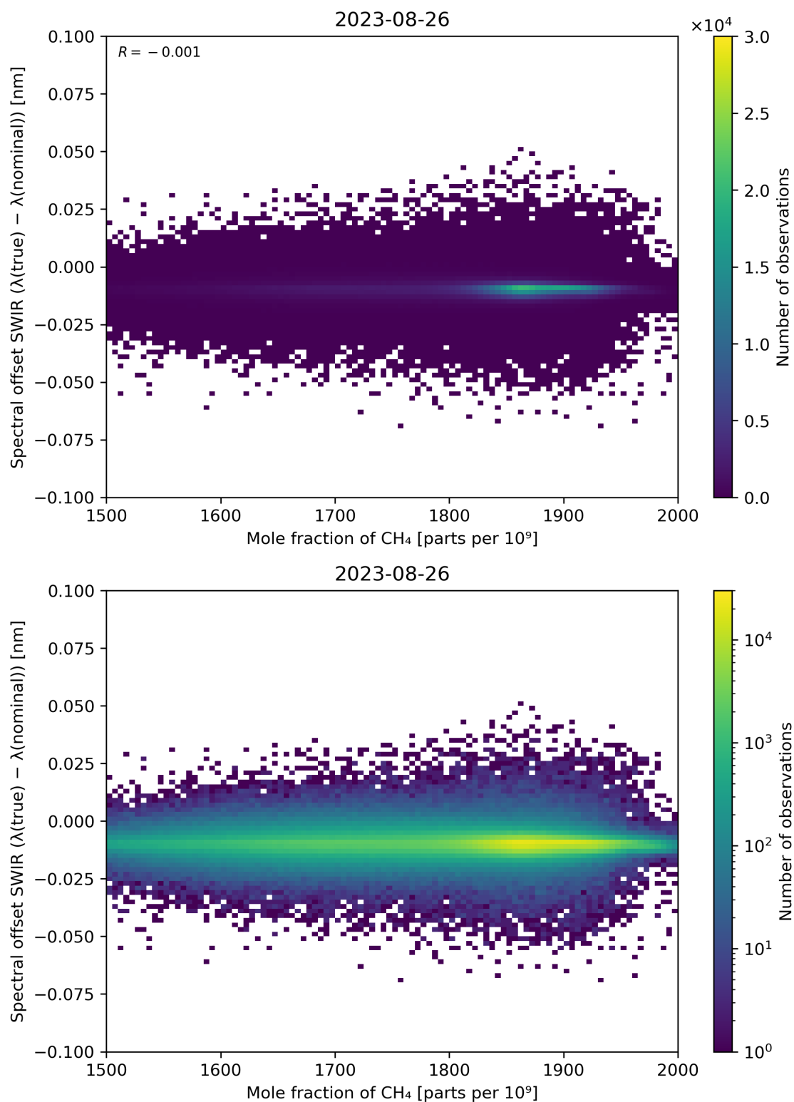
Figure 86: Scatter density plot of “Mole fraction of CH 4 ” against “Spectral offset SWIR ( \lambda(\text{true}) - \lambda(\text{nominal}) )” for 2023-08-25 to 2023-08-27.
