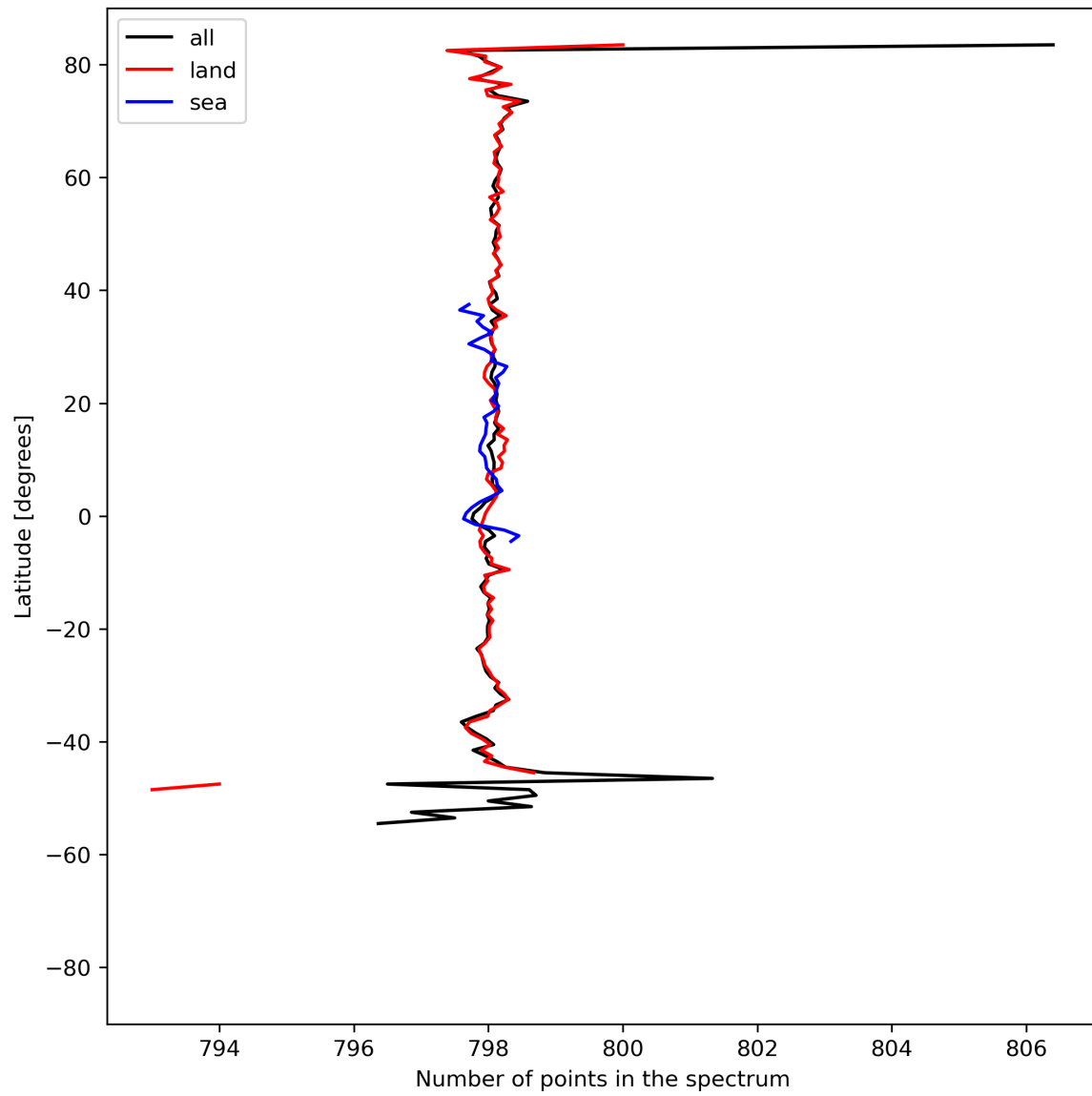
Figure 15: Zonal average of “Number of points in the spectrum” for 2023-08-25 to 2023-08-27.
