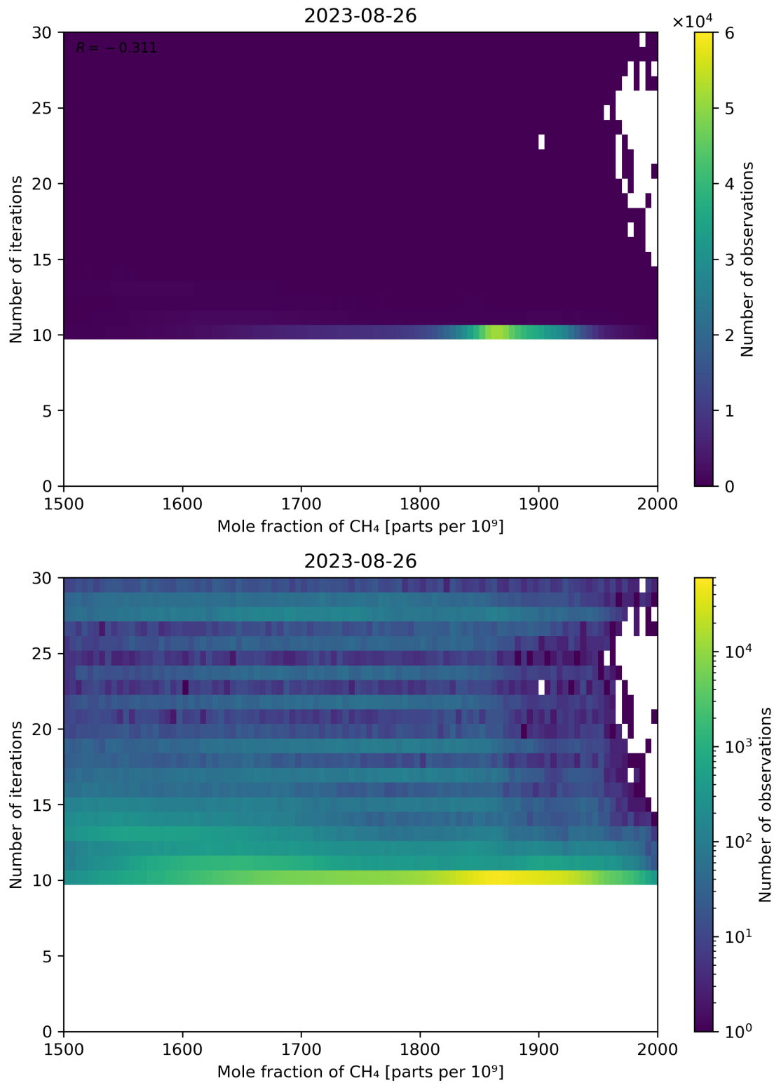
Figure 76: Scatter density plot of “Mole fraction of CH 4 ” against “Number of iterations” for 2023-08-25 to 2023-08-27.
