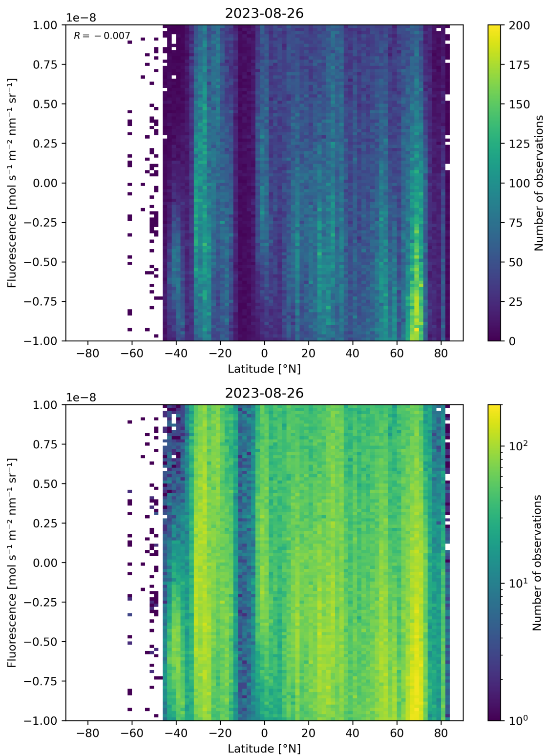
Figure 56: Scatter density plot of “Latitude” against “Fluorescence” for 2023-08-25 to 2023-08-27.
