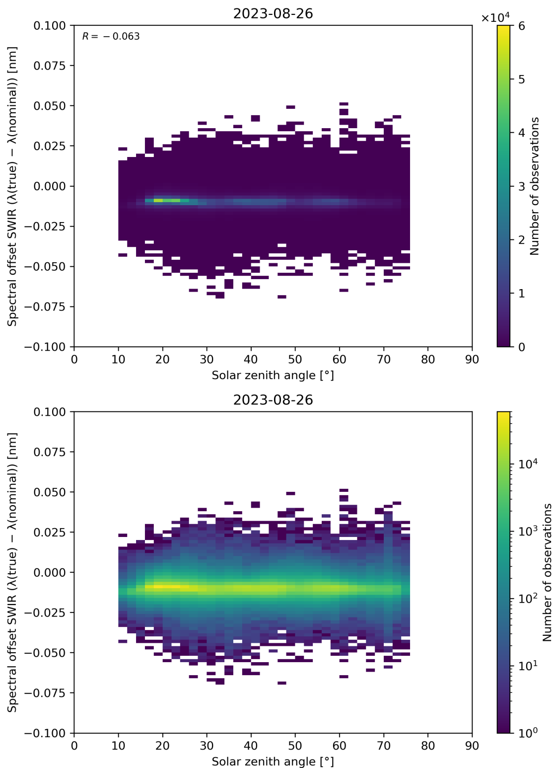
Figure 104: Scatter density plot of “Solar zenith angle” against “Spectral offset SWIR ( \lambda(\text{true}) - \lambda(\text{nominal}) )” for 2023-08-25 to 2023-08-27.
