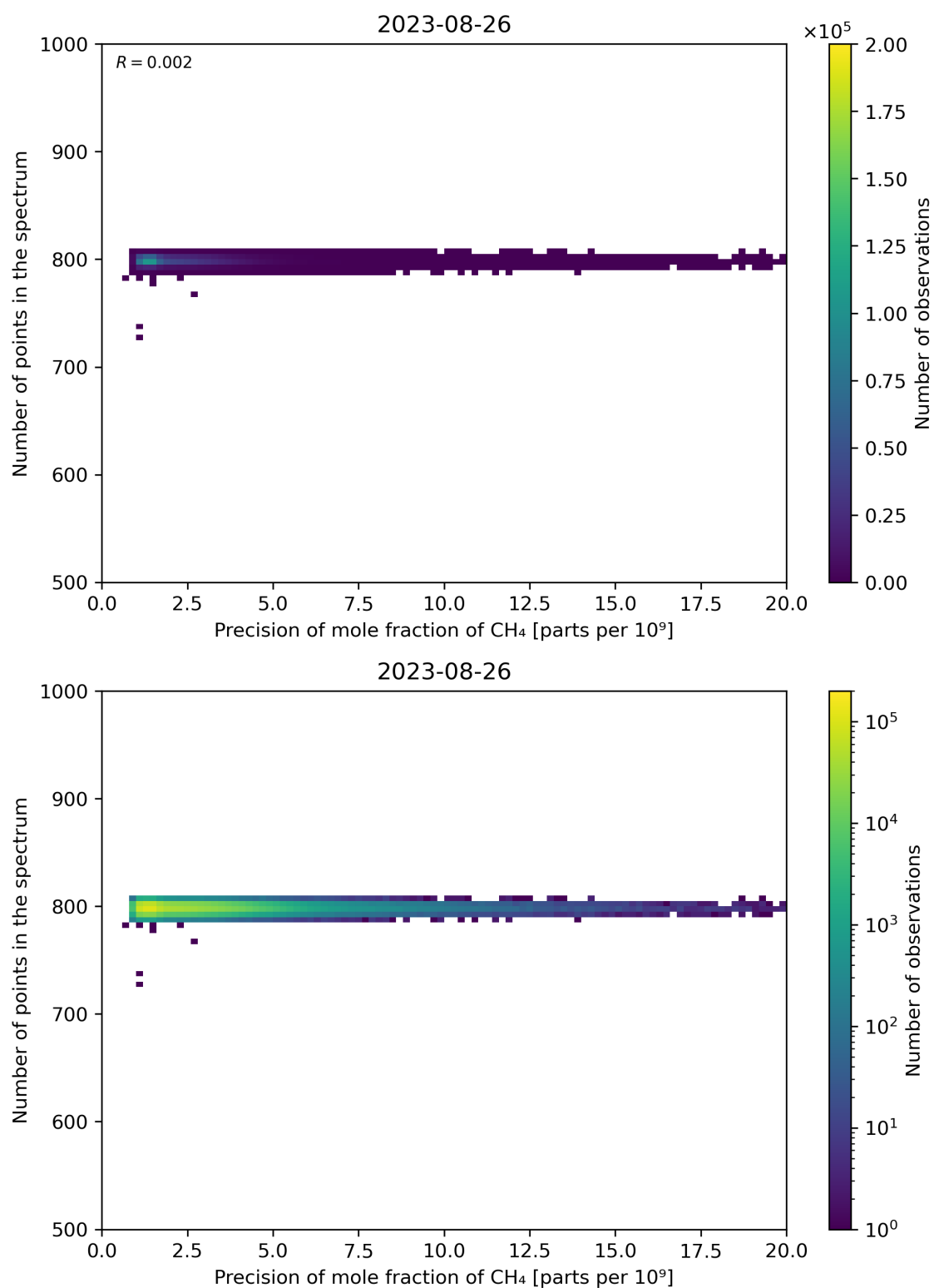
Figure 84: Scatter density plot of “Precision of mole fraction of CH 4 ” against “Number of points in the spectrum” for 2023-08-25 to 2023-08-27.
