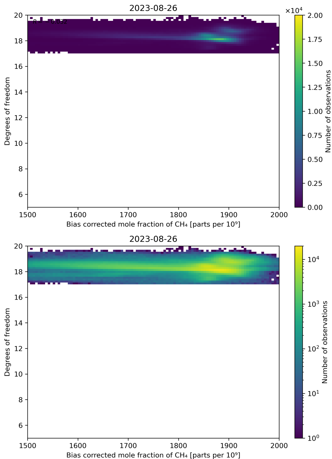
Figure 65: Scatter density plot of “Bias corrected mole fraction of CH 4 ” against “Degrees of freedom” for 2023-08-25 to 2023-08-27.
