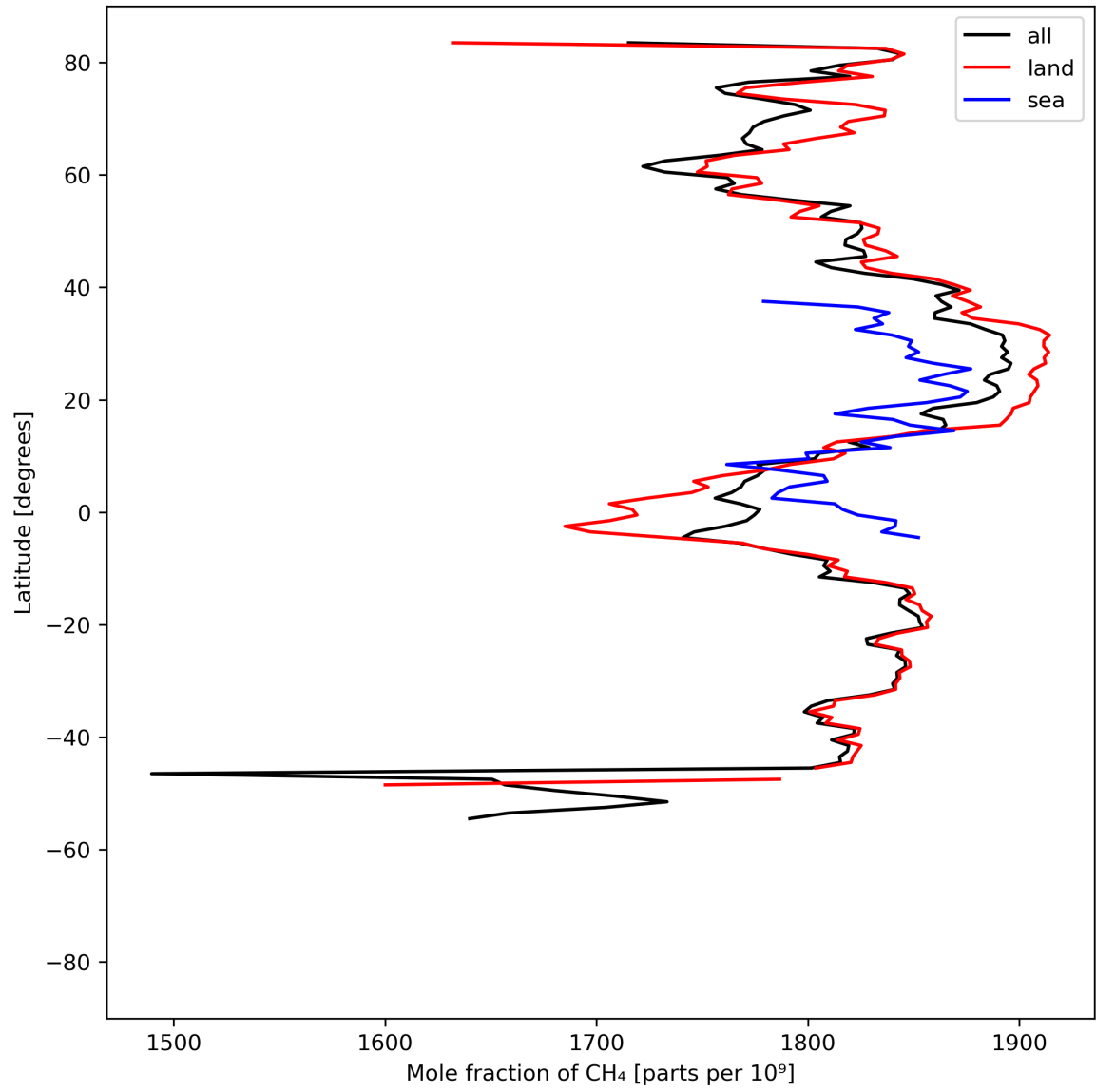
Figure 12: Zonal average of “Mole fraction of \text{CH}_4 ” for 2023-08-25 to 2023-08-27.
