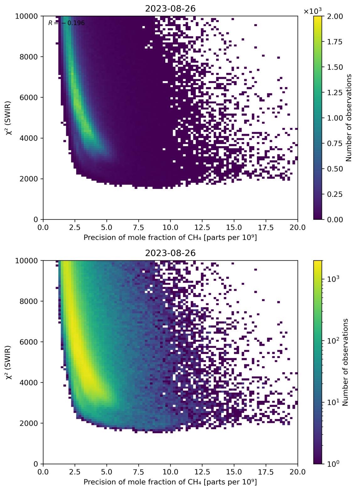
Figure 79: Scatter density plot of “Precision of mole fraction of \text{CH}_4 ” against “ \chi^2 (SWIR)” for 2023-08-25 to 2023-08-27.
