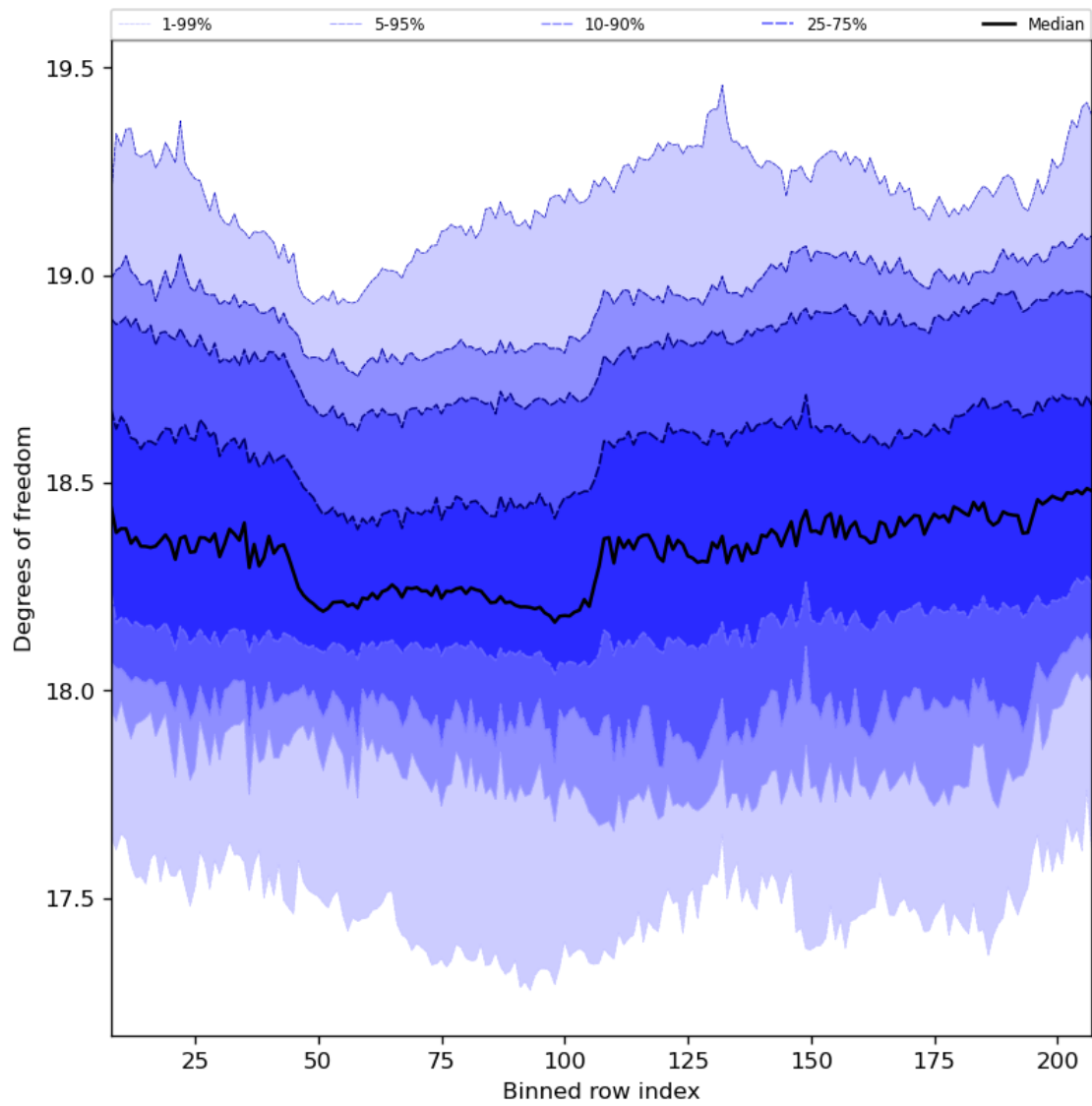
Figure 41: Along track statistics of “Degrees of freedom” for 2023-08-25 to 2023-08-27
