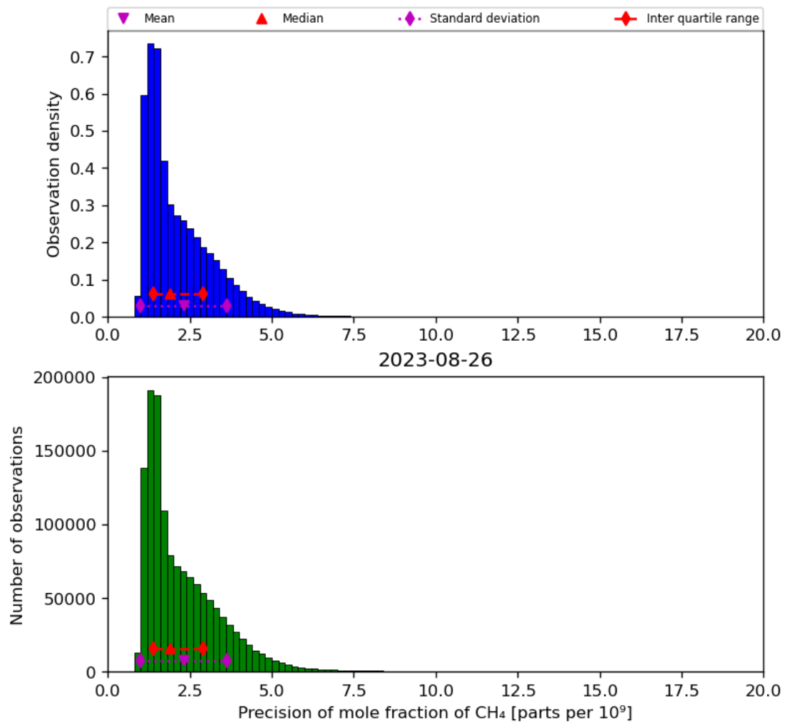
Figure 24: Histogram of “Precision of mole fraction of CH 4 ” for 2023-08-25 to 2023-08-27
