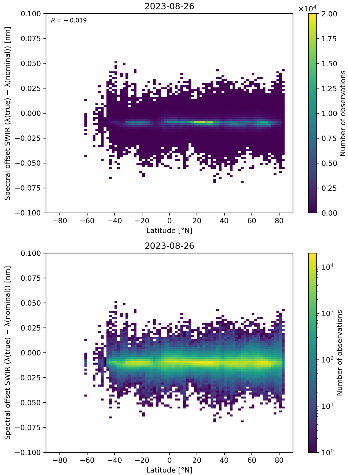
Figure 62: Scatter density plot of “Latitude” against “Spectral offset SWIR ( \lambda(\text{true}) - \lambda(\text{nominal}) )” for 2023-08-25 to 2023-08-27.
