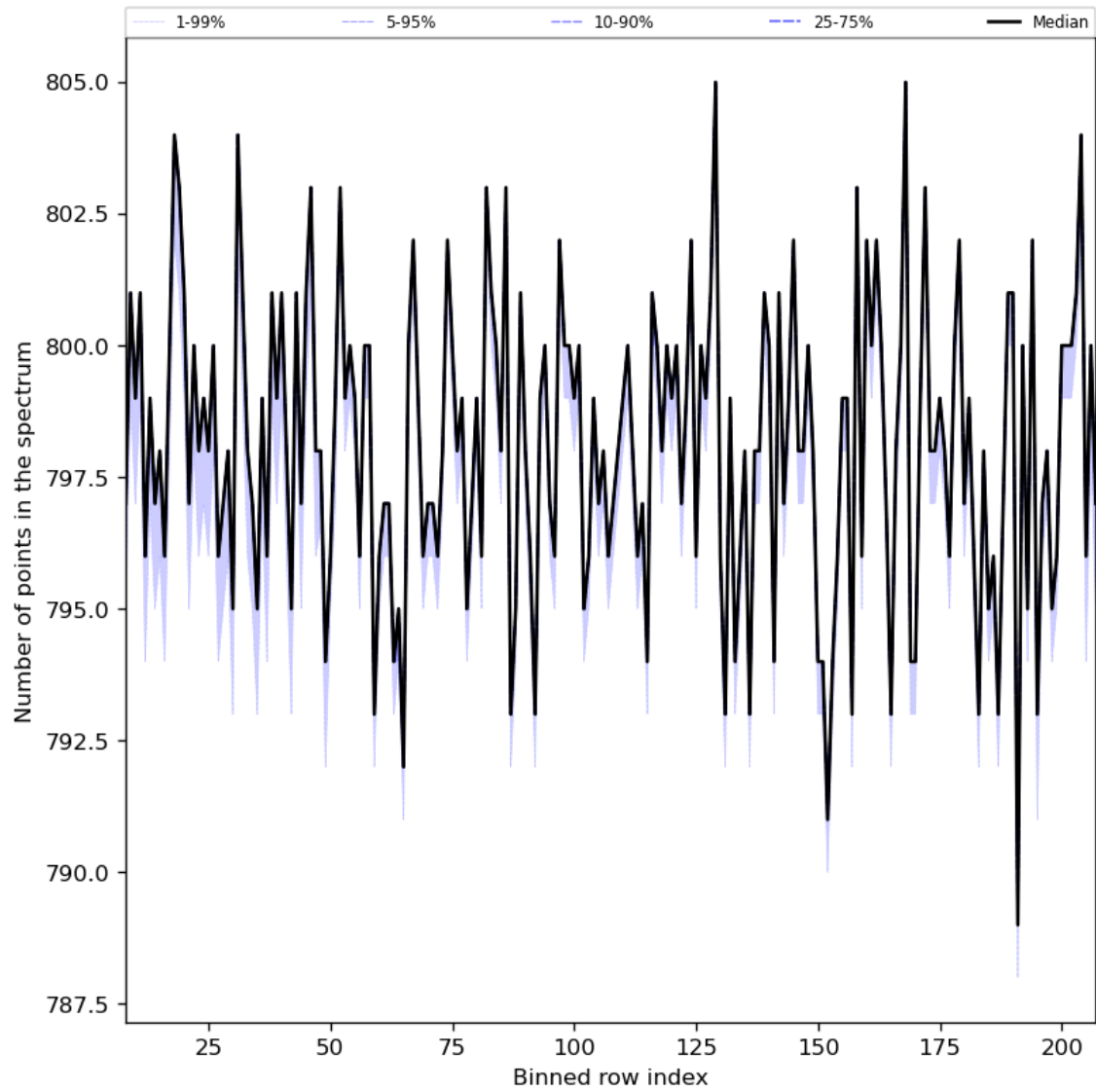
Figure 37: Along track statistics of “Number of points in the spectrum” for 2023-08-25 to 2023-08-27
