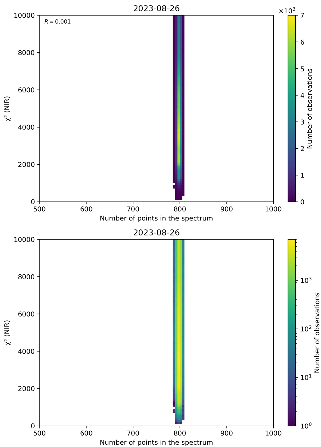
Figure 88: Scatter density plot of “Number of points in the spectrum” against “ \chi^2 (NIR)” for 2023-08-25 to 2023-08-27.
