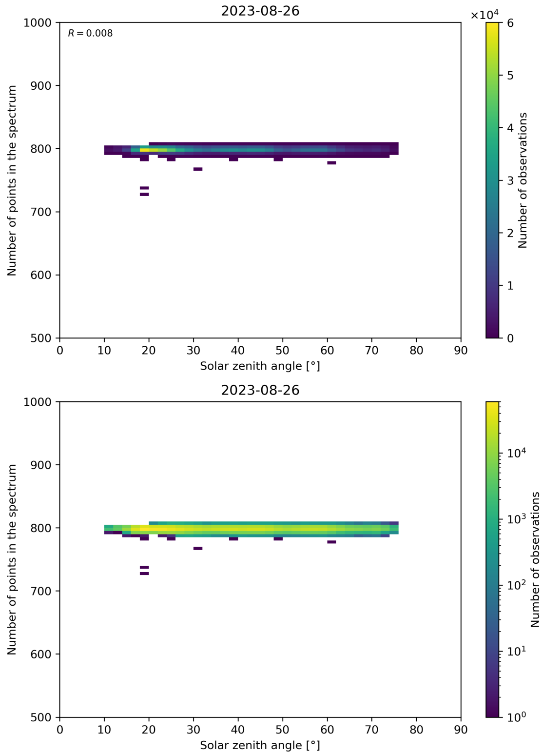
Figure 103: Scatter density plot of “Solar zenith angle” against “Number of points in the spectrum” for 2023-08-25 to 2023-08-27.
