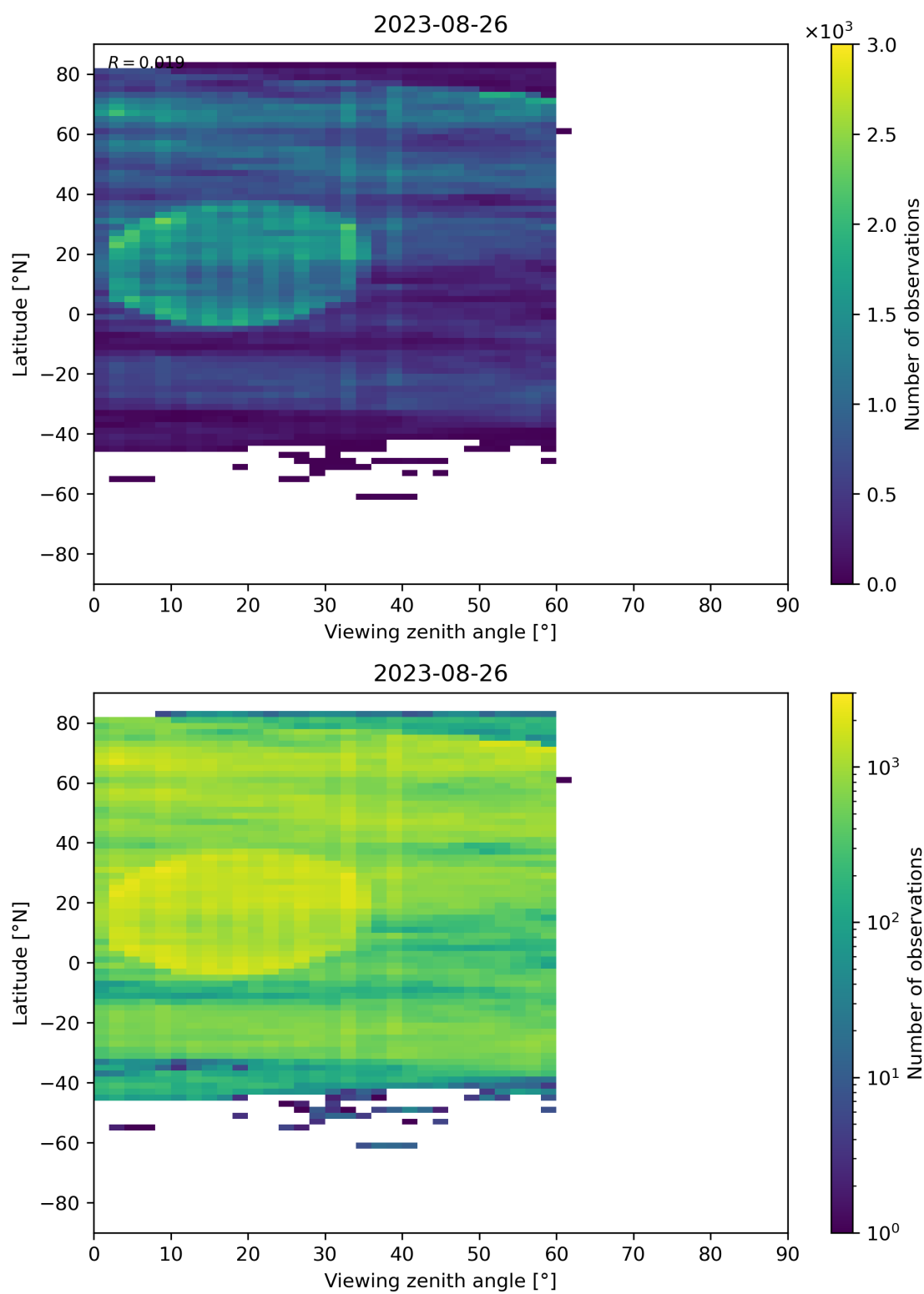
Figure 109: Scatter density plot of “Viewing zenith angle” against “Latitude” for 2023-08-25 to 2023-08-27.
