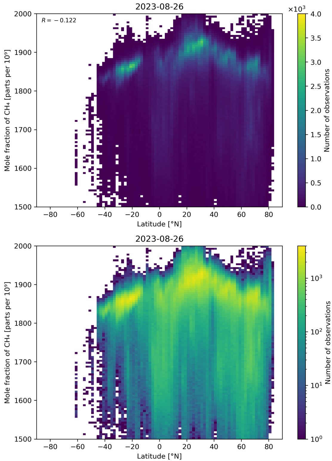
Figure 57: Scatter density plot of “Latitude” against “Mole fraction of \text{CH}_4 ” for 2023-08-25 to 2023-08-27.
