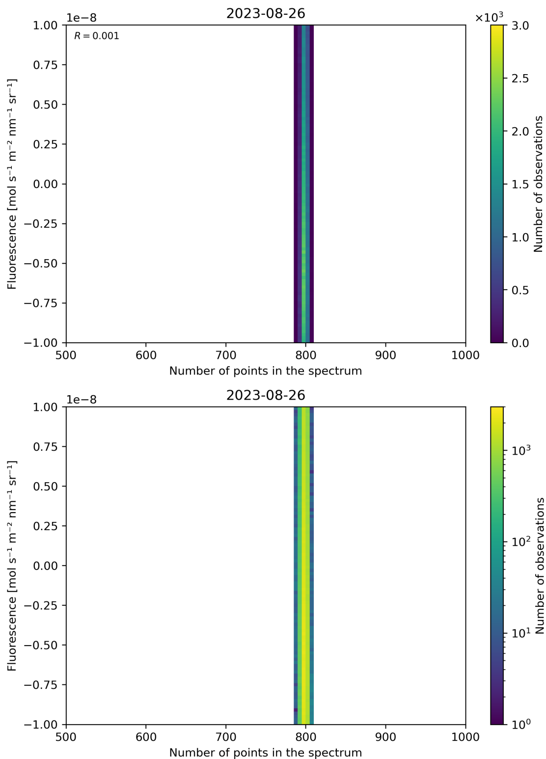
Figure 91: Scatter density plot of “Number of points in the spectrum” against “Fluorescence” for 2023-08-25 to 2023-08-27.
