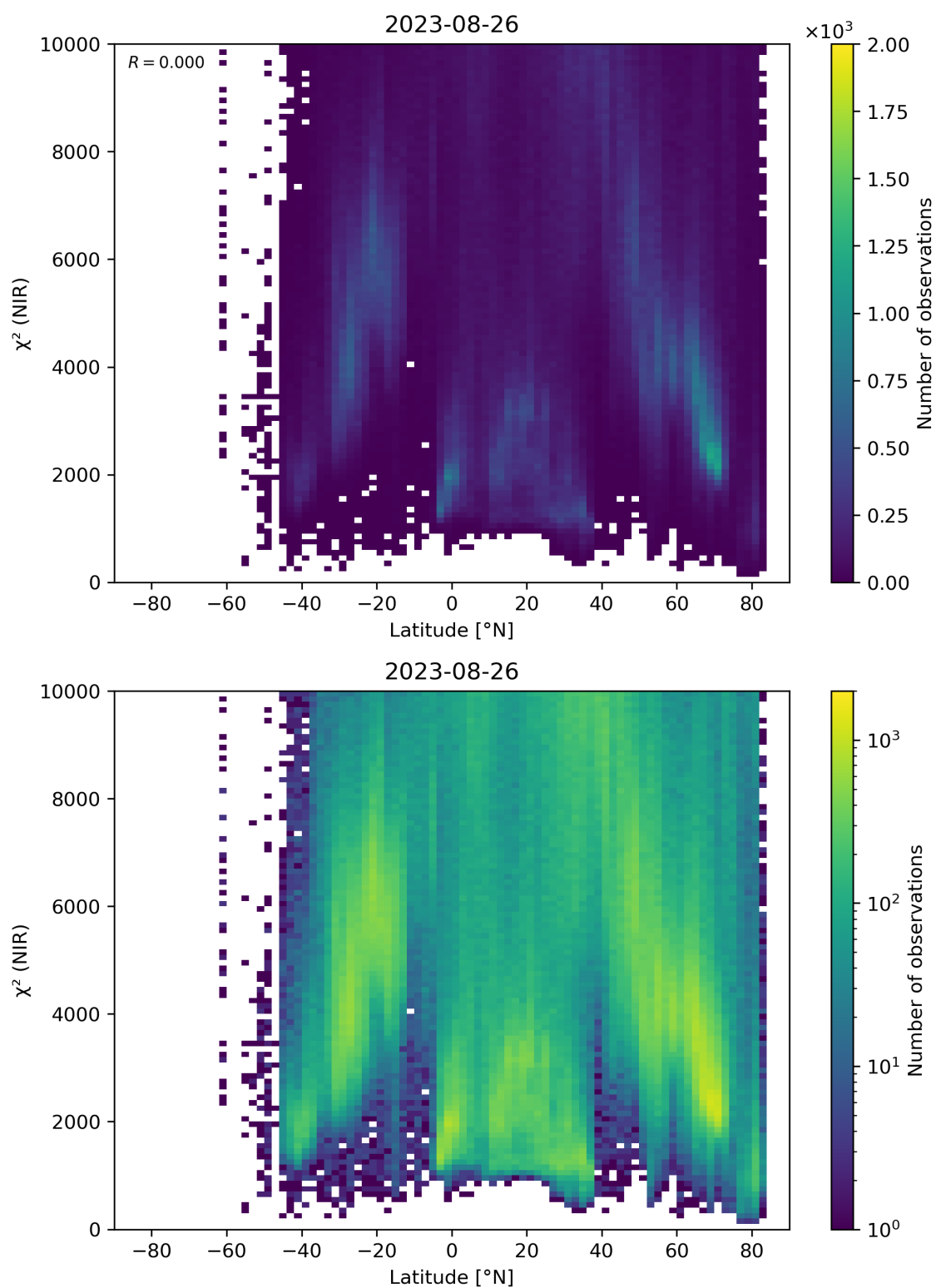
Figure 53: Scatter density plot of “Latitude” against “ \chi^2 (NIR)” for 2023-08-25 to 2023-08-27.
