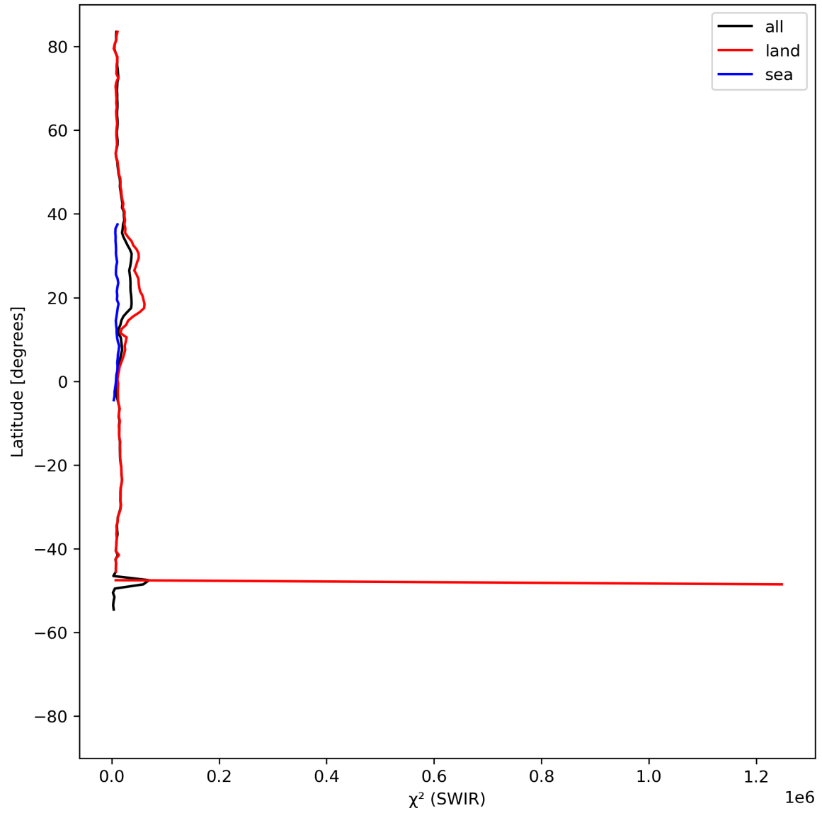
Figure 17: Zonal average of “ \chi^2 (SWIR)” for 2023-08-25 to 2023-08-27.
