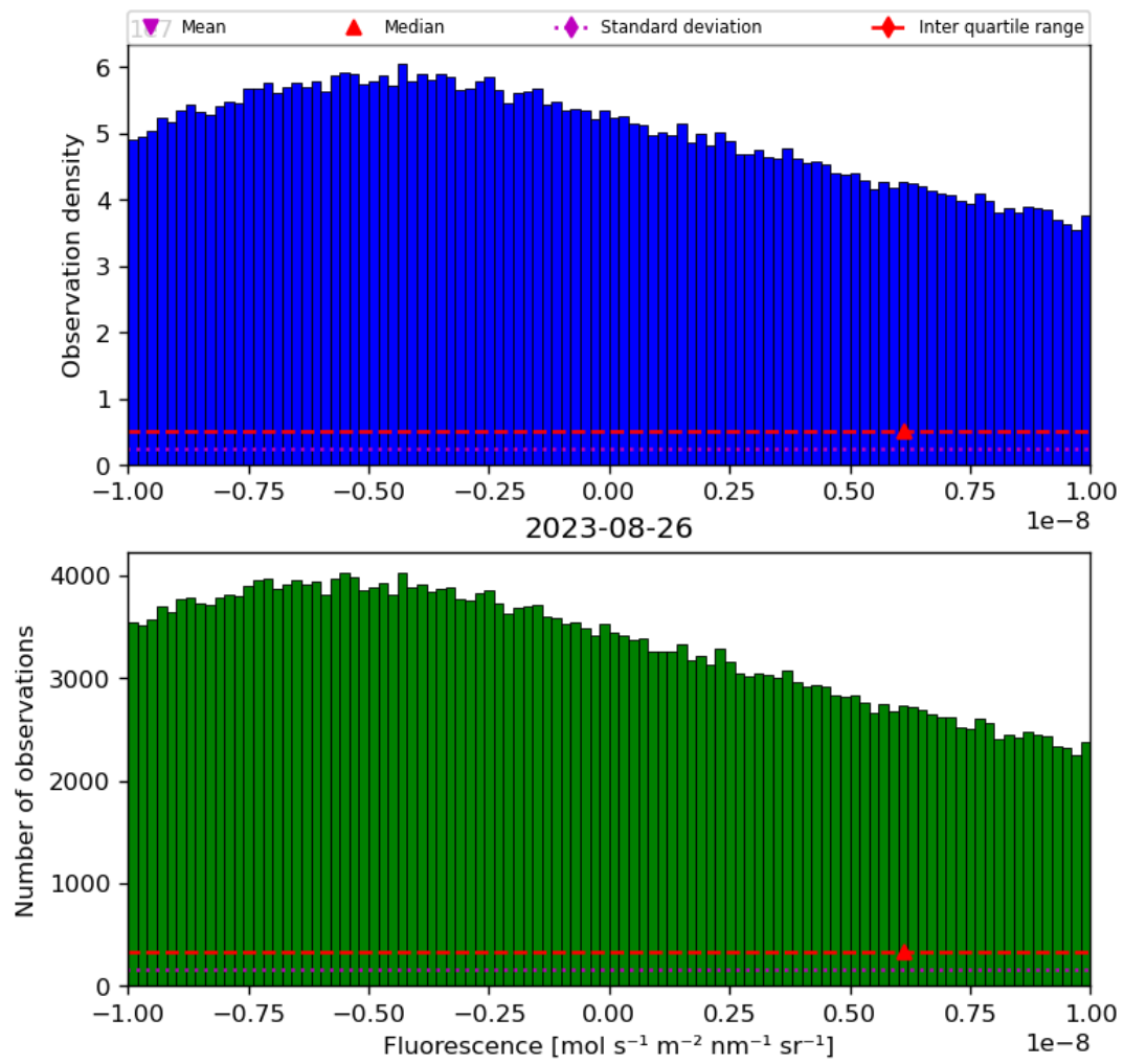
Figure 32: Histogram of “Fluorescence” for 2023-08-25 to 2023-08-27
