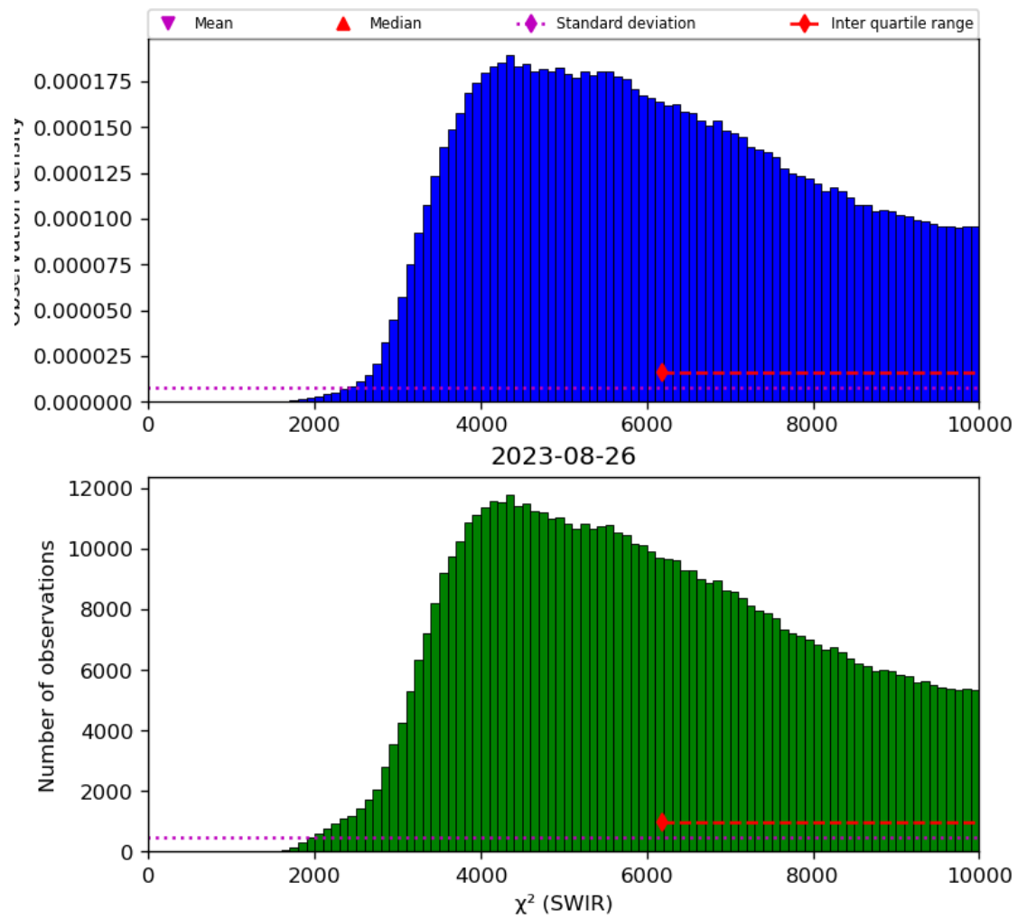
Figure 28: Histogram of “ \chi^2 (SWIR)” for 2023-08-25 to 2023-08-27
