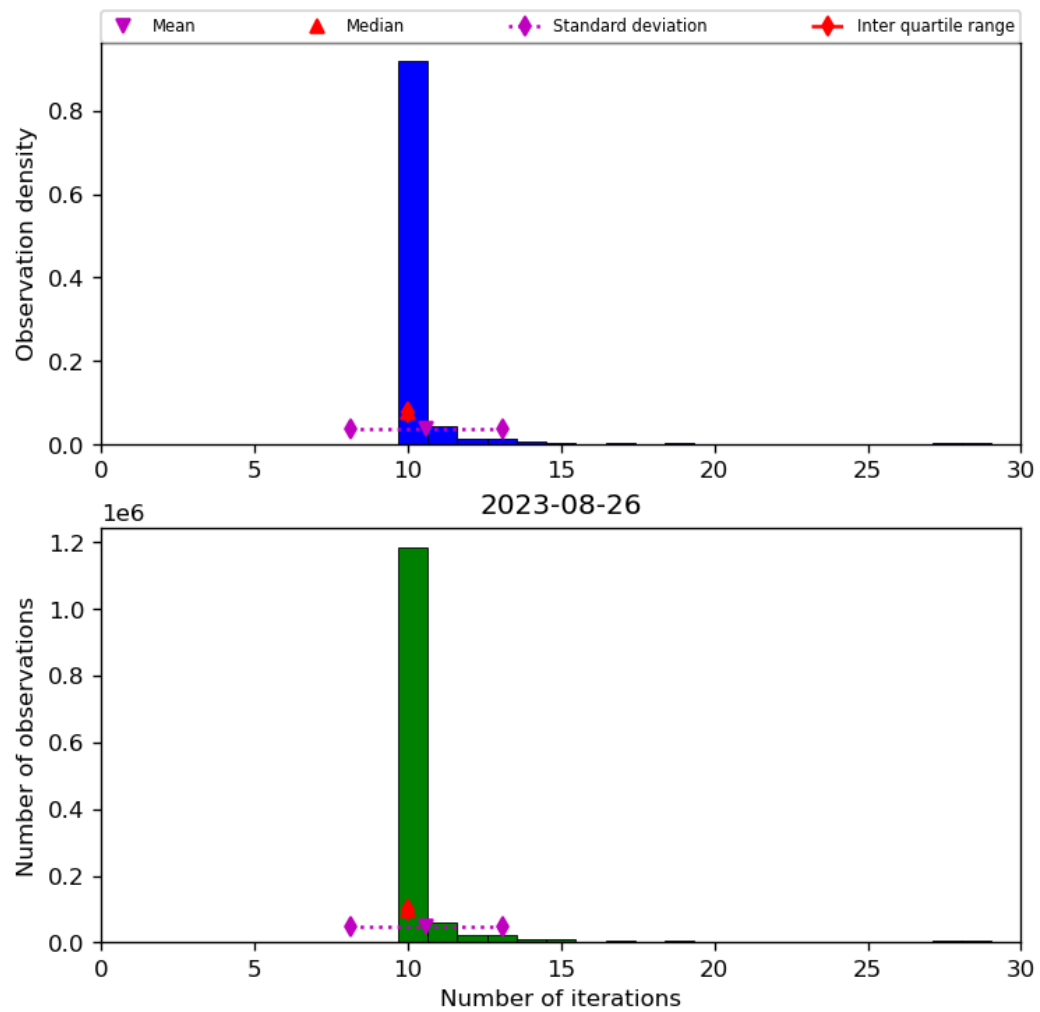
Figure 31: Histogram of “Number of iterations” for 2023-08-25 to 2023-08-27
