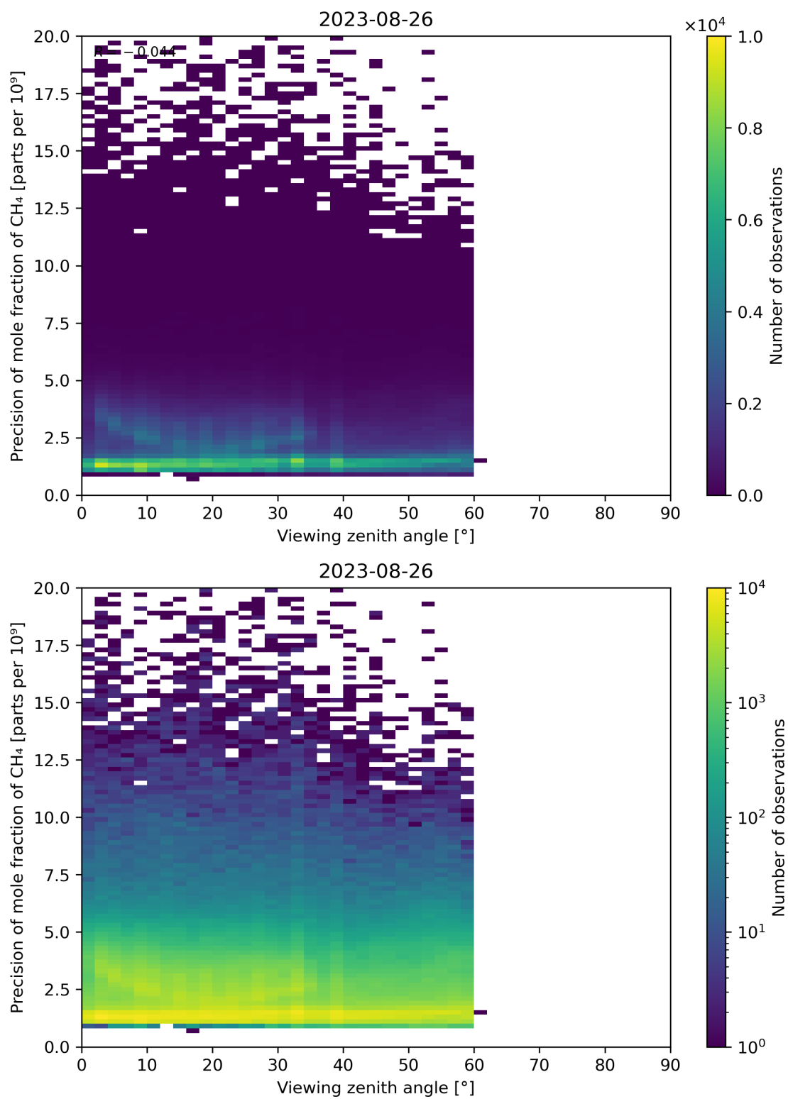
Figure 112: Scatter density plot of “Viewing zenith angle” against “Precision of mole fraction of CH 4 ” for 2023-08-25 to 2023-08-27.
