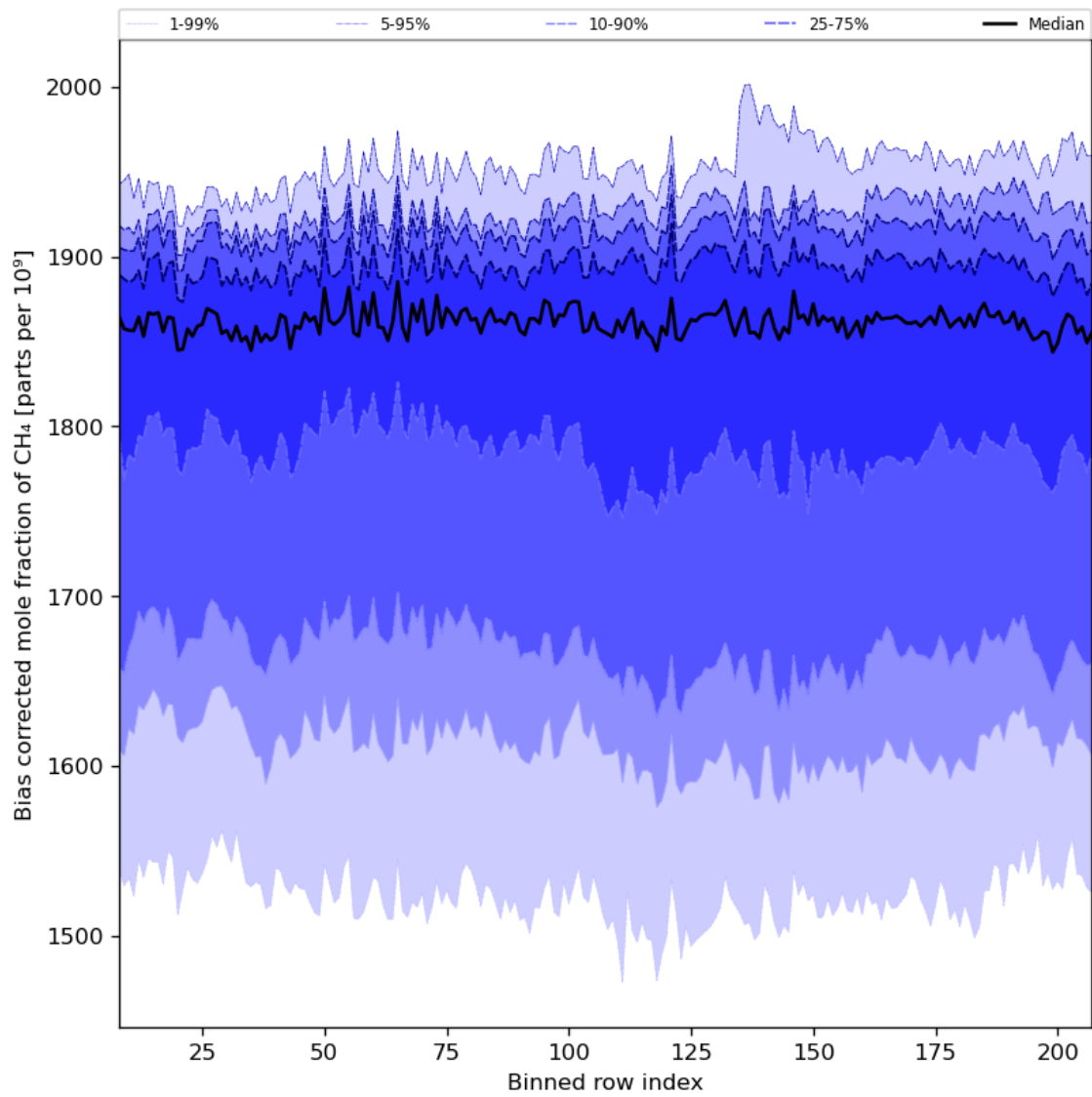
Figure 36: Along track statistics of “Bias corrected mole fraction of CH 4 ” for 2023-08-25 to 2023-08-27
