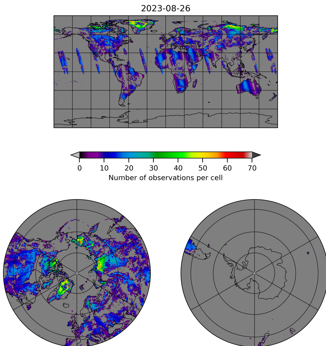
Figure 10: Map of the number of observations for 2023-08-25 to 2023-08-27
