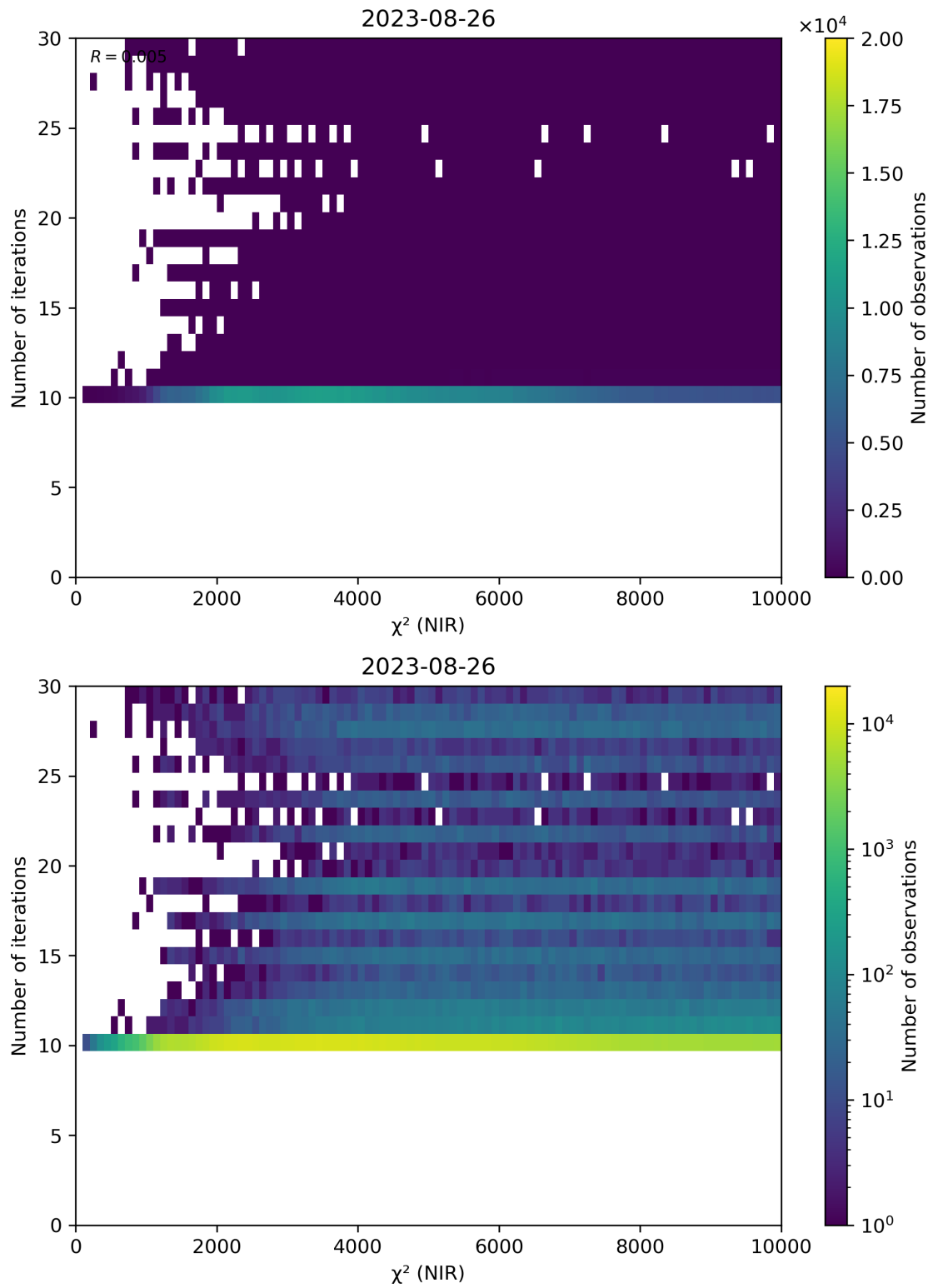
Figure 46: Scatter density plot of “ \chi^2 (NIR)” against “Number of iterations” for 2023-08-25 to 2023-08-27.
