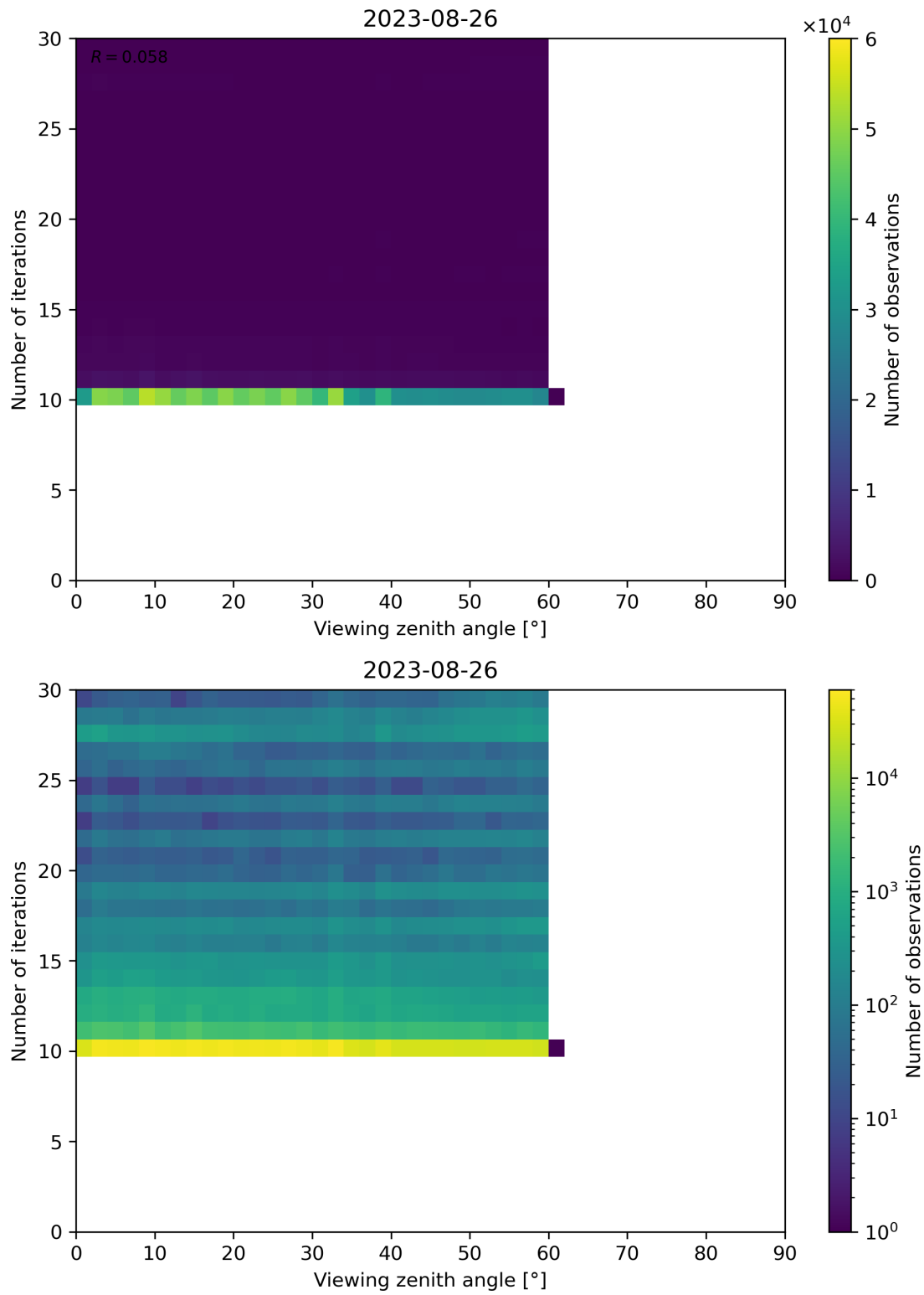
Figure 113: Scatter density plot of “Viewing zenith angle” against “Number of iterations” for 2023-08-25 to 2023-08-27.
