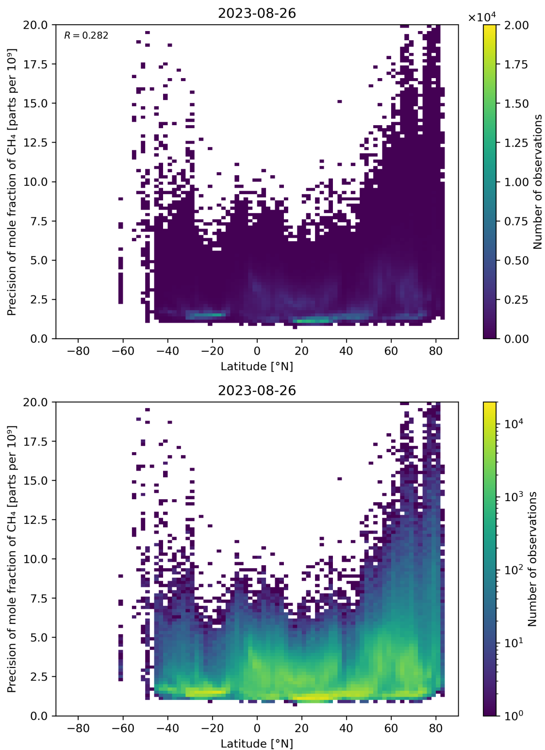
Figure 59: Scatter density plot of “Latitude” against “Precision of mole fraction of \text{CH}_4 ” for 2023-08-25 to 2023-08-27.
