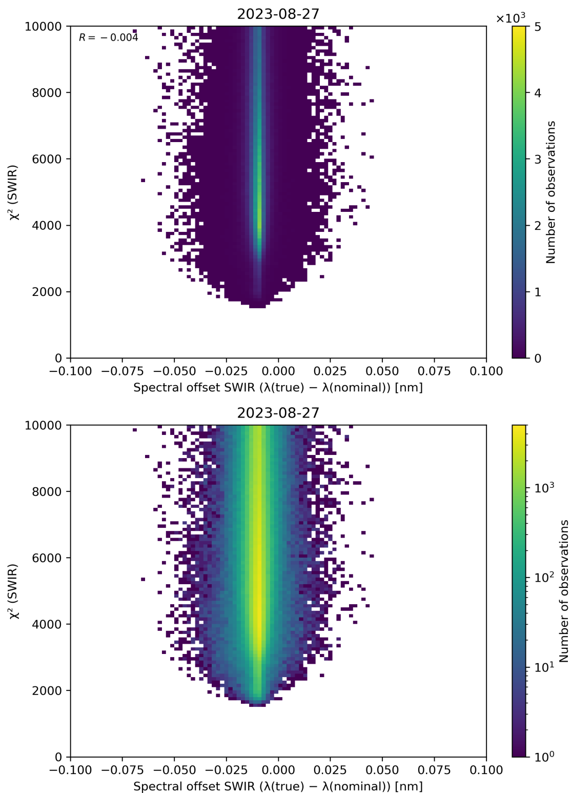
Figure 118: Scatter density plot of “Spectral offset SWIR ( \lambda(\text{true}) - \lambda(\text{nominal}) )” against “ \chi^2 (SWIR)” for 2023-08-26 to 2023-08-28.
