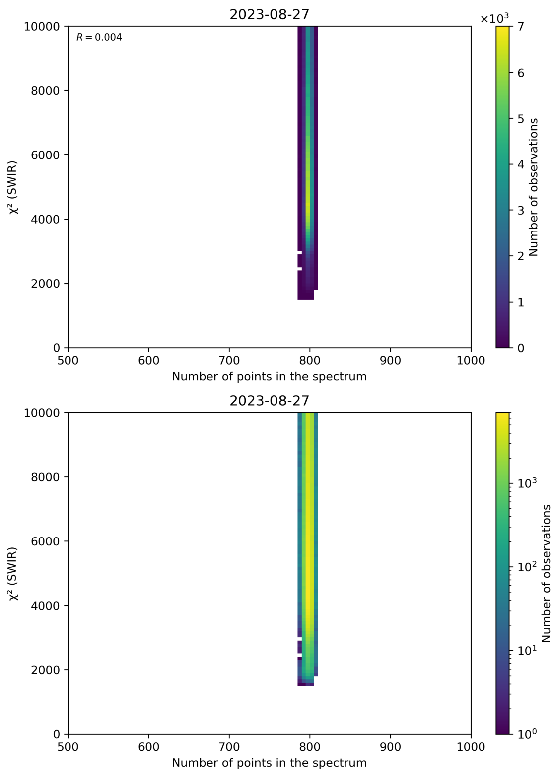
Figure 89: Scatter density plot of “Number of points in the spectrum” against “ \chi^2 (SWIR)” for 2023-08-26 to 2023-08-28.
