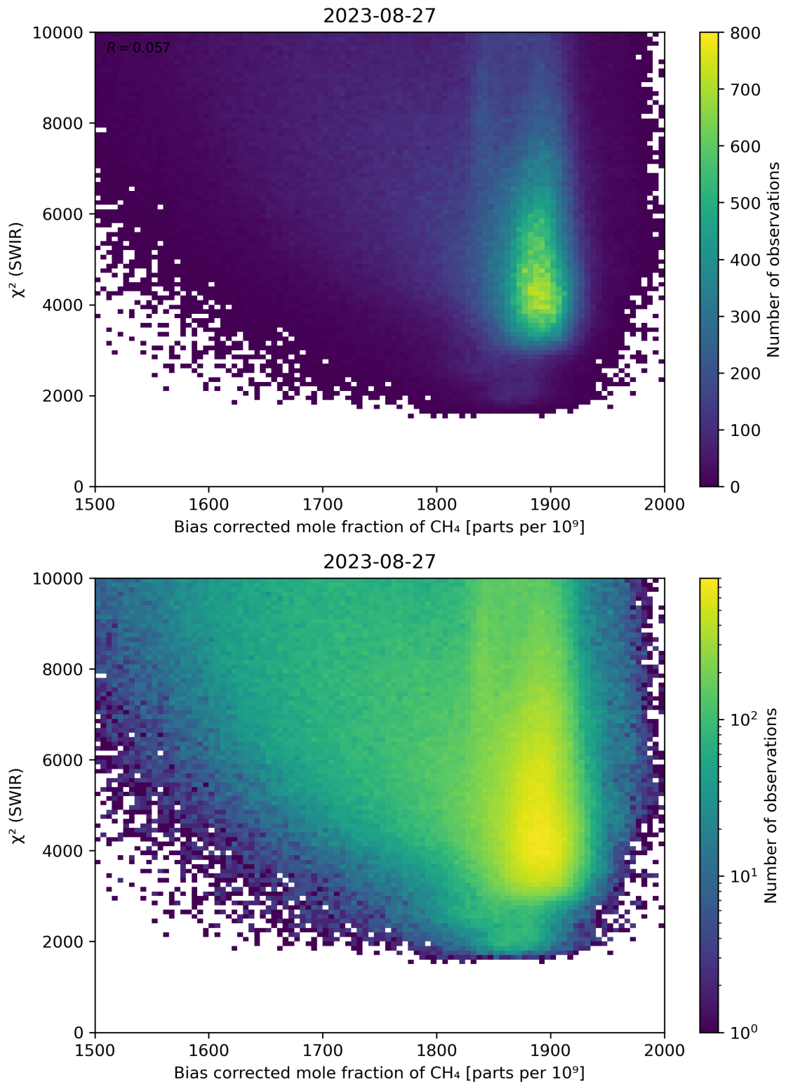
Figure 64: Scatter density plot of “Bias corrected mole fraction of CH 4 ” against “ \chi^2 (SWIR)” for 2023-08-26 to 2023-08-28.
