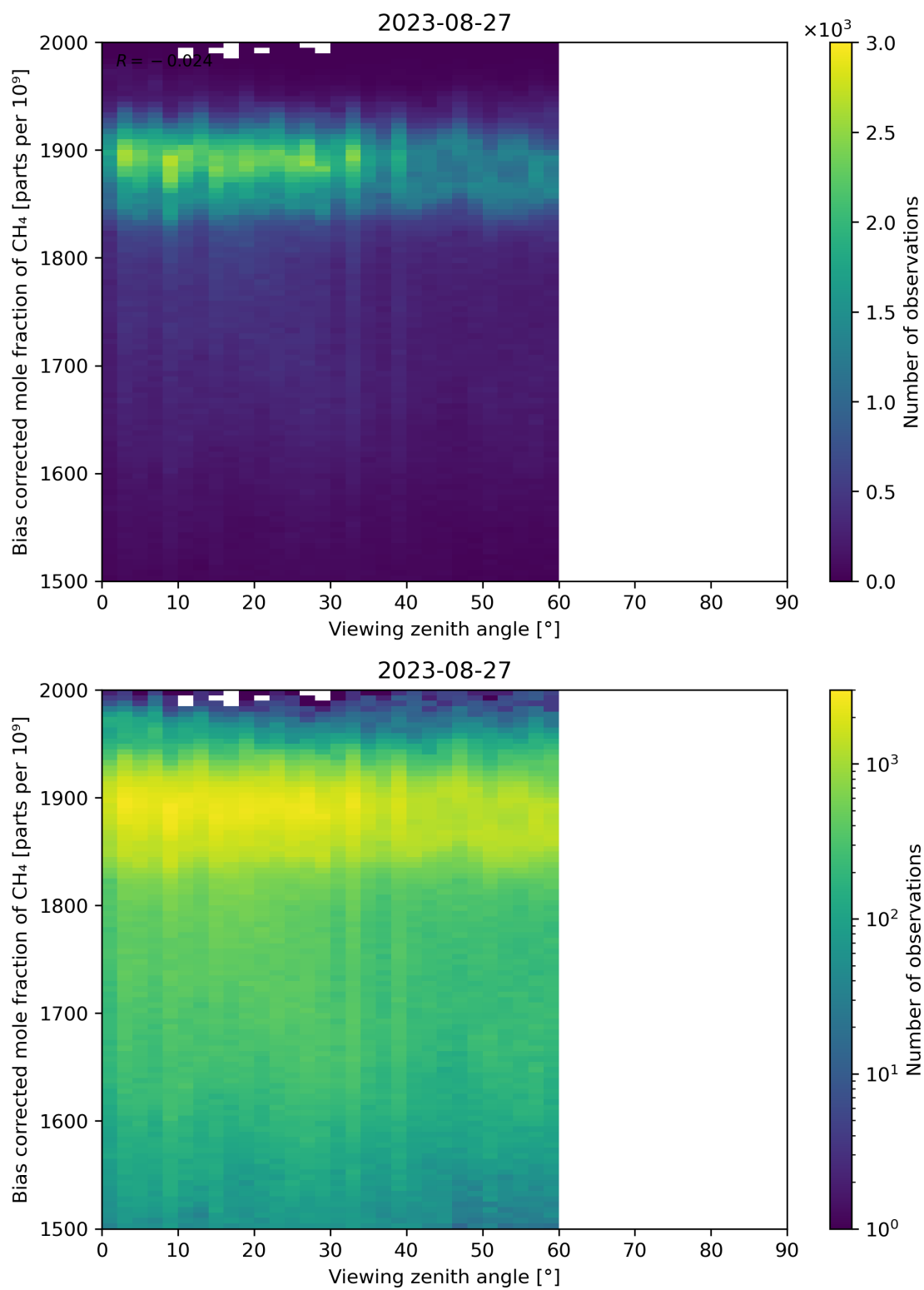
Figure 111: Scatter density plot of “Viewing zenith angle” against “Bias corrected mole fraction of CH 4 ” for 2023-08-26 to 2023-08-28.
