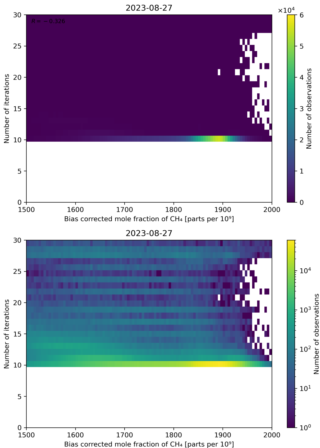
Figure 67: Scatter density plot of “Bias corrected mole fraction of CH 4 ” against “Number of iterations” for 2023-08-26 to 2023-08-28.
