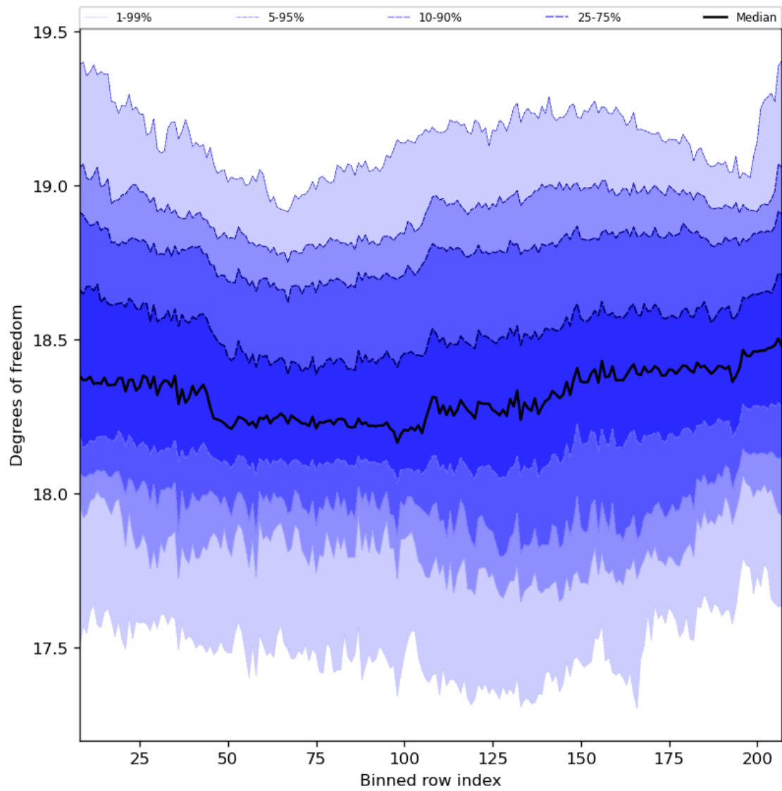
Figure 41: Along track statistics of “Degrees of freedom” for 2023-08-26 to 2023-08-28
