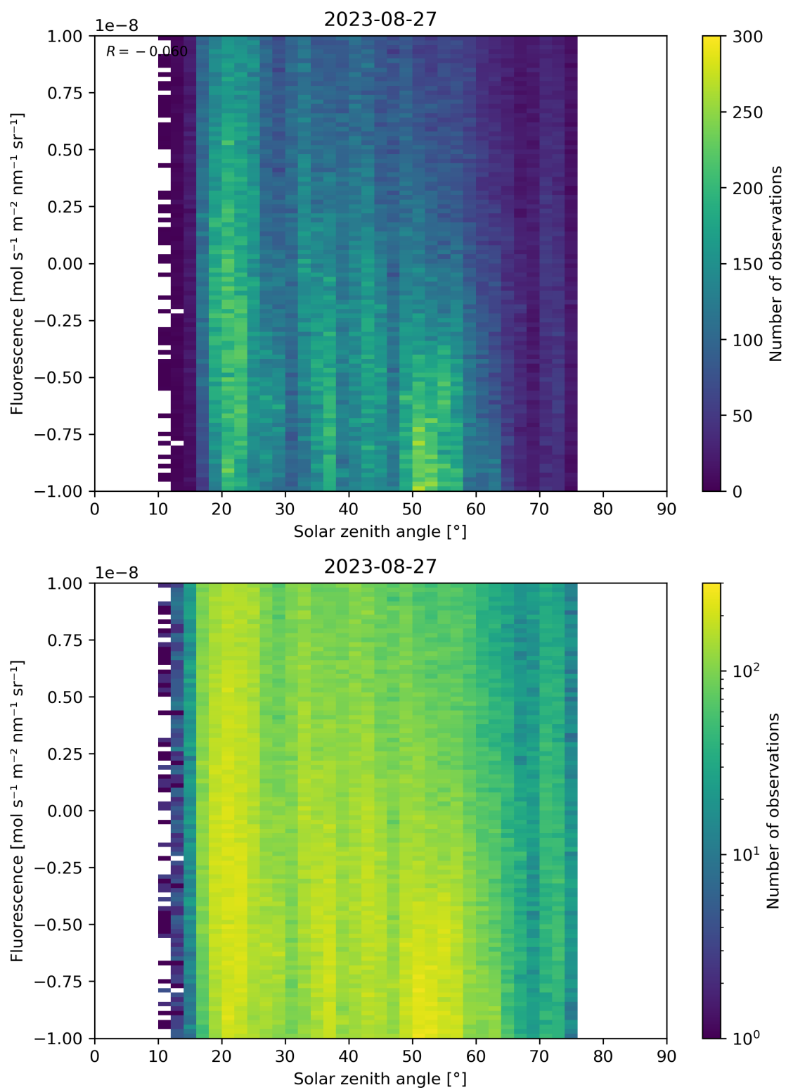
Figure 97: Scatter density plot of “Solar zenith angle” against “Fluorescence” for 2023-08-26 to 2023-08-28.
