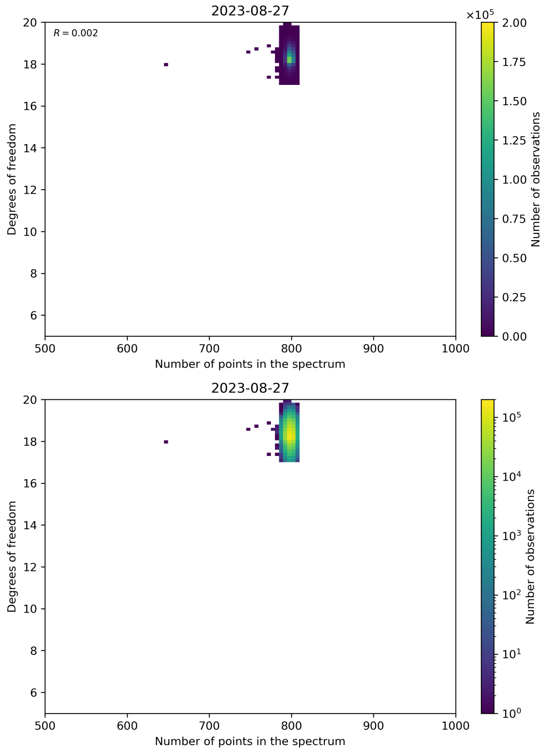
Figure 90: Scatter density plot of “Number of points in the spectrum” against “Degrees of freedom” for 2023-08-26 to 2023-08-28.
