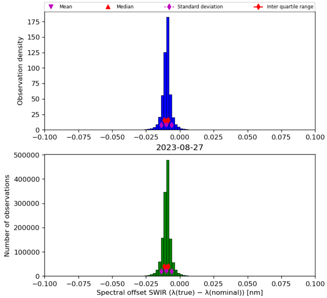
Figure 27: Histogram of “Spectral offset SWIR ( \lambda(\text{true}) - \lambda(\text{nominal}) )” for 2023-08-26 to 2023-08-28
