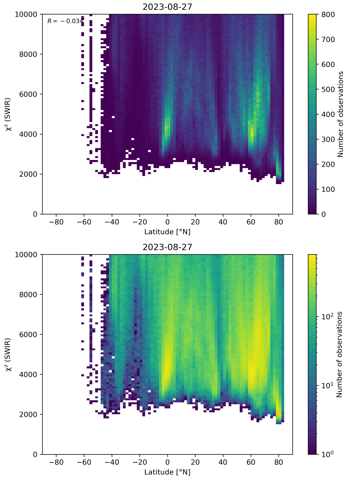
Figure 54: Scatter density plot of “Latitude” against “ \chi^2 (SWIR)” for 2023-08-26 to 2023-08-28.
