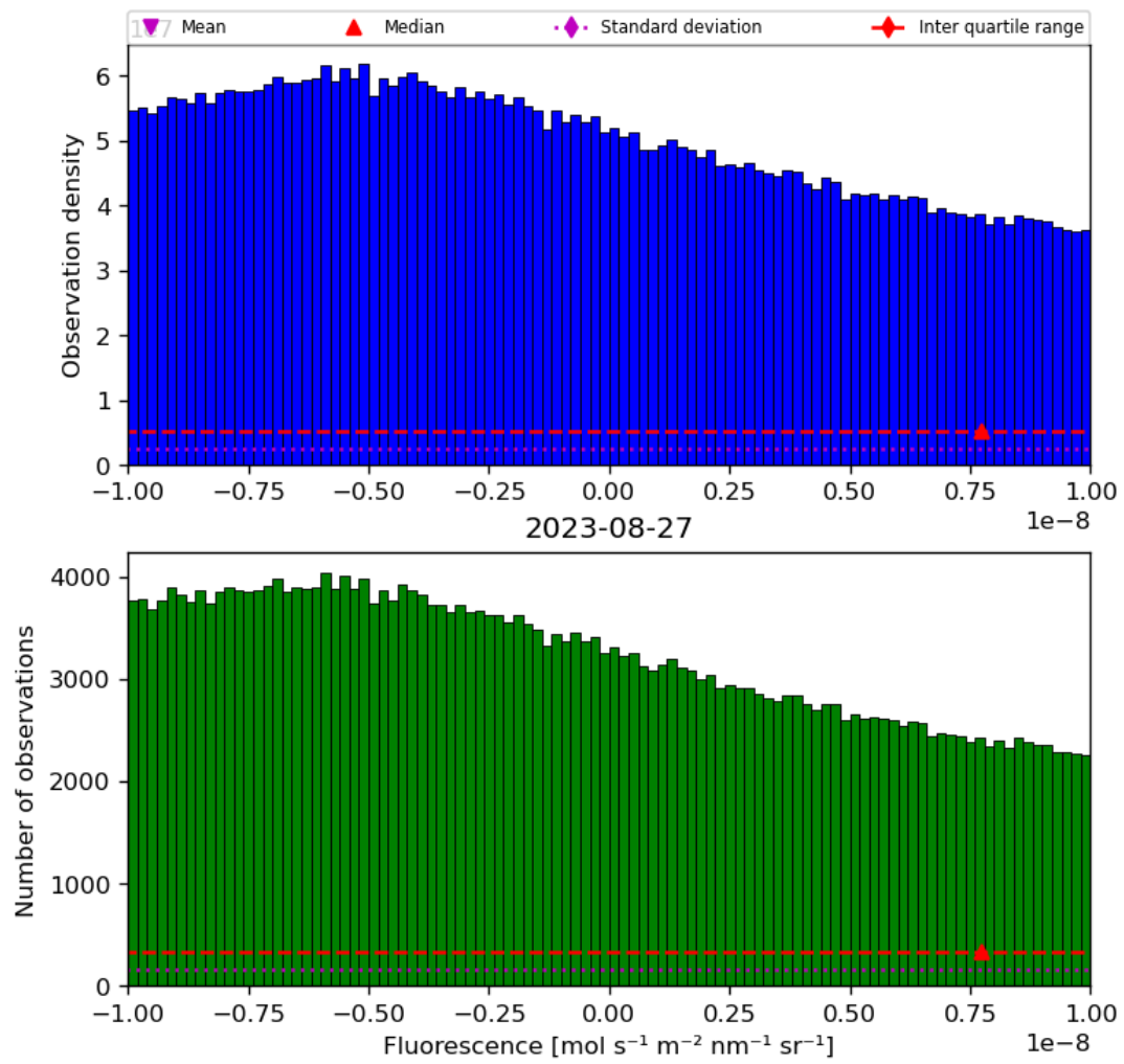
Figure 32: Histogram of “Fluorescence” for 2023-08-26 to 2023-08-28
