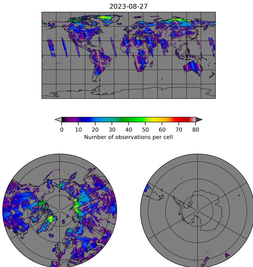
Figure 10: Map of the number of observations for 2023-08-26 to 2023-08-28
