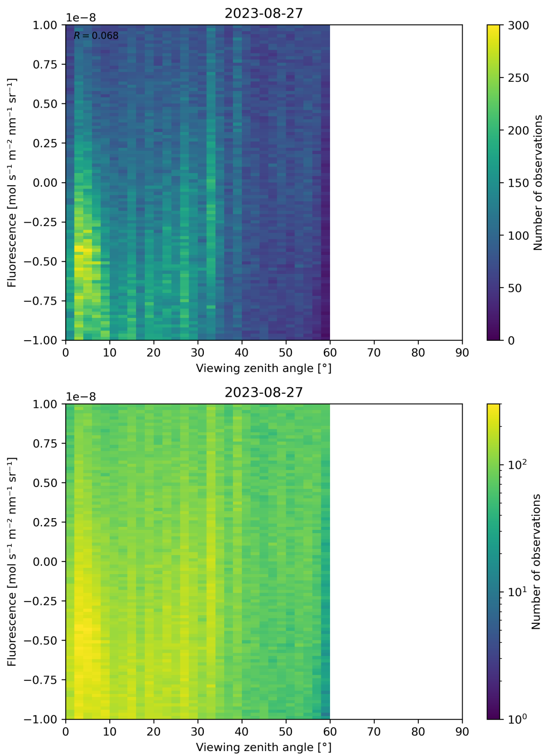
Figure 108: Scatter density plot of “Viewing zenith angle” against “Fluorescence” for 2023-08-26 to 2023-08-28.
