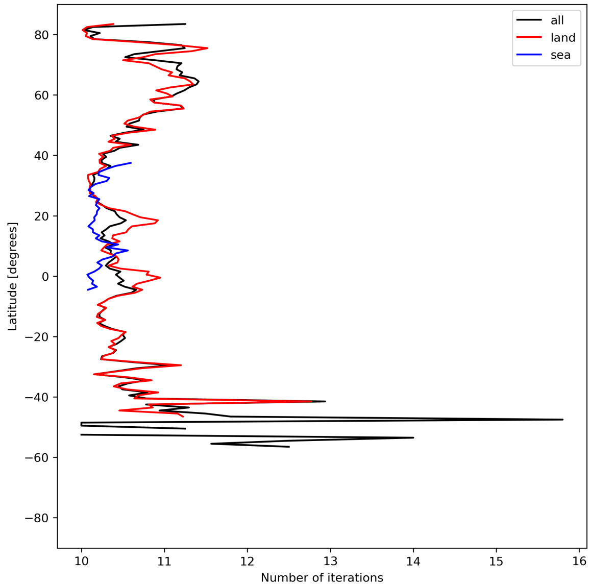
Figure 20: Zonal average of “Number of iterations” for 2023-08-26 to 2023-08-28.
