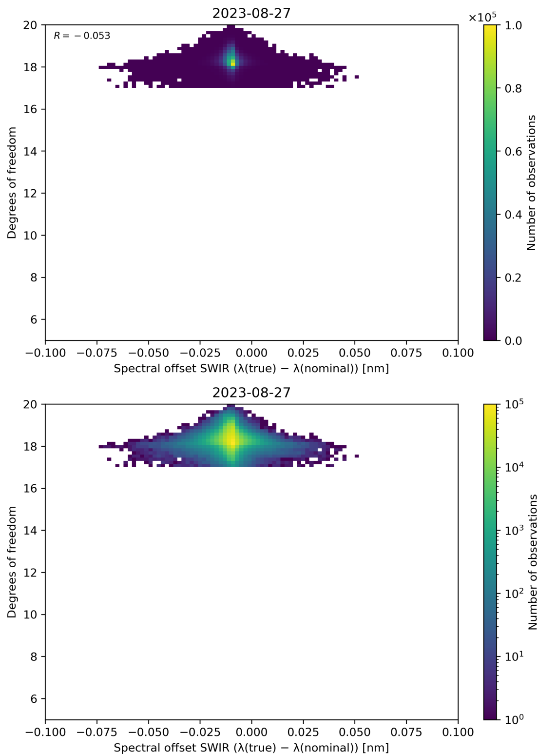
Figure 119: Scatter density plot of “Spectral offset SWIR ( \lambda(\text{true}) - \lambda(\text{nominal}) )” against “Degrees of freedom” for 2023-08-26 to 2023-08-28.
