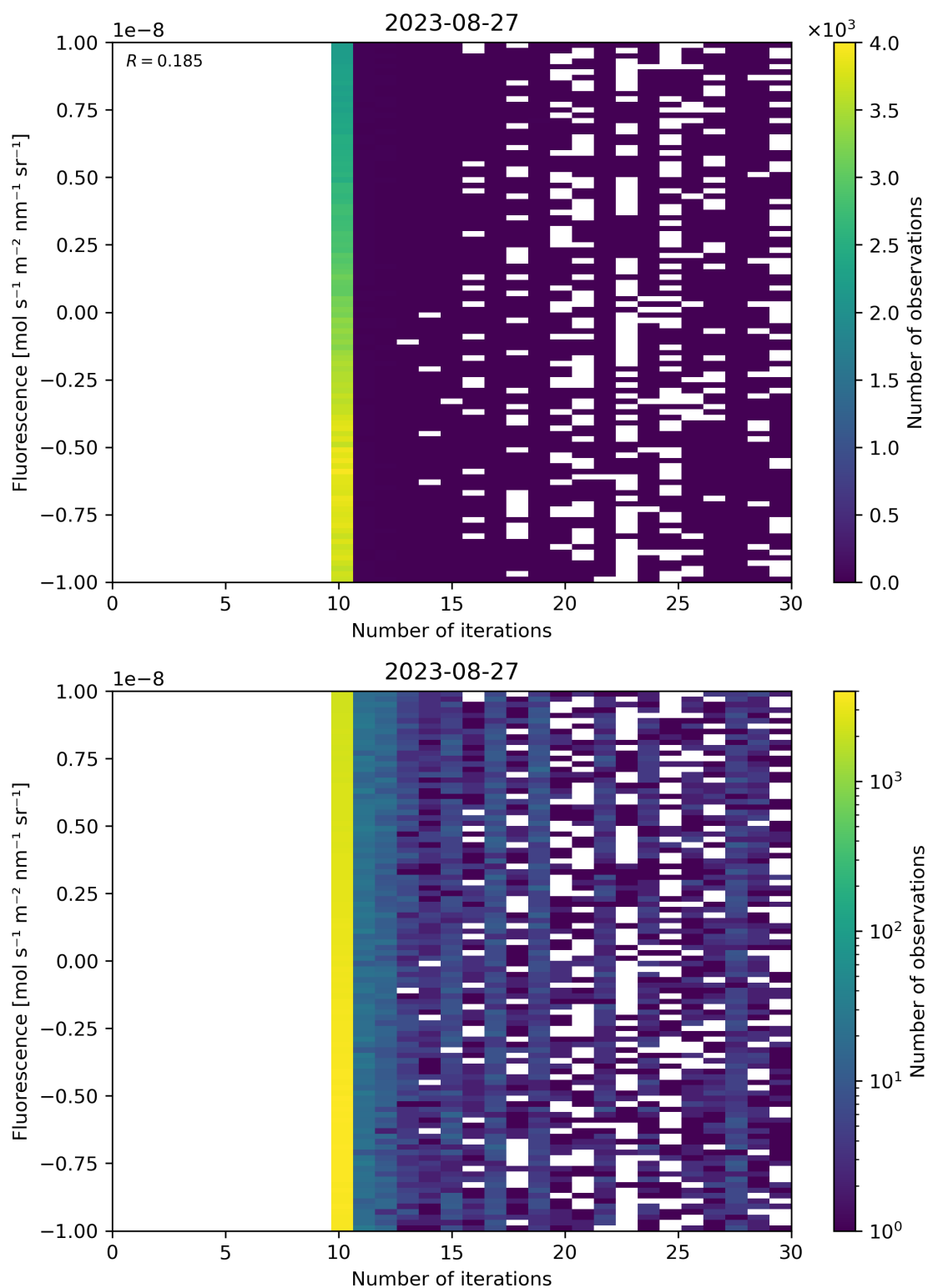
Figure 87: Scatter density plot of “Number of iterations” against “Fluorescence” for 2023-08-26 to 2023-08-28.
