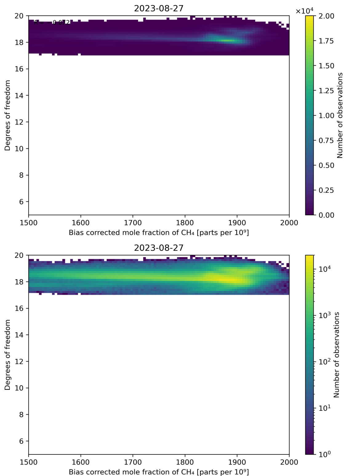
Figure 65: Scatter density plot of “Bias corrected mole fraction of CH 4 ” against “Degrees of freedom” for 2023-08-26 to 2023-08-28.
