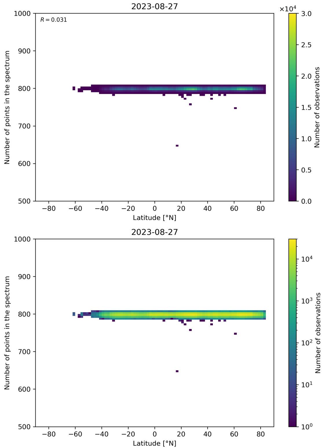
Figure 61: Scatter density plot of “Latitude” against “Number of points in the spectrum” for 2023-08-26 to 2023-08-28.
