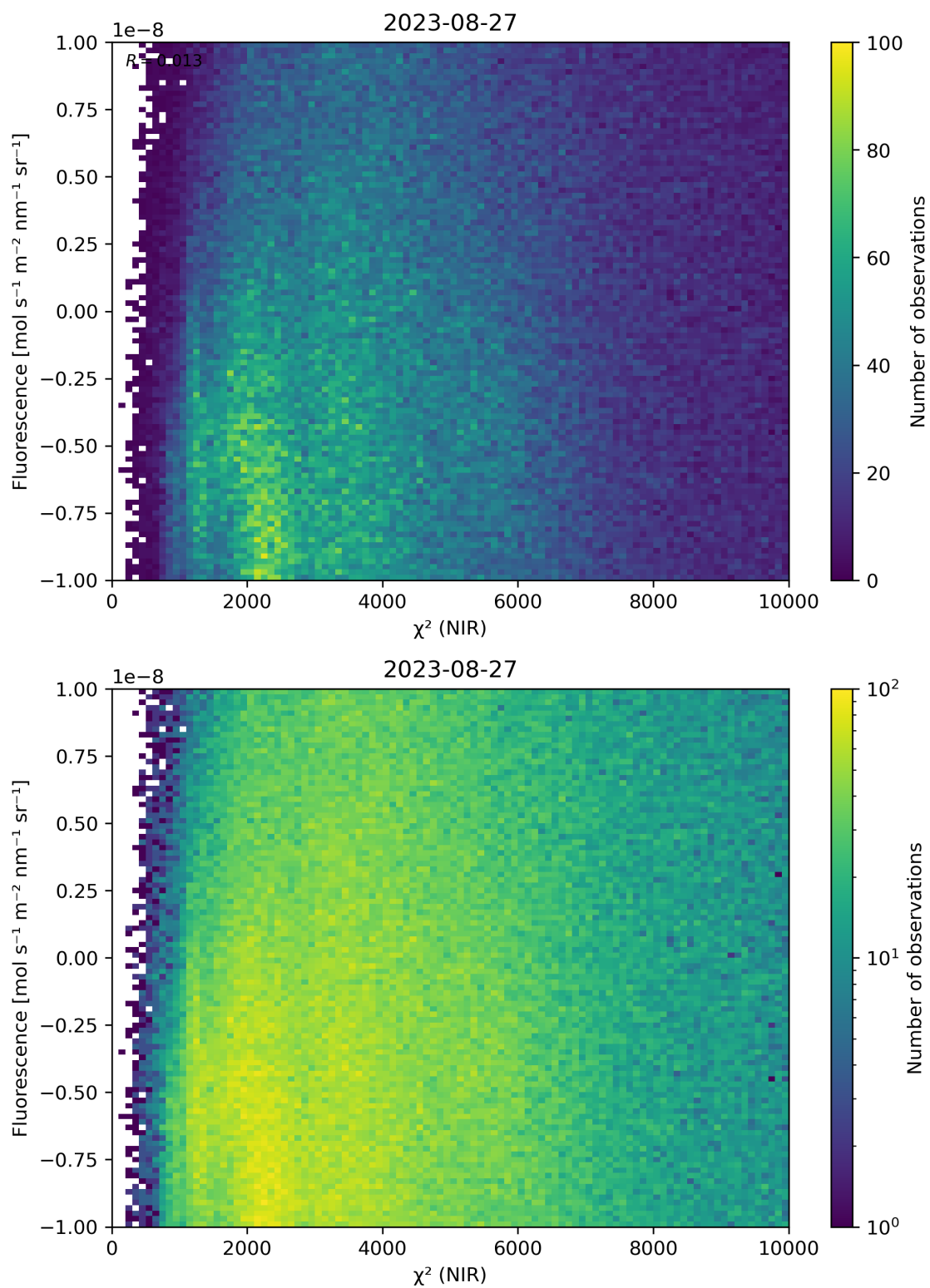
Figure 45: Scatter density plot of “ \chi^2 (NIR)” against “Fluorescence” for 2023-08-26 to 2023-08-28.
