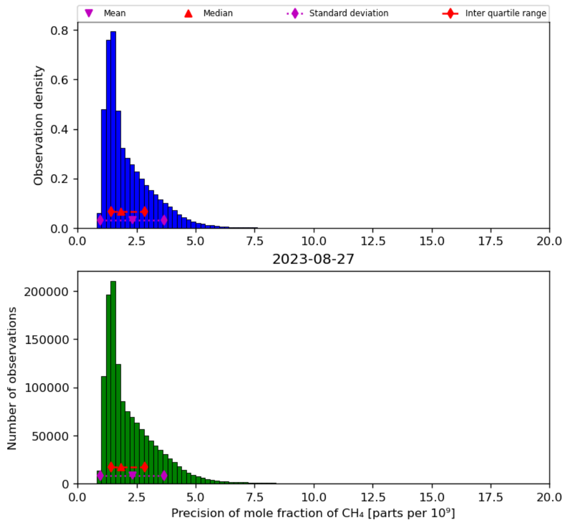
Figure 24: Histogram of “Precision of mole fraction of CH 4 ” for 2023-08-26 to 2023-08-28
