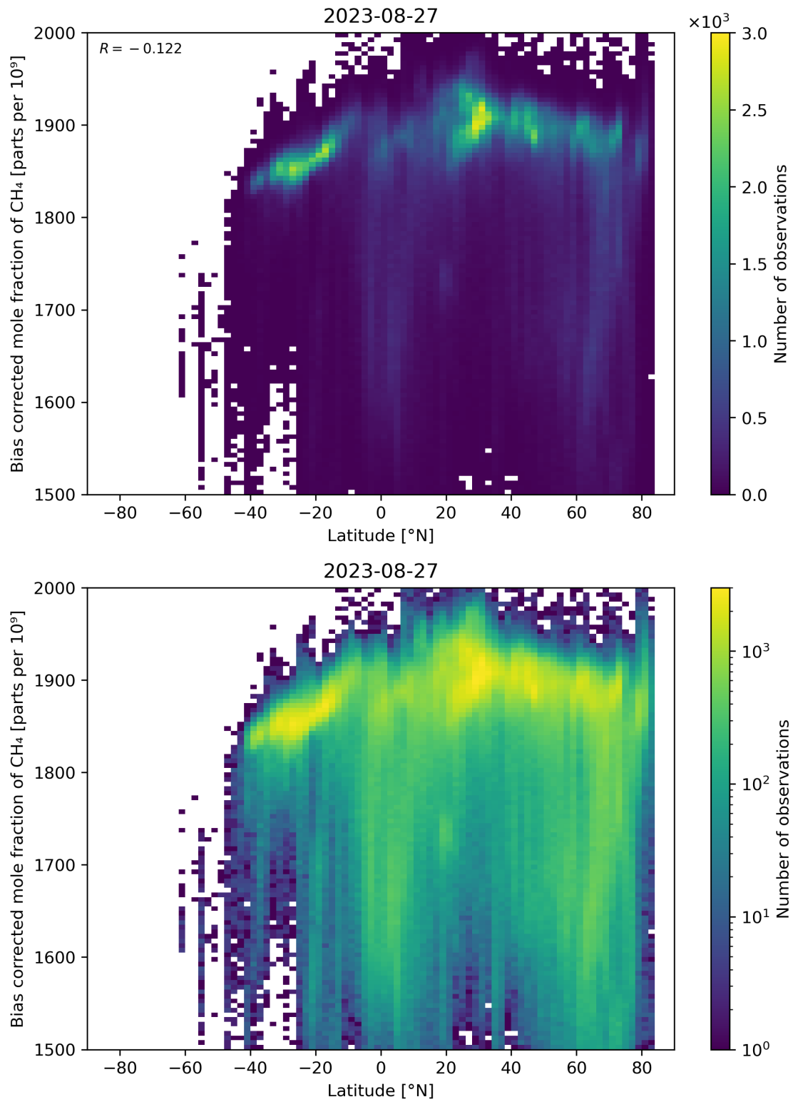
Figure 58: Scatter density plot of “Latitude” against “Bias corrected mole fraction of \text{CH}_4 ” for 2023-08-26 to 2023-08-28.
