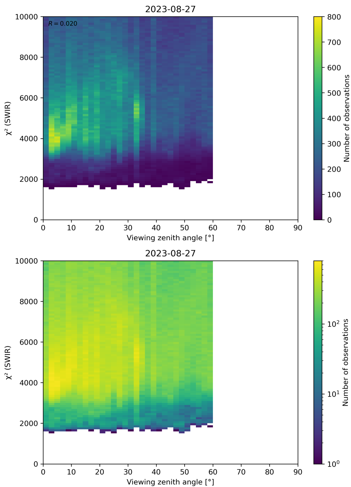
Figure 106: Scatter density plot of “Viewing zenith angle” against “ \chi^2 (SWIR)” for 2023-08-26 to 2023-08-28.
