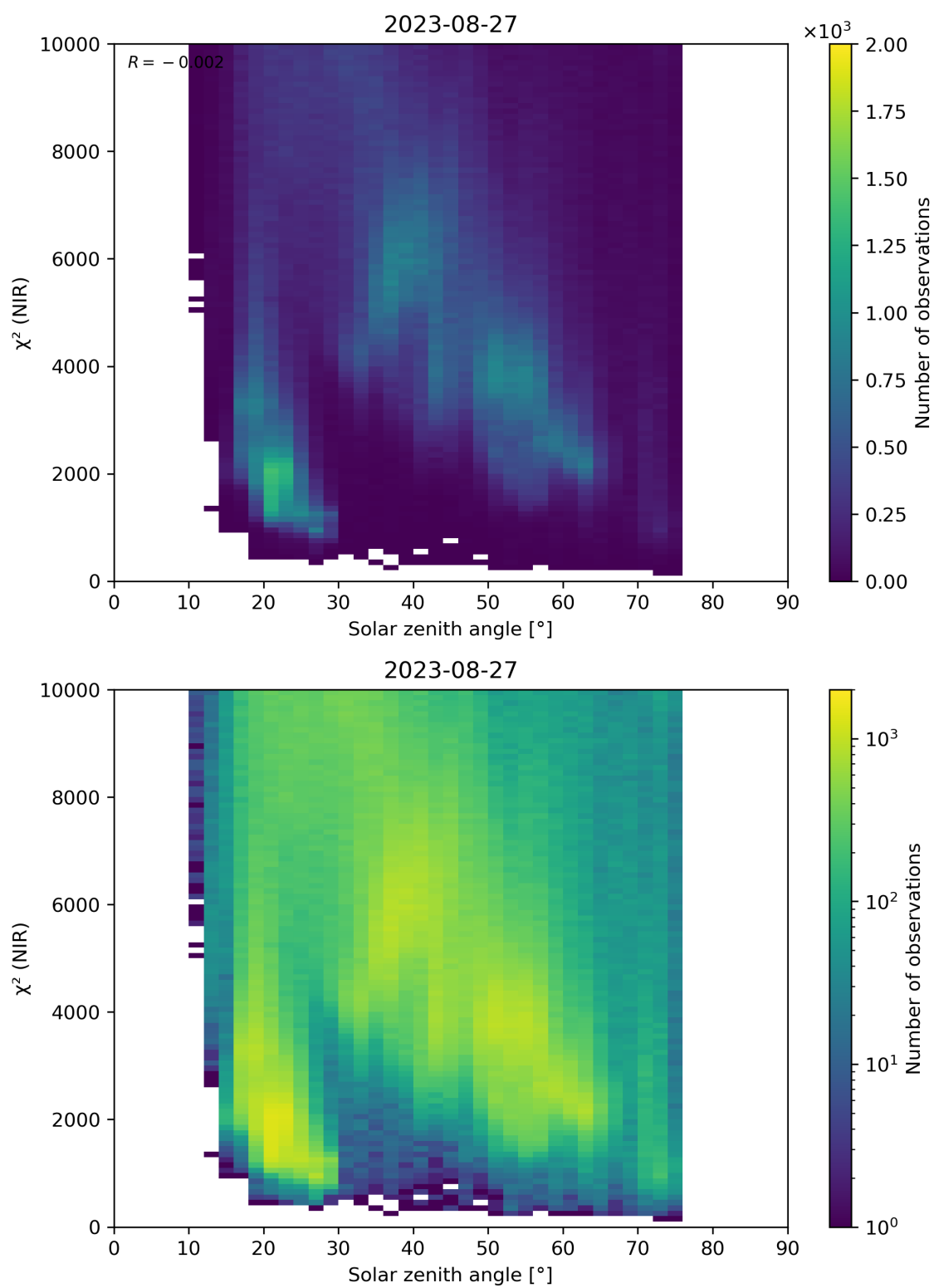
Figure 94: Scatter density plot of “Solar zenith angle” against “ \chi^2 (NIR)” for 2023-08-26 to 2023-08-28.
