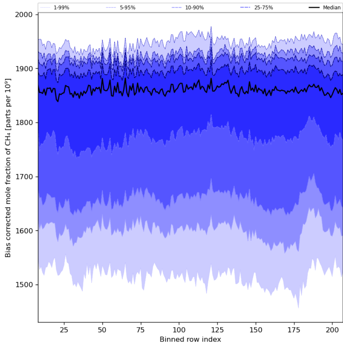
Figure 36: Along track statistics of “Bias corrected mole fraction of CH 4 ” for 2023-08-26 to 2023-08-28
