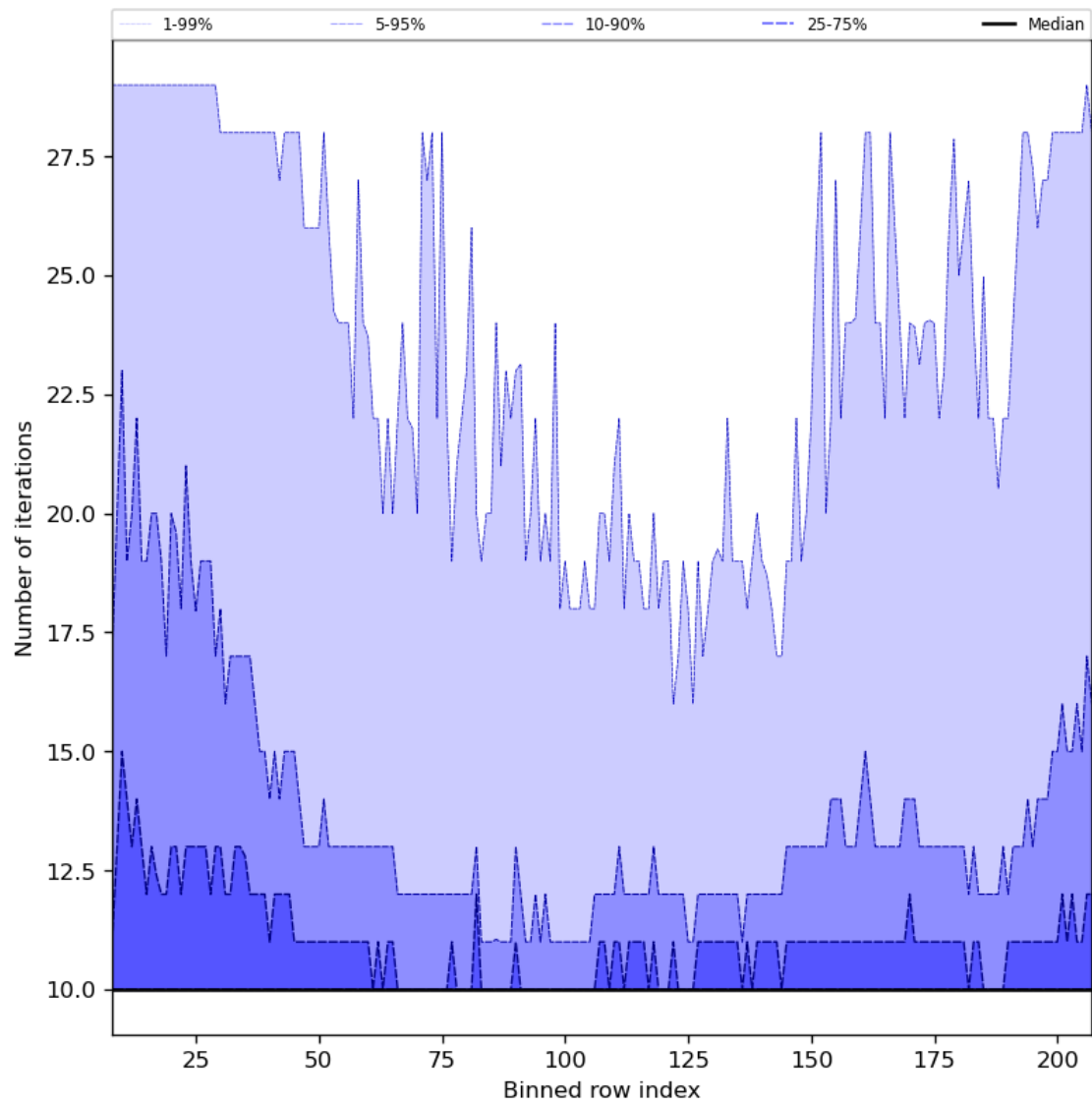
Figure 42: Along track statistics of “Number of iterations” for 2023-08-26 to 2023-08-28
