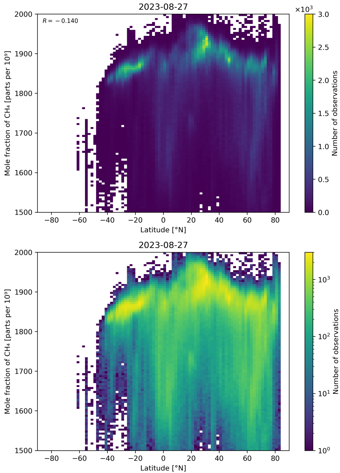
Figure 57: Scatter density plot of “Latitude” against “Mole fraction of CH 4 ” for 2023-08-26 to 2023-08-28.
