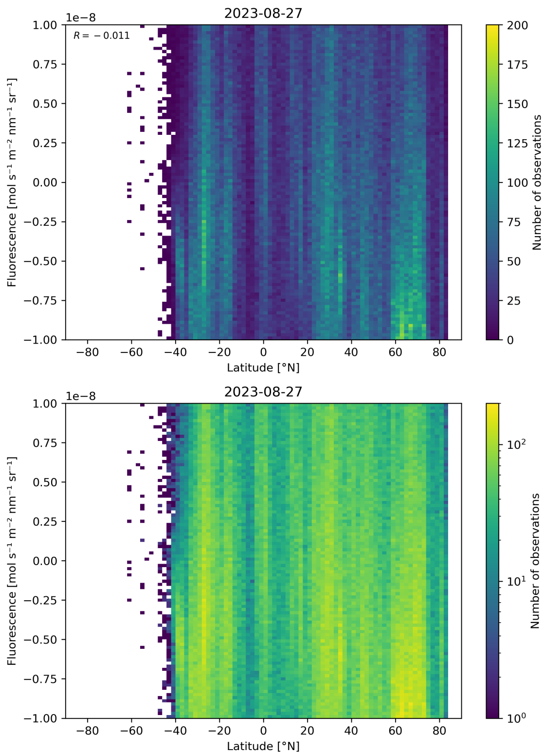
Figure 56: Scatter density plot of “Latitude” against “Fluorescence” for 2023-08-26 to 2023-08-28.
