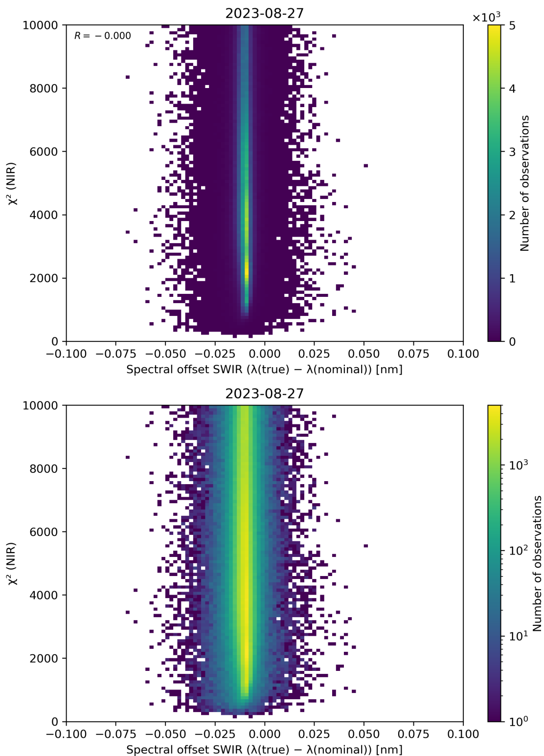
Figure 117: Scatter density plot of “Spectral offset SWIR ( \lambda(\text{true}) - \lambda(\text{nominal}) )” against “ \chi^2 (NIR)” for 2023-08-26 to 2023-08-28.
