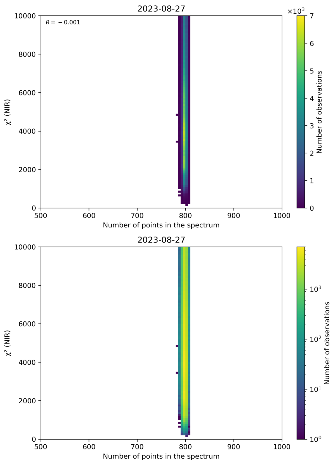
Figure 88: Scatter density plot of “Number of points in the spectrum” against “ \chi^2 (NIR)” for 2023-08-26 to 2023-08-28.
