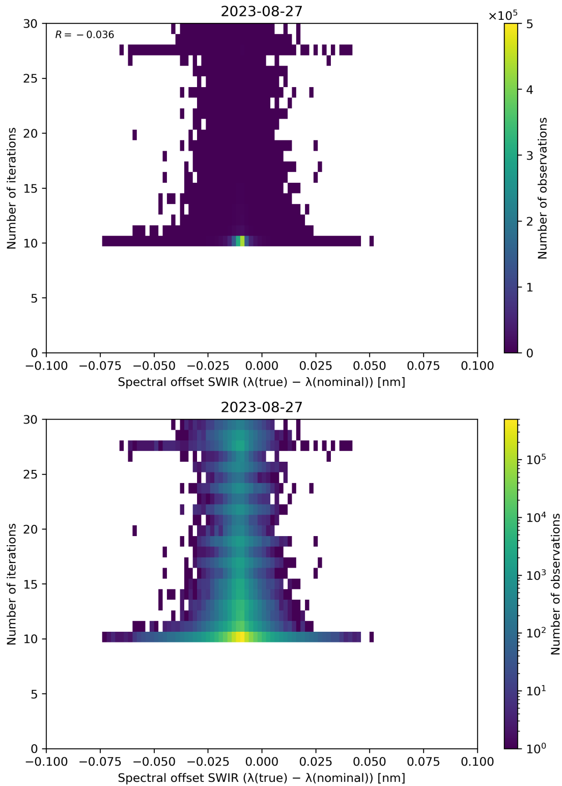
Figure 121: Scatter density plot of “Spectral offset SWIR ( \lambda(\text{true}) - \lambda(\text{nominal}) )” against “Number of iterations” for 2023-08-26 to 2023-08-28.
