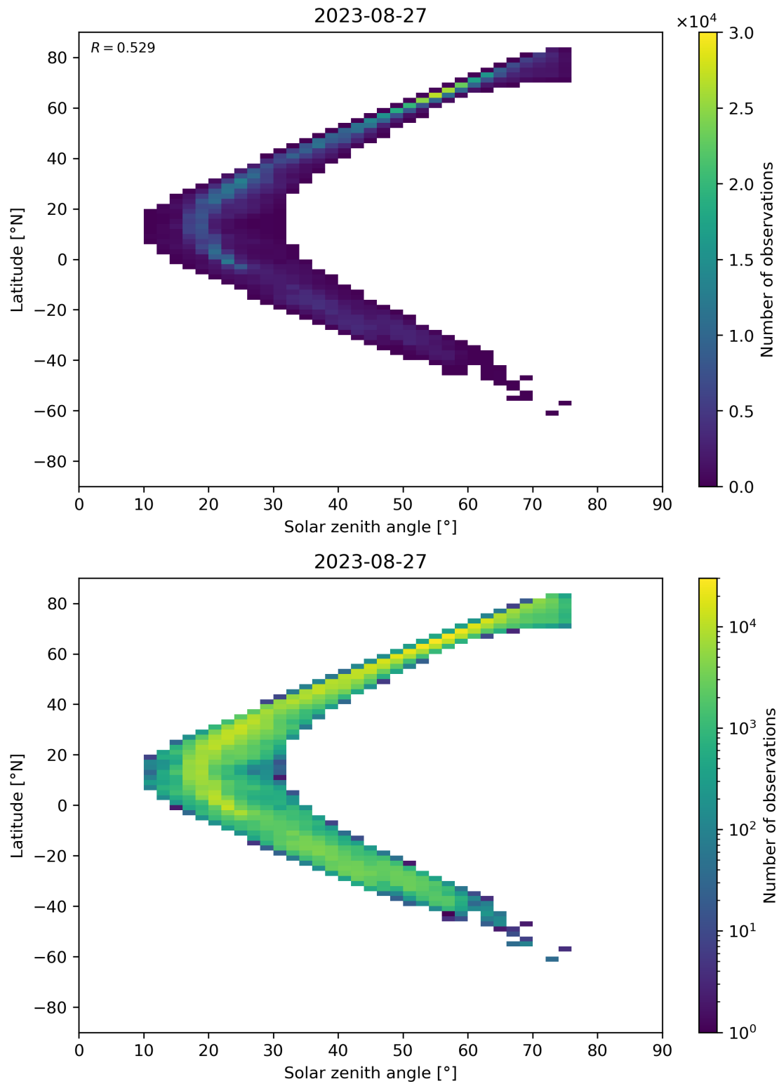
Figure 98: Scatter density plot of “Solar zenith angle” against “Latitude” for 2023-08-26 to 2023-08-28.
