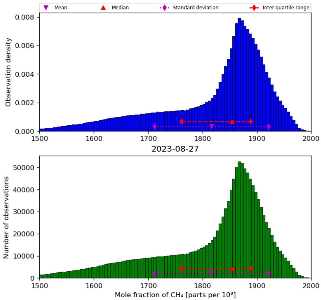
Figure 23: Histogram of “Mole fraction of CH 4 ” for 2023-08-26 to 2023-08-28
