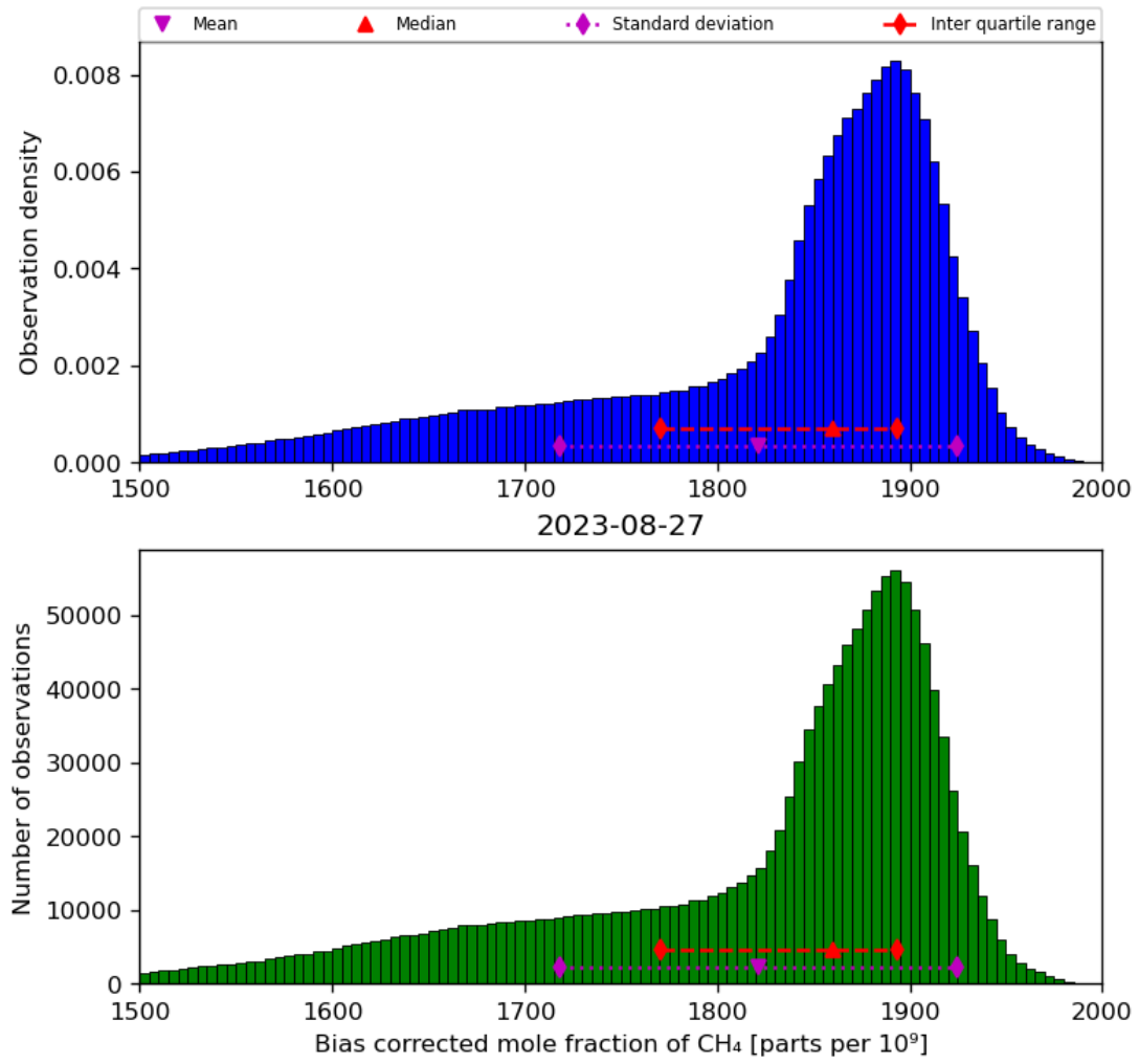
Figure 25: Histogram of “Bias corrected mole fraction of CH 4 ” for 2023-08-26 to 2023-08-28
