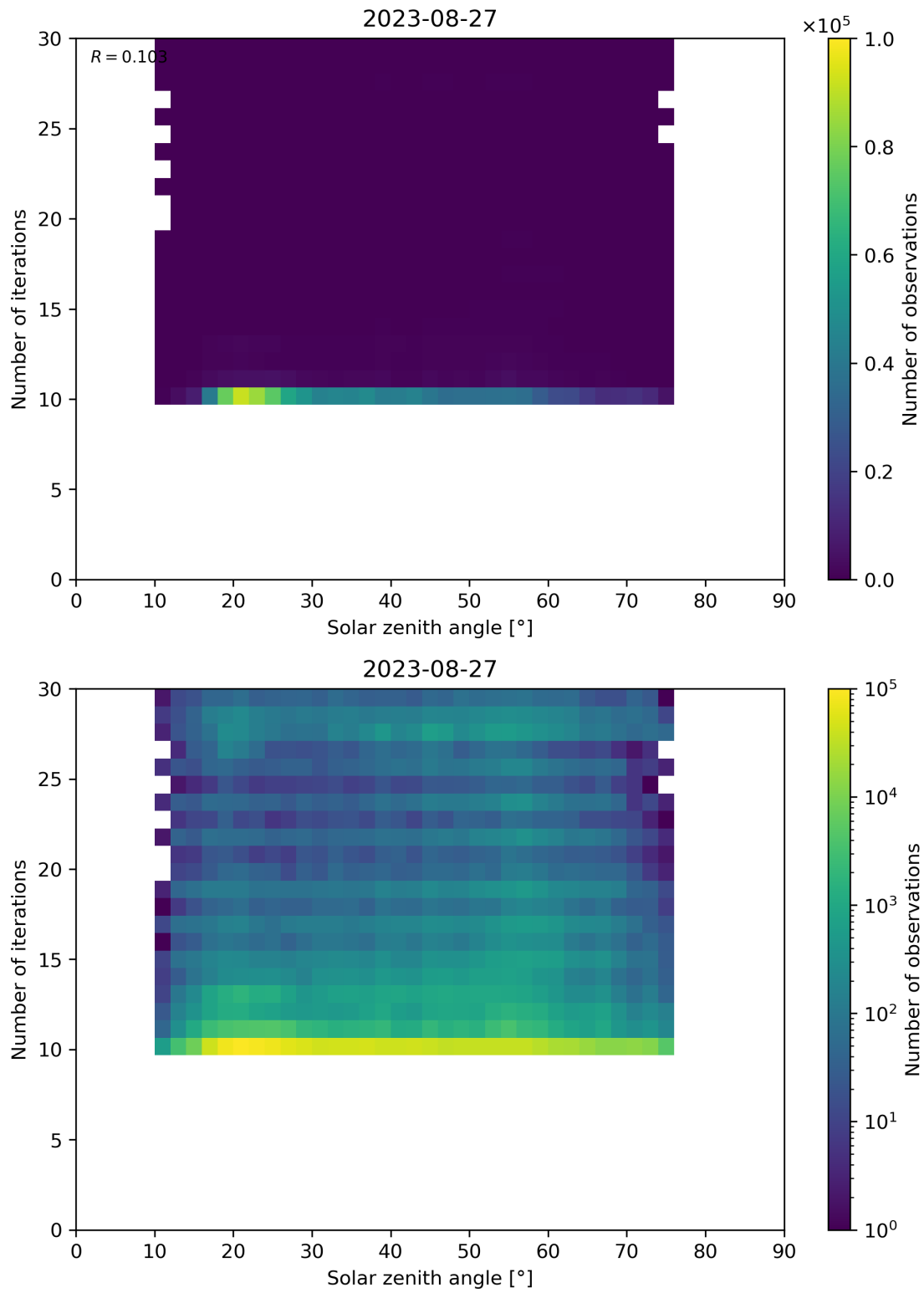
Figure 102: Scatter density plot of “Solar zenith angle” against “Number of iterations” for 2023-08-26 to 2023-08-28.
