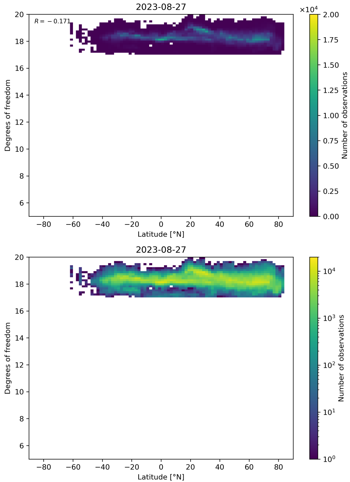
Figure 55: Scatter density plot of “Latitude” against “Degrees of freedom” for 2023-08-26 to 2023-08-28.
