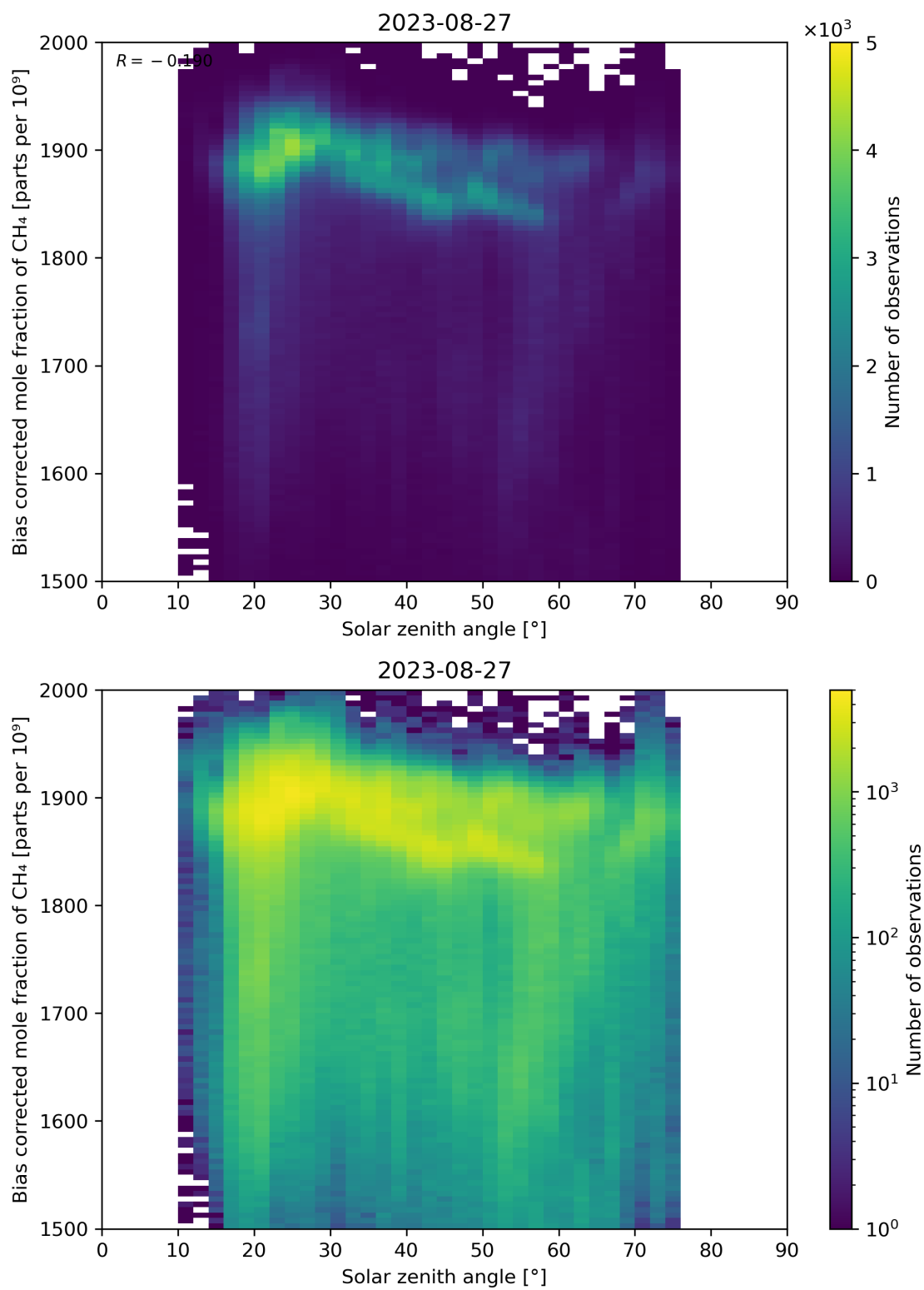
Figure 100: Scatter density plot of “Solar zenith angle” against “Bias corrected mole fraction of CH 4 ” for 2023-08-26 to 2023-08-28.
