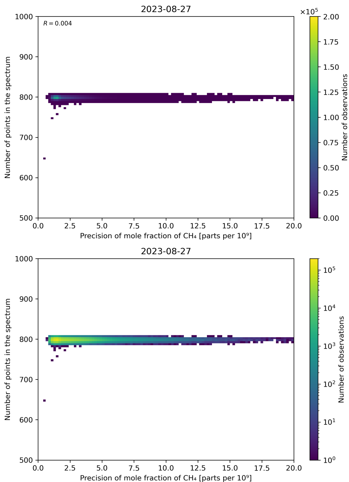
Figure 84: Scatter density plot of “Precision of mole fraction of CH 4 ” against “Number of points in the spectrum” for 2023-08-26 to 2023-08-28.
