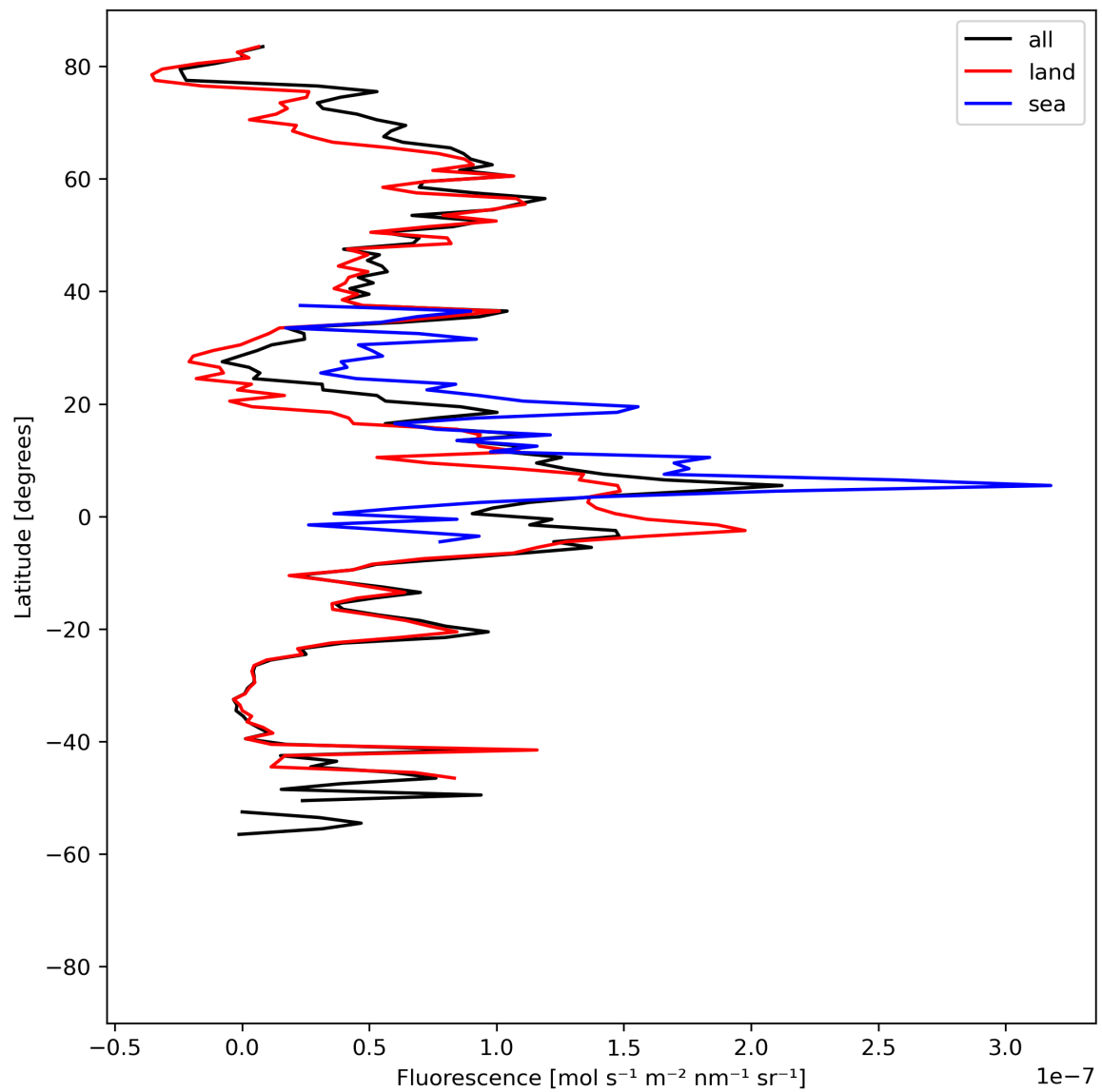
Figure 21: Zonal average of “Fluorescence” for 2023-08-26 to 2023-08-28.
