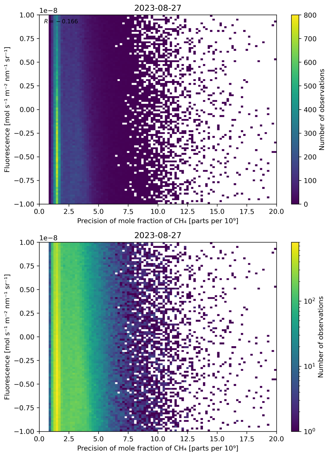
Figure 81: Scatter density plot of “Precision of mole fraction of \text{CH}_4 ” against “Fluorescence” for 2023-08-26 to 2023-08-28.
