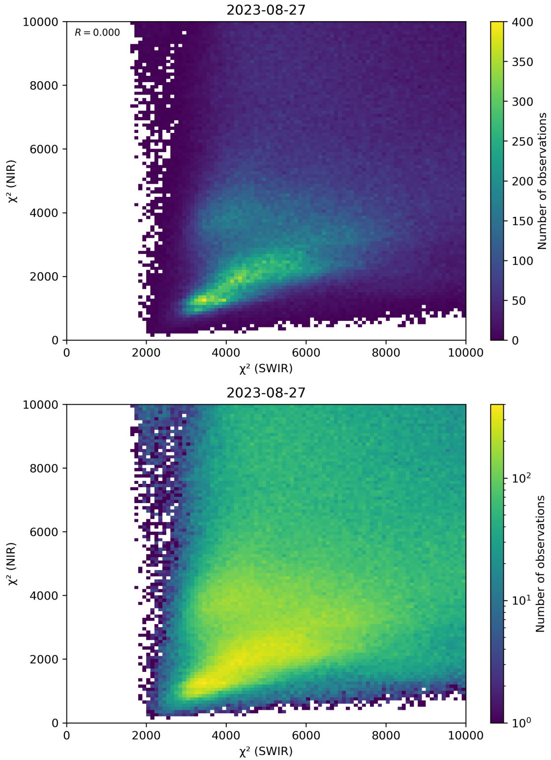
Figure 47: Scatter density plot of “ \chi^2 (SWIR)” against “ \chi^2 (NIR)” for 2023-08-26 to 2023-08-28.
