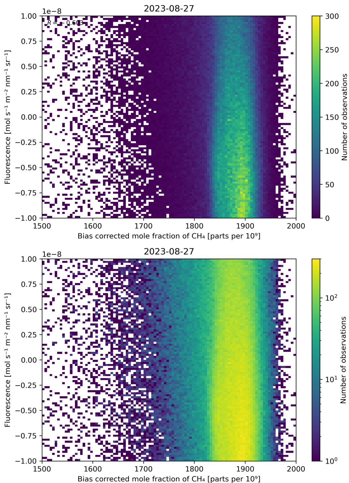
Figure 66: Scatter density plot of “Bias corrected mole fraction of \text{CH}_4 ” against “Fluorescence” for 2023-08-26 to 2023-08-28.
