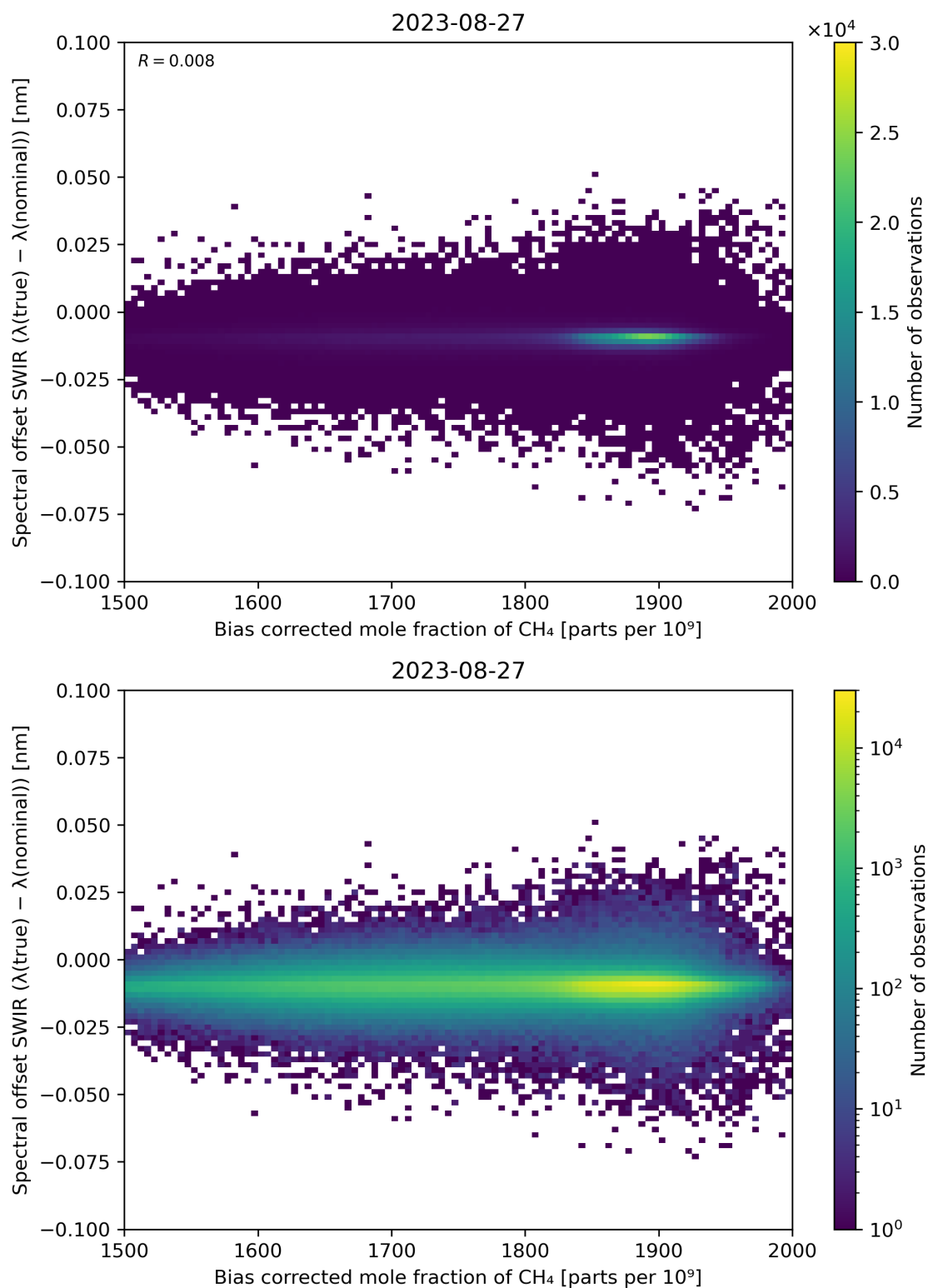
Figure 69: Scatter density plot of “Bias corrected mole fraction of \text{CH}_4 ” against “Spectral offset SWIR ( \lambda(\text{true}) - \lambda(\text{nominal}) )” for 2023-08-26 to 2023-08-28.
