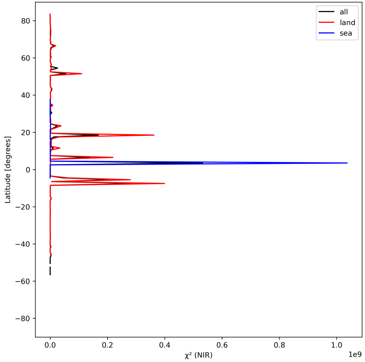
Figure 18: Zonal average of “ \chi^2 (NIR)” for 2023-08-26 to 2023-08-28.
