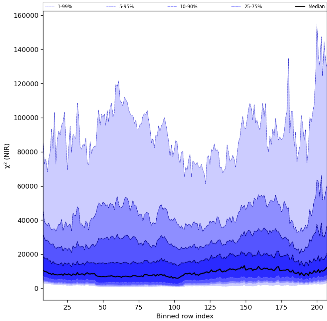
Figure 40: Along track statistics of " \chi^2 (NIR)" for 2023-08-26 to 2023-08-28
