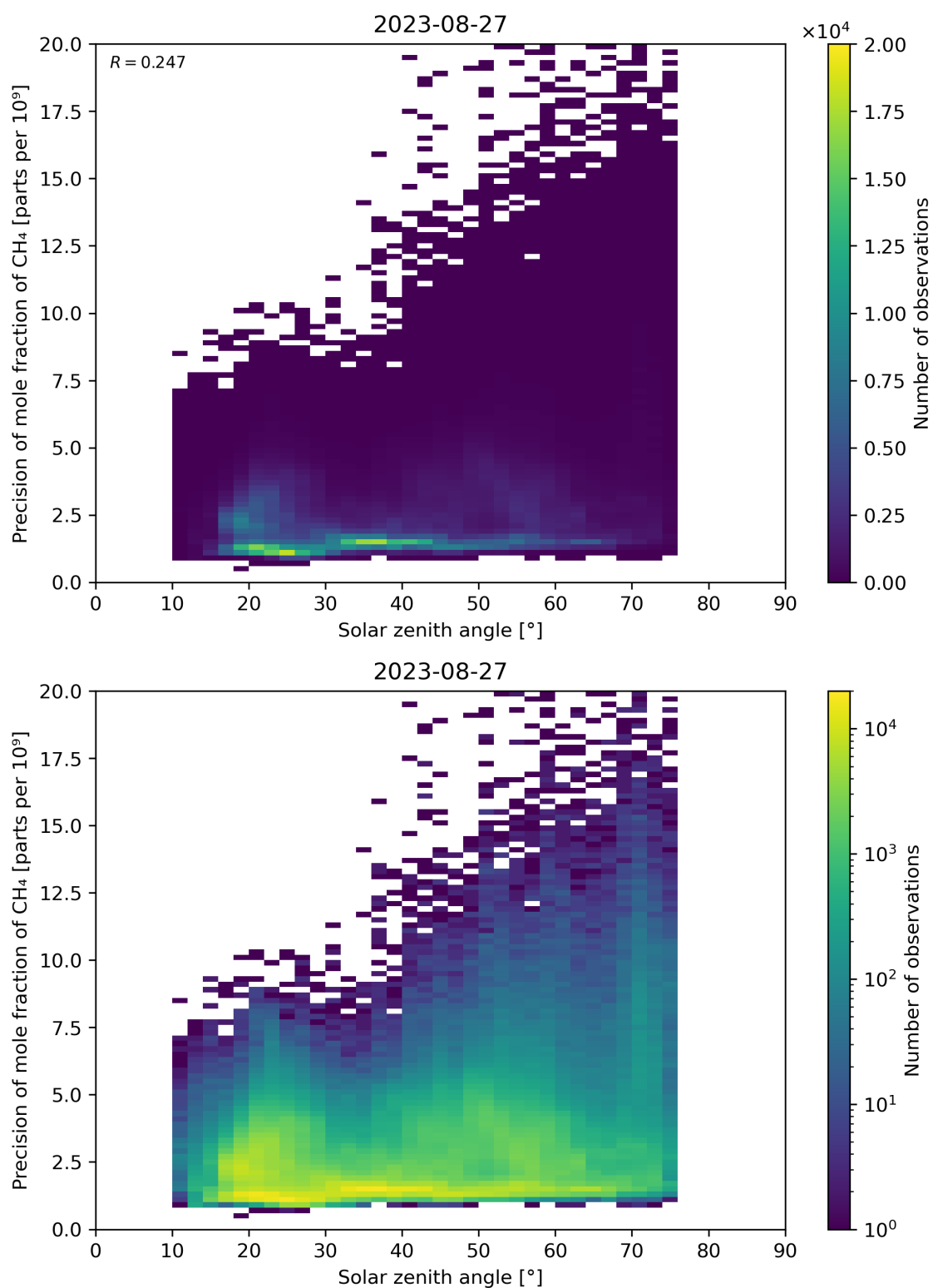
Figure 101: Scatter density plot of “Solar zenith angle” against “Precision of mole fraction of CH 4 ” for 2023-08-26 to 2023-08-28.
