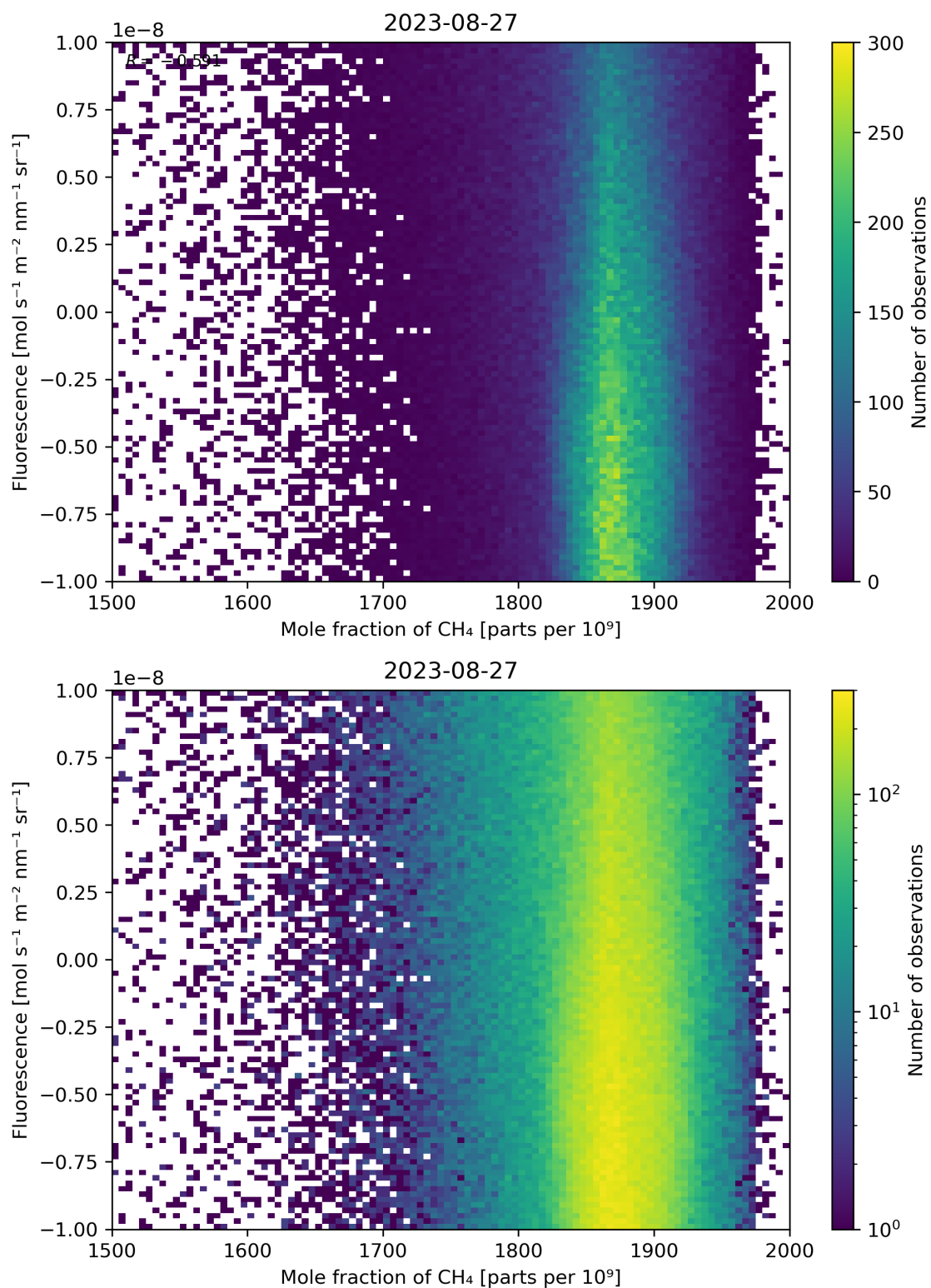
Figure 73: Scatter density plot of “Mole fraction of CH 4 ” against “Fluorescence” for 2023-08-26 to 2023-08-28.
