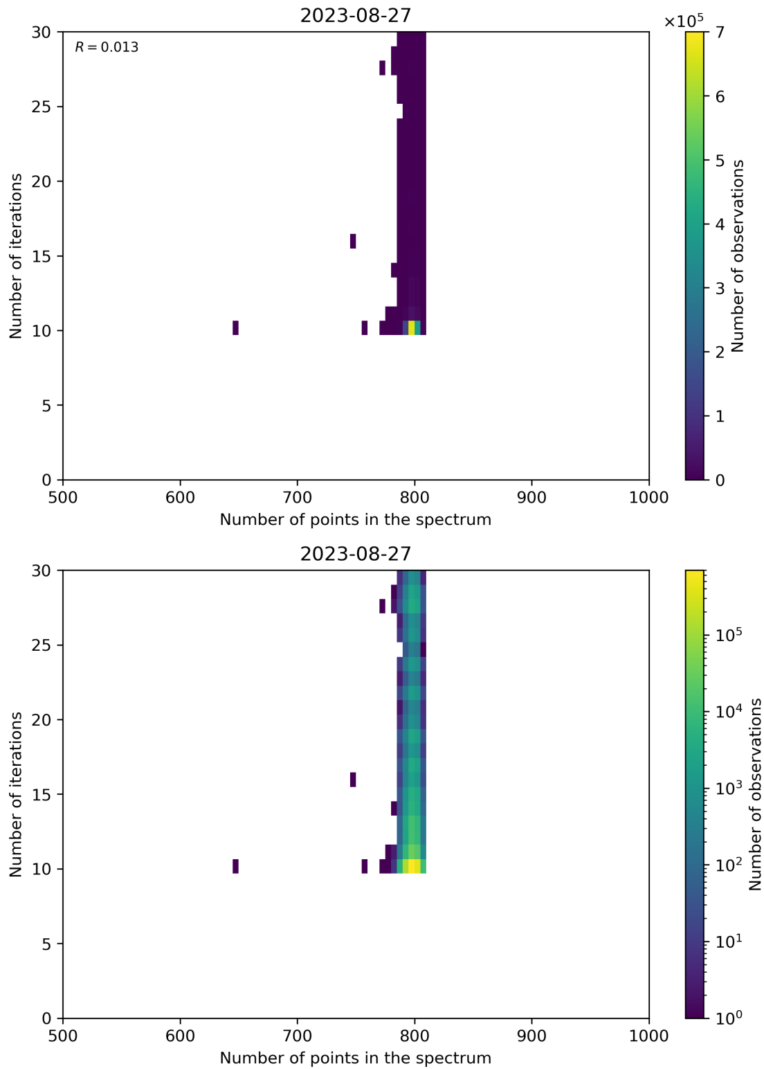
Figure 92: Scatter density plot of “Number of points in the spectrum” against “Number of iterations” for 2023-08-26 to 2023-08-28.
