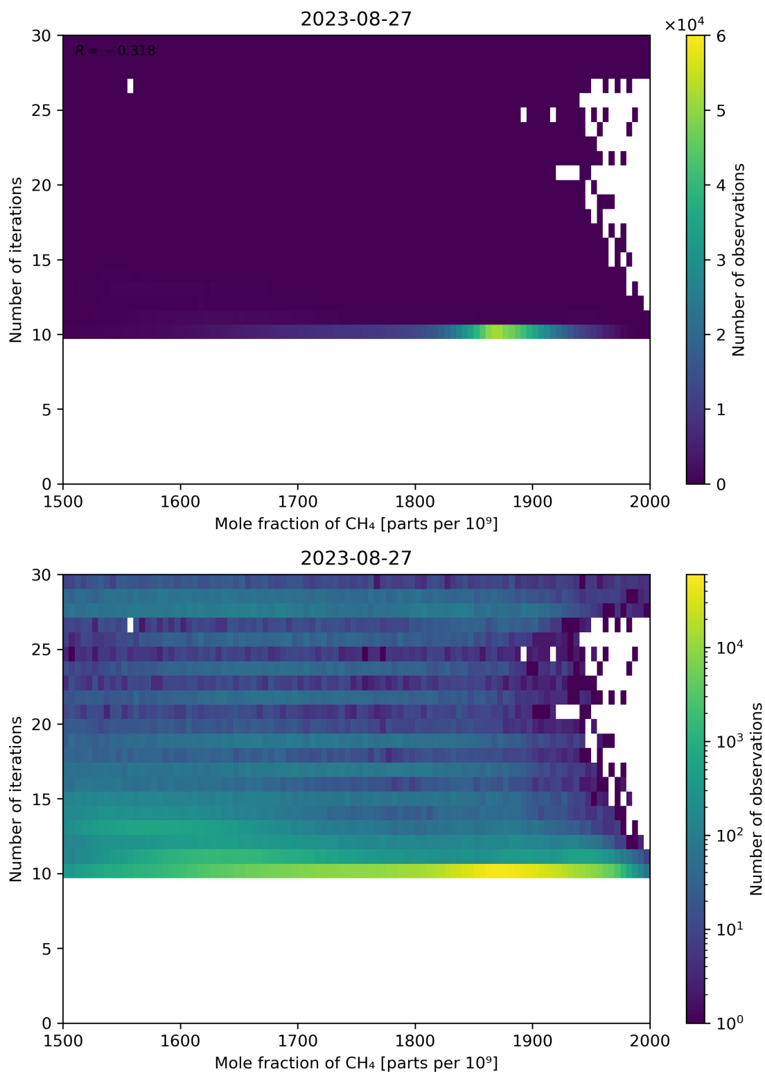
Figure 76: Scatter density plot of “Mole fraction of CH 4 ” against “Number of iterations” for 2023-08-26 to 2023-08-28.
