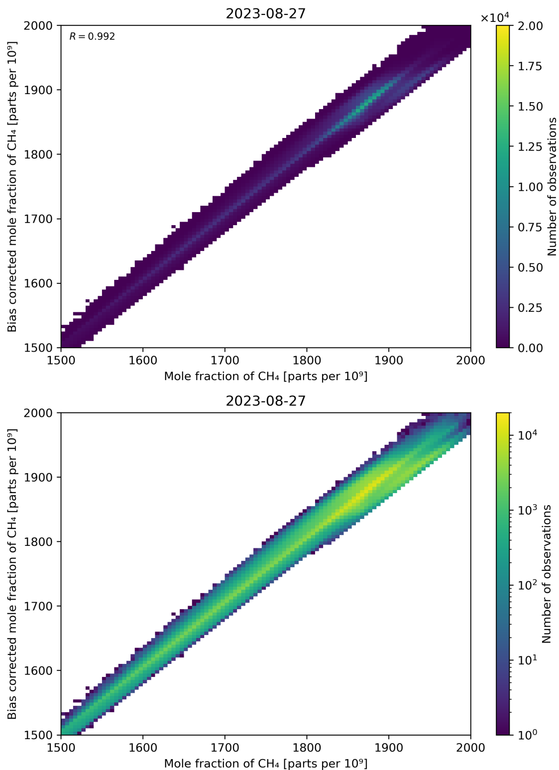
Figure 74: Scatter density plot of “Mole fraction of CH 4 ” against “Bias corrected mole fraction of CH 4 ” for 2023-08-26 to 2023-08-28.
