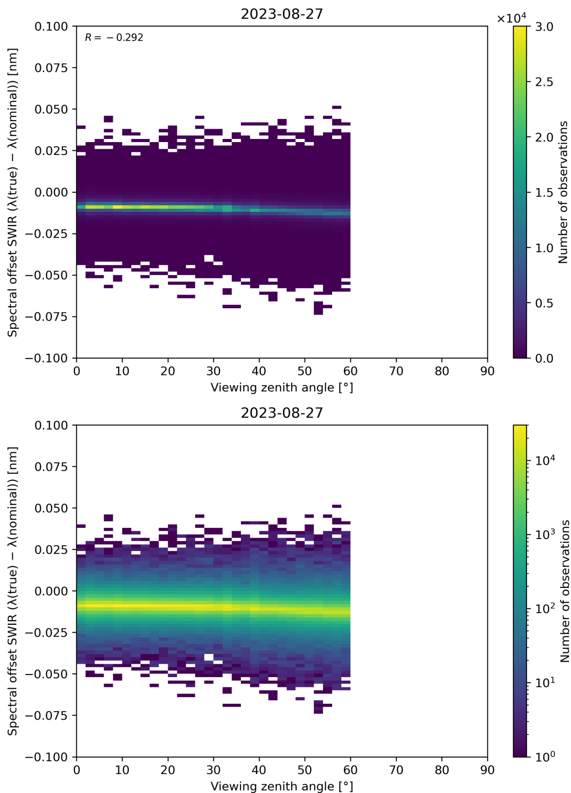
Figure 116: Scatter density plot of “Viewing zenith angle” against “Spectral offset SWIR ( \lambda(\text{true}) - \lambda(\text{nominal}) )” for 2023-08-26 to 2023-08-28.
