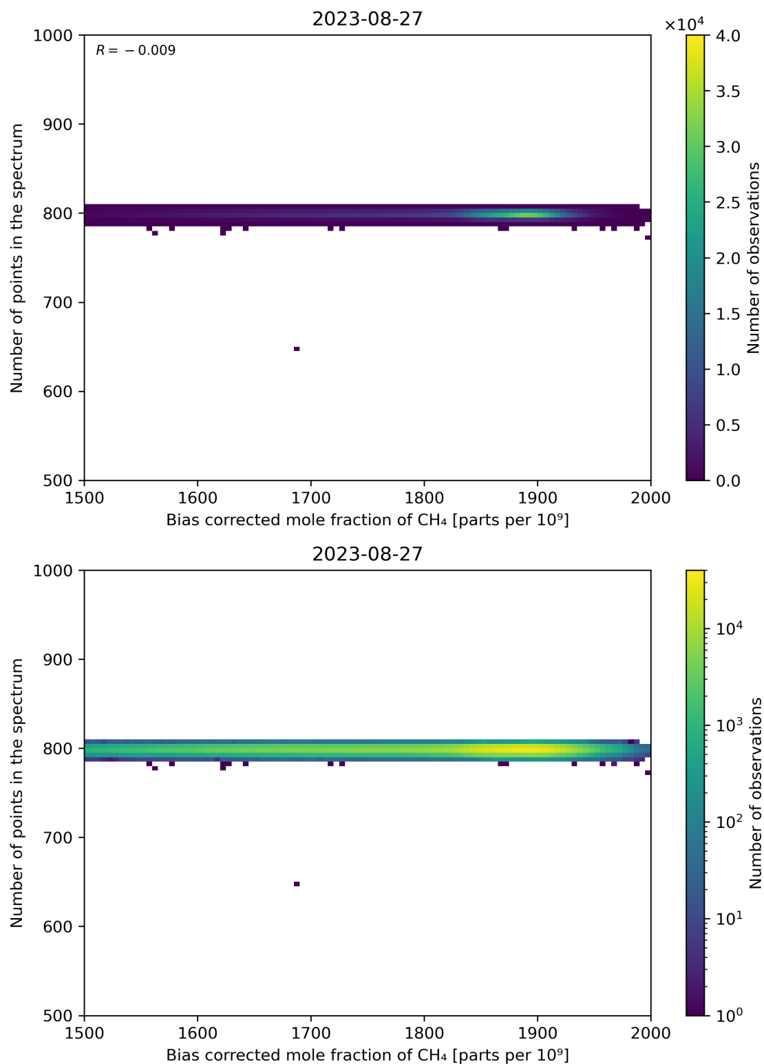
Figure 68: Scatter density plot of “Bias corrected mole fraction of CH 4 ” against “Number of points in the spectrum” for 2023-08-26 to 2023-08-28.
