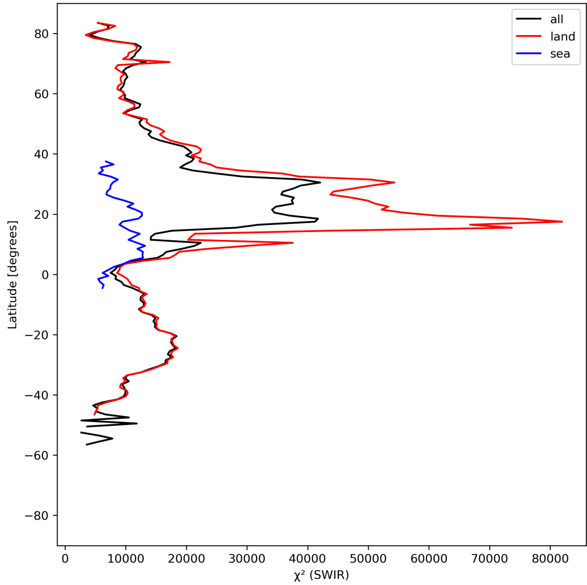
Figure 17: Zonal average of “ \chi^2 (SWIR)” for 2023-08-26 to 2023-08-28.
