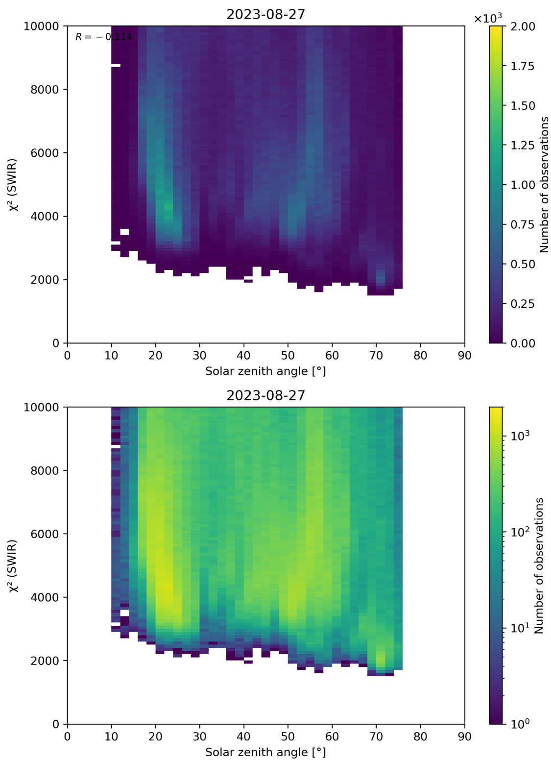
Figure 95: Scatter density plot of “Solar zenith angle” against “ \chi^2 (SWIR)” for 2023-08-26 to 2023-08-28.
