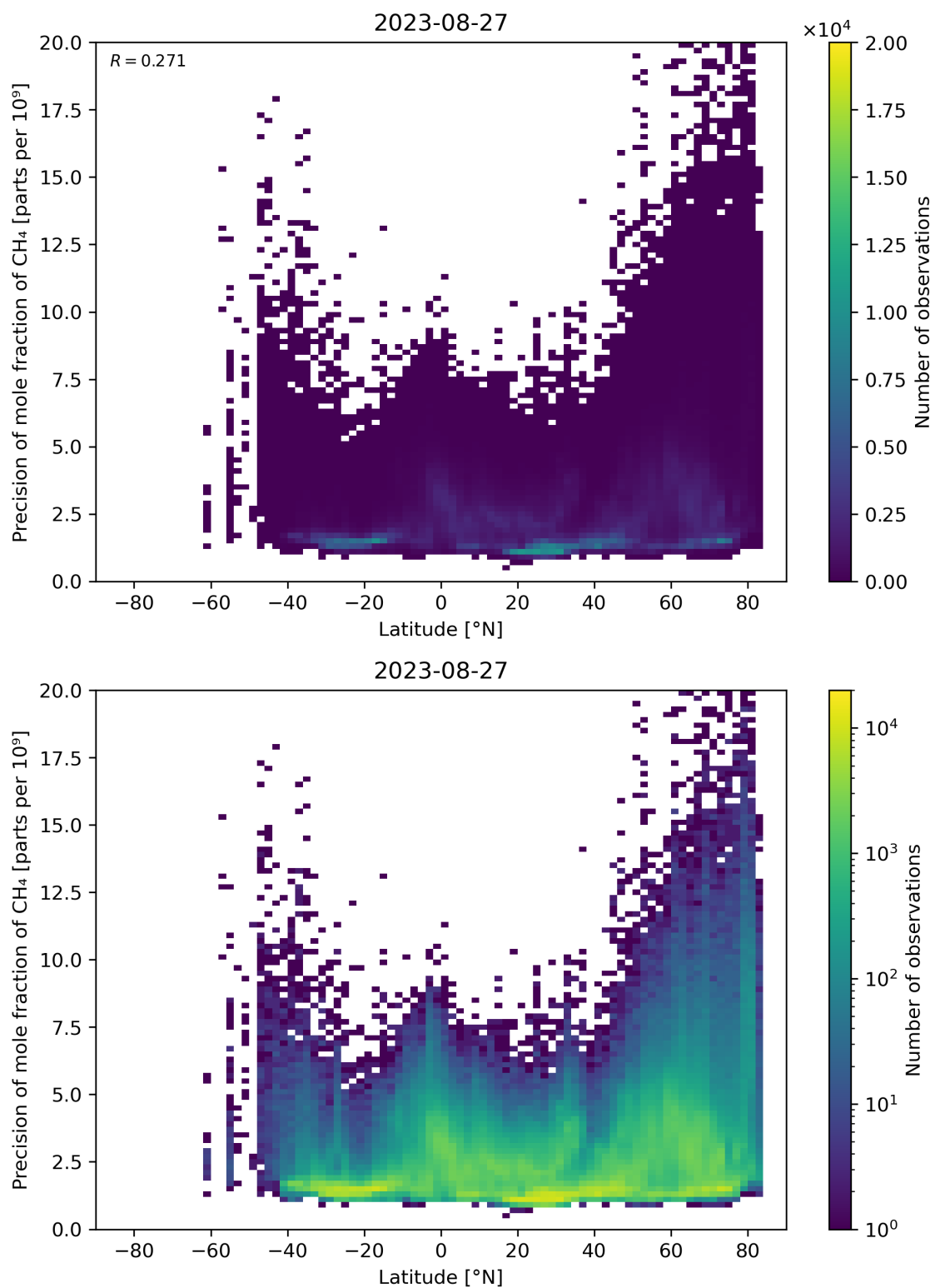
Figure 59: Scatter density plot of “Latitude” against “Precision of mole fraction of \text{CH}_4 ” for 2023-08-26 to 2023-08-28.
