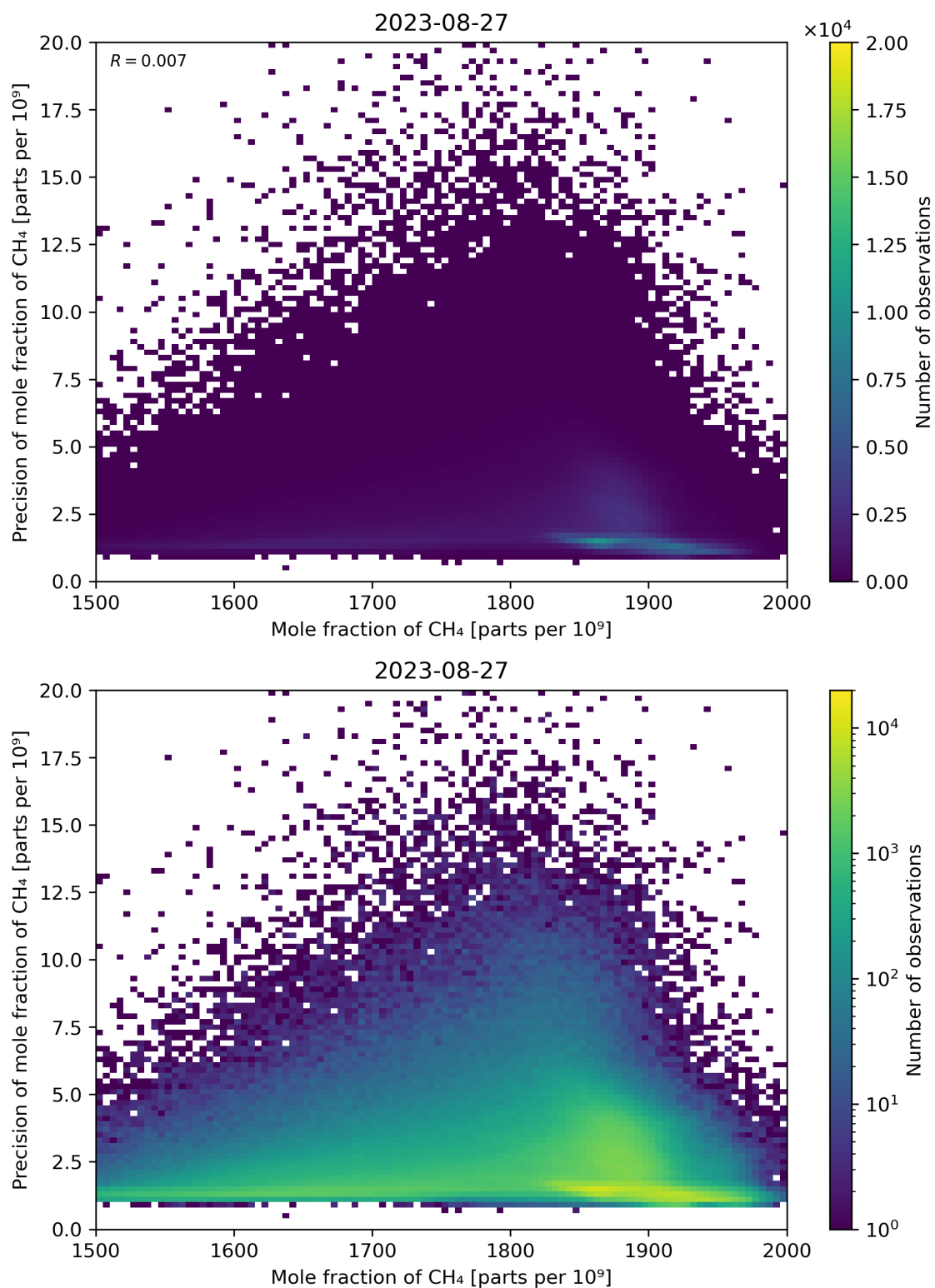
Figure 75: Scatter density plot of “Mole fraction of CH 4 ” against “Precision of mole fraction of CH 4 ” for 2023-08-26 to 2023-08-28.
