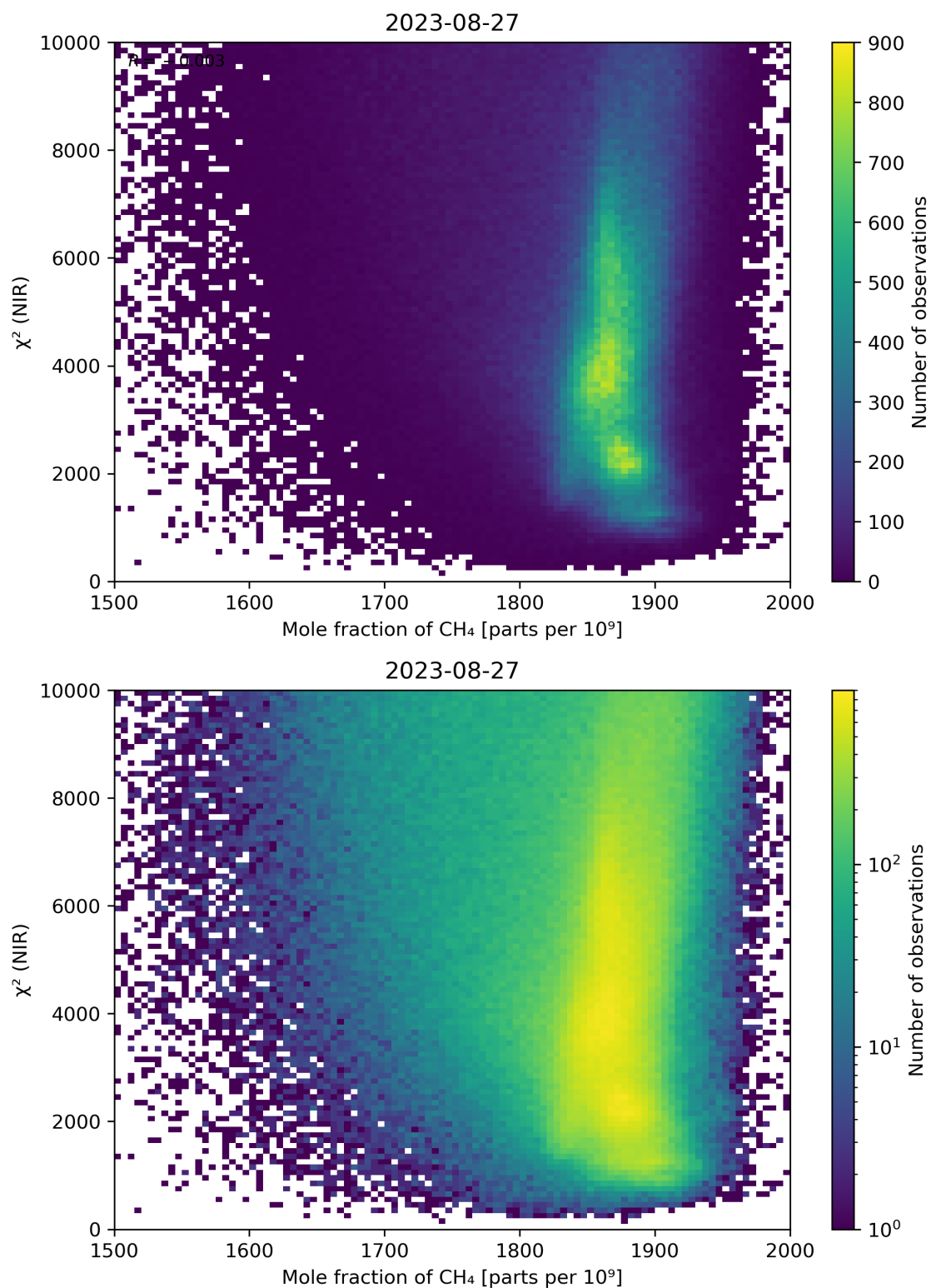
Figure 70: Scatter density plot of “Mole fraction of \text{CH}_4 ” against “ \chi^2 (NIR)” for 2023-08-26 to 2023-08-28.
