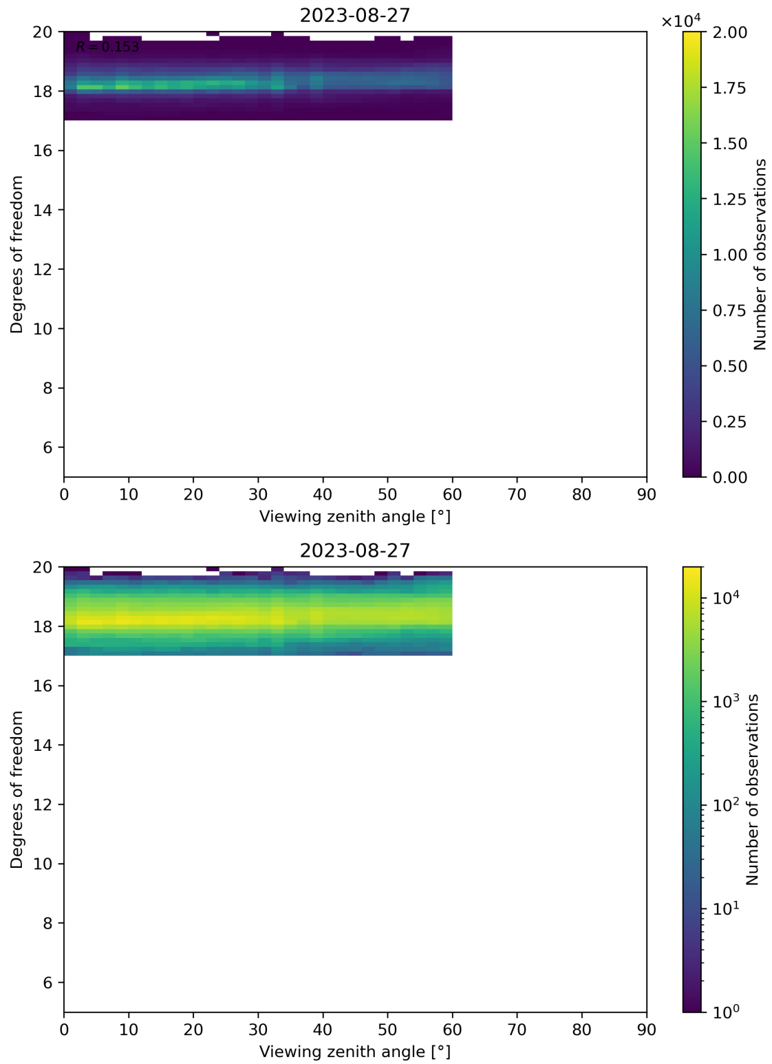
Figure 107: Scatter density plot of “Viewing zenith angle” against “Degrees of freedom” for 2023-08-26 to 2023-08-28.
