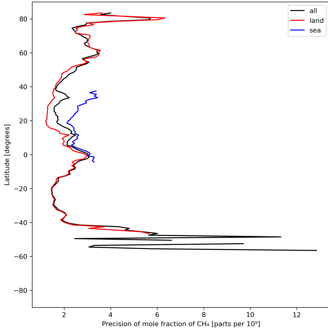
Figure 13: Zonal average of “Precision of mole fraction of CH 4 ” for 2023-08-26 to 2023-08-28.
