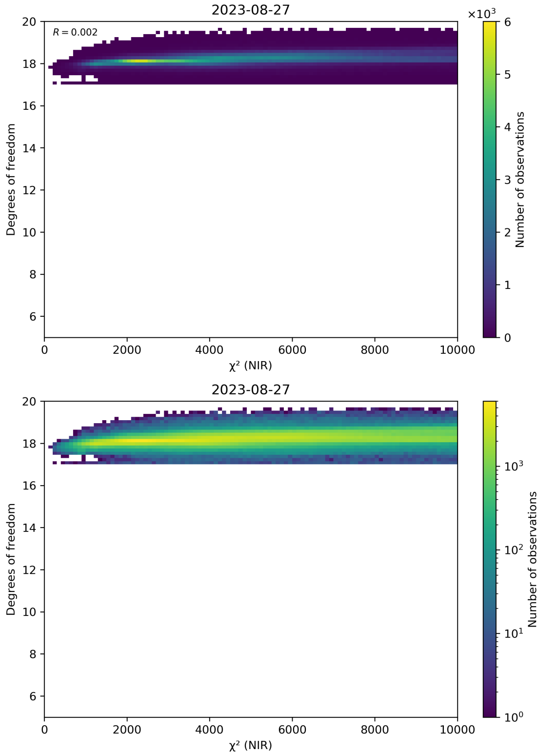
Figure 44: Scatter density plot of “ \chi^2 (NIR)” against “Degrees of freedom” for 2023-08-26 to 2023-08-28.
