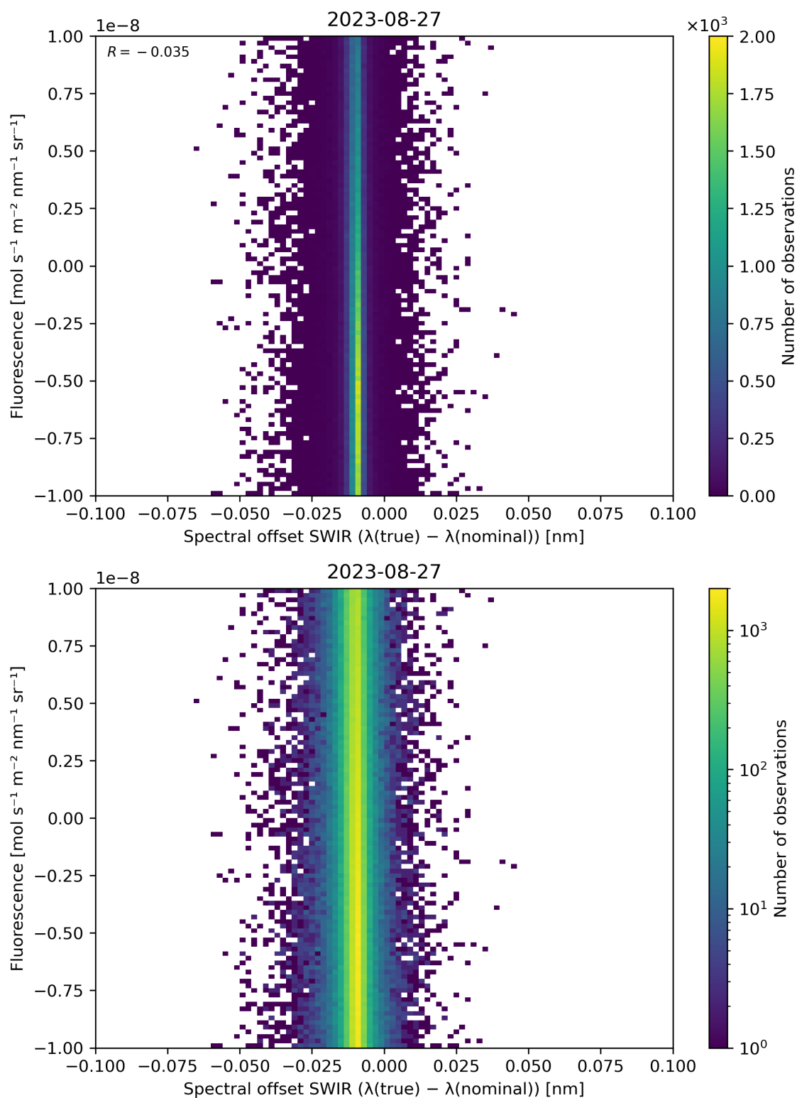
Figure 120: Scatter density plot of “Spectral offset SWIR ( \lambda(\text{true}) - \lambda(\text{nominal}) )” against “Fluorescence” for 2023-08-26 to 2023-08-28.
