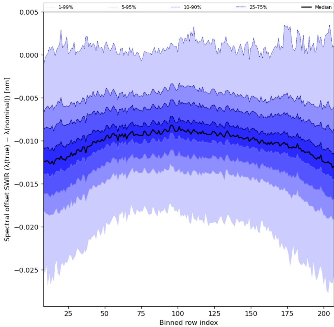
Figure 38: Along track statistics of “Spectral offset SWIR ( \lambda(\text{true}) - \lambda(\text{nominal}) )” for 2023-08-26 to 2023-08-28
