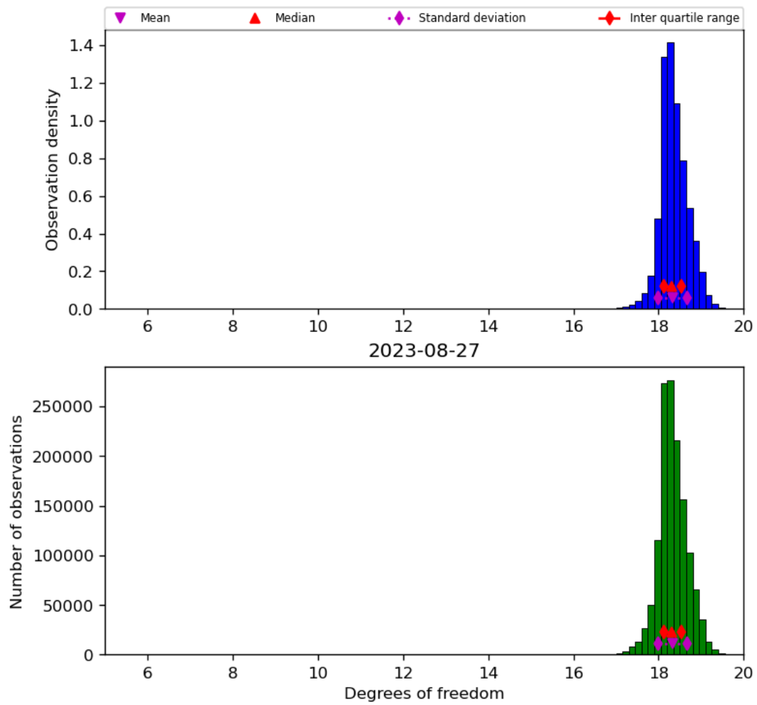
Figure 30: Histogram of “Degrees of freedom” for 2023-08-26 to 2023-08-28
