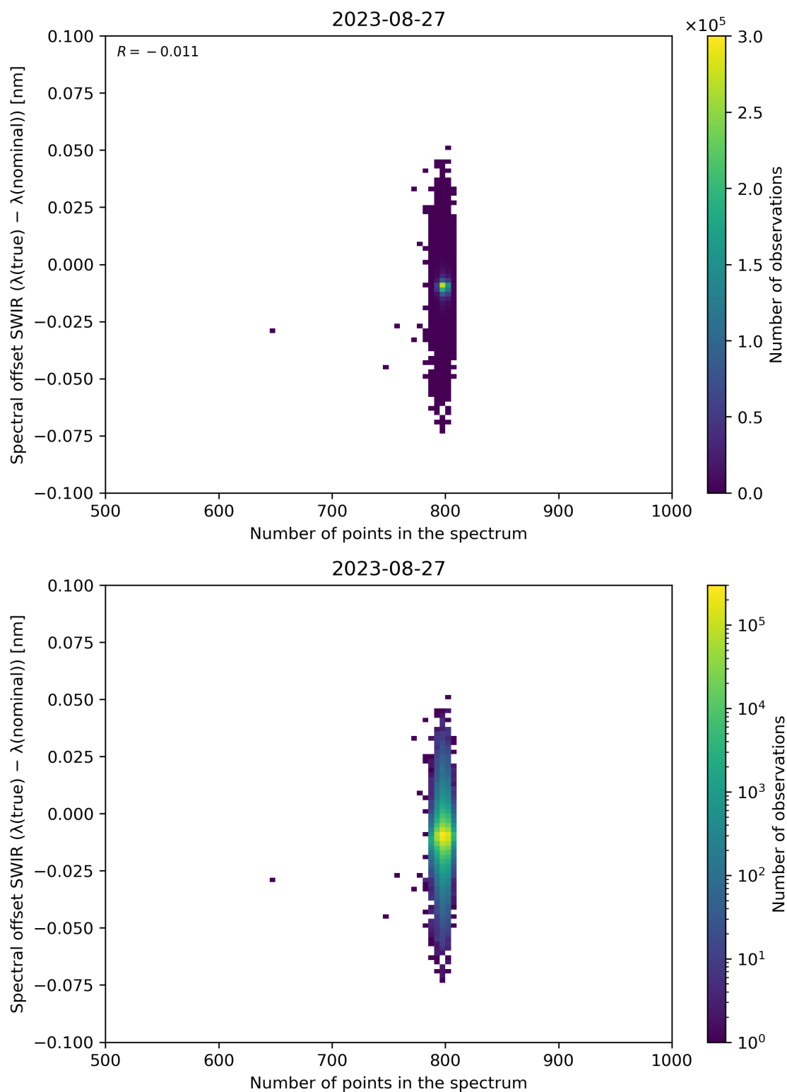
Figure 93: Scatter density plot of “Number of points in the spectrum” against “Spectral offset SWIR ( \lambda(\text{true}) - \lambda(\text{nominal}) )” for 2023-08-26 to 2023-08-28.
