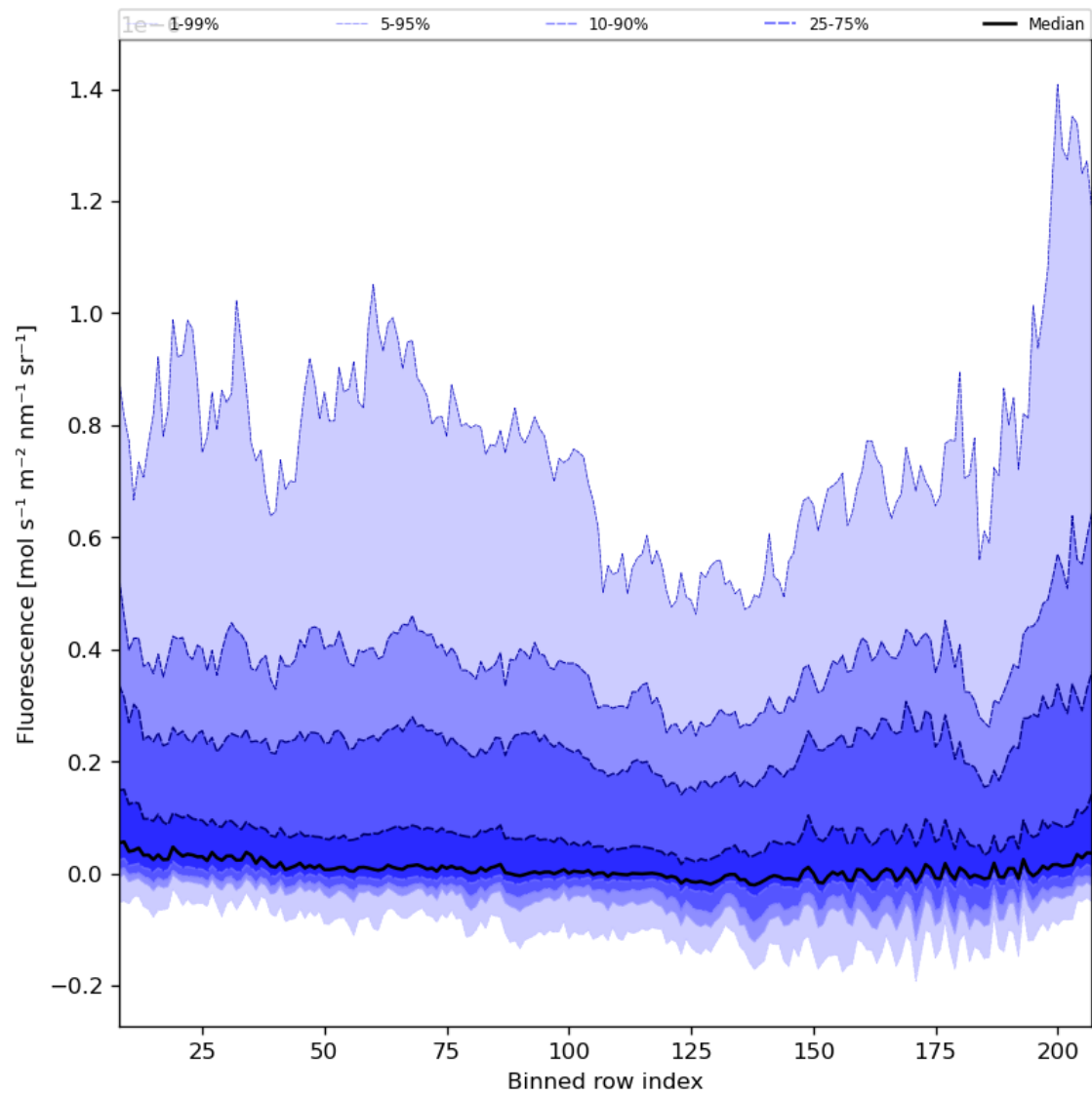
Figure 43: Along track statistics of “Fluorescence” for 2023-08-26 to 2023-08-28
