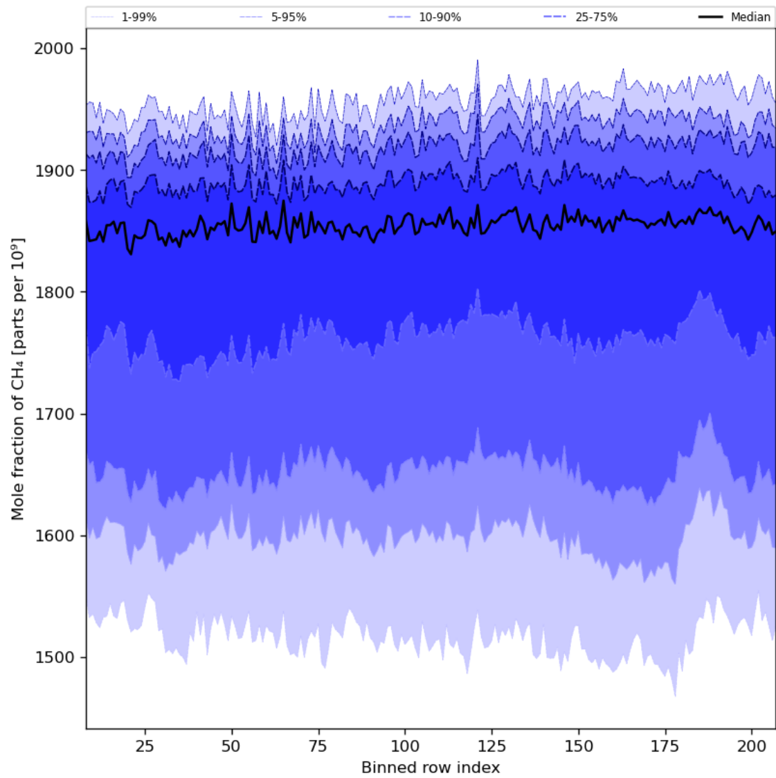
Figure 34: Along track statistics of “Mole fraction of CH 4 ” for 2023-08-26 to 2023-08-28
