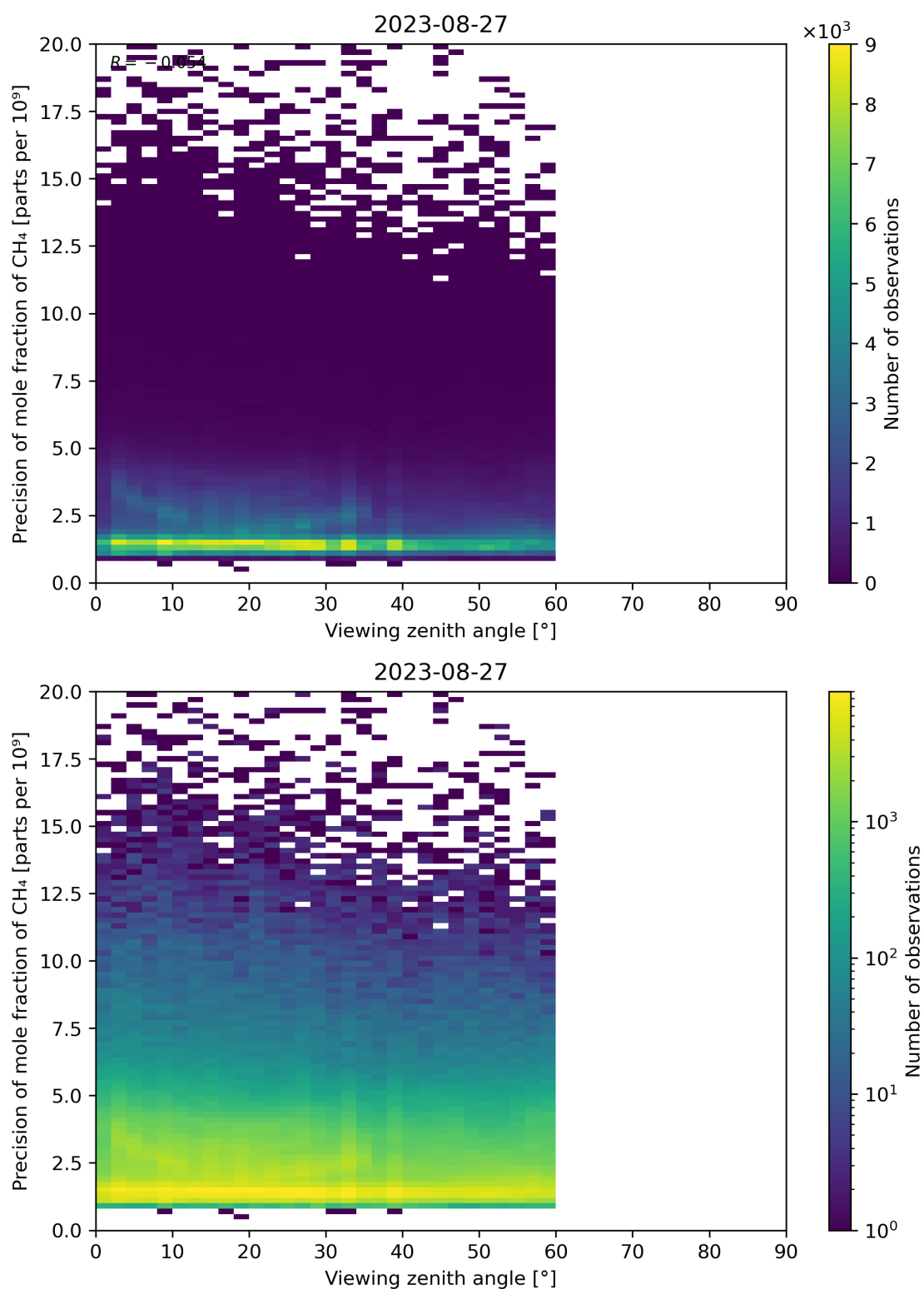
Figure 112: Scatter density plot of “Viewing zenith angle” against “Precision of mole fraction of CH 4 ” for 2023-08-26 to 2023-08-28.
