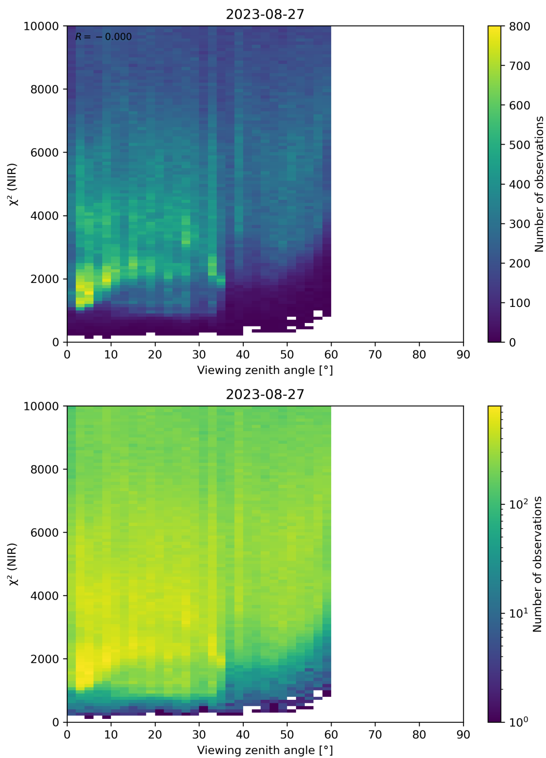
Figure 105: Scatter density plot of “Viewing zenith angle” against “ \chi^2 (NIR)” for 2023-08-26 to 2023-08-28.
