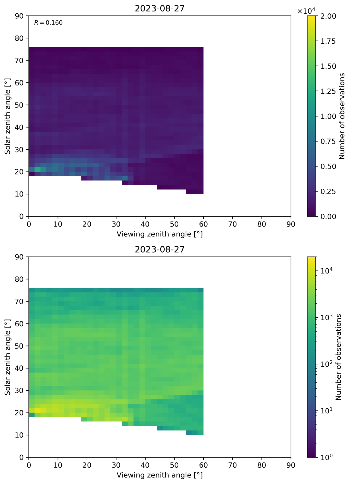
Figure 115: Scatter density plot of “Viewing zenith angle” against “Solar zenith angle” for 2023-08-26 to 2023-08-28.
