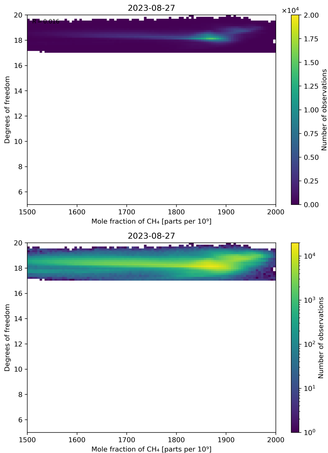
Figure 72: Scatter density plot of “Mole fraction of CH 4 ” against “Degrees of freedom” for 2023-08-26 to 2023-08-28.
