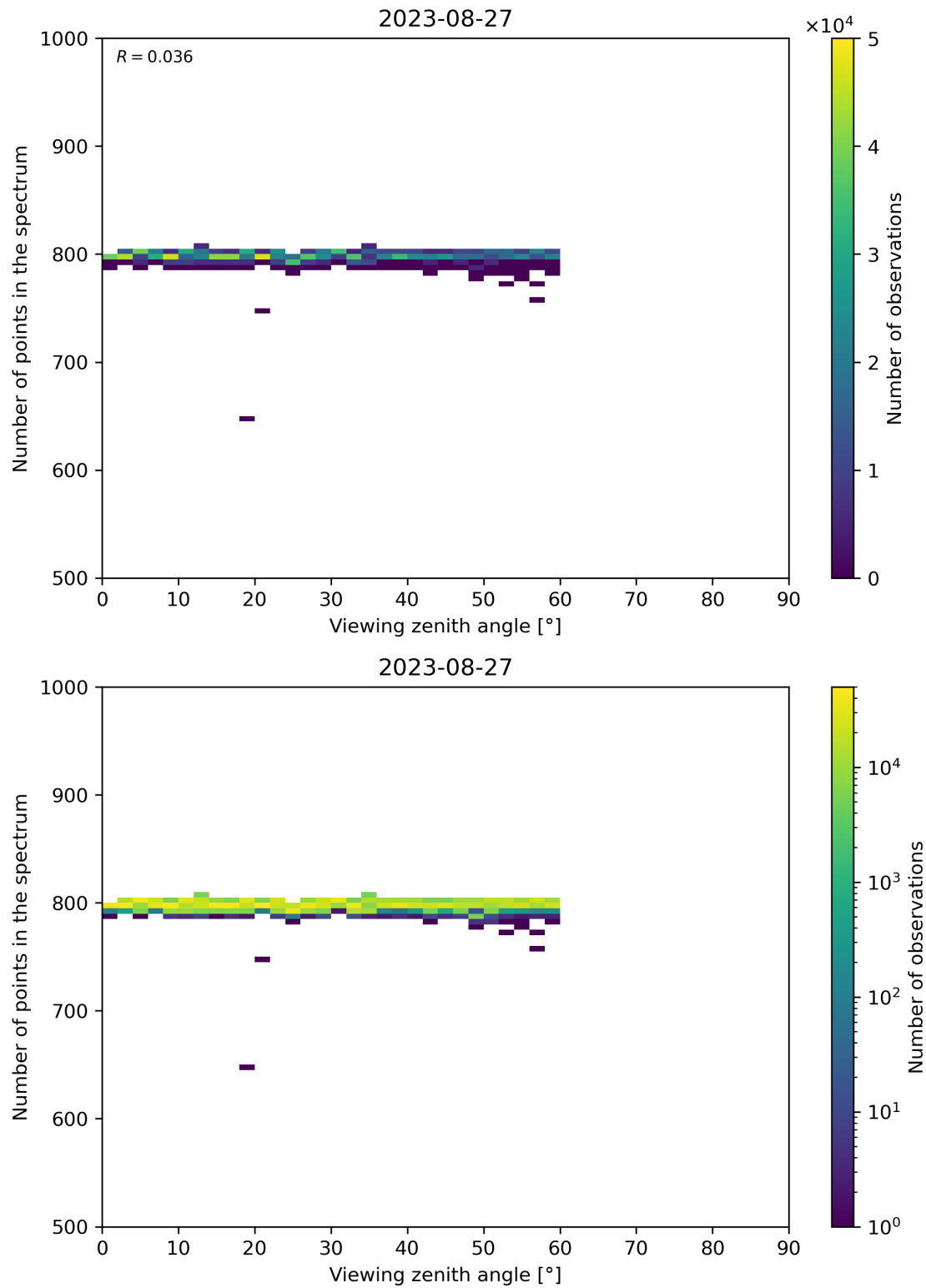
Figure 114: Scatter density plot of “Viewing zenith angle” against “Number of points in the spectrum” for 2023-08-26 to 2023-08-28.
