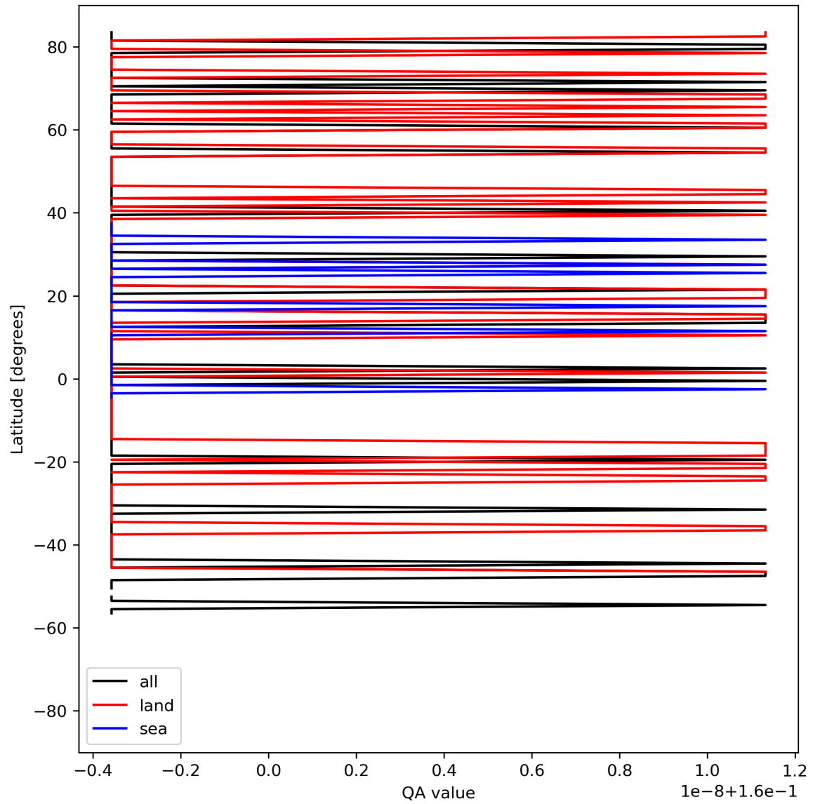
Figure 11: Zonal average of “QA value” for 2023-08-26 to 2023-08-28.
