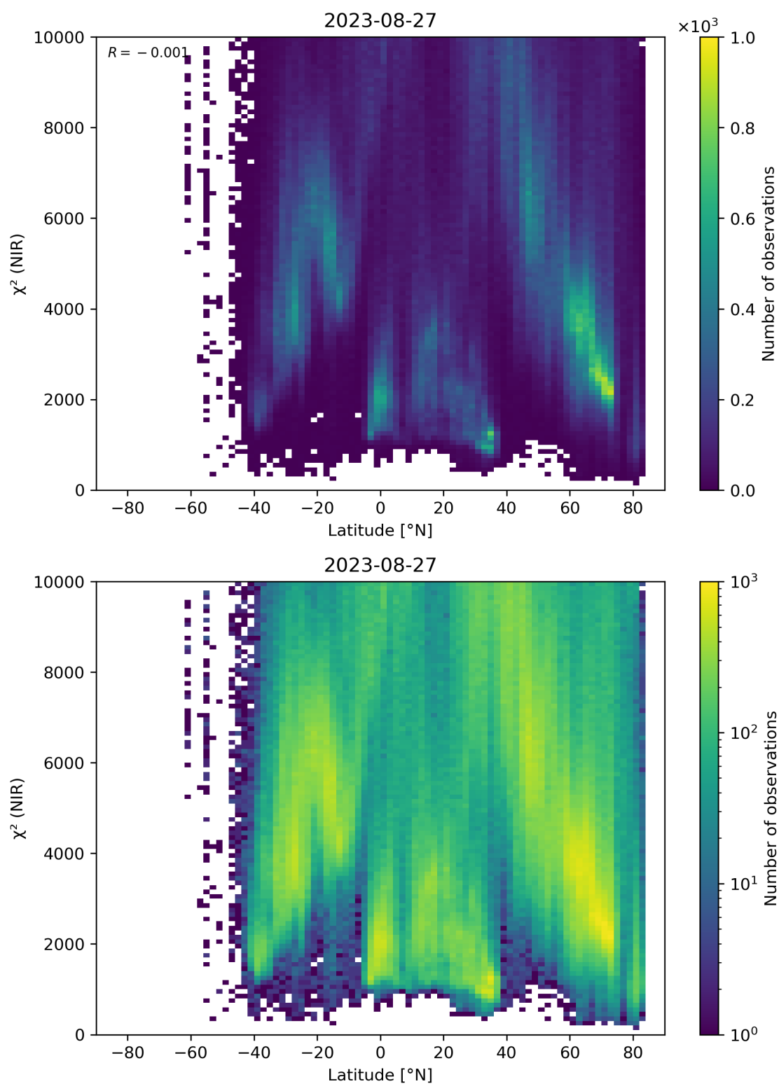
Figure 53: Scatter density plot of “Latitude” against “ \chi^2 (NIR)” for 2023-08-26 to 2023-08-28.
