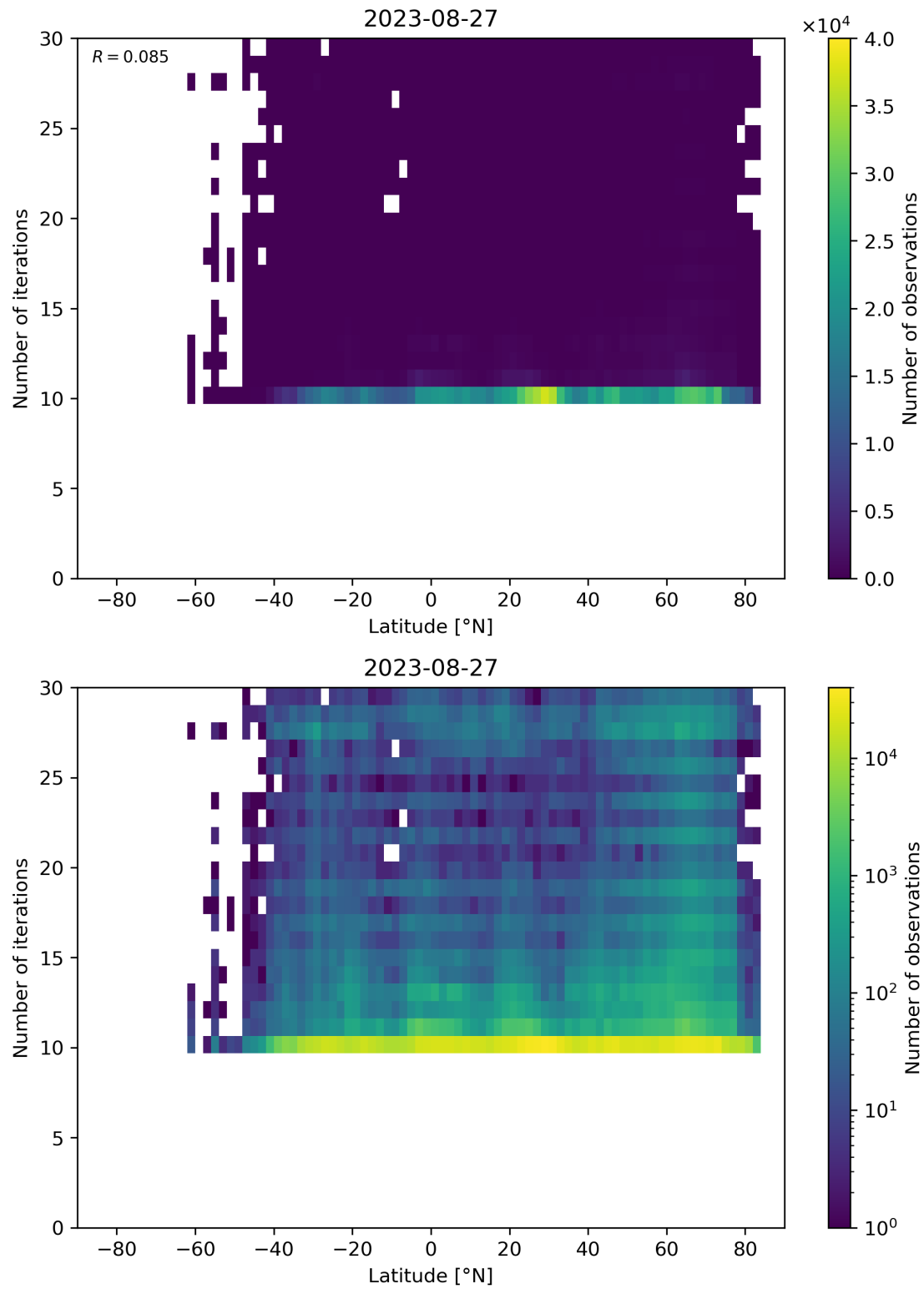
Figure 60: Scatter density plot of “Latitude” against “Number of iterations” for 2023-08-26 to 2023-08-28.
