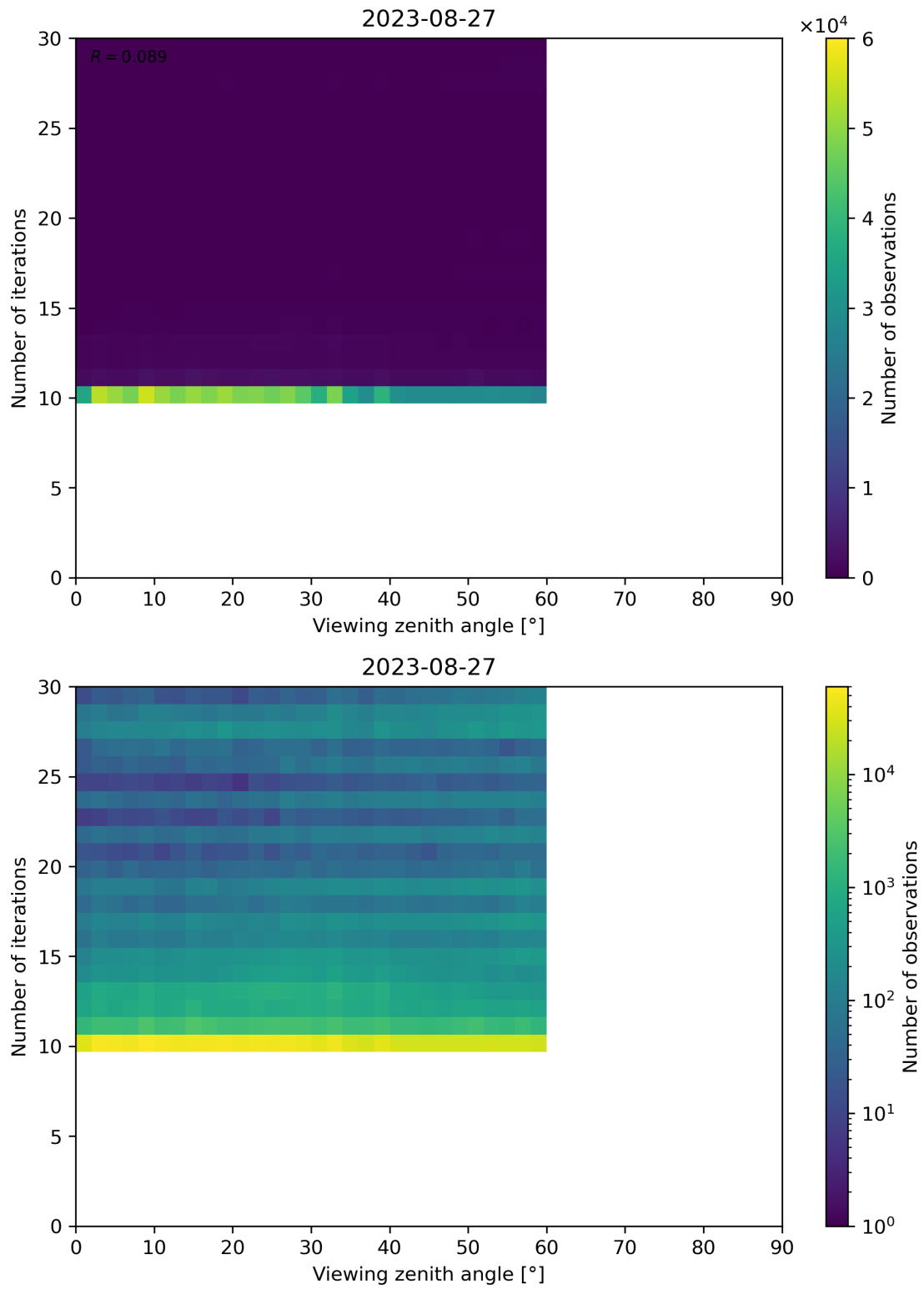
Figure 113: Scatter density plot of “Viewing zenith angle” against “Number of iterations” for 2023-08-26 to 2023-08-28.
