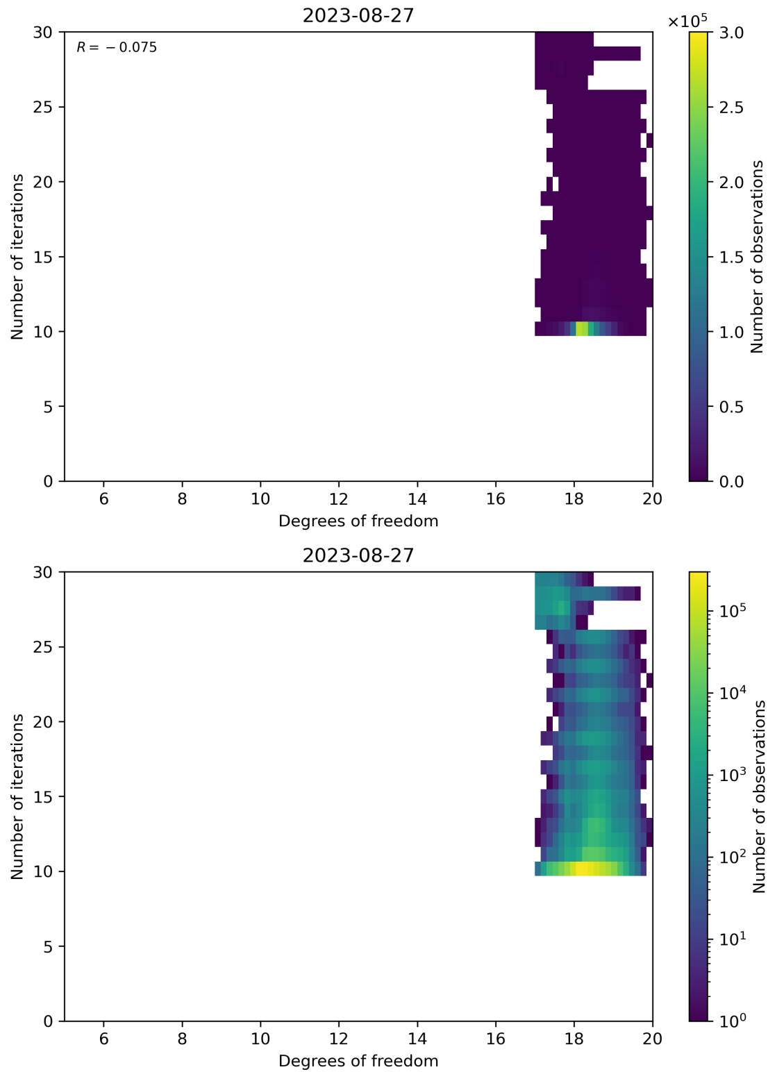
Figure 52: Scatter density plot of “Degrees of freedom” against “Number of iterations” for 2023-08-26 to 2023-08-28.
