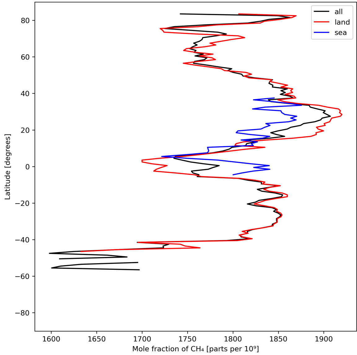
Figure 12: Zonal average of “Mole fraction of \text{CH}_4 ” for 2023-08-26 to 2023-08-28.
