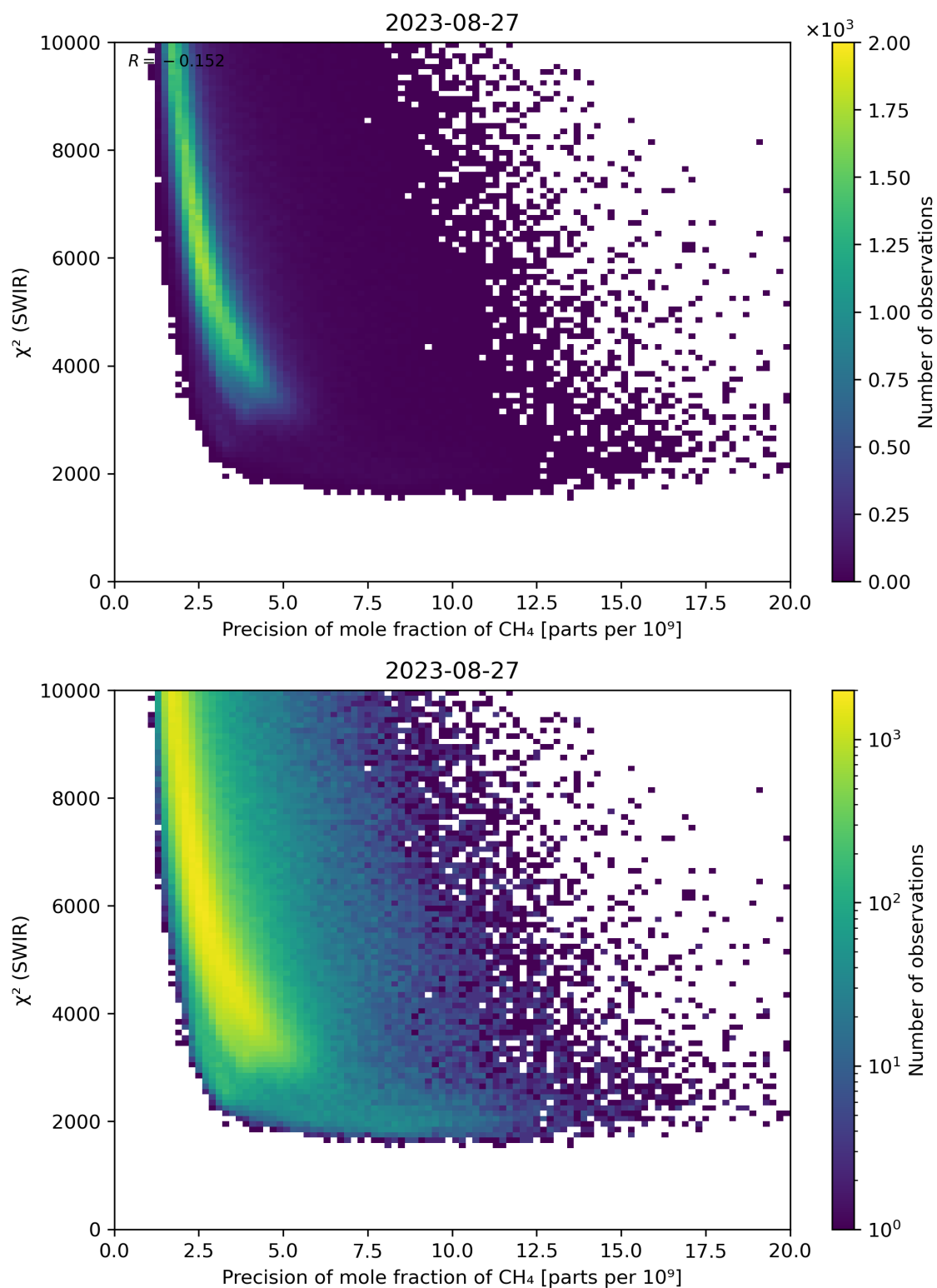
Figure 79: Scatter density plot of “Precision of mole fraction of CH 4 ” against “ \chi^2 (SWIR)” for 2023-08-26 to 2023-08-28.
