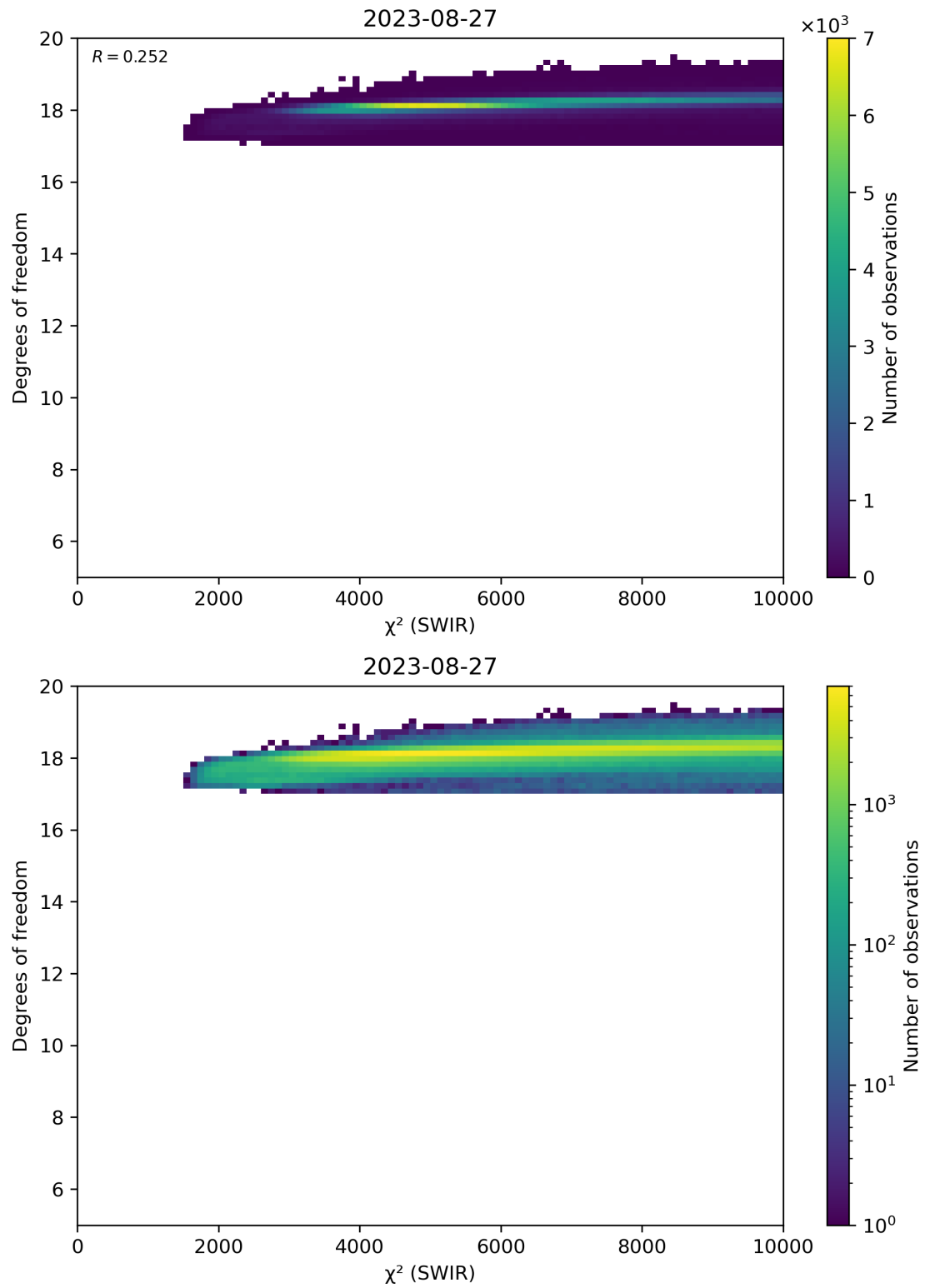
Figure 48: Scatter density plot of “ \chi^2 (SWIR)” against “Degrees of freedom” for 2023-08-26 to 2023-08-28.
