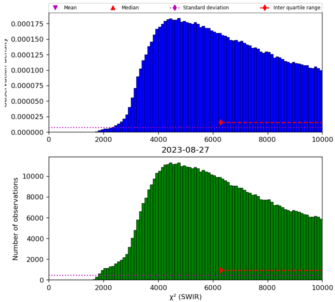
Figure 28: Histogram of “ \chi^2 (SWIR)” for 2023-08-26 to 2023-08-28
