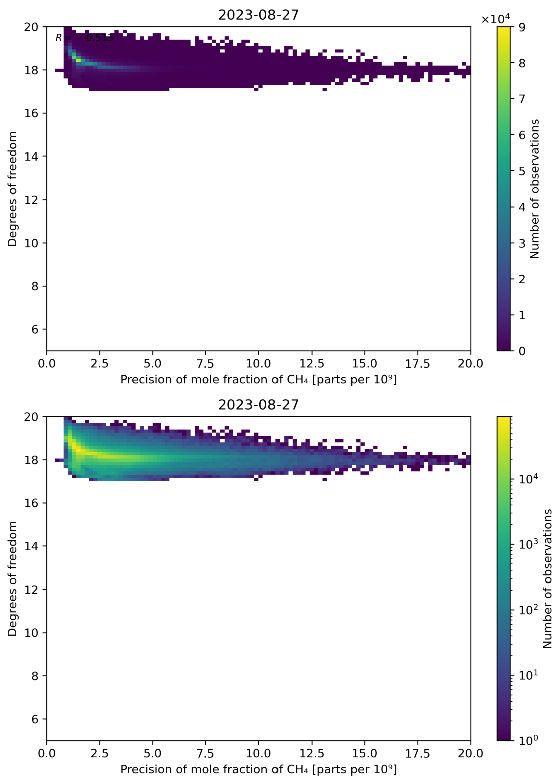
Figure 80: Scatter density plot of “Precision of mole fraction of CH 4 ” against “Degrees of freedom” for 2023-08-26 to 2023-08-28.
