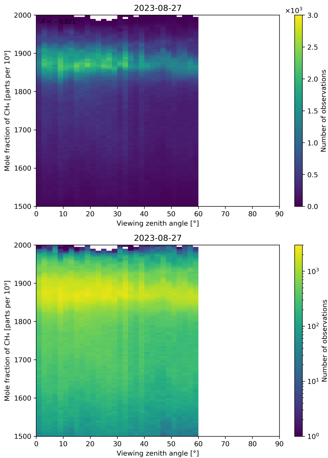
Figure 110: Scatter density plot of “Viewing zenith angle” against “Mole fraction of \text{CH}_4 ” for 2023-08-26 to 2023-08-28.
