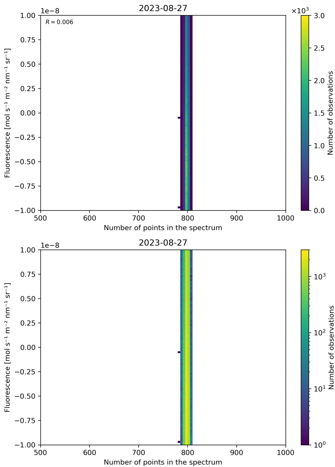
Figure 91: Scatter density plot of “Number of points in the spectrum” against “Fluorescence” for 2023-08-26 to 2023-08-28.
