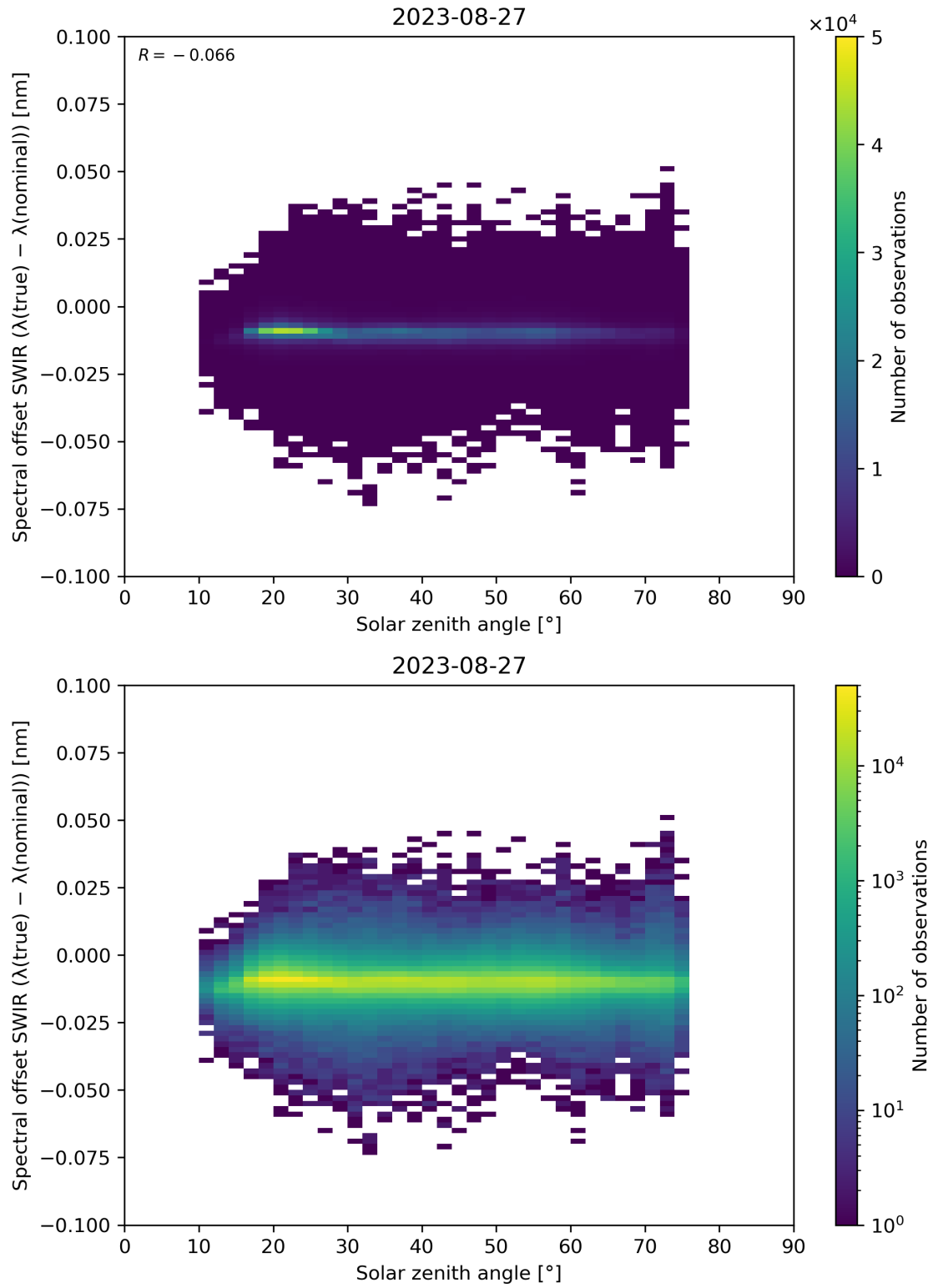
Figure 104: Scatter density plot of “Solar zenith angle” against “Spectral offset SWIR ( \lambda(\text{true}) - \lambda(\text{nominal}) )” for 2023-08-26 to 2023-08-28.
