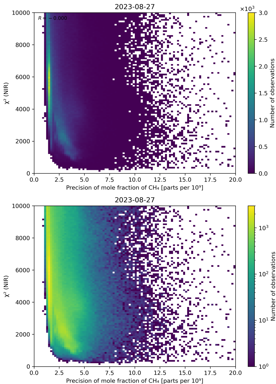
Figure 78: Scatter density plot of “Precision of mole fraction of CH 4 ” against “ \chi^2 (NIR)” for 2023-08-26 to 2023-08-28.
