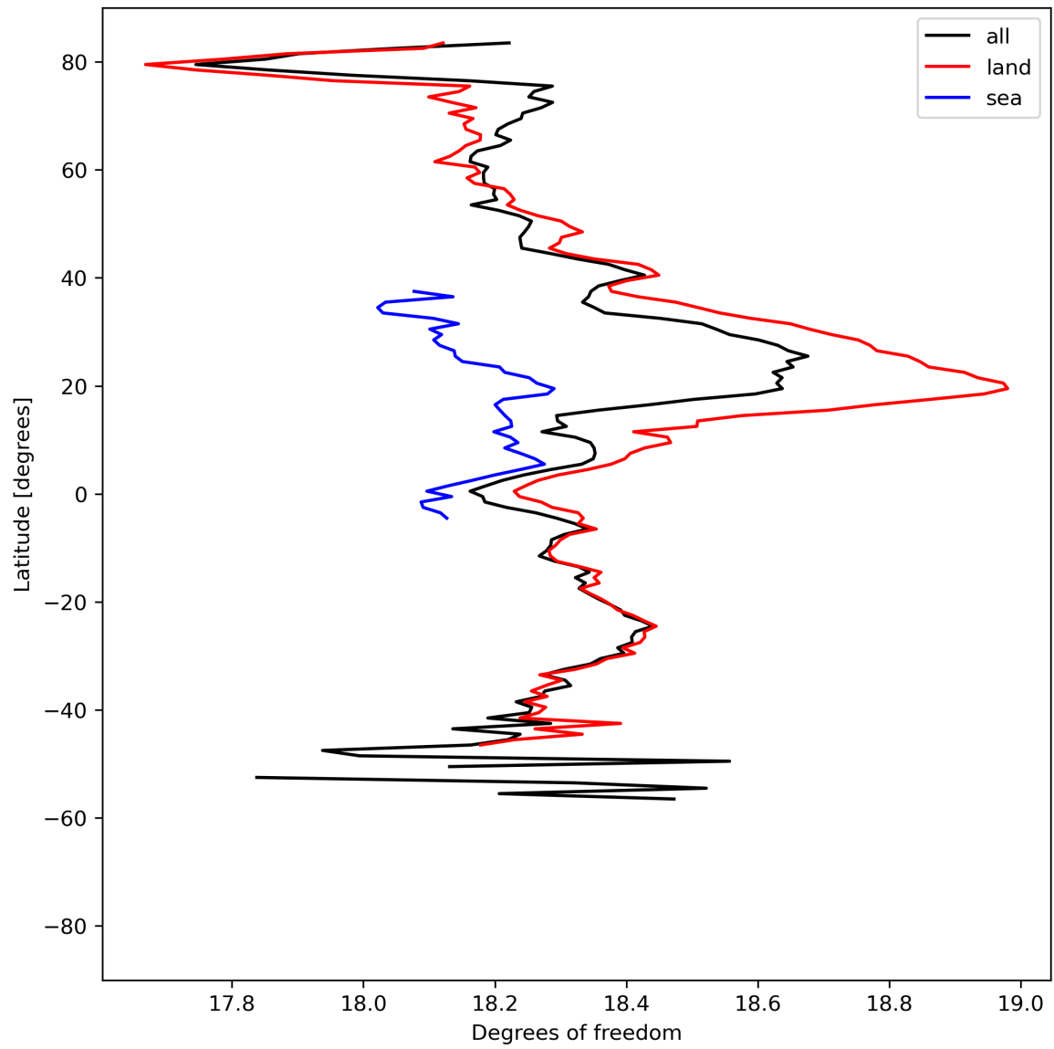
Figure 19: Zonal average of “Degrees of freedom” for 2023-08-26 to 2023-08-28.
