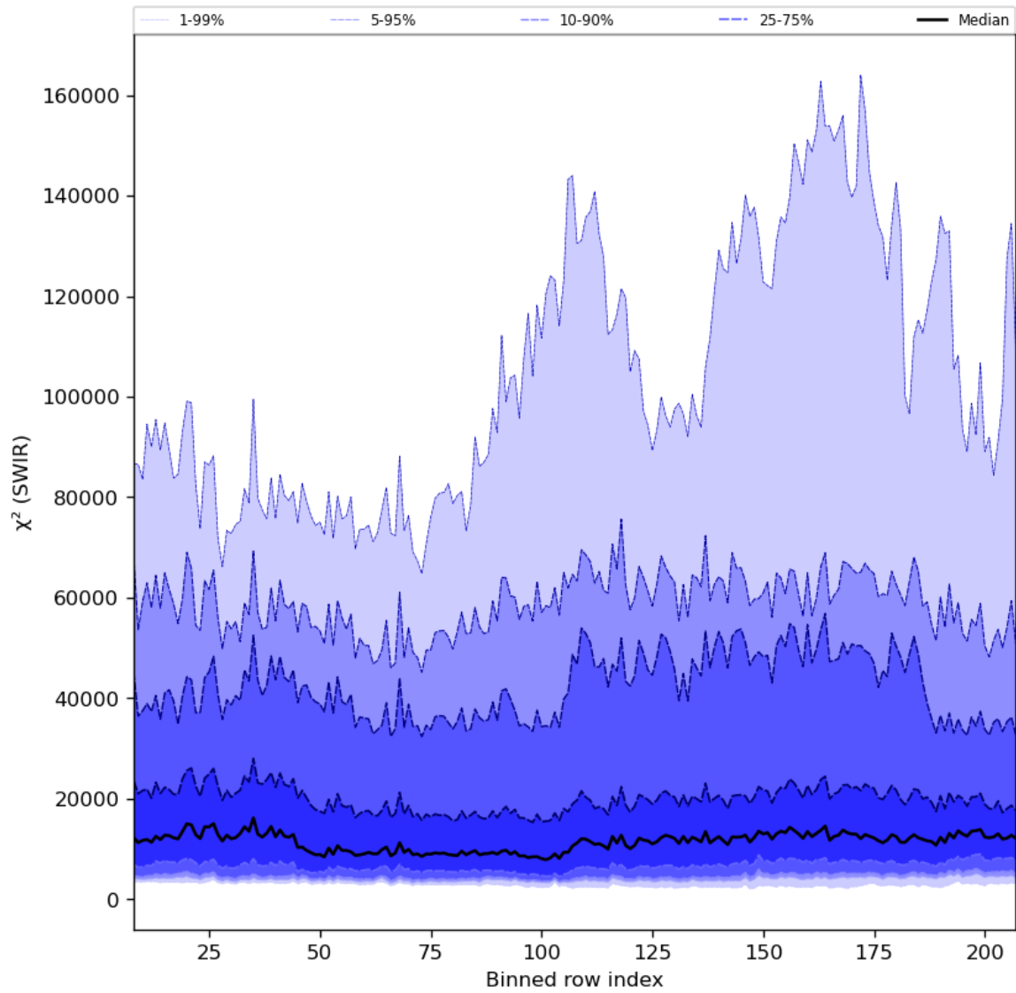
Figure 39: Along track statistics of " \chi^2 (SWIR)" for 2023-08-26 to 2023-08-28
