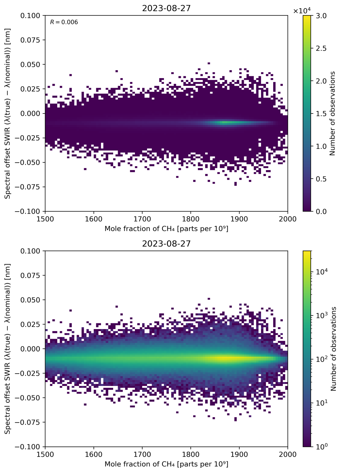
Figure 86: Scatter density plot of “Mole fraction of CH 4 ” against “Spectral offset SWIR ( \lambda(\text{true}) - \lambda(\text{nominal}) )” for 2023-08-26 to 2023-08-28.
