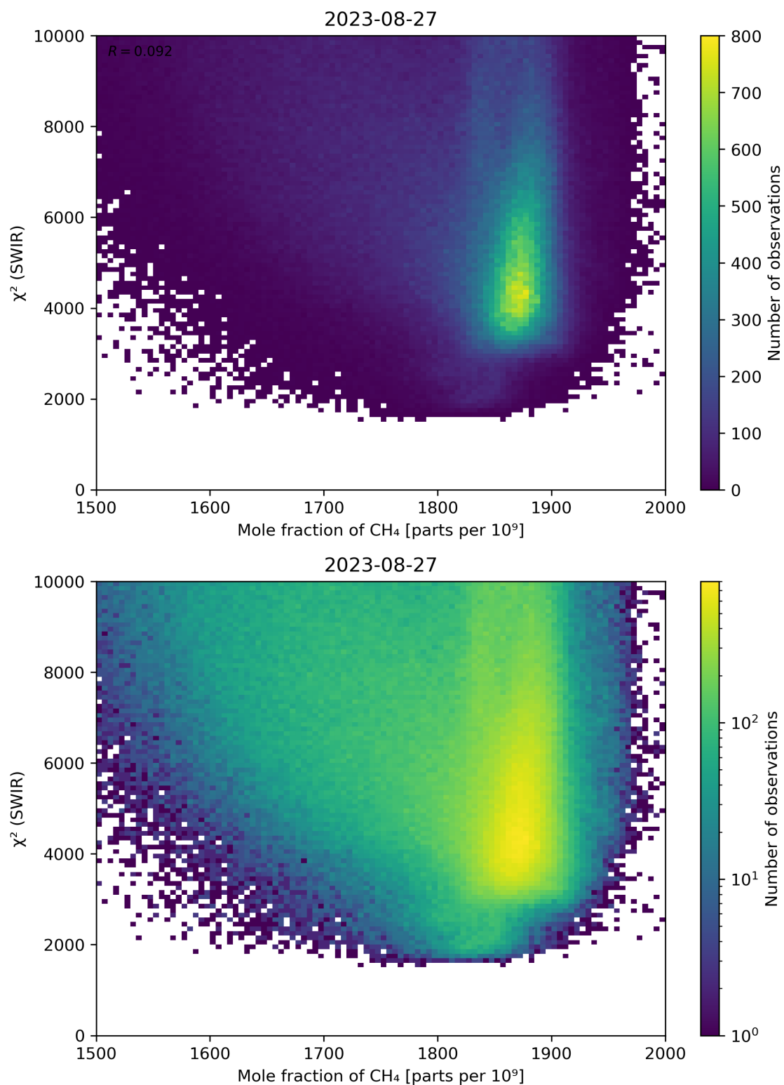
Figure 71: Scatter density plot of “Mole fraction of \text{CH}_4 ” against “ \chi^2 (SWIR)” for 2023-08-26 to 2023-08-28.
