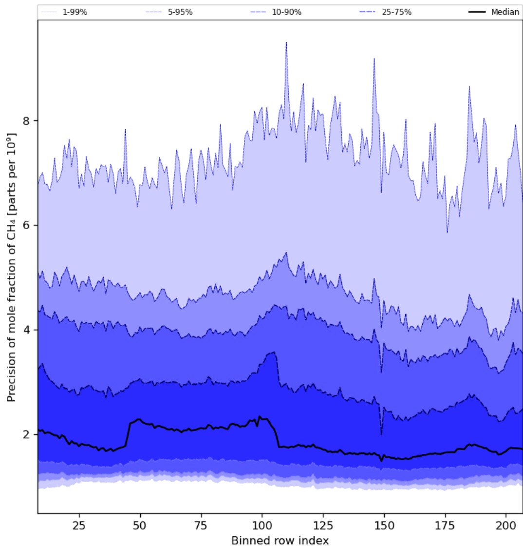
Figure 35: Along track statistics of “Precision of mole fraction of CH 4 ” for 2023-08-26 to 2023-08-28
