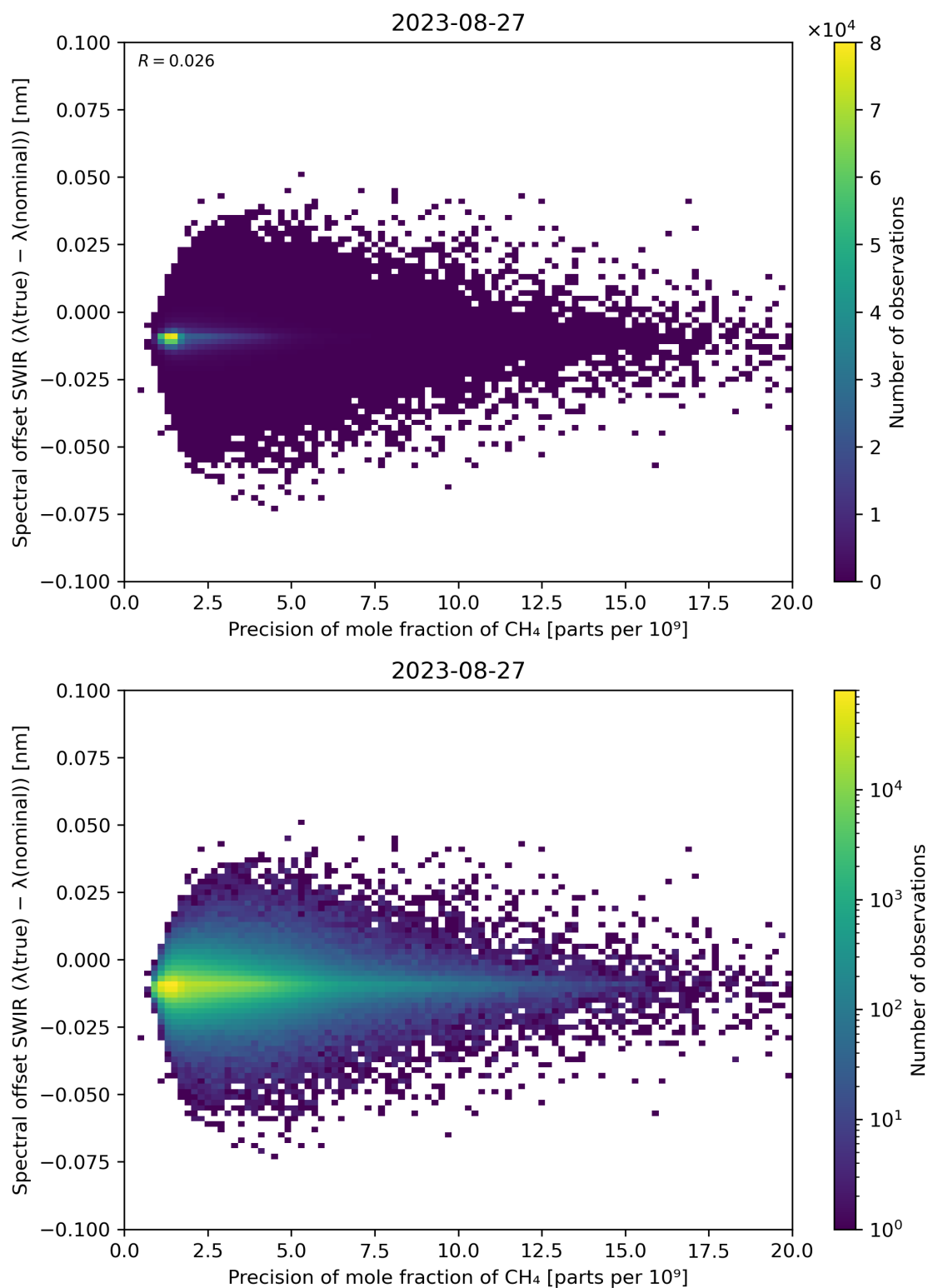
Figure 85: Scatter density plot of “Precision of mole fraction of CH 4 ” against “Spectral offset SWIR ( \lambda(\text{true}) - \lambda(\text{nominal}) )” for 2023-08-26 to 2023-08-28.
