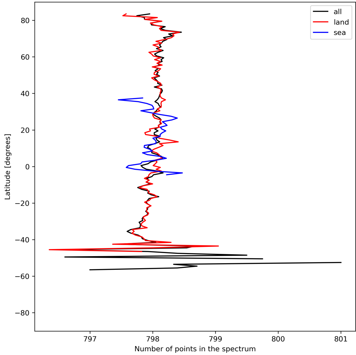
Figure 15: Zonal average of “Number of points in the spectrum” for 2023-08-26 to 2023-08-28.
