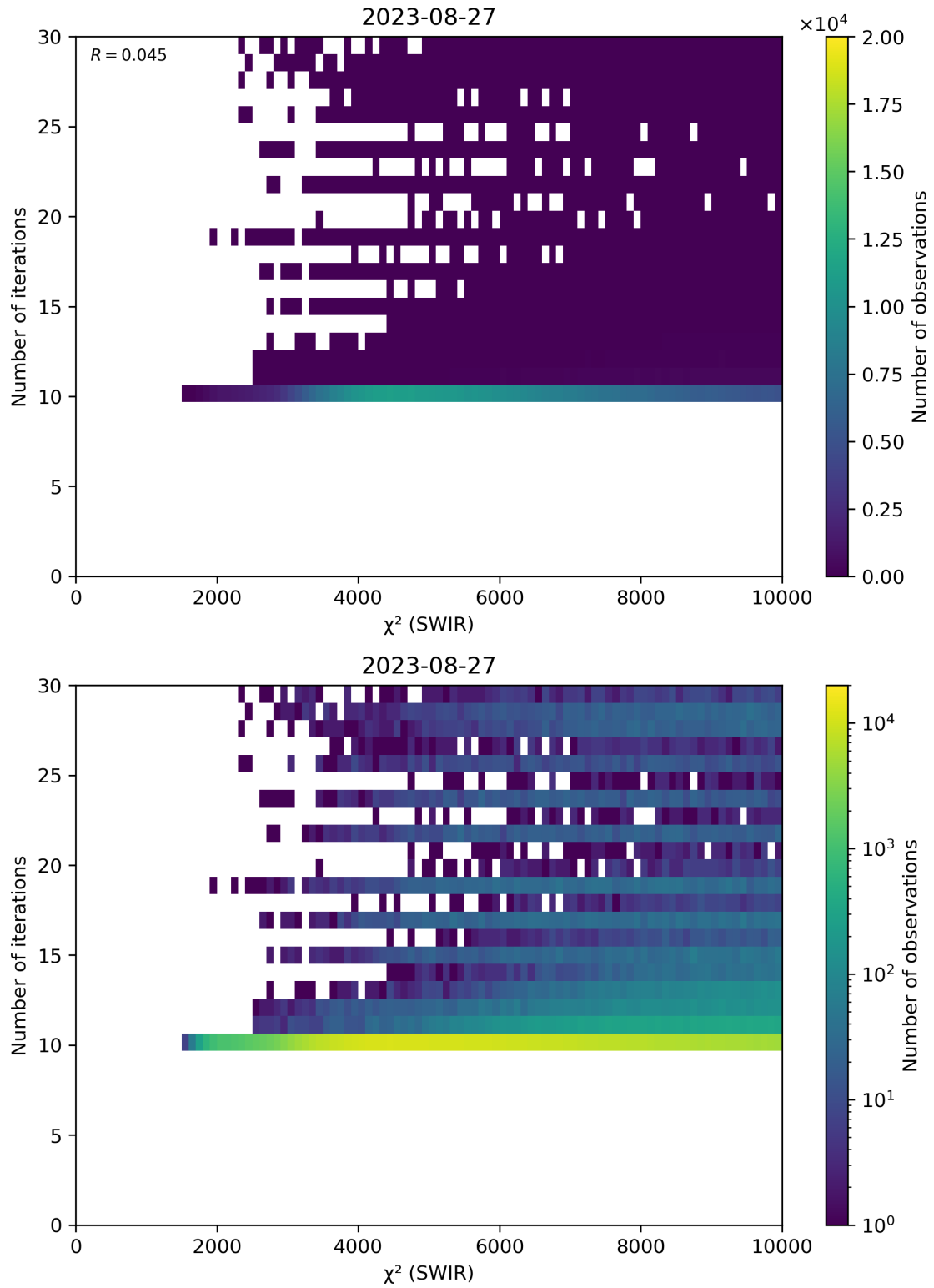
Figure 50: Scatter density plot of “ \chi^2 (SWIR)” against “Number of iterations” for 2023-08-26 to 2023-08-28.
