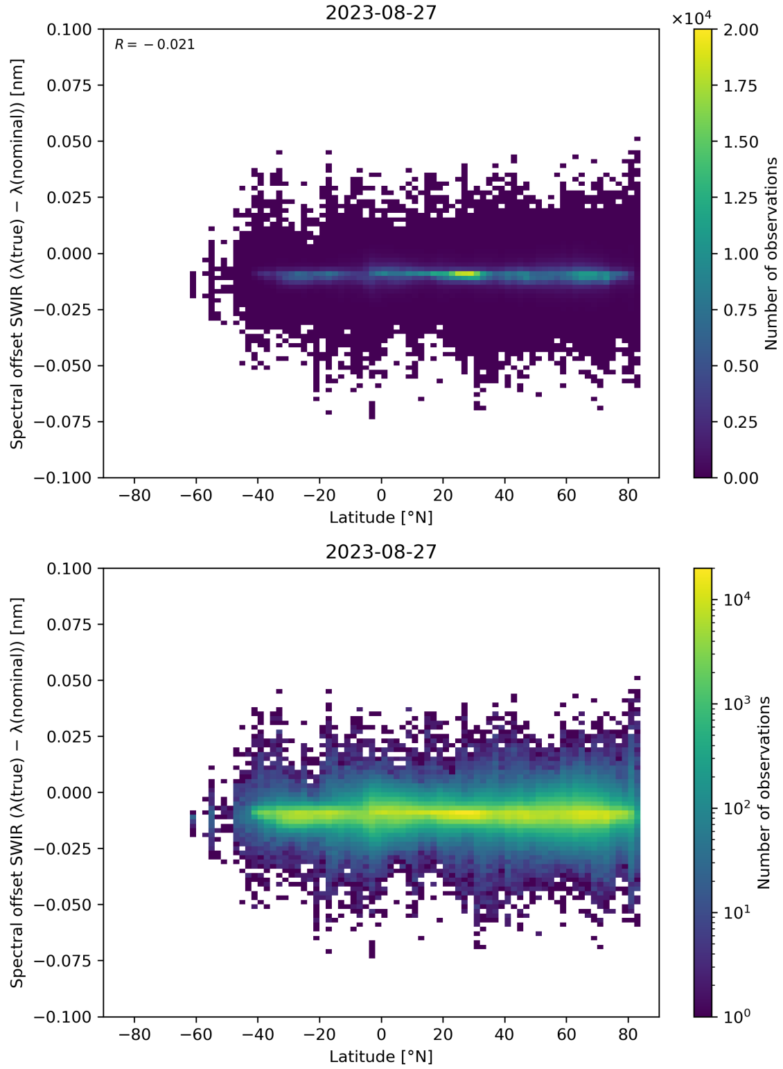
Figure 62: Scatter density plot of “Latitude” against “Spectral offset SWIR ( \lambda(\text{true}) - \lambda(\text{nominal}) )” for 2023-08-26 to 2023-08-28.
