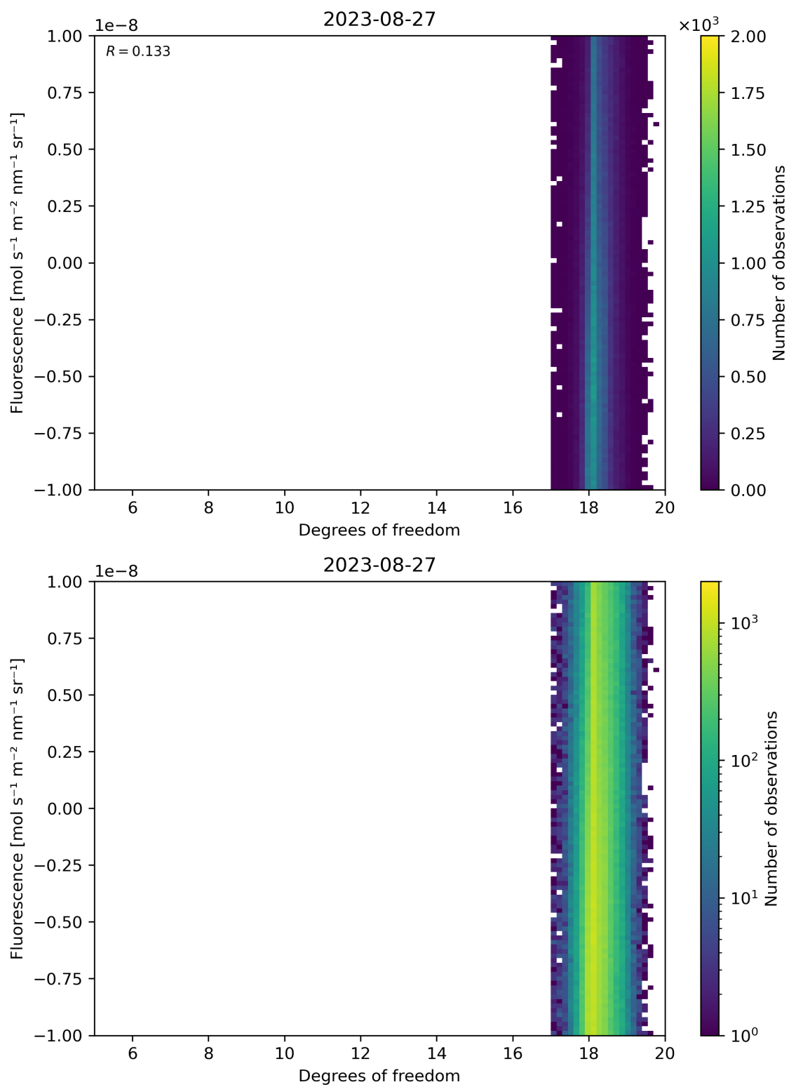
Figure 51: Scatter density plot of “Degrees of freedom” against “Fluorescence” for 2023-08-26 to 2023-08-28.
