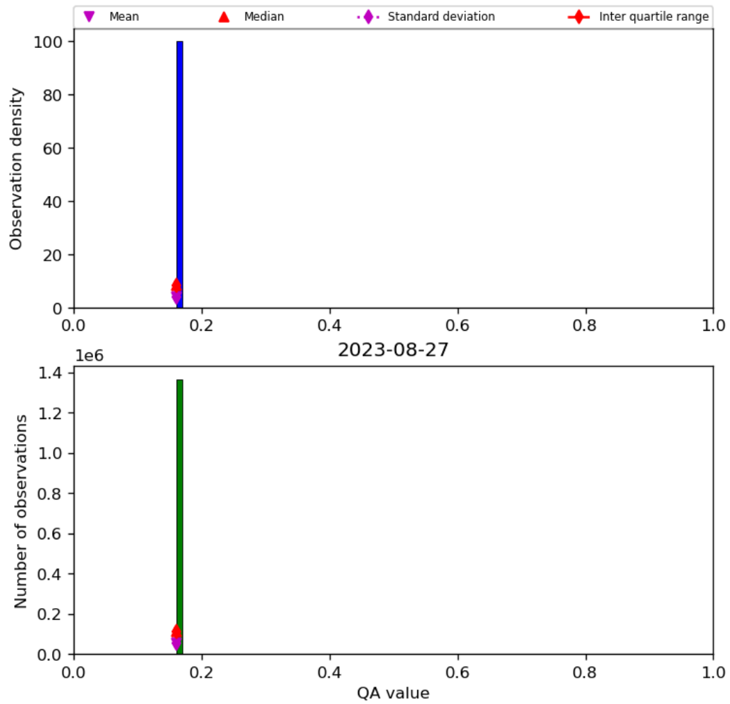
Figure 22: Histogram of “QA value” for 2023-08-26 to 2023-08-28
