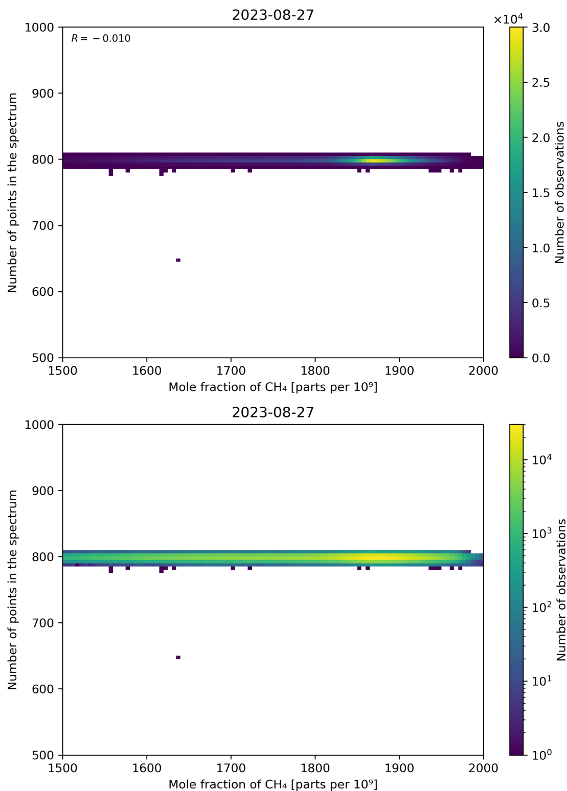
Figure 77: Scatter density plot of “Mole fraction of CH 4 ” against “Number of points in the spectrum” for 2023-08-26 to 2023-08-28.
