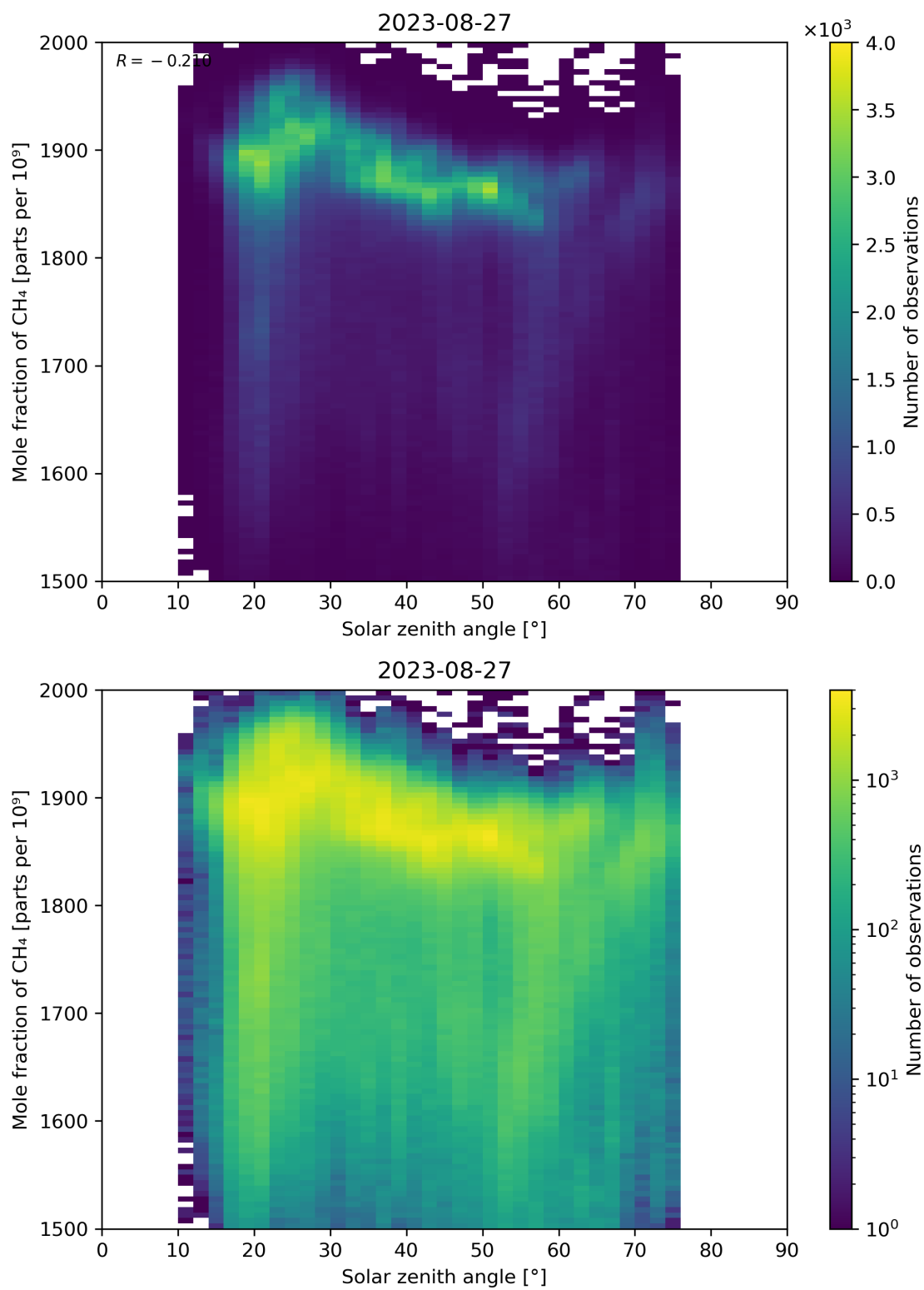
Figure 99: Scatter density plot of “Solar zenith angle” against “Mole fraction of CH 4 ” for 2023-08-26 to 2023-08-28.
