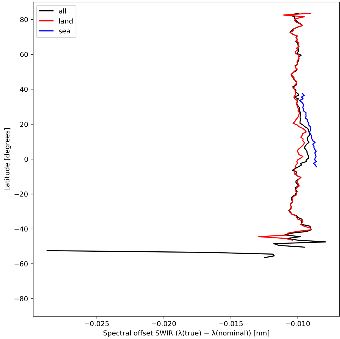
Figure 16: Zonal average of “Spectral offset SWIR ( \lambda(\text{true}) - \lambda(\text{nominal}) )” for 2023-08-26 to 2023-08-28.
