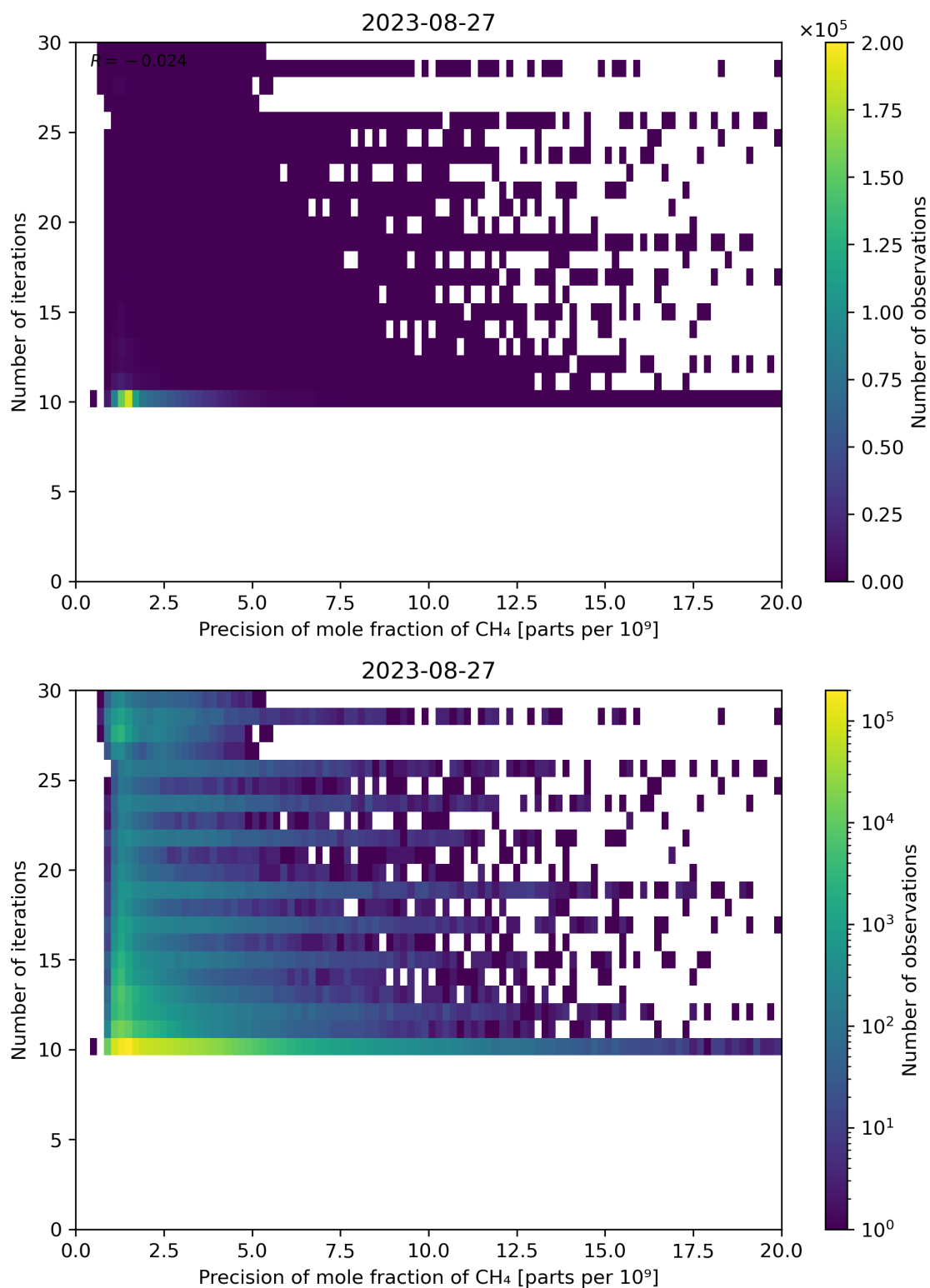
Figure 83: Scatter density plot of “Precision of mole fraction of CH 4 ” against “Number of iterations” for 2023-08-26 to 2023-08-28.
