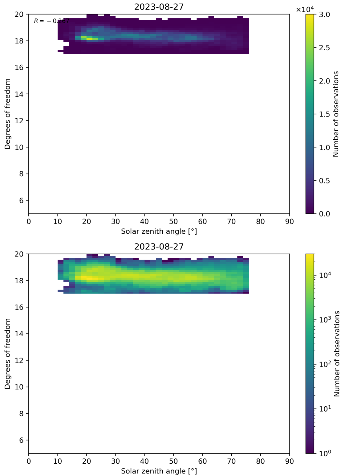
Figure 96: Scatter density plot of “Solar zenith angle” against “Degrees of freedom” for 2023-08-26 to 2023-08-28.
