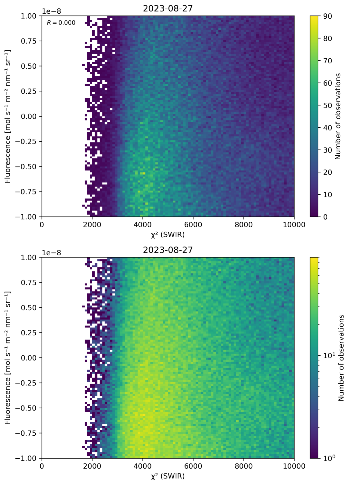
Figure 49: Scatter density plot of “ \chi^2 (SWIR)” against “Fluorescence” for 2023-08-26 to 2023-08-28.
