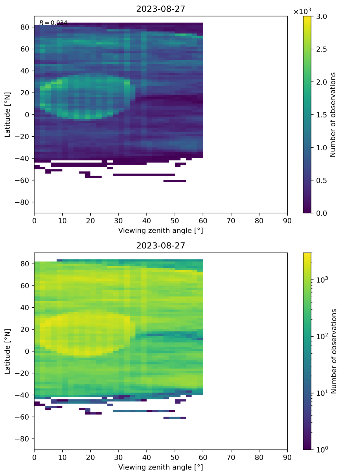
Figure 109: Scatter density plot of “Viewing zenith angle” against “Latitude” for 2023-08-26 to 2023-08-28.
