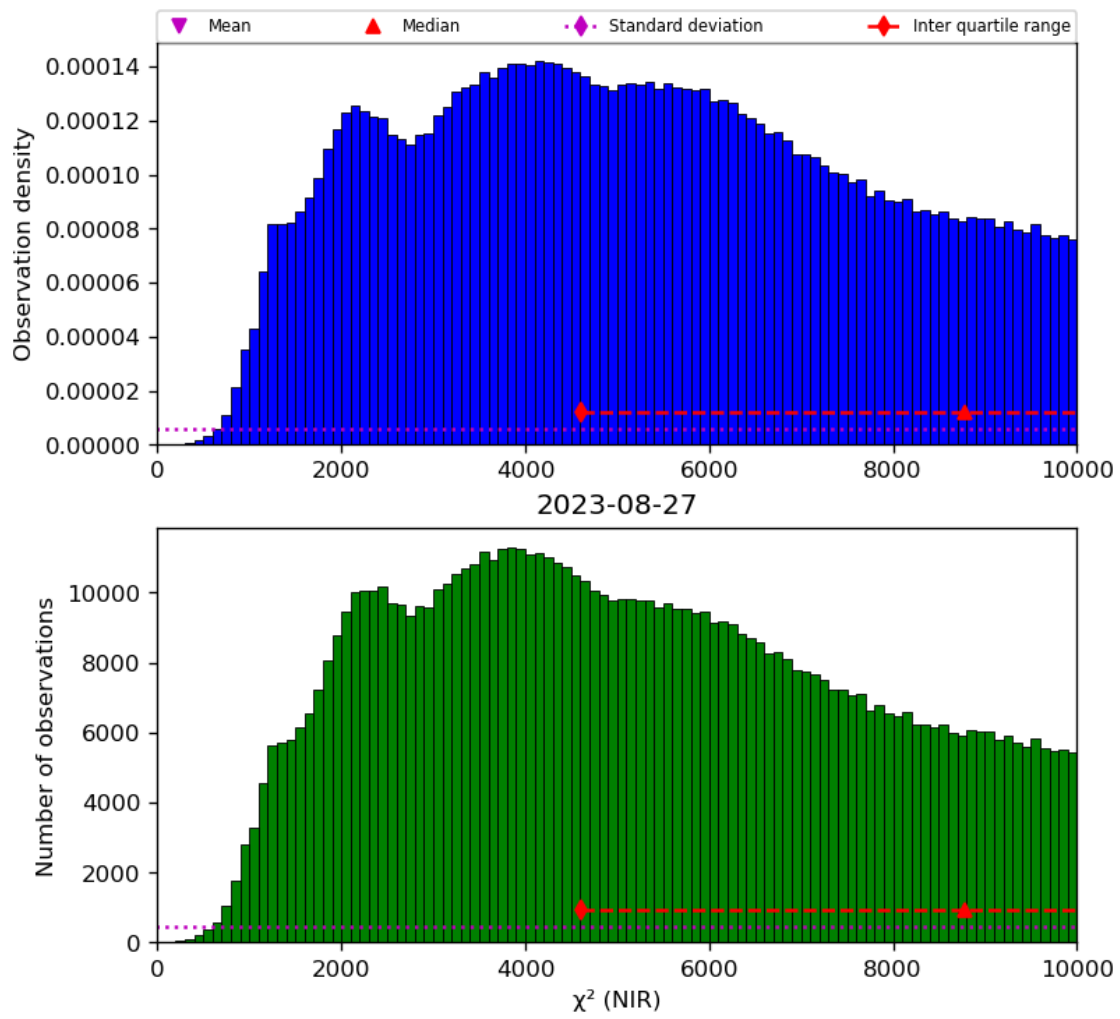
Figure 29: Histogram of “ \chi^2 (NIR)” for 2023-08-26 to 2023-08-28
