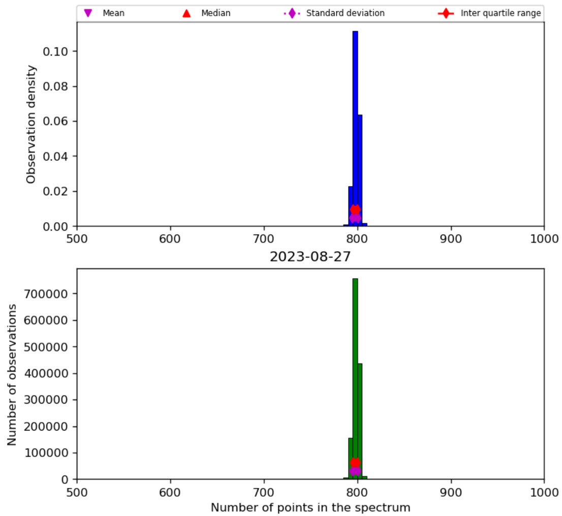
Figure 26: Histogram of “Number of points in the spectrum” for 2023-08-26 to 2023-08-28
