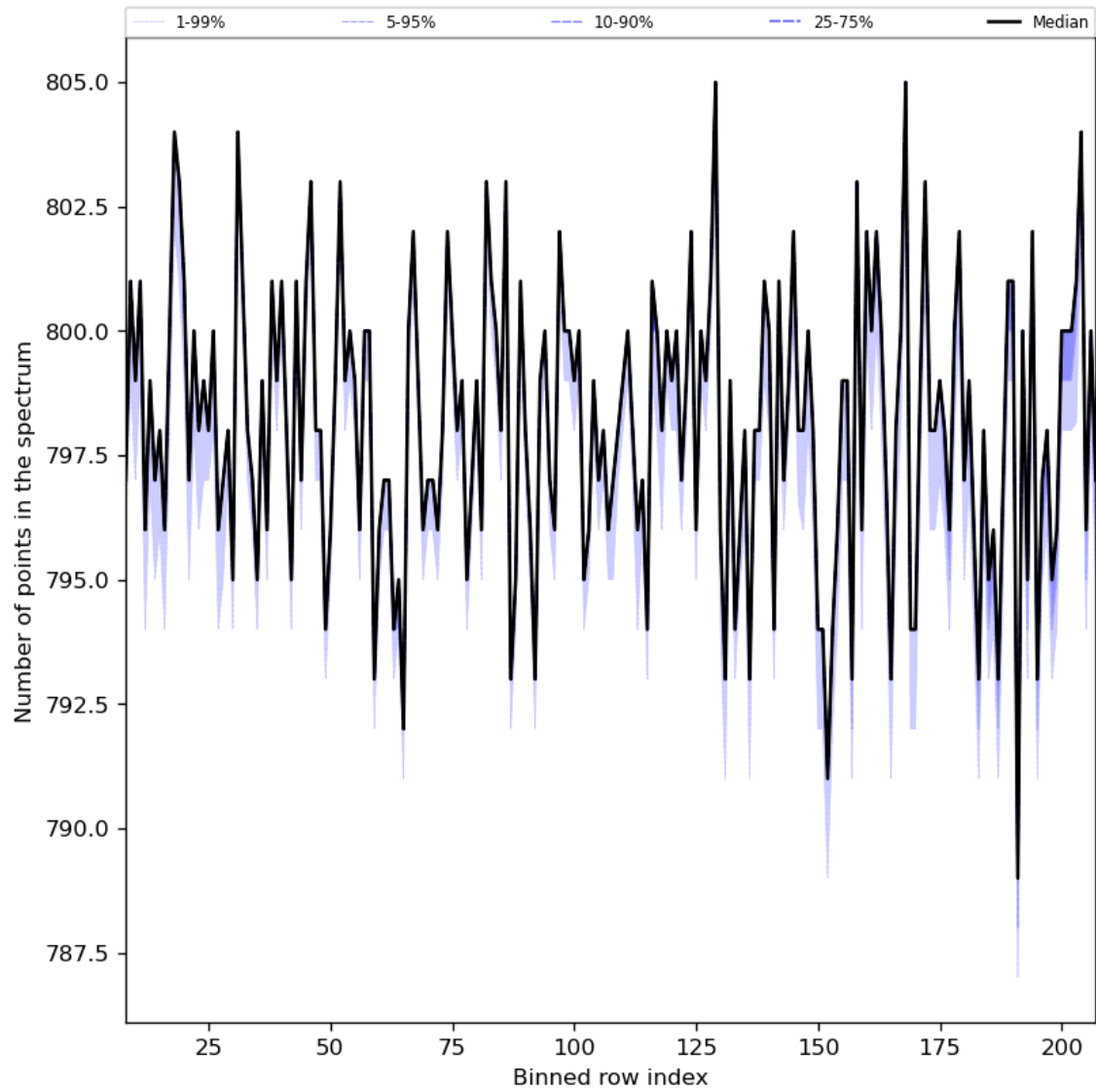
Figure 37: Along track statistics of “Number of points in the spectrum” for 2023-08-26 to 2023-08-28
