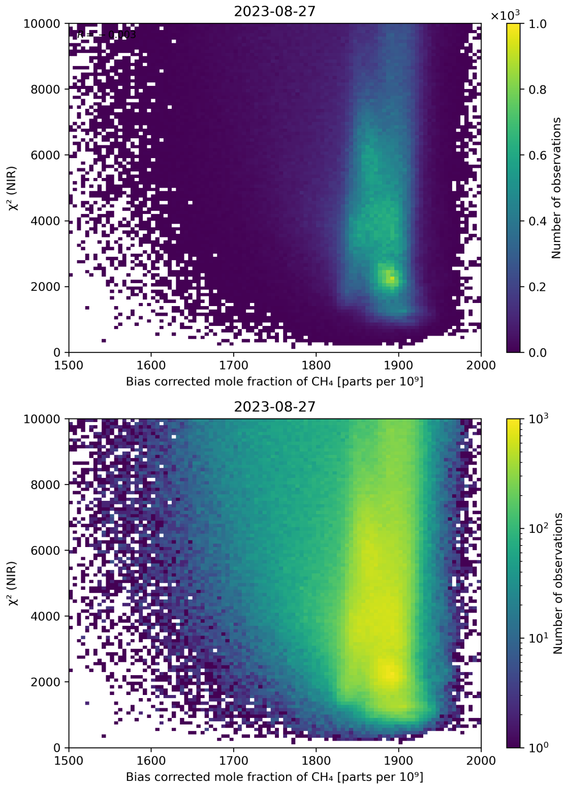
Figure 63: Scatter density plot of “Bias corrected mole fraction of CH 4 ” against “ \chi^2 (NIR)” for 2023-08-26 to 2023-08-28.
