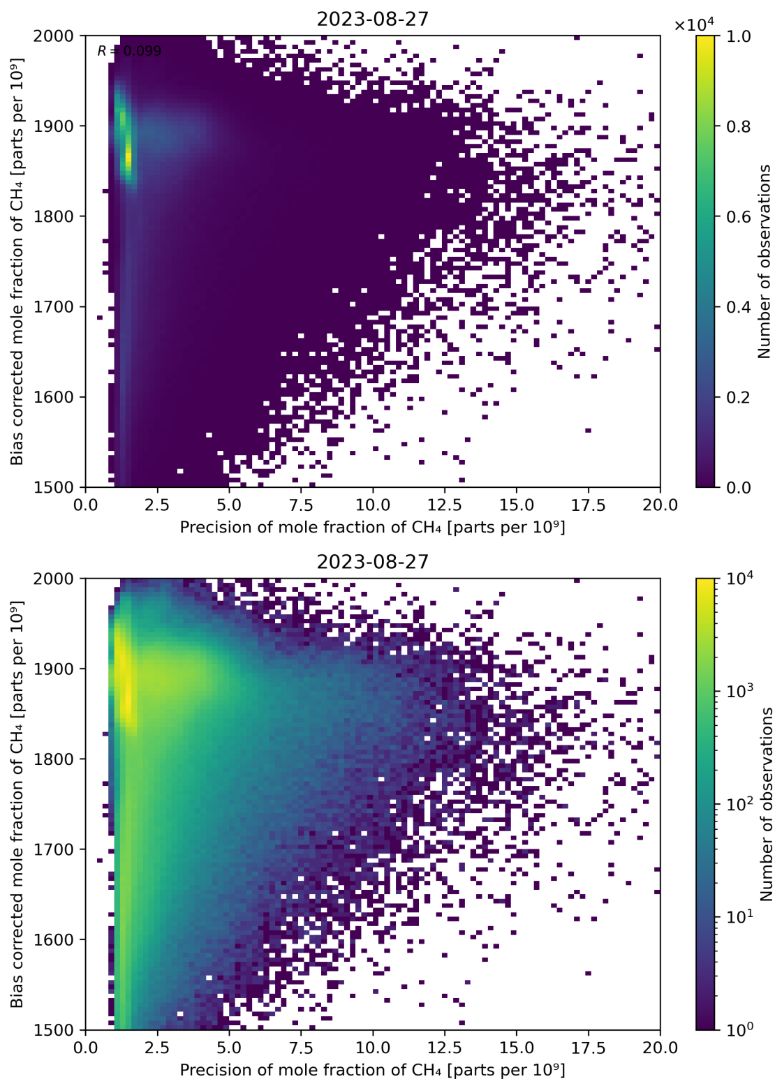
Figure 82: Scatter density plot of “Precision of mole fraction of CH 4 ” against “Bias corrected mole fraction of CH 4 ” for 2023-08-26 to 2023-08-28.
