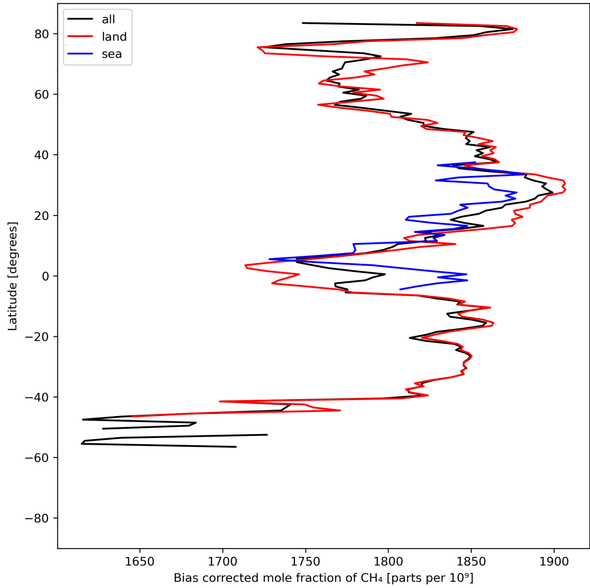
Figure 14: Zonal average of “Bias corrected mole fraction of CH 4 ” for 2023-08-26 to 2023-08-28.
