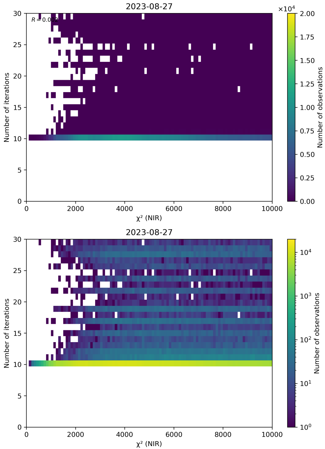
Figure 46: Scatter density plot of “ \chi^2 (NIR)” against “Number of iterations” for 2023-08-26 to 2023-08-28.
