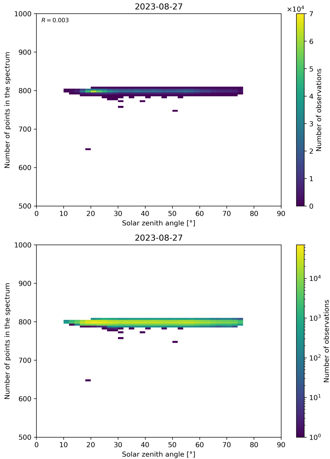
Figure 103: Scatter density plot of “Solar zenith angle” against “Number of points in the spectrum” for 2023-08-26 to 2023-08-28.
