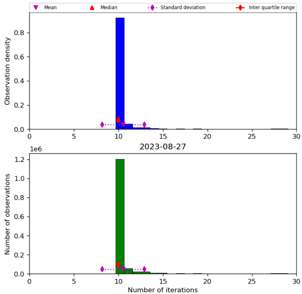
Figure 31: Histogram of “Number of iterations” for 2023-08-26 to 2023-08-28
