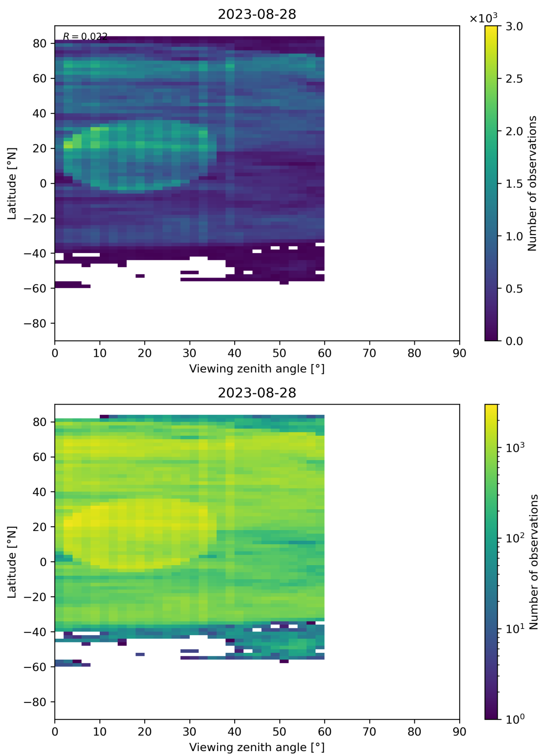
Figure 109: Scatter density plot of “Viewing zenith angle” against “Latitude” for 2023-08-27 to 2023-08-29.
