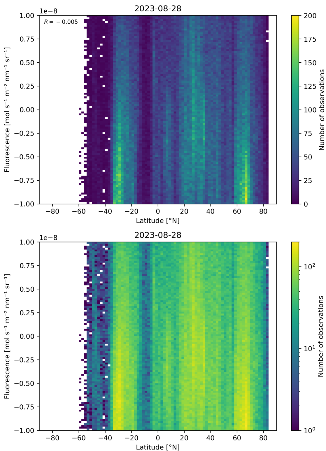
Figure 56: Scatter density plot of “Latitude” against “Fluorescence” for 2023-08-27 to 2023-08-29.
