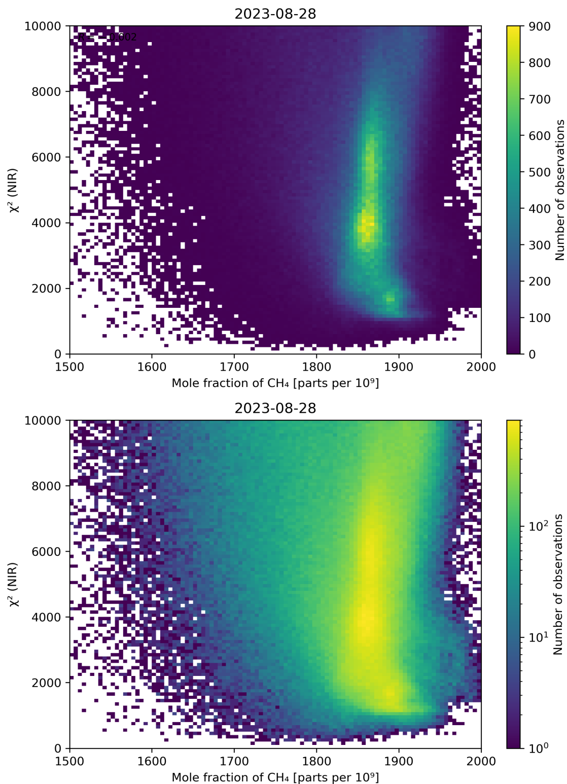
Figure 70: Scatter density plot of “Mole fraction of CH 4 ” against “ \chi^2 (NIR)” for 2023-08-27 to 2023-08-29.
