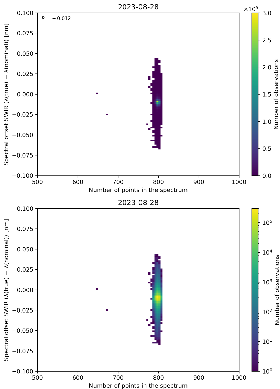
Figure 93: Scatter density plot of “Number of points in the spectrum” against “Spectral offset SWIR ( \lambda(\text{true}) - \lambda(\text{nominal}) )” for 2023-08-27 to 2023-08-29.
