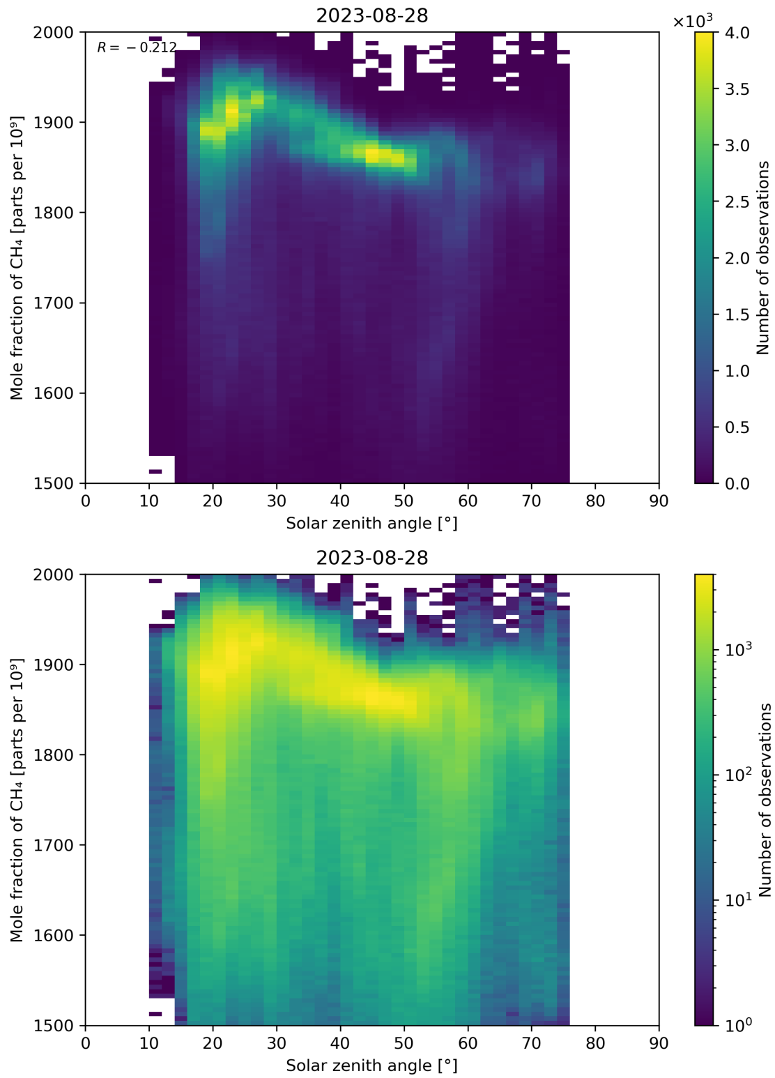
Figure 99: Scatter density plot of “Solar zenith angle” against “Mole fraction of CH 4 ” for 2023-08-27 to 2023-08-29.
