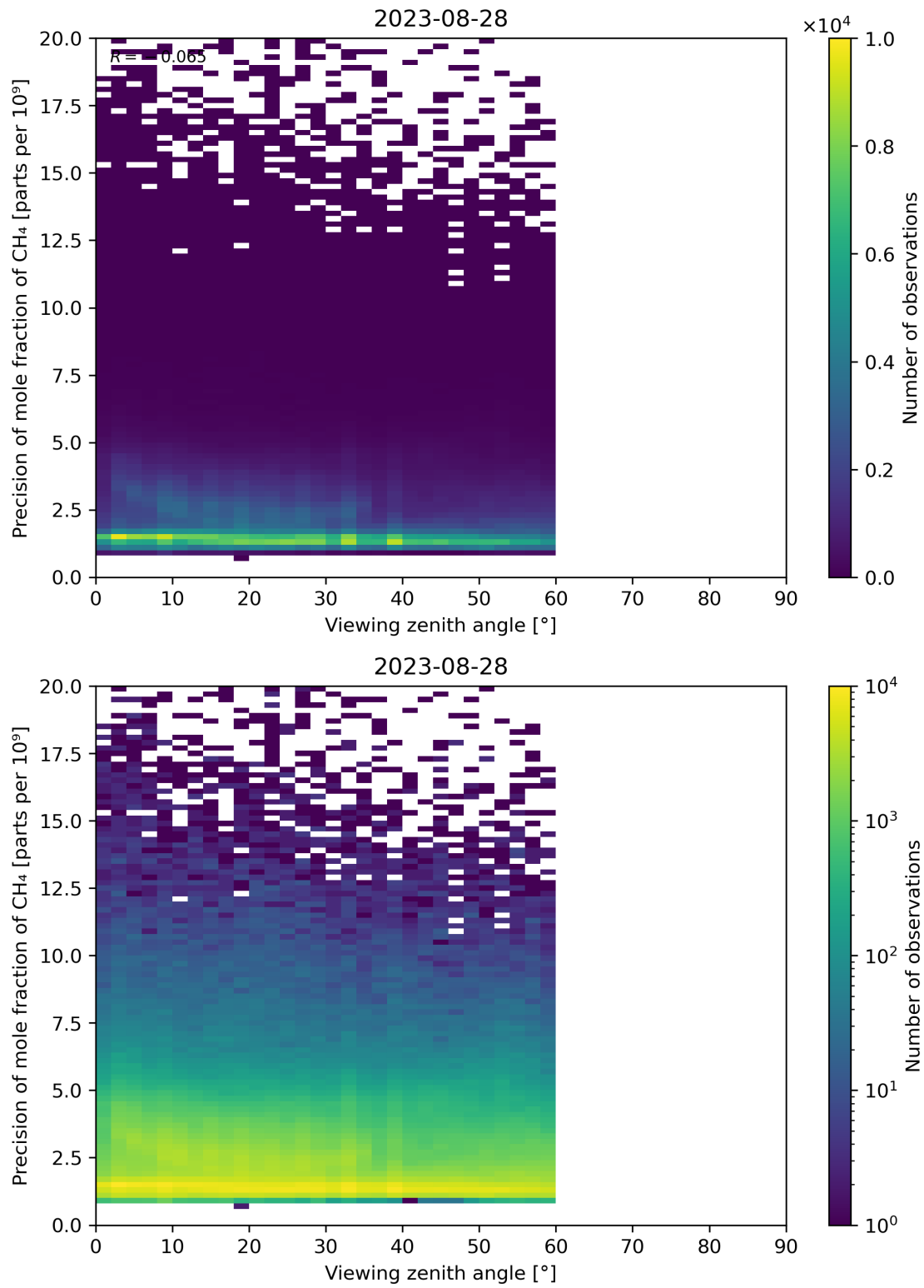
Figure 112: Scatter density plot of “Viewing zenith angle” against “Precision of mole fraction of CH 4 ” for 2023-08-27 to 2023-08-29.
