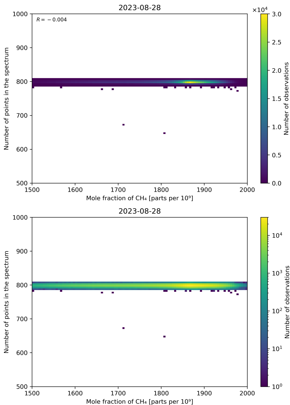
Figure 77: Scatter density plot of “Mole fraction of CH 4 ” against “Number of points in the spectrum” for 2023-08-27 to 2023-08-29.
