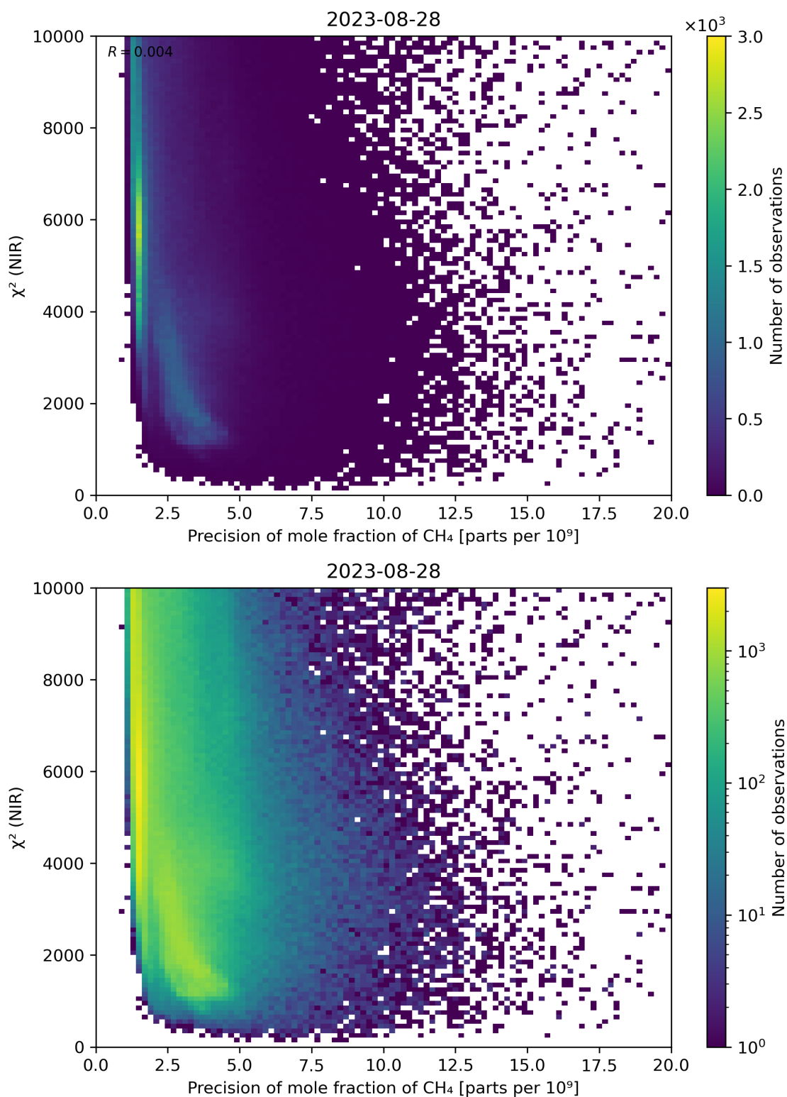
Figure 78: Scatter density plot of “Precision of mole fraction of CH 4 ” against “ \chi^2 (NIR)” for 2023-08-27 to 2023-08-29.
