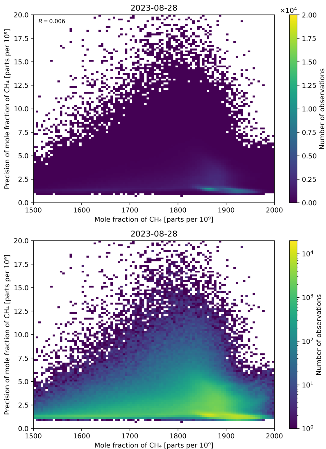
Figure 75: Scatter density plot of “Mole fraction of CH 4 ” against “Precision of mole fraction of CH 4 ” for 2023-08-27 to 2023-08-29.
