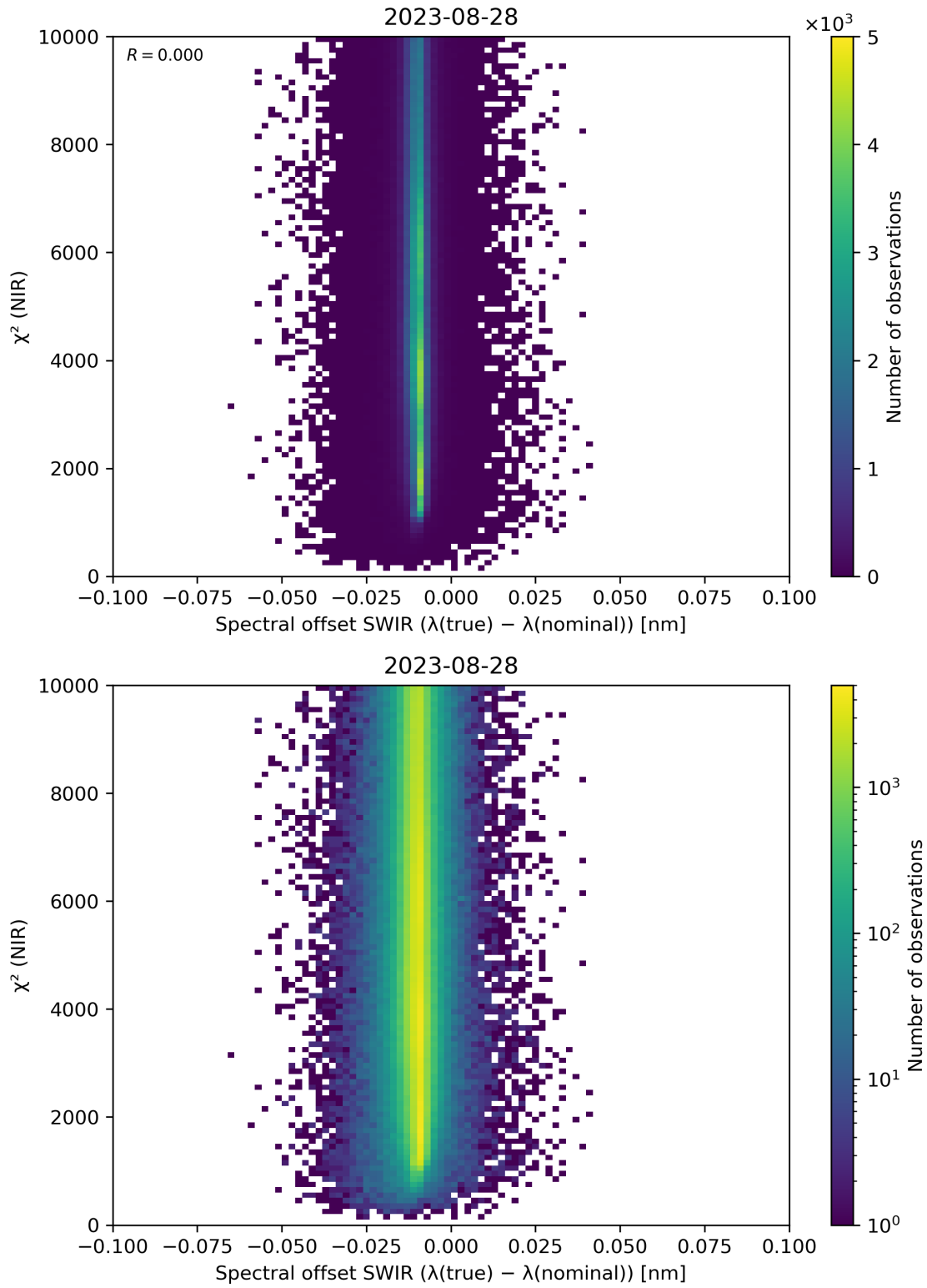
Figure 117: Scatter density plot of “Spectral offset SWIR ( \lambda(\text{true}) - \lambda(\text{nominal}) )” against “ \chi^2 (NIR)” for 2023-08-27 to 2023-08-29.
