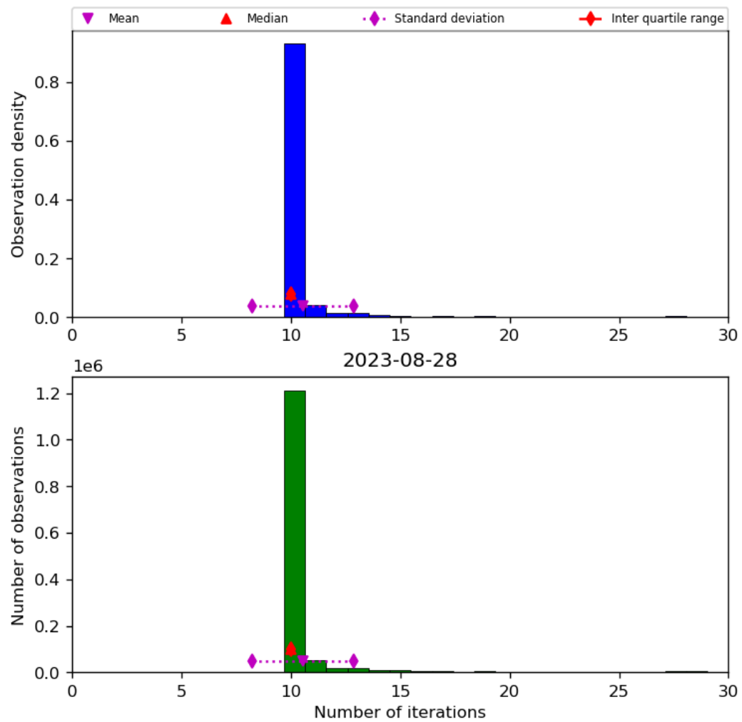
Figure 31: Histogram of “Number of iterations” for 2023-08-27 to 2023-08-29
