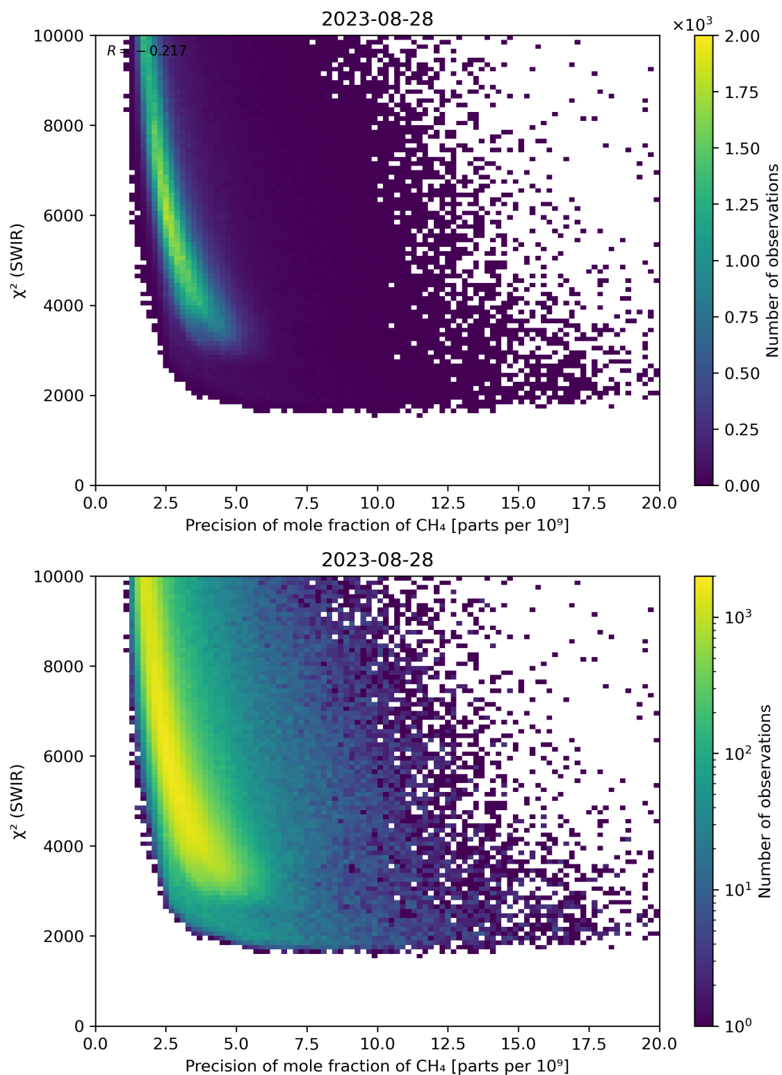
Figure 79: Scatter density plot of “Precision of mole fraction of CH 4 ” against “ \chi^2 (SWIR)” for 2023-08-27 to 2023-08-29.
