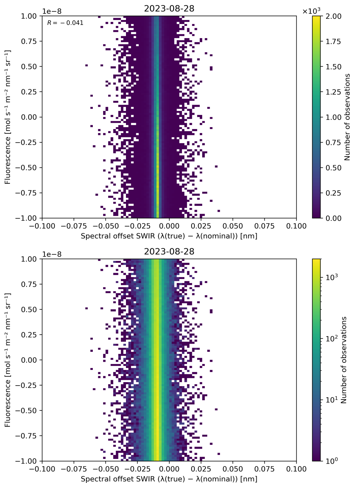
Figure 120: Scatter density plot of “Spectral offset SWIR ( \lambda(\text{true}) - \lambda(\text{nominal}) )” against “Fluorescence” for 2023-08-27 to 2023-08-29.
