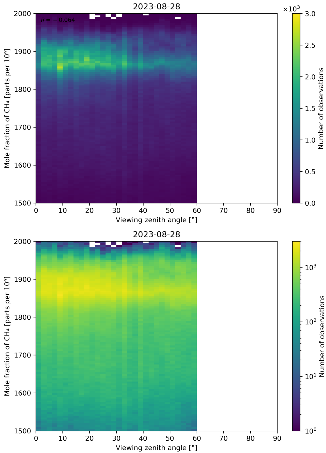
Figure 110: Scatter density plot of “Viewing zenith angle” against “Mole fraction of CH 4 ” for 2023-08-27 to 2023-08-29.
