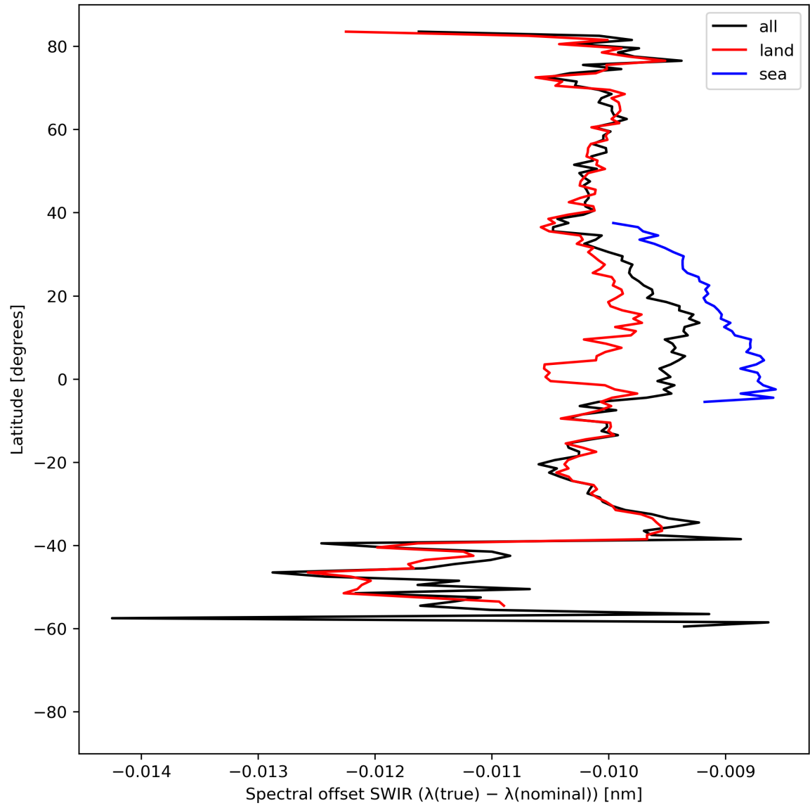
Figure 16: Zonal average of “Spectral offset SWIR ( \lambda(\text{true}) - \lambda(\text{nominal}) )” for 2023-08-27 to 2023-08-29.
