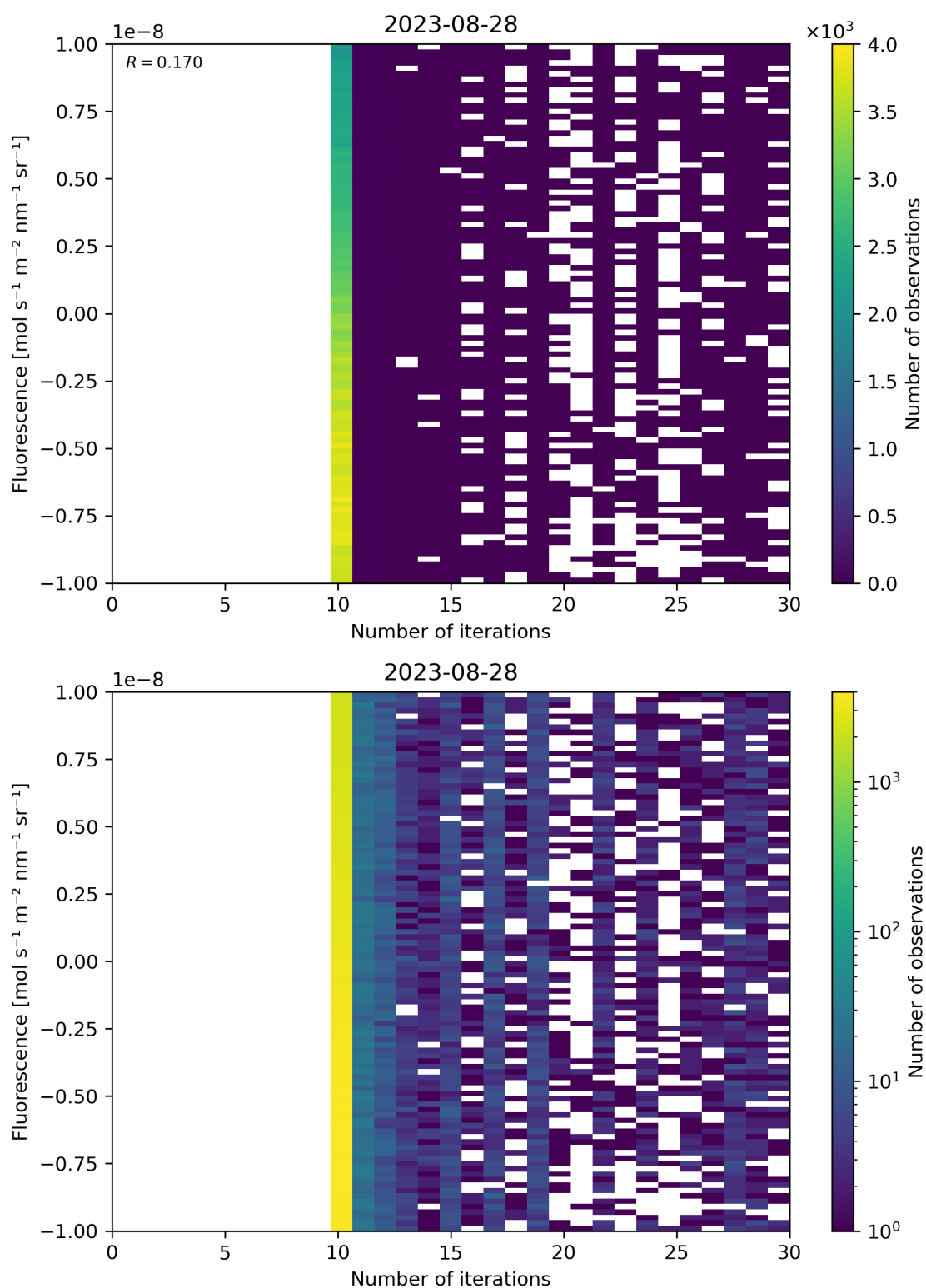
Figure 87: Scatter density plot of “Number of iterations” against “Fluorescence” for 2023-08-27 to 2023-08-29.
