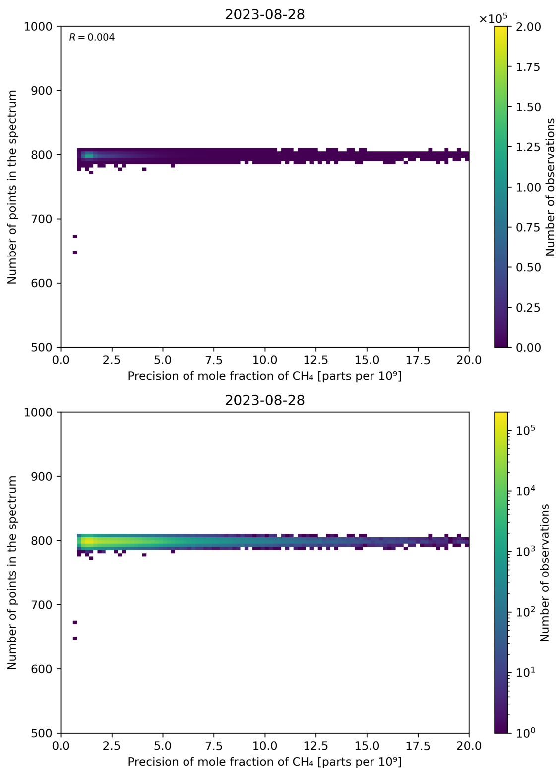
Figure 84: Scatter density plot of “Precision of mole fraction of CH 4 ” against “Number of points in the spectrum” for 2023-08-27 to 2023-08-29.
