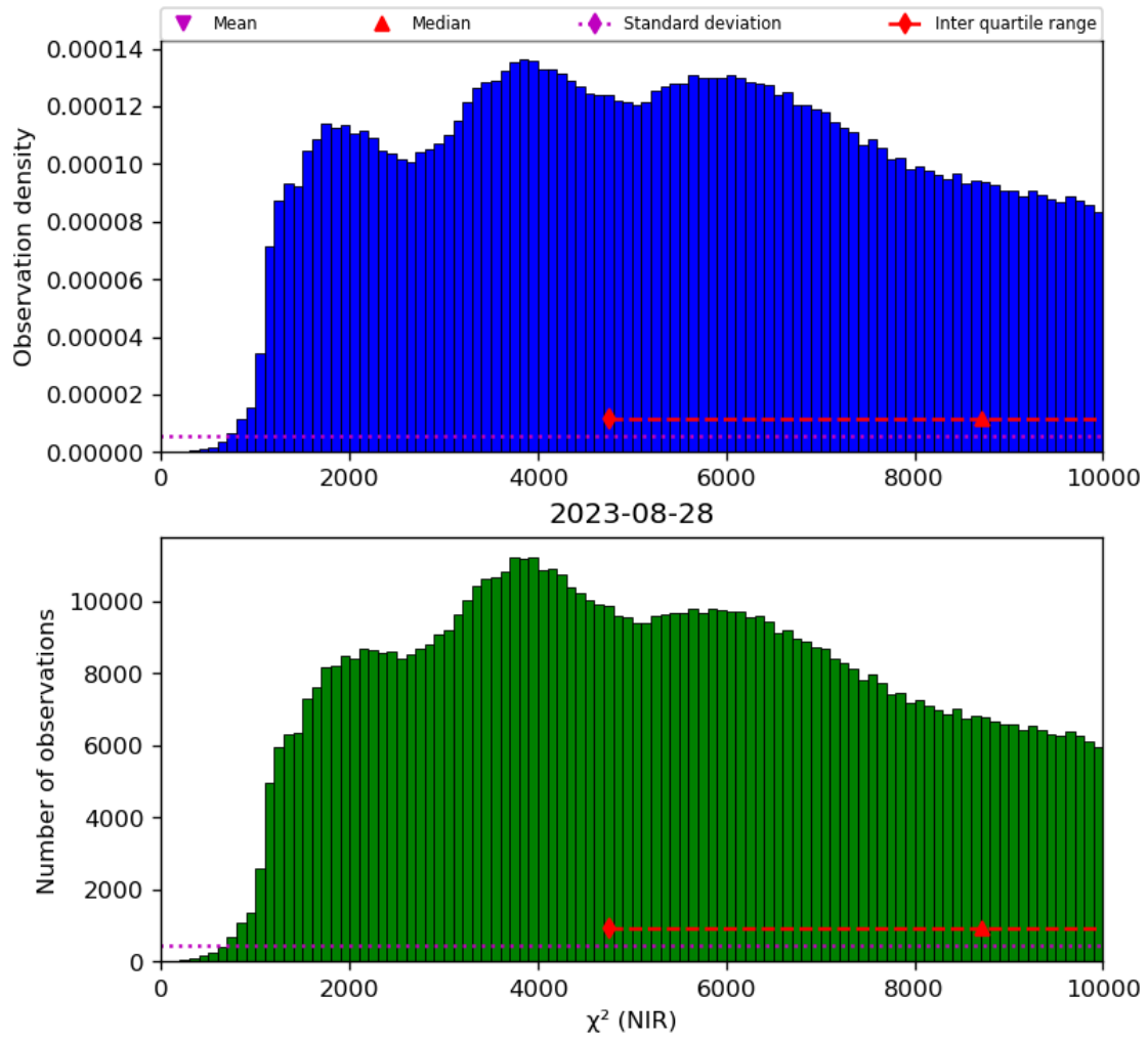
Figure 29: Histogram of " \chi^2 (NIR)" for 2023-08-27 to 2023-08-29
