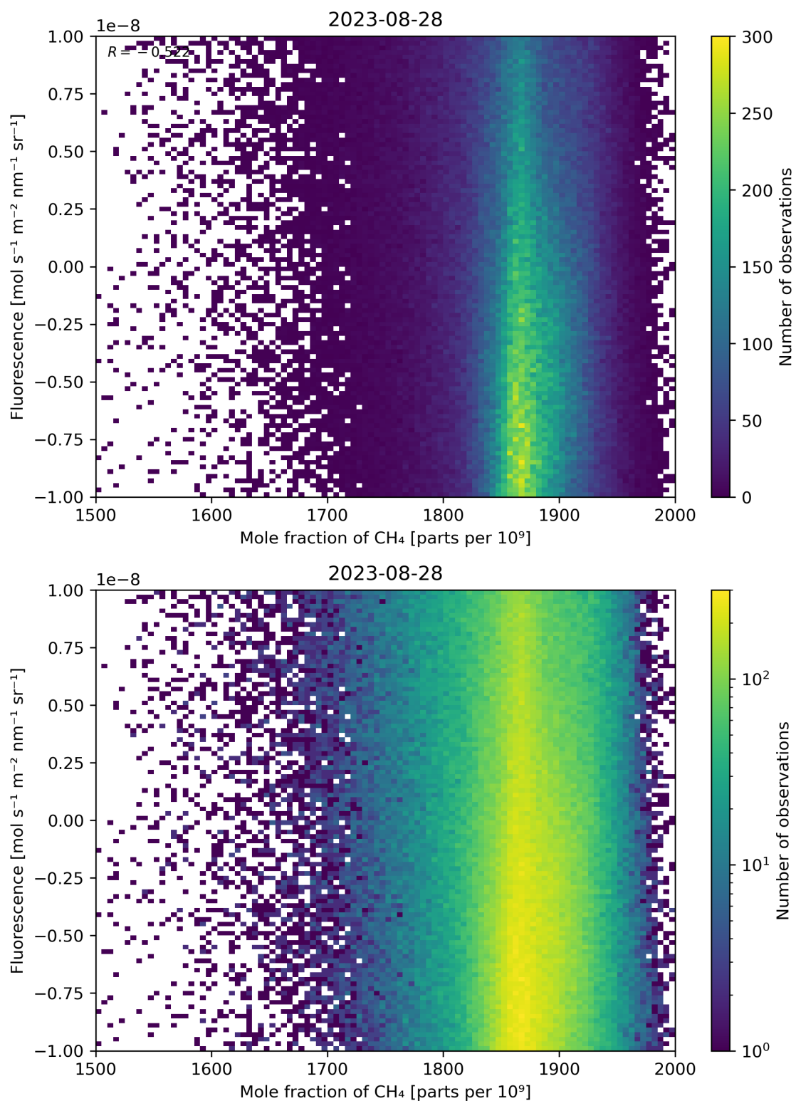
Figure 73: Scatter density plot of “Mole fraction of \text{CH}_4 ” against “Fluorescence” for 2023-08-27 to 2023-08-29.
