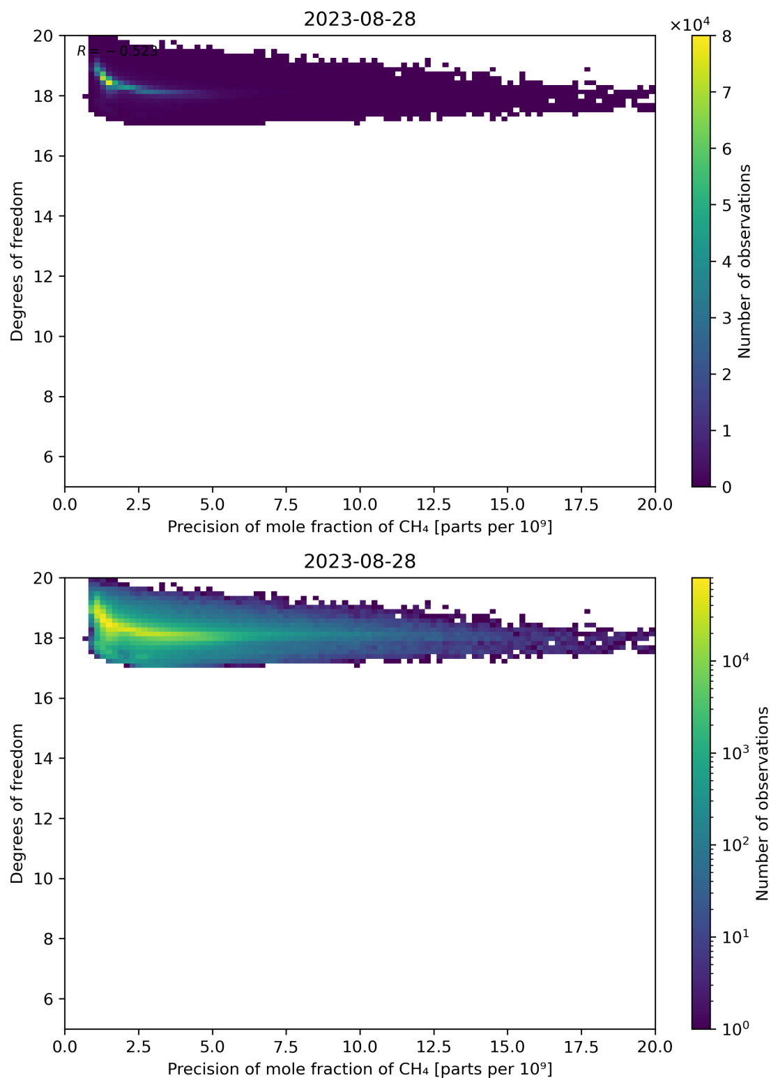
Figure 80: Scatter density plot of “Precision of mole fraction of CH 4 ” against “Degrees of freedom” for 2023-08-27 to 2023-08-29.
