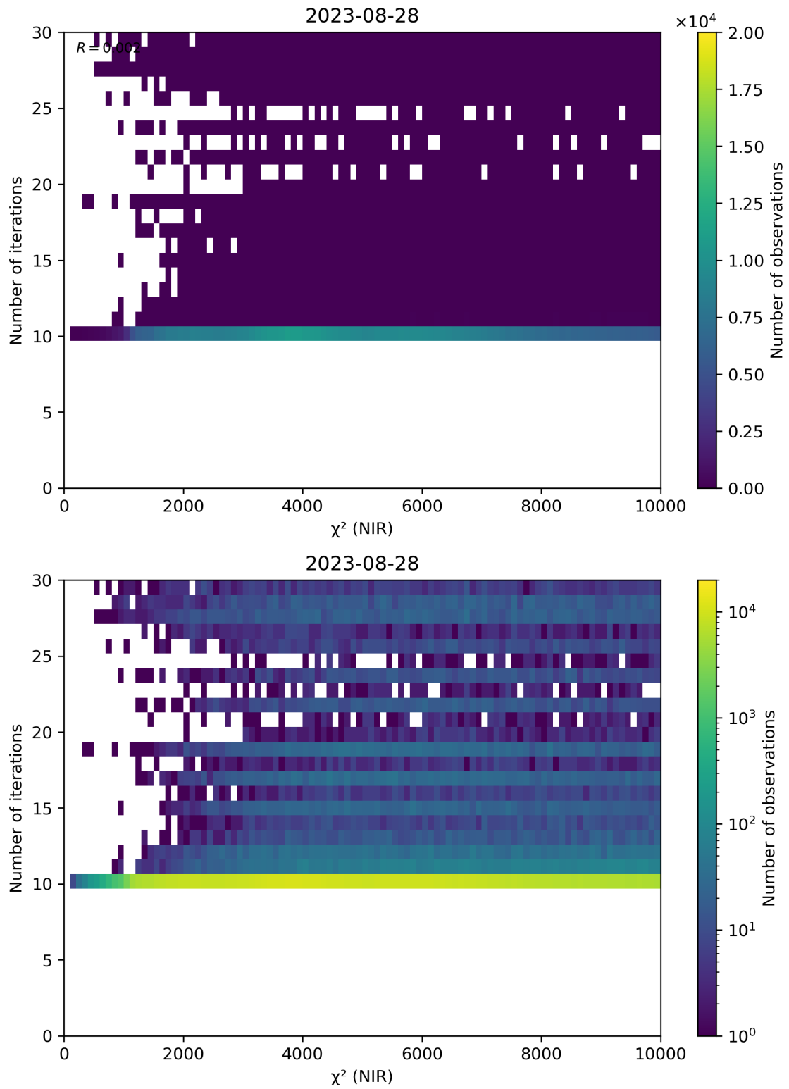
Figure 46: Scatter density plot of “ \chi^2 (NIR)” against “Number of iterations” for 2023-08-27 to 2023-08-29.
