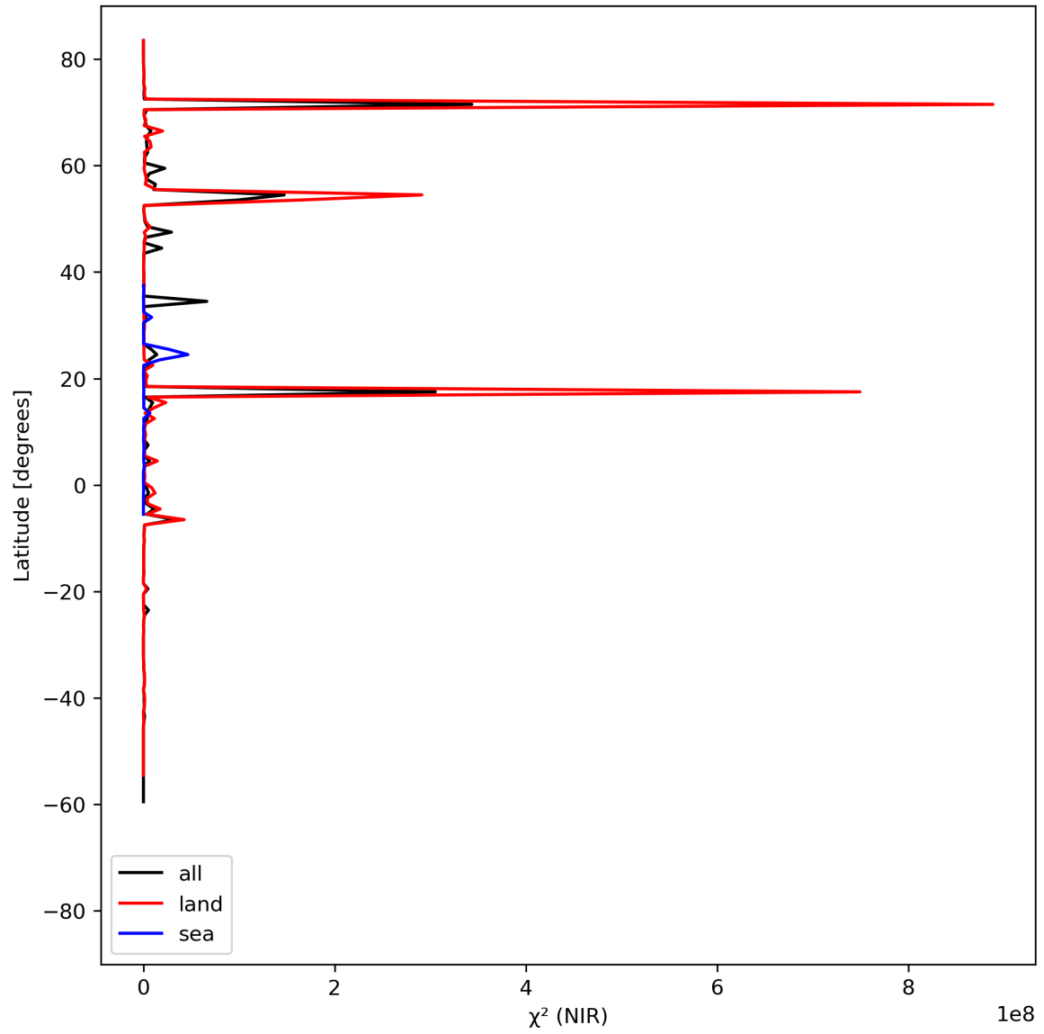
Figure 18: Zonal average of “ \chi^2 (NIR)” for 2023-08-27 to 2023-08-29.
