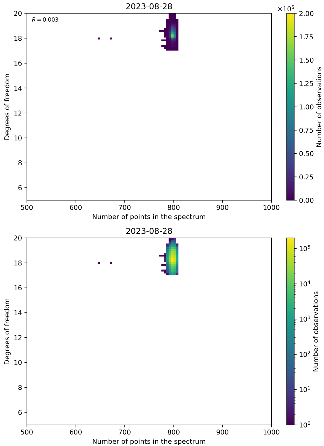
Figure 90: Scatter density plot of “Number of points in the spectrum” against “Degrees of freedom” for 2023-08-27 to 2023-08-29.
