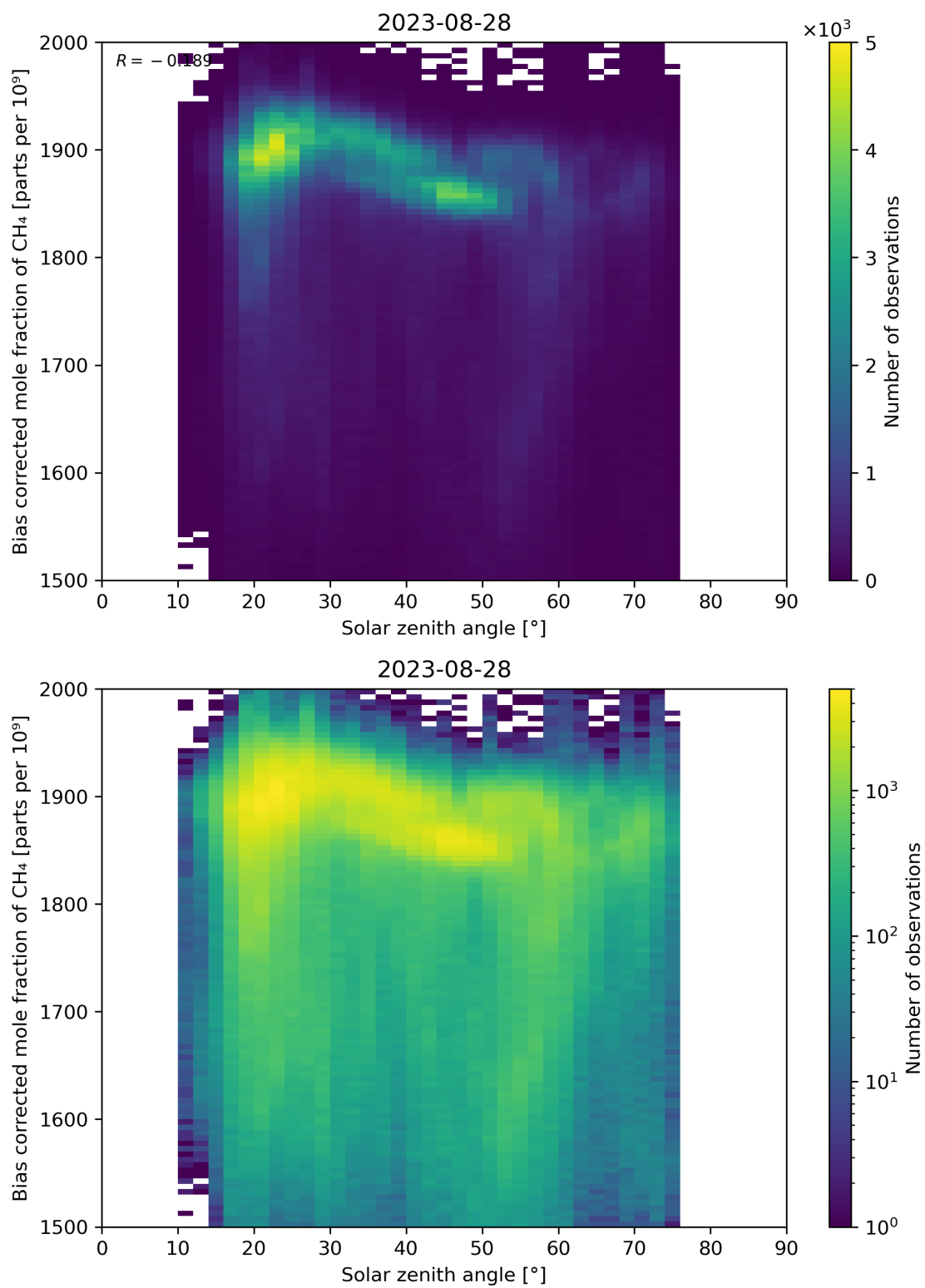
Figure 100: Scatter density plot of “Solar zenith angle” against “Bias corrected mole fraction of CH 4 ” for 2023-08-27 to 2023-08-29.
