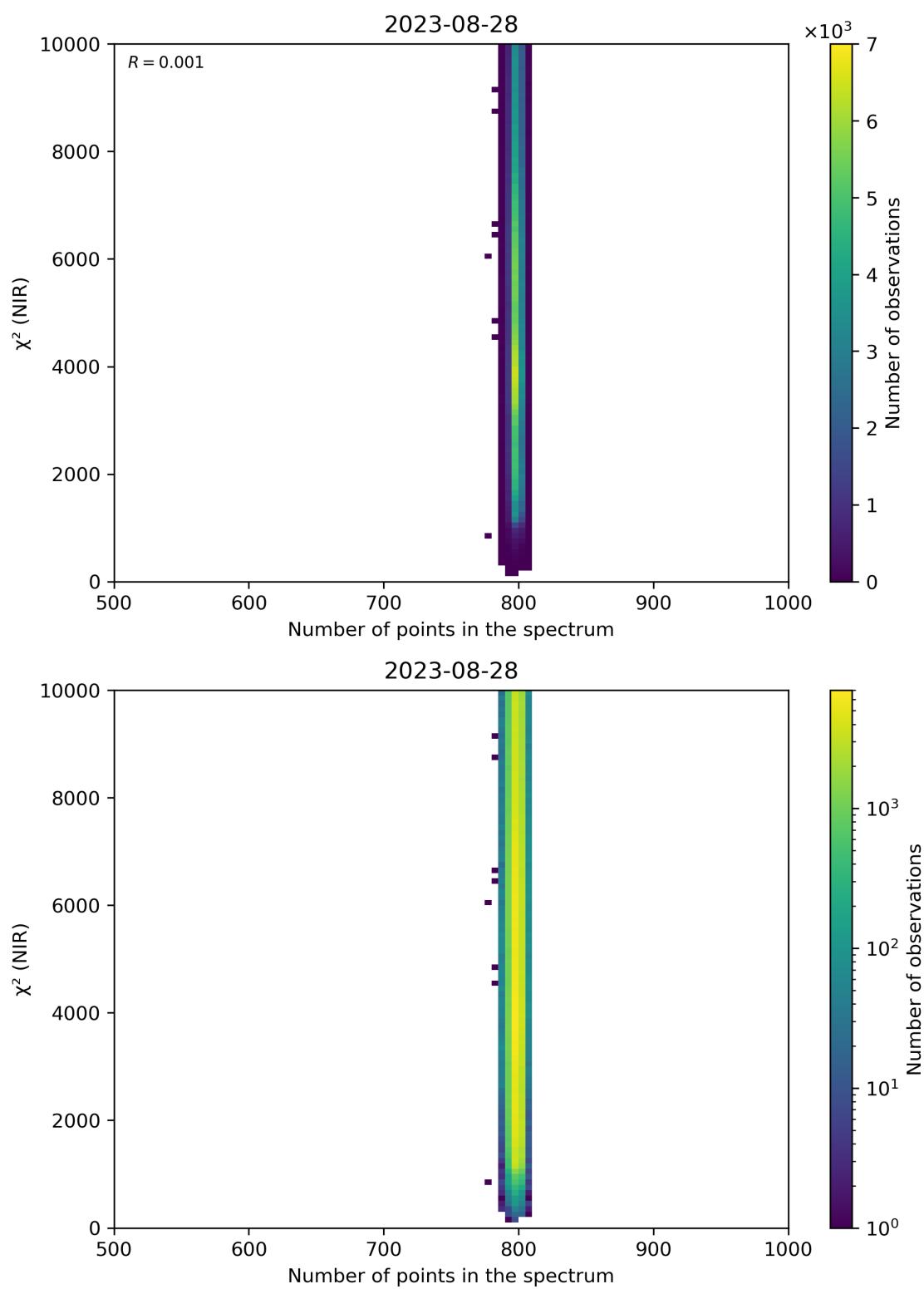
Figure 88: Scatter density plot of “Number of points in the spectrum” against “ \chi^2 (NIR)” for 2023-08-27 to 2023-08-29.
