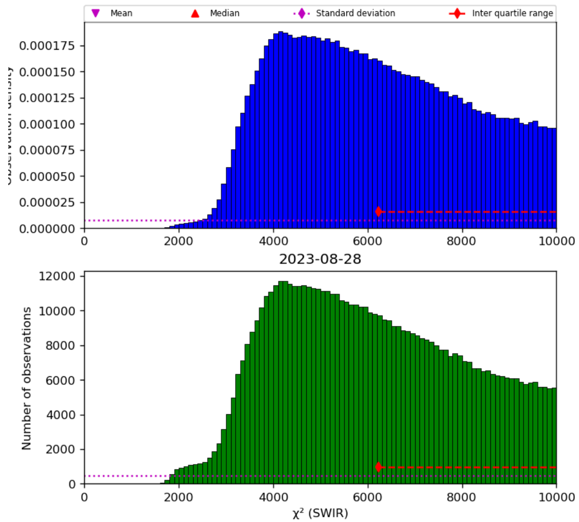
Figure 28: Histogram of “ \chi^2 (SWIR)” for 2023-08-27 to 2023-08-29
