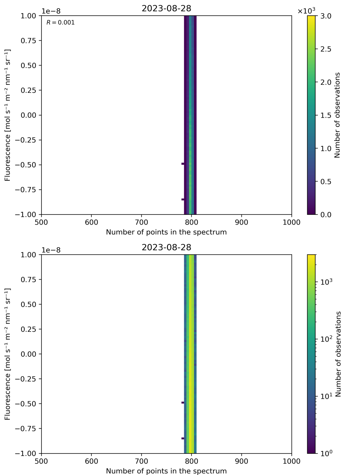
Figure 91: Scatter density plot of “Number of points in the spectrum” against “Fluorescence” for 2023-08-27 to 2023-08-29.
