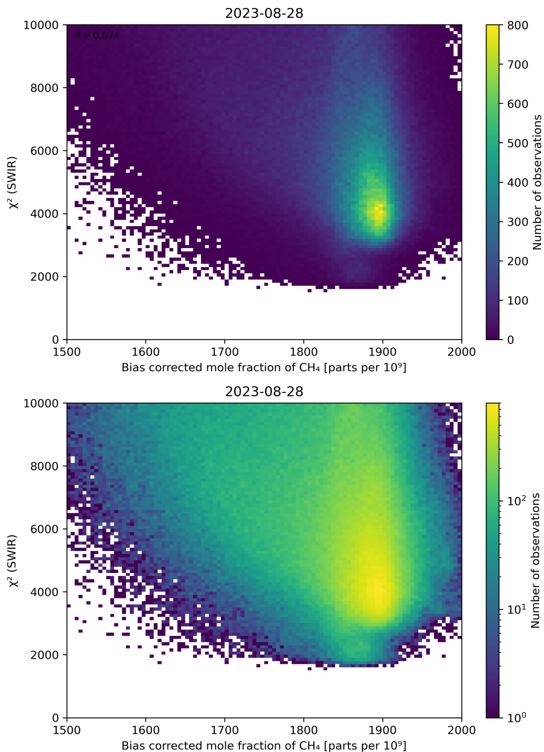
Figure 64: Scatter density plot of “Bias corrected mole fraction of CH 4 ” against “ \chi^2 (SWIR)” for 2023-08-27 to 2023-08-29.
