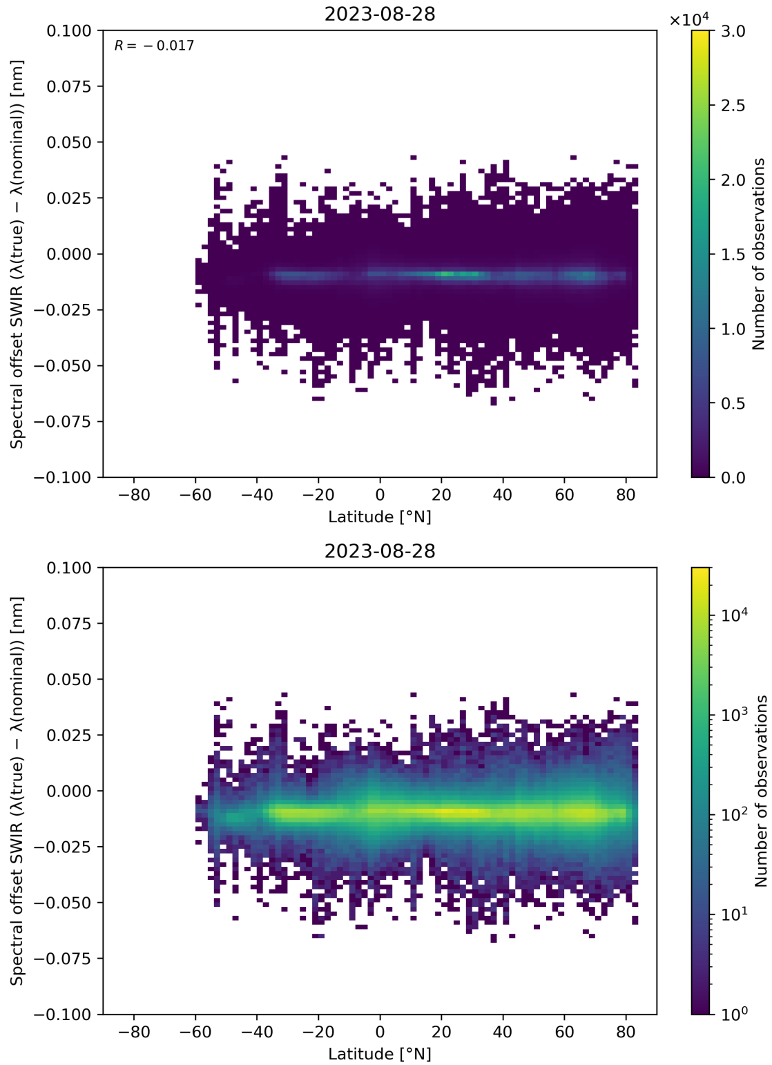
Figure 62: Scatter density plot of “Latitude” against “Spectral offset SWIR ( \lambda(\text{true}) - \lambda(\text{nominal}) )” for 2023-08-27 to 2023-08-29.
