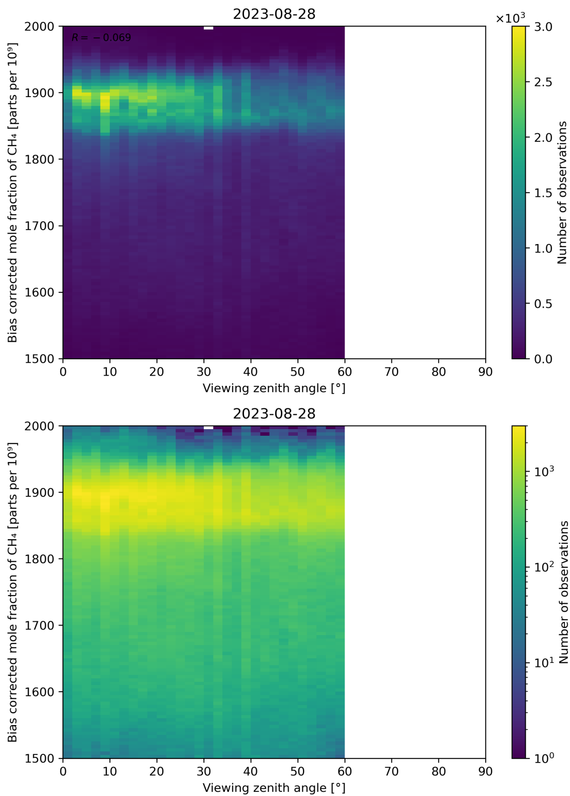
Figure 111: Scatter density plot of “Viewing zenith angle” against “Bias corrected mole fraction of CH 4 ” for 2023-08-27 to 2023-08-29.
