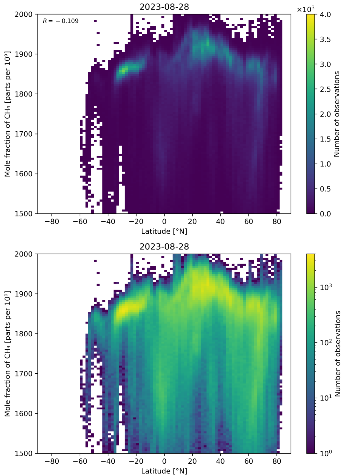
Figure 57: Scatter density plot of “Latitude” against “Mole fraction of CH 4 ” for 2023-08-27 to 2023-08-29.
