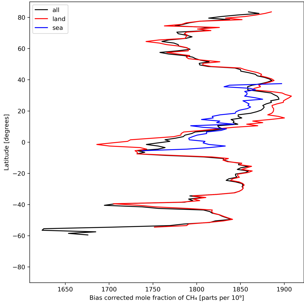
Figure 14: Zonal average of “Bias corrected mole fraction of \text{CH}_4 ” for 2023-08-27 to 2023-08-29.
