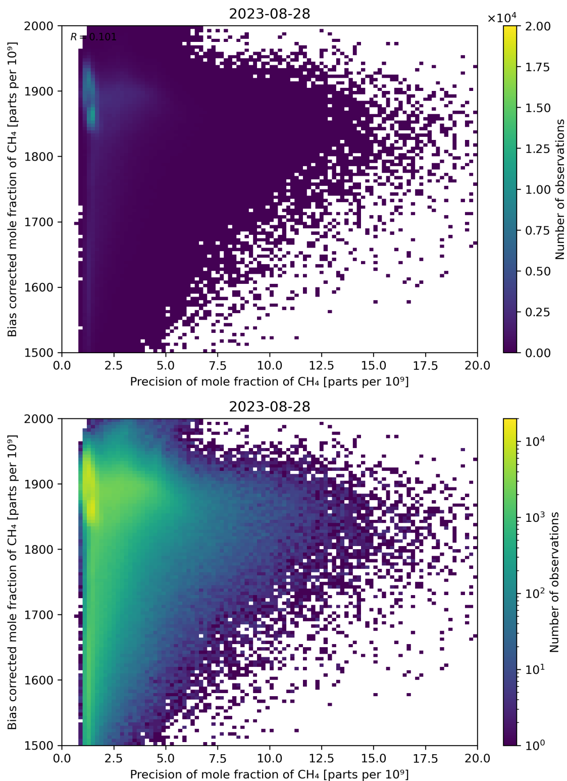
Figure 82: Scatter density plot of “Precision of mole fraction of CH 4 ” against “Bias corrected mole fraction of CH 4 ” for 2023-08-27 to 2023-08-29.
