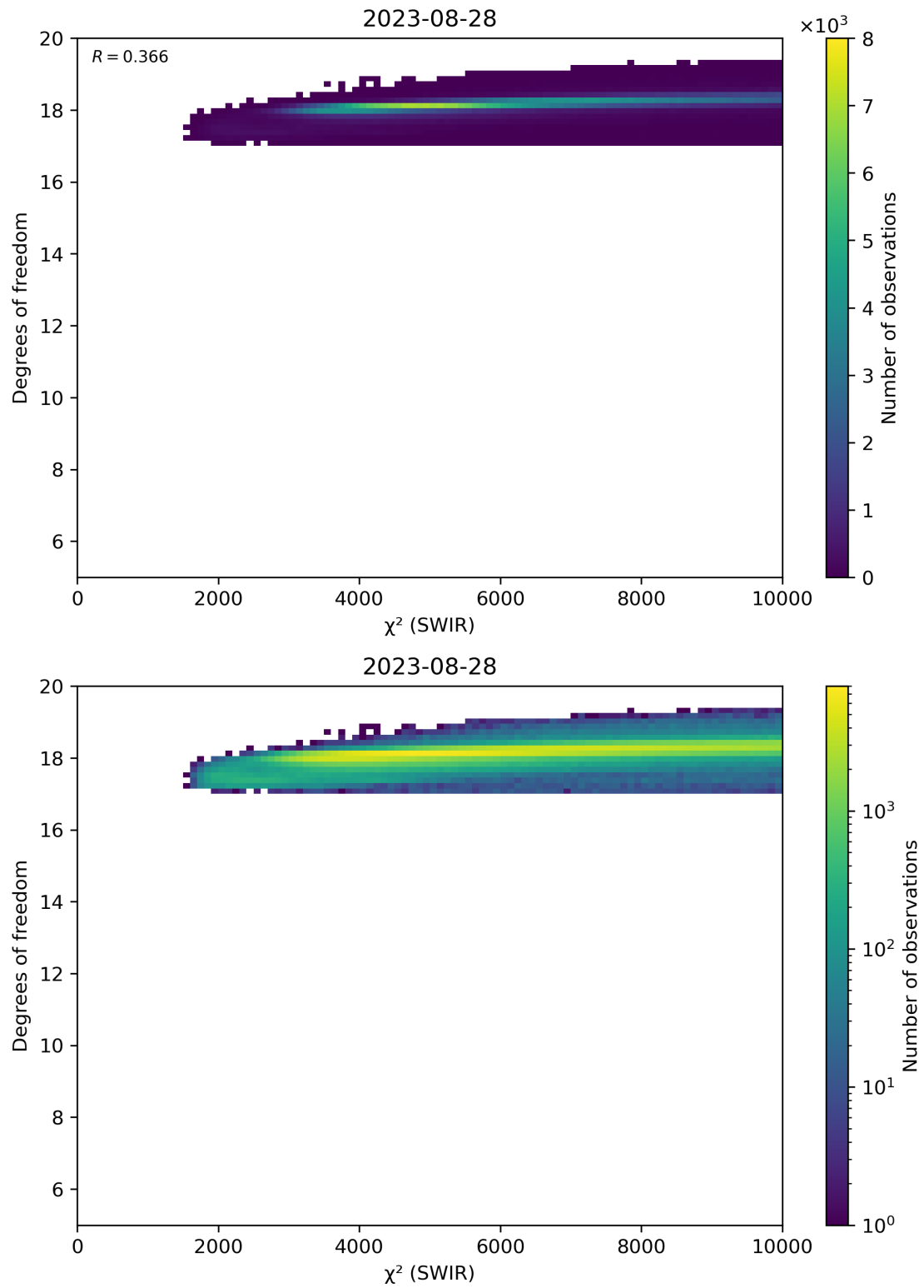
Figure 48: Scatter density plot of “ \chi^2 (SWIR)” against “Degrees of freedom” for 2023-08-27 to 2023-08-29.
