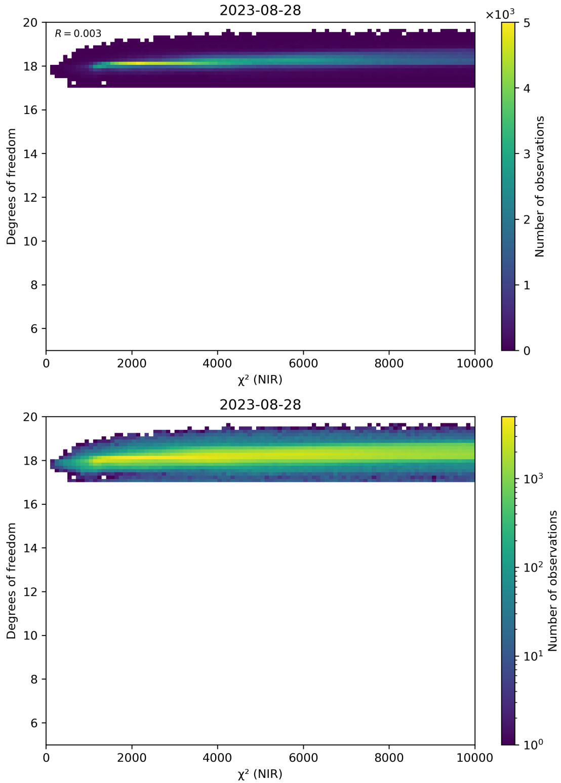
Figure 44: Scatter density plot of “ \chi^2 (NIR)” against “Degrees of freedom” for 2023-08-27 to 2023-08-29.
