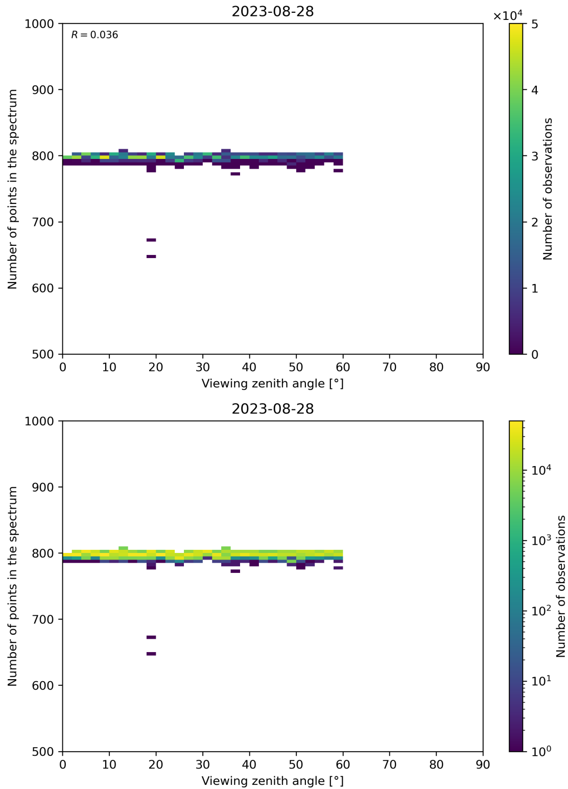
Figure 114: Scatter density plot of “Viewing zenith angle” against “Number of points in the spectrum” for 2023-08-27 to 2023-08-29.
