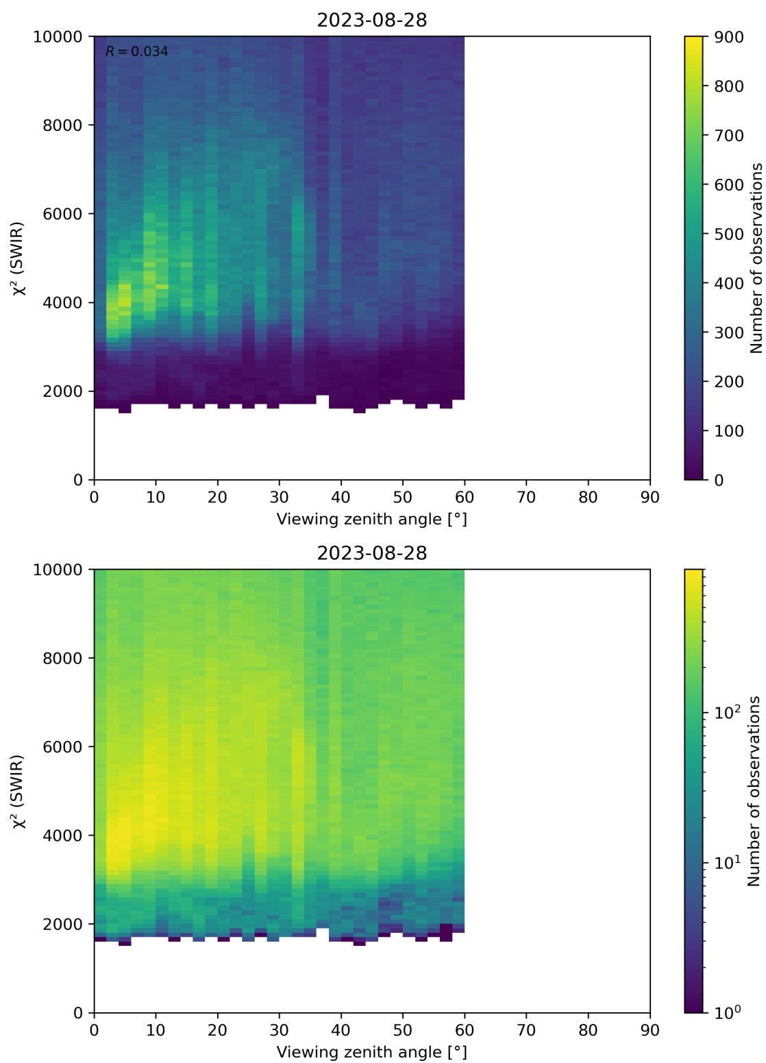
Figure 106: Scatter density plot of “Viewing zenith angle” against “ \chi^2 (SWIR)” for 2023-08-27 to 2023-08-29.
