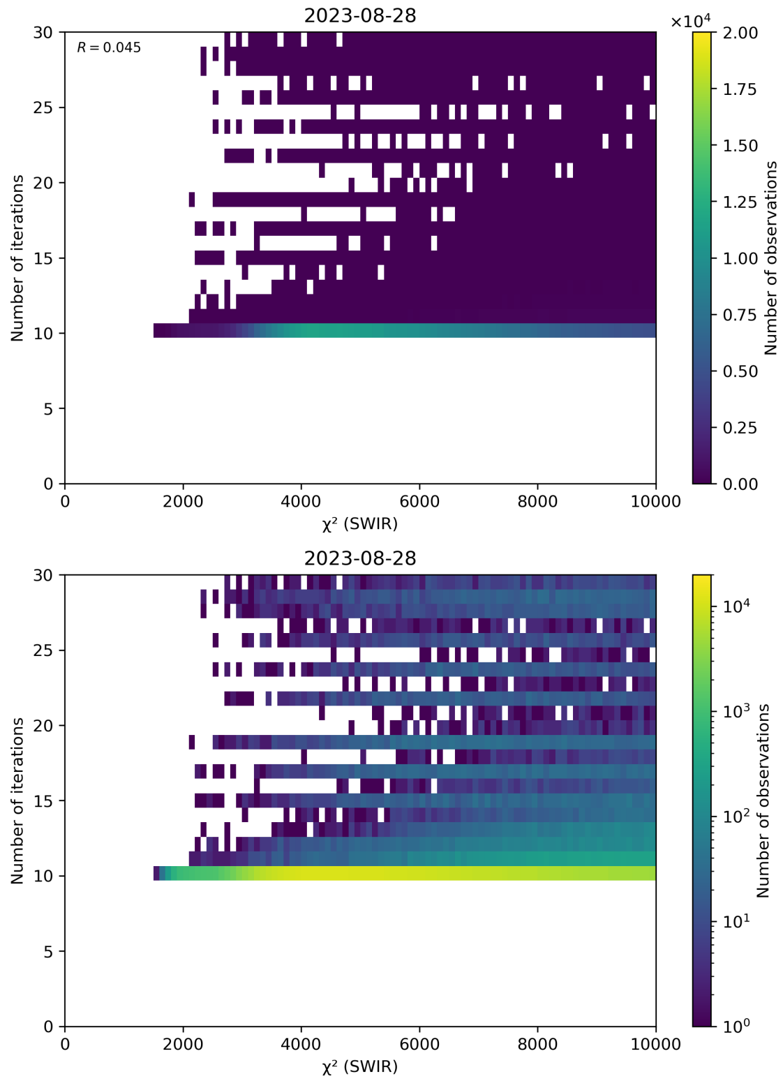
Figure 50: Scatter density plot of “ \chi^2 (SWIR)” against “Number of iterations” for 2023-08-27 to 2023-08-29.
