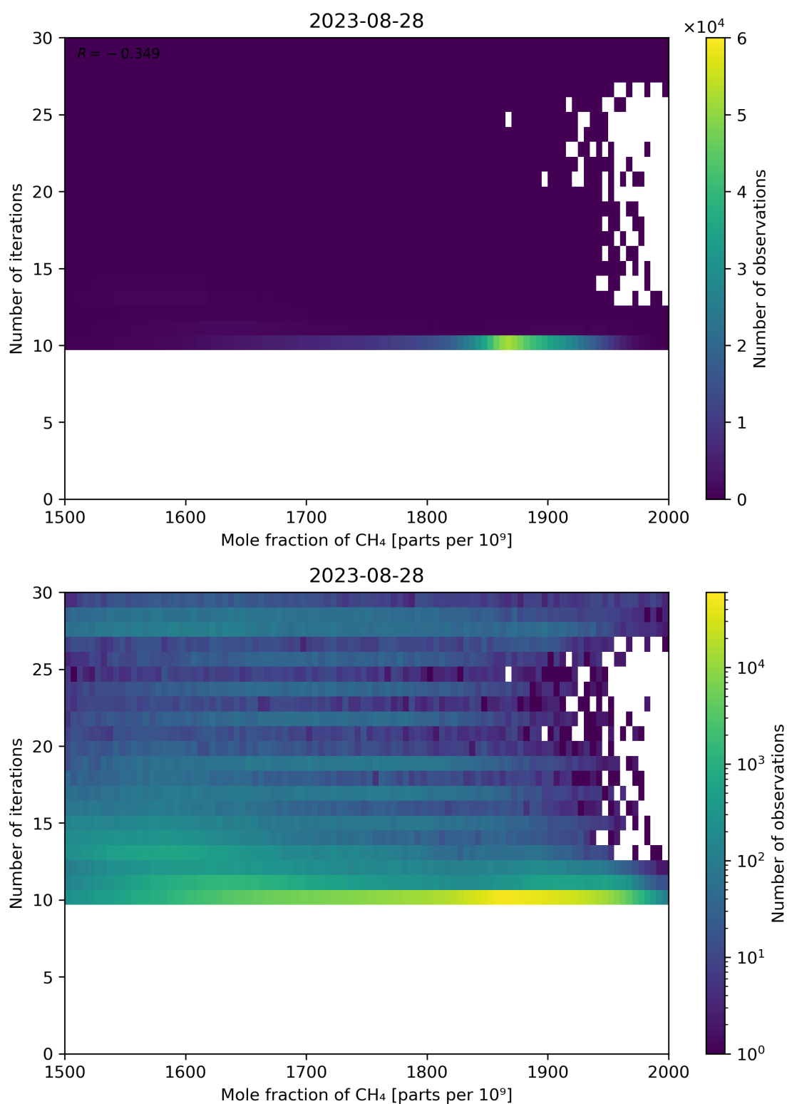
Figure 76: Scatter density plot of “Mole fraction of CH 4 ” against “Number of iterations” for 2023-08-27 to 2023-08-29.
