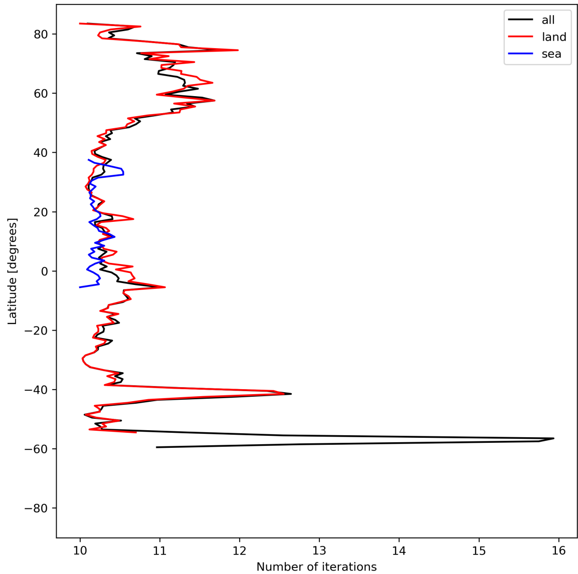
Figure 20: Zonal average of “Number of iterations” for 2023-08-27 to 2023-08-29.
