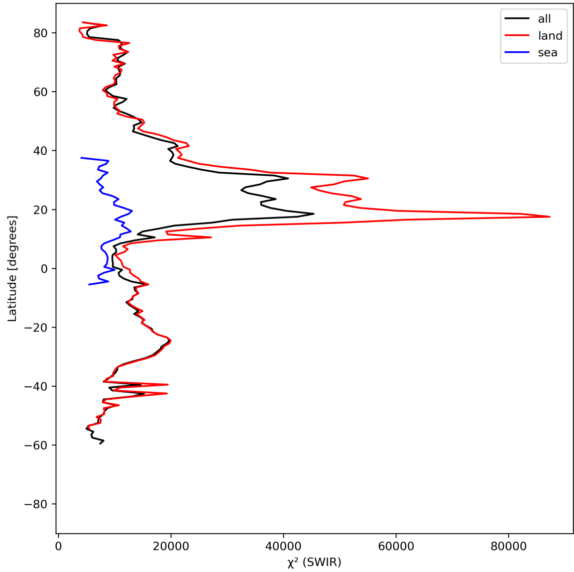
Figure 17: Zonal average of “ \chi^2 (SWIR)” for 2023-08-27 to 2023-08-29.
