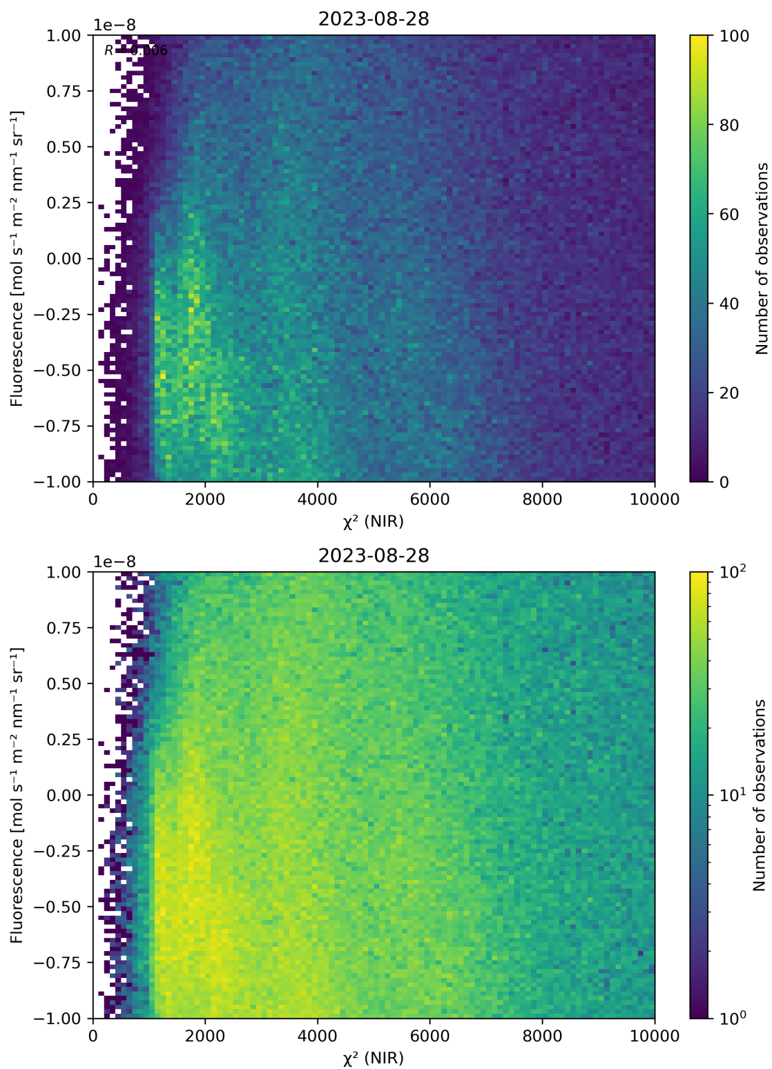
Figure 45: Scatter density plot of “ \chi^2 (NIR)” against “Fluorescence” for 2023-08-27 to 2023-08-29.
