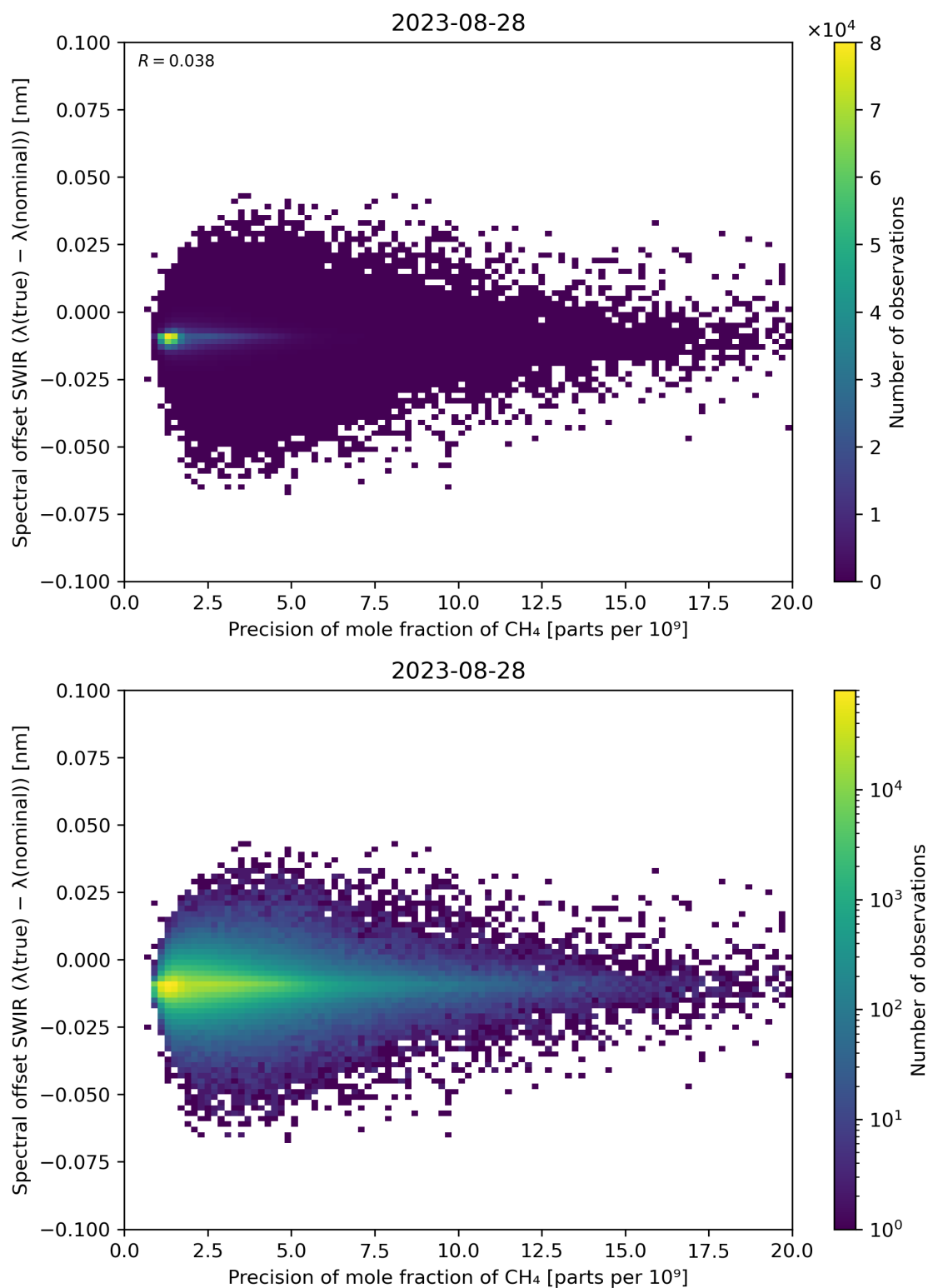
Figure 85: Scatter density plot of “Precision of mole fraction of CH 4 ” against “Spectral offset SWIR ( \lambda(\text{true}) - \lambda(\text{nominal}) )” for 2023-08-27 to 2023-08-29.
