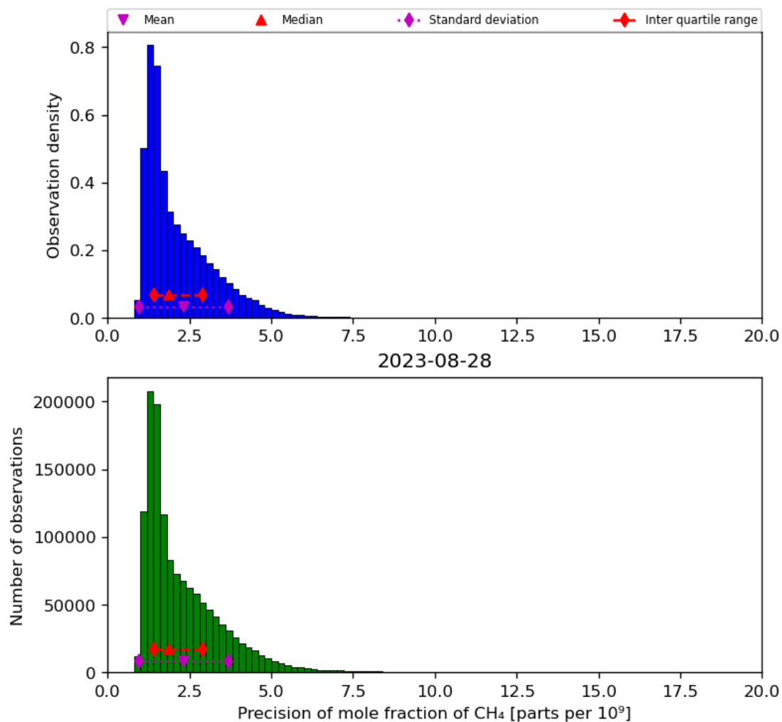
Figure 24: Histogram of “Precision of mole fraction of CH 4 ” for 2023-08-27 to 2023-08-29
