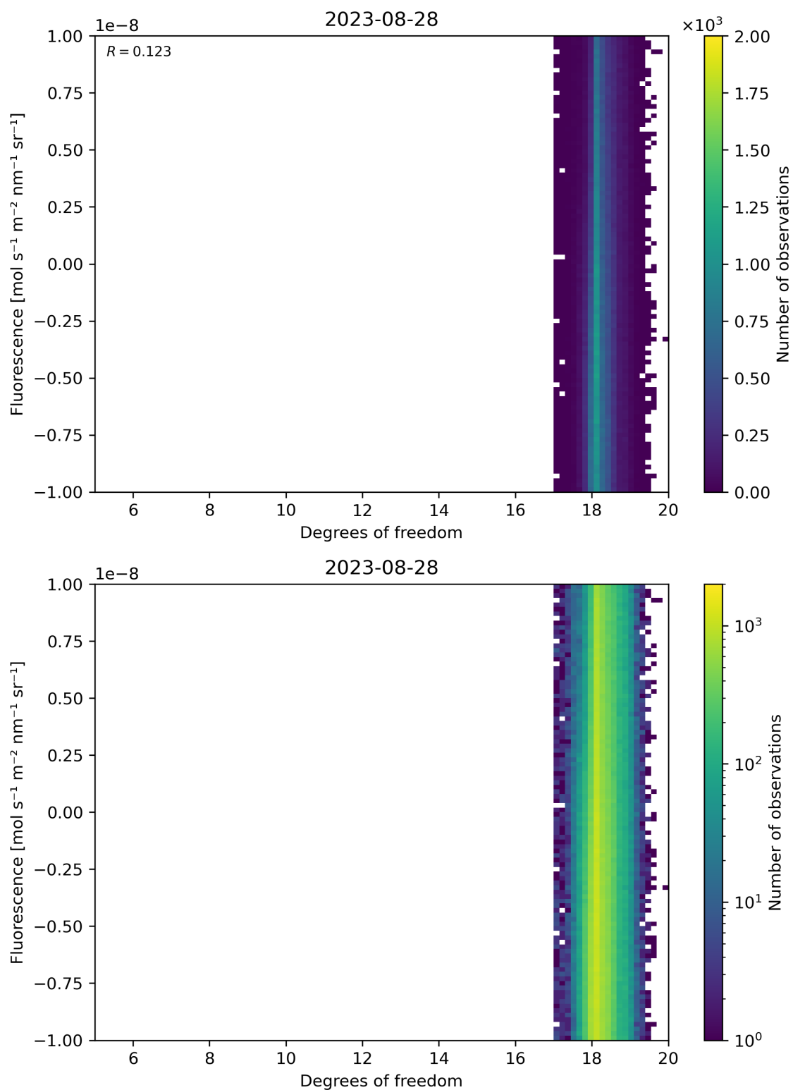
Figure 51: Scatter density plot of “Degrees of freedom” against “Fluorescence” for 2023-08-27 to 2023-08-29.
