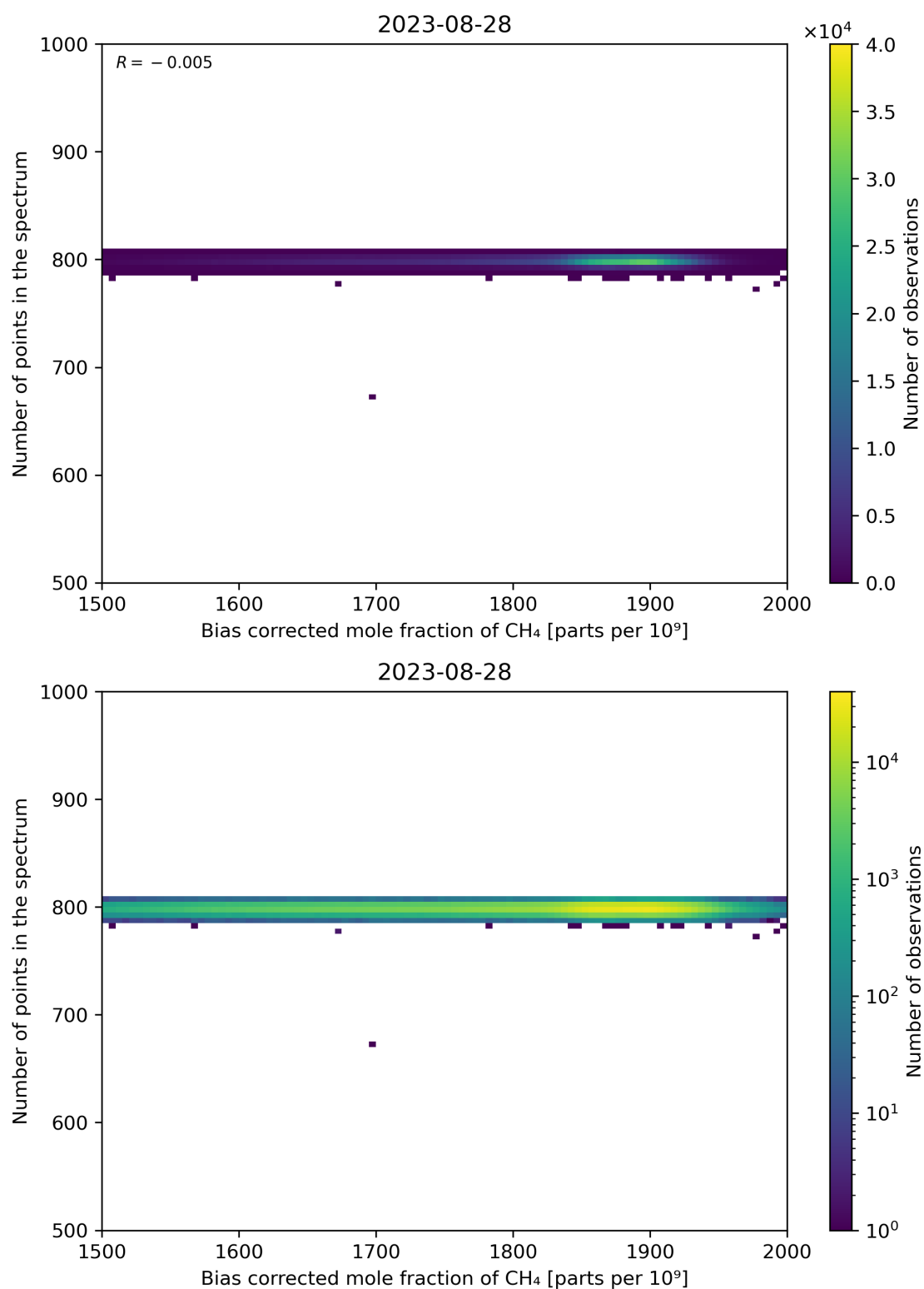
Figure 68: Scatter density plot of “Bias corrected mole fraction of CH 4 ” against “Number of points in the spectrum” for 2023-08-27 to 2023-08-29.
