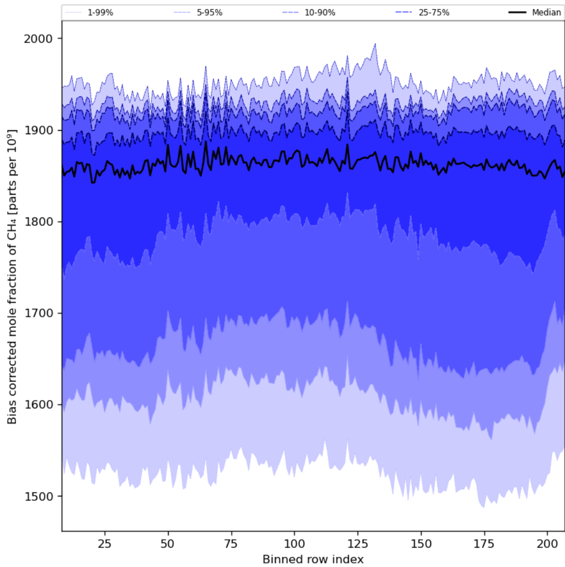
Figure 36: Along track statistics of “Bias corrected mole fraction of CH 4 ” for 2023-08-27 to 2023-08-29
