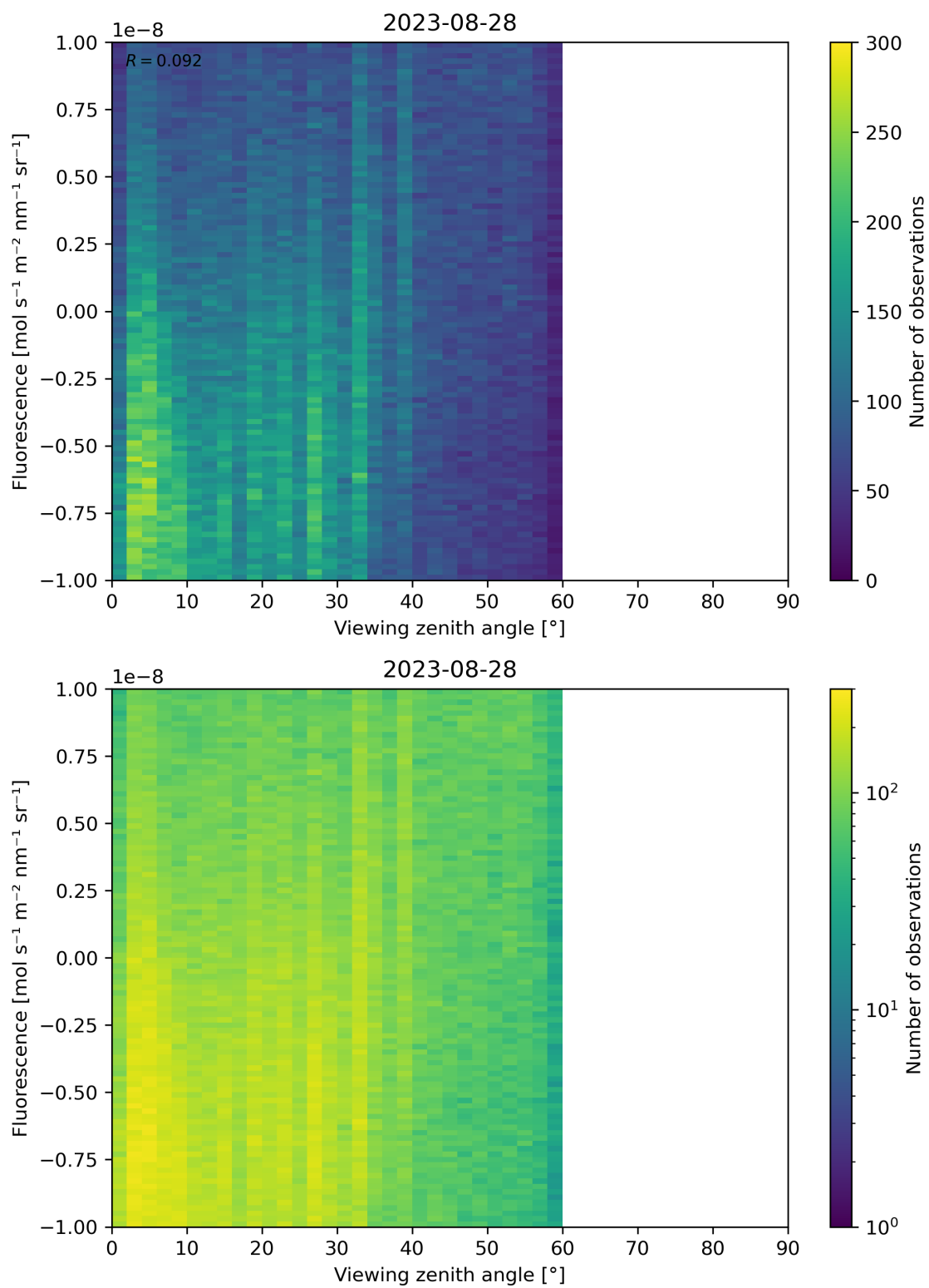
Figure 108: Scatter density plot of “Viewing zenith angle” against “Fluorescence” for 2023-08-27 to 2023-08-29.
