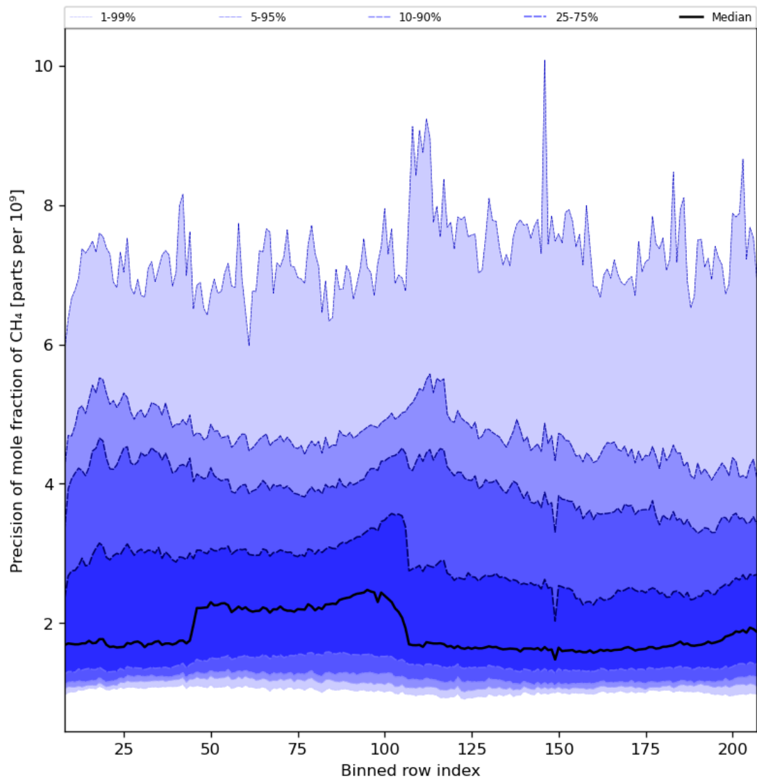
Figure 35: Along track statistics of “Precision of mole fraction of CH 4 ” for 2023-08-27 to 2023-08-29
