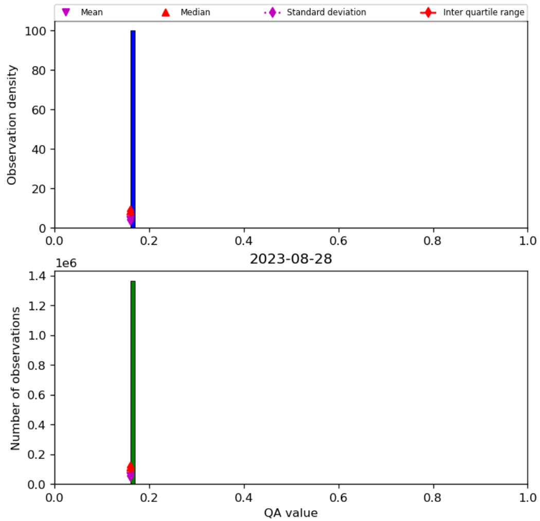
Figure 22: Histogram of “QA value” for 2023-08-27 to 2023-08-29
