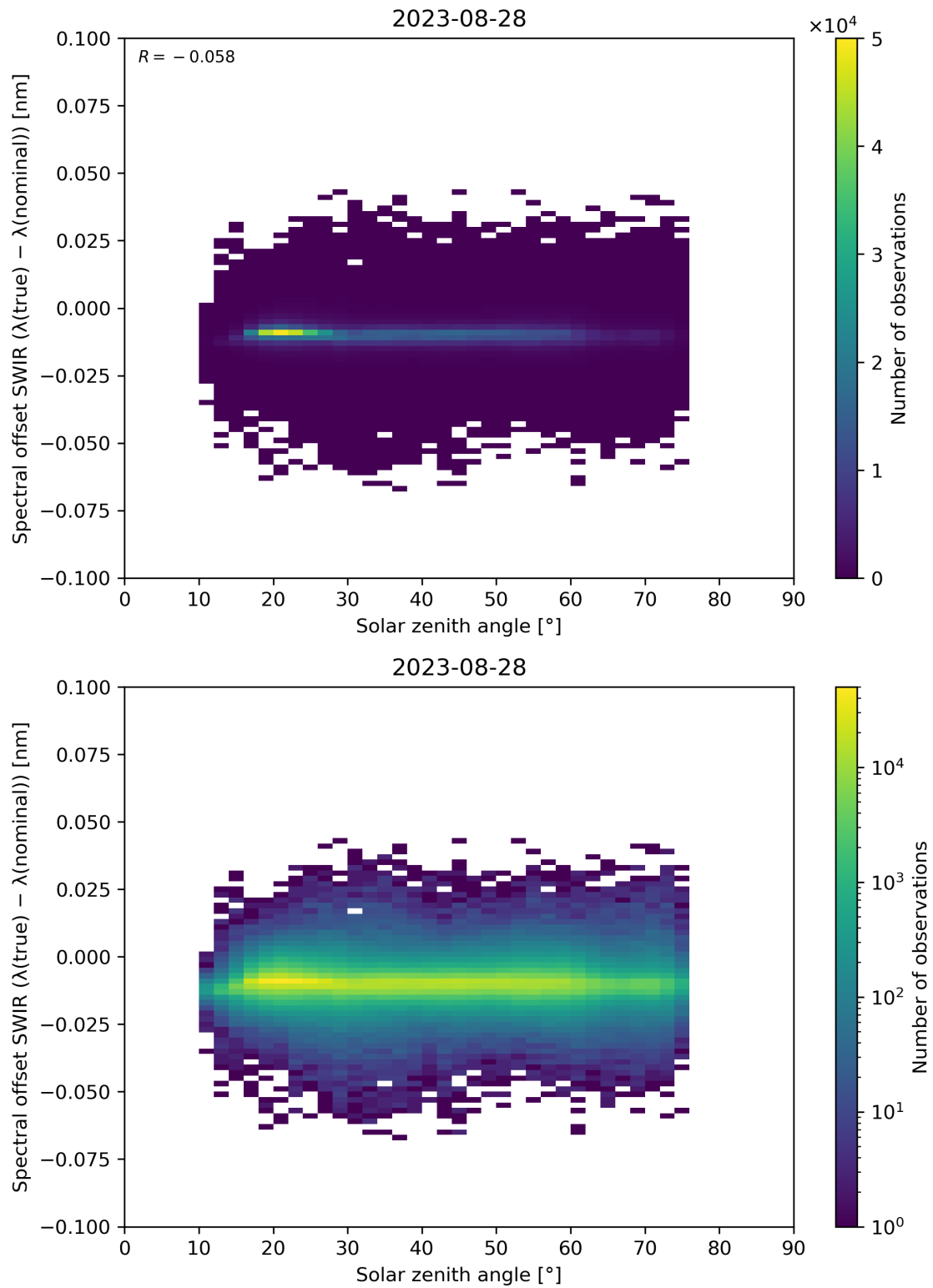
Figure 104: Scatter density plot of “Solar zenith angle” against “Spectral offset SWIR ( \lambda(\text{true}) - \lambda(\text{nominal}) )” for 2023-08-27 to 2023-08-29.
