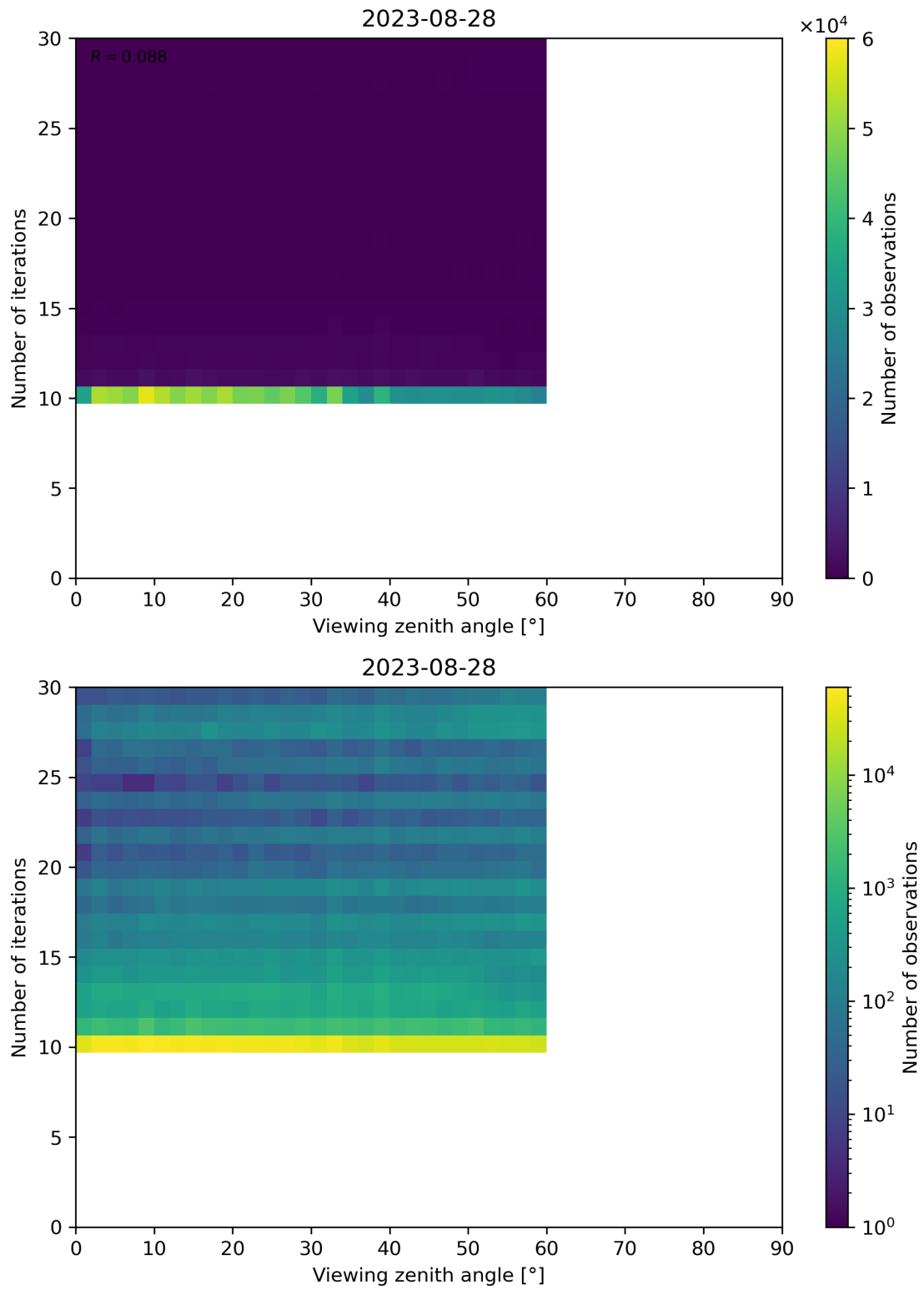
Figure 113: Scatter density plot of “Viewing zenith angle” against “Number of iterations” for 2023-08-27 to 2023-08-29.
