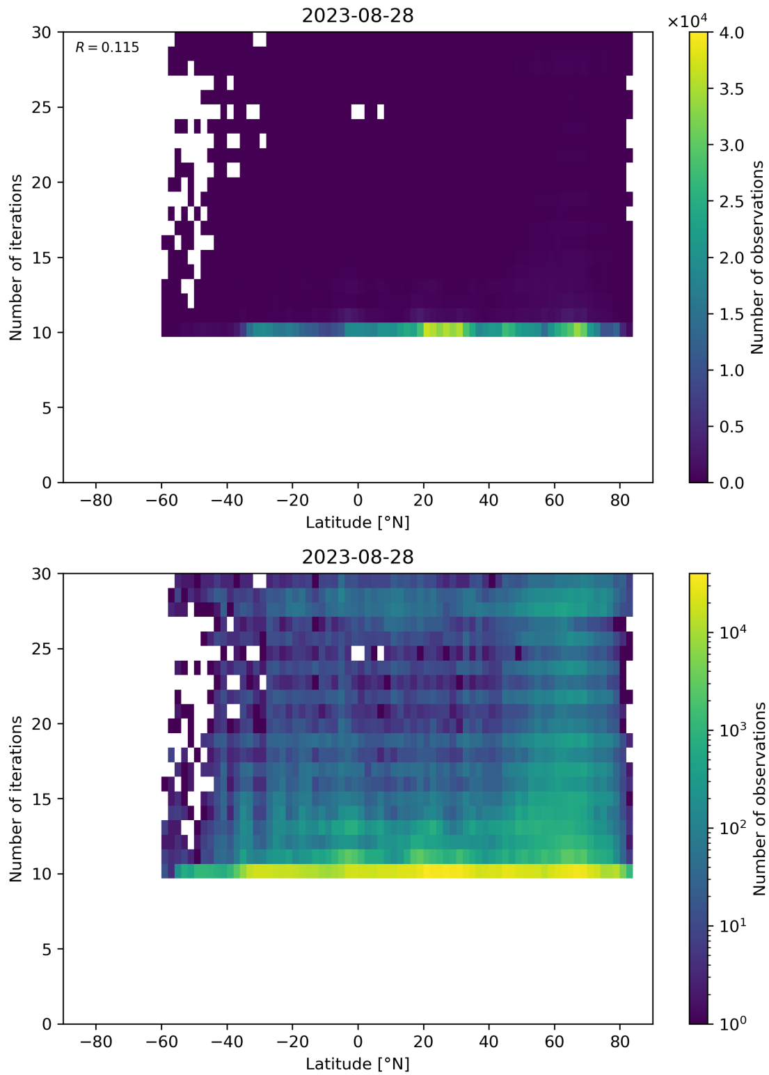
Figure 60: Scatter density plot of “Latitude” against “Number of iterations” for 2023-08-27 to 2023-08-29.
