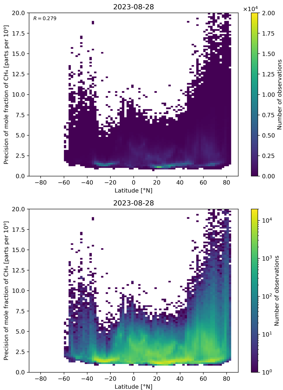
Figure 59: Scatter density plot of “Latitude” against “Precision of mole fraction of \text{CH}_4 ” for 2023-08-27 to 2023-08-29.
