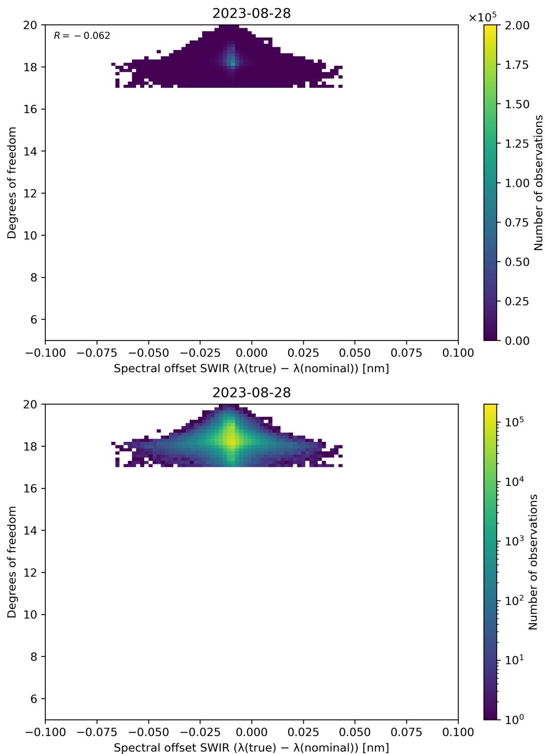
Figure 119: Scatter density plot of “Spectral offset SWIR ( \lambda(\text{true}) - \lambda(\text{nominal}) )” against “Degrees of freedom” for 2023-08-27 to 2023-08-29.
