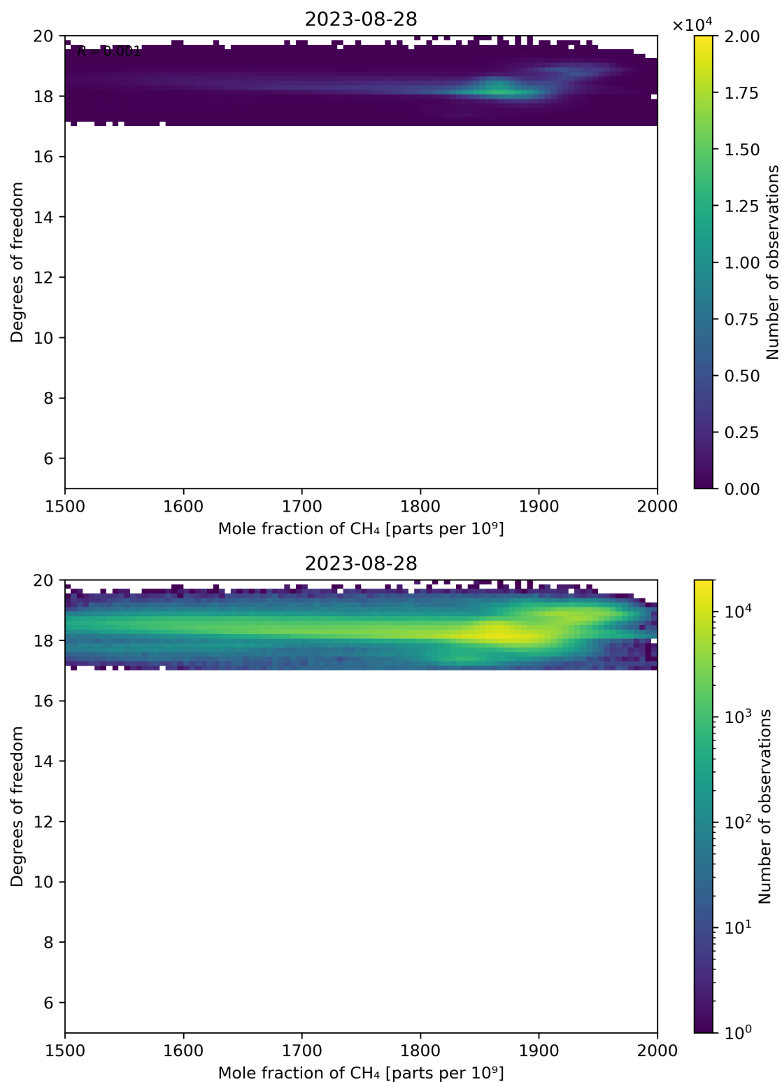
Figure 72: Scatter density plot of “Mole fraction of CH 4 ” against “Degrees of freedom” for 2023-08-27 to 2023-08-29.
