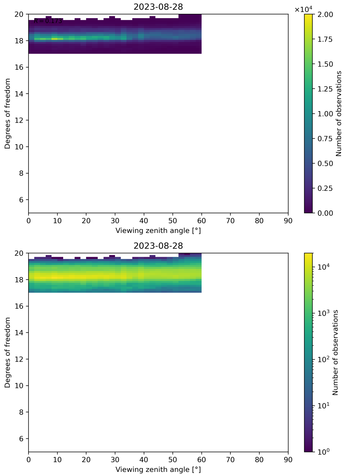
Figure 107: Scatter density plot of “Viewing zenith angle” against “Degrees of freedom” for 2023-08-27 to 2023-08-29.
