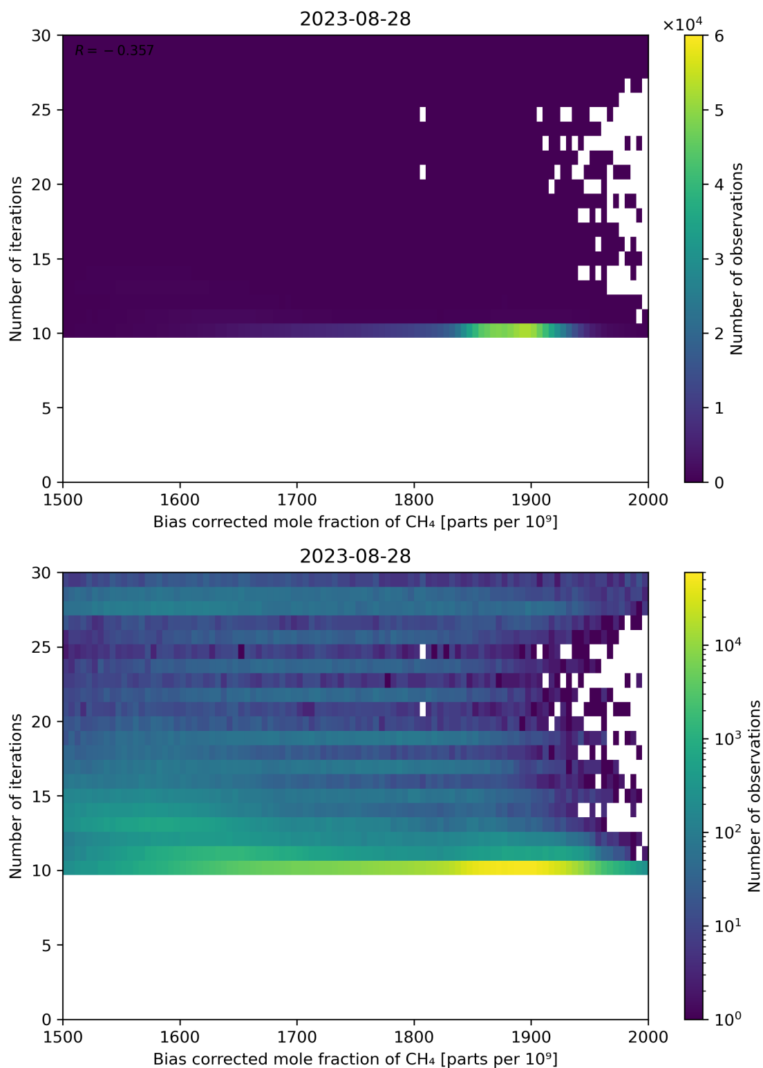
Figure 67: Scatter density plot of “Bias corrected mole fraction of CH 4 ” against “Number of iterations” for 2023-08-27 to 2023-08-29.
