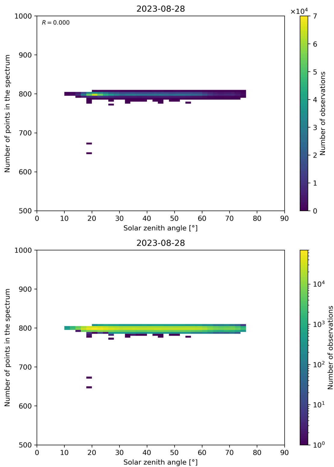
Figure 103: Scatter density plot of “Solar zenith angle” against “Number of points in the spectrum” for 2023-08-27 to 2023-08-29.
