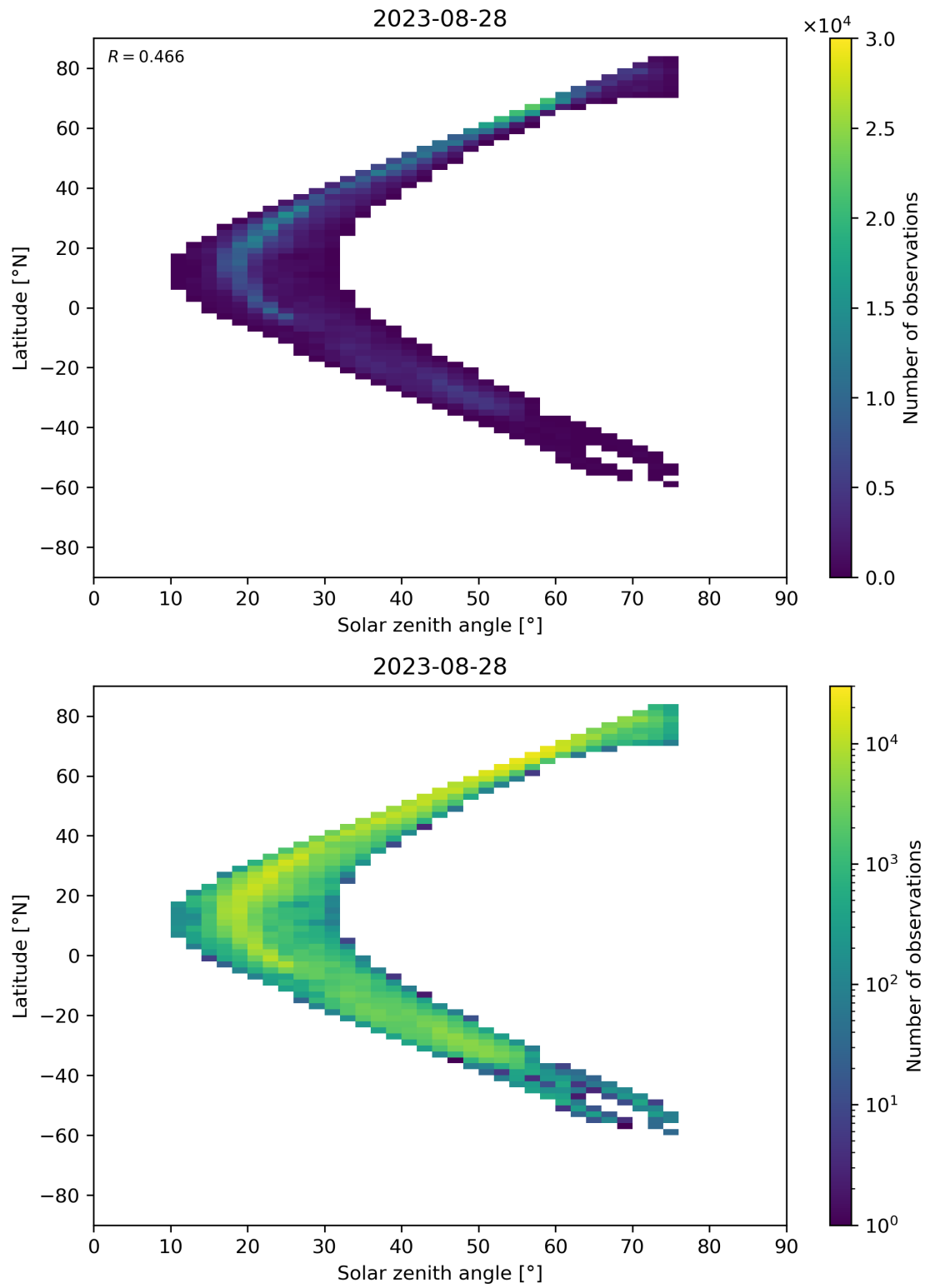
Figure 98: Scatter density plot of “Solar zenith angle” against “Latitude” for 2023-08-27 to 2023-08-29.
