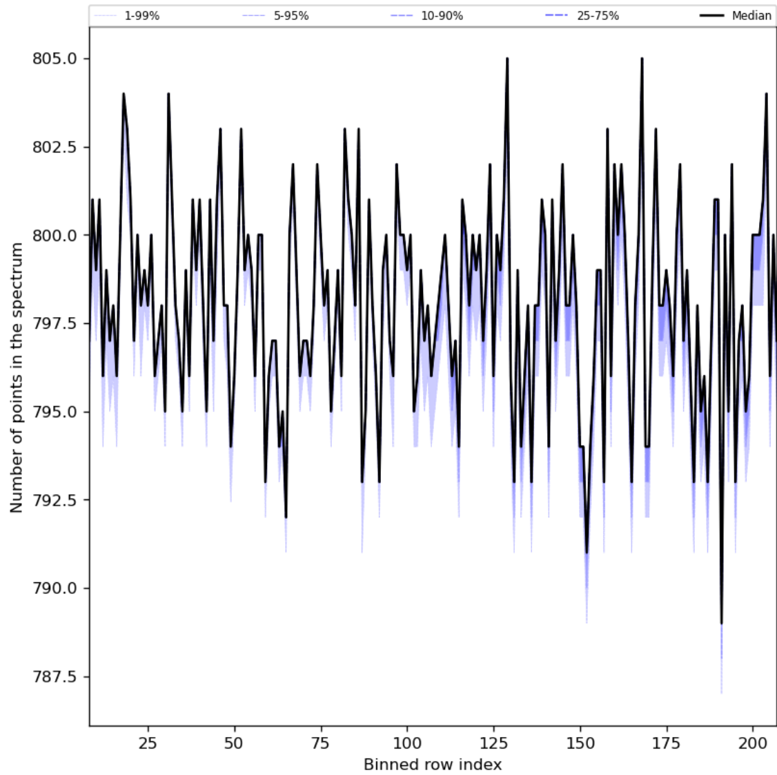
Figure 37: Along track statistics of “Number of points in the spectrum” for 2023-08-27 to 2023-08-29
