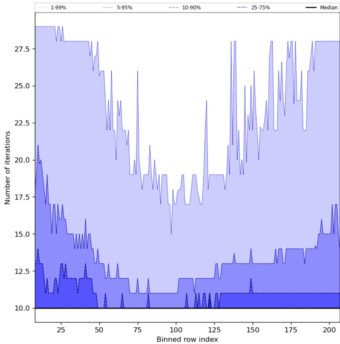
Figure 42: Along track statistics of “Number of iterations” for 2023-08-27 to 2023-08-29
