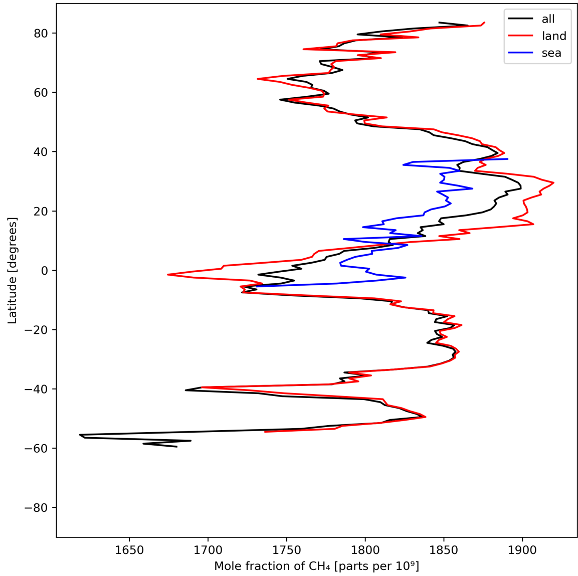
Figure 12: Zonal average of “Mole fraction of \text{CH}_4 ” for 2023-08-27 to 2023-08-29.
