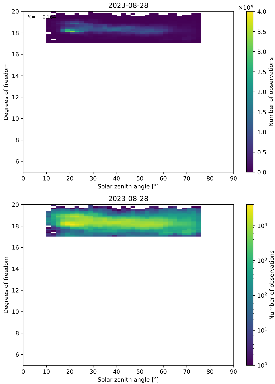
Figure 96: Scatter density plot of “Solar zenith angle” against “Degrees of freedom” for 2023-08-27 to 2023-08-29.
