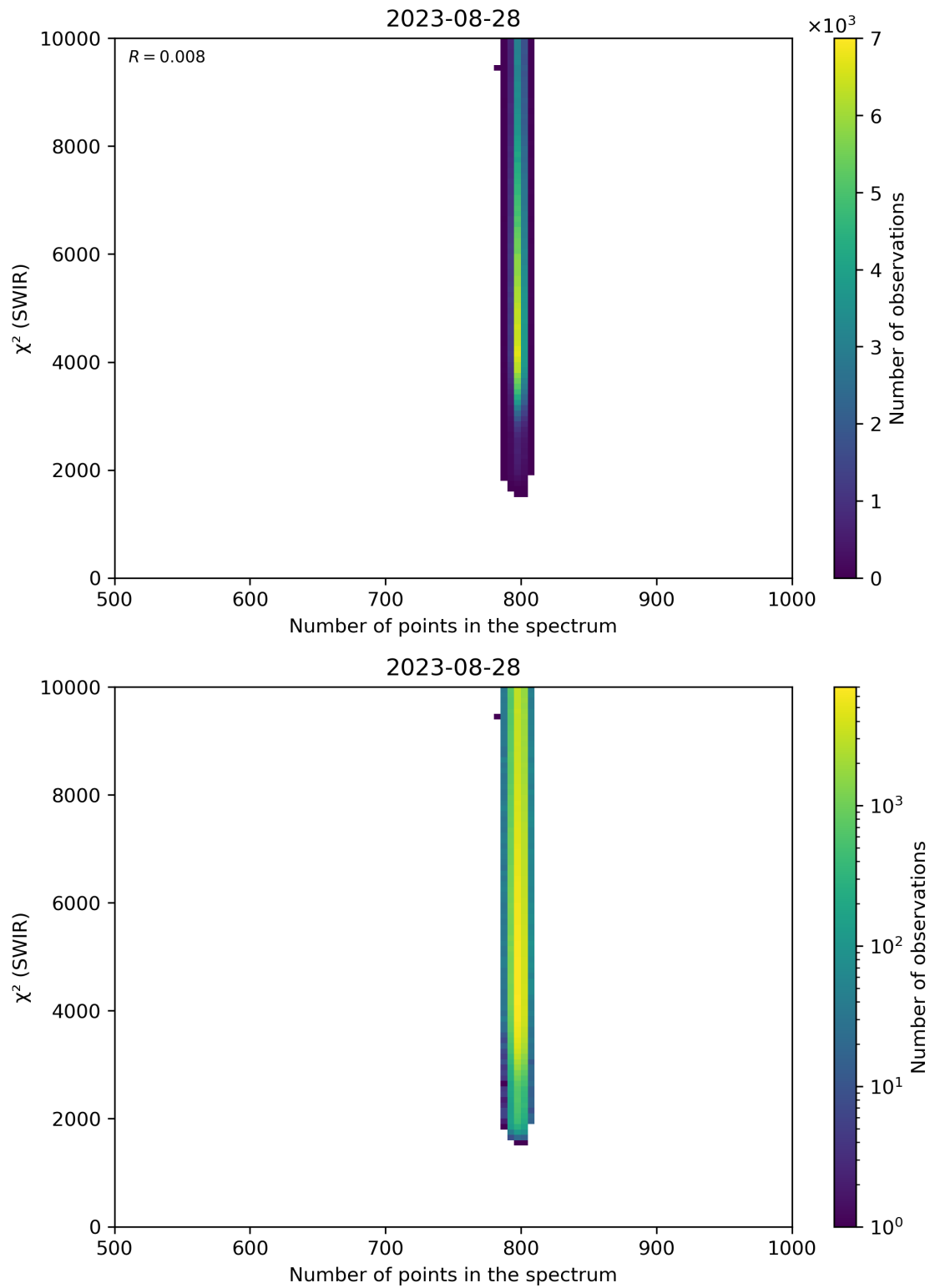
Figure 89: Scatter density plot of “Number of points in the spectrum” against “ \chi^2 (SWIR)” for 2023-08-27 to 2023-08-29.
