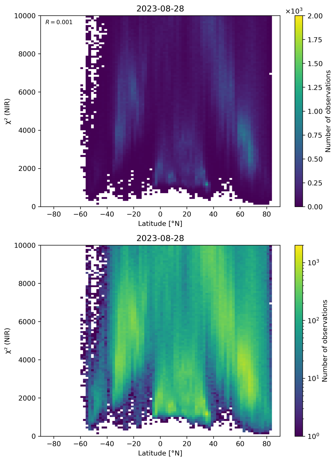
Figure 53: Scatter density plot of “Latitude” against “ \chi^2 (NIR)” for 2023-08-27 to 2023-08-29.
