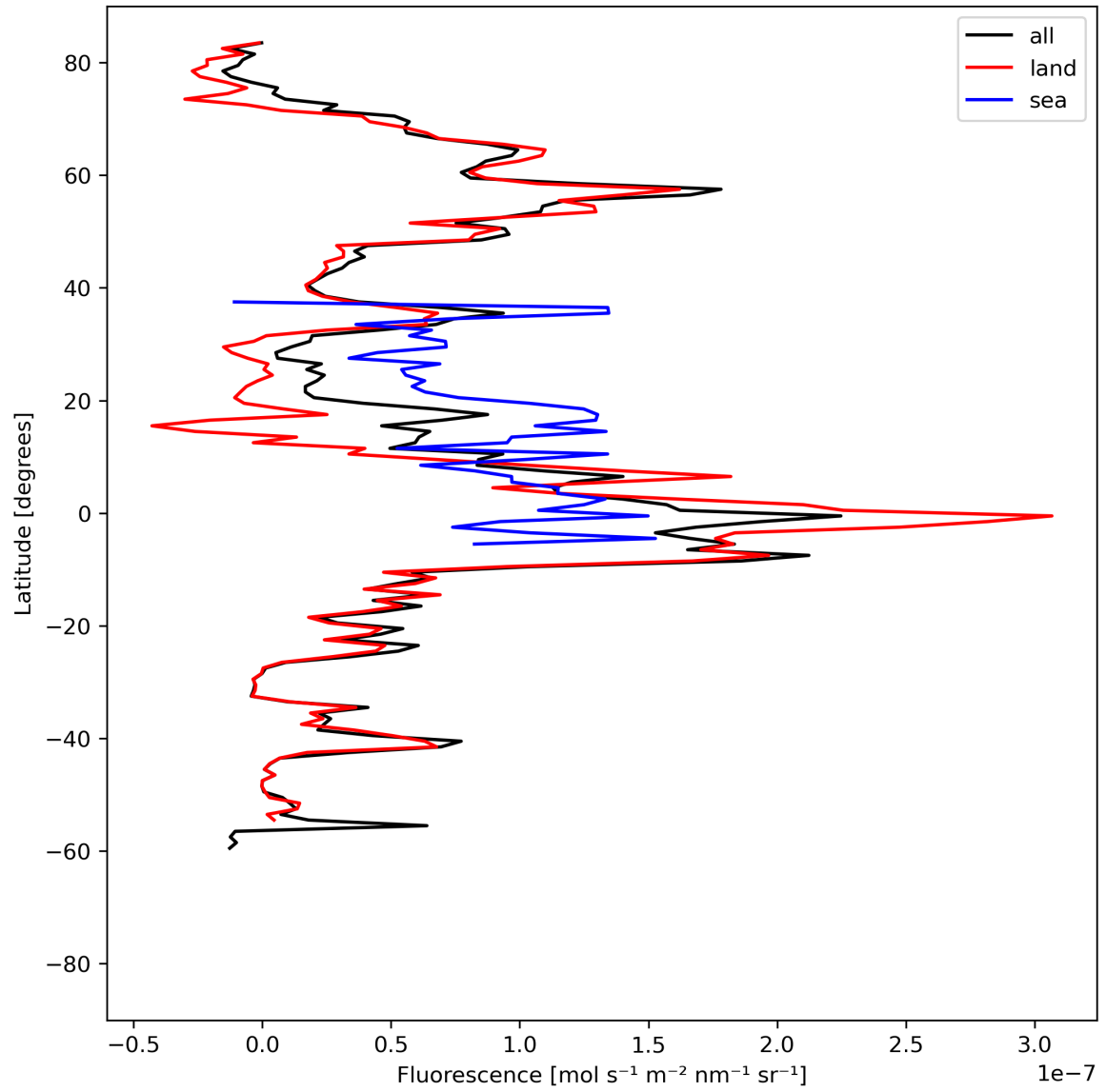
Figure 21: Zonal average of “Fluorescence” for 2023-08-27 to 2023-08-29.
