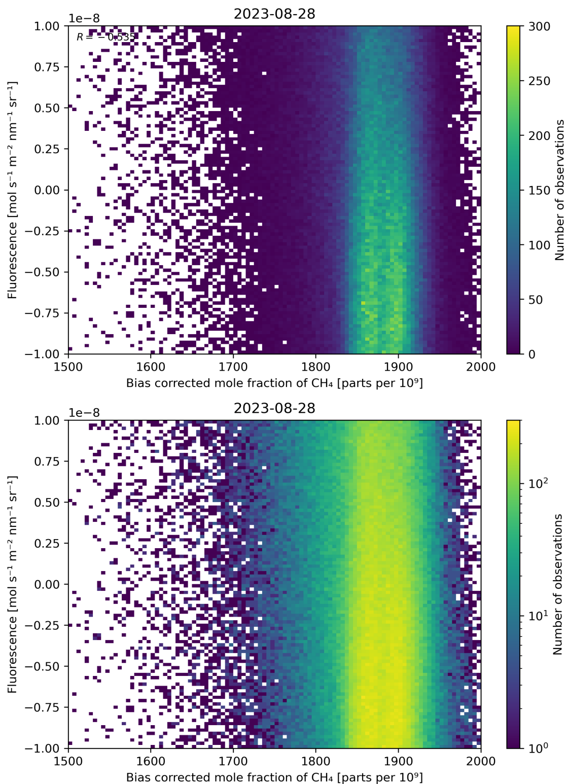
Figure 66: Scatter density plot of “Bias corrected mole fraction of \text{CH}_4 ” against “Fluorescence” for 2023-08-27 to 2023-08-29.
