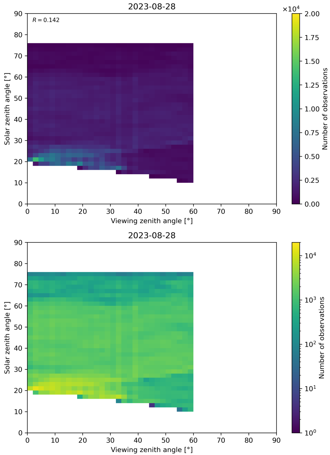
Figure 115: Scatter density plot of “Viewing zenith angle” against “Solar zenith angle” for 2023-08-27 to 2023-08-29.
