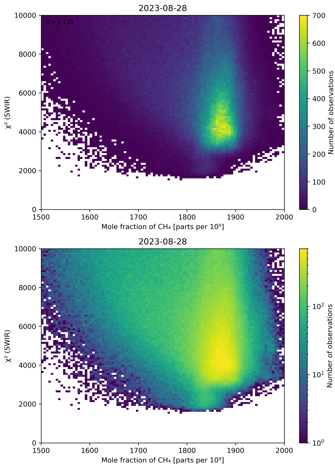
Figure 71: Scatter density plot of “Mole fraction of \text{CH}_4 ” against “ \chi^2 (SWIR)” for 2023-08-27 to 2023-08-29.
