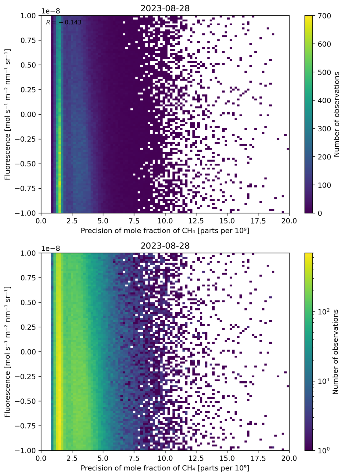
Figure 81: Scatter density plot of “Precision of mole fraction of CH 4 ” against “Fluorescence” for 2023-08-27 to 2023-08-29.
