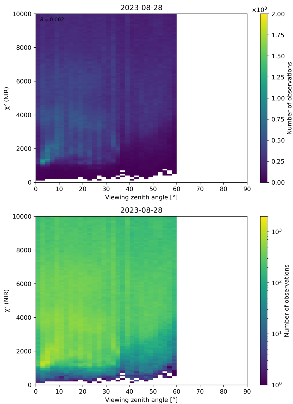
Figure 105: Scatter density plot of “Viewing zenith angle” against “ \chi^2 (NIR)” for 2023-08-27 to 2023-08-29.
