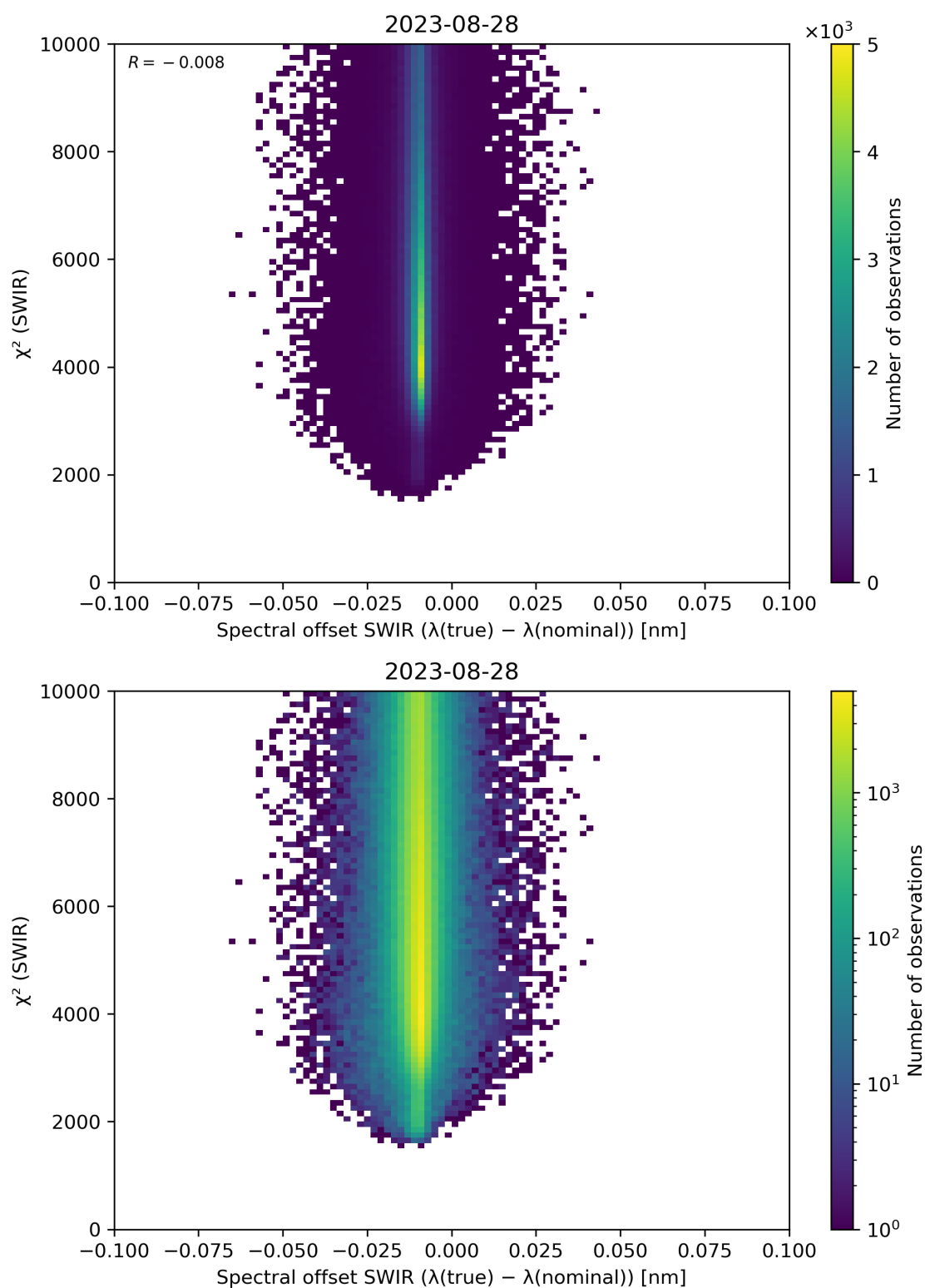
Figure 118: Scatter density plot of “Spectral offset SWIR ( \lambda(\text{true}) - \lambda(\text{nominal}) )” against “ \chi^2 (SWIR)” for 2023-08-27 to 2023-08-29.
