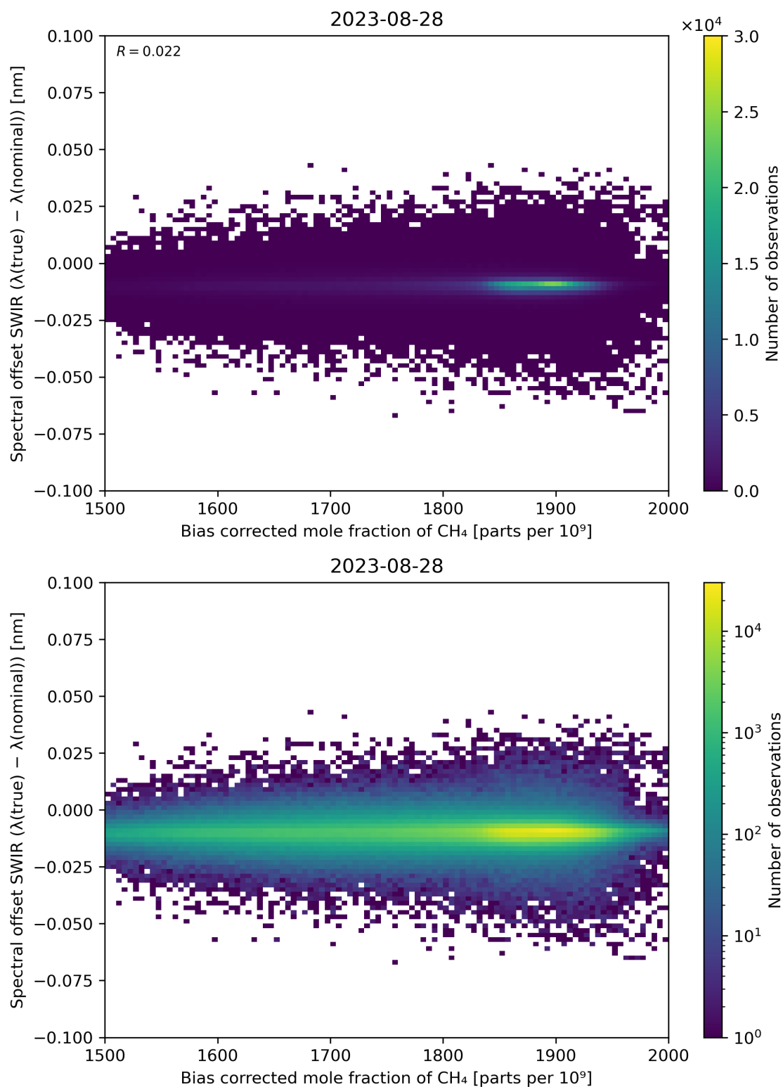
Figure 69: Scatter density plot of “Bias corrected mole fraction of \text{CH}_4 ” against “Spectral offset SWIR ( \lambda(\text{true}) - \lambda(\text{nominal}) )” for 2023-08-27 to 2023-08-29.
