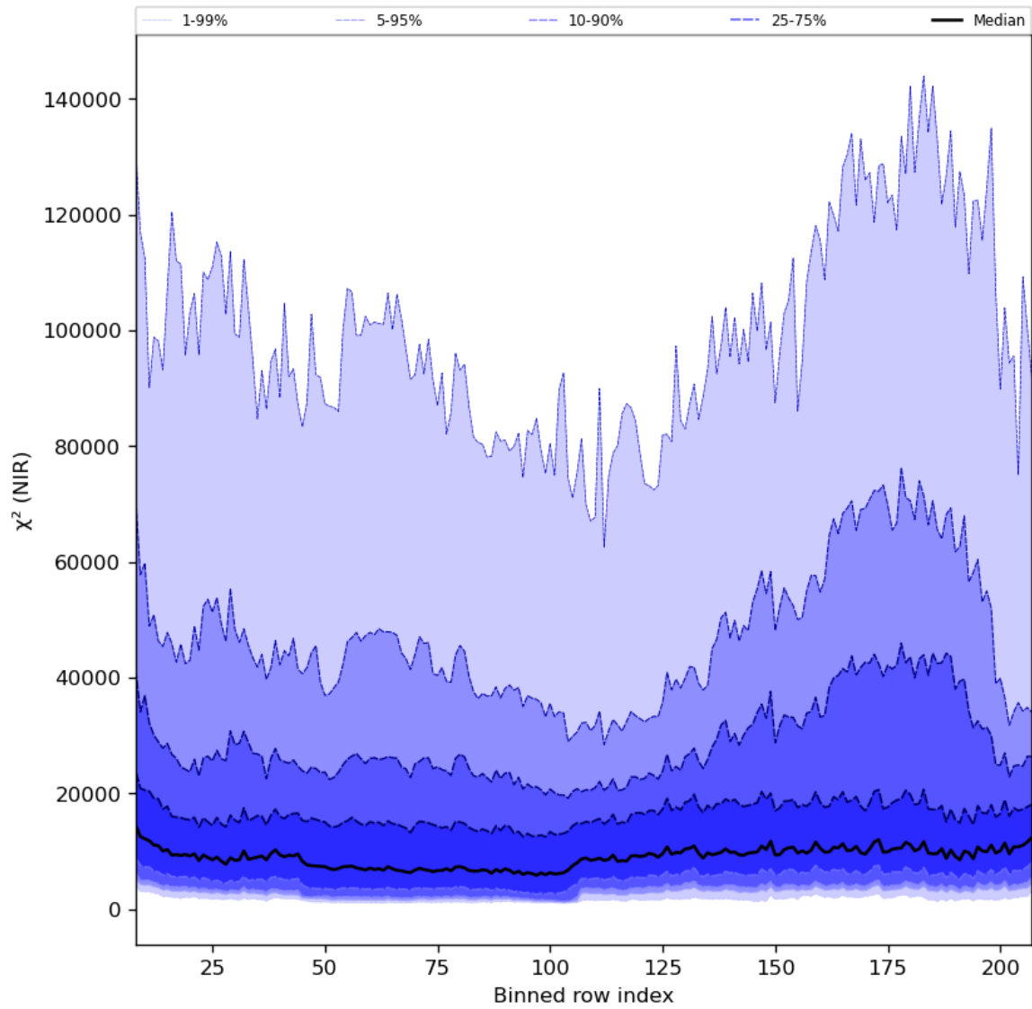
Figure 40: Along track statistics of " \chi^2 (NIR)" for 2023-08-27 to 2023-08-29
