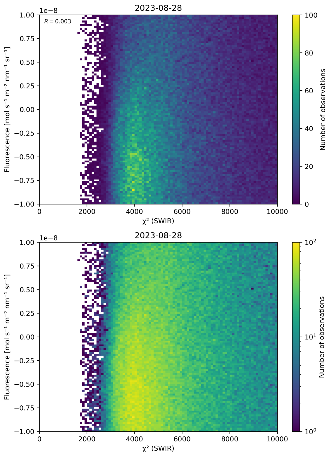
Figure 49: Scatter density plot of “ \chi^2 (SWIR)” against “Fluorescence” for 2023-08-27 to 2023-08-29.
