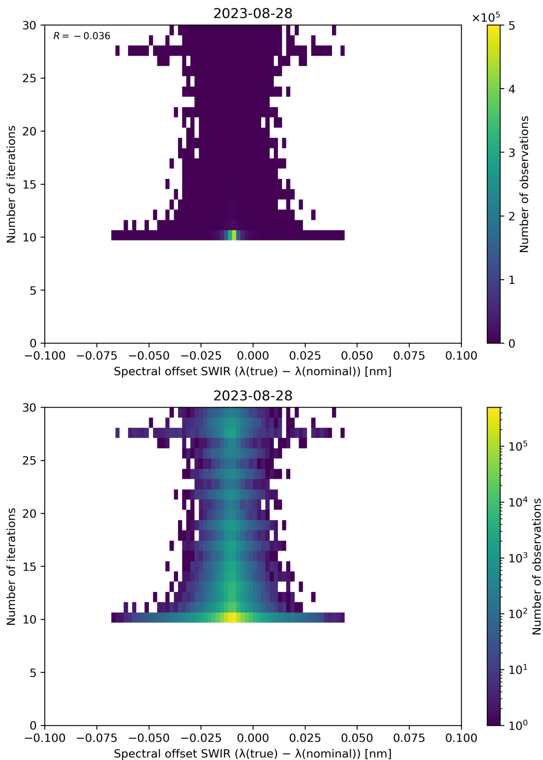
Figure 121: Scatter density plot of “Spectral offset SWIR ( \lambda(\text{true}) - \lambda(\text{nominal}) )” against “Number of iterations” for 2023-08-27 to 2023-08-29.
