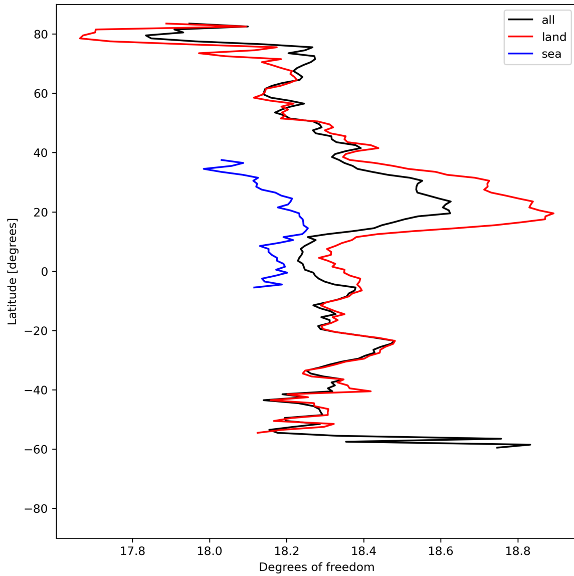
Figure 19: Zonal average of “Degrees of freedom” for 2023-08-27 to 2023-08-29.
