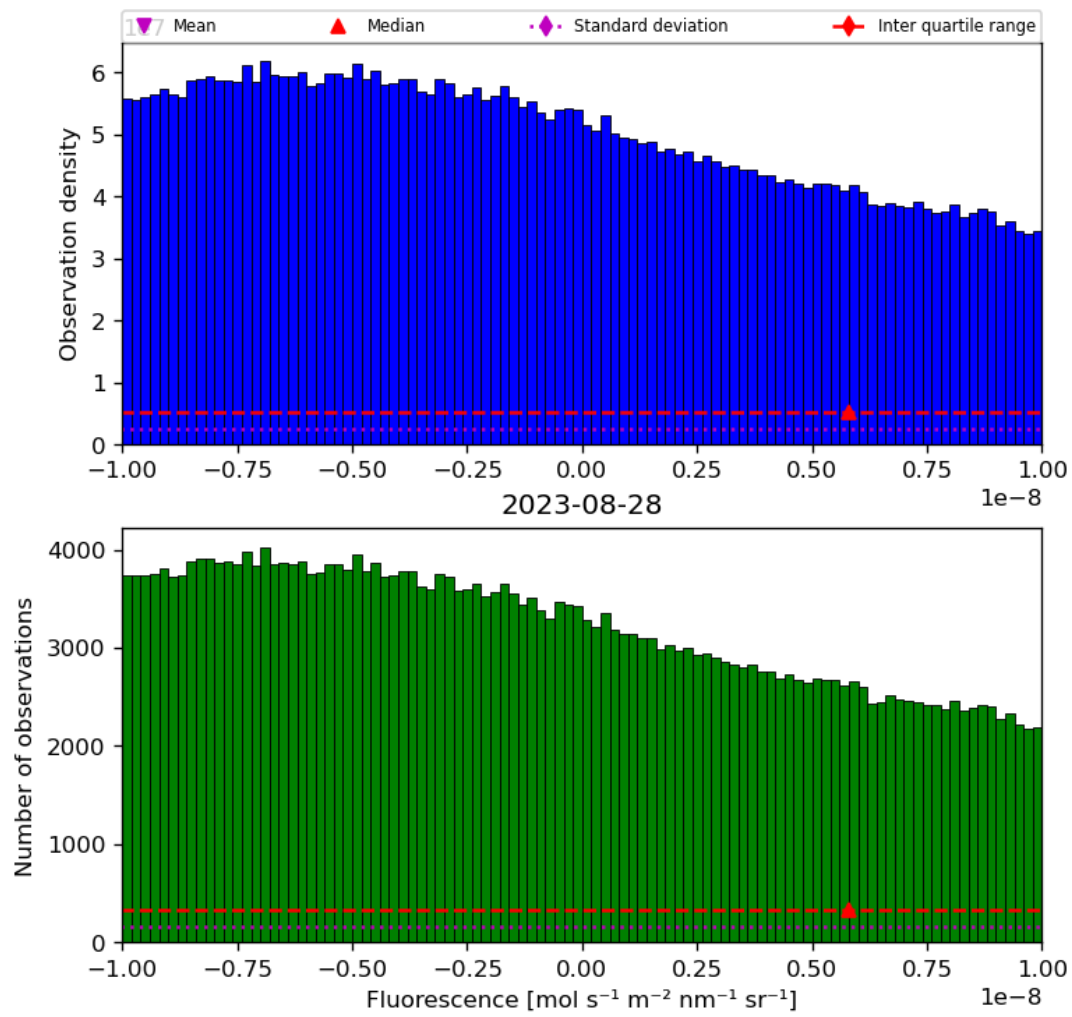
Figure 32: Histogram of “Fluorescence” for 2023-08-27 to 2023-08-29
