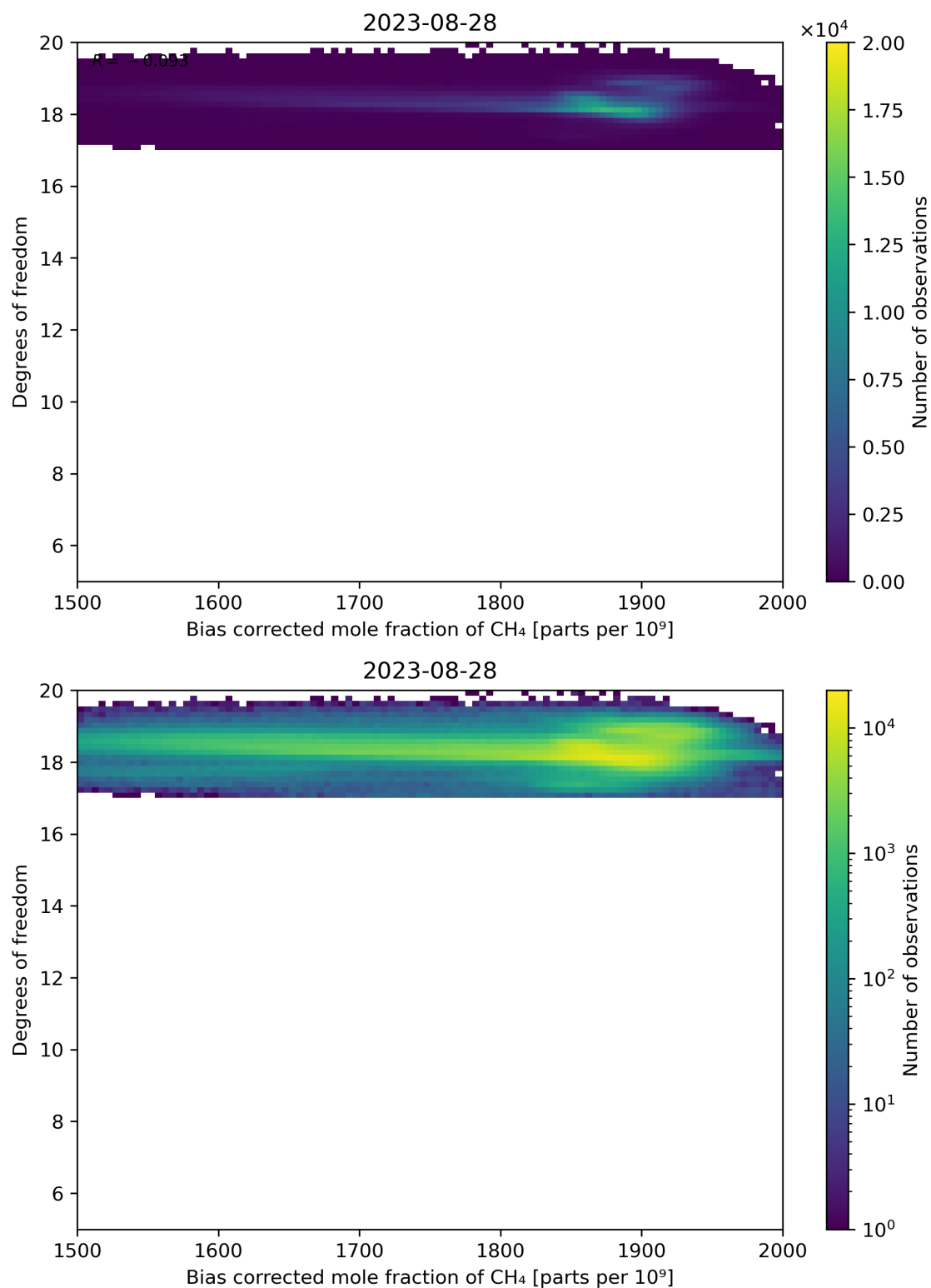
Figure 65: Scatter density plot of “Bias corrected mole fraction of CH 4 ” against “Degrees of freedom” for 2023-08-27 to 2023-08-29.
