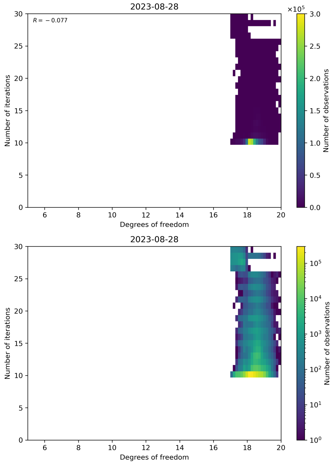
Figure 52: Scatter density plot of “Degrees of freedom” against “Number of iterations” for 2023-08-27 to 2023-08-29.
