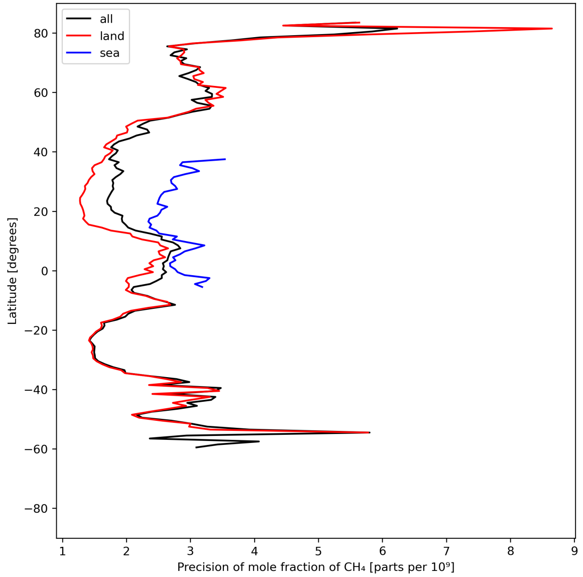
Figure 13: Zonal average of “Precision of mole fraction of CH 4 ” for 2023-08-27 to 2023-08-29.
