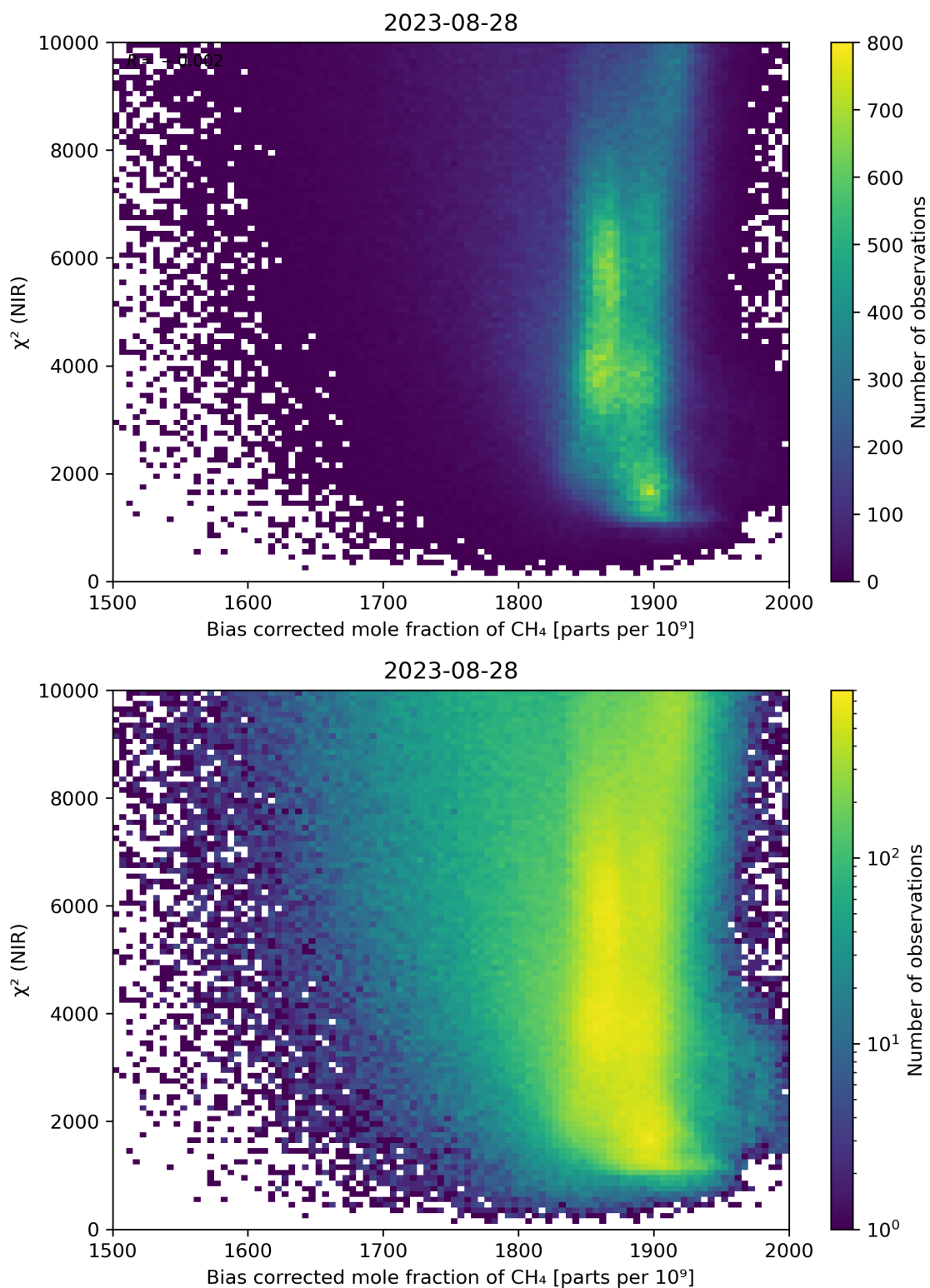
Figure 63: Scatter density plot of “Bias corrected mole fraction of CH 4 ” against “ \chi^2 (NIR)” for 2023-08-27 to 2023-08-29.
