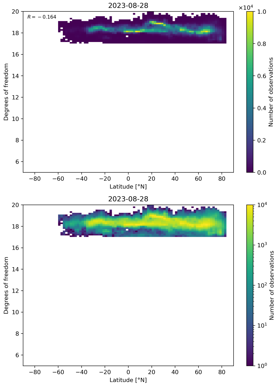
Figure 55: Scatter density plot of “Latitude” against “Degrees of freedom” for 2023-08-27 to 2023-08-29.
