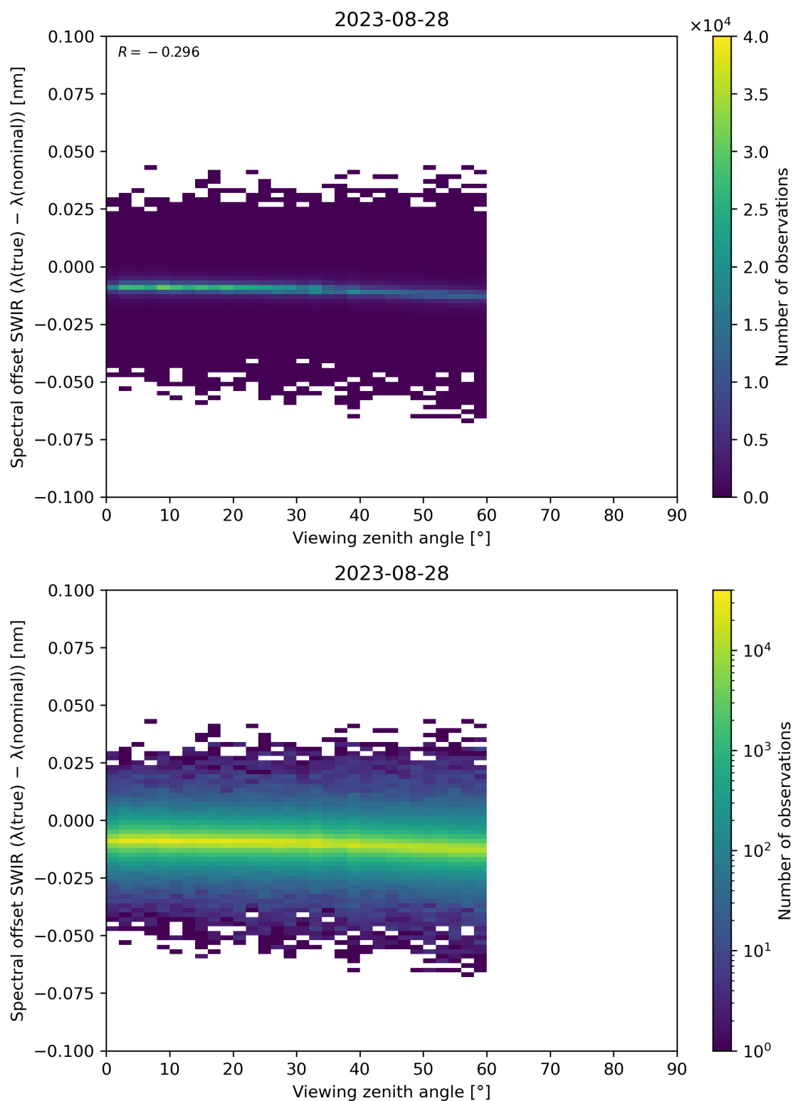
Figure 116: Scatter density plot of “Viewing zenith angle” against “Spectral offset SWIR ( \lambda(\text{true}) - \lambda(\text{nominal}) )” for 2023-08-27 to 2023-08-29.
