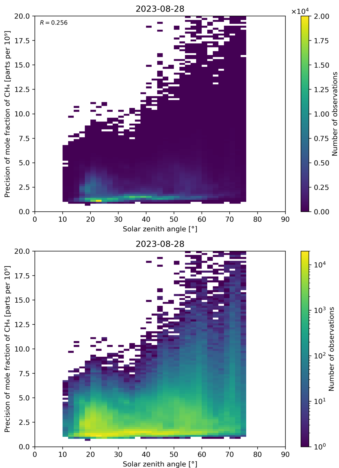
Figure 101: Scatter density plot of “Solar zenith angle” against “Precision of mole fraction of CH 4 ” for 2023-08-27 to 2023-08-29.
