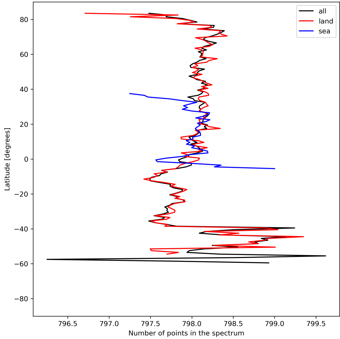
Figure 15: Zonal average of “Number of points in the spectrum” for 2023-08-27 to 2023-08-29.
