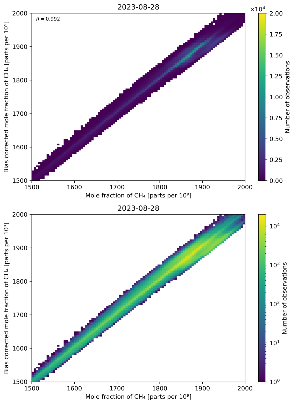
Figure 74: Scatter density plot of “Mole fraction of CH 4 ” against “Bias corrected mole fraction of CH 4 ” for 2023-08-27 to 2023-08-29.
