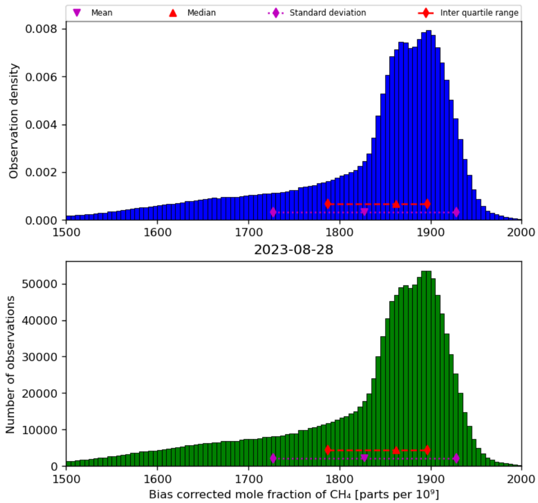
Figure 25: Histogram of “Bias corrected mole fraction of CH 4 ” for 2023-08-27 to 2023-08-29
