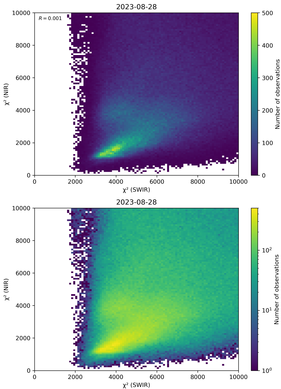
Figure 47: Scatter density plot of “ \chi^2 (SWIR)” against “ \chi^2 (NIR)” for 2023-08-27 to 2023-08-29.
