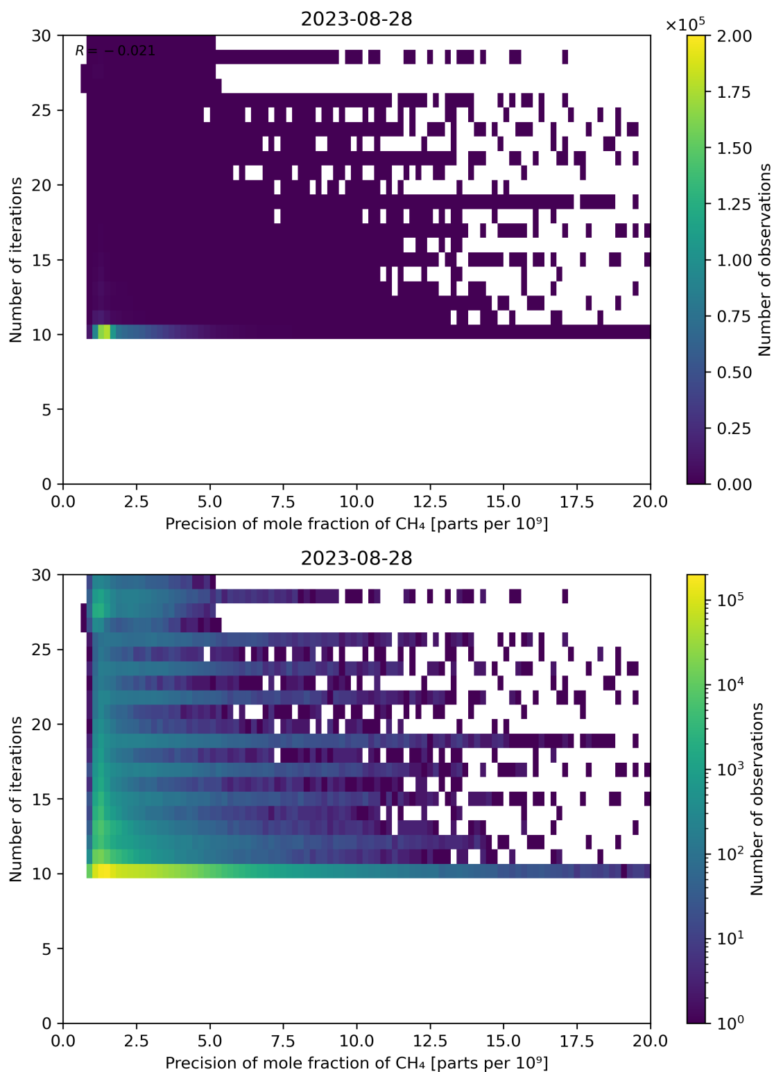
Figure 83: Scatter density plot of “Precision of mole fraction of CH 4 ” against “Number of iterations” for 2023-08-27 to 2023-08-29.
