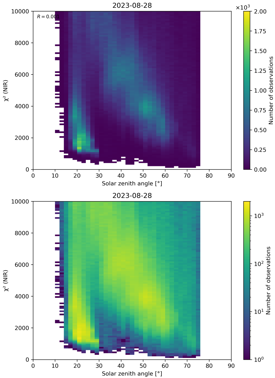
Figure 94: Scatter density plot of “Solar zenith angle” against “ \chi^2 (NIR)” for 2023-08-27 to 2023-08-29.
