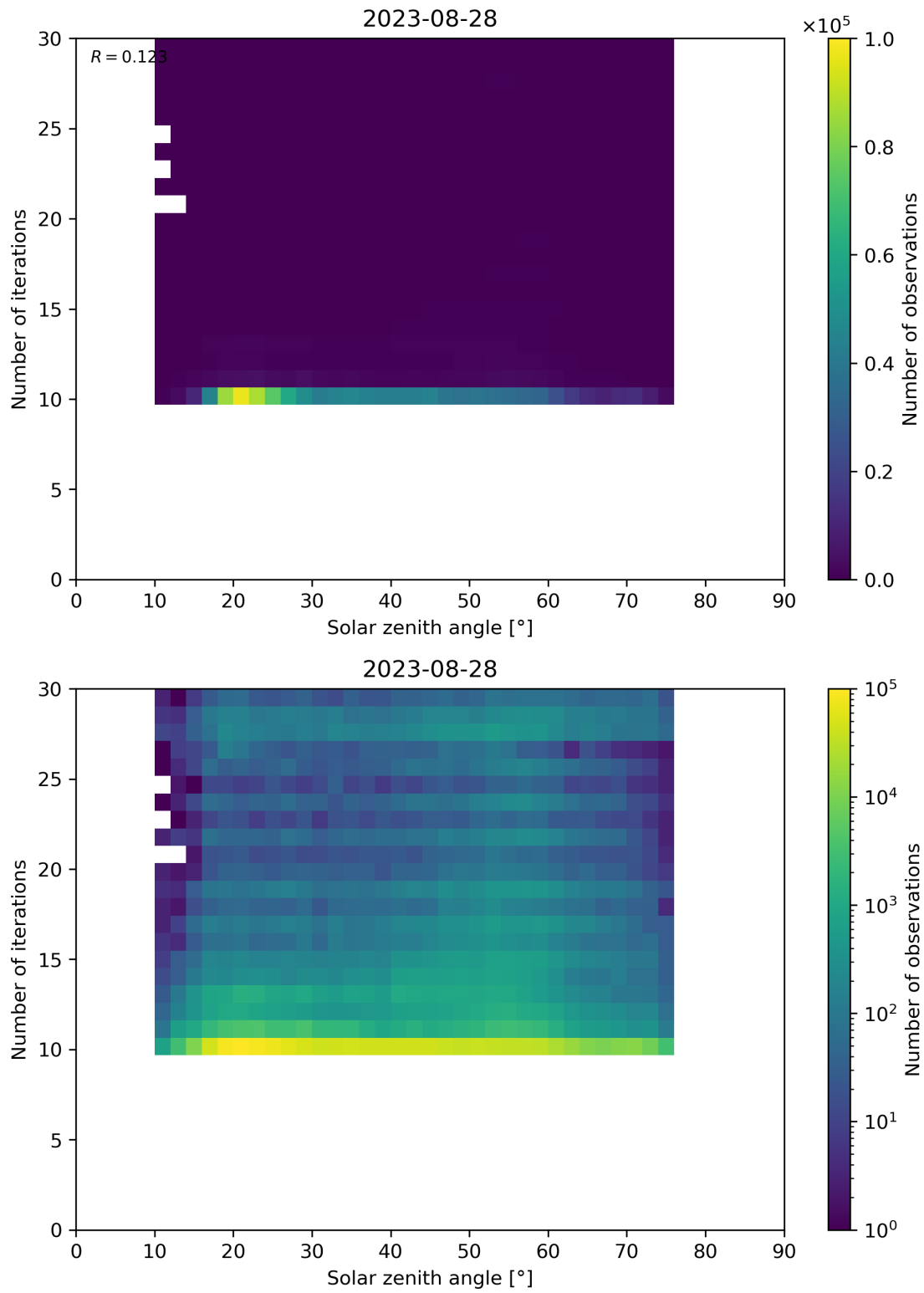
Figure 102: Scatter density plot of “Solar zenith angle” against “Number of iterations” for 2023-08-27 to 2023-08-29.
