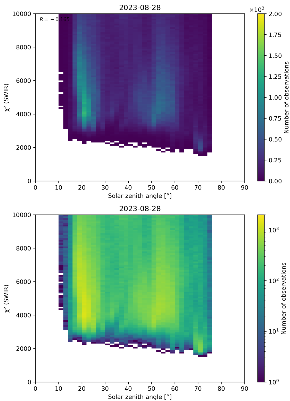
Figure 95: Scatter density plot of “Solar zenith angle” against “ \chi^2 (SWIR)” for 2023-08-27 to 2023-08-29.
