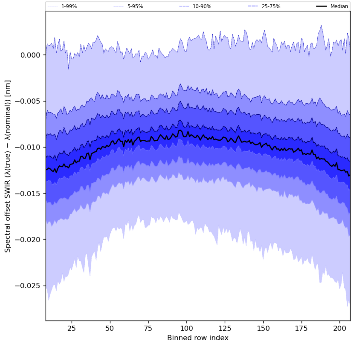
Figure 38: Along track statistics of “Spectral offset SWIR ( \lambda(\text{true}) - \lambda(\text{nominal}) )” for 2023-08-27 to 2023-08-29
