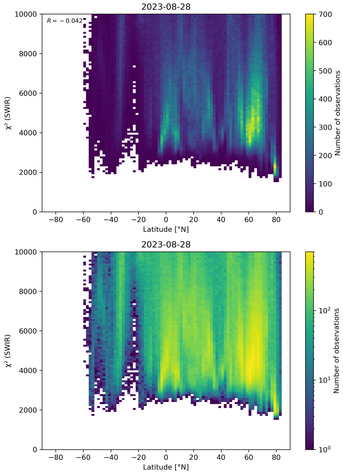
Figure 54: Scatter density plot of “Latitude” against “ \chi^2 (SWIR)” for 2023-08-27 to 2023-08-29.
