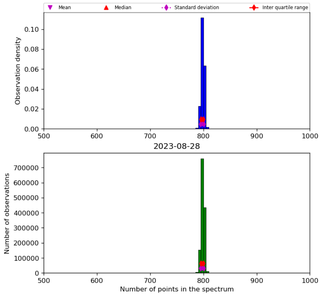
Figure 26: Histogram of “Number of points in the spectrum” for 2023-08-27 to 2023-08-29
