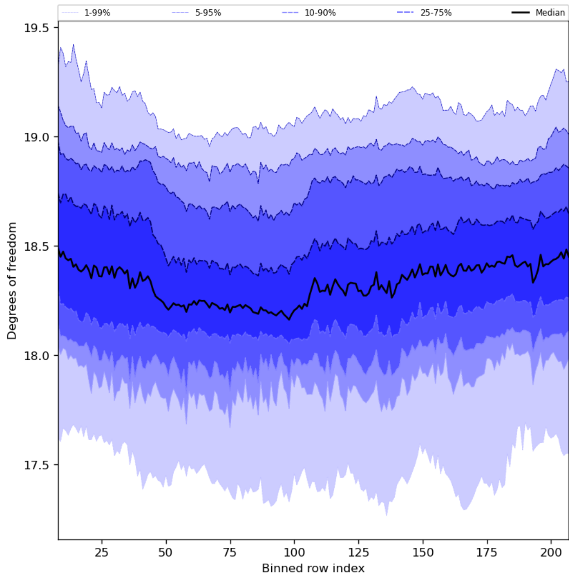
Figure 41: Along track statistics of “Degrees of freedom” for 2023-08-27 to 2023-08-29
