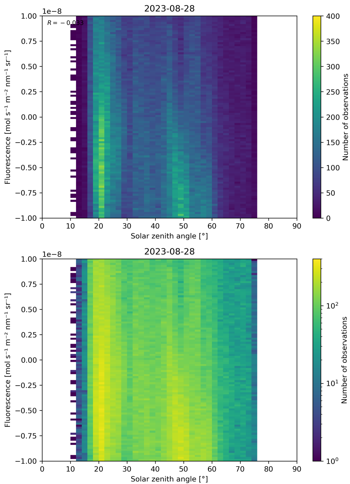
Figure 97: Scatter density plot of “Solar zenith angle” against “Fluorescence” for 2023-08-27 to 2023-08-29.
