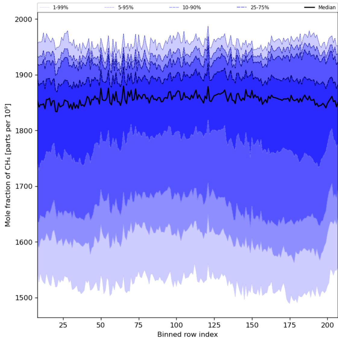
Figure 34: Along track statistics of “Mole fraction of CH 4 ” for 2023-08-27 to 2023-08-29
