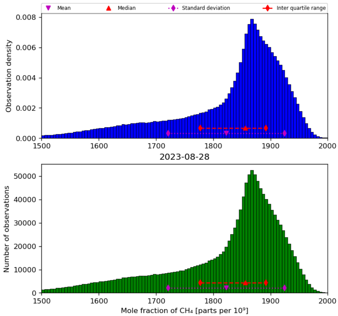
Figure 23: Histogram of “Mole fraction of CH 4 ” for 2023-08-27 to 2023-08-29
