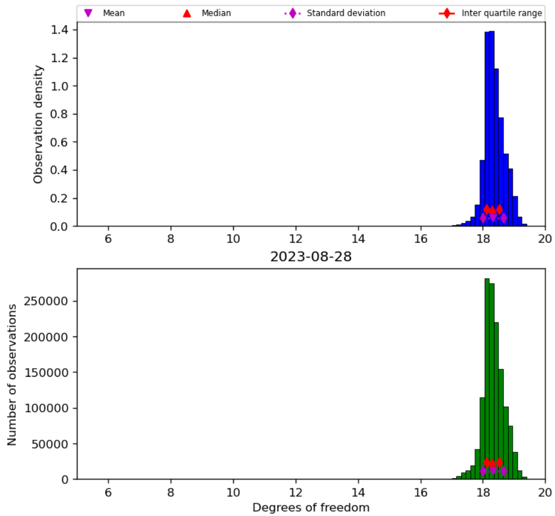
Figure 30: Histogram of “Degrees of freedom” for 2023-08-27 to 2023-08-29
