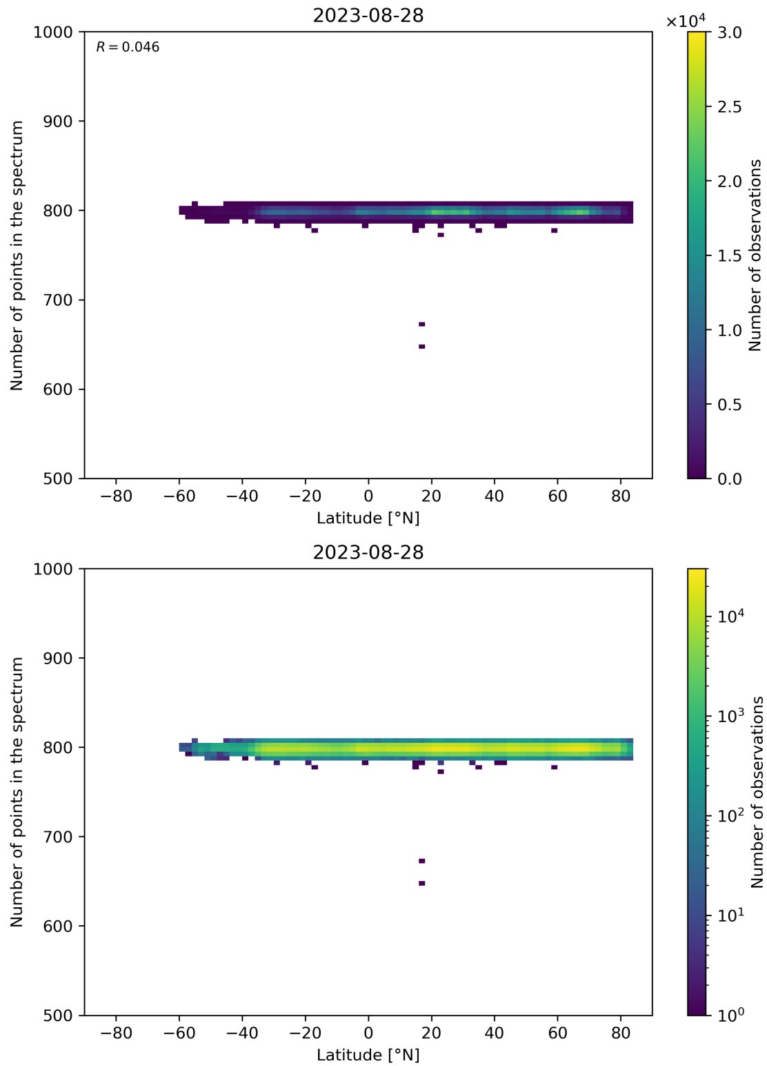
Figure 61: Scatter density plot of “Latitude” against “Number of points in the spectrum” for 2023-08-27 to 2023-08-29.
