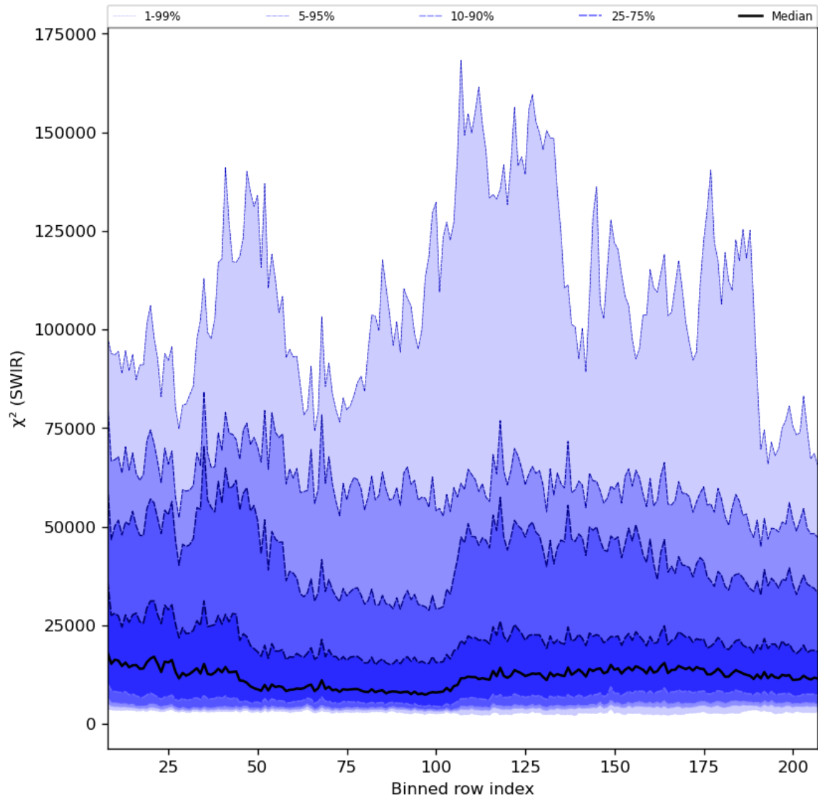
Figure 39: Along track statistics of “ \chi^2 (SWIR)” for 2023-08-27 to 2023-08-29
