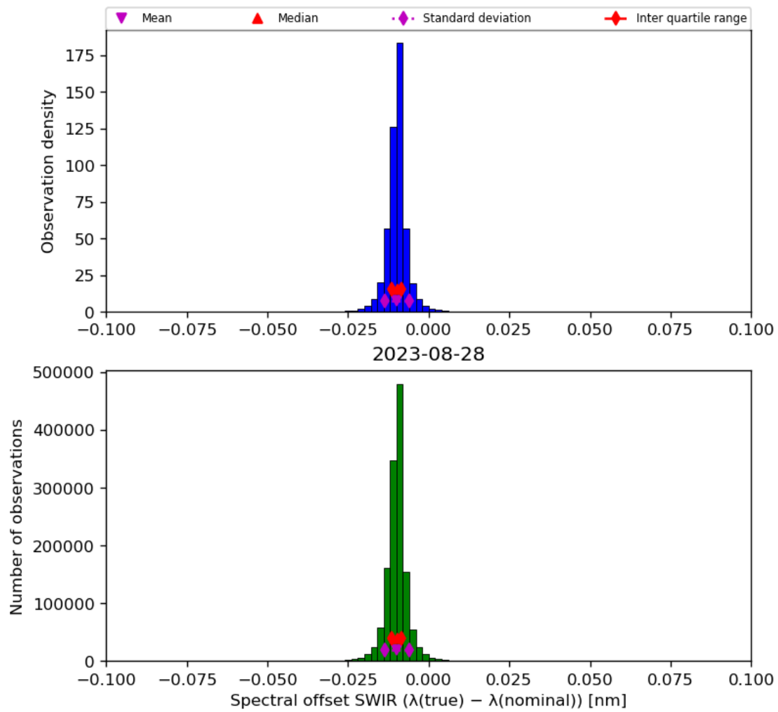
Figure 27: Histogram of “Spectral offset SWIR ( \lambda(\text{true}) - \lambda(\text{nominal}) )” for 2023-08-27 to 2023-08-29
