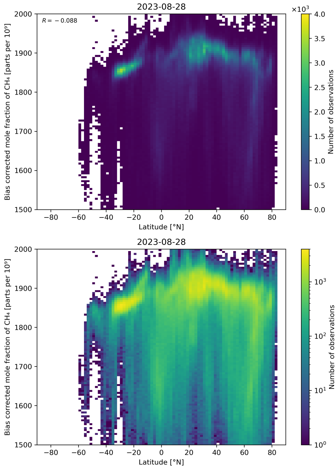
Figure 58: Scatter density plot of “Latitude” against “Bias corrected mole fraction of CH 4 ” for 2023-08-27 to 2023-08-29.
