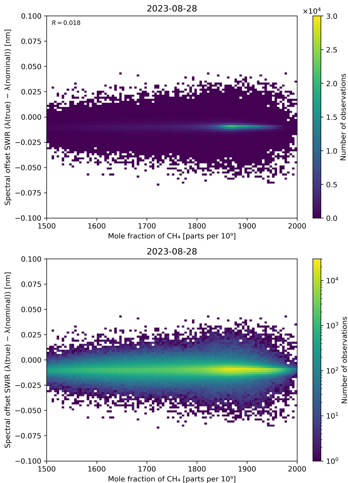
Figure 86: Scatter density plot of “Mole fraction of CH 4 ” against “Spectral offset SWIR ( \lambda(\text{true}) - \lambda(\text{nominal}) )” for 2023-08-27 to 2023-08-29.
