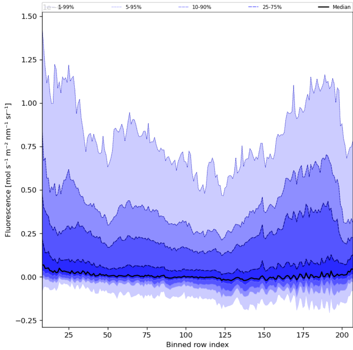
Figure 43: Along track statistics of “Fluorescence” for 2023-08-27 to 2023-08-29
