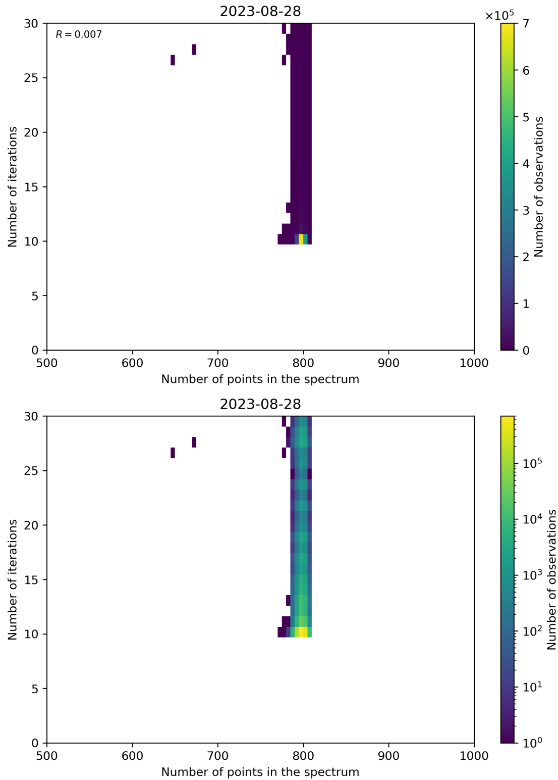
Figure 92: Scatter density plot of “Number of points in the spectrum” against “Number of iterations” for 2023-08-27 to 2023-08-29.
