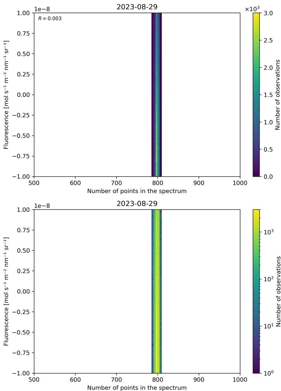
Figure 91: Scatter density plot of “Number of points in the spectrum” against “Fluorescence” for 2023-08-28 to 2023-08-30.
