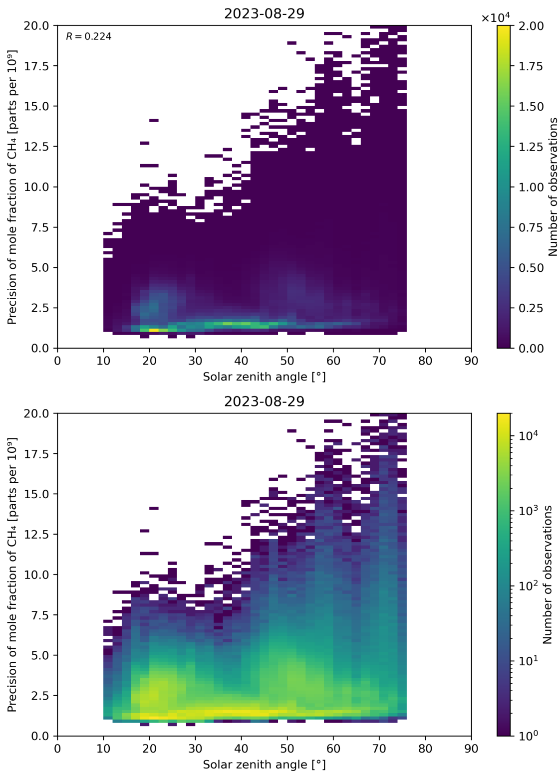
Figure 101: Scatter density plot of “Solar zenith angle” against “Precision of mole fraction of CH 4 ” for 2023-08-28 to 2023-08-30.
