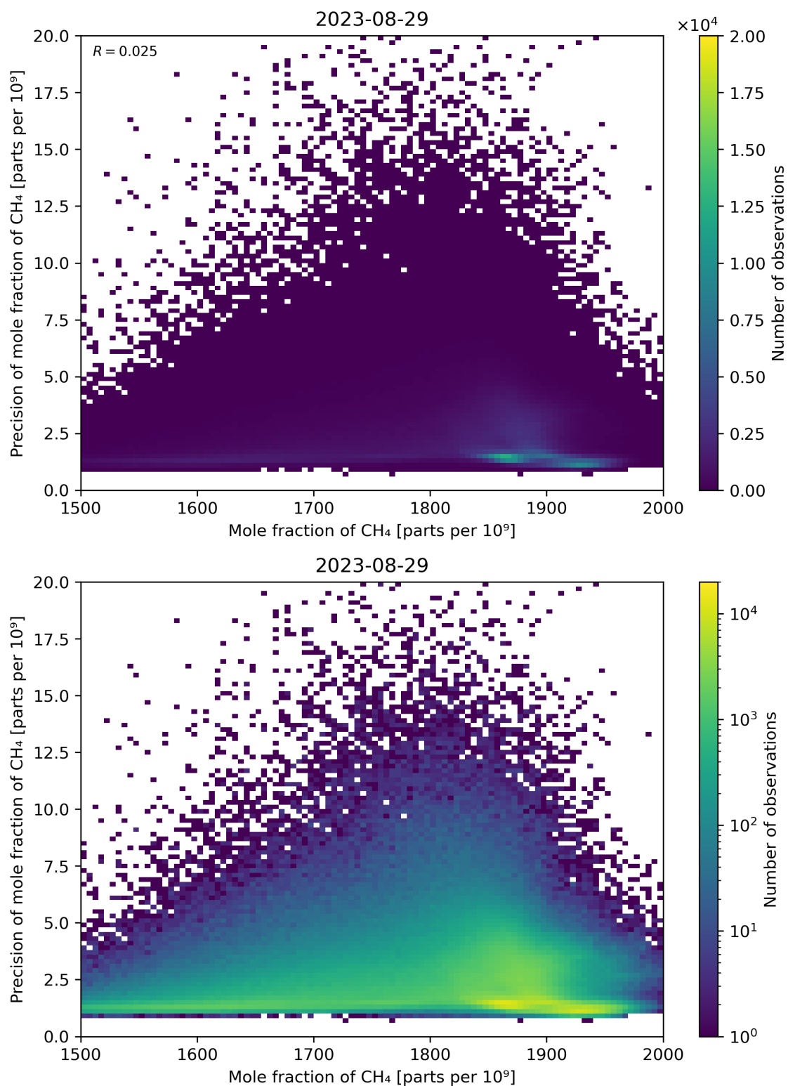
Figure 75: Scatter density plot of “Mole fraction of CH 4 ” against “Precision of mole fraction of CH 4 ” for 2023-08-28 to 2023-08-30.
