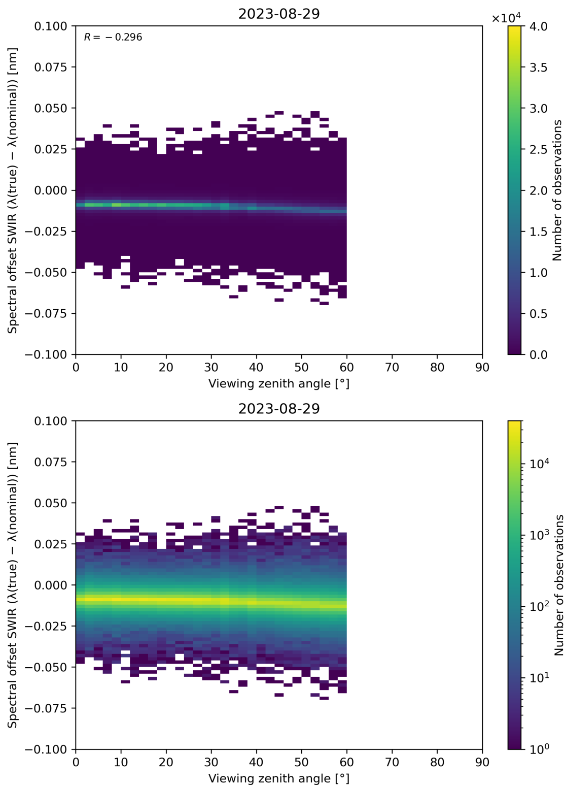
Figure 116: Scatter density plot of “Viewing zenith angle” against “Spectral offset SWIR ( \lambda(\text{true}) - \lambda(\text{nominal}) )” for 2023-08-28 to 2023-08-30.
