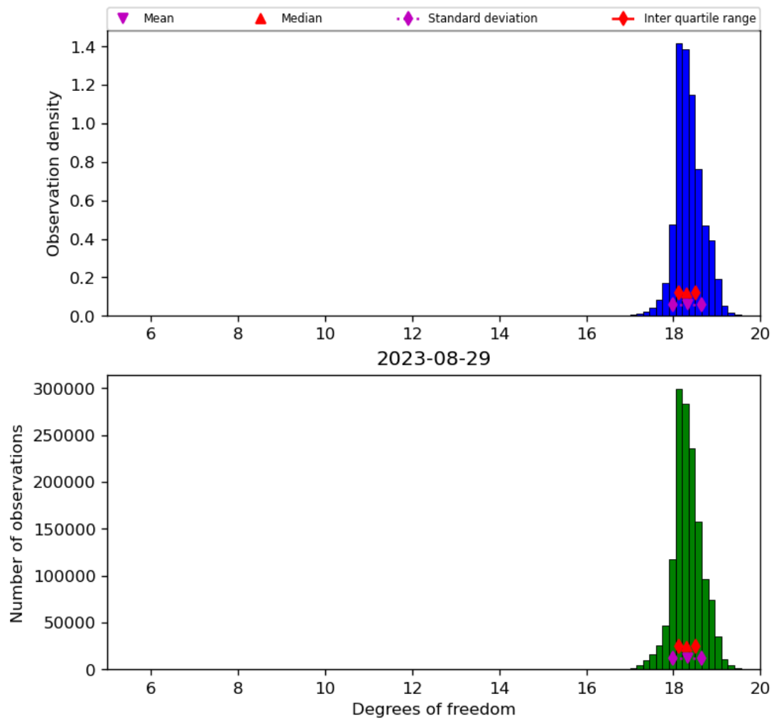
Figure 30: Histogram of “Degrees of freedom” for 2023-08-28 to 2023-08-30
