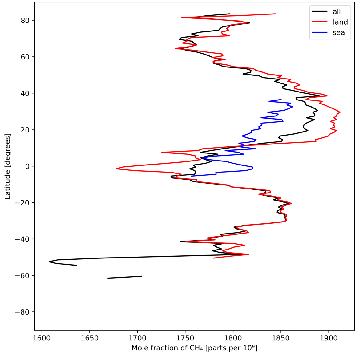
Figure 12: Zonal average of “Mole fraction of CH 4 ” for 2023-08-28 to 2023-08-30.
