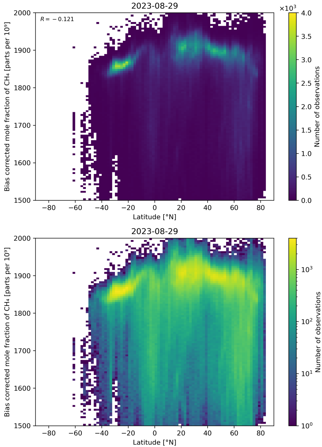
Figure 58: Scatter density plot of “Latitude” against “Bias corrected mole fraction of \text{CH}_4 ” for 2023-08-28 to 2023-08-30.
