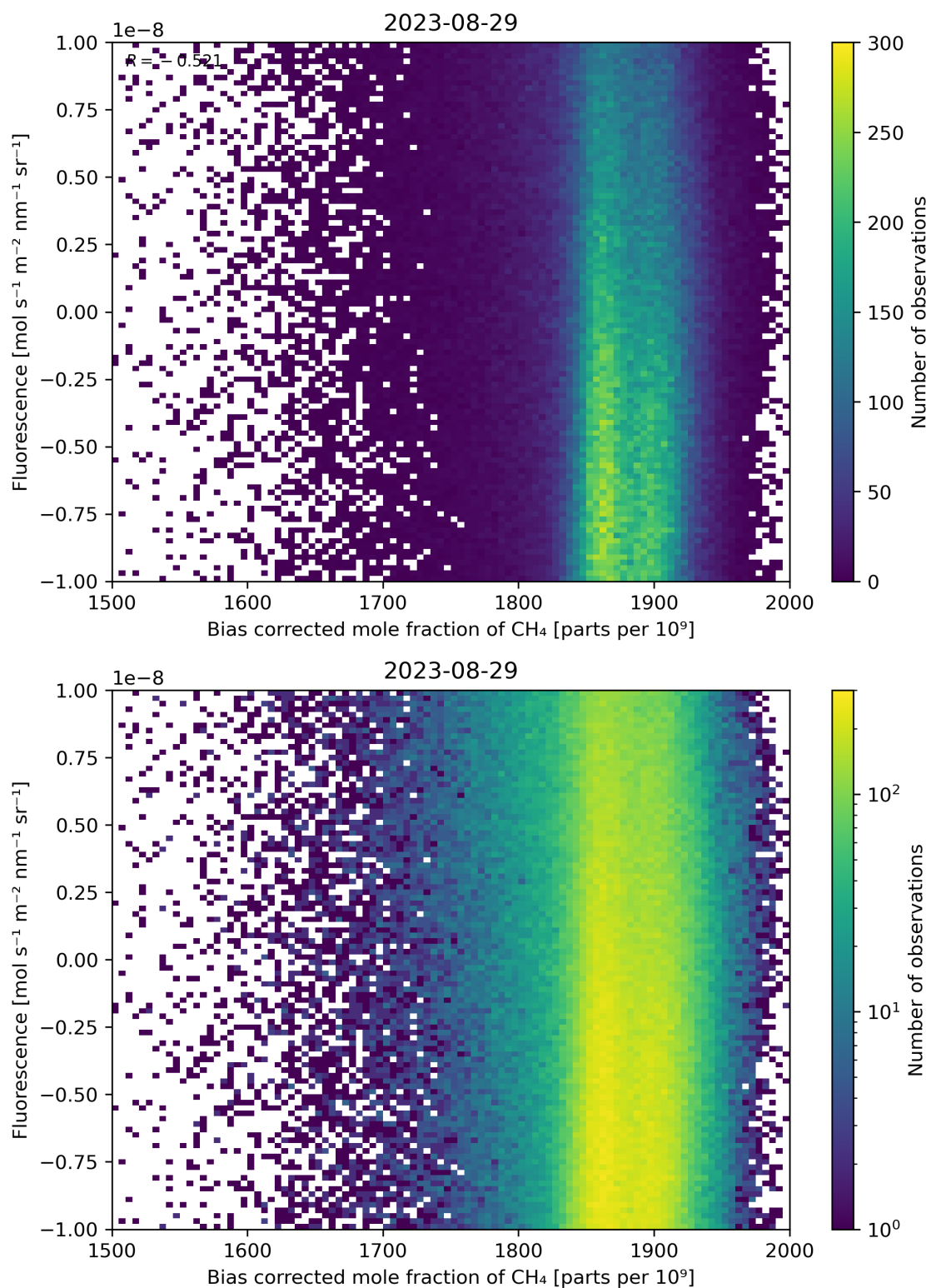
Figure 66: Scatter density plot of “Bias corrected mole fraction of \text{CH}_4 ” against “Fluorescence” for 2023-08-28 to 2023-08-30.
