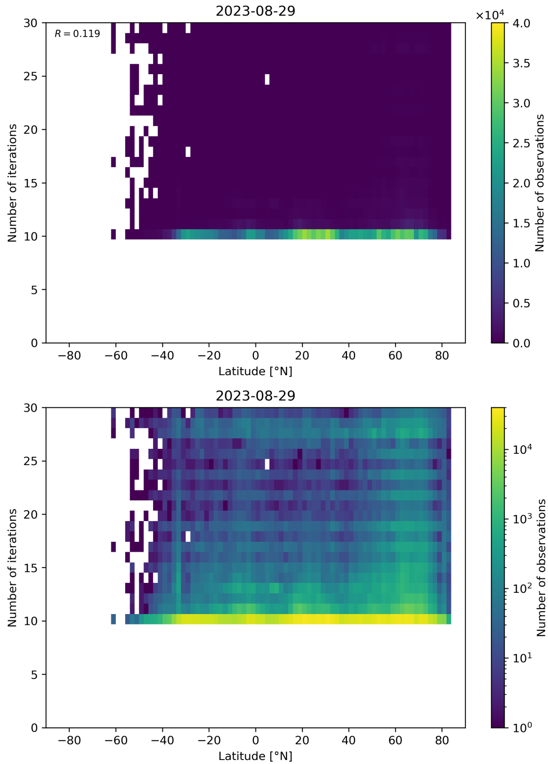
Figure 60: Scatter density plot of “Latitude” against “Number of iterations” for 2023-08-28 to 2023-08-30.
