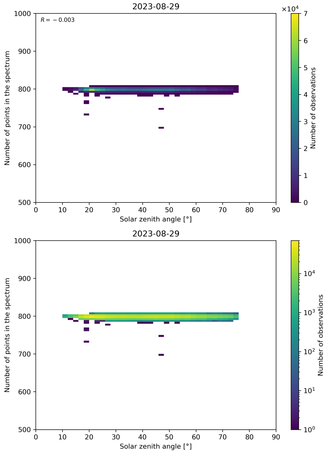
Figure 103: Scatter density plot of “Solar zenith angle” against “Number of points in the spectrum” for 2023-08-28 to 2023-08-30.
