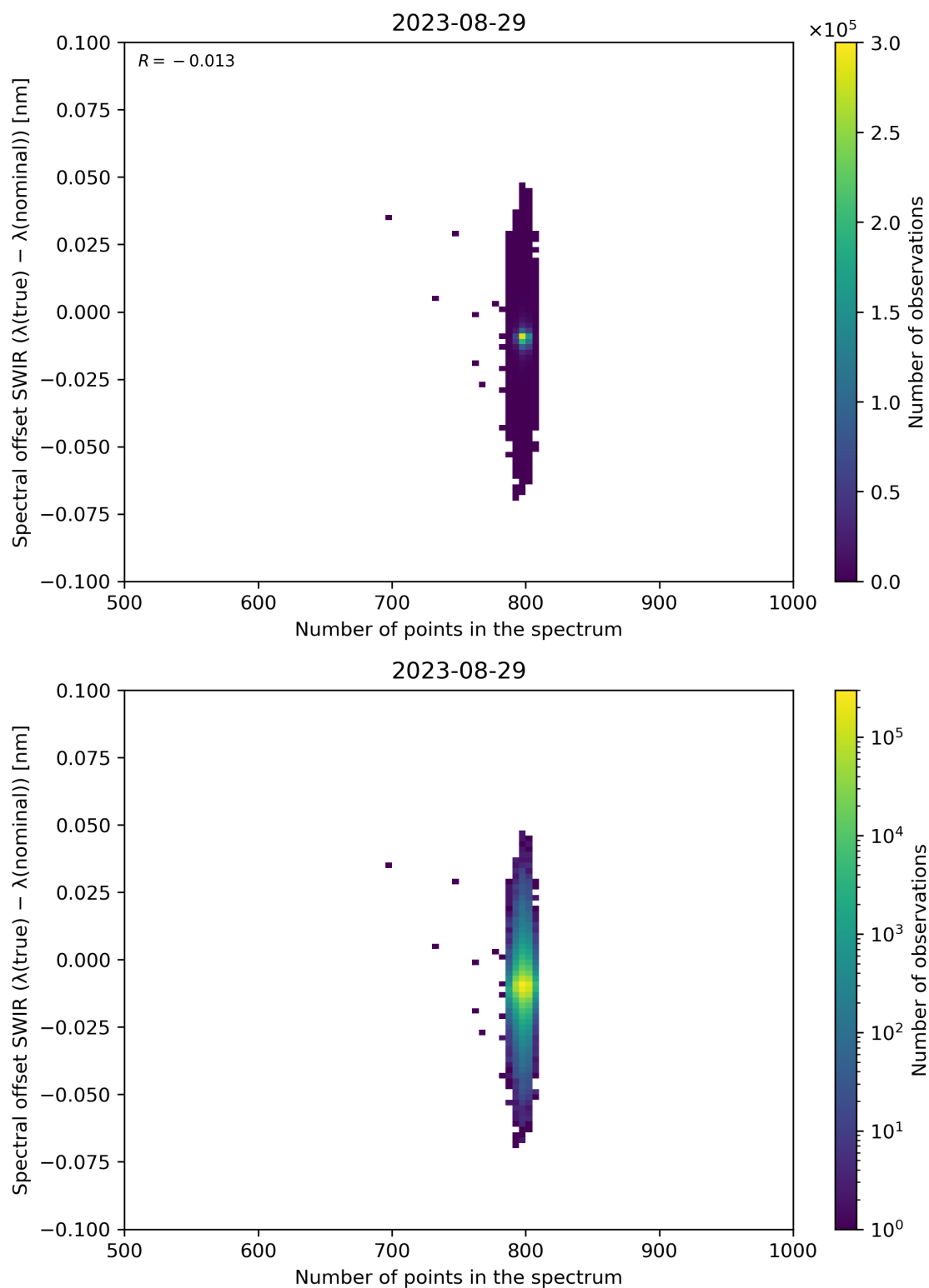
Figure 93: Scatter density plot of “Number of points in the spectrum” against “Spectral offset SWIR ( \lambda(\text{true}) - \lambda(\text{nominal}) )” for 2023-08-28 to 2023-08-30.
