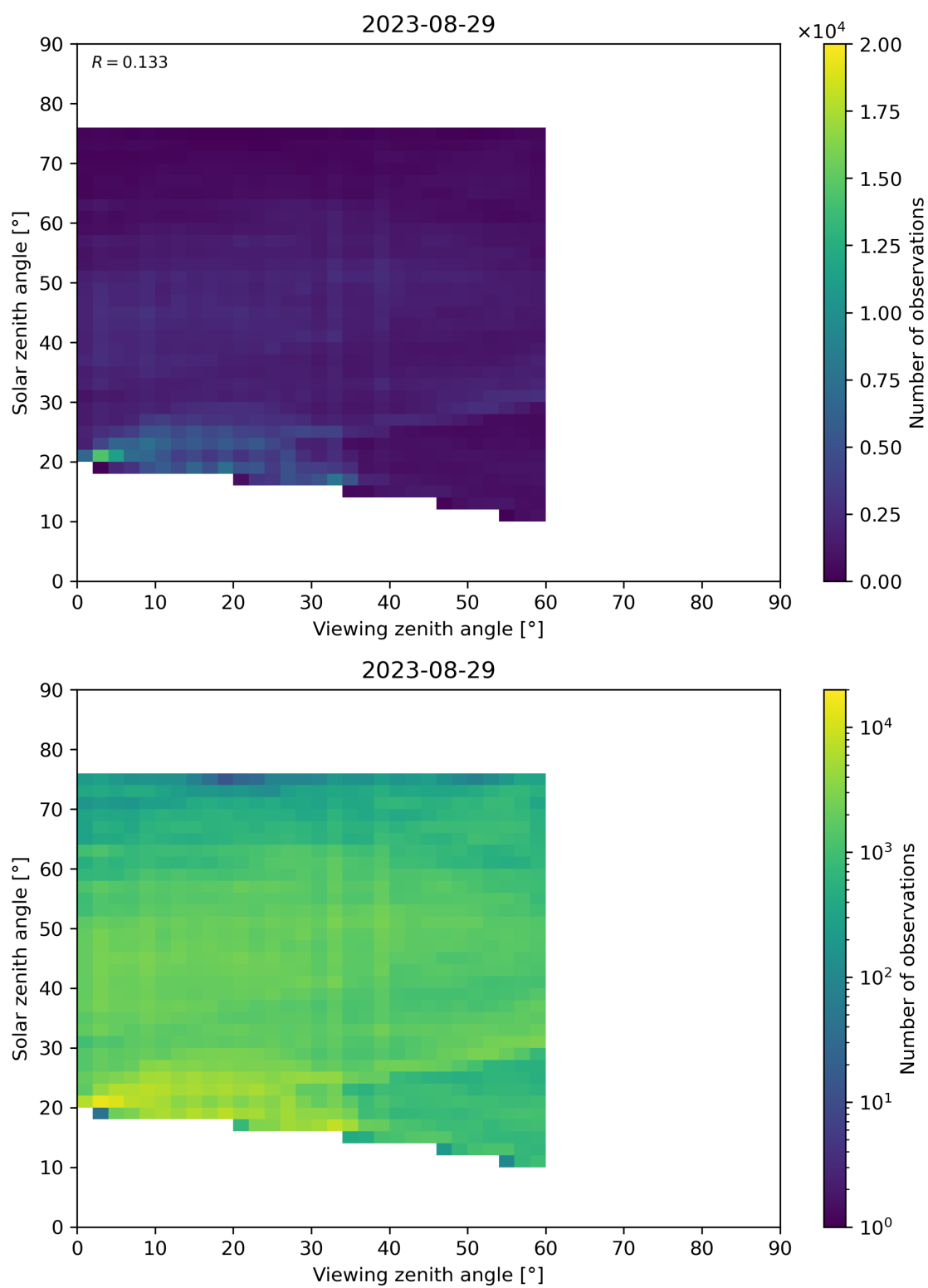
Figure 115: Scatter density plot of “Viewing zenith angle” against “Solar zenith angle” for 2023-08-28 to 2023-08-30.
