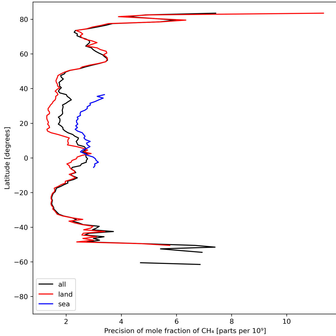
Figure 13: Zonal average of “Precision of mole fraction of CH 4 ” for 2023-08-28 to 2023-08-30.
