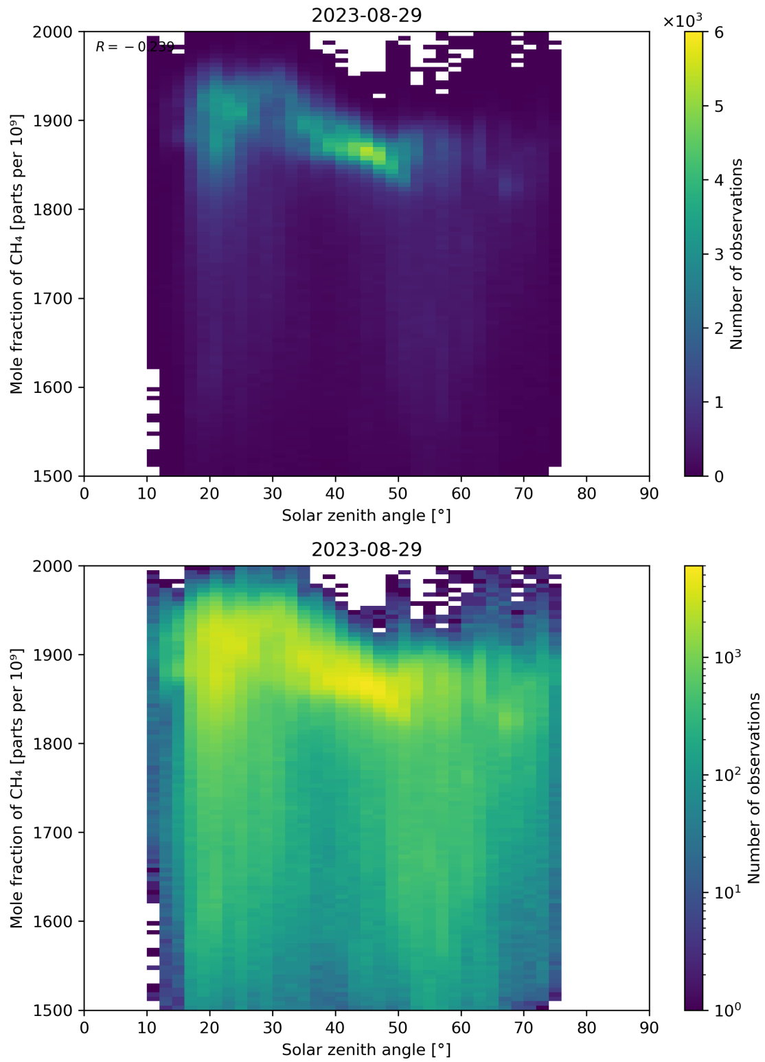
Figure 99: Scatter density plot of “Solar zenith angle” against “Mole fraction of CH 4 ” for 2023-08-28 to 2023-08-30.
