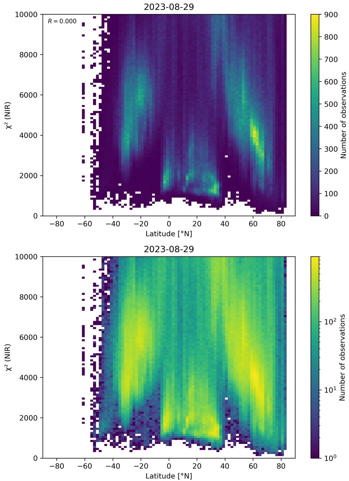
Figure 53: Scatter density plot of “Latitude” against “ \chi^2 (NIR)” for 2023-08-28 to 2023-08-30.
