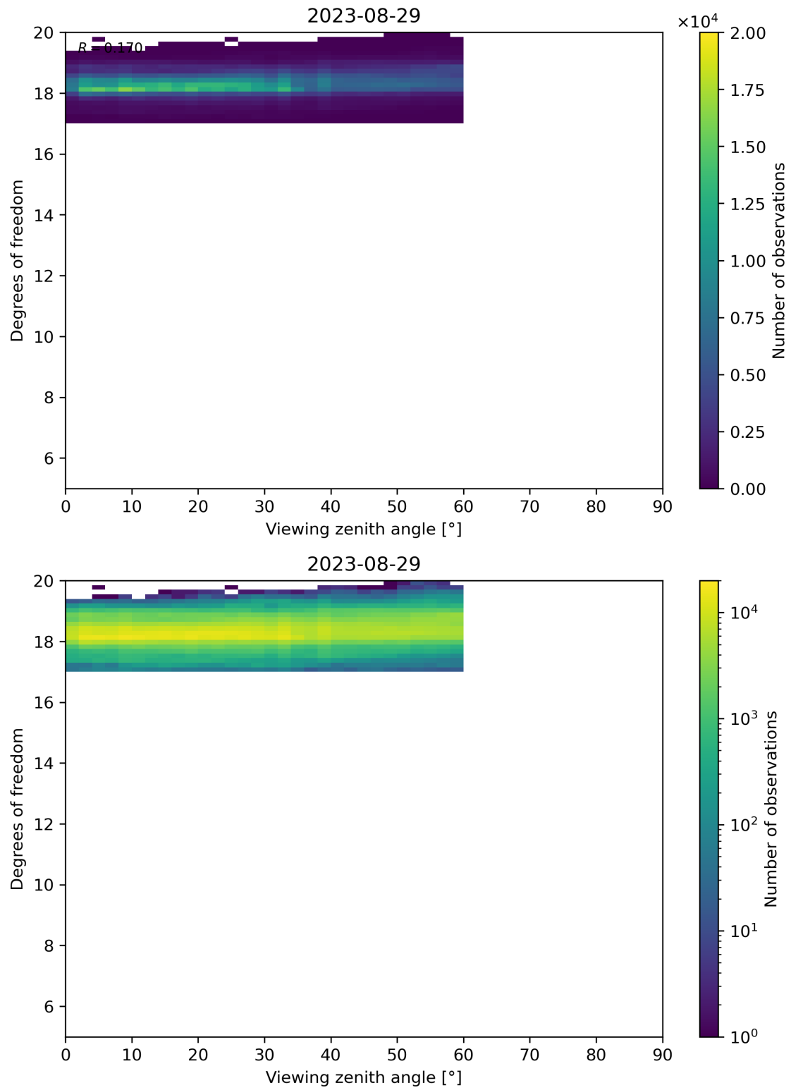
Figure 107: Scatter density plot of “Viewing zenith angle” against “Degrees of freedom” for 2023-08-28 to 2023-08-30.
