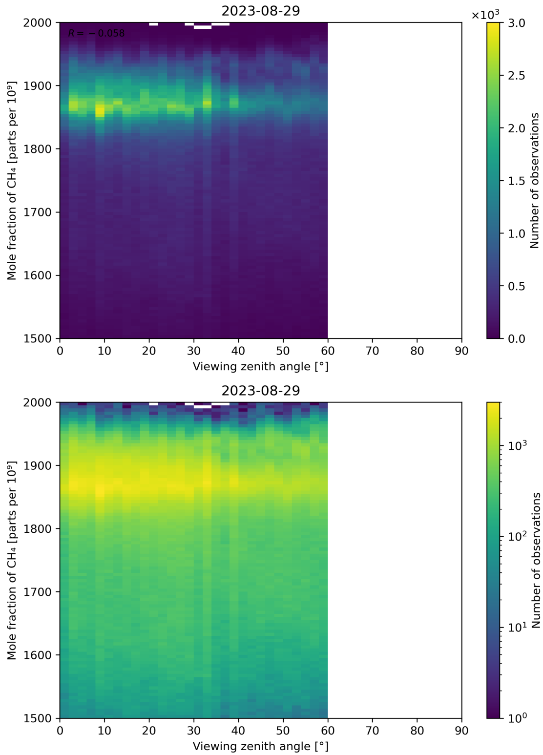
Figure 110: Scatter density plot of “Viewing zenith angle” against “Mole fraction of \text{CH}_4 ” for 2023-08-28 to 2023-08-30.
