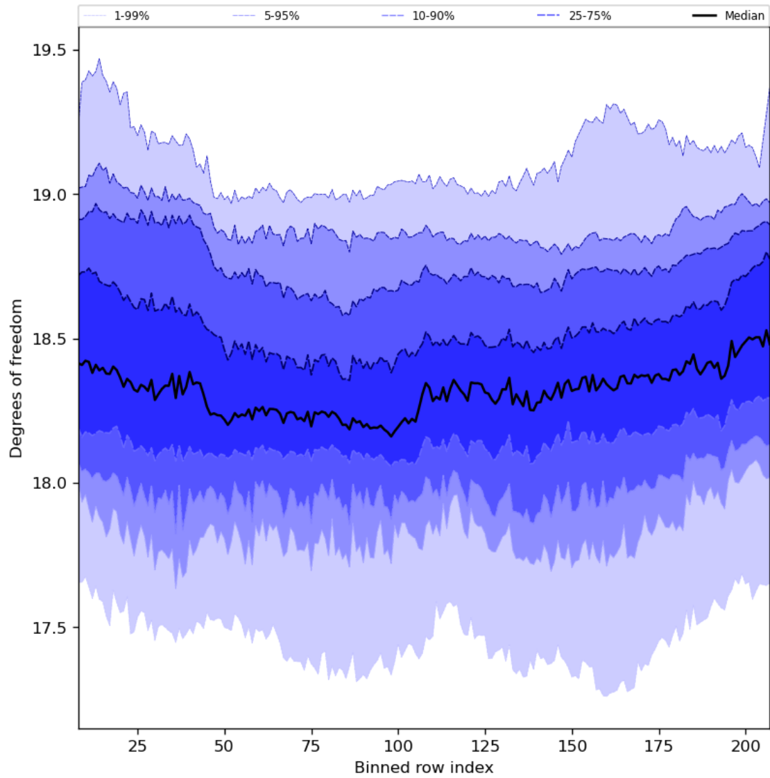
Figure 41: Along track statistics of “Degrees of freedom” for 2023-08-28 to 2023-08-30
