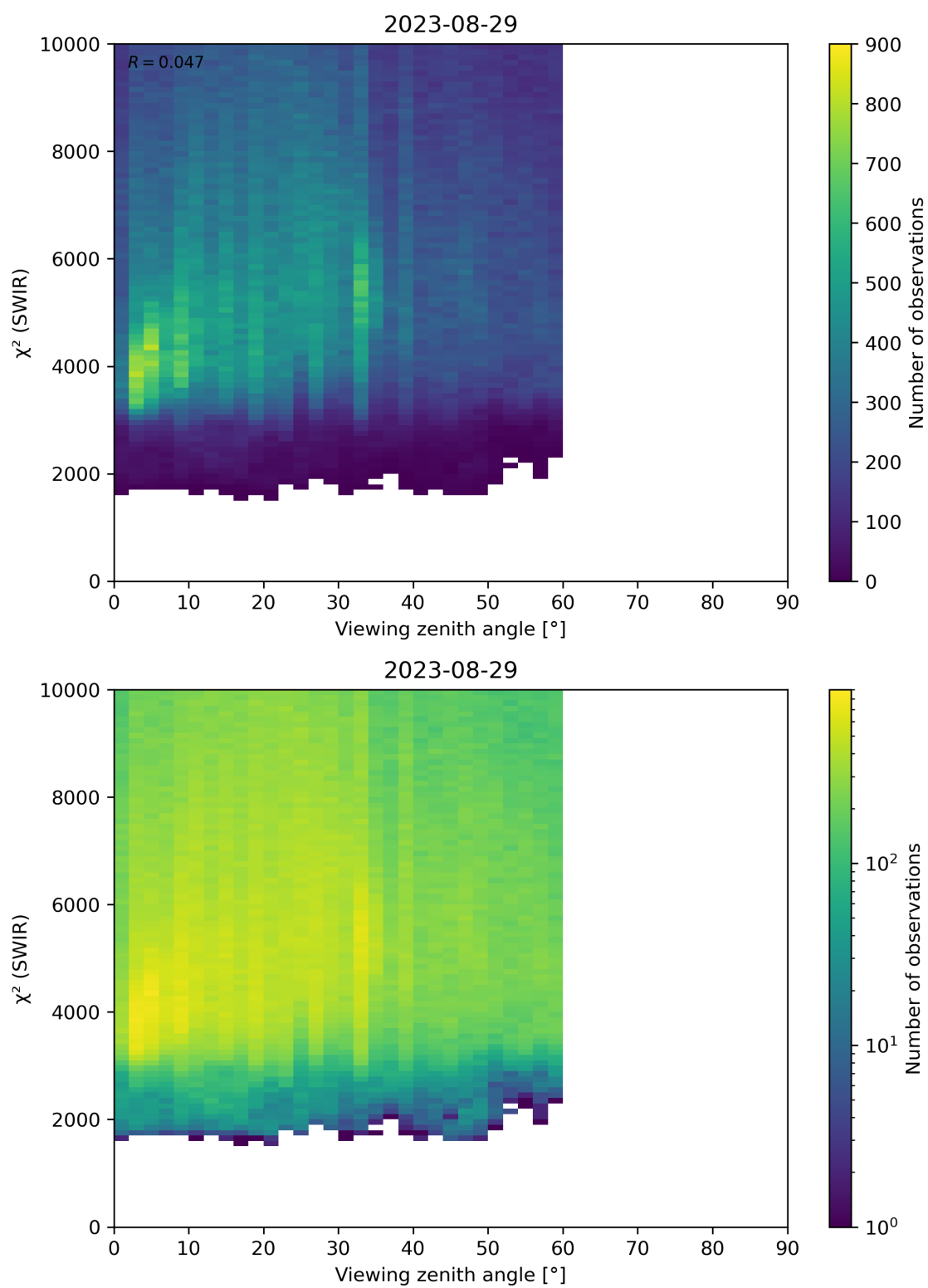
Figure 106: Scatter density plot of “Viewing zenith angle” against “ \chi^2 (SWIR)” for 2023-08-28 to 2023-08-30.
