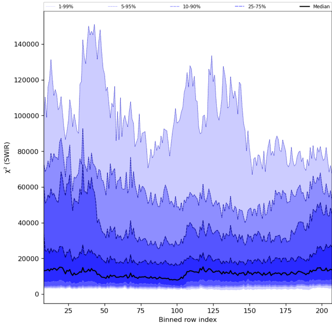
Figure 39: Along track statistics of “ \chi^2 (SWIR)” for 2023-08-28 to 2023-08-30
