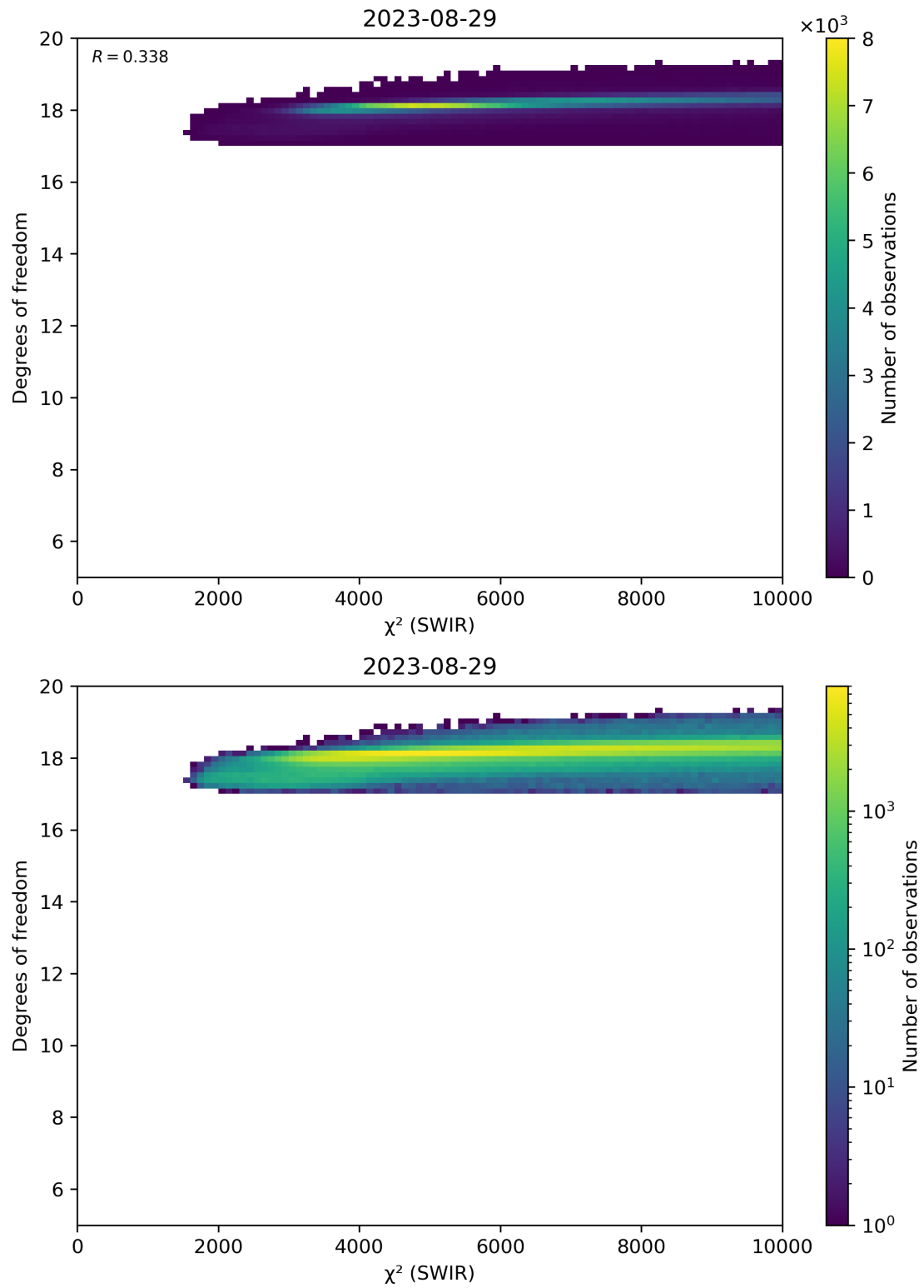
Figure 48: Scatter density plot of “ \chi^2 (SWIR)” against “Degrees of freedom” for 2023-08-28 to 2023-08-30.
