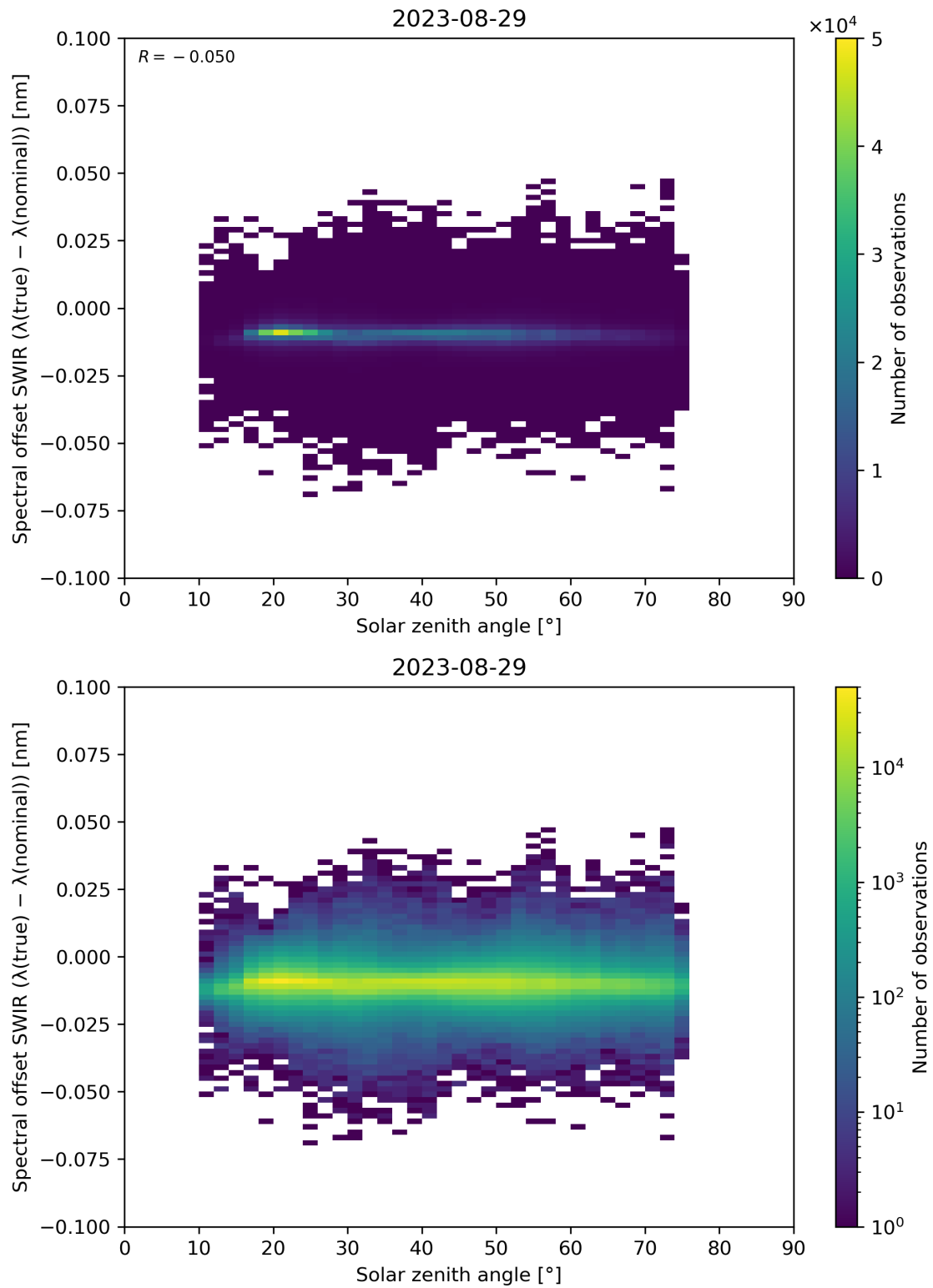
Figure 104: Scatter density plot of “Solar zenith angle” against “Spectral offset SWIR ( \lambda(\text{true}) - \lambda(\text{nominal}) )” for 2023-08-28 to 2023-08-30.
