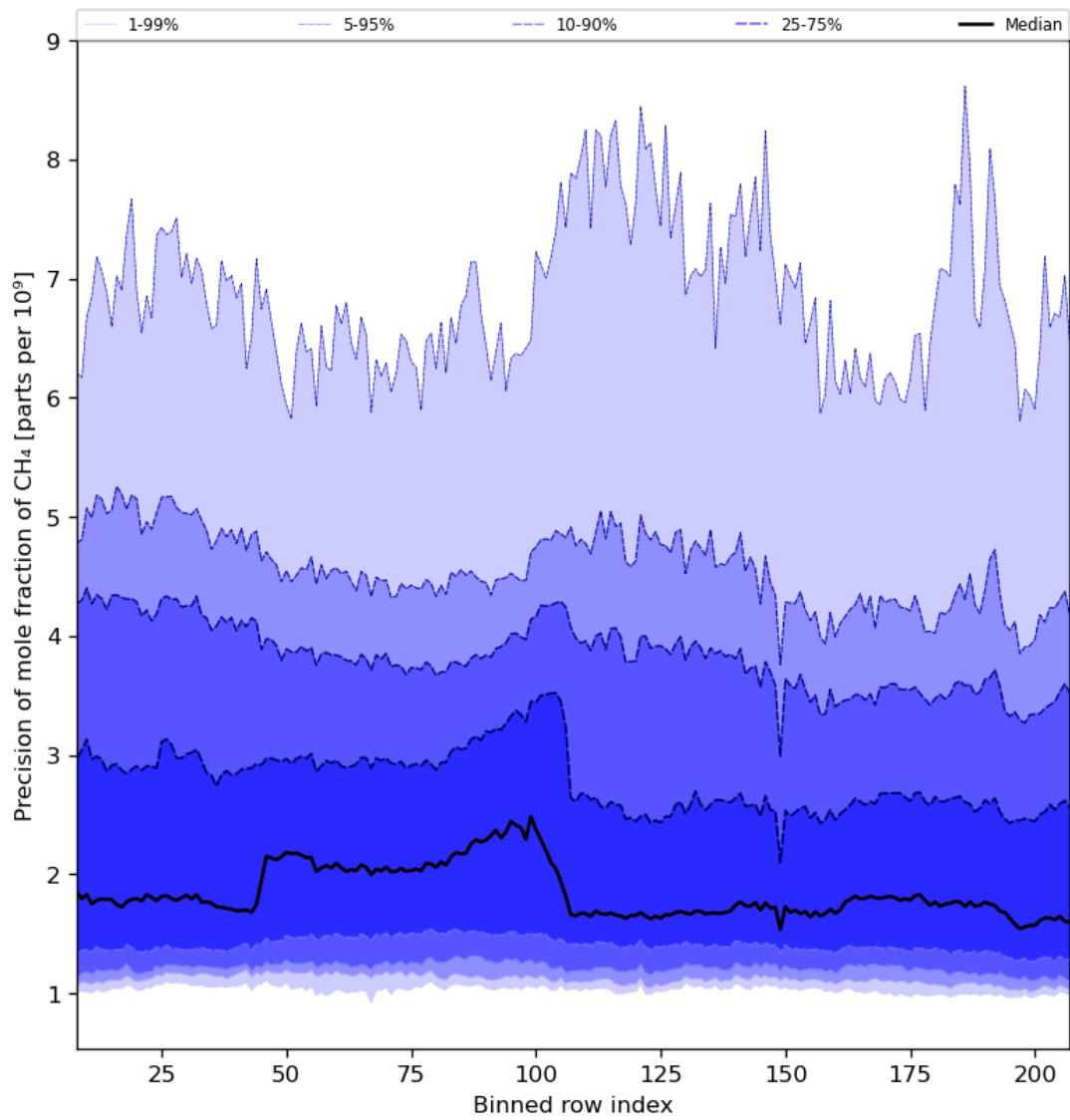
Figure 35: Along track statistics of “Precision of mole fraction of CH 4 ” for 2023-08-28 to 2023-08-30
