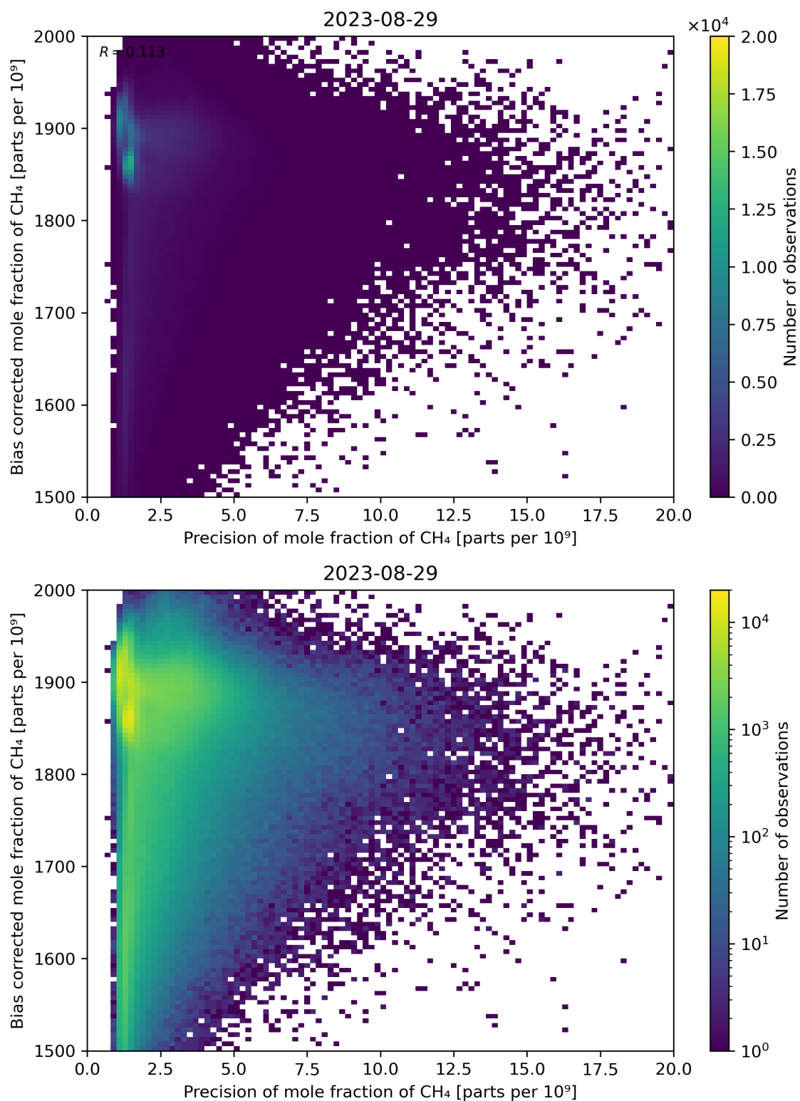
Figure 82: Scatter density plot of “Precision of mole fraction of CH 4 ” against “Bias corrected mole fraction of CH 4 ” for 2023-08-28 to 2023-08-30.
