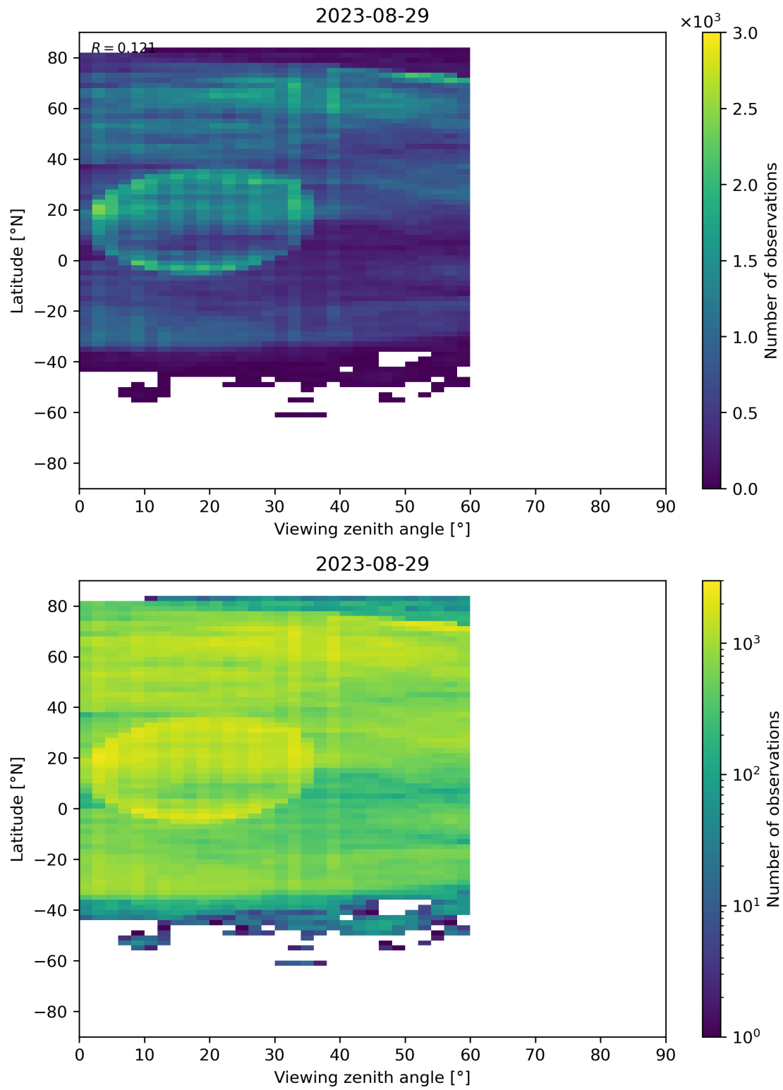
Figure 109: Scatter density plot of “Viewing zenith angle” against “Latitude” for 2023-08-28 to 2023-08-30.
