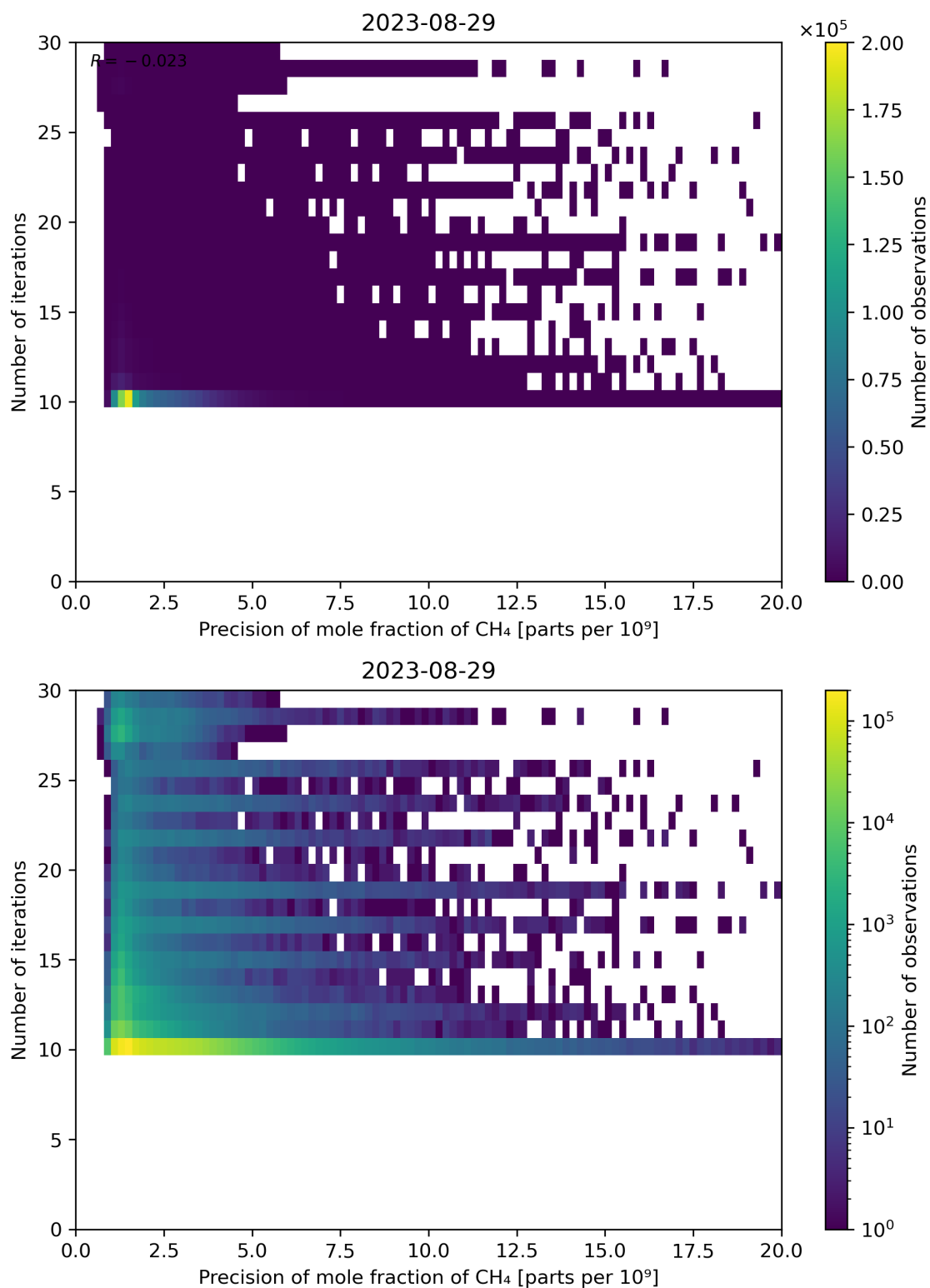
Figure 83: Scatter density plot of “Precision of mole fraction of CH 4 ” against “Number of iterations” for 2023-08-28 to 2023-08-30.
