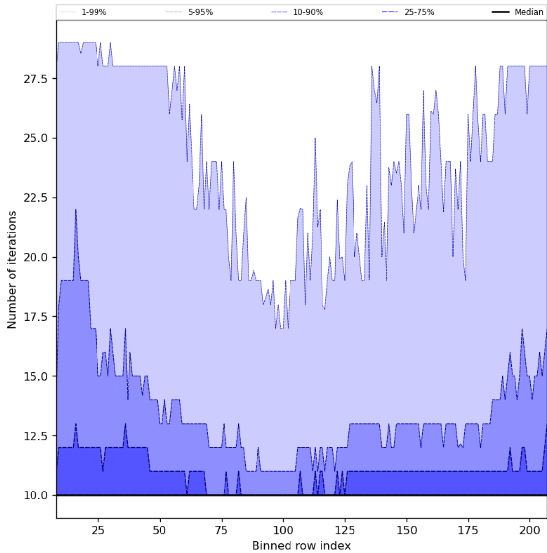
Figure 42: Along track statistics of “Number of iterations” for 2023-08-28 to 2023-08-30
