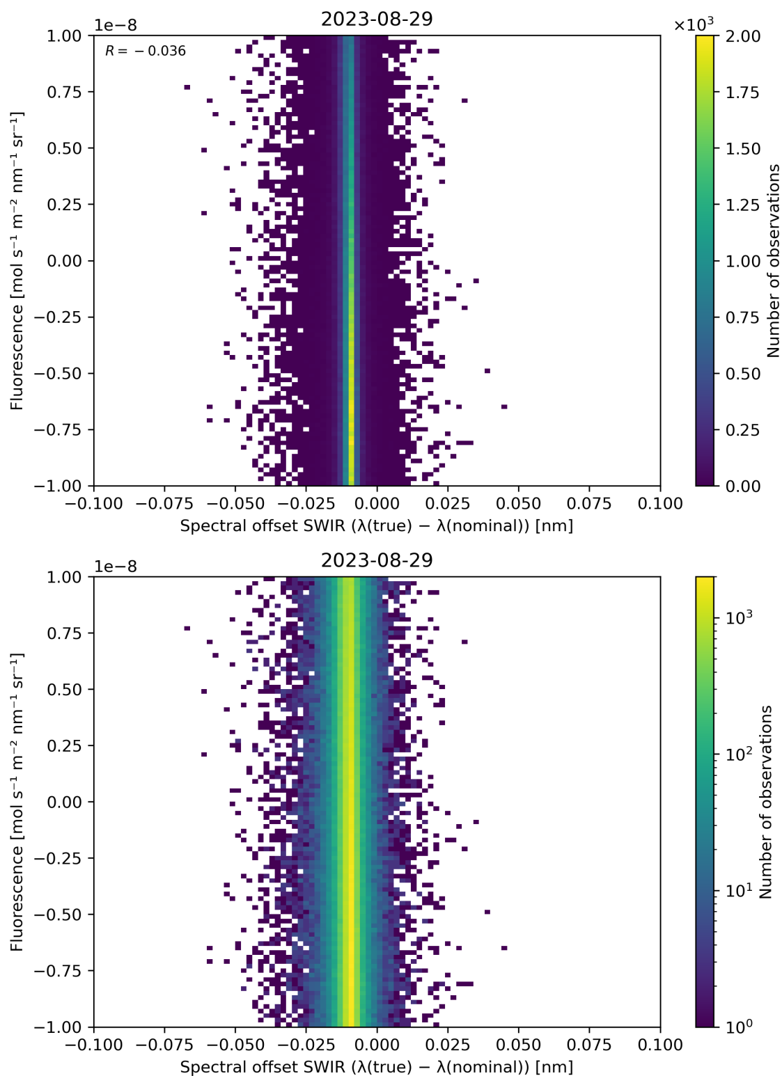
Figure 120: Scatter density plot of “Spectral offset SWIR ( \lambda(\text{true}) - \lambda(\text{nominal}) )” against “Fluorescence” for 2023-08-28 to 2023-08-30.
