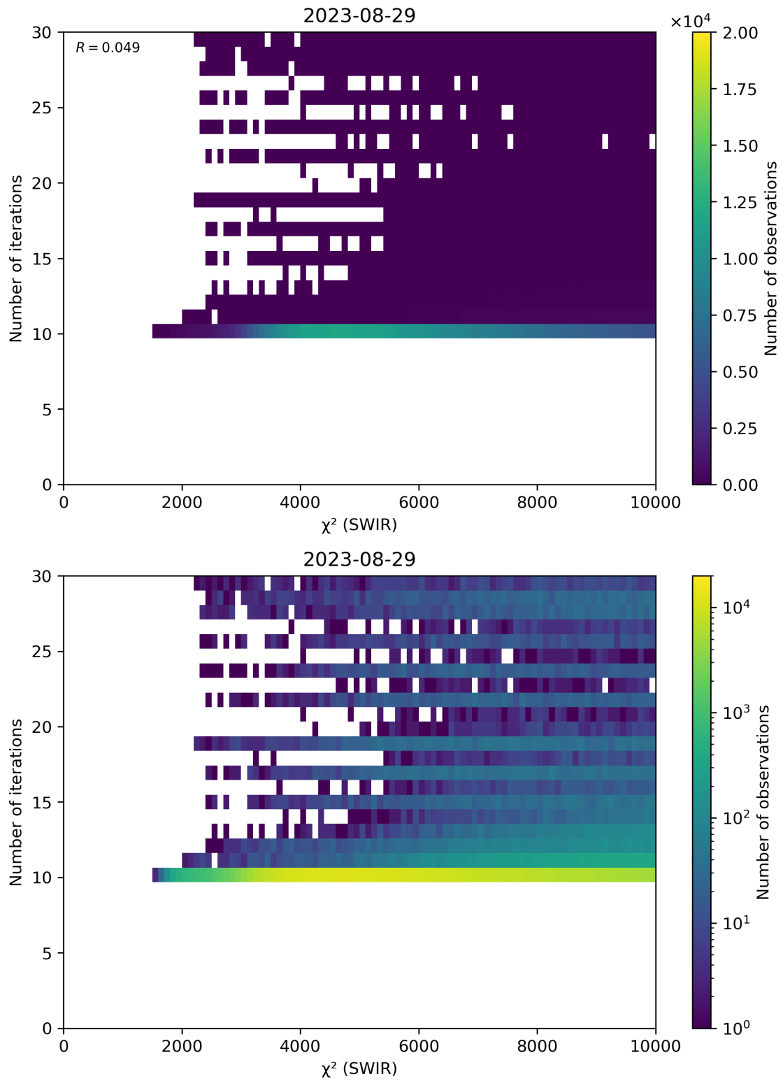
Figure 50: Scatter density plot of “ \chi^2 (SWIR)” against “Number of iterations” for 2023-08-28 to 2023-08-30.
