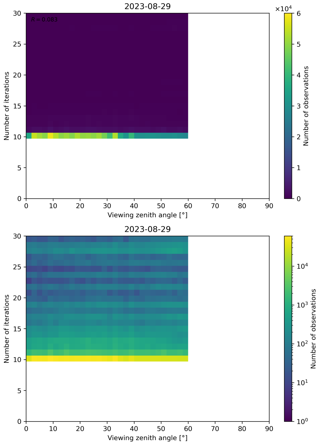
Figure 113: Scatter density plot of “Viewing zenith angle” against “Number of iterations” for 2023-08-28 to 2023-08-30.
