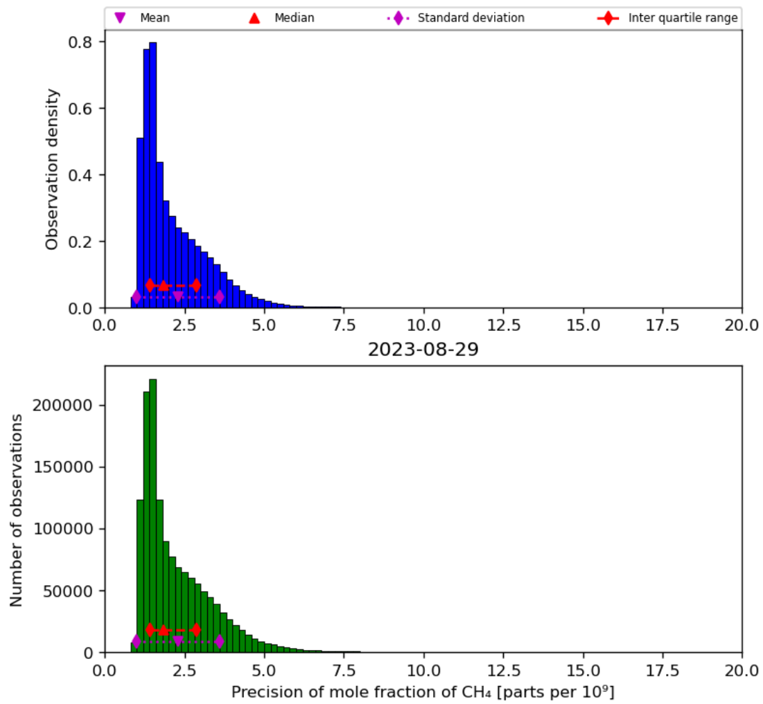
Figure 24: Histogram of “Precision of mole fraction of CH 4 ” for 2023-08-28 to 2023-08-30
