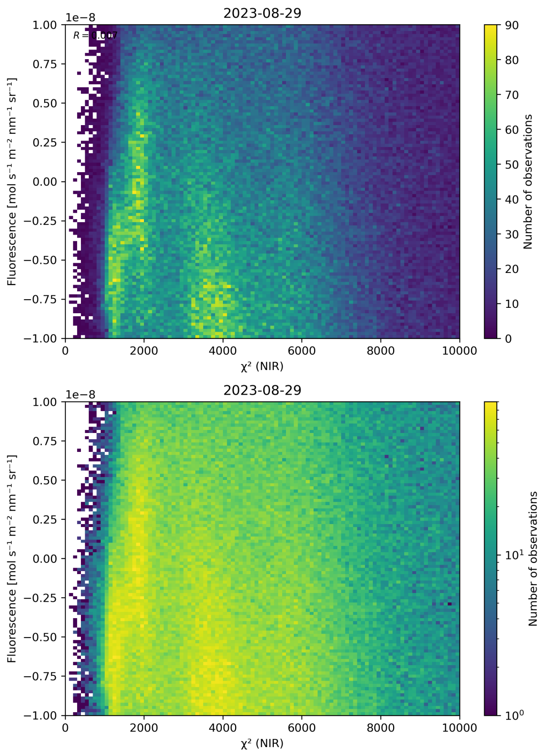
Figure 45: Scatter density plot of “ \chi^2 (NIR)” against “Fluorescence” for 2023-08-28 to 2023-08-30.
