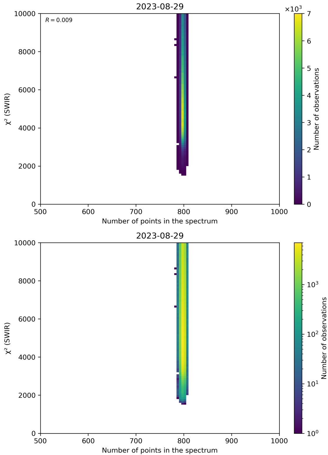
Figure 89: Scatter density plot of “Number of points in the spectrum” against “ \chi^2 (SWIR)” for 2023-08-28 to 2023-08-30.
