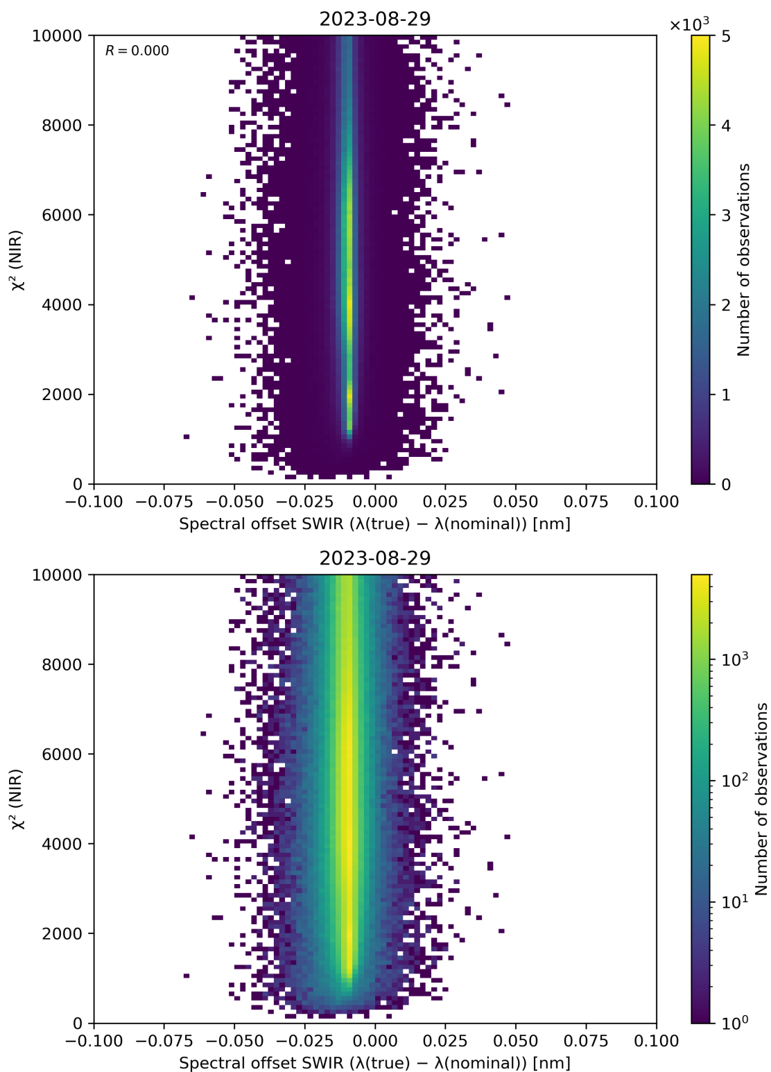
Figure 117: Scatter density plot of “Spectral offset SWIR ( \lambda(\text{true}) - \lambda(\text{nominal}) )” against “ \chi^2 (NIR)” for 2023-08-28 to 2023-08-30.
