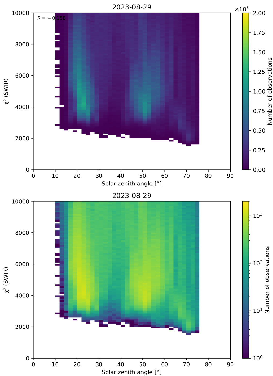
Figure 95: Scatter density plot of “Solar zenith angle” against “ \chi^2 (SWIR)” for 2023-08-28 to 2023-08-30.
