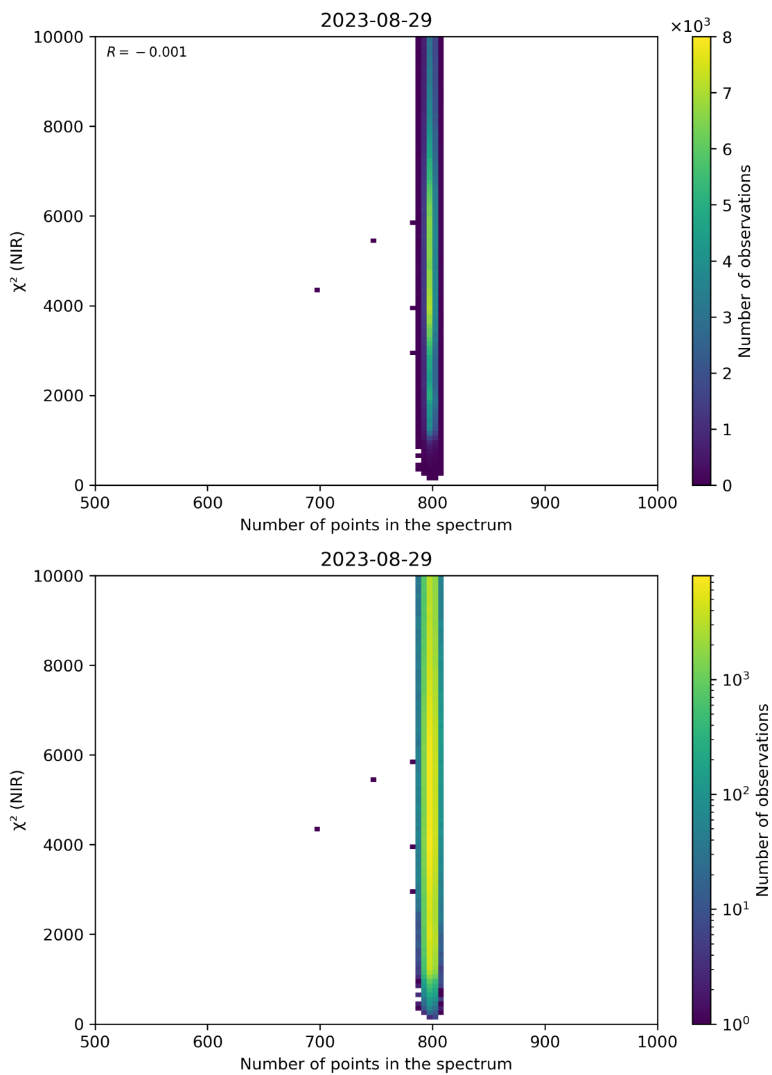
Figure 88: Scatter density plot of “Number of points in the spectrum” against “ \chi^2 (NIR)” for 2023-08-28 to 2023-08-30.
