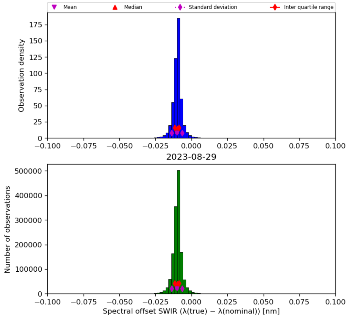
Figure 27: Histogram of “Spectral offset SWIR ( \lambda(\text{true}) - \lambda(\text{nominal}) )” for 2023-08-28 to 2023-08-30
