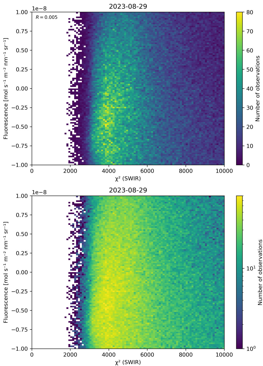
Figure 49: Scatter density plot of “ \chi^2 (SWIR)” against “Fluorescence” for 2023-08-28 to 2023-08-30.
