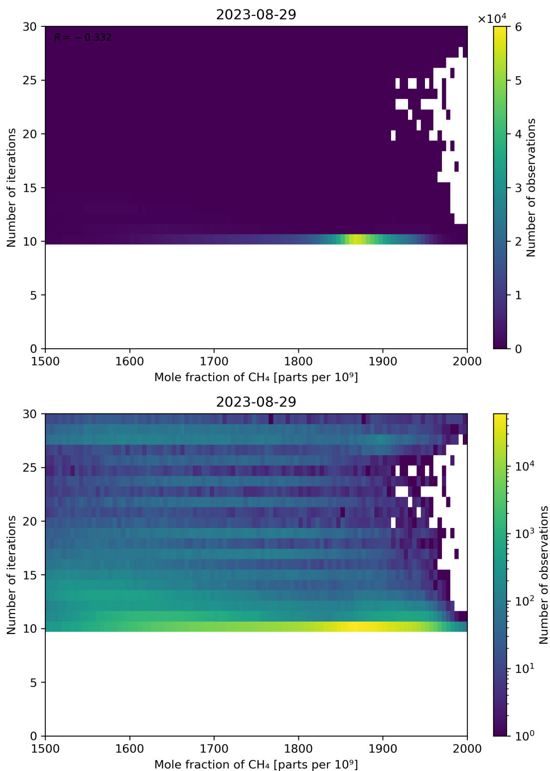
Figure 76: Scatter density plot of “Mole fraction of CH 4 ” against “Number of iterations” for 2023-08-28 to 2023-08-30.
