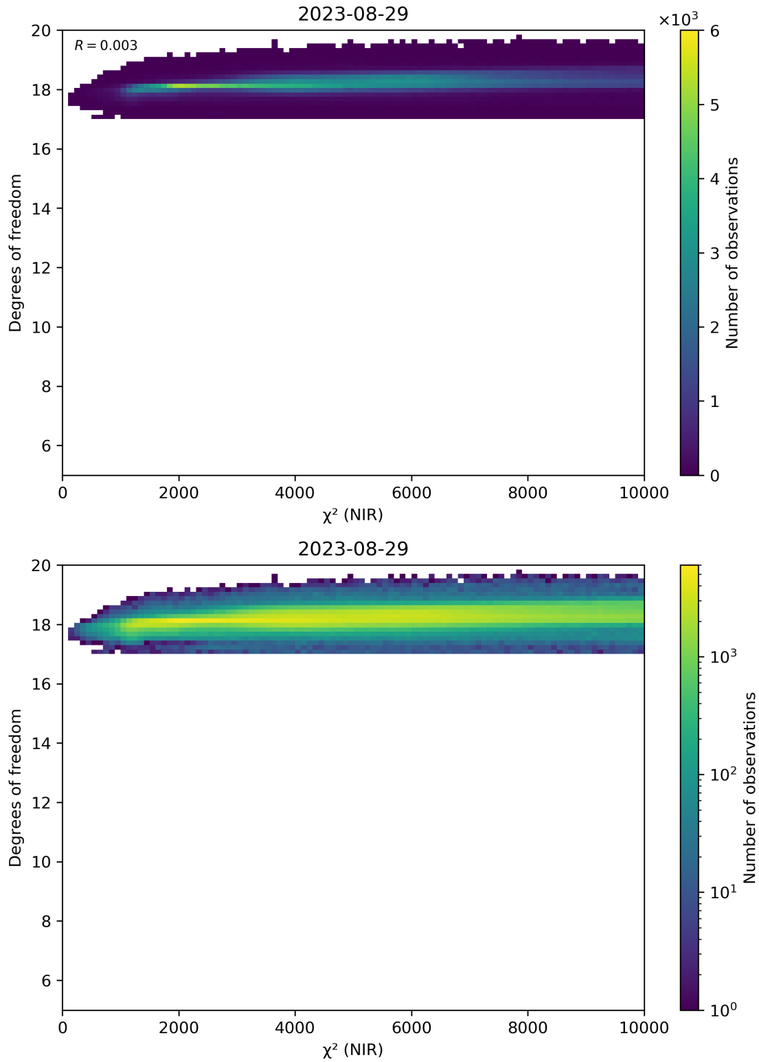
Figure 44: Scatter density plot of “ \chi^2 (NIR)” against “Degrees of freedom” for 2023-08-28 to 2023-08-30.
