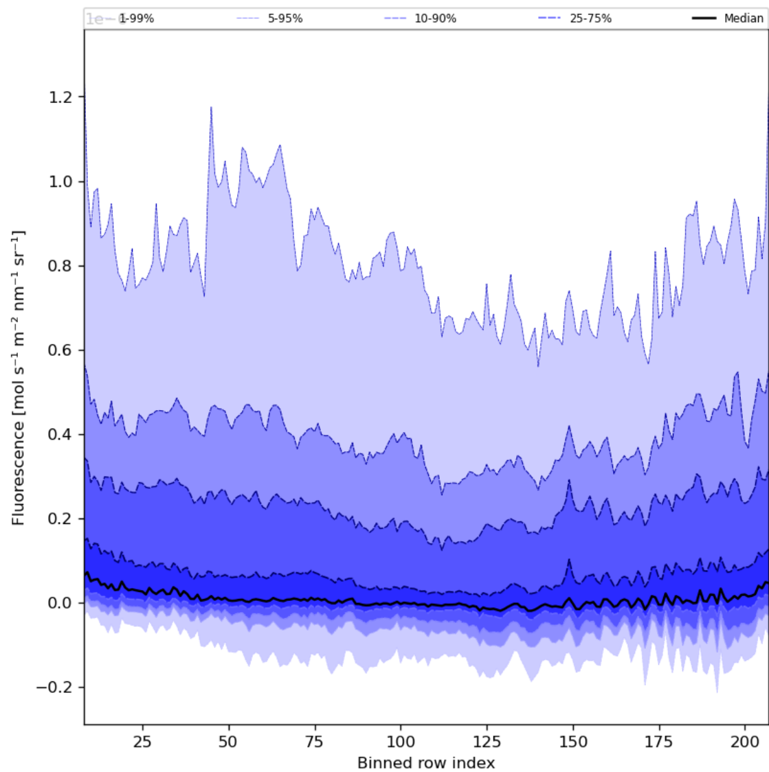
Figure 43: Along track statistics of “Fluorescence” for 2023-08-28 to 2023-08-30
