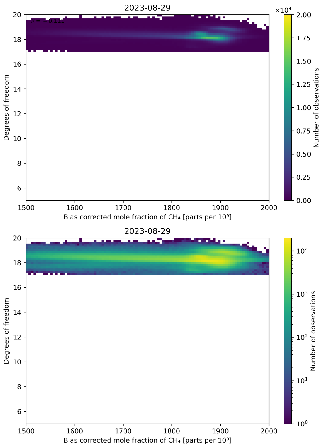
Figure 65: Scatter density plot of “Bias corrected mole fraction of CH 4 ” against “Degrees of freedom” for 2023-08-28 to 2023-08-30.
