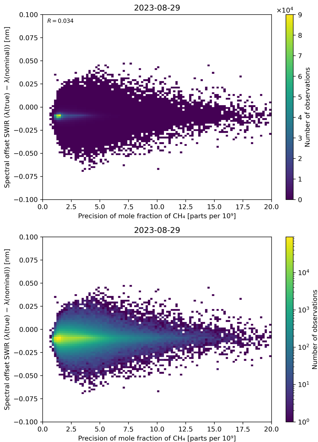
Figure 85: Scatter density plot of “Precision of mole fraction of CH 4 ” against “Spectral offset SWIR ( \lambda(\text{true}) - \lambda(\text{nominal}) )” for 2023-08-28 to 2023-08-30.
