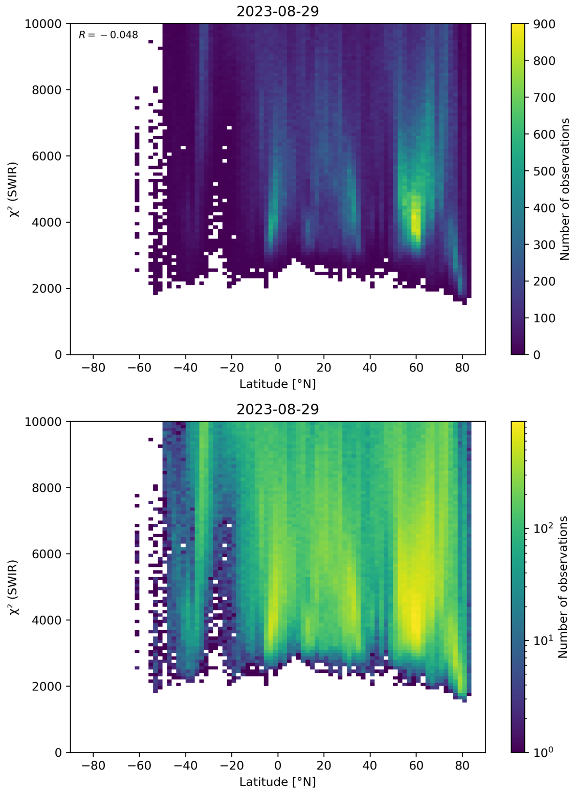
Figure 54: Scatter density plot of “Latitude” against “ \chi^2 (SWIR)” for 2023-08-28 to 2023-08-30.
