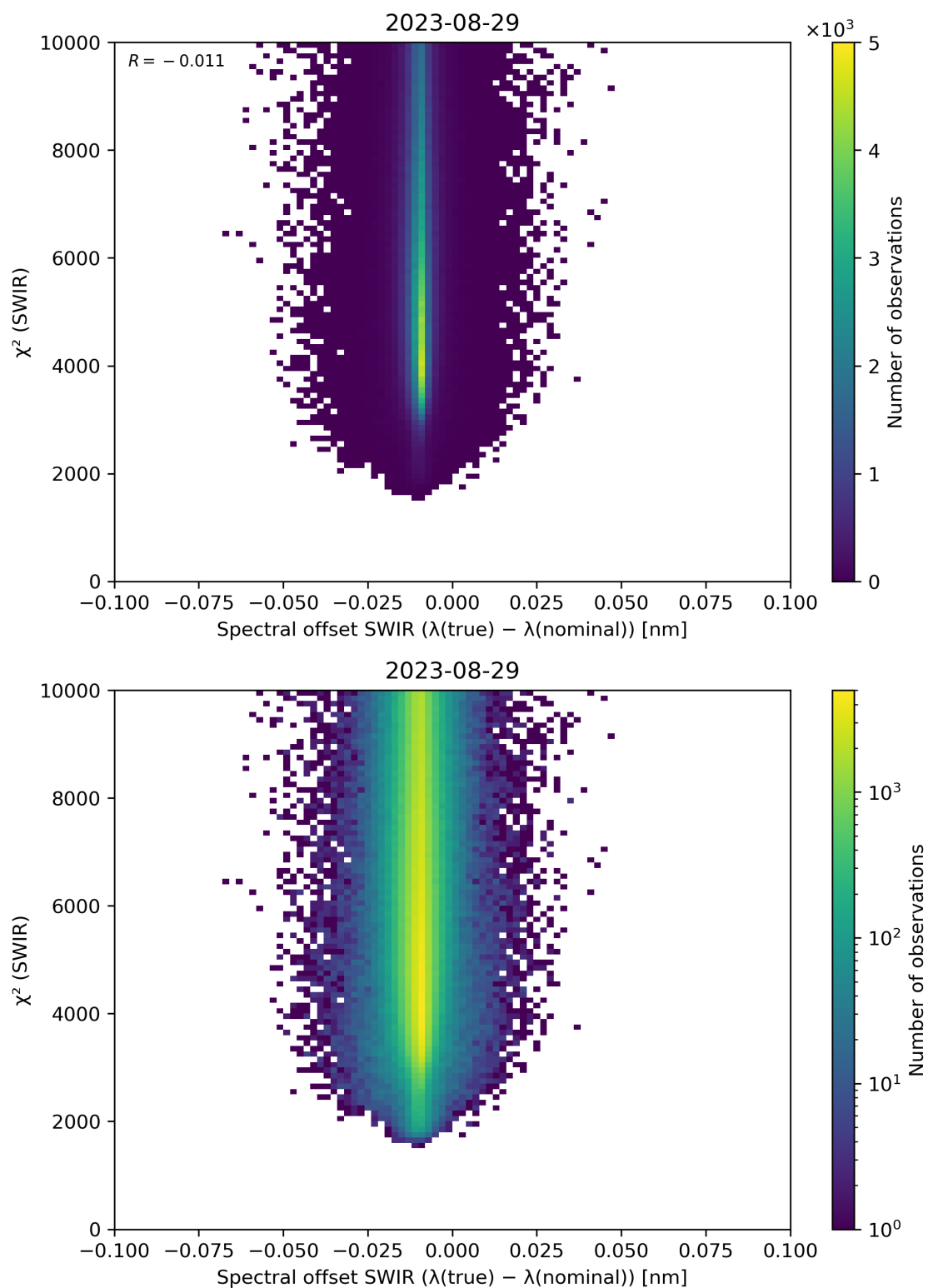
Figure 118: Scatter density plot of “Spectral offset SWIR ( \lambda(\text{true}) - \lambda(\text{nominal}) )” against “ \chi^2 (SWIR)” for 2023-08-28 to 2023-08-30.
