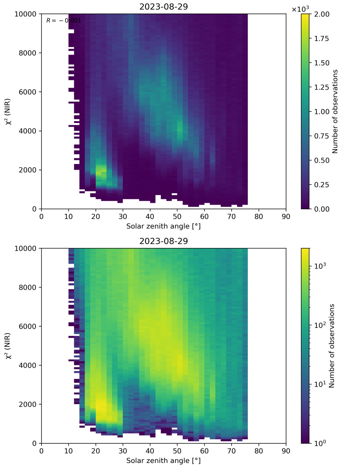
Figure 94: Scatter density plot of “Solar zenith angle” against “ \chi^2 (NIR)” for 2023-08-28 to 2023-08-30.
