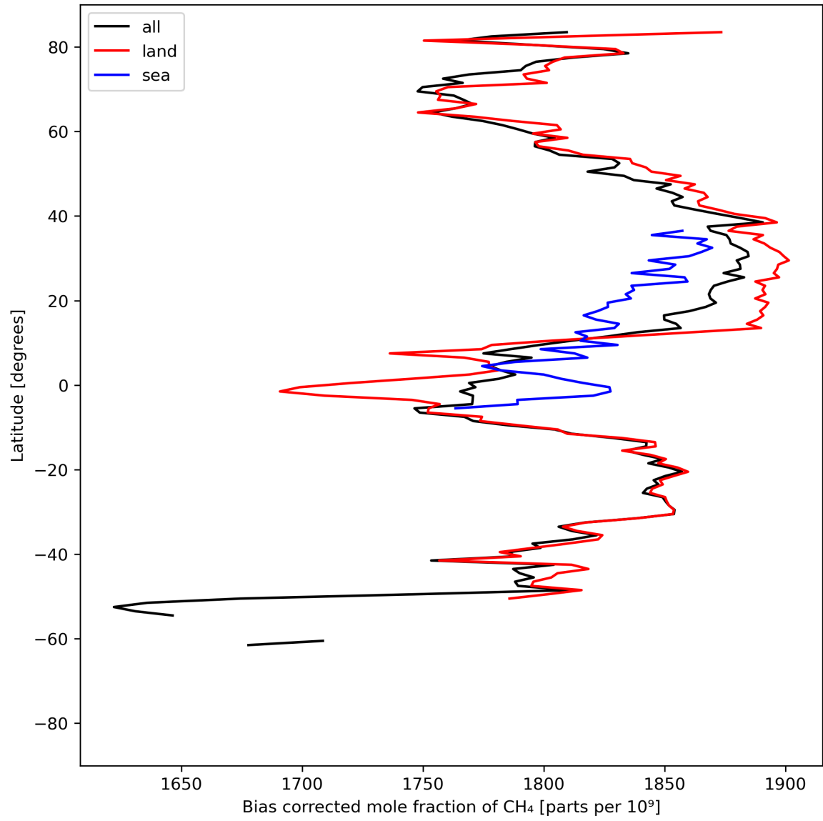
Figure 14: Zonal average of “Bias corrected mole fraction of CH 4 ” for 2023-08-28 to 2023-08-30.
