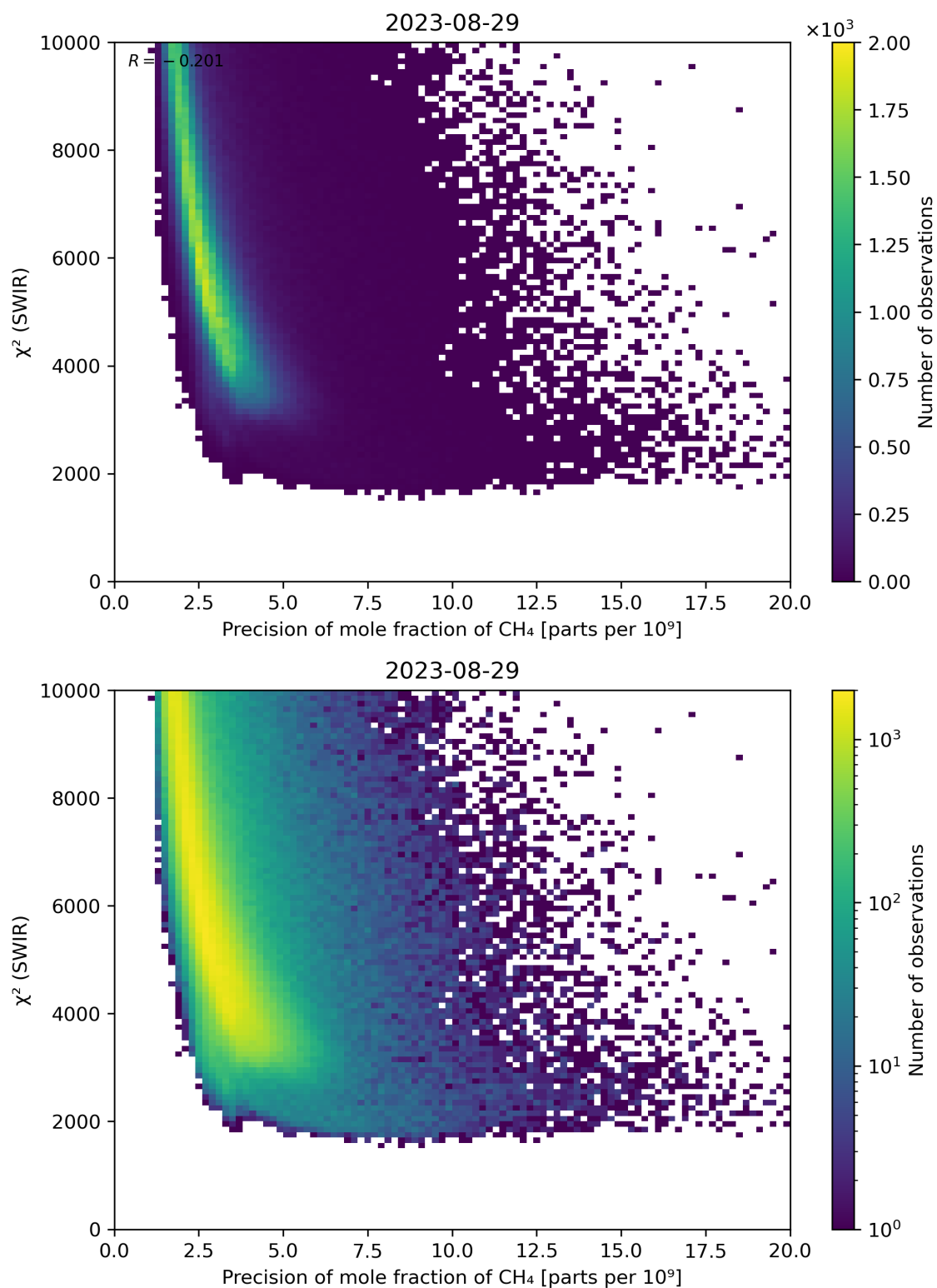
Figure 79: Scatter density plot of “Precision of mole fraction of \text{CH}_4 ” against “ \chi^2 (SWIR)” for 2023-08-28 to 2023-08-30.
