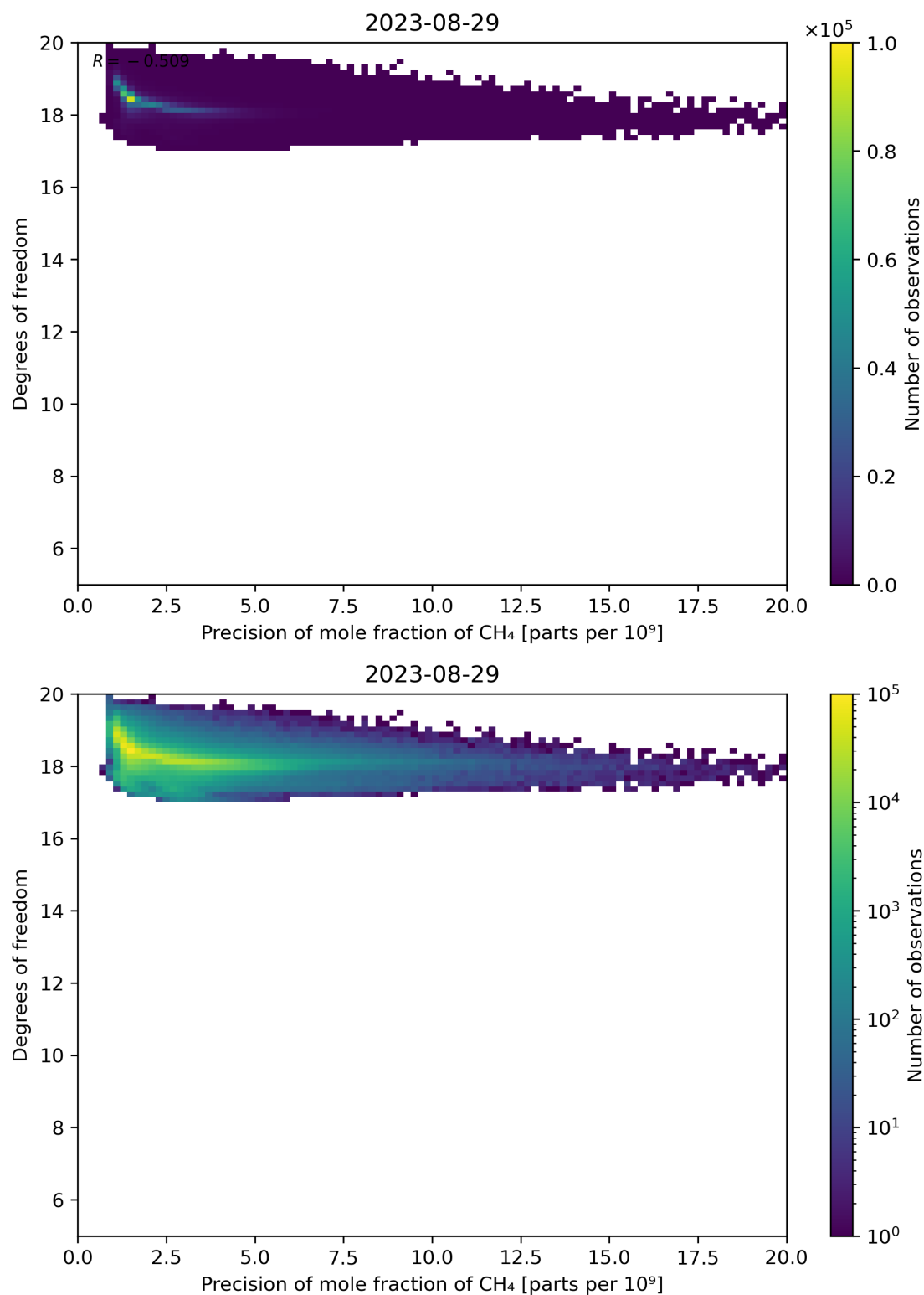
Figure 80: Scatter density plot of “Precision of mole fraction of CH 4 ” against “Degrees of freedom” for 2023-08-28 to 2023-08-30.
