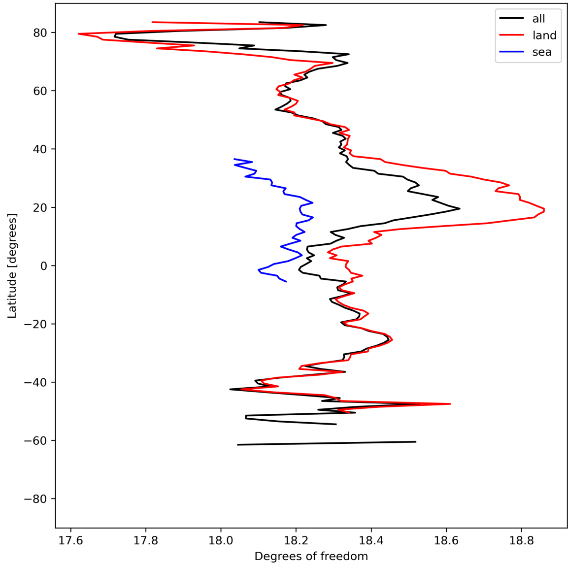
Figure 19: Zonal average of “Degrees of freedom” for 2023-08-28 to 2023-08-30.
