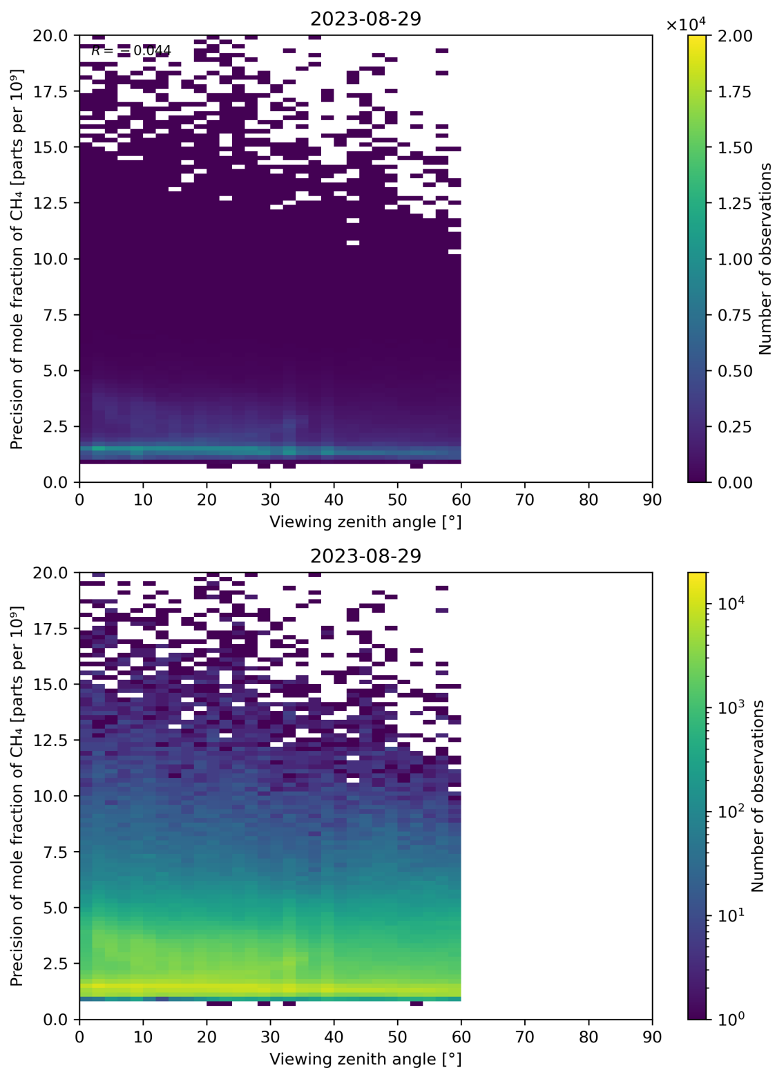
Figure 112: Scatter density plot of “Viewing zenith angle” against “Precision of mole fraction of CH 4 ” for 2023-08-28 to 2023-08-30.
