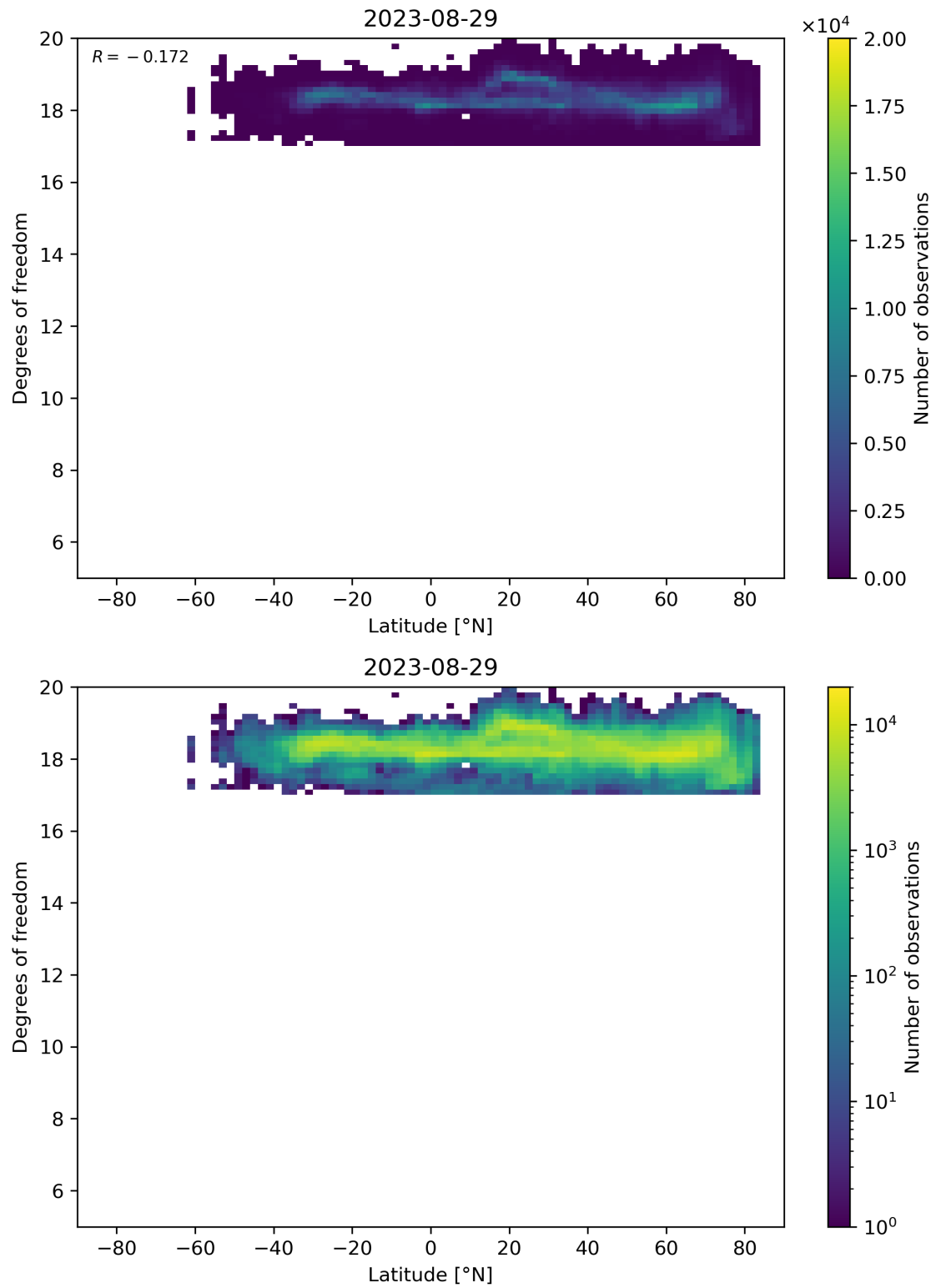
Figure 55: Scatter density plot of “Latitude” against “Degrees of freedom” for 2023-08-28 to 2023-08-30.
