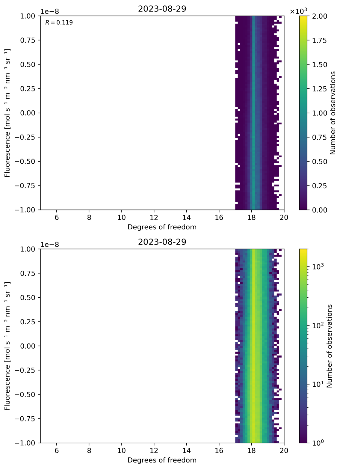
Figure 51: Scatter density plot of “Degrees of freedom” against “Fluorescence” for 2023-08-28 to 2023-08-30.
