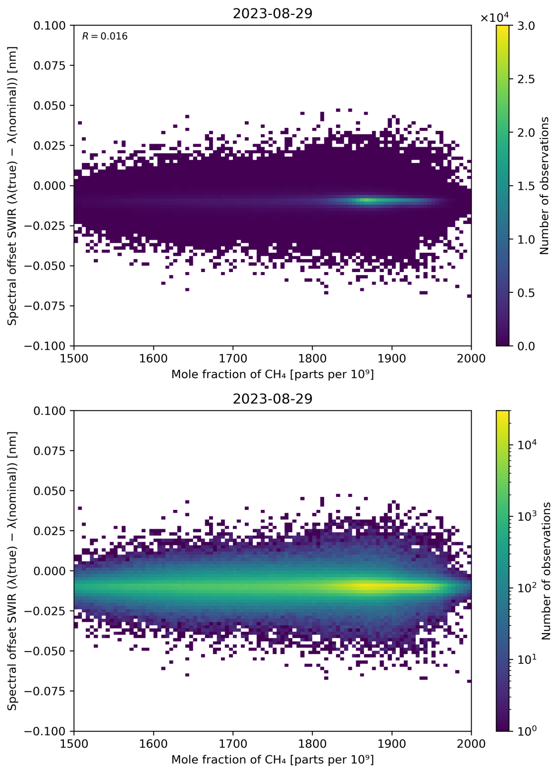
Figure 86: Scatter density plot of “Mole fraction of CH 4 ” against “Spectral offset SWIR ( \lambda(\text{true}) - \lambda(\text{nominal}) )” for 2023-08-28 to 2023-08-30.
