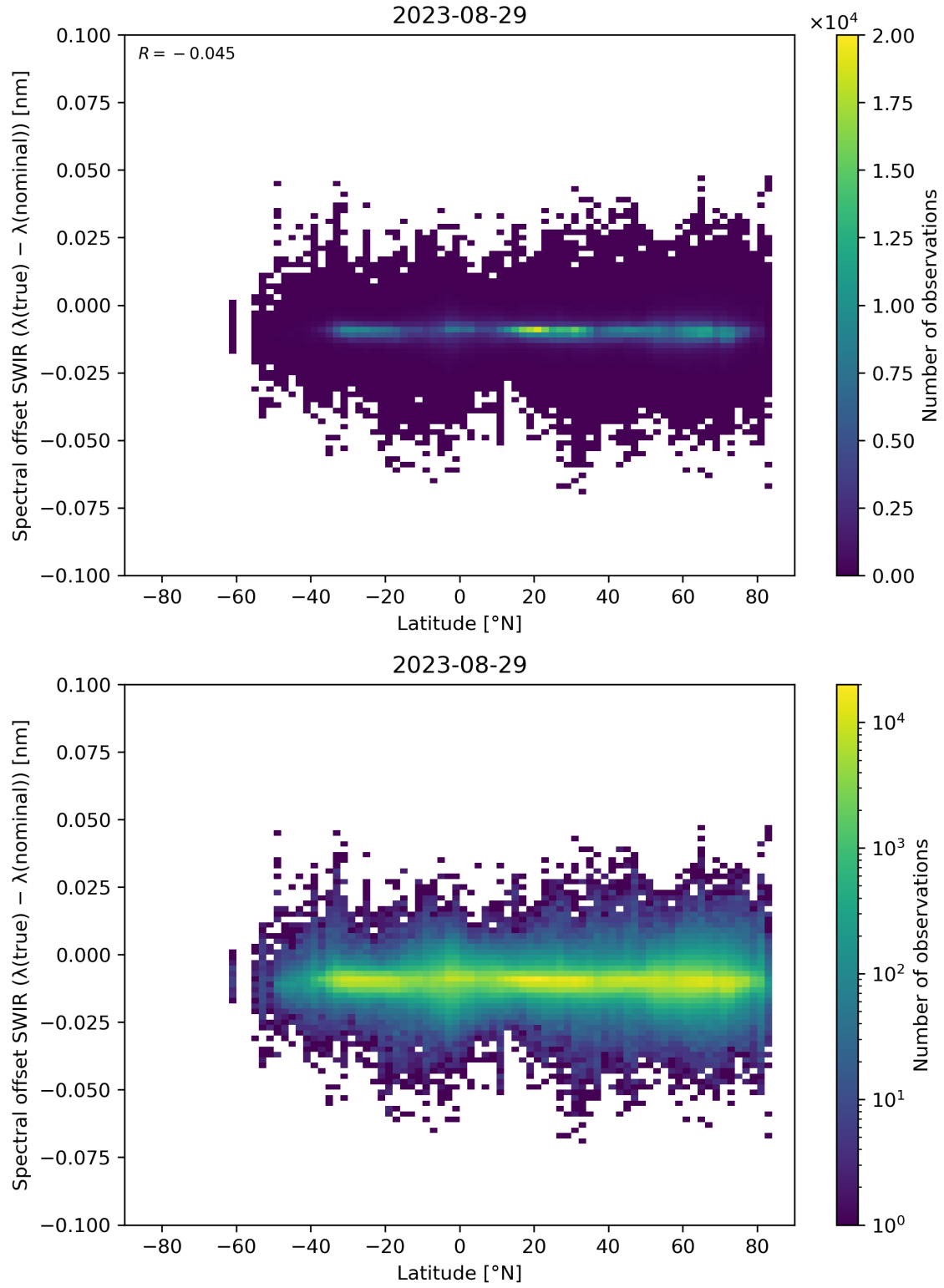
Figure 62: Scatter density plot of “Latitude” against “Spectral offset SWIR ( \lambda(\text{true}) - \lambda(\text{nominal}) )” for 2023-08-28 to 2023-08-30.
