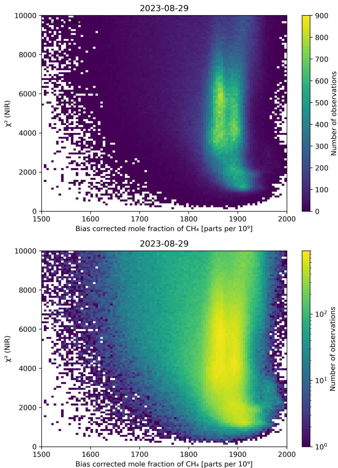
Figure 63: Scatter density plot of “Bias corrected mole fraction of CH 4 ” against “ \chi^2 (NIR)” for 2023-08-28 to 2023-08-30.
