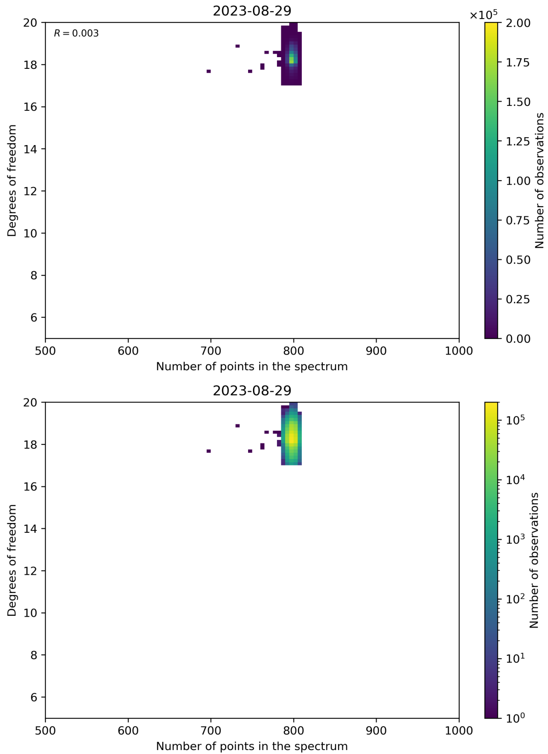
Figure 90: Scatter density plot of “Number of points in the spectrum” against “Degrees of freedom” for 2023-08-28 to 2023-08-30.
