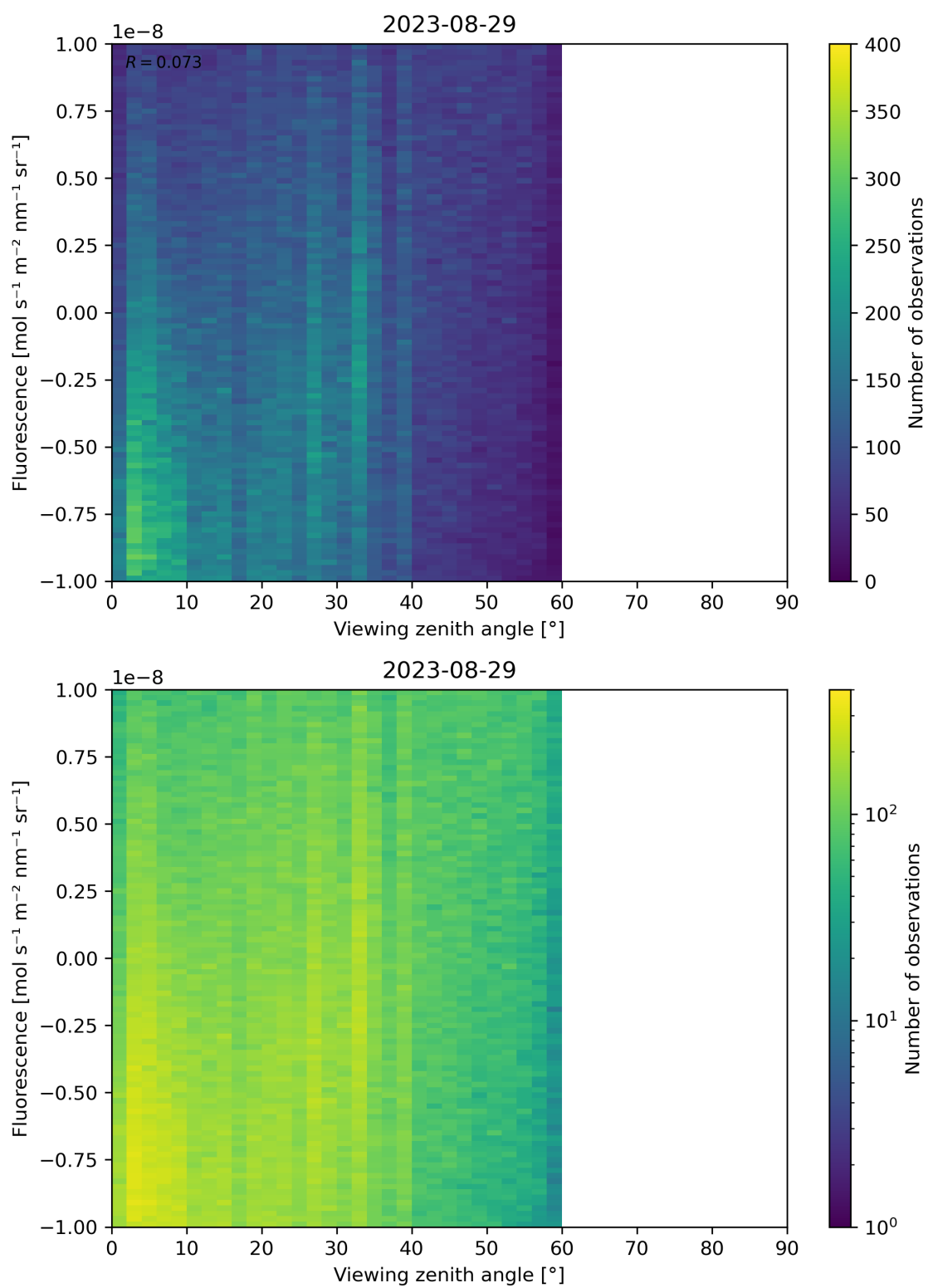
Figure 108: Scatter density plot of “Viewing zenith angle” against “Fluorescence” for 2023-08-28 to 2023-08-30.
