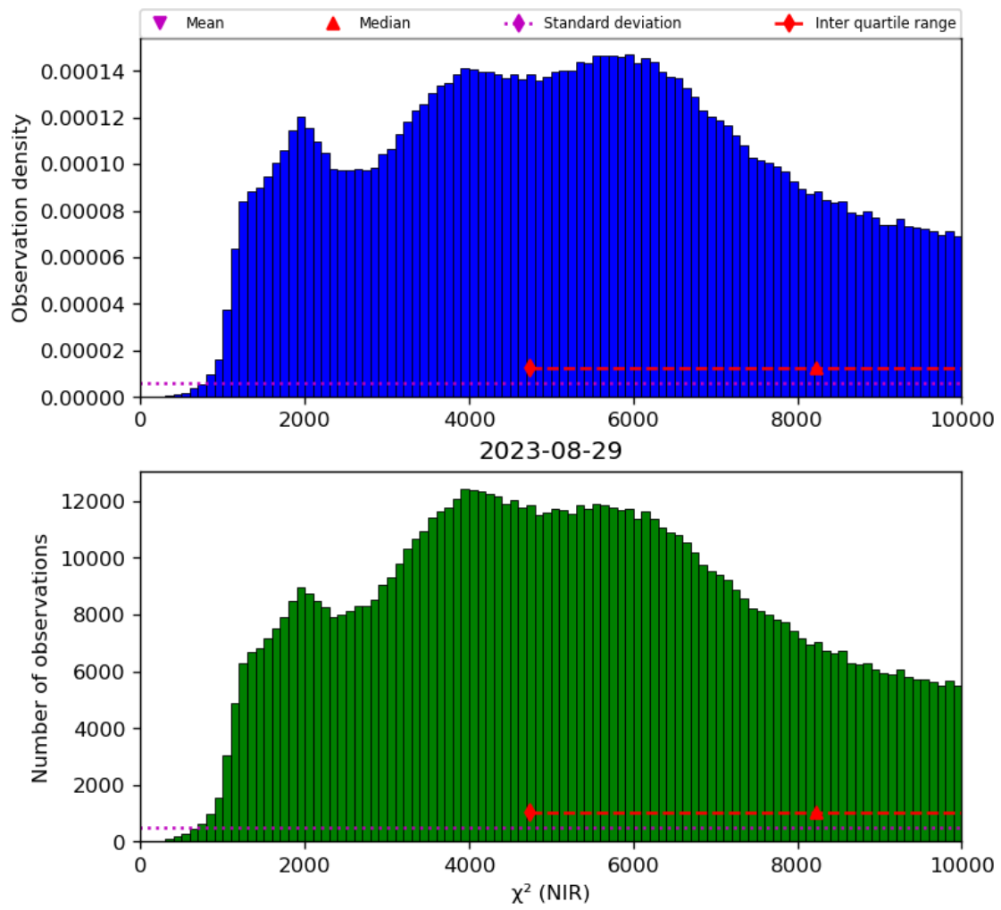
Figure 29: Histogram of " \chi^2 (NIR)" for 2023-08-28 to 2023-08-30
