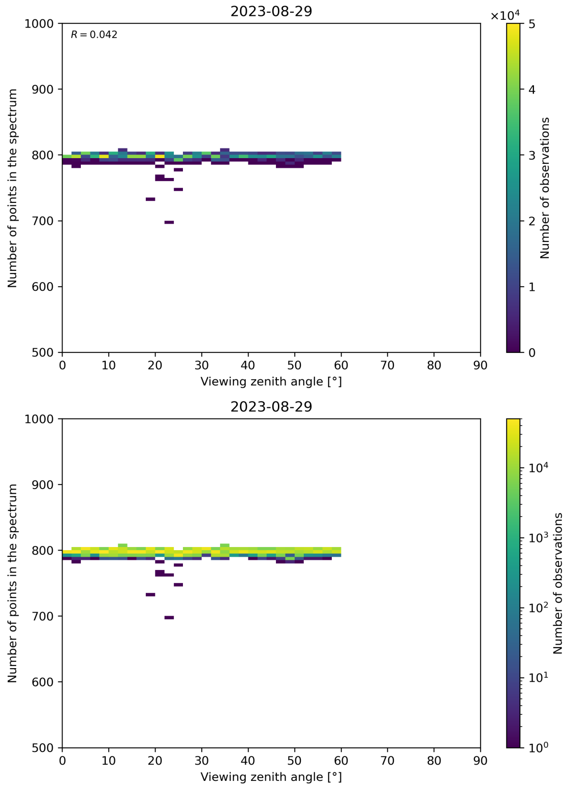
Figure 114: Scatter density plot of “Viewing zenith angle” against “Number of points in the spectrum” for 2023-08-28 to 2023-08-30.
