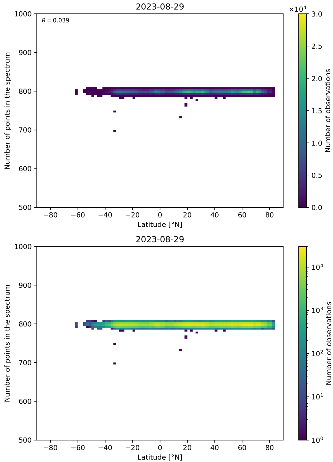
Figure 61: Scatter density plot of “Latitude” against “Number of points in the spectrum” for 2023-08-28 to 2023-08-30.
