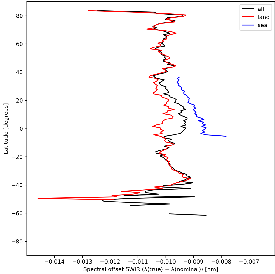
Figure 16: Zonal average of “Spectral offset SWIR ( \lambda(\text{true}) - \lambda(\text{nominal}) )” for 2023-08-28 to 2023-08-30.
