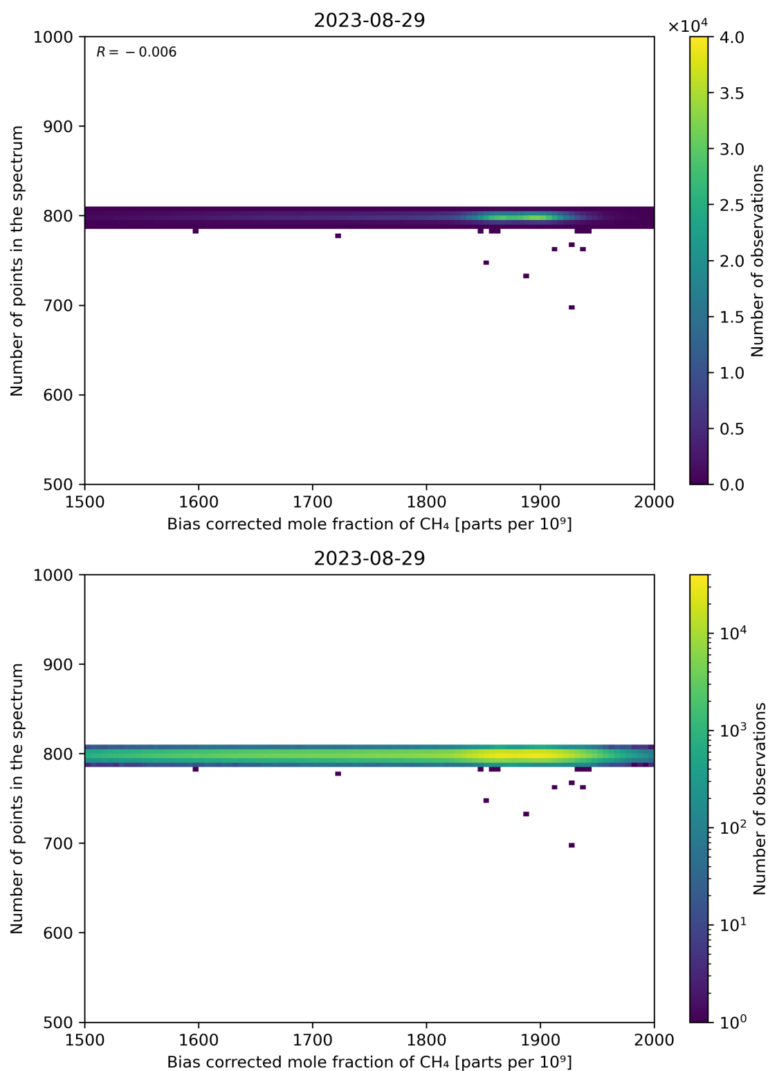
Figure 68: Scatter density plot of “Bias corrected mole fraction of CH 4 ” against “Number of points in the spectrum” for 2023-08-28 to 2023-08-30.
