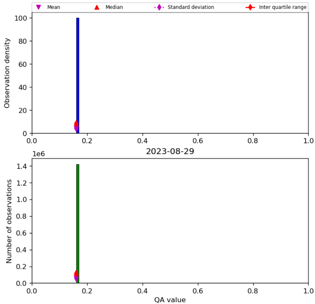
Figure 22: Histogram of “QA value” for 2023-08-28 to 2023-08-30
