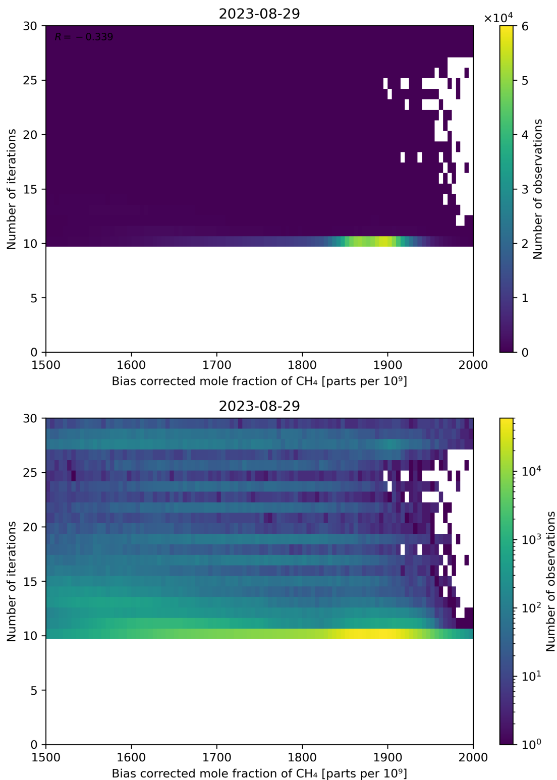
Figure 67: Scatter density plot of “Bias corrected mole fraction of CH 4 ” against “Number of iterations” for 2023-08-28 to 2023-08-30.
