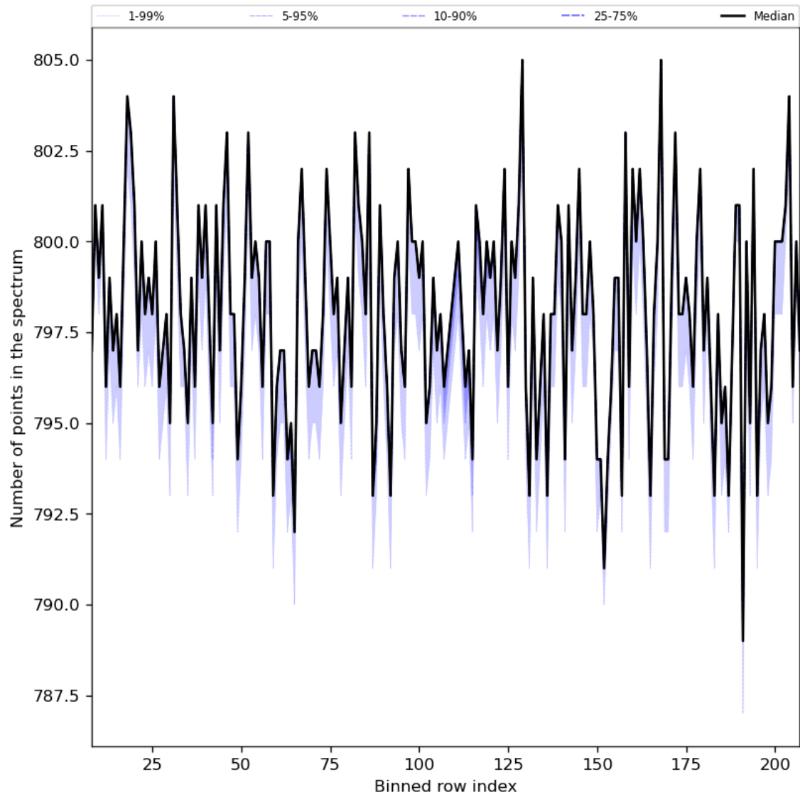
Figure 37: Along track statistics of “Number of points in the spectrum” for 2023-08-28 to 2023-08-30
