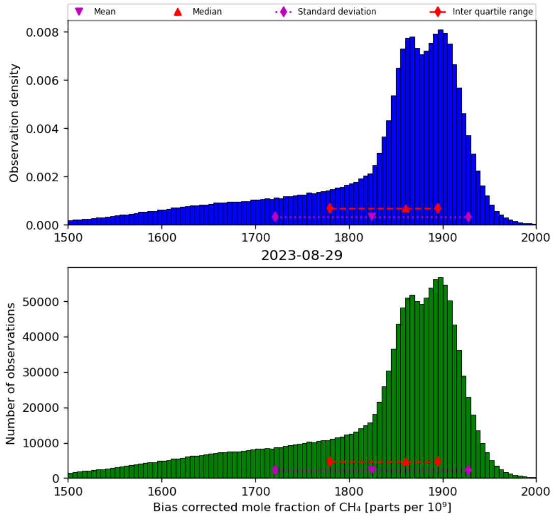
Figure 25: Histogram of “Bias corrected mole fraction of CH 4 ” for 2023-08-28 to 2023-08-30
