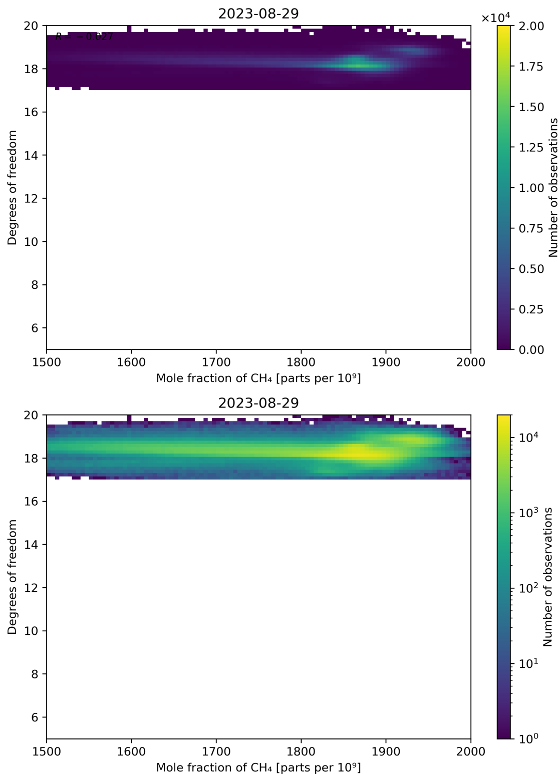
Figure 72: Scatter density plot of “Mole fraction of CH 4 ” against “Degrees of freedom” for 2023-08-28 to 2023-08-30.
