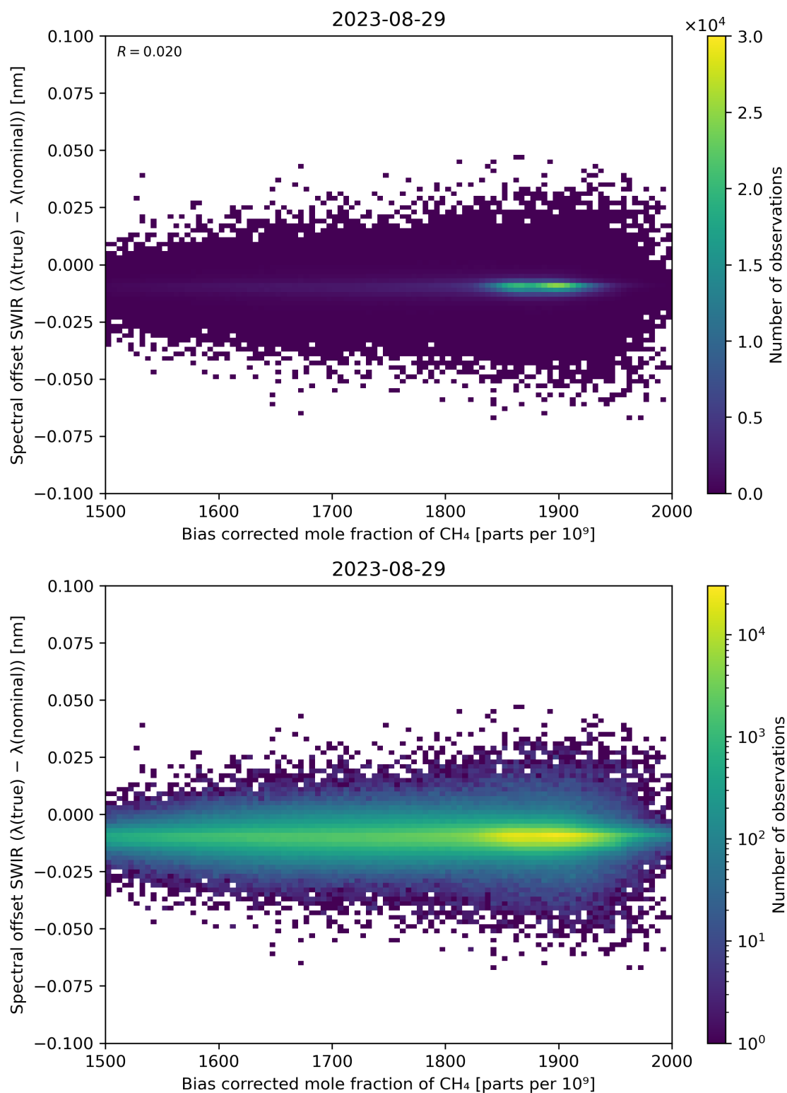
Figure 69: Scatter density plot of “Bias corrected mole fraction of \text{CH}_4 ” against “Spectral offset SWIR ( \lambda(\text{true}) - \lambda(\text{nominal}) )” for 2023-08-28 to 2023-08-30.
