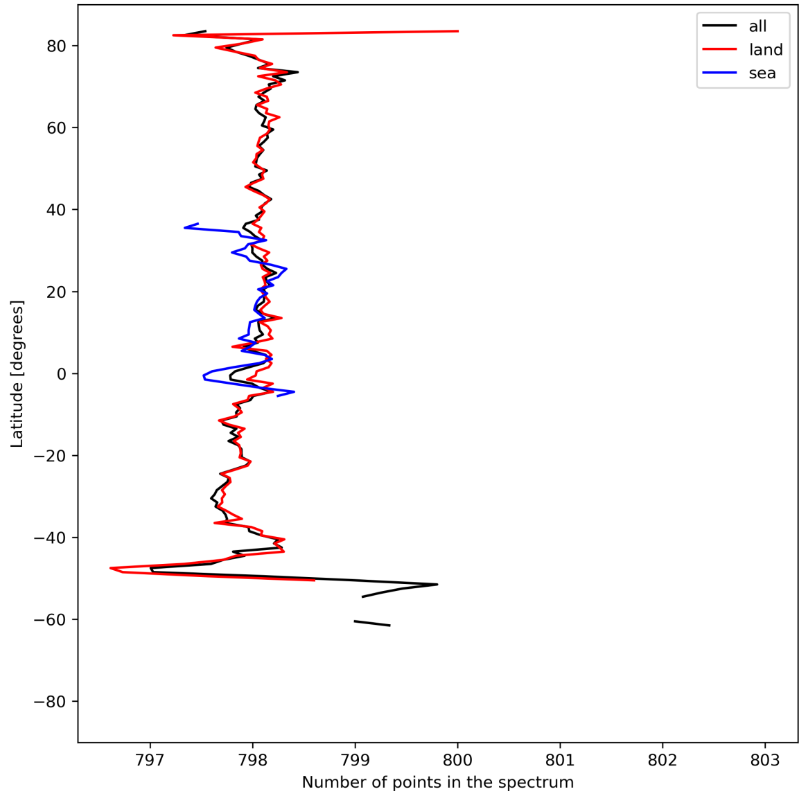
Figure 15: Zonal average of “Number of points in the spectrum” for 2023-08-28 to 2023-08-30.
