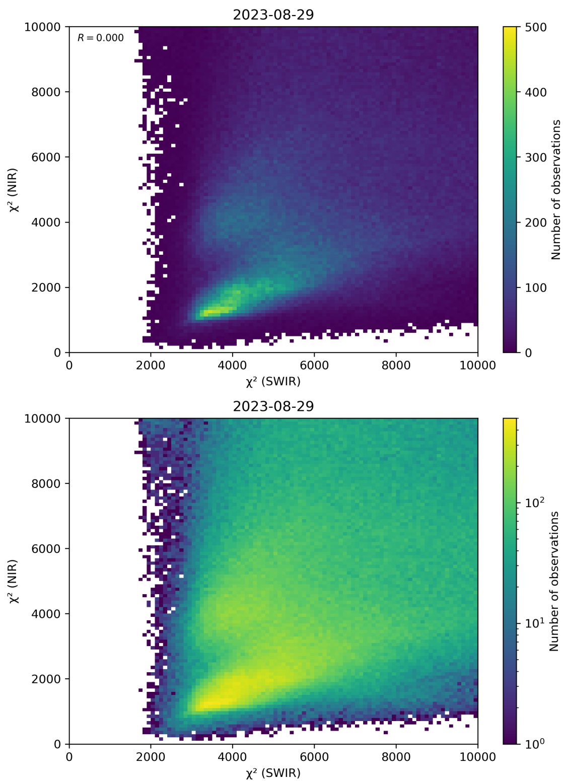
Figure 47: Scatter density plot of “ \chi^2 (SWIR)” against “ \chi^2 (NIR)” for 2023-08-28 to 2023-08-30.
