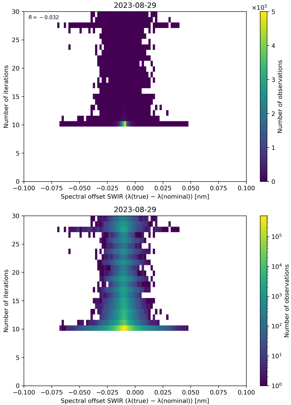
Figure 121: Scatter density plot of “Spectral offset SWIR ( \lambda(\text{true}) - \lambda(\text{nominal}) )” against “Number of iterations” for 2023-08-28 to 2023-08-30.
