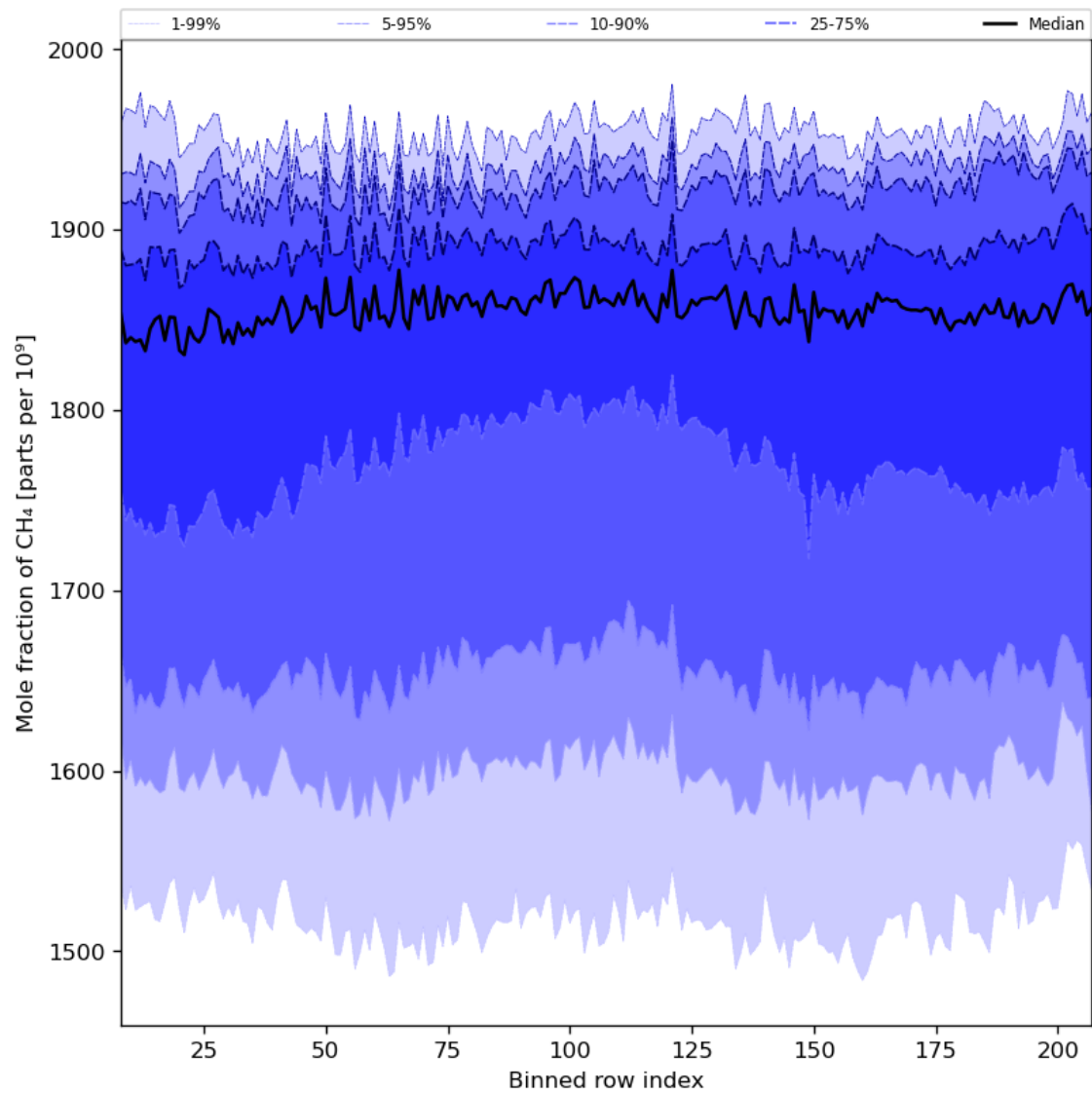
Figure 34: Along track statistics of “Mole fraction of CH 4 ” for 2023-08-28 to 2023-08-30
