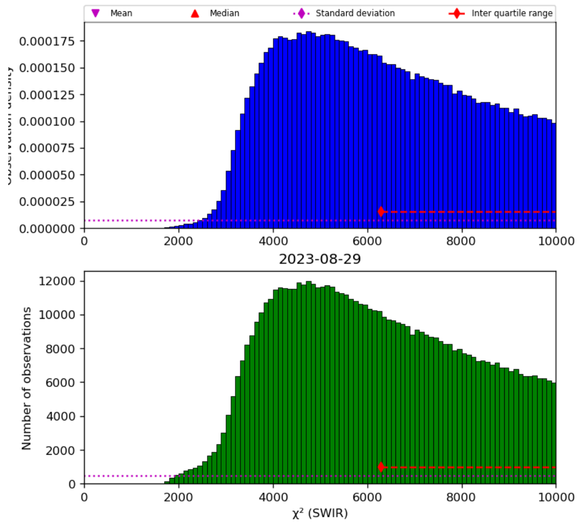
Figure 28: Histogram of “ \chi^2 (SWIR)” for 2023-08-28 to 2023-08-30
