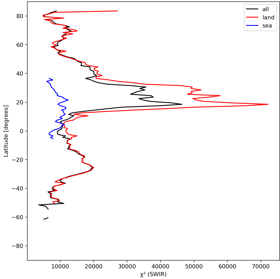
Figure 17: Zonal average of “ \chi^2 (SWIR)” for 2023-08-28 to 2023-08-30.
