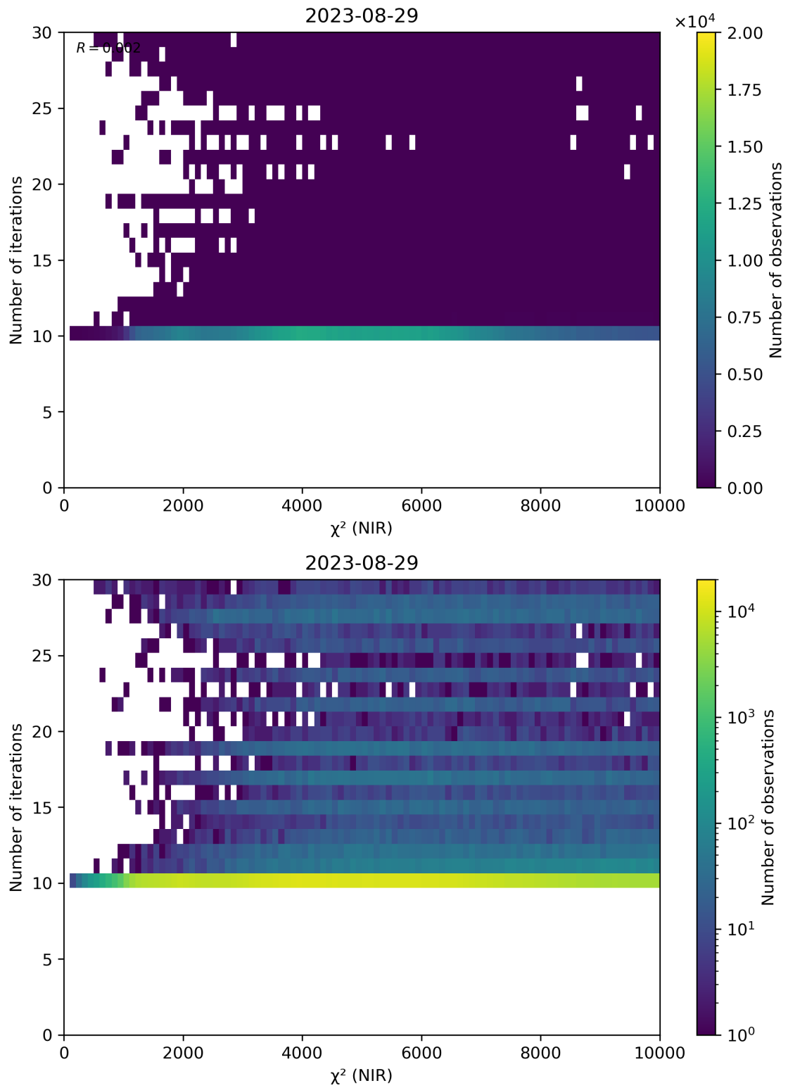
Figure 46: Scatter density plot of “ \chi^2 (NIR)” against “Number of iterations” for 2023-08-28 to 2023-08-30.
