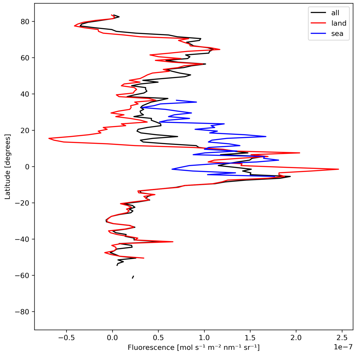
Figure 21: Zonal average of “Fluorescence” for 2023-08-28 to 2023-08-30.
