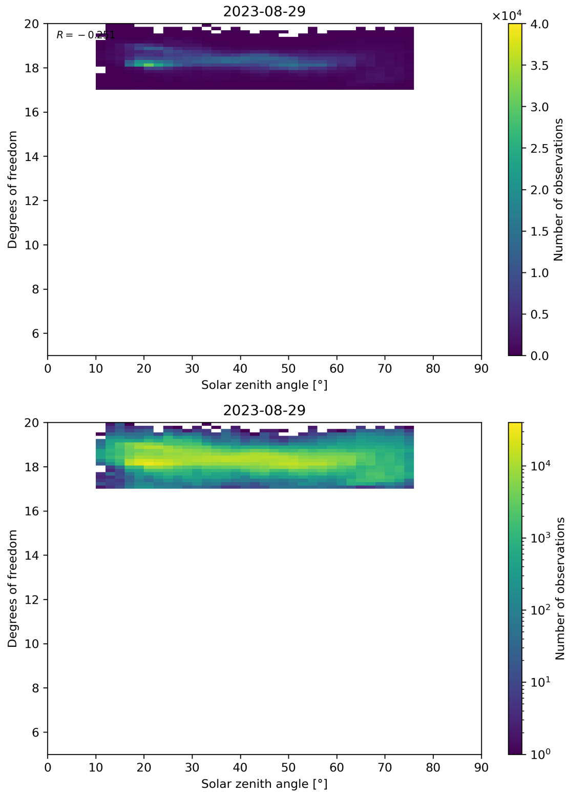
Figure 96: Scatter density plot of “Solar zenith angle” against “Degrees of freedom” for 2023-08-28 to 2023-08-30.
