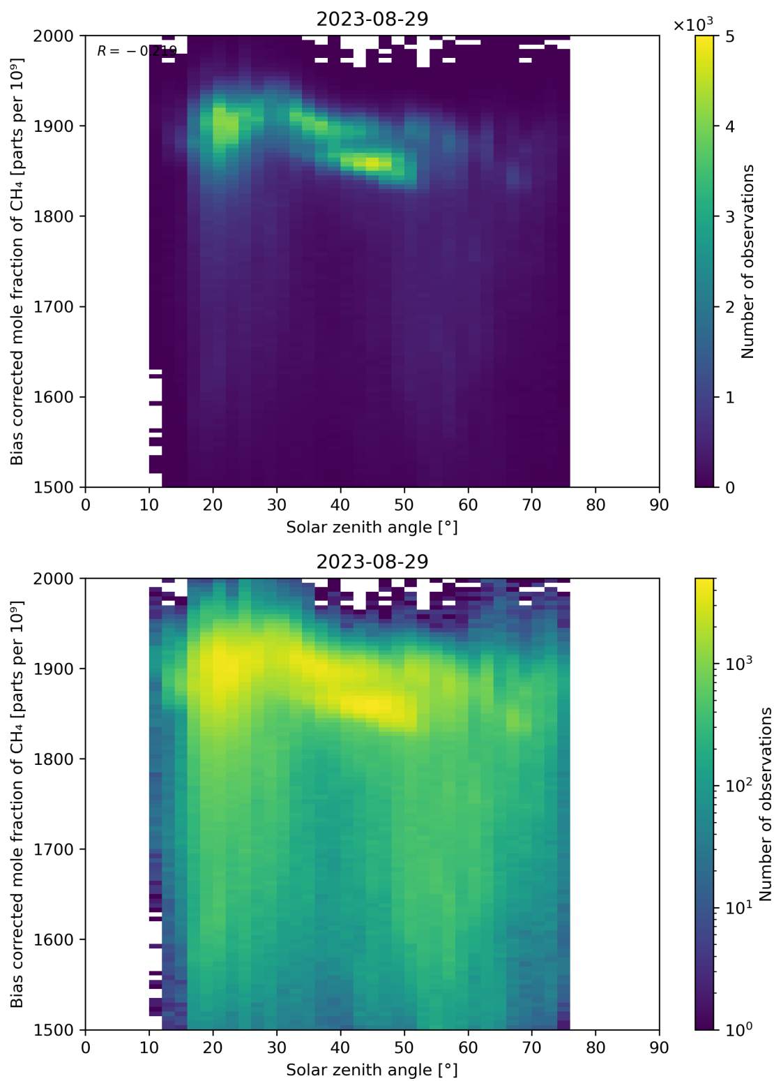
Figure 100: Scatter density plot of “Solar zenith angle” against “Bias corrected mole fraction of CH 4 ” for 2023-08-28 to 2023-08-30.
