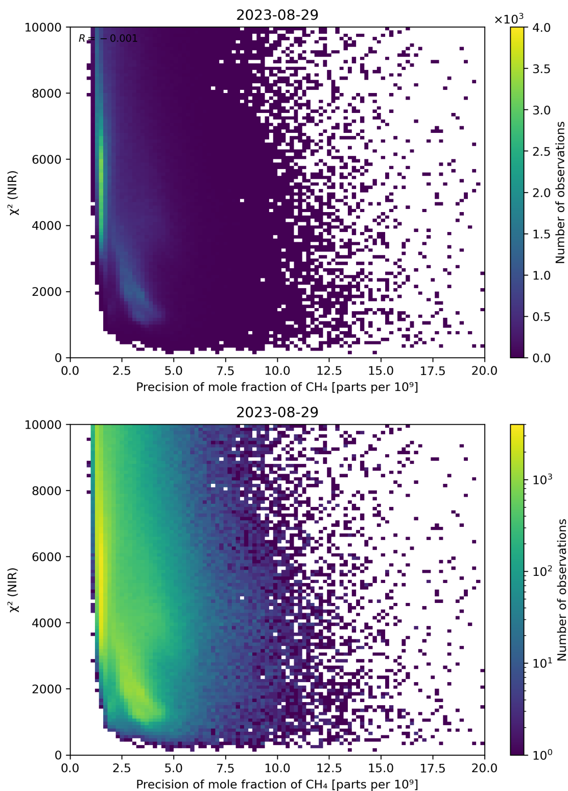
Figure 78: Scatter density plot of “Precision of mole fraction of \text{CH}_4 ” against “ \chi^2 (NIR)” for 2023-08-28 to 2023-08-30.
