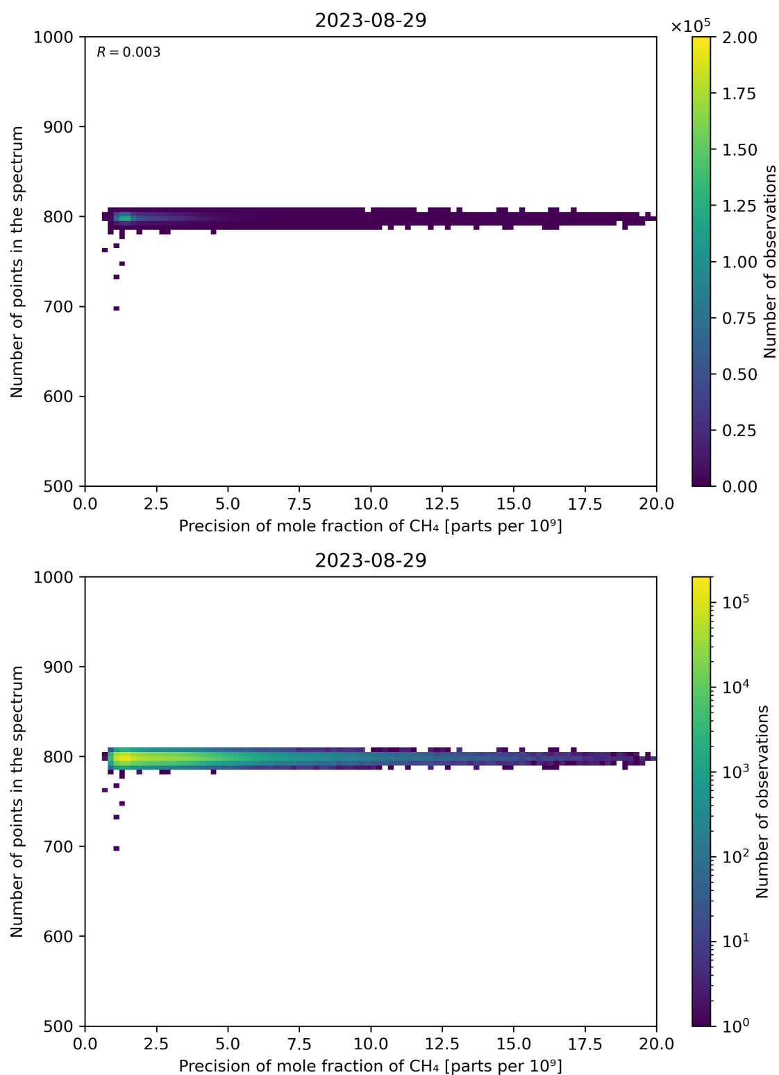
Figure 84: Scatter density plot of “Precision of mole fraction of CH 4 ” against “Number of points in the spectrum” for 2023-08-28 to 2023-08-30.
