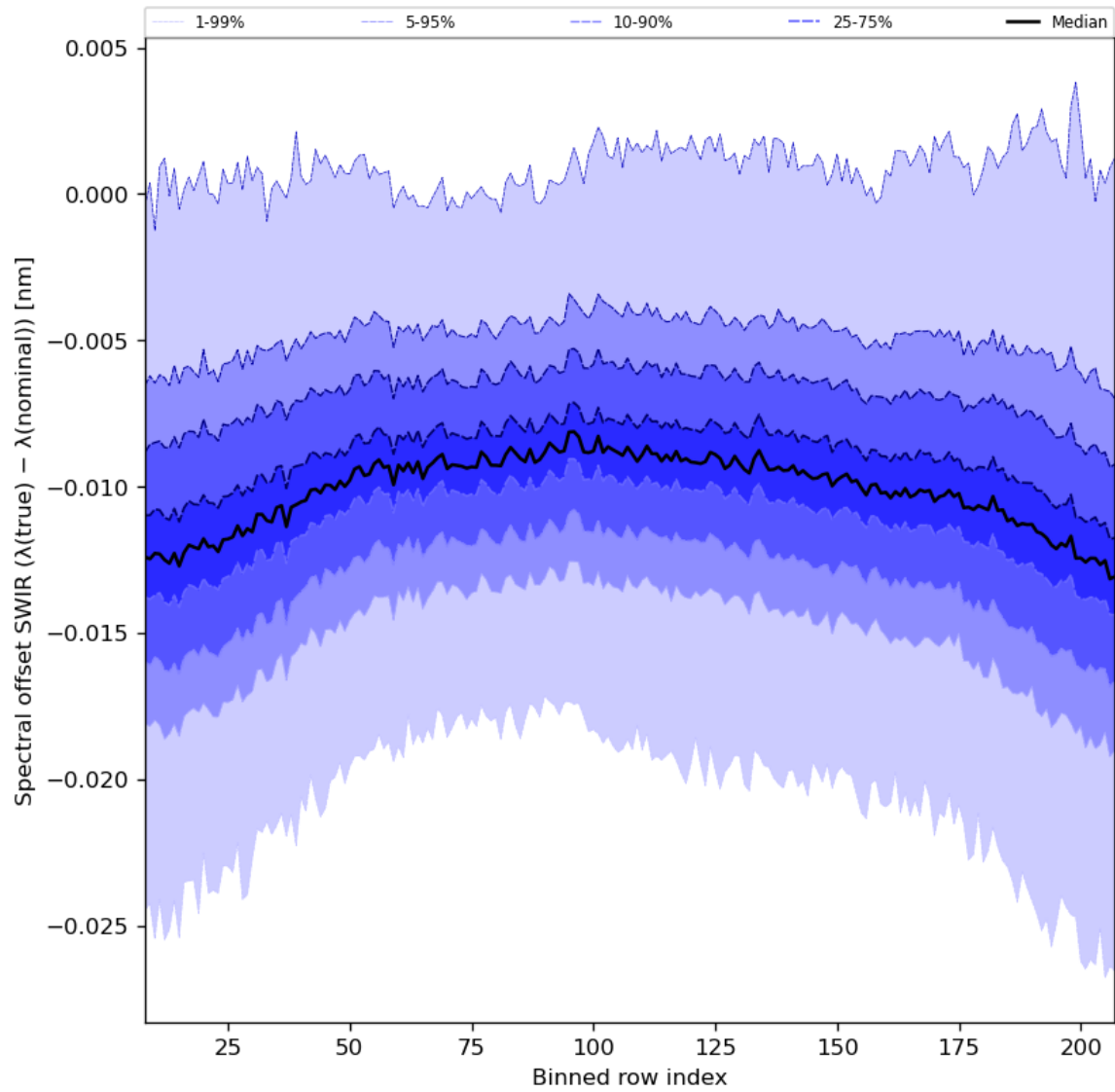
Figure 38: Along track statistics of “Spectral offset SWIR ( \lambda(\text{true}) - \lambda(\text{nominal}) )” for 2023-08-28 to 2023-08-30
