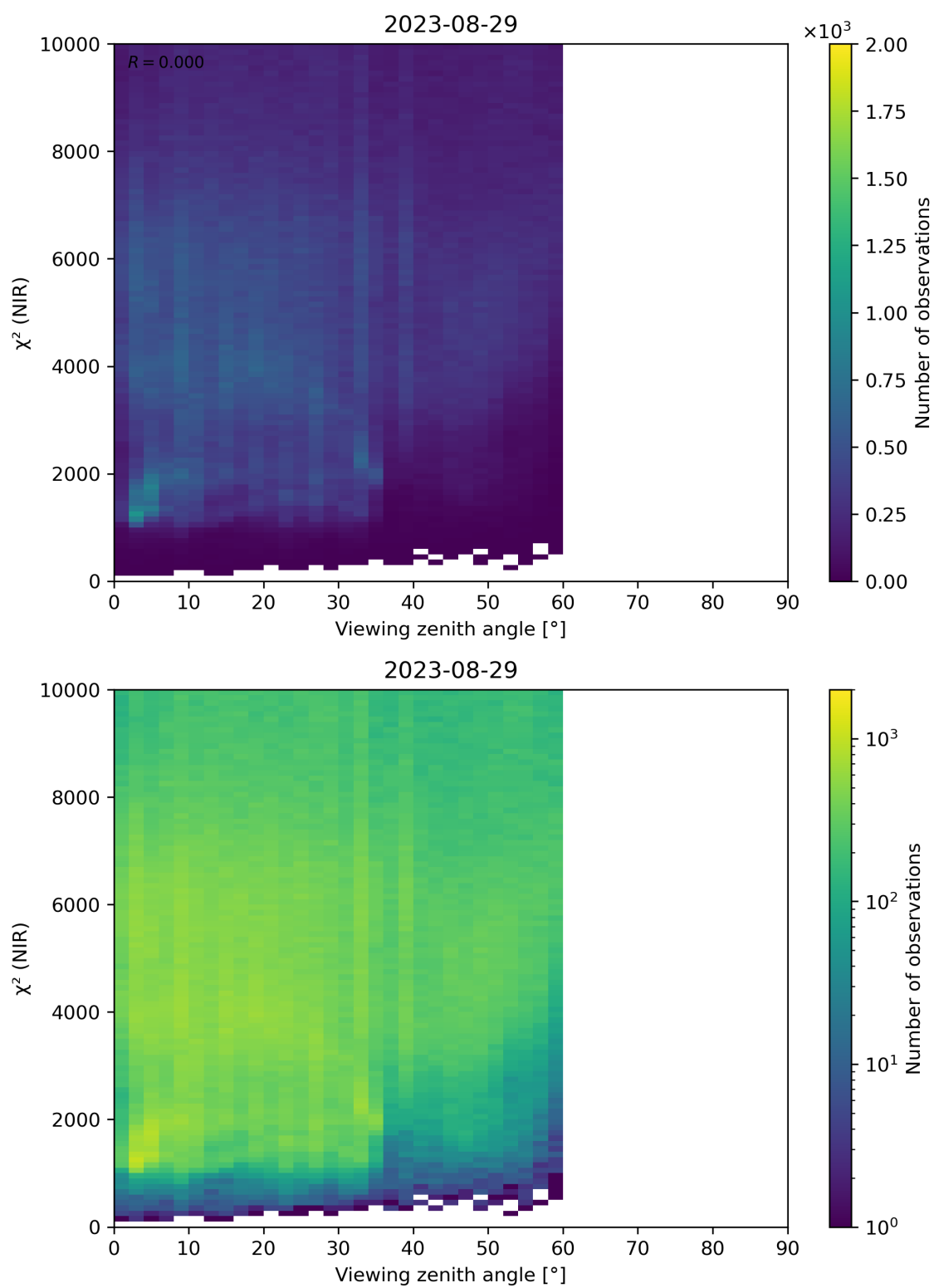
Figure 105: Scatter density plot of “Viewing zenith angle” against “ \chi^2 (NIR)” for 2023-08-28 to 2023-08-30.
