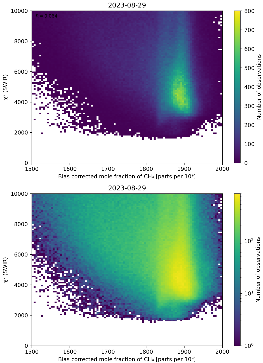
Figure 64: Scatter density plot of “Bias corrected mole fraction of CH 4 ” against “ \chi^2 (SWIR)” for 2023-08-28 to 2023-08-30.
