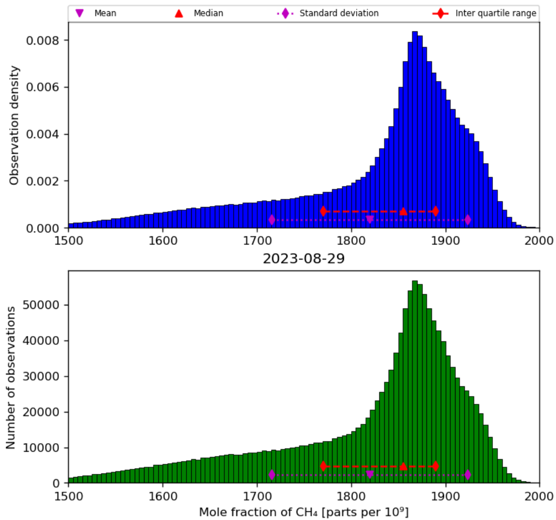
Figure 23: Histogram of “Mole fraction of CH 4 ” for 2023-08-28 to 2023-08-30
