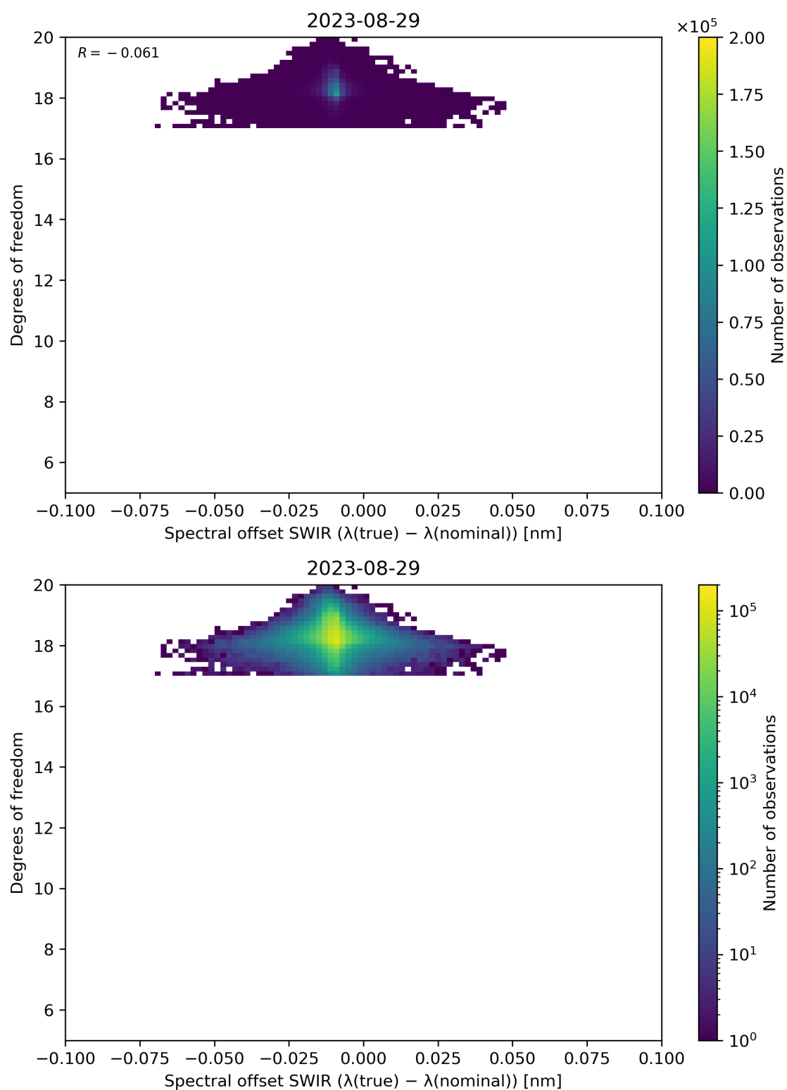
Figure 119: Scatter density plot of “Spectral offset SWIR ( \lambda(\text{true}) - \lambda(\text{nominal}) )” against “Degrees of freedom” for 2023-08-28 to 2023-08-30.
