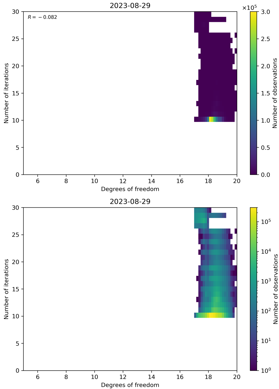
Figure 52: Scatter density plot of “Degrees of freedom” against “Number of iterations” for 2023-08-28 to 2023-08-30.
