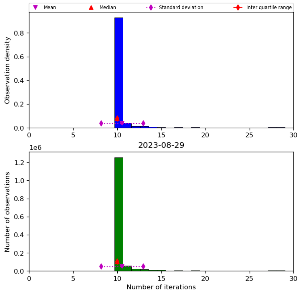
Figure 31: Histogram of “Number of iterations” for 2023-08-28 to 2023-08-30
