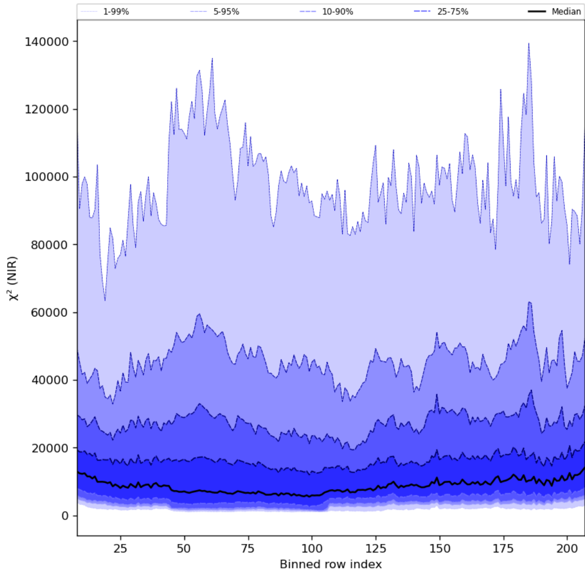
Figure 40: Along track statistics of " \chi^2 (NIR)" for 2023-08-28 to 2023-08-30
