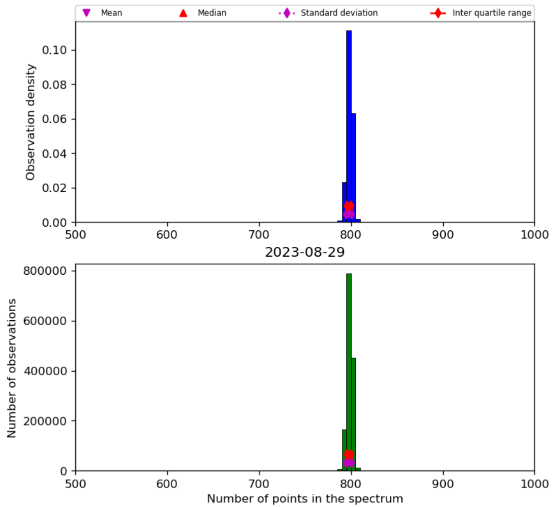
Figure 26: Histogram of “Number of points in the spectrum” for 2023-08-28 to 2023-08-30
