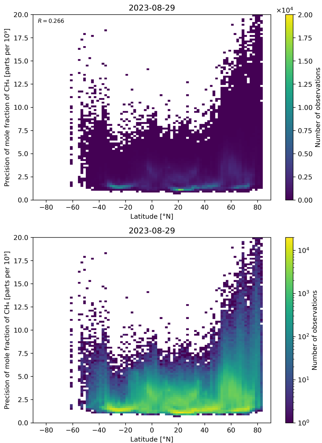
Figure 59: Scatter density plot of “Latitude” against “Precision of mole fraction of \text{CH}_4 ” for 2023-08-28 to 2023-08-30.
