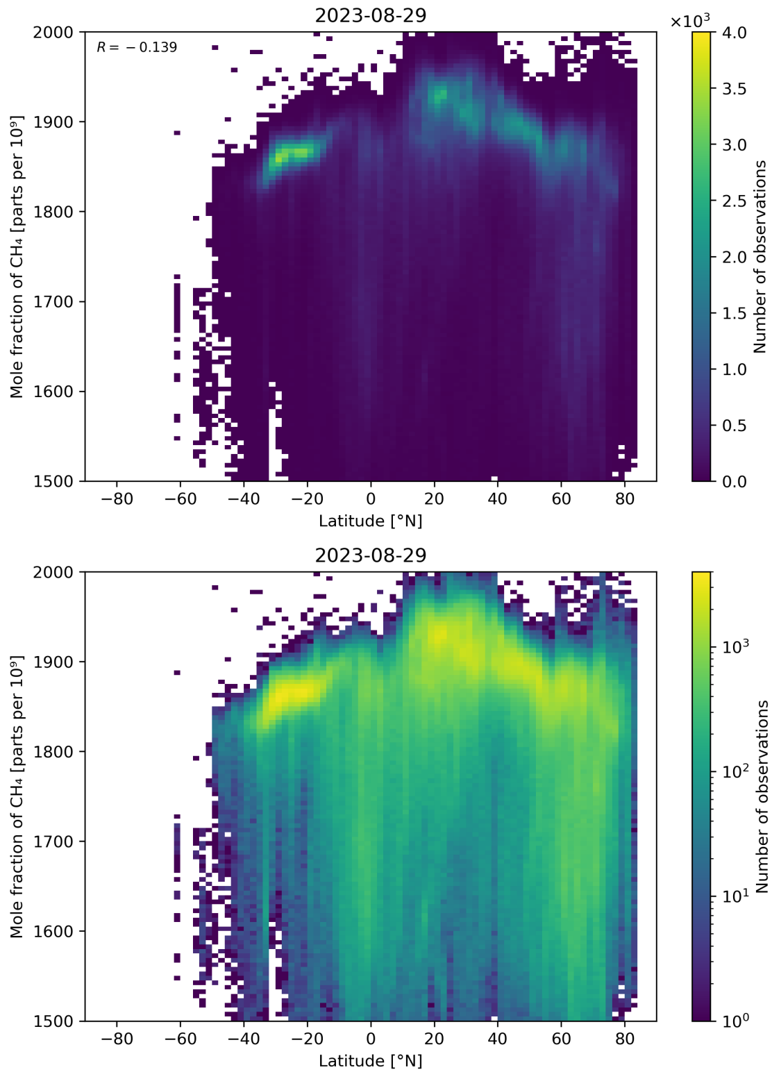
Figure 57: Scatter density plot of “Latitude” against “Mole fraction of \text{CH}_4 ” for 2023-08-28 to 2023-08-30.
