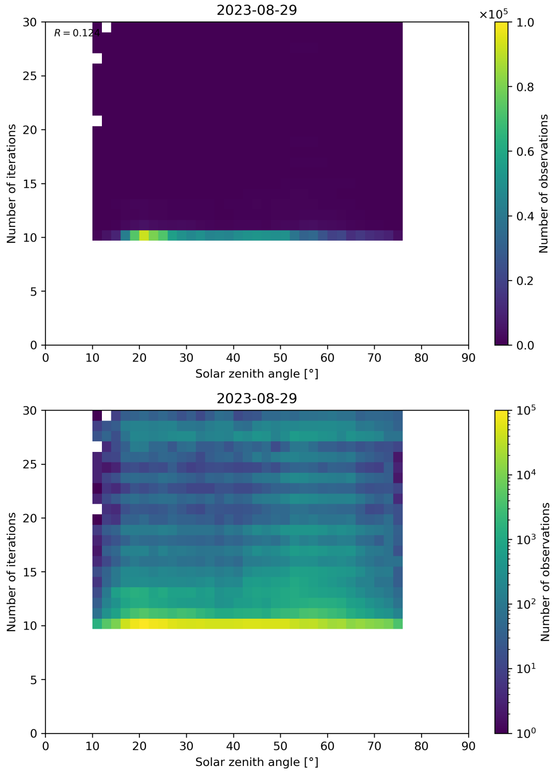
Figure 102: Scatter density plot of “Solar zenith angle” against “Number of iterations” for 2023-08-28 to 2023-08-30.
