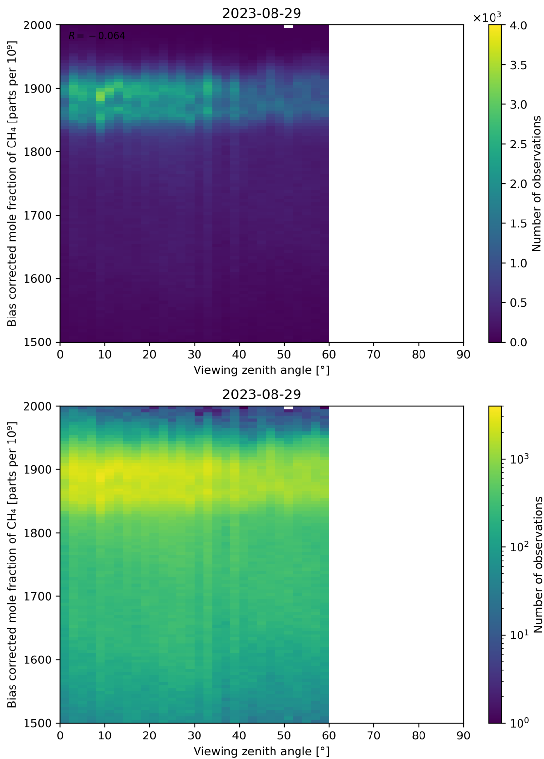
Figure 111: Scatter density plot of “Viewing zenith angle” against “Bias corrected mole fraction of CH 4 ” for 2023-08-28 to 2023-08-30.
