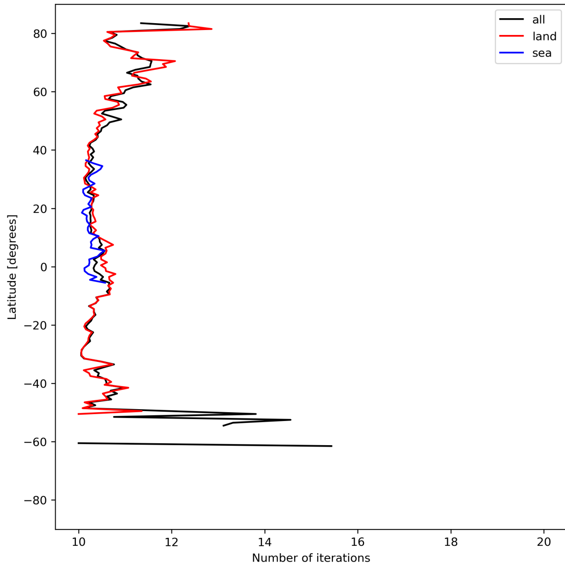
Figure 20: Zonal average of “Number of iterations” for 2023-08-28 to 2023-08-30.
