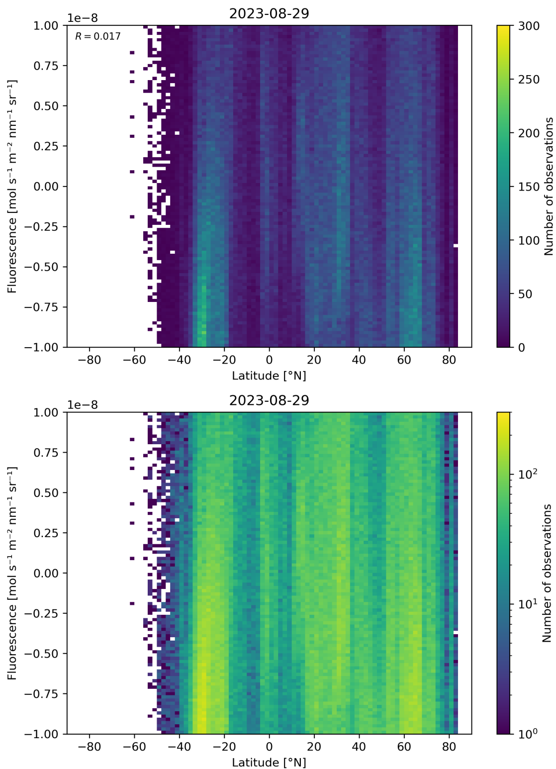
Figure 56: Scatter density plot of “Latitude” against “Fluorescence” for 2023-08-28 to 2023-08-30.
