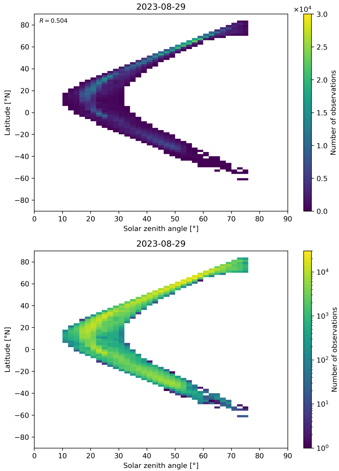
Figure 98: Scatter density plot of “Solar zenith angle” against “Latitude” for 2023-08-28 to 2023-08-30.
