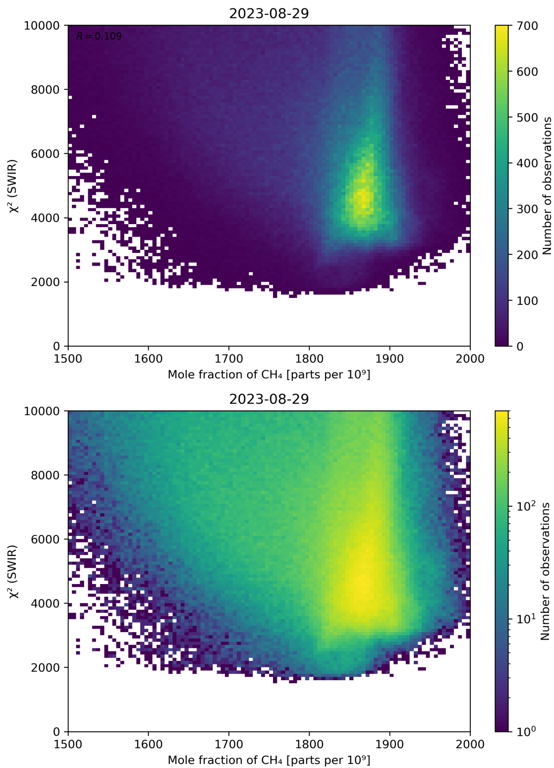
Figure 71: Scatter density plot of “Mole fraction of CH 4 ” against “ \chi^2 (SWIR)” for 2023-08-28 to 2023-08-30.
