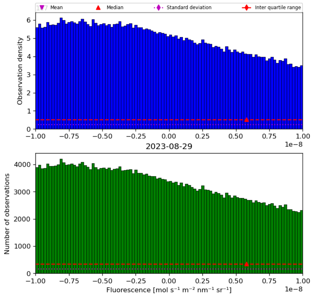
Figure 32: Histogram of “Fluorescence” for 2023-08-28 to 2023-08-30
