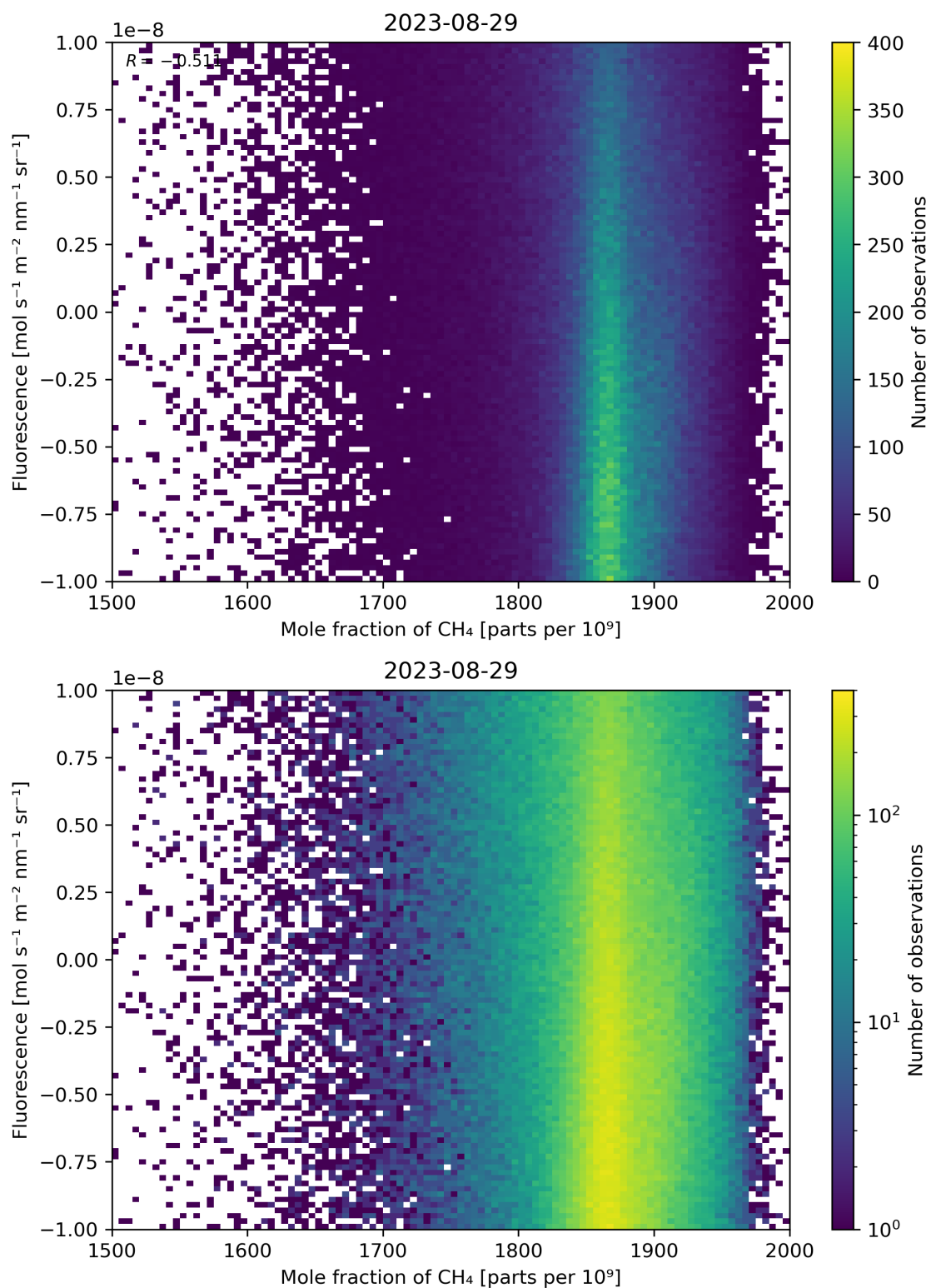
Figure 73: Scatter density plot of “Mole fraction of \text{CH}_4 ” against “Fluorescence” for 2023-08-28 to 2023-08-30.
