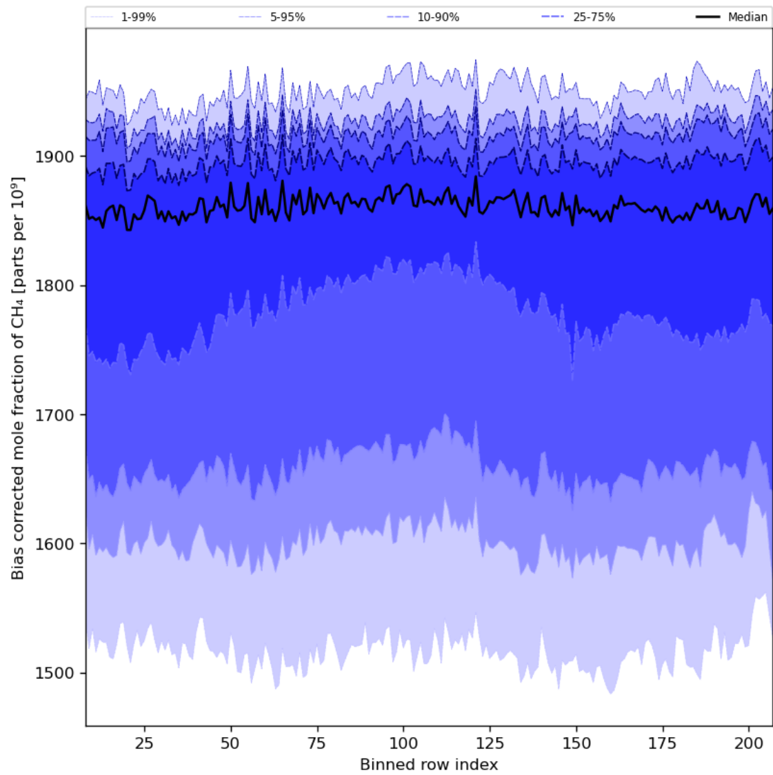
Figure 36: Along track statistics of “Bias corrected mole fraction of CH 4 ” for 2023-08-28 to 2023-08-30
