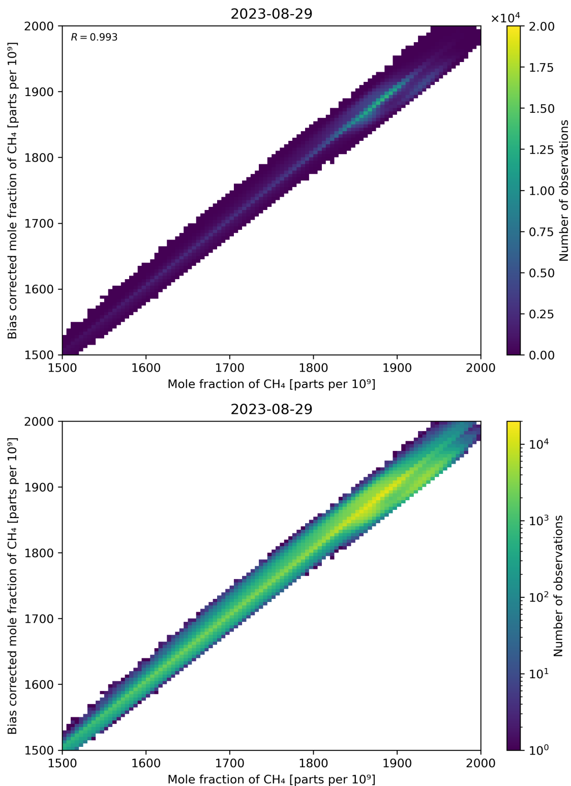
Figure 74: Scatter density plot of “Mole fraction of CH 4 ” against “Bias corrected mole fraction of CH 4 ” for 2023-08-28 to 2023-08-30.
