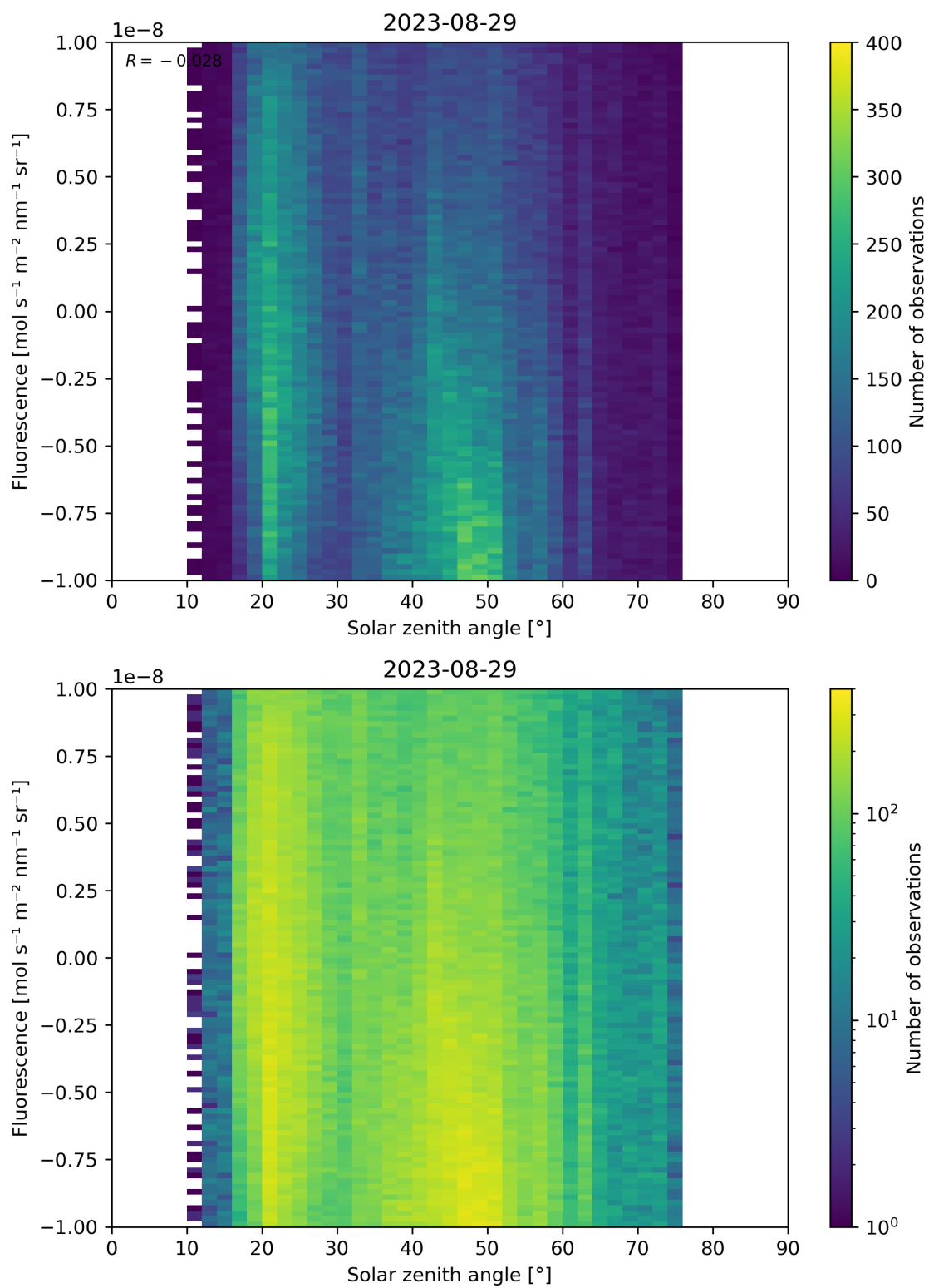
Figure 97: Scatter density plot of “Solar zenith angle” against “Fluorescence” for 2023-08-28 to 2023-08-30.
