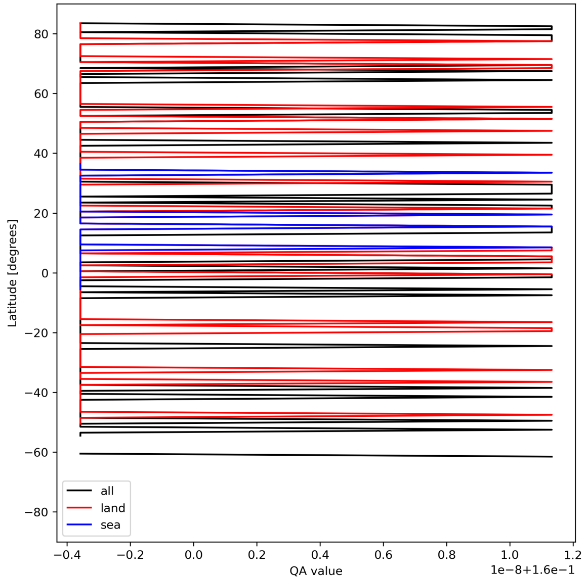
Figure 11: Zonal average of “QA value” for 2023-08-28 to 2023-08-30.
