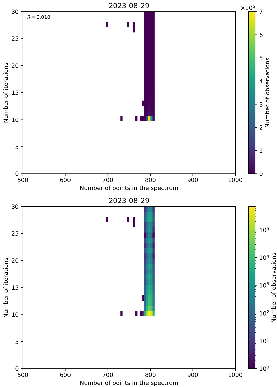
Figure 92: Scatter density plot of “Number of points in the spectrum” against “Number of iterations” for 2023-08-28 to 2023-08-30.
