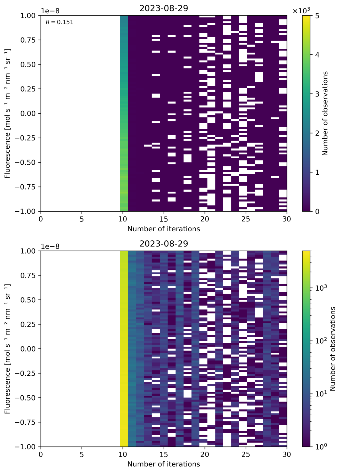
Figure 87: Scatter density plot of “Number of iterations” against “Fluorescence” for 2023-08-28 to 2023-08-30.
