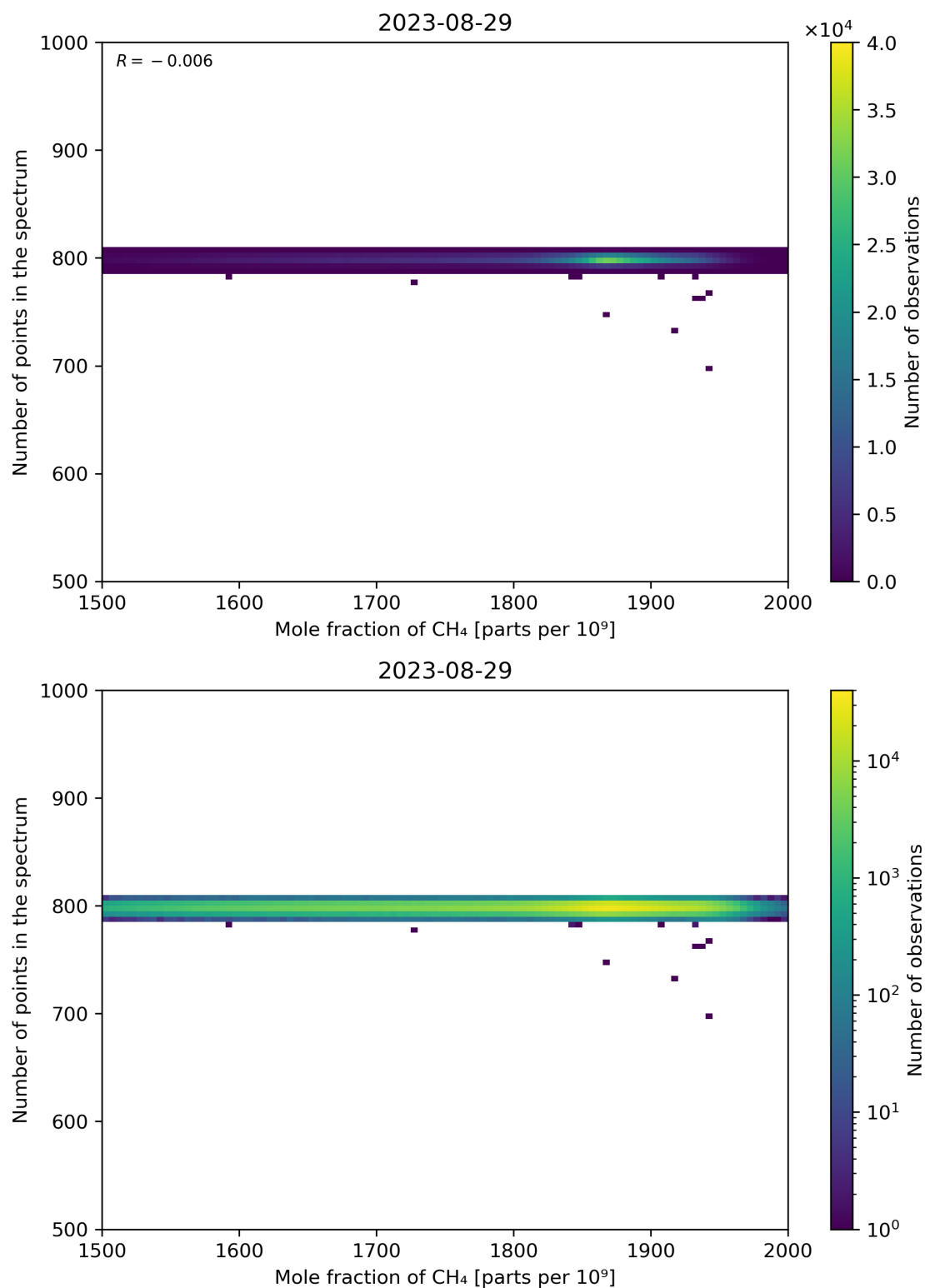
Figure 77: Scatter density plot of “Mole fraction of CH 4 ” against “Number of points in the spectrum” for 2023-08-28 to 2023-08-30.
