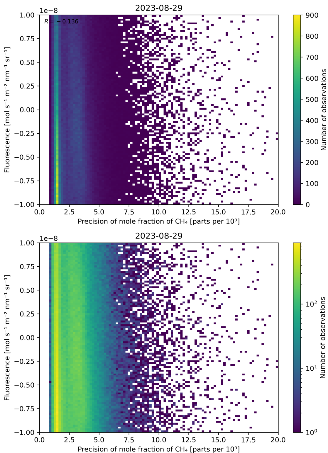
Figure 81: Scatter density plot of “Precision of mole fraction of \text{CH}_4 ” against “Fluorescence” for 2023-08-28 to 2023-08-30.
