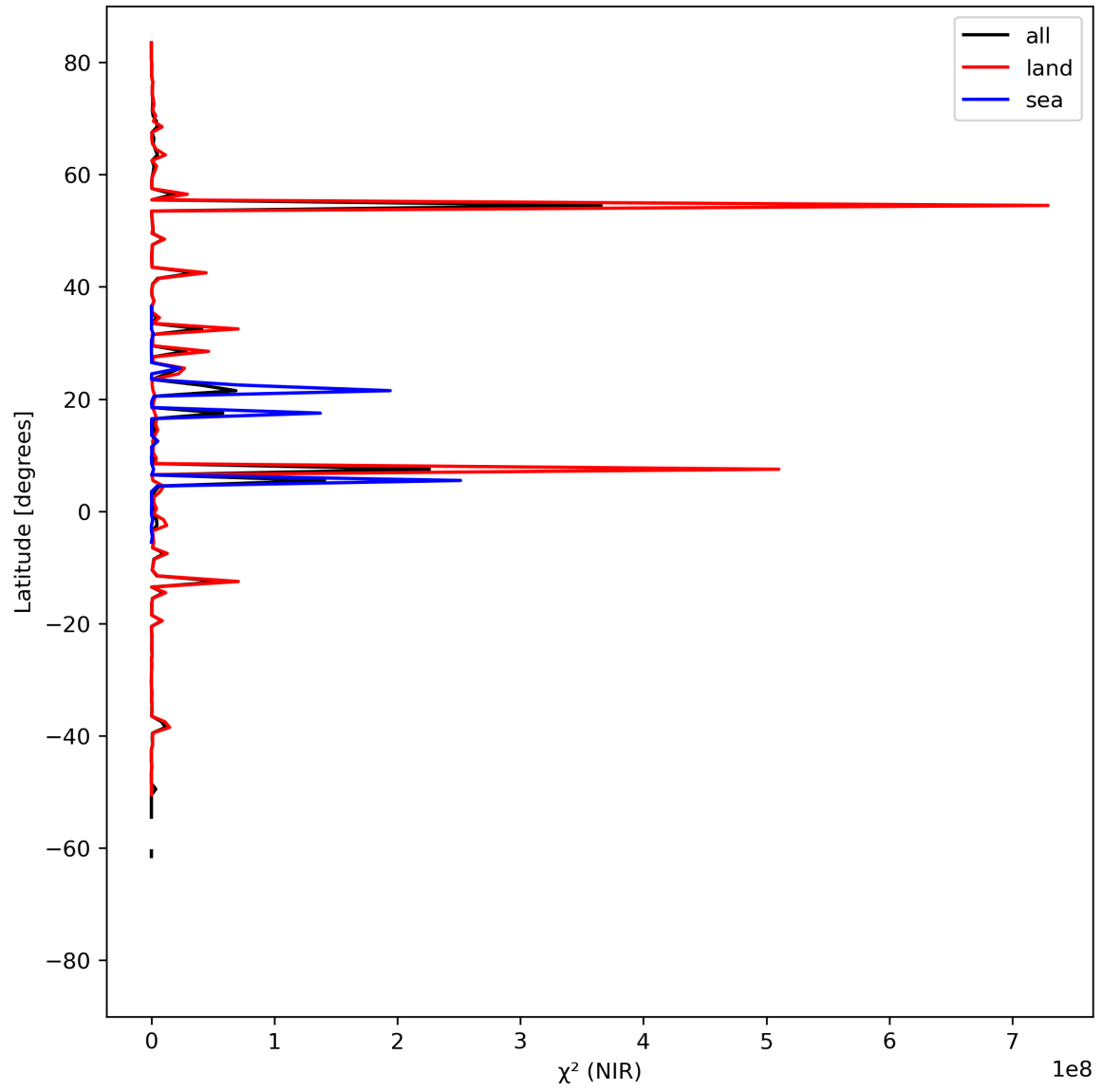
Figure 18: Zonal average of “ \chi^2 (NIR)” for 2023-08-28 to 2023-08-30.
