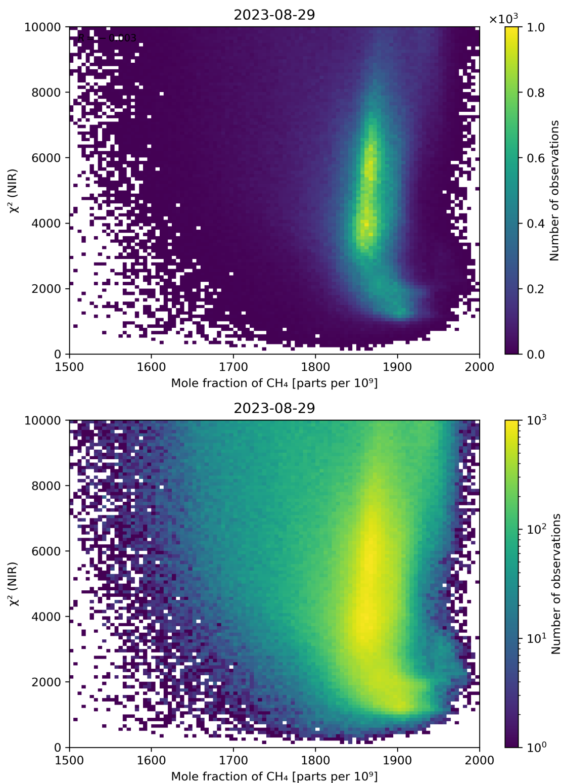
Figure 70: Scatter density plot of “Mole fraction of CH 4 ” against “ \chi^2 (NIR)” for 2023-08-28 to 2023-08-30.
