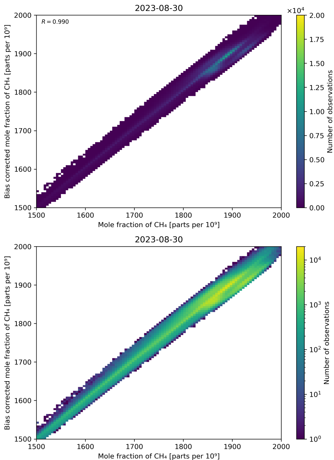
Figure 74: Scatter density plot of “Mole fraction of CH 4 ” against “Bias corrected mole fraction of CH 4 ” for 2023-08-30 to 2023-08-31.
