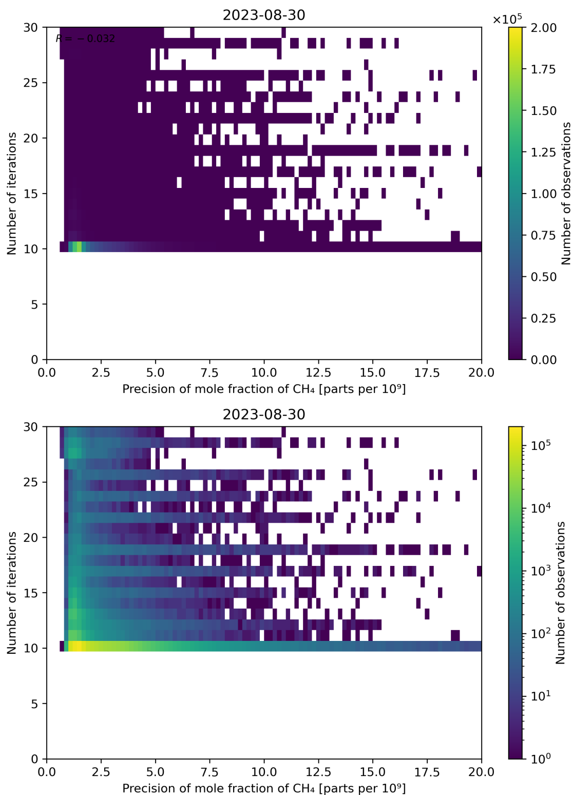
Figure 83: Scatter density plot of “Precision of mole fraction of CH 4 ” against “Number of iterations” for 2023-08-30 to 2023-08-31.
