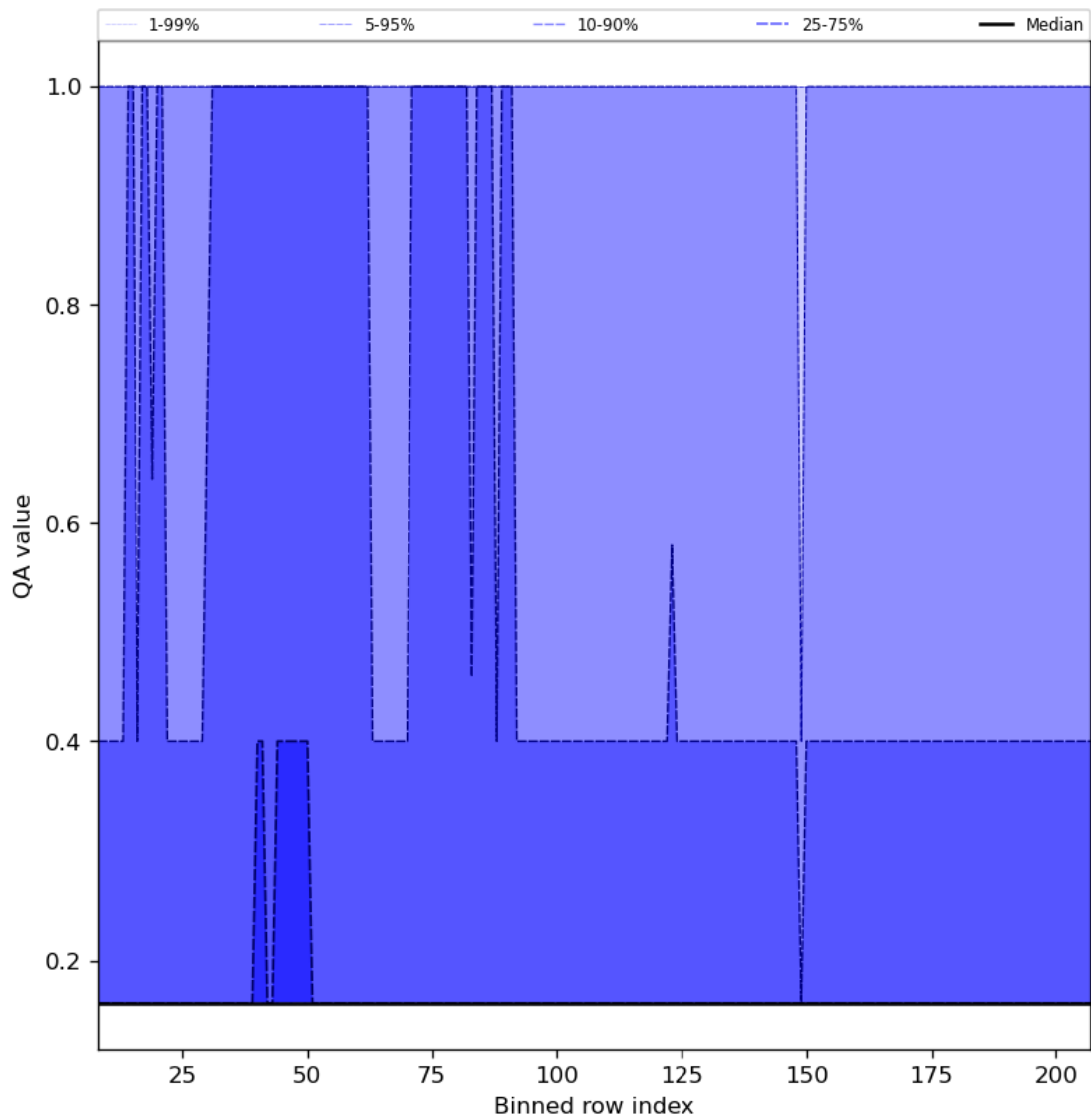
Figure 33: Along track statistics of “QA value” for 2023-08-30 to 2023-08-31
