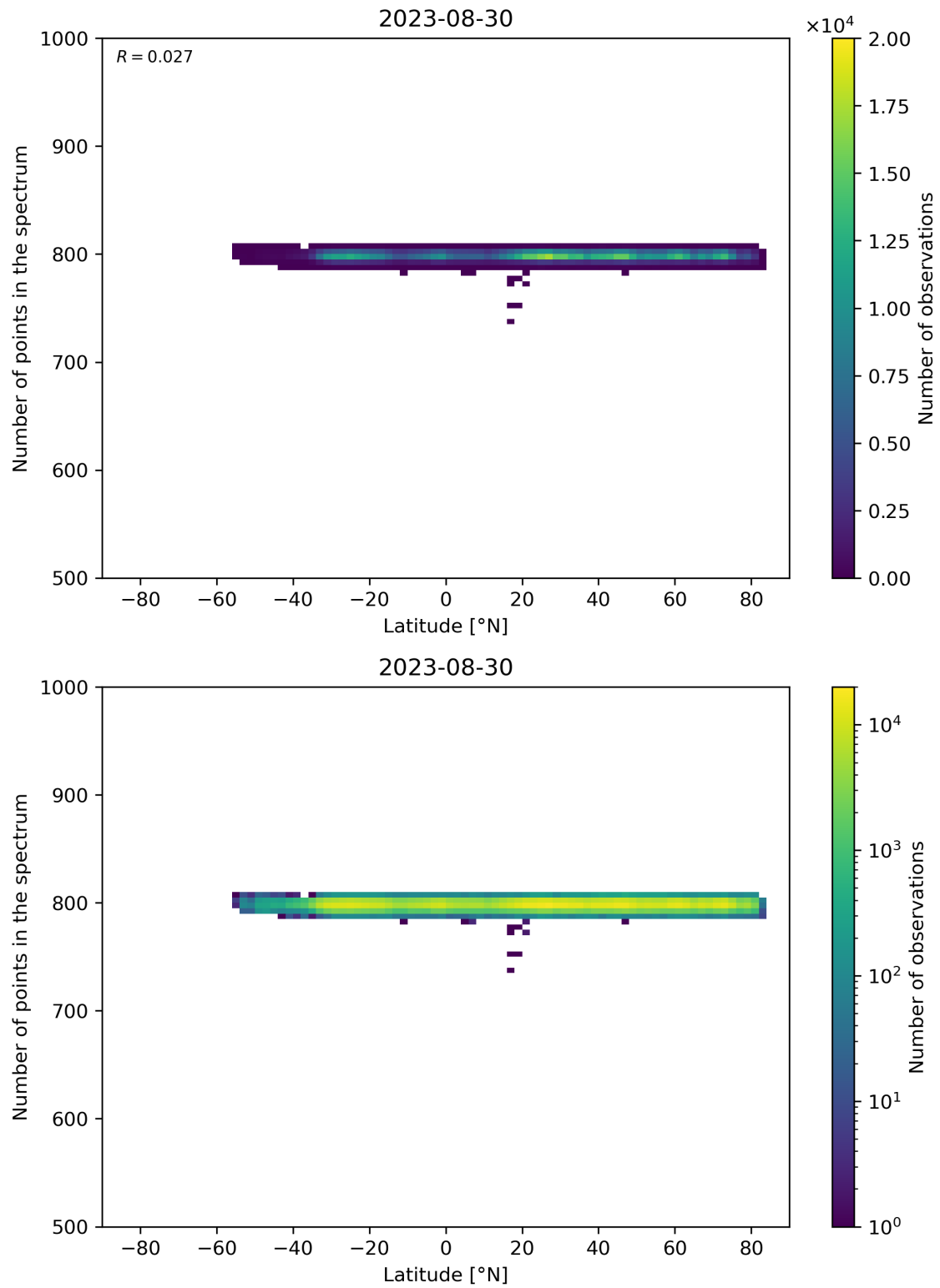
Figure 61: Scatter density plot of “Latitude” against “Number of points in the spectrum” for 2023-08-30 to 2023-08-31.
