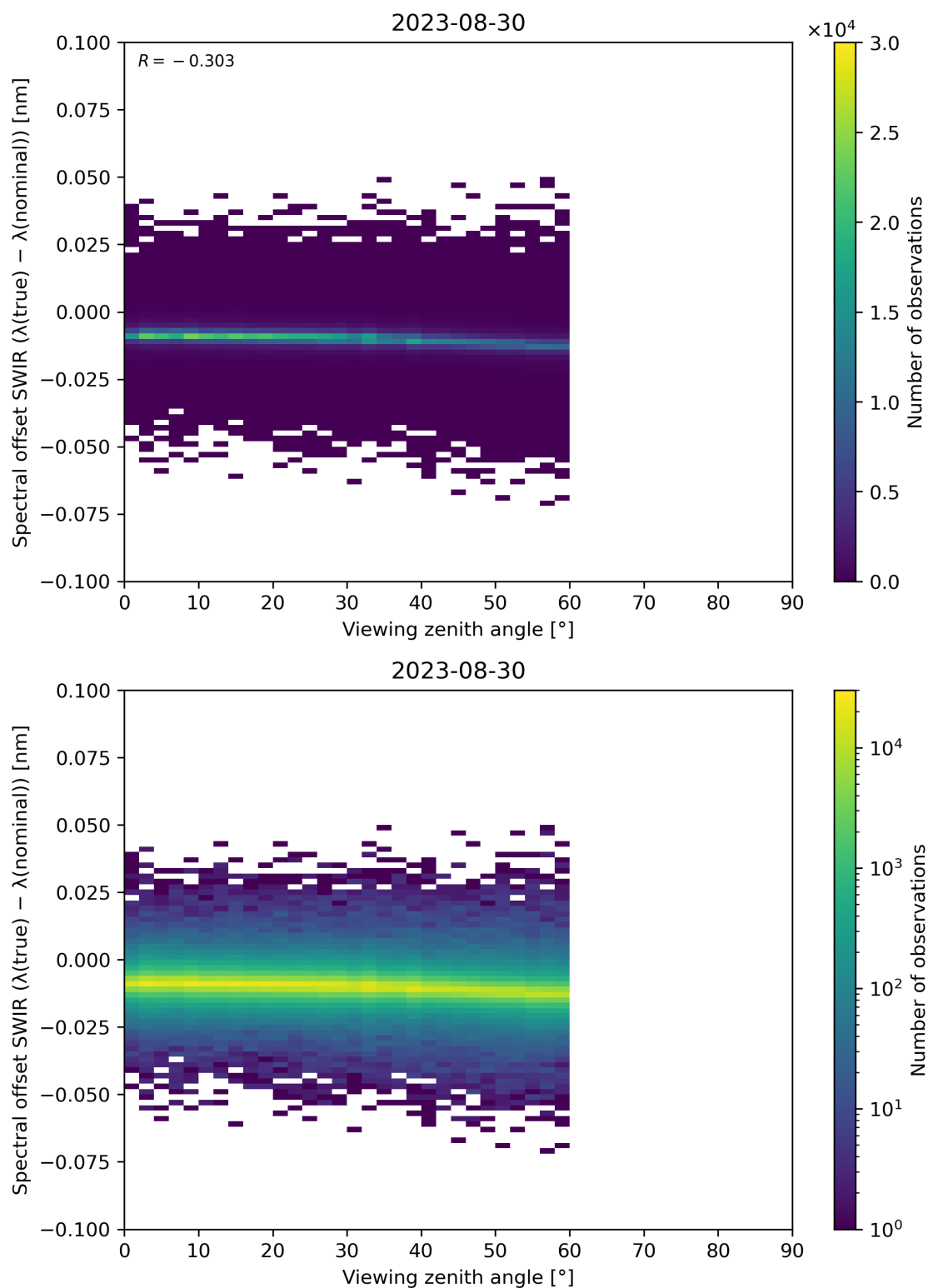
Figure 116: Scatter density plot of “Viewing zenith angle” against “Spectral offset SWIR ( \lambda(\text{true}) - \lambda(\text{nominal}) )” for 2023-08-30 to 2023-08-31.
