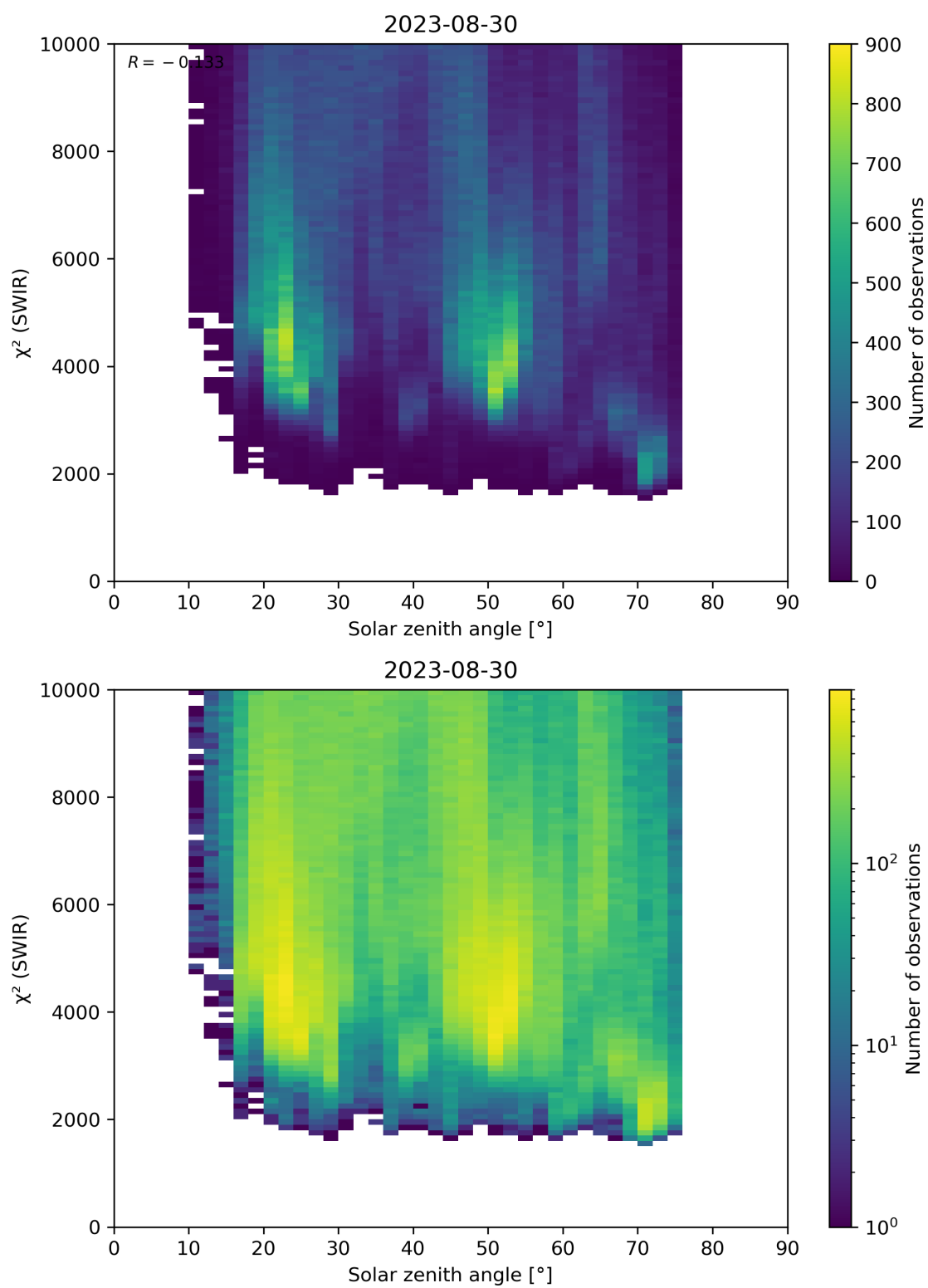
Figure 95: Scatter density plot of “Solar zenith angle” against “ \chi^2 (SWIR)” for 2023-08-30 to 2023-08-31.
