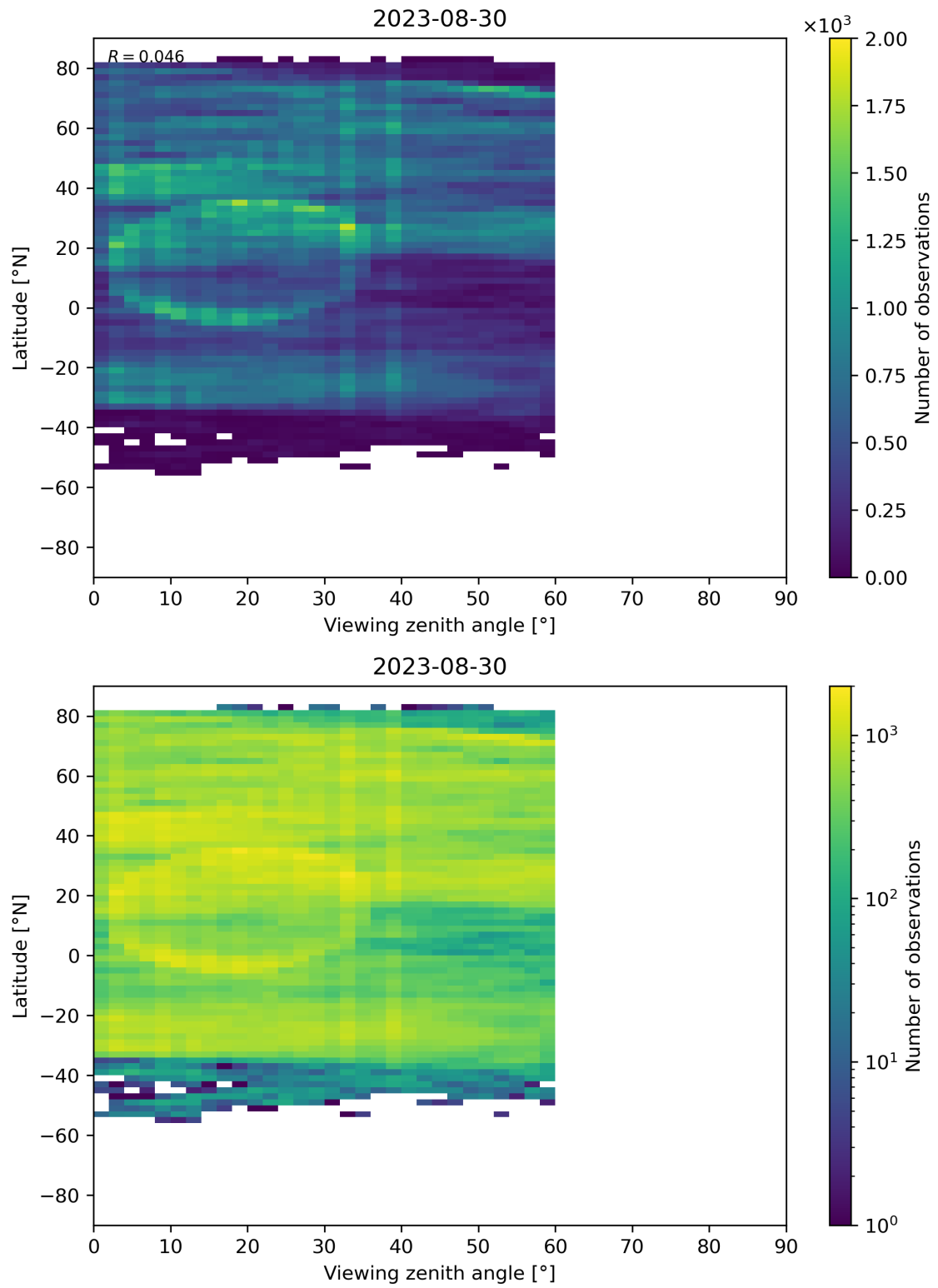
Figure 109: Scatter density plot of “Viewing zenith angle” against “Latitude” for 2023-08-30 to 2023-08-31.
