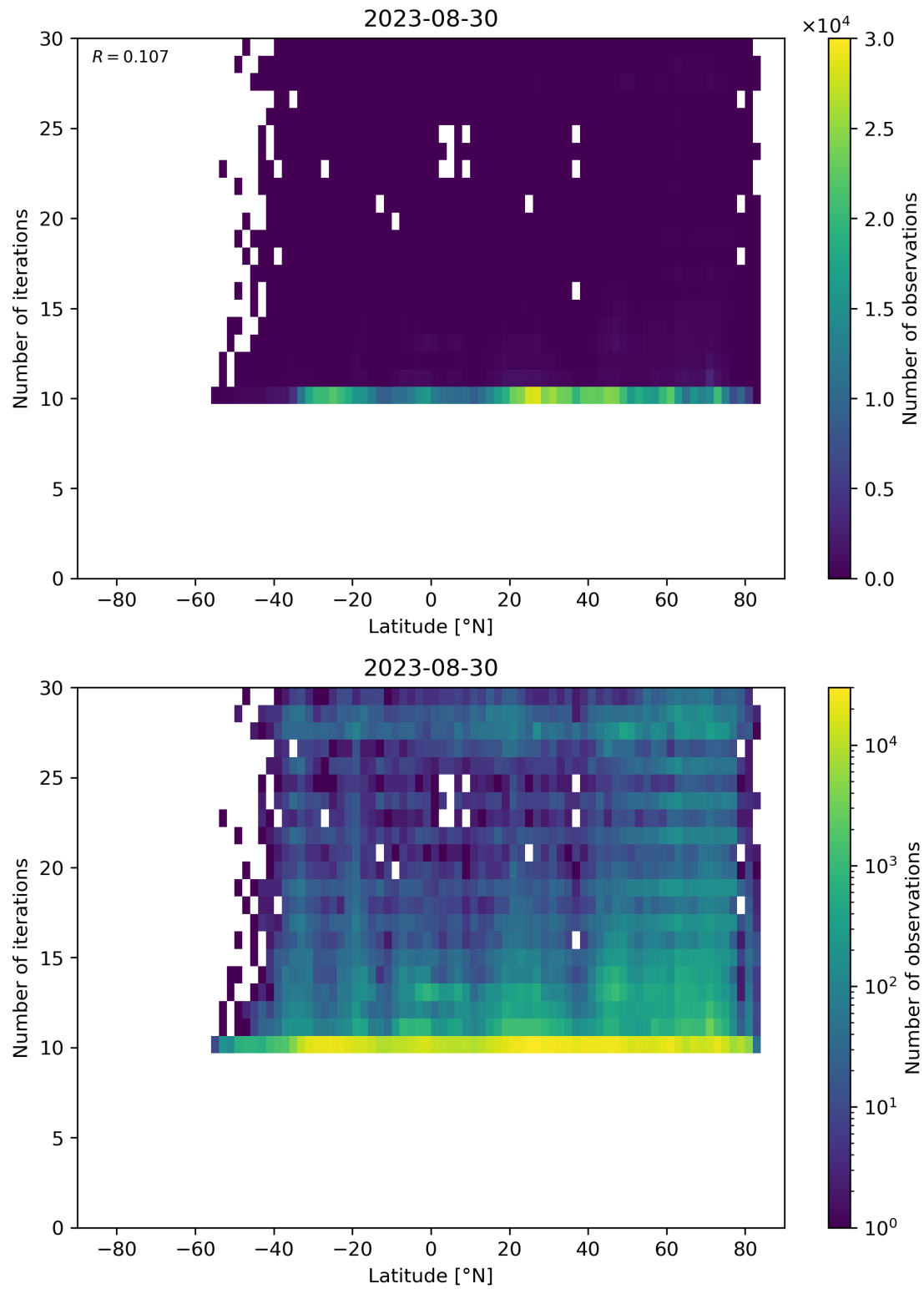
Figure 60: Scatter density plot of “Latitude” against “Number of iterations” for 2023-08-30 to 2023-08-31.
