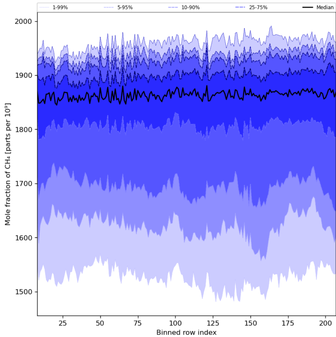
Figure 34: Along track statistics of “Mole fraction of CH 4 ” for 2023-08-30 to 2023-08-31
