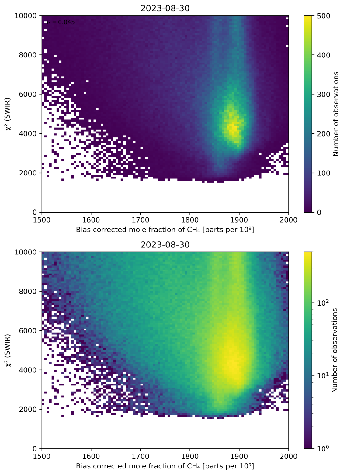
Figure 64: Scatter density plot of “Bias corrected mole fraction of CH 4 ” against “ \chi^2 (SWIR)” for 2023-08-30 to 2023-08-31.
