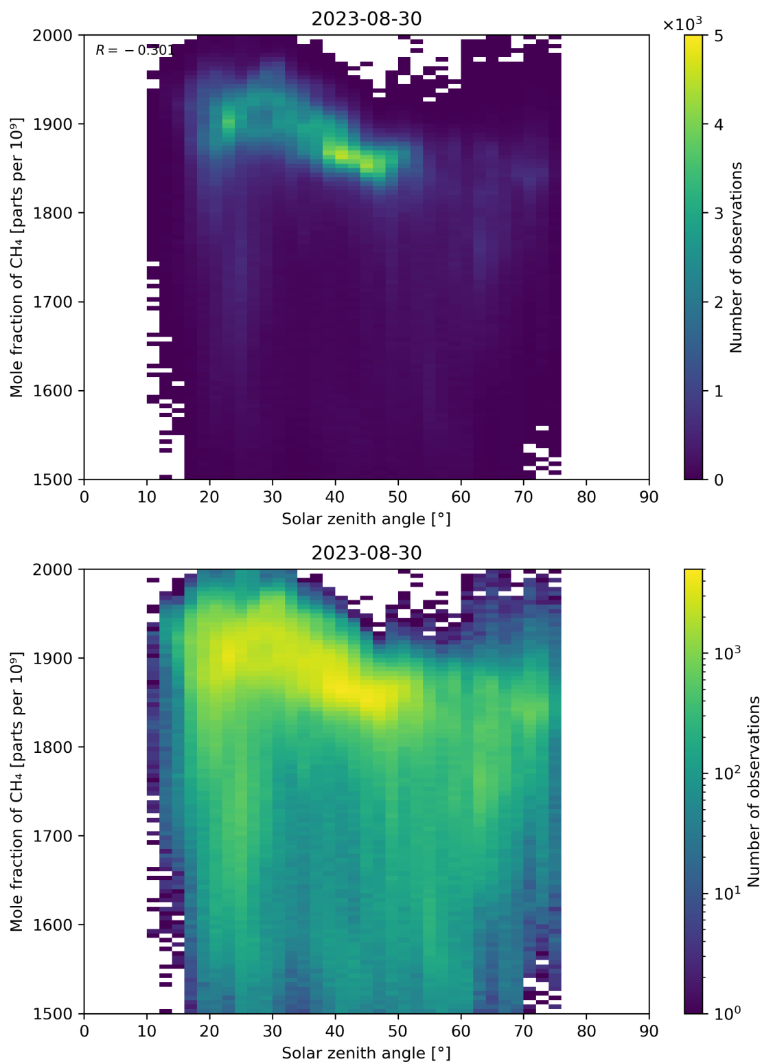
Figure 99: Scatter density plot of “Solar zenith angle” against “Mole fraction of \text{CH}_4 ” for 2023-08-30 to 2023-08-31.
