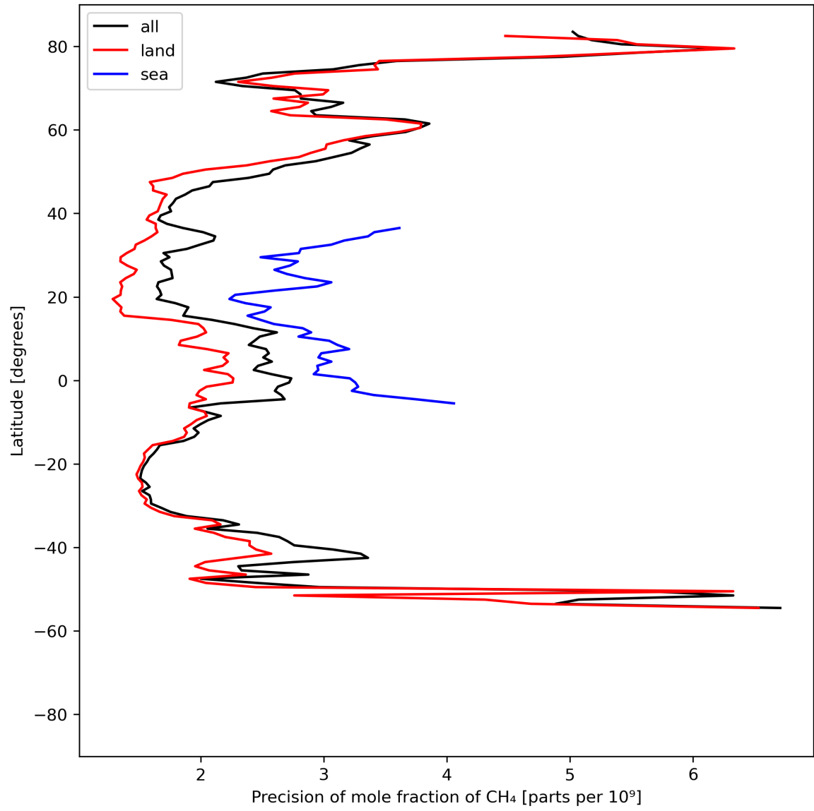
Figure 13: Zonal average of “Precision of mole fraction of CH 4 ” for 2023-08-30 to 2023-08-31.
