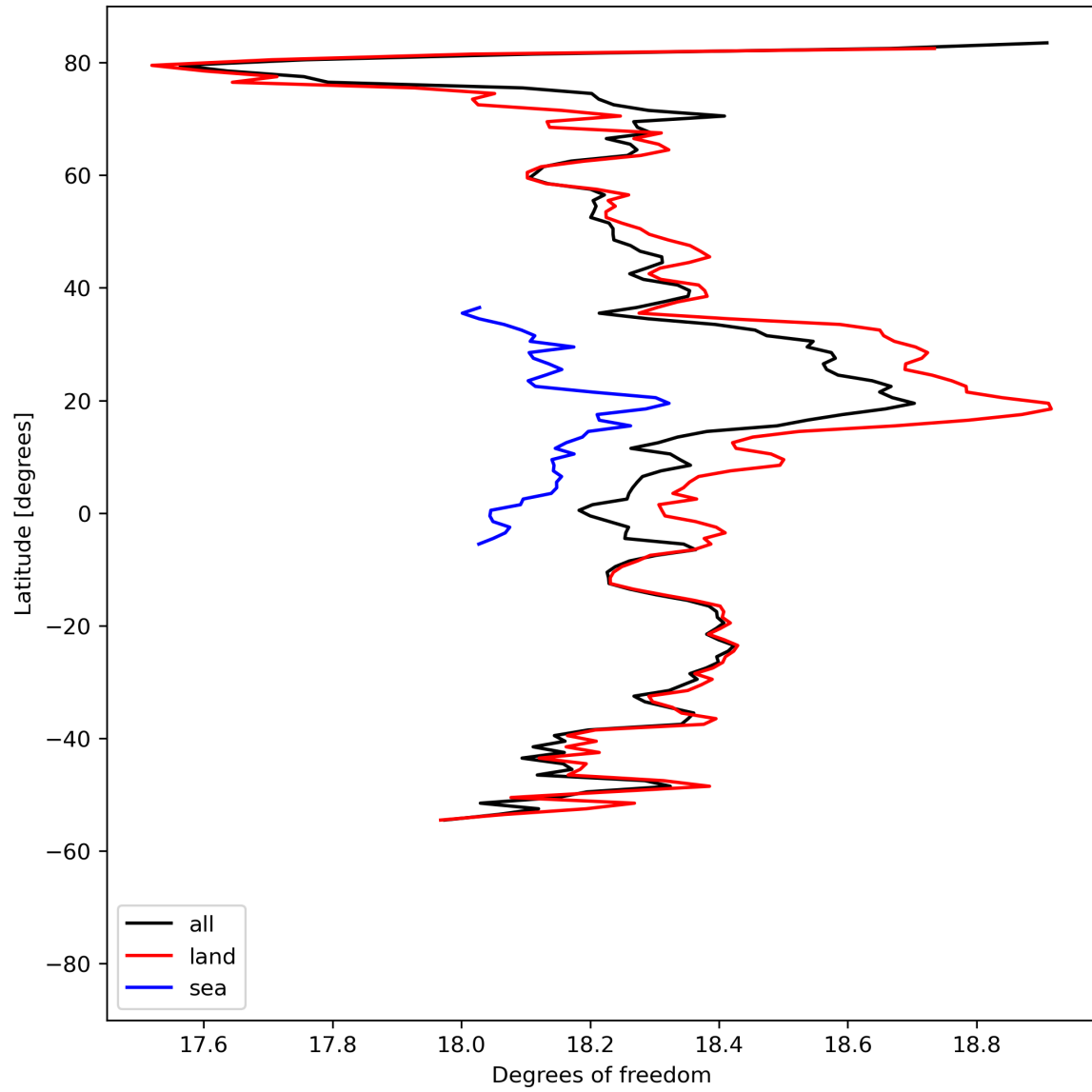
Figure 19: Zonal average of “Degrees of freedom” for 2023-08-30 to 2023-08-31.
