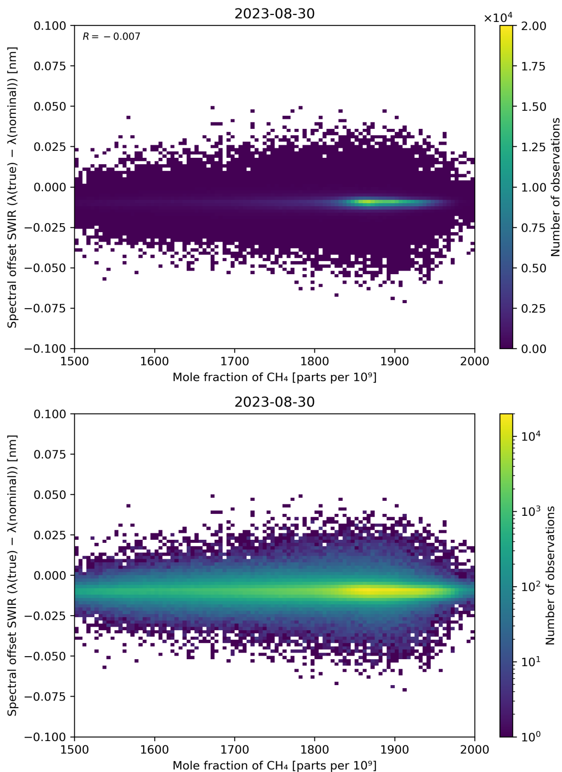
Figure 86: Scatter density plot of “Mole fraction of CH 4 ” against “Spectral offset SWIR ( \lambda(\text{true}) - \lambda(\text{nominal}) )” for 2023-08-30 to 2023-08-31.
