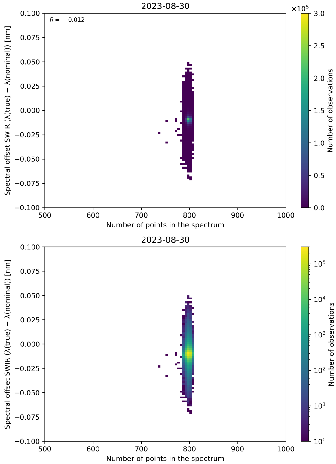
Figure 93: Scatter density plot of “Number of points in the spectrum” against “Spectral offset SWIR ( \lambda(\text{true}) - \lambda(\text{nominal}) )” for 2023-08-30 to 2023-08-31.
