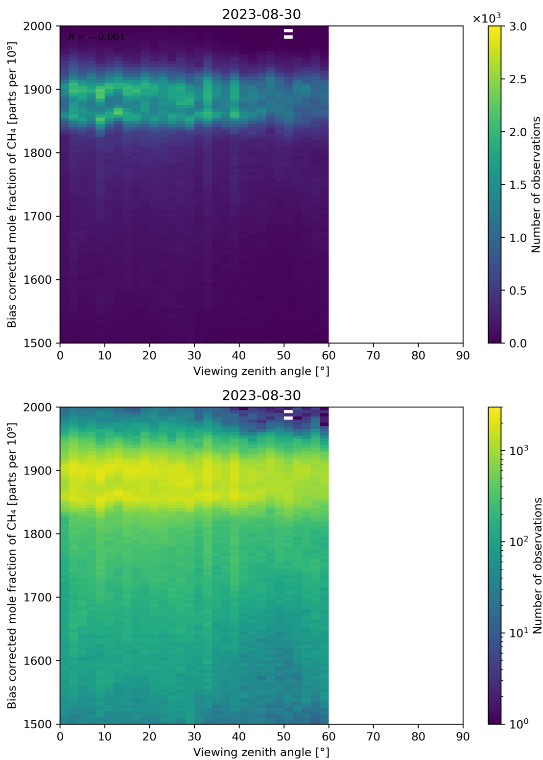
Figure 111: Scatter density plot of “Viewing zenith angle” against “Bias corrected mole fraction of CH 4 ” for 2023-08-30 to 2023-08-31.
