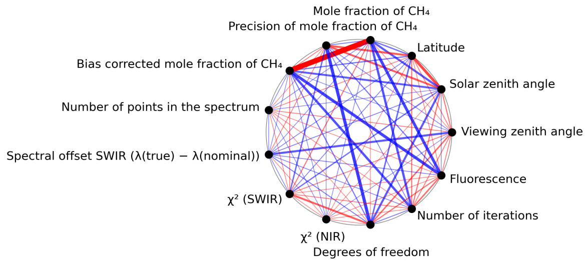
Figure 1: Map of correlation graph for 2023-08-30 to 2023-08-31.
