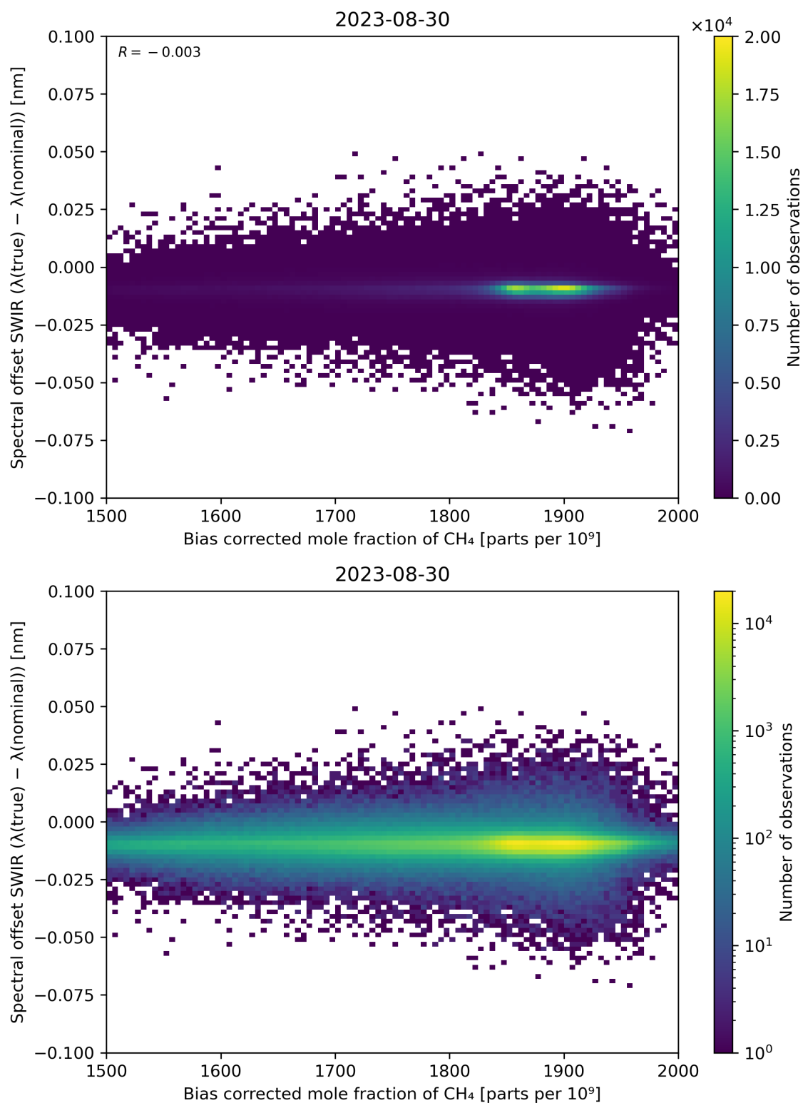
Figure 69: Scatter density plot of “Bias corrected mole fraction of \text{CH}_4 ” against “Spectral offset SWIR ( \lambda(\text{true}) - \lambda(\text{nominal}) )” for 2023-08-30 to 2023-08-31.
