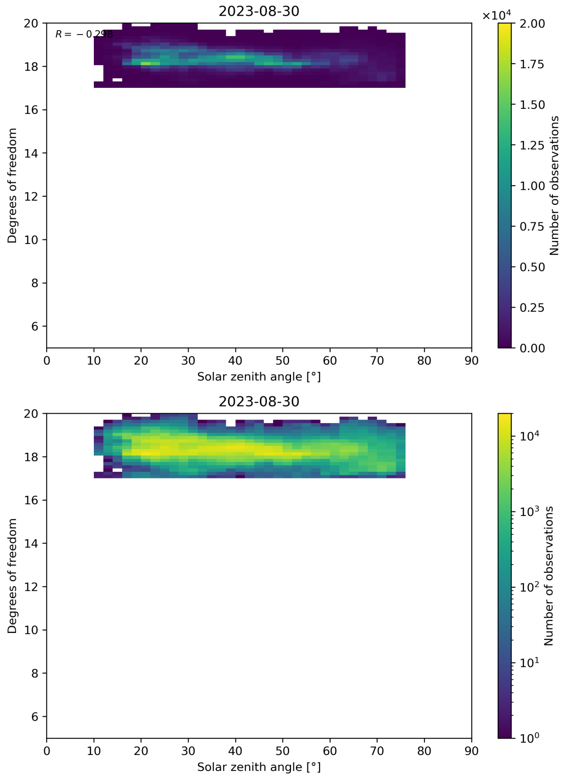
Figure 96: Scatter density plot of “Solar zenith angle” against “Degrees of freedom” for 2023-08-30 to 2023-08-31.
