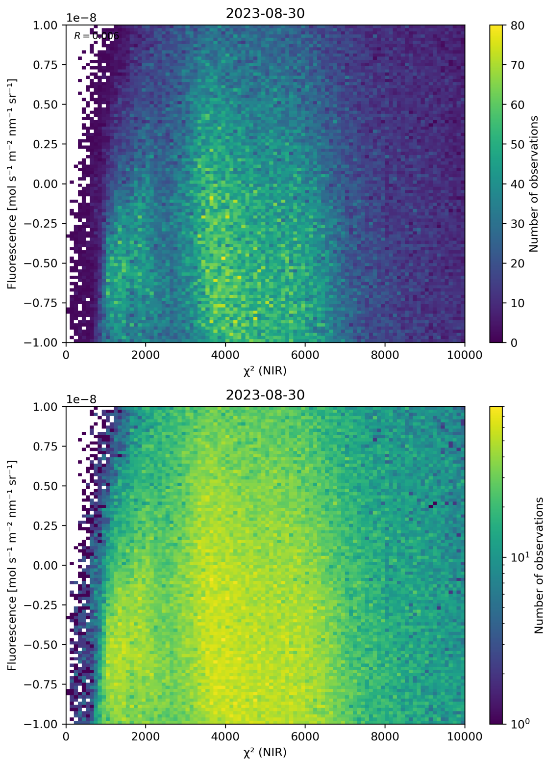
Figure 45: Scatter density plot of “ \chi^2 (NIR)” against “Fluorescence” for 2023-08-30 to 2023-08-31.
