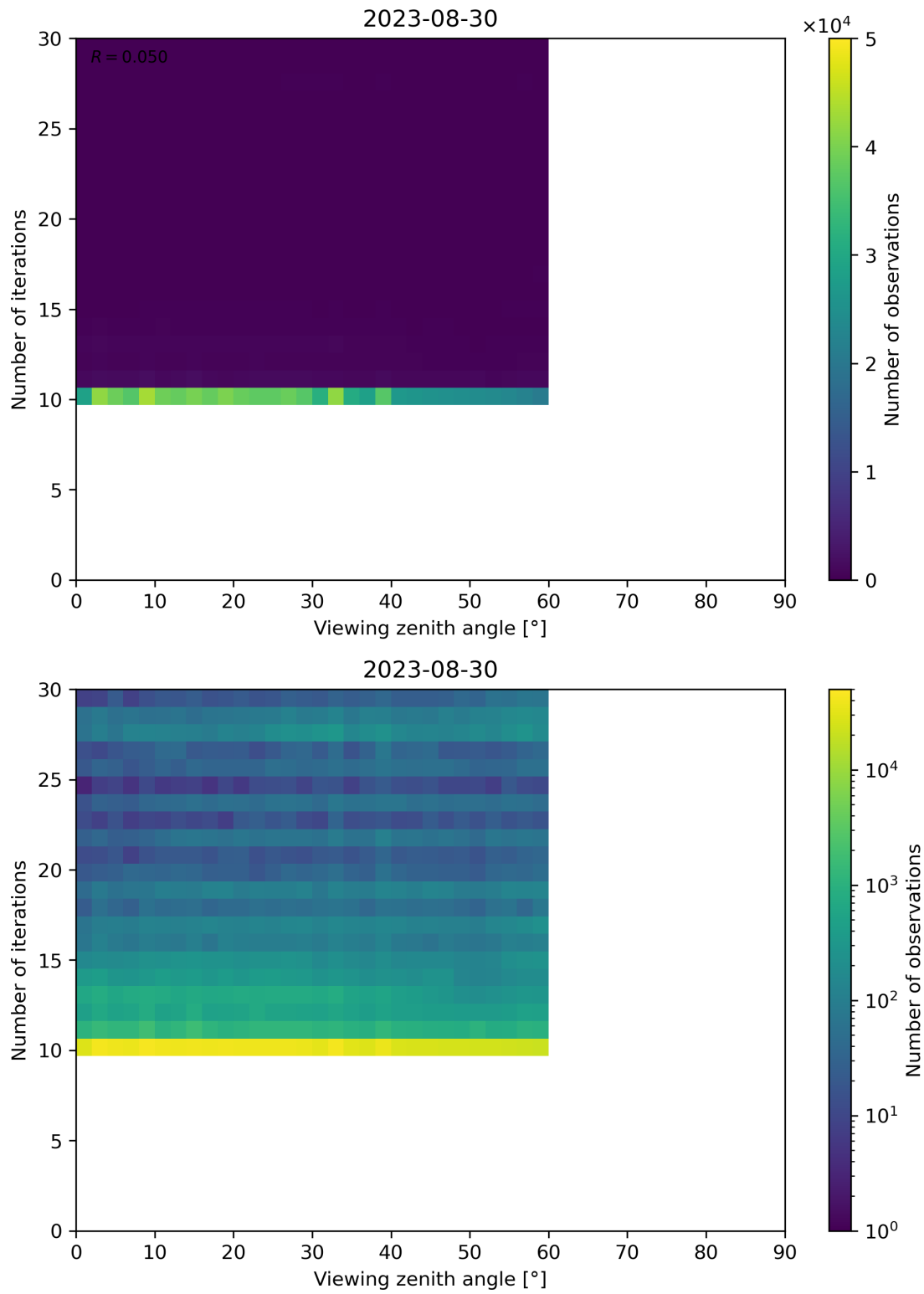
Figure 113: Scatter density plot of “Viewing zenith angle” against “Number of iterations” for 2023-08-30 to 2023-08-31.
