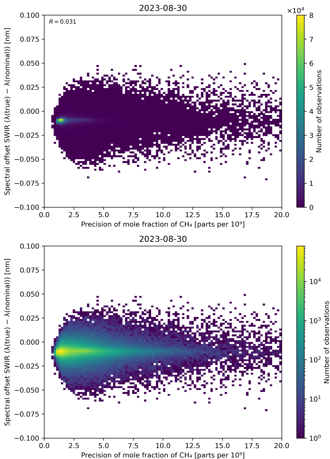
Figure 85: Scatter density plot of “Precision of mole fraction of \text{CH}_4 ” against “Spectral offset SWIR ( \lambda(\text{true}) - \lambda(\text{nominal}) )” for 2023-08-30 to 2023-08-31.
