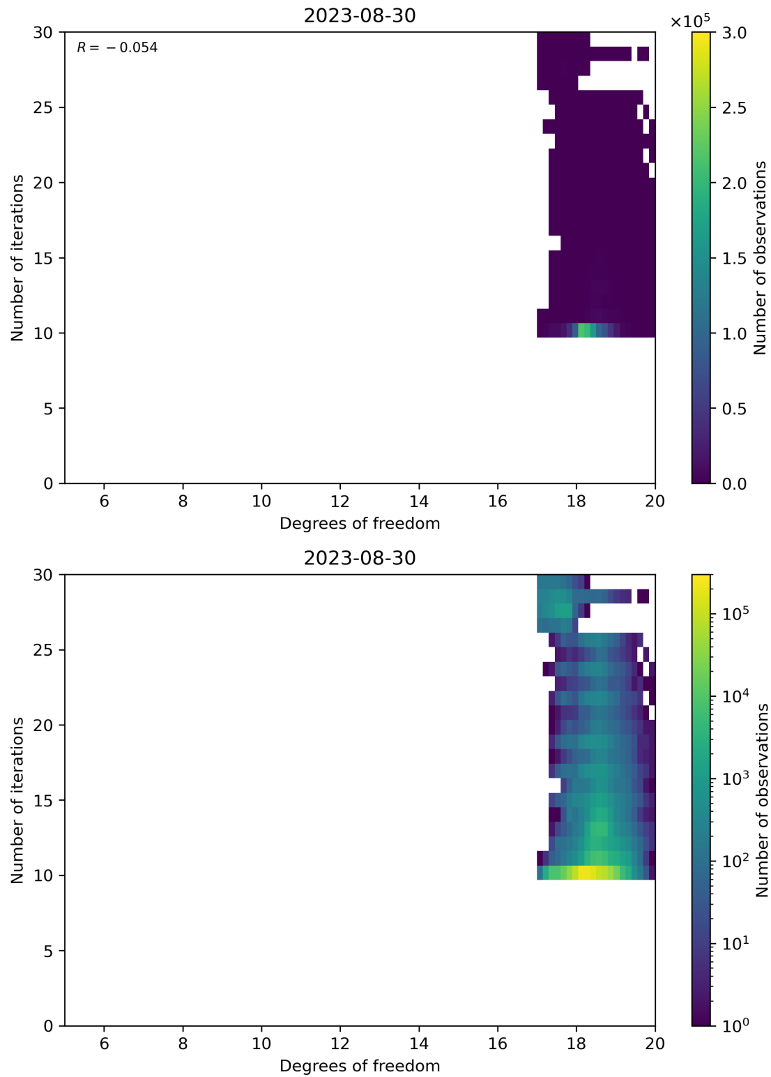
Figure 52: Scatter density plot of “Degrees of freedom” against “Number of iterations” for 2023-08-30 to 2023-08-31.
