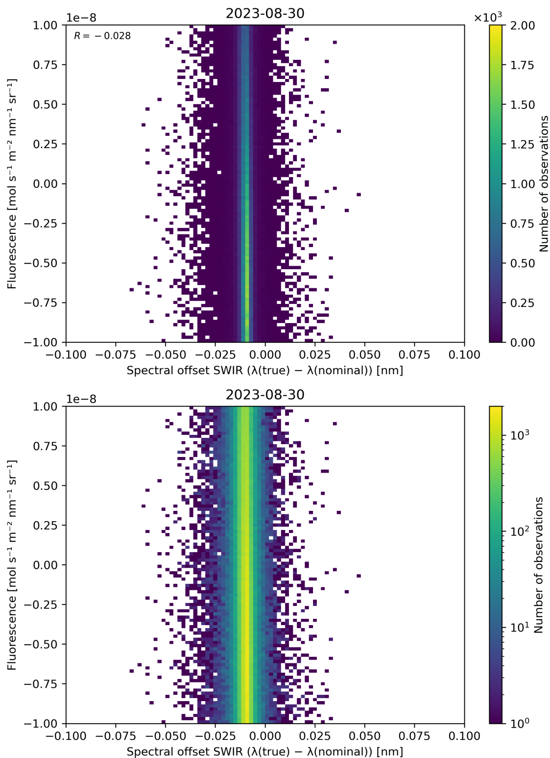
Figure 120: Scatter density plot of “Spectral offset SWIR ( \lambda(\text{true}) - \lambda(\text{nominal}) )” against “Fluorescence” for 2023-08-30 to 2023-08-31.
