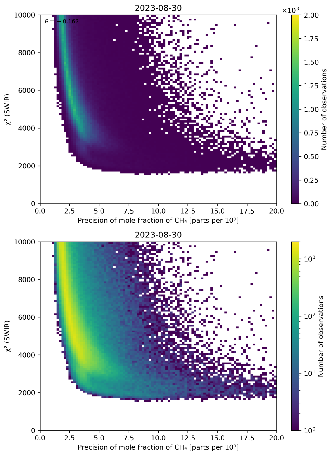
Figure 79: Scatter density plot of “Precision of mole fraction of \text{CH}_4 ” against “ \chi^2 (SWIR)” for 2023-08-30 to 2023-08-31.
