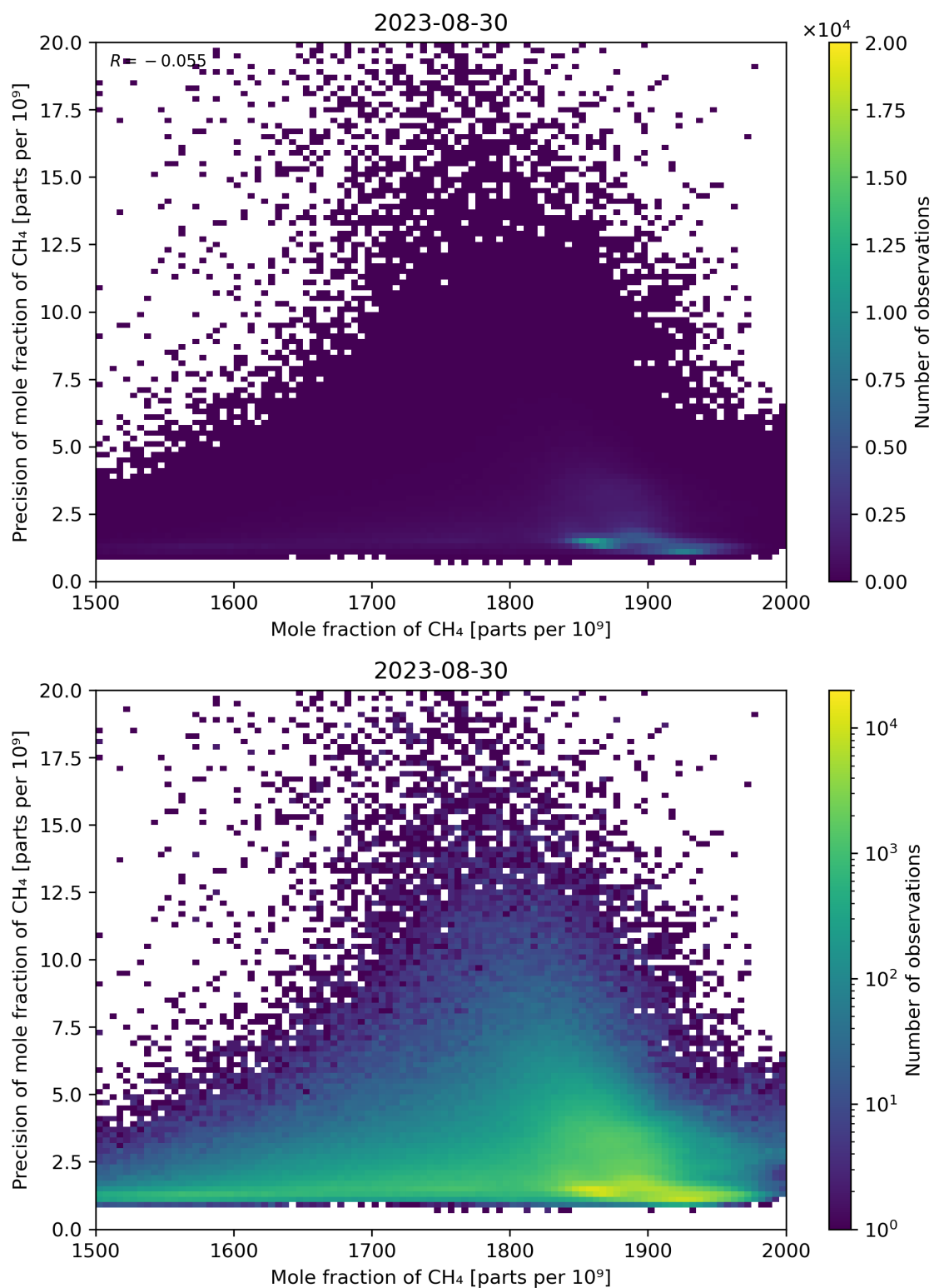
Figure 75: Scatter density plot of “Mole fraction of CH 4 ” against “Precision of mole fraction of CH 4 ” for 2023-08-30 to 2023-08-31.
