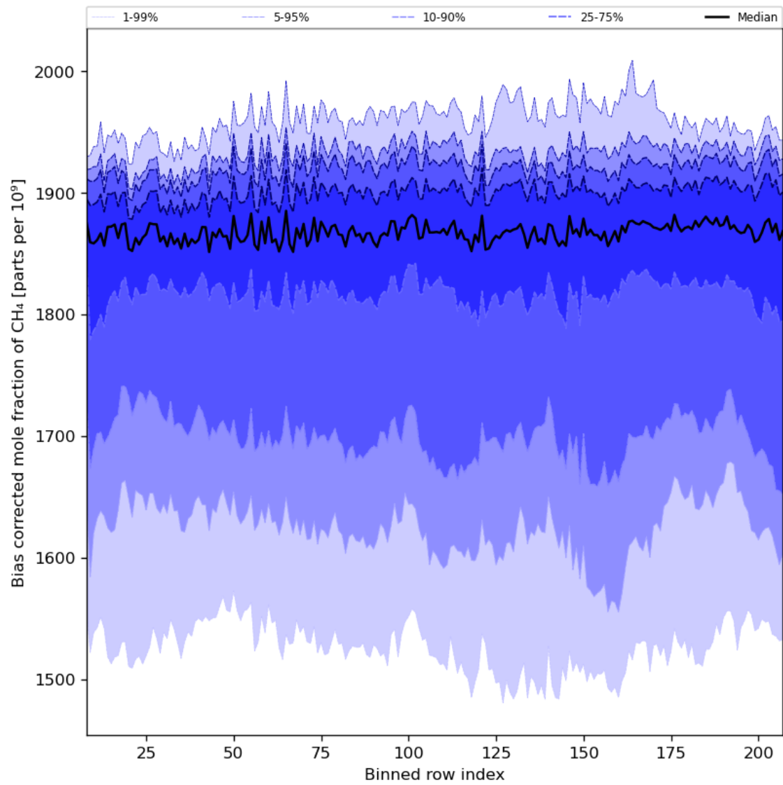
Figure 36: Along track statistics of “Bias corrected mole fraction of CH 4 ” for 2023-08-30 to 2023-08-31
