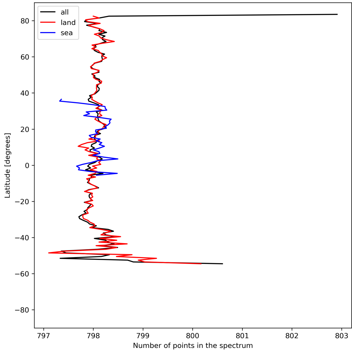
Figure 15: Zonal average of “Number of points in the spectrum” for 2023-08-30 to 2023-08-31.
