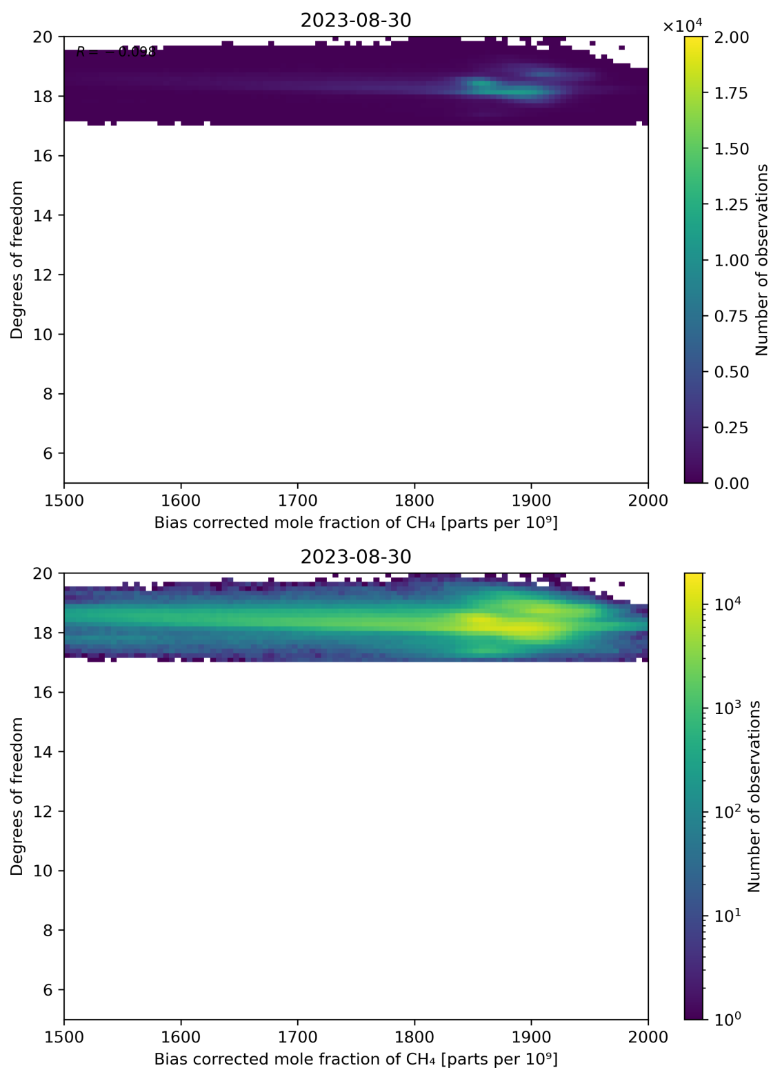
Figure 65: Scatter density plot of “Bias corrected mole fraction of CH 4 ” against “Degrees of freedom” for 2023-08-30 to 2023-08-31.
