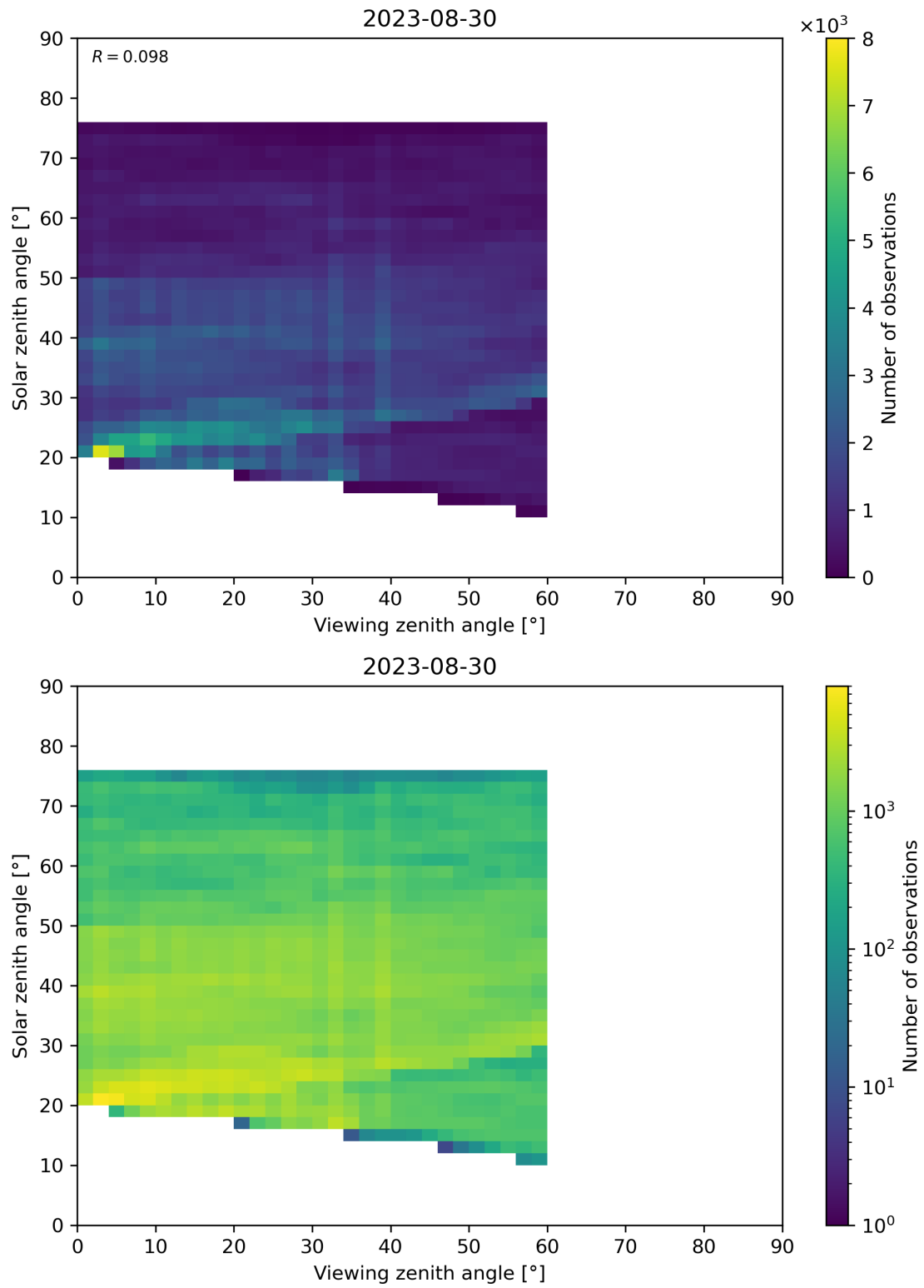
Figure 115: Scatter density plot of “Viewing zenith angle” against “Solar zenith angle” for 2023-08-30 to 2023-08-31.
