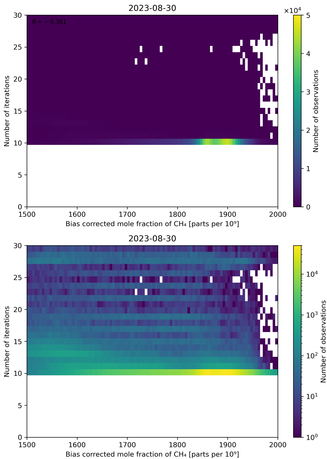
Figure 67: Scatter density plot of “Bias corrected mole fraction of \text{CH}_4 ” against “Number of iterations” for 2023-08-30 to 2023-08-31.
