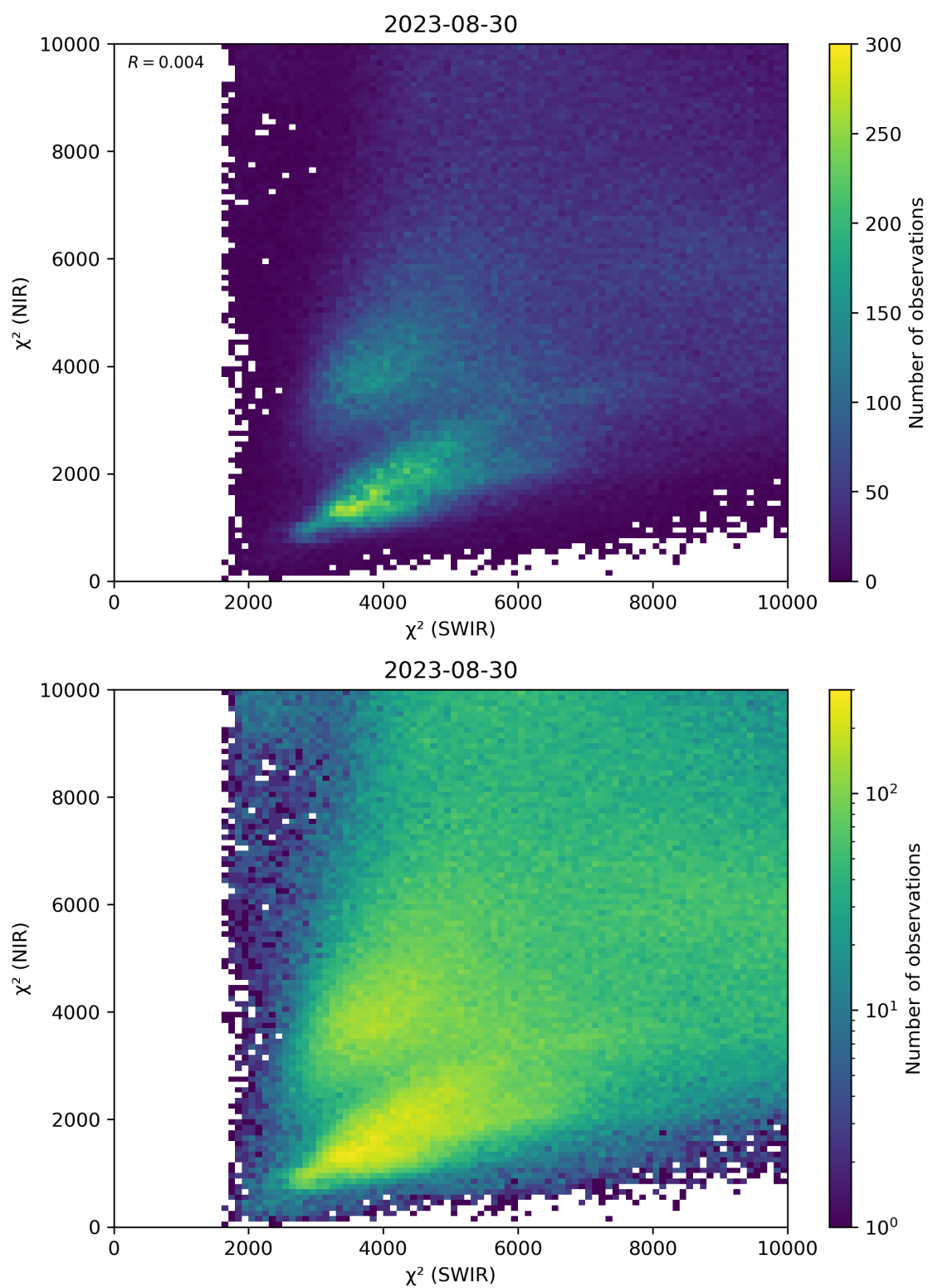
Figure 47: Scatter density plot of “ \chi^2 (SWIR)” against “ \chi^2 (NIR)” for 2023-08-30 to 2023-08-31.
