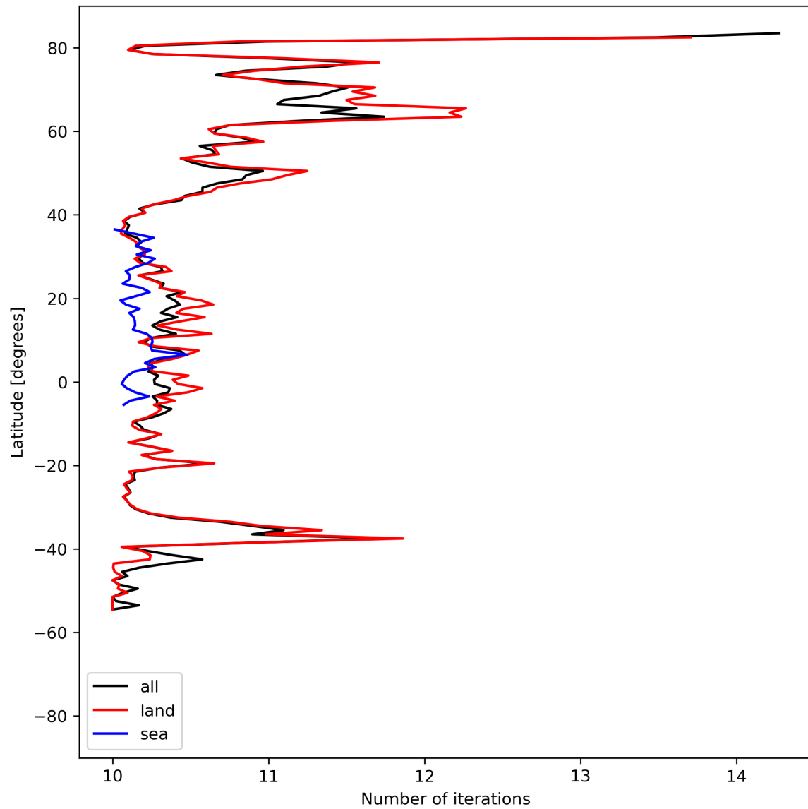
Figure 20: Zonal average of “Number of iterations” for 2023-08-30 to 2023-08-31.
