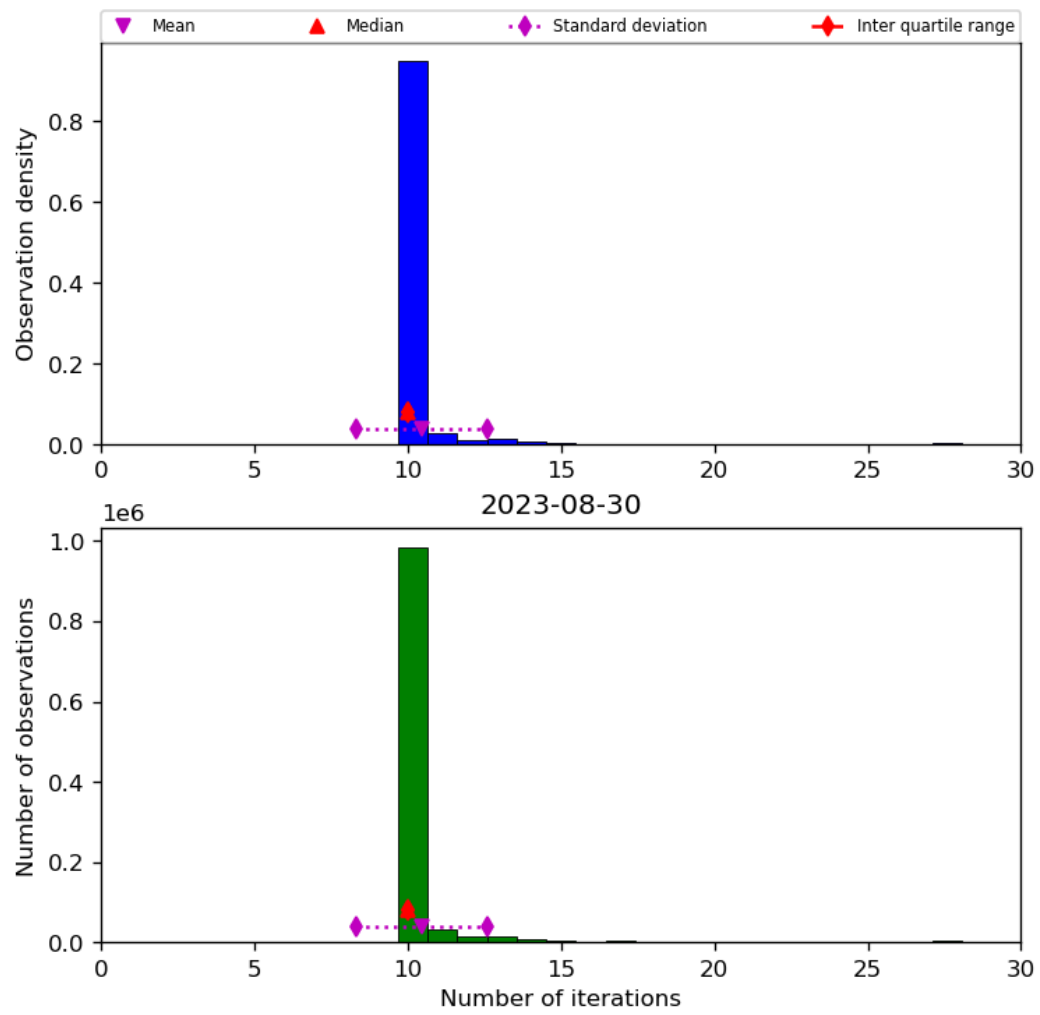
Figure 31: Histogram of “Number of iterations” for 2023-08-30 to 2023-08-31
