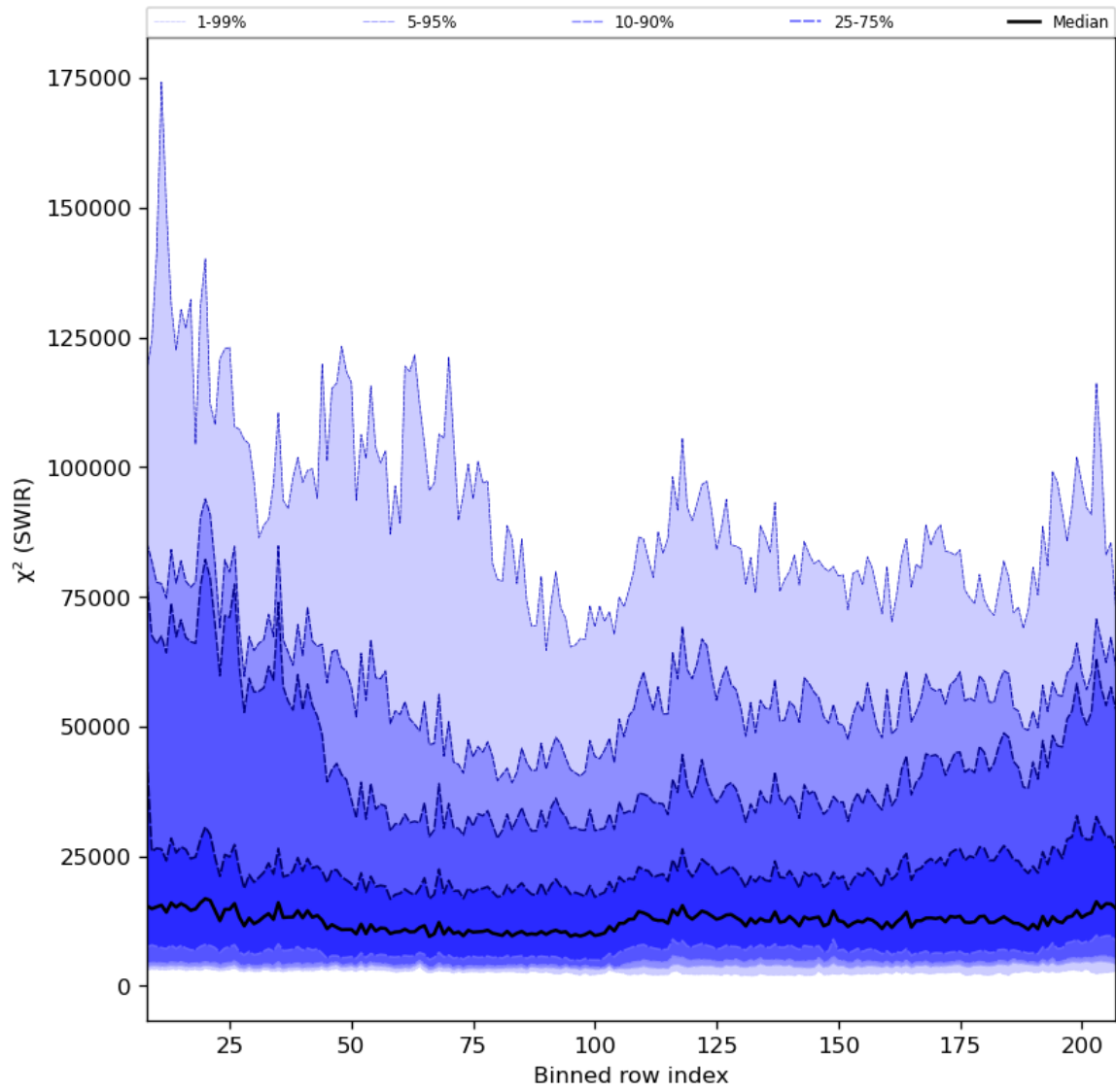
Figure 39: Along track statistics of “ \chi^2 (SWIR)” for 2023-08-30 to 2023-08-31
