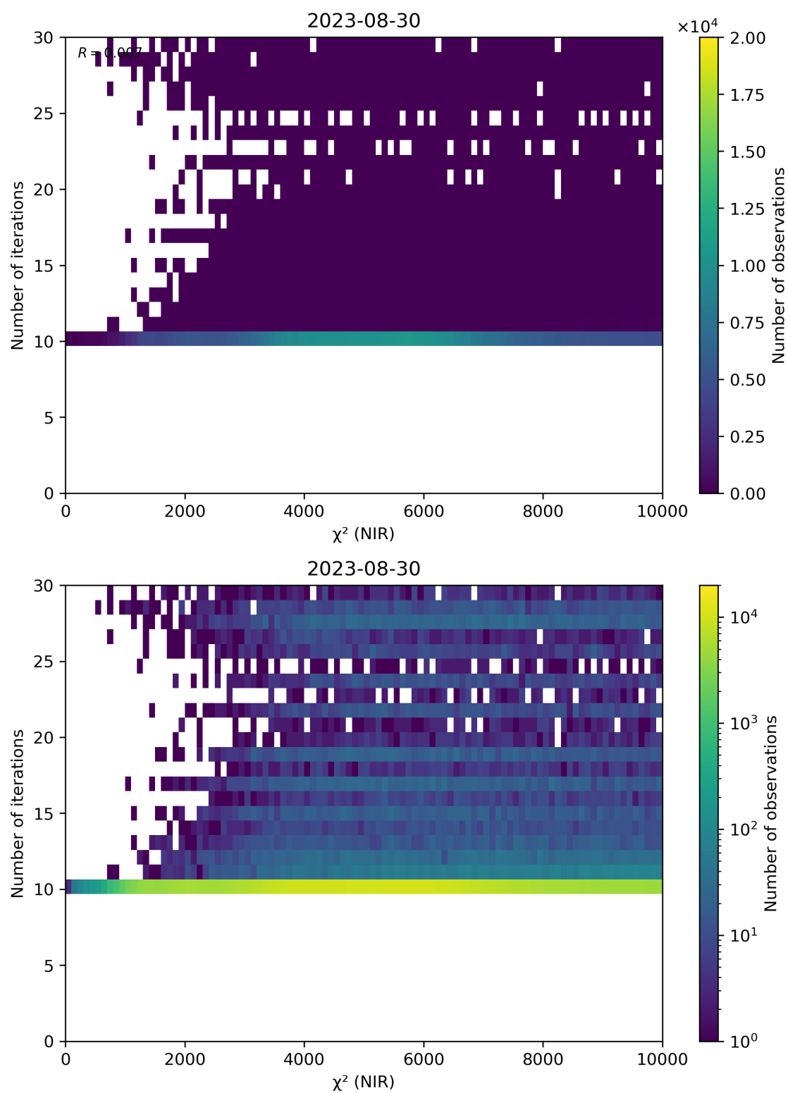
Figure 46: Scatter density plot of “ \chi^2 (NIR)” against “Number of iterations” for 2023-08-30 to 2023-08-31.
