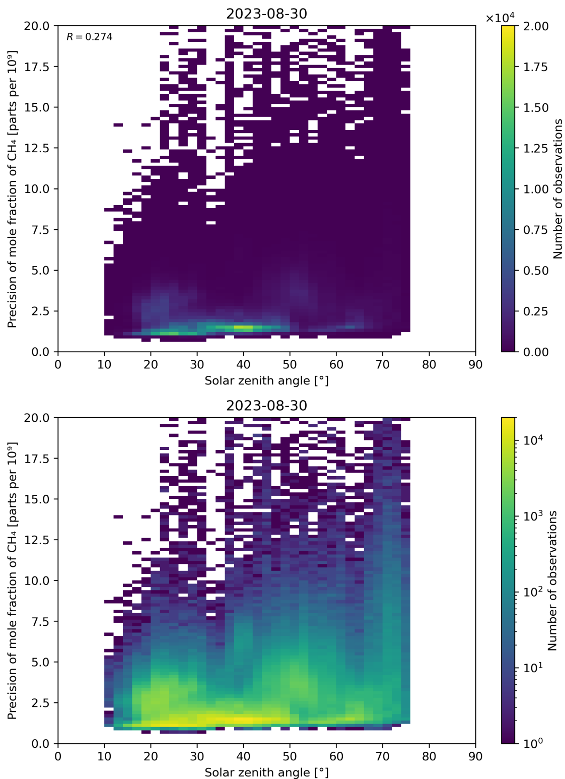
Figure 101: Scatter density plot of “Solar zenith angle” against “Precision of mole fraction of \text{CH}_4 ” for 2023-08-30 to 2023-08-31.
