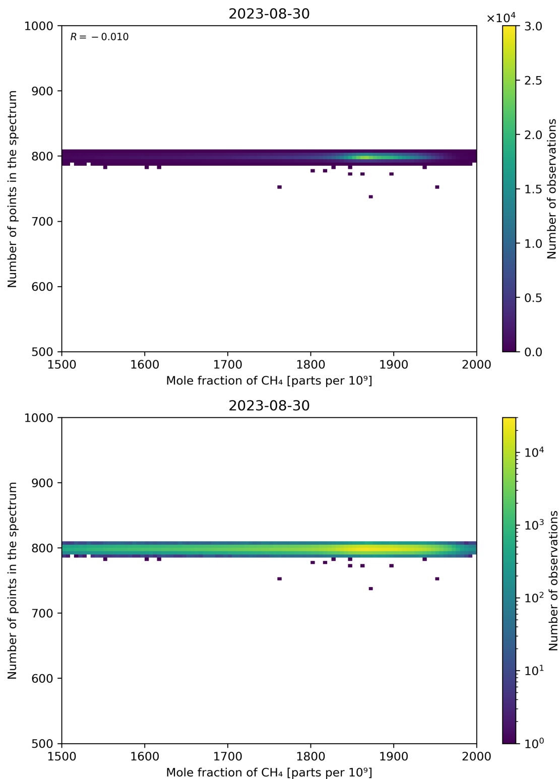
Figure 77: Scatter density plot of “Mole fraction of CH 4 ” against “Number of points in the spectrum” for 2023-08-30 to 2023-08-31.
