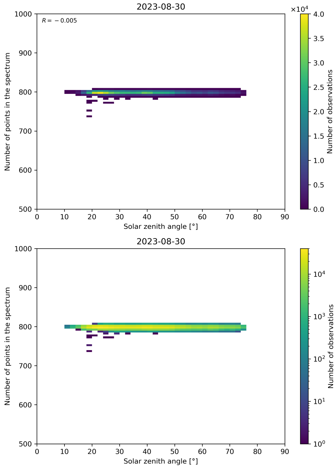
Figure 103: Scatter density plot of “Solar zenith angle” against “Number of points in the spectrum” for 2023-08-30 to 2023-08-31.
