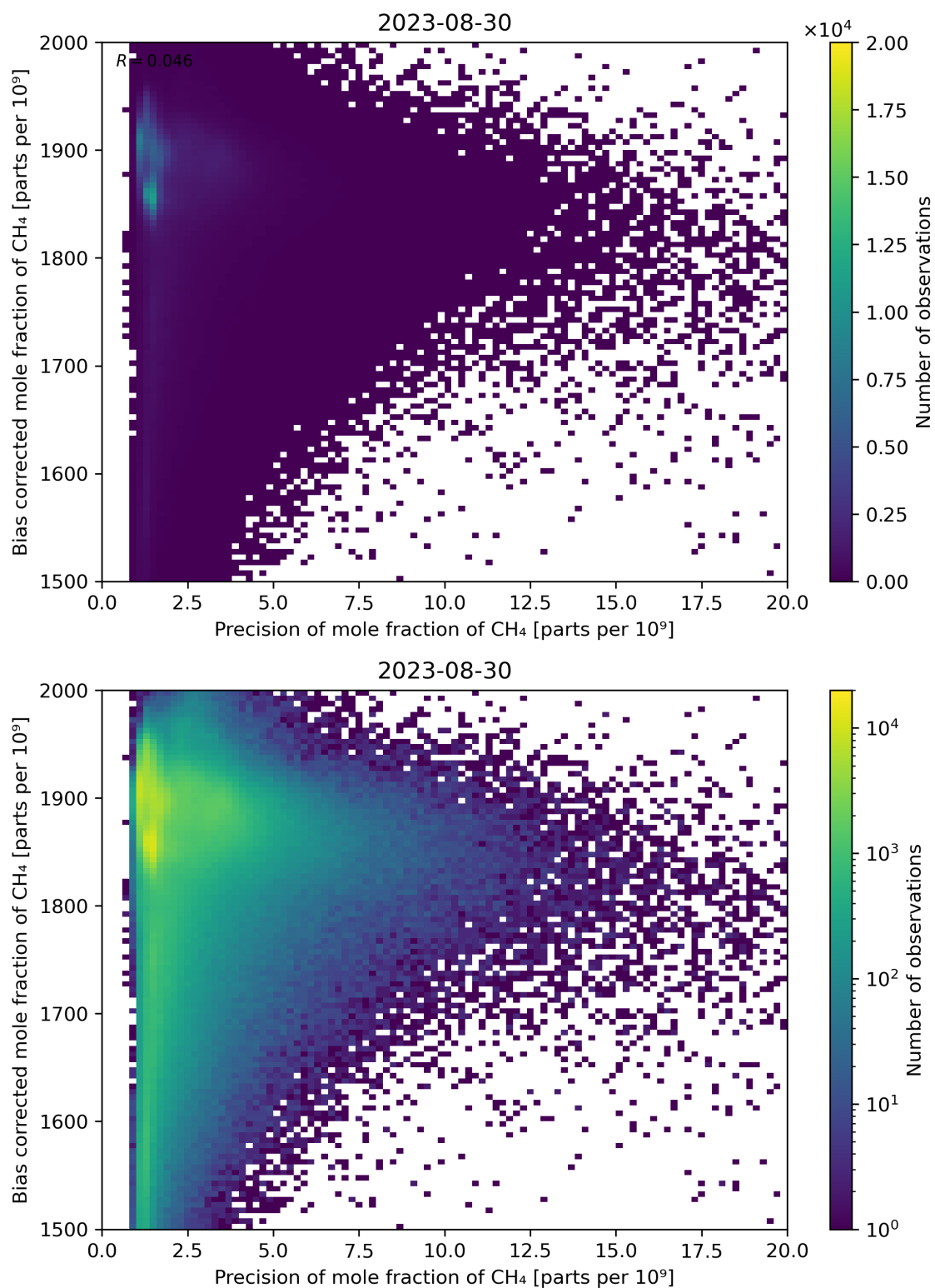
Figure 82: Scatter density plot of “Precision of mole fraction of CH 4 ” against “Bias corrected mole fraction of CH 4 ” for 2023-08-30 to 2023-08-31.
