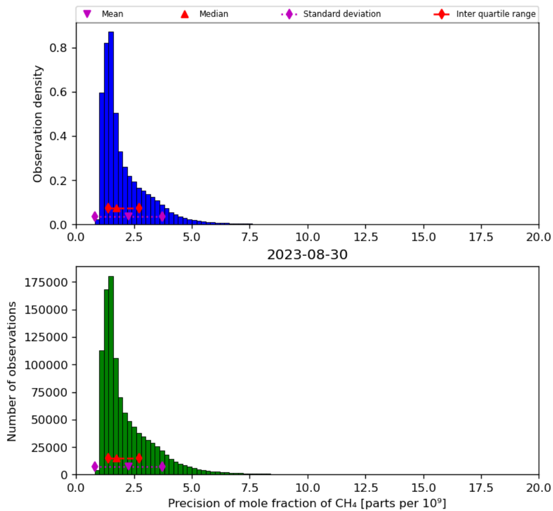
Figure 24: Histogram of “Precision of mole fraction of CH 4 ” for 2023-08-30 to 2023-08-31
