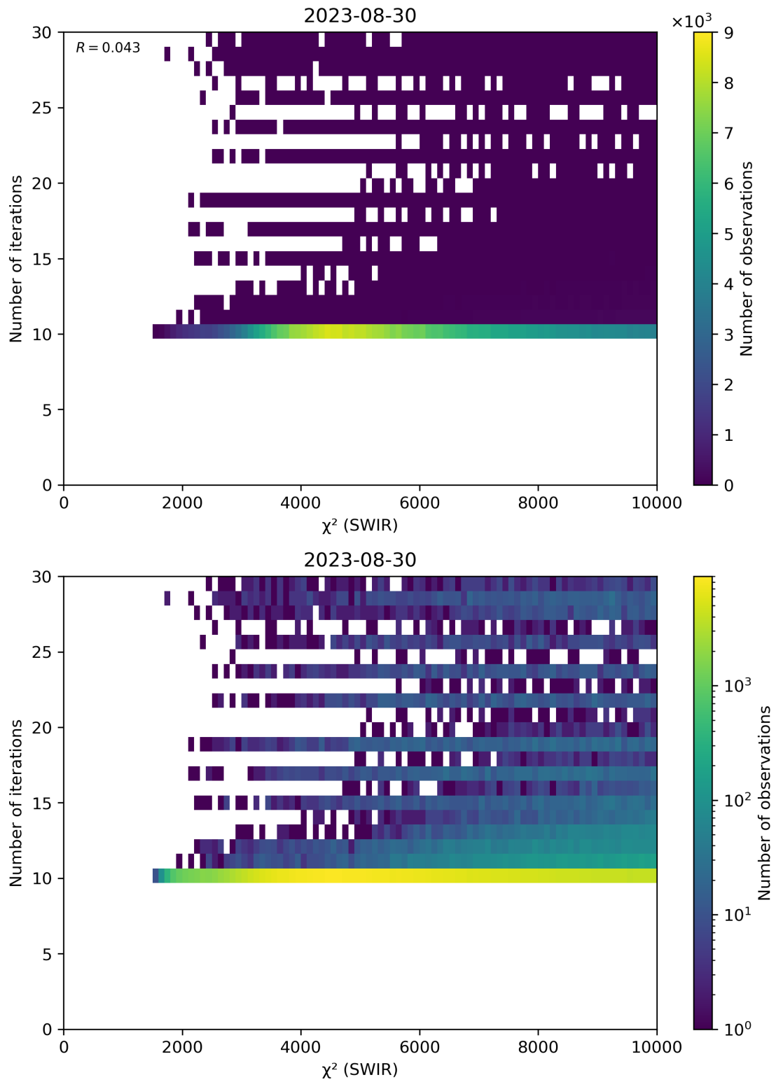
Figure 50: Scatter density plot of “ \chi^2 (SWIR)” against “Number of iterations” for 2023-08-30 to 2023-08-31.
