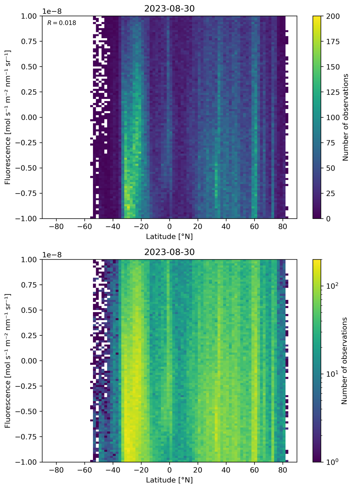
Figure 56: Scatter density plot of “Latitude” against “Fluorescence” for 2023-08-30 to 2023-08-31.
