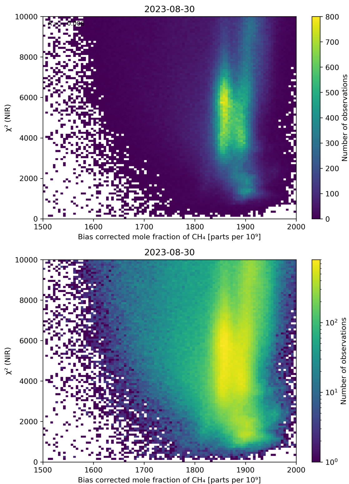
Figure 63: Scatter density plot of “Bias corrected mole fraction of CH 4 ” against “ \chi^2 (NIR)” for 2023-08-30 to 2023-08-31.
