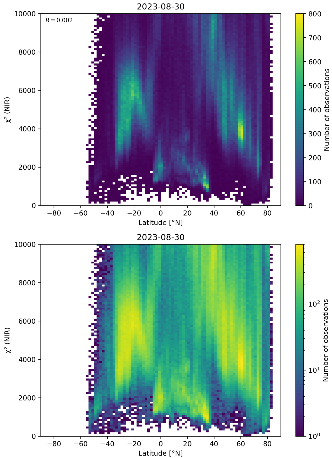
Figure 53: Scatter density plot of “Latitude” against “ \chi^2 (NIR)” for 2023-08-30 to 2023-08-31.
