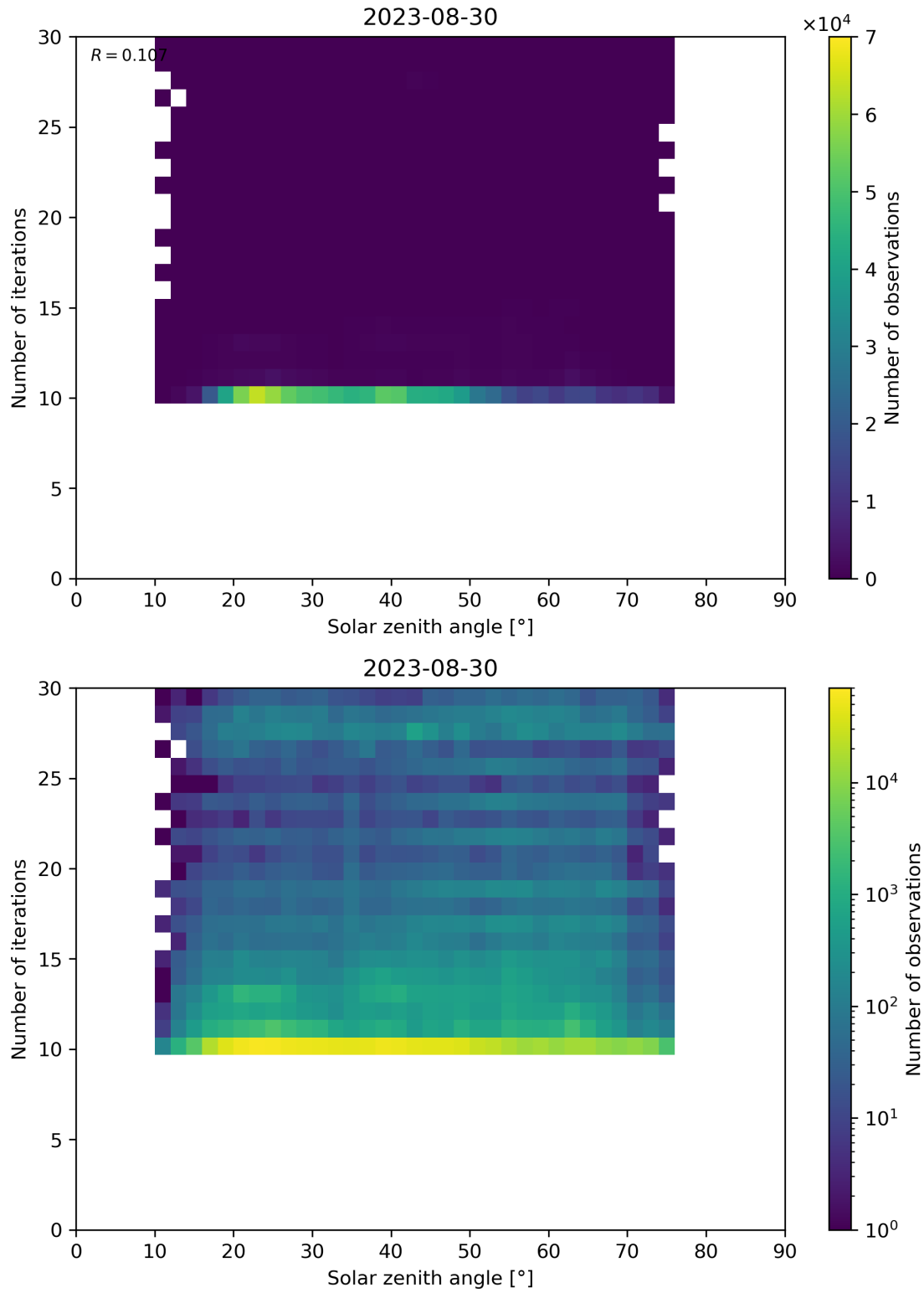
Figure 102: Scatter density plot of “Solar zenith angle” against “Number of iterations” for 2023-08-30 to 2023-08-31.
