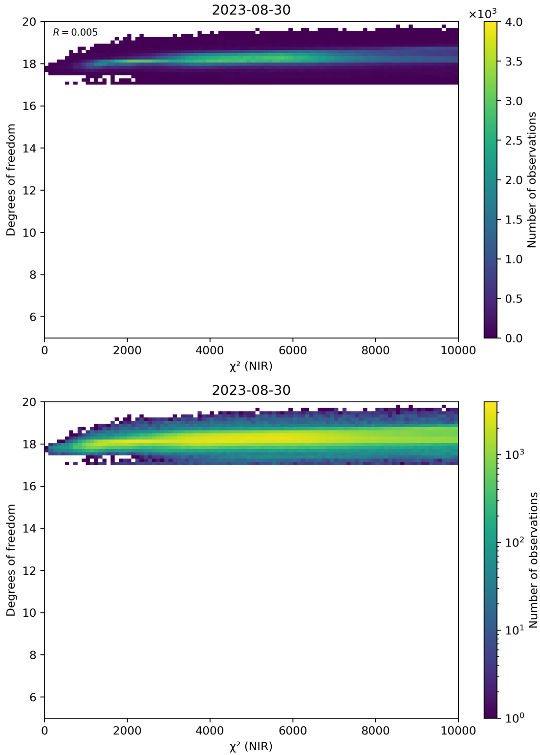
Figure 44: Scatter density plot of “ \chi^2 (NIR)” against “Degrees of freedom” for 2023-08-30 to 2023-08-31.
