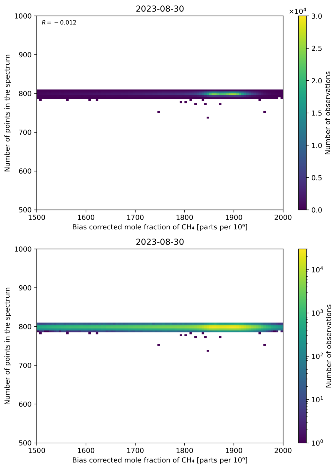
Figure 68: Scatter density plot of “Bias corrected mole fraction of CH 4 ” against “Number of points in the spectrum” for 2023-08-30 to 2023-08-31.
