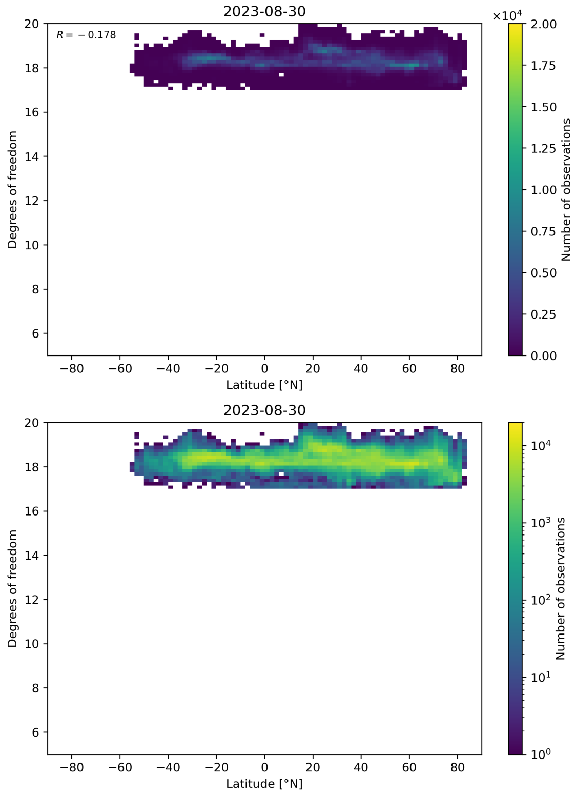
Figure 55: Scatter density plot of “Latitude” against “Degrees of freedom” for 2023-08-30 to 2023-08-31.
