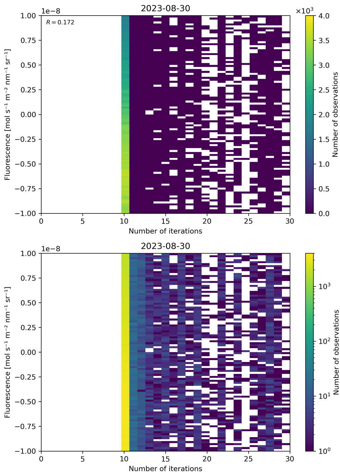
Figure 87: Scatter density plot of “Number of iterations” against “Fluorescence” for 2023-08-30 to 2023-08-31.
