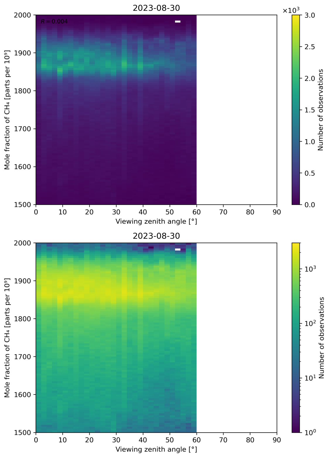
Figure 110: Scatter density plot of “Viewing zenith angle” against “Mole fraction of CH 4 ” for 2023-08-30 to 2023-08-31.
