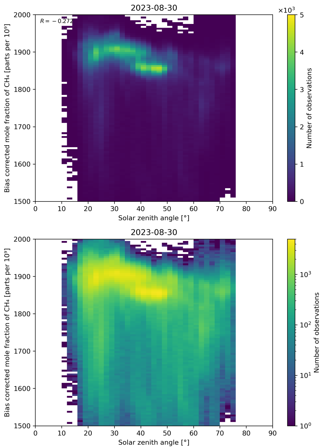
Figure 100: Scatter density plot of “Solar zenith angle” against “Bias corrected mole fraction of \text{CH}_4 ” for 2023-08-30 to 2023-08-31.
