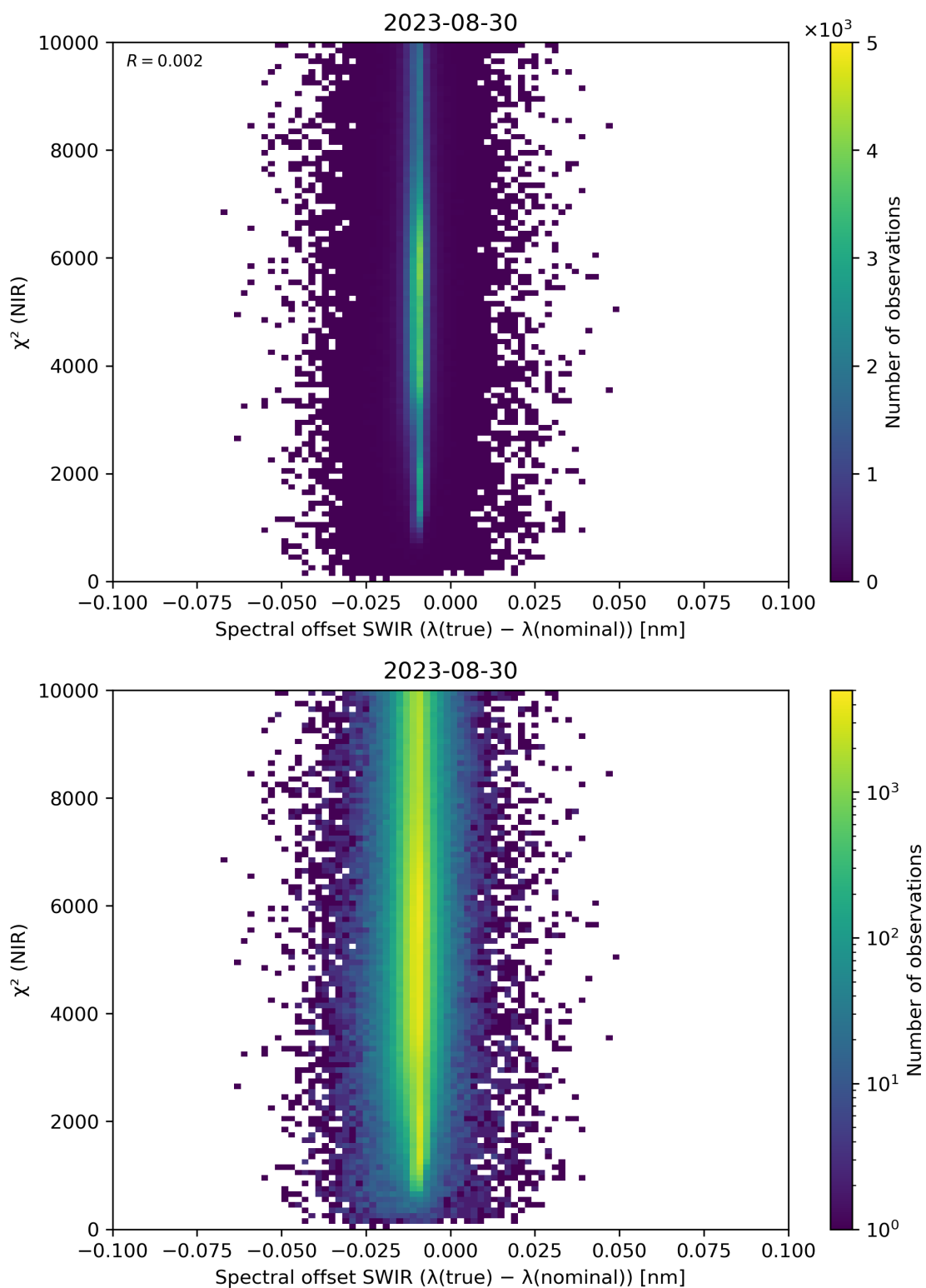
Figure 117: Scatter density plot of “Spectral offset SWIR ( \lambda(\text{true}) - \lambda(\text{nominal}) )” against “ \chi^2 (NIR)” for 2023-08-30 to 2023-08-31.
