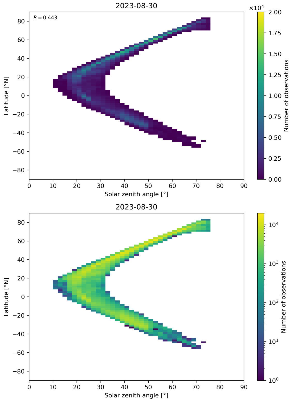
Figure 98: Scatter density plot of “Solar zenith angle” against “Latitude” for 2023-08-30 to 2023-08-31.
