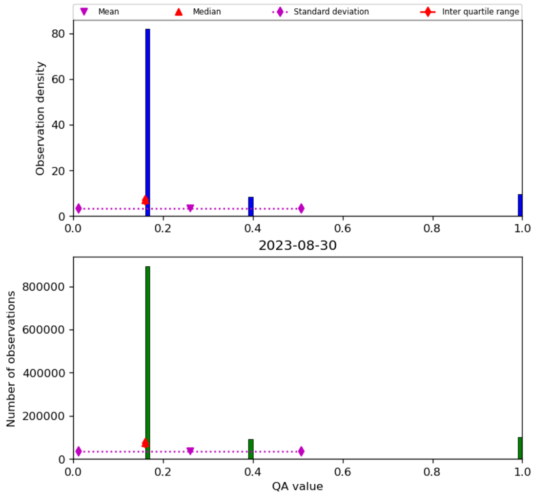
Figure 22: Histogram of “QA value” for 2023-08-30 to 2023-08-31
