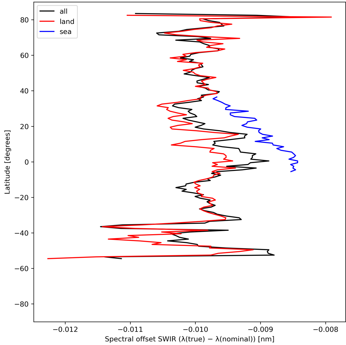
Figure 16: Zonal average of “Spectral offset SWIR ( \lambda(\text{true}) - \lambda(\text{nominal}) )” for 2023-08-30 to 2023-08-31.
