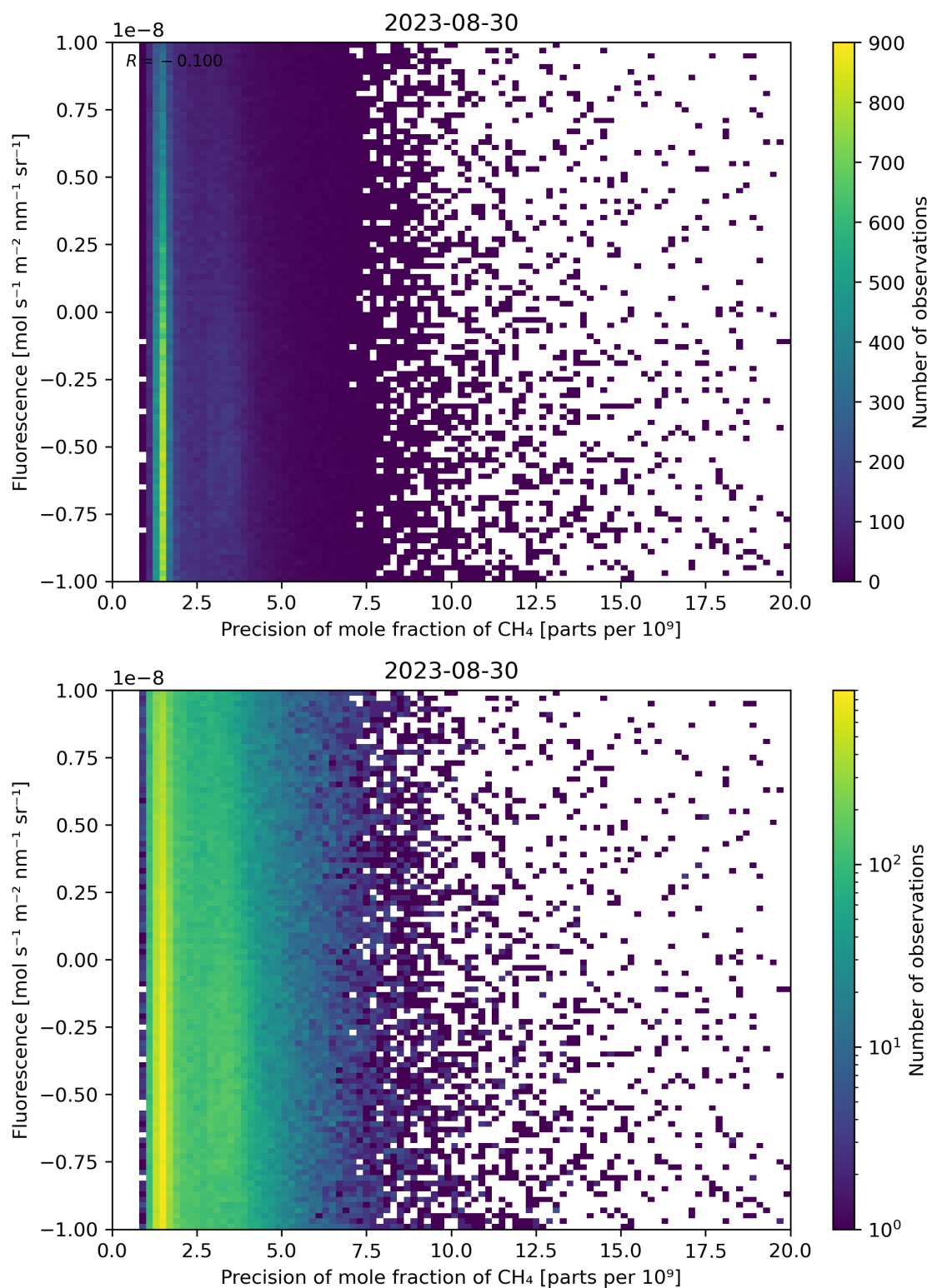
Figure 81: Scatter density plot of “Precision of mole fraction of \text{CH}_4 ” against “Fluorescence” for 2023-08-30 to 2023-08-31.
