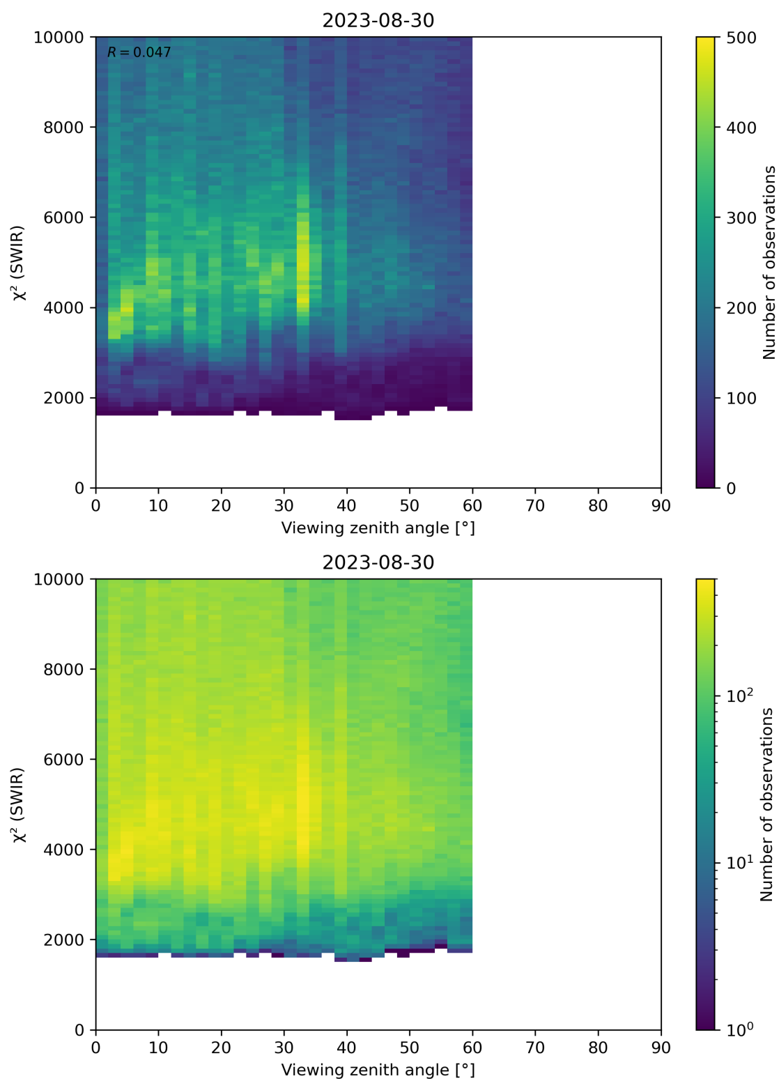
Figure 106: Scatter density plot of “Viewing zenith angle” against “ \chi^2 (SWIR)” for 2023-08-30 to 2023-08-31.
