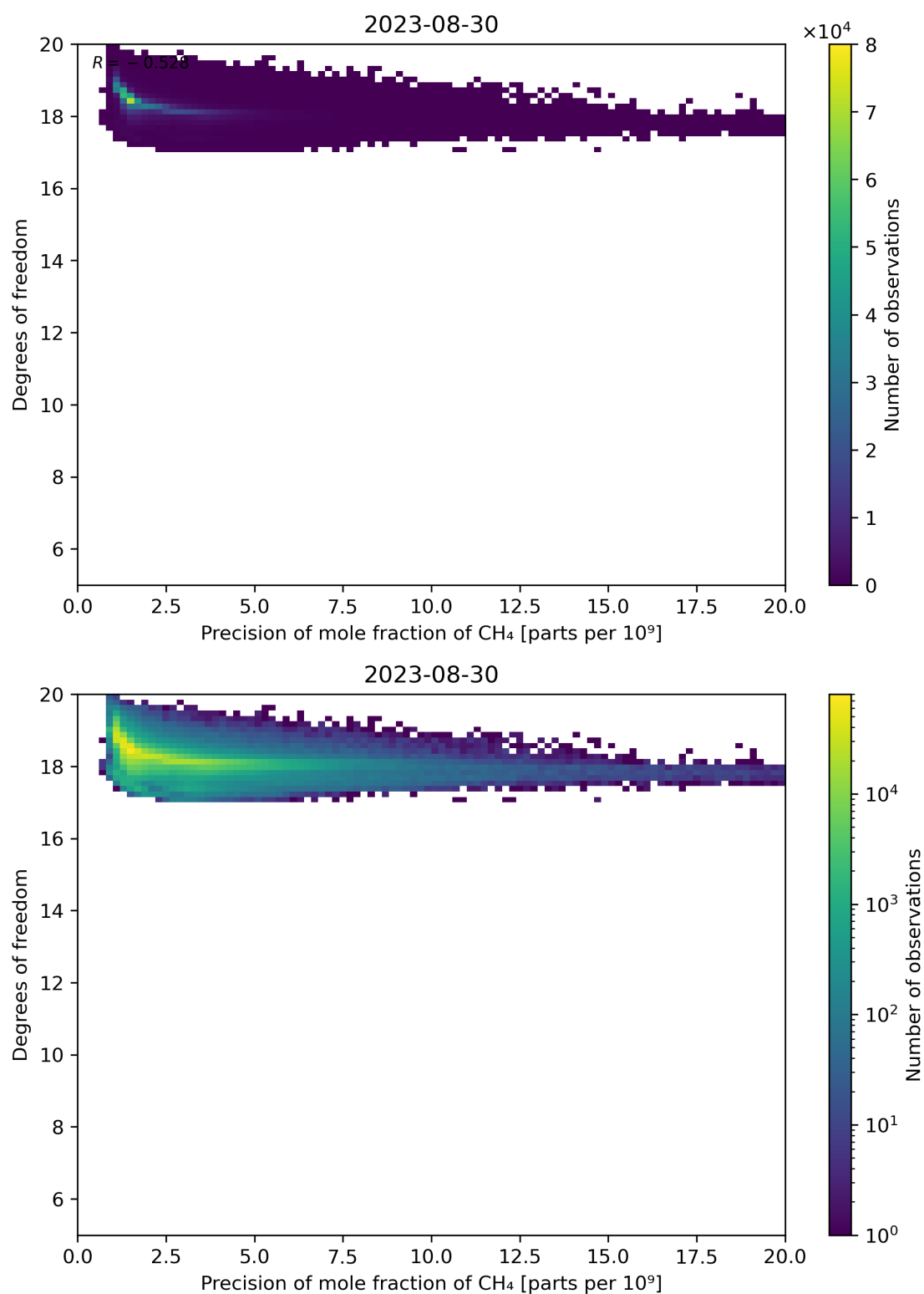
Figure 80: Scatter density plot of “Precision of mole fraction of CH 4 ” against “Degrees of freedom” for 2023-08-30 to 2023-08-31.
