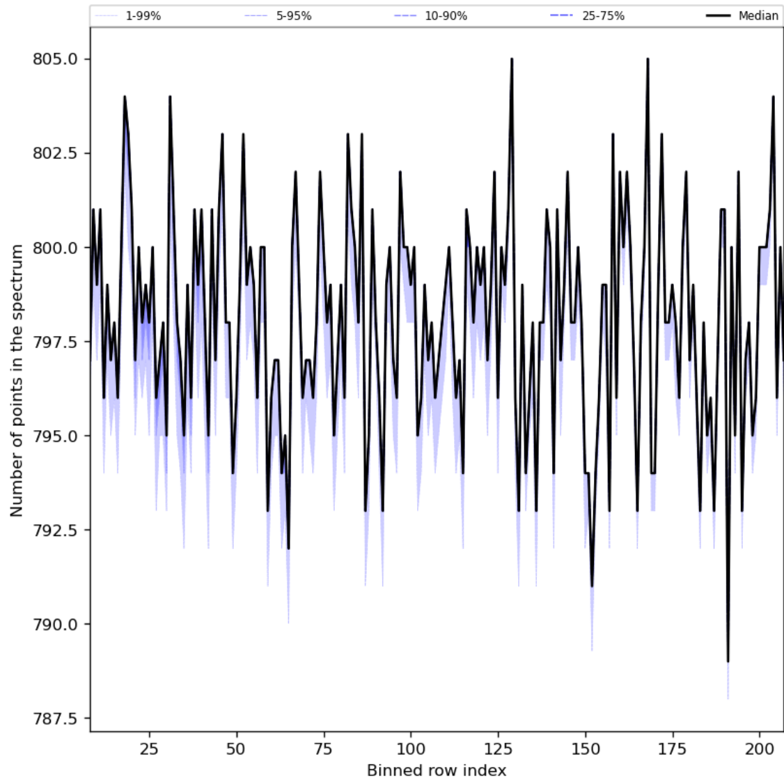
Figure 37: Along track statistics of “Number of points in the spectrum” for 2023-08-30 to 2023-08-31
