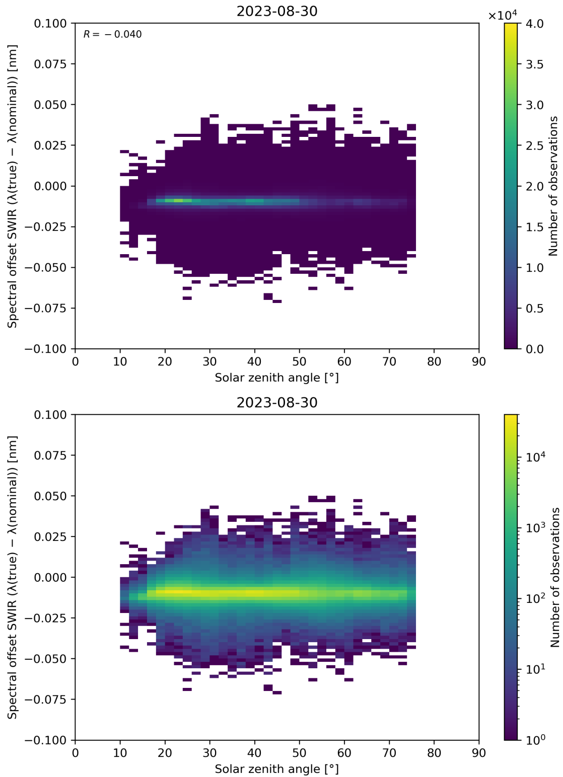
Figure 104: Scatter density plot of “Solar zenith angle” against “Spectral offset SWIR ( \lambda(\text{true}) - \lambda(\text{nominal}) )” for 2023-08-30 to 2023-08-31.
