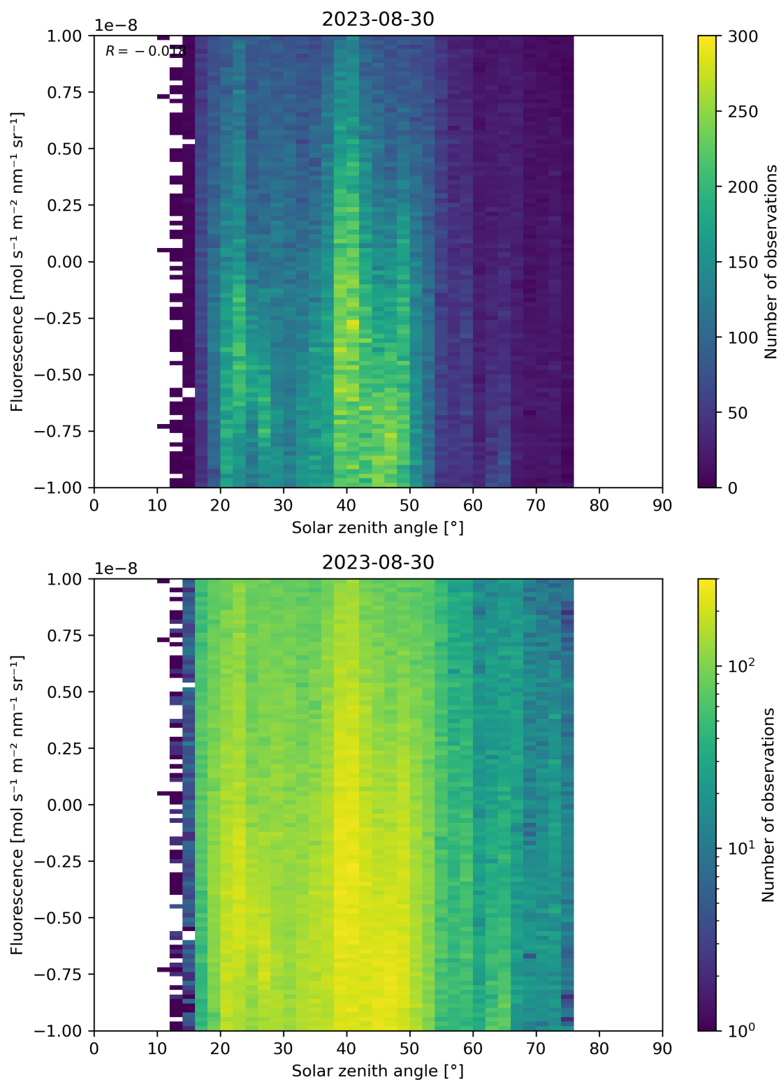
Figure 97: Scatter density plot of “Solar zenith angle” against “Fluorescence” for 2023-08-30 to 2023-08-31.
