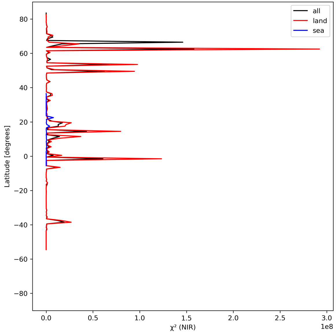
Figure 18: Zonal average of “ \chi^2 (NIR)” for 2023-08-30 to 2023-08-31.
