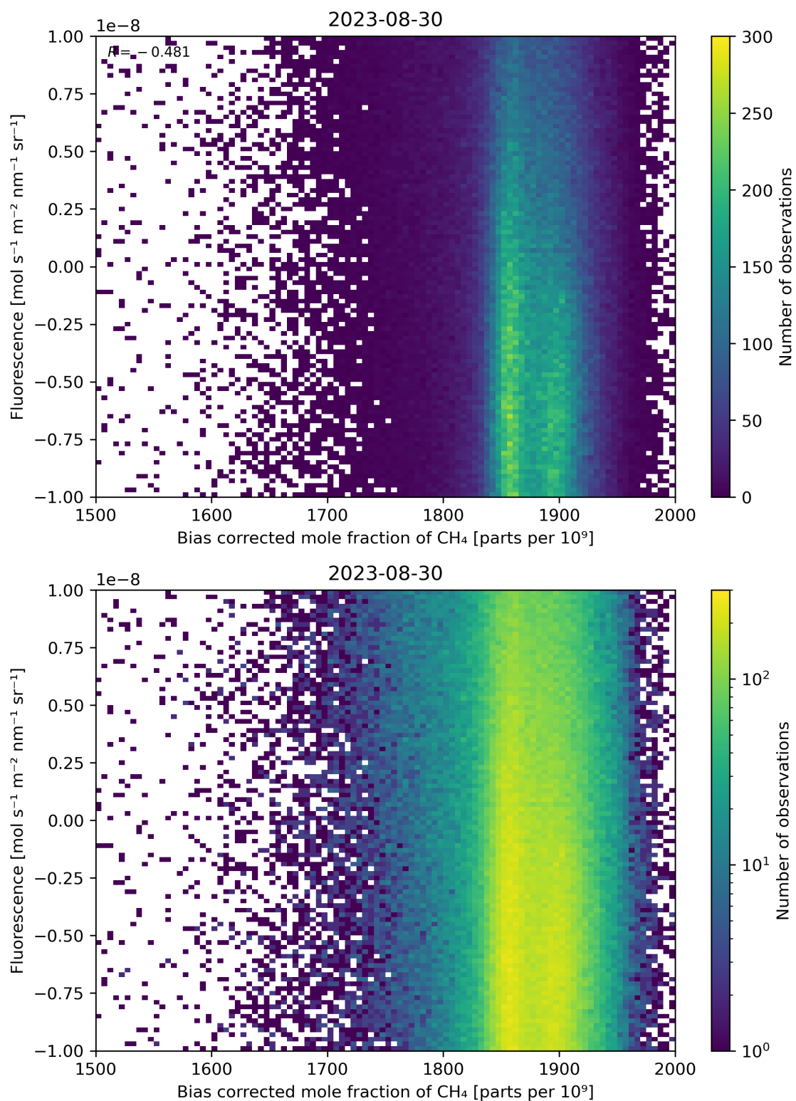
Figure 66: Scatter density plot of “Bias corrected mole fraction of \text{CH}_4 ” against “Fluorescence” for 2023-08-30 to 2023-08-31.
