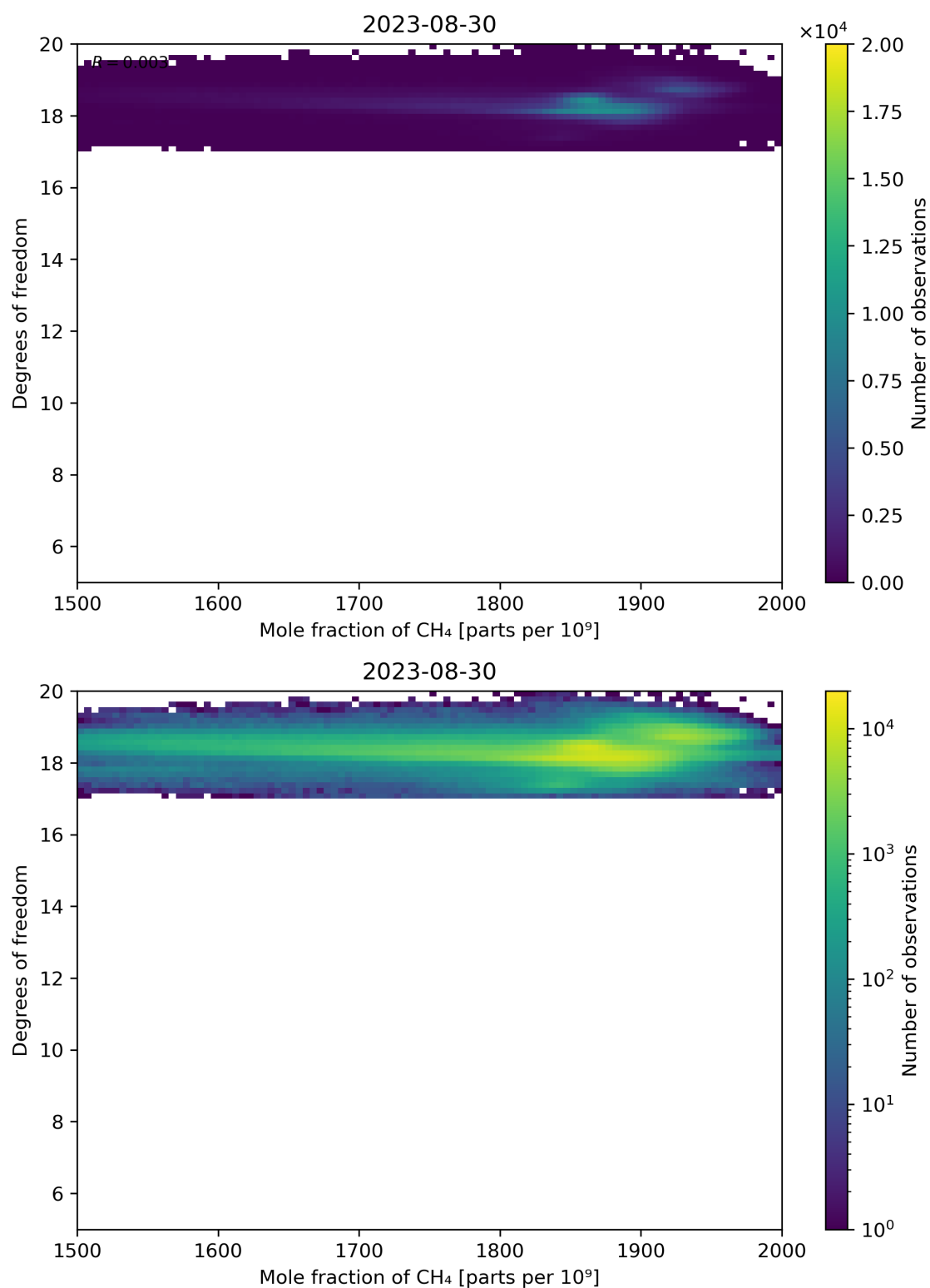
Figure 72: Scatter density plot of “Mole fraction of CH 4 ” against “Degrees of freedom” for 2023-08-30 to 2023-08-31.
