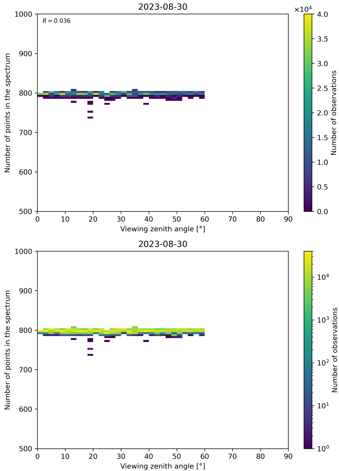
Figure 114: Scatter density plot of “Viewing zenith angle” against “Number of points in the spectrum” for 2023-08-30 to 2023-08-31.
