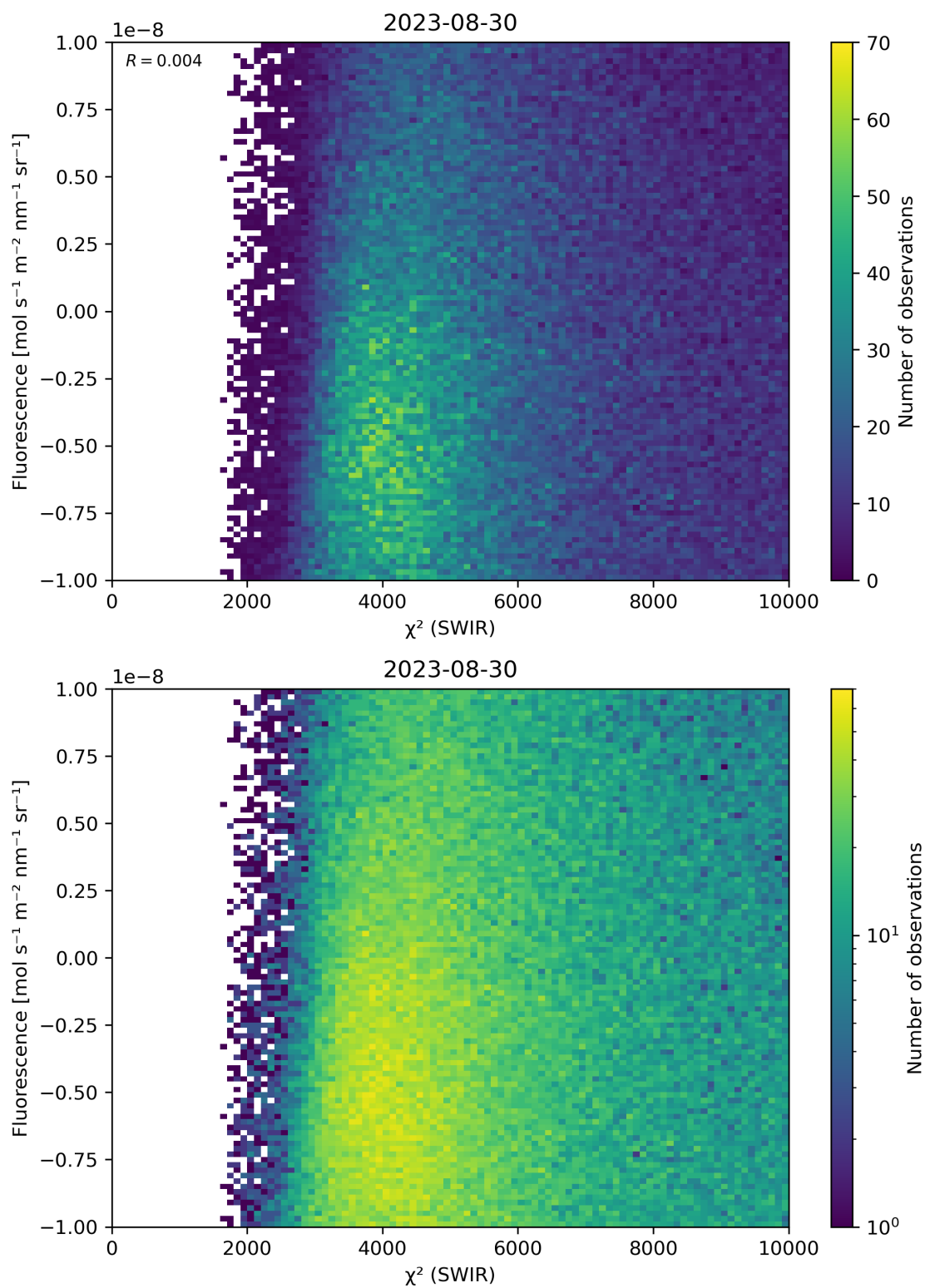
Figure 49: Scatter density plot of “ \chi^2 (SWIR)” against “Fluorescence” for 2023-08-30 to 2023-08-31.
