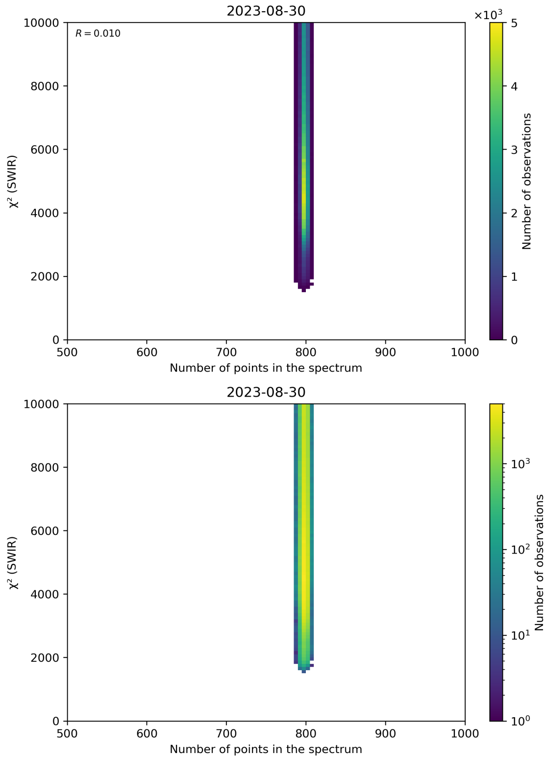
Figure 89: Scatter density plot of “Number of points in the spectrum” against “ \chi^2 (SWIR)” for 2023-08-30 to 2023-08-31.
