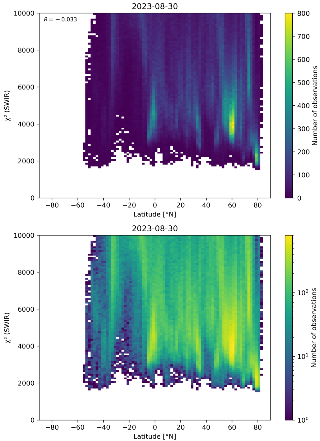
Figure 54: Scatter density plot of “Latitude” against “ \chi^2 (SWIR)” for 2023-08-30 to 2023-08-31.
