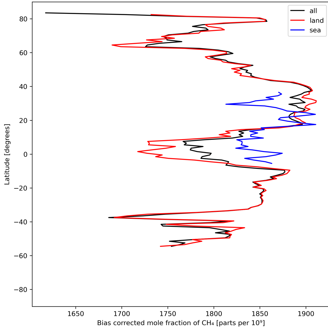
Figure 14: Zonal average of “Bias corrected mole fraction of \text{CH}_4 ” for 2023-08-30 to 2023-08-31.
