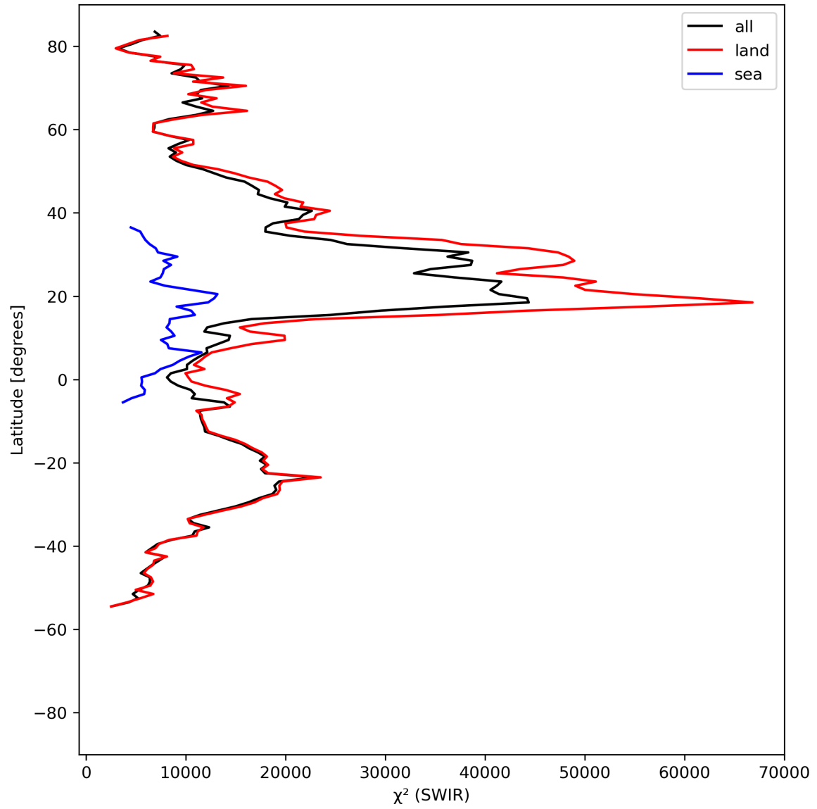
Figure 17: Zonal average of “ \chi^2 (SWIR)” for 2023-08-30 to 2023-08-31.
