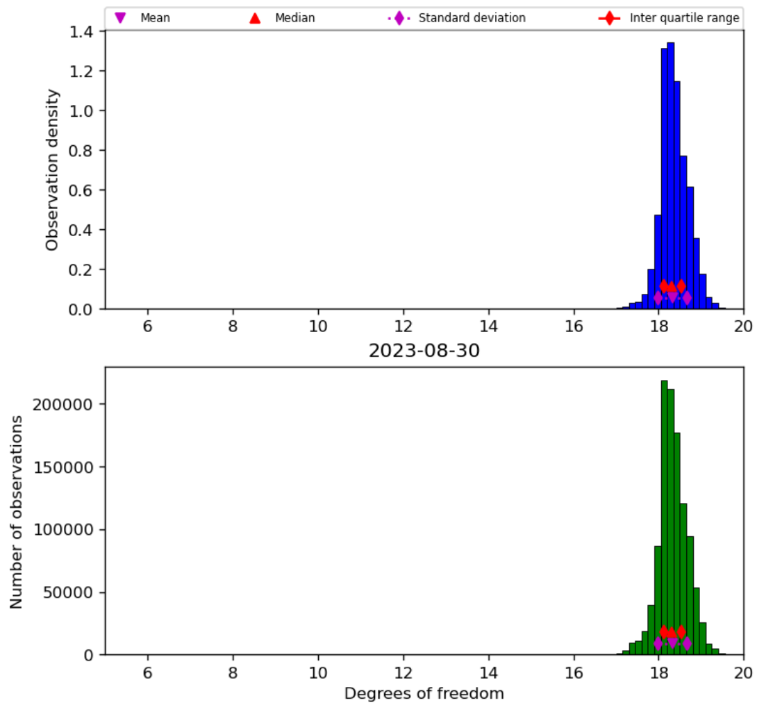
Figure 30: Histogram of “Degrees of freedom” for 2023-08-30 to 2023-08-31
