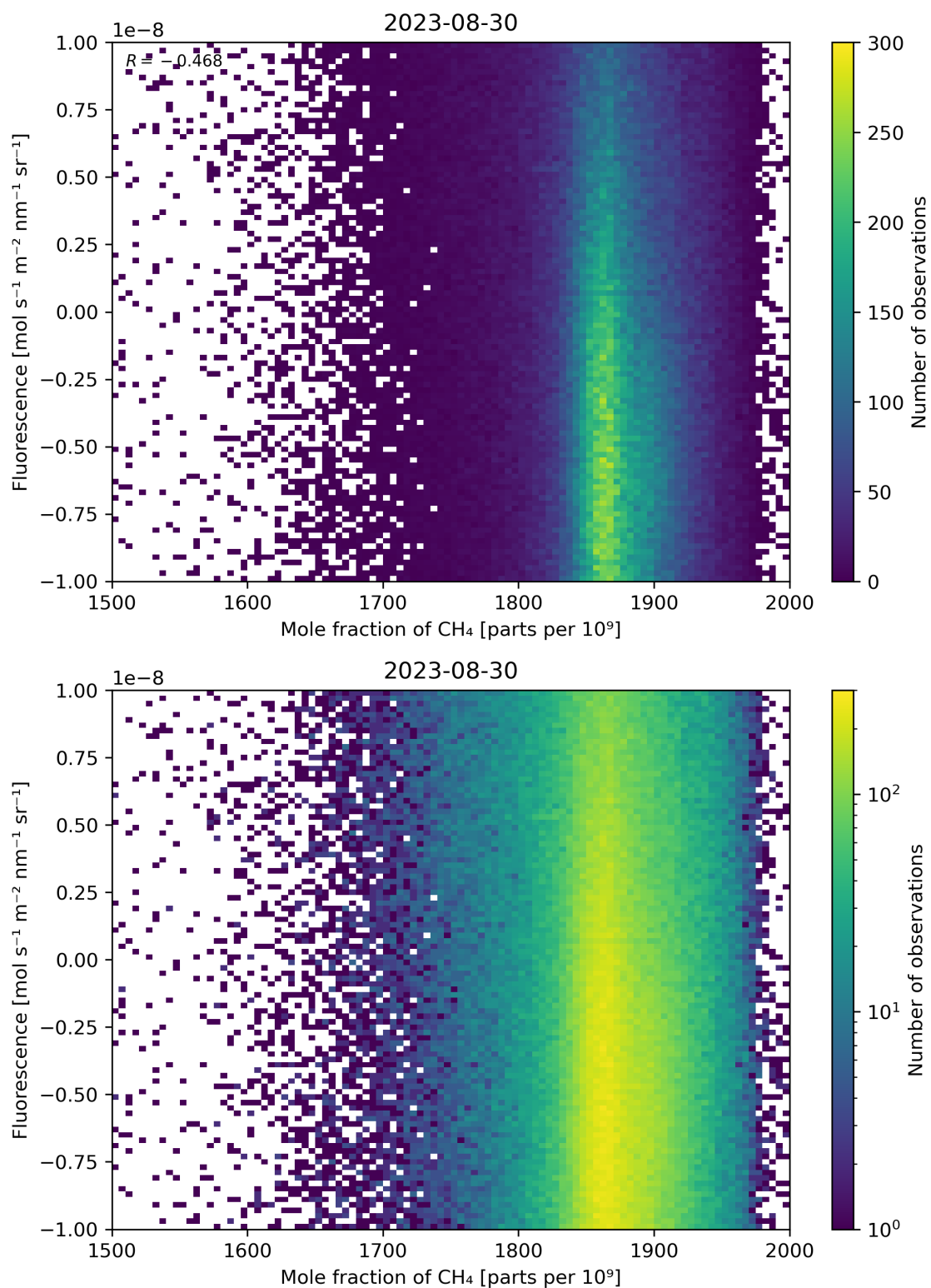
Figure 73: Scatter density plot of “Mole fraction of \text{CH}_4 ” against “Fluorescence” for 2023-08-30 to 2023-08-31.
