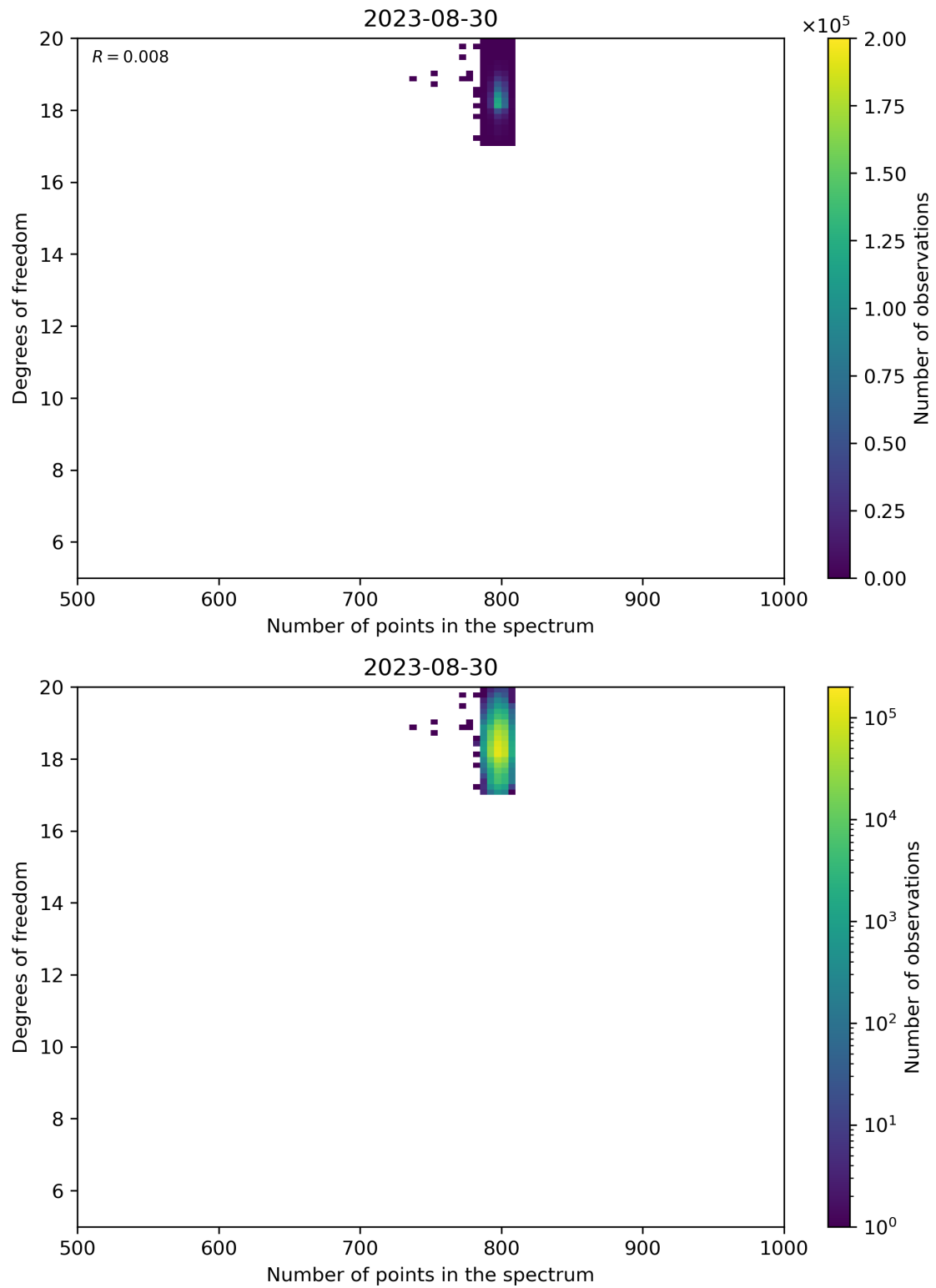
Figure 90: Scatter density plot of “Number of points in the spectrum” against “Degrees of freedom” for 2023-08-30 to 2023-08-31.
