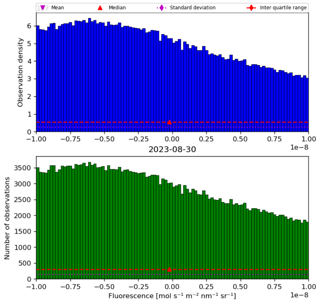
Figure 32: Histogram of “Fluorescence” for 2023-08-30 to 2023-08-31
