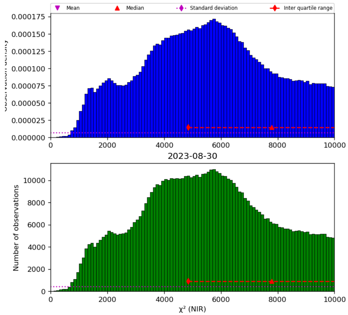
Figure 29: Histogram of “ \chi^2 (NIR)” for 2023-08-30 to 2023-08-31
