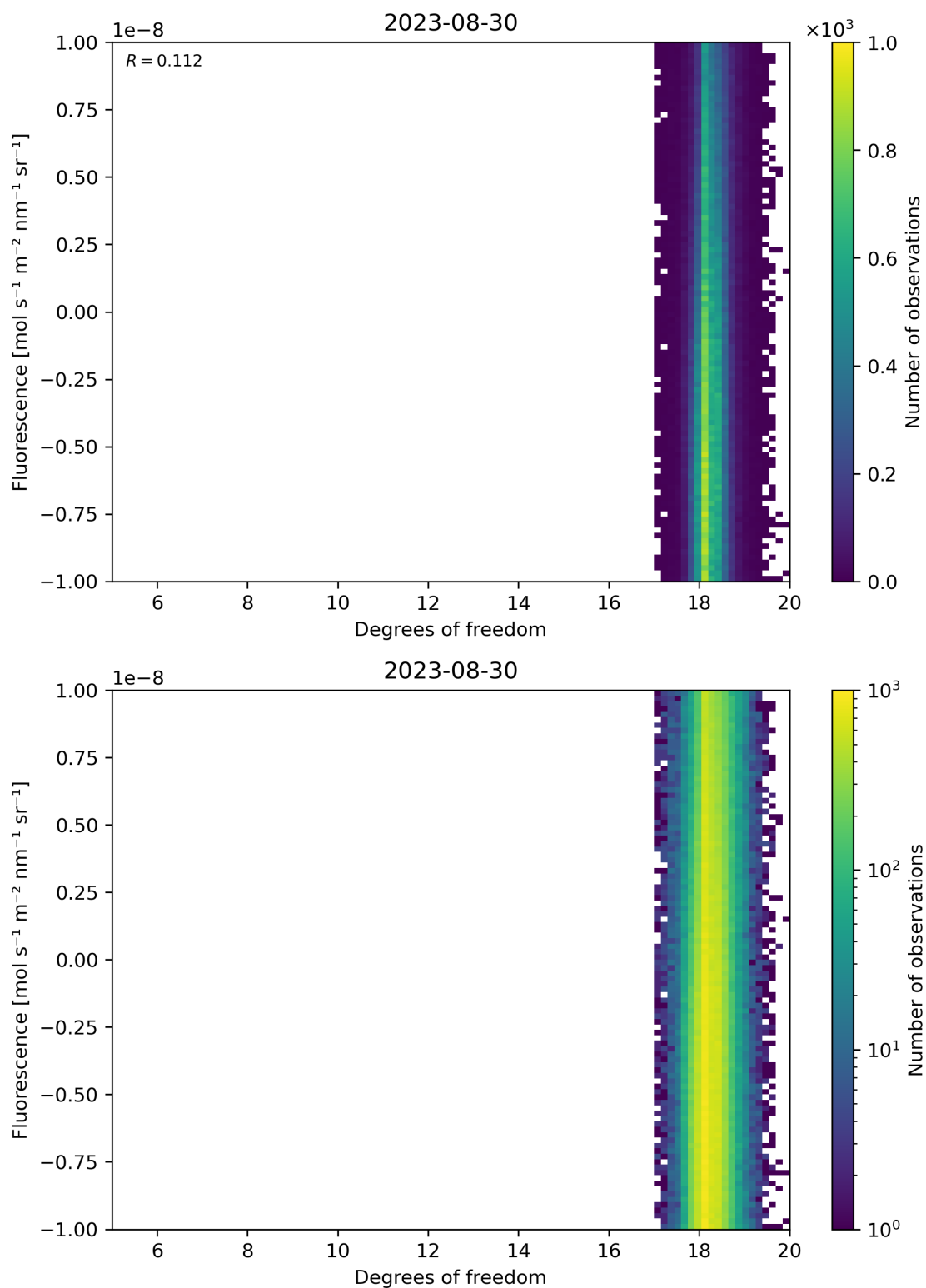
Figure 51: Scatter density plot of “Degrees of freedom” against “Fluorescence” for 2023-08-30 to 2023-08-31.
