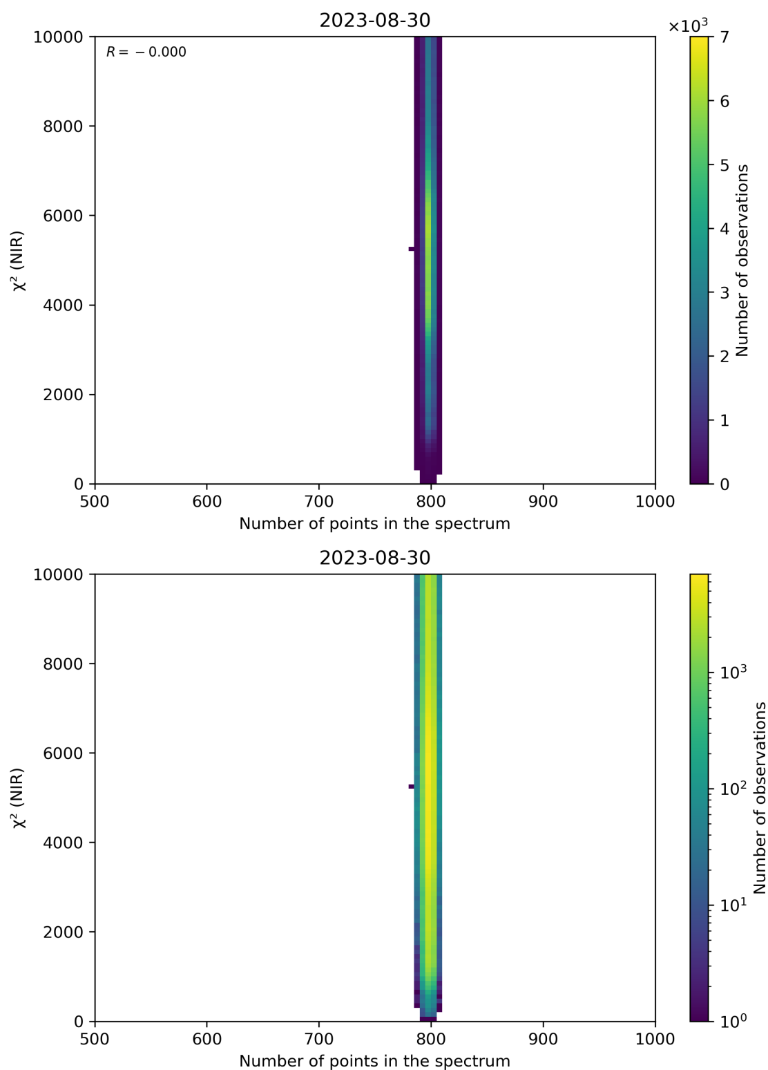
Figure 88: Scatter density plot of “Number of points in the spectrum” against “ \chi^2 (NIR)” for 2023-08-30 to 2023-08-31.
