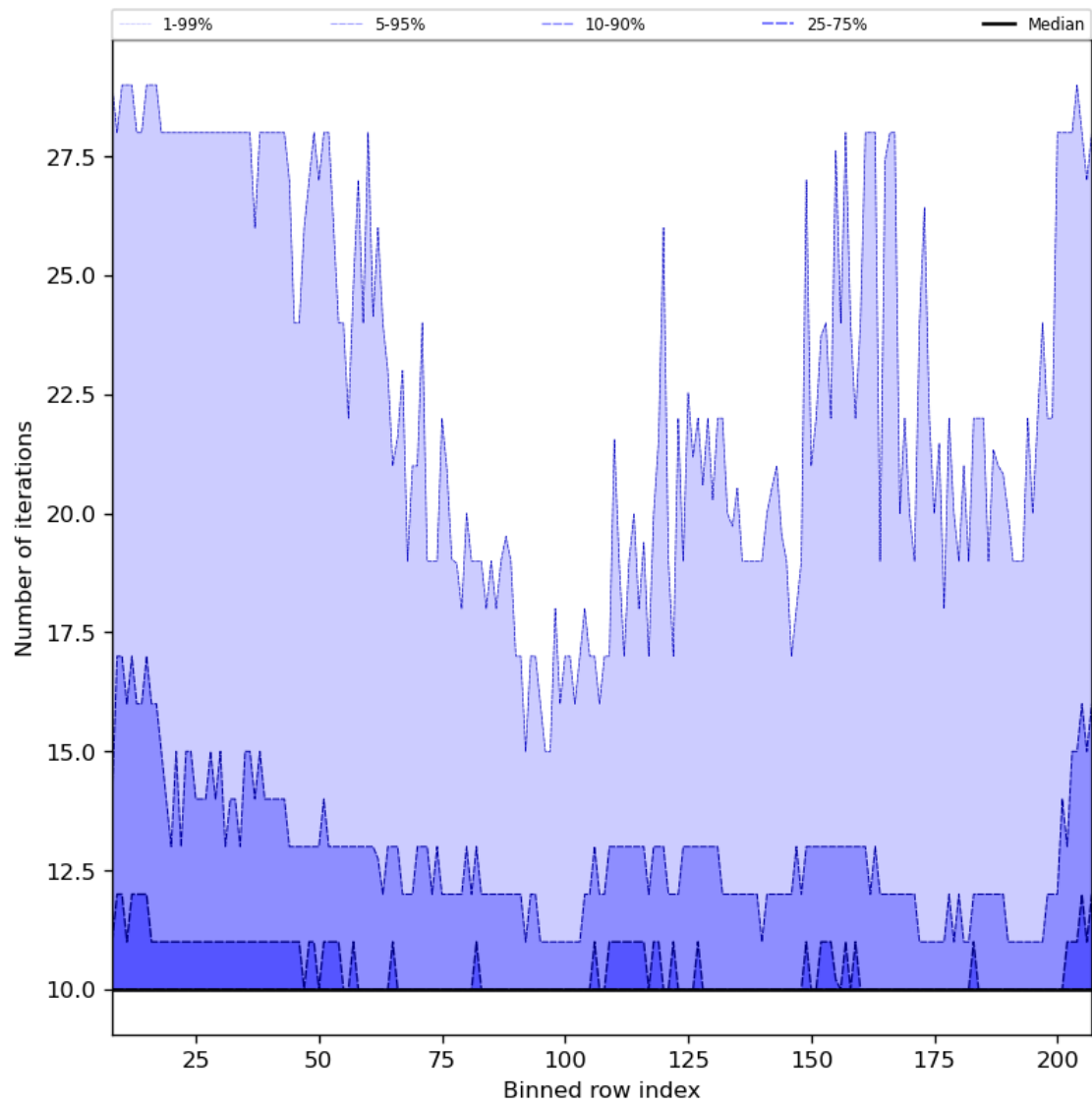
Figure 42: Along track statistics of “Number of iterations” for 2023-08-30 to 2023-08-31
