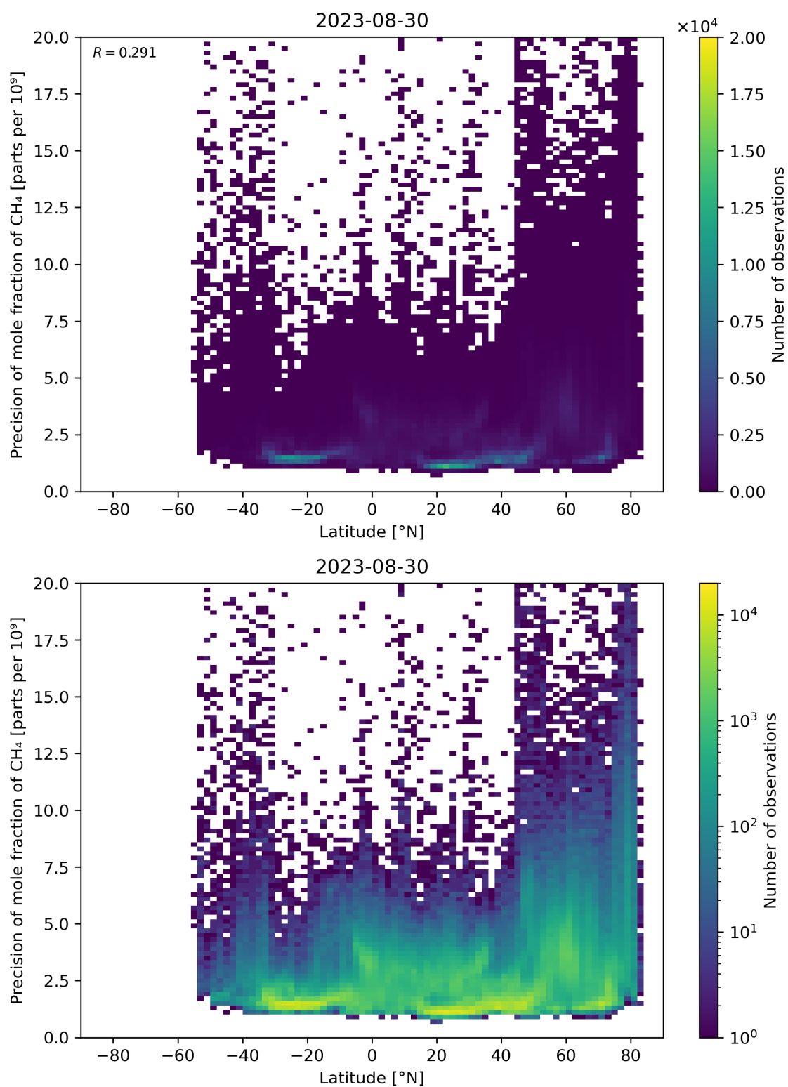
Figure 59: Scatter density plot of “Latitude” against “Precision of mole fraction of \text{CH}_4 ” for 2023-08-30 to 2023-08-31.
