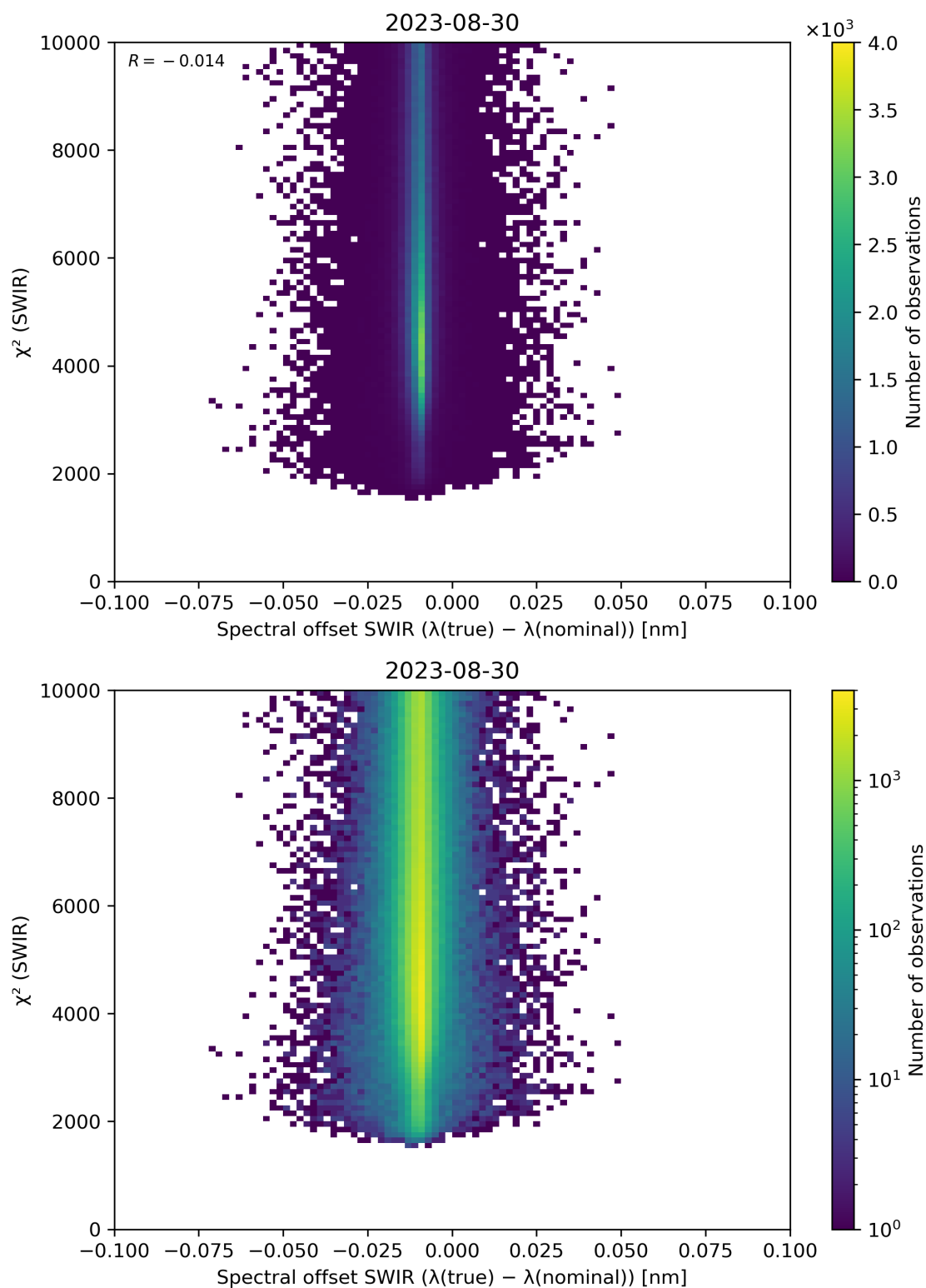
Figure 118: Scatter density plot of “Spectral offset SWIR ( \lambda(\text{true}) - \lambda(\text{nominal}) )” against “ \chi^2 (SWIR)” for 2023-08-30 to 2023-08-31.
