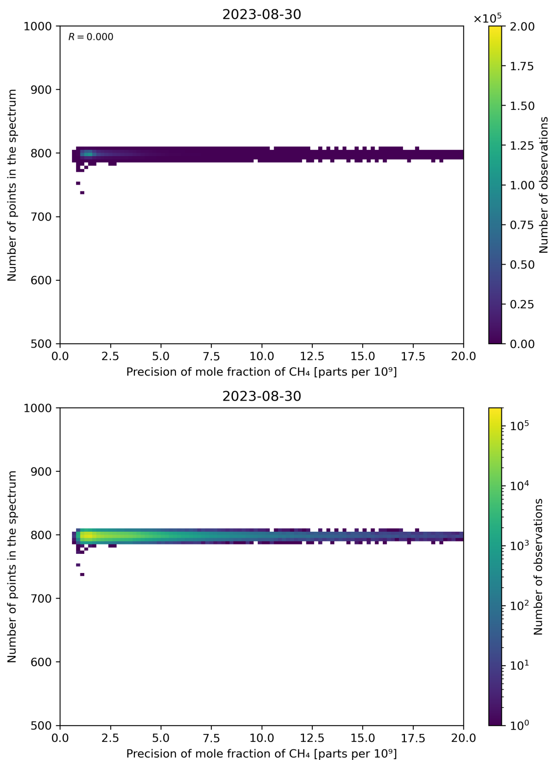
Figure 84: Scatter density plot of “Precision of mole fraction of CH 4 ” against “Number of points in the spectrum” for 2023-08-30 to 2023-08-31.
