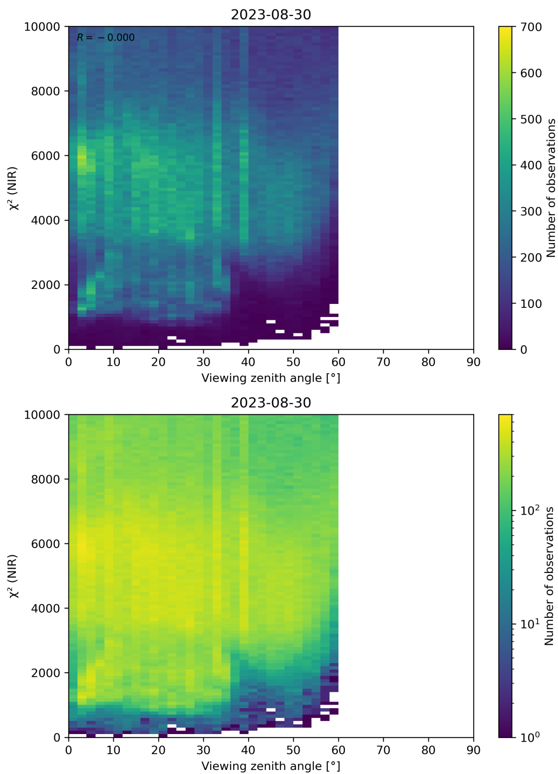
Figure 105: Scatter density plot of “Viewing zenith angle” against “ \chi^2 (NIR)” for 2023-08-30 to 2023-08-31.
