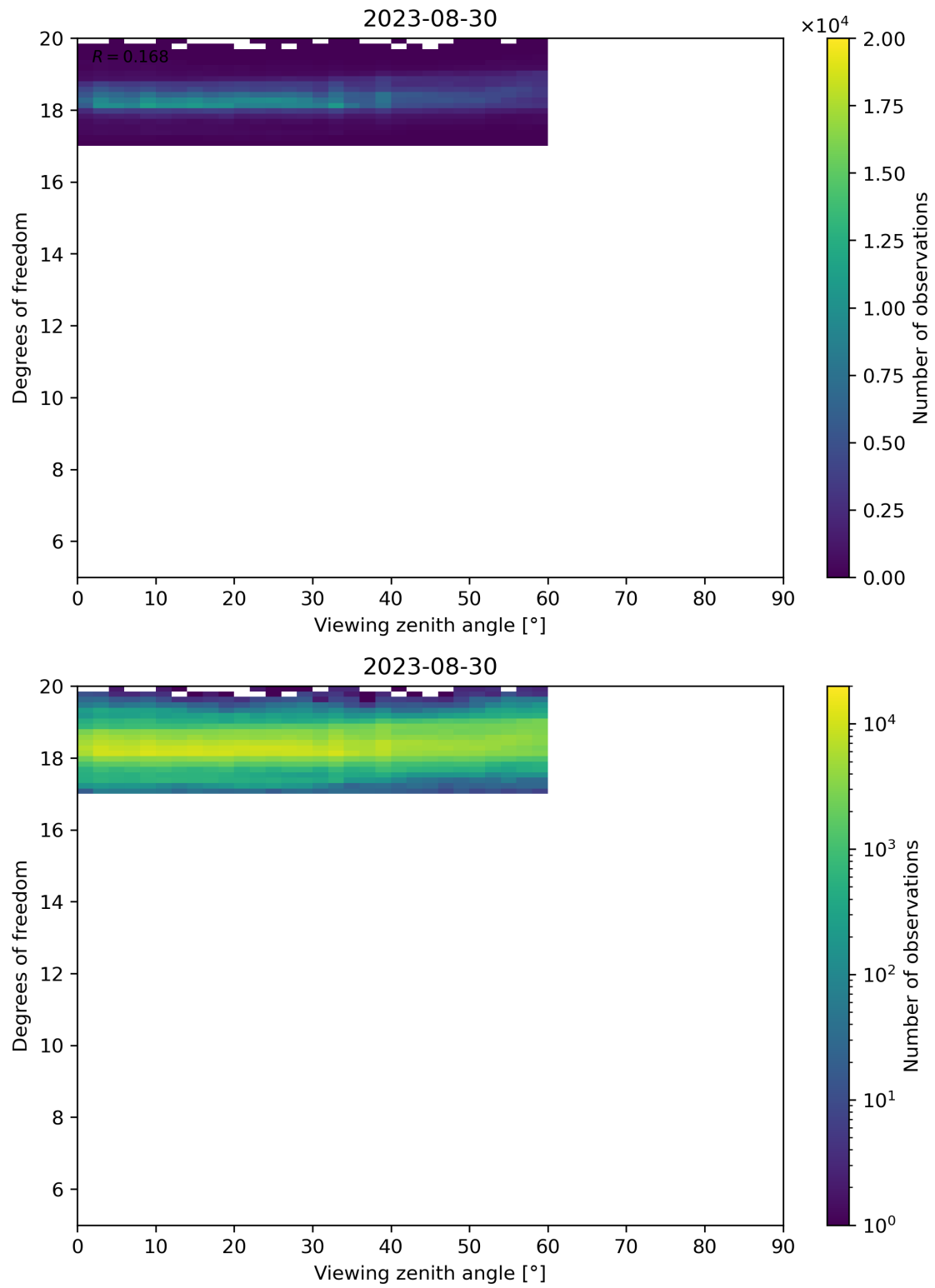
Figure 107: Scatter density plot of “Viewing zenith angle” against “Degrees of freedom” for 2023-08-30 to 2023-08-31.
