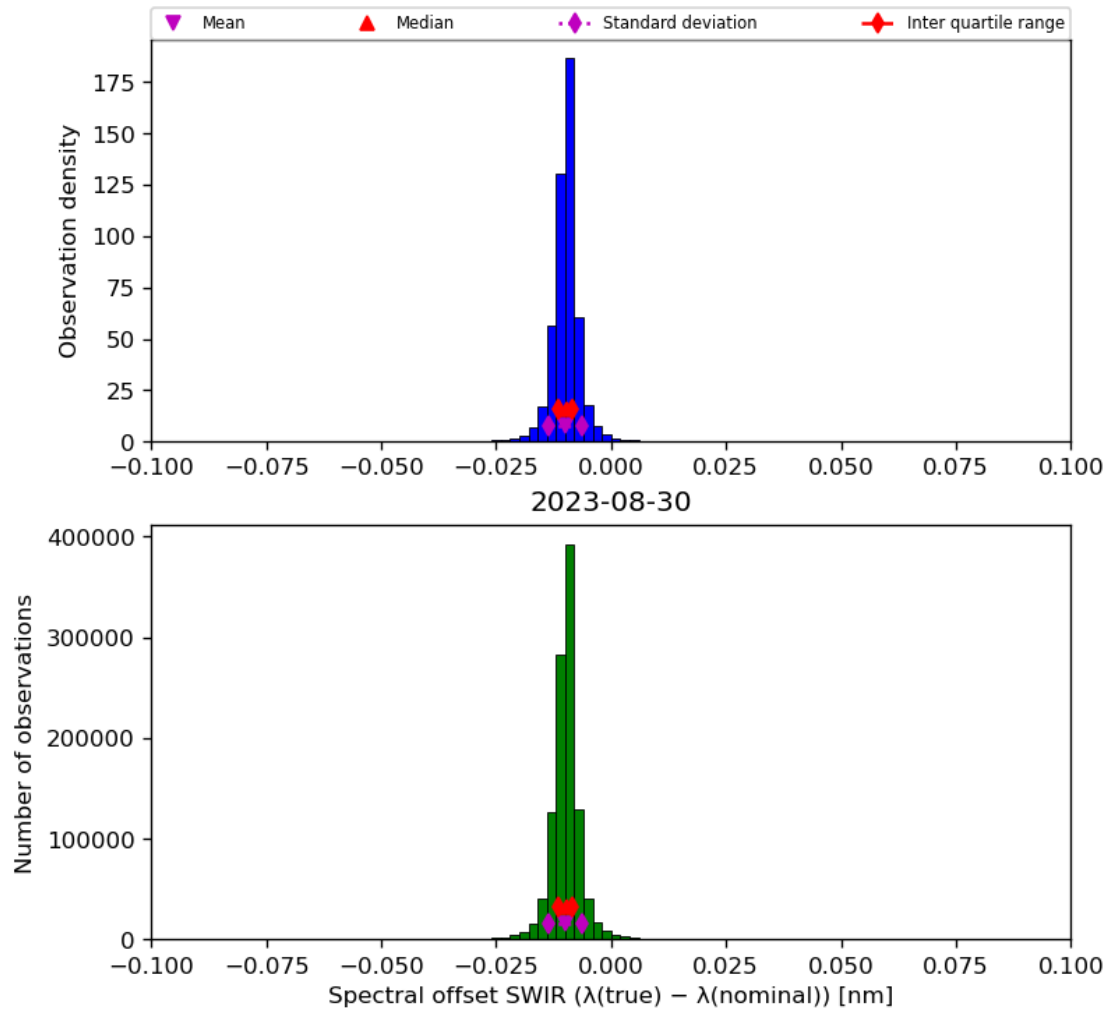
Figure 27: Histogram of “Spectral offset SWIR ( \lambda(\text{true}) - \lambda(\text{nominal}) )” for 2023-08-30 to 2023-08-31
