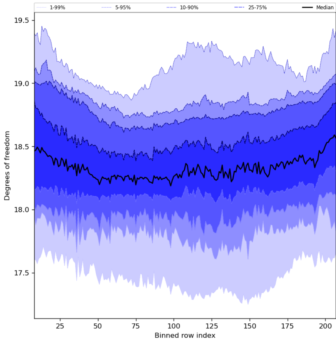
Figure 41: Along track statistics of “Degrees of freedom” for 2023-08-30 to 2023-08-31
