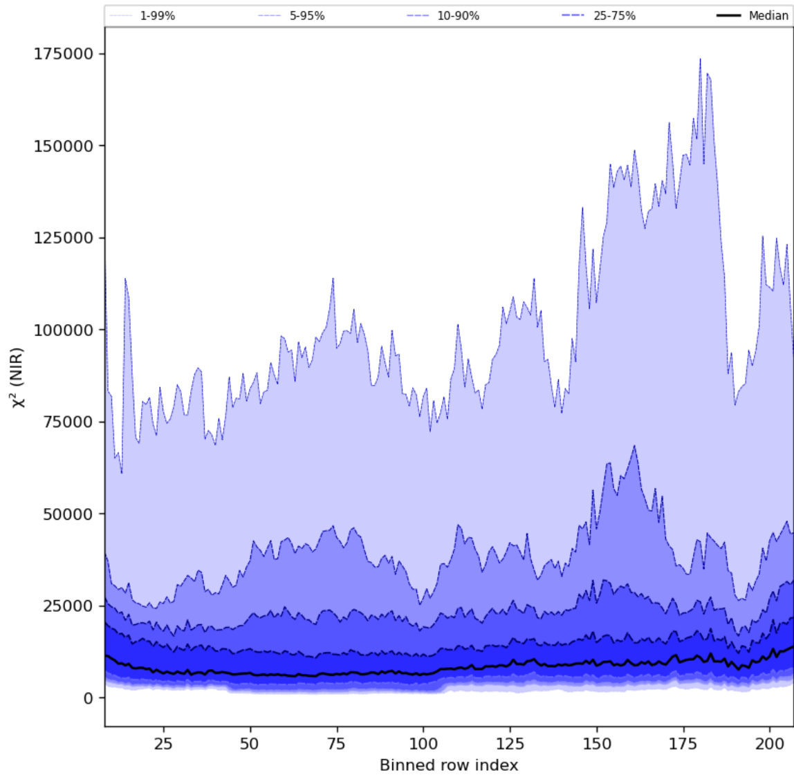
Figure 40: Along track statistics of “ \chi^2 (NIR)” for 2023-08-30 to 2023-08-31
