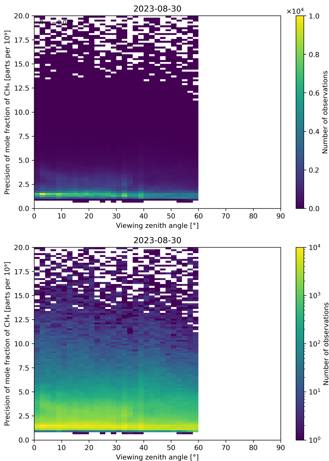
Figure 112: Scatter density plot of “Viewing zenith angle” against “Precision of mole fraction of CH 4 ” for 2023-08-30 to 2023-08-31.
