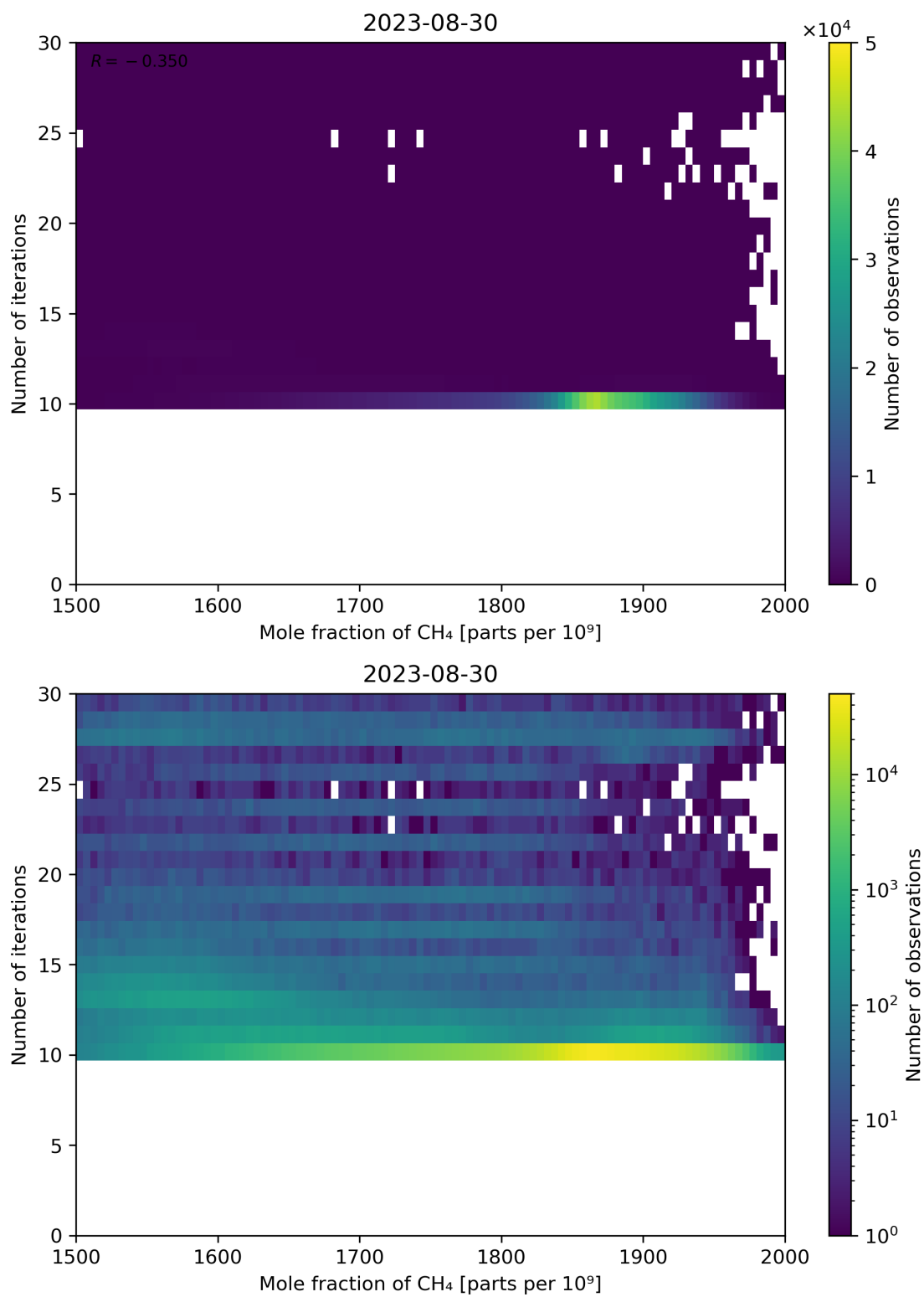
Figure 76: Scatter density plot of “Mole fraction of CH 4 ” against “Number of iterations” for 2023-08-30 to 2023-08-31.
