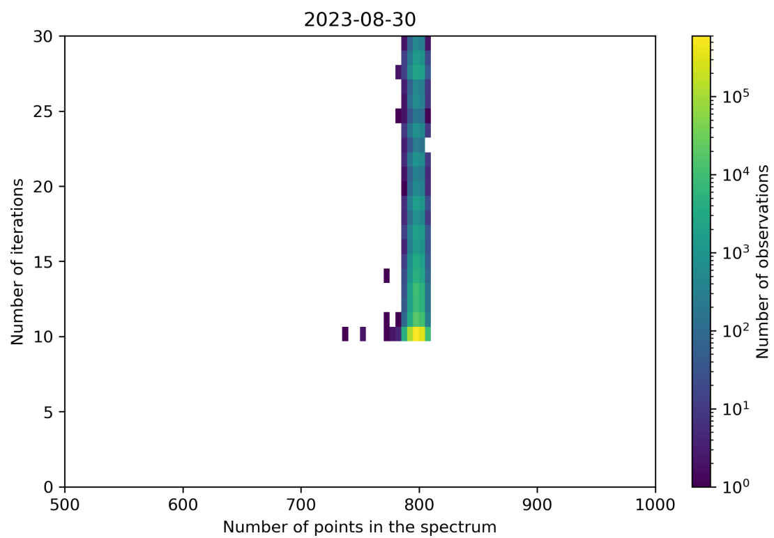
Figure 92: Scatter density plot of “Number of points in the spectrum” against “Number of iterations” for 2023-08-30 to 2023-08-31.
