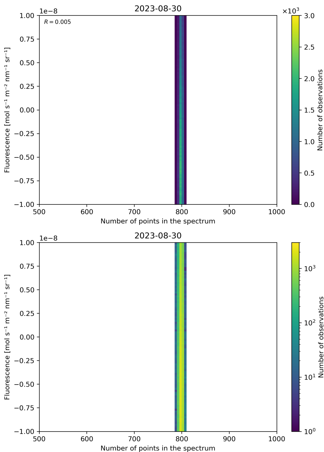
Figure 91: Scatter density plot of “Number of points in the spectrum” against “Fluorescence” for 2023-08-30 to 2023-08-31.
