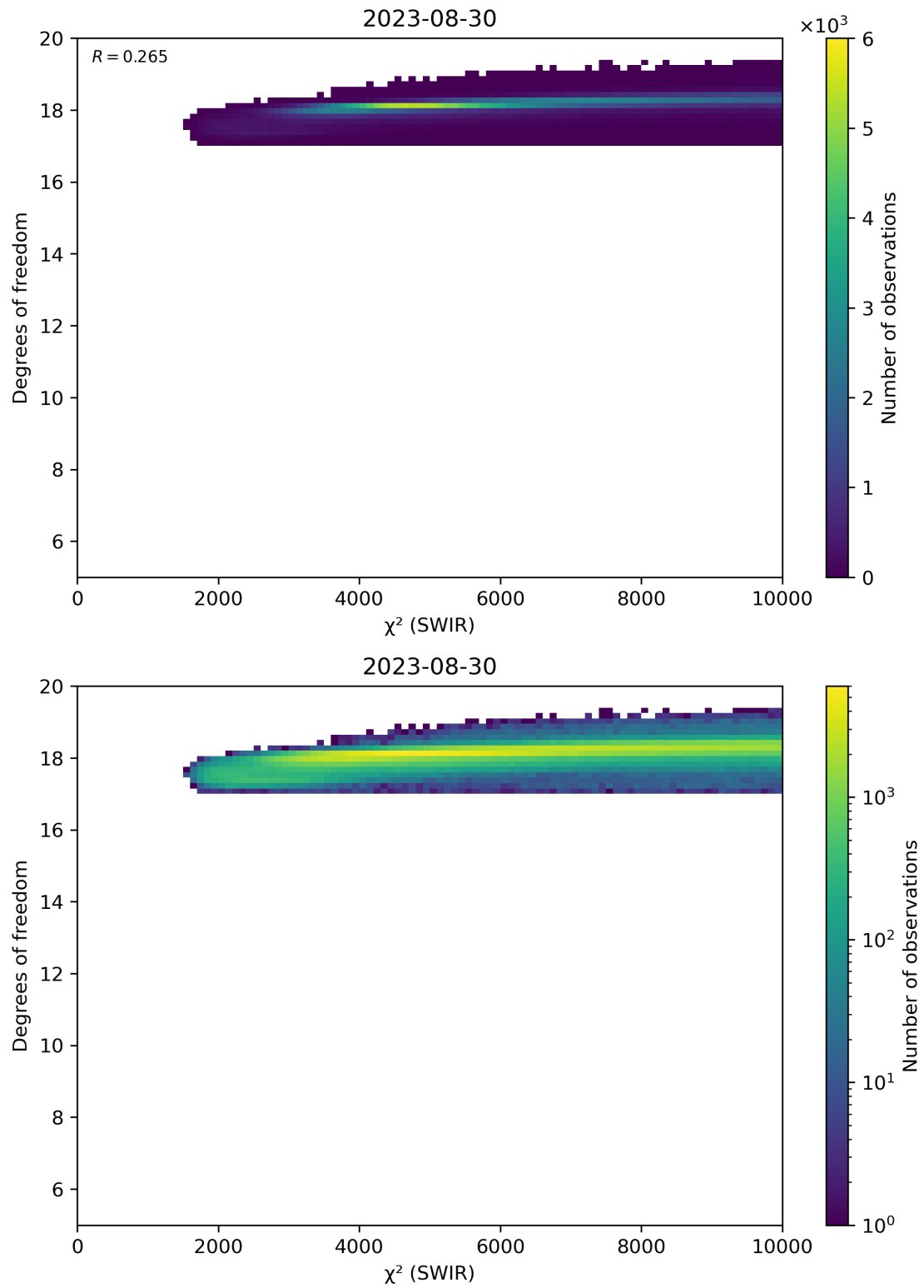
Figure 48: Scatter density plot of “ \chi^2 (SWIR)” against “Degrees of freedom” for 2023-08-30 to 2023-08-31.
