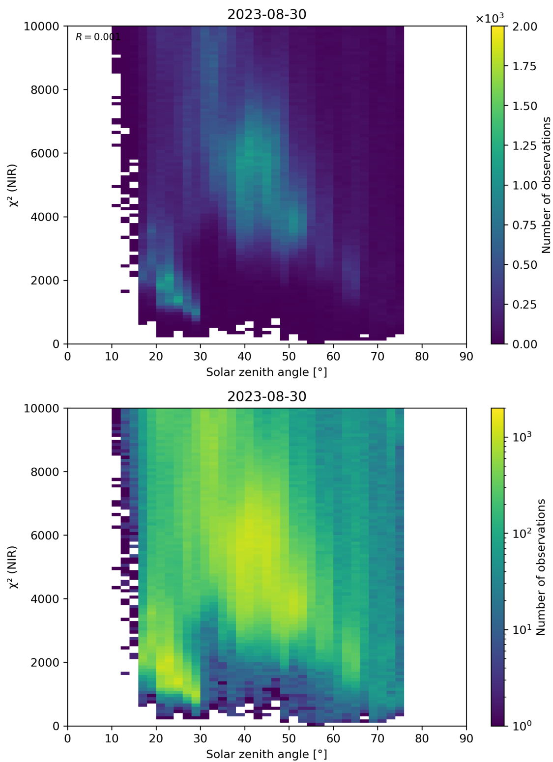
Figure 94: Scatter density plot of “Solar zenith angle” against “ \chi^2 (NIR)” for 2023-08-30 to 2023-08-31.
