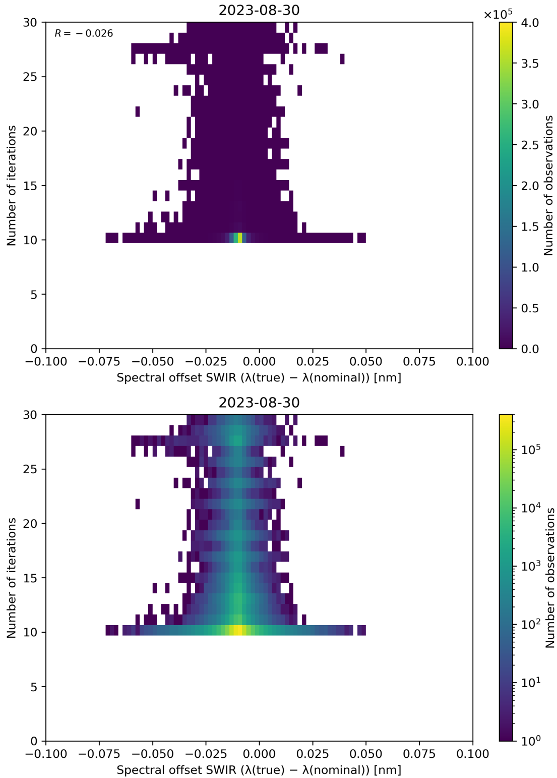
Figure 121: Scatter density plot of “Spectral offset SWIR ( \lambda(\text{true}) - \lambda(\text{nominal}) )” against “Number of iterations” for 2023-08-30 to 2023-08-31.
