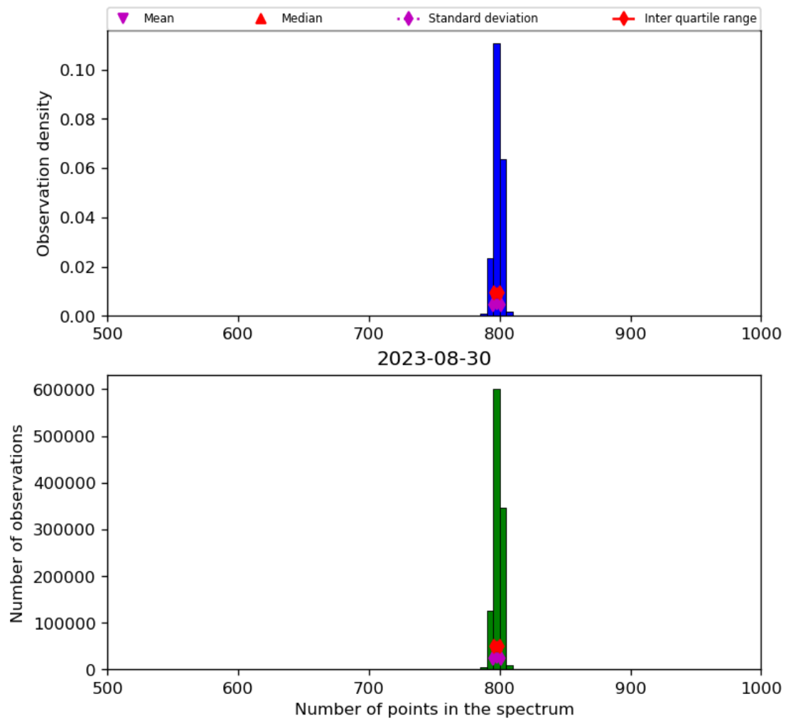
Figure 26: Histogram of “Number of points in the spectrum” for 2023-08-30 to 2023-08-31
