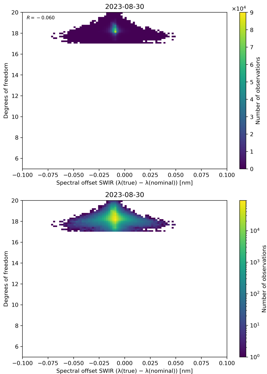
Figure 119: Scatter density plot of “Spectral offset SWIR ( \lambda(\text{true}) - \lambda(\text{nominal}) )” against “Degrees of freedom” for 2023-08-30 to 2023-08-31.
