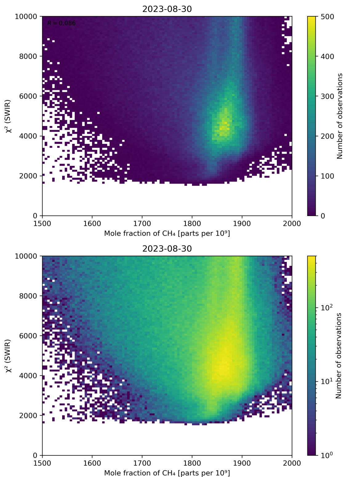
Figure 71: Scatter density plot of “Mole fraction of CH 4 ” against “ \chi^2 (SWIR)” for 2023-08-30 to 2023-08-31.
