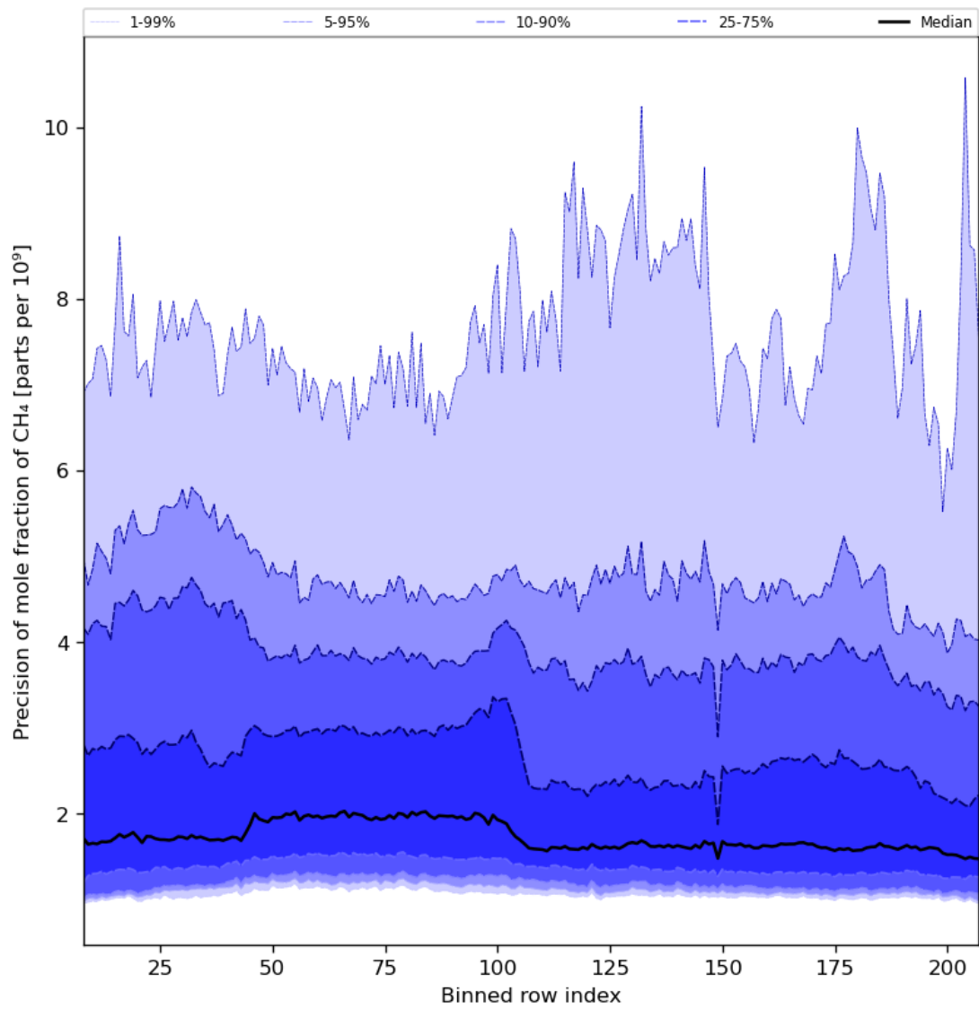
Figure 35: Along track statistics of “Precision of mole fraction of CH 4 ” for 2023-08-30 to 2023-08-31
