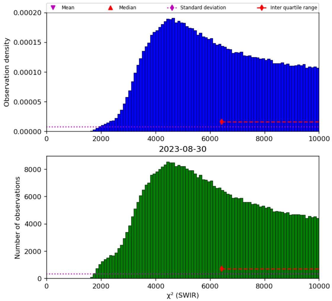
Figure 28: Histogram of " \chi^2 (SWIR)" for 2023-08-30 to 2023-08-31
