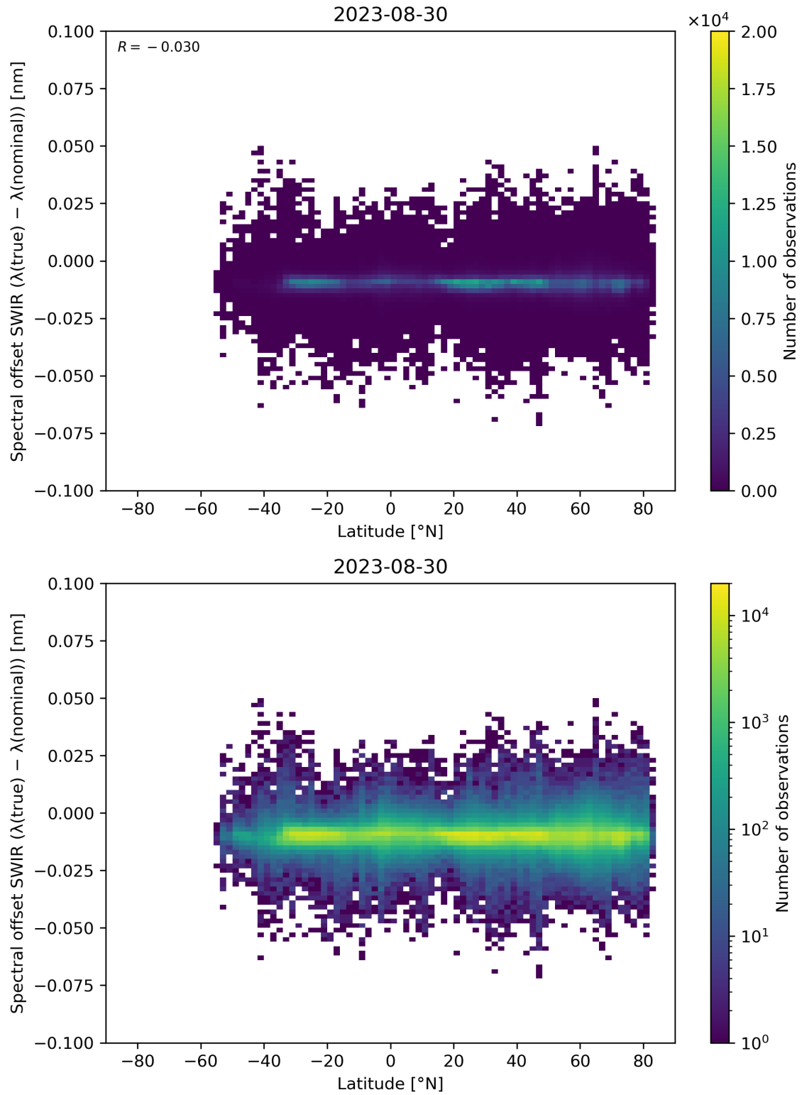
Figure 62: Scatter density plot of “Latitude” against “Spectral offset SWIR ( \lambda(\text{true}) - \lambda(\text{nominal}) )” for 2023-08-30 to 2023-08-31.
