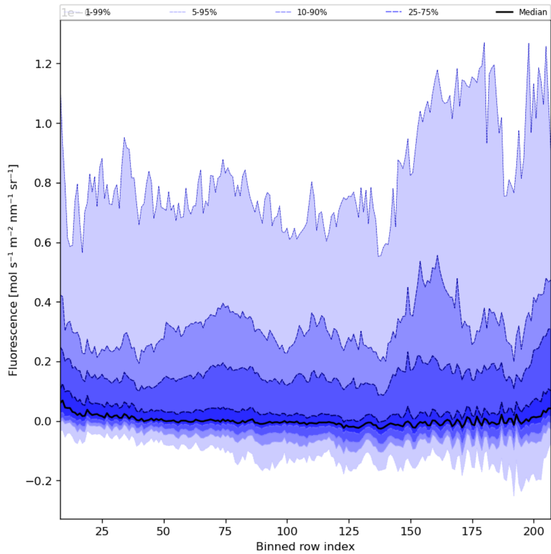
Figure 43: Along track statistics of “Fluorescence” for 2023-08-30 to 2023-08-31
