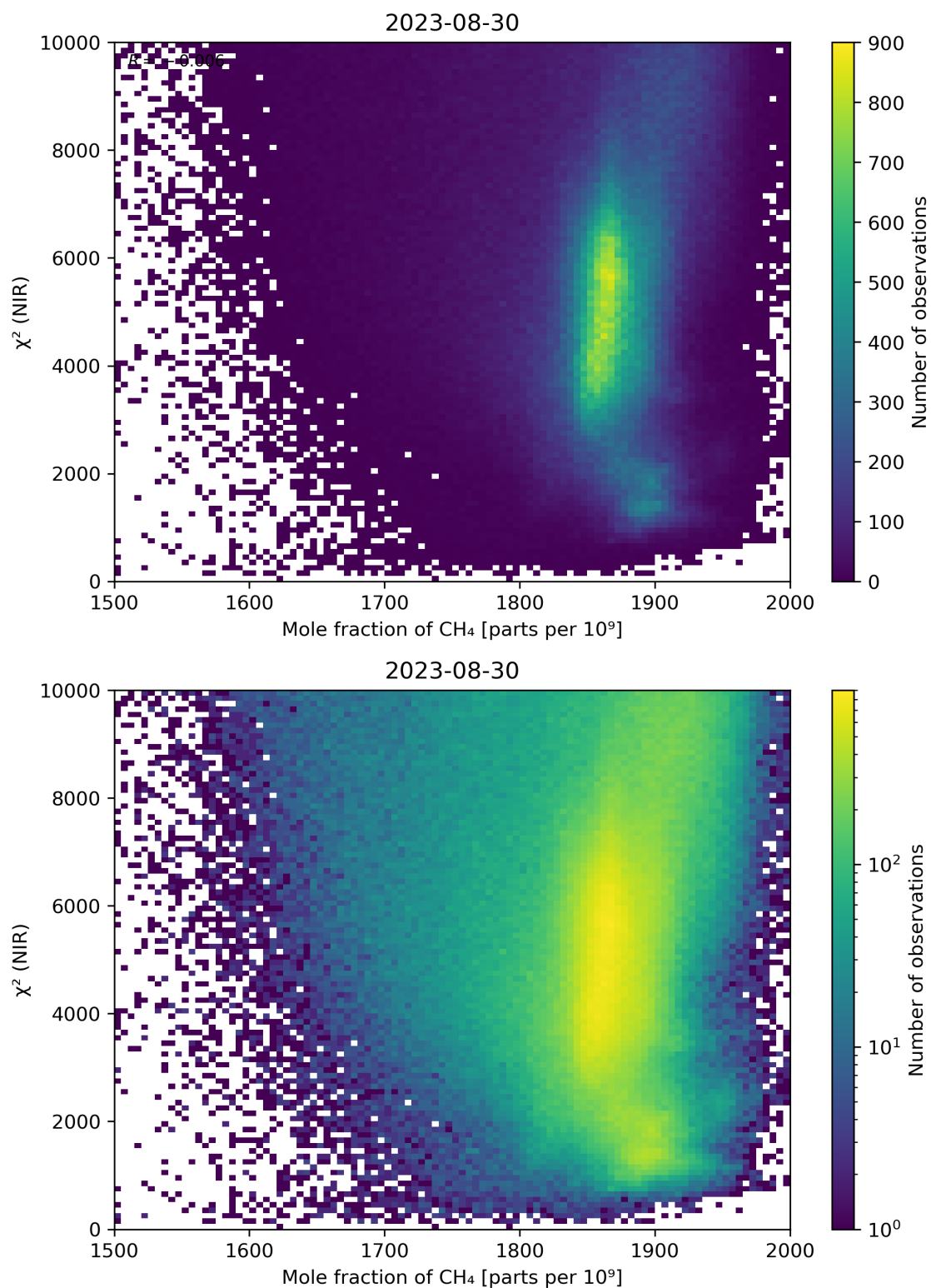
Figure 70: Scatter density plot of “Mole fraction of CH 4 ” against “ \chi^2 (NIR)” for 2023-08-30 to 2023-08-31.
