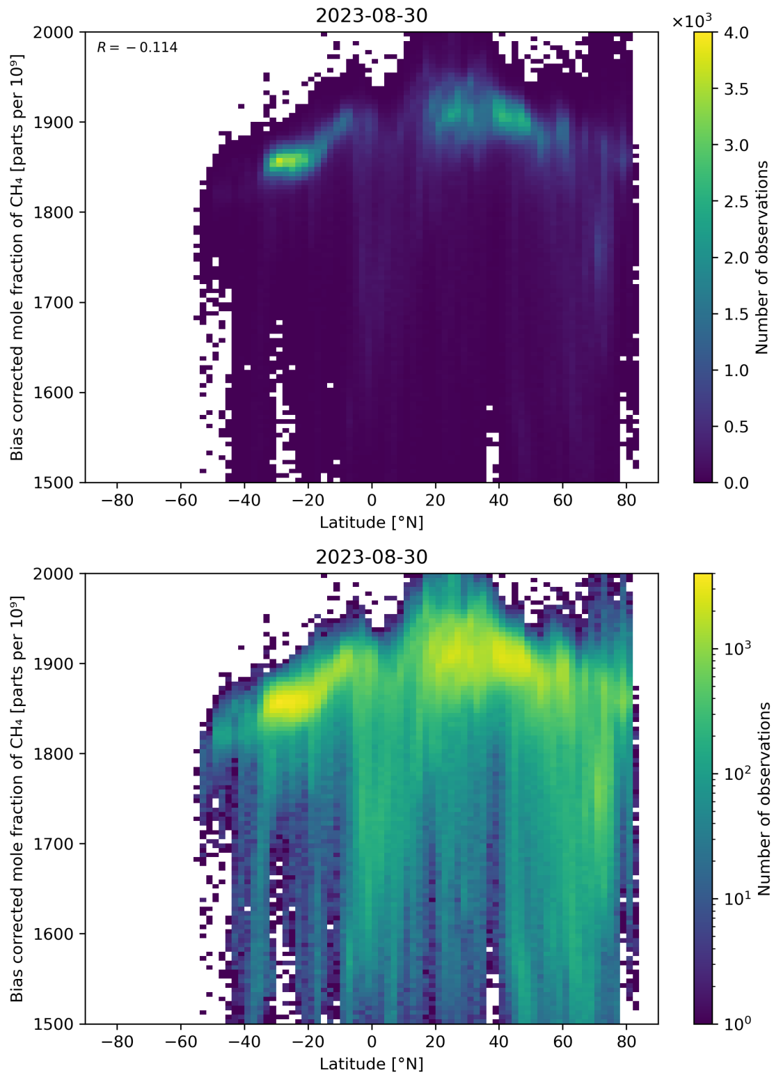
Figure 58: Scatter density plot of “Latitude” against “Bias corrected mole fraction of CH 4 ” for 2023-08-30 to 2023-08-31.
