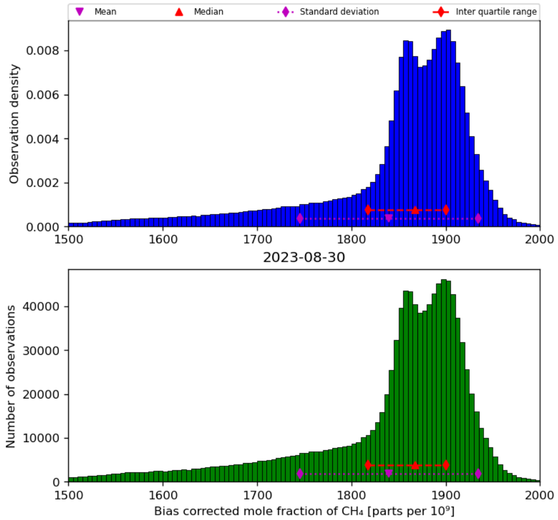
Figure 25: Histogram of “Bias corrected mole fraction of CH 4 ” for 2023-08-30 to 2023-08-31
