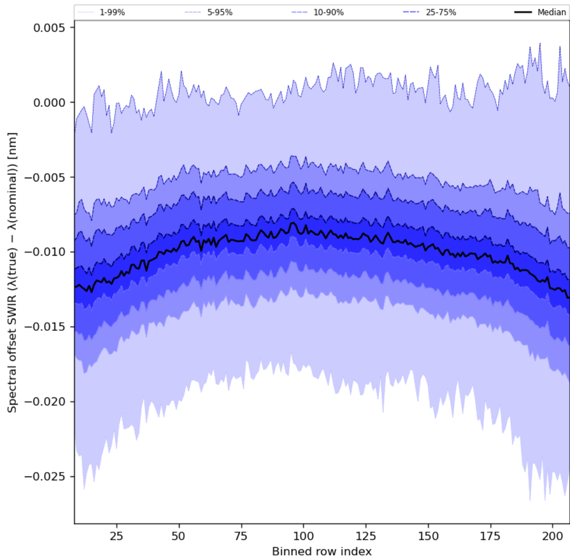
Figure 38: Along track statistics of “Spectral offset SWIR ( \lambda(\text{true}) - \lambda(\text{nominal}) )” for 2023-08-30 to 2023-08-31
