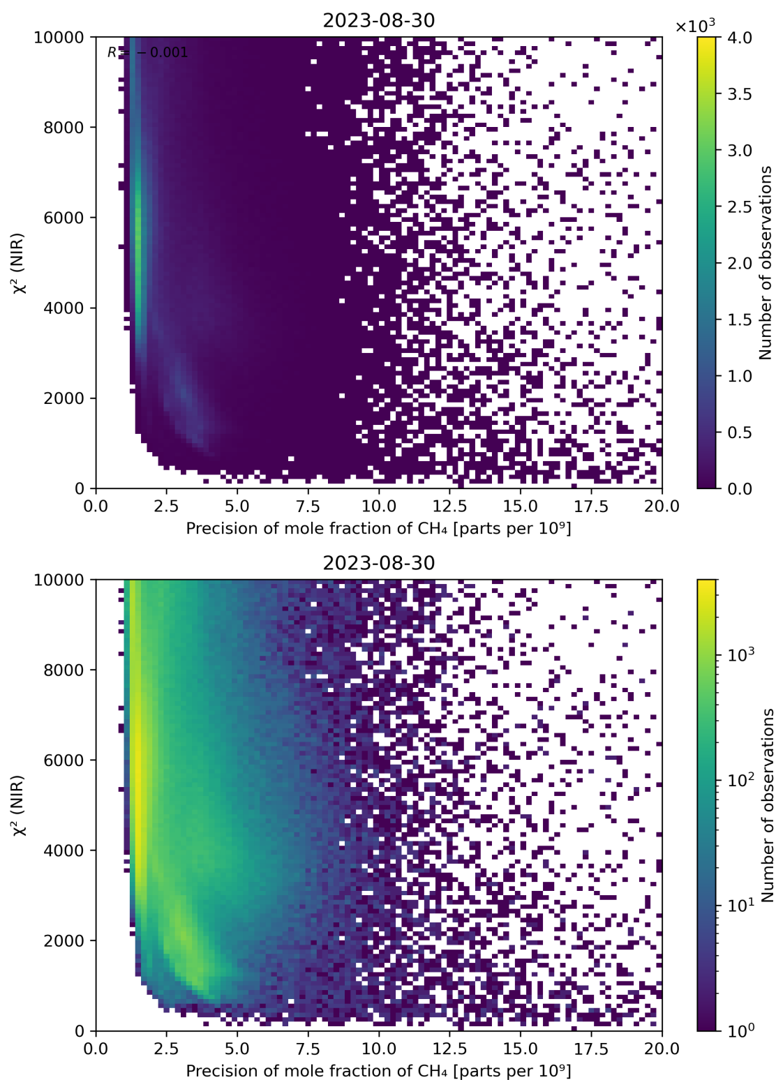
Figure 78: Scatter density plot of “Precision of mole fraction of \text{CH}_4 ” against “ \chi^2 (NIR)” for 2023-08-30 to 2023-08-31.
