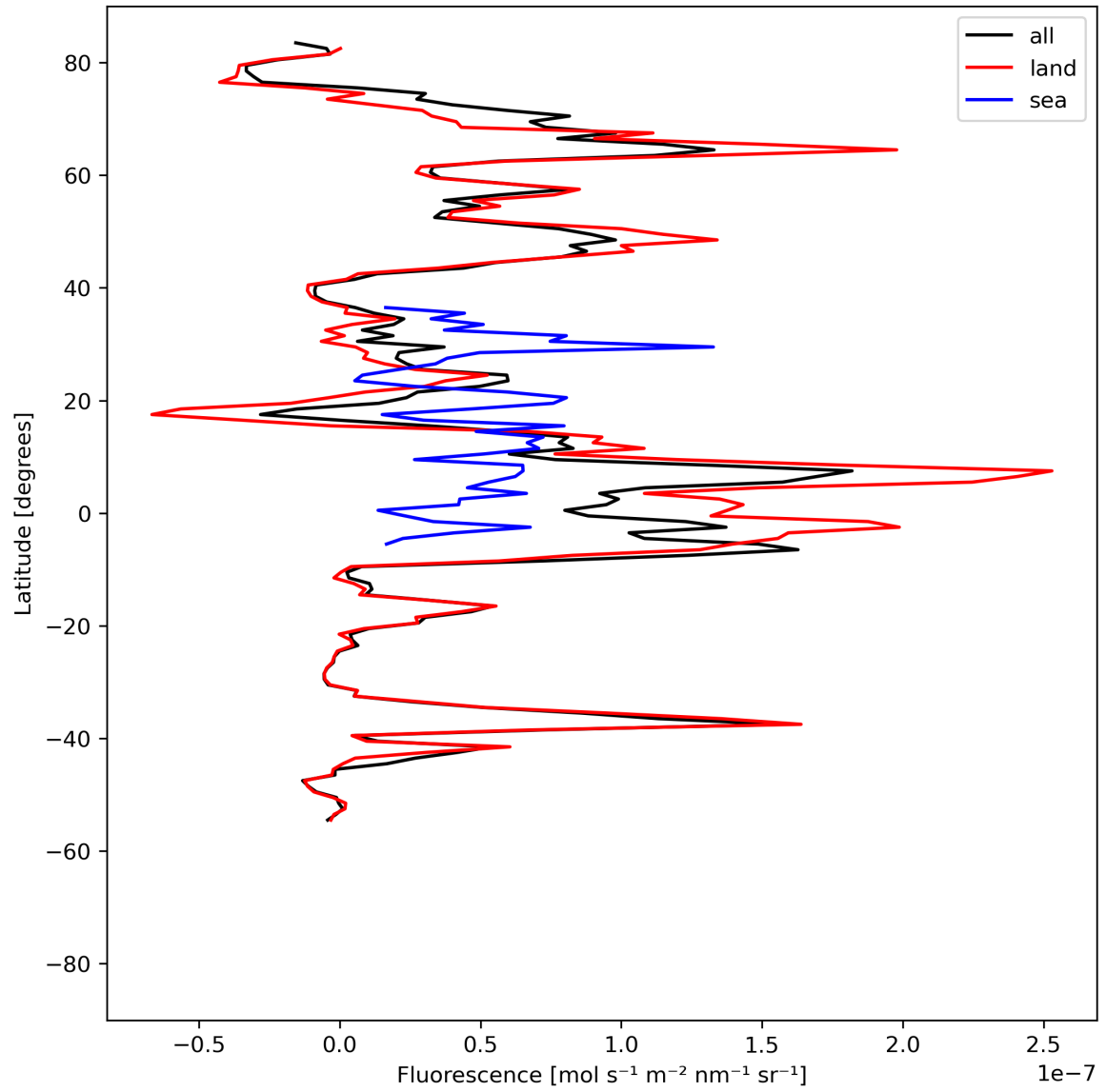
Figure 21: Zonal average of “Fluorescence” for 2023-08-30 to 2023-08-31.
