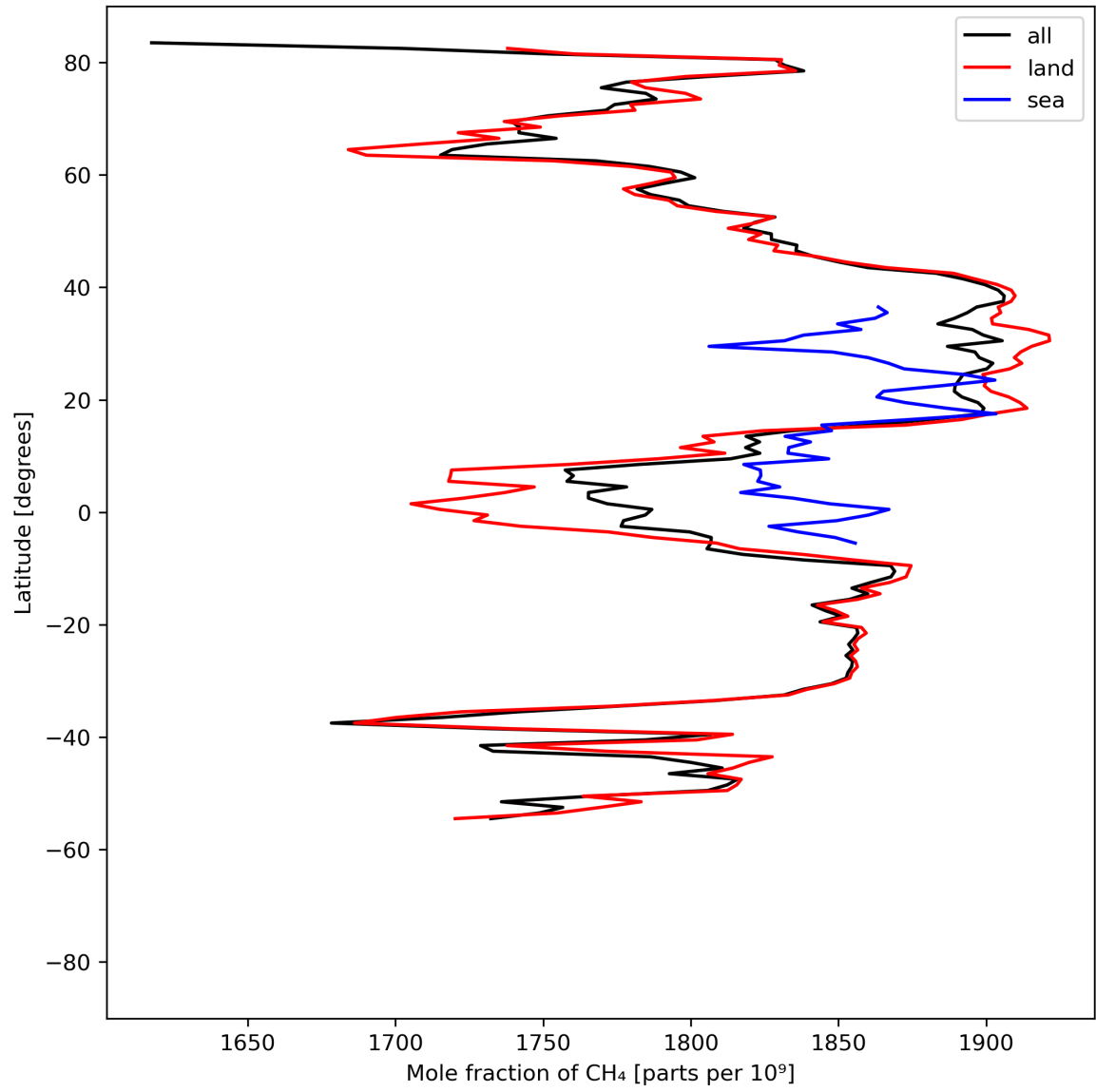
Figure 12: Zonal average of “Mole fraction of \text{CH}_4 ” for 2023-08-30 to 2023-08-31.
