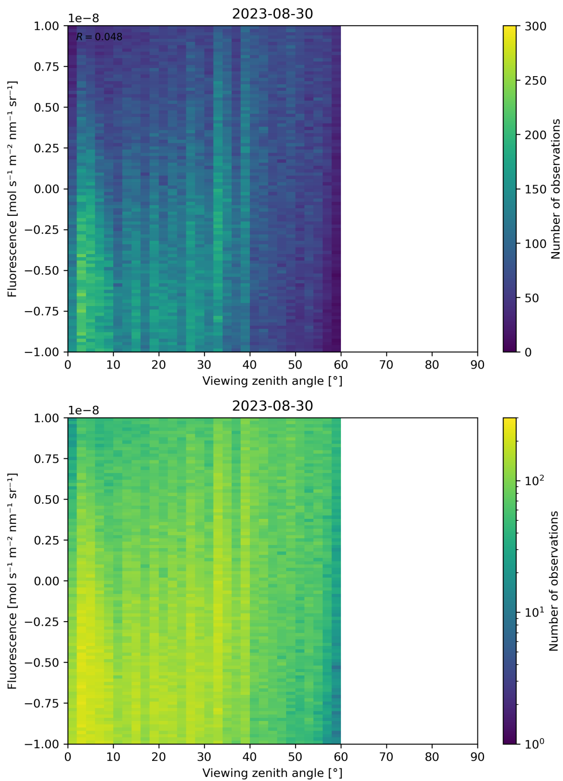
Figure 108: Scatter density plot of “Viewing zenith angle” against “Fluorescence” for 2023-08-30 to 2023-08-31.
