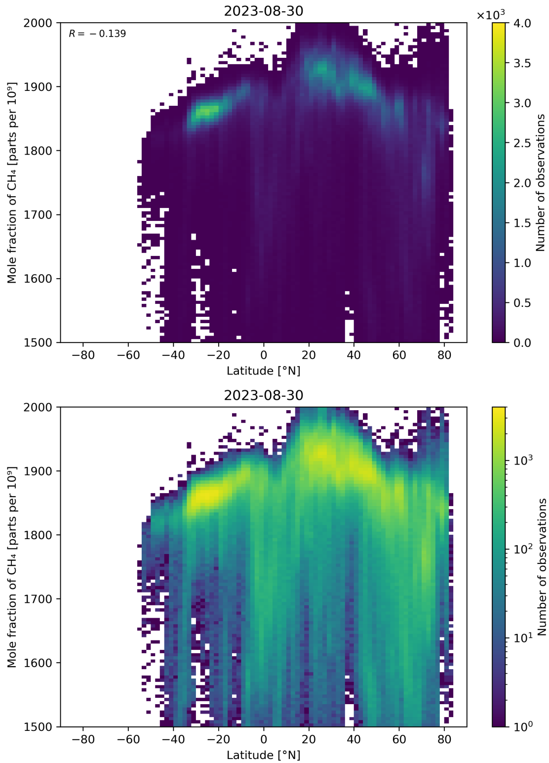
Figure 57: Scatter density plot of “Latitude” against “Mole fraction of CH 4 ” for 2023-08-30 to 2023-08-31.
