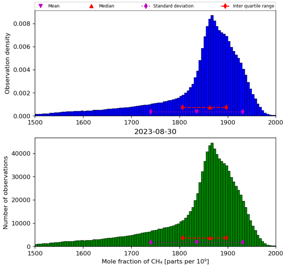
Figure 23: Histogram of “Mole fraction of CH 4 ” for 2023-08-30 to 2023-08-31
