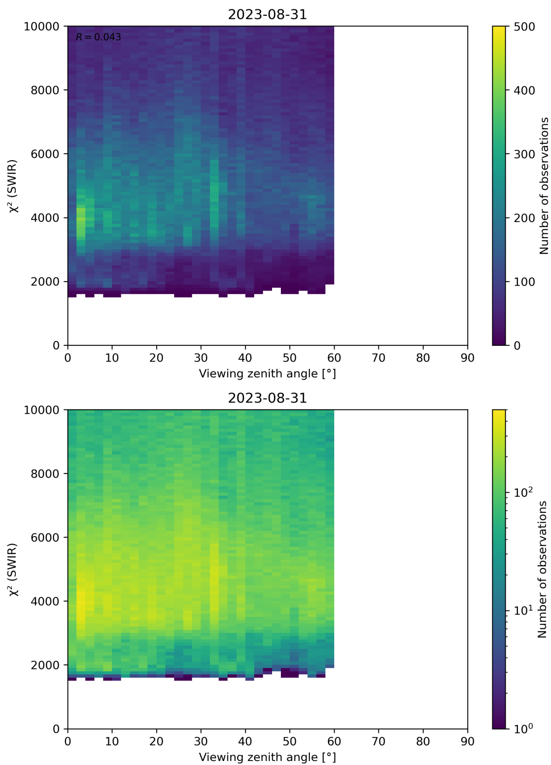
Figure 106: Scatter density plot of “Viewing zenith angle” against “ \chi^2 (SWIR)” for 2023-08-30 to 2023-09-01.
