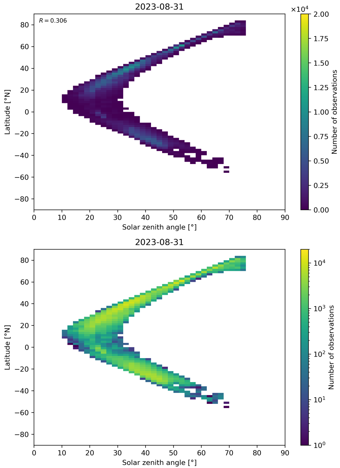
Figure 98: Scatter density plot of “Solar zenith angle” against “Latitude” for 2023-08-30 to 2023-09-01.
