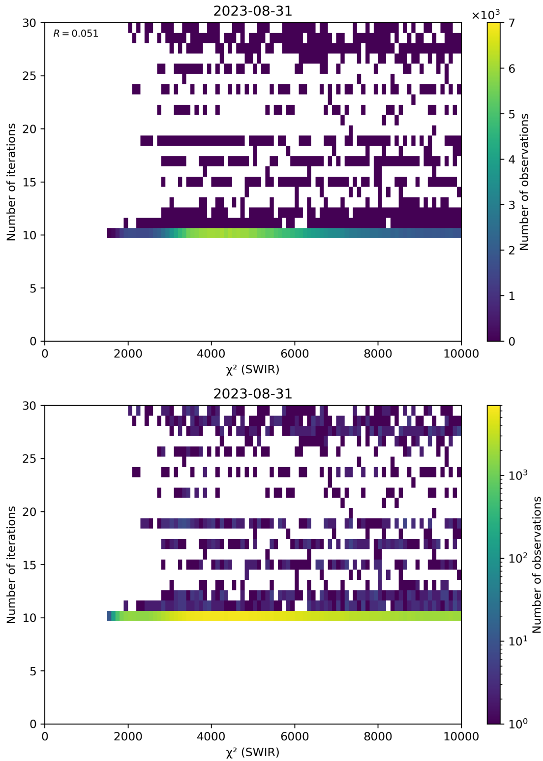
Figure 50: Scatter density plot of “ \chi^2 (SWIR)” against “Number of iterations” for 2023-08-30 to 2023-09-01.
