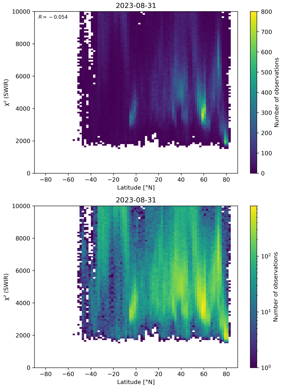
Figure 54: Scatter density plot of “Latitude” against “ \chi^2 (SWIR)” for 2023-08-30 to 2023-09-01.
