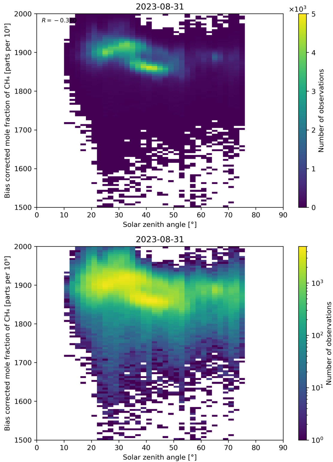
Figure 100: Scatter density plot of “Solar zenith angle” against “Bias corrected mole fraction of CH 4 ” for 2023-08-30 to 2023-09-01.
