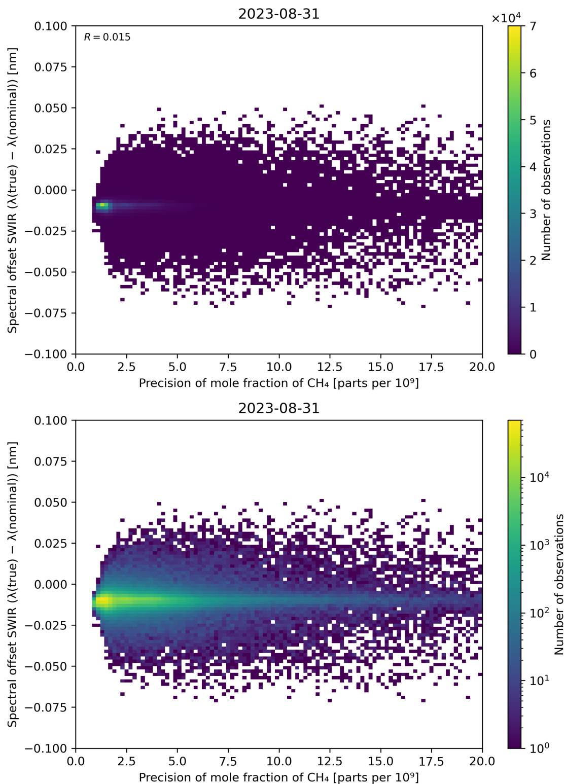
Figure 85: Scatter density plot of “Precision of mole fraction of CH 4 ” against “Spectral offset SWIR ( \lambda(\text{true}) - \lambda(\text{nominal}) )” for 2023-08-30 to 2023-09-01.
