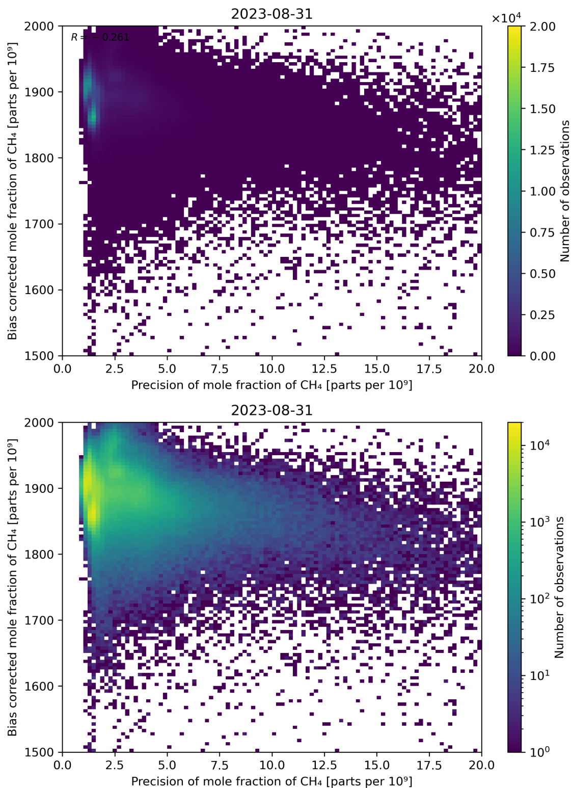
Figure 82: Scatter density plot of “Precision of mole fraction of CH 4 ” against “Bias corrected mole fraction of CH 4 ” for 2023-08-30 to 2023-09-01.
