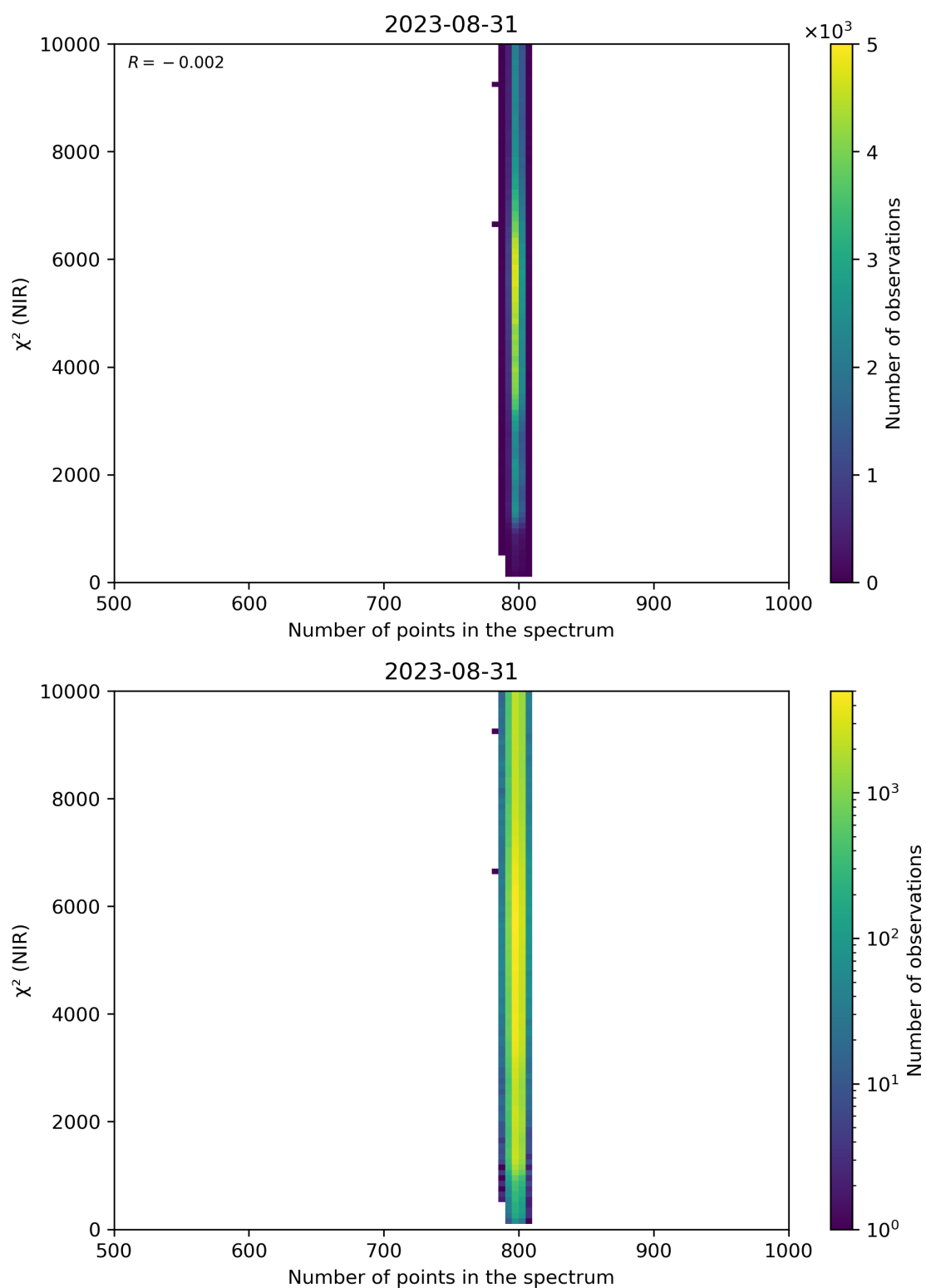
Figure 88: Scatter density plot of “Number of points in the spectrum” against “ \chi^2 (NIR)” for 2023-08-30 to 2023-09-01.
