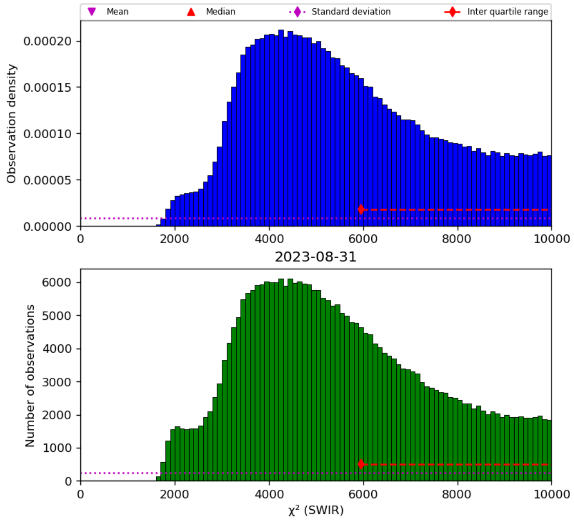
Figure 28: Histogram of " \chi^2 (SWIR)" for 2023-08-30 to 2023-09-01
