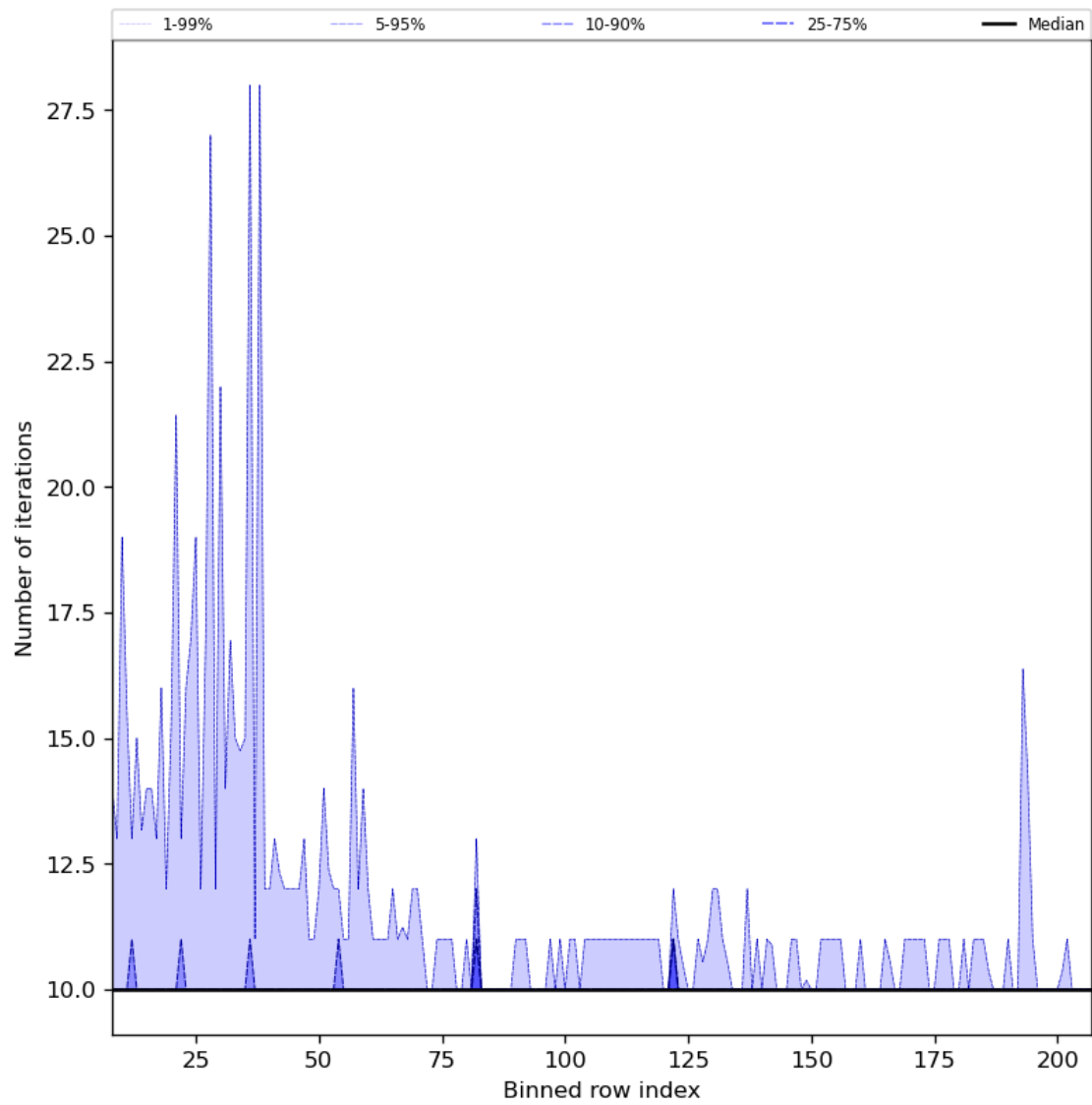
Figure 42: Along track statistics of “Number of iterations” for 2023-08-30 to 2023-09-01
