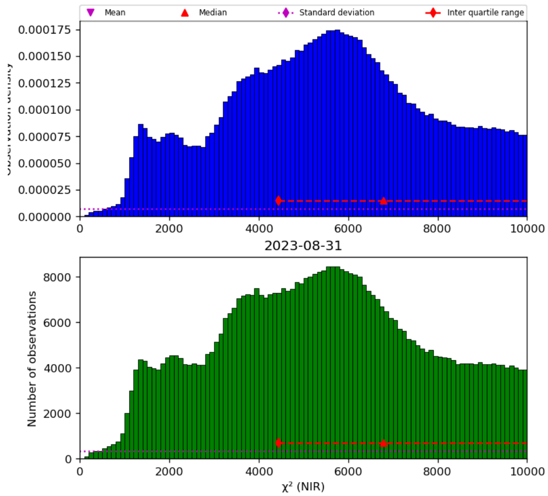
Figure 29: Histogram of “ \chi^2 (NIR)” for 2023-08-30 to 2023-09-01
