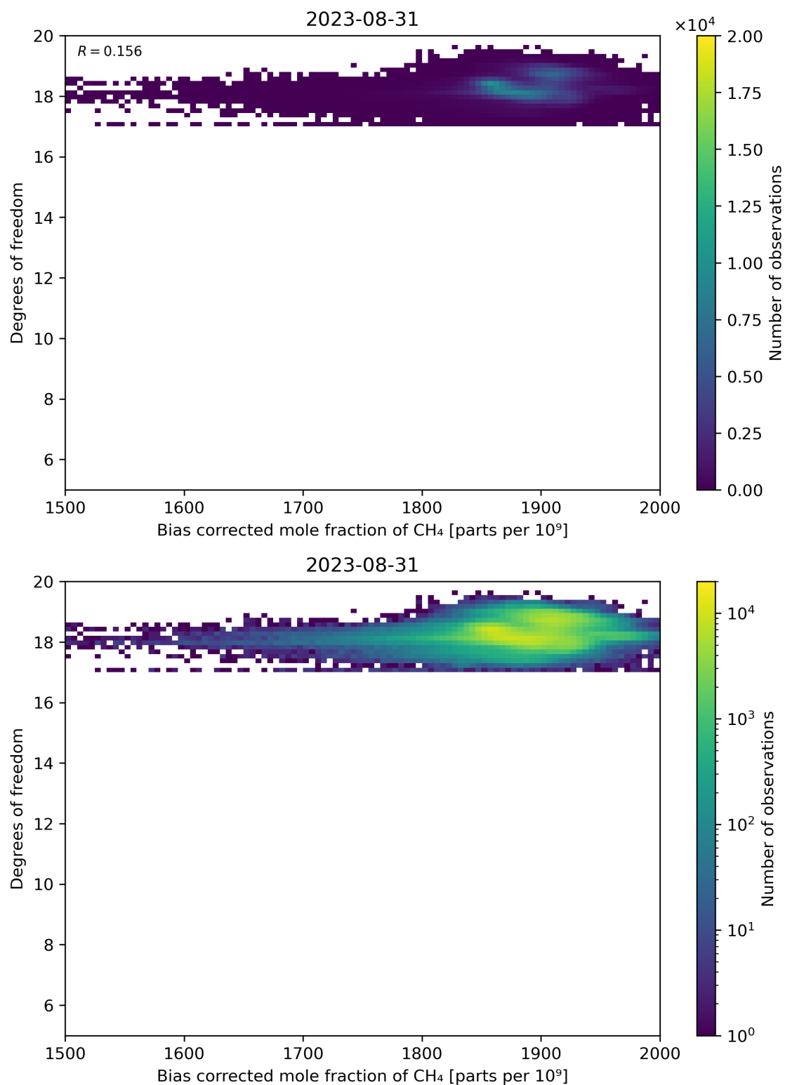
Figure 65: Scatter density plot of “Bias corrected mole fraction of CH 4 ” against “Degrees of freedom” for 2023-08-30 to 2023-09-01.
