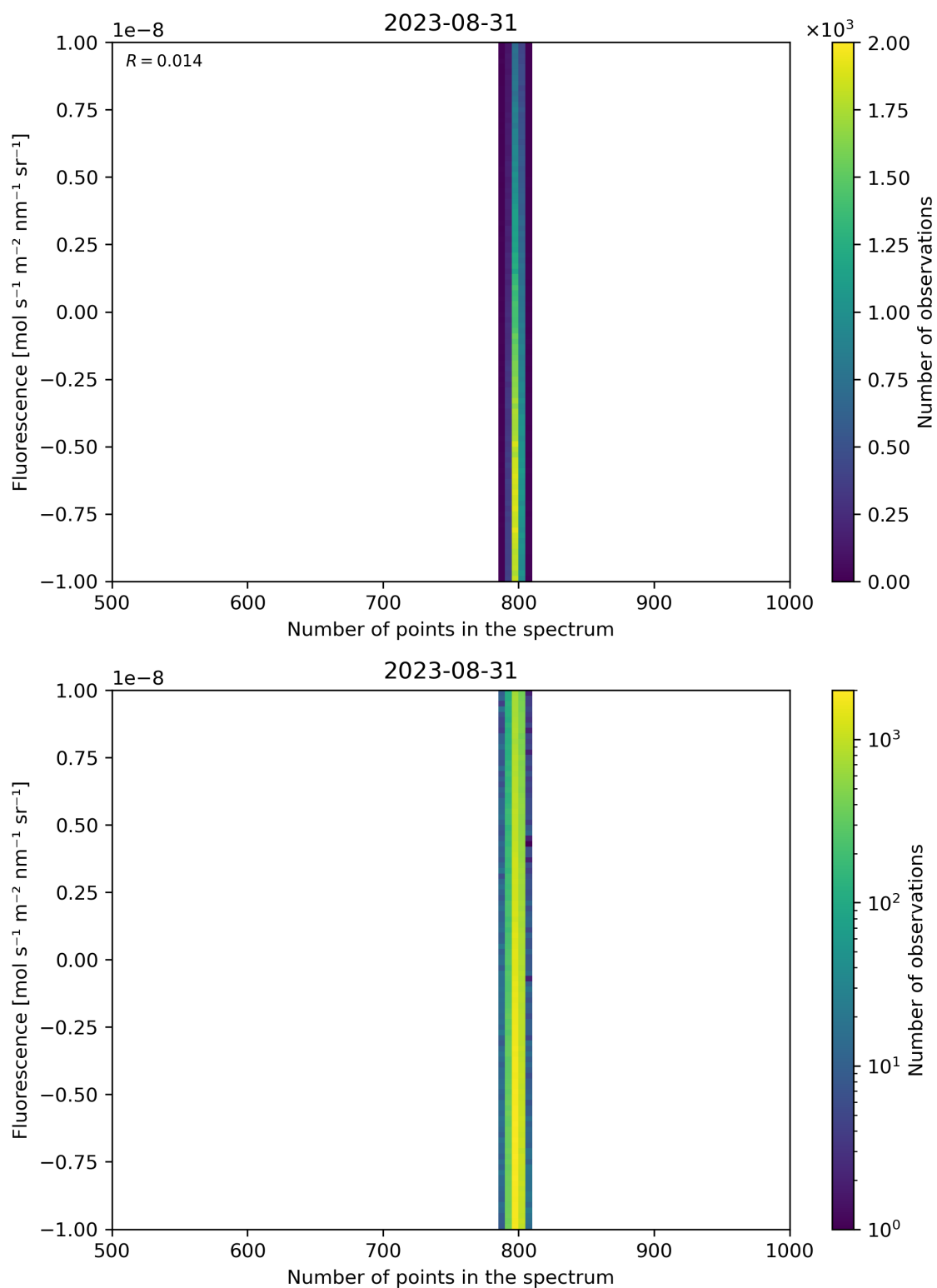
Figure 91: Scatter density plot of “Number of points in the spectrum” against “Fluorescence” for 2023-08-30 to 2023-09-01.
