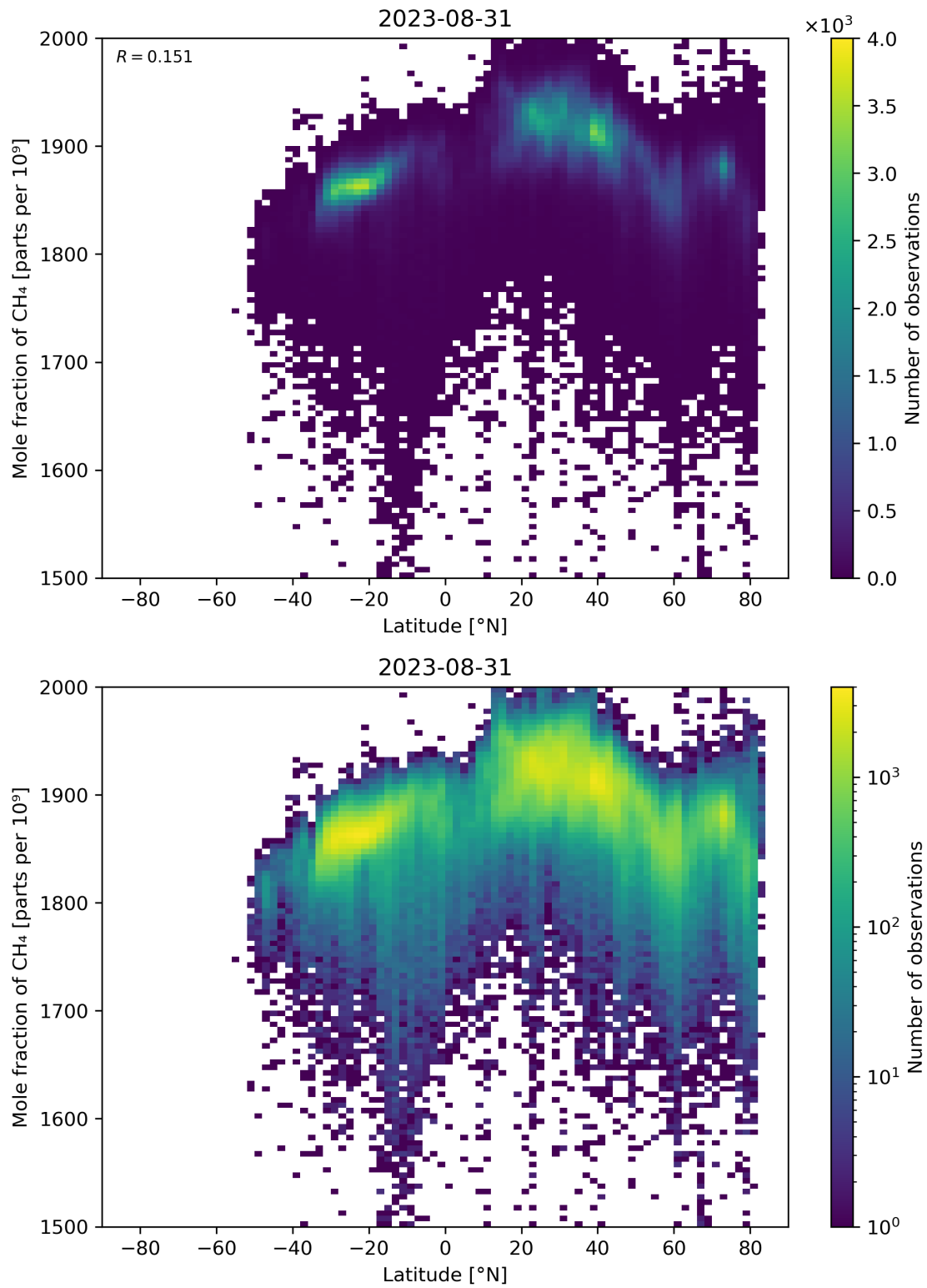
Figure 57: Scatter density plot of “Latitude” against “Mole fraction of CH 4 ” for 2023-08-30 to 2023-09-01.
