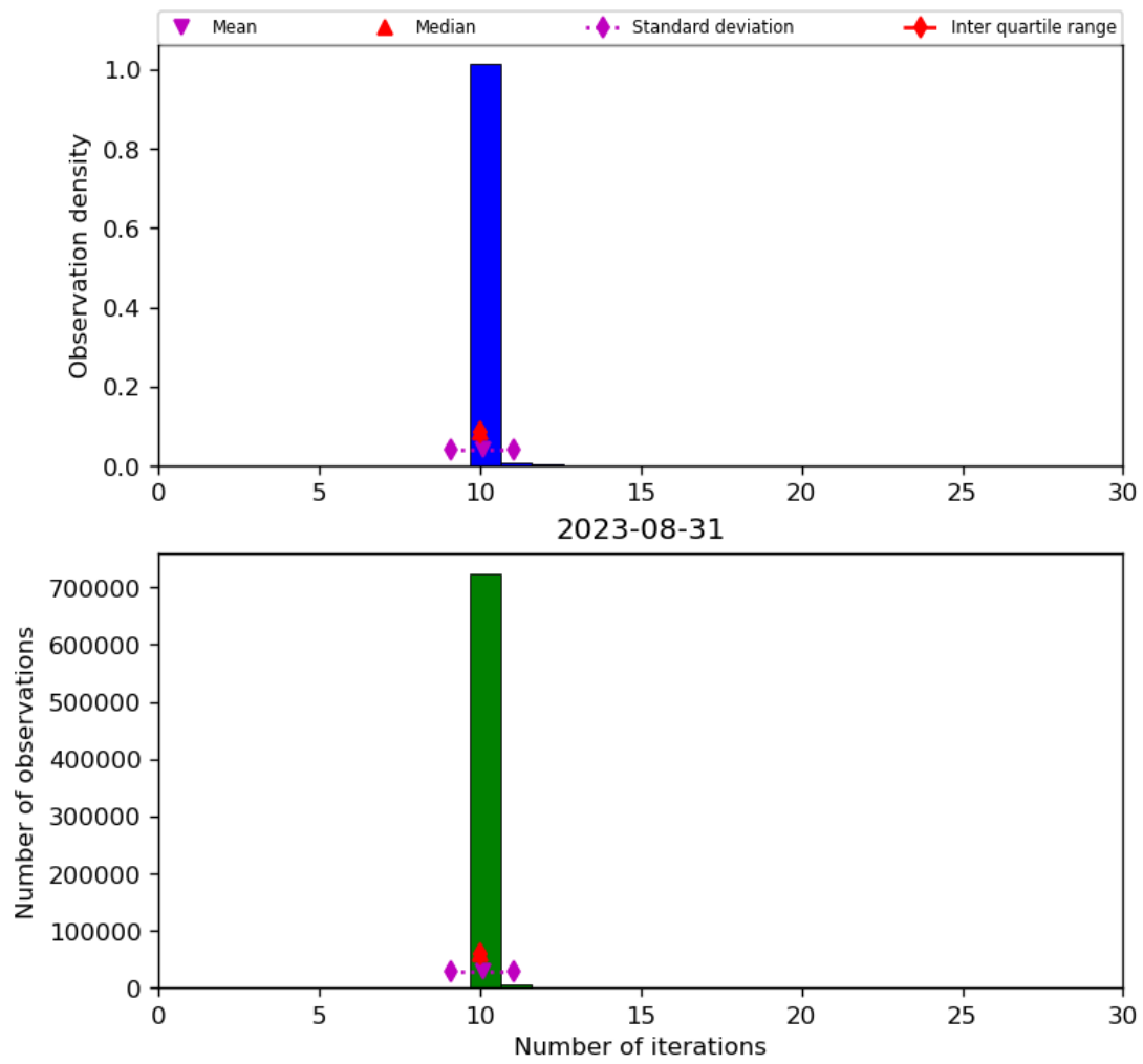
Figure 31: Histogram of “Number of iterations” for 2023-08-30 to 2023-09-01
