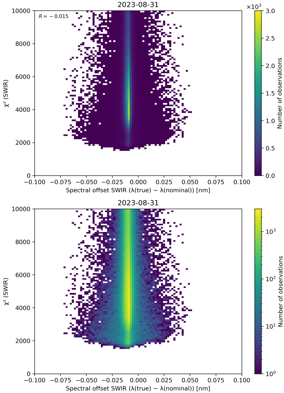
Figure 118: Scatter density plot of “Spectral offset SWIR ( \lambda(\text{true}) - \lambda(\text{nominal}) )” against “ \chi^2 (SWIR)” for 2023-08-30 to 2023-09-01.
