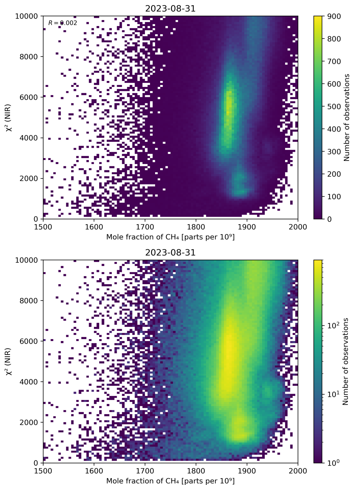
Figure 70: Scatter density plot of “Mole fraction of CH 4 ” against “ \chi^2 (NIR)” for 2023-08-30 to 2023-09-01.
