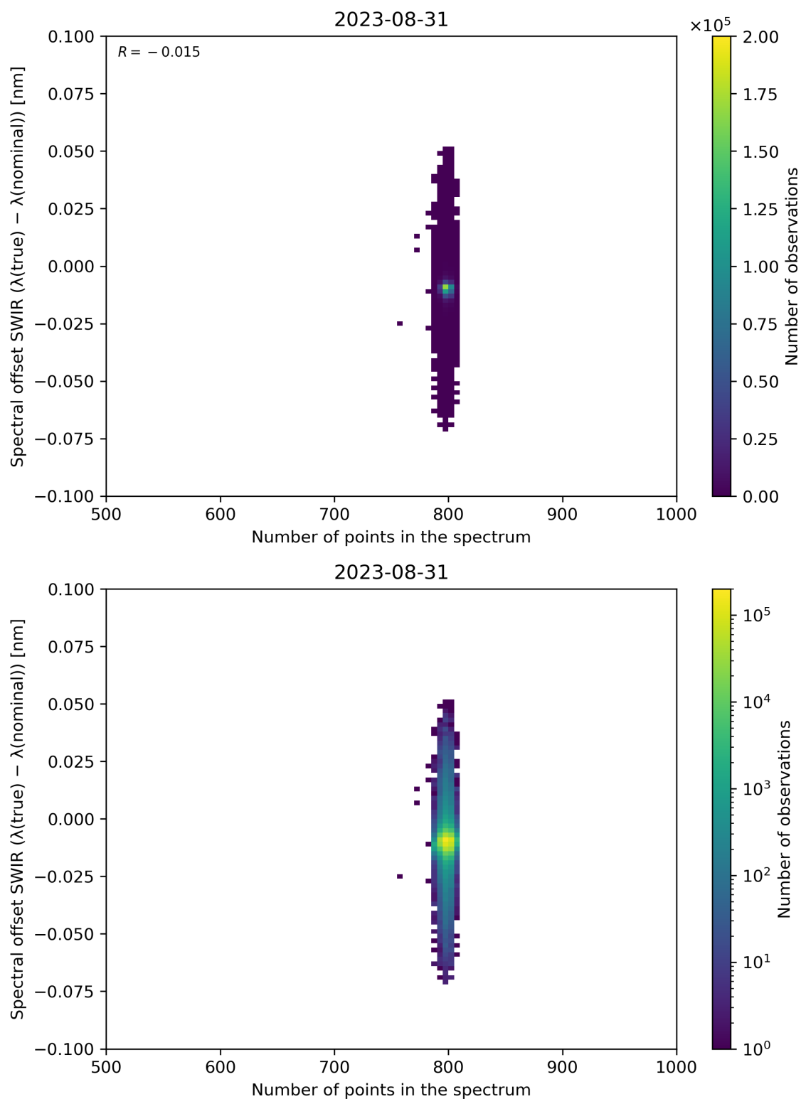
Figure 93: Scatter density plot of “Number of points in the spectrum” against “Spectral offset SWIR ( \lambda(\text{true}) - \lambda(\text{nominal}) )” for 2023-08-30 to 2023-09-01.
