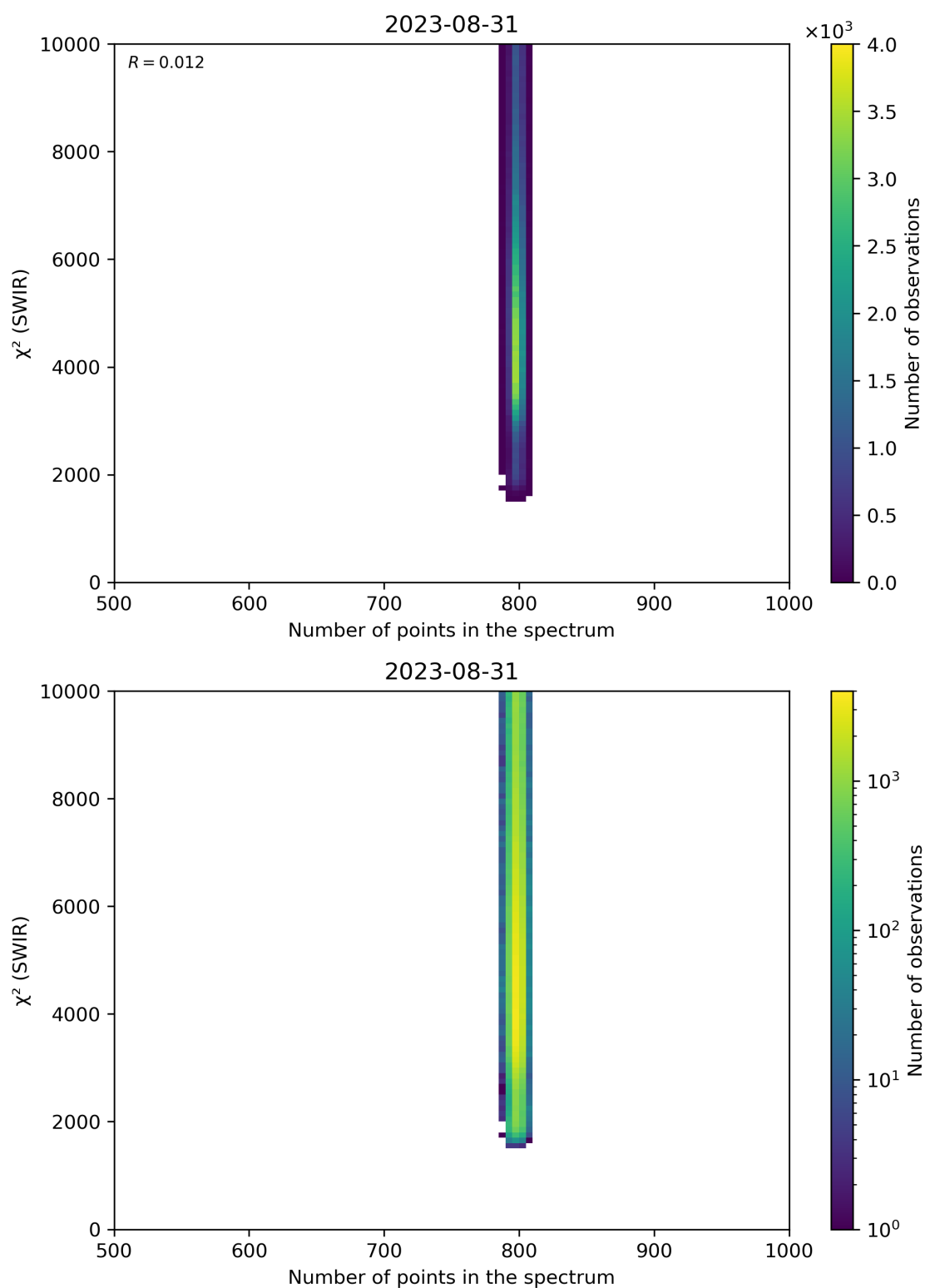
Figure 89: Scatter density plot of “Number of points in the spectrum” against “ \chi^2 (SWIR)” for 2023-08-30 to 2023-09-01.
