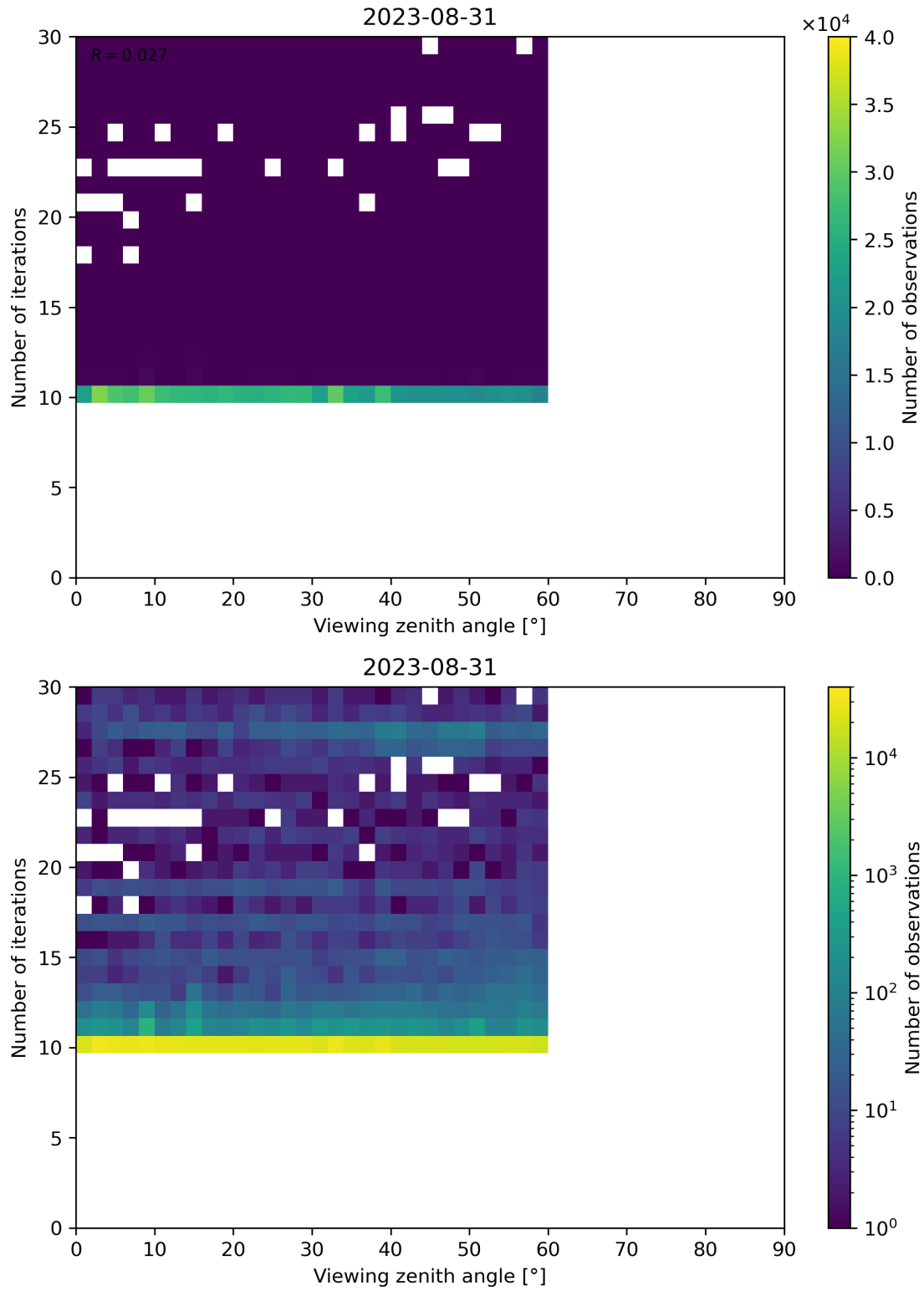
Figure 113: Scatter density plot of “Viewing zenith angle” against “Number of iterations” for 2023-08-30 to 2023-09-01.
