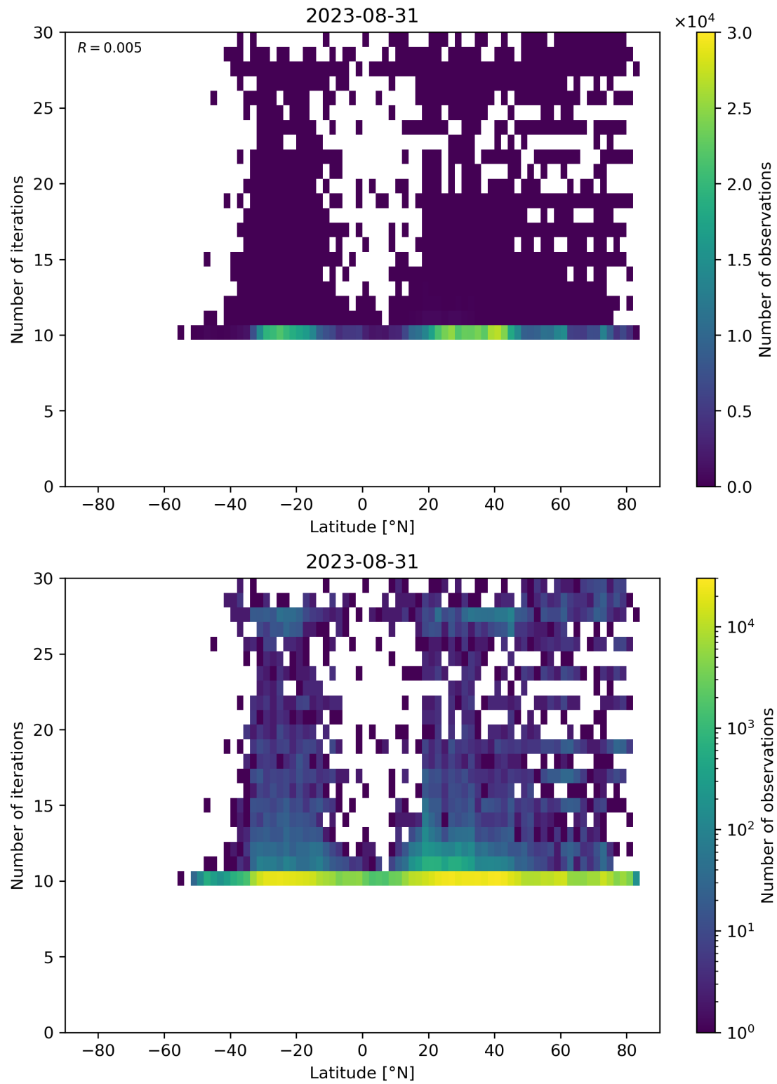
Figure 60: Scatter density plot of “Latitude” against “Number of iterations” for 2023-08-30 to 2023-09-01.
