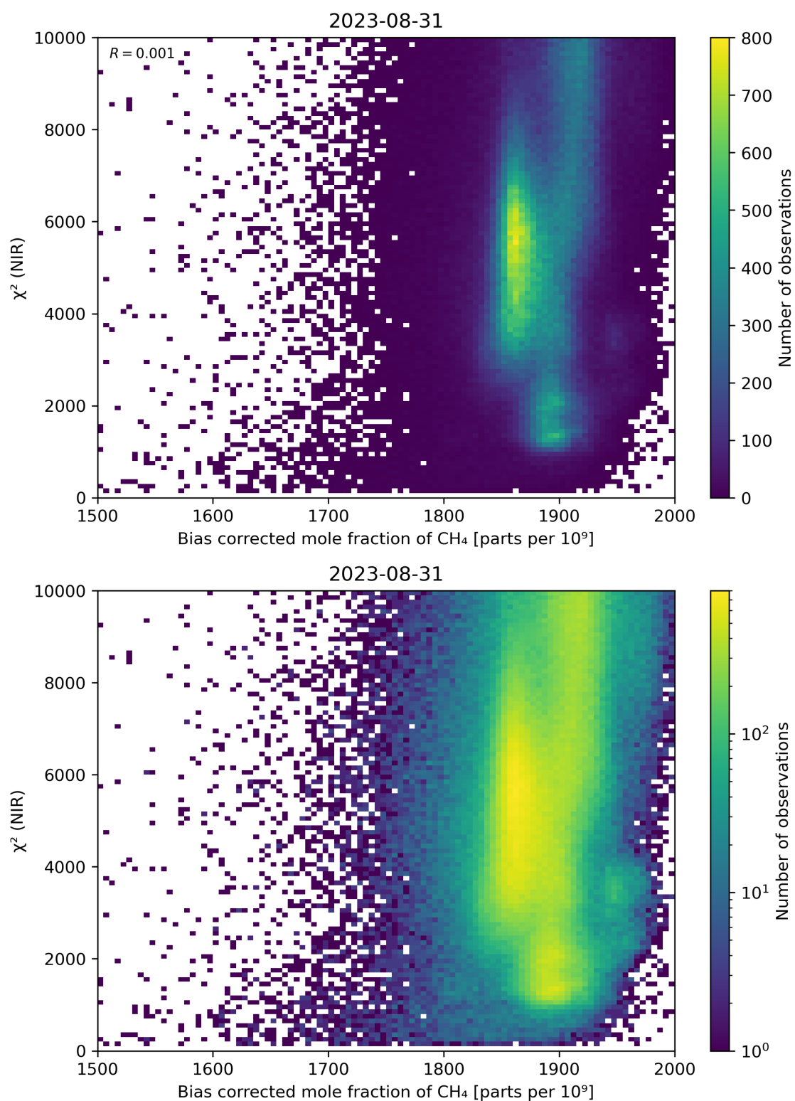
Figure 63: Scatter density plot of “Bias corrected mole fraction of CH 4 ” against “ \chi^2 (NIR)” for 2023-08-30 to 2023-09-01.
