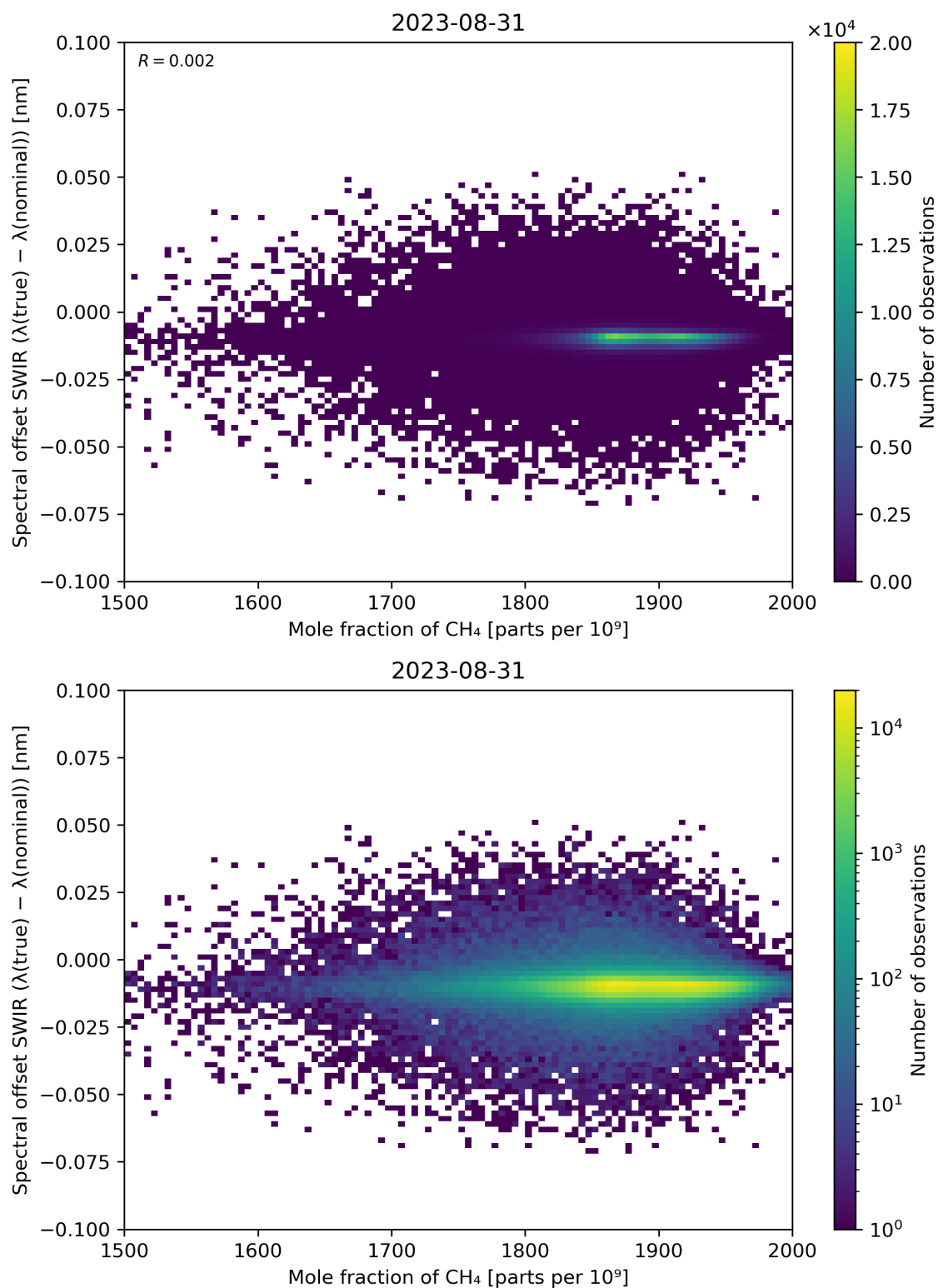
Figure 86: Scatter density plot of “Mole fraction of CH 4 ” against “Spectral offset SWIR ( \lambda(\text{true}) - \lambda(\text{nominal}) )” for 2023-08-30 to 2023-09-01.
