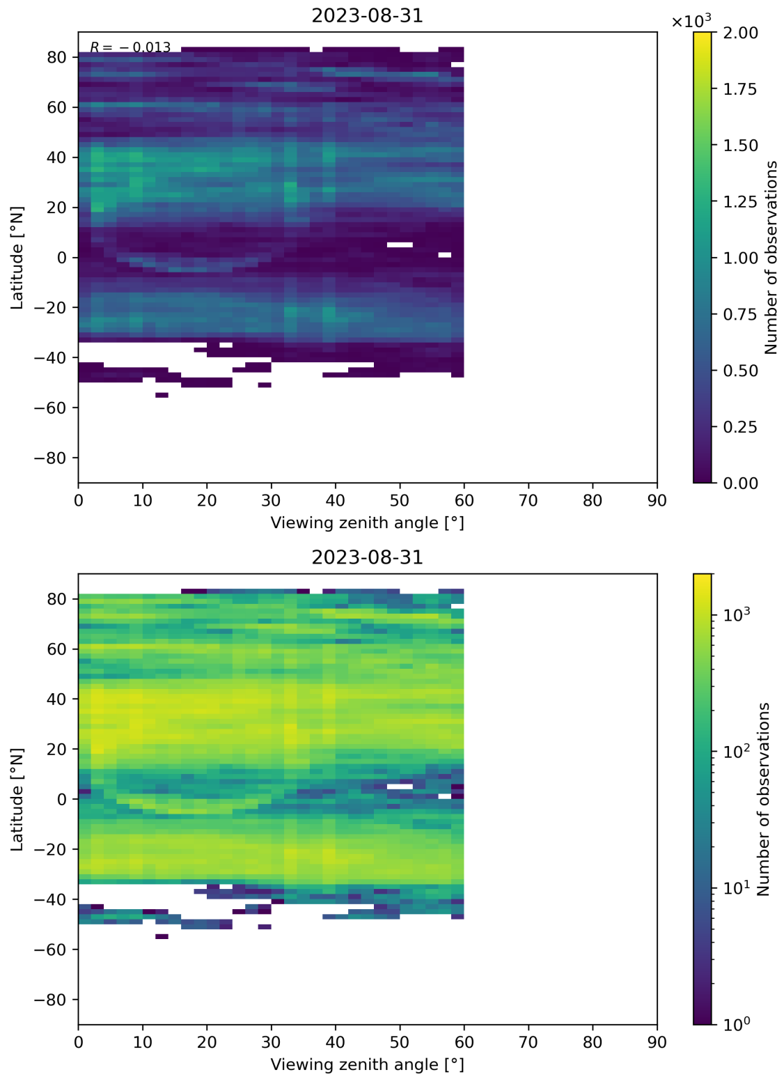
Figure 109: Scatter density plot of “Viewing zenith angle” against “Latitude” for 2023-08-30 to 2023-09-01.
