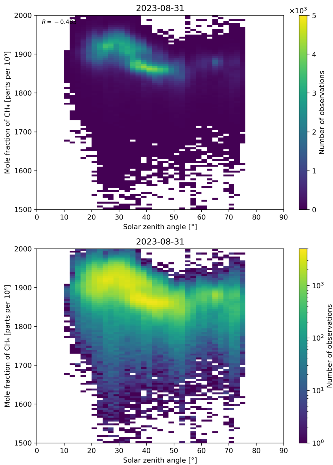
Figure 99: Scatter density plot of “Solar zenith angle” against “Mole fraction of CH 4 ” for 2023-08-30 to 2023-09-01.
