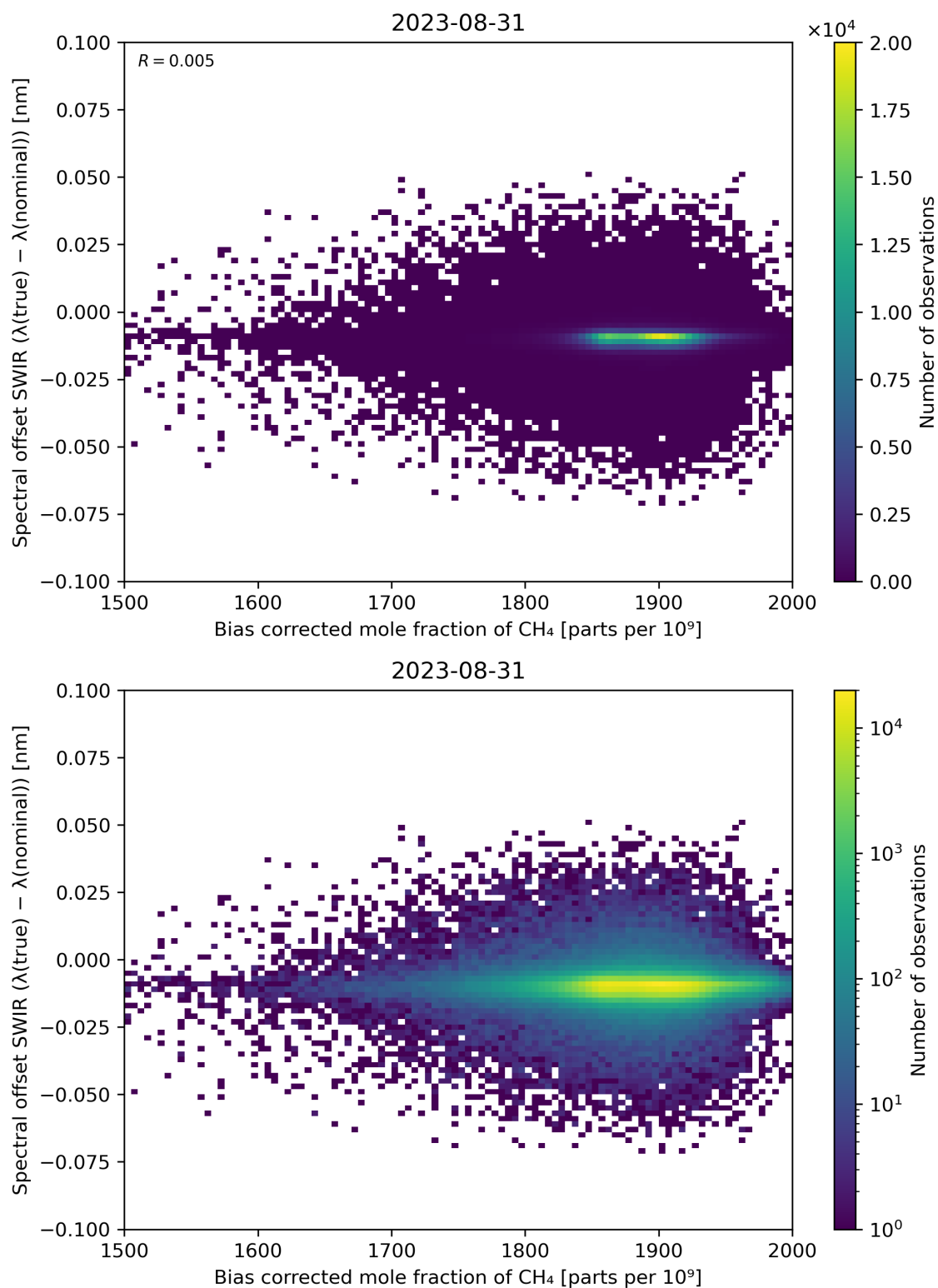
Figure 69: Scatter density plot of “Bias corrected mole fraction of \text{CH}_4 ” against “Spectral offset SWIR ( \lambda(\text{true}) - \lambda(\text{nominal}) )” for 2023-08-30 to 2023-09-01.
