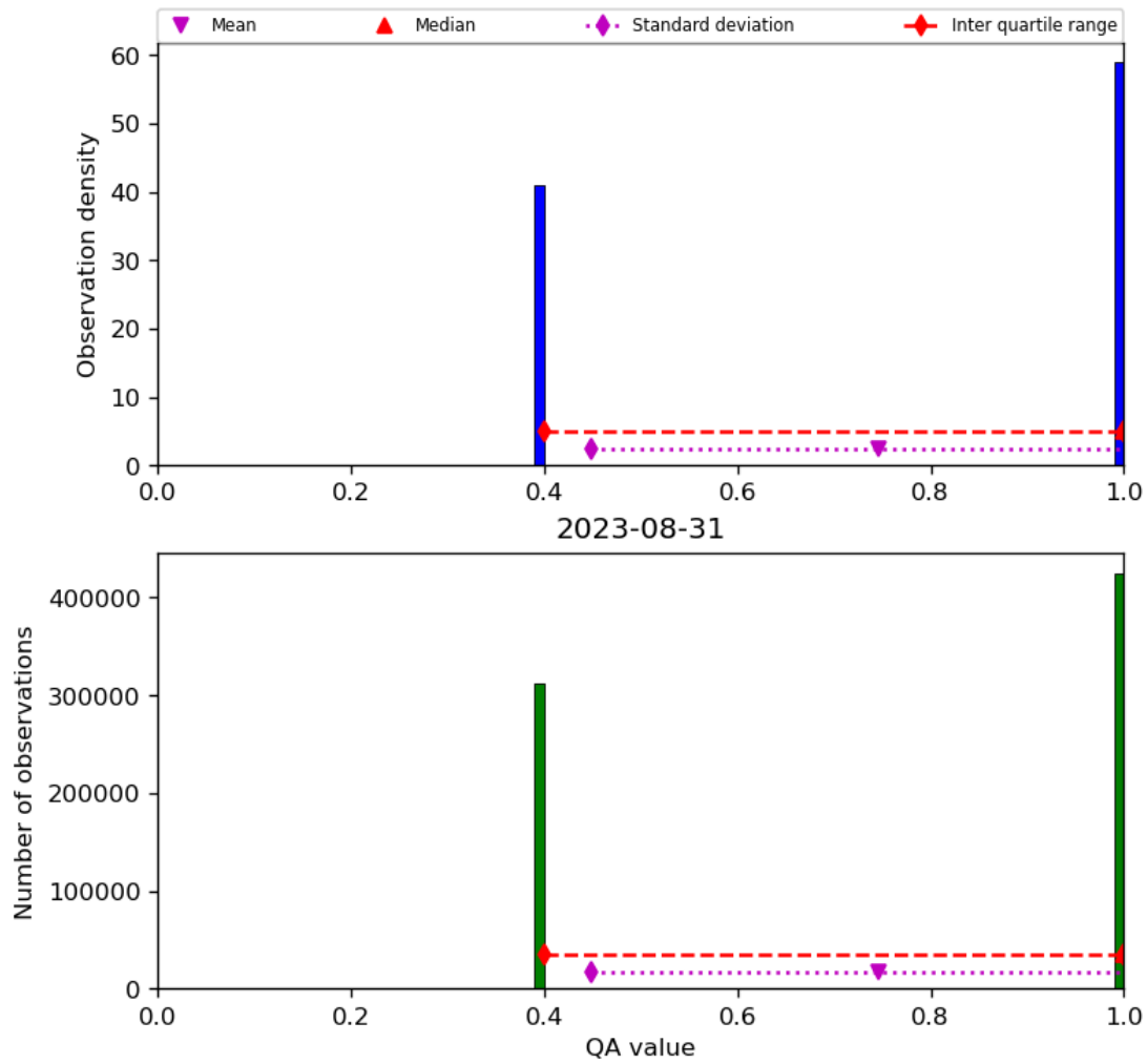
Figure 22: Histogram of “QA value” for 2023-08-30 to 2023-09-01
