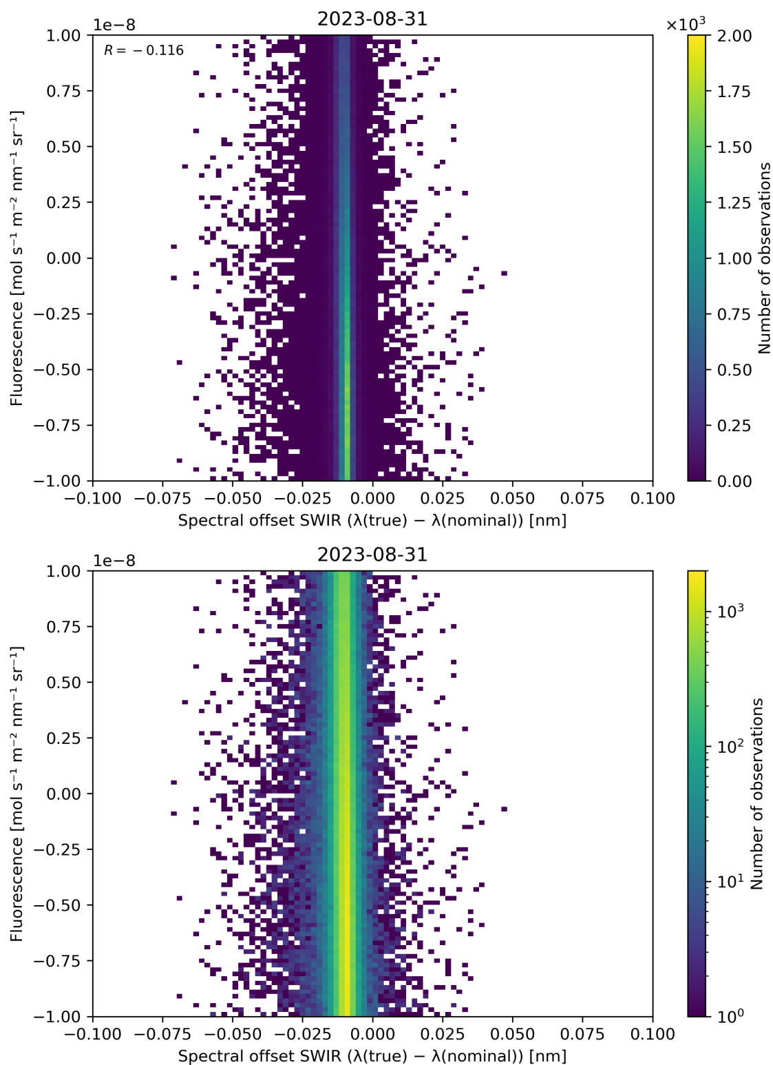
Figure 120: Scatter density plot of “Spectral offset SWIR ( \lambda(\text{true}) - \lambda(\text{nominal}) )” against “Fluorescence” for 2023-08-30 to 2023-09-01.
