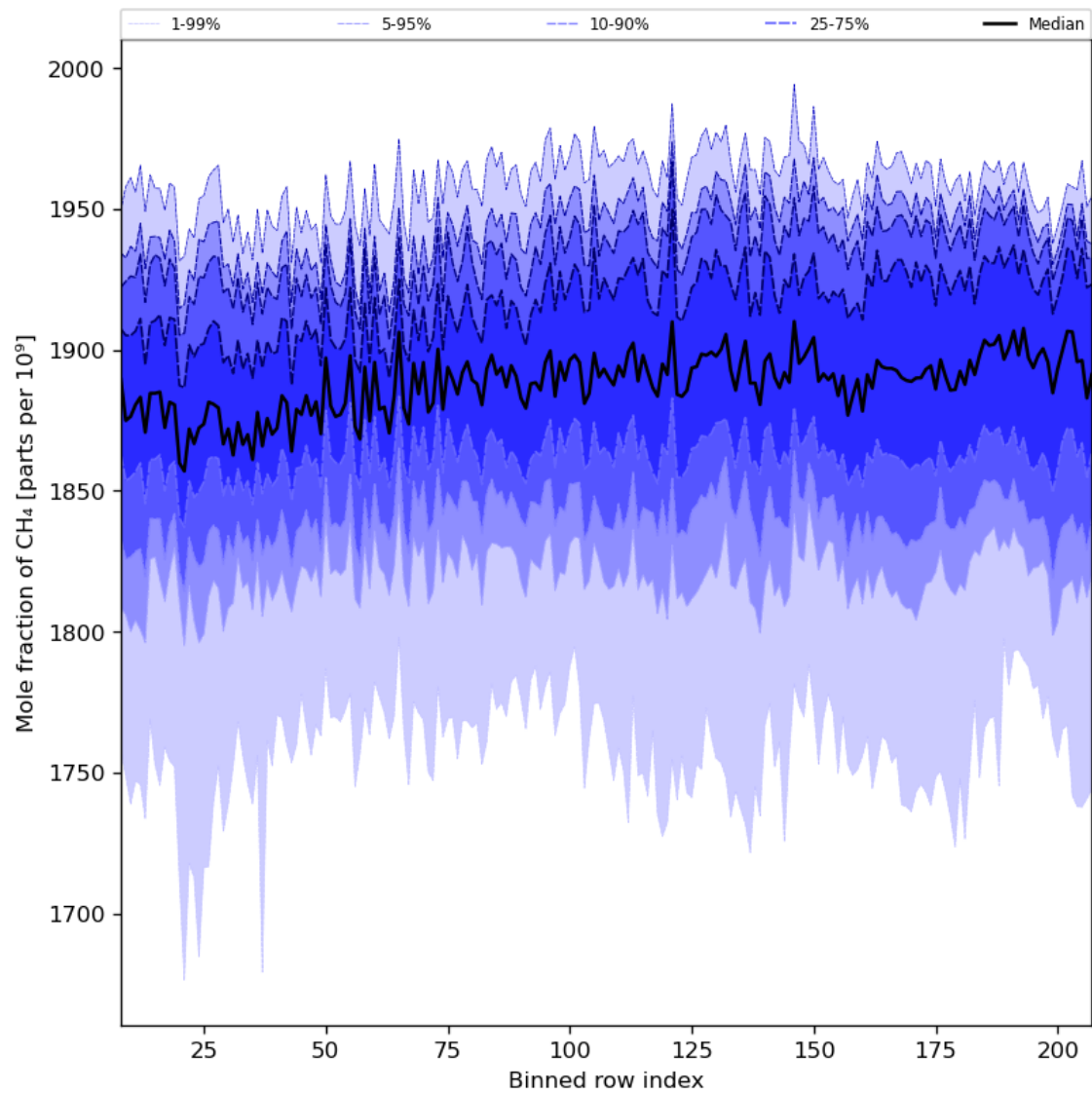
Figure 34: Along track statistics of “Mole fraction of CH 4 ” for 2023-08-30 to 2023-09-01
