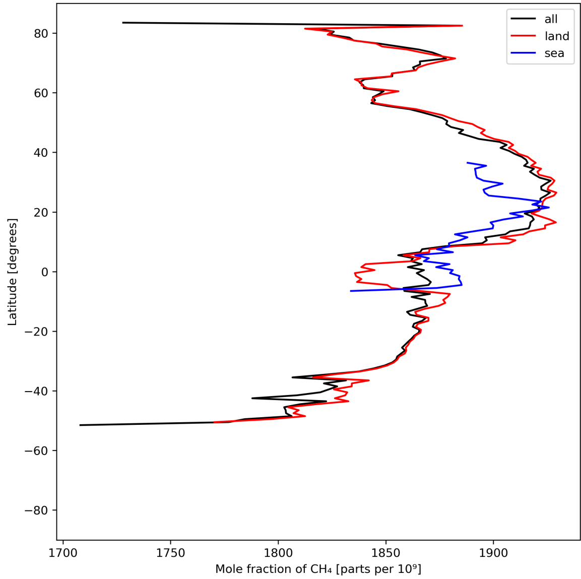
Figure 12: Zonal average of “Mole fraction of \text{CH}_4 ” for 2023-08-30 to 2023-09-01.
