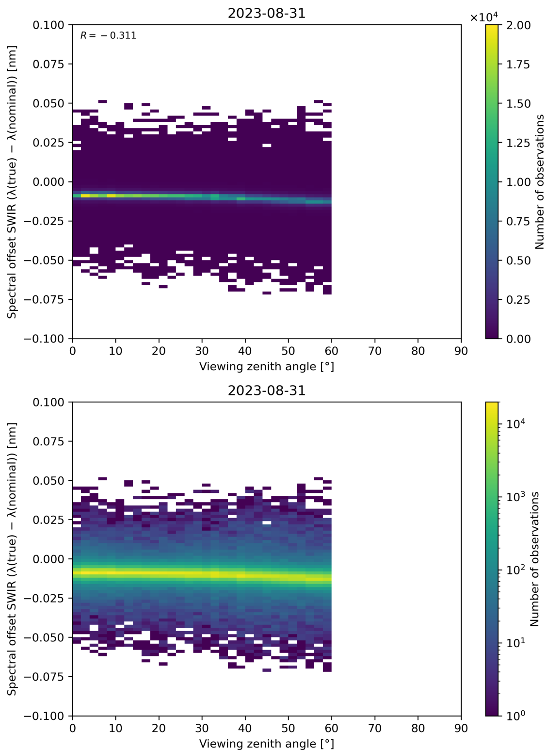
Figure 116: Scatter density plot of “Viewing zenith angle” against “Spectral offset SWIR ( \lambda(\text{true}) - \lambda(\text{nominal}) )” for 2023-08-30 to 2023-09-01.
