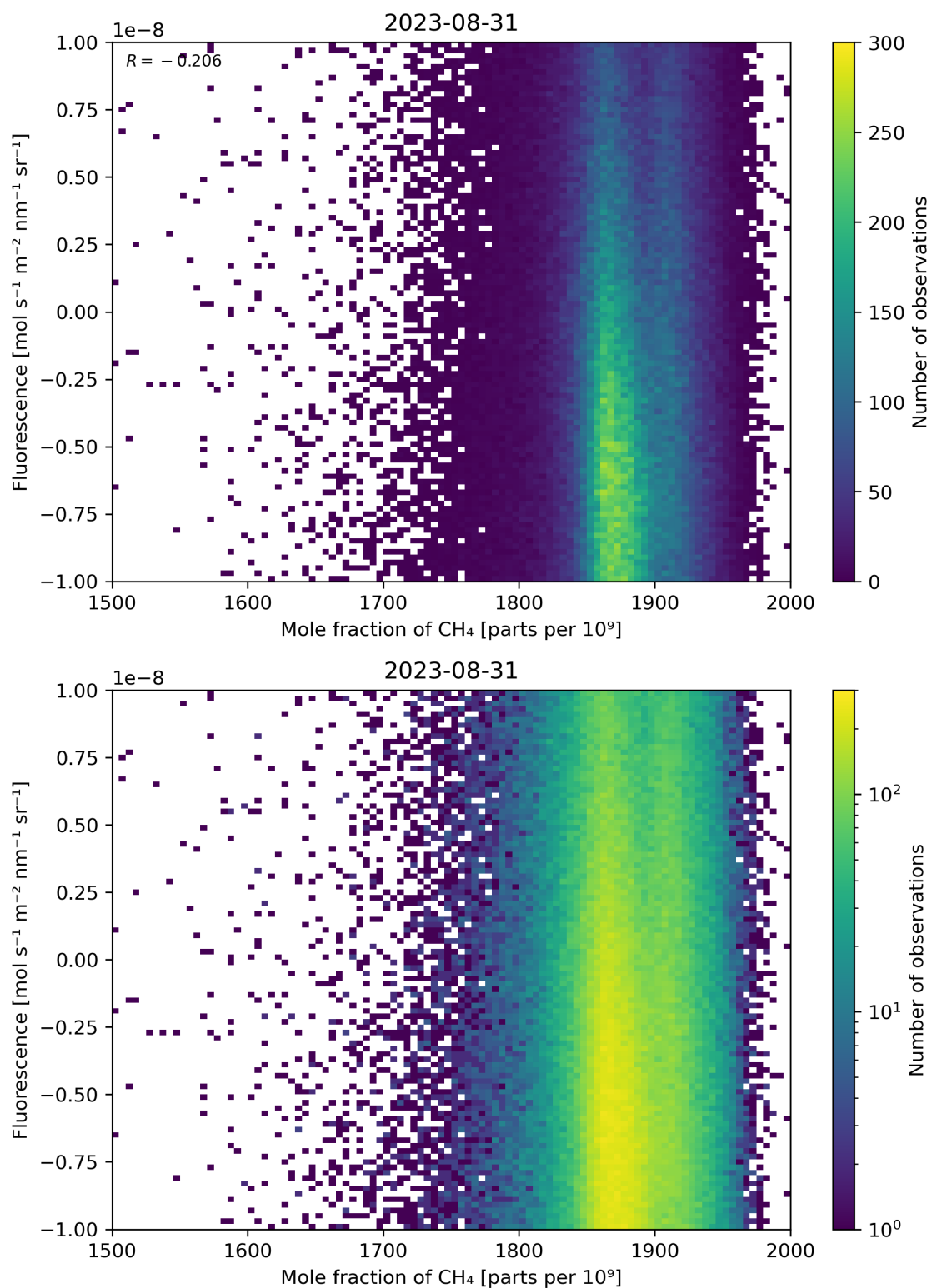
Figure 73: Scatter density plot of “Mole fraction of \text{CH}_4 ” against “Fluorescence” for 2023-08-30 to 2023-09-01.
