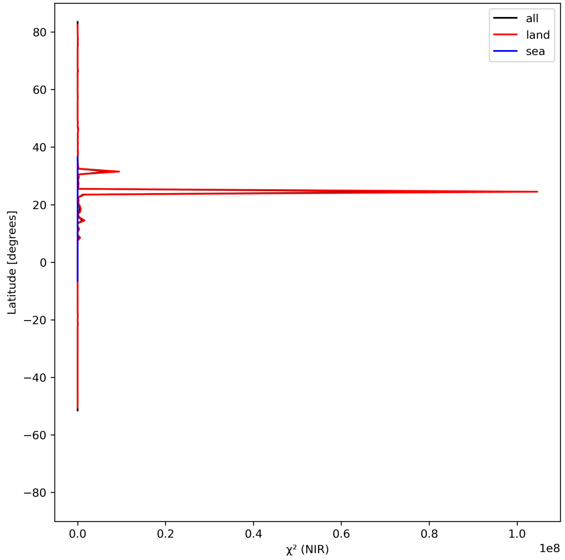
Figure 18: Zonal average of “ \chi^2 (NIR)” for 2023-08-30 to 2023-09-01.
