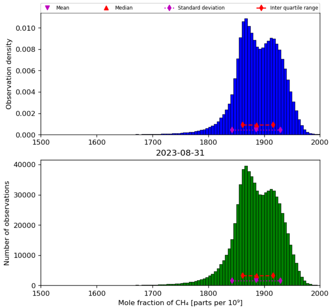
Figure 23: Histogram of “Mole fraction of CH 4 ” for 2023-08-30 to 2023-09-01
