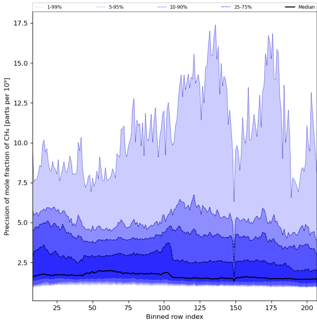
Figure 35: Along track statistics of “Precision of mole fraction of CH 4 ” for 2023-08-30 to 2023-09-01
