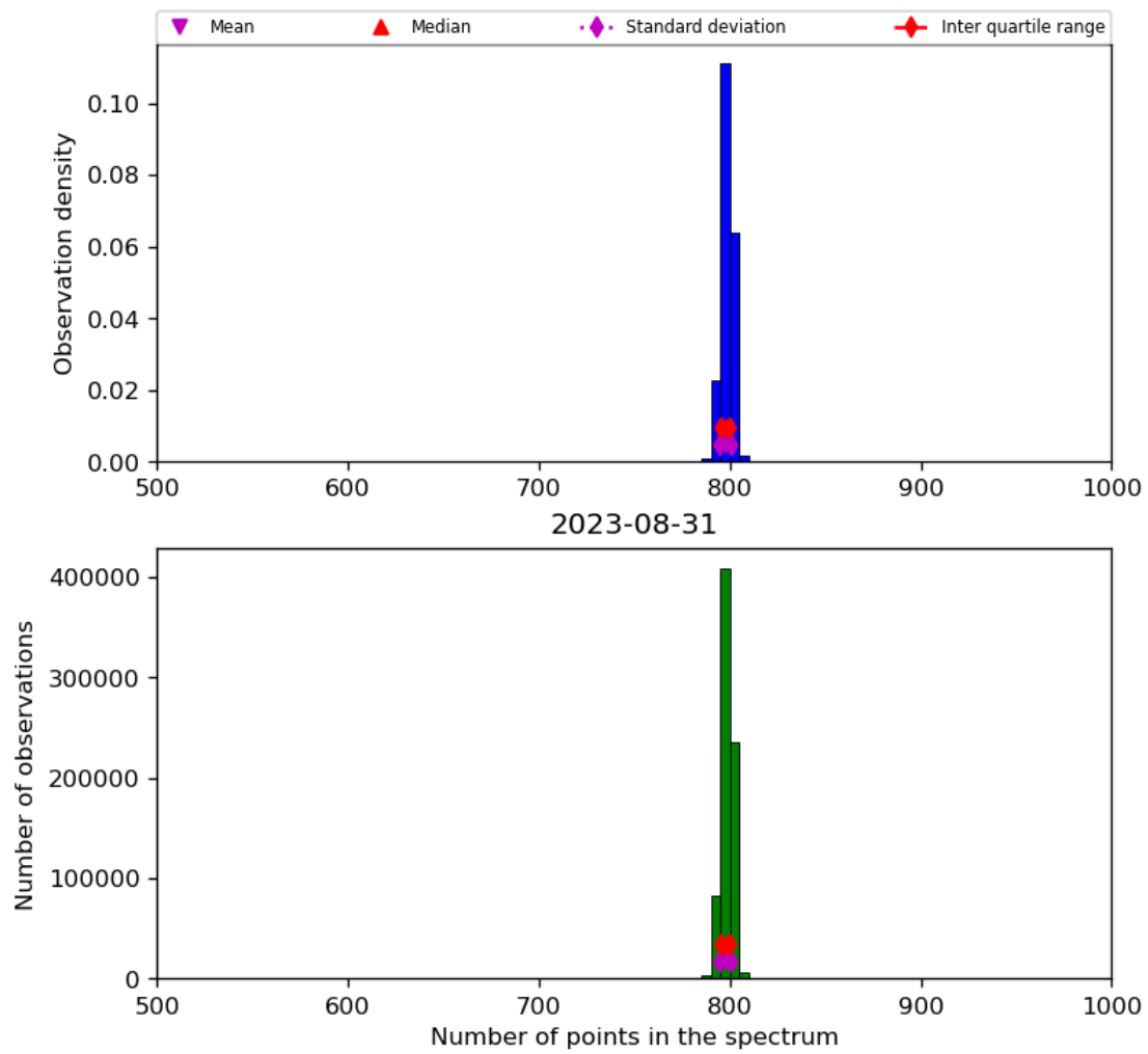
Figure 26: Histogram of “Number of points in the spectrum” for 2023-08-30 to 2023-09-01
