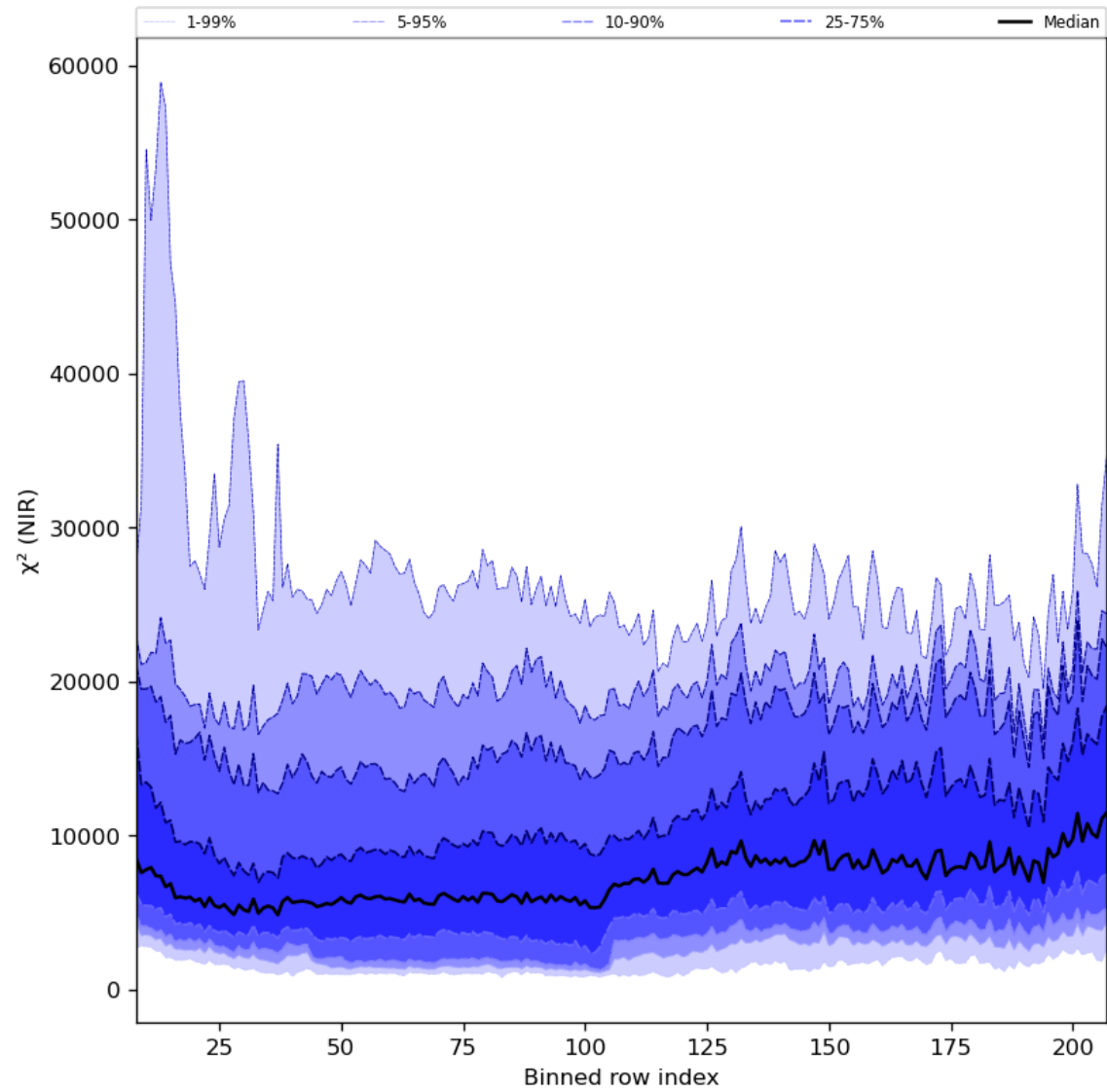
Figure 40: Along track statistics of “ \chi^2 (NIR)” for 2023-08-30 to 2023-09-01
