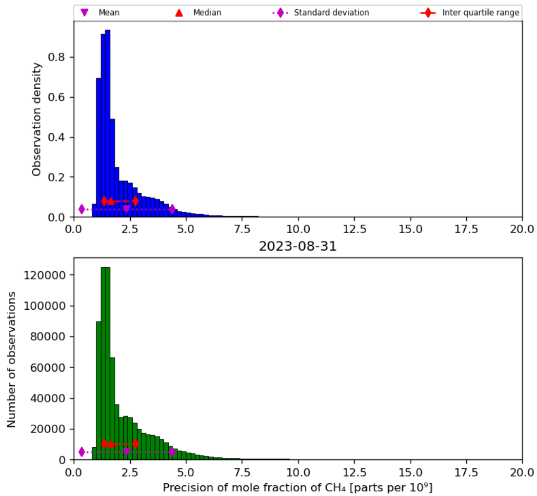
Figure 24: Histogram of “Precision of mole fraction of CH 4 ” for 2023-08-30 to 2023-09-01
