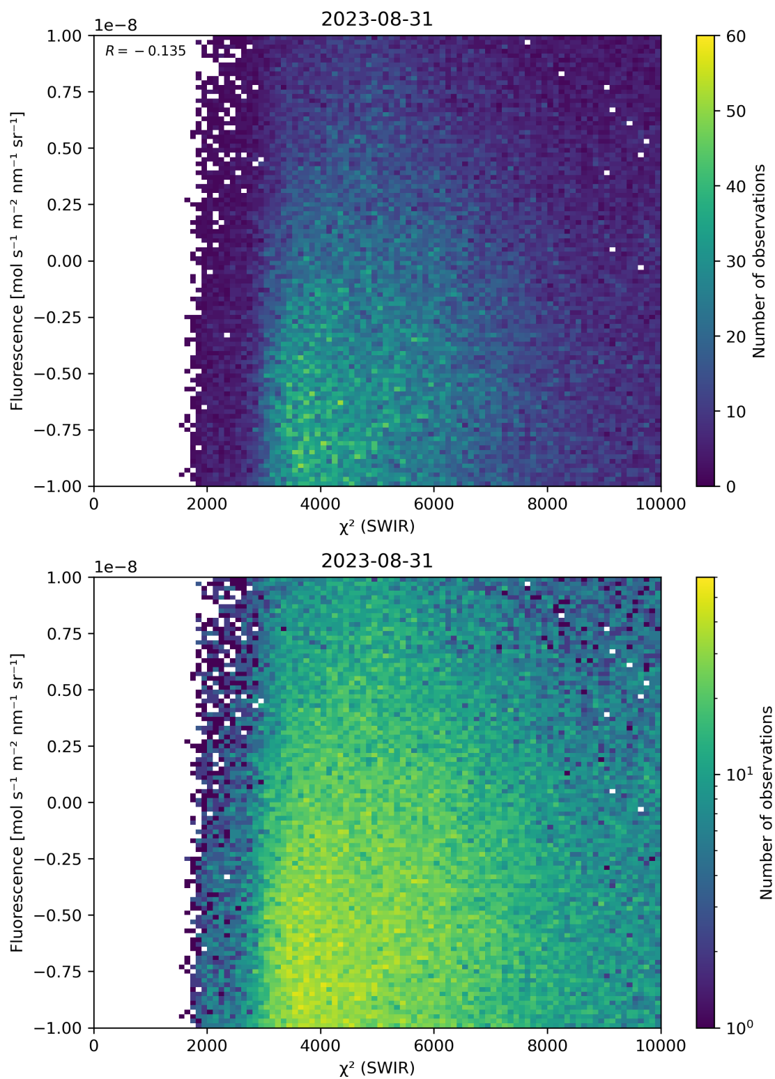
Figure 49: Scatter density plot of “ \chi^2 (SWIR)” against “Fluorescence” for 2023-08-30 to 2023-09-01.
