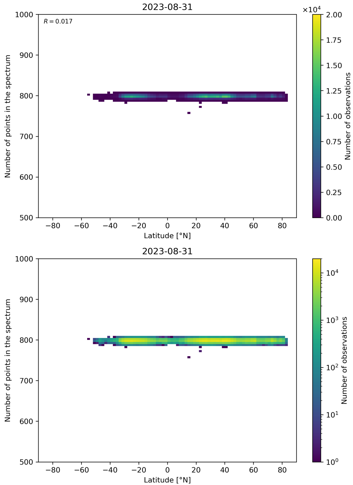
Figure 61: Scatter density plot of “Latitude” against “Number of points in the spectrum” for 2023-08-30 to 2023-09-01.
