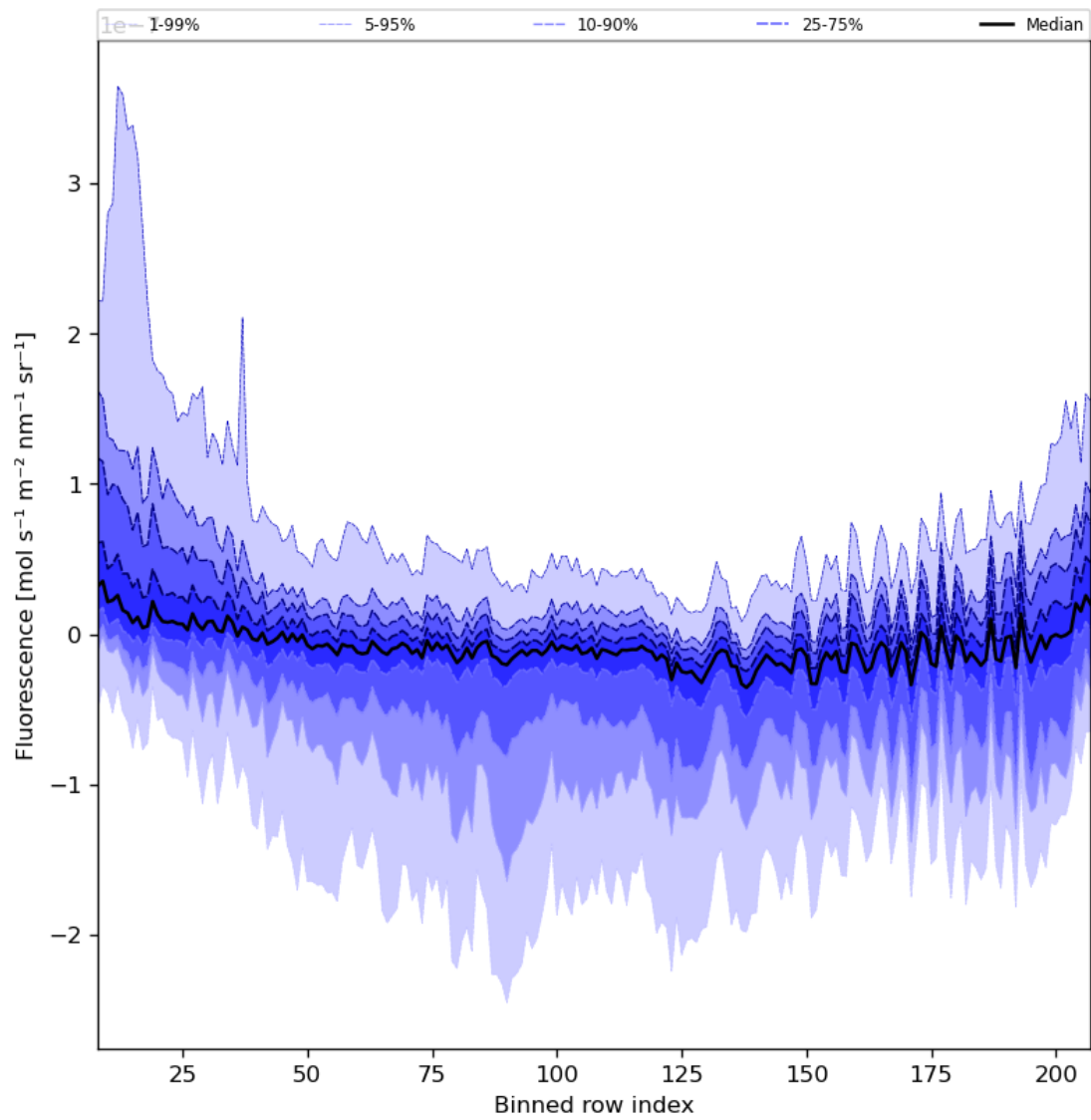
Figure 43: Along track statistics of “Fluorescence” for 2023-08-30 to 2023-09-01
