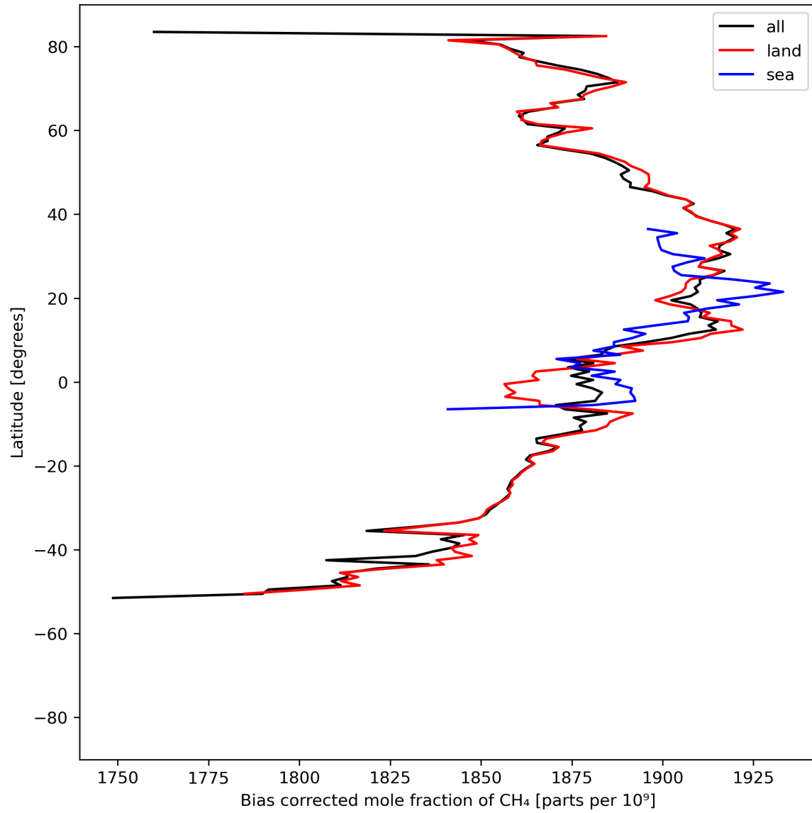
Figure 14: Zonal average of “Bias corrected mole fraction of CH 4 ” for 2023-08-30 to 2023-09-01.
