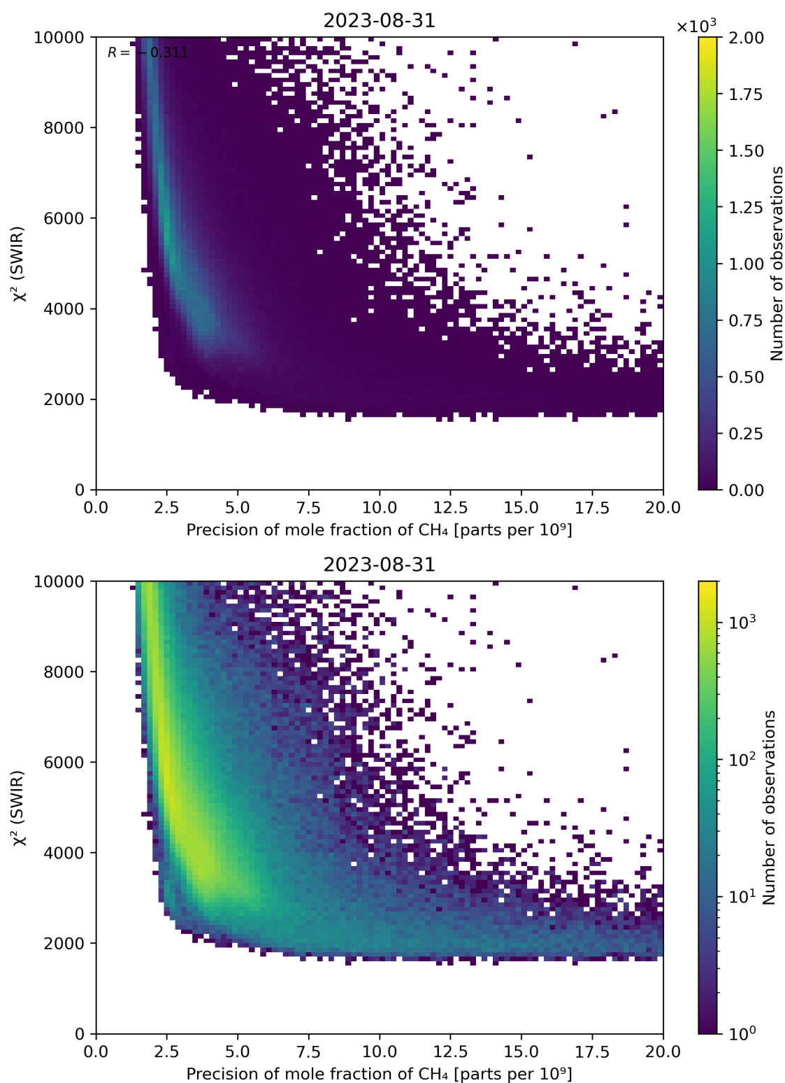
Figure 79: Scatter density plot of “Precision of mole fraction of CH 4 ” against “ \chi^2 (SWIR)” for 2023-08-30 to 2023-09-01.
