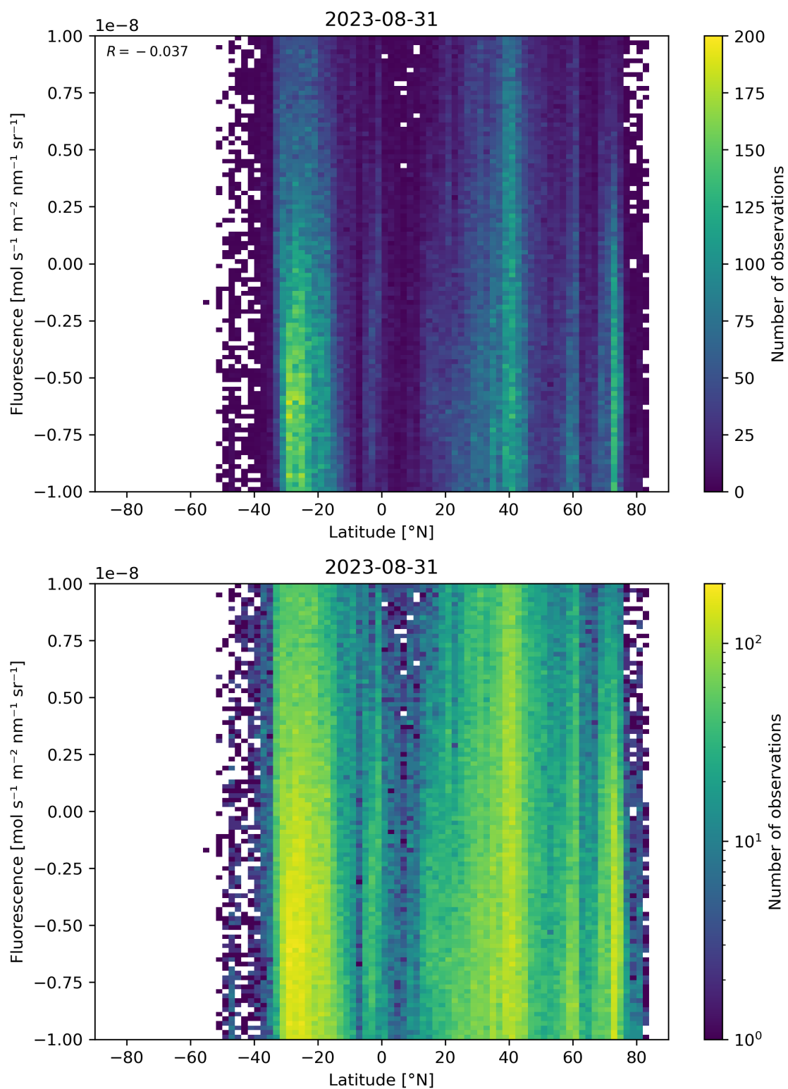
Figure 56: Scatter density plot of “Latitude” against “Fluorescence” for 2023-08-30 to 2023-09-01.
