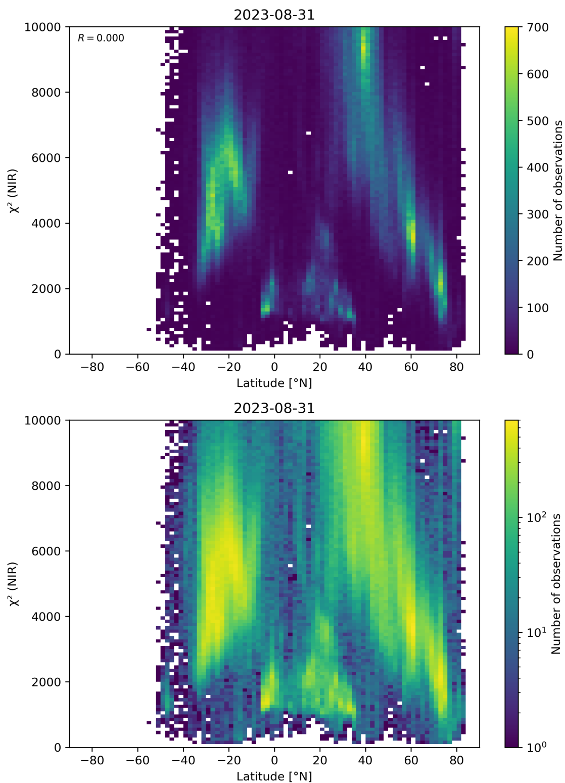
Figure 53: Scatter density plot of “Latitude” against “ \chi^2 (NIR)” for 2023-08-30 to 2023-09-01.
