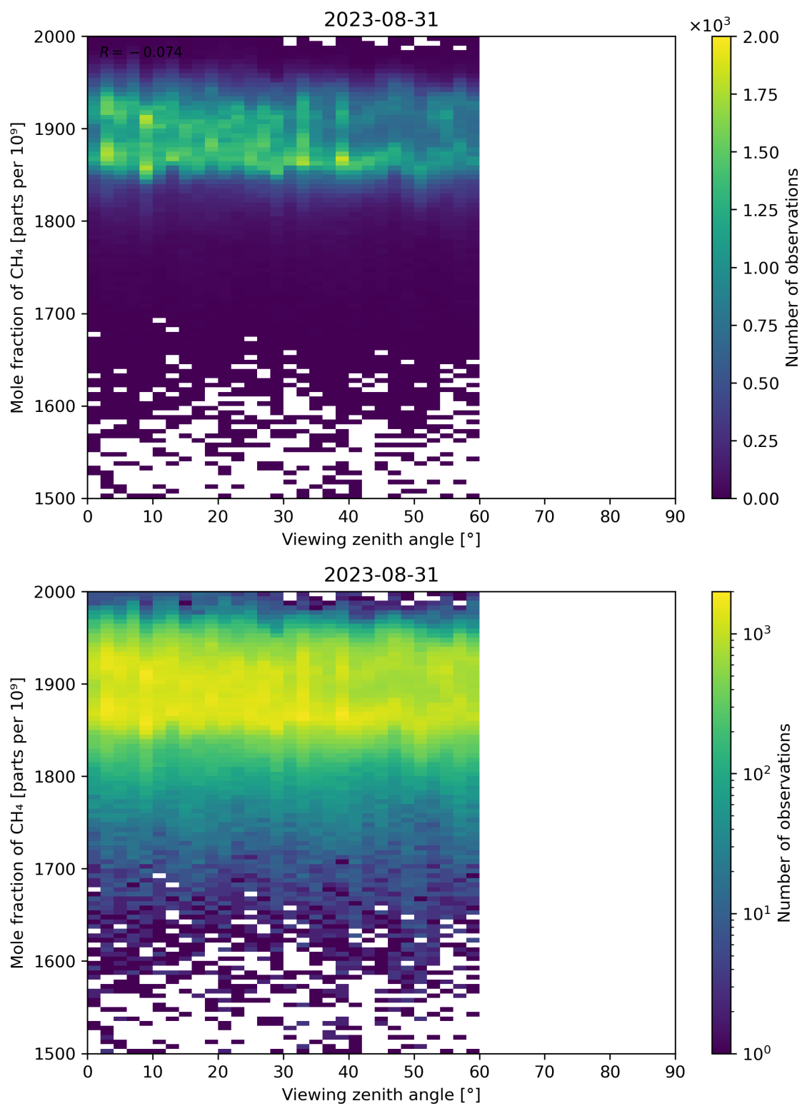
Figure 110: Scatter density plot of “Viewing zenith angle” against “Mole fraction of CH 4 ” for 2023-08-30 to 2023-09-01.
