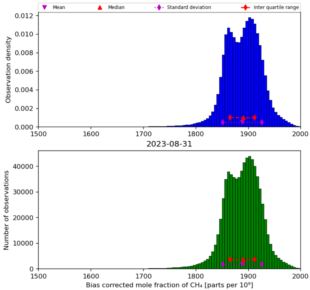
Figure 25: Histogram of “Bias corrected mole fraction of CH 4 ” for 2023-08-30 to 2023-09-01
