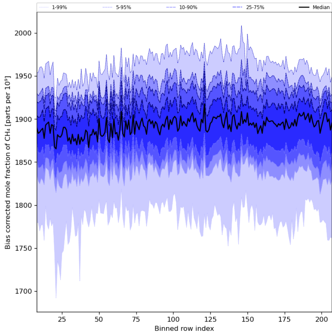
Figure 36: Along track statistics of “Bias corrected mole fraction of CH 4 ” for 2023-08-30 to 2023-09-01
