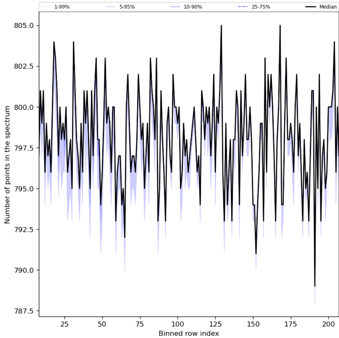
Figure 37: Along track statistics of “Number of points in the spectrum” for 2023-08-30 to 2023-09-01
