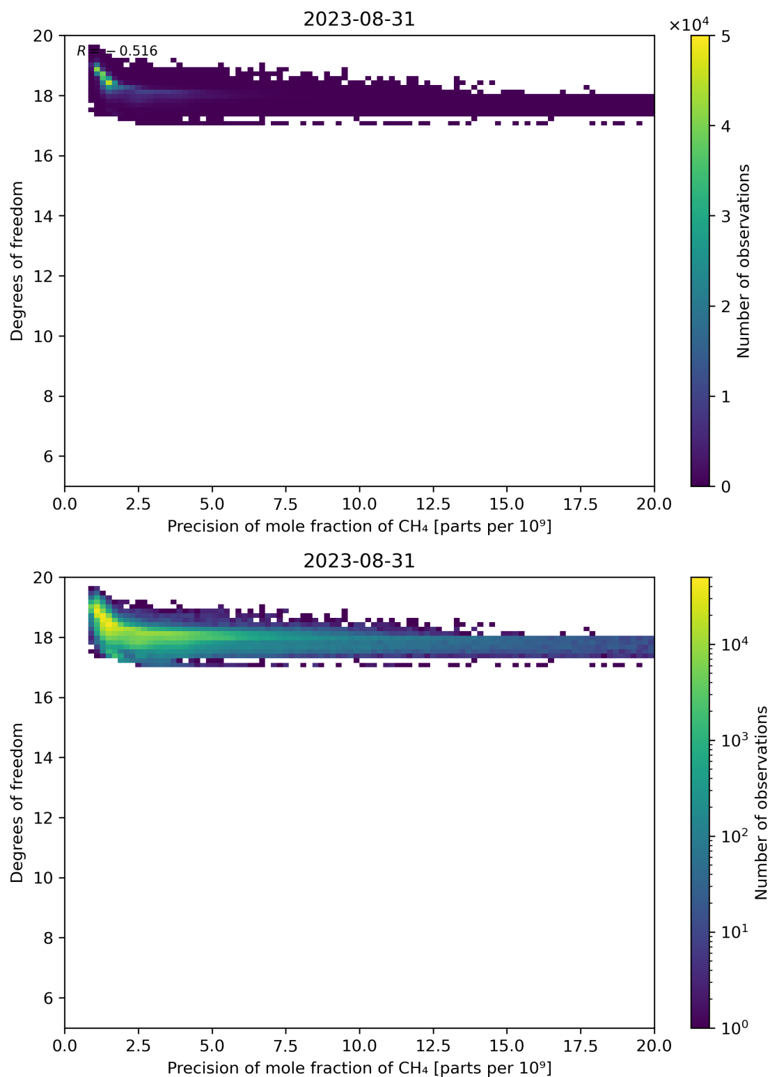
Figure 80: Scatter density plot of “Precision of mole fraction of CH 4 ” against “Degrees of freedom” for 2023-08-30 to 2023-09-01.
