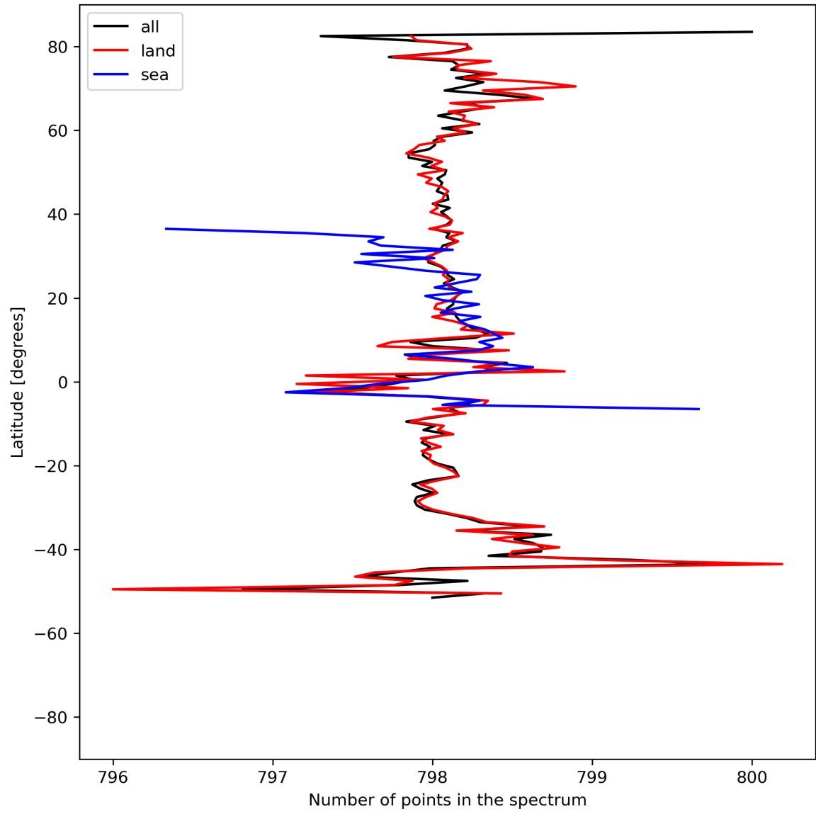
Figure 15: Zonal average of “Number of points in the spectrum” for 2023-08-30 to 2023-09-01.
