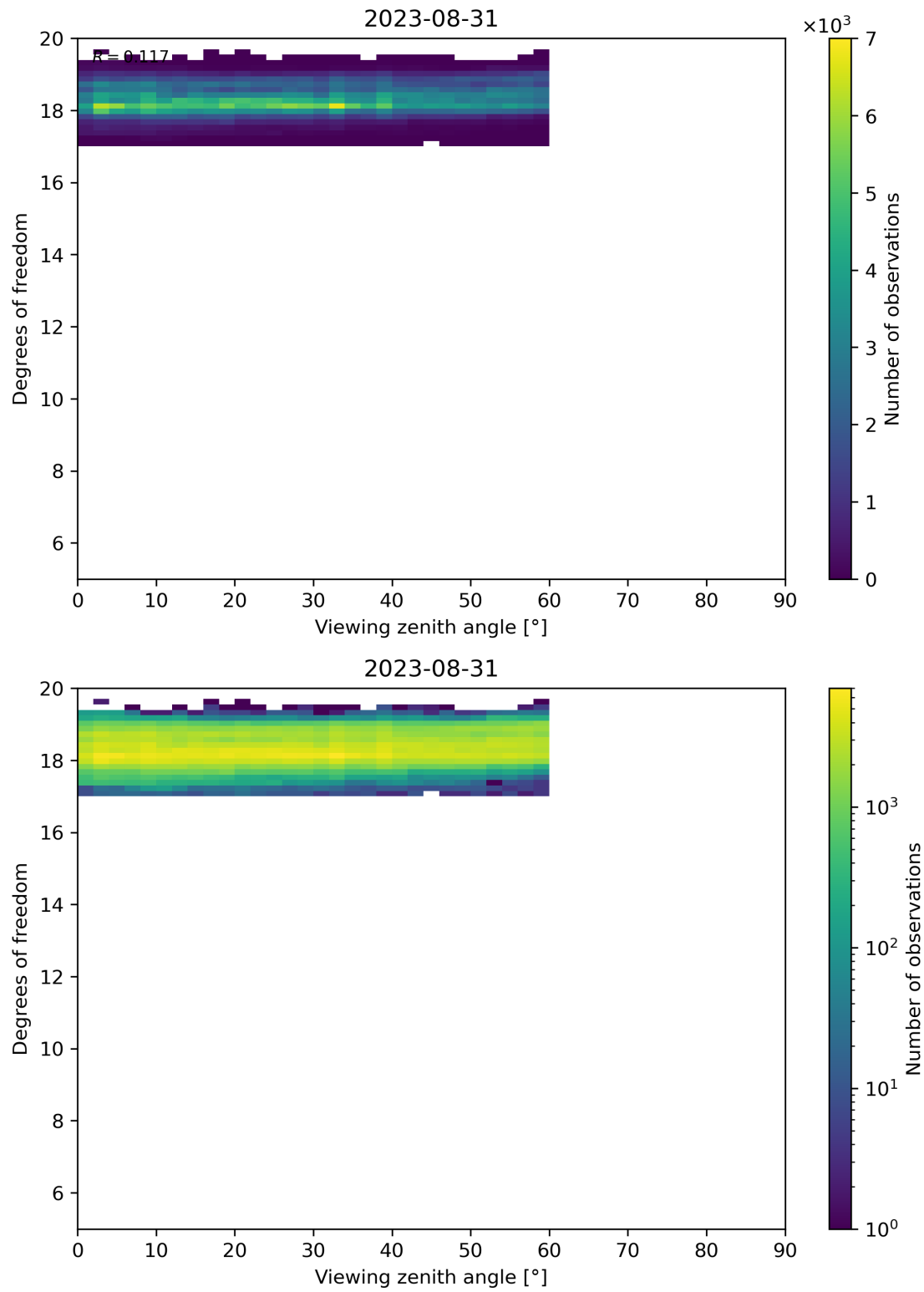
Figure 107: Scatter density plot of “Viewing zenith angle” against “Degrees of freedom” for 2023-08-30 to 2023-09-01.
