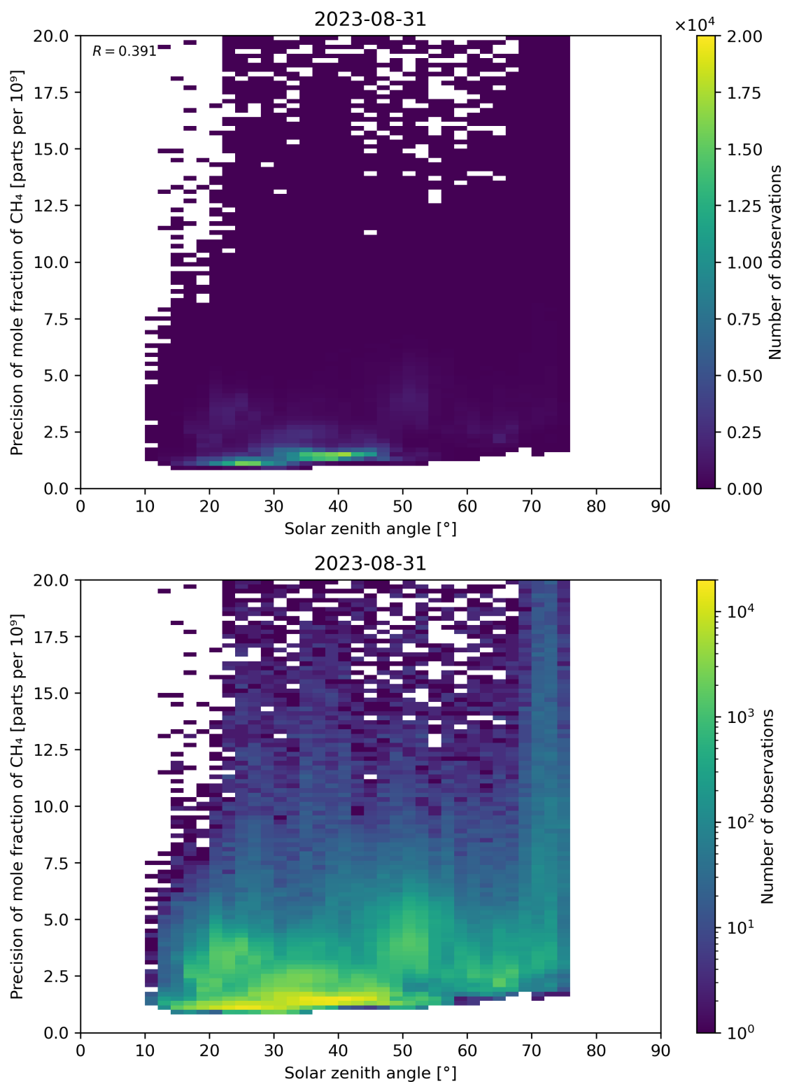
Figure 101: Scatter density plot of “Solar zenith angle” against “Precision of mole fraction of CH 4 ” for 2023-08-30 to 2023-09-01.
