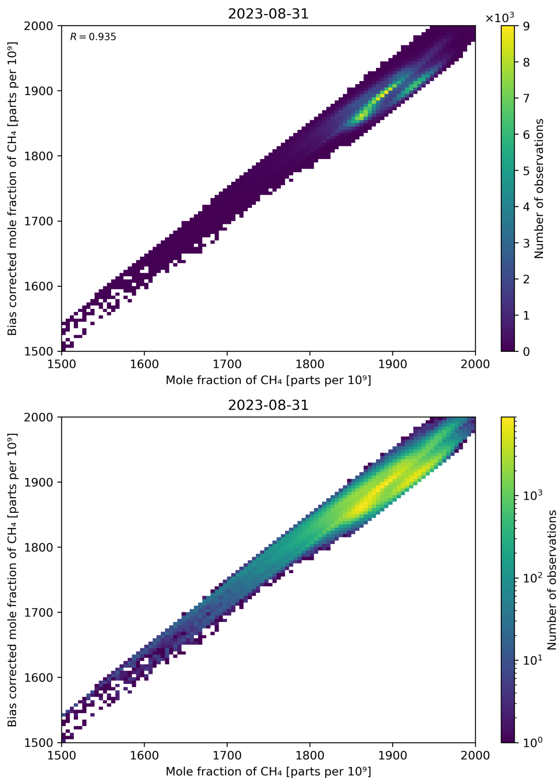
Figure 74: Scatter density plot of “Mole fraction of CH 4 ” against “Bias corrected mole fraction of CH 4 ” for 2023-08-30 to 2023-09-01.
