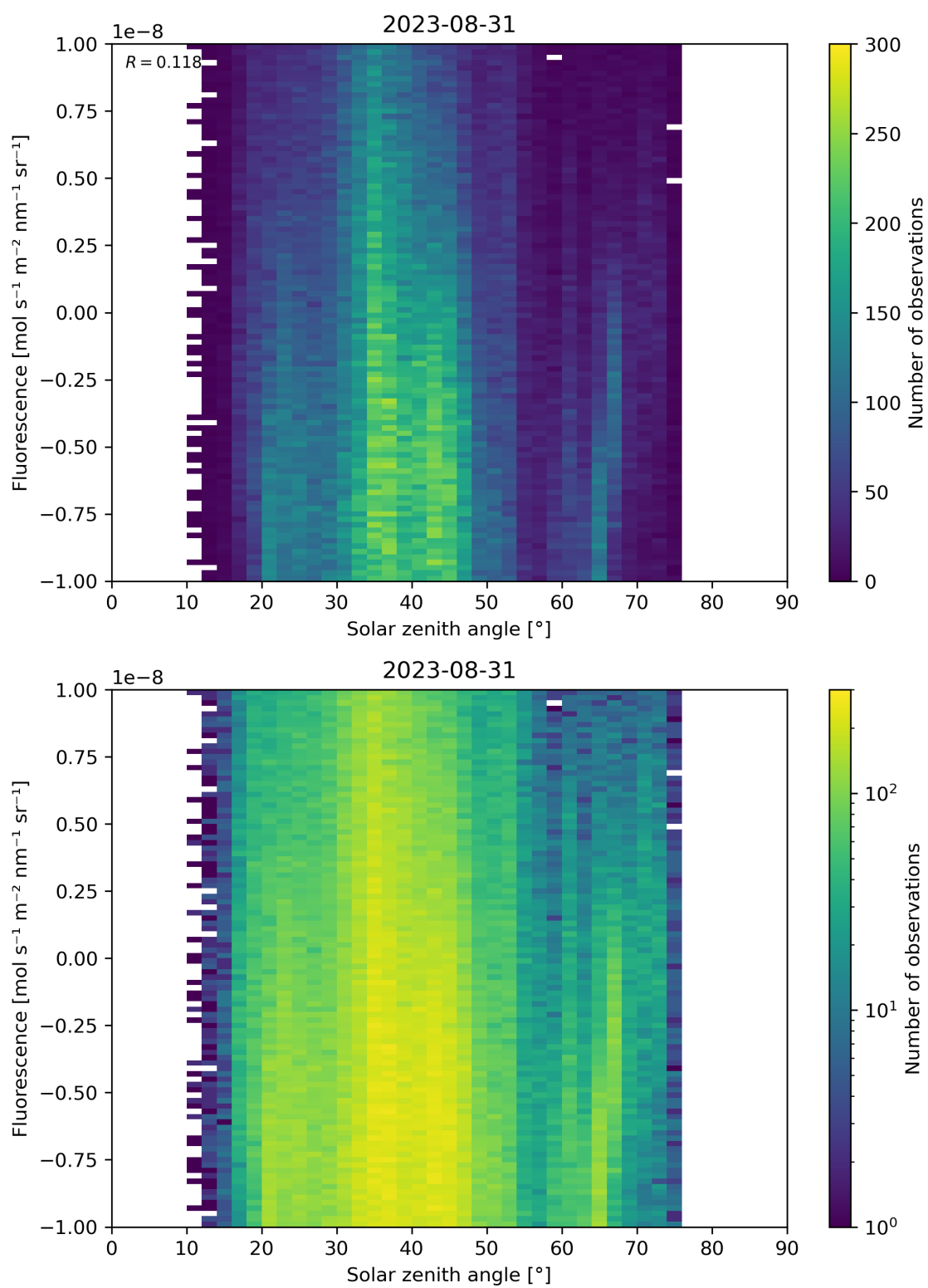
Figure 97: Scatter density plot of “Solar zenith angle” against “Fluorescence” for 2023-08-30 to 2023-09-01.
