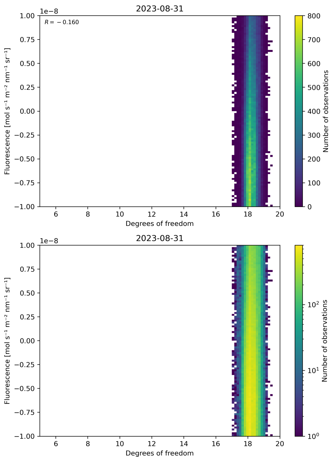
Figure 51: Scatter density plot of “Degrees of freedom” against “Fluorescence” for 2023-08-30 to 2023-09-01.
