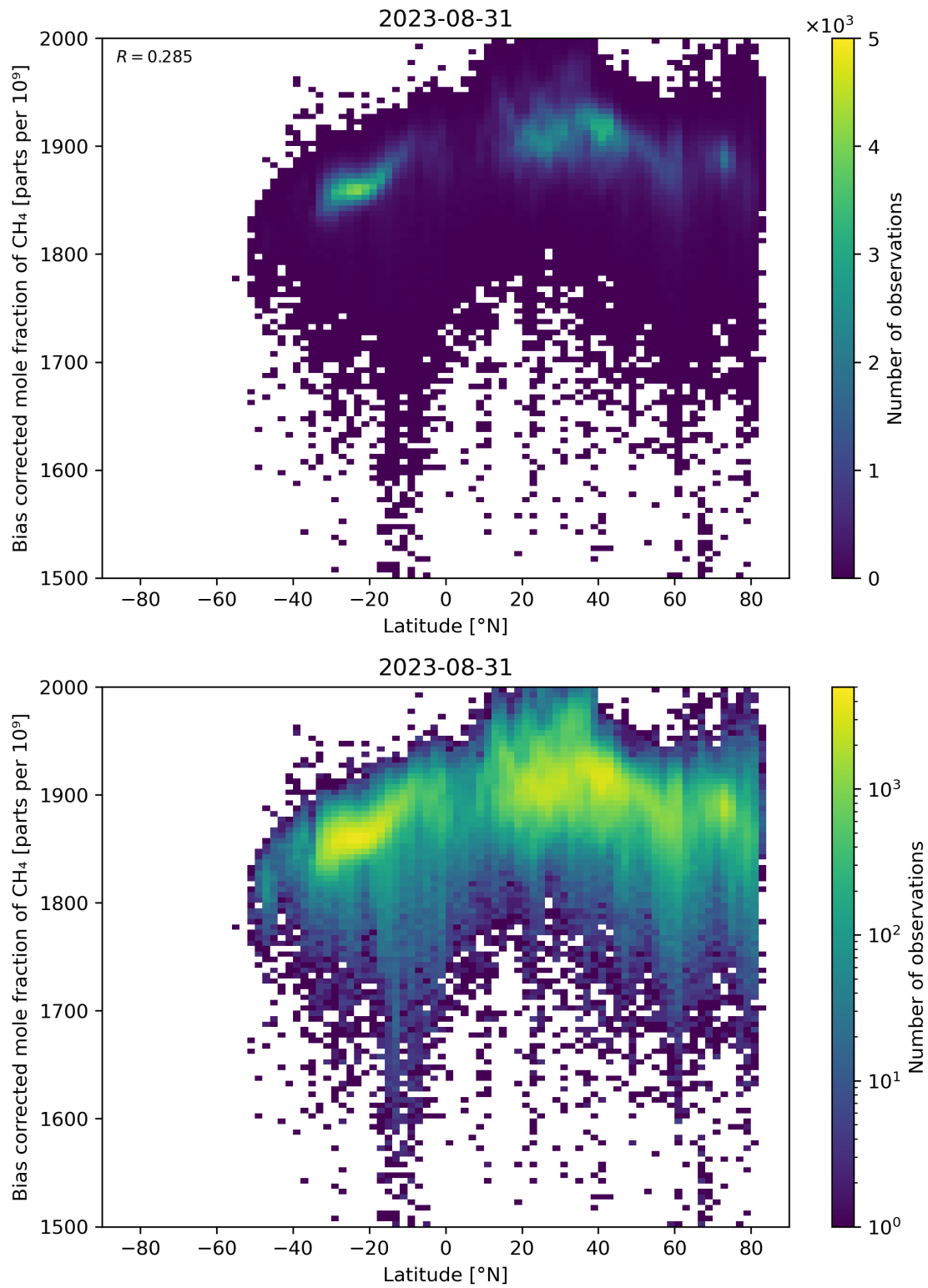
Figure 58: Scatter density plot of “Latitude” against “Bias corrected mole fraction of \text{CH}_4 ” for 2023-08-30 to 2023-09-01.
