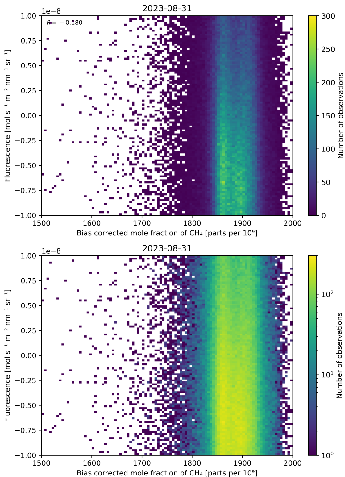
Figure 66: Scatter density plot of “Bias corrected mole fraction of \text{CH}_4 ” against “Fluorescence” for 2023-08-30 to 2023-09-01.
