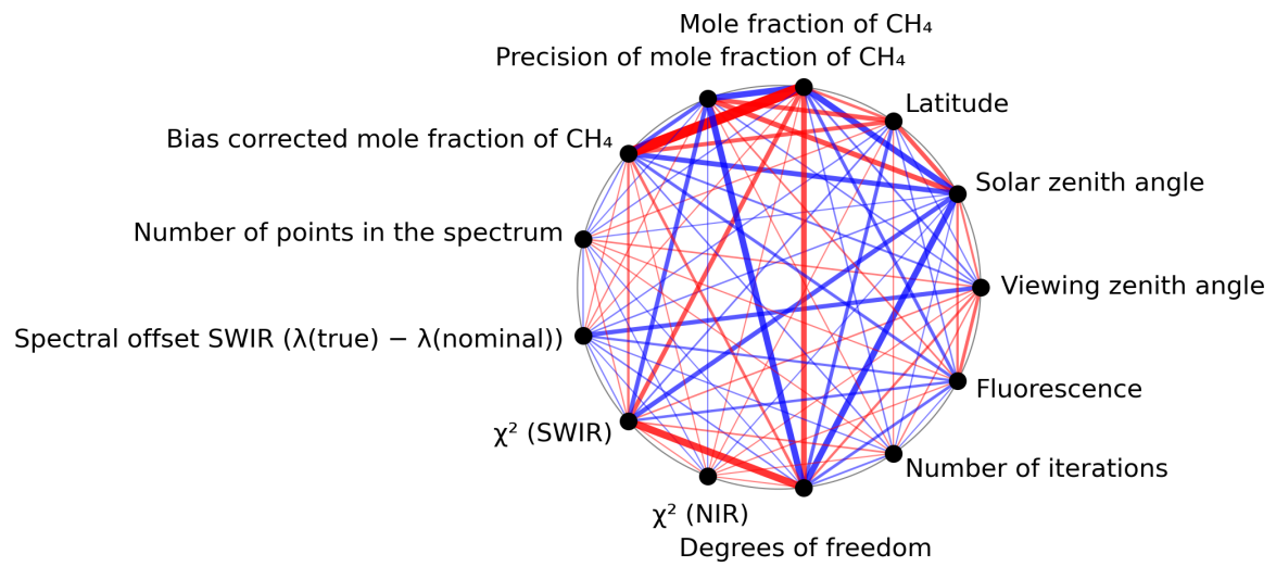
Figure 1: Map of correlation graph for 2023-08-30 to 2023-09-01.
