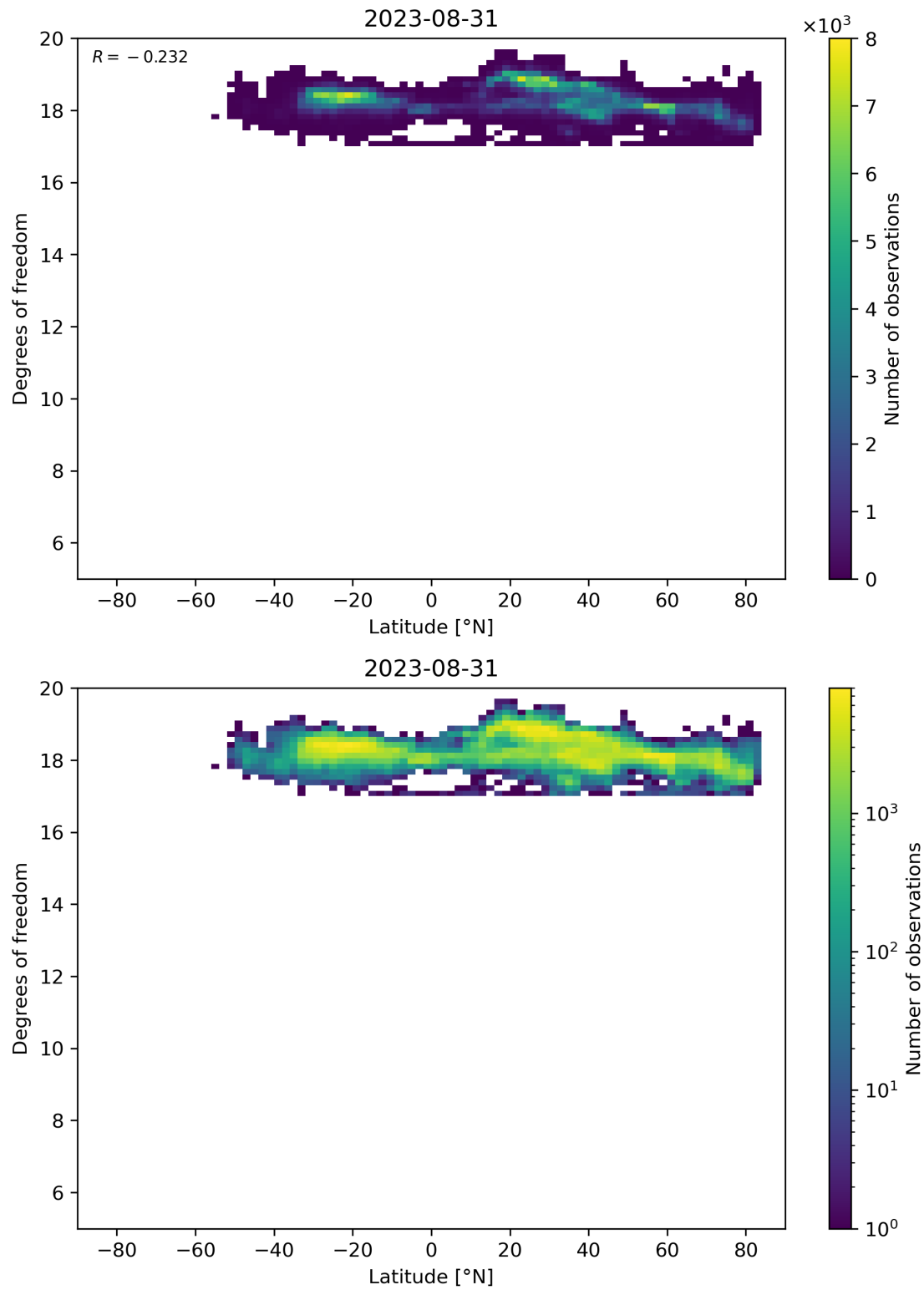
Figure 55: Scatter density plot of “Latitude” against “Degrees of freedom” for 2023-08-30 to 2023-09-01.
