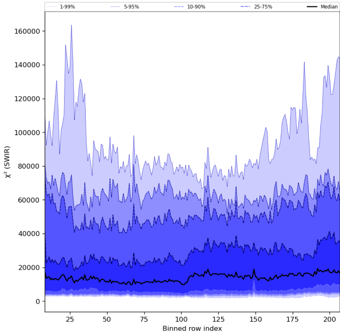
Figure 39: Along track statistics of " \chi^2 (SWIR)" for 2023-08-30 to 2023-09-01
