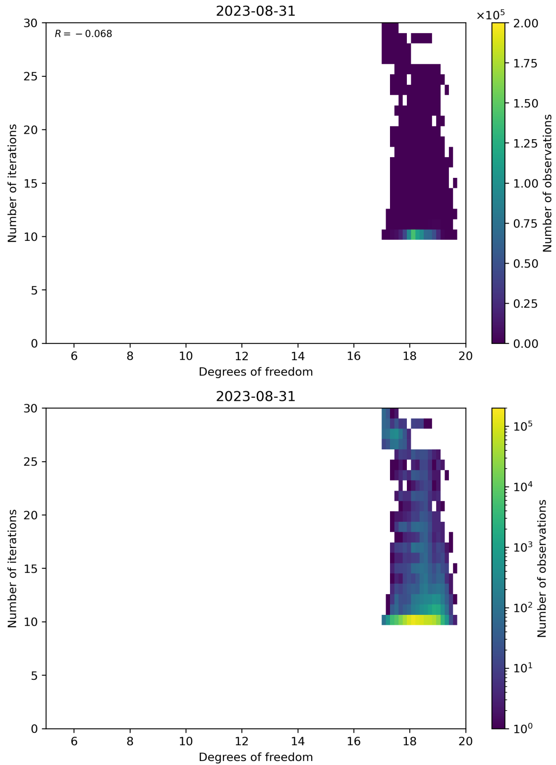
Figure 52: Scatter density plot of “Degrees of freedom” against “Number of iterations” for 2023-08-30 to 2023-09-01.
