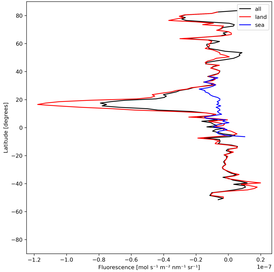
Figure 21: Zonal average of “Fluorescence” for 2023-08-30 to 2023-09-01.
