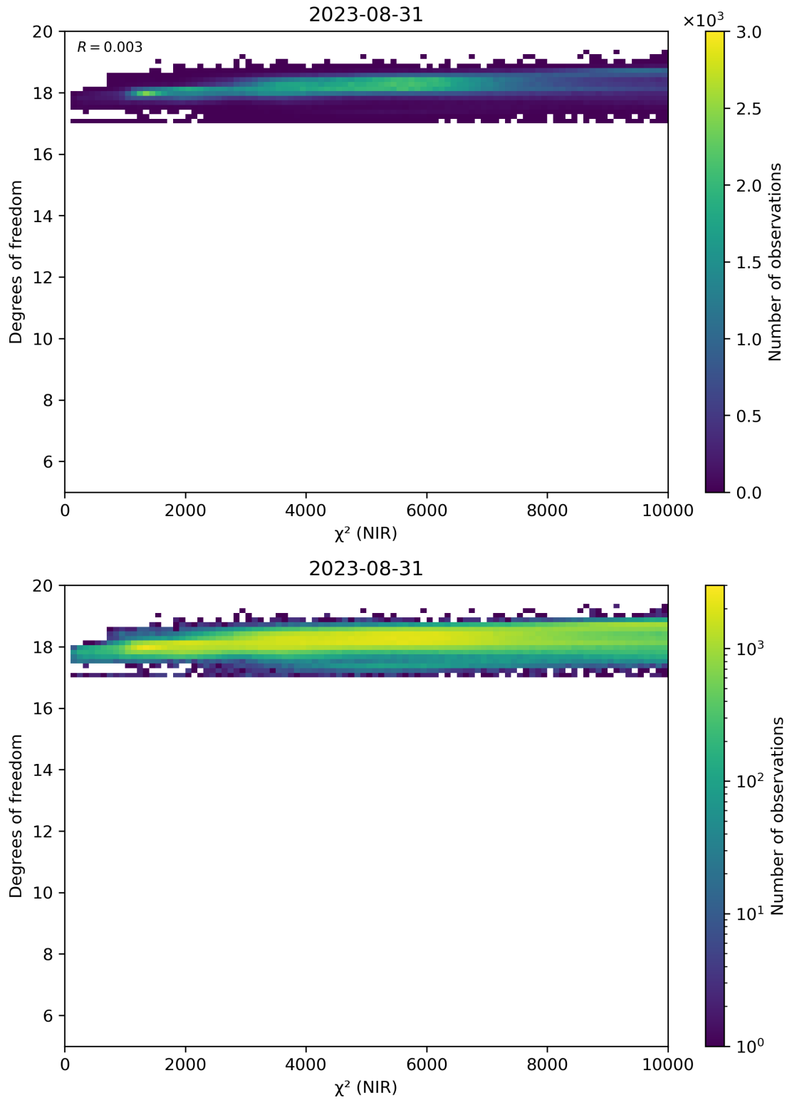
Figure 44: Scatter density plot of “ \chi^2 (NIR)” against “Degrees of freedom” for 2023-08-30 to 2023-09-01.
