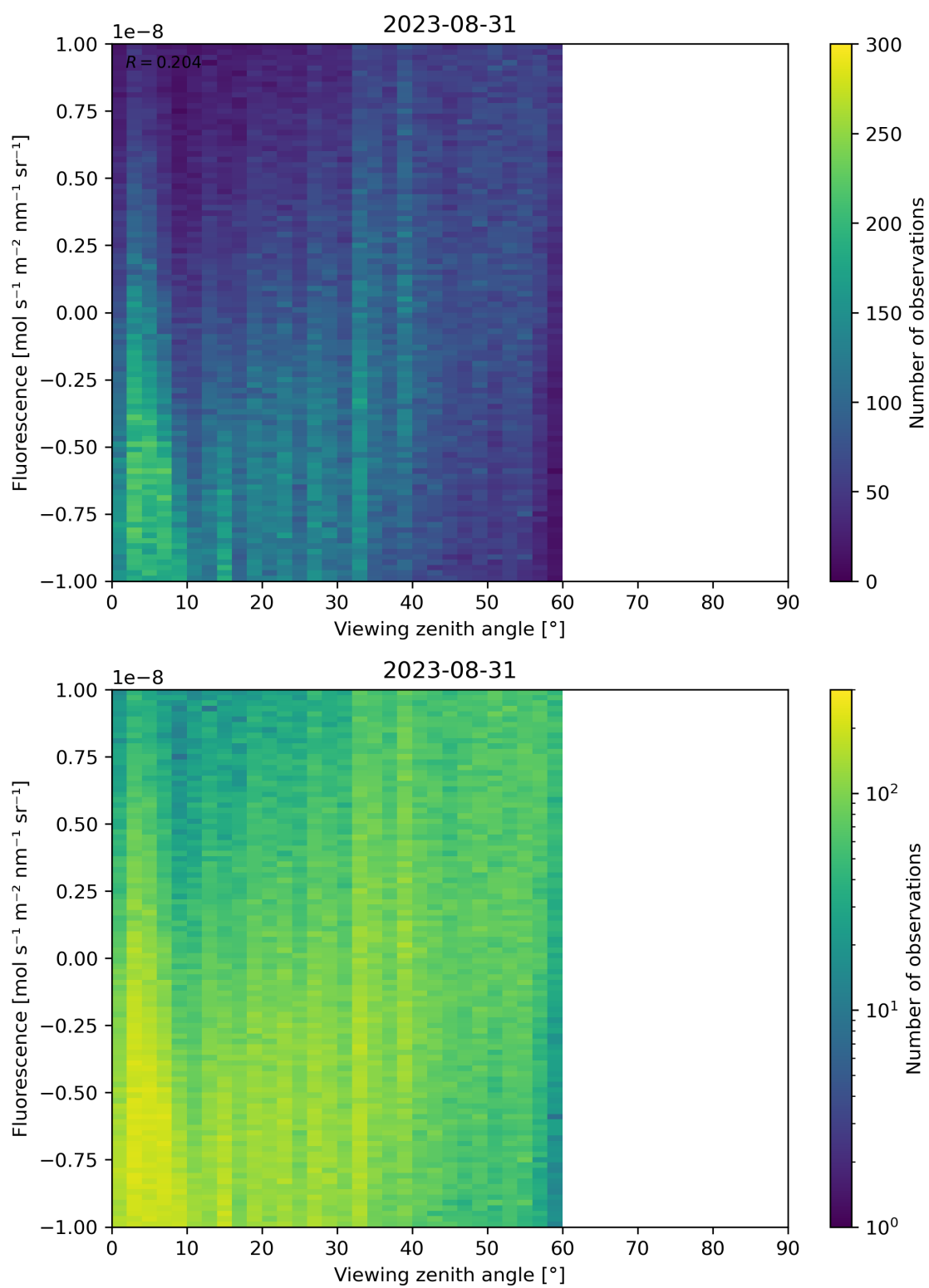
Figure 108: Scatter density plot of “Viewing zenith angle” against “Fluorescence” for 2023-08-30 to 2023-09-01.
