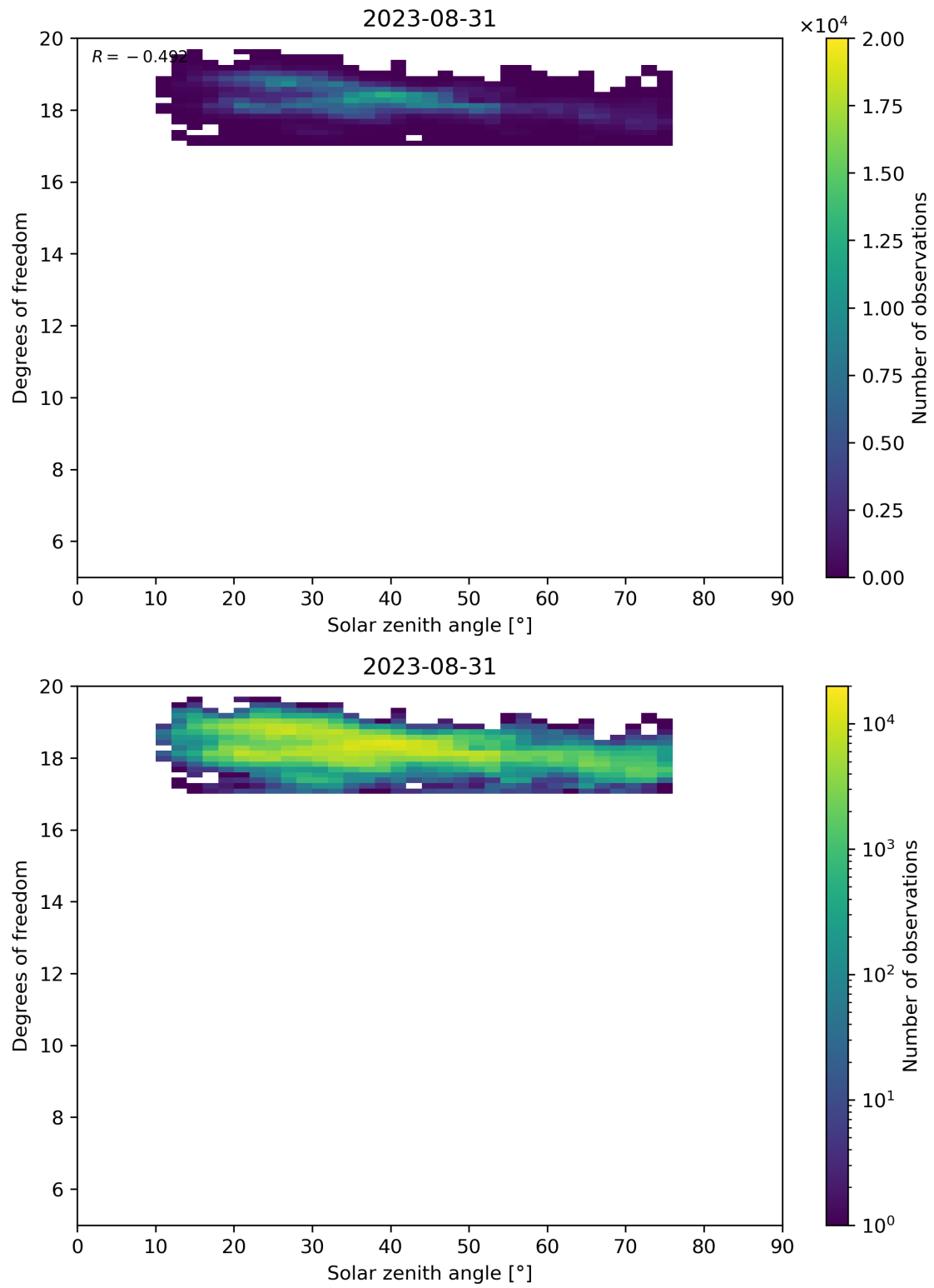
Figure 96: Scatter density plot of “Solar zenith angle” against “Degrees of freedom” for 2023-08-30 to 2023-09-01.
