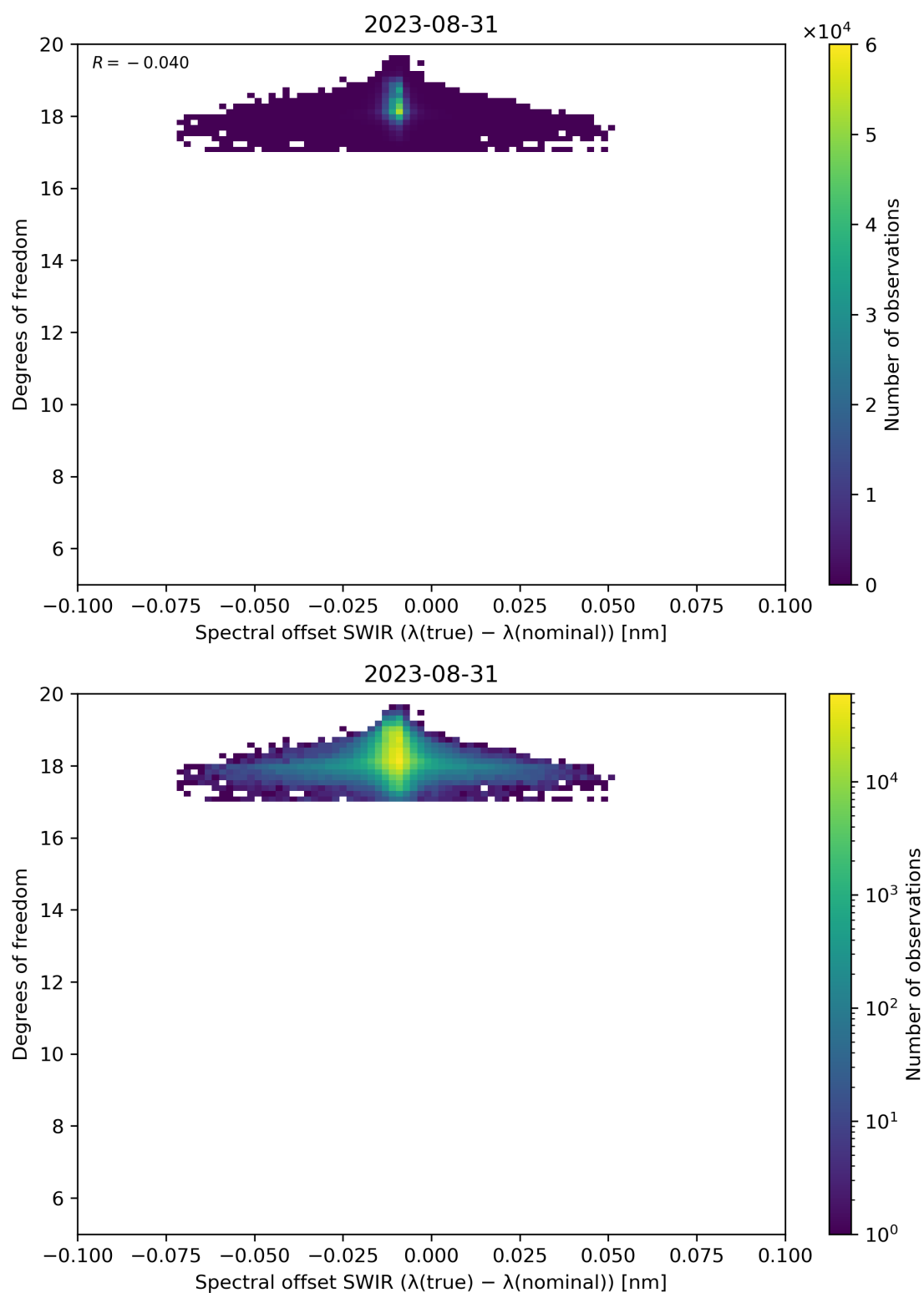
Figure 119: Scatter density plot of “Spectral offset SWIR ( \lambda(\text{true}) - \lambda(\text{nominal}) )” against “Degrees of freedom” for 2023-08-30 to 2023-09-01.
