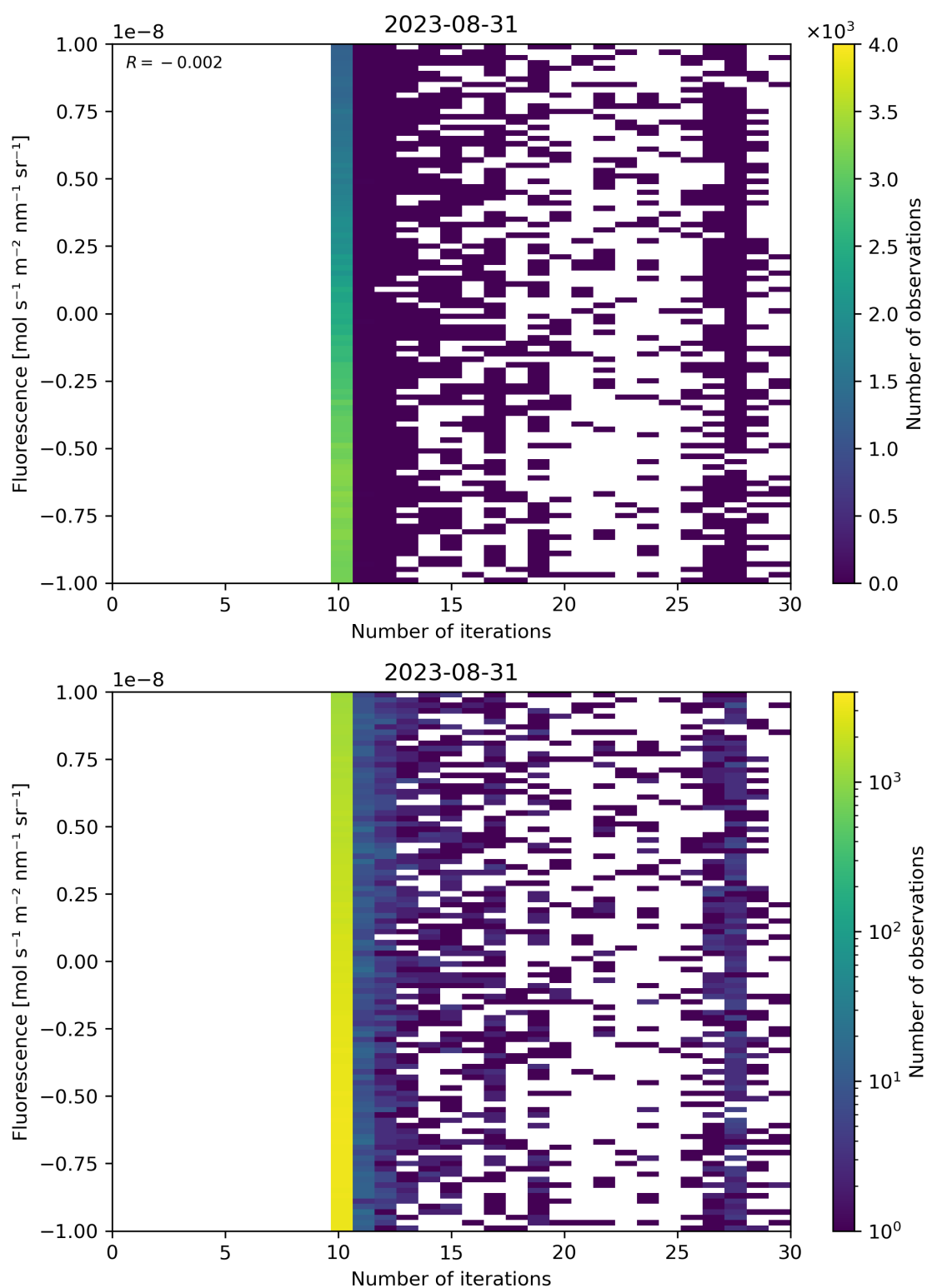
Figure 87: Scatter density plot of “Number of iterations” against “Fluorescence” for 2023-08-30 to 2023-09-01.
