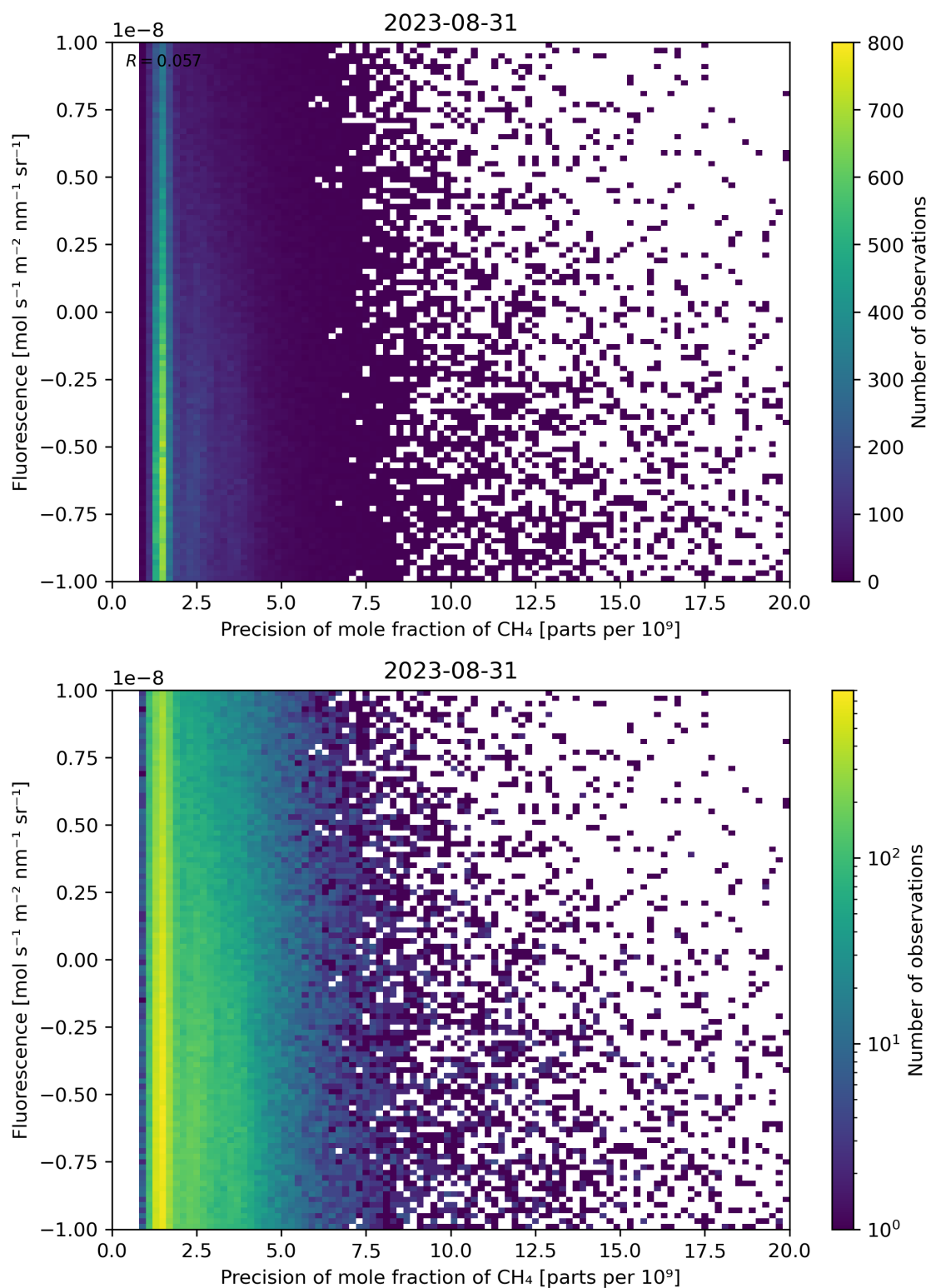
Figure 81: Scatter density plot of “Precision of mole fraction of \text{CH}_4 ” against “Fluorescence” for 2023-08-30 to 2023-09-01.
