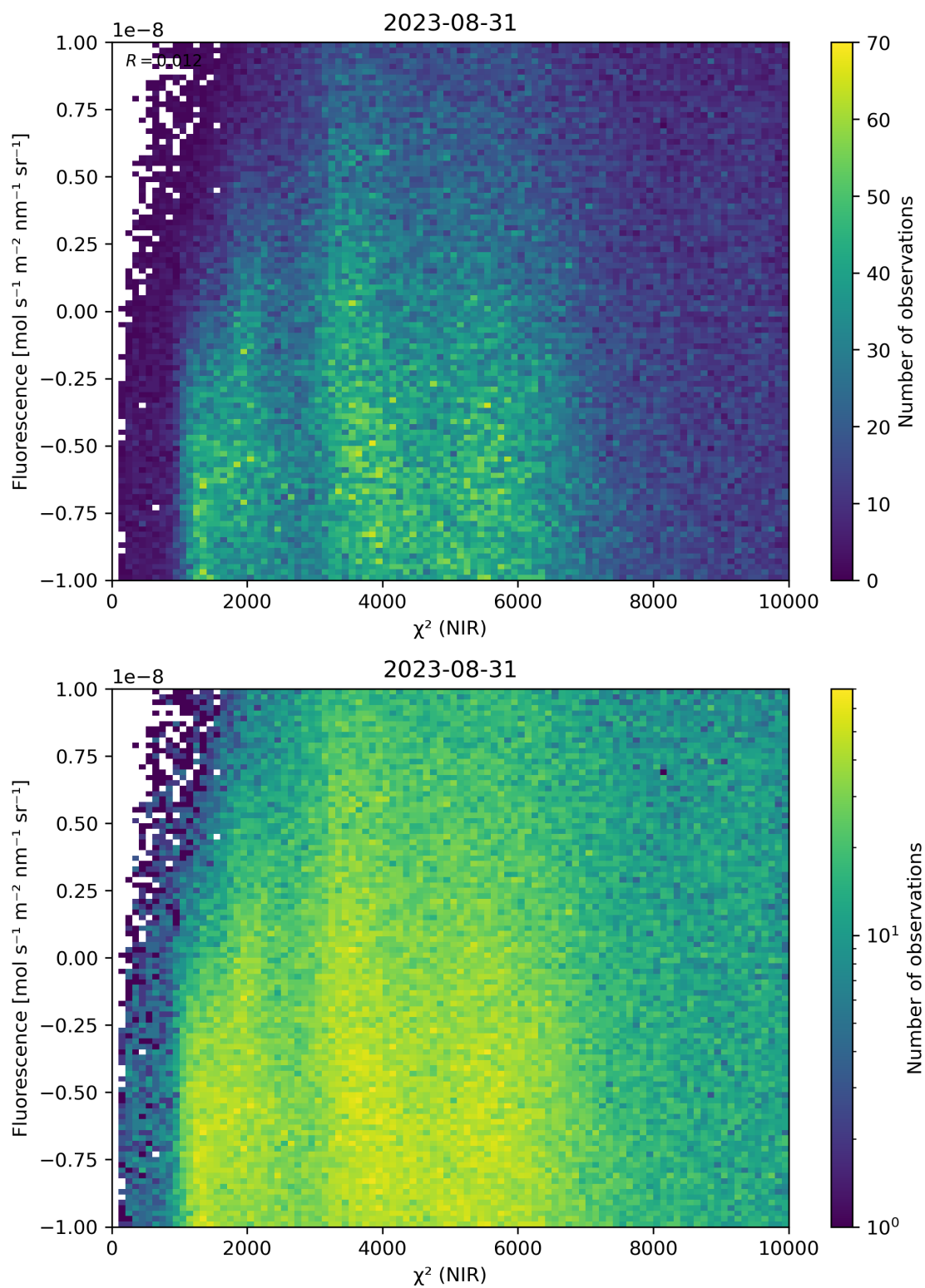
Figure 45: Scatter density plot of “ \chi^2 (NIR)” against “Fluorescence” for 2023-08-30 to 2023-09-01.
