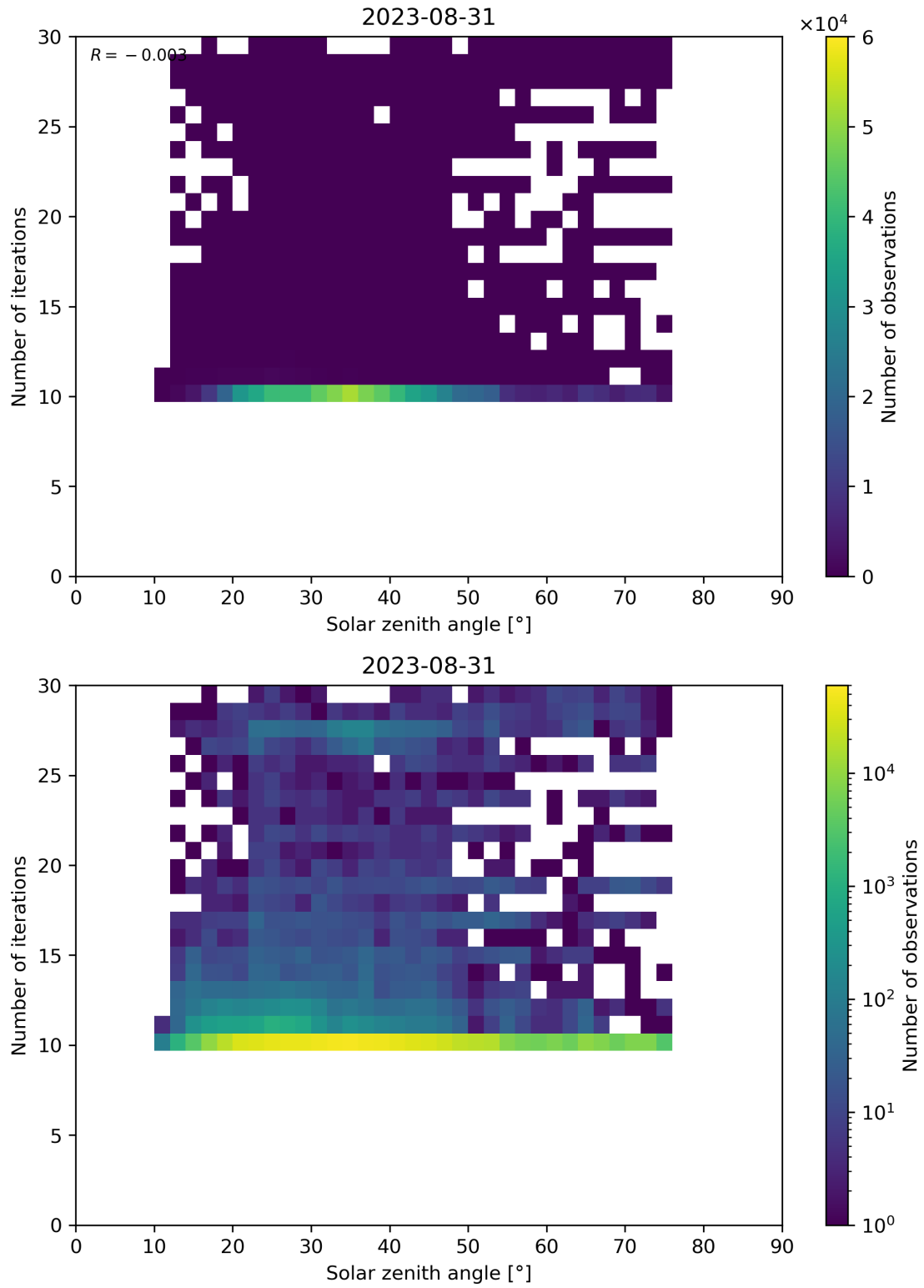
Figure 102: Scatter density plot of “Solar zenith angle” against “Number of iterations” for 2023-08-30 to 2023-09-01.
