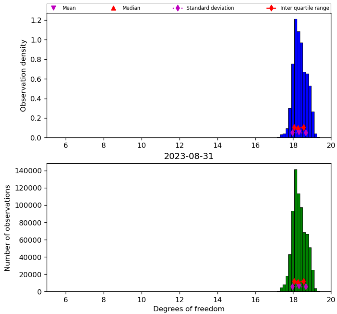
Figure 30: Histogram of “Degrees of freedom” for 2023-08-30 to 2023-09-01
