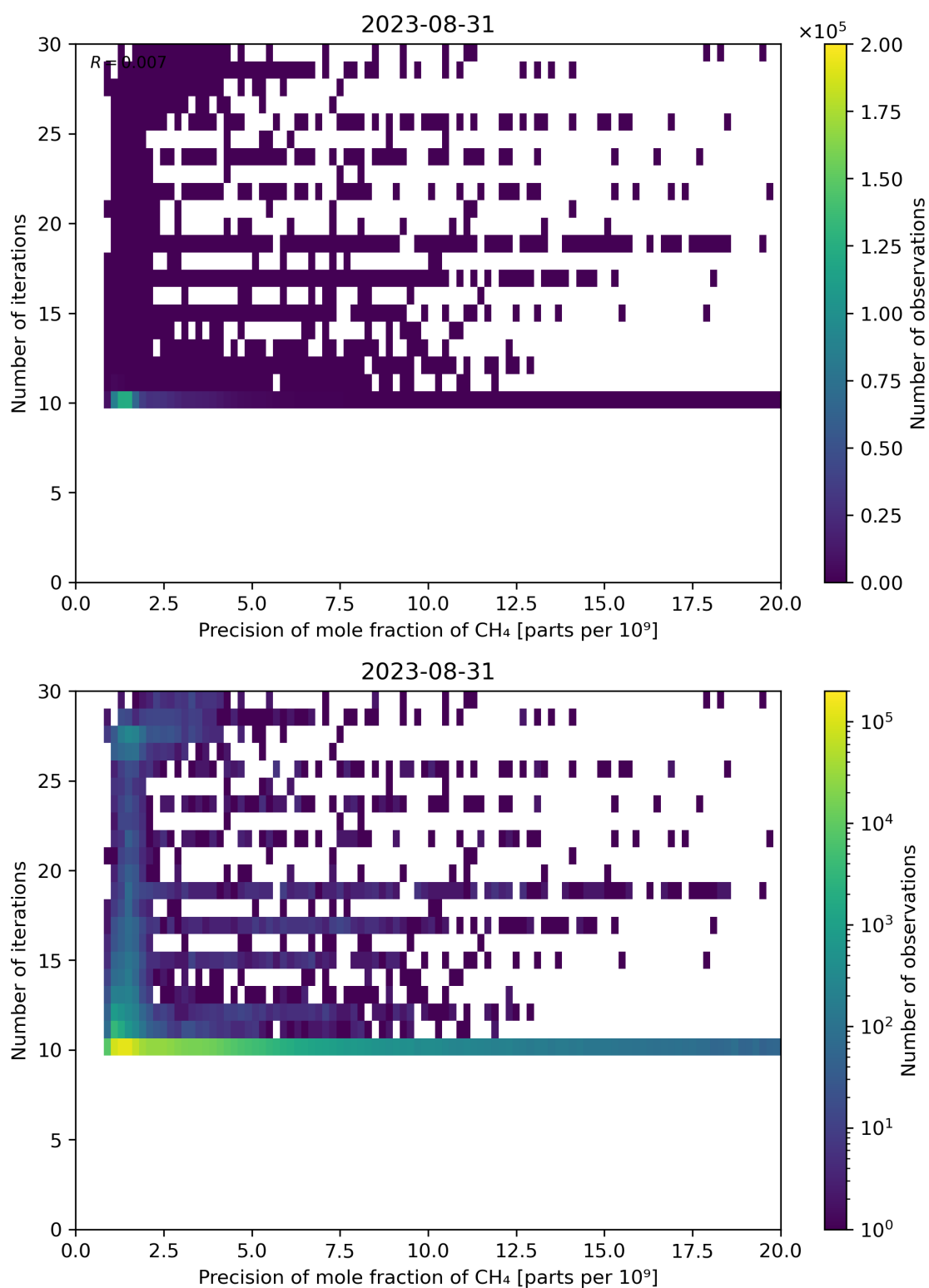
Figure 83: Scatter density plot of “Precision of mole fraction of CH 4 ” against “Number of iterations” for 2023-08-30 to 2023-09-01.
