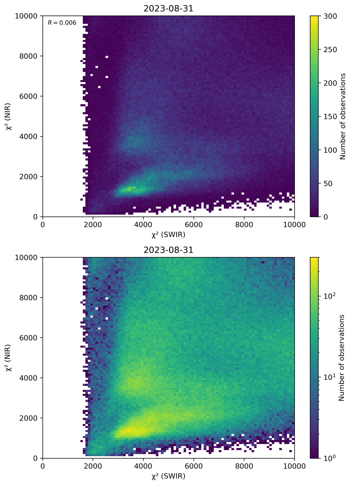
Figure 47: Scatter density plot of “ \chi^2 (SWIR)” against “ \chi^2 (NIR)” for 2023-08-30 to 2023-09-01.
