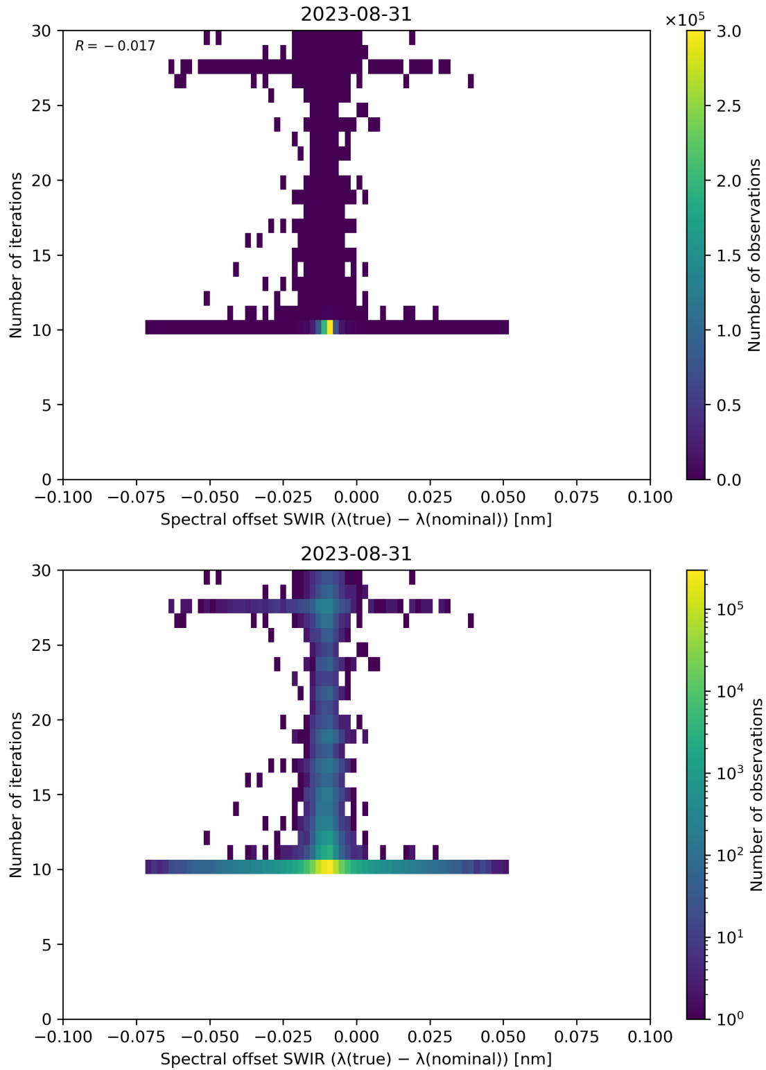
Figure 121: Scatter density plot of “Spectral offset SWIR ( \lambda(\text{true}) - \lambda(\text{nominal}) )” against “Number of iterations” for 2023-08-30 to 2023-09-01.
