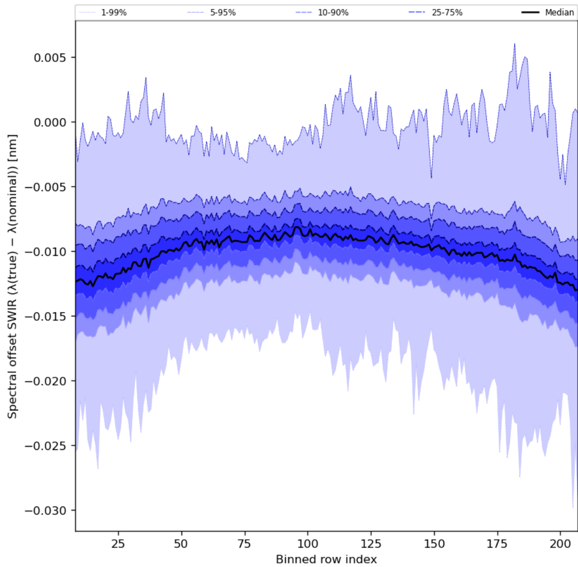
Figure 38: Along track statistics of “Spectral offset SWIR ( \lambda(\text{true}) - \lambda(\text{nominal}) )” for 2023-08-30 to 2023-09-01
