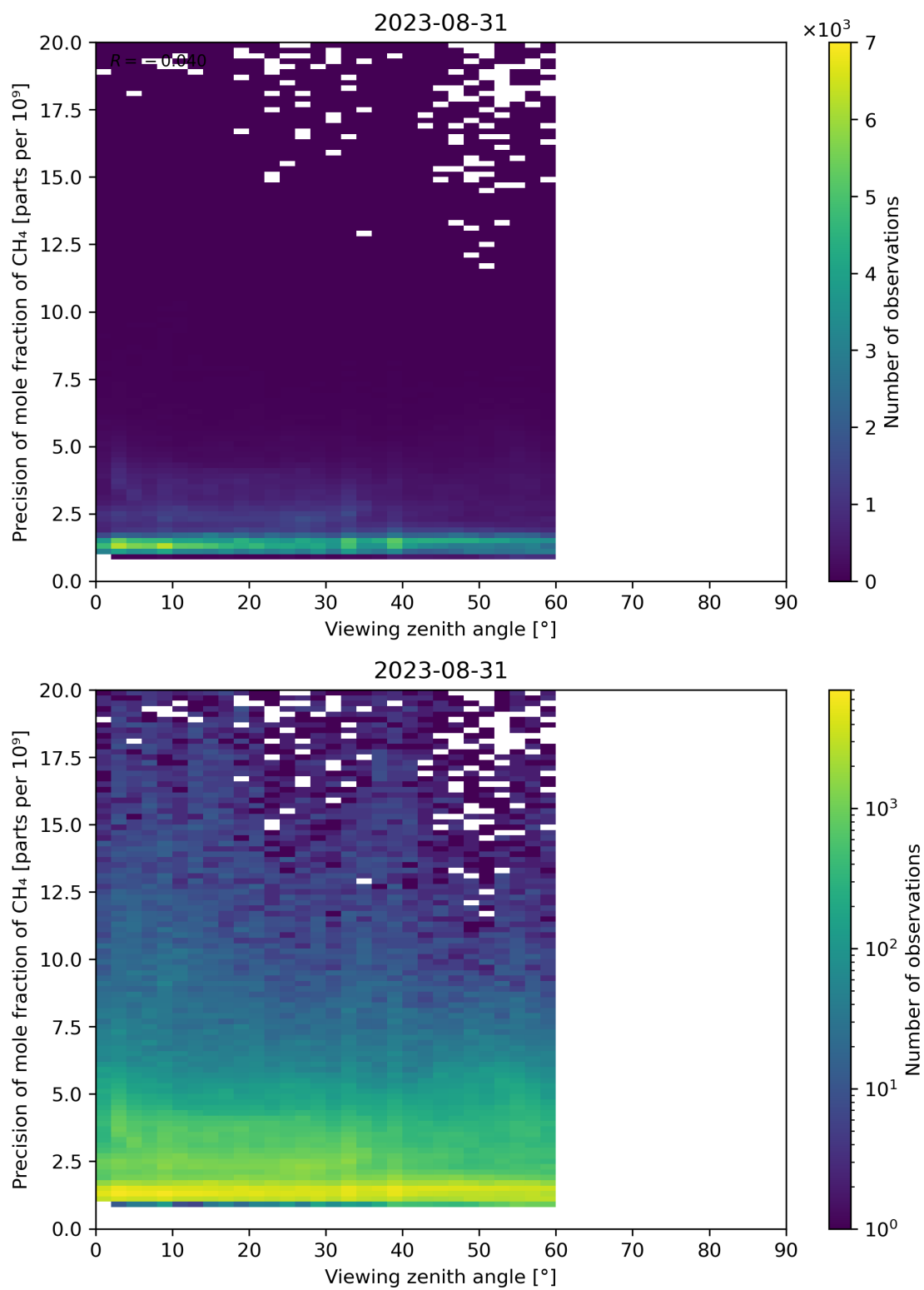
Figure 112: Scatter density plot of “Viewing zenith angle” against “Precision of mole fraction of CH 4 ” for 2023-08-30 to 2023-09-01.
