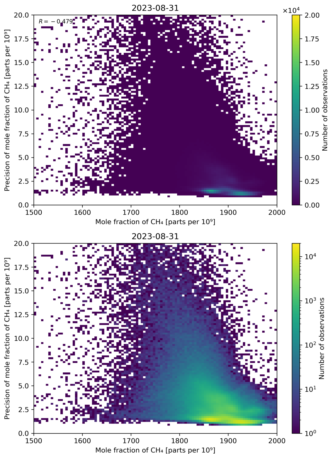
Figure 75: Scatter density plot of “Mole fraction of CH 4 ” against “Precision of mole fraction of CH 4 ” for 2023-08-30 to 2023-09-01.
