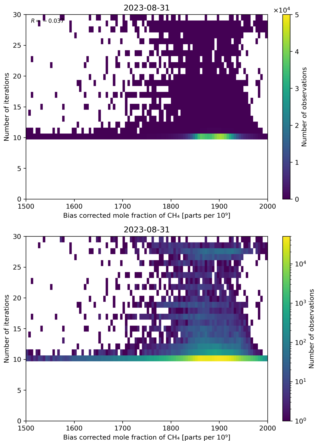
Figure 67: Scatter density plot of “Bias corrected mole fraction of CH 4 ” against “Number of iterations” for 2023-08-30 to 2023-09-01.
