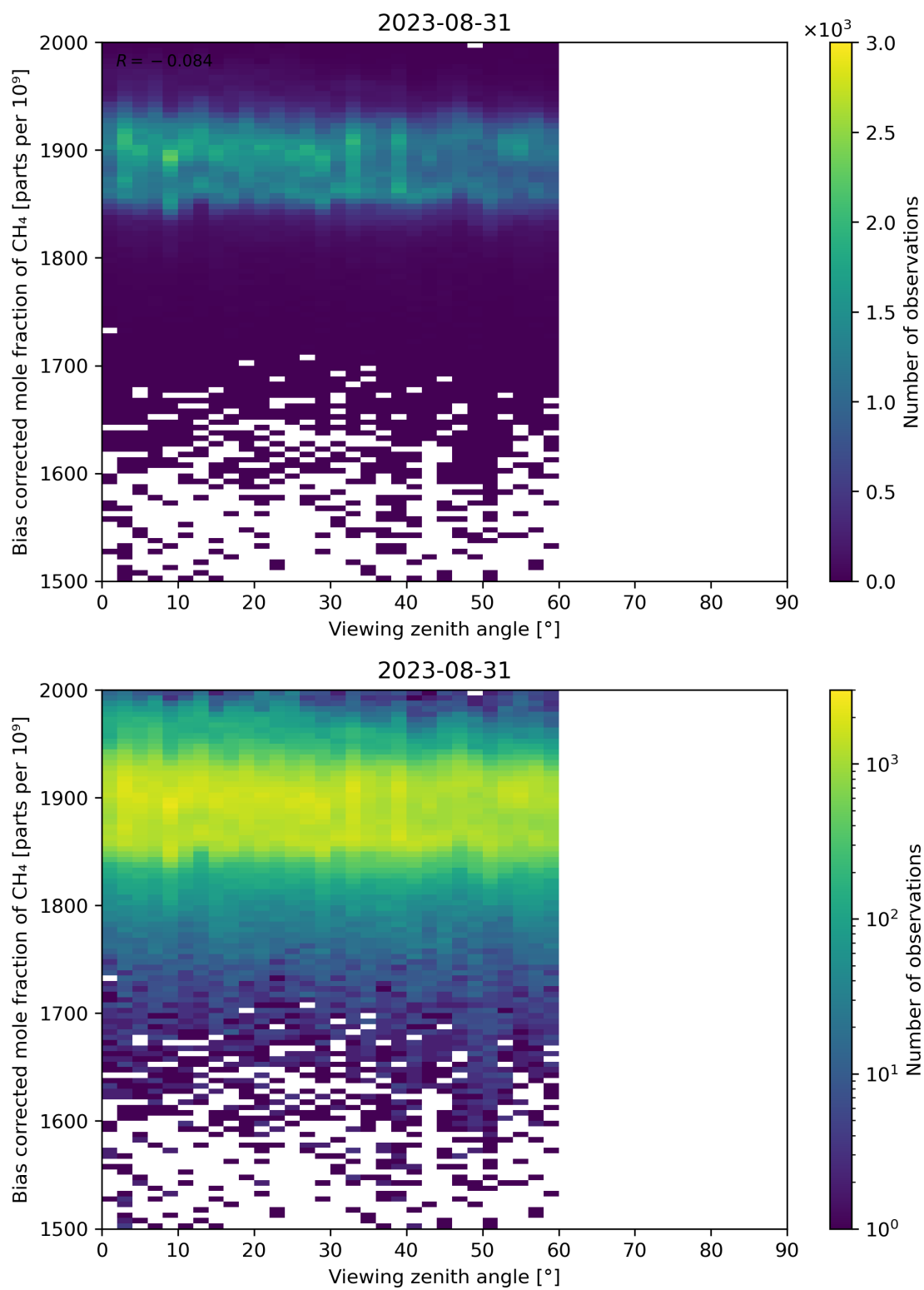
Figure 111: Scatter density plot of “Viewing zenith angle” against “Bias corrected mole fraction of CH 4 ” for 2023-08-30 to 2023-09-01.
