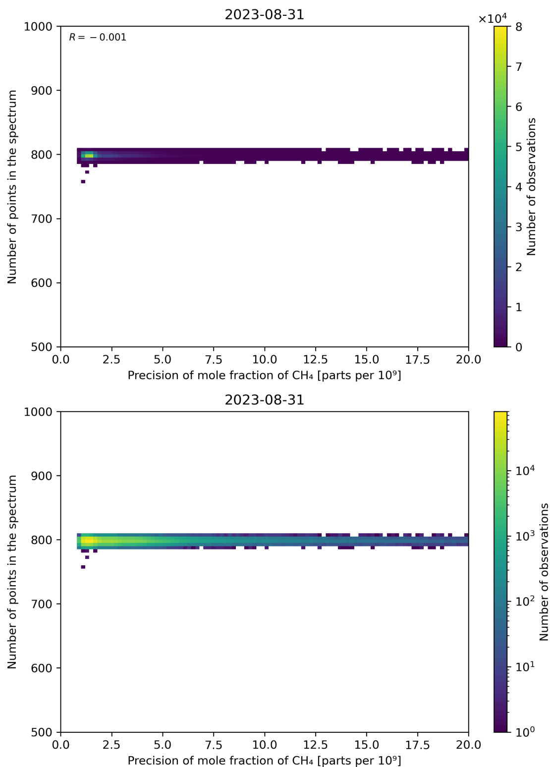
Figure 84: Scatter density plot of “Precision of mole fraction of CH 4 ” against “Number of points in the spectrum” for 2023-08-30 to 2023-09-01.
