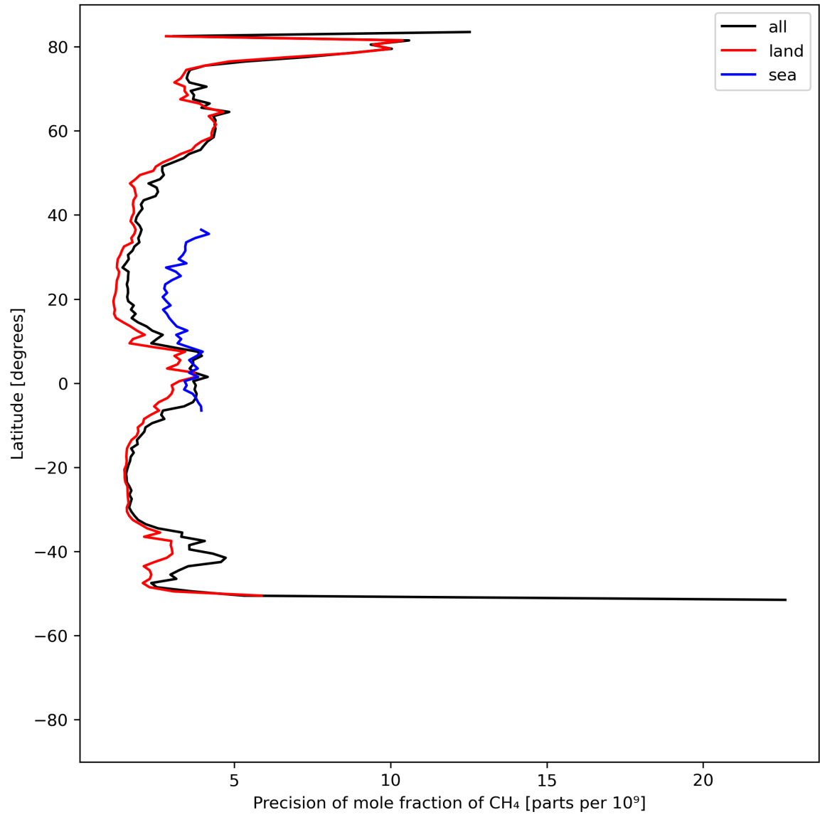
Figure 13: Zonal average of “Precision of mole fraction of CH 4 ” for 2023-08-30 to 2023-09-01.
