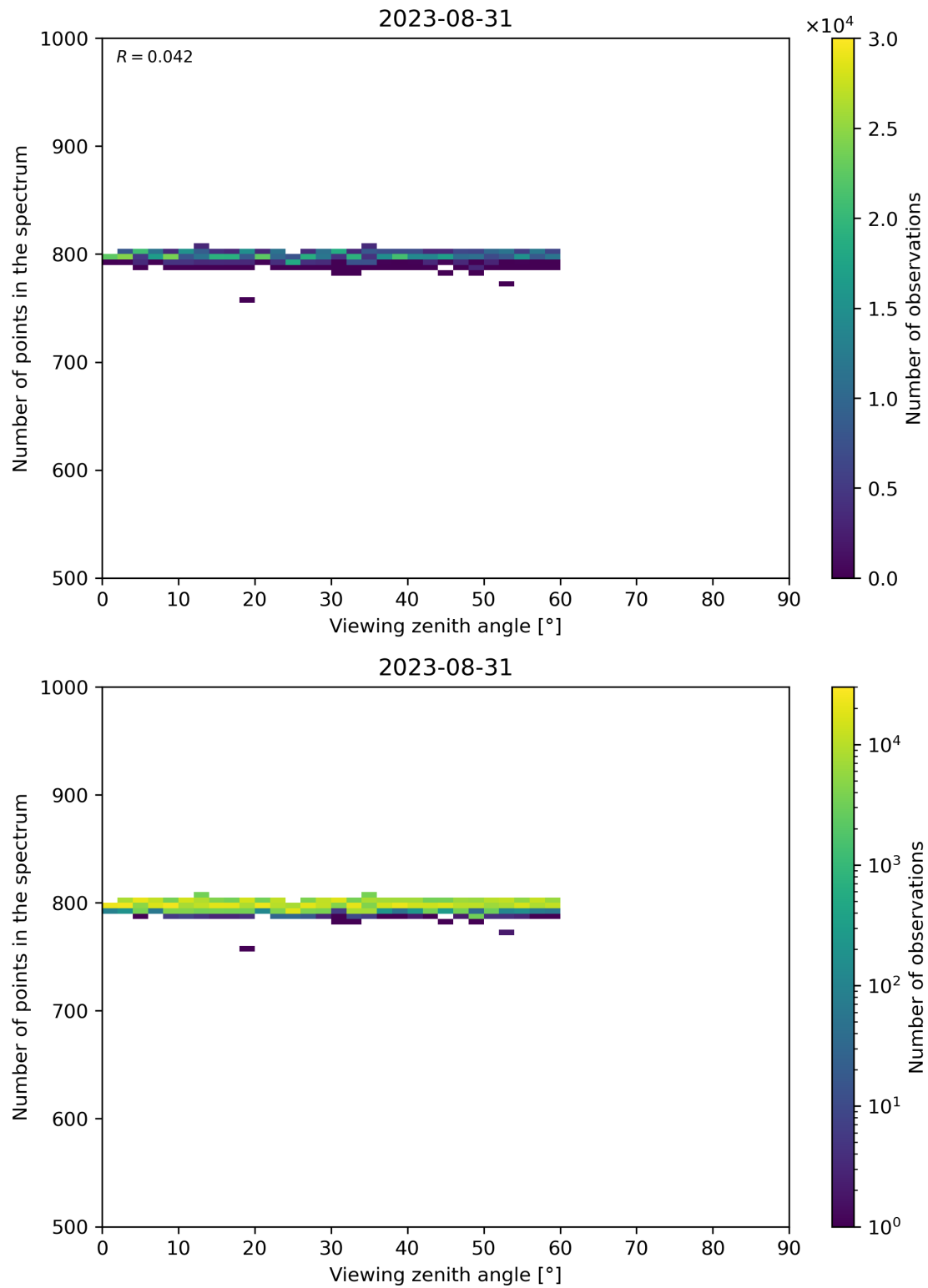
Figure 114: Scatter density plot of “Viewing zenith angle” against “Number of points in the spectrum” for 2023-08-30 to 2023-09-01.
