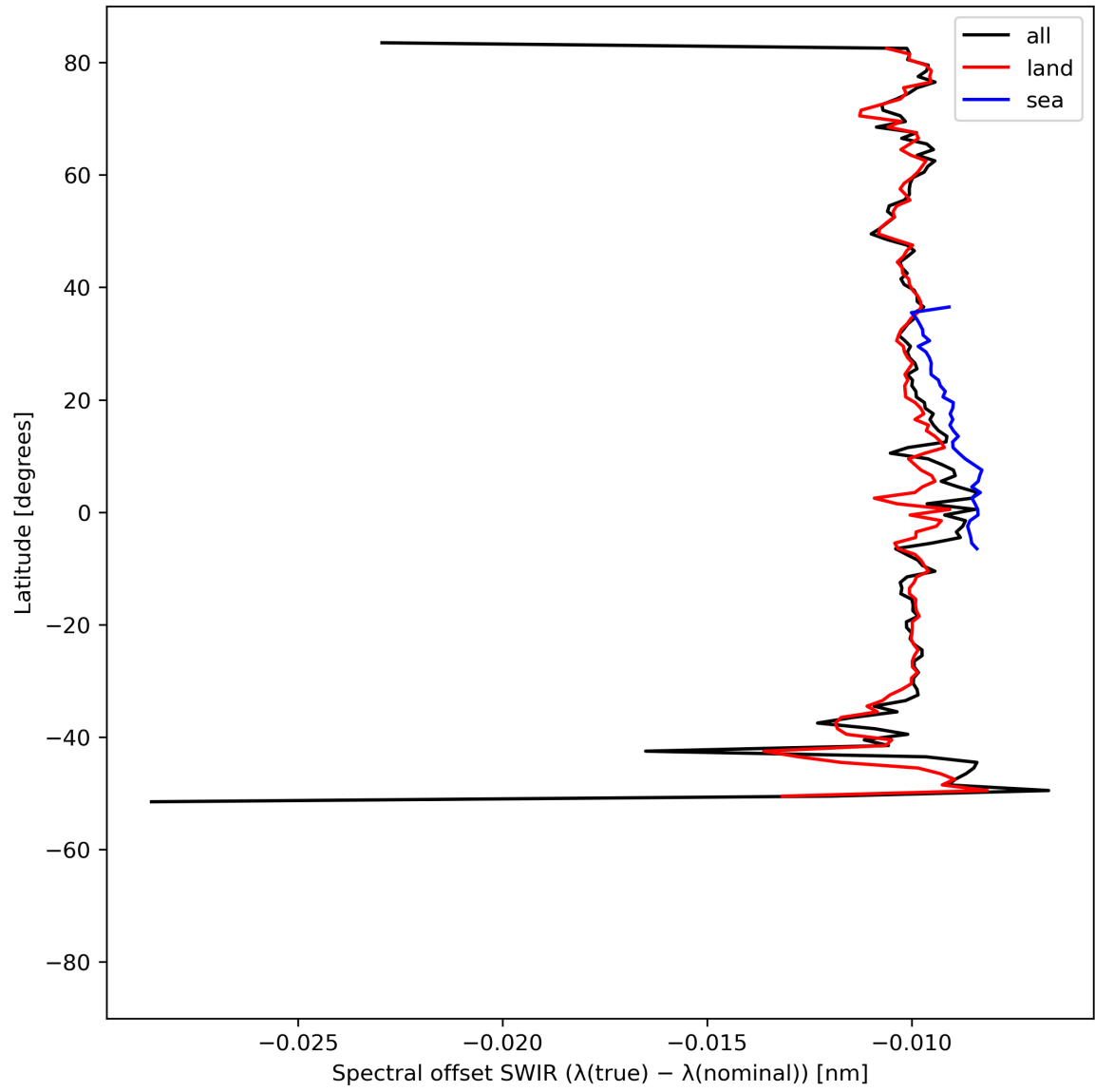
Figure 16: Zonal average of “Spectral offset SWIR ( \lambda(\text{true}) - \lambda(\text{nominal}) )” for 2023-08-30 to 2023-09-01.
