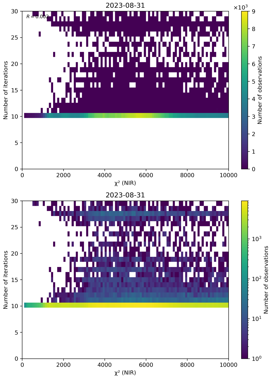
Figure 46: Scatter density plot of “ \chi^2 (NIR)” against “Number of iterations” for 2023-08-30 to 2023-09-01.
