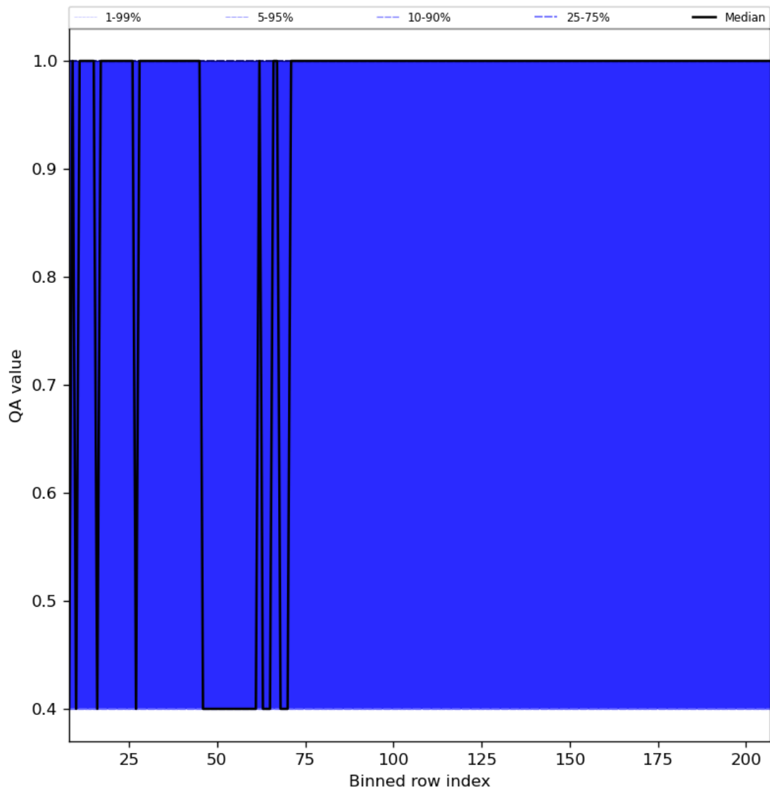
Figure 33: Along track statistics of “QA value” for 2023-08-30 to 2023-09-01
