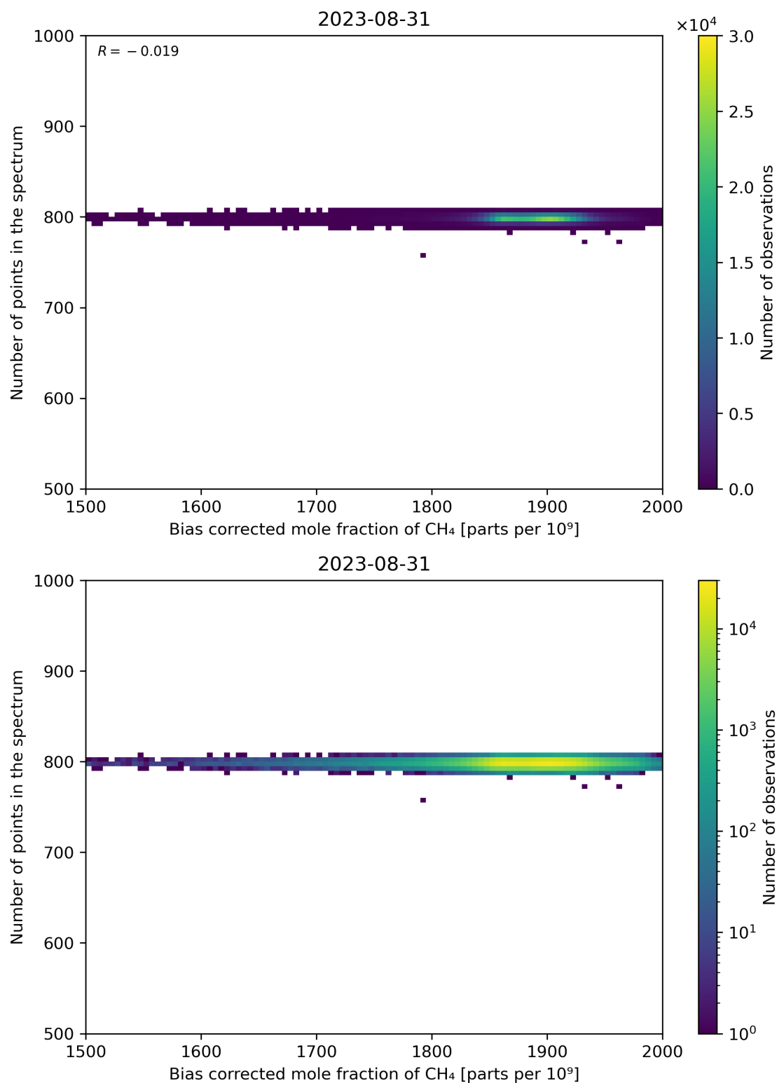
Figure 68: Scatter density plot of “Bias corrected mole fraction of CH 4 ” against “Number of points in the spectrum” for 2023-08-30 to 2023-09-01.
