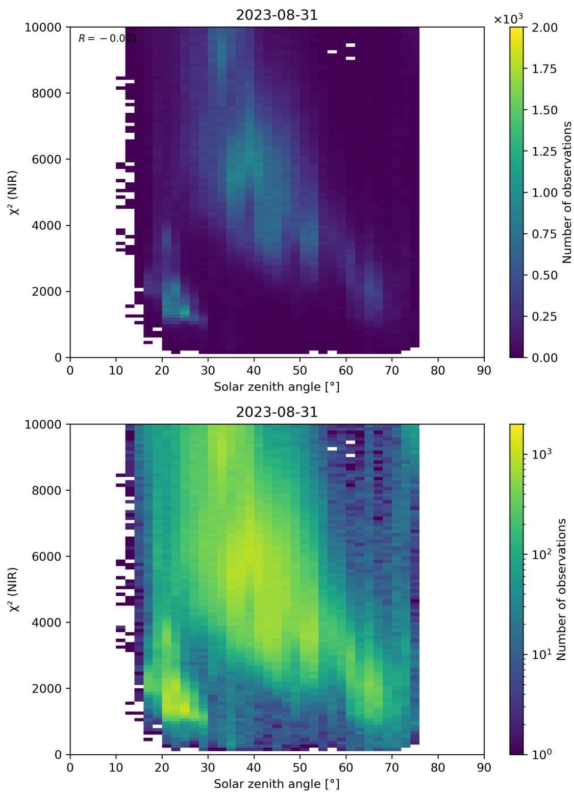
Figure 94: Scatter density plot of “Solar zenith angle” against “ \chi^2 (NIR)” for 2023-08-30 to 2023-09-01.
