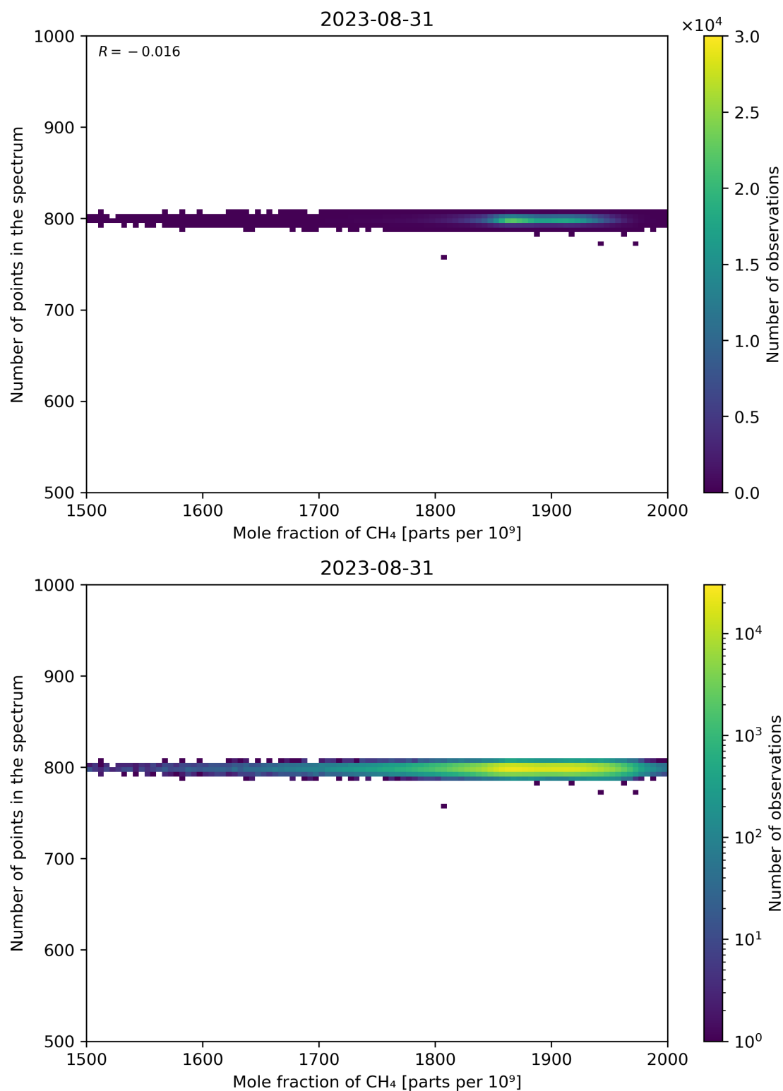
Figure 77: Scatter density plot of “Mole fraction of CH 4 ” against “Number of points in the spectrum” for 2023-08-30 to 2023-09-01.
