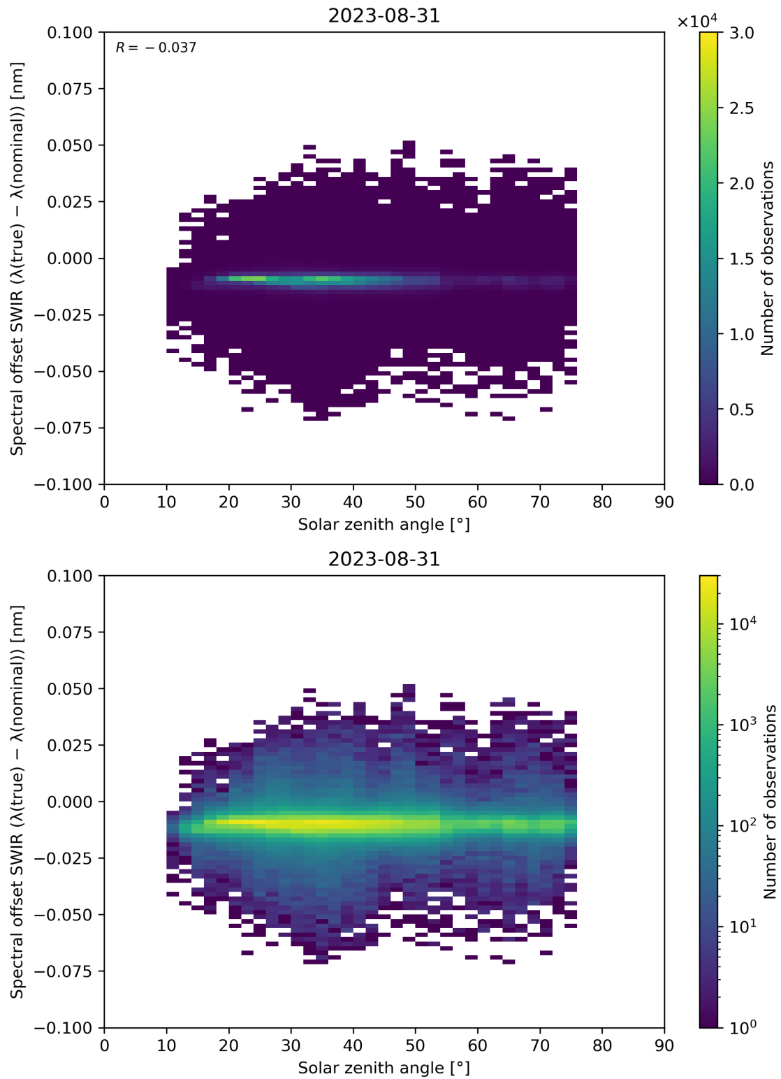
Figure 104: Scatter density plot of “Solar zenith angle” against “Spectral offset SWIR ( \lambda(\text{true}) - \lambda(\text{nominal}) )” for 2023-08-30 to 2023-09-01.
