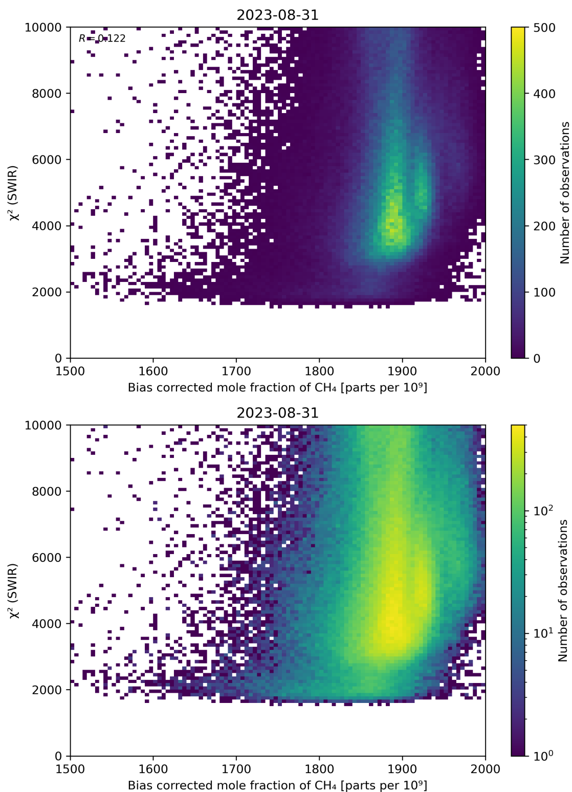
Figure 64: Scatter density plot of “Bias corrected mole fraction of \text{CH}_4 ” against “ \chi^2 (SWIR)” for 2023-08-30 to 2023-09-01.
