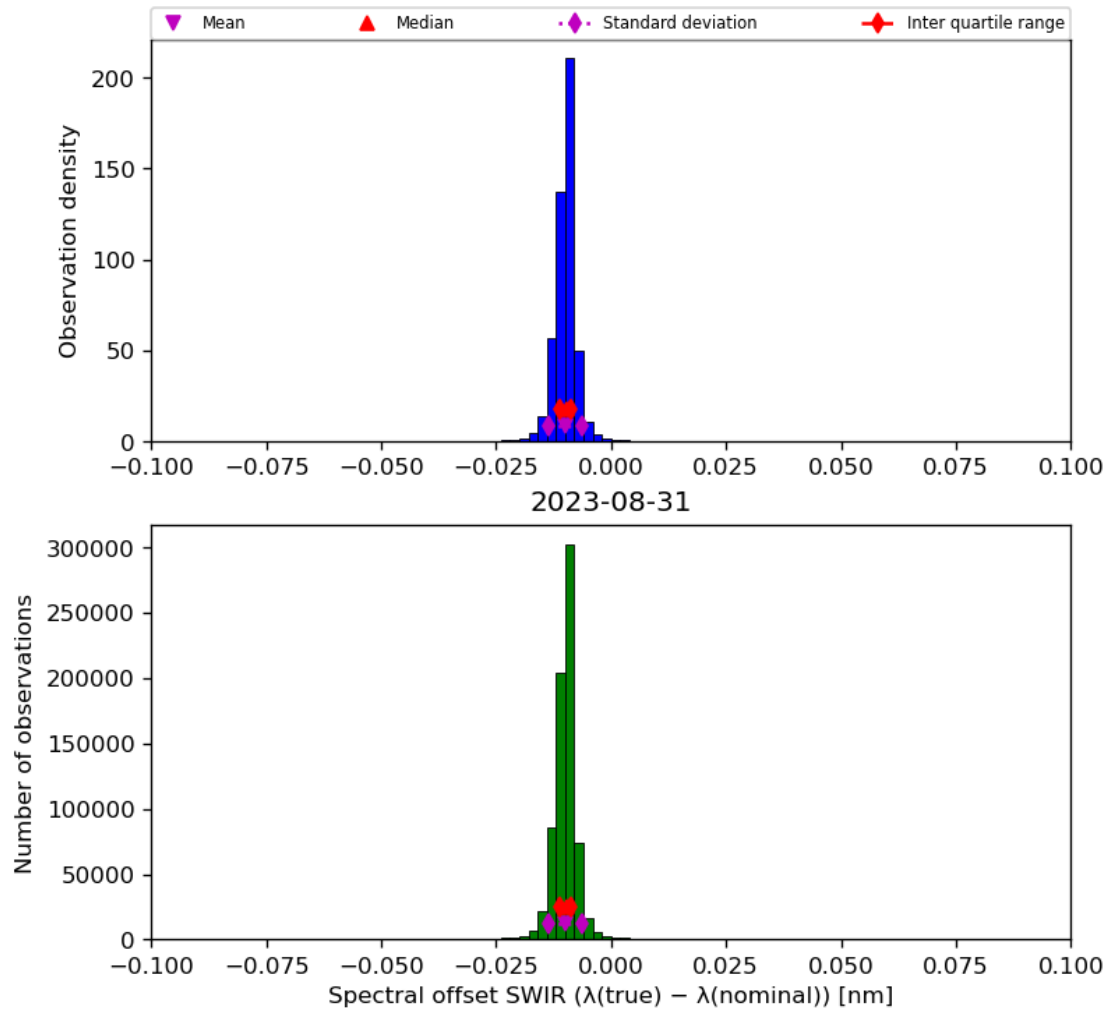
Figure 27: Histogram of “Spectral offset SWIR ( \lambda(\text{true}) - \lambda(\text{nominal}) )” for 2023-08-30 to 2023-09-01
