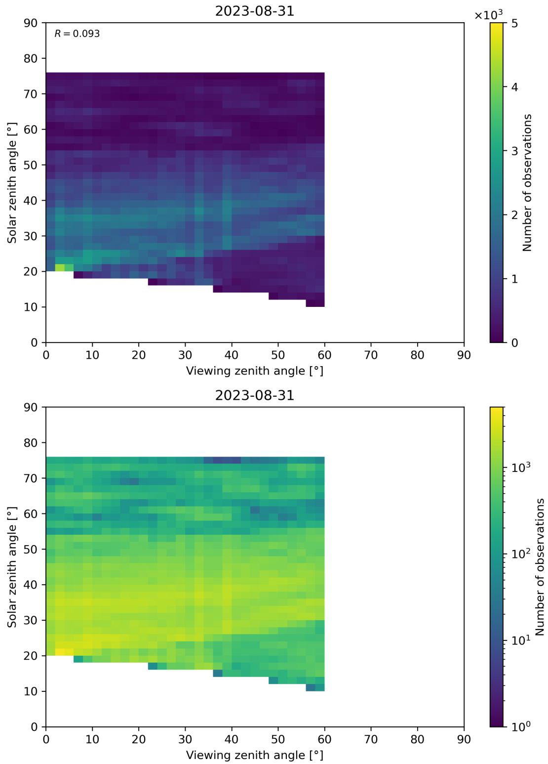
Figure 115: Scatter density plot of “Viewing zenith angle” against “Solar zenith angle” for 2023-08-30 to 2023-09-01.
