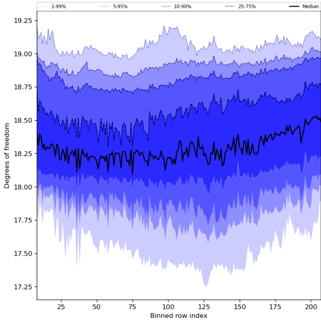
Figure 41: Along track statistics of “Degrees of freedom” for 2023-08-30 to 2023-09-01
