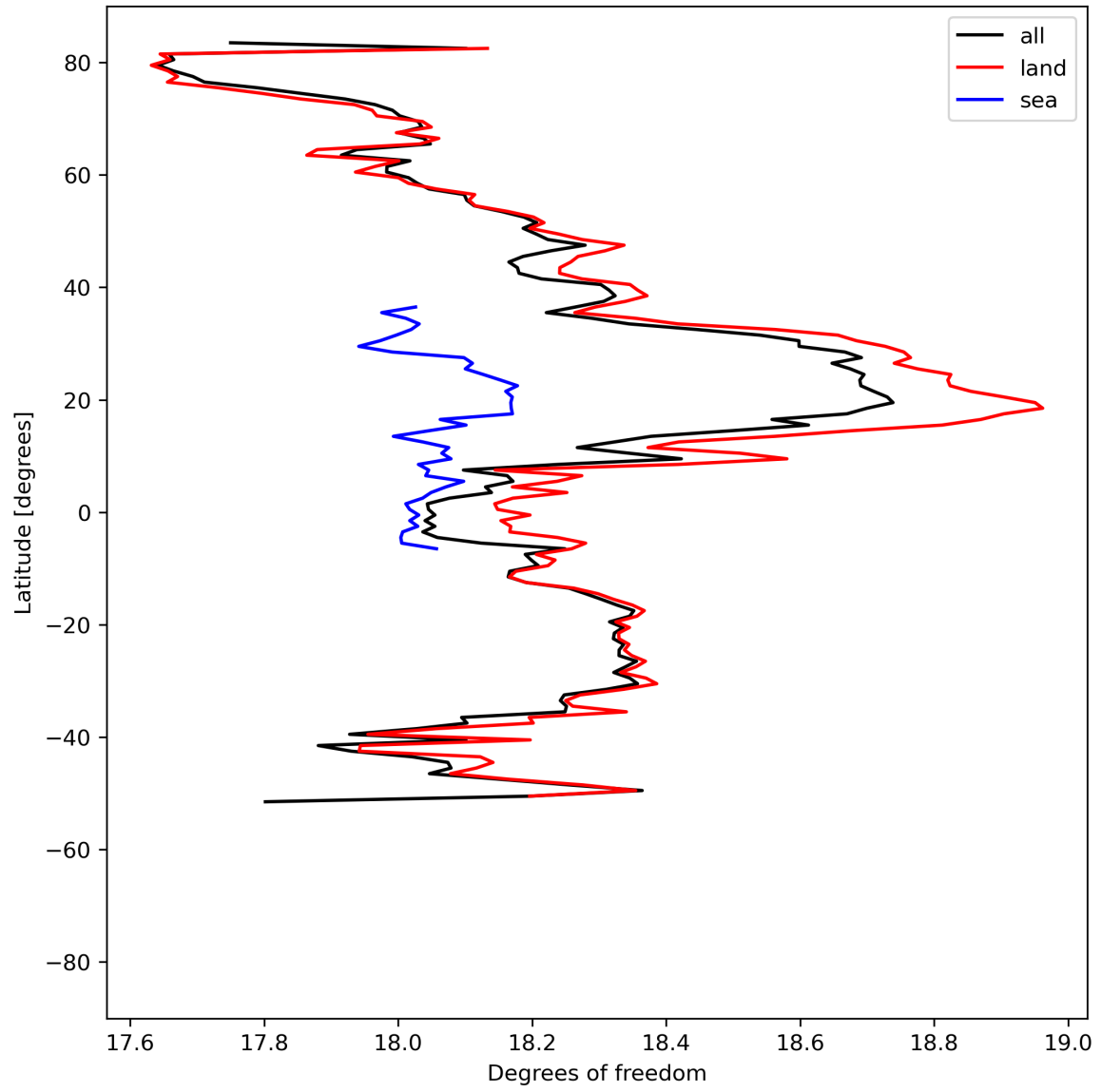
Figure 19: Zonal average of “Degrees of freedom” for 2023-08-30 to 2023-09-01.
