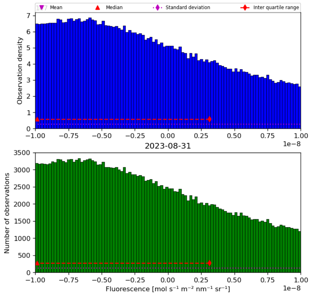
Figure 32: Histogram of “Fluorescence” for 2023-08-30 to 2023-09-01
