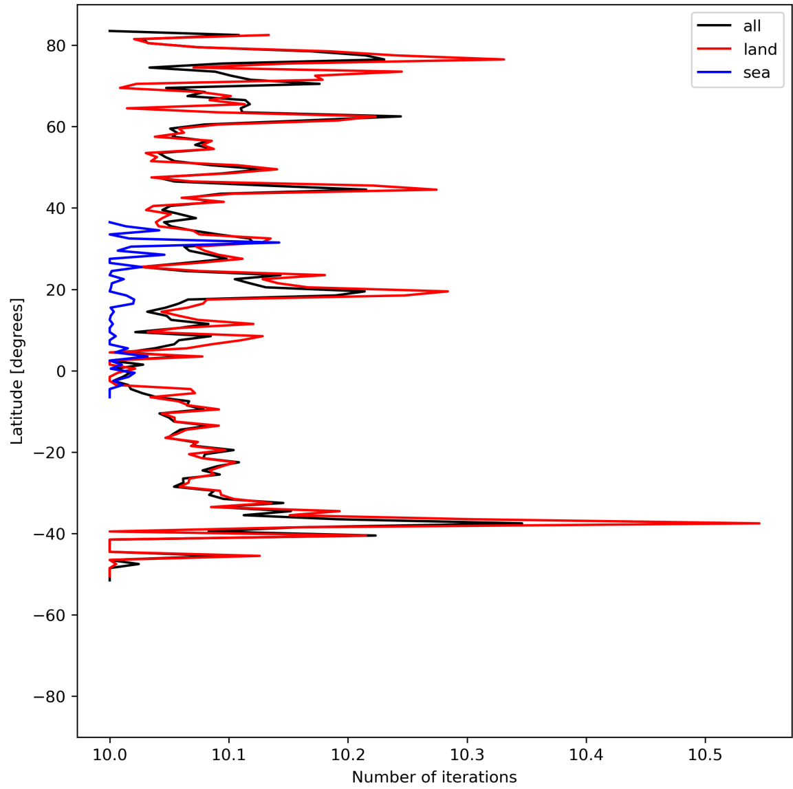
Figure 20: Zonal average of “Number of iterations” for 2023-08-30 to 2023-09-01.
