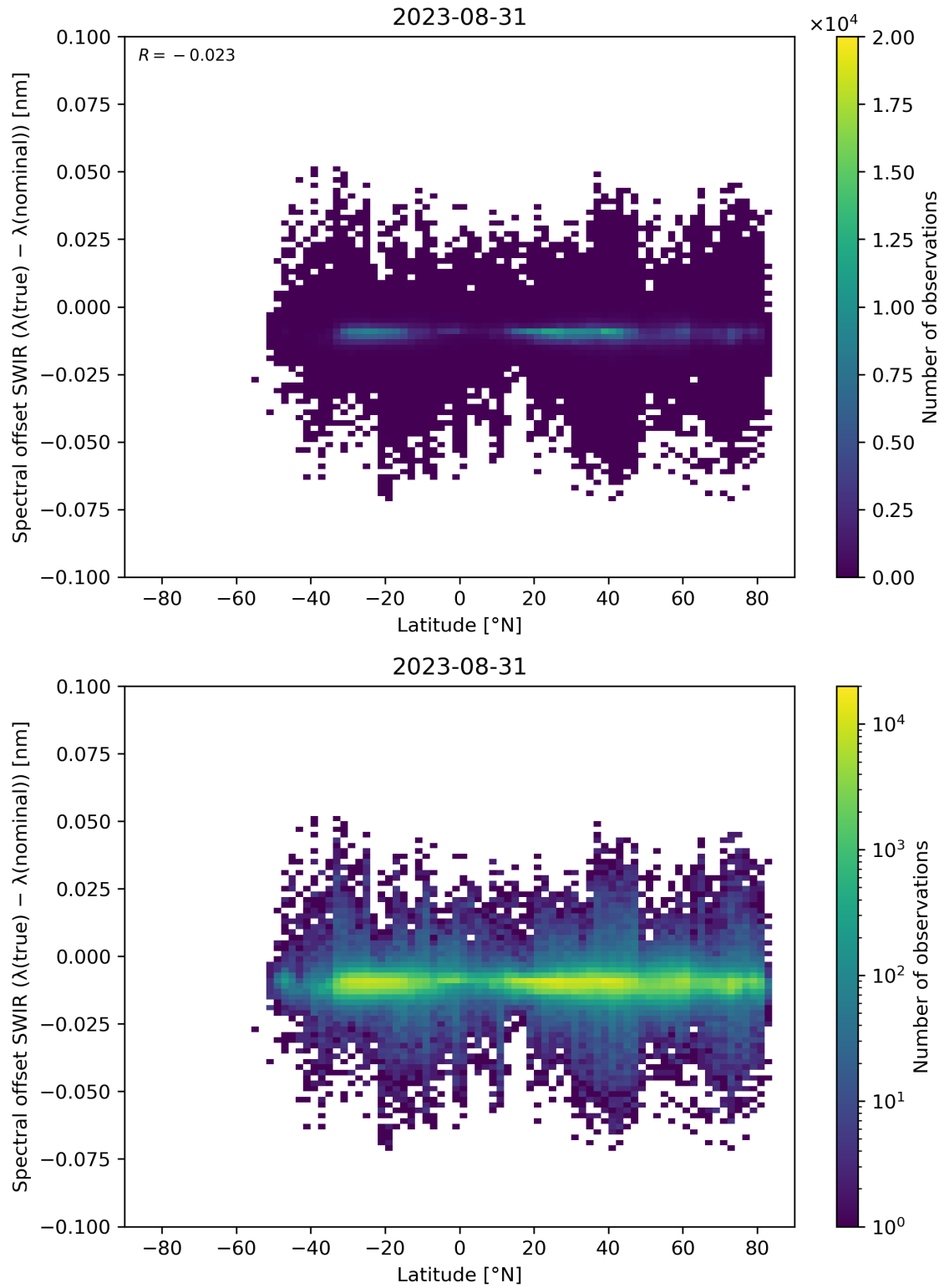
Figure 62: Scatter density plot of “Latitude” against “Spectral offset SWIR ( \lambda(\text{true}) - \lambda(\text{nominal}) )” for 2023-08-30 to 2023-09-01.
