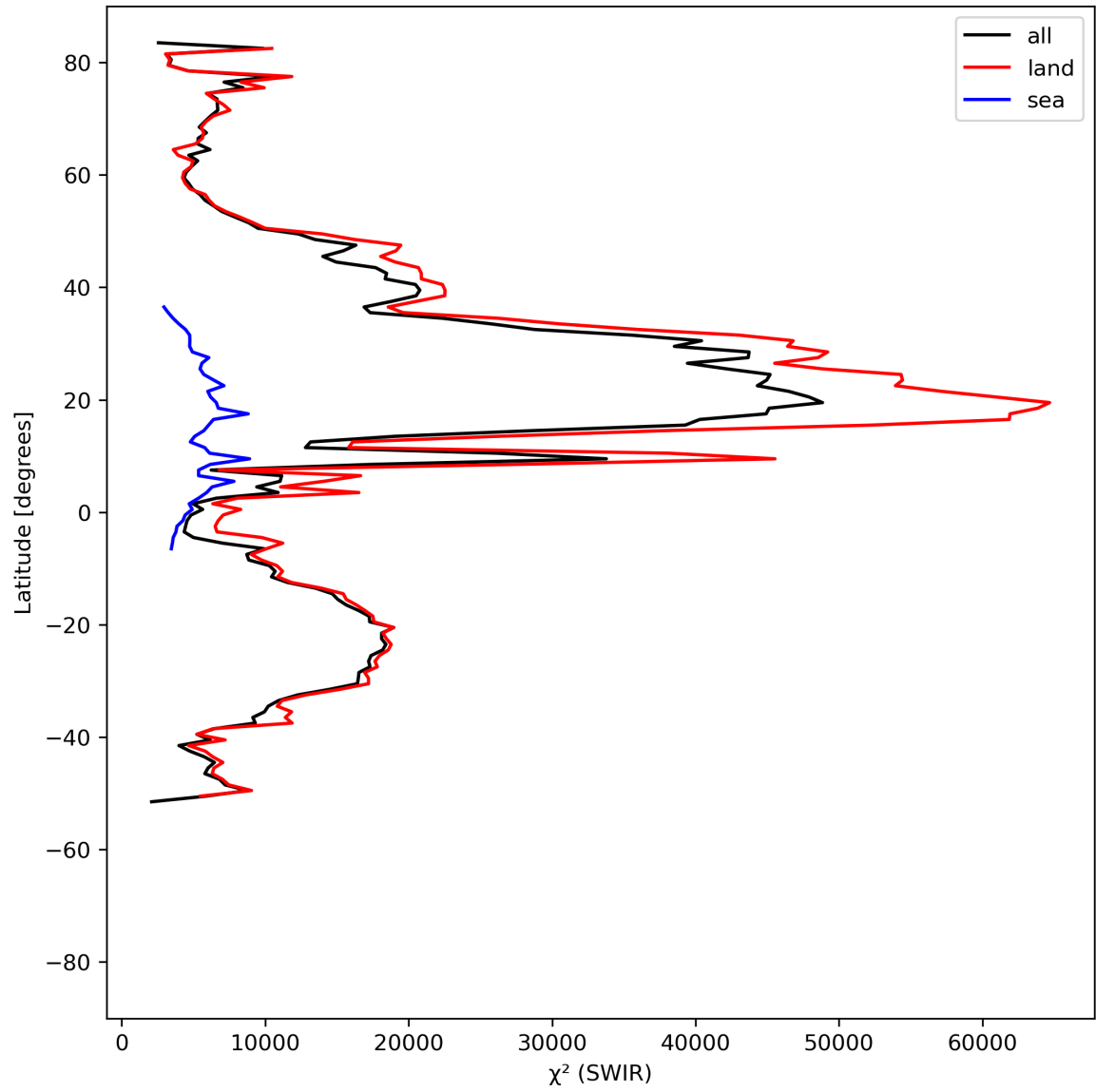
Figure 17: Zonal average of “ \chi^2 (SWIR)” for 2023-08-30 to 2023-09-01.
