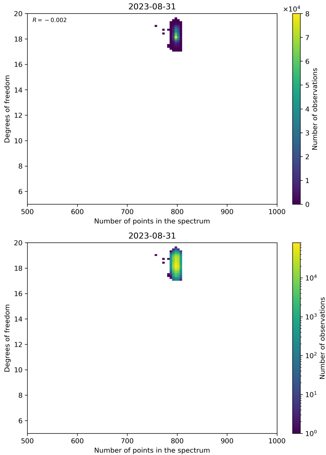
Figure 90: Scatter density plot of “Number of points in the spectrum” against “Degrees of freedom” for 2023-08-30 to 2023-09-01.
