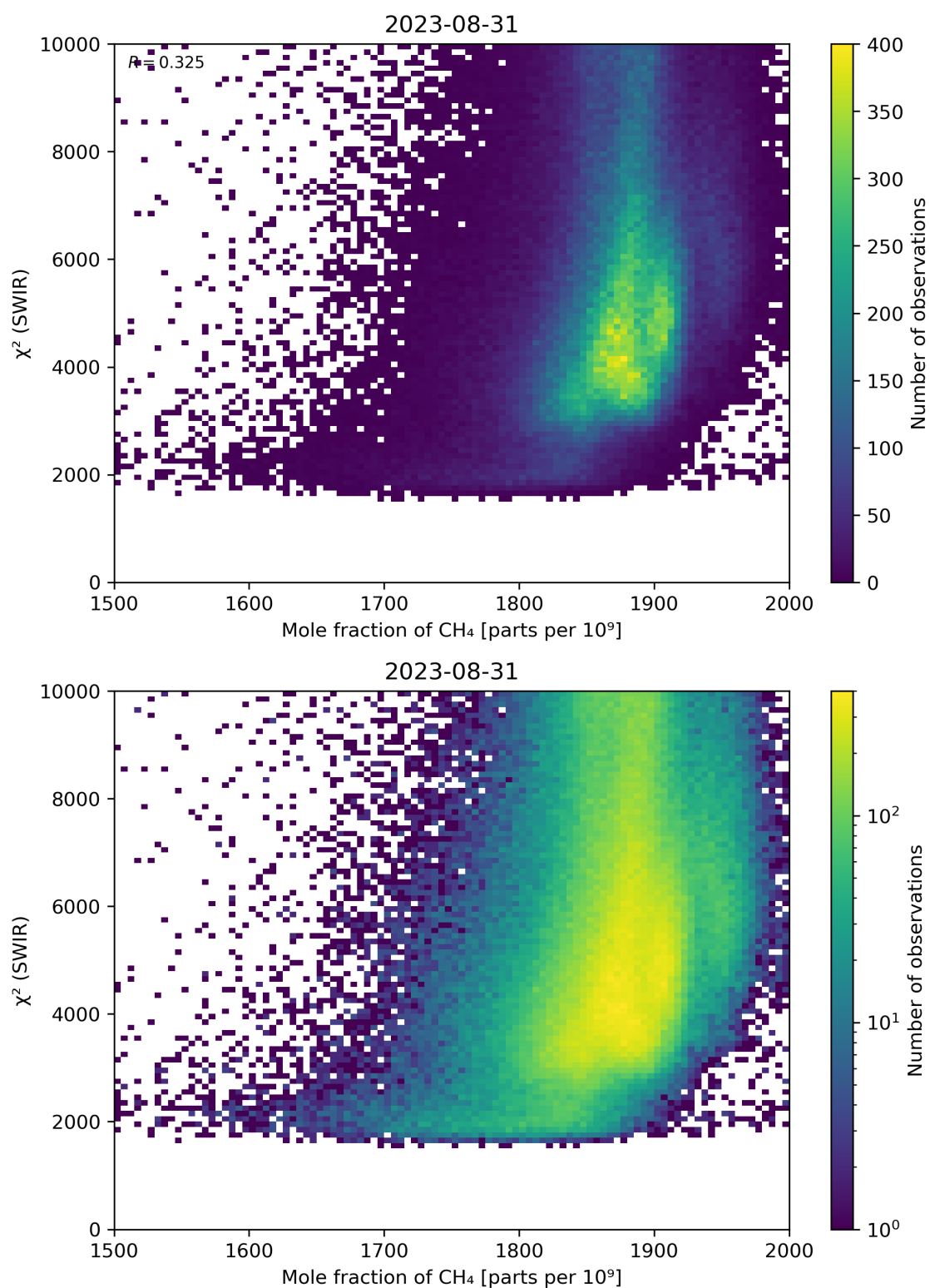
Figure 71: Scatter density plot of “Mole fraction of \text{CH}_4 ” against “ \chi^2 (SWIR)” for 2023-08-30 to 2023-09-01.
