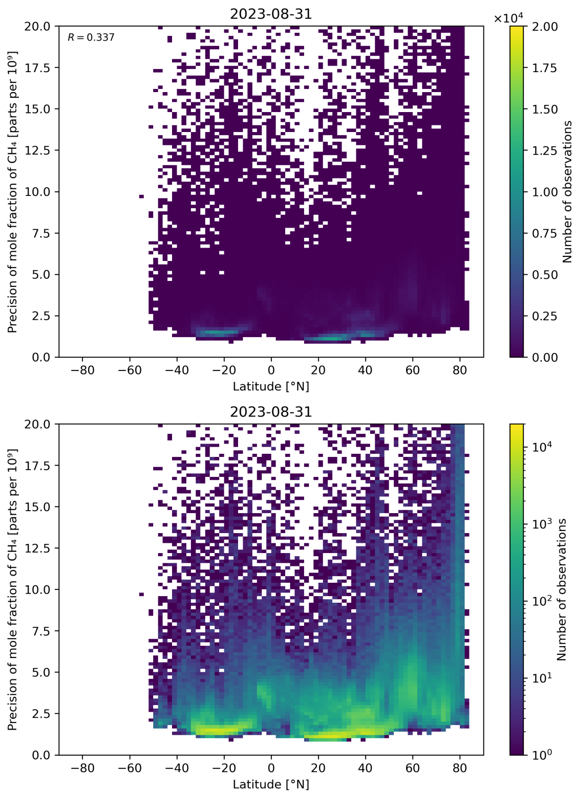
Figure 59: Scatter density plot of “Latitude” against “Precision of mole fraction of \text{CH}_4 ” for 2023-08-30 to 2023-09-01.
