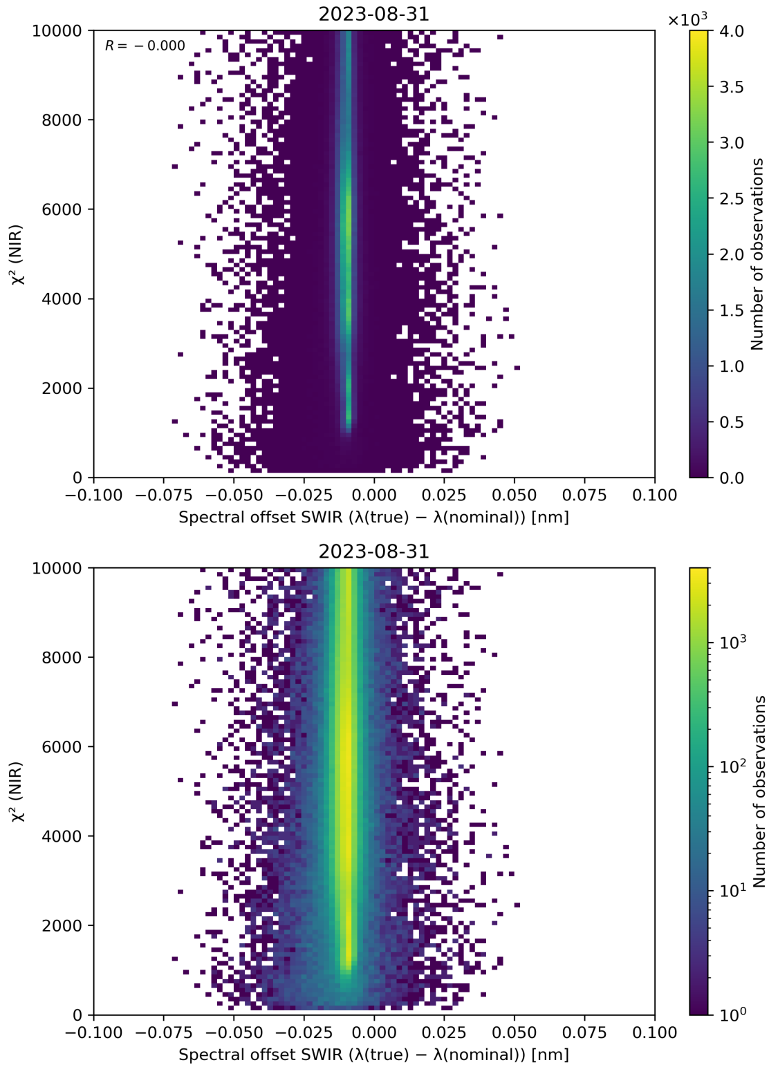
Figure 117: Scatter density plot of “Spectral offset SWIR ( \lambda(\text{true}) - \lambda(\text{nominal}) )” against “ \chi^2 (NIR)” for 2023-08-30 to 2023-09-01.
