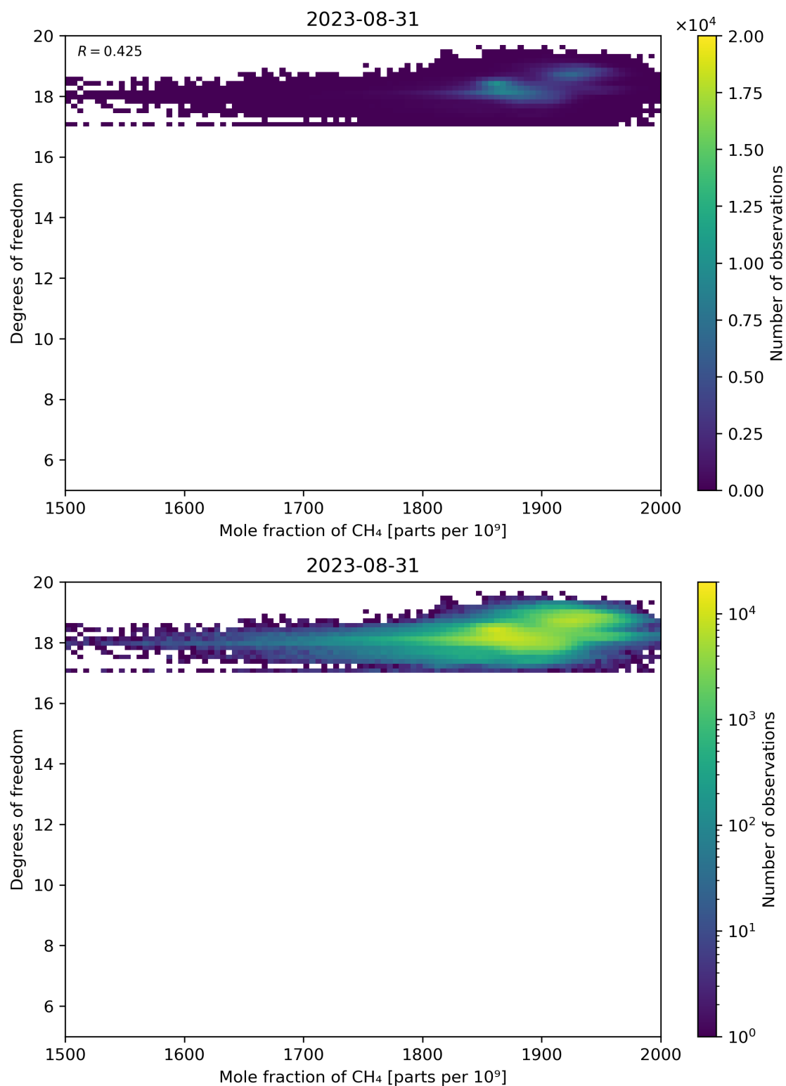
Figure 72: Scatter density plot of “Mole fraction of CH 4 ” against “Degrees of freedom” for 2023-08-30 to 2023-09-01.
