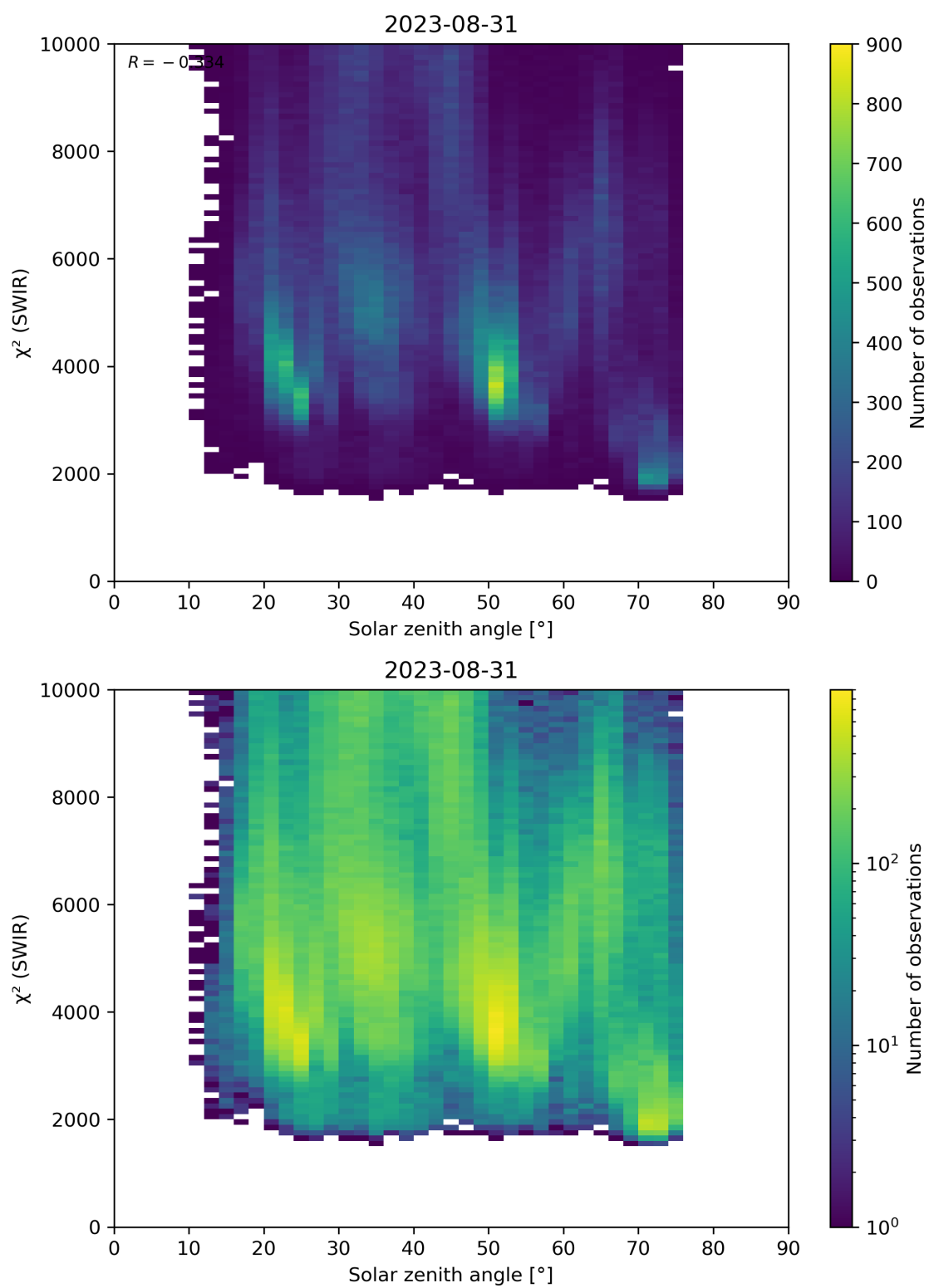
Figure 95: Scatter density plot of “Solar zenith angle” against “ \chi^2 (SWIR)” for 2023-08-30 to 2023-09-01.
