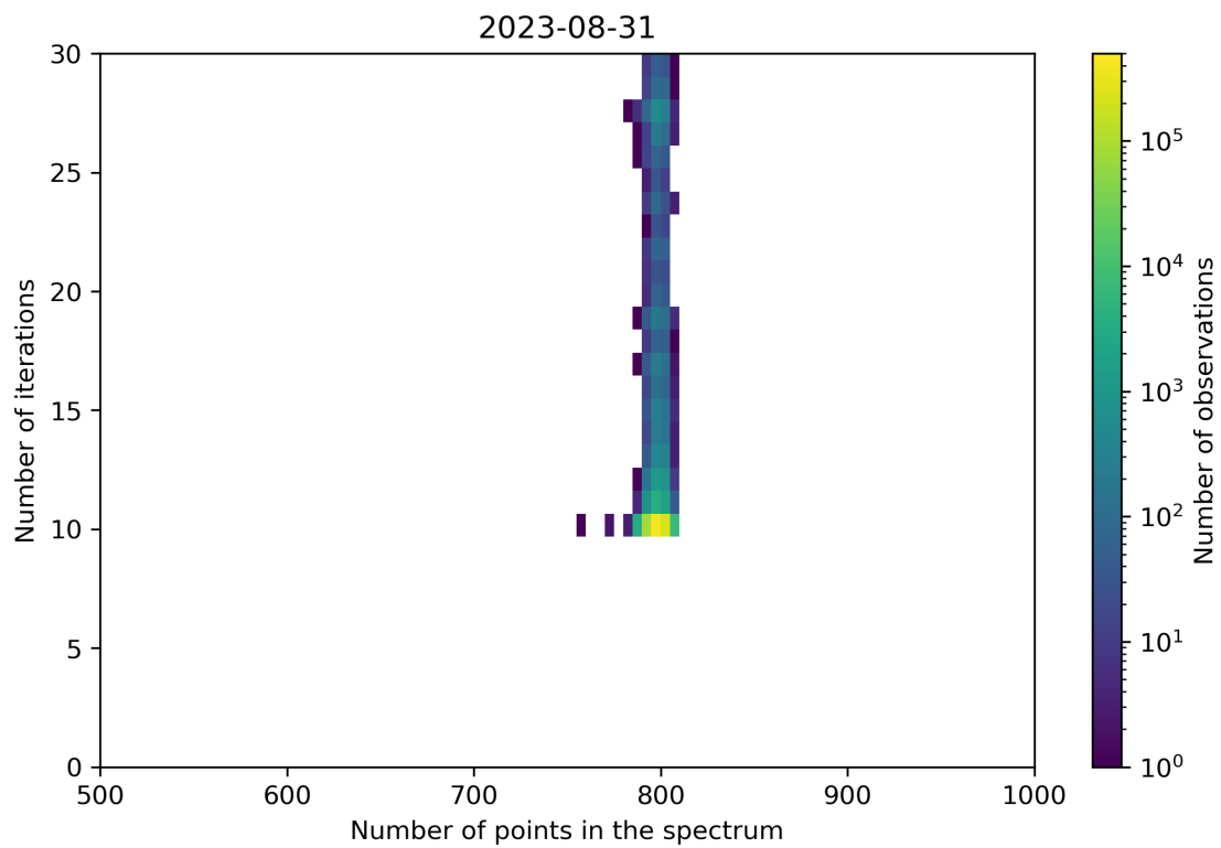
Figure 92: Scatter density plot of “Number of points in the spectrum” against “Number of iterations” for 2023-08-30 to 2023-09-01.
