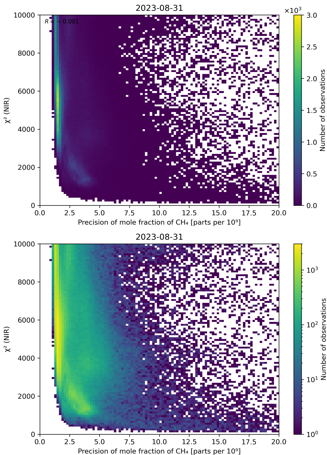
Figure 78: Scatter density plot of “Precision of mole fraction of CH 4 ” against “ \chi^2 (NIR)” for 2023-08-30 to 2023-09-01.
