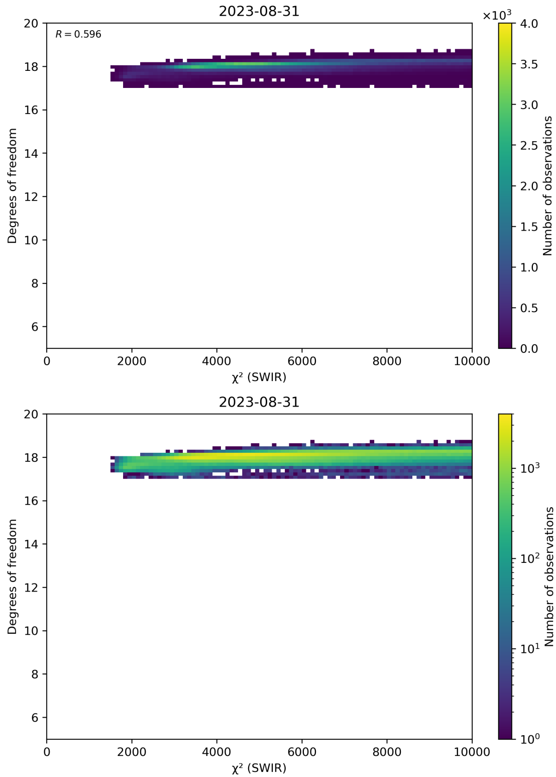
Figure 48: Scatter density plot of " \chi^2 (SWIR)" against "Degrees of freedom" for 2023-08-30 to 2023-09-01.
