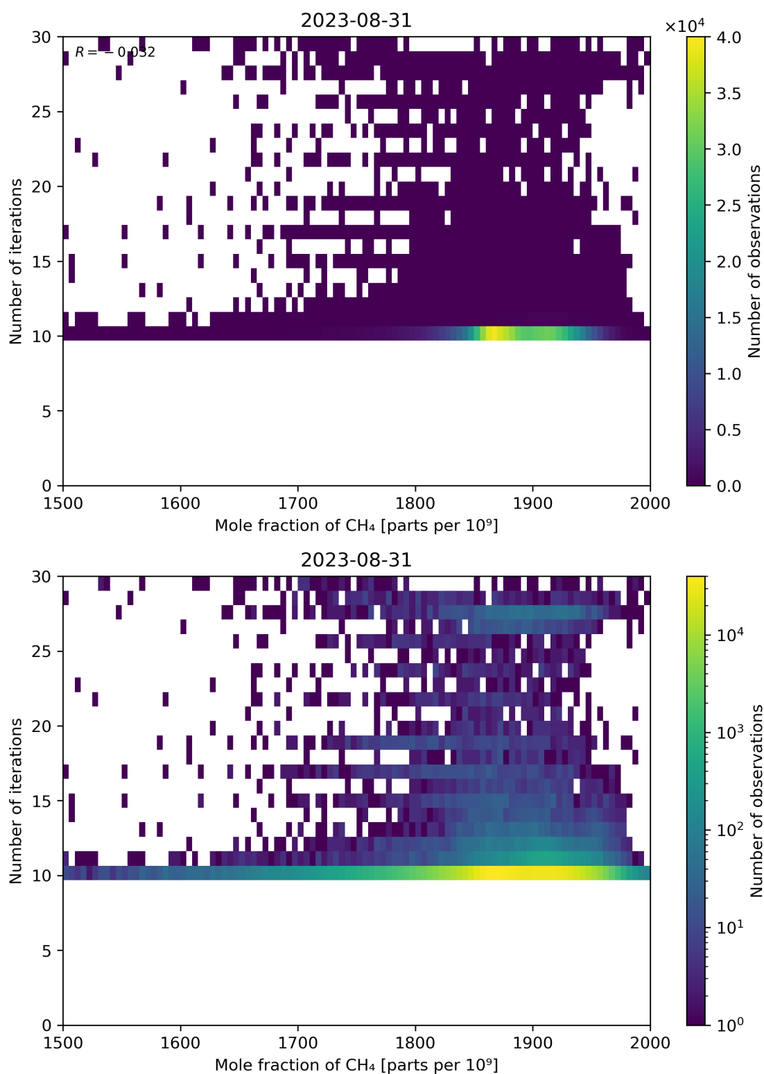
Figure 76: Scatter density plot of “Mole fraction of CH 4 ” against “Number of iterations” for 2023-08-30 to 2023-09-01.
