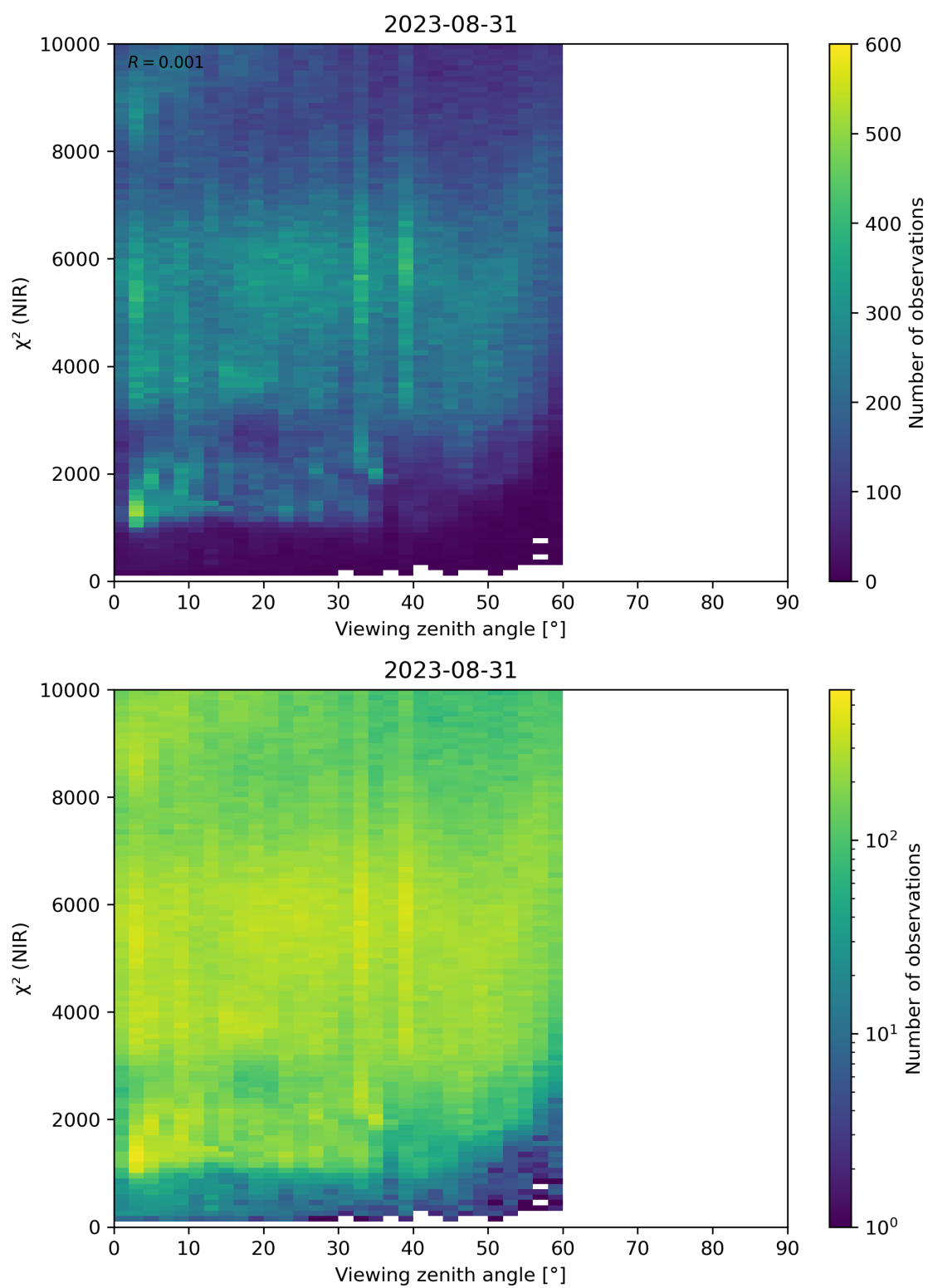
Figure 105: Scatter density plot of “Viewing zenith angle” against “ \chi^2 (NIR)” for 2023-08-30 to 2023-09-01.
