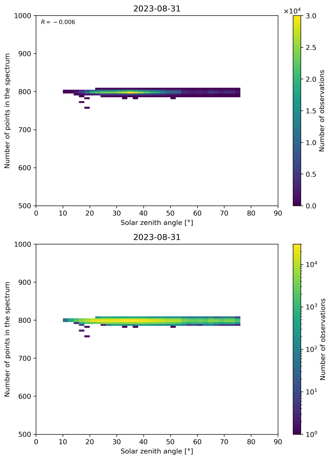
Figure 103: Scatter density plot of “Solar zenith angle” against “Number of points in the spectrum” for 2023-08-30 to 2023-09-01.
