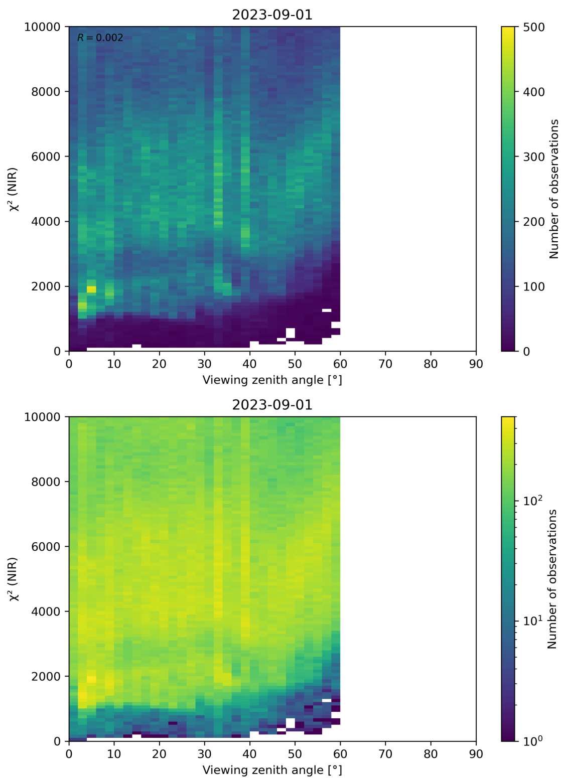
Figure 105: Scatter density plot of “Viewing zenith angle” against “ \chi^2 (NIR)” for 2023-08-31 to 2023-09-02.
