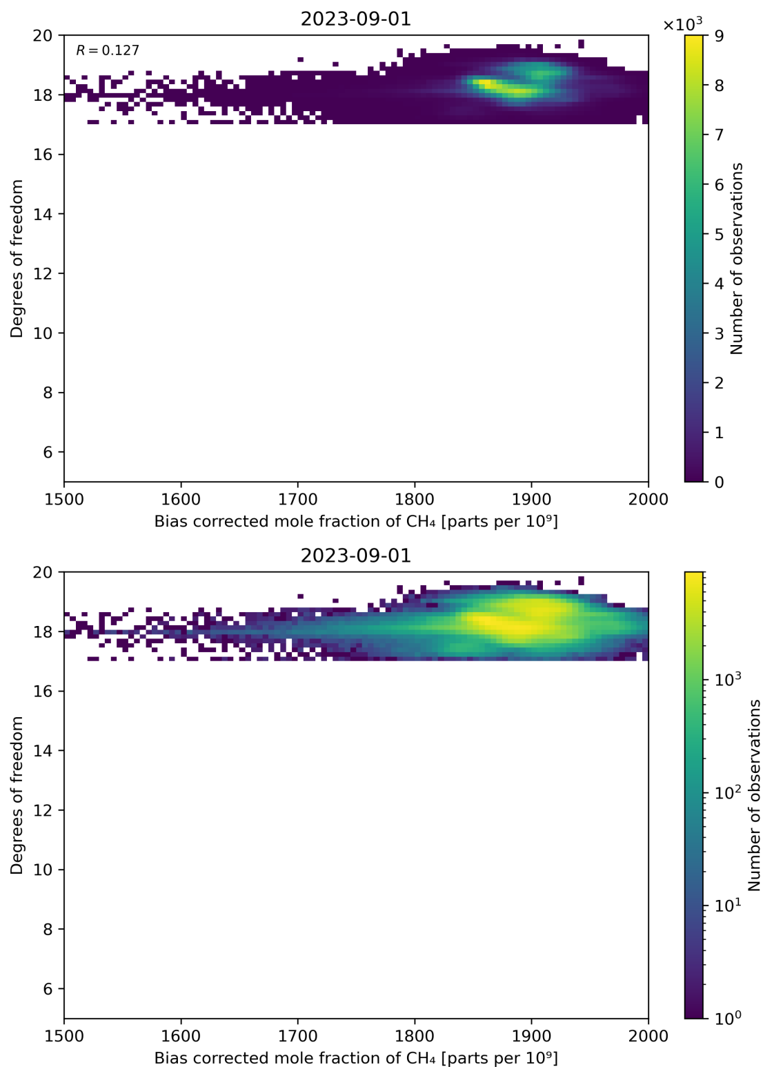
Figure 65: Scatter density plot of “Bias corrected mole fraction of CH 4 ” against “Degrees of freedom” for 2023-08-31 to 2023-09-02.
