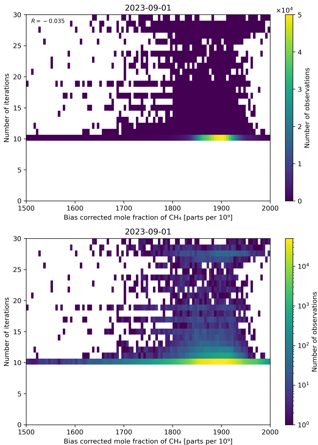
Figure 67: Scatter density plot of “Bias corrected mole fraction of CH 4 ” against “Number of iterations” for 2023-08-31 to 2023-09-02.
