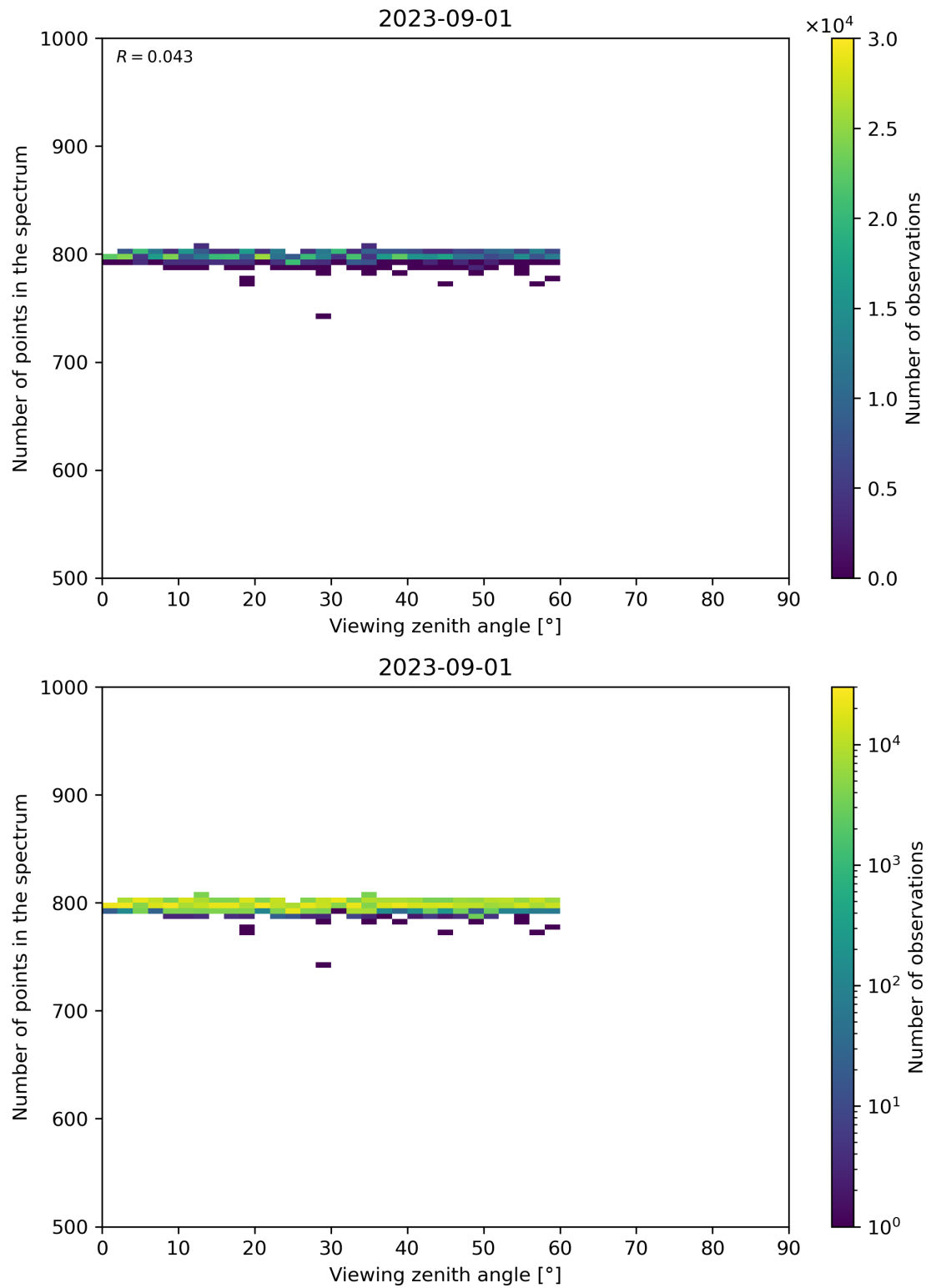
Figure 114: Scatter density plot of “Viewing zenith angle” against “Number of points in the spectrum” for 2023-08-31 to 2023-09-02.
