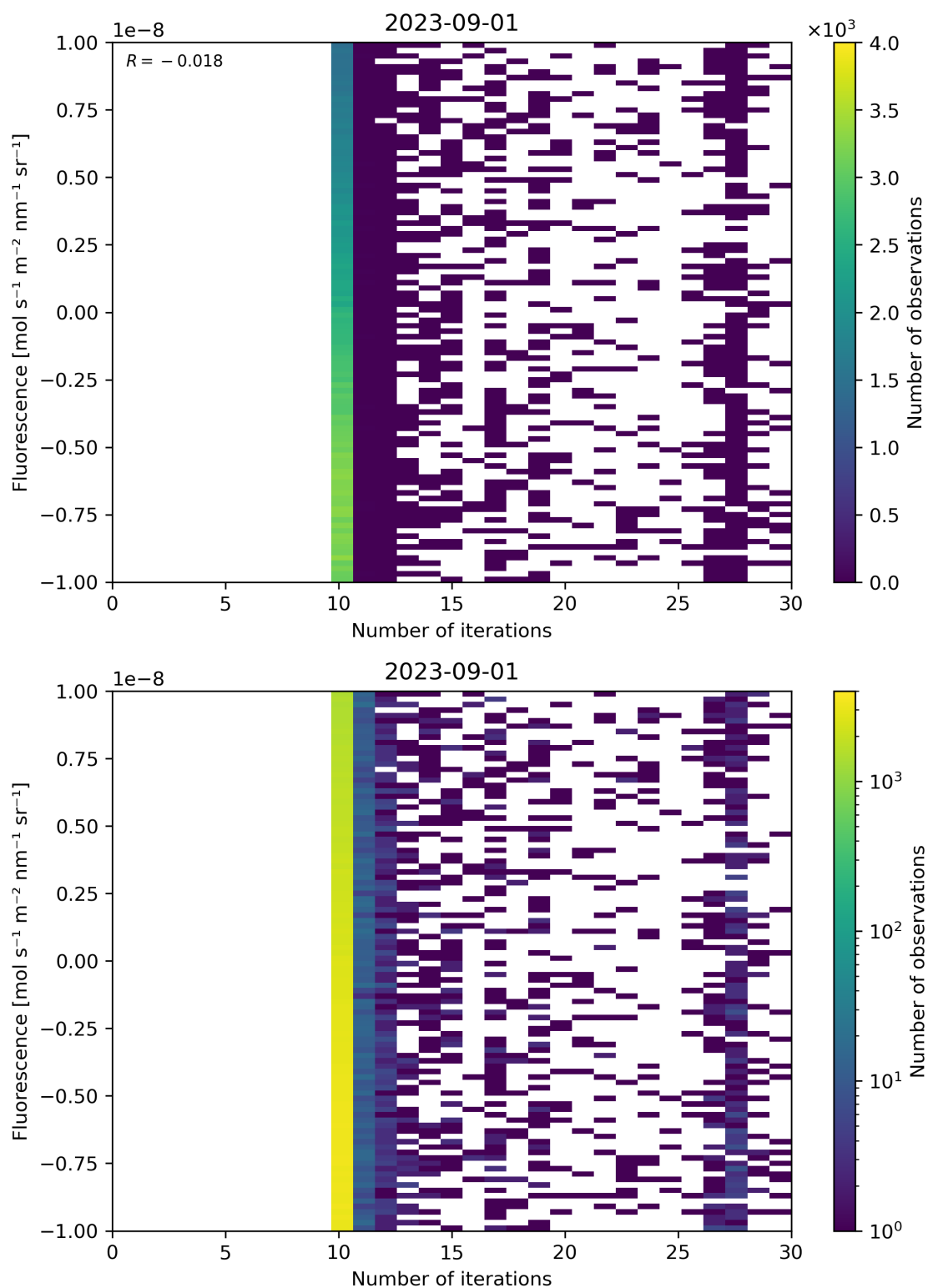
Figure 87: Scatter density plot of “Number of iterations” against “Fluorescence” for 2023-08-31 to 2023-09-02.
