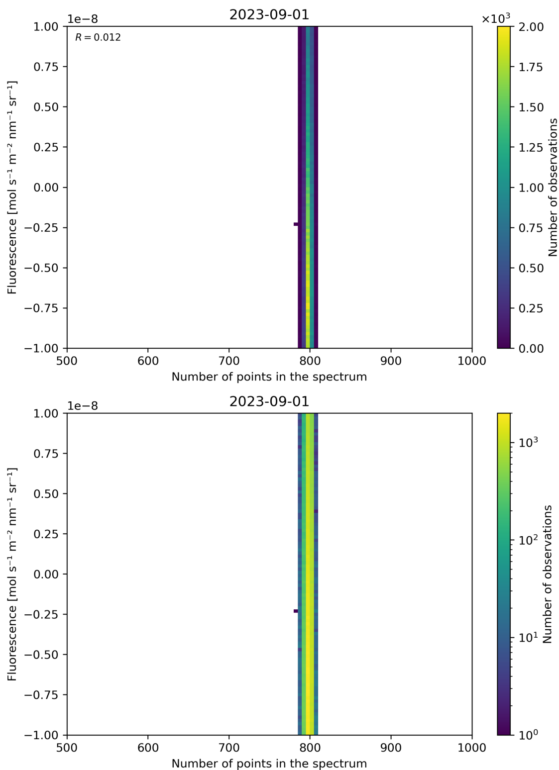
Figure 91: Scatter density plot of “Number of points in the spectrum” against “Fluorescence” for 2023-08-31 to 2023-09-02.
