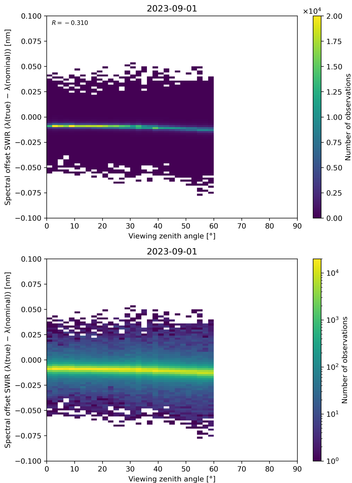
Figure 116: Scatter density plot of “Viewing zenith angle” against “Spectral offset SWIR ( \lambda(\text{true}) - \lambda(\text{nominal}) )” for 2023-08-31 to 2023-09-02.
