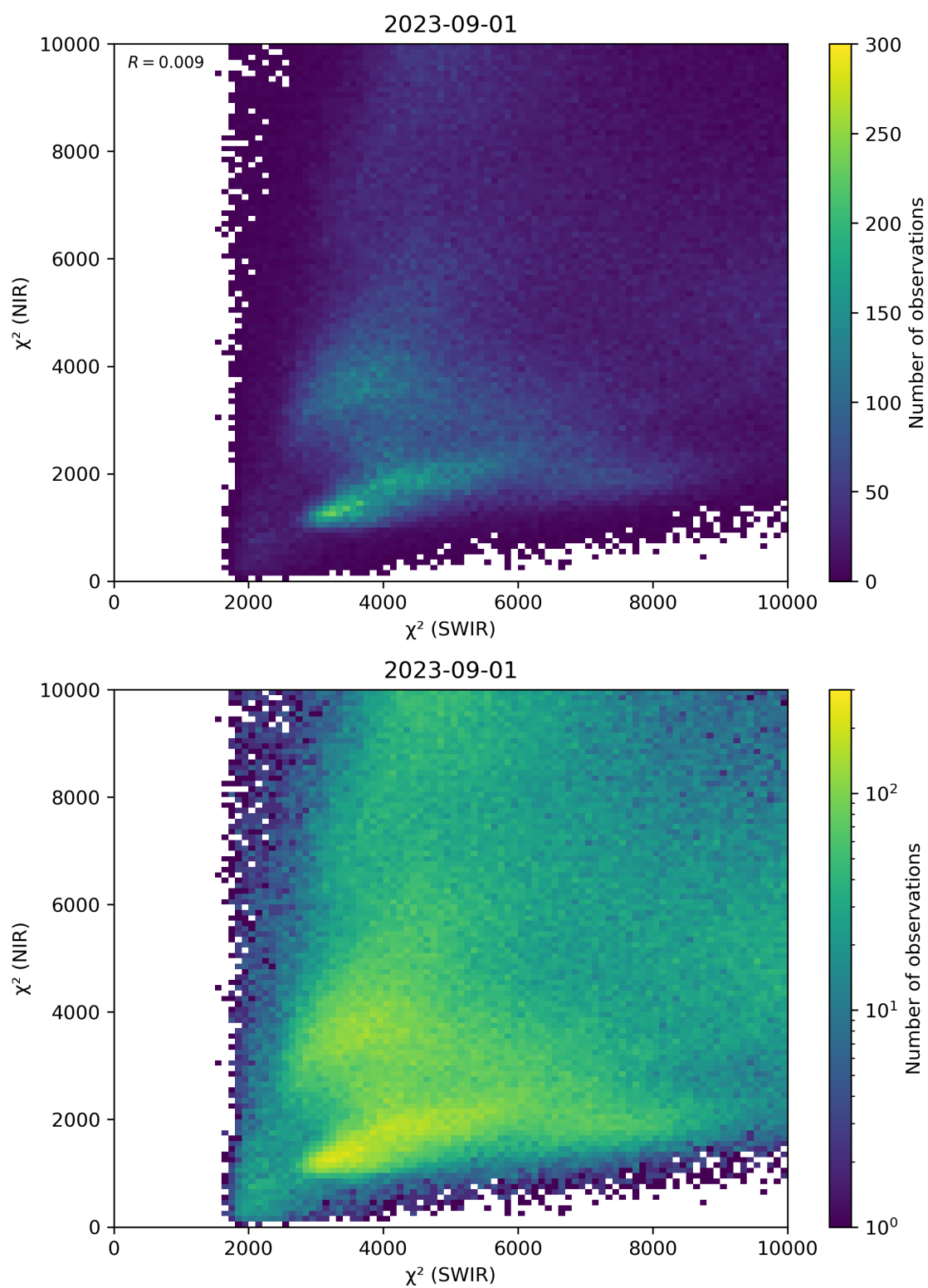
Figure 47: Scatter density plot of “ \chi^2 (SWIR)” against “ \chi^2 (NIR)” for 2023-08-31 to 2023-09-02.
