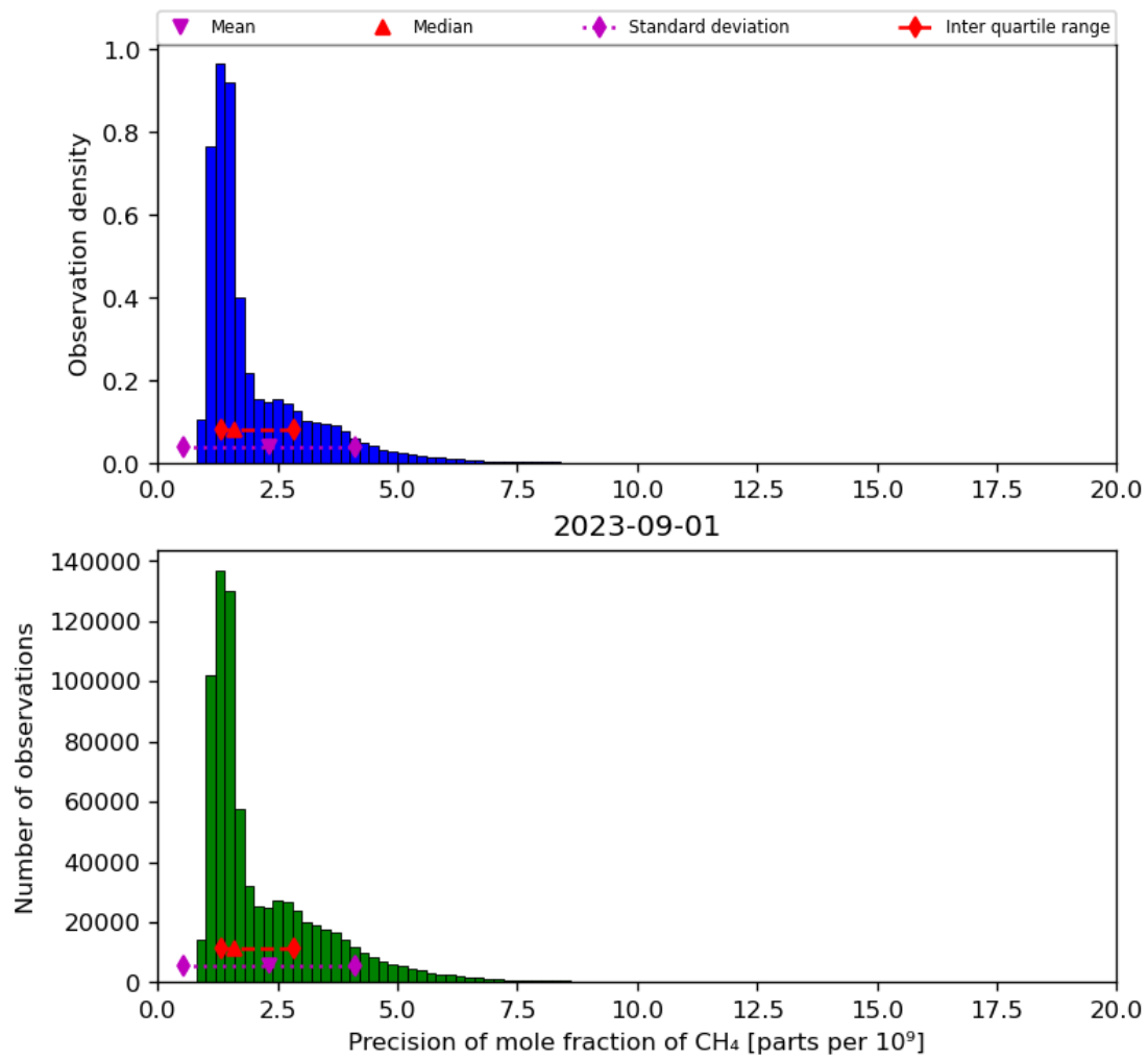
Figure 24: Histogram of “Precision of mole fraction of CH 4 ” for 2023-08-31 to 2023-09-02
