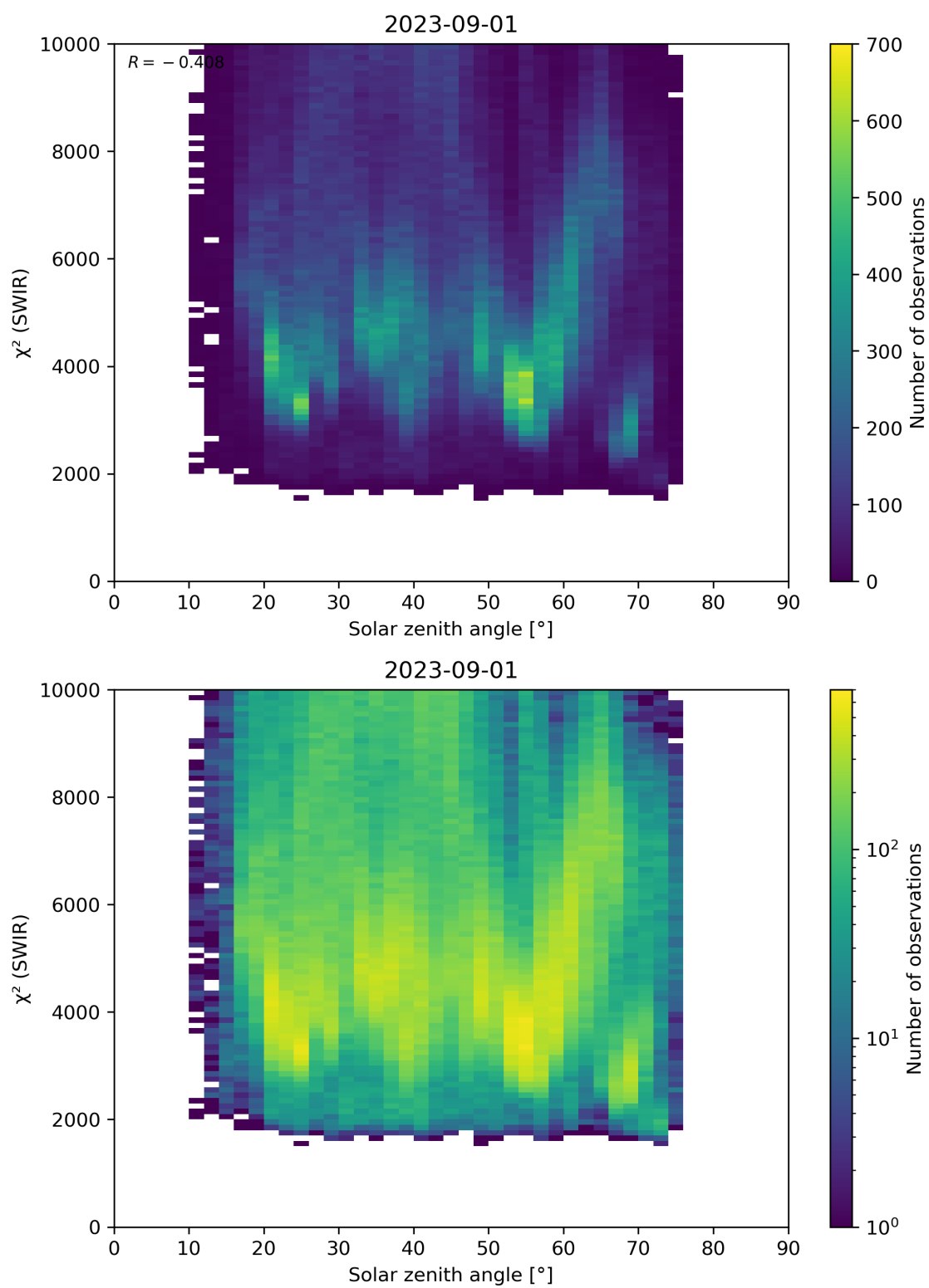
Figure 95: Scatter density plot of “Solar zenith angle” against “ \chi^2 (SWIR)” for 2023-08-31 to 2023-09-02.
