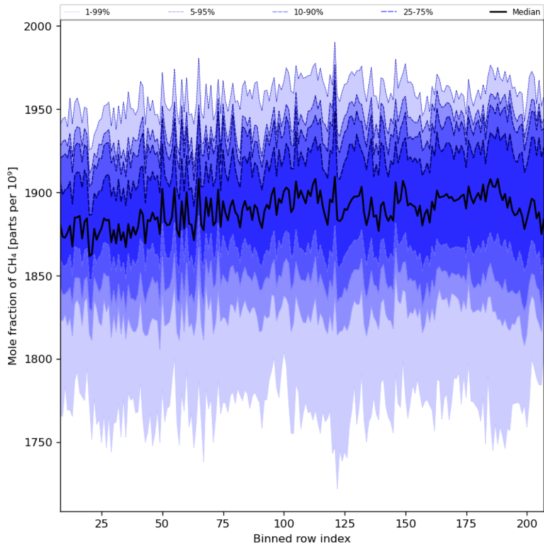
Figure 34: Along track statistics of “Mole fraction of CH 4 ” for 2023-08-31 to 2023-09-02
