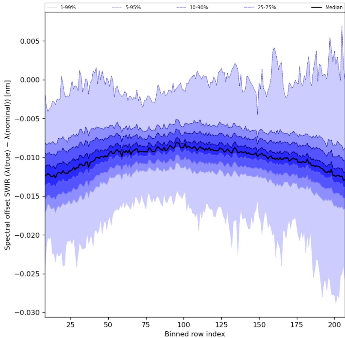
Figure 38: Along track statistics of “Spectral offset SWIR ( \lambda(\text{true}) - \lambda(\text{nominal}) )” for 2023-08-31 to 2023-09-02
