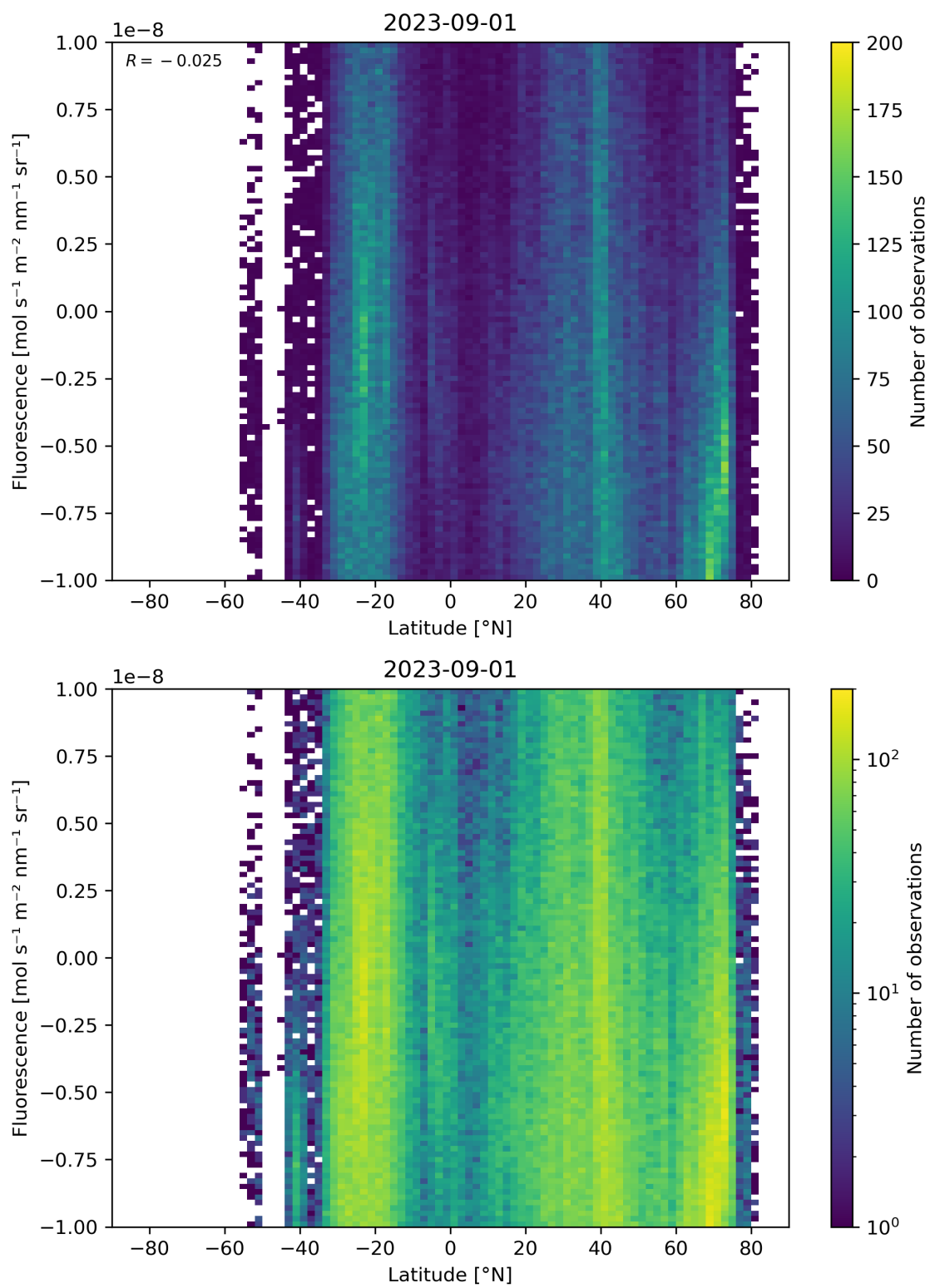
Figure 56: Scatter density plot of “Latitude” against “Fluorescence” for 2023-08-31 to 2023-09-02.
