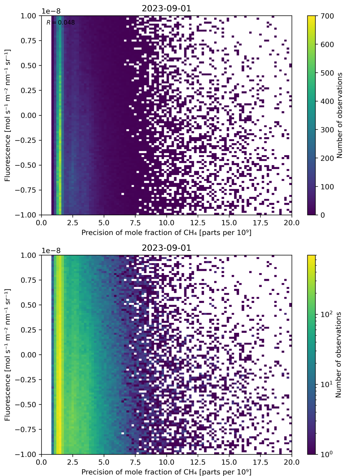
Figure 81: Scatter density plot of “Precision of mole fraction of \text{CH}_4 ” against “Fluorescence” for 2023-08-31 to 2023-09-02.
