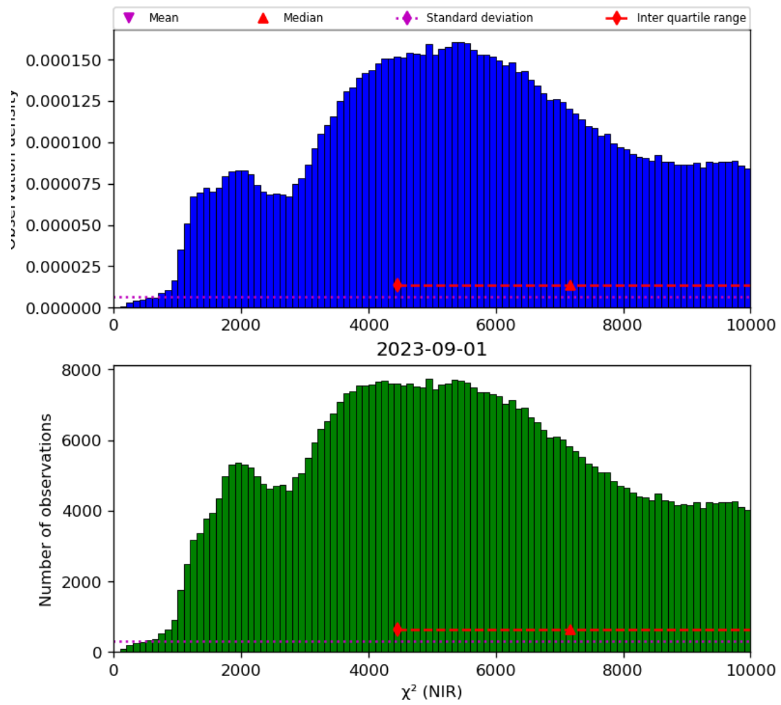
Figure 29: Histogram of “ \chi^2 (NIR)” for 2023-08-31 to 2023-09-02
