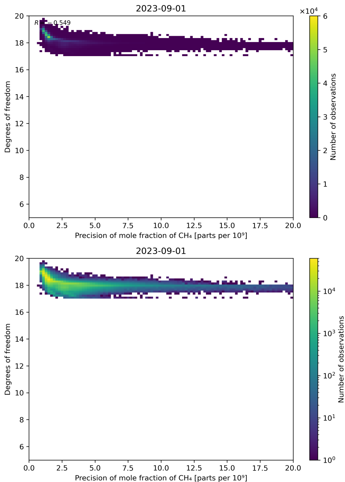
Figure 80: Scatter density plot of “Precision of mole fraction of CH 4 ” against “Degrees of freedom” for 2023-08-31 to 2023-09-02.
