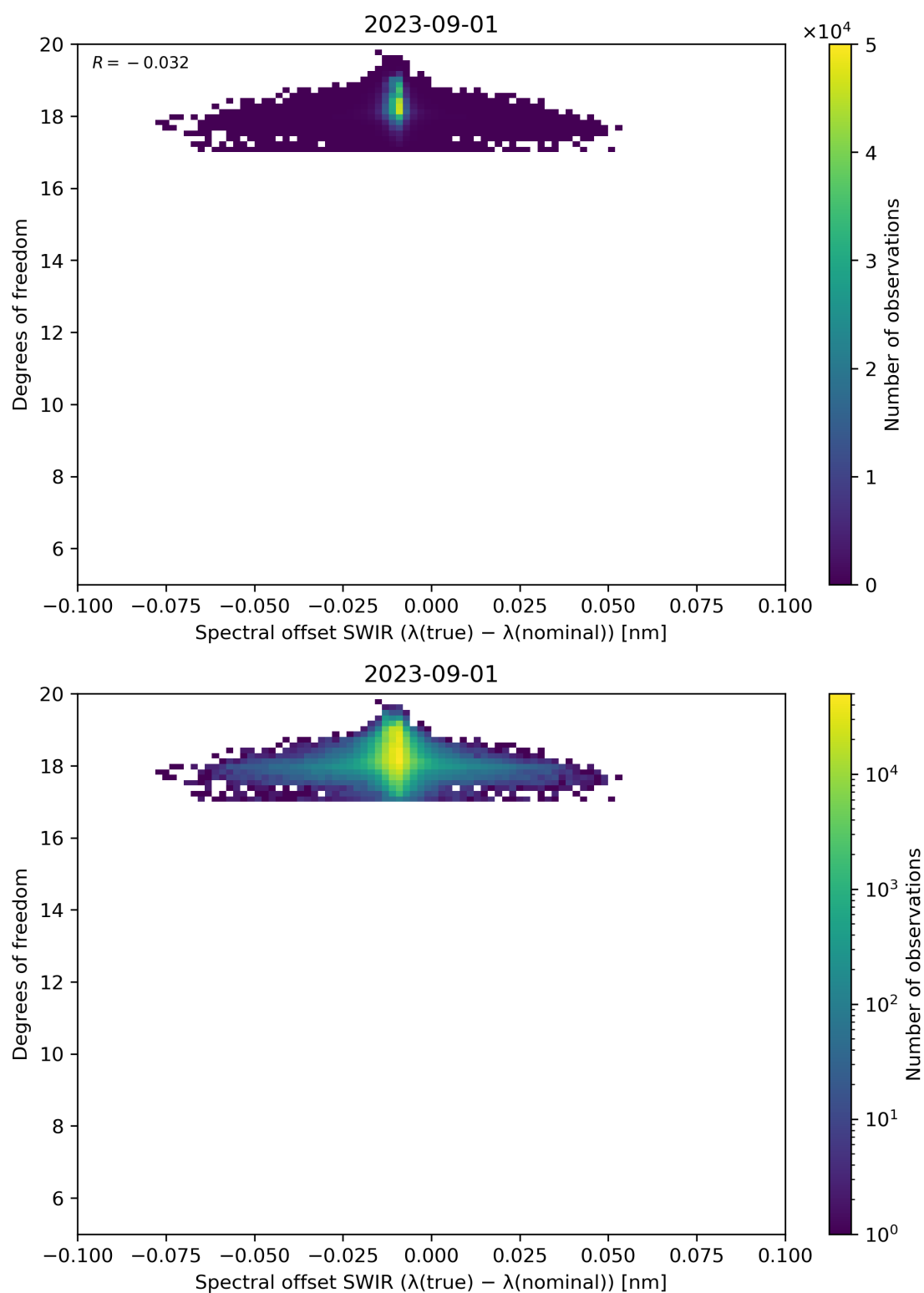
Figure 119: Scatter density plot of “Spectral offset SWIR ( \lambda(\text{true}) - \lambda(\text{nominal}) )” against “Degrees of freedom” for 2023-08-31 to 2023-09-02.
