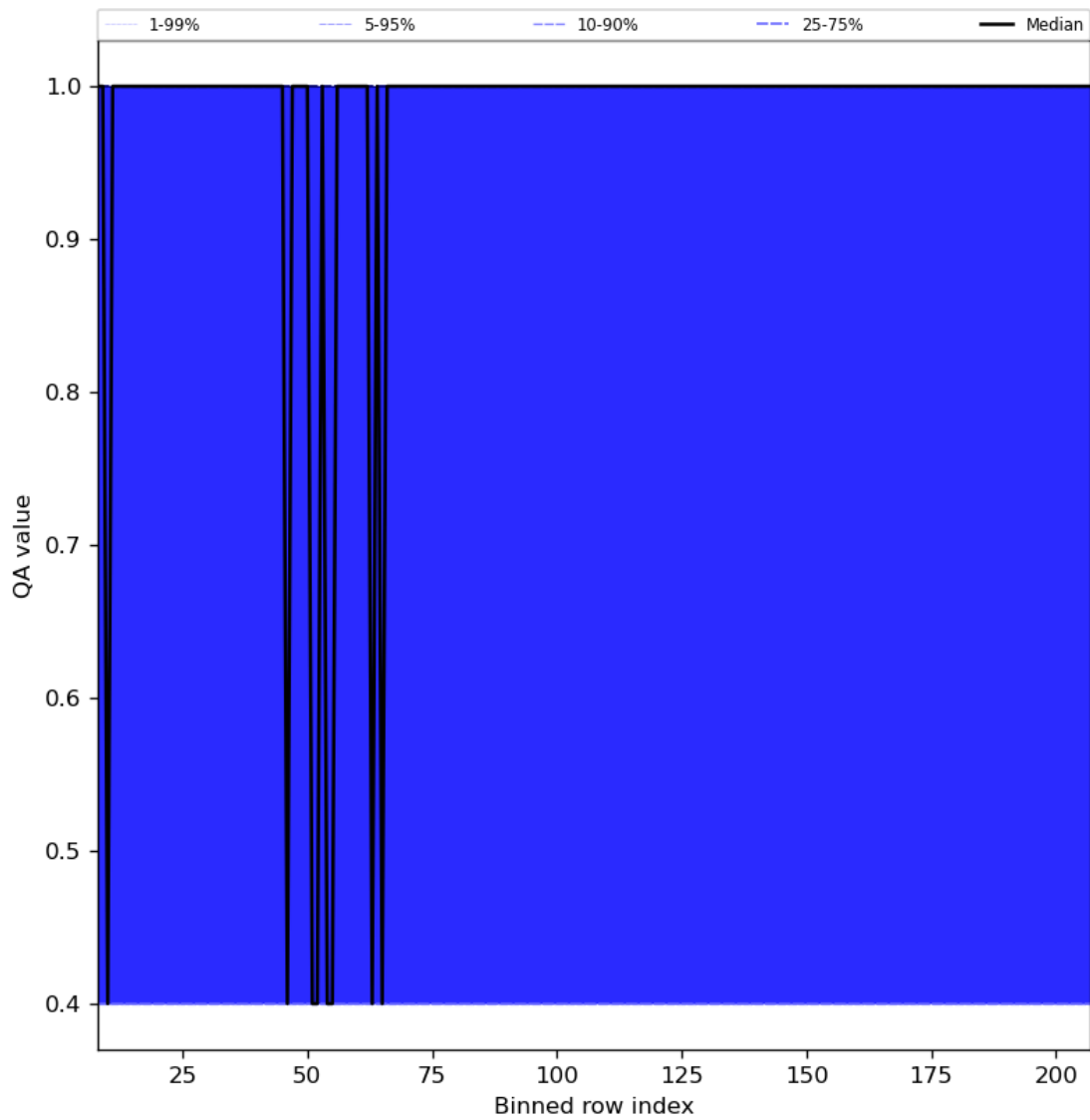
Figure 33: Along track statistics of “QA value” for 2023-08-31 to 2023-09-02
