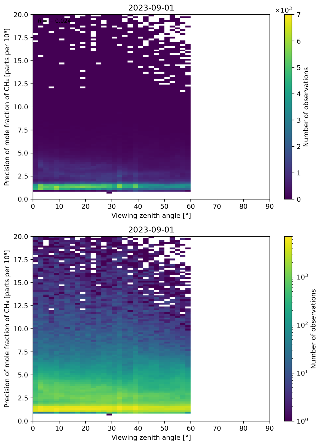
Figure 112: Scatter density plot of “Viewing zenith angle” against “Precision of mole fraction of CH 4 ” for 2023-08-31 to 2023-09-02.
