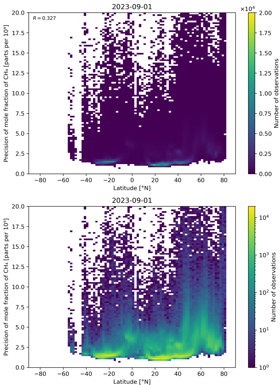
Figure 59: Scatter density plot of “Latitude” against “Precision of mole fraction of CH 4 ” for 2023-08-31 to 2023-09-02.
