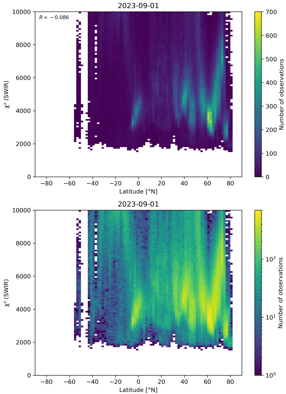
Figure 54: Scatter density plot of “Latitude” against “ \chi^2 (SWIR)” for 2023-08-31 to 2023-09-02.
