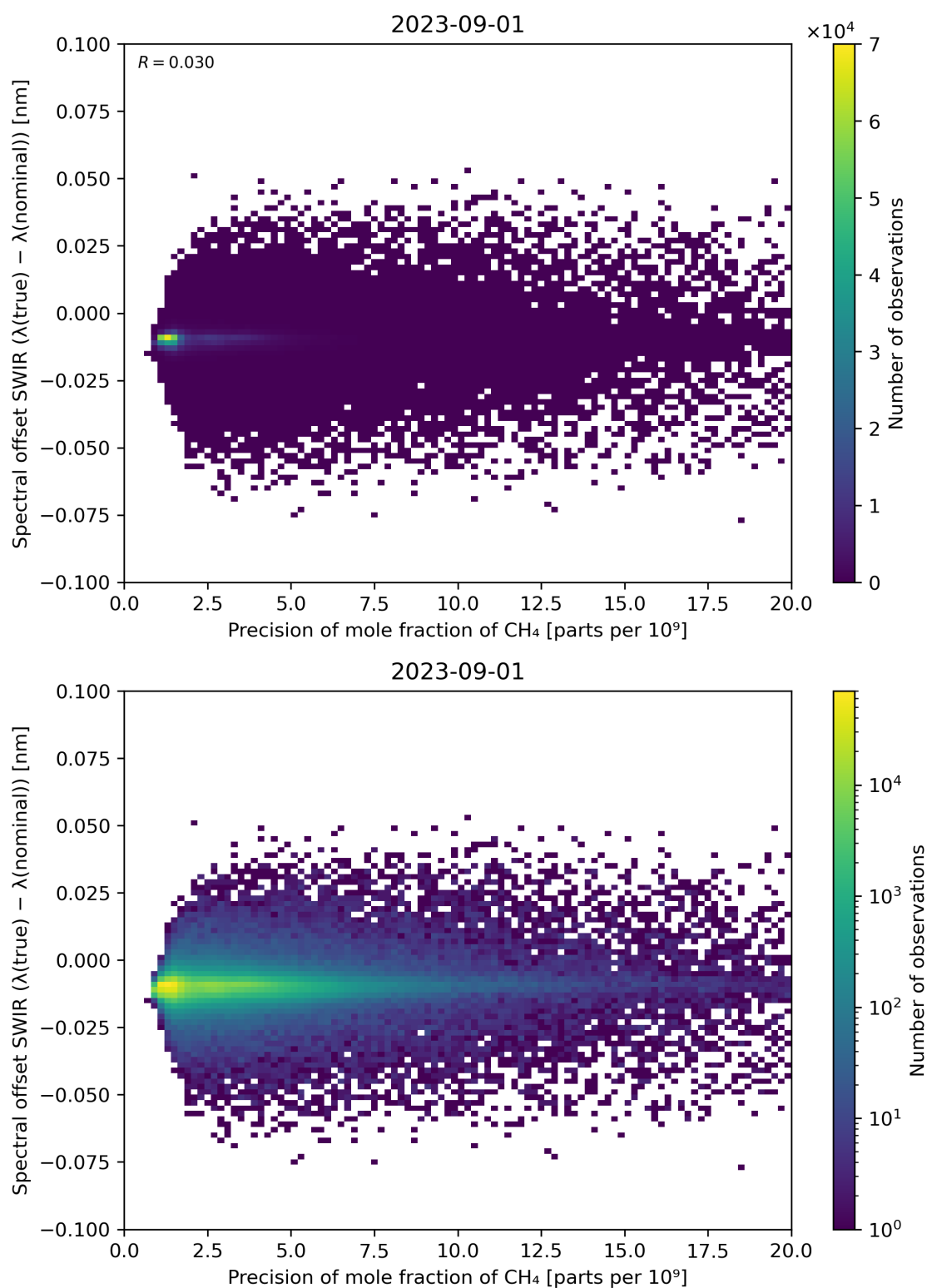
Figure 85: Scatter density plot of “Precision of mole fraction of CH 4 ” against “Spectral offset SWIR ( \lambda(\text{true}) - \lambda(\text{nominal}) )” for 2023-08-31 to 2023-09-02.
