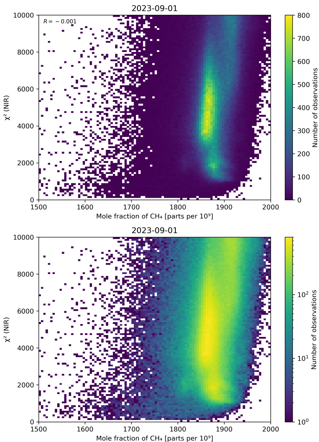
Figure 70: Scatter density plot of “Mole fraction of \text{CH}_4 ” against “ \chi^2 (NIR)” for 2023-08-31 to 2023-09-02.
