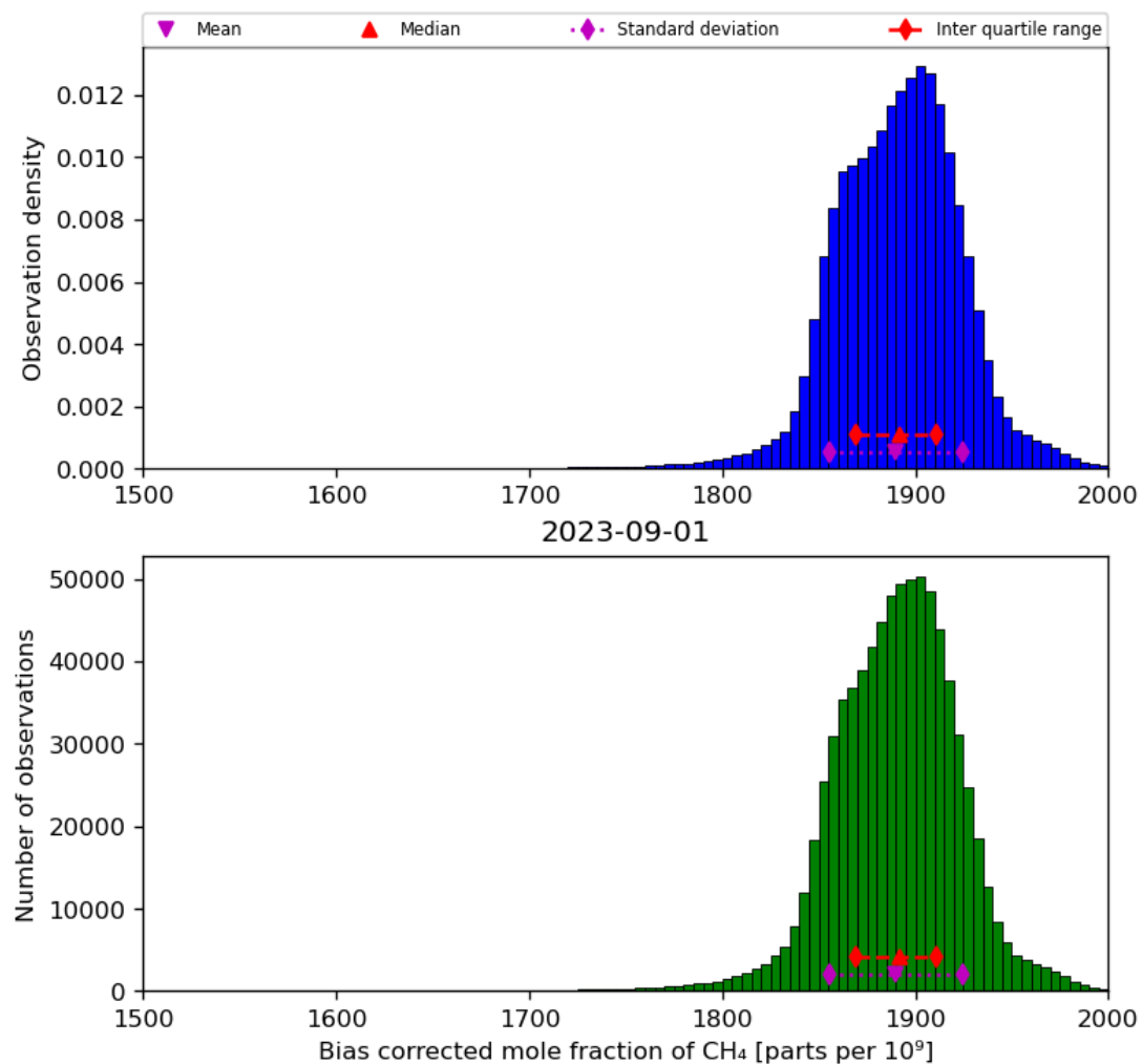
Figure 25: Histogram of “Bias corrected mole fraction of CH 4 ” for 2023-08-31 to 2023-09-02
