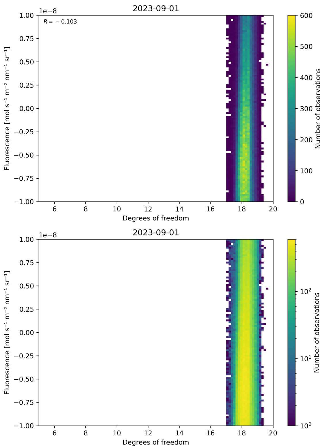
Figure 51: Scatter density plot of “Degrees of freedom” against “Fluorescence” for 2023-08-31 to 2023-09-02.
