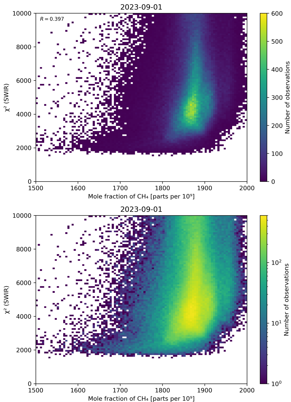
Figure 71: Scatter density plot of “Mole fraction of \text{CH}_4 ” against “ \chi^2 (SWIR)” for 2023-08-31 to 2023-09-02.
