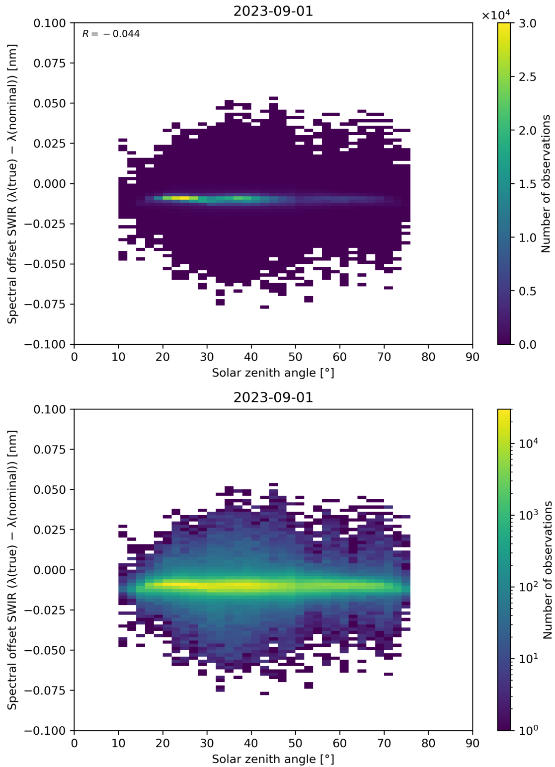
Figure 104: Scatter density plot of “Solar zenith angle” against “Spectral offset SWIR ( \lambda(\text{true}) - \lambda(\text{nominal}) )” for 2023-08-31 to 2023-09-02.
