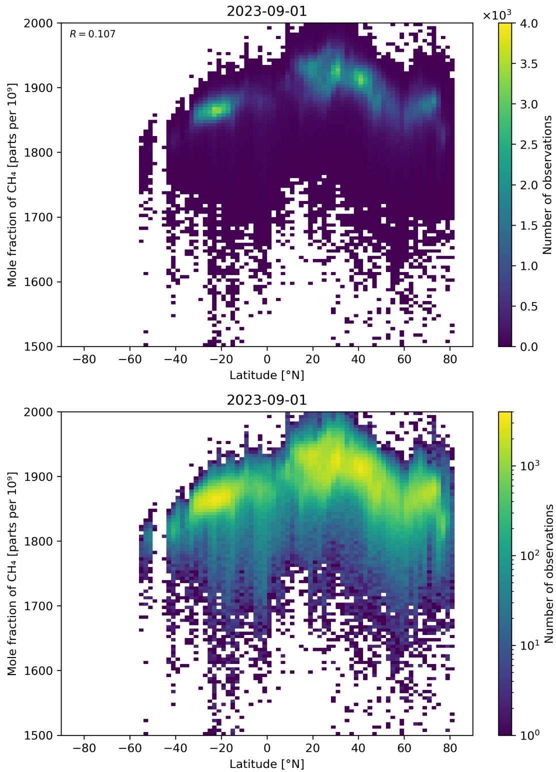
Figure 57: Scatter density plot of “Latitude” against “Mole fraction of CH 4 ” for 2023-08-31 to 2023-09-02.
