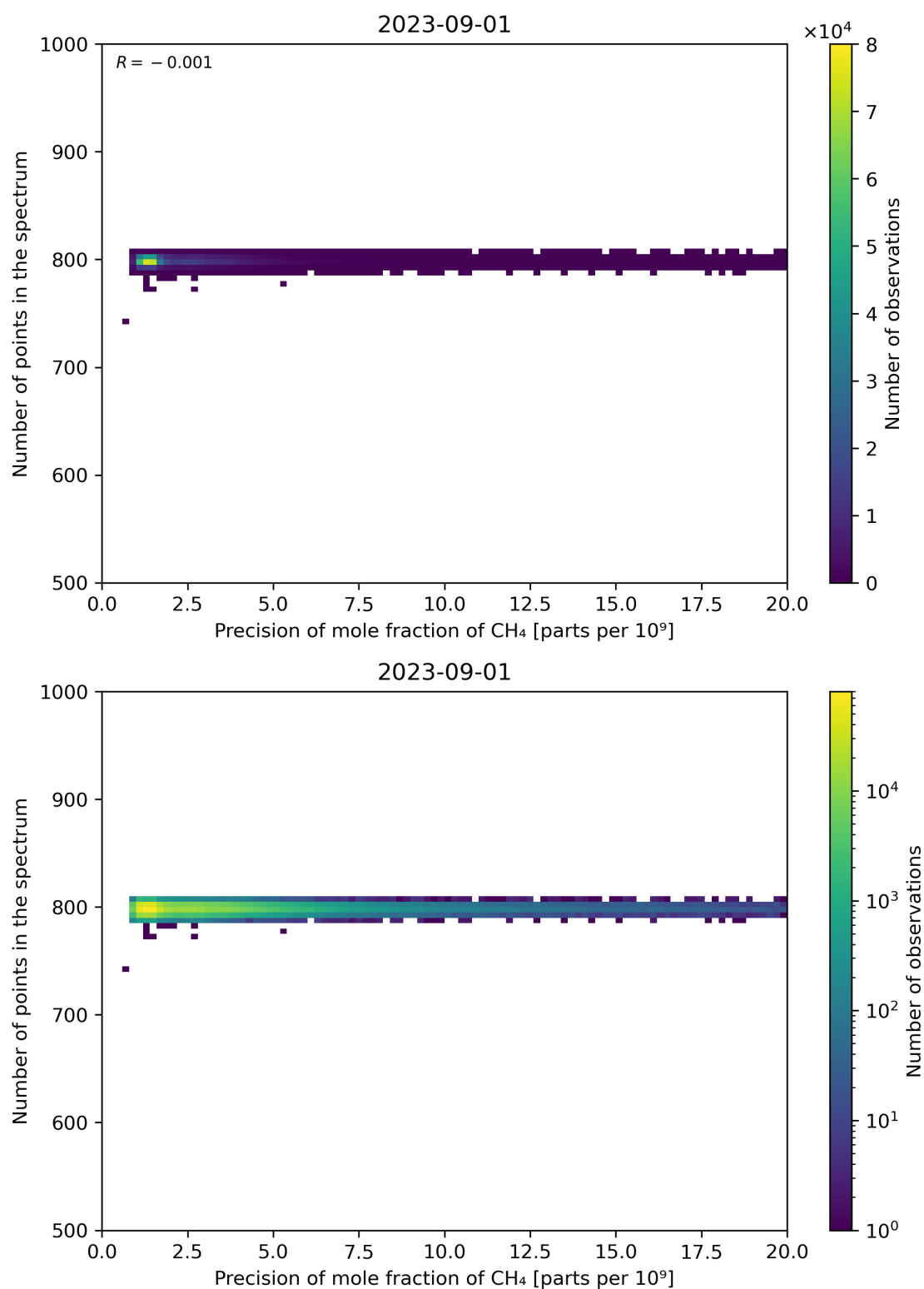
Figure 84: Scatter density plot of “Precision of mole fraction of CH 4 ” against “Number of points in the spectrum” for 2023-08-31 to 2023-09-02.
