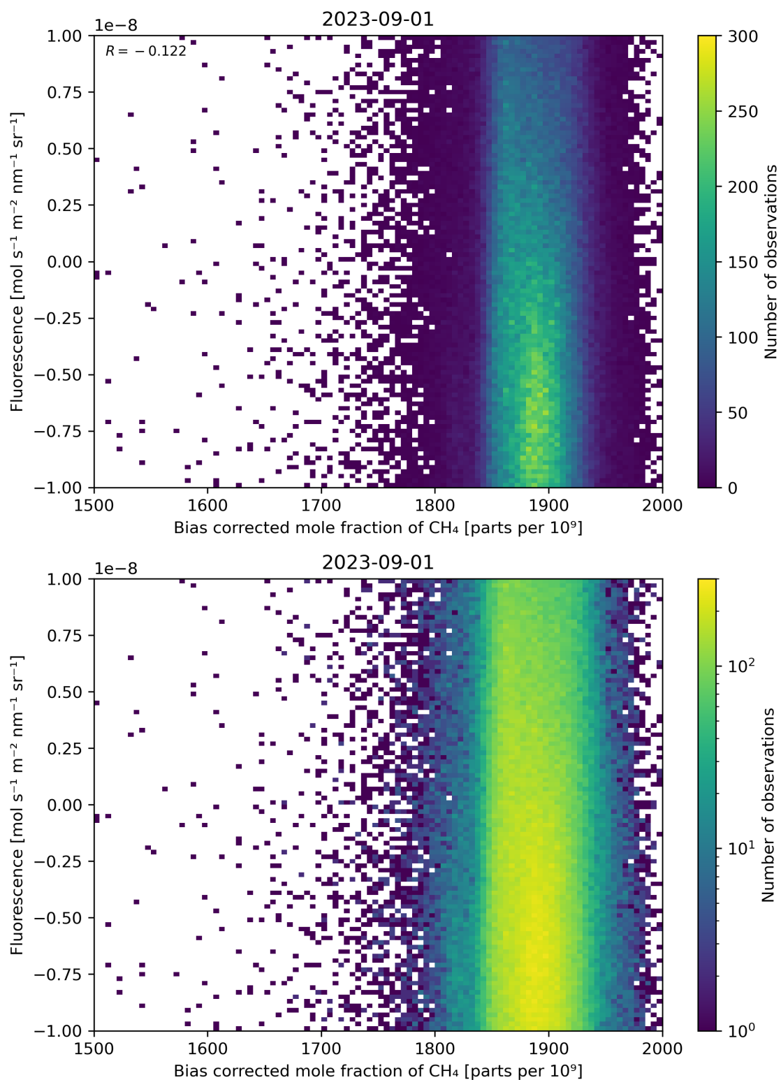
Figure 66: Scatter density plot of “Bias corrected mole fraction of \text{CH}_4 ” against “Fluorescence” for 2023-08-31 to 2023-09-02.
