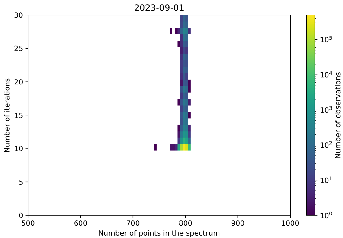
Figure 92: Scatter density plot of “Number of points in the spectrum” against “Number of iterations” for 2023-08-31 to 2023-09-02.
