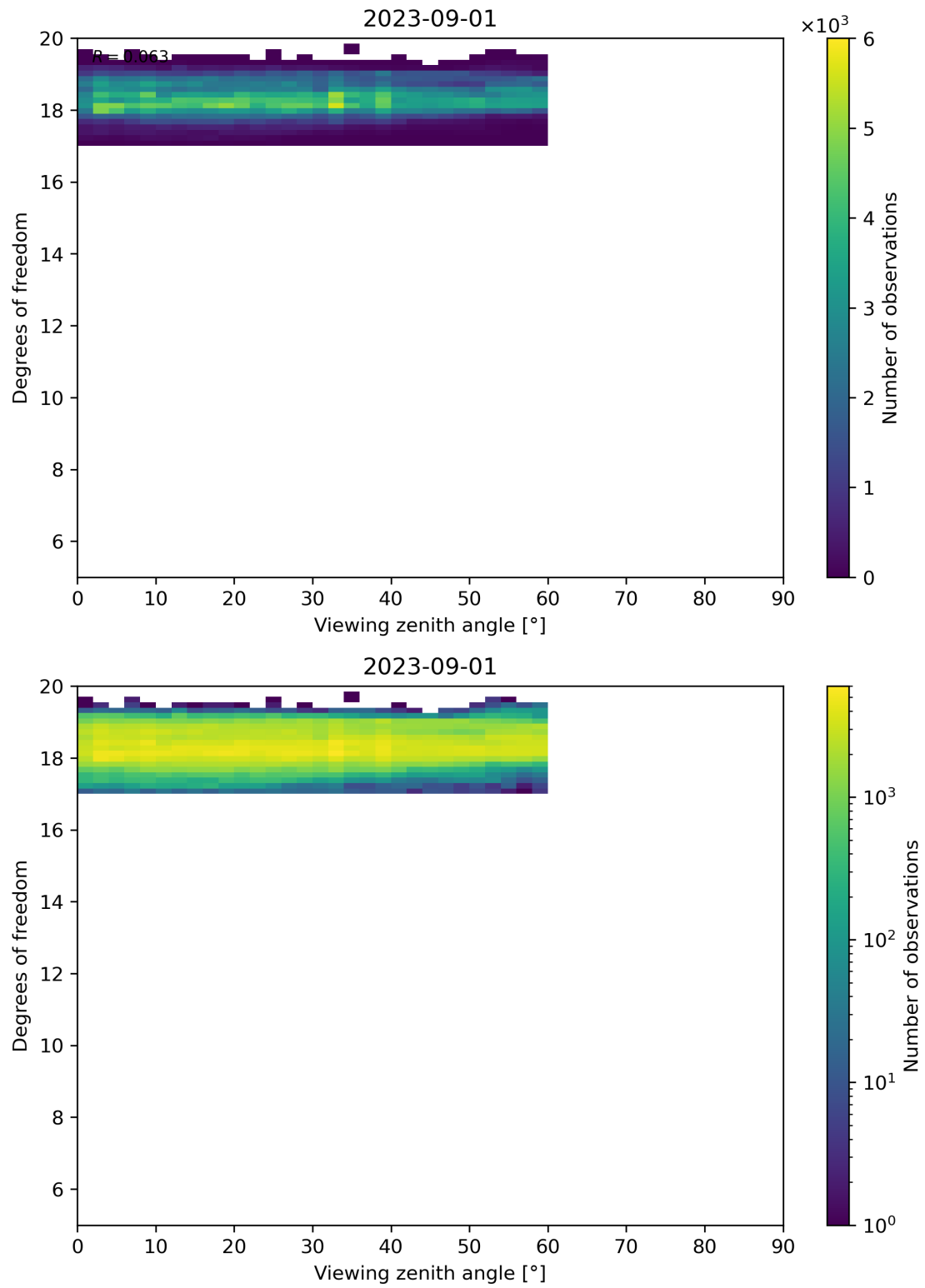
Figure 107: Scatter density plot of “Viewing zenith angle” against “Degrees of freedom” for 2023-08-31 to 2023-09-02.
