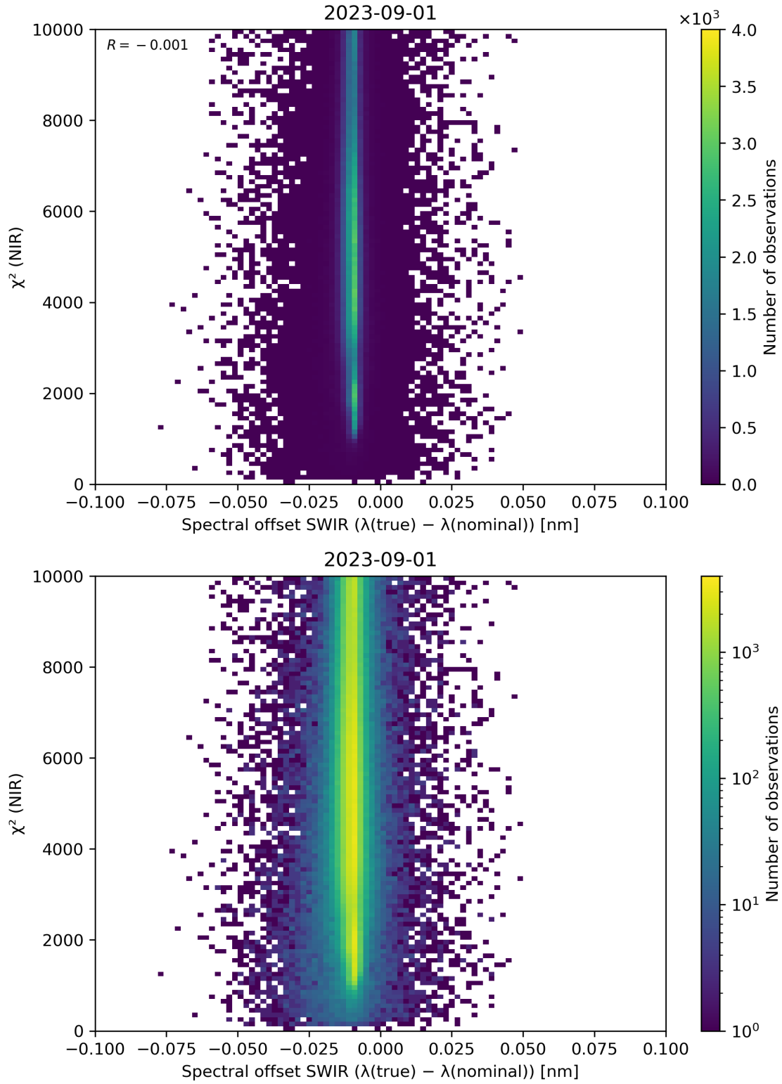
Figure 117: Scatter density plot of “Spectral offset SWIR ( \lambda(\text{true}) - \lambda(\text{nominal}) )” against “ \chi^2 (NIR)” for 2023-08-31 to 2023-09-02.
