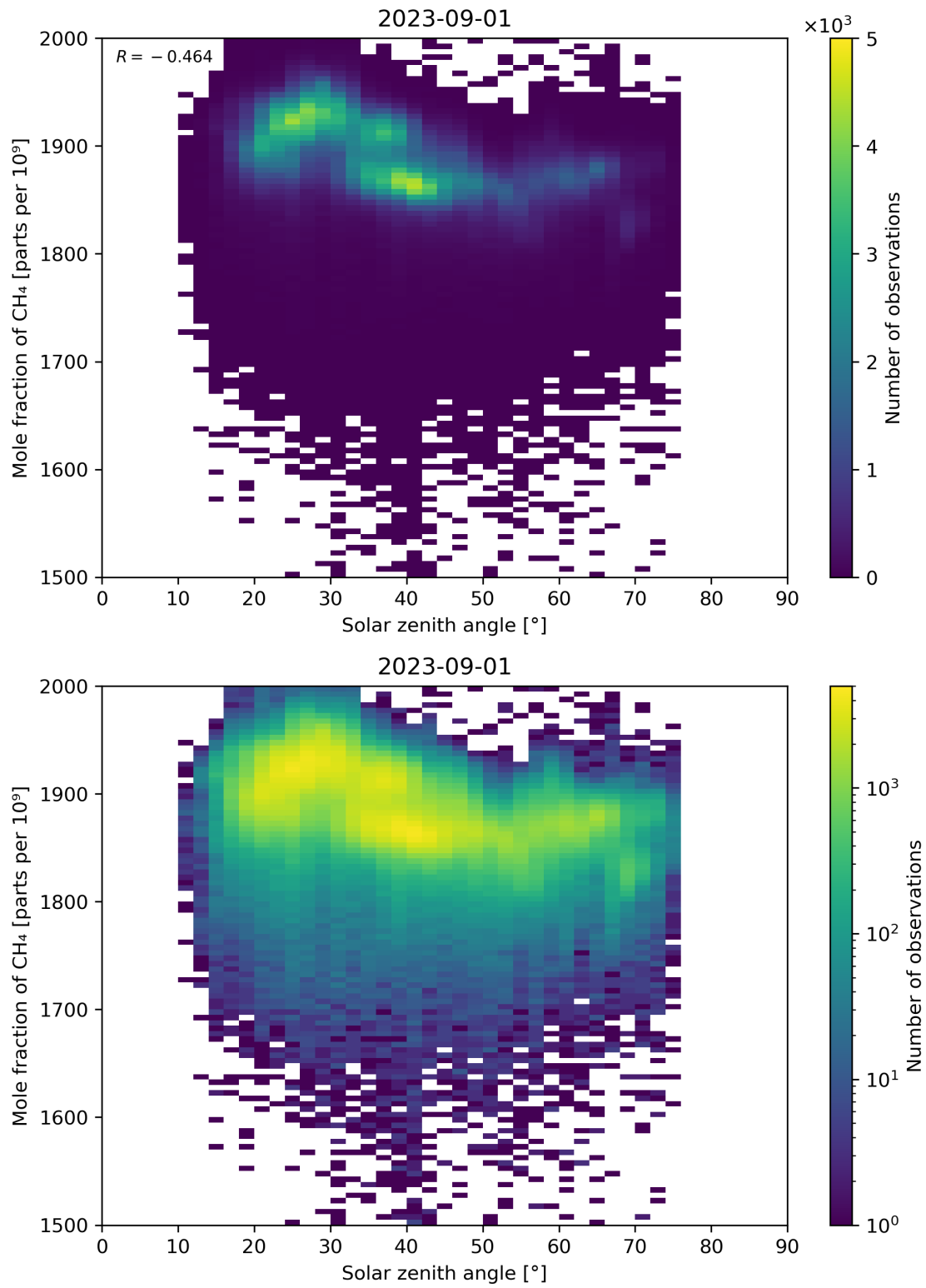
Figure 99: Scatter density plot of “Solar zenith angle” against “Mole fraction of \text{CH}_4 ” for 2023-08-31 to 2023-09-02.
