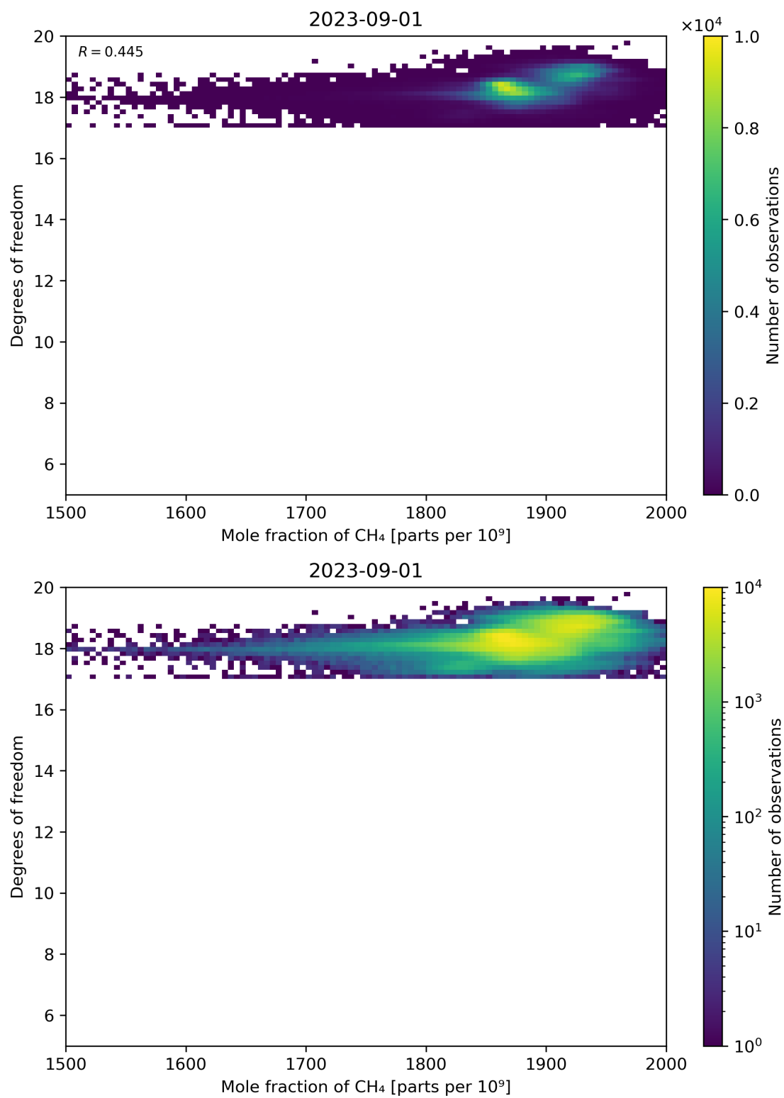
Figure 72: Scatter density plot of “Mole fraction of CH 4 ” against “Degrees of freedom” for 2023-08-31 to 2023-09-02.
