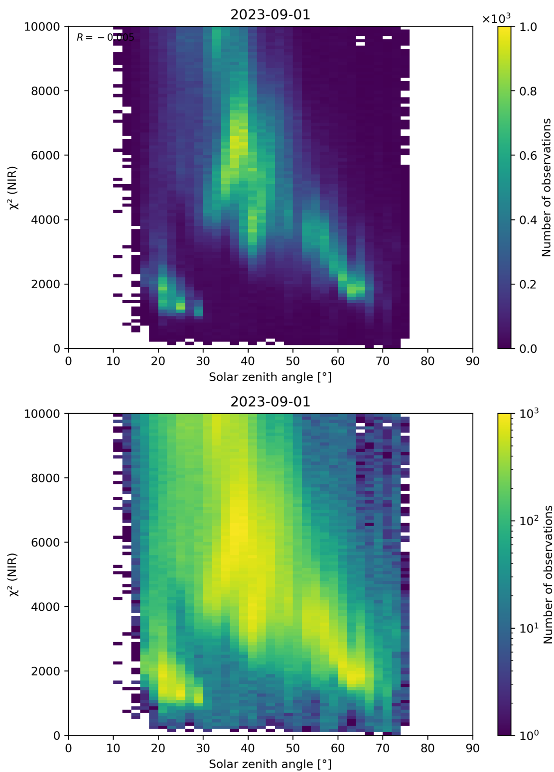
Figure 94: Scatter density plot of “Solar zenith angle” against “ \chi^2 (NIR)” for 2023-08-31 to 2023-09-02.
