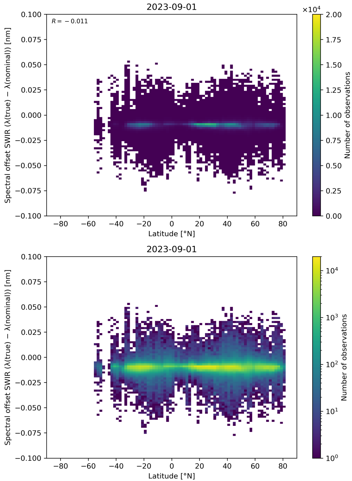
Figure 62: Scatter density plot of “Latitude” against “Spectral offset SWIR ( \lambda(\text{true}) - \lambda(\text{nominal}) )” for 2023-08-31 to 2023-09-02.
