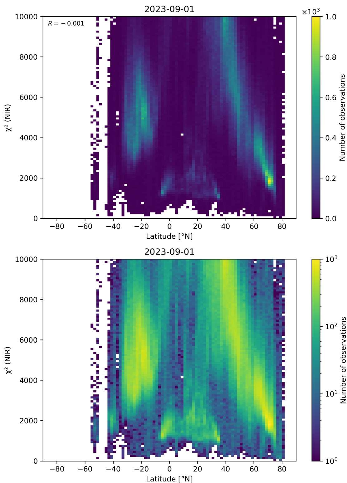
Figure 53: Scatter density plot of “Latitude” against “ \chi^2 (NIR)” for 2023-08-31 to 2023-09-02.
