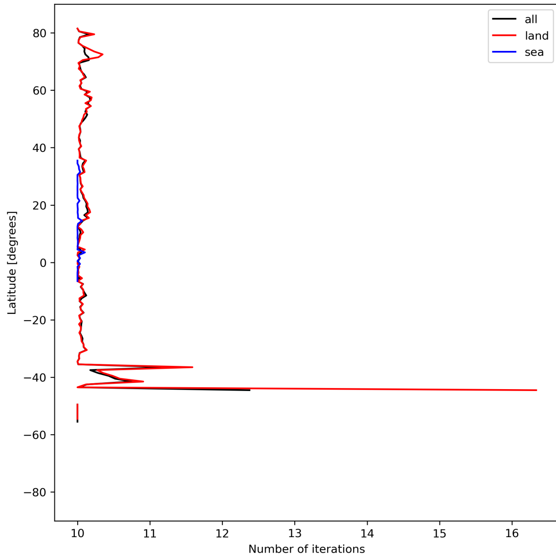
Figure 20: Zonal average of “Number of iterations” for 2023-08-31 to 2023-09-02.
