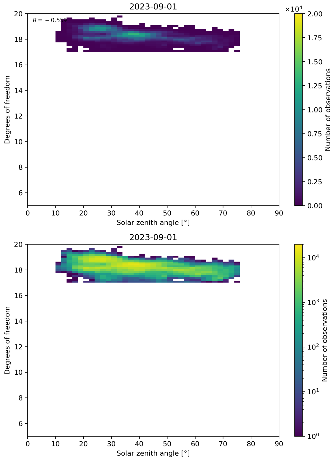
Figure 96: Scatter density plot of “Solar zenith angle” against “Degrees of freedom” for 2023-08-31 to 2023-09-02.
