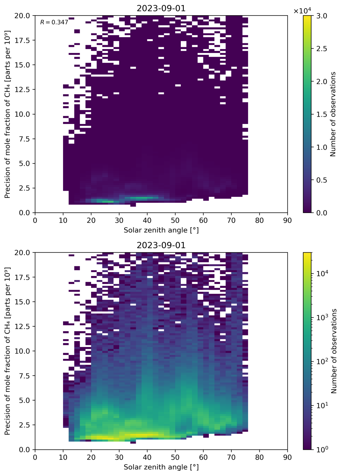
Figure 101: Scatter density plot of “Solar zenith angle” against “Precision of mole fraction of CH 4 ” for 2023-08-31 to 2023-09-02.
