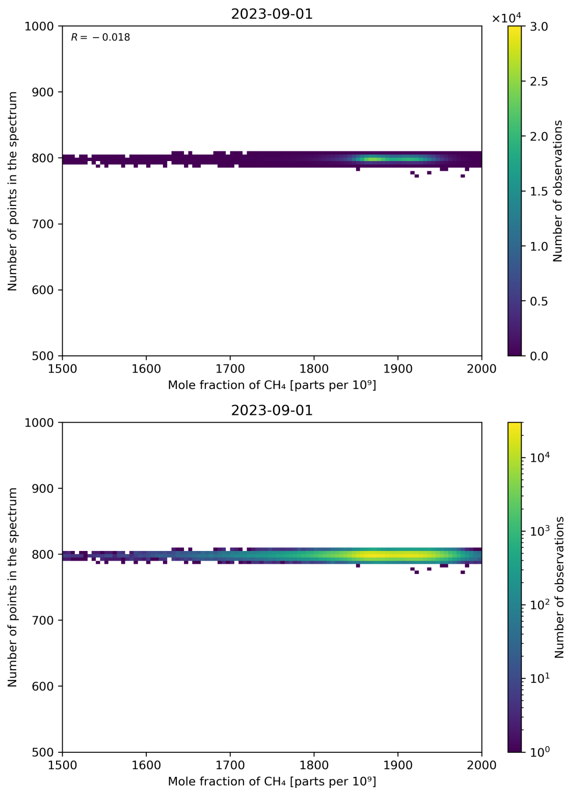
Figure 77: Scatter density plot of “Mole fraction of CH 4 ” against “Number of points in the spectrum” for 2023-08-31 to 2023-09-02.
