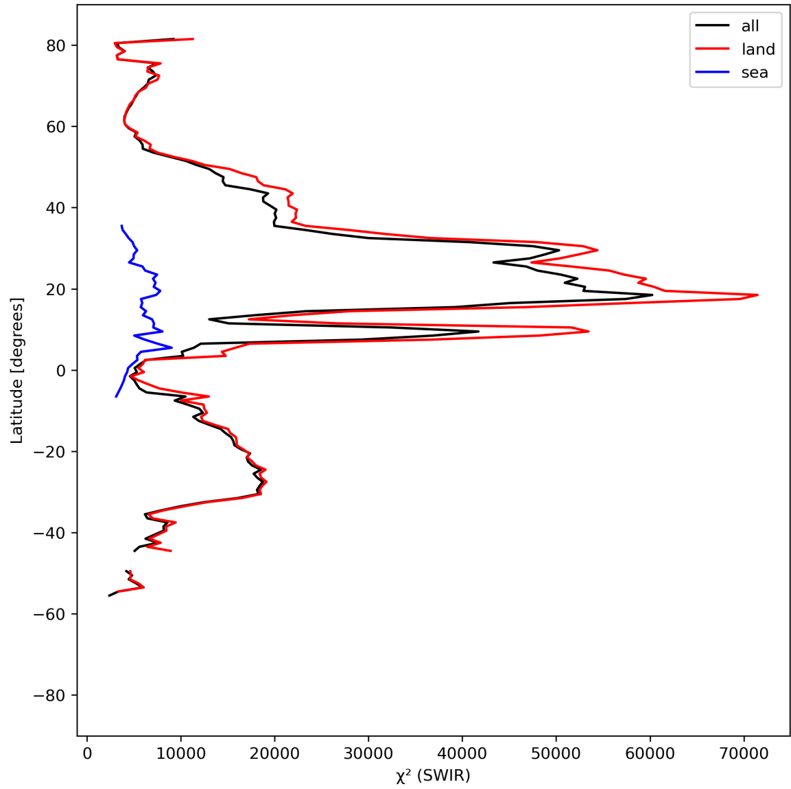
Figure 17: Zonal average of “ \chi^2 (SWIR)” for 2023-08-31 to 2023-09-02.
