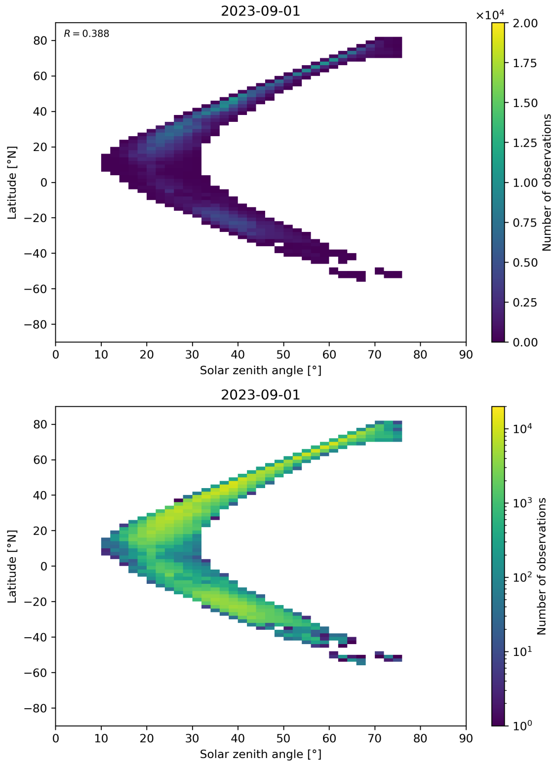
Figure 98: Scatter density plot of “Solar zenith angle” against “Latitude” for 2023-08-31 to 2023-09-02.
