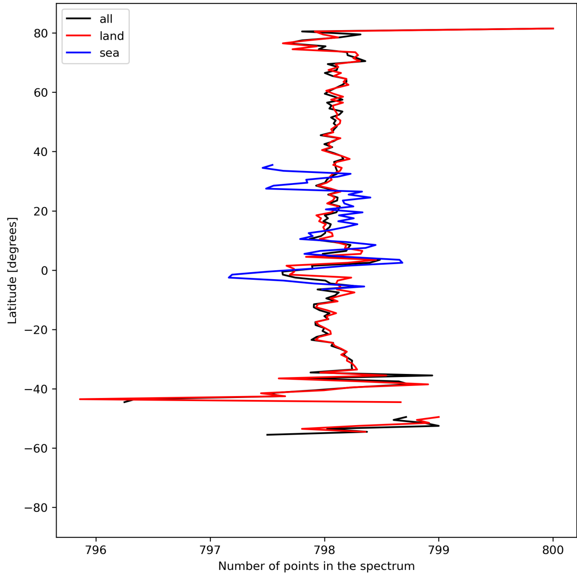
Figure 15: Zonal average of “Number of points in the spectrum” for 2023-08-31 to 2023-09-02.
