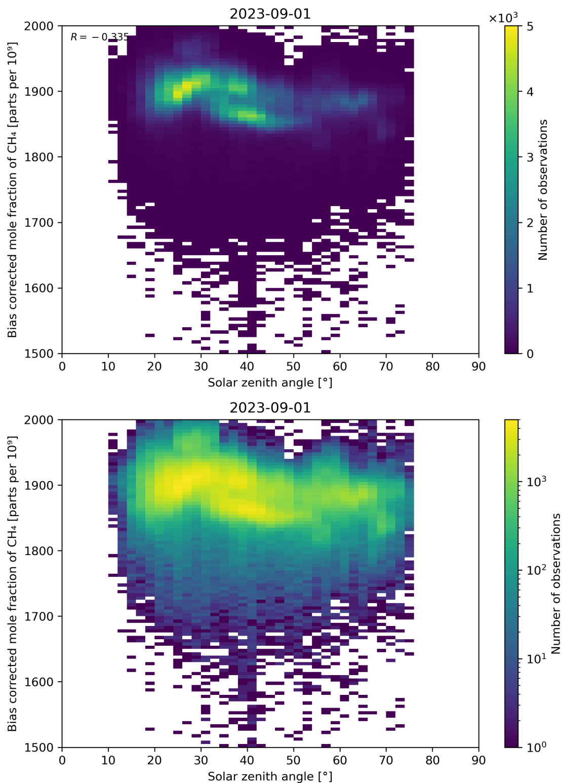
Figure 100: Scatter density plot of “Solar zenith angle” against “Bias corrected mole fraction of CH 4 ” for 2023-08-31 to 2023-09-02.
