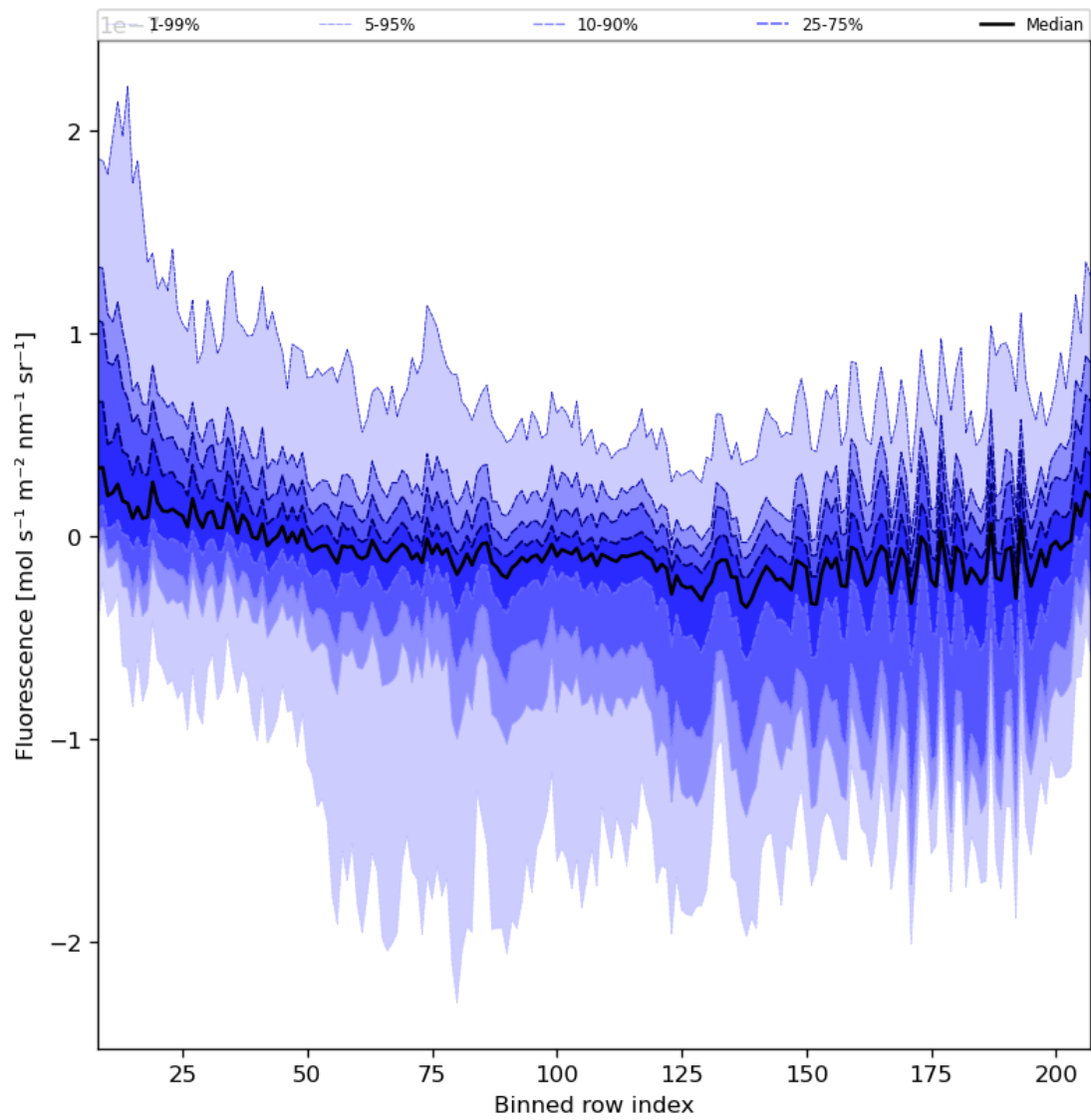
Figure 43: Along track statistics of “Fluorescence” for 2023-08-31 to 2023-09-02
