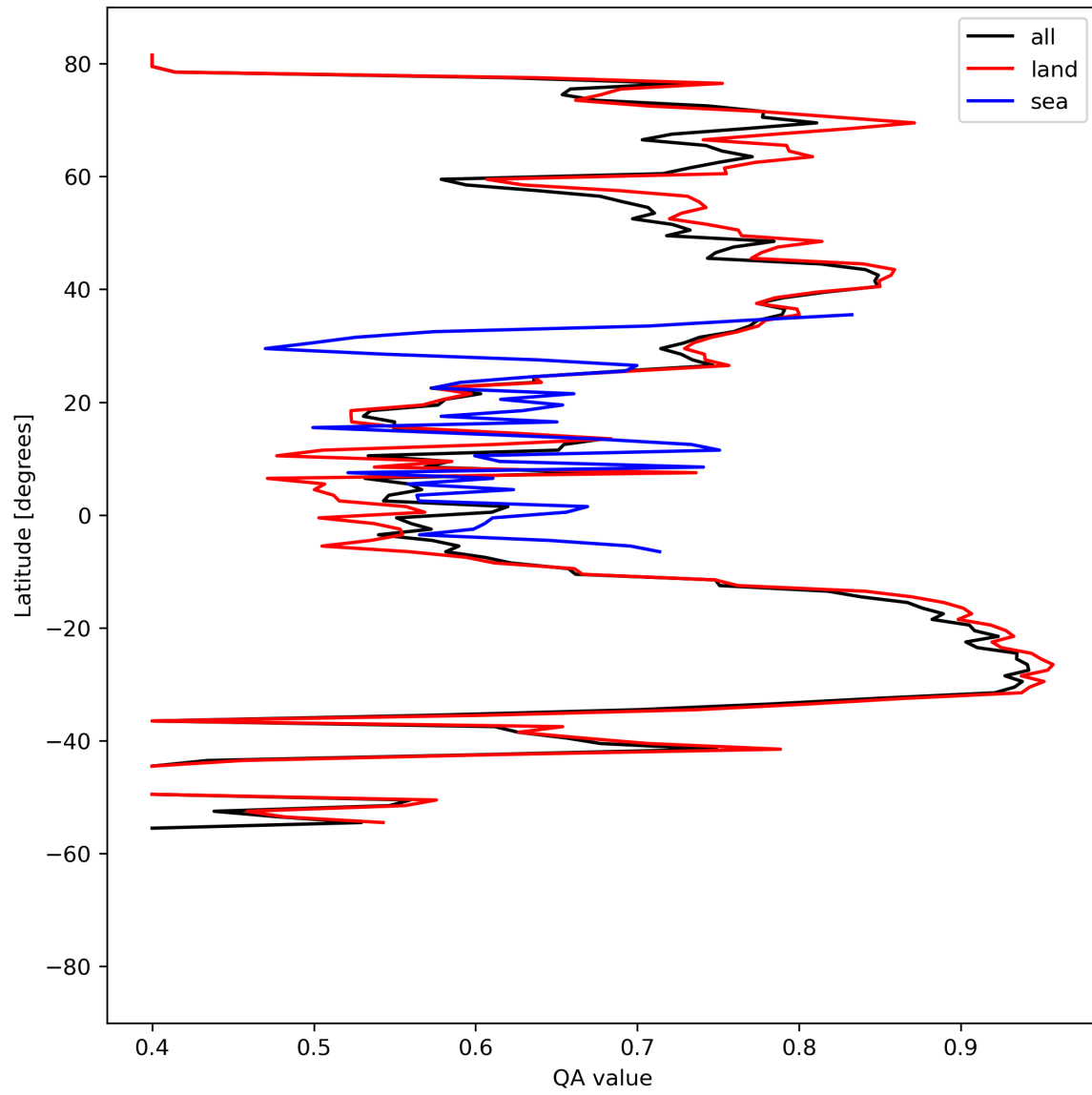
Figure 11: Zonal average of “QA value” for 2023-08-31 to 2023-09-02.
