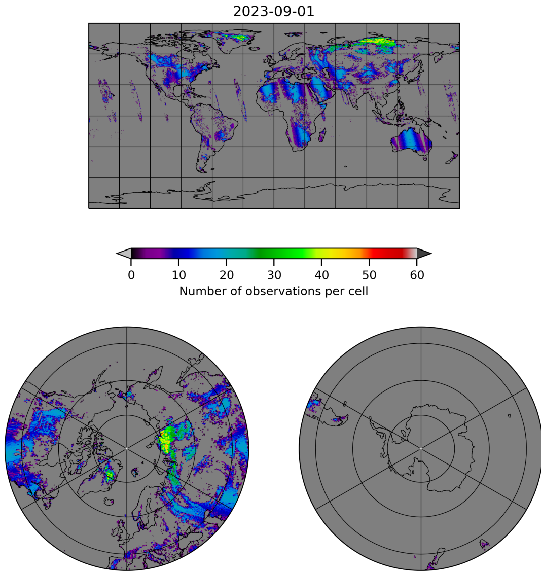
Figure 10: Map of the number of observations for 2023-08-31 to 2023-09-02
