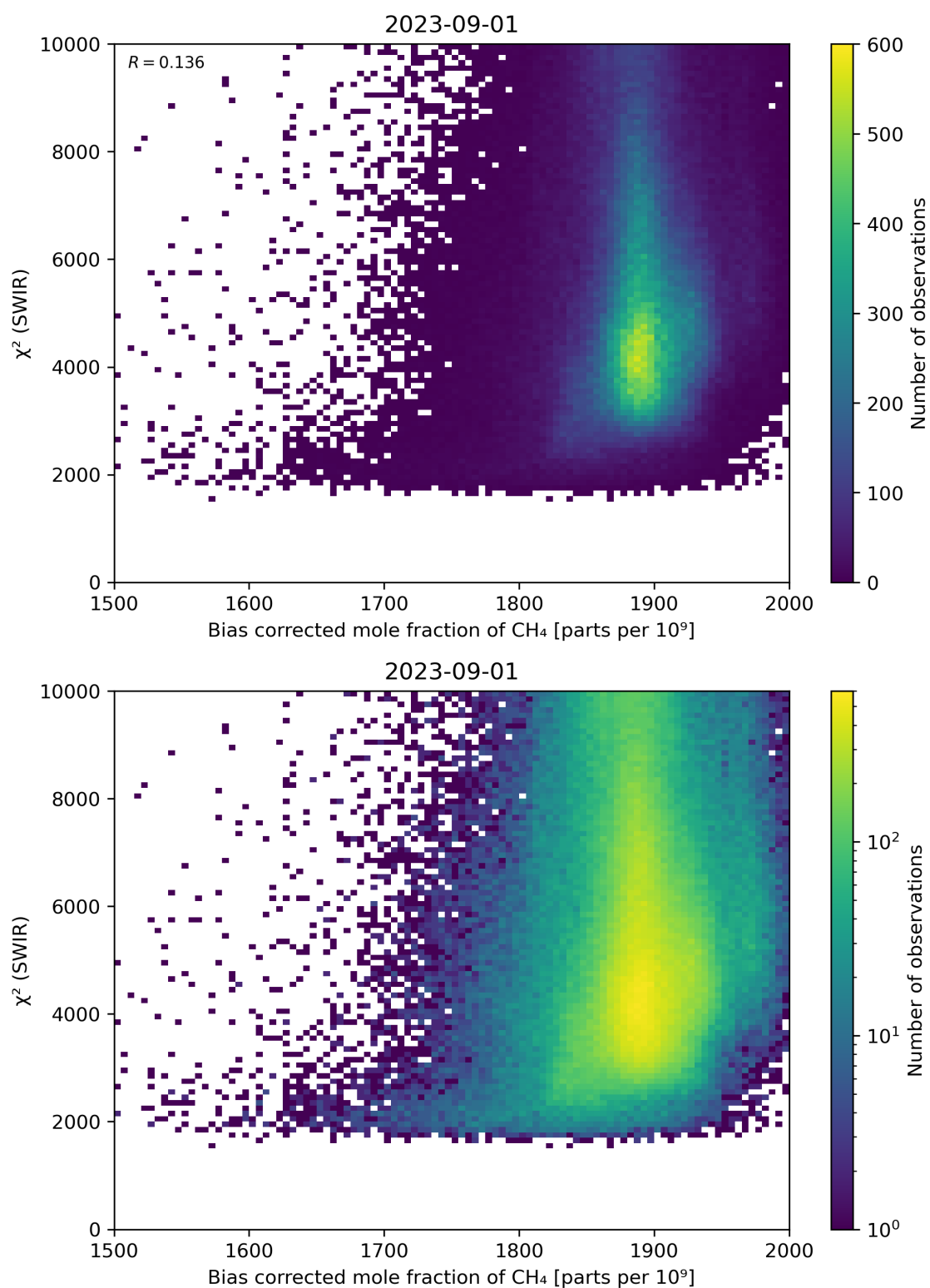
Figure 64: Scatter density plot of “Bias corrected mole fraction of \text{CH}_4 ” against “ \chi^2 (SWIR)” for 2023-08-31 to 2023-09-02.
