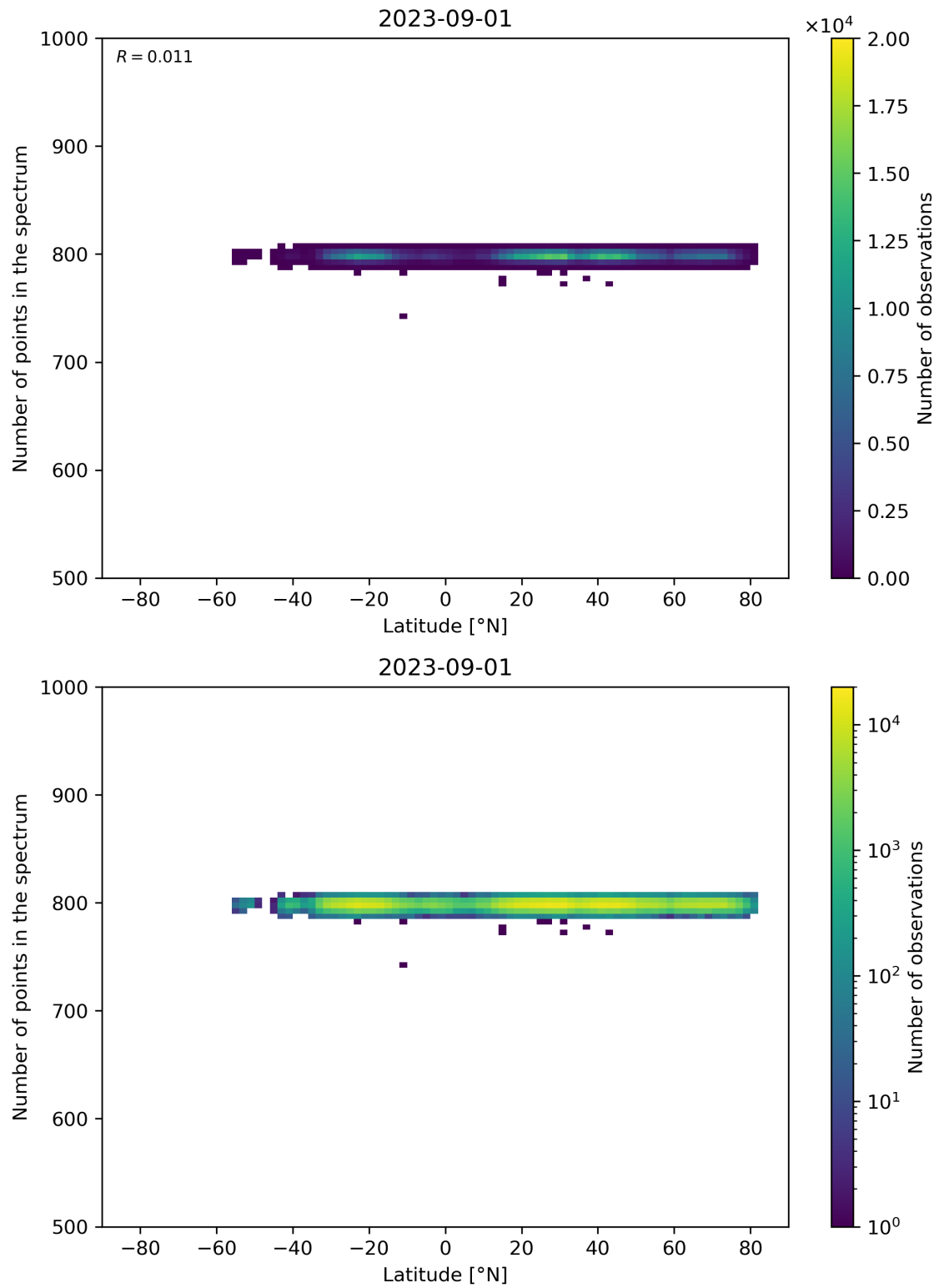
Figure 61: Scatter density plot of “Latitude” against “Number of points in the spectrum” for 2023-08-31 to 2023-09-02.
