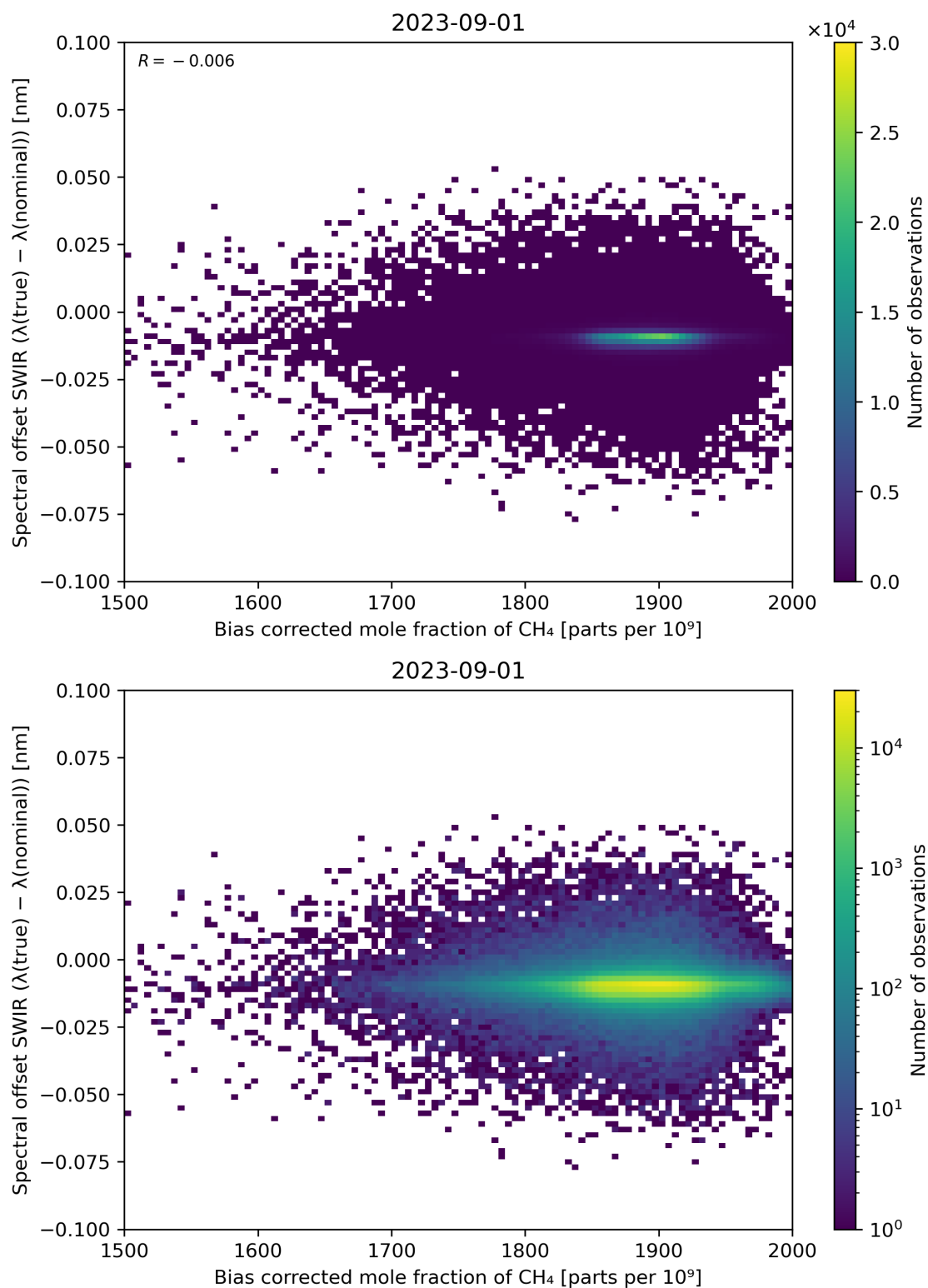
Figure 69: Scatter density plot of “Bias corrected mole fraction of \text{CH}_4 ” against “Spectral offset SWIR ( \lambda(\text{true}) - \lambda(\text{nominal}) )” for 2023-08-31 to 2023-09-02.
