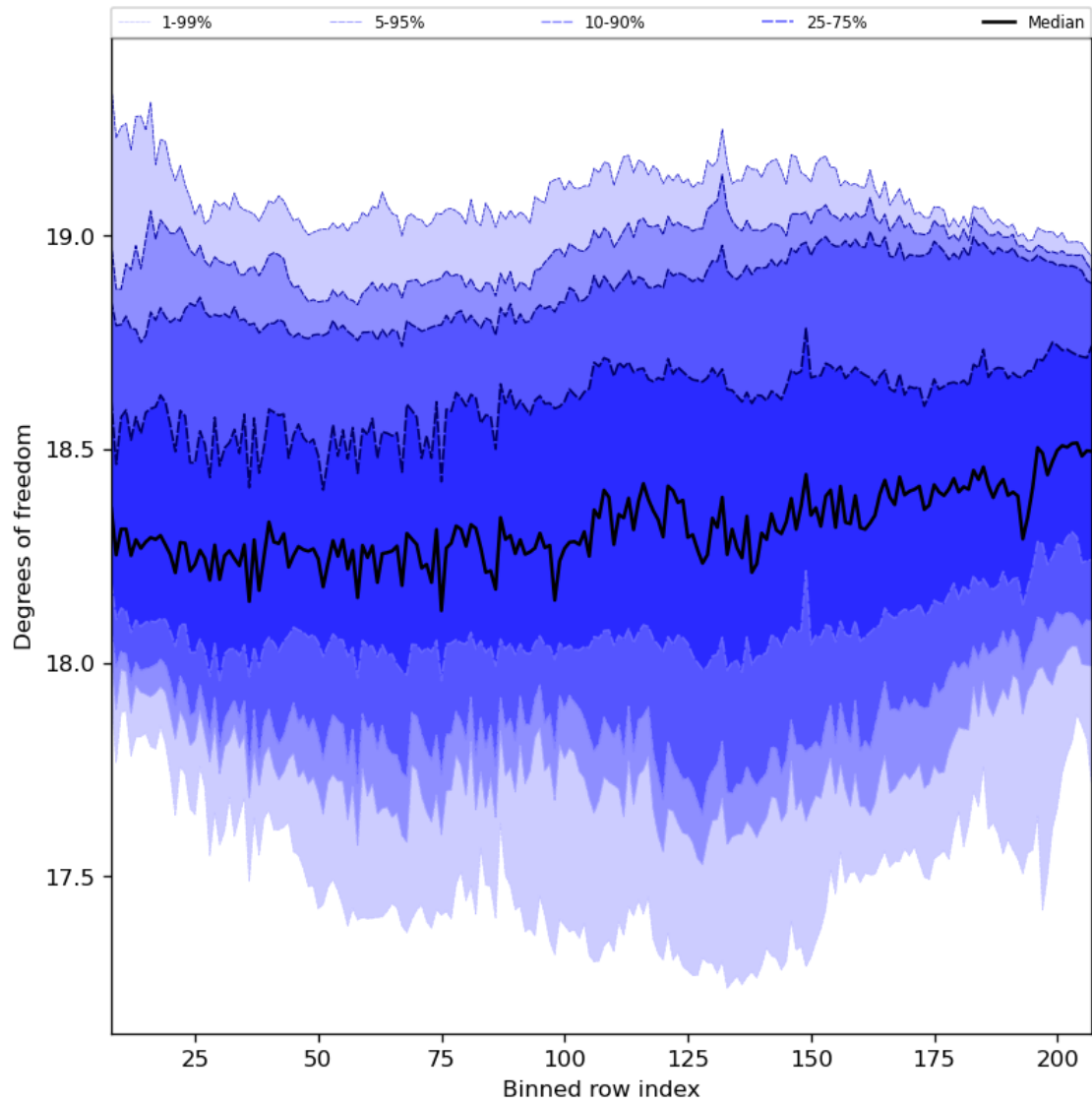
Figure 41: Along track statistics of “Degrees of freedom” for 2023-08-31 to 2023-09-02
