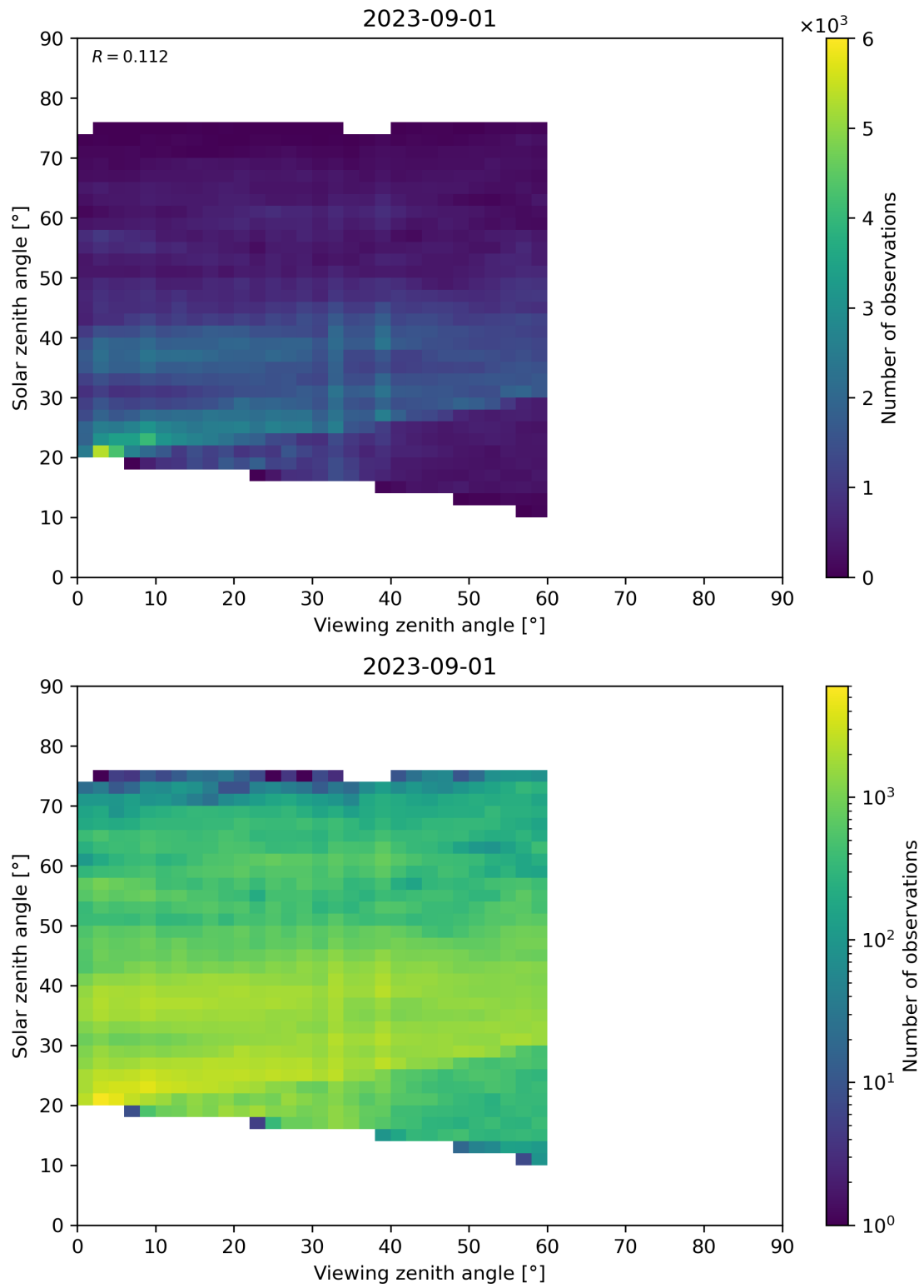
Figure 115: Scatter density plot of “Viewing zenith angle” against “Solar zenith angle” for 2023-08-31 to 2023-09-02.
