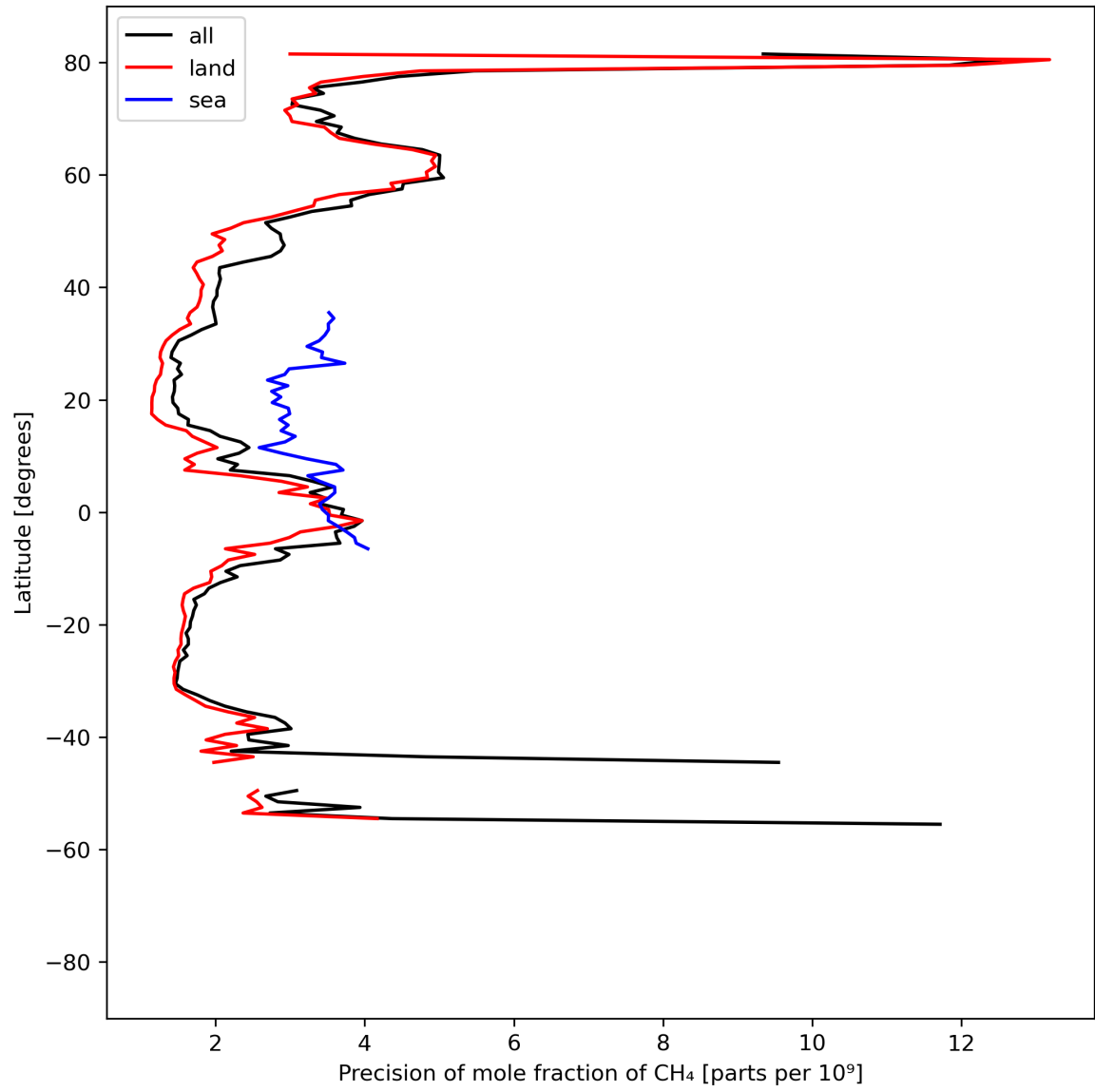
Figure 13: Zonal average of “Precision of mole fraction of CH 4 ” for 2023-08-31 to 2023-09-02.
