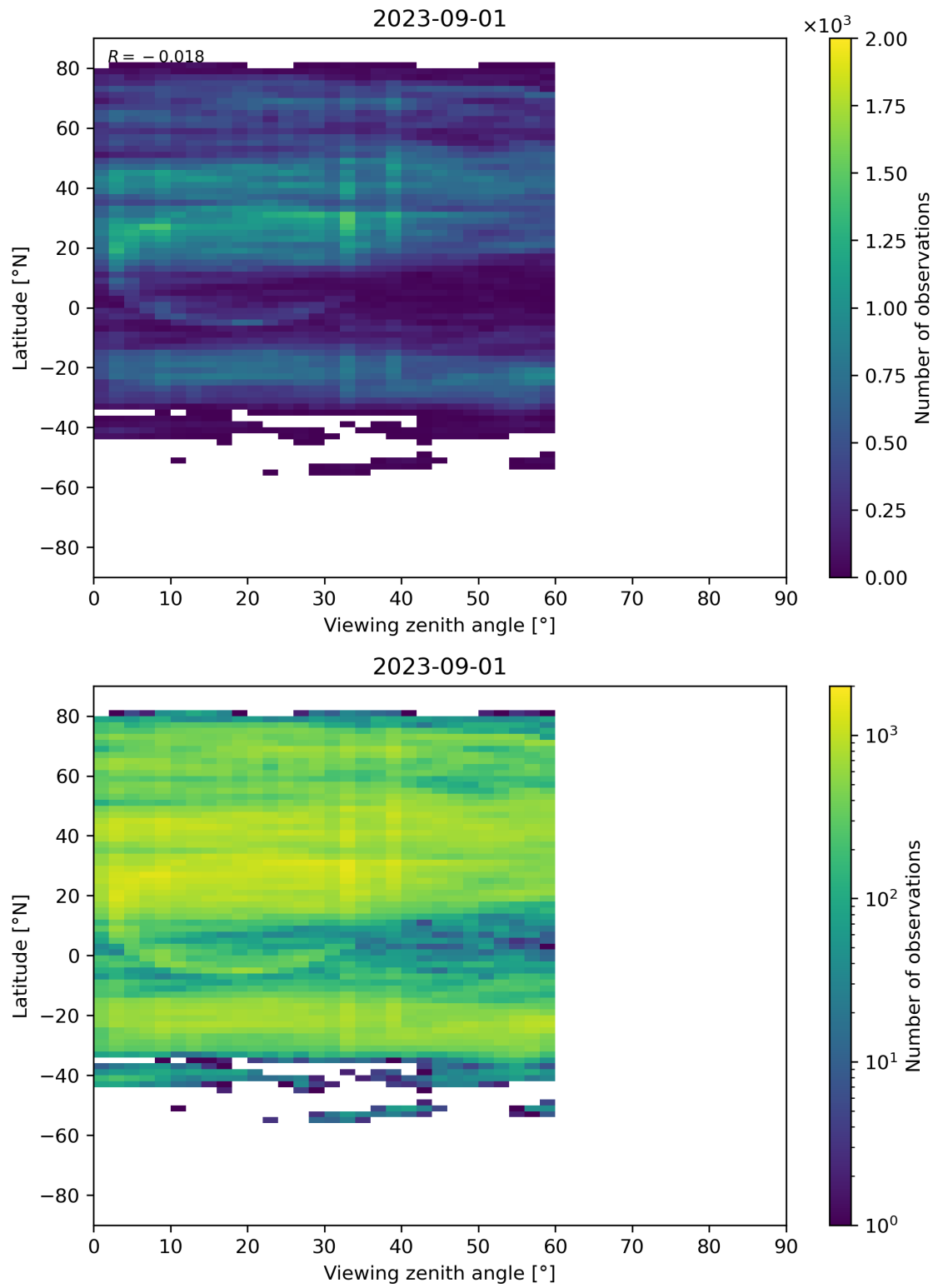
Figure 109: Scatter density plot of “Viewing zenith angle” against “Latitude” for 2023-08-31 to 2023-09-02.
