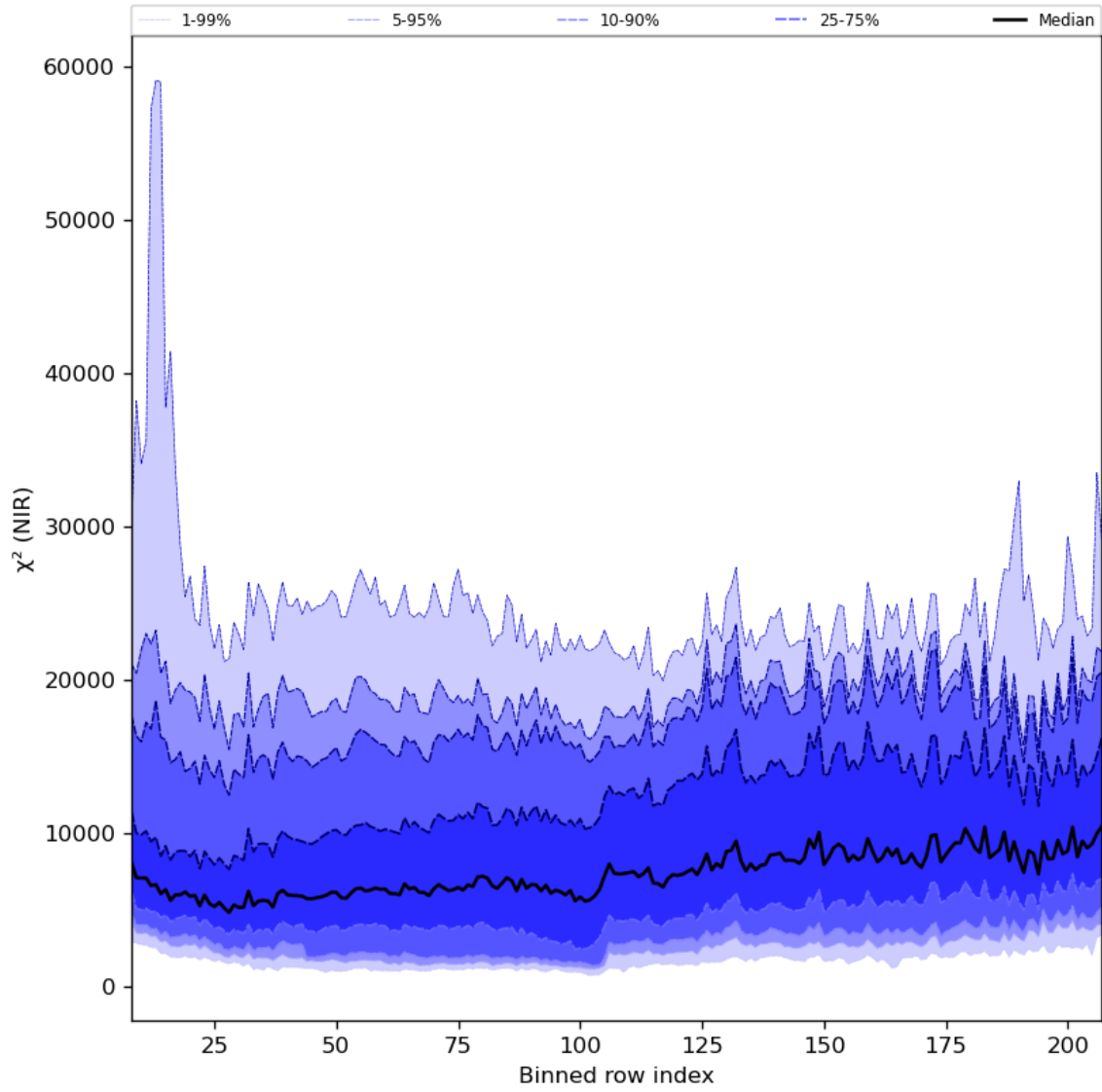
Figure 40: Along track statistics of “ \chi^2 (NIR)” for 2023-08-31 to 2023-09-02
