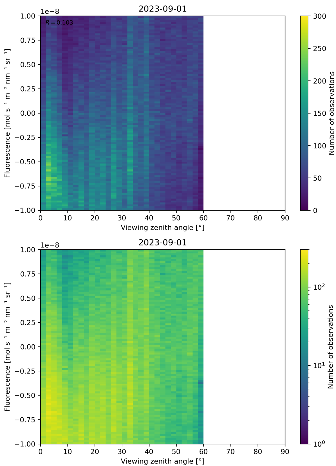
Figure 108: Scatter density plot of “Viewing zenith angle” against “Fluorescence” for 2023-08-31 to 2023-09-02.
