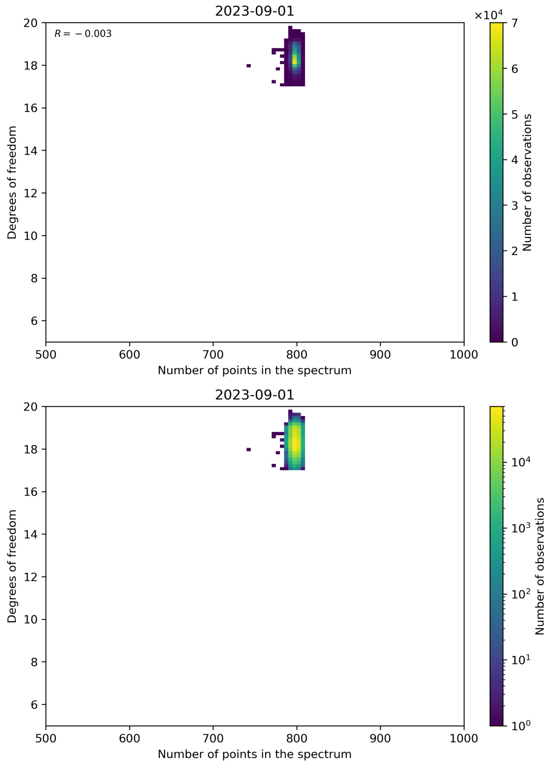
Figure 90: Scatter density plot of “Number of points in the spectrum” against “Degrees of freedom” for 2023-08-31 to 2023-09-02.
