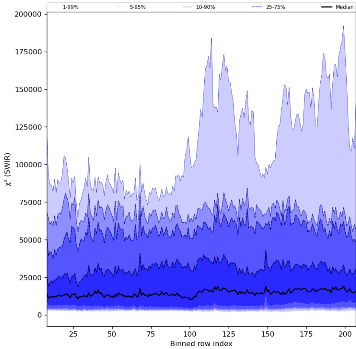
Figure 39: Along track statistics of “ \chi^2 (SWIR)” for 2023-08-31 to 2023-09-02
