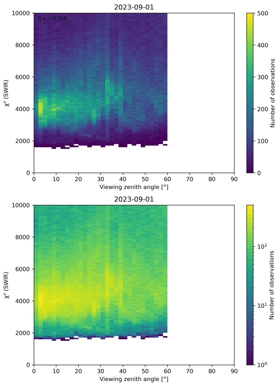
Figure 106: Scatter density plot of “Viewing zenith angle” against “ \chi^2 (SWIR)” for 2023-08-31 to 2023-09-02.
