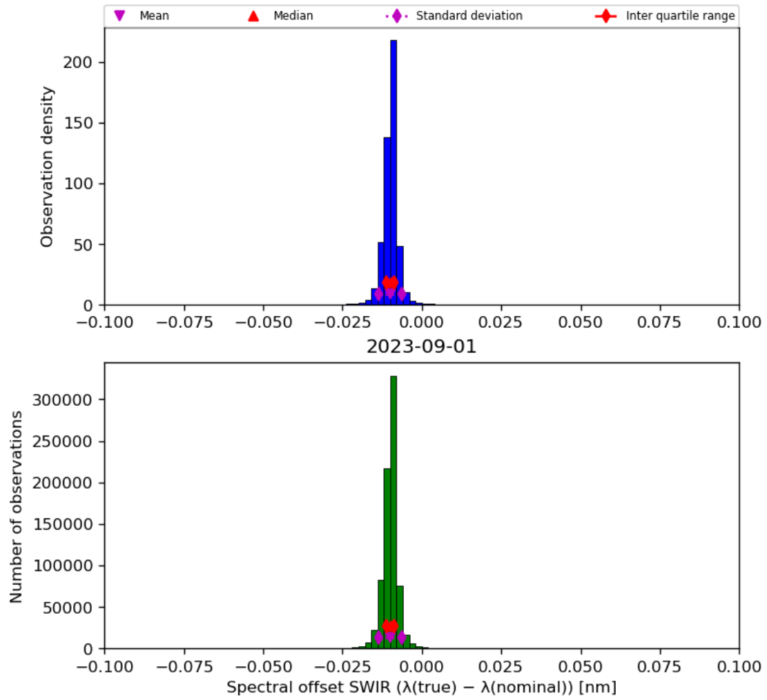
Figure 27: Histogram of “Spectral offset SWIR ( \lambda(\text{true}) - \lambda(\text{nominal}) )” for 2023-08-31 to 2023-09-02
