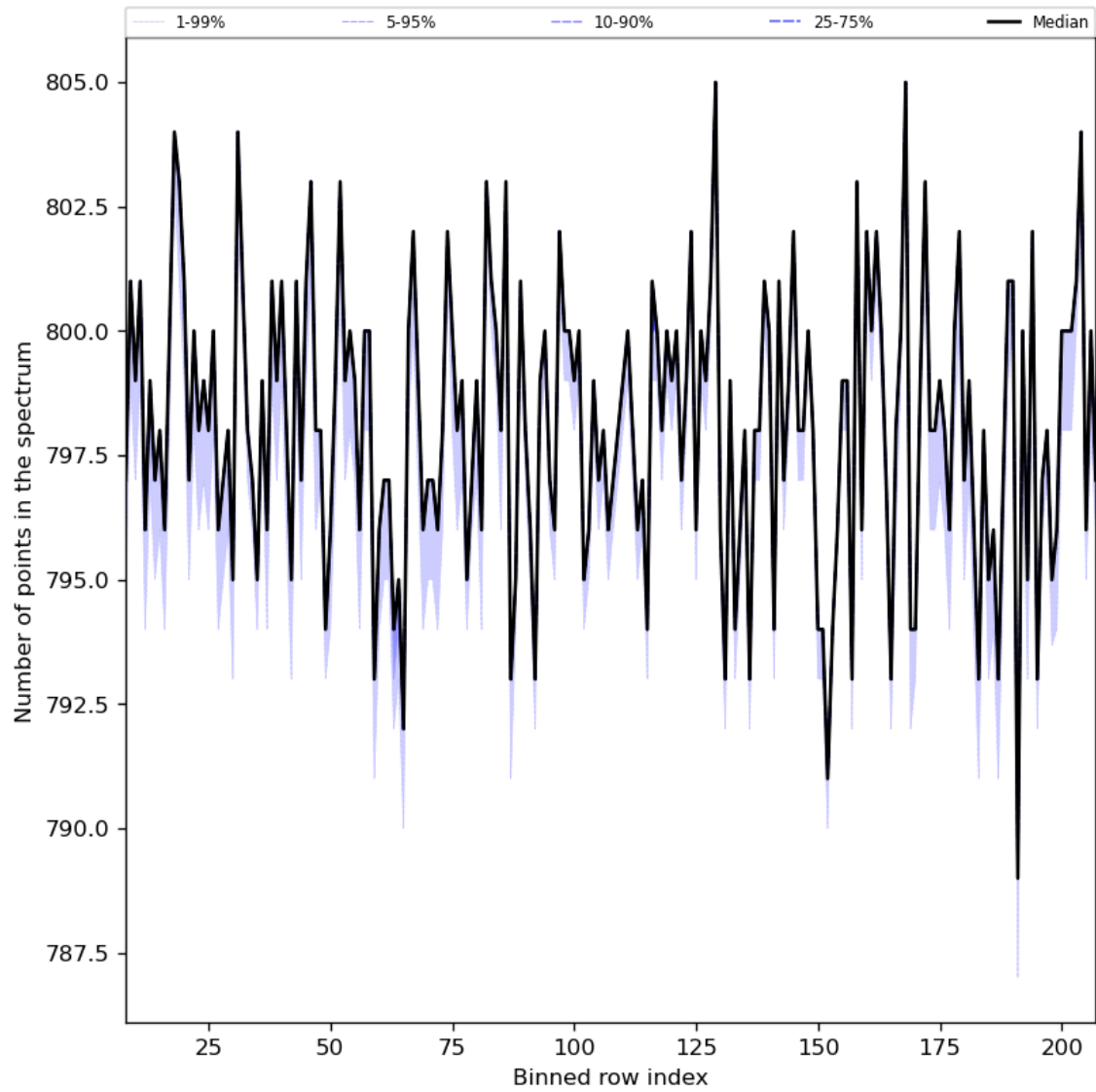
Figure 37: Along track statistics of “Number of points in the spectrum” for 2023-08-31 to 2023-09-02
