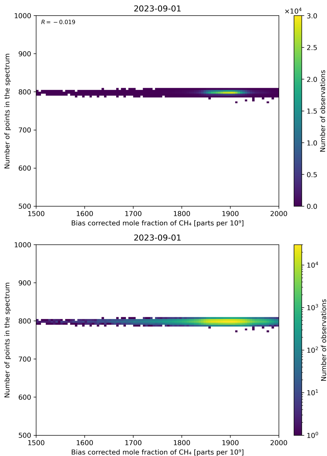
Figure 68: Scatter density plot of “Bias corrected mole fraction of CH 4 ” against “Number of points in the spectrum” for 2023-08-31 to 2023-09-02.
