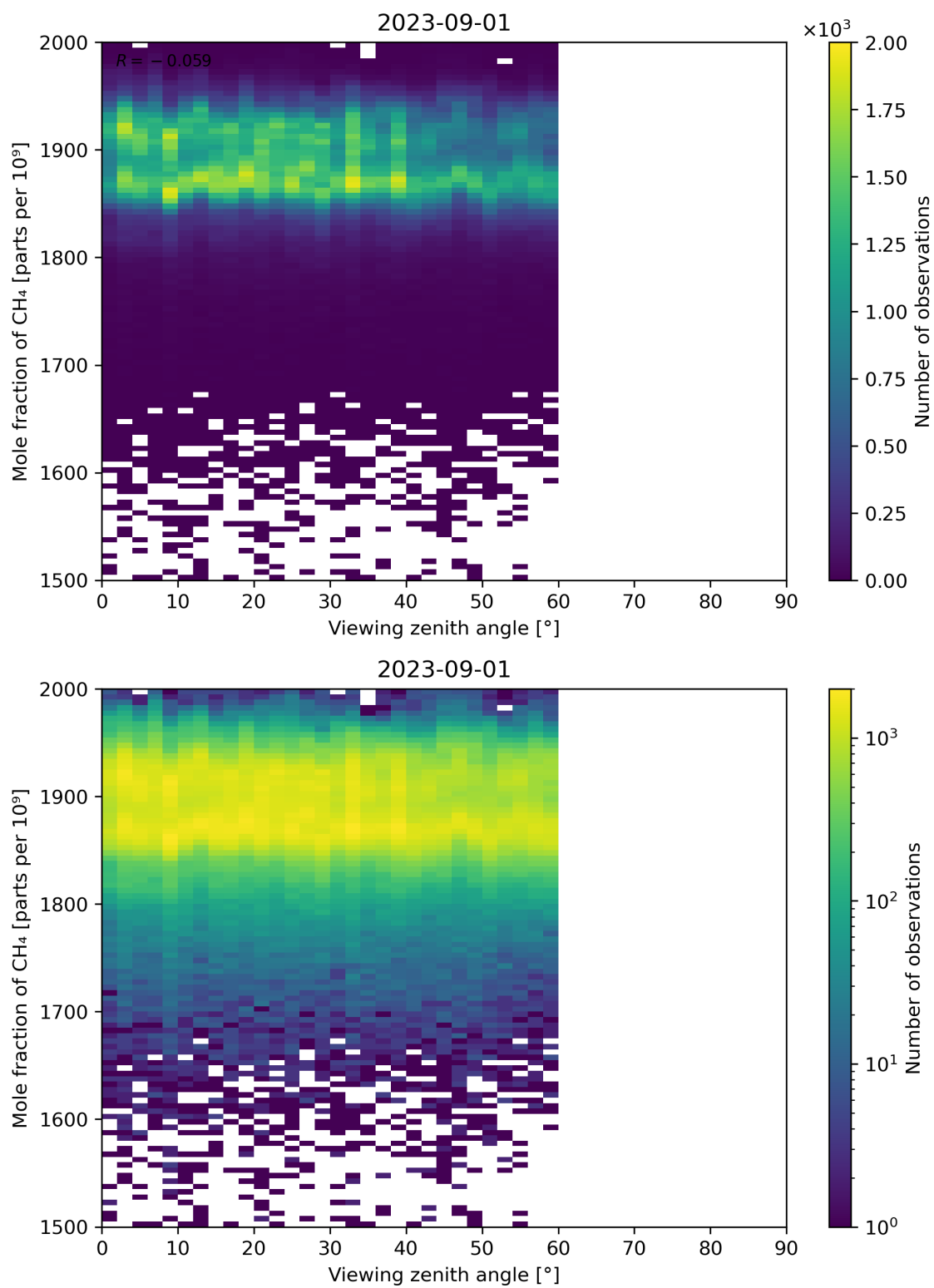
Figure 110: Scatter density plot of “Viewing zenith angle” against “Mole fraction of CH 4 ” for 2023-08-31 to 2023-09-02.
