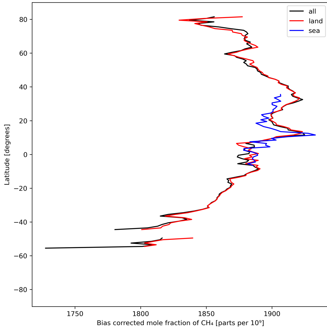
Figure 14: Zonal average of “Bias corrected mole fraction of CH 4 ” for 2023-08-31 to 2023-09-02.
