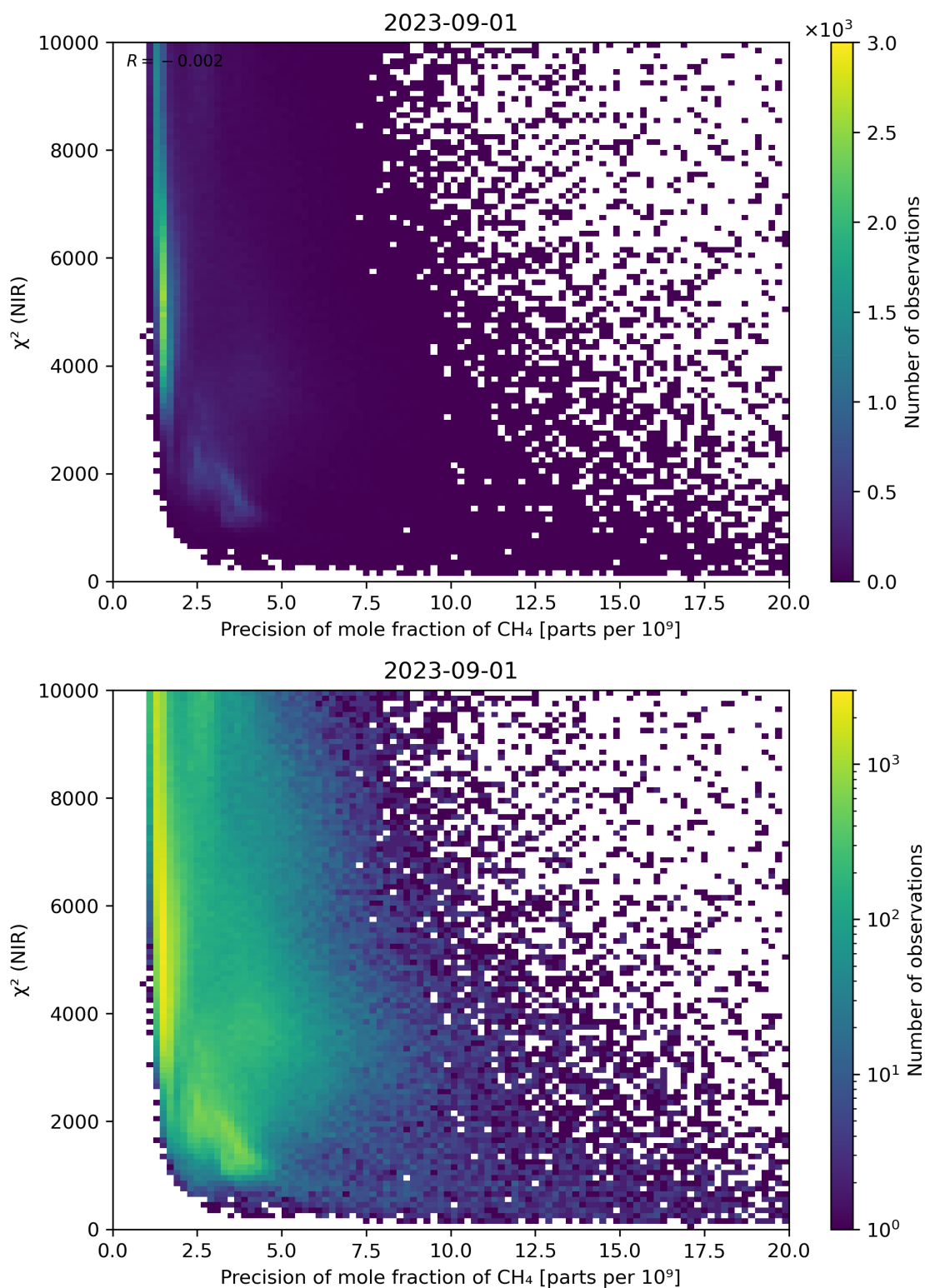
Figure 78: Scatter density plot of “Precision of mole fraction of CH 4 ” against “ \chi^2 (NIR)” for 2023-08-31 to 2023-09-02.
