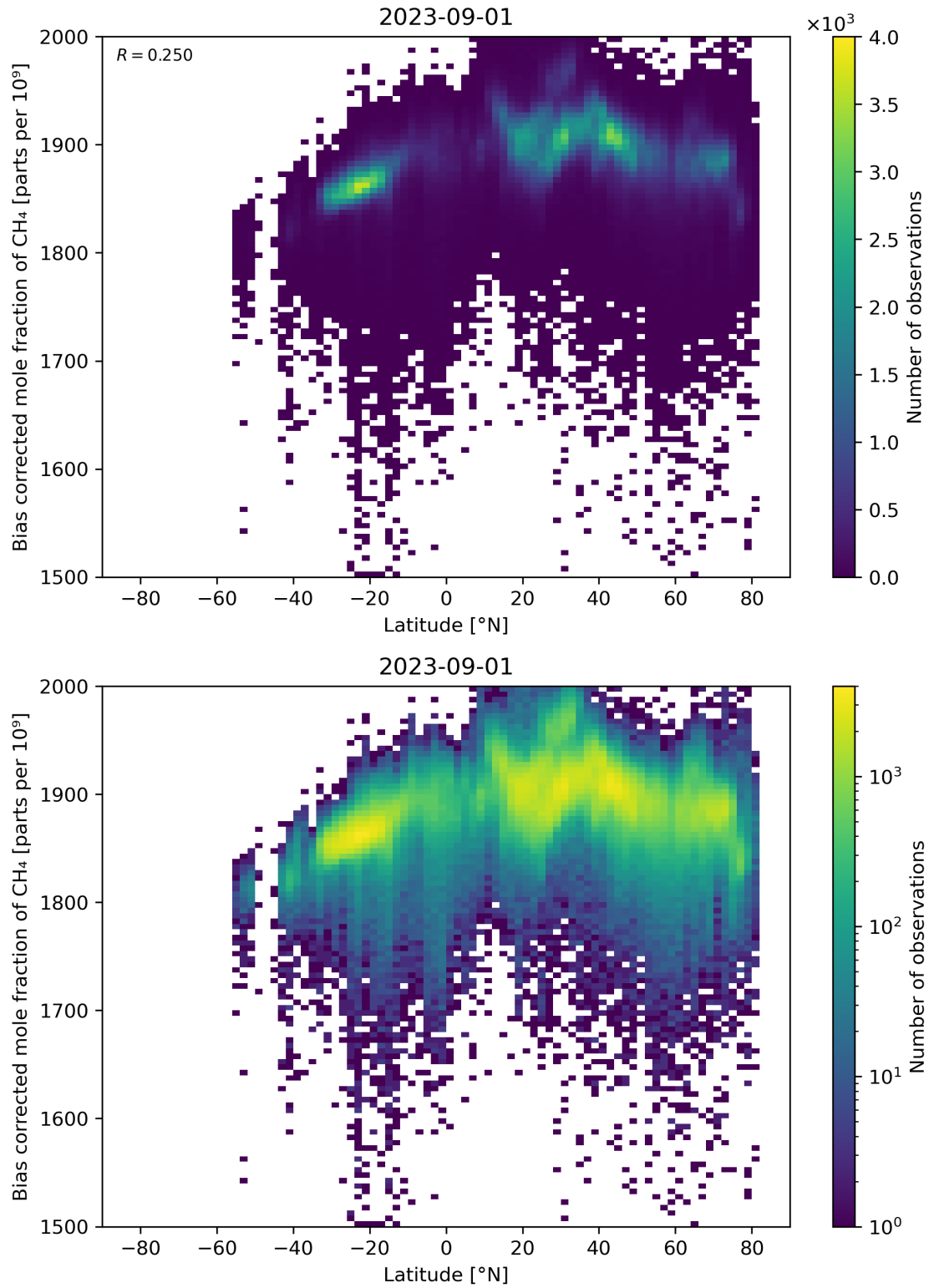
Figure 58: Scatter density plot of “Latitude” against “Bias corrected mole fraction of \text{CH}_4 ” for 2023-08-31 to 2023-09-02.
