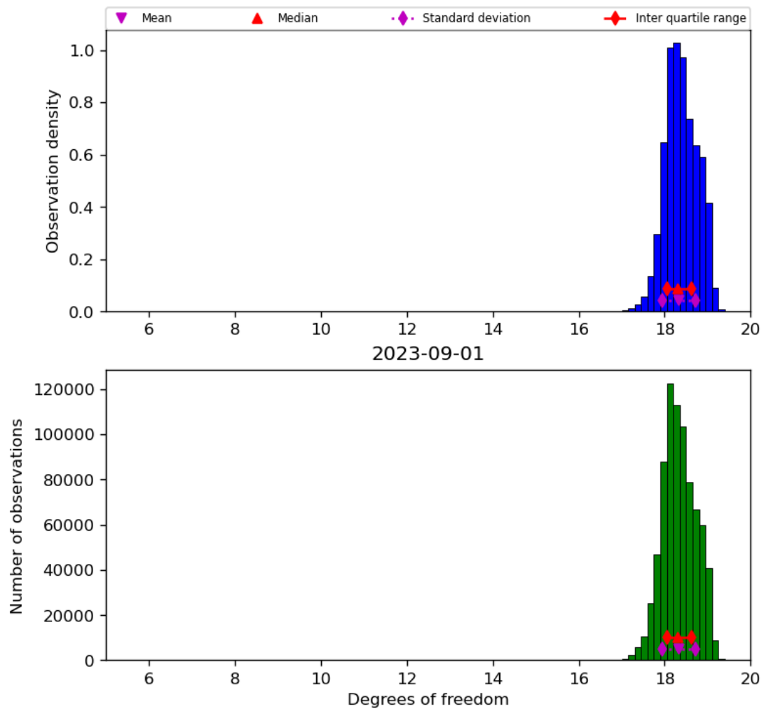
Figure 30: Histogram of “Degrees of freedom” for 2023-08-31 to 2023-09-02
