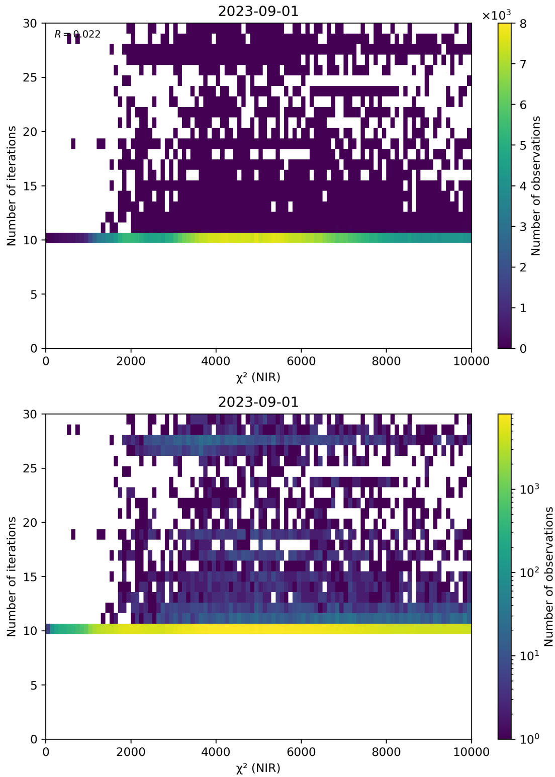
Figure 46: Scatter density plot of “ \chi^2 (NIR)” against “Number of iterations” for 2023-08-31 to 2023-09-02.
