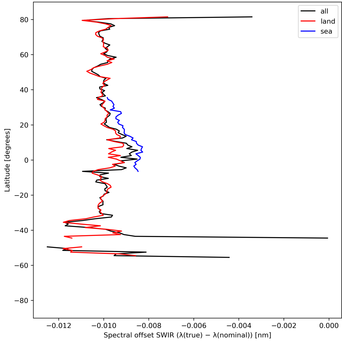
Figure 16: Zonal average of “Spectral offset SWIR ( \lambda(\text{true}) - \lambda(\text{nominal}) )” for 2023-08-31 to 2023-09-02.
