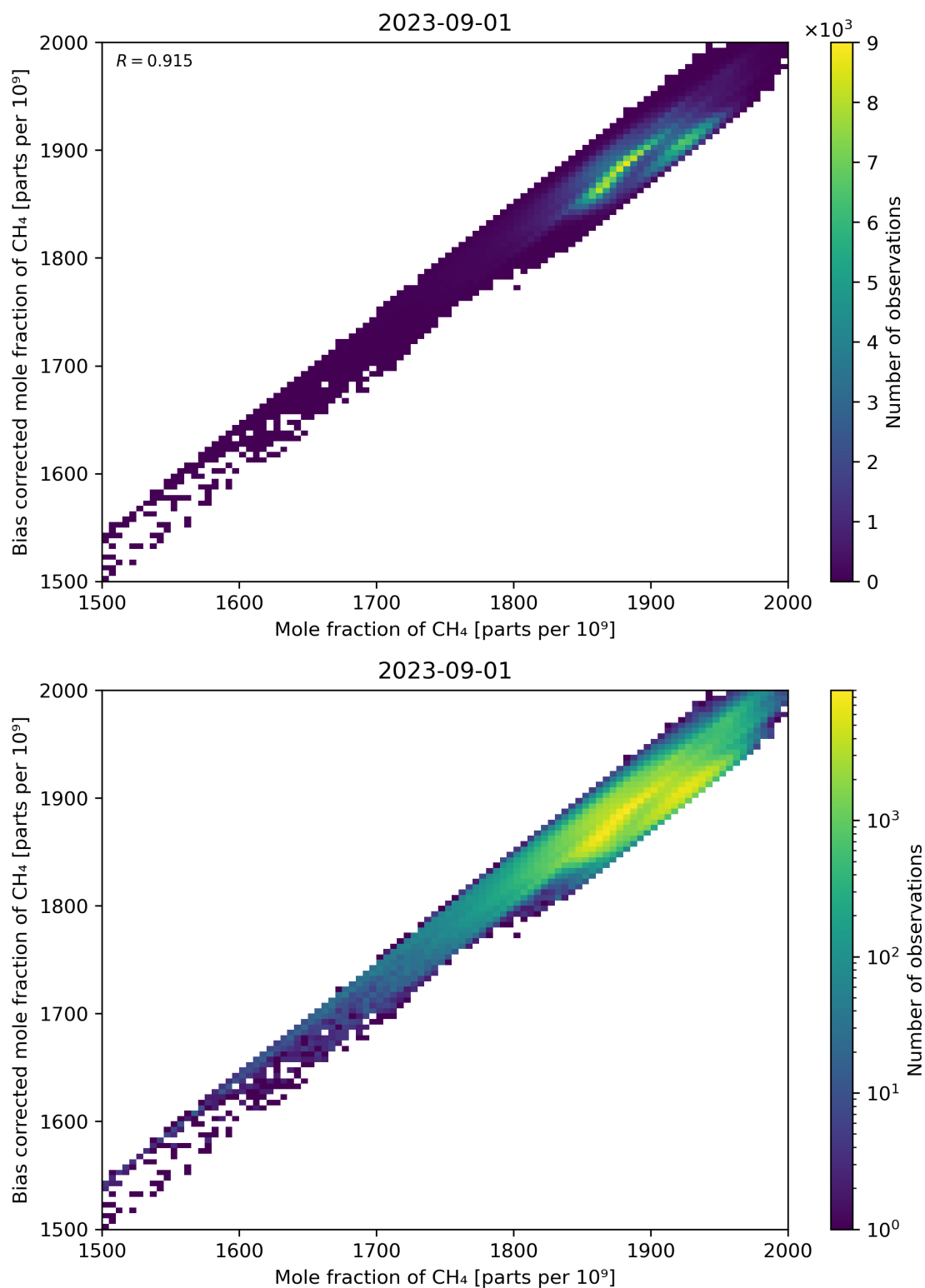
Figure 74: Scatter density plot of “Mole fraction of CH 4 ” against “Bias corrected mole fraction of CH 4 ” for 2023-08-31 to 2023-09-02.
