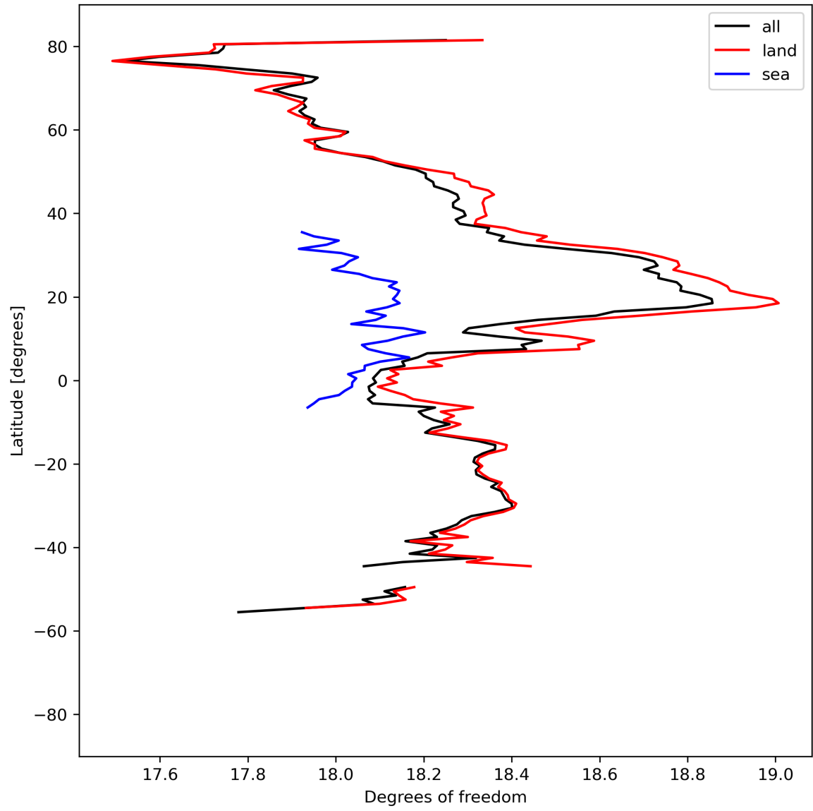
Figure 19: Zonal average of “Degrees of freedom” for 2023-08-31 to 2023-09-02.
