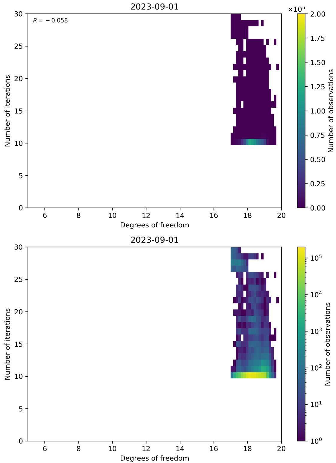
Figure 52: Scatter density plot of “Degrees of freedom” against “Number of iterations” for 2023-08-31 to 2023-09-02.
