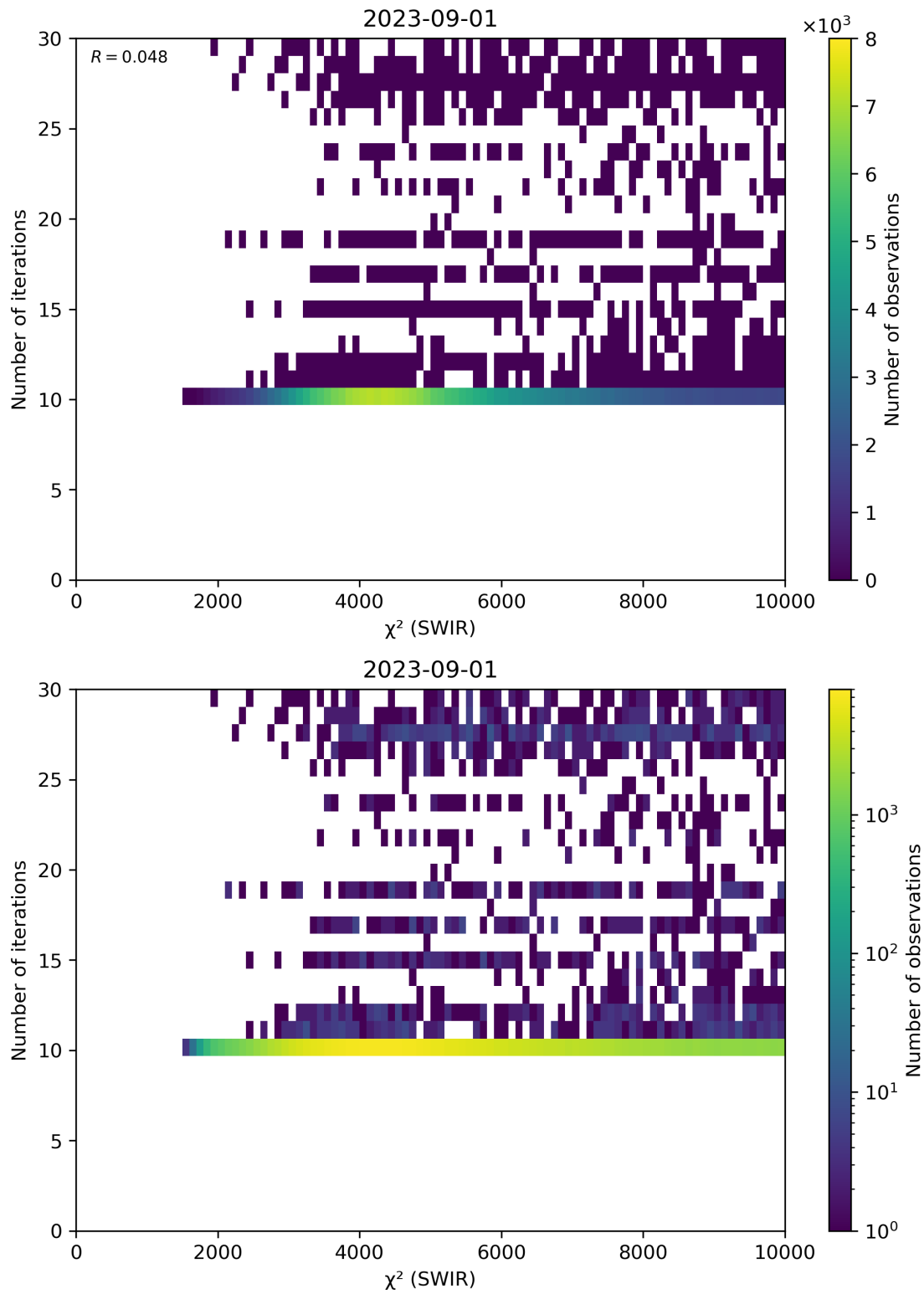
Figure 50: Scatter density plot of " \chi^2 (SWIR)" against "Number of iterations" for 2023-08-31 to 2023-09-02.
