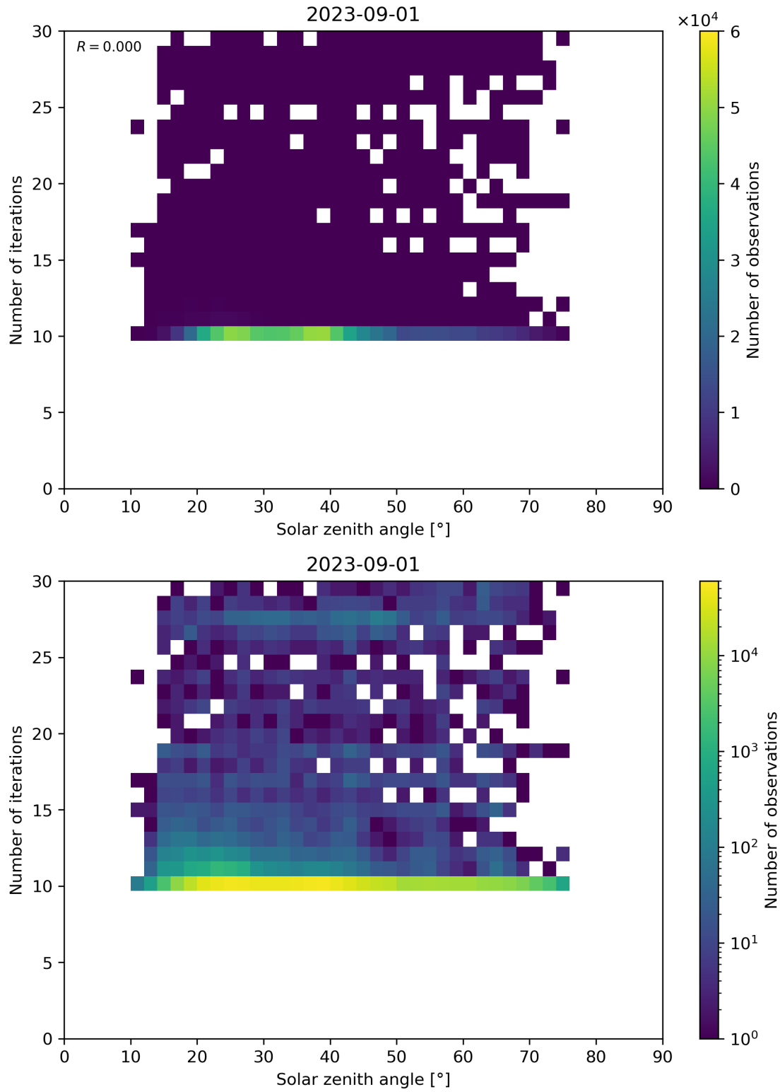
Figure 102: Scatter density plot of “Solar zenith angle” against “Number of iterations” for 2023-08-31 to 2023-09-02.
