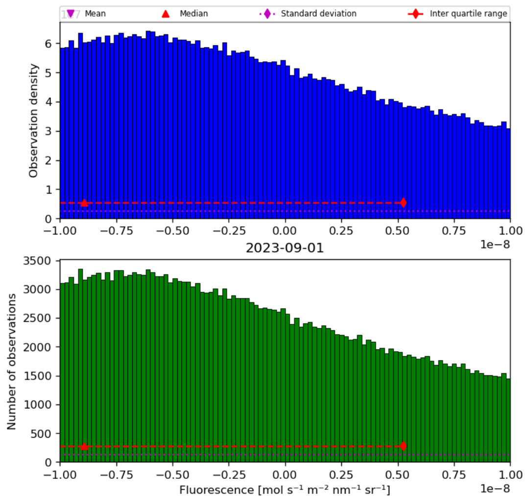
Figure 32: Histogram of “Fluorescence” for 2023-08-31 to 2023-09-02
