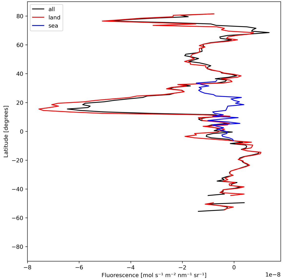
Figure 21: Zonal average of “Fluorescence” for 2023-08-31 to 2023-09-02.
