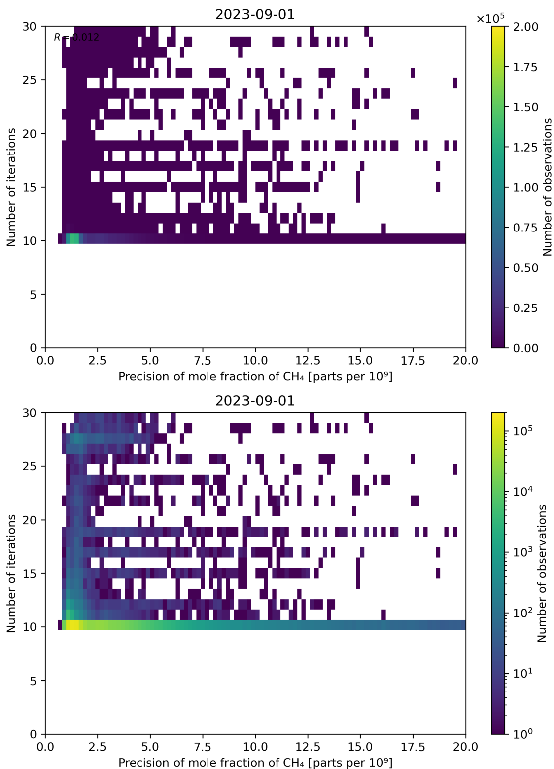
Figure 83: Scatter density plot of “Precision of mole fraction of CH 4 ” against “Number of iterations” for 2023-08-31 to 2023-09-02.
