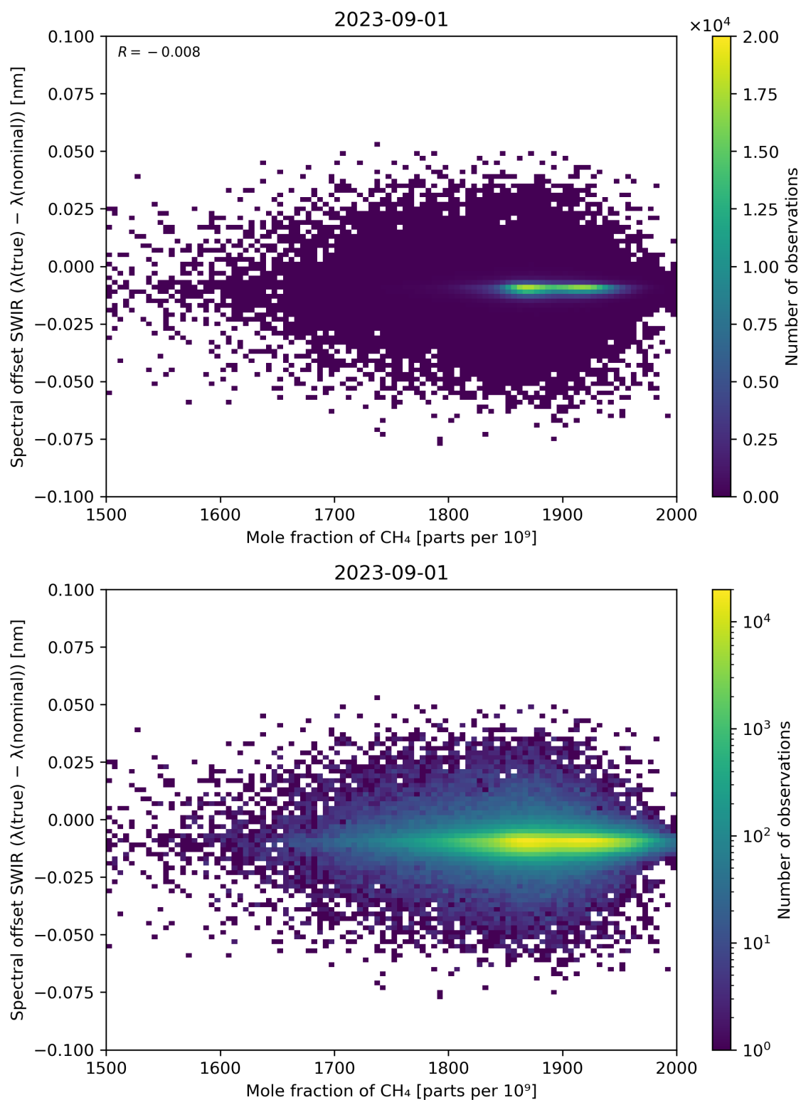
Figure 86: Scatter density plot of “Mole fraction of CH 4 ” against “Spectral offset SWIR ( \lambda(\text{true}) - \lambda(\text{nominal}) )” for 2023-08-31 to 2023-09-02.
