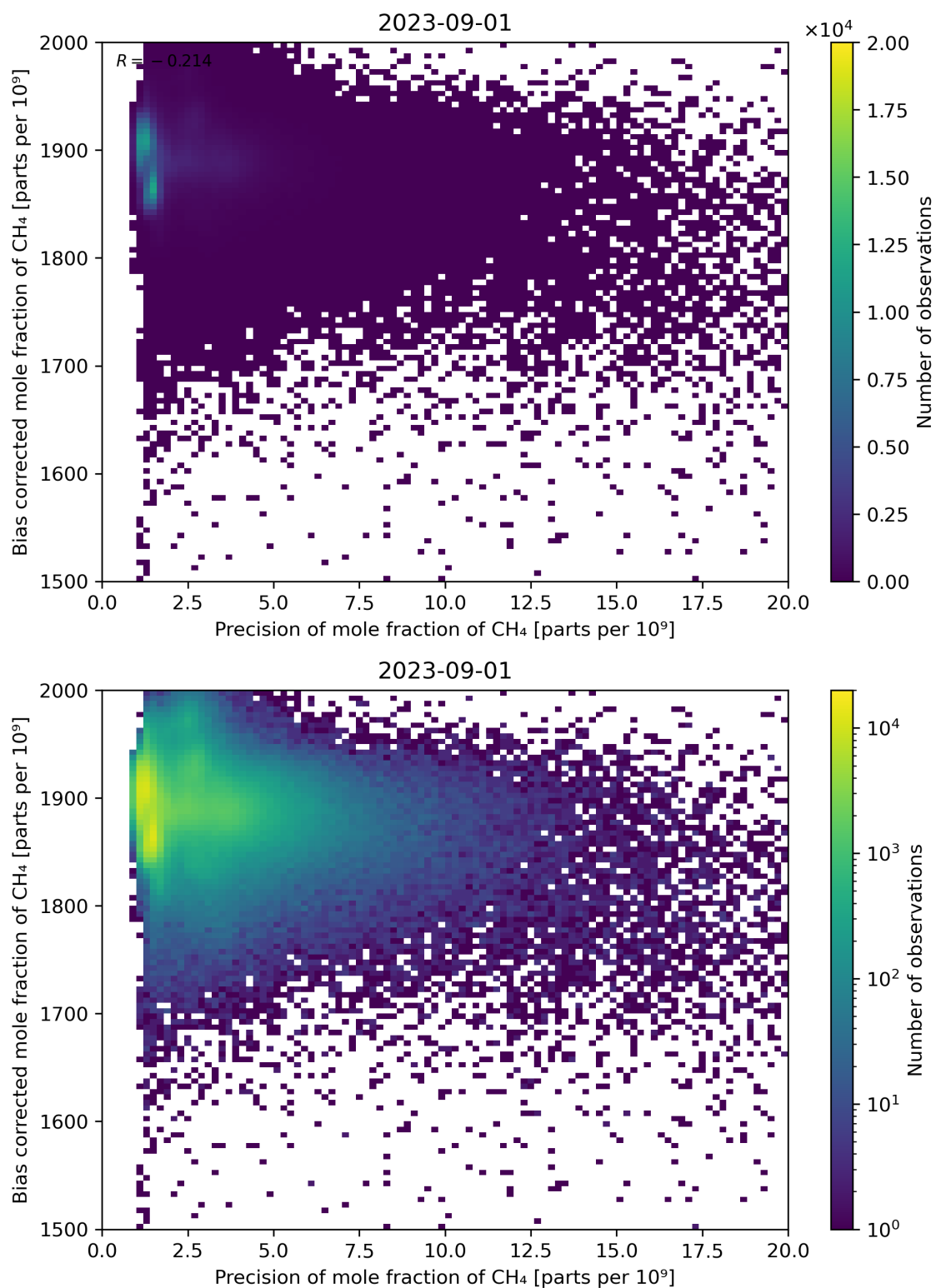
Figure 82: Scatter density plot of “Precision of mole fraction of \text{CH}_4 ” against “Bias corrected mole fraction of \text{CH}_4 ” for 2023-08-31 to 2023-09-02.
