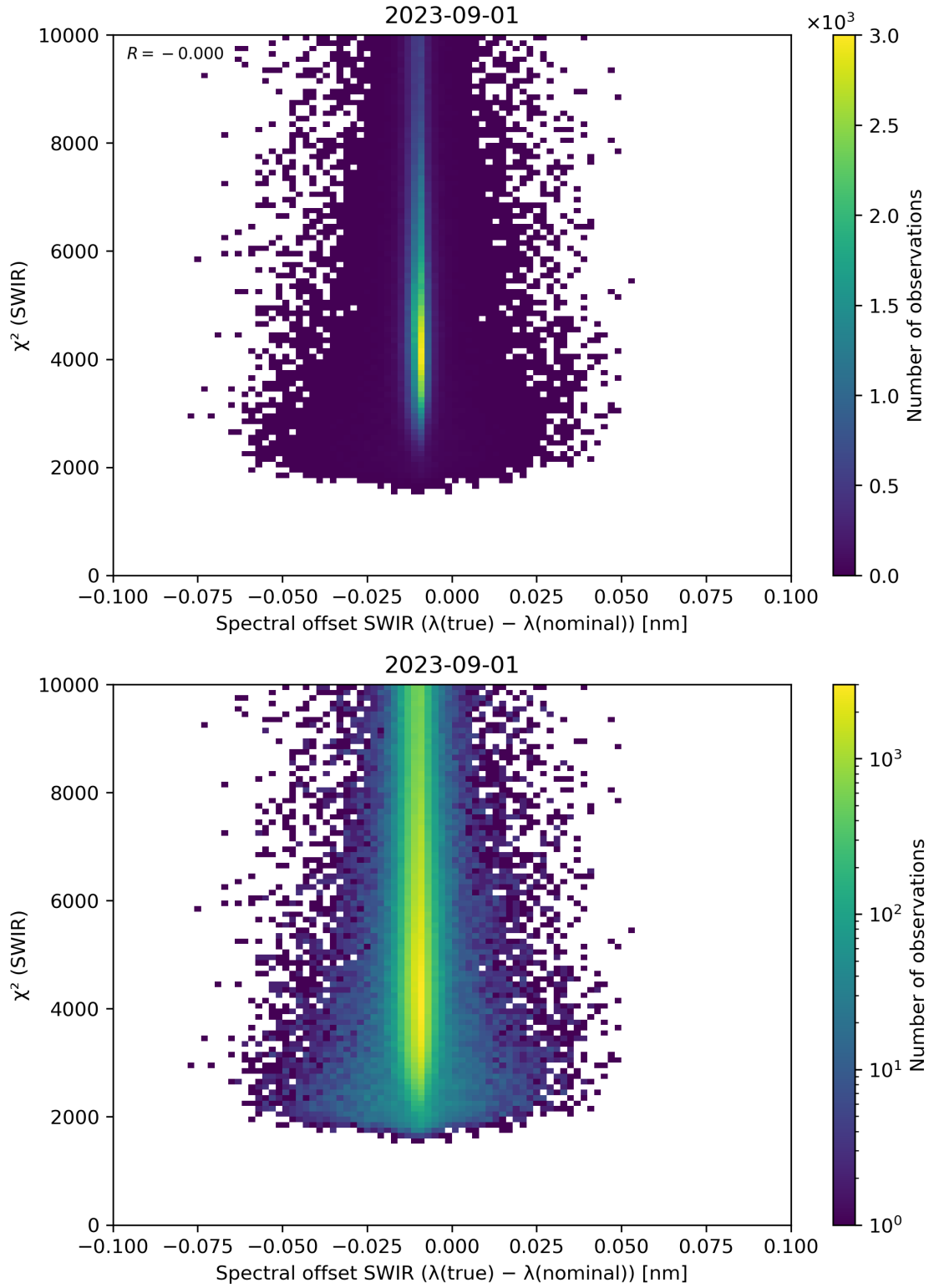
Figure 118: Scatter density plot of “Spectral offset SWIR ( \lambda(\text{true}) - \lambda(\text{nominal}) )” against “ \chi^2 (SWIR)” for 2023-08-31 to 2023-09-02.
