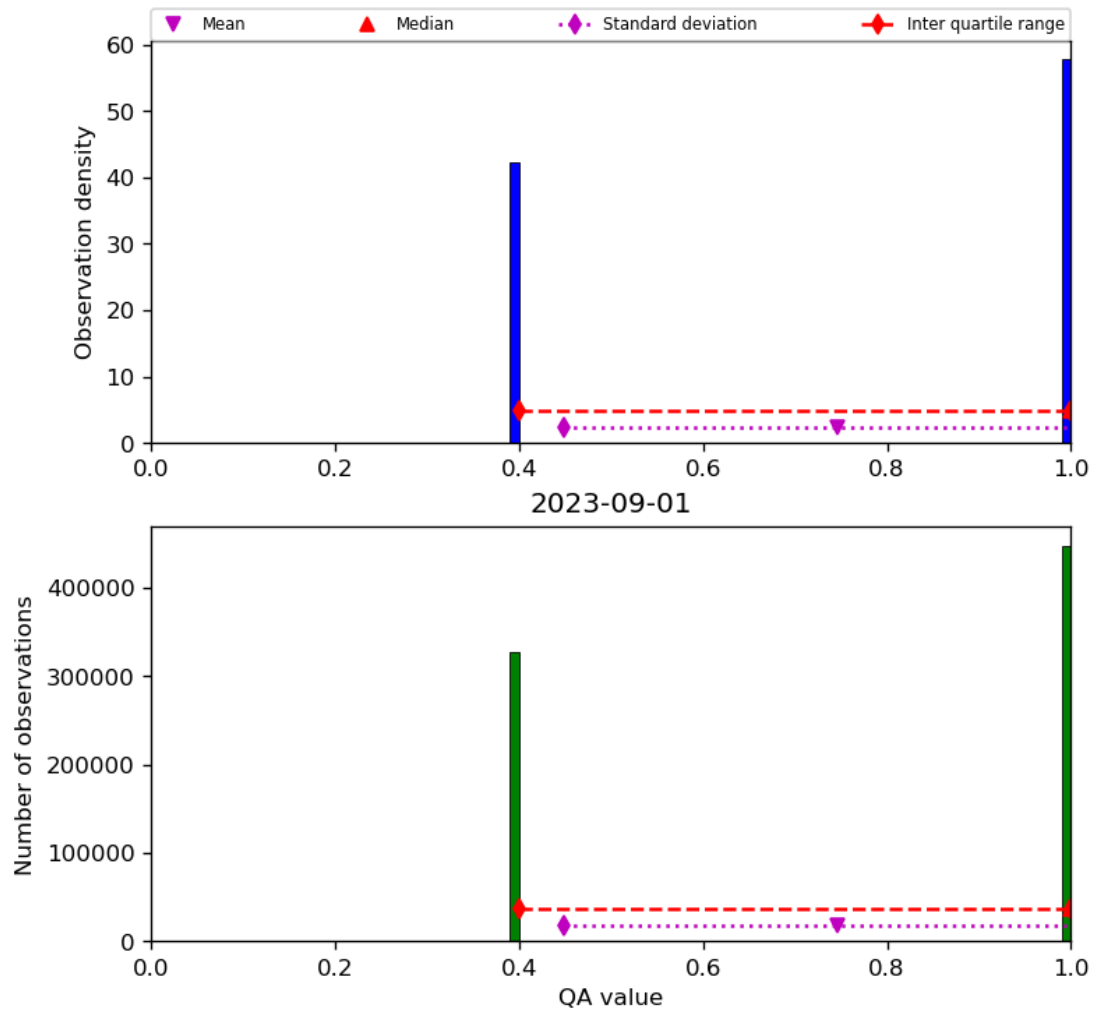
Figure 22: Histogram of “QA value” for 2023-08-31 to 2023-09-02
