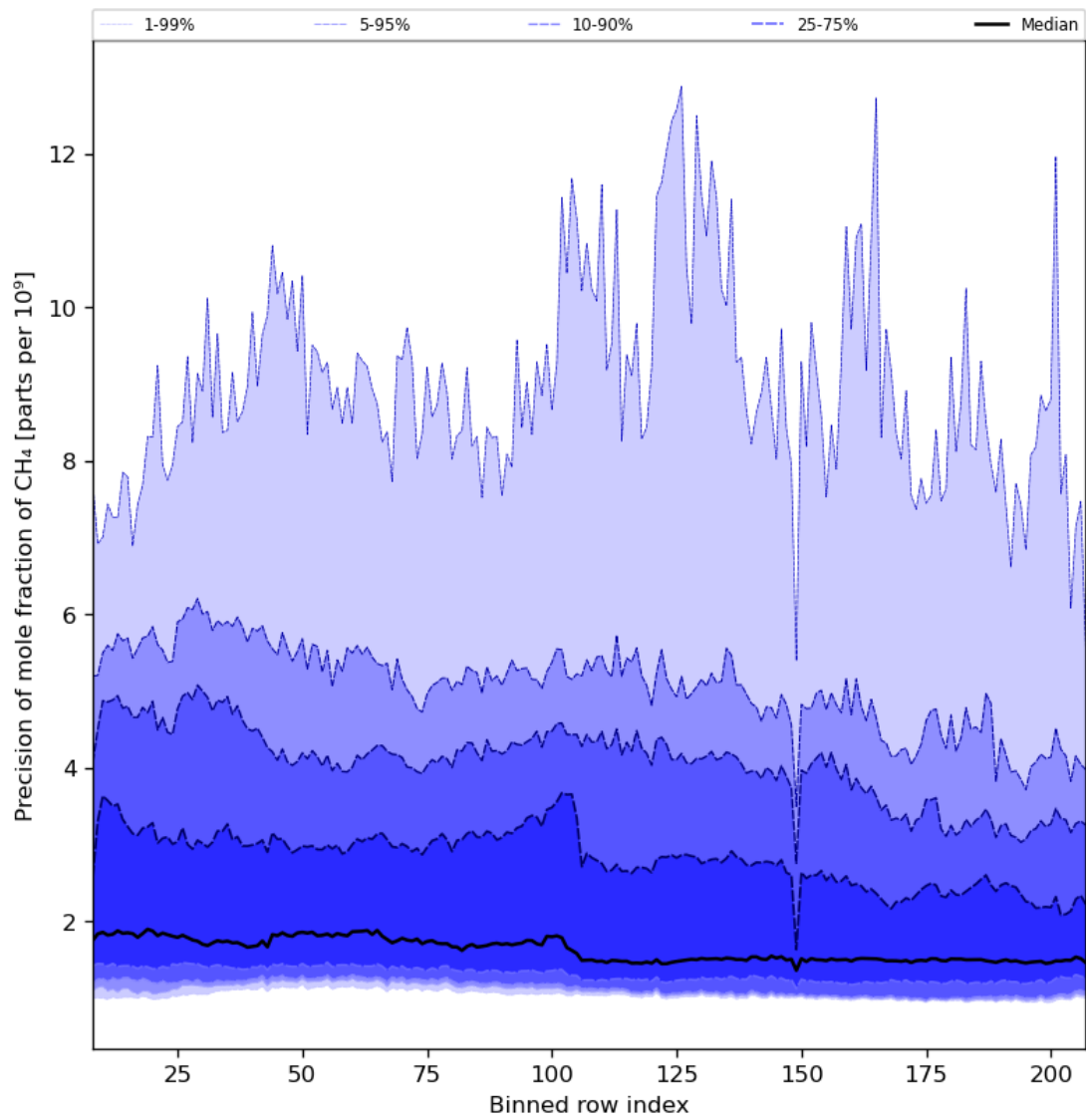
Figure 35: Along track statistics of "Precision of mole fraction of CH 4 " for 2023-08-31 to 2023-09-02
