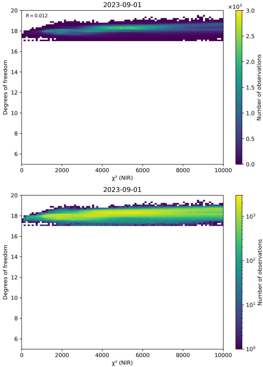
Figure 44: Scatter density plot of “ \chi^2 (NIR)” against “Degrees of freedom” for 2023-08-31 to 2023-09-02.
