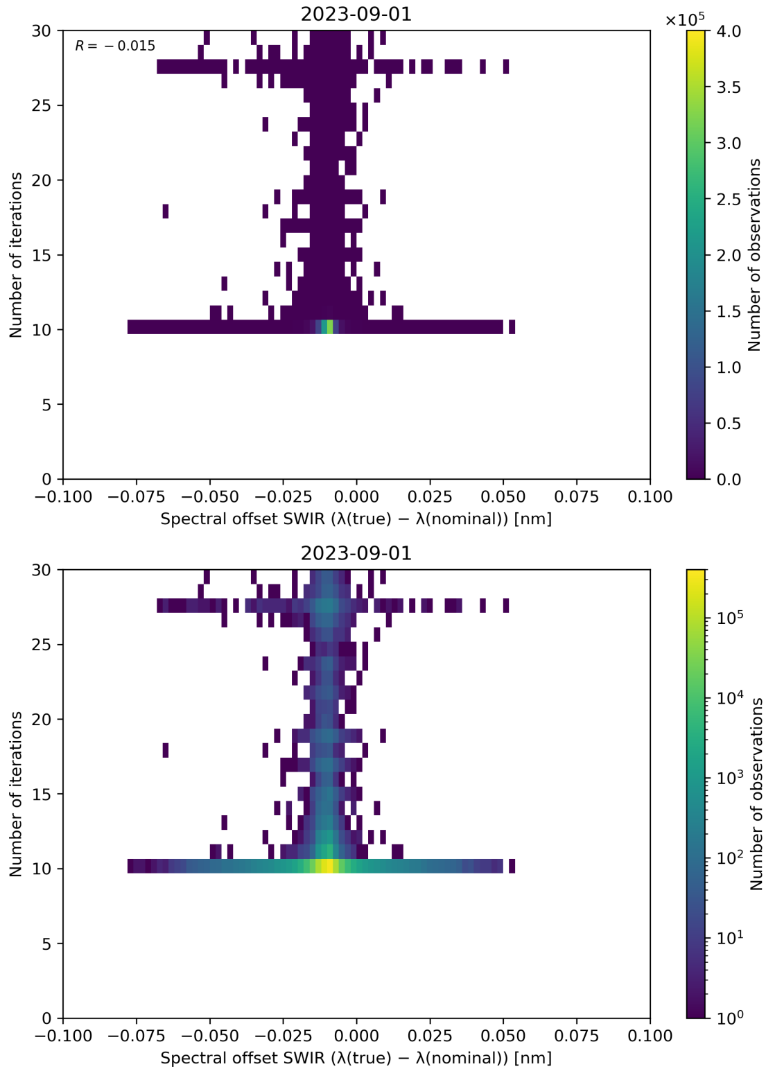
Figure 121: Scatter density plot of “Spectral offset SWIR ( \lambda(\text{true}) - \lambda(\text{nominal}) )” against “Number of iterations” for 2023-08-31 to 2023-09-02.
