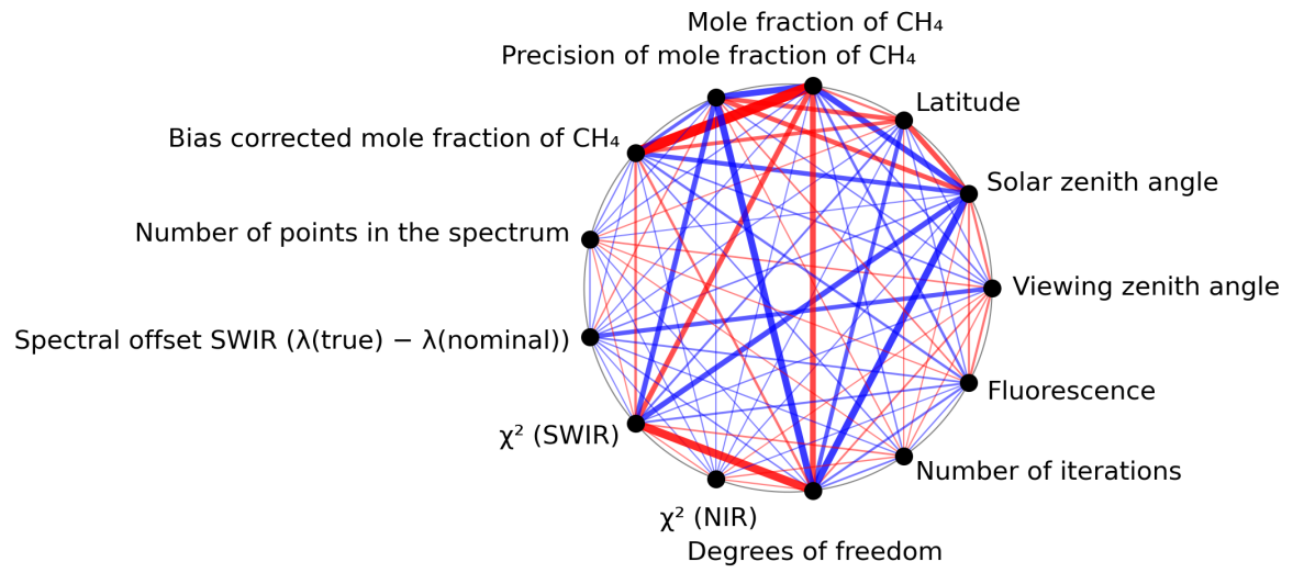
Figure 1: Map of correlation graph for 2023-08-31 to 2023-09-02.
