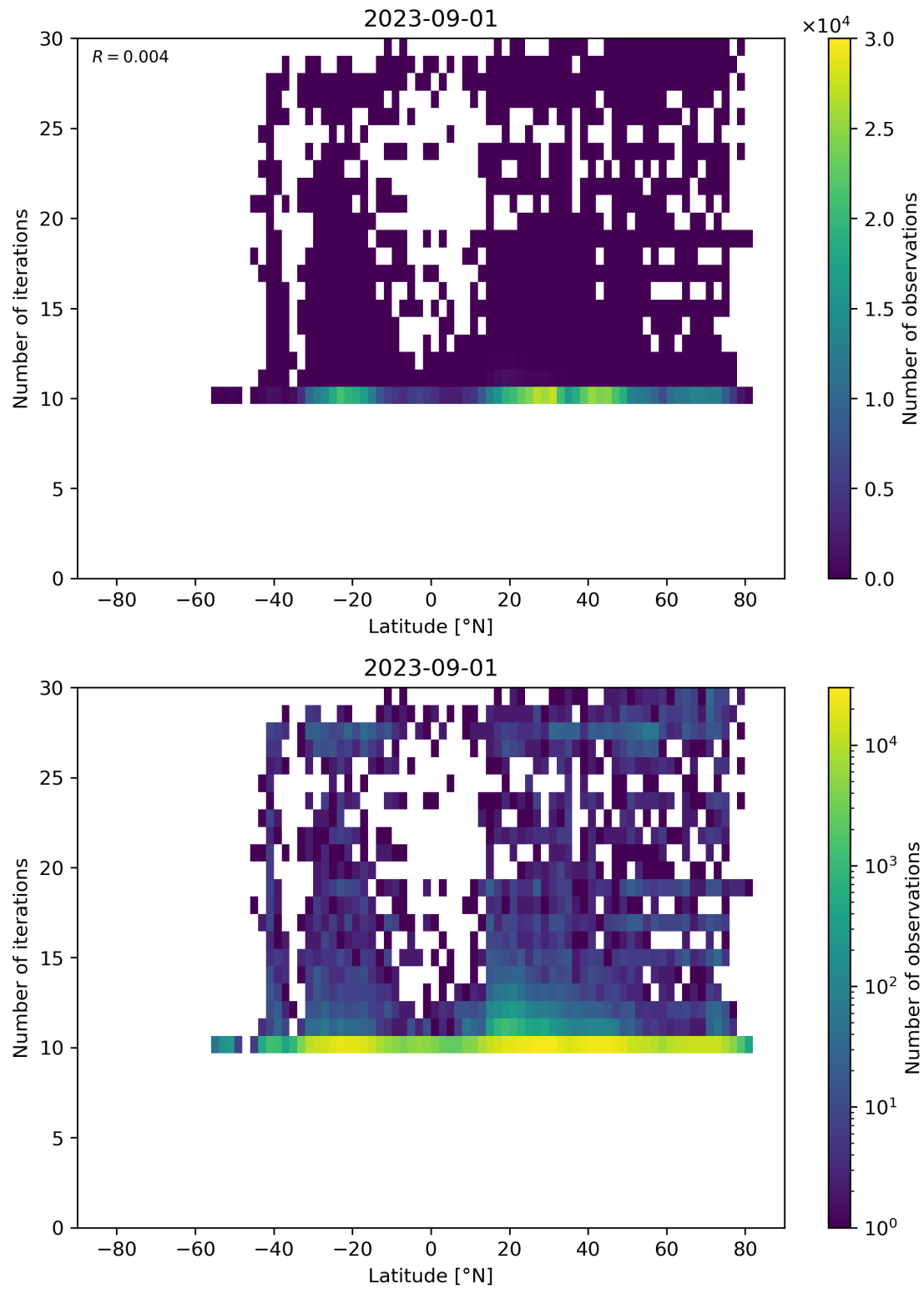
Figure 60: Scatter density plot of “Latitude” against “Number of iterations” for 2023-08-31 to 2023-09-02.
