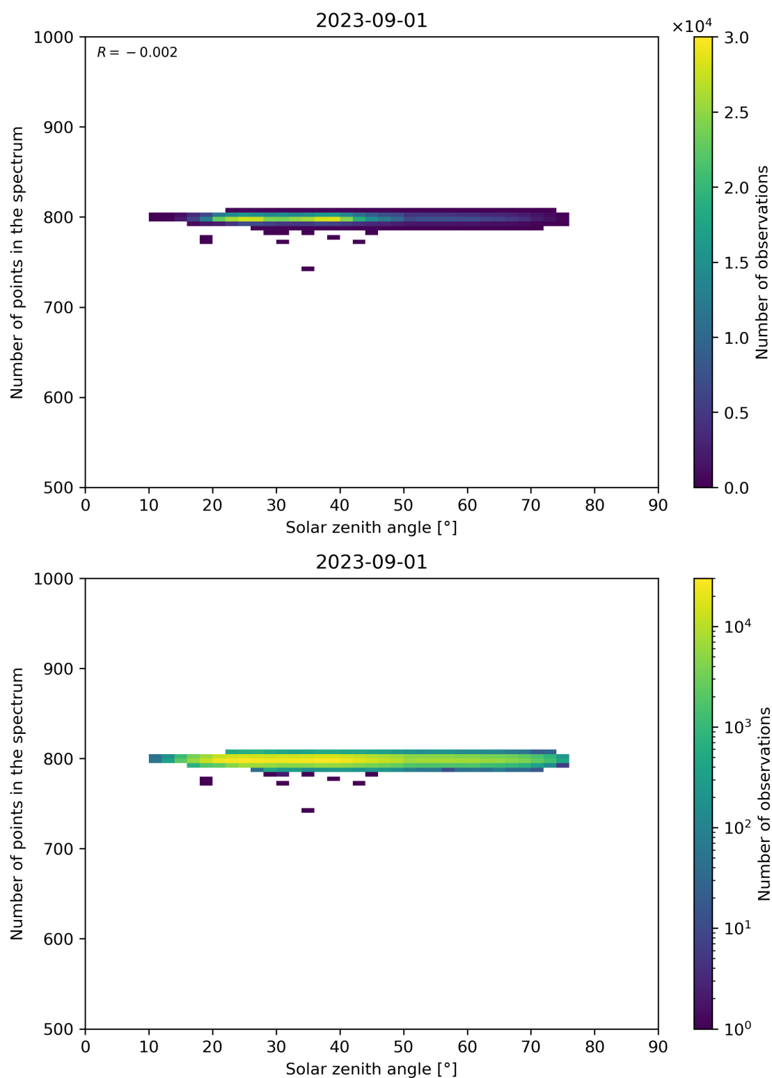
Figure 103: Scatter density plot of “Solar zenith angle” against “Number of points in the spectrum” for 2023-08-31 to 2023-09-02.
