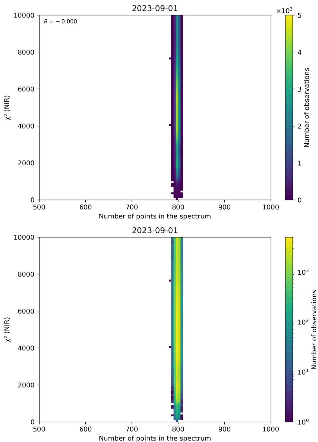
Figure 88: Scatter density plot of “Number of points in the spectrum” against “ \chi^2 (NIR)” for 2023-08-31 to 2023-09-02.
