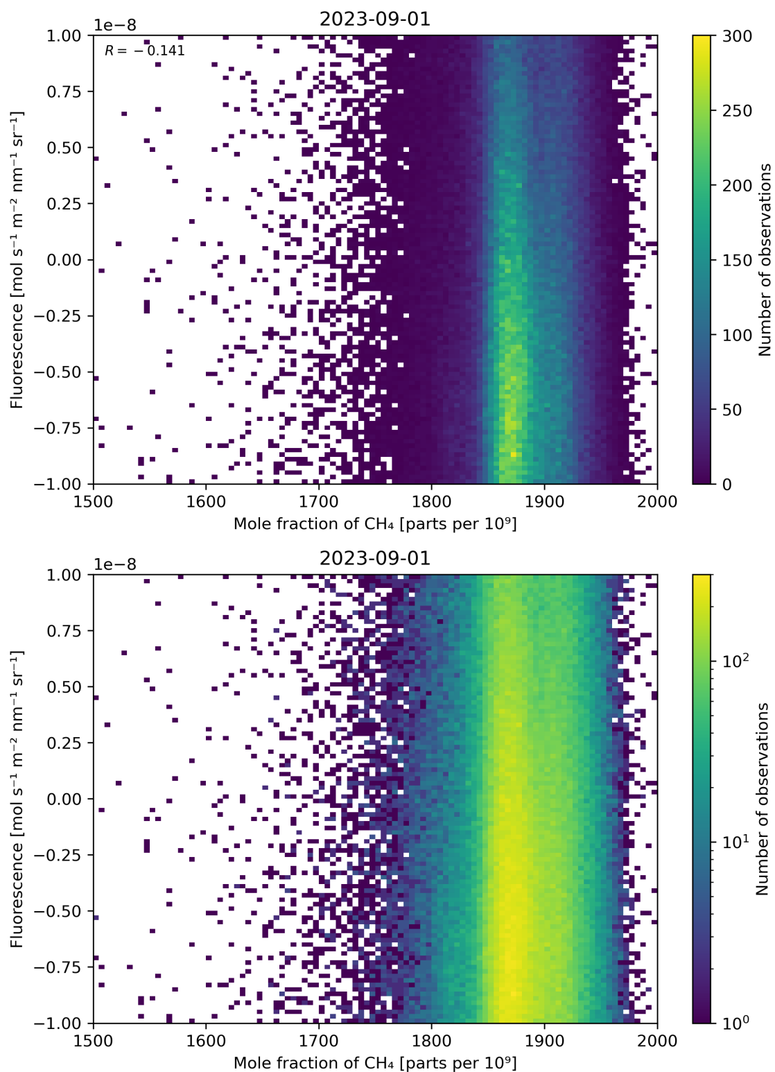
Figure 73: Scatter density plot of “Mole fraction of \text{CH}_4 ” against “Fluorescence” for 2023-08-31 to 2023-09-02.
