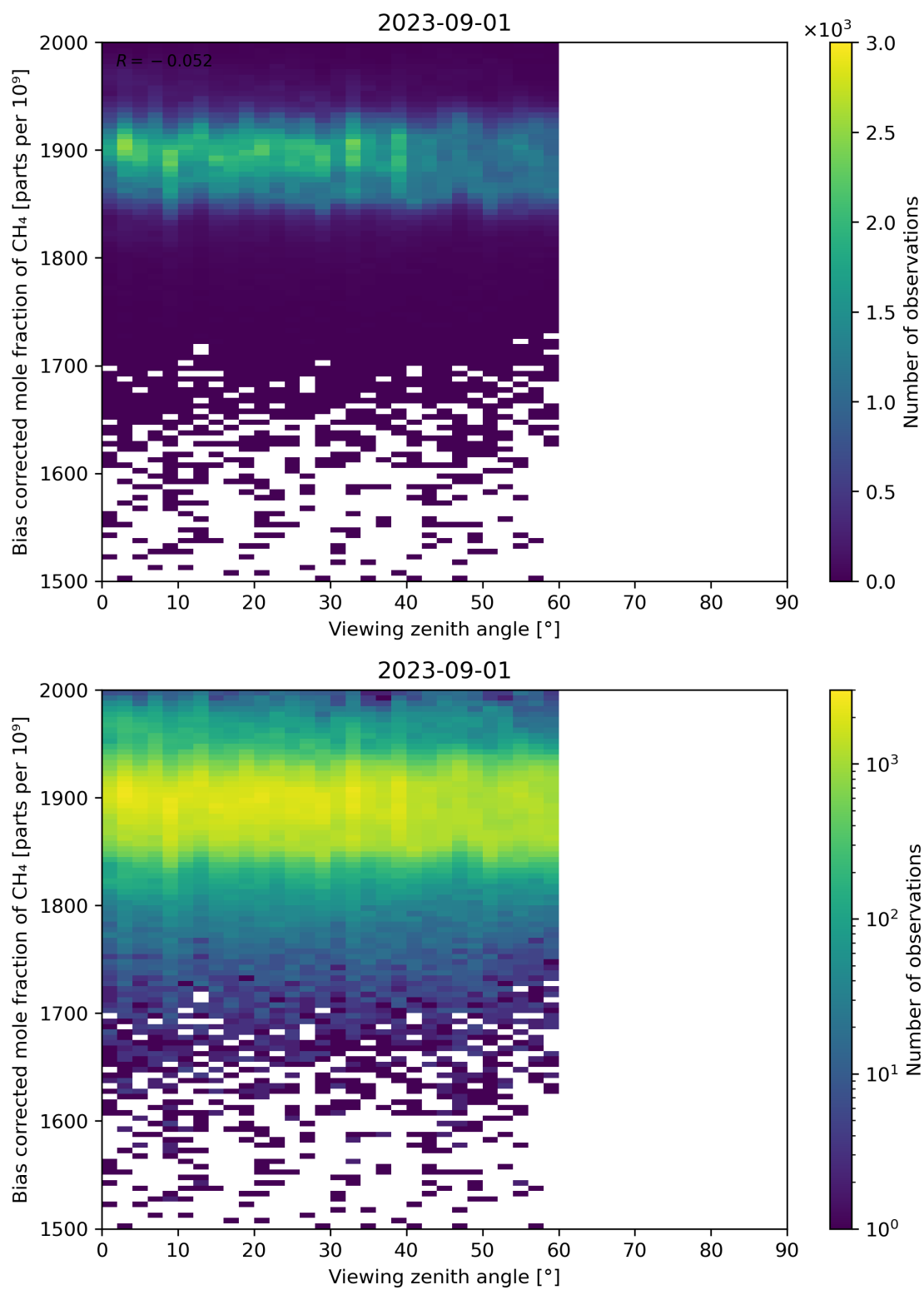
Figure 111: Scatter density plot of “Viewing zenith angle” against “Bias corrected mole fraction of CH 4 ” for 2023-08-31 to 2023-09-02.
