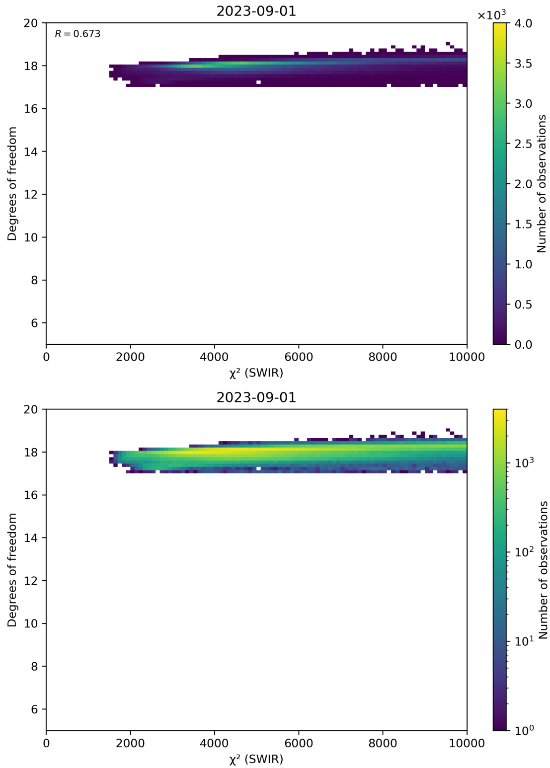
Figure 48: Scatter density plot of “ \chi^2 (SWIR)” against “Degrees of freedom” for 2023-08-31 to 2023-09-02.
