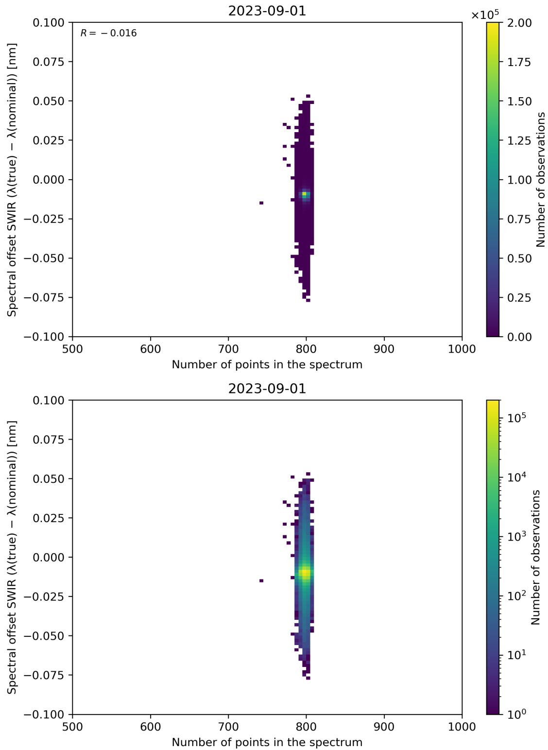
Figure 93: Scatter density plot of “Number of points in the spectrum” against “Spectral offset SWIR ( \lambda(\text{true}) - \lambda(\text{nominal}) )” for 2023-08-31 to 2023-09-02.
