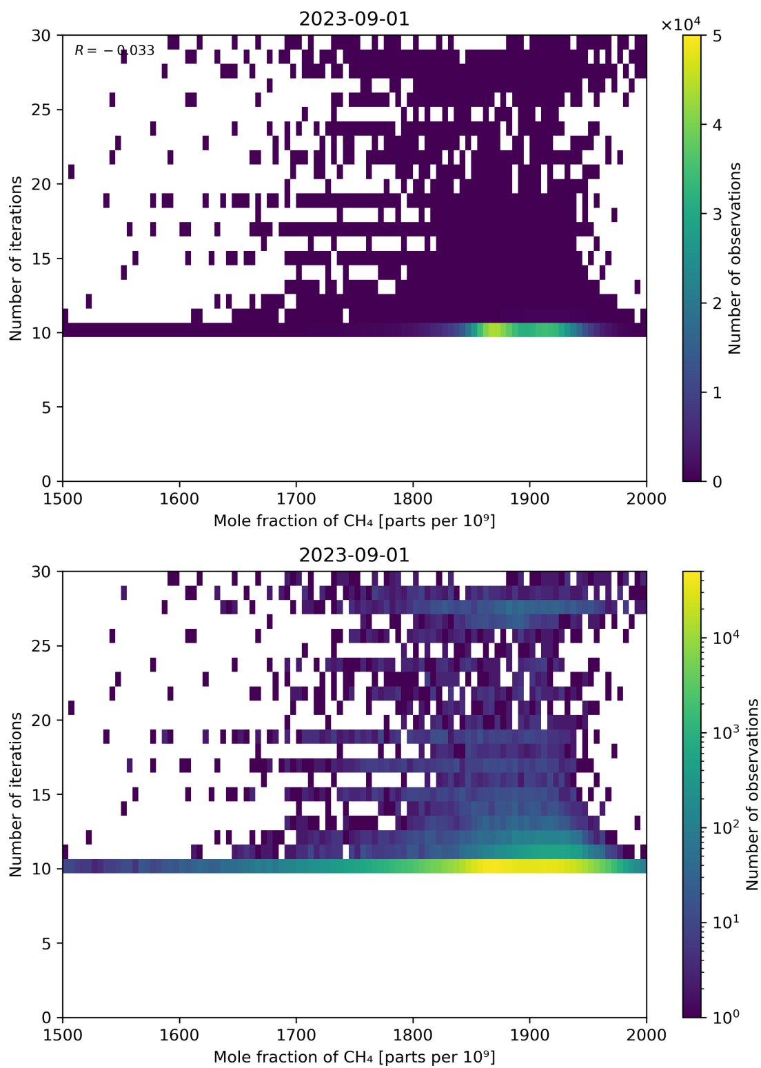
Figure 76: Scatter density plot of “Mole fraction of CH 4 ” against “Number of iterations” for 2023-08-31 to 2023-09-02.
