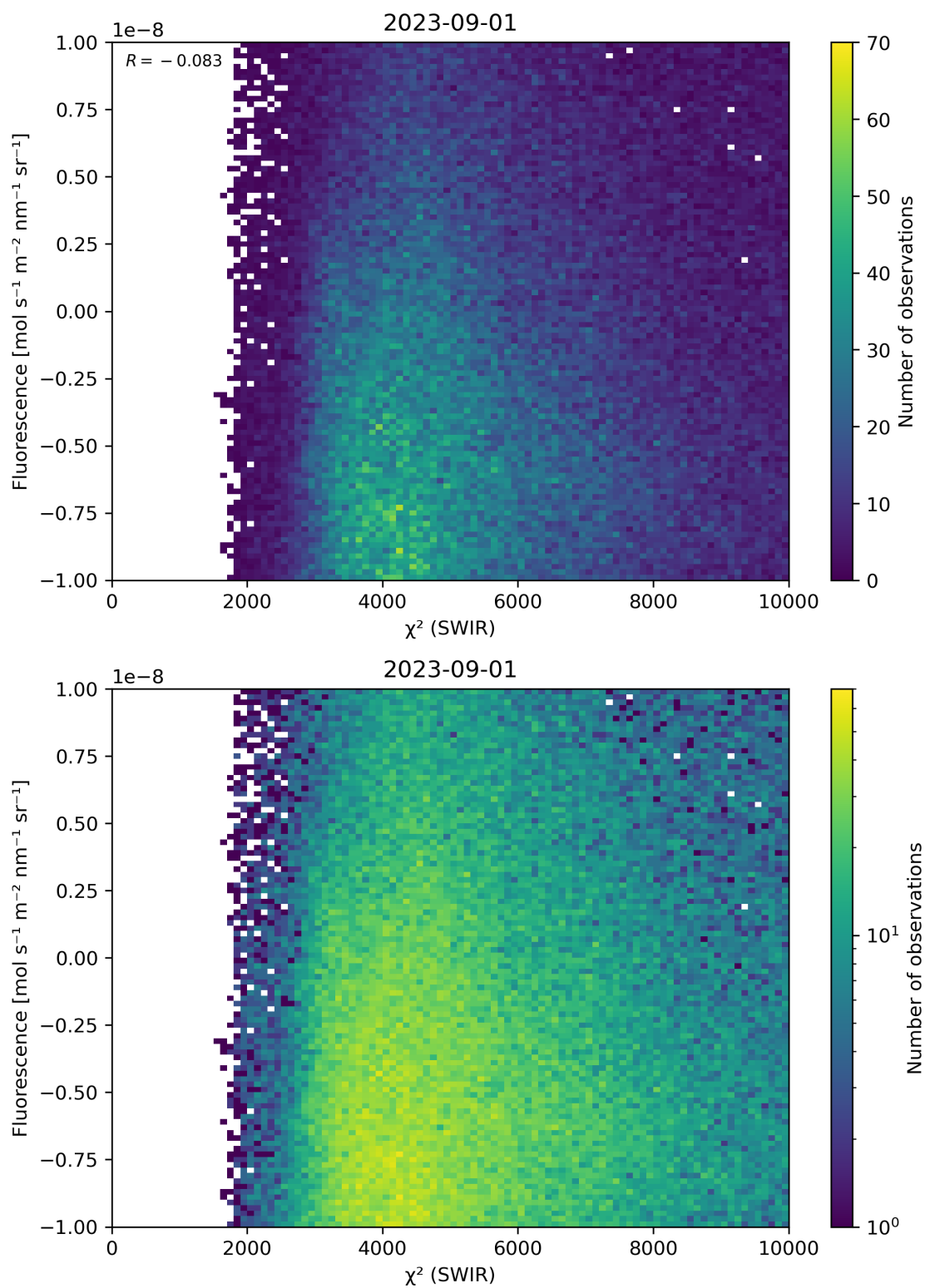
Figure 49: Scatter density plot of “ \chi^2 (SWIR)” against “Fluorescence” for 2023-08-31 to 2023-09-02.
