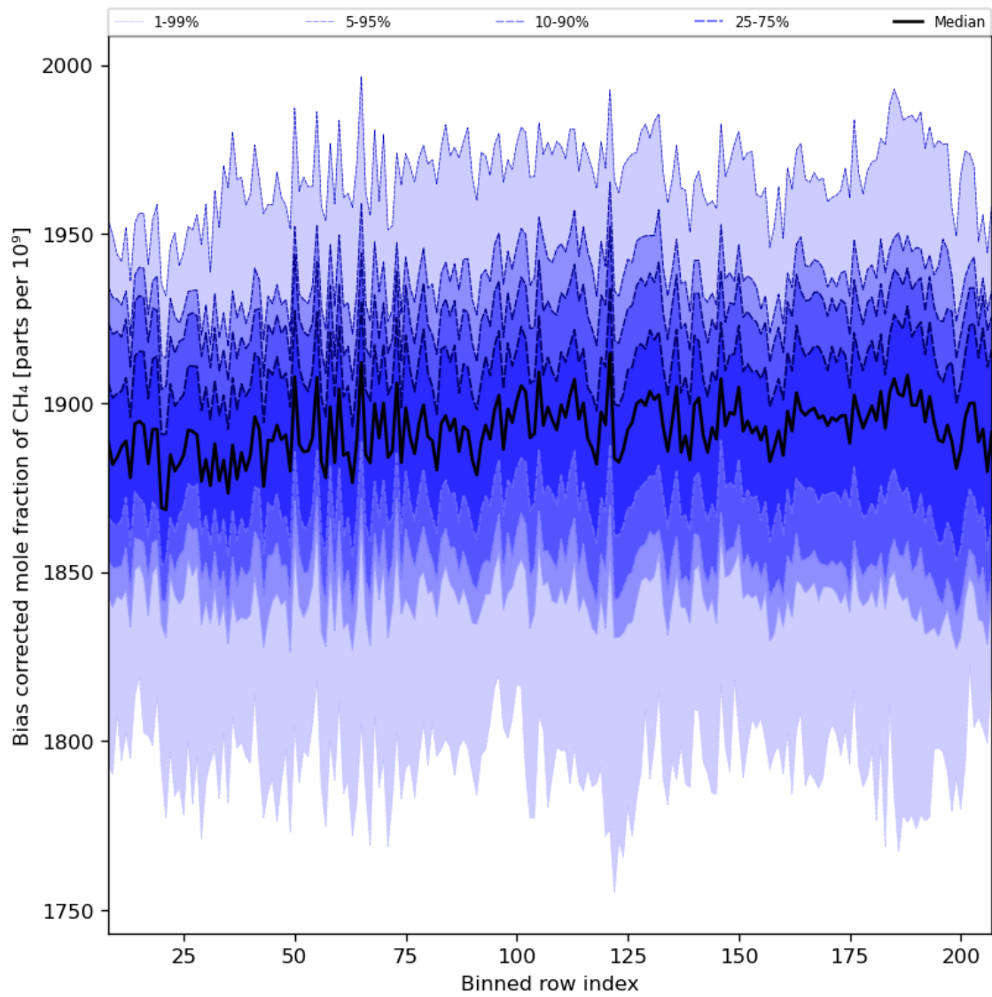
Figure 36: Along track statistics of “Bias corrected mole fraction of CH 4 ” for 2023-08-31 to 2023-09-02
