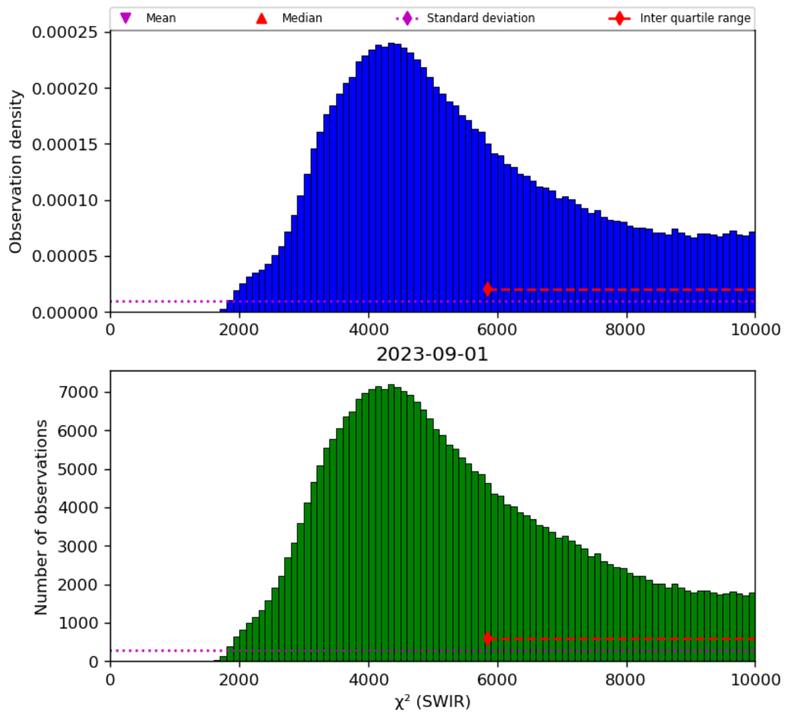
Figure 28: Histogram of " \chi^2 (SWIR)" for 2023-08-31 to 2023-09-02
