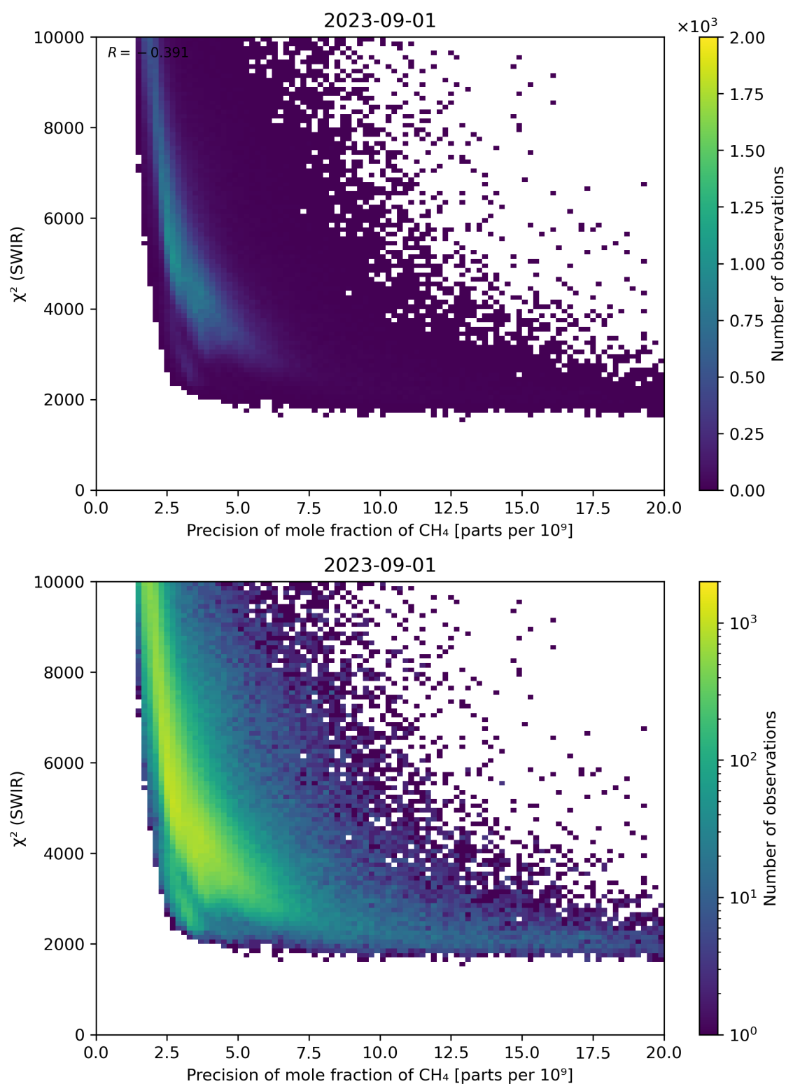
Figure 79: Scatter density plot of “Precision of mole fraction of \text{CH}_4 ” against “ \chi^2 (SWIR)” for 2023-08-31 to 2023-09-02.
