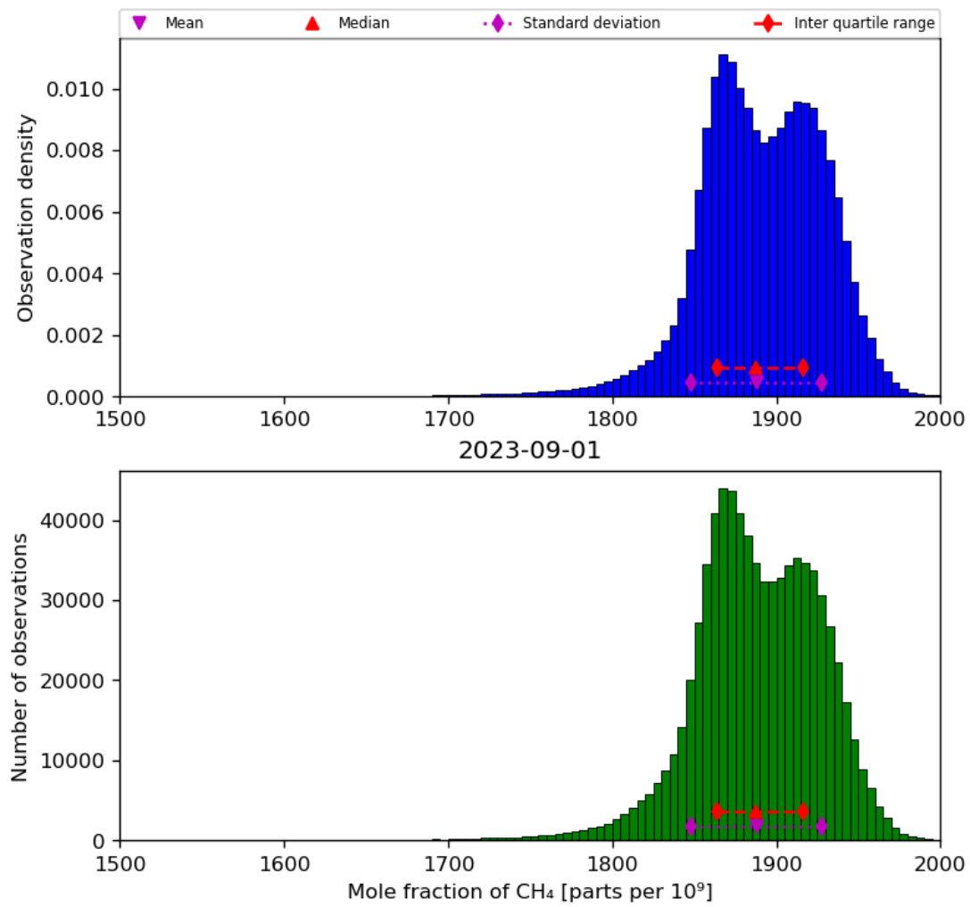
Figure 23: Histogram of “Mole fraction of CH 4 ” for 2023-08-31 to 2023-09-02
