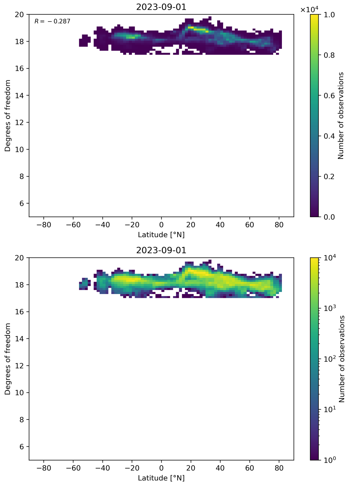
Figure 55: Scatter density plot of “Latitude” against “Degrees of freedom” for 2023-08-31 to 2023-09-02.
