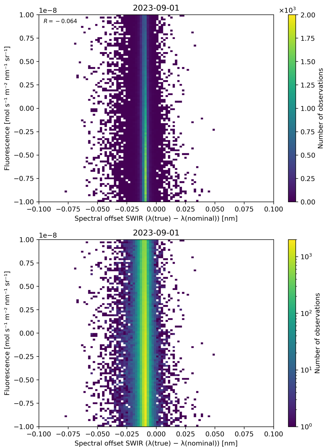
Figure 120: Scatter density plot of “Spectral offset SWIR ( \lambda(\text{true}) - \lambda(\text{nominal}) )” against “Fluorescence” for 2023-08-31 to 2023-09-02.
