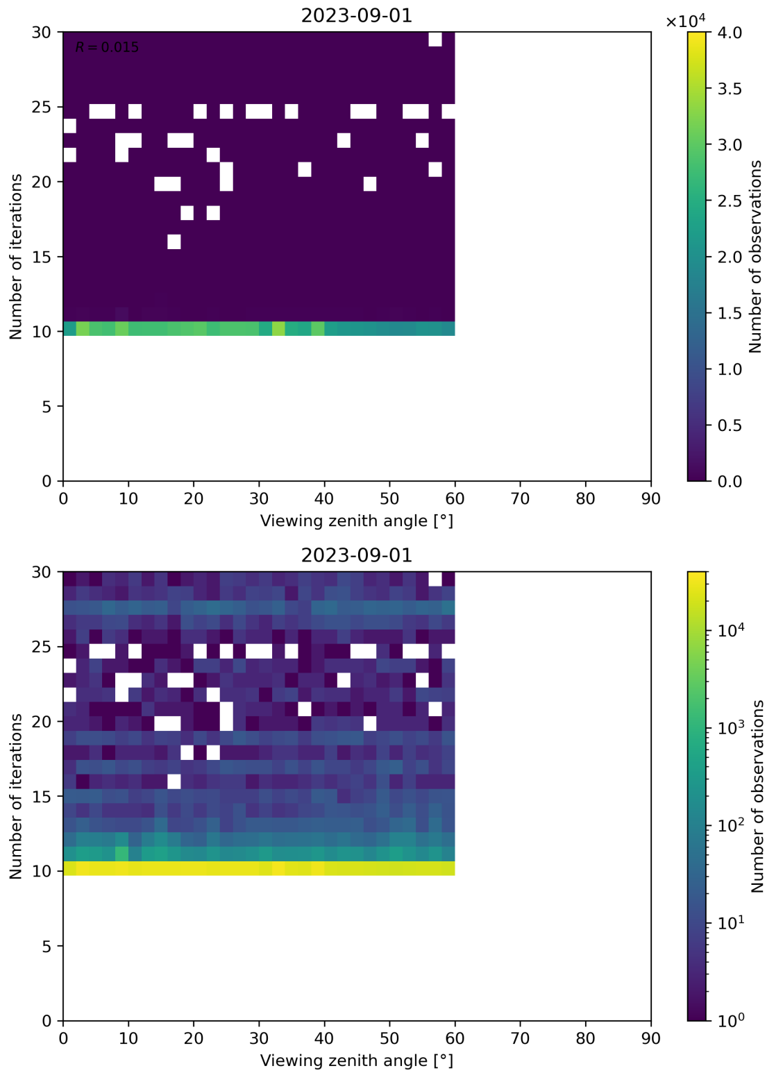
Figure 113: Scatter density plot of “Viewing zenith angle” against “Number of iterations” for 2023-08-31 to 2023-09-02.
