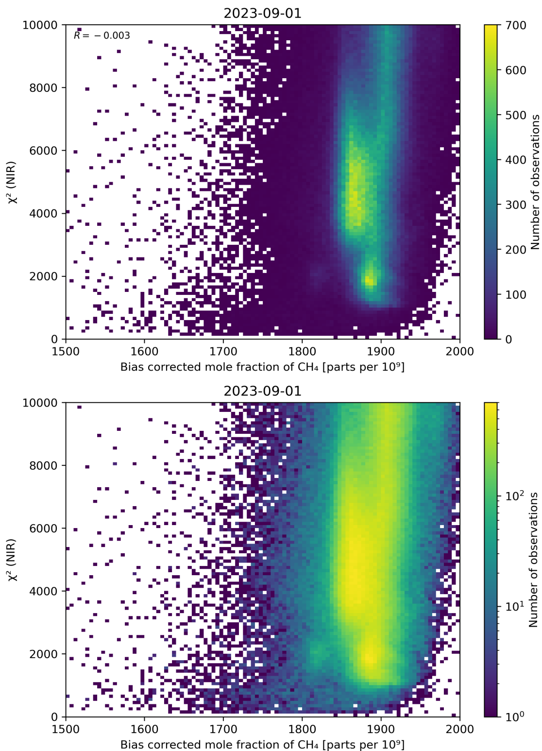
Figure 63: Scatter density plot of “Bias corrected mole fraction of CH 4 ” against “ \chi^2 (NIR)” for 2023-08-31 to 2023-09-02.
