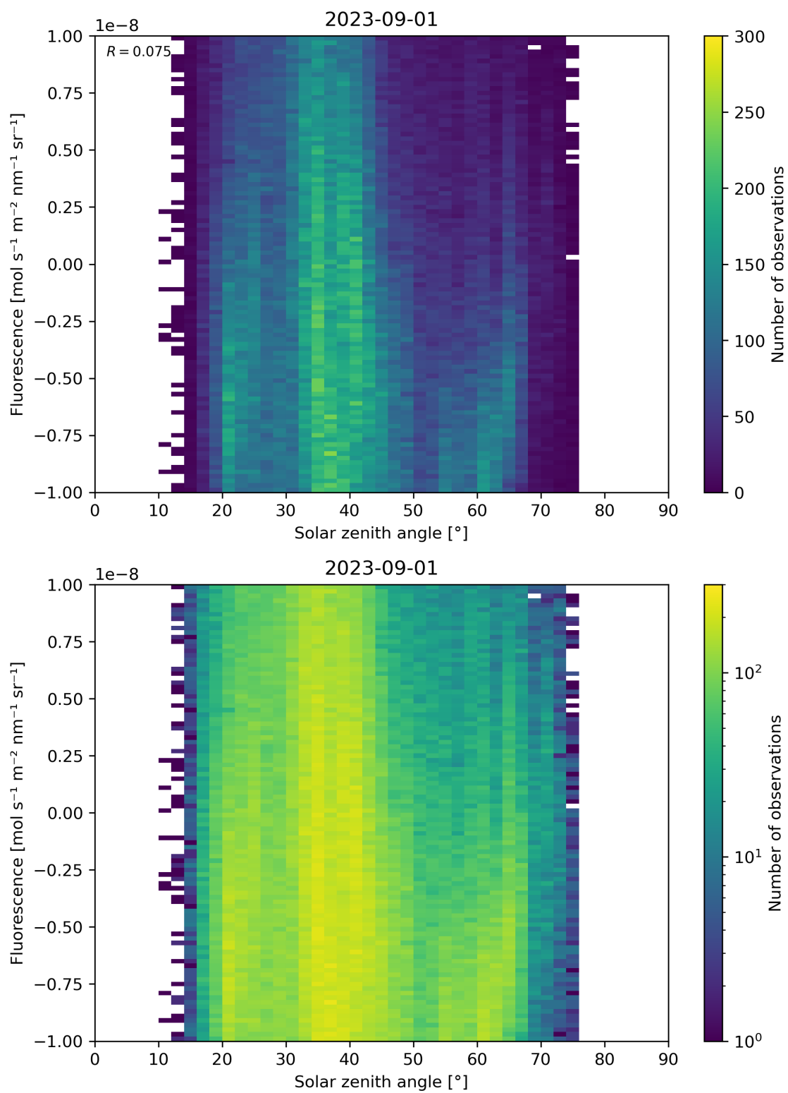
Figure 97: Scatter density plot of “Solar zenith angle” against “Fluorescence” for 2023-08-31 to 2023-09-02.
