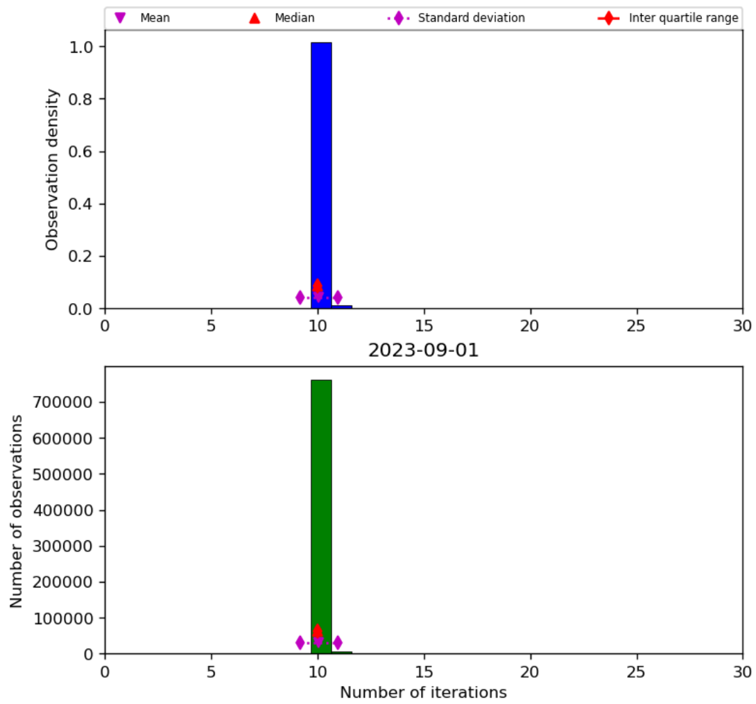
Figure 31: Histogram of “Number of iterations” for 2023-08-31 to 2023-09-02
