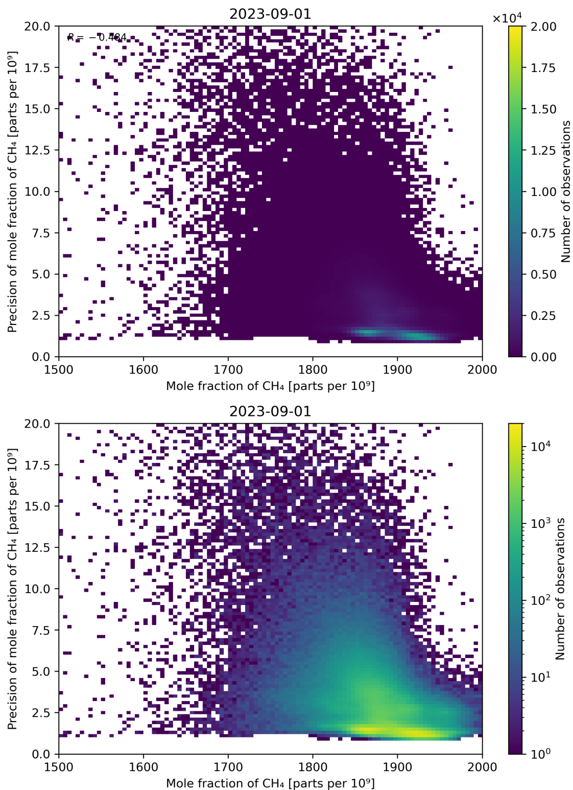
Figure 75: Scatter density plot of “Mole fraction of CH 4 ” against “Precision of mole fraction of CH 4 ” for 2023-08-31 to 2023-09-02.
