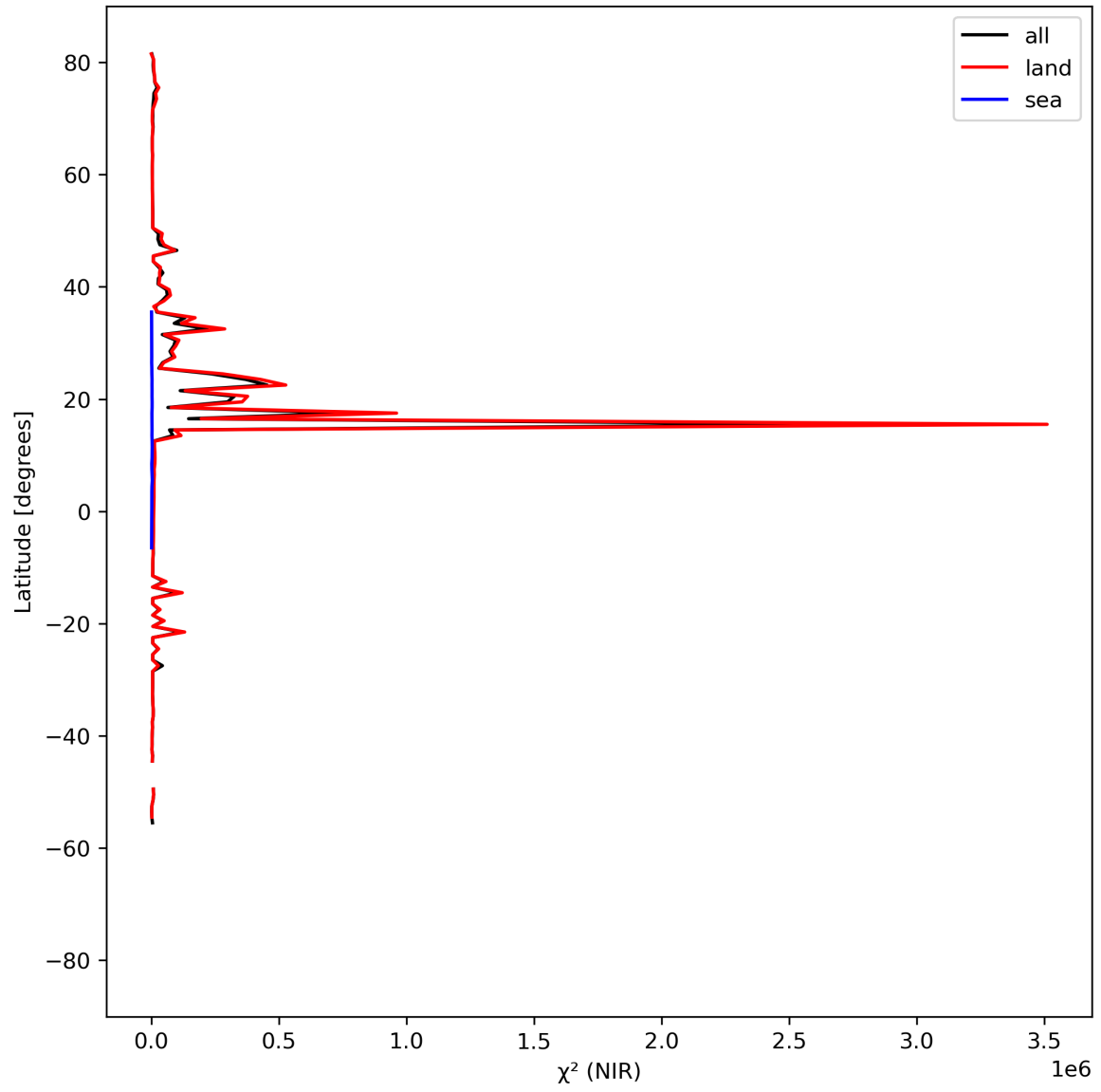
Figure 18: Zonal average of “ \chi^2 (NIR)” for 2023-08-31 to 2023-09-02.
