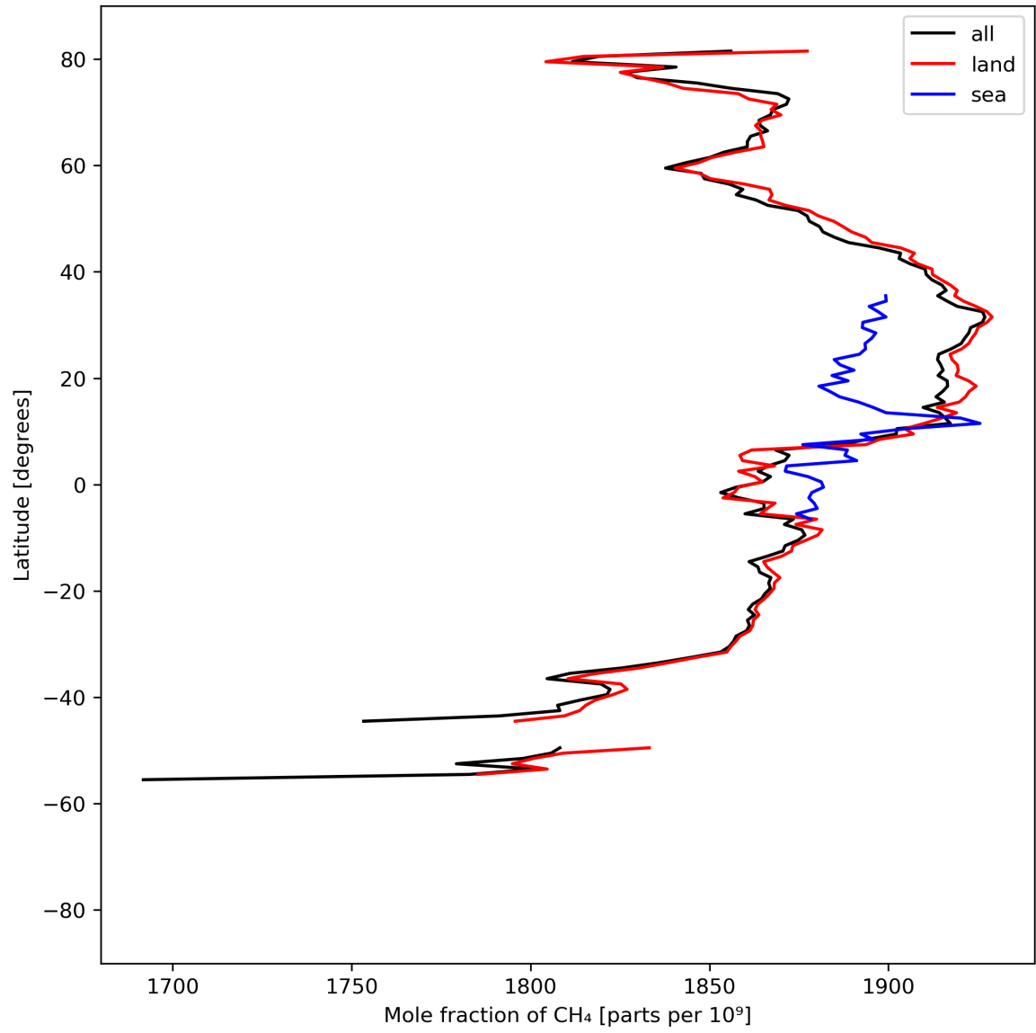
Figure 12: Zonal average of “Mole fraction of \text{CH}_4 ” for 2023-08-31 to 2023-09-02.
