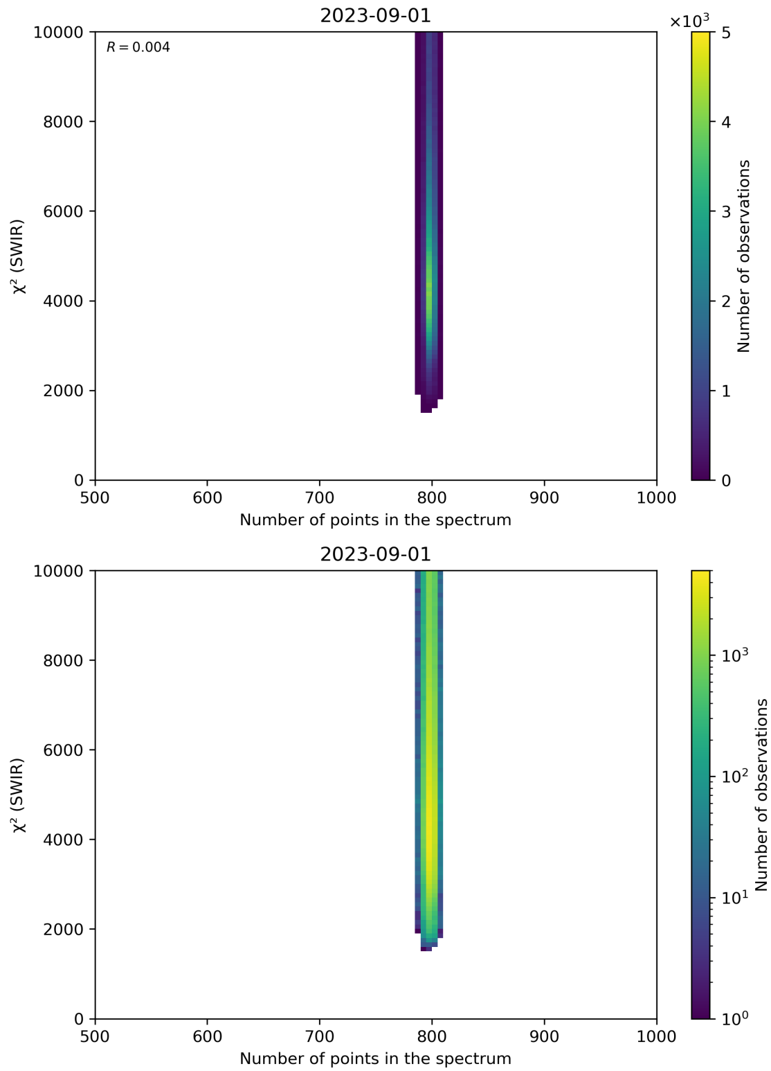
Figure 89: Scatter density plot of “Number of points in the spectrum” against “ \chi^2 (SWIR)” for 2023-08-31 to 2023-09-02.
