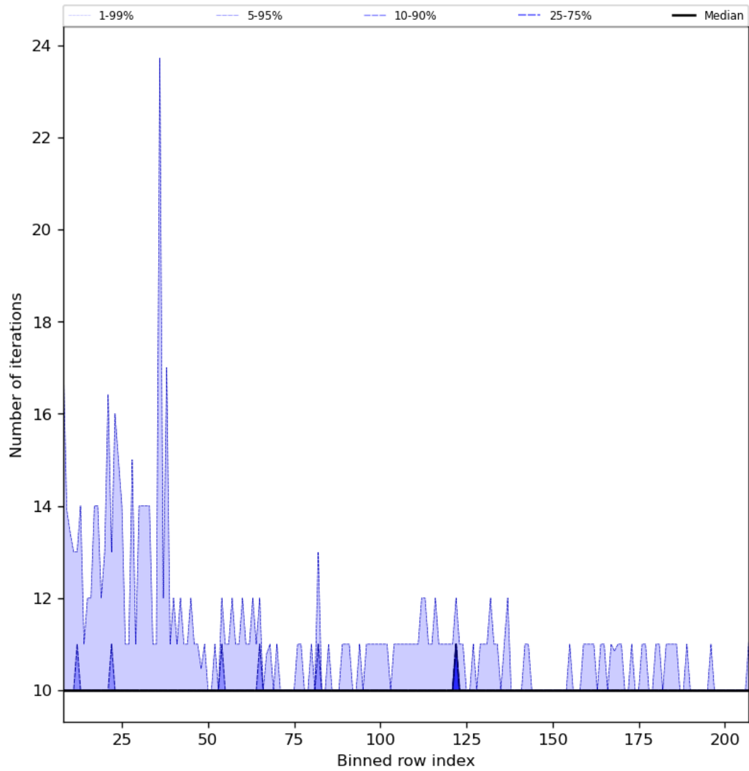
Figure 42: Along track statistics of “Number of iterations” for 2023-08-31 to 2023-09-02
