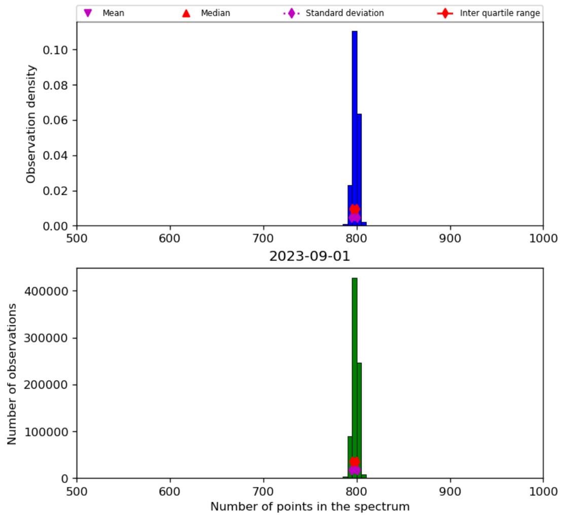
Figure 26: Histogram of “Number of points in the spectrum” for 2023-08-31 to 2023-09-02
