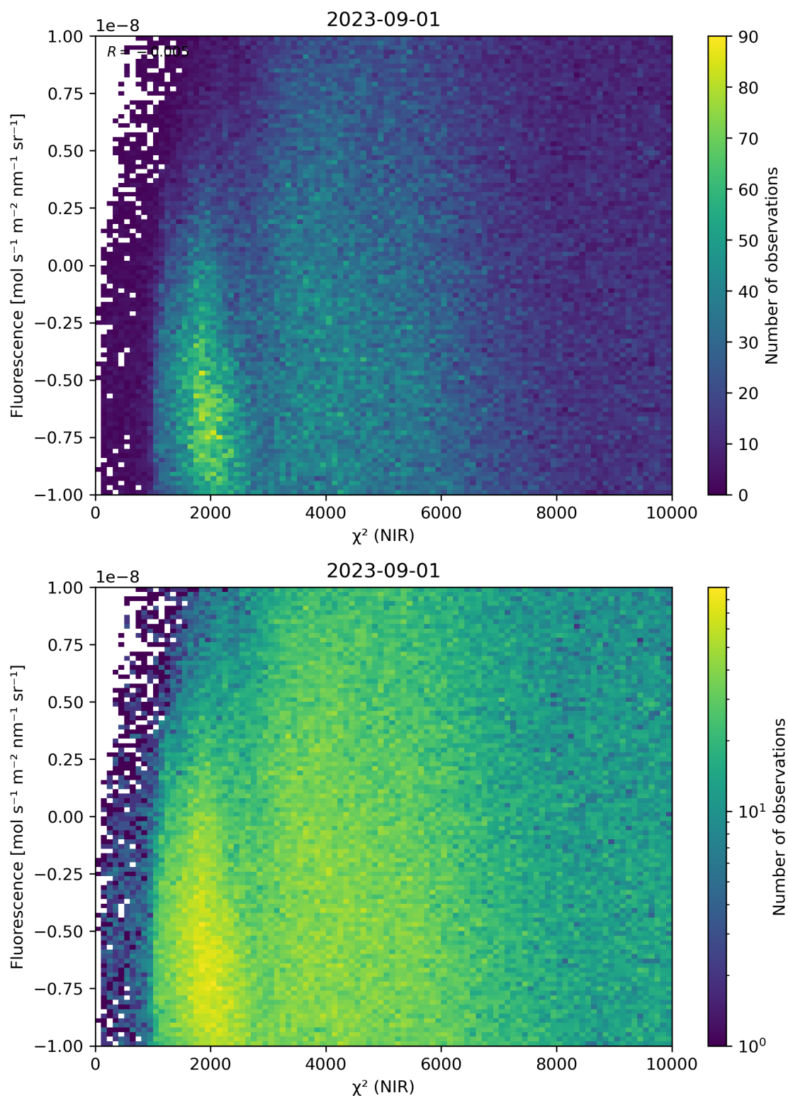
Figure 45: Scatter density plot of “ \chi^2 (NIR)” against “Fluorescence” for 2023-08-31 to 2023-09-02.
