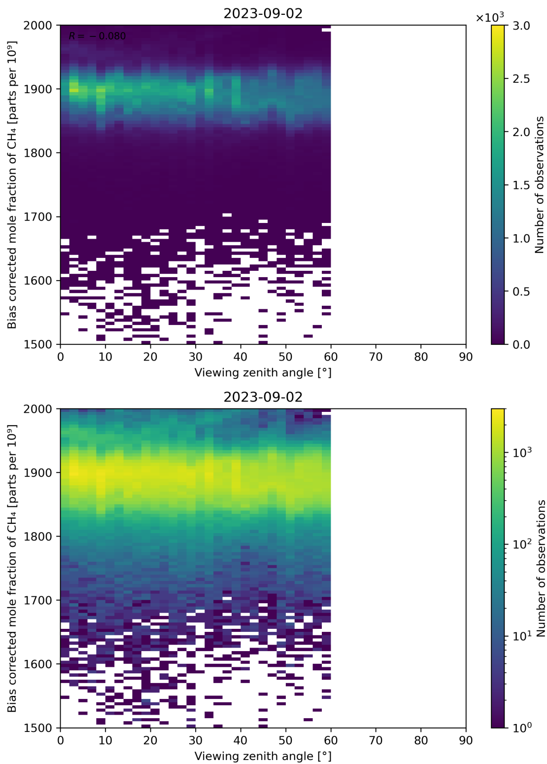
Figure 111: Scatter density plot of “Viewing zenith angle” against “Bias corrected mole fraction of CH 4 ” for 2023-09-01 to 2023-09-03.
