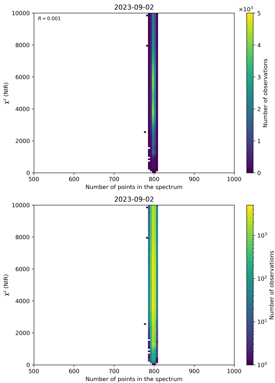
Figure 88: Scatter density plot of “Number of points in the spectrum” against “ \chi^2 (NIR)” for 2023-09-01 to 2023-09-03.
