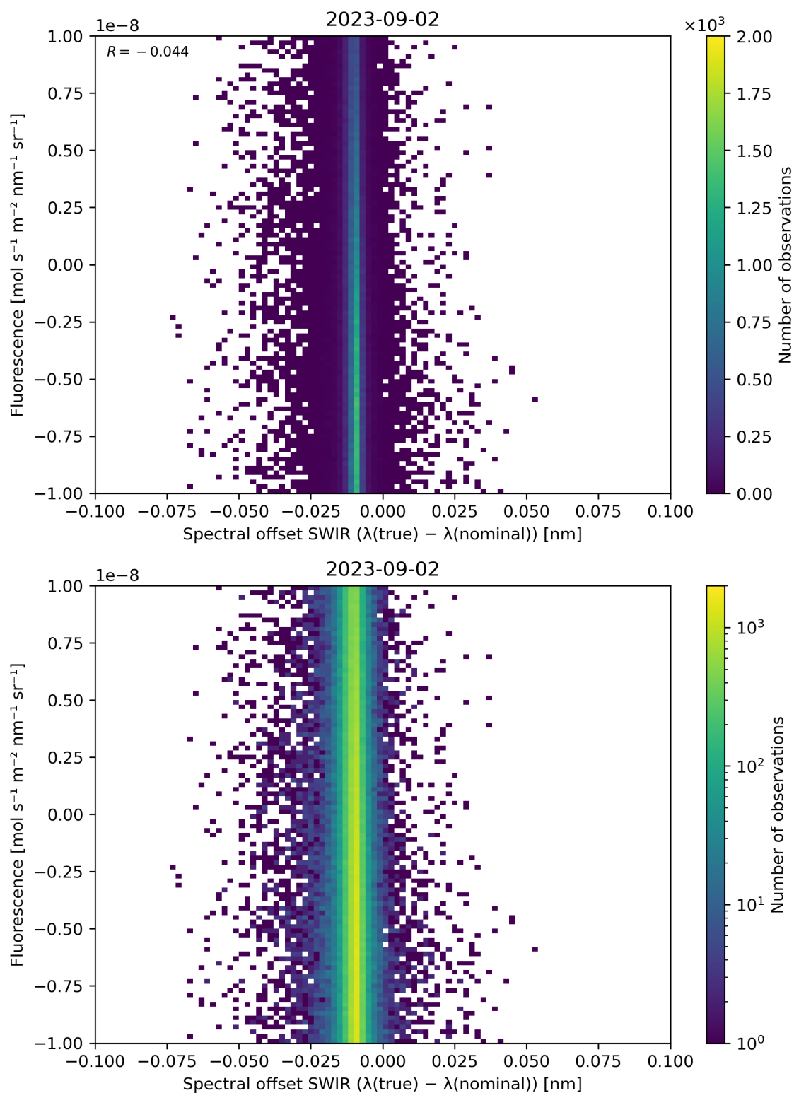
Figure 120: Scatter density plot of “Spectral offset SWIR ( \lambda(\text{true}) - \lambda(\text{nominal}) )” against “Fluorescence” for 2023-09-01 to 2023-09-03.
