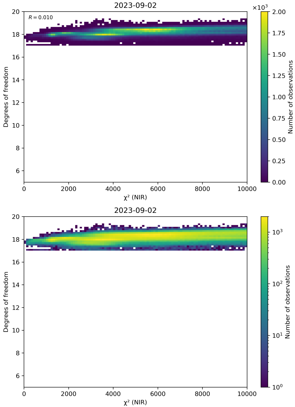
Figure 44: Scatter density plot of “ \chi^2 (NIR)” against “Degrees of freedom” for 2023-09-01 to 2023-09-03.
