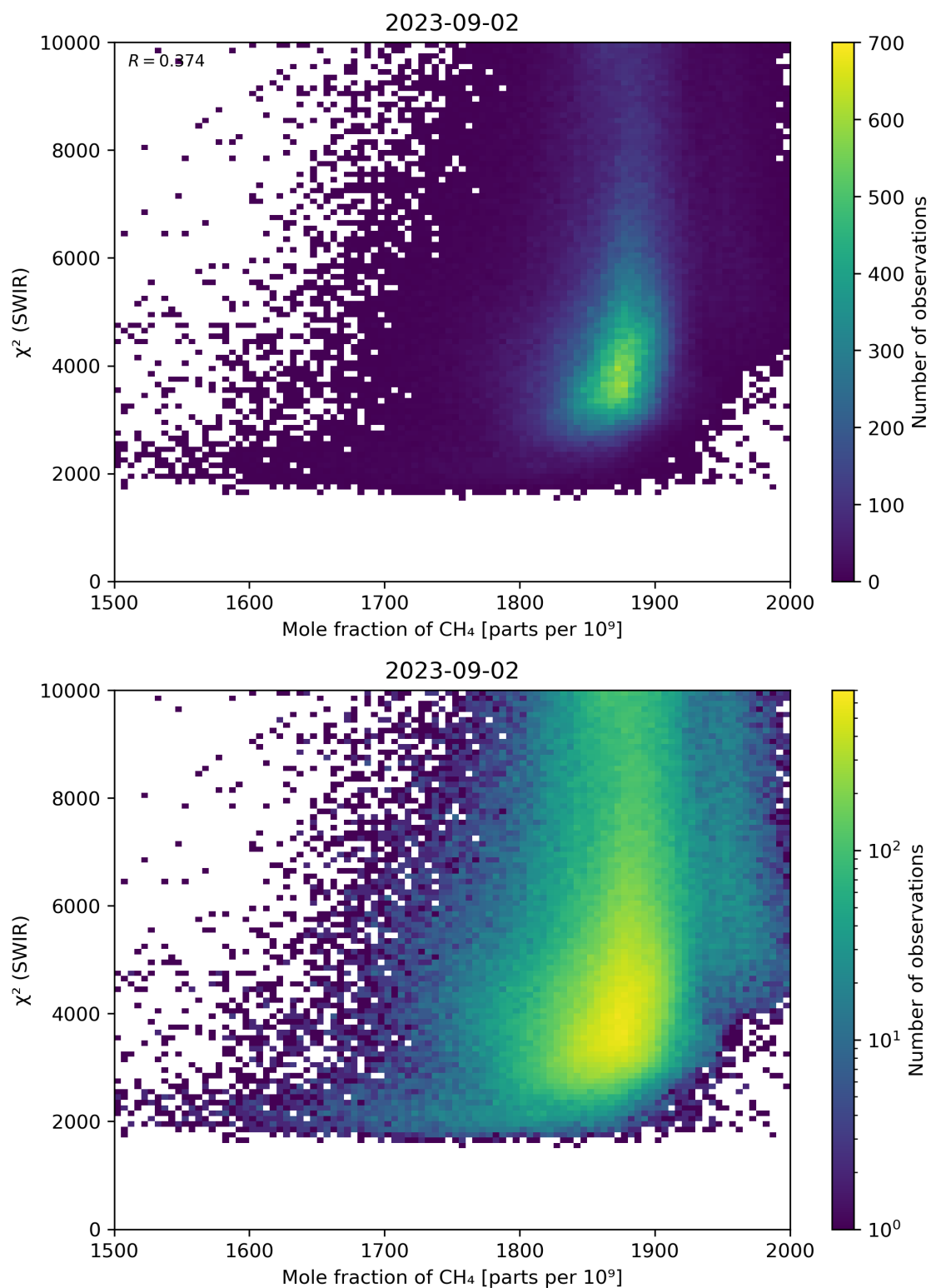
Figure 71: Scatter density plot of “Mole fraction of \text{CH}_4 ” against “ \chi^2 (SWIR)” for 2023-09-01 to 2023-09-03.
