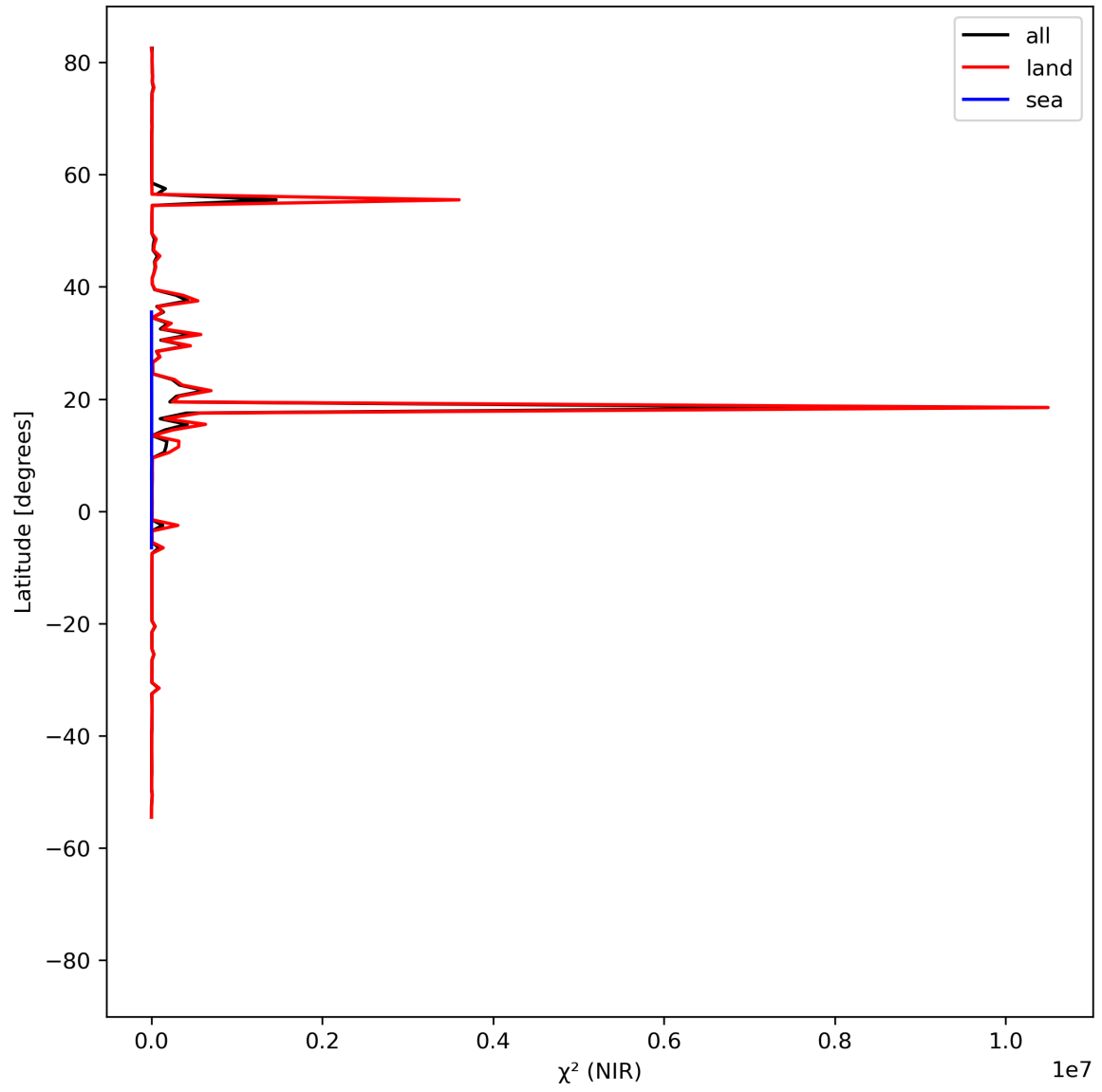
Figure 18: Zonal average of “ \chi^2 (NIR)” for 2023-09-01 to 2023-09-03.
