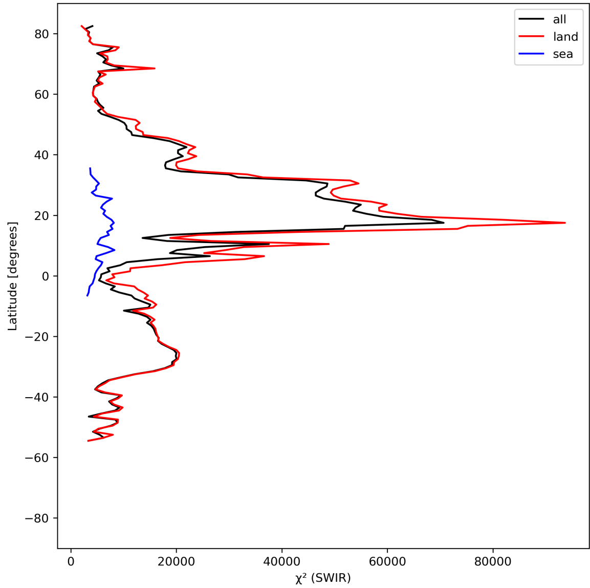
Figure 17: Zonal average of “ \chi^2 (SWIR)” for 2023-09-01 to 2023-09-03.
