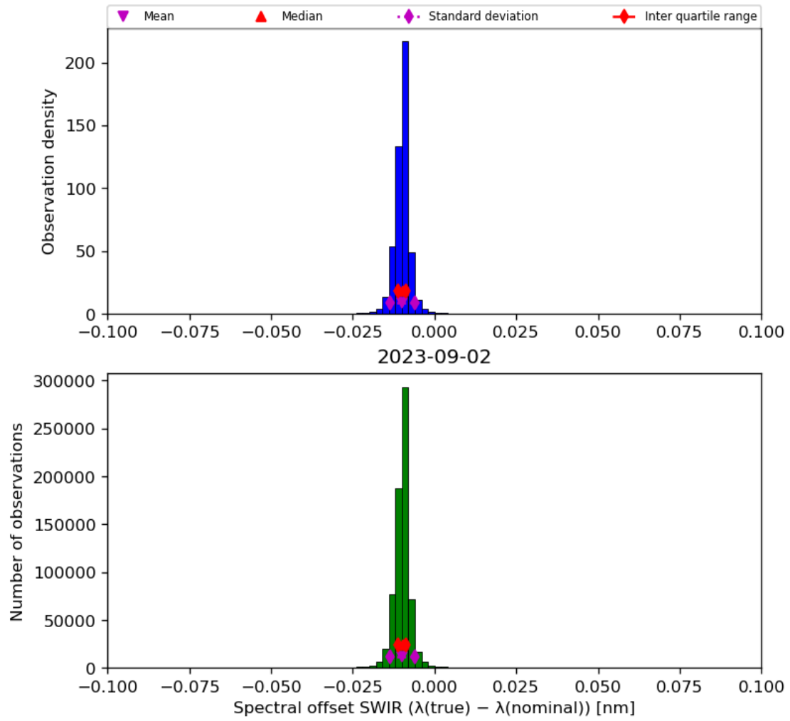
Figure 27: Histogram of “Spectral offset SWIR ( \lambda(\text{true}) - \lambda(\text{nominal}) )” for 2023-09-01 to 2023-09-03
