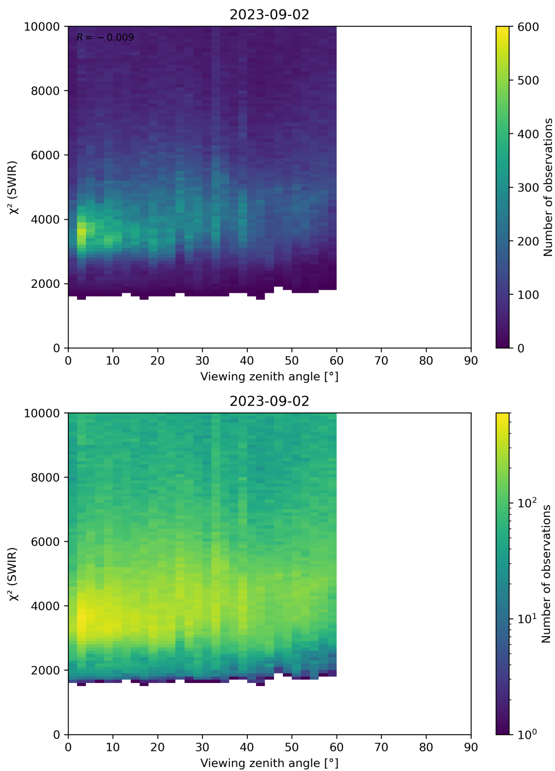
Figure 106: Scatter density plot of “Viewing zenith angle” against “ \chi^2 (SWIR)” for 2023-09-01 to 2023-09-03.
