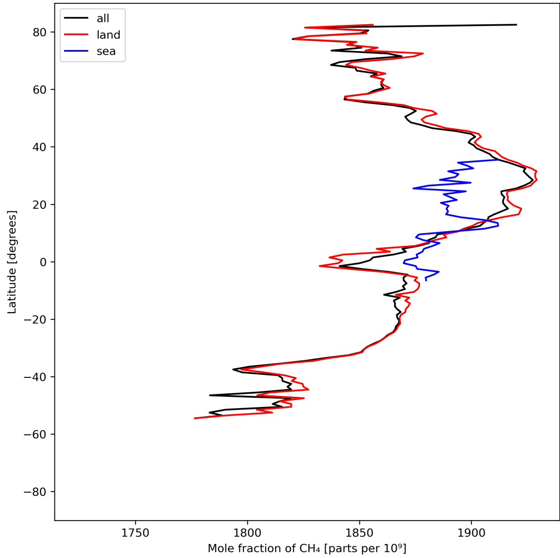
Figure 12: Zonal average of “Mole fraction of \text{CH}_4 ” for 2023-09-01 to 2023-09-03.
