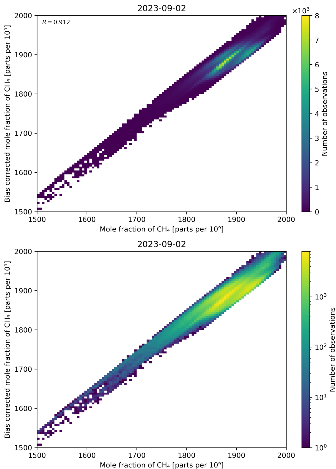
Figure 74: Scatter density plot of “Mole fraction of CH 4 ” against “Bias corrected mole fraction of CH 4 ” for 2023-09-01 to 2023-09-03.
