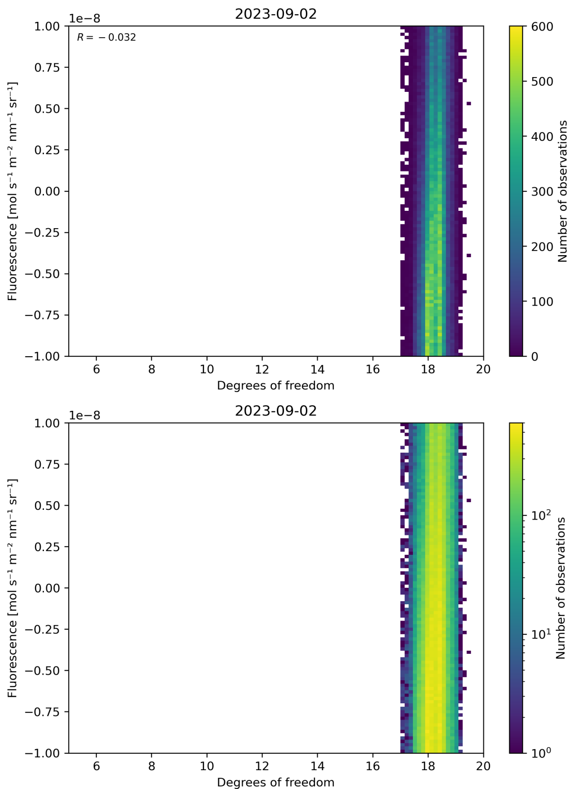
Figure 51: Scatter density plot of “Degrees of freedom” against “Fluorescence” for 2023-09-01 to 2023-09-03.
