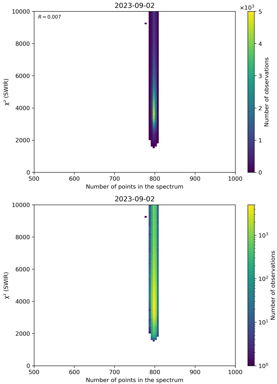
Figure 89: Scatter density plot of “Number of points in the spectrum” against “ \chi^2 (SWIR)” for 2023-09-01 to 2023-09-03.
