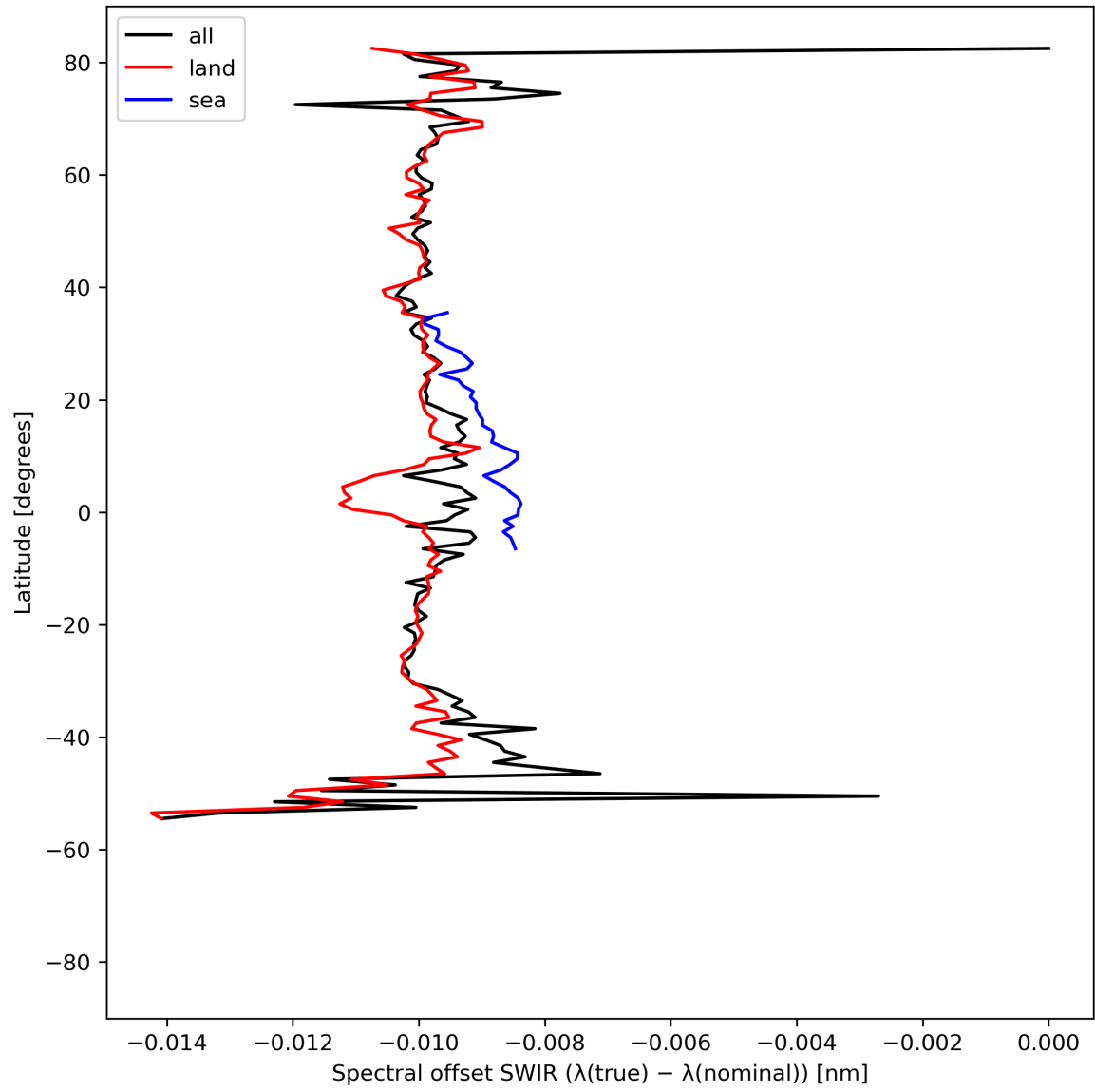
Figure 16: Zonal average of “Spectral offset SWIR ( \lambda(\text{true}) - \lambda(\text{nominal}) )” for 2023-09-01 to 2023-09-03.
