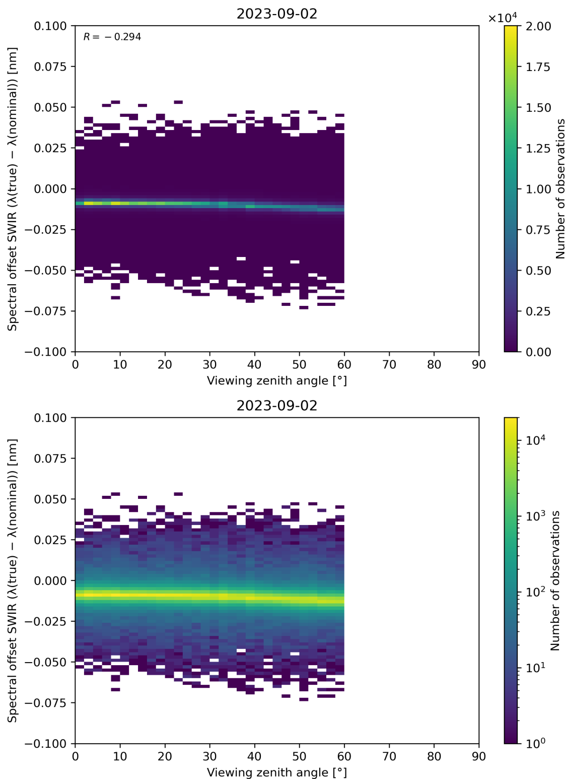
Figure 116: Scatter density plot of “Viewing zenith angle” against “Spectral offset SWIR ( \lambda(\text{true}) - \lambda(\text{nominal}) )” for 2023-09-01 to 2023-09-03.
