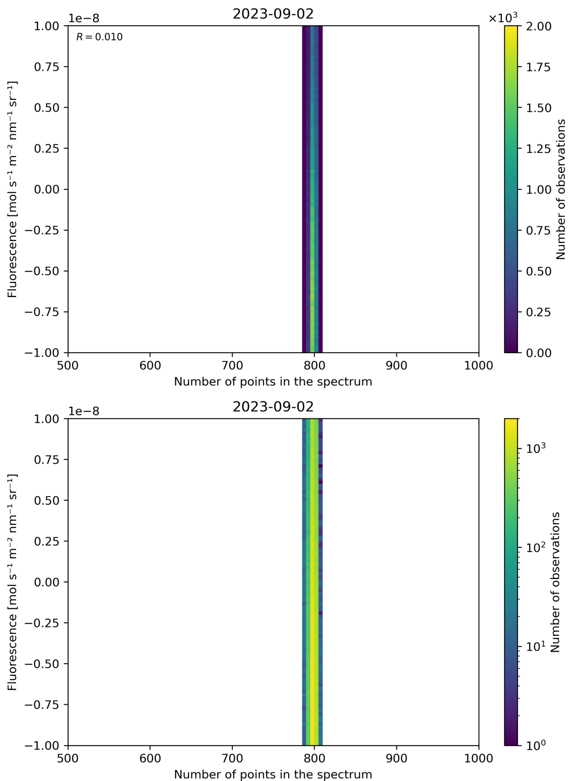
Figure 91: Scatter density plot of “Number of points in the spectrum” against “Fluorescence” for 2023-09-01 to 2023-09-03.
