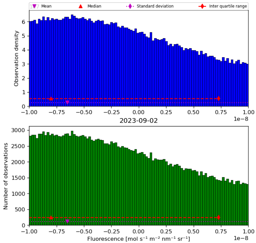
Figure 32: Histogram of “Fluorescence” for 2023-09-01 to 2023-09-03
