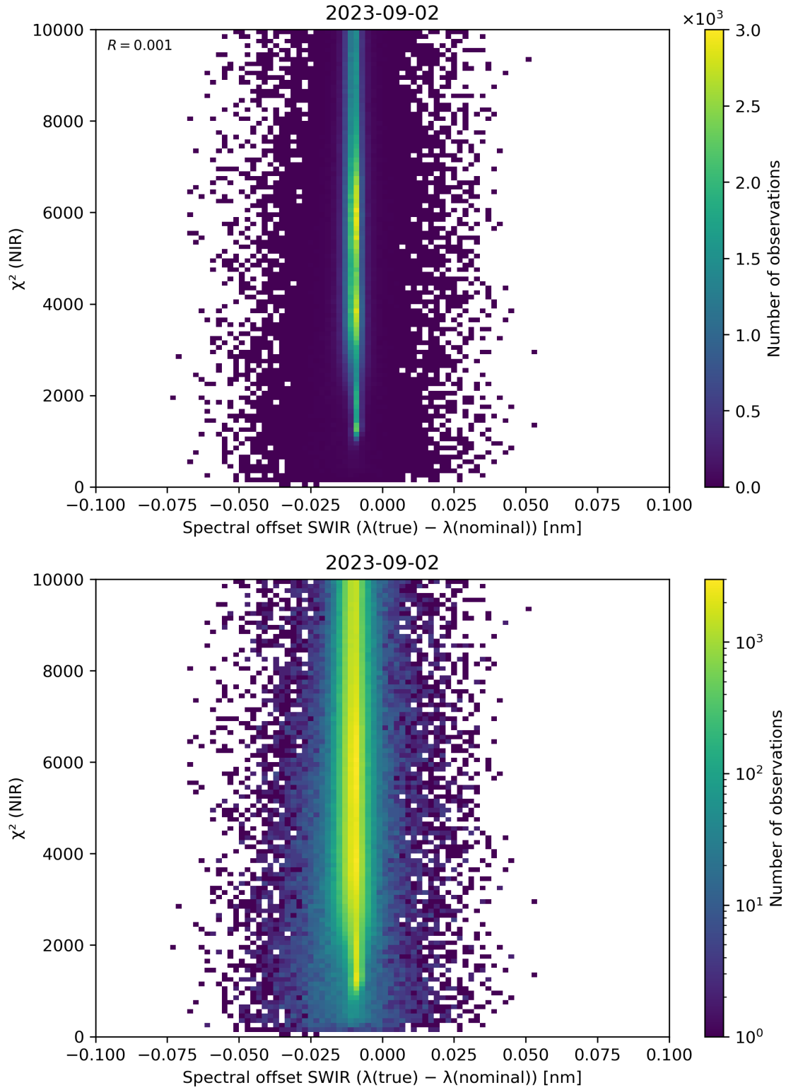
Figure 117: Scatter density plot of “Spectral offset SWIR ( \lambda(\text{true}) - \lambda(\text{nominal}) )” against “ \chi^2 (NIR)” for 2023-09-01 to 2023-09-03.
