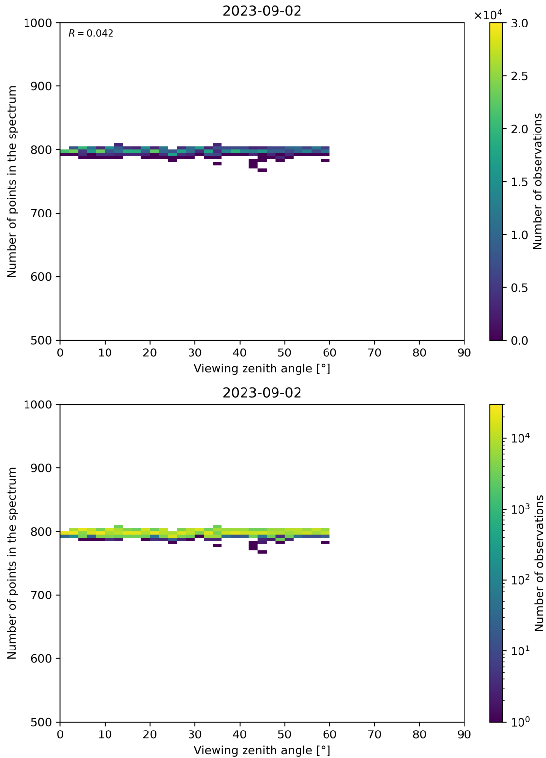
Figure 114: Scatter density plot of “Viewing zenith angle” against “Number of points in the spectrum” for 2023-09-01 to 2023-09-03.
