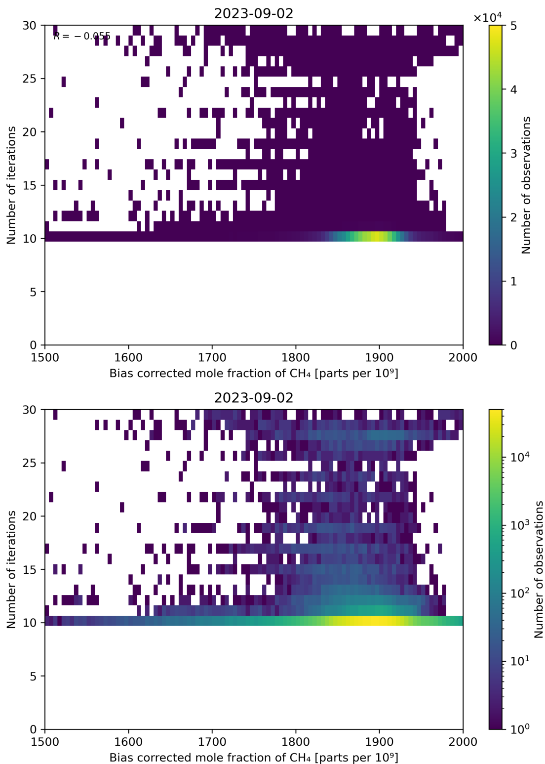
Figure 67: Scatter density plot of “Bias corrected mole fraction of CH 4 ” against “Number of iterations” for 2023-09-01 to 2023-09-03.
