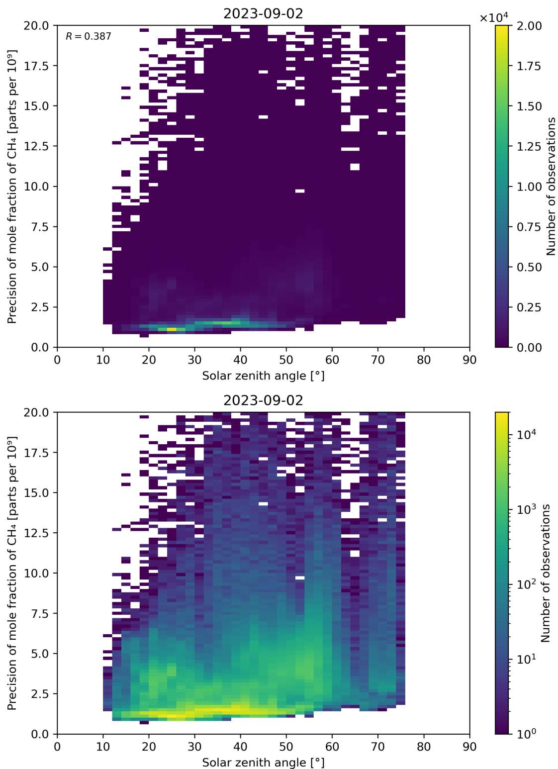
Figure 101: Scatter density plot of “Solar zenith angle” against “Precision of mole fraction of \text{CH}_4 ” for 2023-09-01 to 2023-09-03.
