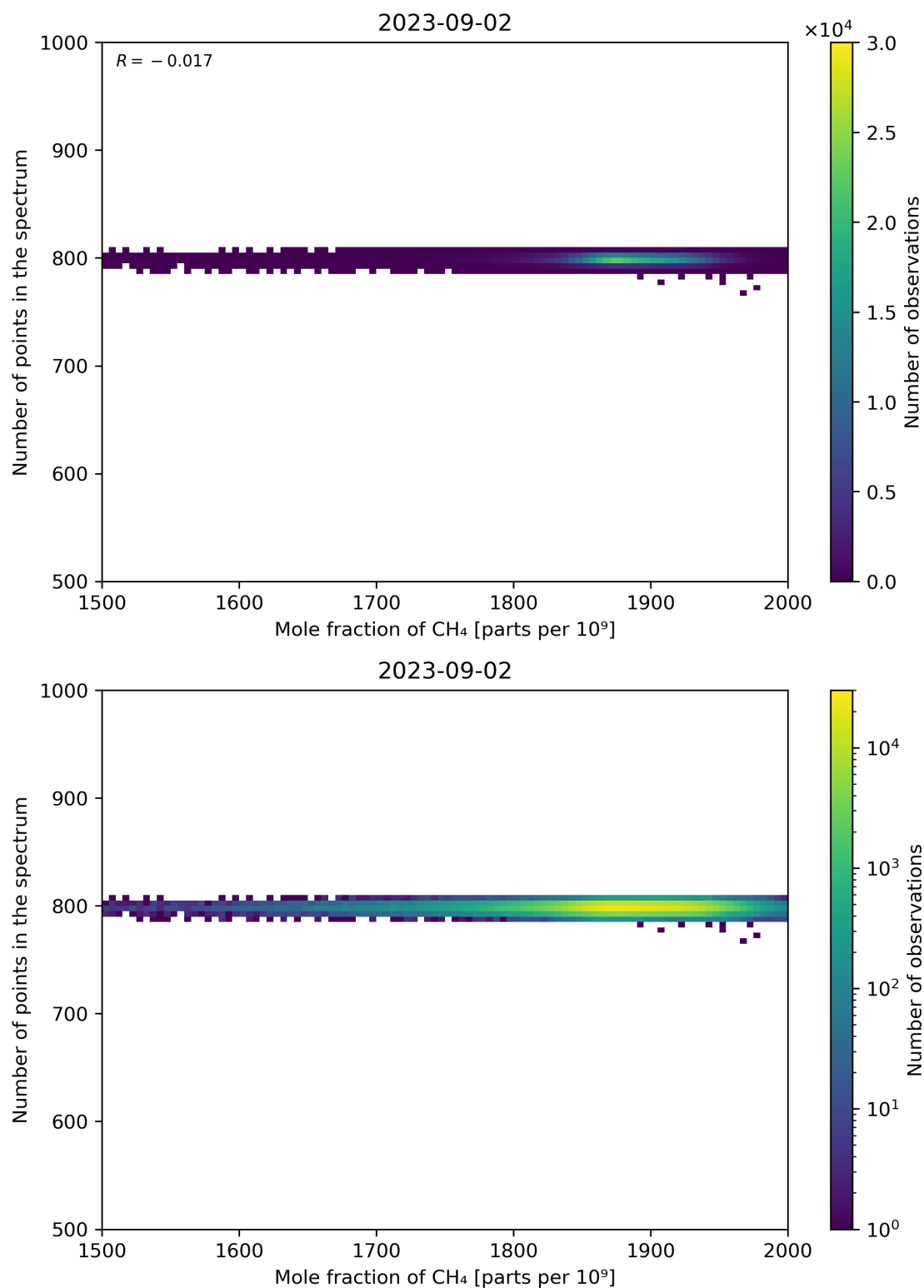
Figure 77: Scatter density plot of “Mole fraction of CH 4 ” against “Number of points in the spectrum” for 2023-09-01 to 2023-09-03.
