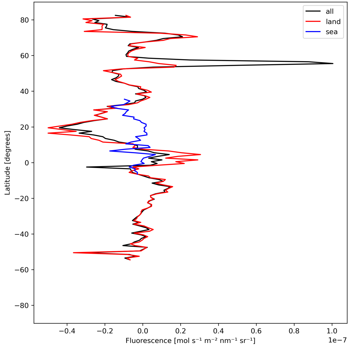
Figure 21: Zonal average of “Fluorescence” for 2023-09-01 to 2023-09-03.
