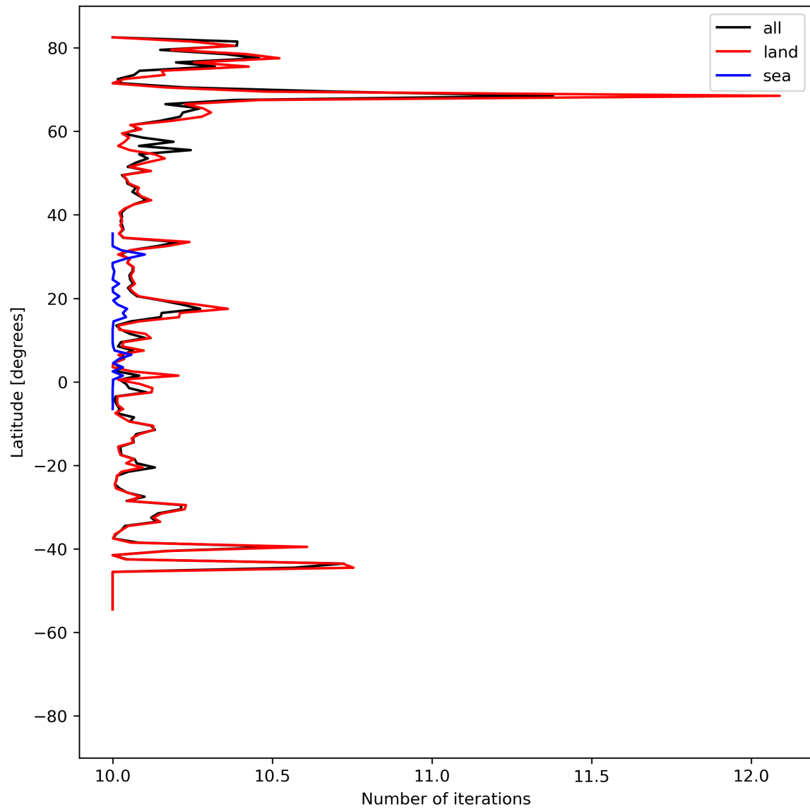
Figure 20: Zonal average of “Number of iterations” for 2023-09-01 to 2023-09-03.
