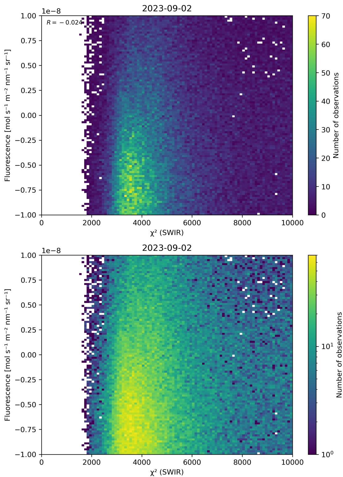
Figure 49: Scatter density plot of “ \chi^2 (SWIR)” against “Fluorescence” for 2023-09-01 to 2023-09-03.
