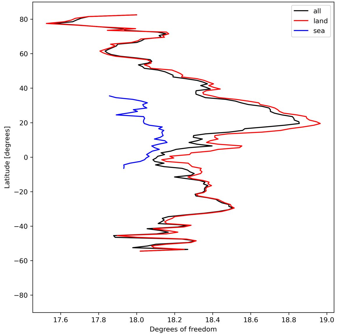
Figure 19: Zonal average of “Degrees of freedom” for 2023-09-01 to 2023-09-03.
