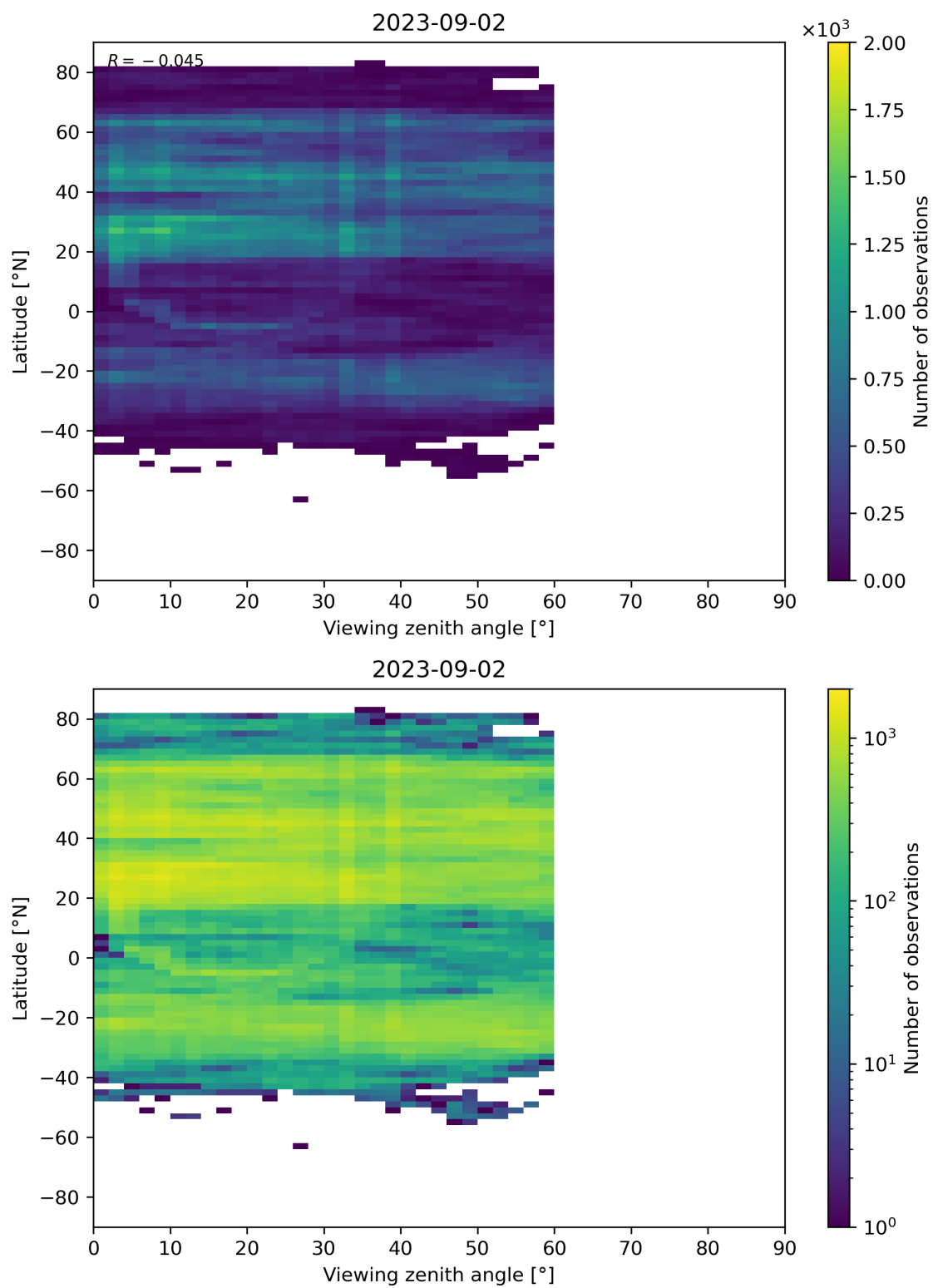
Figure 109: Scatter density plot of “Viewing zenith angle” against “Latitude” for 2023-09-01 to 2023-09-03.
