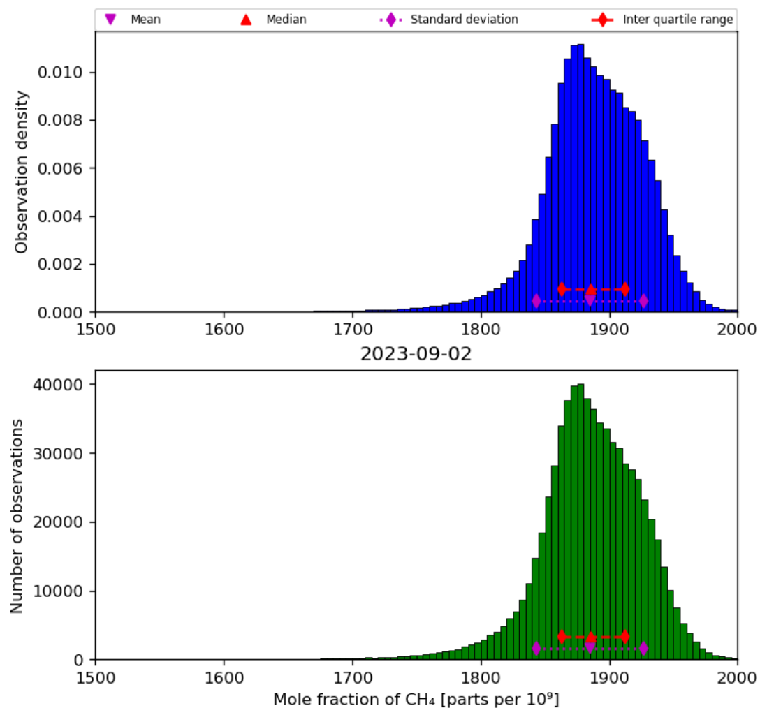
Figure 23: Histogram of “Mole fraction of CH 4 ” for 2023-09-01 to 2023-09-03
