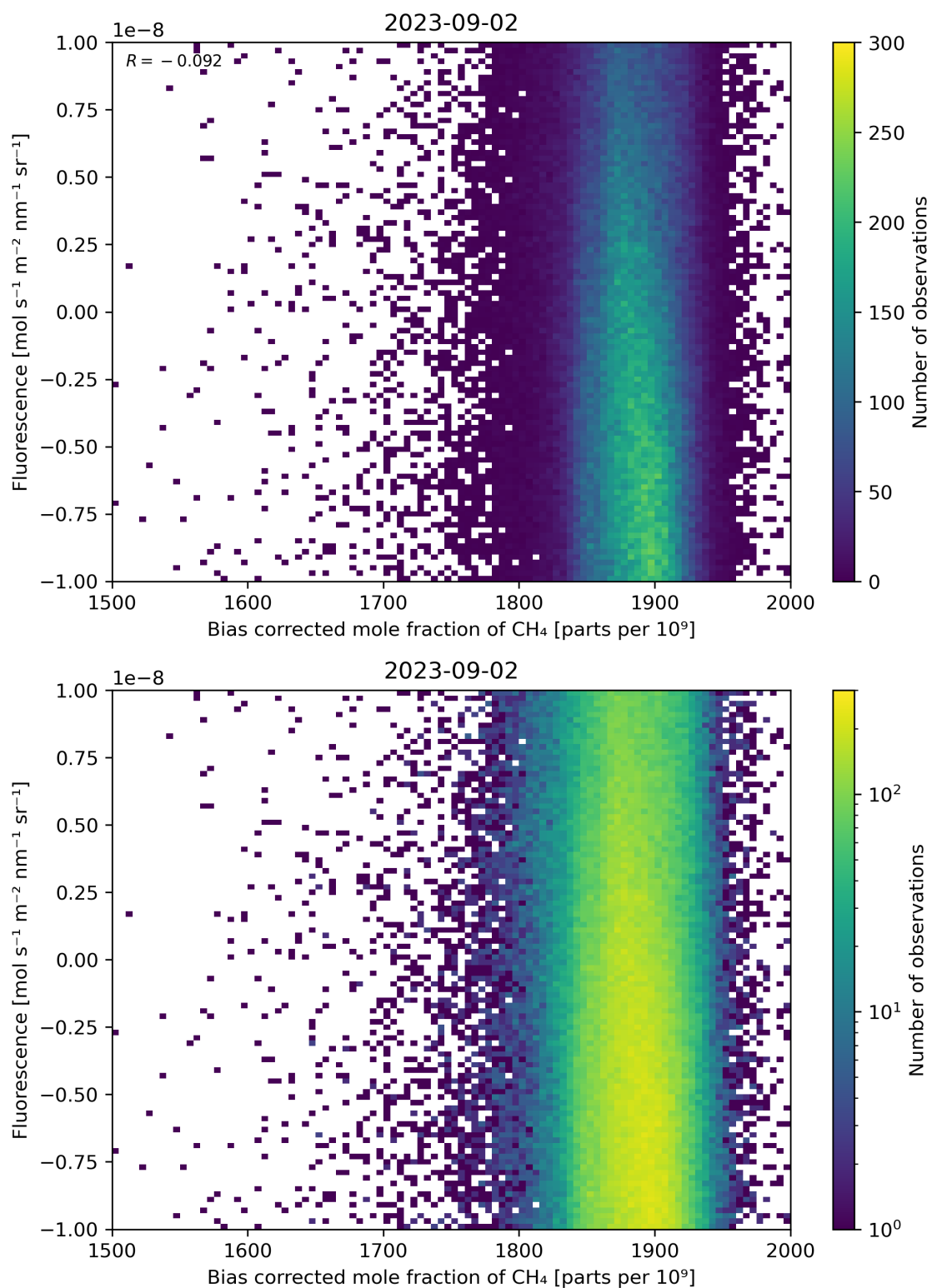
Figure 66: Scatter density plot of “Bias corrected mole fraction of \text{CH}_4 ” against “Fluorescence” for 2023-09-01 to 2023-09-03.
