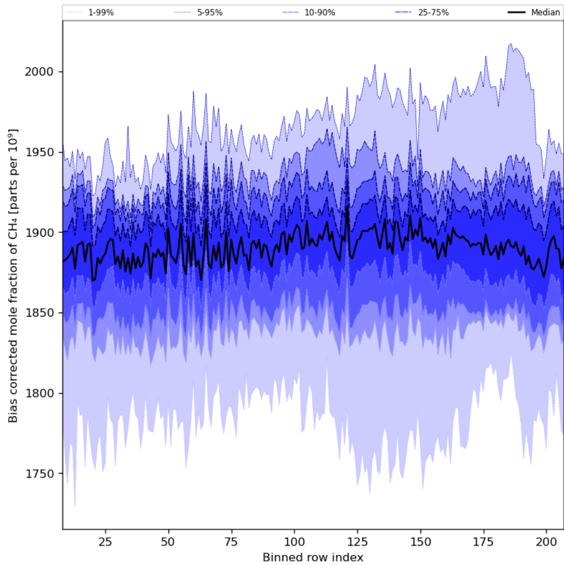
Figure 36: Along track statistics of “Bias corrected mole fraction of CH 4 ” for 2023-09-01 to 2023-09-03
