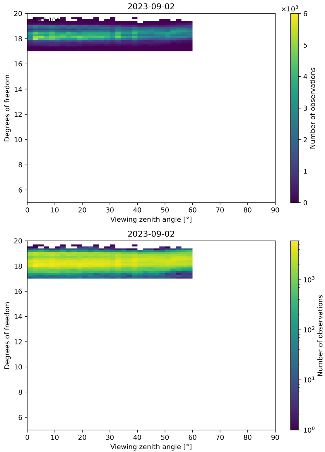
Figure 107: Scatter density plot of “Viewing zenith angle” against “Degrees of freedom” for 2023-09-01 to 2023-09-03.
