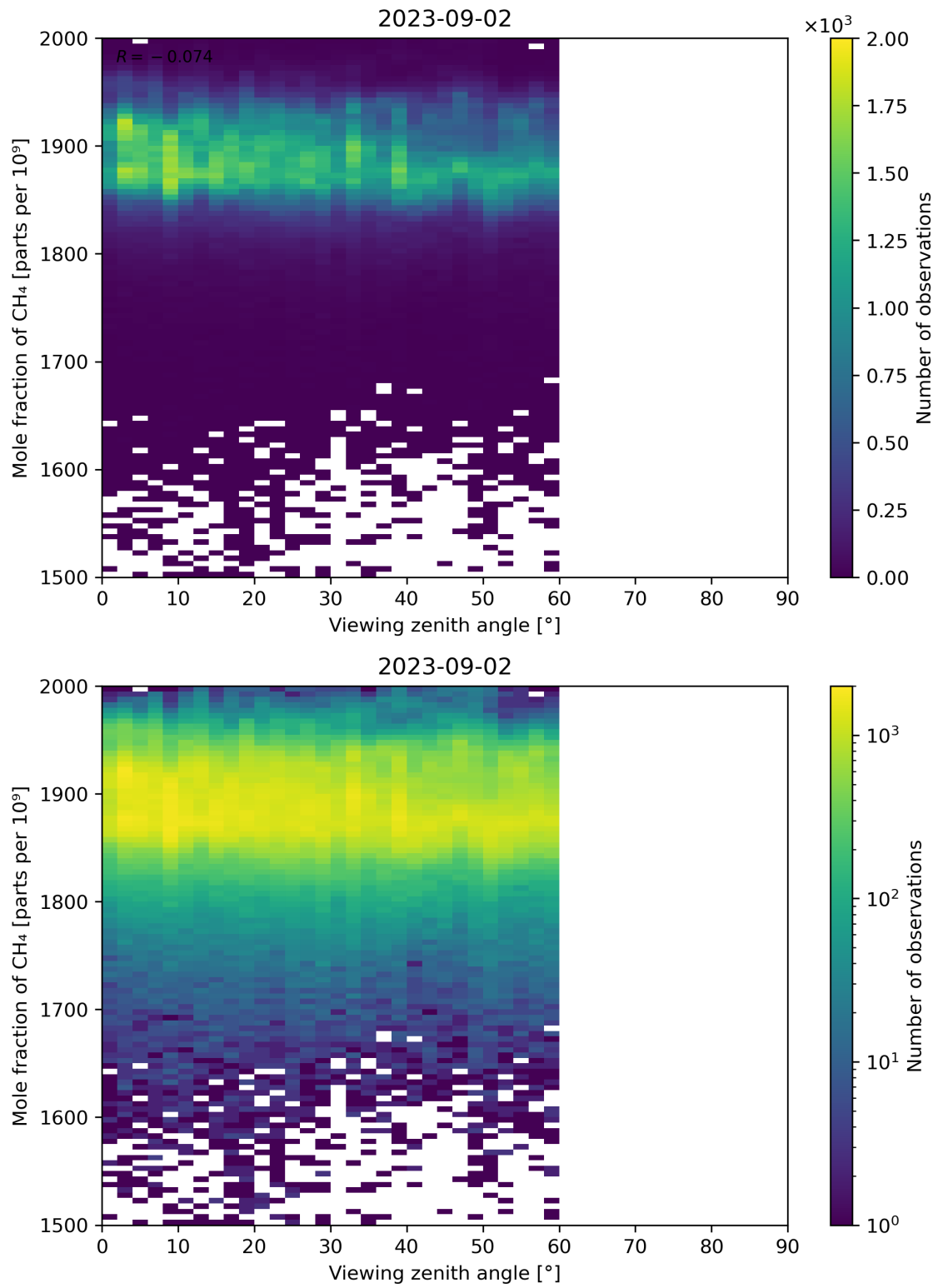
Figure 110: Scatter density plot of “Viewing zenith angle” against “Mole fraction of CH 4 ” for 2023-09-01 to 2023-09-03.
