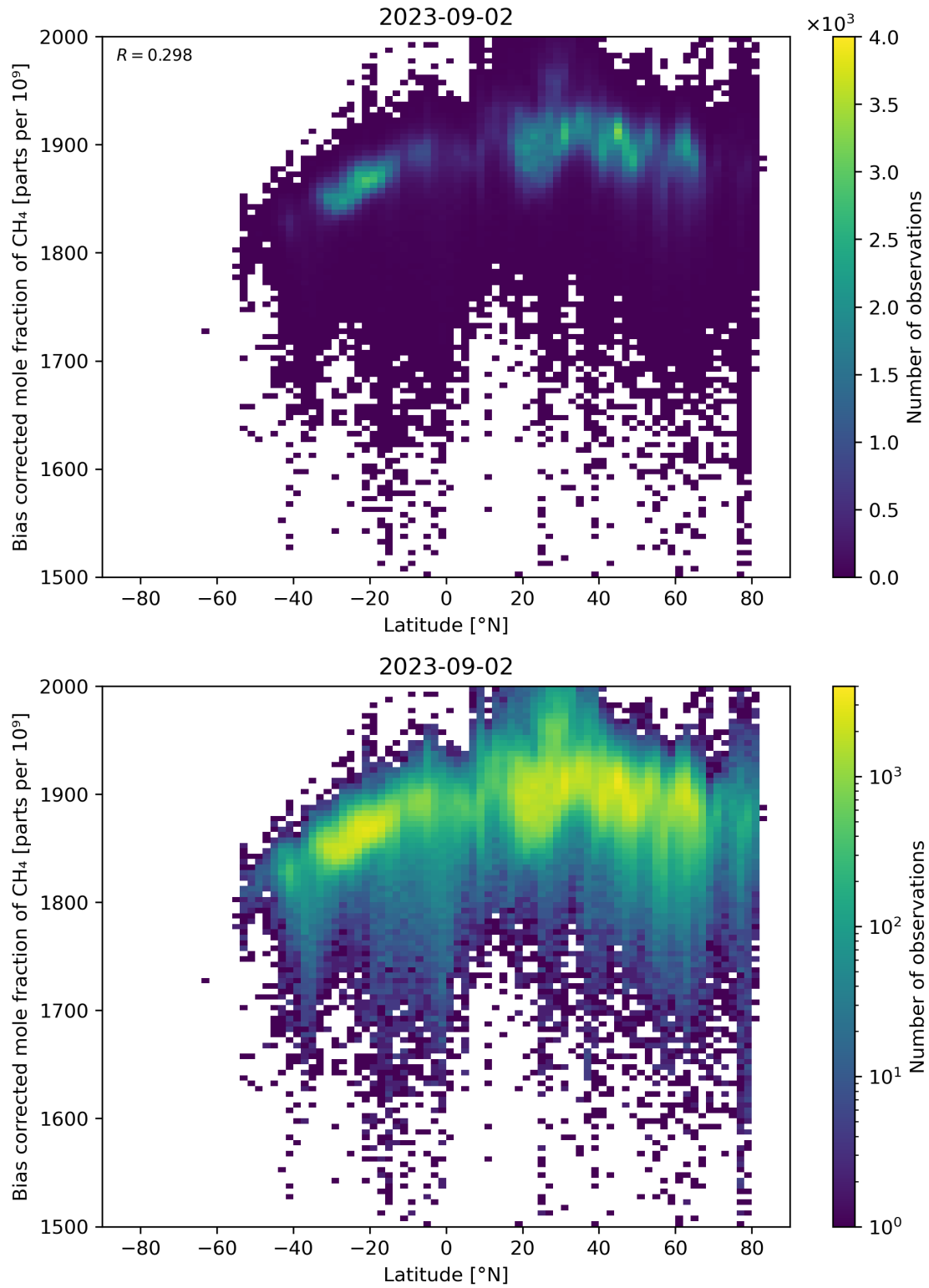
Figure 58: Scatter density plot of “Latitude” against “Bias corrected mole fraction of CH 4 ” for 2023-09-01 to 2023-09-03.
