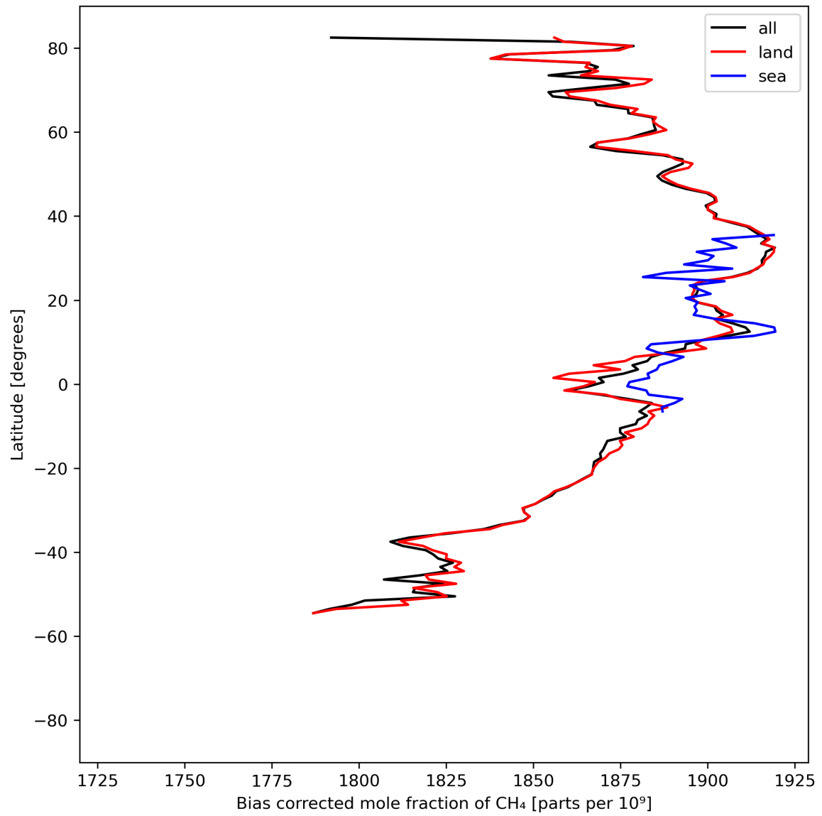
Figure 14: Zonal average of “Bias corrected mole fraction of \text{CH}_4 ” for 2023-09-01 to 2023-09-03.
