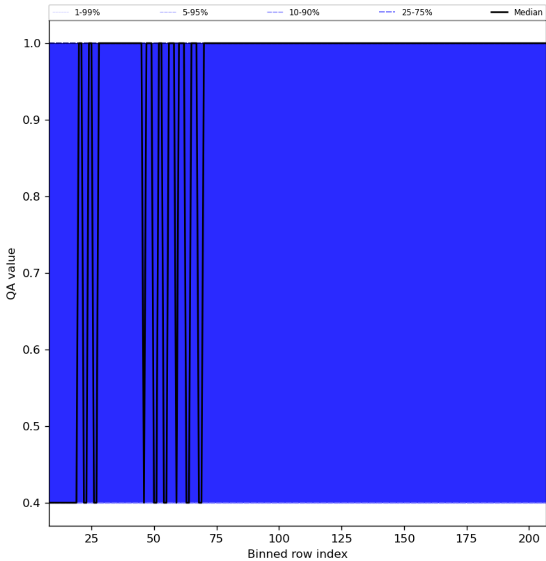
Figure 33: Along track statistics of “QA value” for 2023-09-01 to 2023-09-03
