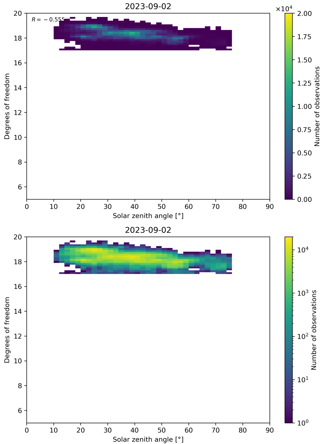
Figure 96: Scatter density plot of “Solar zenith angle” against “Degrees of freedom” for 2023-09-01 to 2023-09-03.
