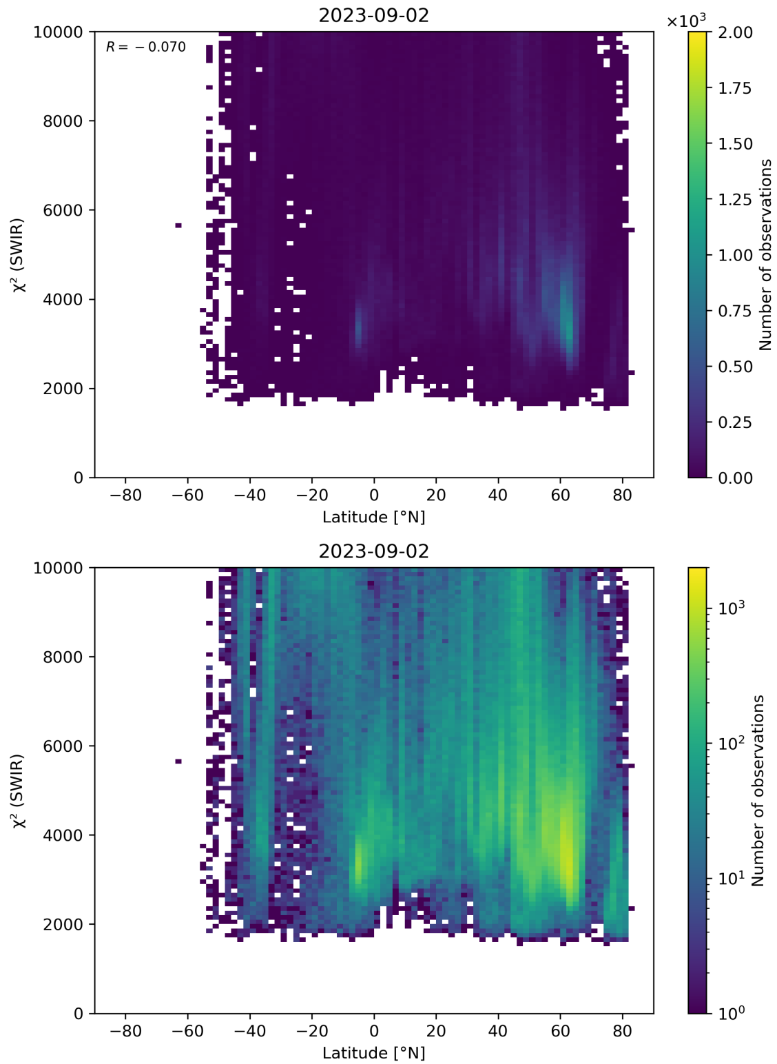
Figure 54: Scatter density plot of “Latitude” against “ \chi^2 (SWIR)” for 2023-09-01 to 2023-09-03.
