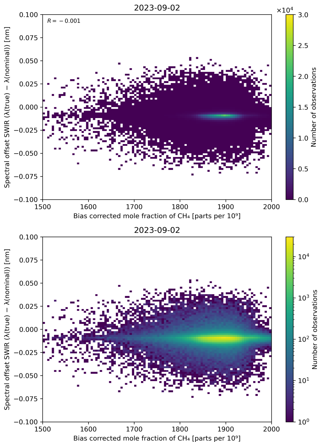
Figure 69: Scatter density plot of “Bias corrected mole fraction of CH 4 ” against “Spectral offset SWIR ( \lambda(\text{true}) - \lambda(\text{nominal}) )” for 2023-09-01 to 2023-09-03.
