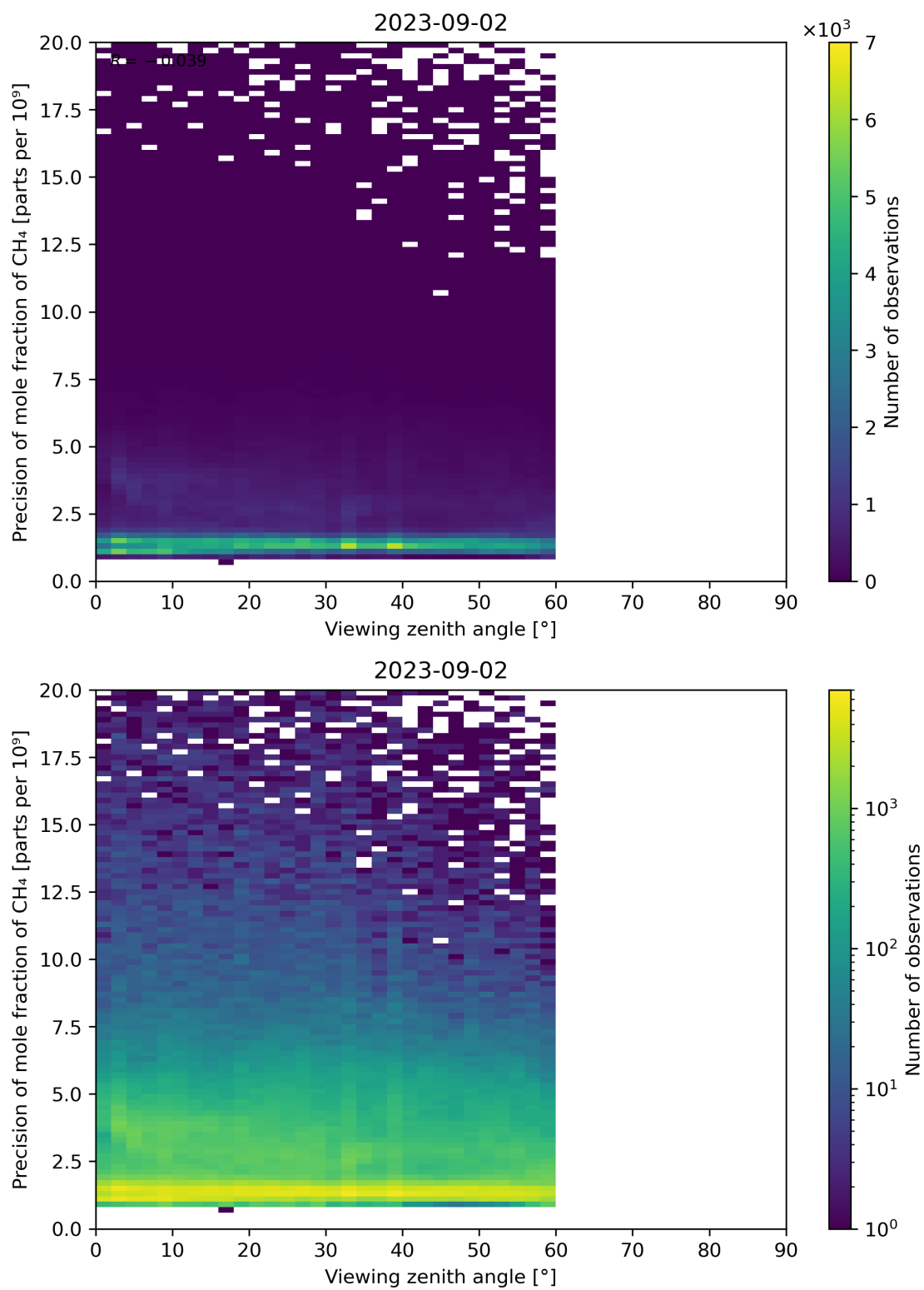
Figure 112: Scatter density plot of “Viewing zenith angle” against “Precision of mole fraction of CH 4 ” for 2023-09-01 to 2023-09-03.
