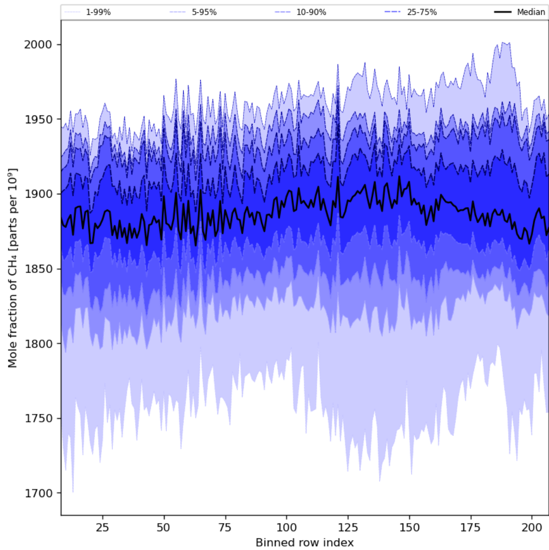
Figure 34: Along track statistics of “Mole fraction of CH 4 ” for 2023-09-01 to 2023-09-03
