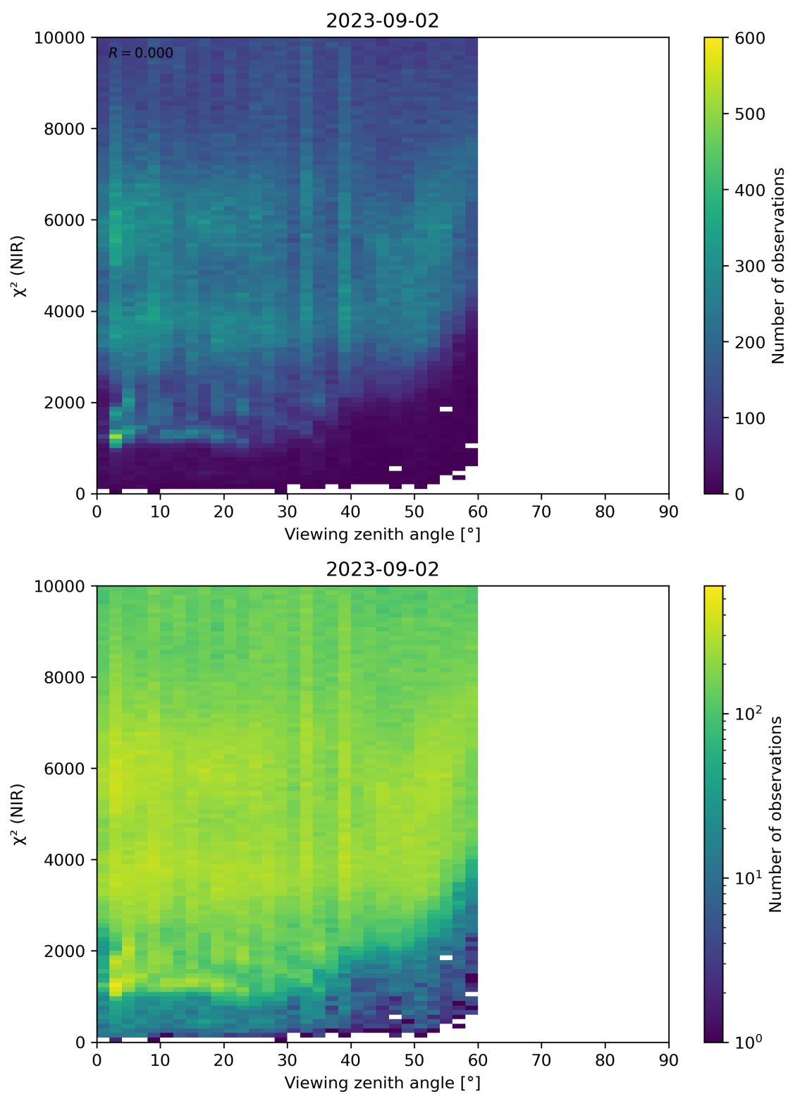
Figure 105: Scatter density plot of “Viewing zenith angle” against “ \chi^2 (NIR)” for 2023-09-01 to 2023-09-03.
