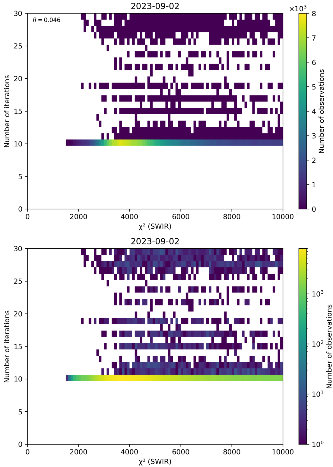
Figure 50: Scatter density plot of “ \chi^2 (SWIR)” against “Number of iterations” for 2023-09-01 to 2023-09-03.
