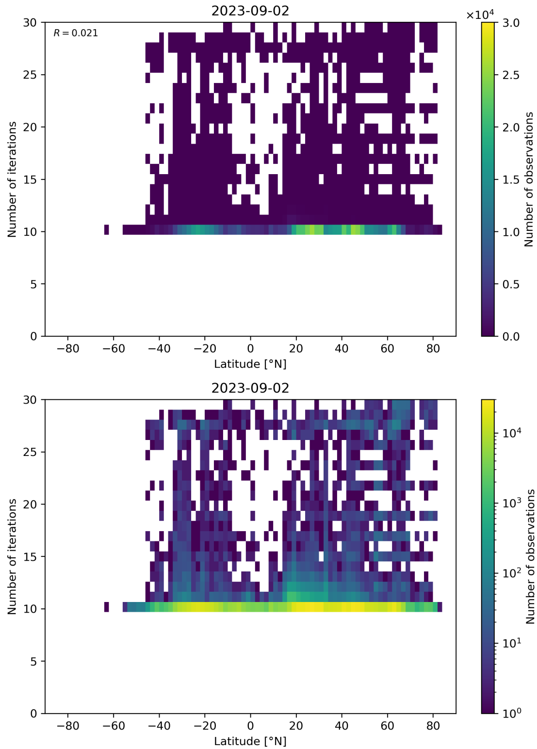
Figure 60: Scatter density plot of “Latitude” against “Number of iterations” for 2023-09-01 to 2023-09-03.
