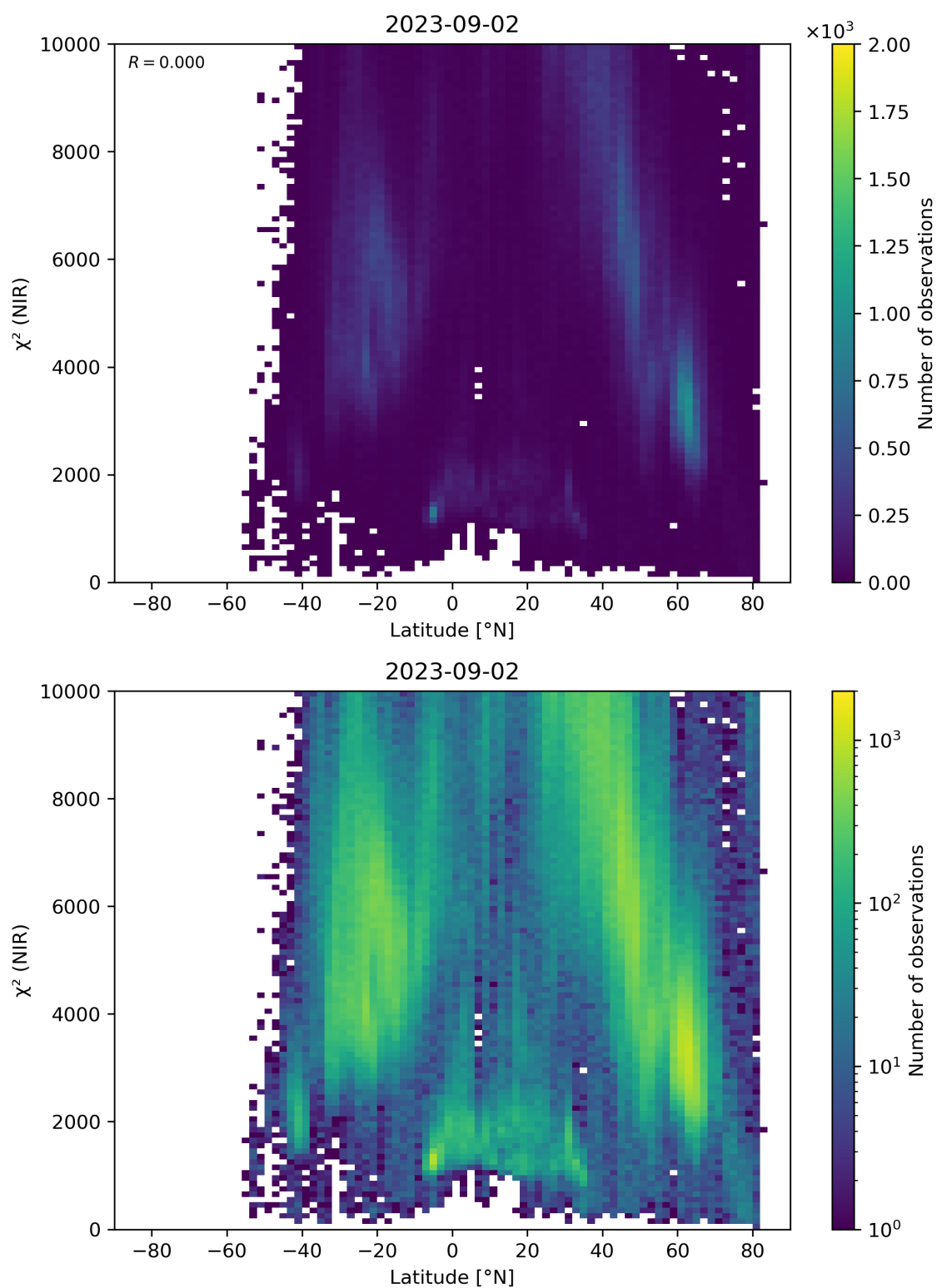
Figure 53: Scatter density plot of “Latitude” against “ \chi^2 (NIR)” for 2023-09-01 to 2023-09-03.
