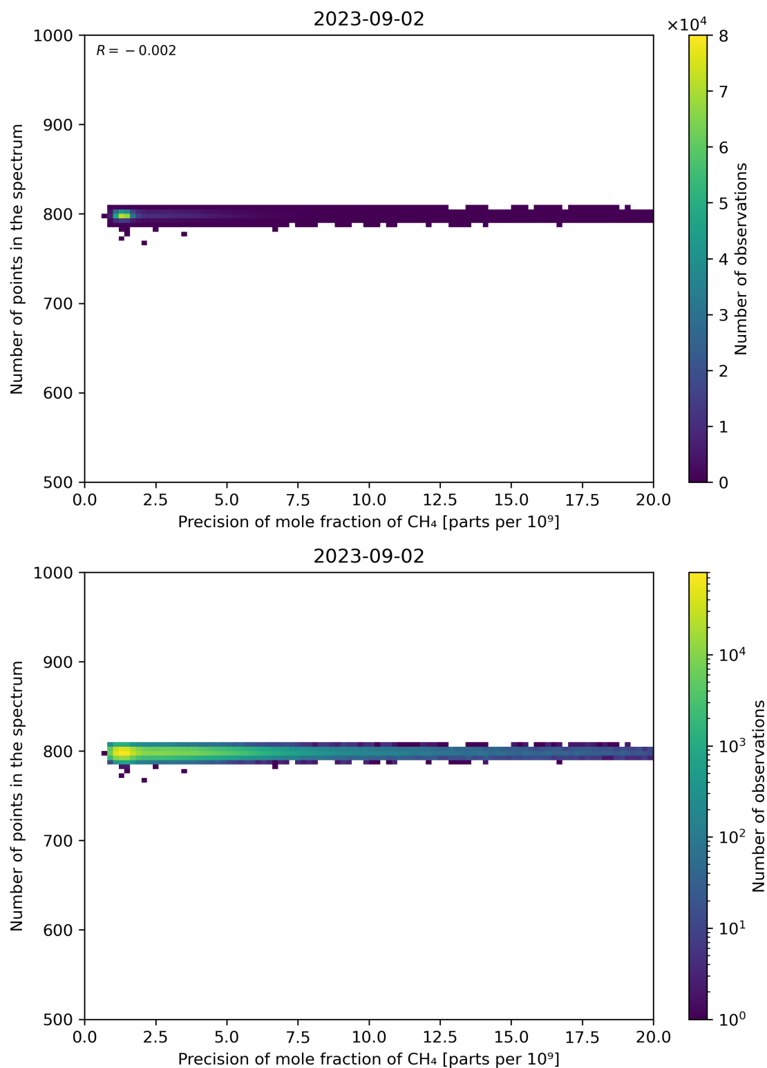
Figure 84: Scatter density plot of “Precision of mole fraction of CH 4 ” against “Number of points in the spectrum” for 2023-09-01 to 2023-09-03.
