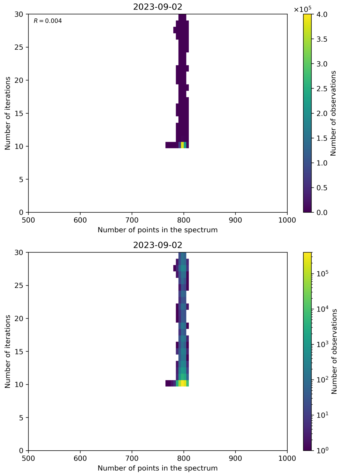
Figure 92: Scatter density plot of “Number of points in the spectrum” against “Number of iterations” for 2023-09-01 to 2023-09-03.
