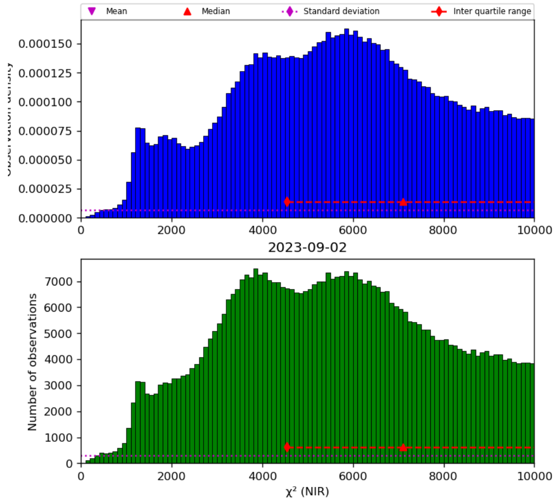
Figure 29: Histogram of “ \chi^2 (NIR)” for 2023-09-01 to 2023-09-03
