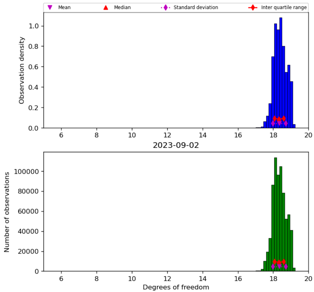
Figure 30: Histogram of “Degrees of freedom” for 2023-09-01 to 2023-09-03
