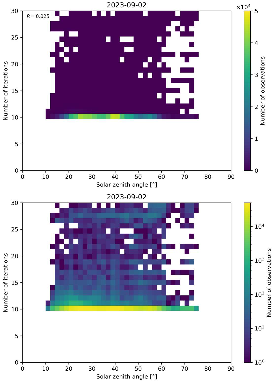
Figure 102: Scatter density plot of “Solar zenith angle” against “Number of iterations” for 2023-09-01 to 2023-09-03.
