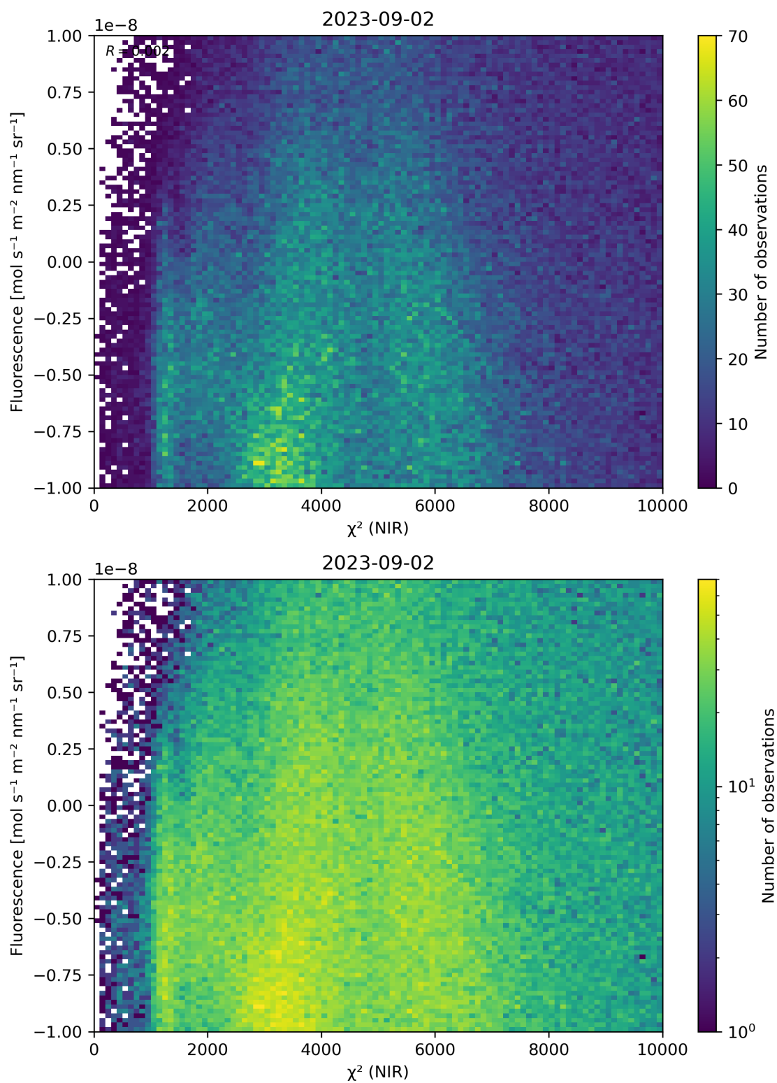
Figure 45: Scatter density plot of “ \chi^2 (NIR)” against “Fluorescence” for 2023-09-01 to 2023-09-03.
