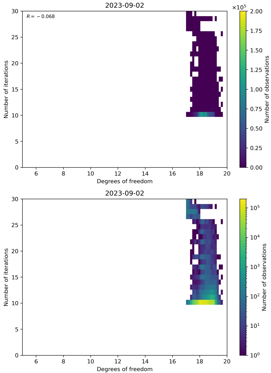
Figure 52: Scatter density plot of “Degrees of freedom” against “Number of iterations” for 2023-09-01 to 2023-09-03.
