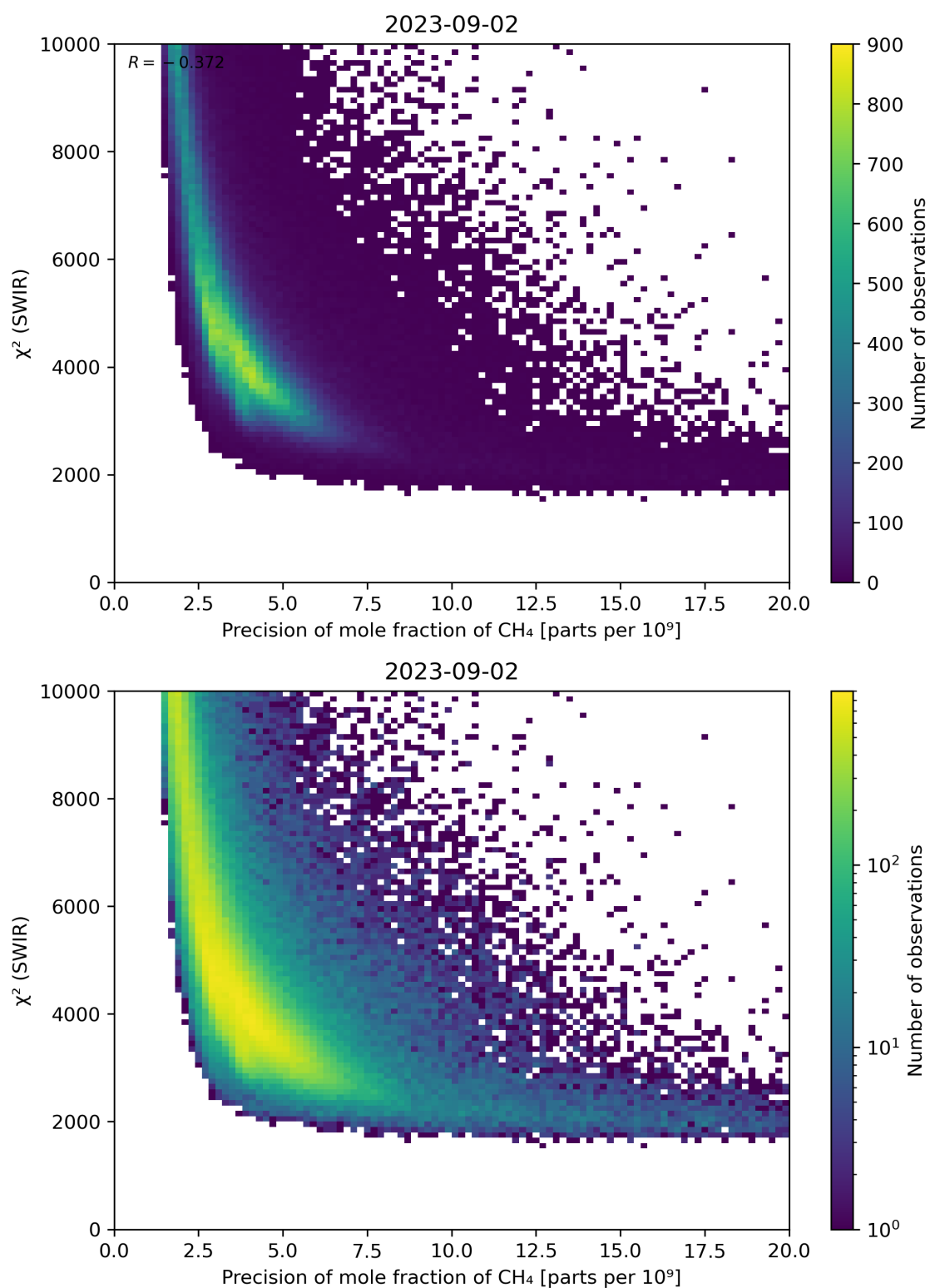
Figure 79: Scatter density plot of “Precision of mole fraction of CH 4 ” against “ \chi^2 (SWIR)” for 2023-09-01 to 2023-09-03.
