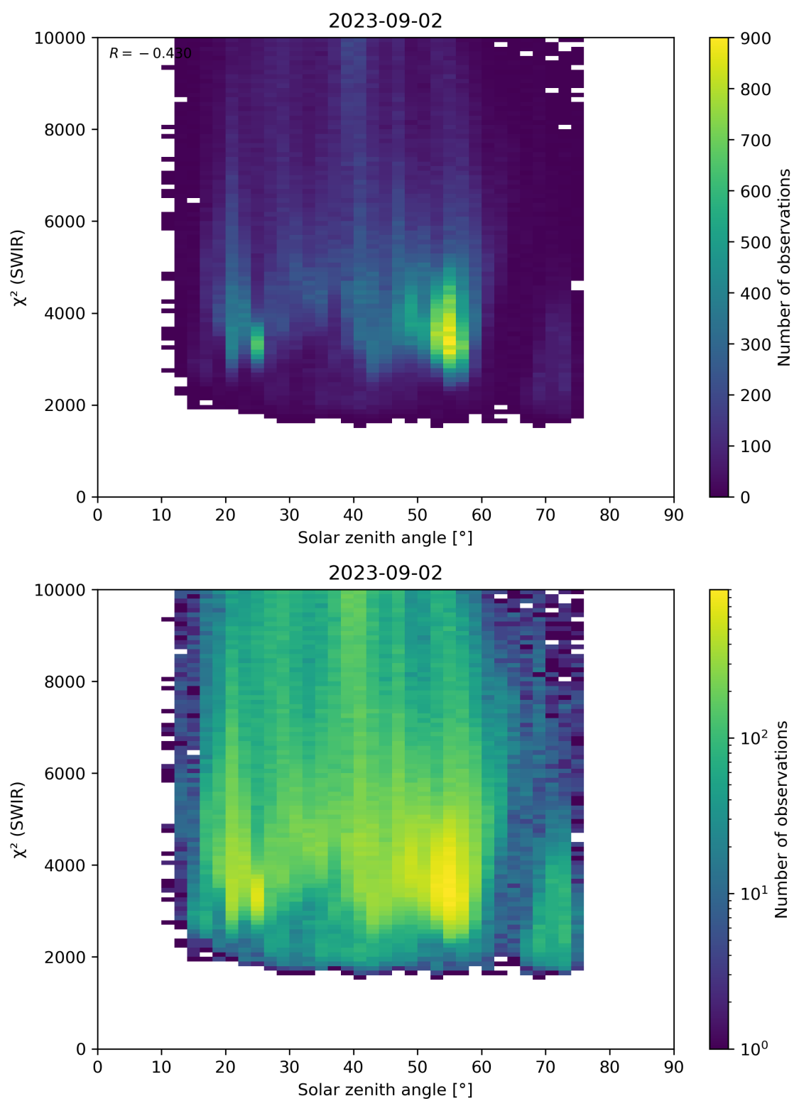
Figure 95: Scatter density plot of “Solar zenith angle” against “ \chi^2 (SWIR)” for 2023-09-01 to 2023-09-03.
