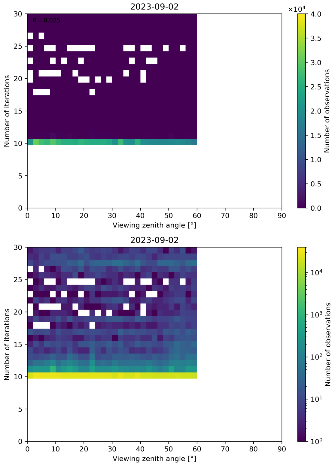
Figure 113: Scatter density plot of “Viewing zenith angle” against “Number of iterations” for 2023-09-01 to 2023-09-03.
