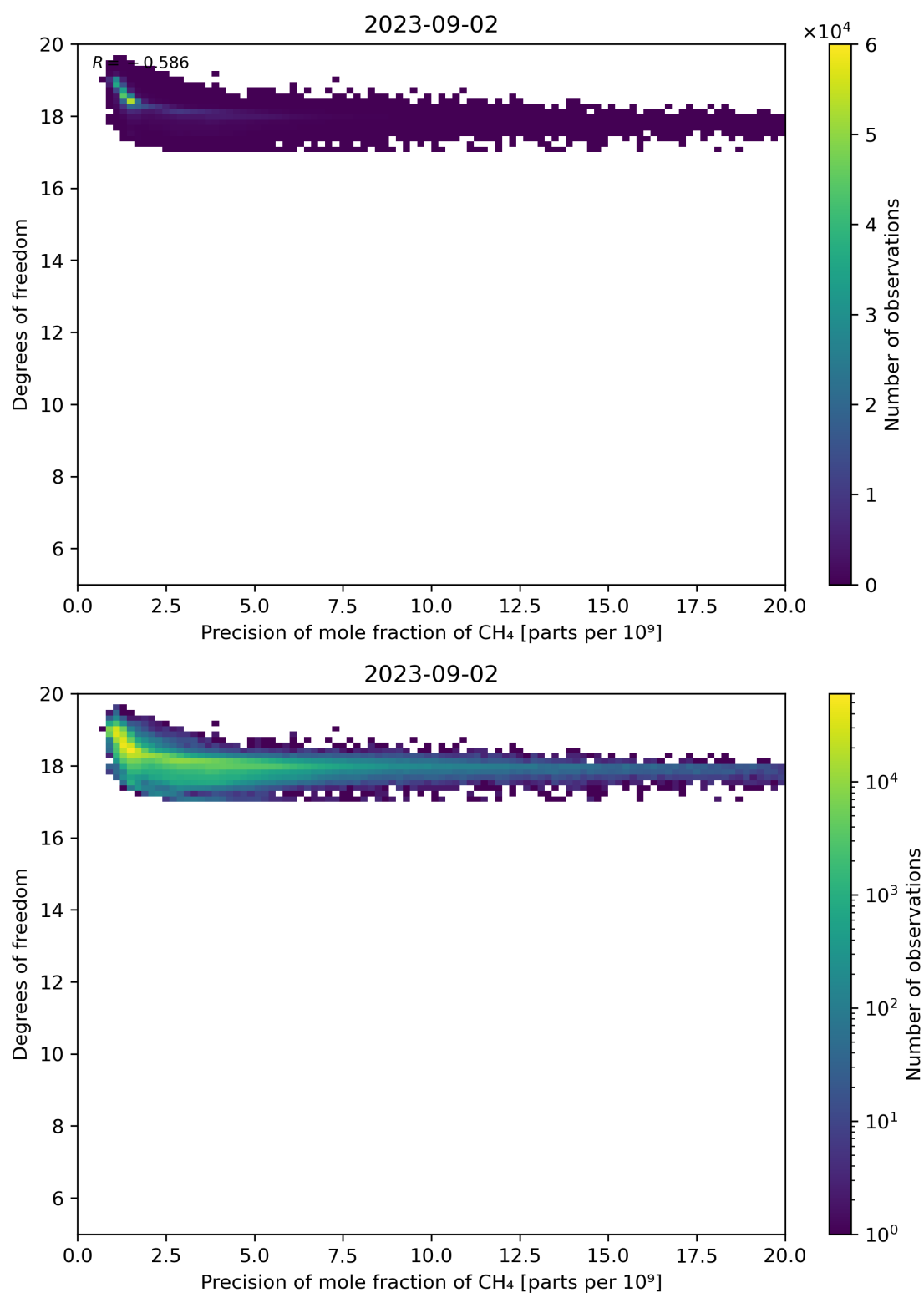
Figure 80: Scatter density plot of “Precision of mole fraction of CH 4 ” against “Degrees of freedom” for 2023-09-01 to 2023-09-03.
