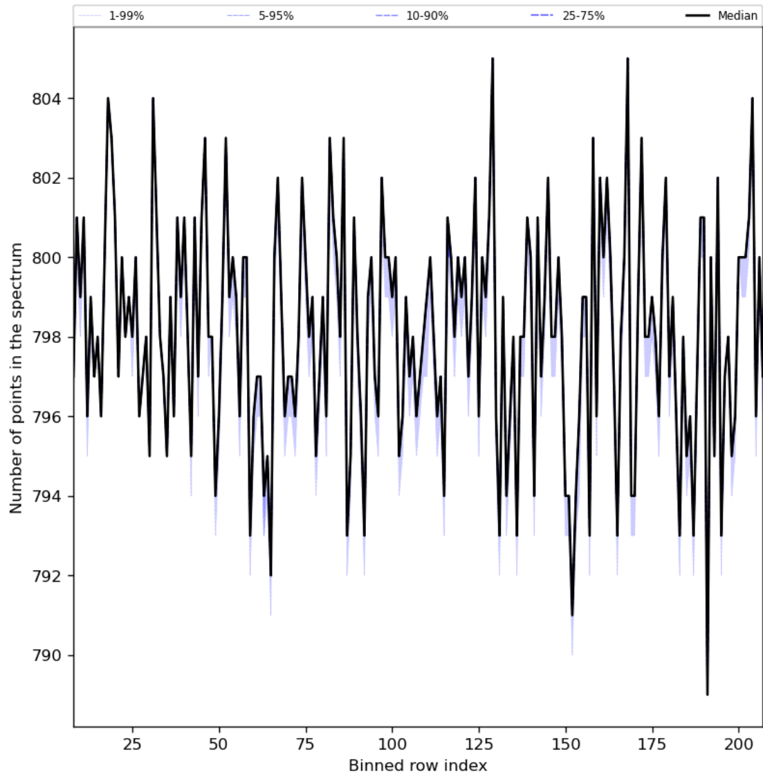
Figure 37: Along track statistics of “Number of points in the spectrum” for 2023-09-01 to 2023-09-03
