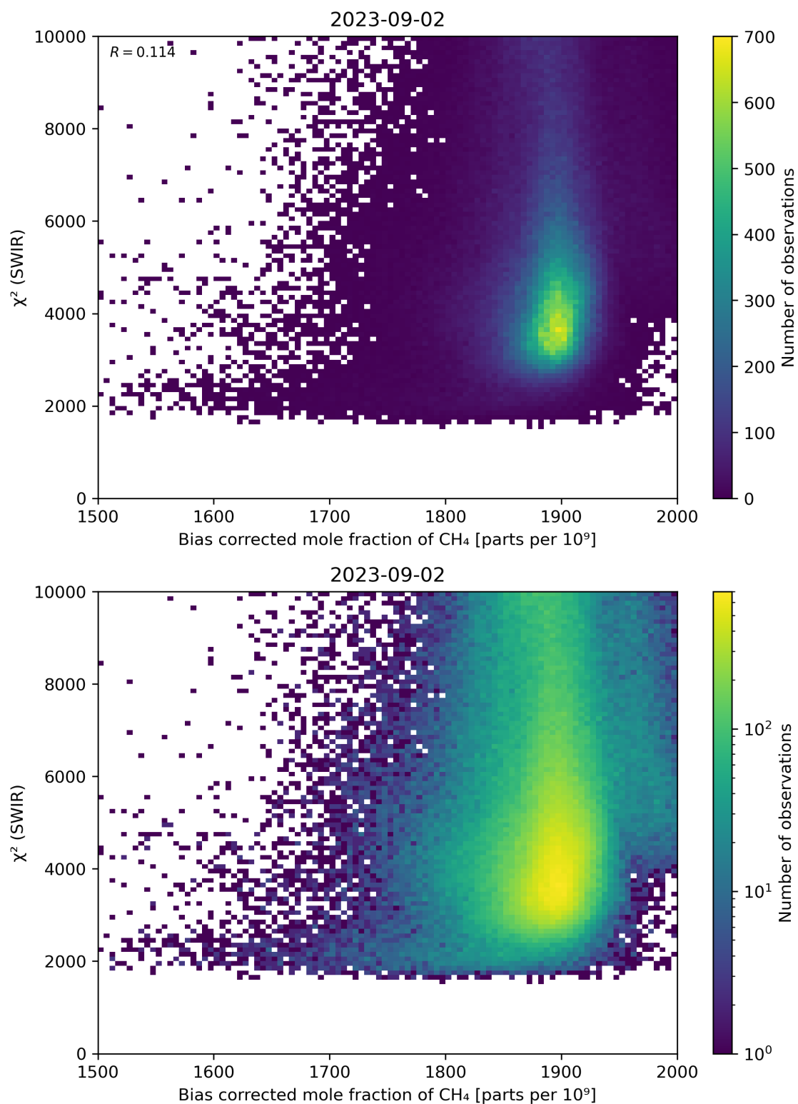
Figure 64: Scatter density plot of “Bias corrected mole fraction of CH 4 ” against “ \chi^2 (SWIR)” for 2023-09-01 to 2023-09-03.
