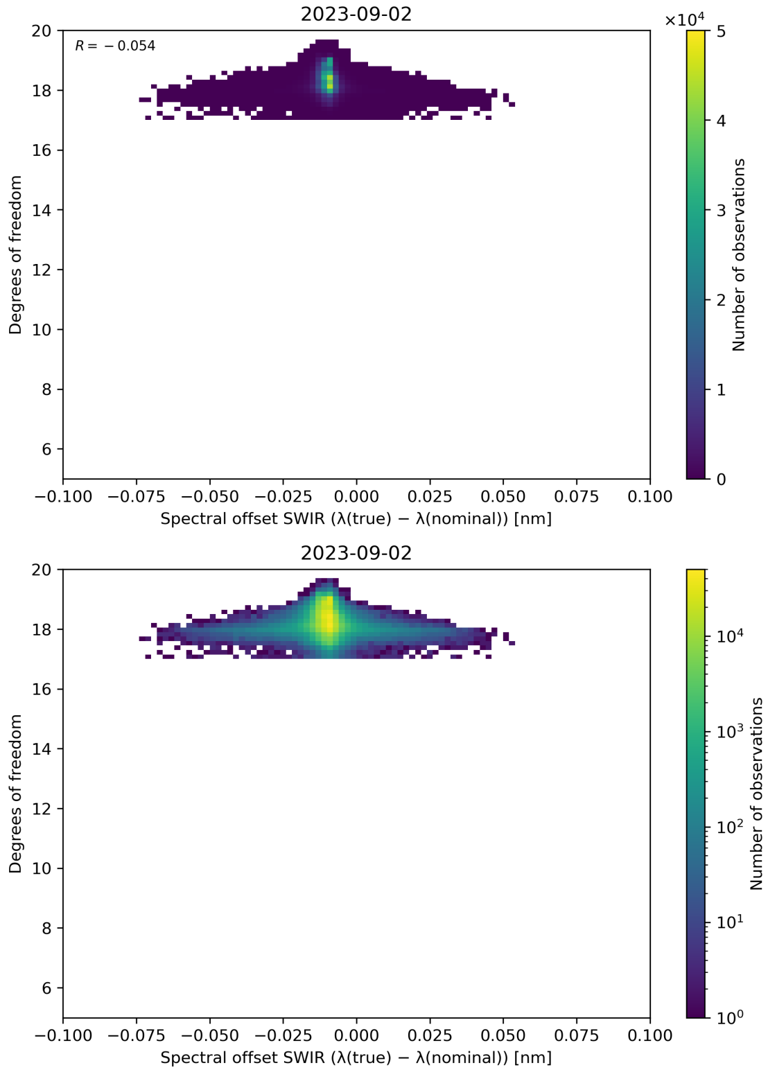
Figure 119: Scatter density plot of “Spectral offset SWIR ( \lambda(\text{true}) - \lambda(\text{nominal}) )” against “Degrees of freedom” for 2023-09-01 to 2023-09-03.
