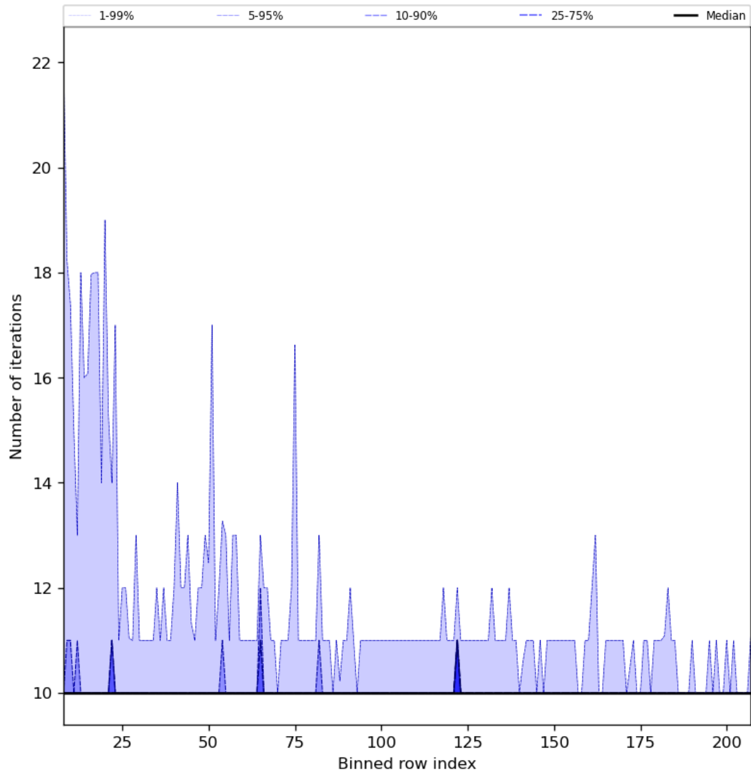
Figure 42: Along track statistics of “Number of iterations” for 2023-09-01 to 2023-09-03
