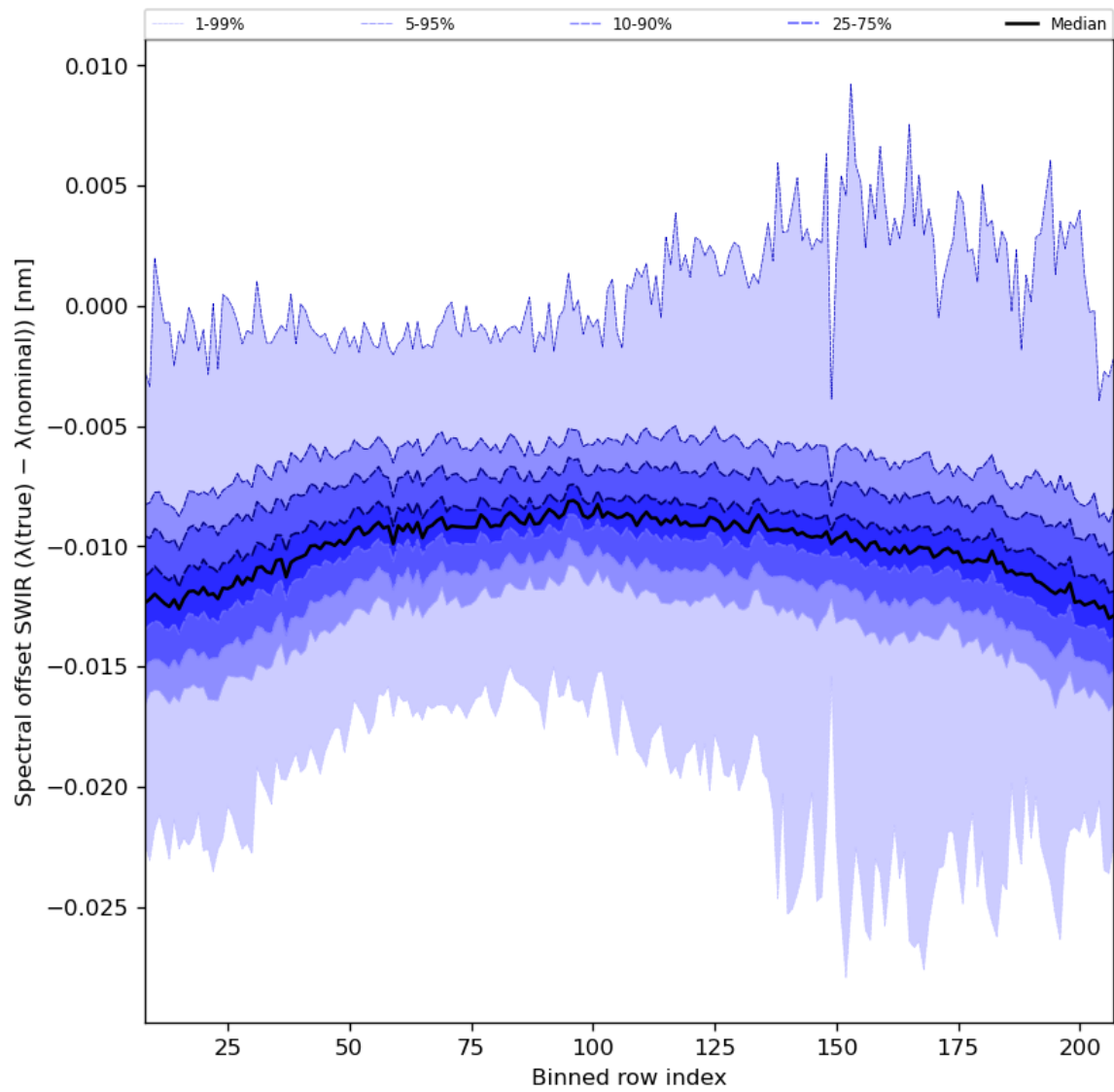
Figure 38: Along track statistics of “Spectral offset SWIR ( \lambda(\text{true}) - \lambda(\text{nominal}) )” for 2023-09-01 to 2023-09-03
