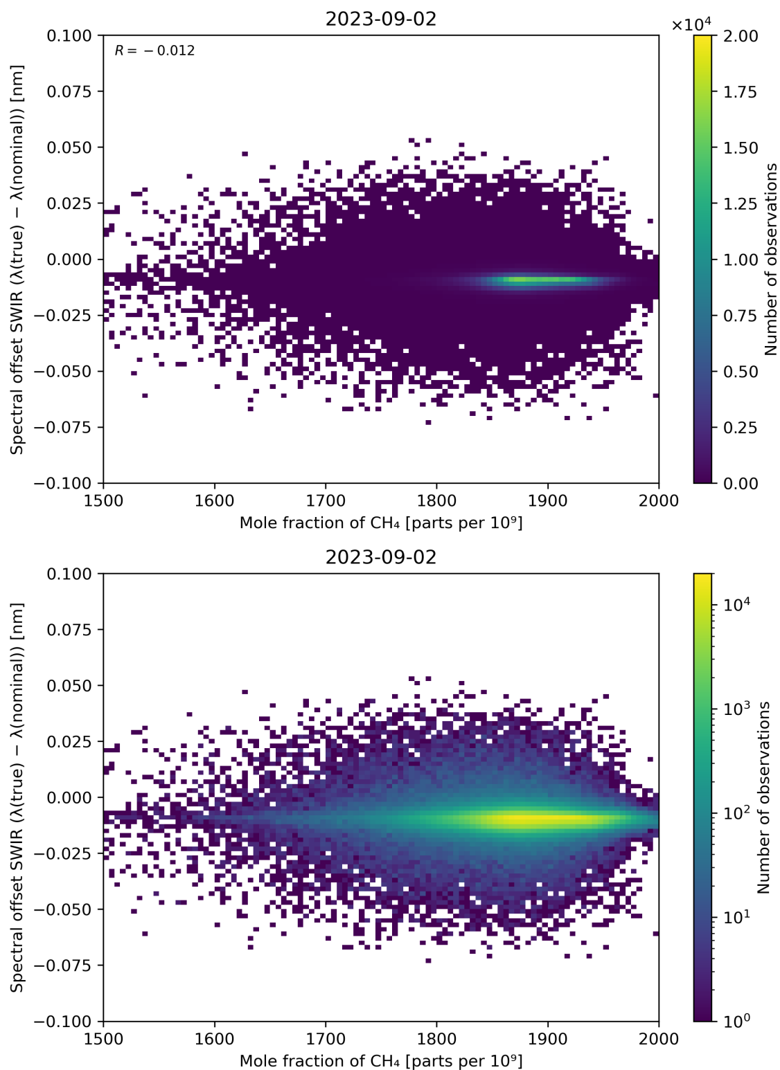
Figure 86: Scatter density plot of “Mole fraction of CH 4 ” against “Spectral offset SWIR ( \lambda(\text{true}) - \lambda(\text{nominal}) )” for 2023-09-01 to 2023-09-03.
