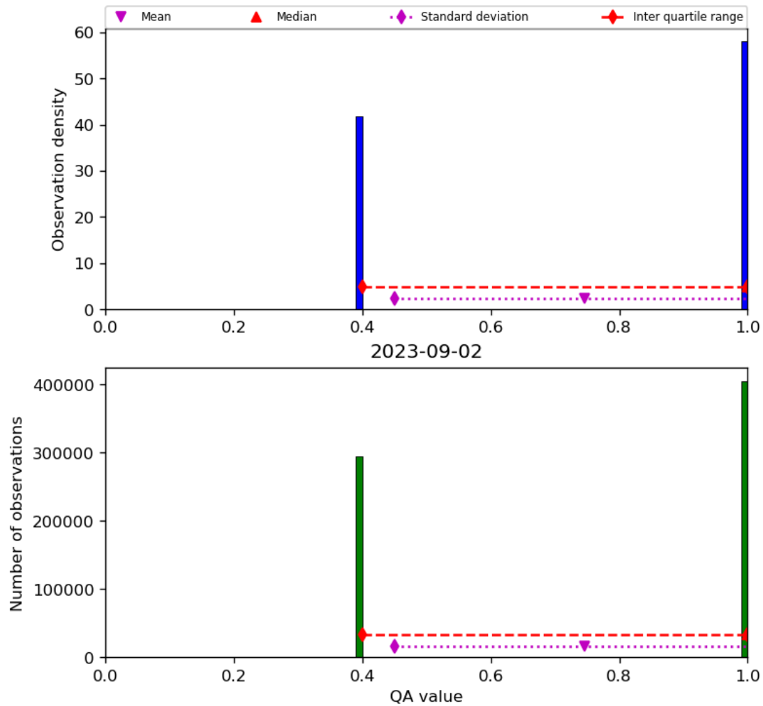
Figure 22: Histogram of “QA value” for 2023-09-01 to 2023-09-03
