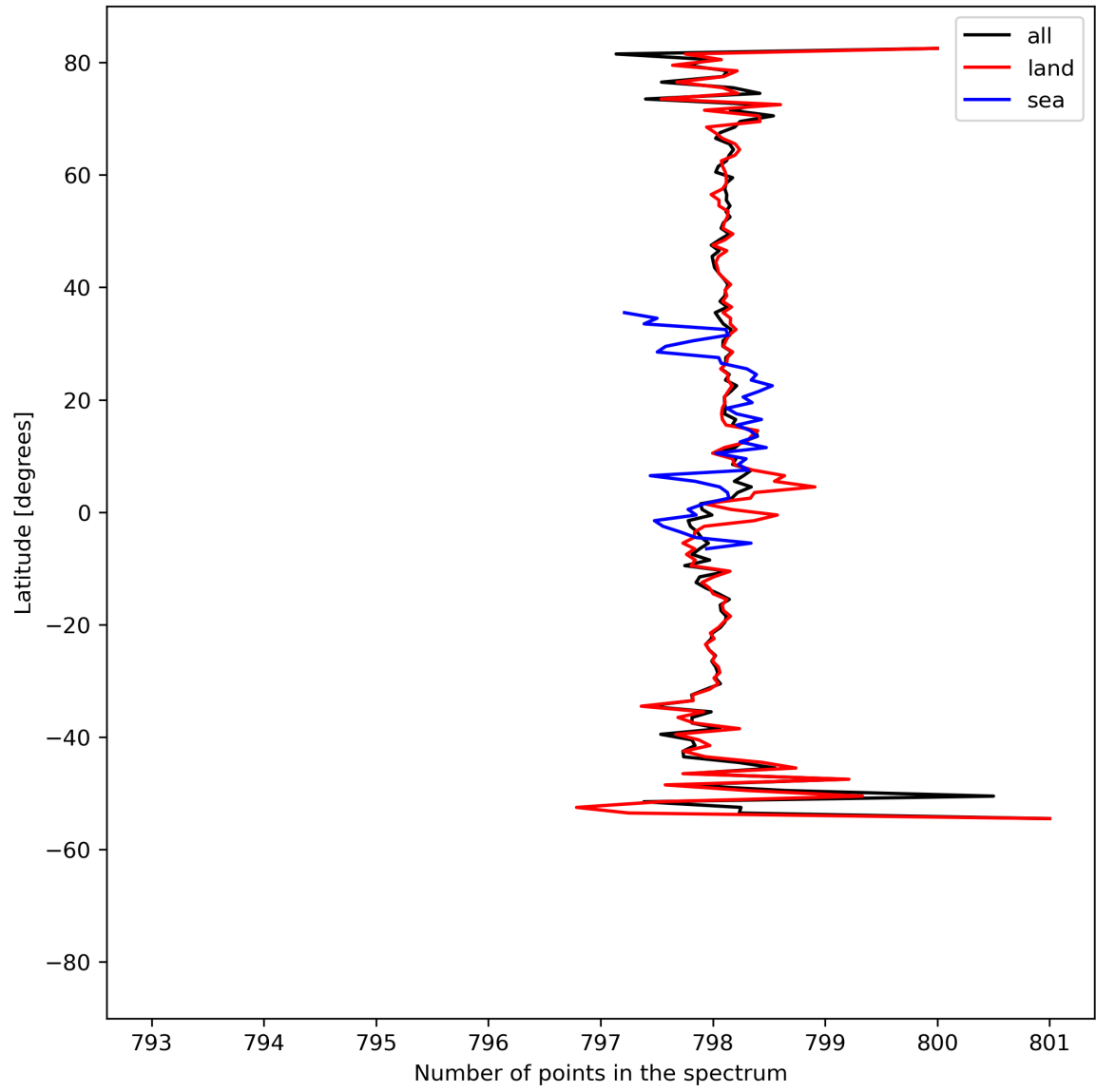
Figure 15: Zonal average of “Number of points in the spectrum” for 2023-09-01 to 2023-09-03.
