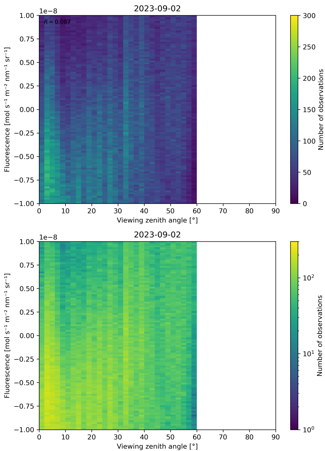
Figure 108: Scatter density plot of “Viewing zenith angle” against “Fluorescence” for 2023-09-01 to 2023-09-03.
