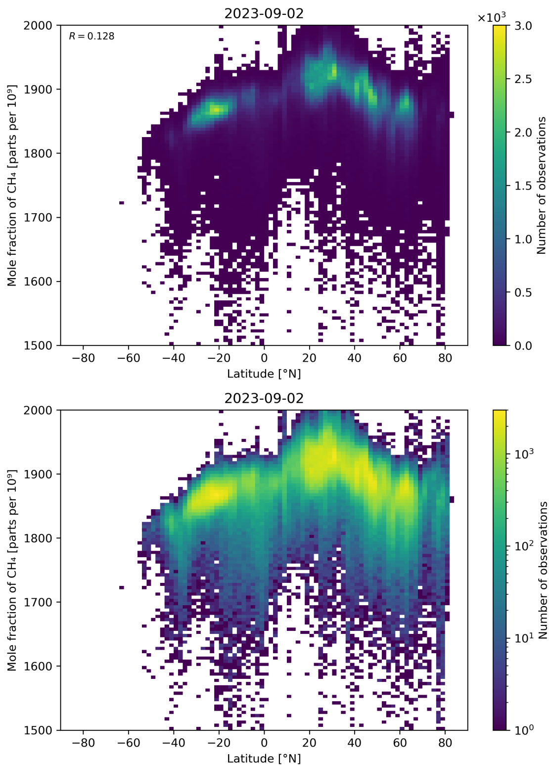
Figure 57: Scatter density plot of “Latitude” against “Mole fraction of \text{CH}_4 ” for 2023-09-01 to 2023-09-03.
