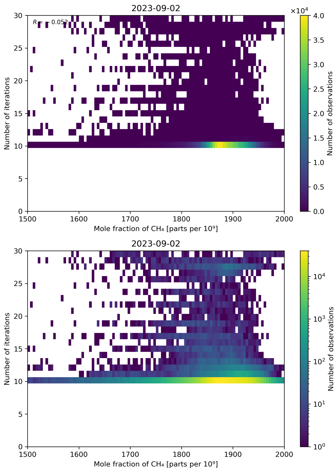
Figure 76: Scatter density plot of “Mole fraction of CH 4 ” against “Number of iterations” for 2023-09-01 to 2023-09-03.
