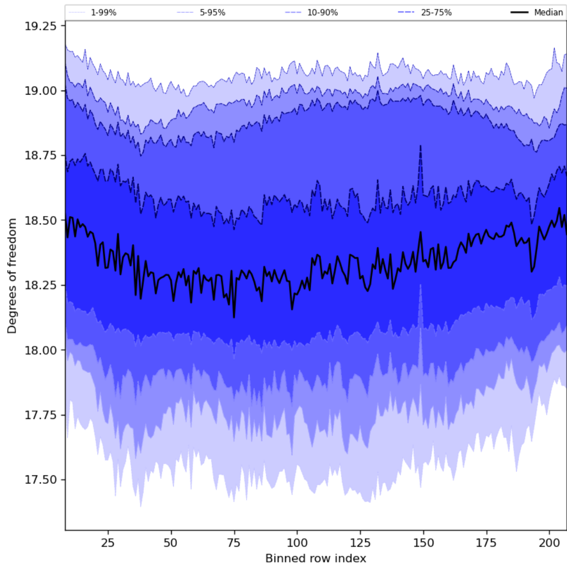
Figure 41: Along track statistics of “Degrees of freedom” for 2023-09-01 to 2023-09-03
