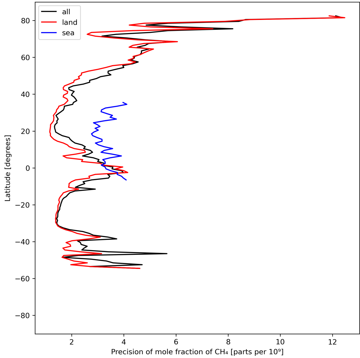
Figure 13: Zonal average of “Precision of mole fraction of CH 4 ” for 2023-09-01 to 2023-09-03.
