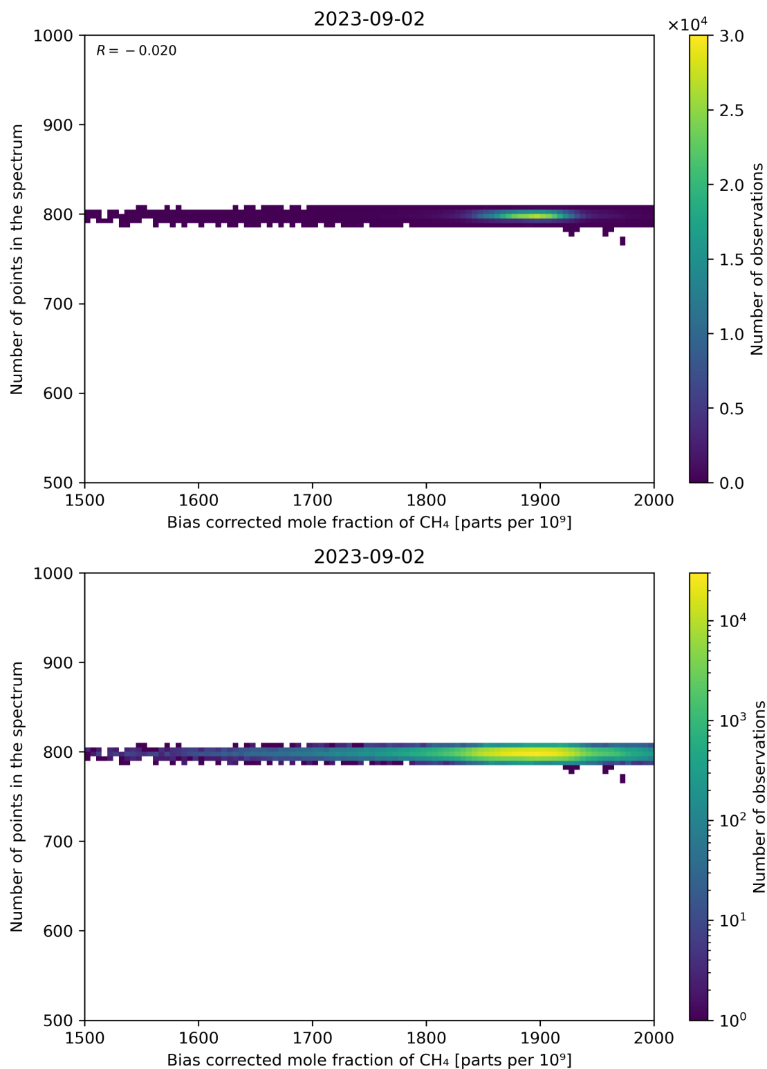
Figure 68: Scatter density plot of “Bias corrected mole fraction of CH 4 ” against “Number of points in the spectrum” for 2023-09-01 to 2023-09-03.
