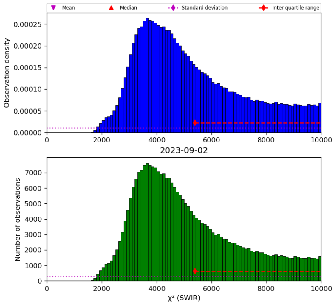
Figure 28: Histogram of “ \chi^2 (SWIR)” for 2023-09-01 to 2023-09-03
