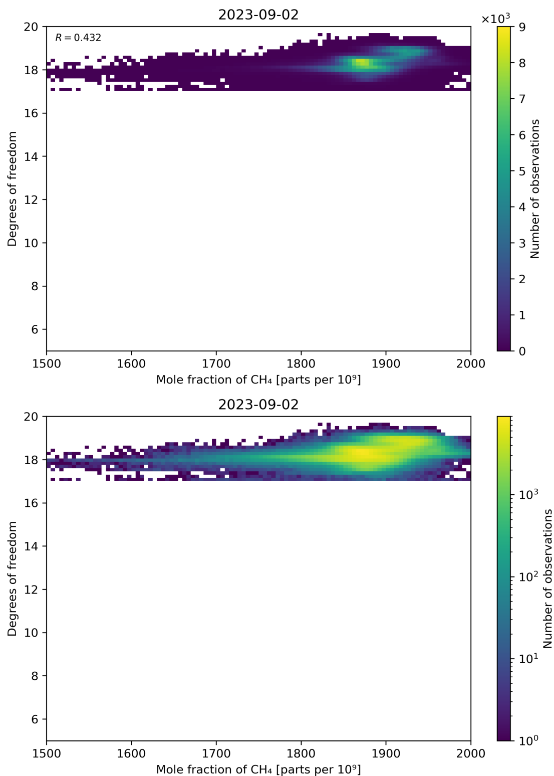
Figure 72: Scatter density plot of “Mole fraction of CH 4 ” against “Degrees of freedom” for 2023-09-01 to 2023-09-03.
