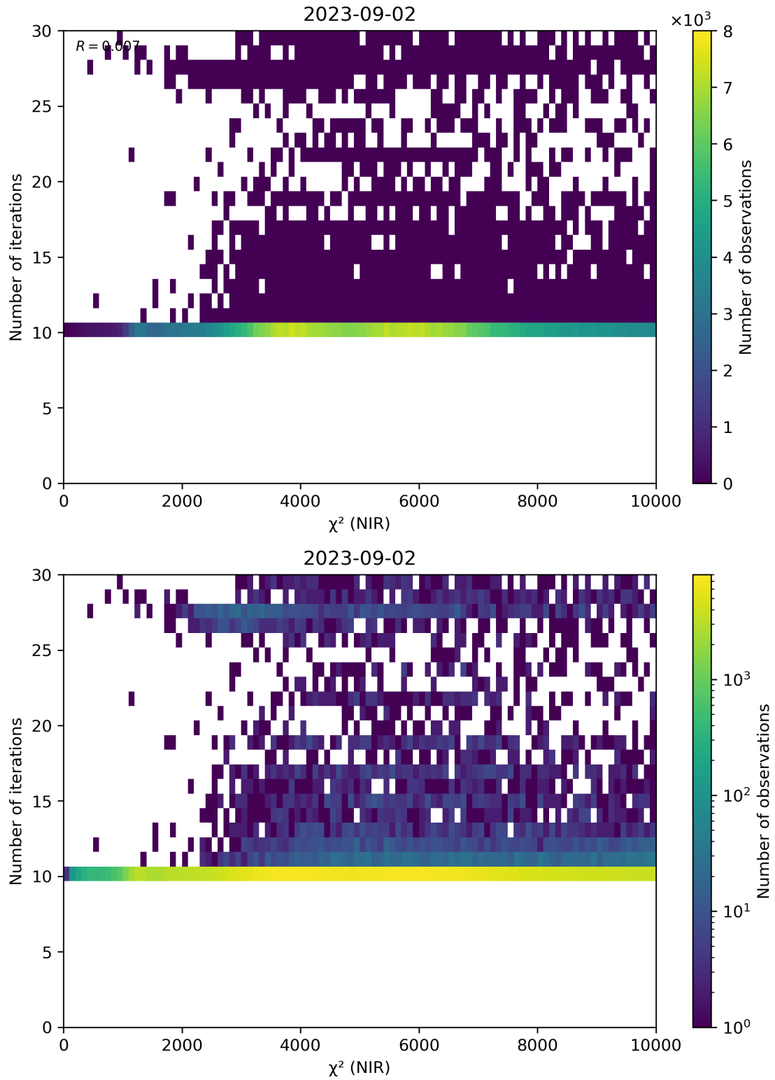
Figure 46: Scatter density plot of “ \chi^2 (NIR)” against “Number of iterations” for 2023-09-01 to 2023-09-03.
