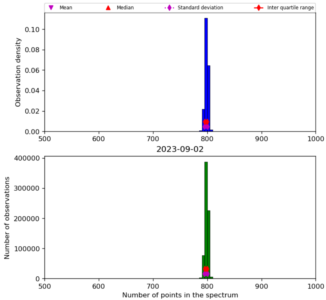
Figure 26: Histogram of “Number of points in the spectrum” for 2023-09-01 to 2023-09-03
