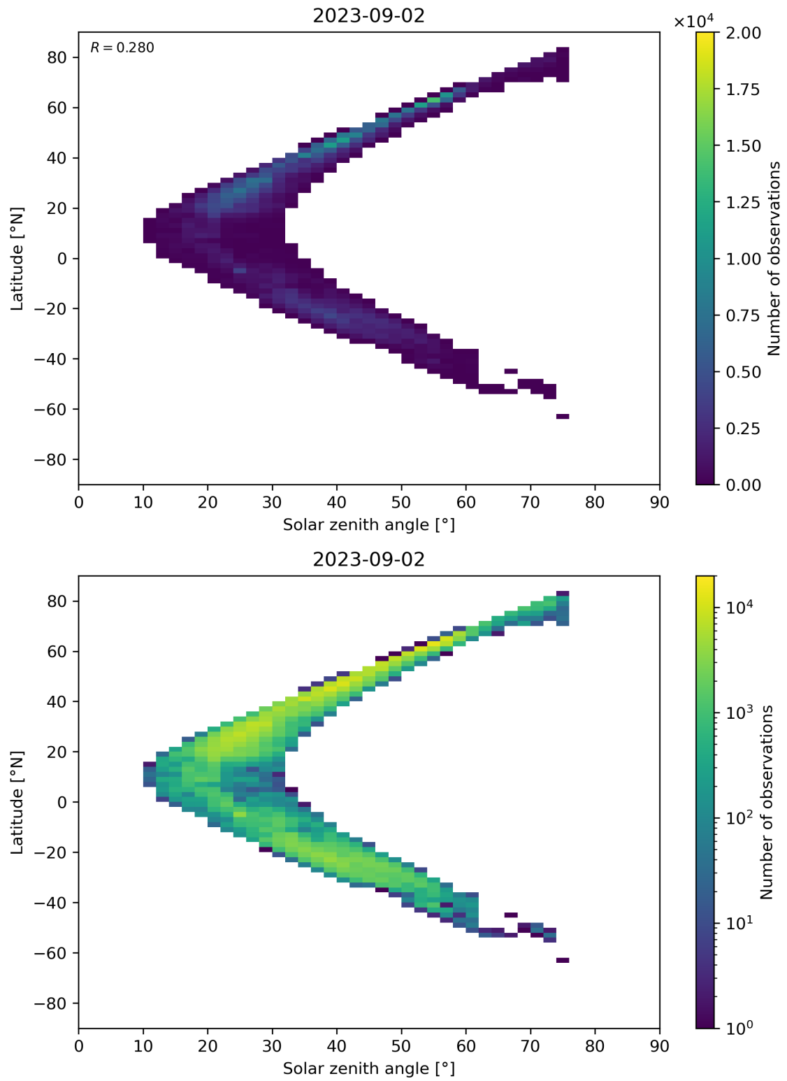
Figure 98: Scatter density plot of “Solar zenith angle” against “Latitude” for 2023-09-01 to 2023-09-03.
