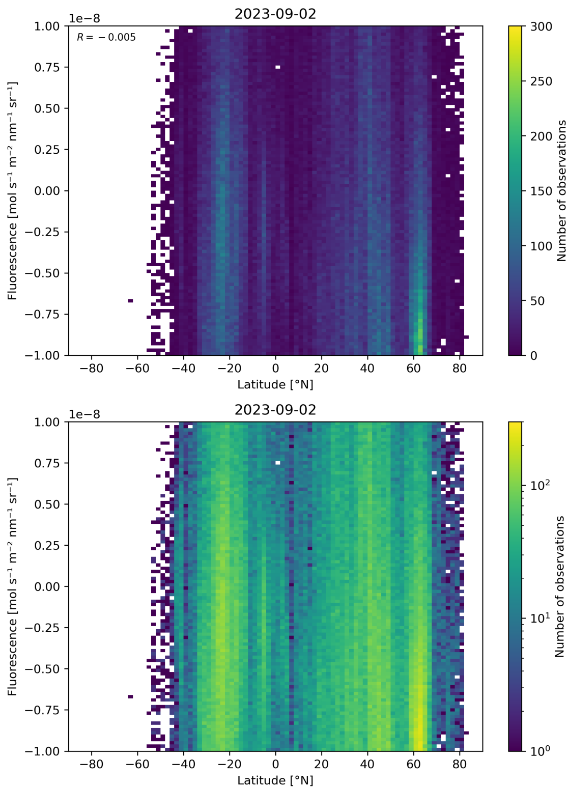
Figure 56: Scatter density plot of “Latitude” against “Fluorescence” for 2023-09-01 to 2023-09-03.
