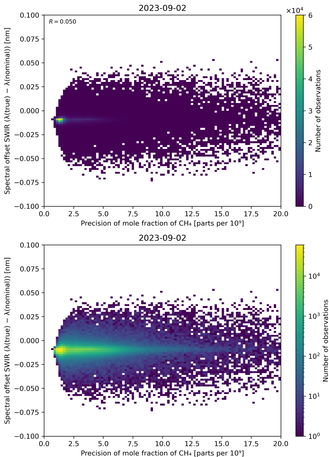
Figure 85: Scatter density plot of “Precision of mole fraction of CH 4 ” against “Spectral offset SWIR ( \lambda(\text{true}) - \lambda(\text{nominal}) )” for 2023-09-01 to 2023-09-03.
