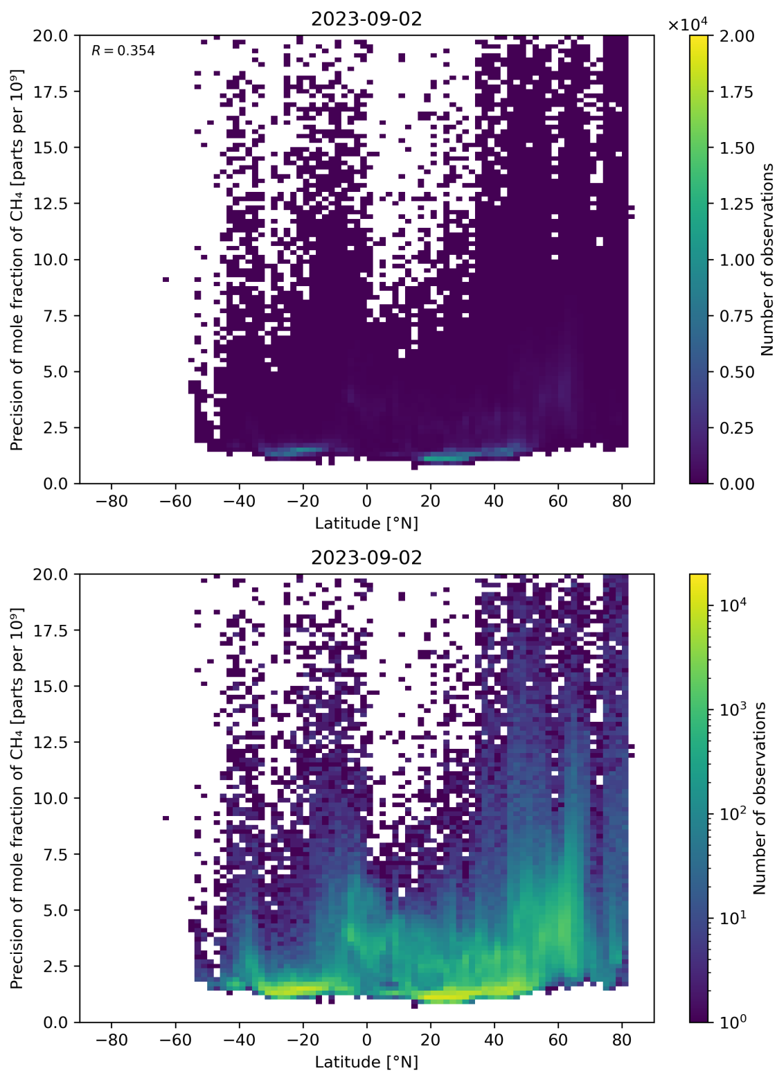
Figure 59: Scatter density plot of “Latitude” against “Precision of mole fraction of \text{CH}_4 ” for 2023-09-01 to 2023-09-03.
