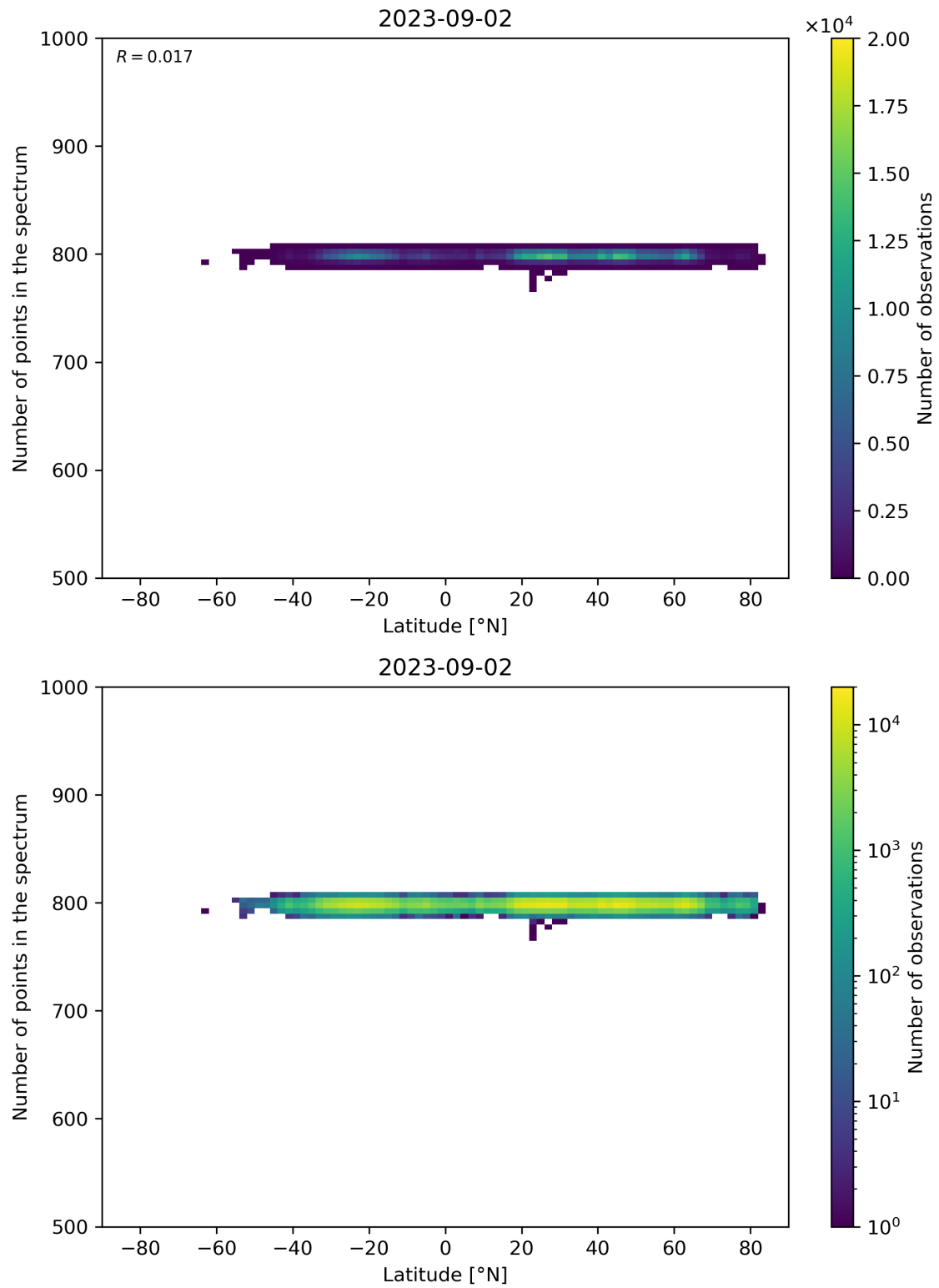
Figure 61: Scatter density plot of “Latitude” against “Number of points in the spectrum” for 2023-09-01 to 2023-09-03.
