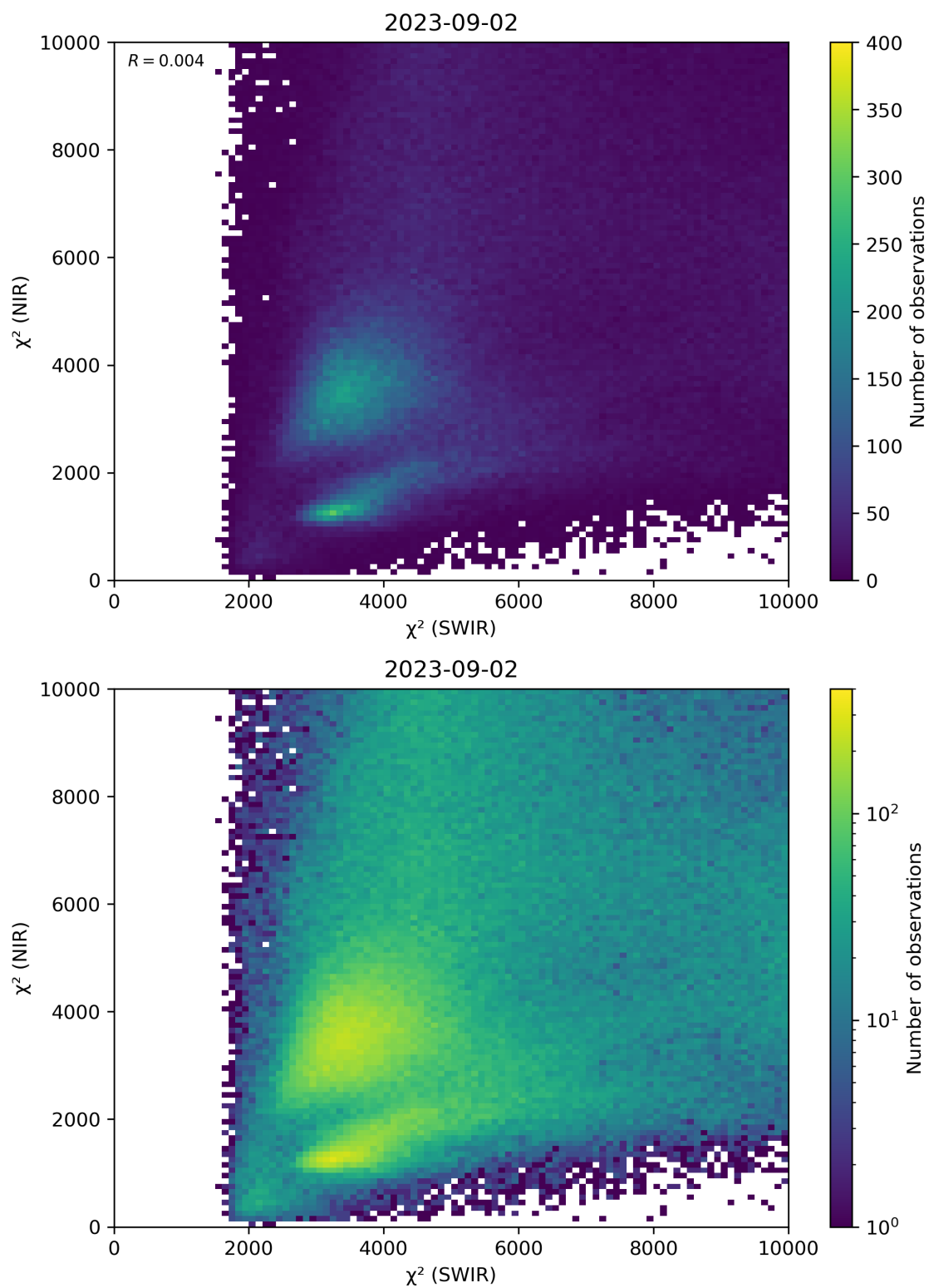
Figure 47: Scatter density plot of “ \chi^2 (SWIR)” against “ \chi^2 (NIR)” for 2023-09-01 to 2023-09-03.
