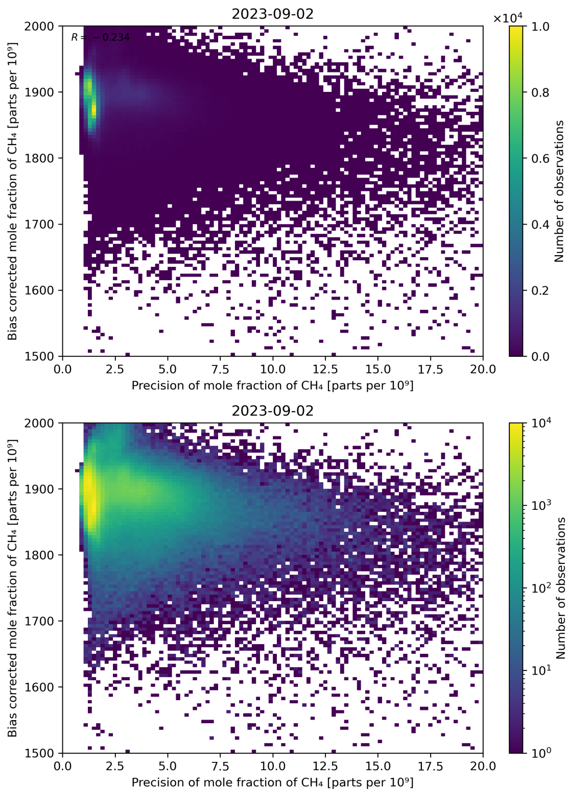
Figure 82: Scatter density plot of “Precision of mole fraction of CH 4 ” against “Bias corrected mole fraction of CH 4 ” for 2023-09-01 to 2023-09-03.
