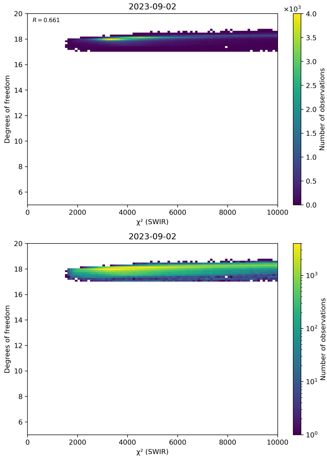
Figure 48: Scatter density plot of “ \chi^2 (SWIR)” against “Degrees of freedom” for 2023-09-01 to 2023-09-03.
