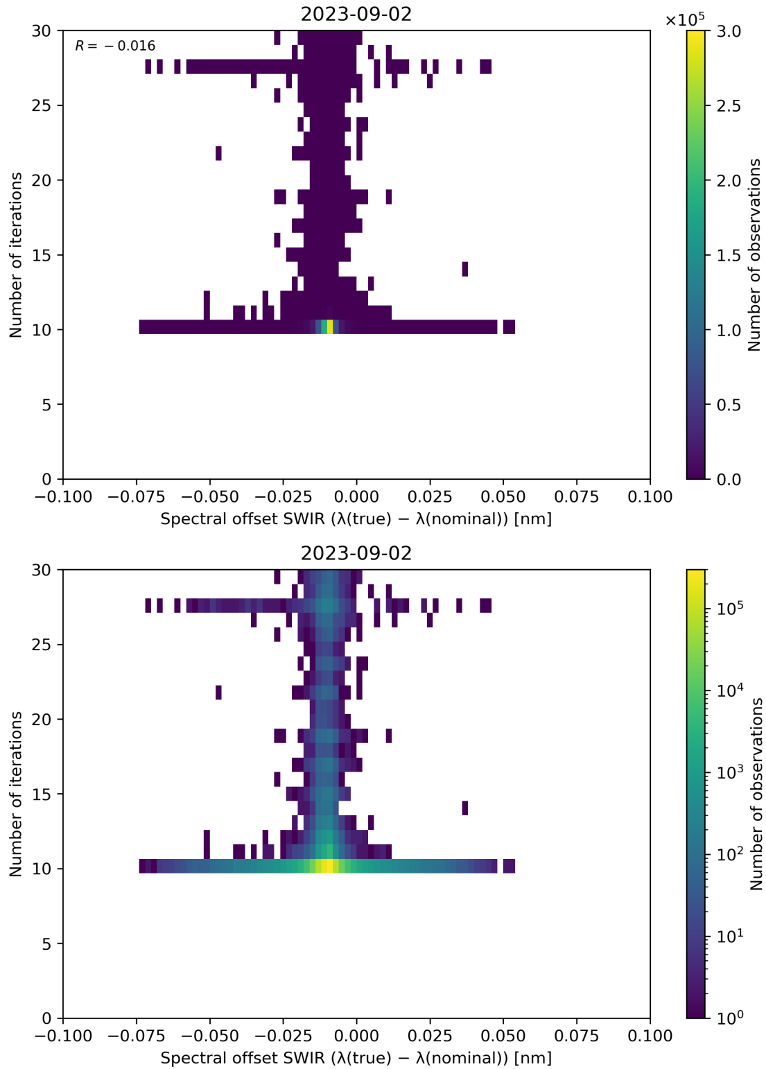
Figure 121: Scatter density plot of “Spectral offset SWIR ( \lambda(\text{true}) - \lambda(\text{nominal}) )” against “Number of iterations” for 2023-09-01 to 2023-09-03.
