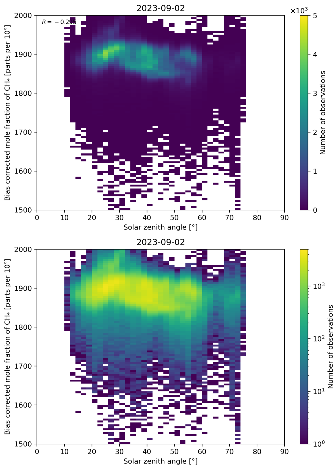
Figure 100: Scatter density plot of “Solar zenith angle” against “Bias corrected mole fraction of \text{CH}_4 ” for 2023-09-01 to 2023-09-03.
