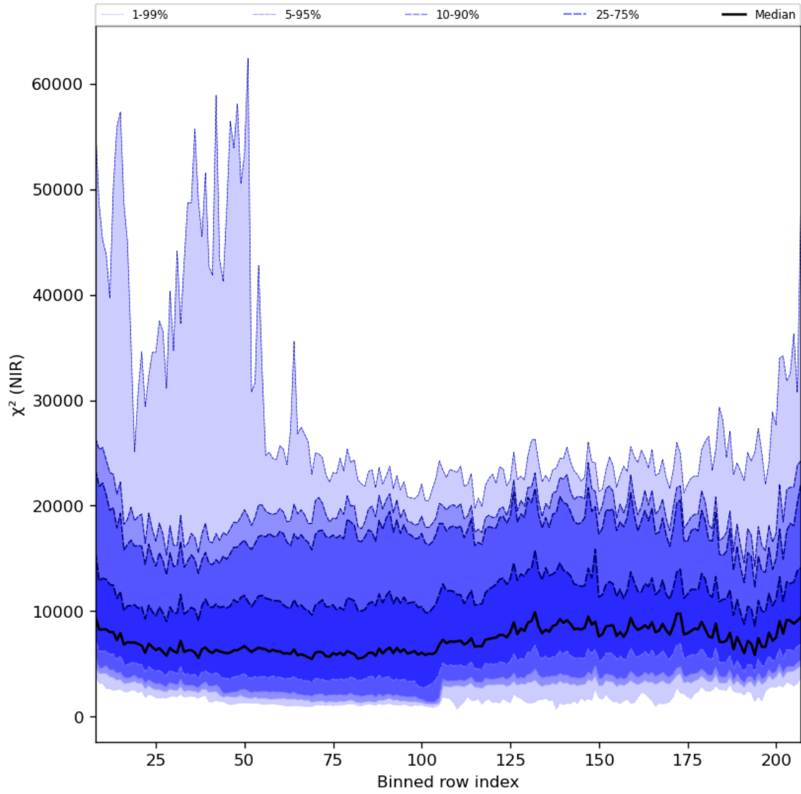
Figure 40: Along track statistics of " \chi^2 (NIR)" for 2023-09-01 to 2023-09-03
