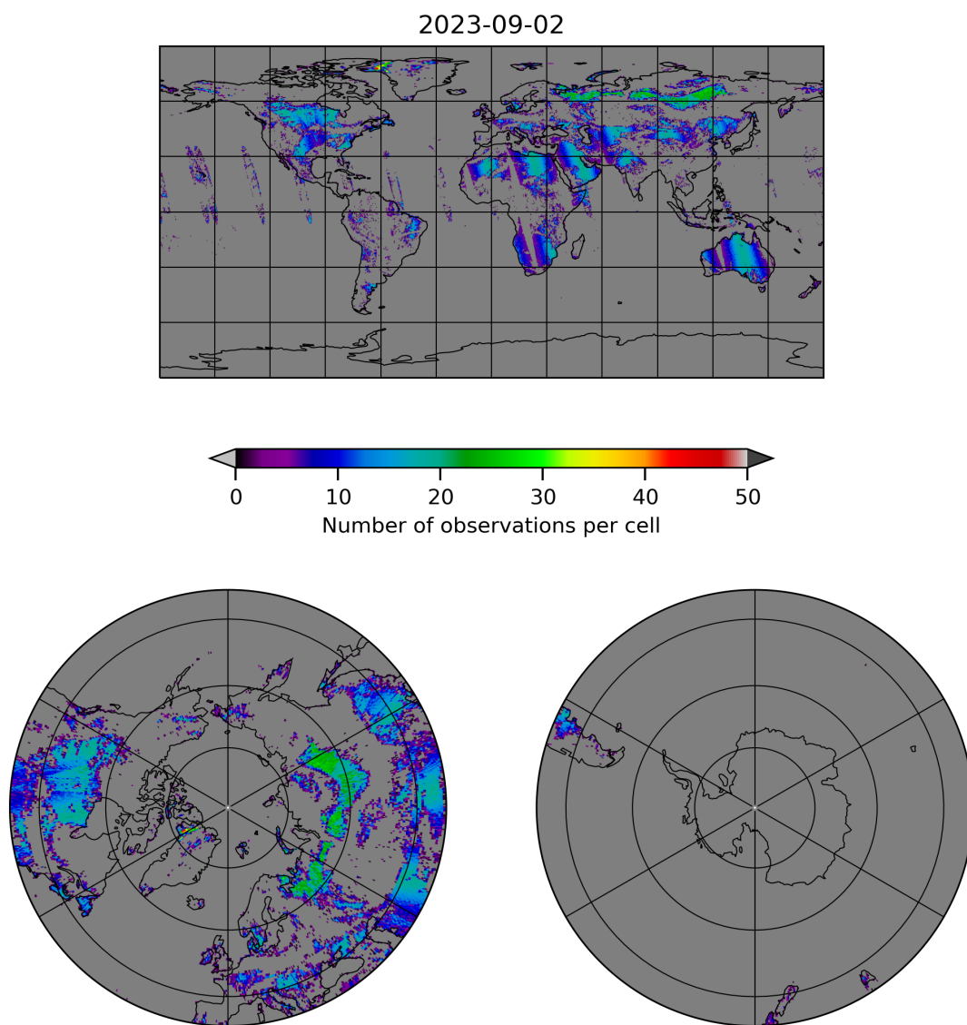
Figure 10: Map of the number of observations for 2023-09-01 to 2023-09-03
