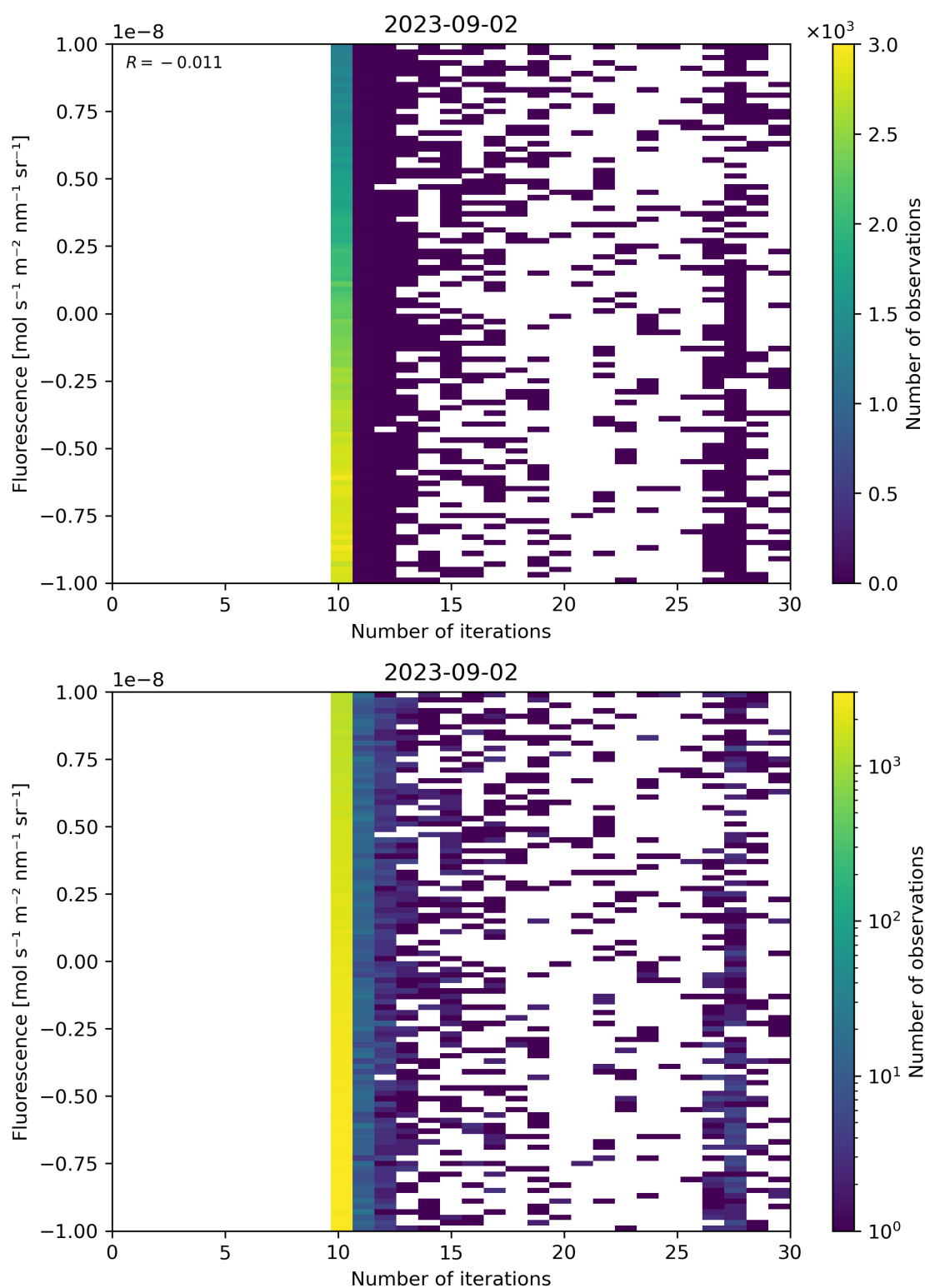
Figure 87: Scatter density plot of “Number of iterations” against “Fluorescence” for 2023-09-01 to 2023-09-03.
