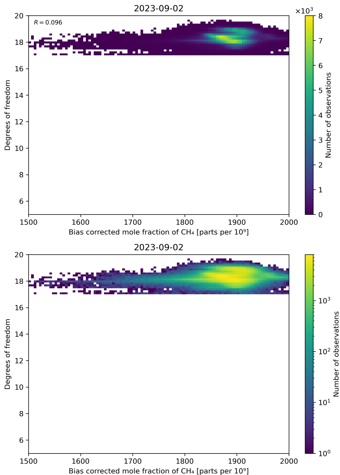
Figure 65: Scatter density plot of “Bias corrected mole fraction of CH 4 ” against “Degrees of freedom” for 2023-09-01 to 2023-09-03.
