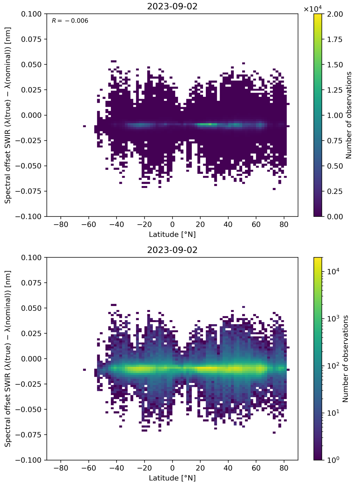
Figure 62: Scatter density plot of “Latitude” against “Spectral offset SWIR ( \lambda(\text{true}) - \lambda(\text{nominal}) )” for 2023-09-01 to 2023-09-03.
