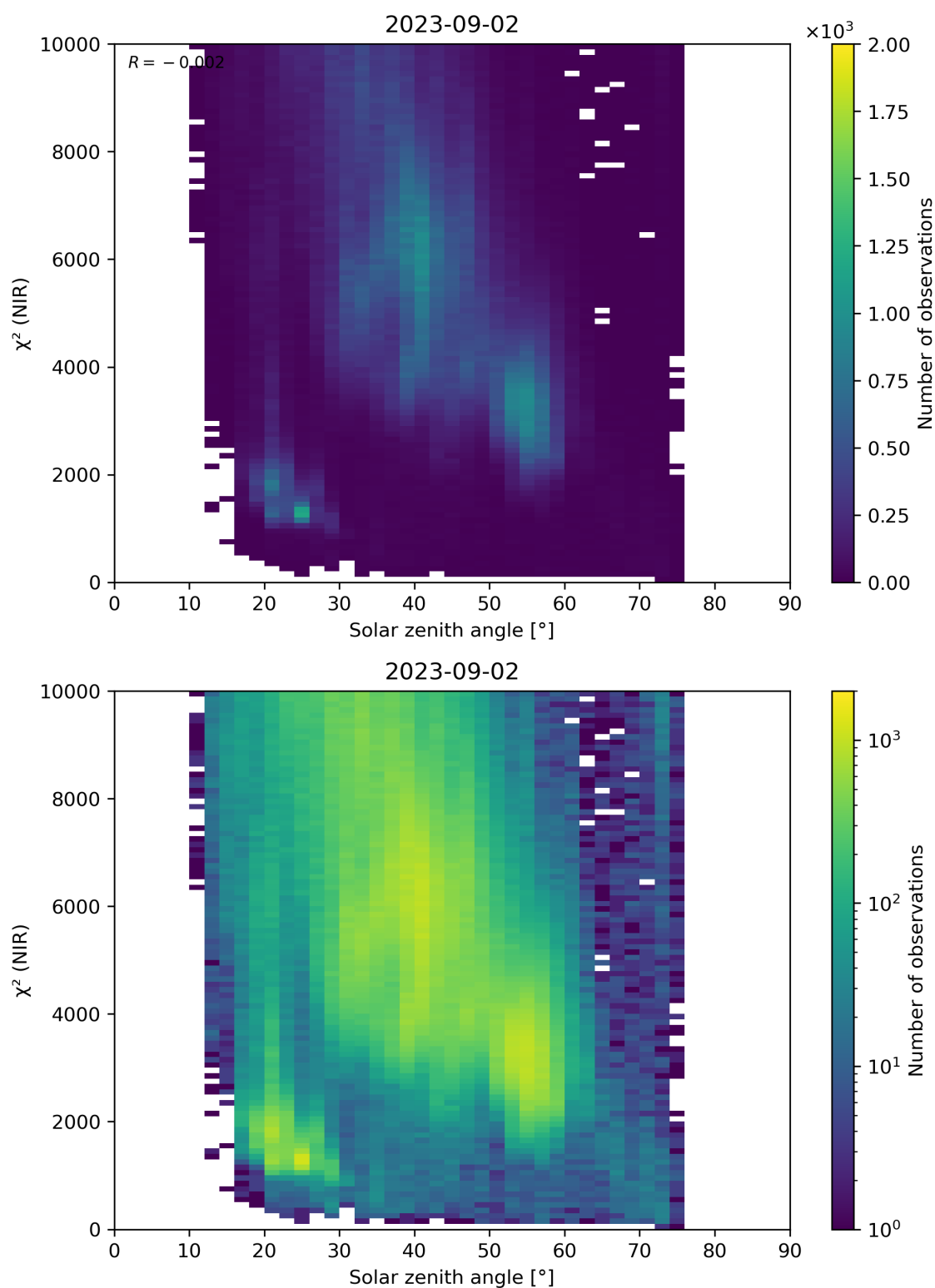
Figure 94: Scatter density plot of “Solar zenith angle” against “ \chi^2 (NIR)” for 2023-09-01 to 2023-09-03.
