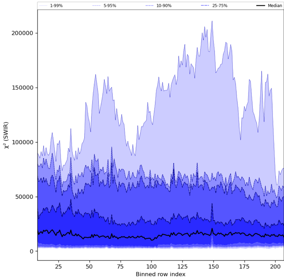
Figure 39: Along track statistics of “ \chi^2 (SWIR)” for 2023-09-01 to 2023-09-03
