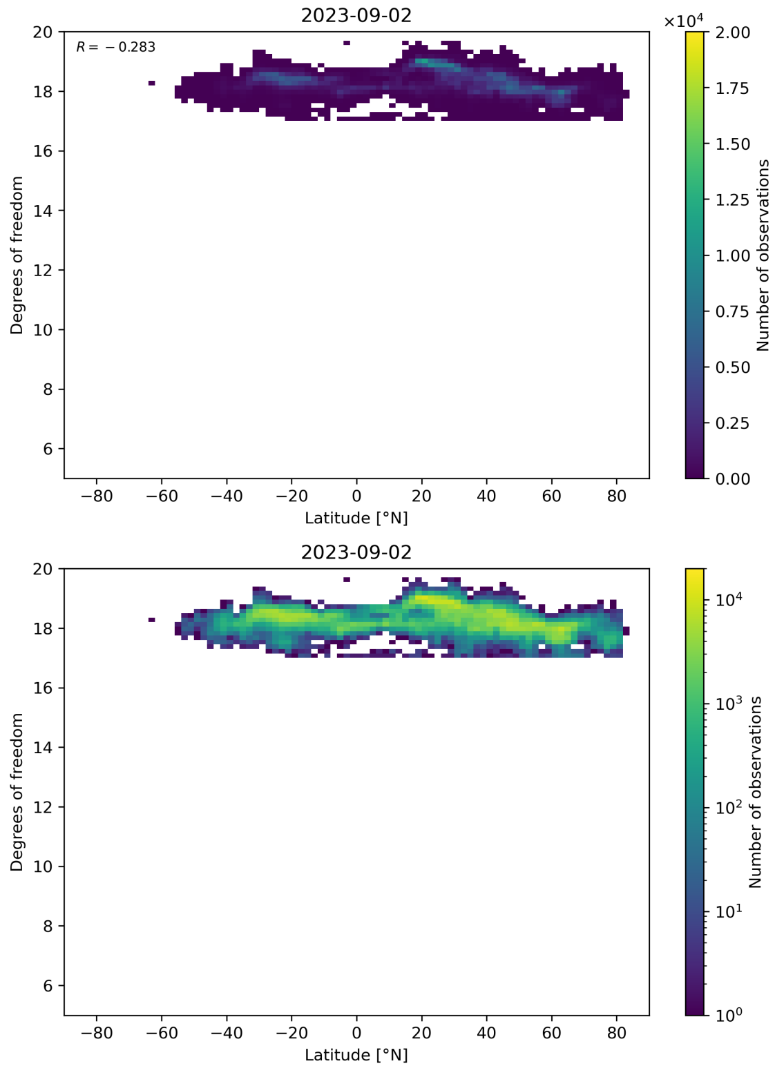
Figure 55: Scatter density plot of “Latitude” against “Degrees of freedom” for 2023-09-01 to 2023-09-03.
