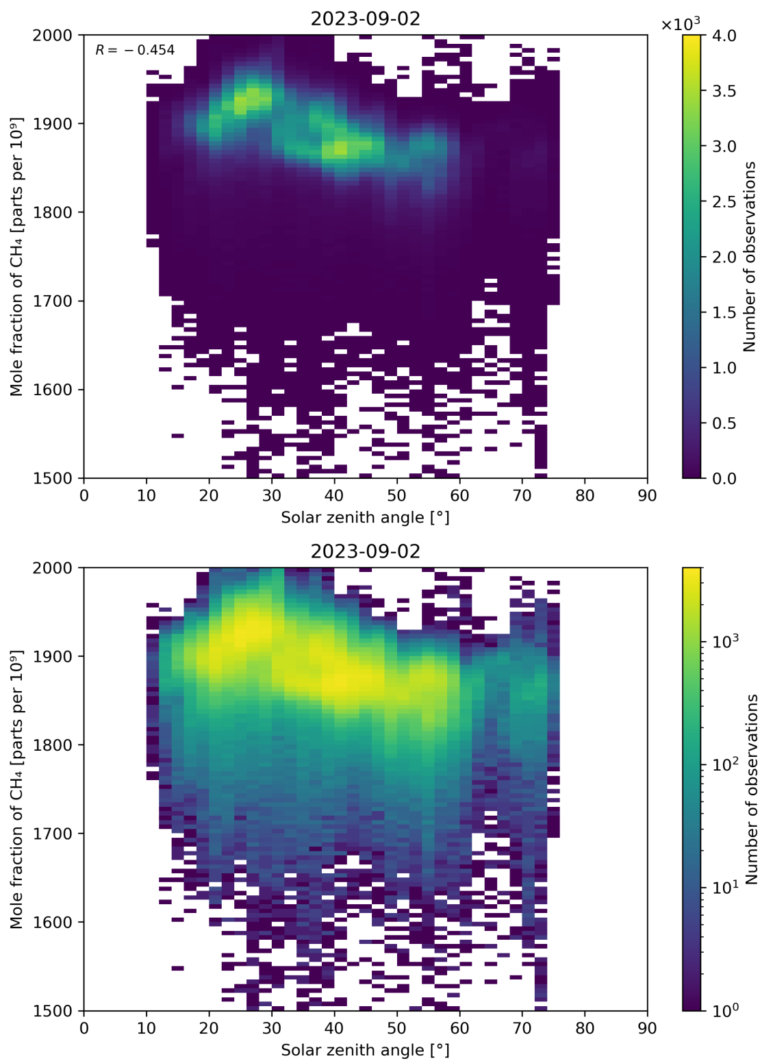
Figure 99: Scatter density plot of “Solar zenith angle” against “Mole fraction of CH 4 ” for 2023-09-01 to 2023-09-03.
