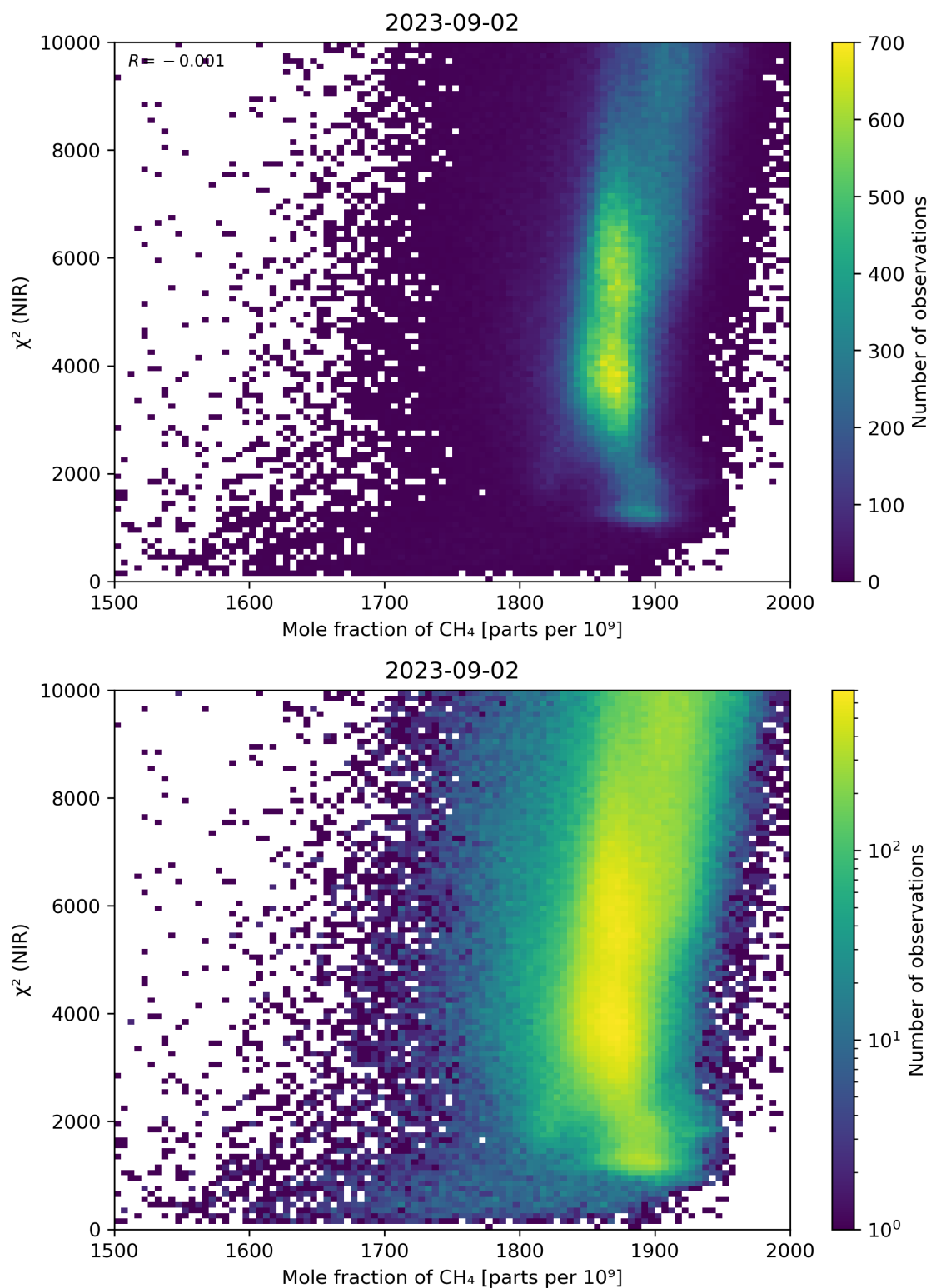
Figure 70: Scatter density plot of “Mole fraction of CH 4 ” against “ \chi^2 (NIR)” for 2023-09-01 to 2023-09-03.
