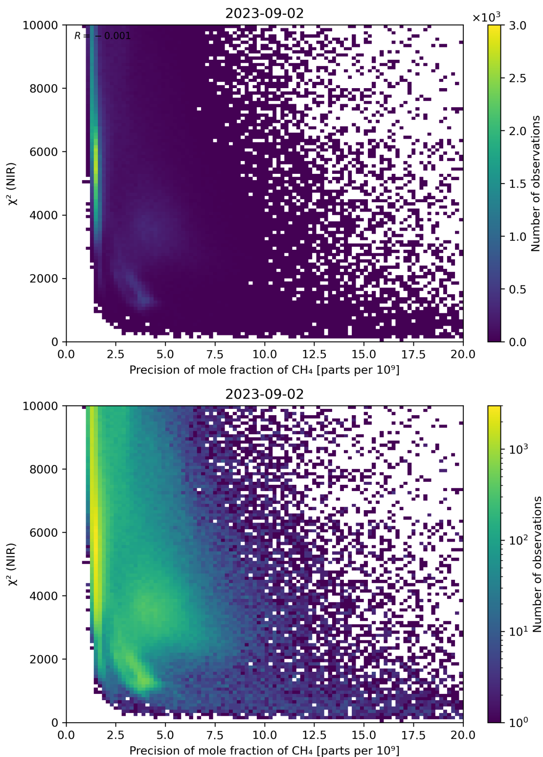
Figure 78: Scatter density plot of “Precision of mole fraction of CH 4 ” against “ \chi^2 (NIR)” for 2023-09-01 to 2023-09-03.
