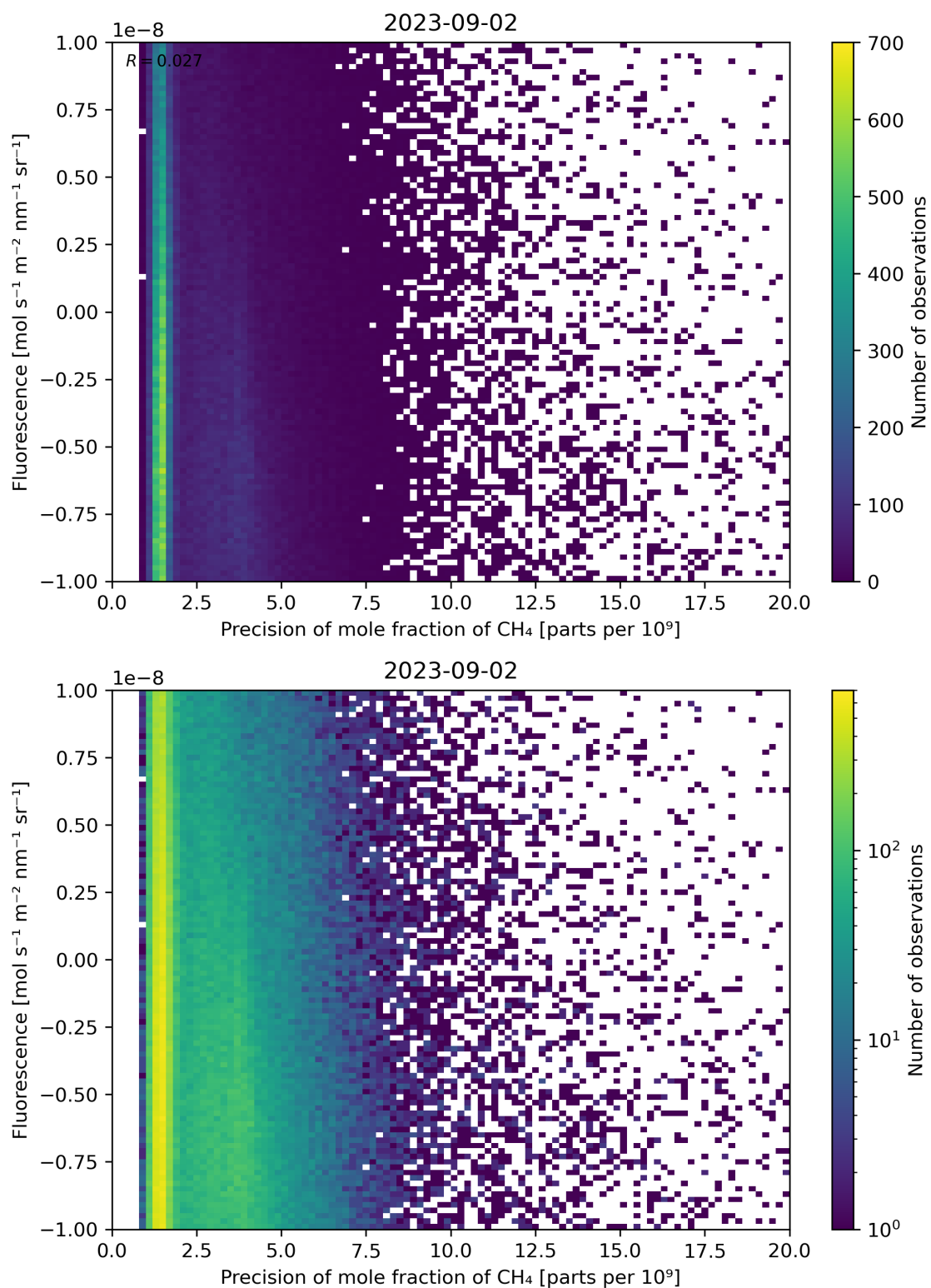
Figure 81: Scatter density plot of “Precision of mole fraction of \text{CH}_4 ” against “Fluorescence” for 2023-09-01 to 2023-09-03.
