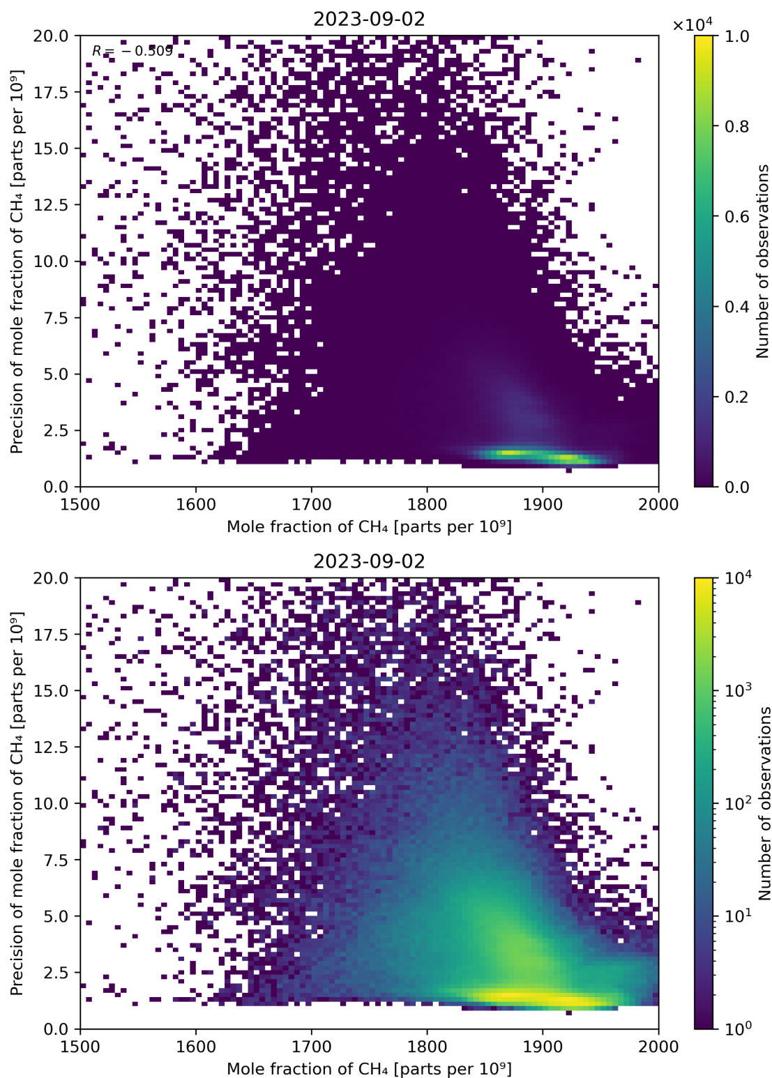
Figure 75: Scatter density plot of “Mole fraction of CH 4 ” against “Precision of mole fraction of CH 4 ” for 2023-09-01 to 2023-09-03.
