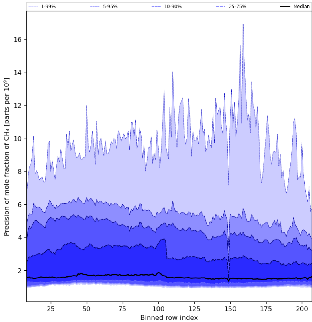
Figure 35: Along track statistics of “Precision of mole fraction of CH 4 ” for 2023-09-01 to 2023-09-03
