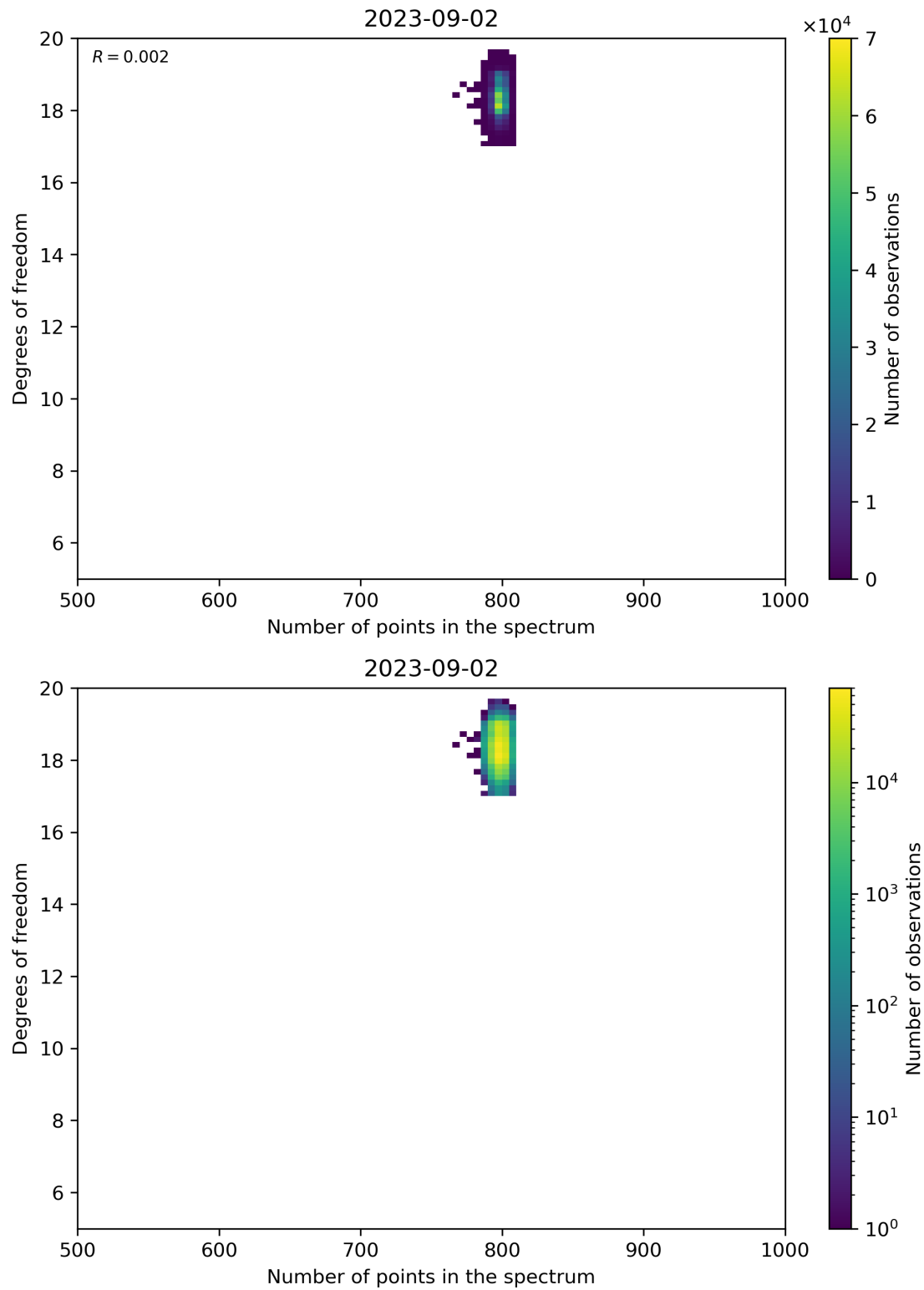
Figure 90: Scatter density plot of “Number of points in the spectrum” against “Degrees of freedom” for 2023-09-01 to 2023-09-03.
