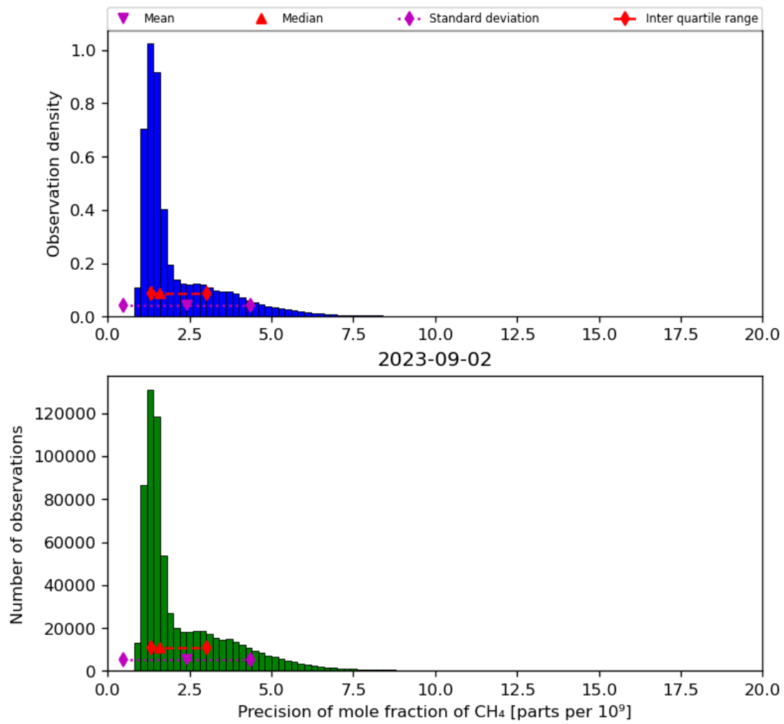
Figure 24: Histogram of “Precision of mole fraction of CH 4 ” for 2023-09-01 to 2023-09-03
