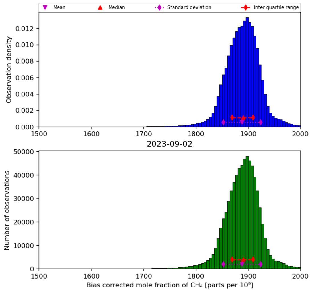
Figure 25: Histogram of “Bias corrected mole fraction of CH 4 ” for 2023-09-01 to 2023-09-03
