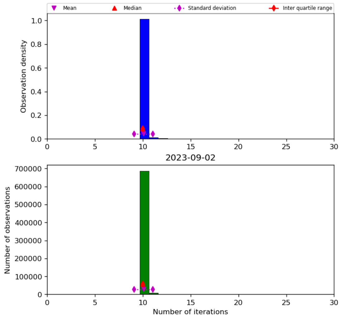
Figure 31: Histogram of “Number of iterations” for 2023-09-01 to 2023-09-03
