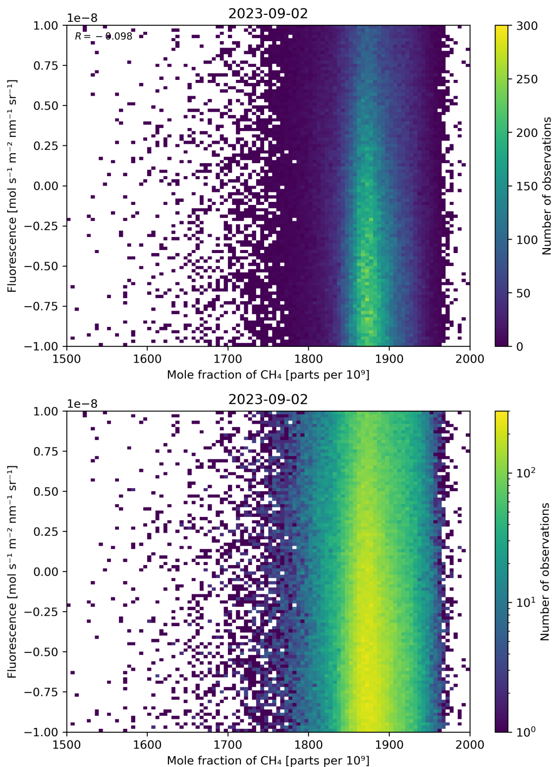
Figure 73: Scatter density plot of “Mole fraction of \text{CH}_4 ” against “Fluorescence” for 2023-09-01 to 2023-09-03.
