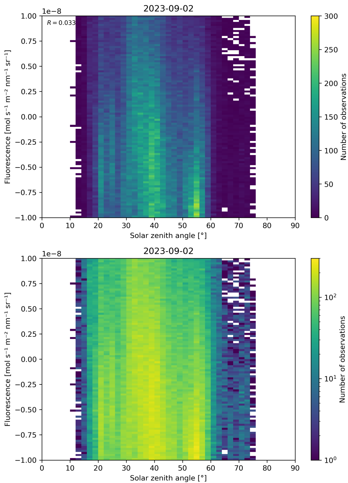
Figure 97: Scatter density plot of “Solar zenith angle” against “Fluorescence” for 2023-09-01 to 2023-09-03.
