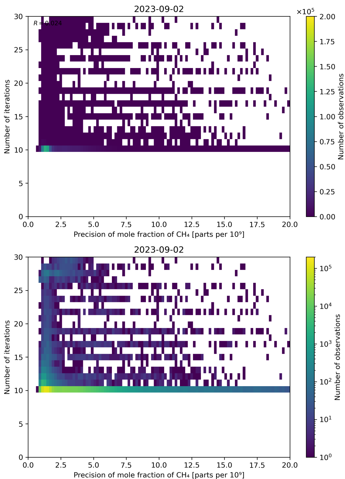
Figure 83: Scatter density plot of “Precision of mole fraction of CH 4 ” against “Number of iterations” for 2023-09-01 to 2023-09-03.
