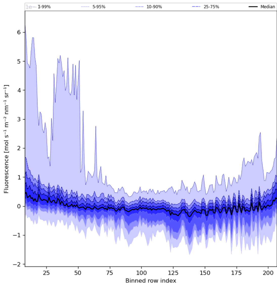
Figure 43: Along track statistics of “Fluorescence” for 2023-09-01 to 2023-09-03
