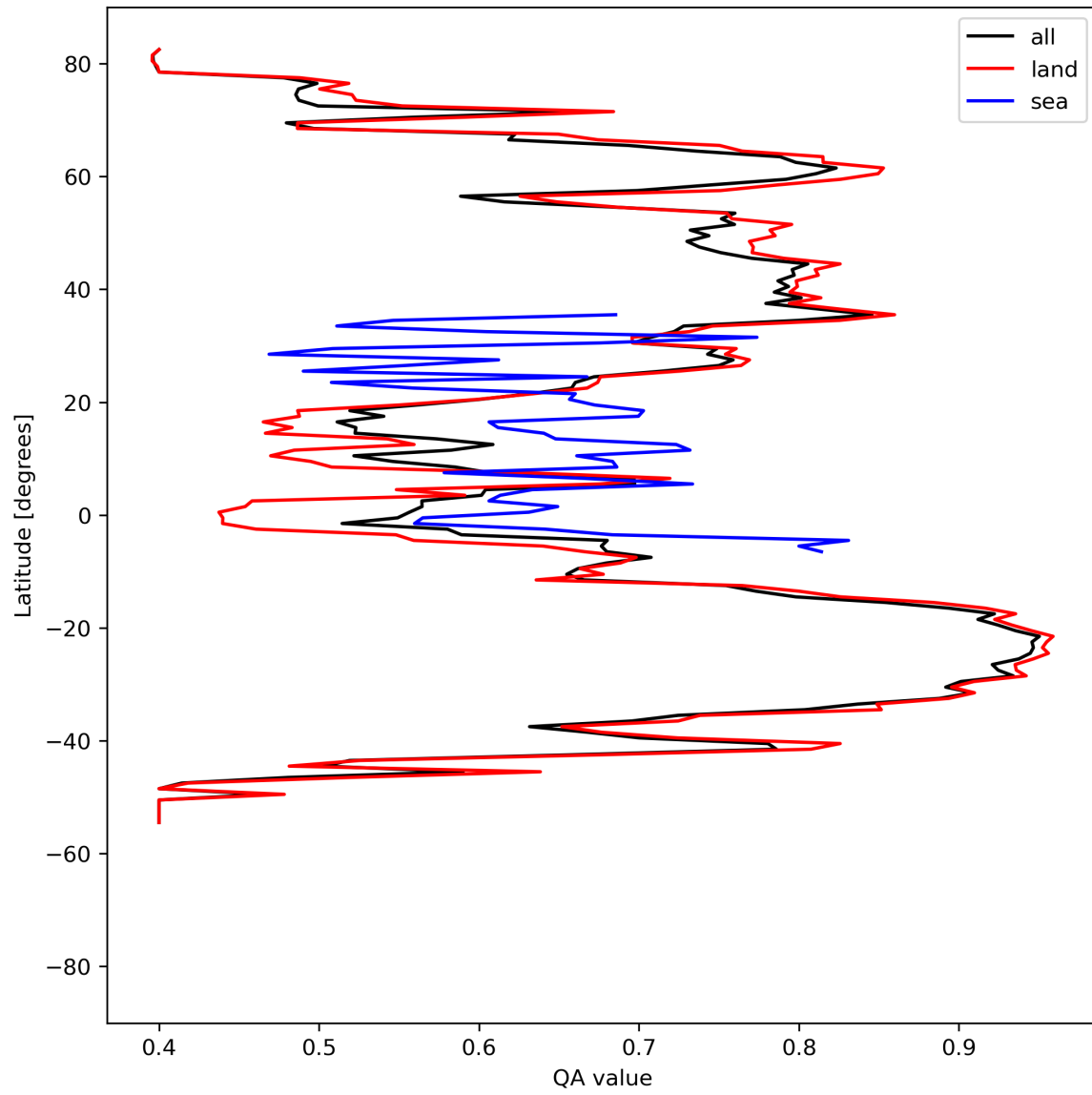
Figure 11: Zonal average of “QA value” for 2023-09-01 to 2023-09-03.
