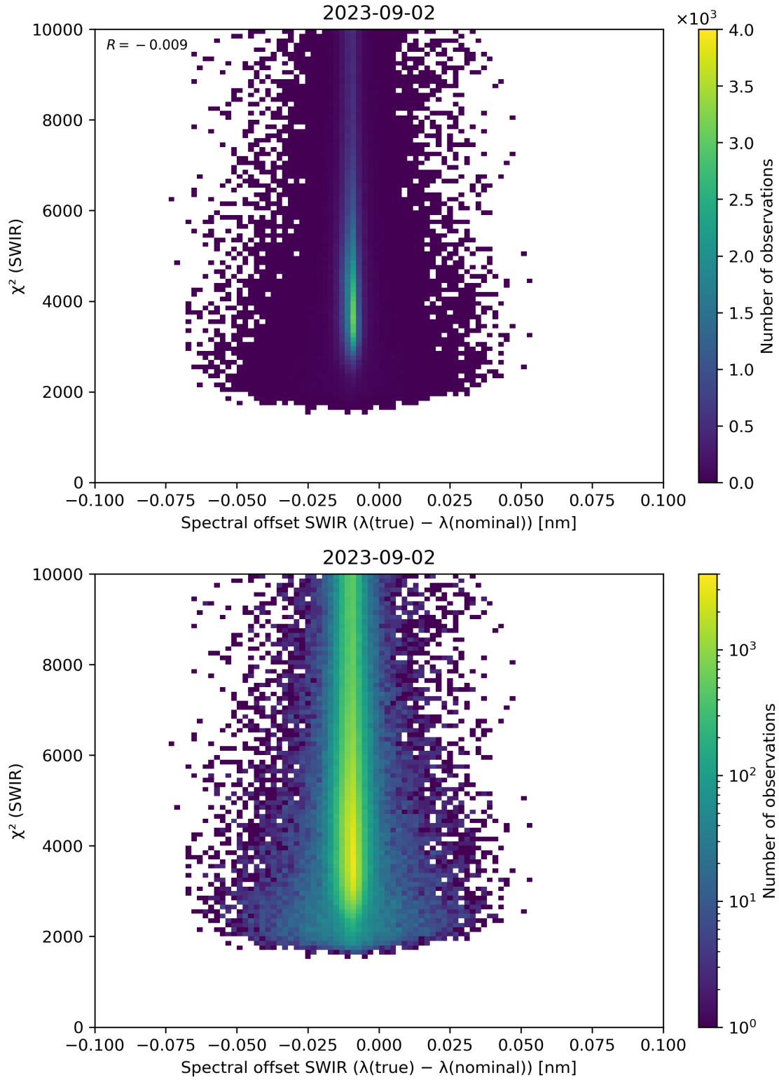
Figure 118: Scatter density plot of “Spectral offset SWIR ( \lambda(\text{true}) - \lambda(\text{nominal}) )” against “ \chi^2 (SWIR)” for 2023-09-01 to 2023-09-03.
