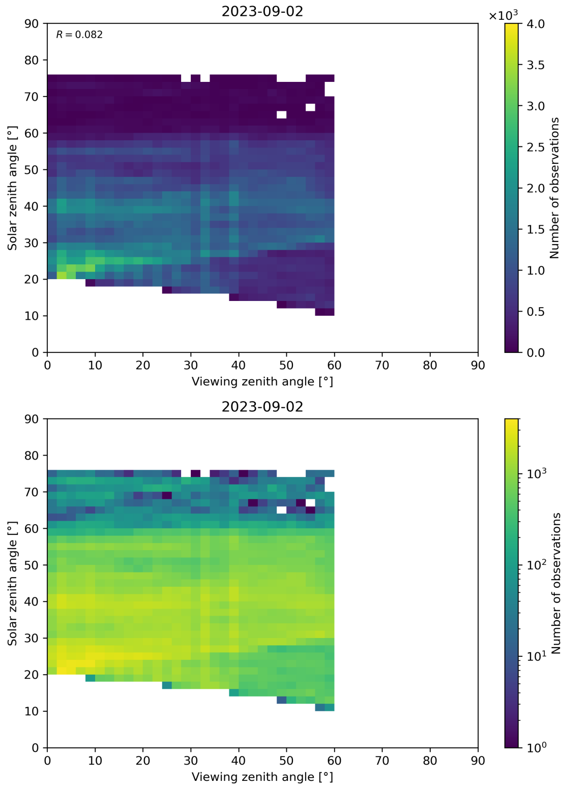
Figure 115: Scatter density plot of “Viewing zenith angle” against “Solar zenith angle” for 2023-09-01 to 2023-09-03.
