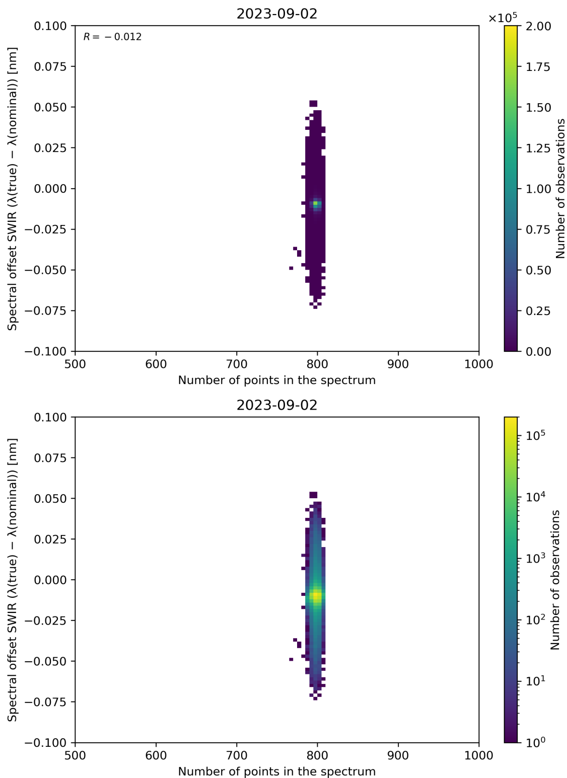
Figure 93: Scatter density plot of “Number of points in the spectrum” against “Spectral offset SWIR ( \lambda(\text{true}) - \lambda(\text{nominal}) )” for 2023-09-01 to 2023-09-03.
