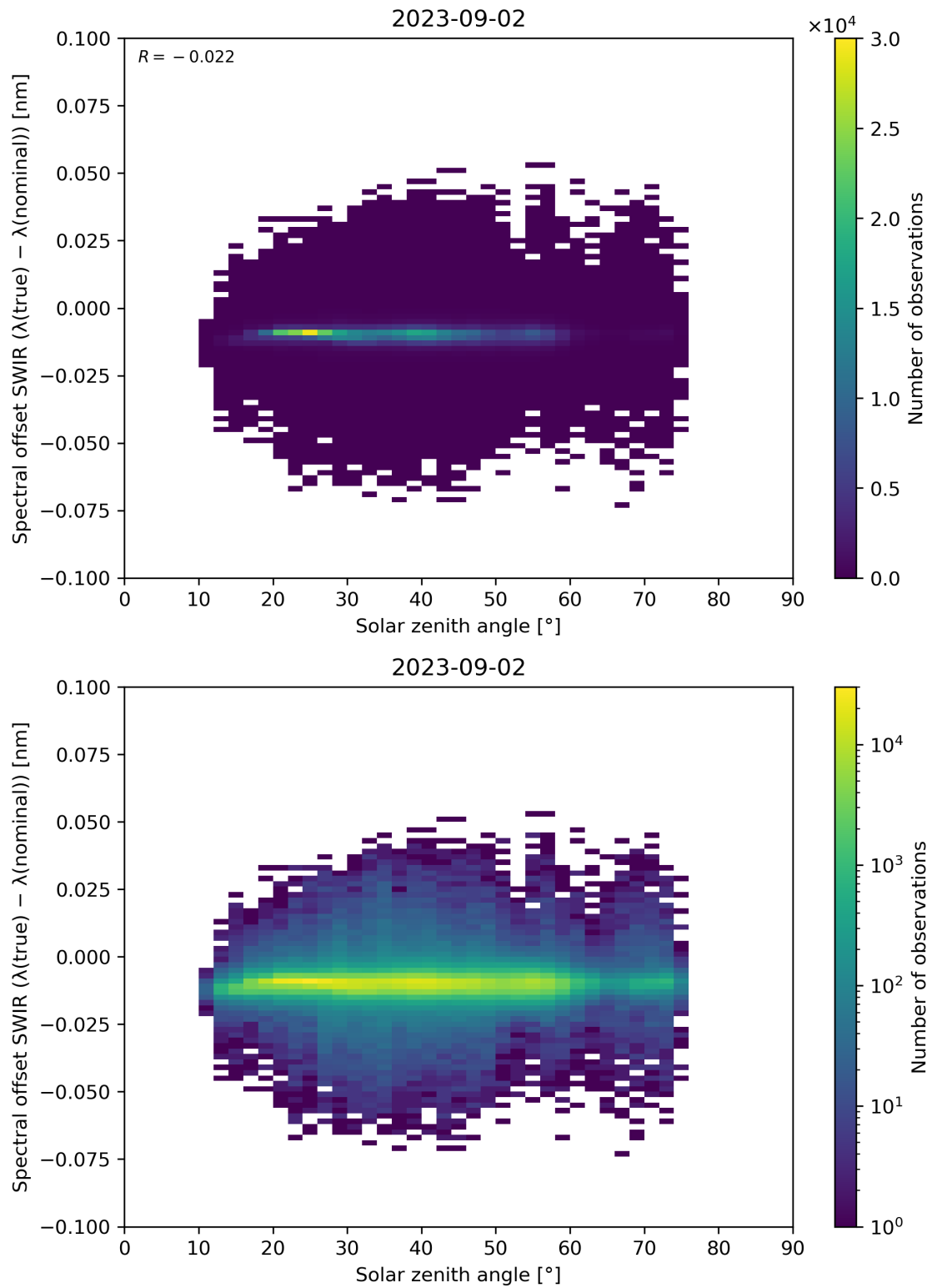
Figure 104: Scatter density plot of “Solar zenith angle” against “Spectral offset SWIR ( \lambda(\text{true}) - \lambda(\text{nominal}) )” for 2023-09-01 to 2023-09-03.
