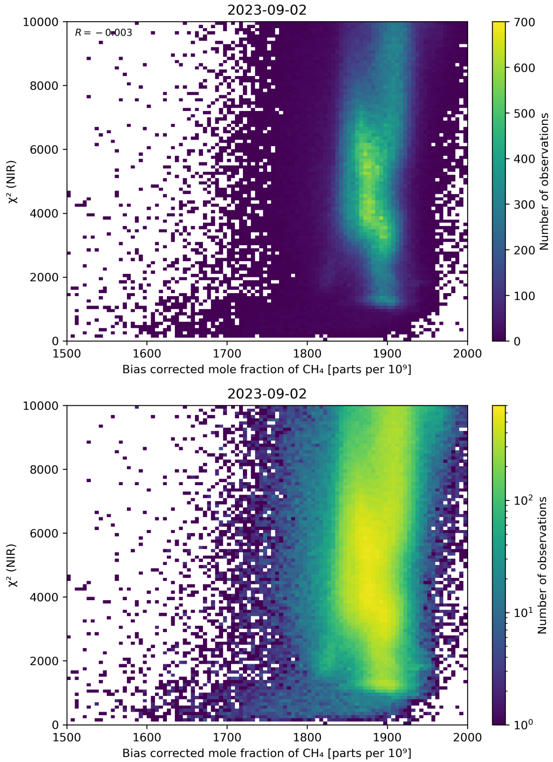
Figure 63: Scatter density plot of “Bias corrected mole fraction of CH 4 ” against “ \chi^2 (NIR)” for 2023-09-01 to 2023-09-03.
