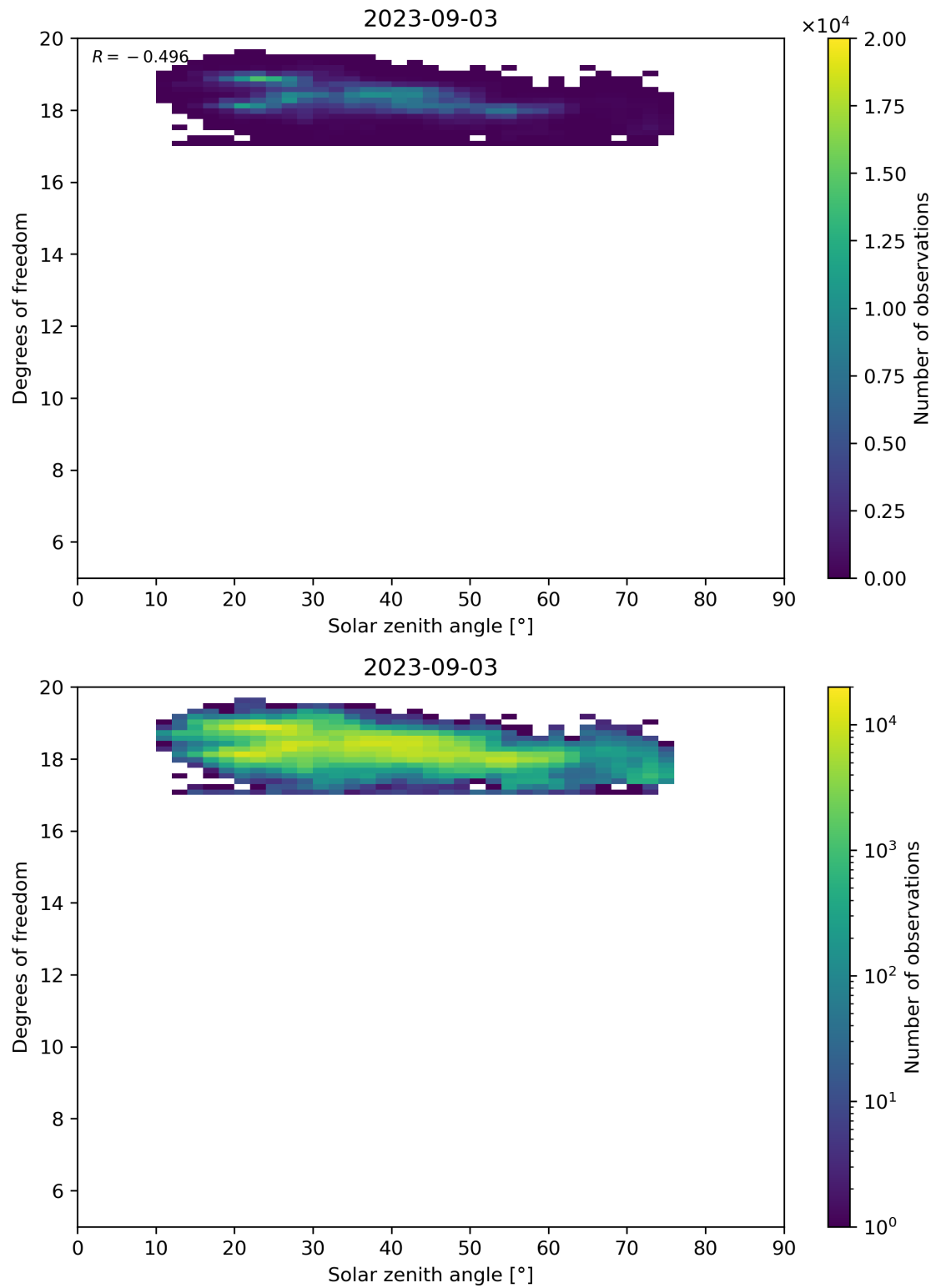
Figure 96: Scatter density plot of “Solar zenith angle” against “Degrees of freedom” for 2023-09-02 to 2023-09-04.
