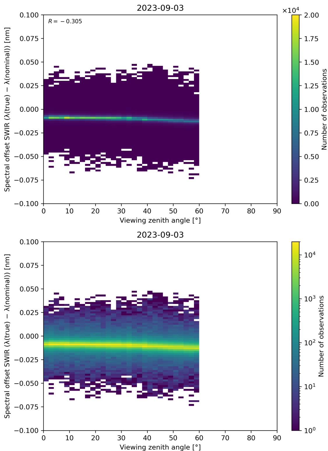
Figure 116: Scatter density plot of “Viewing zenith angle” against “Spectral offset SWIR ( \lambda(\text{true}) - \lambda(\text{nominal}) )” for 2023-09-02 to 2023-09-04.
