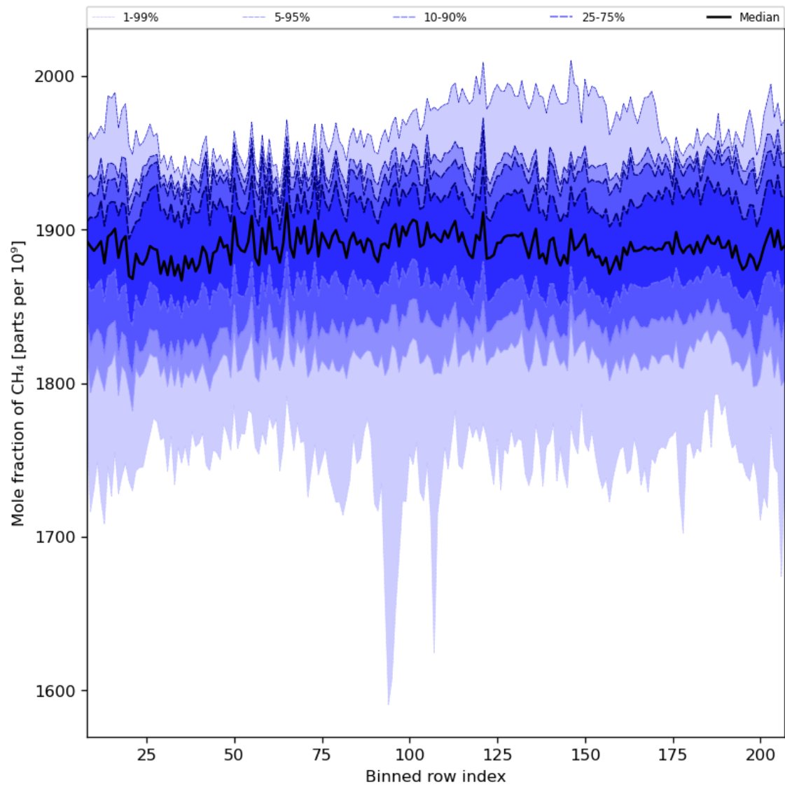
Figure 34: Along track statistics of “Mole fraction of CH 4 ” for 2023-09-02 to 2023-09-04
