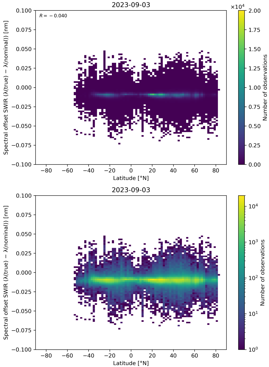
Figure 62: Scatter density plot of “Latitude” against “Spectral offset SWIR ( \lambda(\text{true}) - \lambda(\text{nominal}) )” for 2023-09-02 to 2023-09-04.
