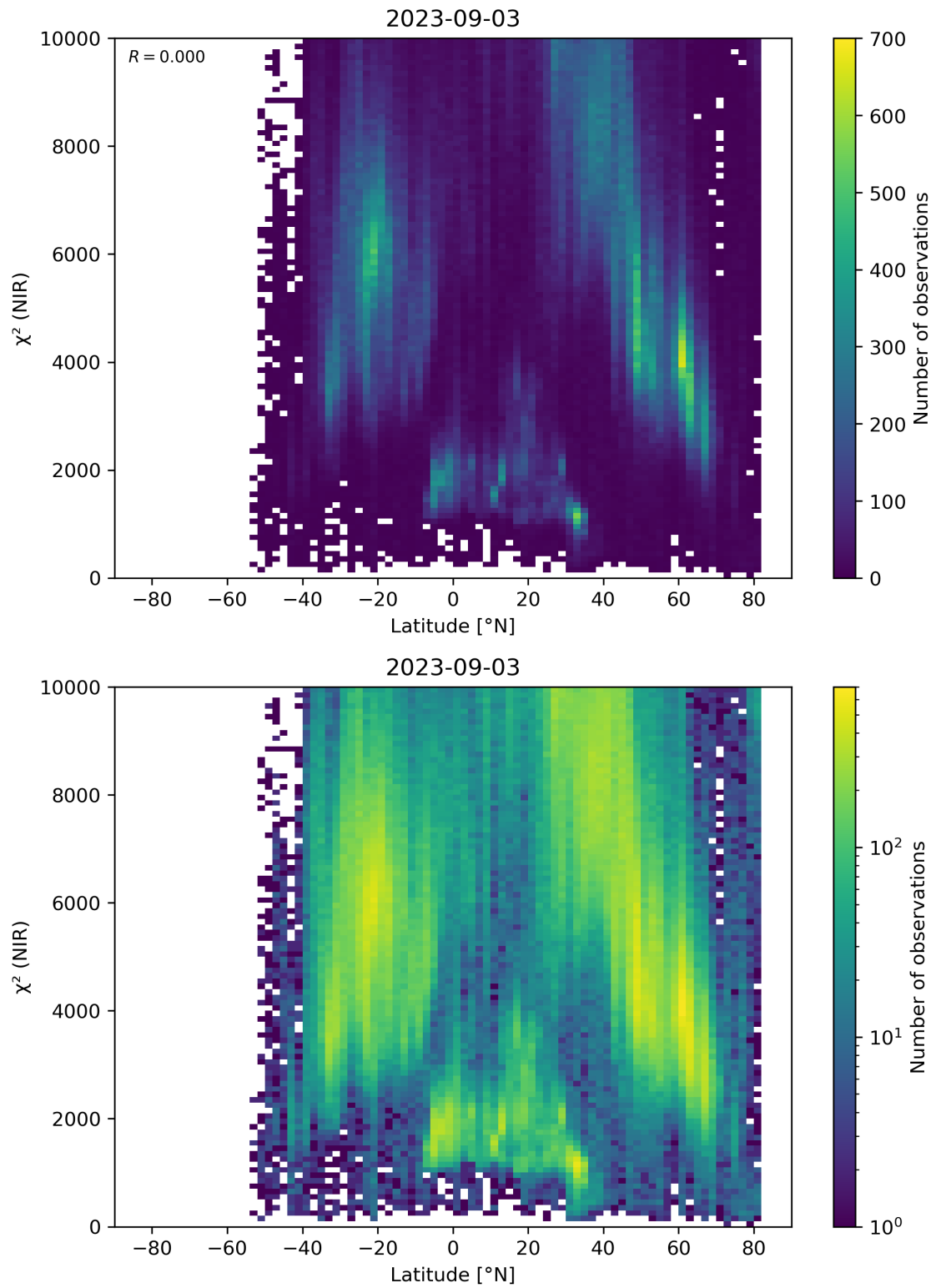
Figure 53: Scatter density plot of “Latitude” against “ \chi^2 (NIR)” for 2023-09-02 to 2023-09-04.
