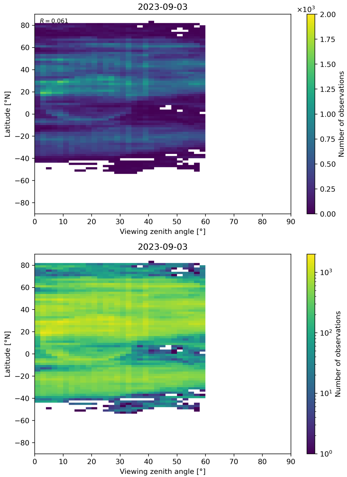
Figure 109: Scatter density plot of “Viewing zenith angle” against “Latitude” for 2023-09-02 to 2023-09-04.
