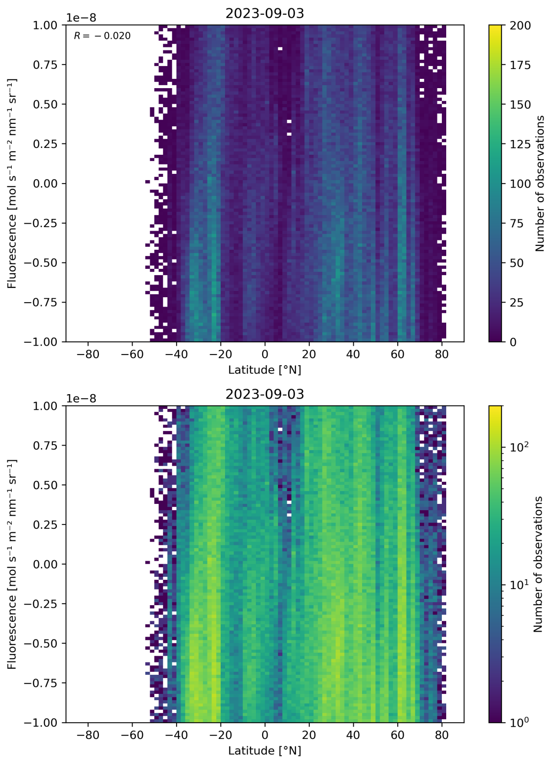
Figure 56: Scatter density plot of “Latitude” against “Fluorescence” for 2023-09-02 to 2023-09-04.
