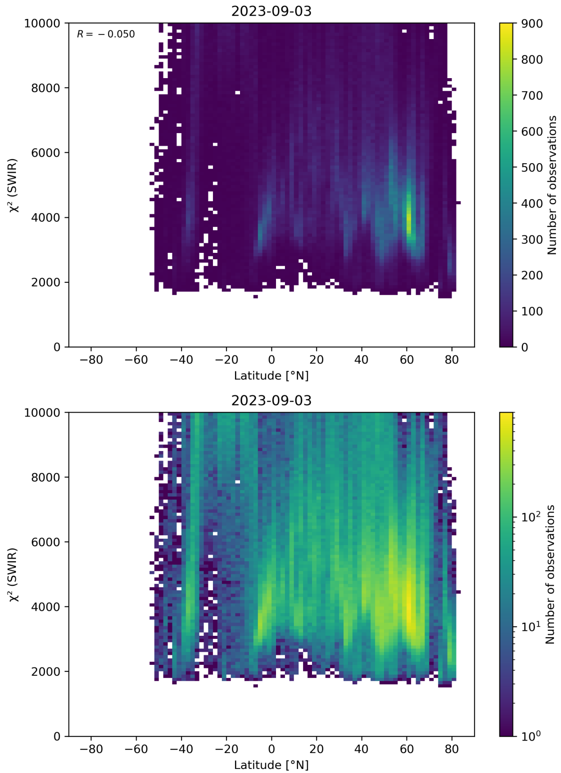
Figure 54: Scatter density plot of “Latitude” against “ \chi^2 (SWIR)” for 2023-09-02 to 2023-09-04.
