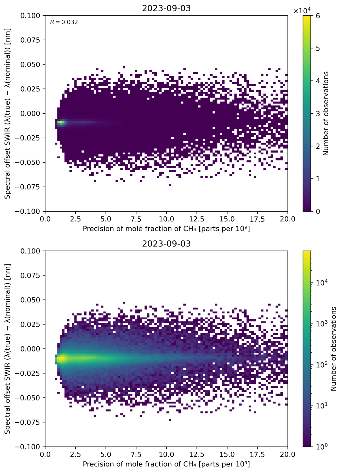
Figure 85: Scatter density plot of “Precision of mole fraction of CH 4 ” against “Spectral offset SWIR ( \lambda(\text{true}) - \lambda(\text{nominal}) )” for 2023-09-02 to 2023-09-04.
