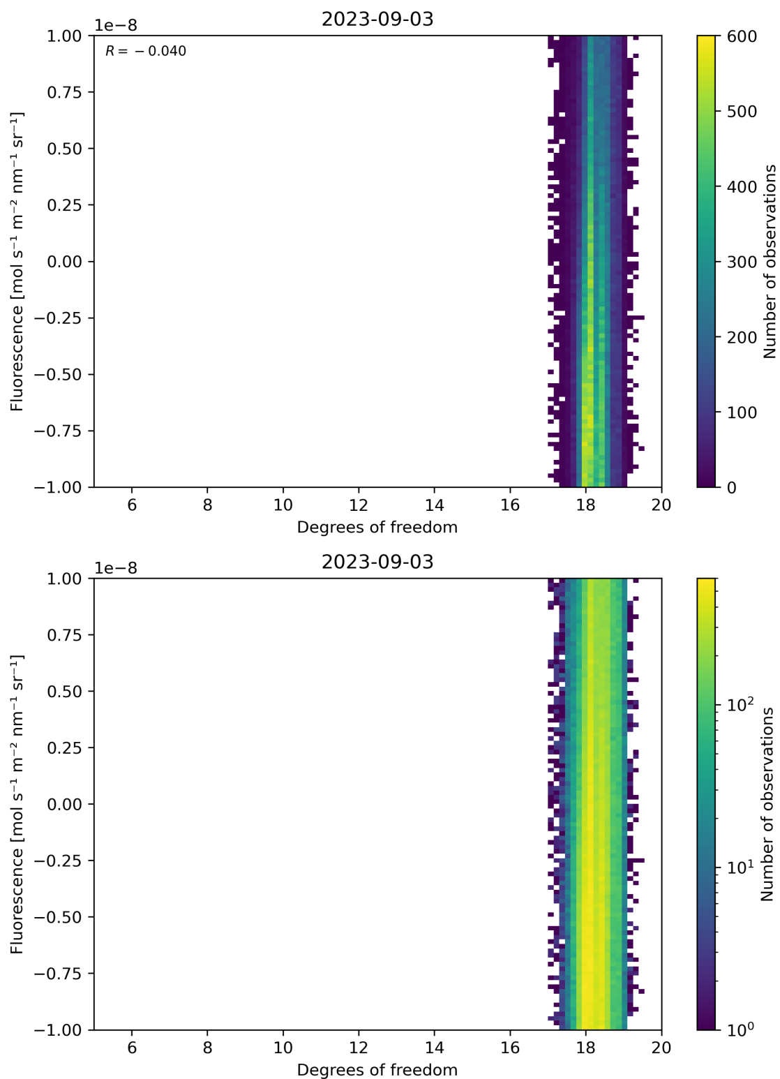
Figure 51: Scatter density plot of “Degrees of freedom” against “Fluorescence” for 2023-09-02 to 2023-09-04.
