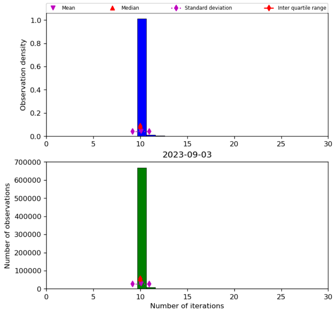
Figure 31: Histogram of “Number of iterations” for 2023-09-02 to 2023-09-04
