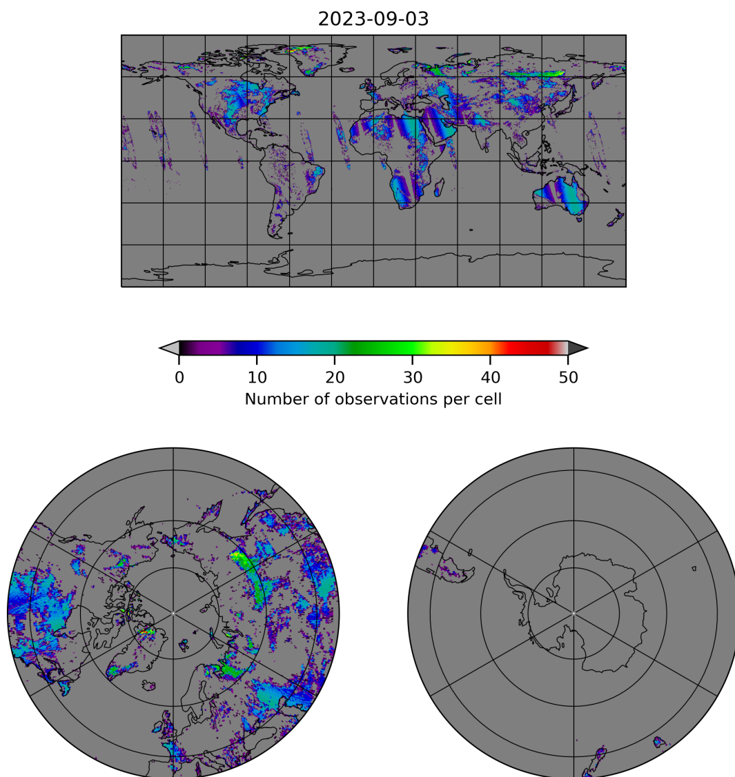
Figure 10: Map of the number of observations for 2023-09-02 to 2023-09-04
