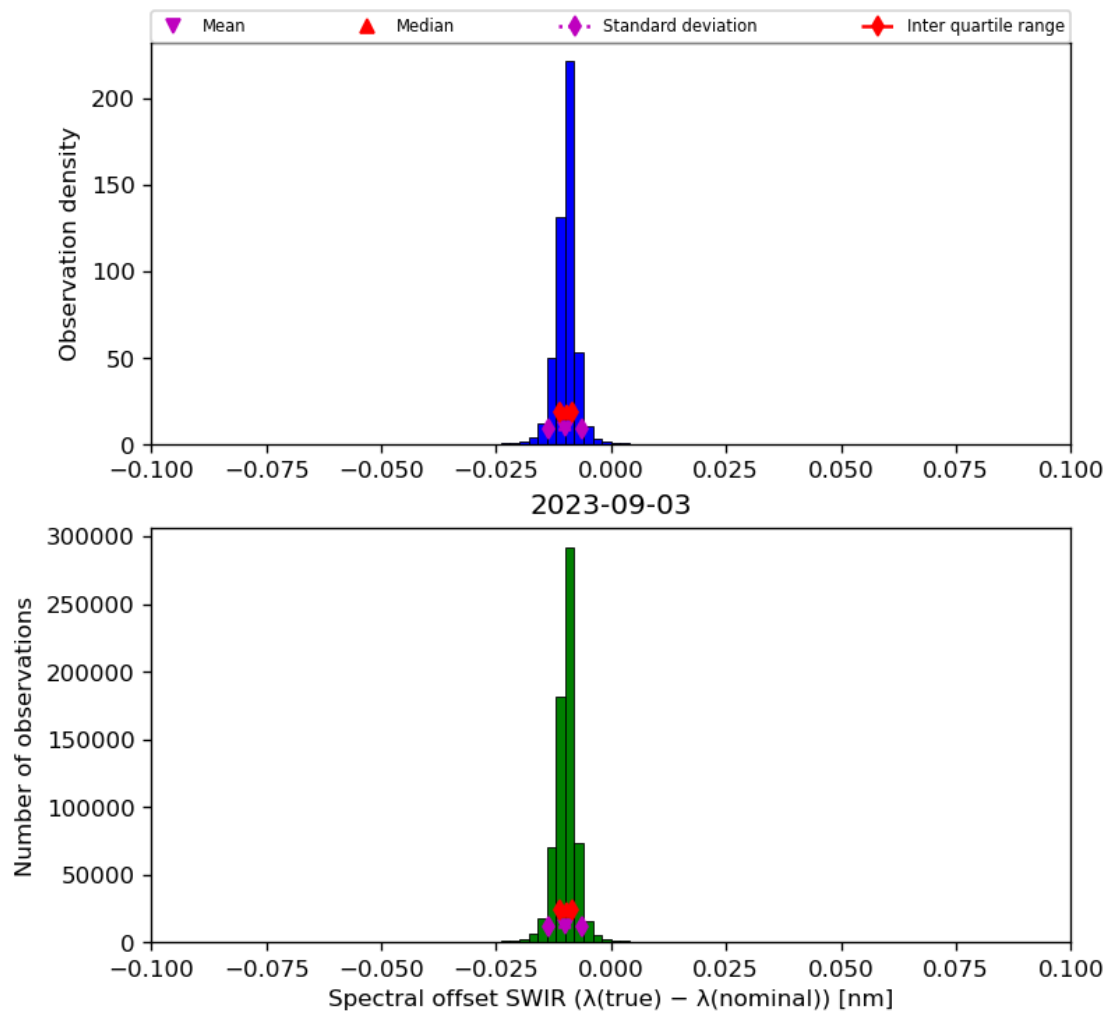
Figure 27: Histogram of “Spectral offset SWIR ( \lambda(\text{true}) - \lambda(\text{nominal}) )” for 2023-09-02 to 2023-09-04
