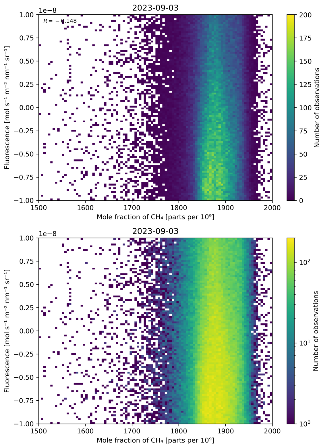
Figure 73: Scatter density plot of “Mole fraction of \text{CH}_4 ” against “Fluorescence” for 2023-09-02 to 2023-09-04.
