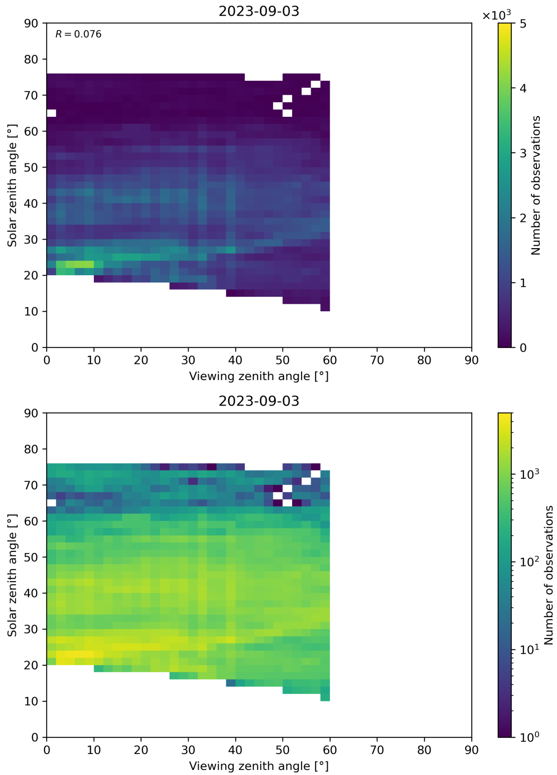
Figure 115: Scatter density plot of “Viewing zenith angle” against “Solar zenith angle” for 2023-09-02 to 2023-09-04.
