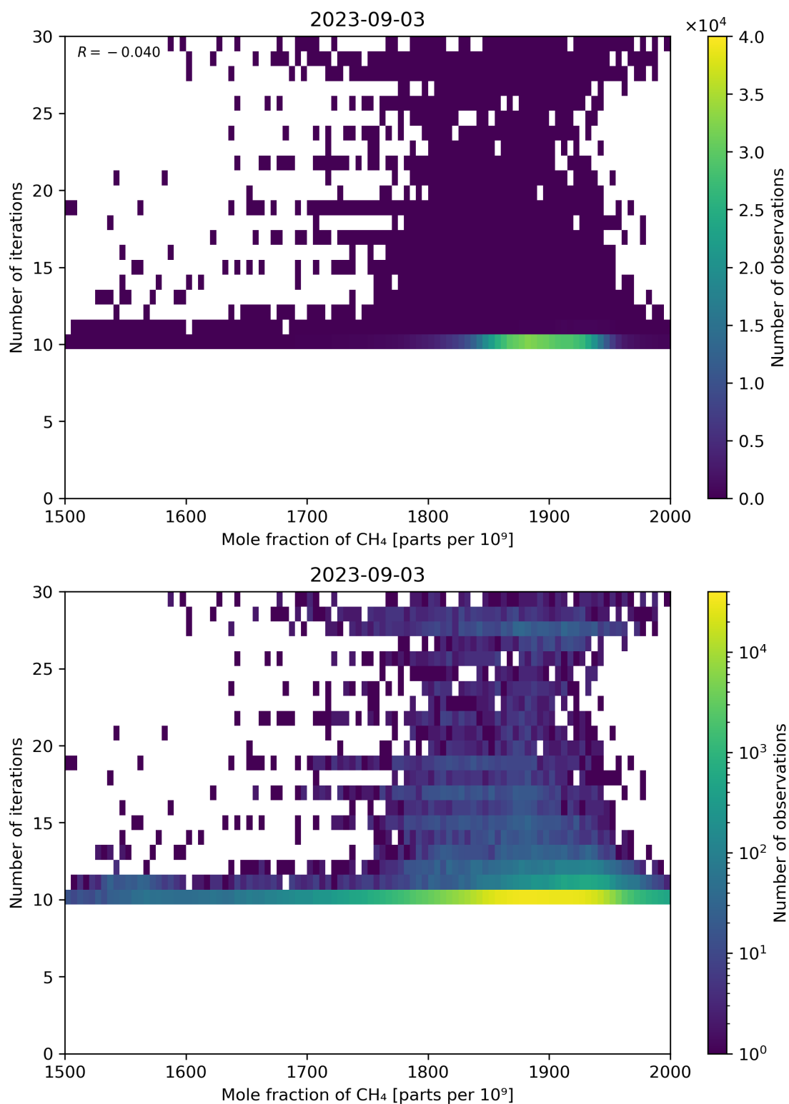
Figure 76: Scatter density plot of “Mole fraction of CH 4 ” against “Number of iterations” for 2023-09-02 to 2023-09-04.
