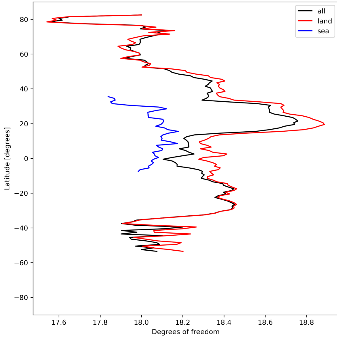
Figure 19: Zonal average of “Degrees of freedom” for 2023-09-02 to 2023-09-04.
