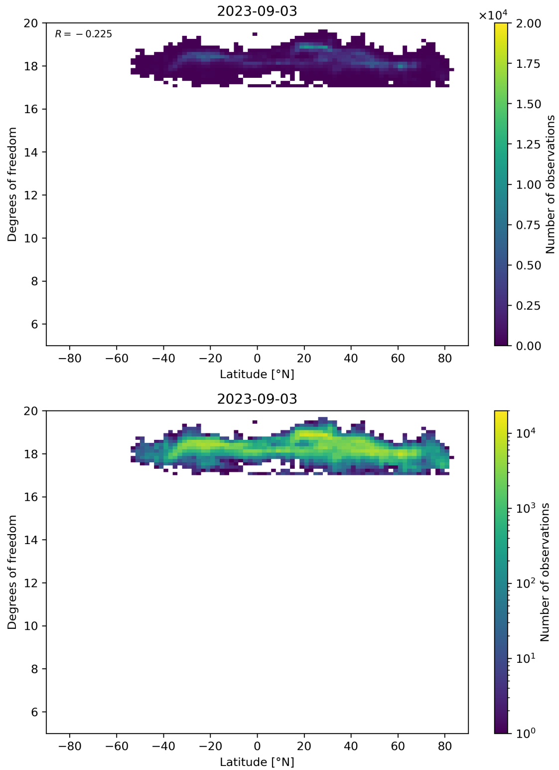
Figure 55: Scatter density plot of “Latitude” against “Degrees of freedom” for 2023-09-02 to 2023-09-04.
