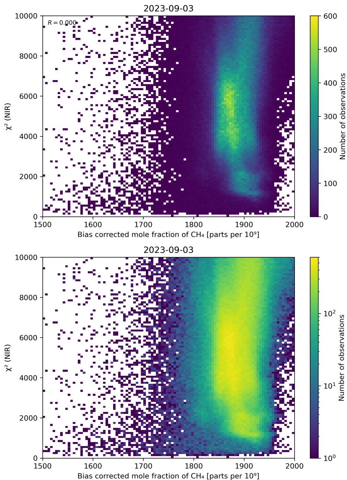
Figure 63: Scatter density plot of “Bias corrected mole fraction of CH 4 ” against “ \chi^2 (NIR)” for 2023-09-02 to 2023-09-04.
