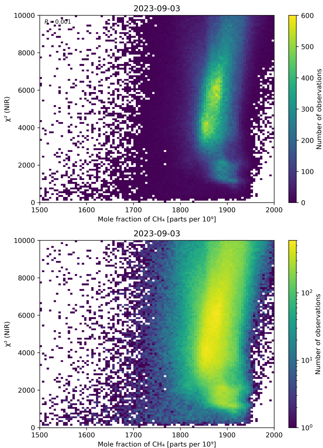
Figure 70: Scatter density plot of “Mole fraction of CH 4 ” against “ \chi^2 (NIR)” for 2023-09-02 to 2023-09-04.
