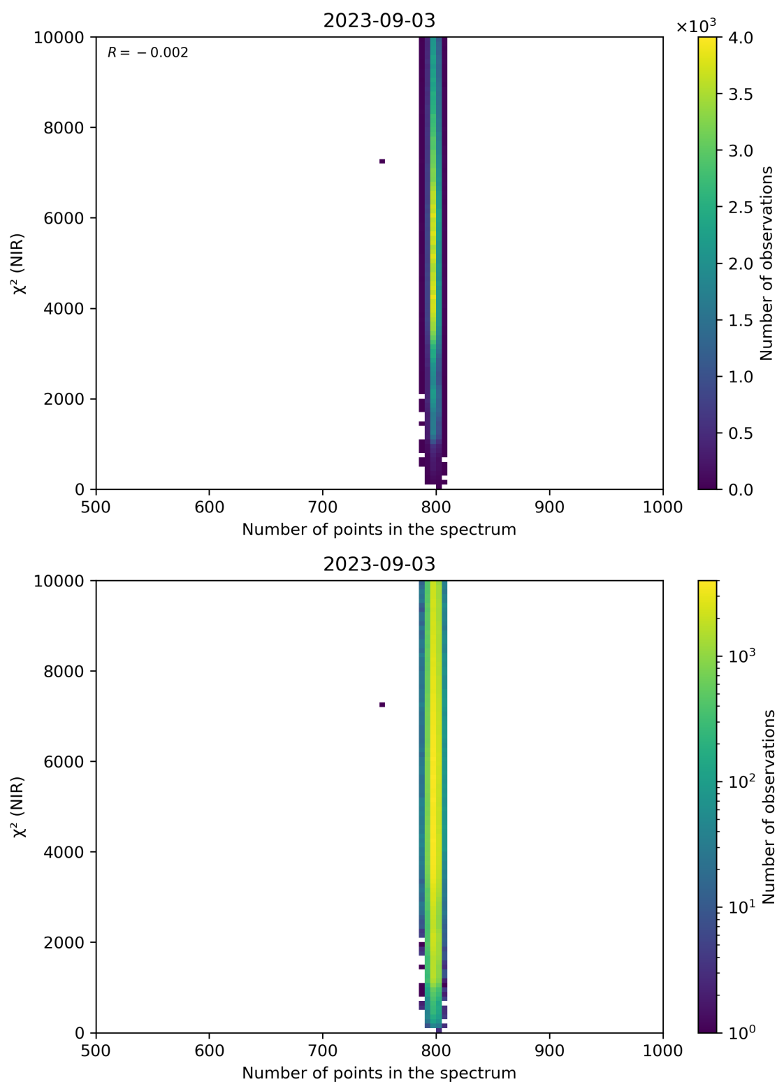
Figure 88: Scatter density plot of “Number of points in the spectrum” against “ \chi^2 (NIR)” for 2023-09-02 to 2023-09-04.
