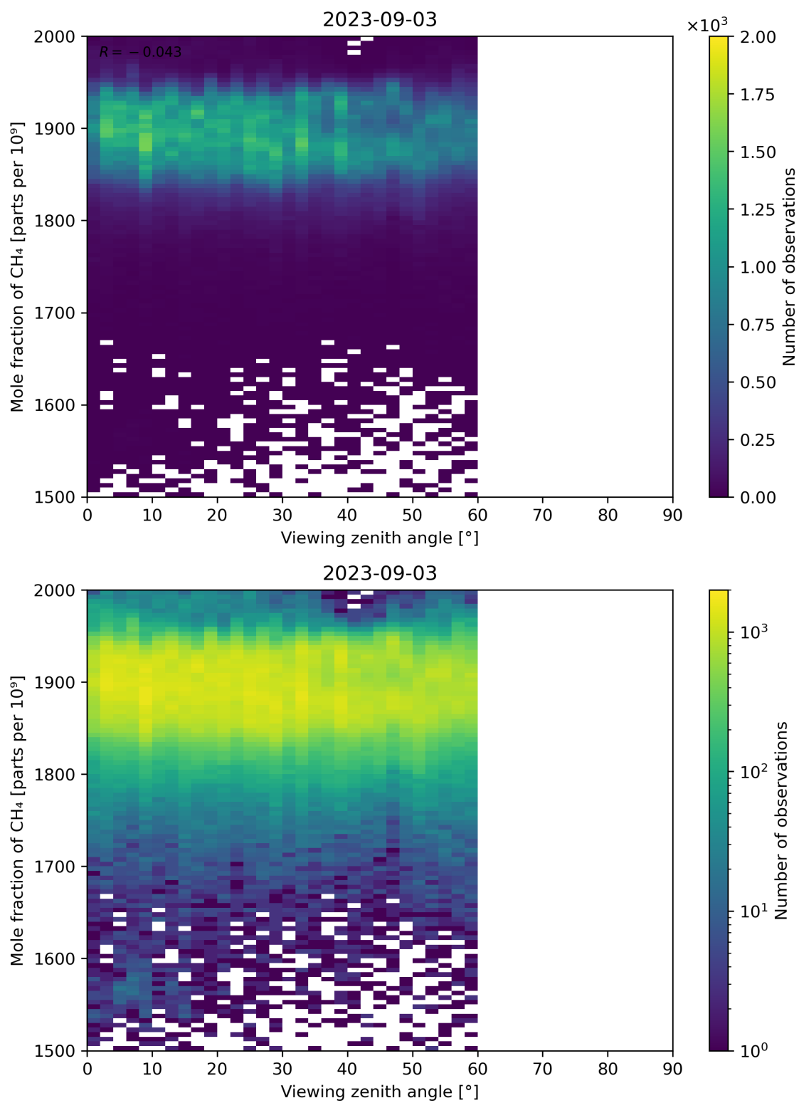
Figure 110: Scatter density plot of “Viewing zenith angle” against “Mole fraction of CH 4 ” for 2023-09-02 to 2023-09-04.
