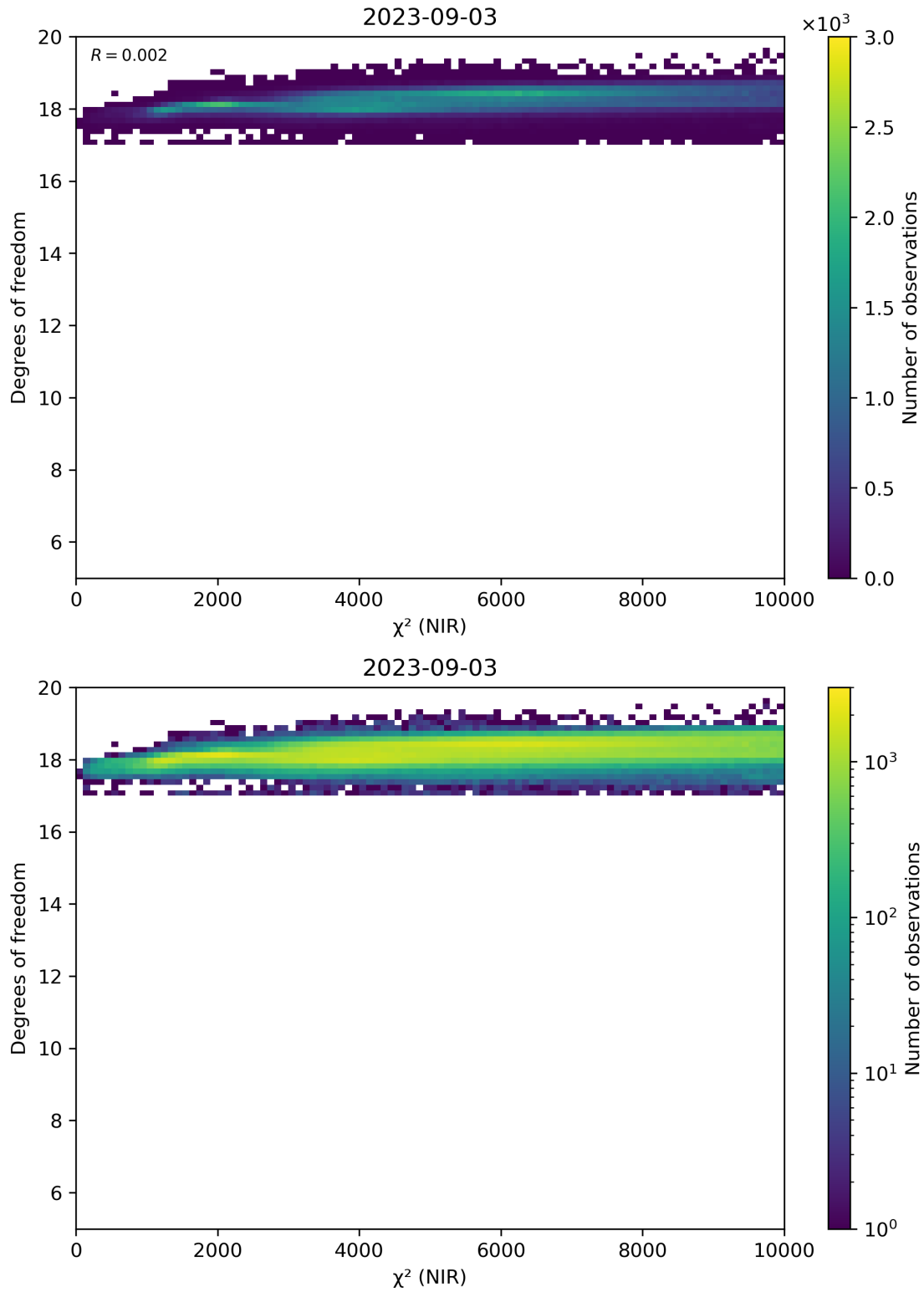
Figure 44: Scatter density plot of “ \chi^2 (NIR)” against “Degrees of freedom” for 2023-09-02 to 2023-09-04.
