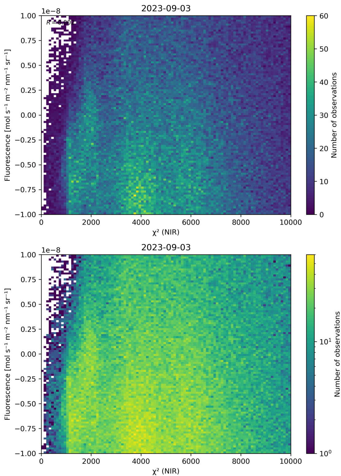
Figure 45: Scatter density plot of “ \chi^2 (NIR)” against “Fluorescence” for 2023-09-02 to 2023-09-04.
