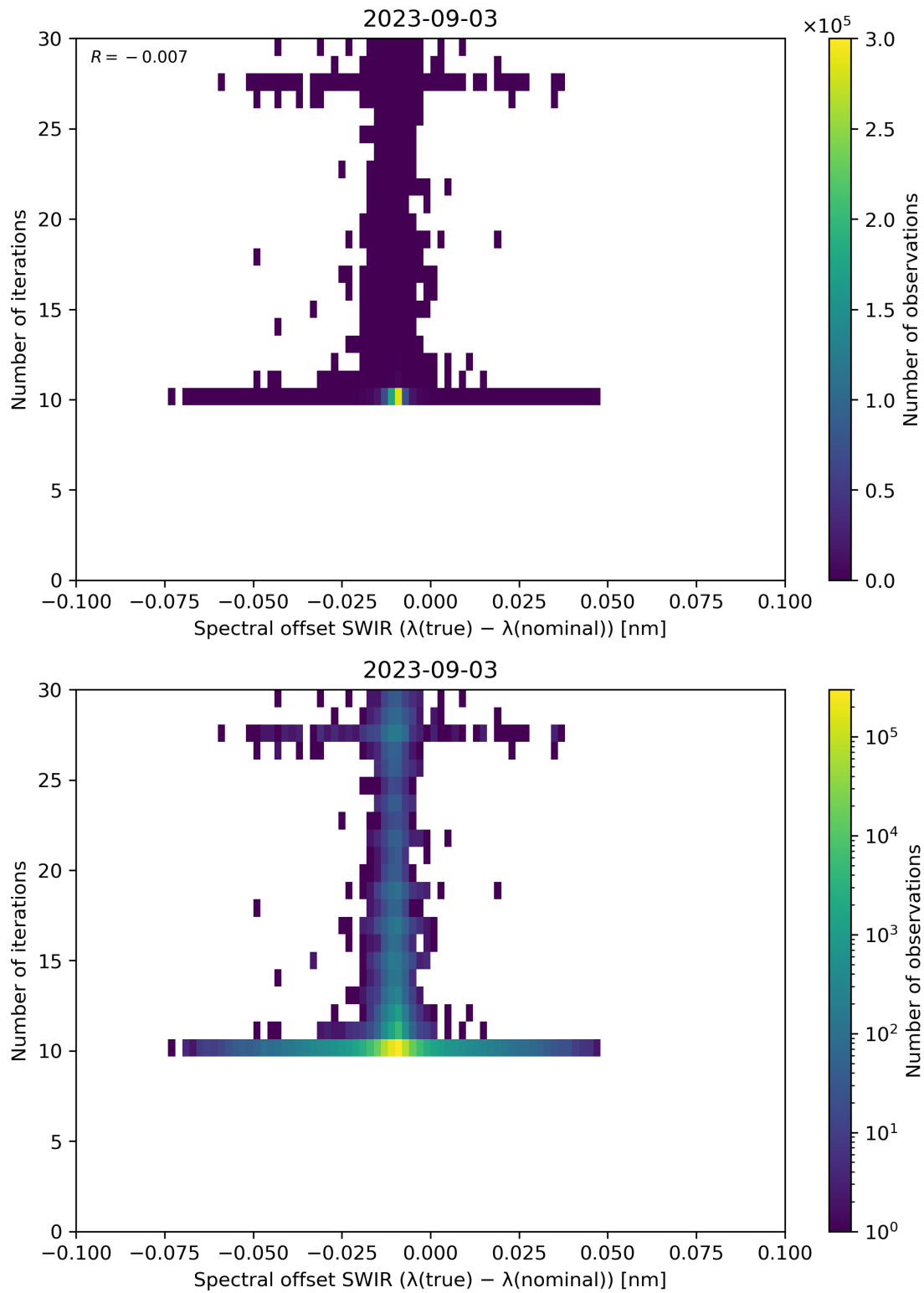
Figure 121: Scatter density plot of “Spectral offset SWIR ( \lambda(\text{true}) - \lambda(\text{nominal}) )” against “Number of iterations” for 2023-09-02 to 2023-09-04.
