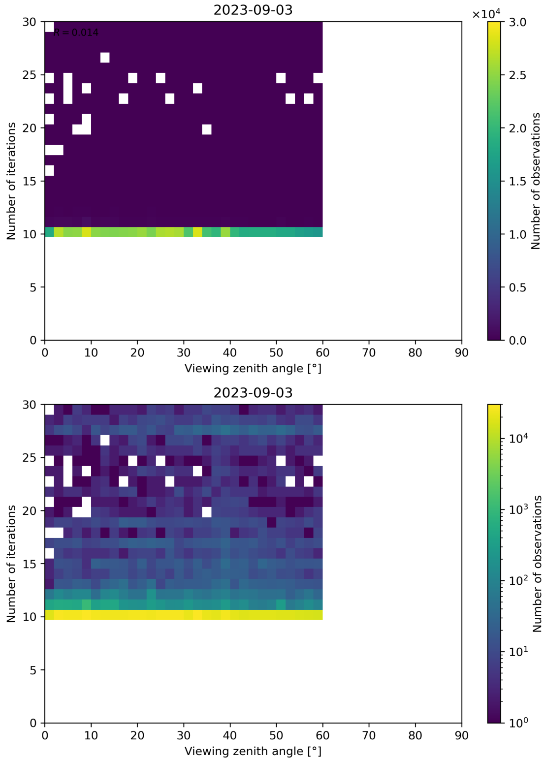
Figure 113: Scatter density plot of “Viewing zenith angle” against “Number of iterations” for 2023-09-02 to 2023-09-04.
