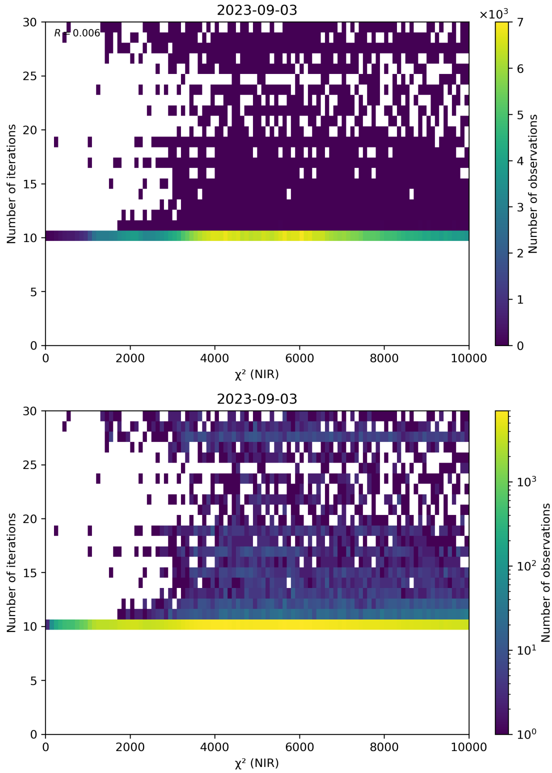
Figure 46: Scatter density plot of “ \chi^2 (NIR)” against “Number of iterations” for 2023-09-02 to 2023-09-04.
