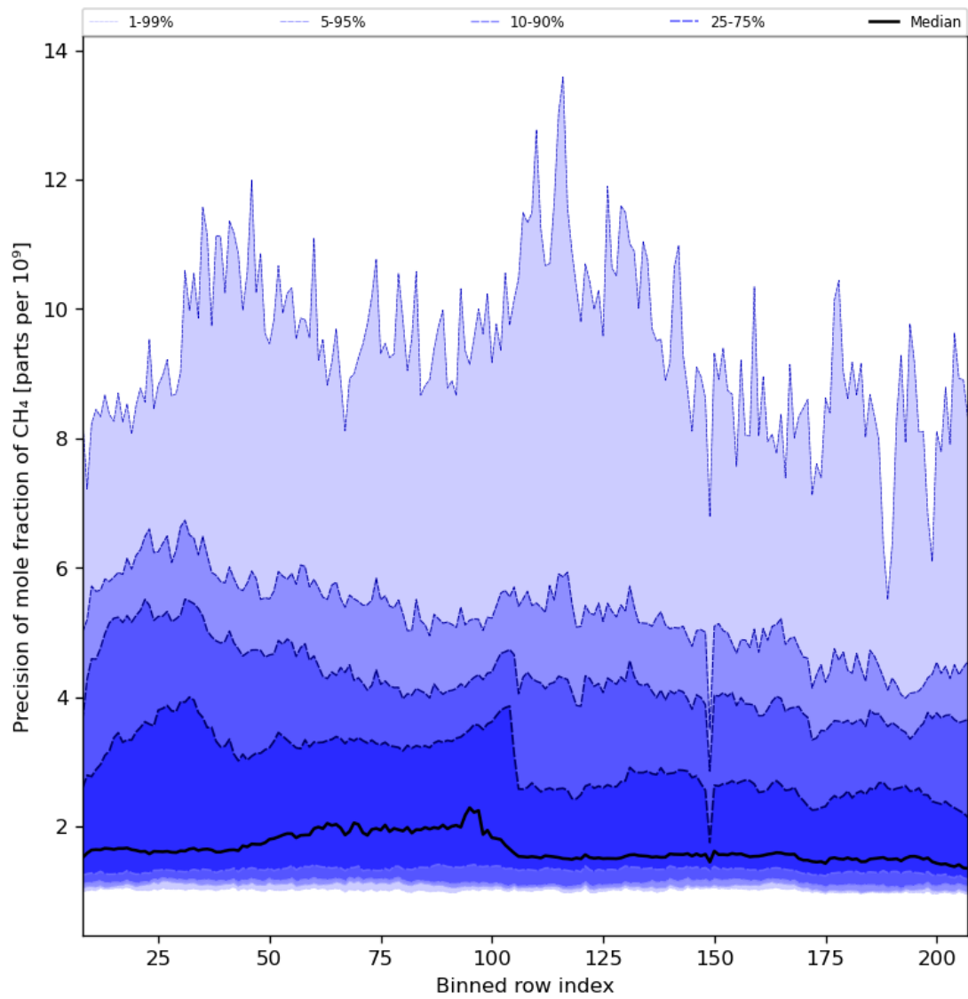
Figure 35: Along track statistics of “Precision of mole fraction of CH 4 ” for 2023-09-02 to 2023-09-04
