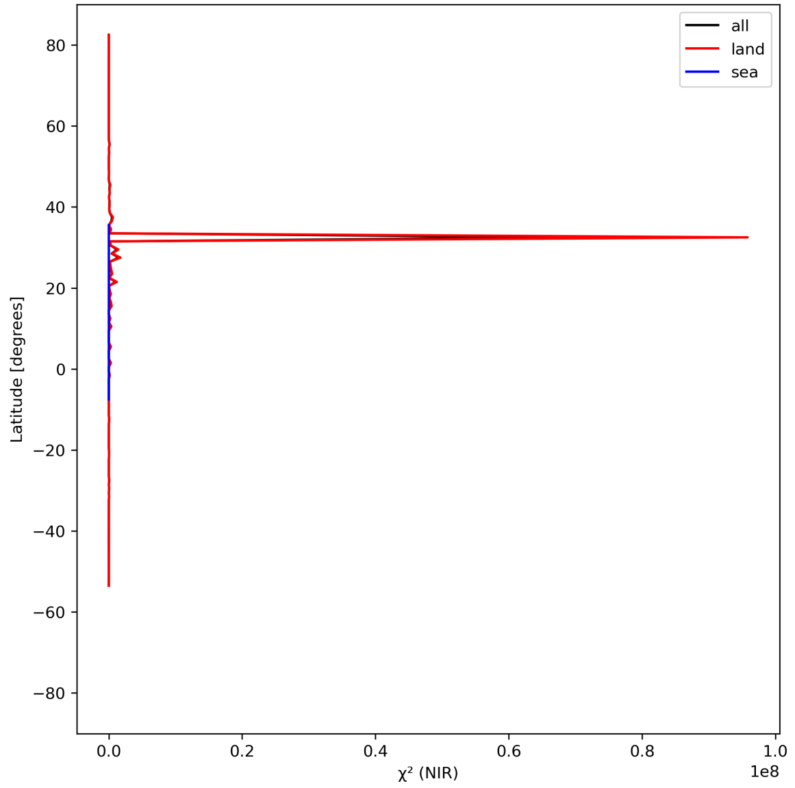
Figure 18: Zonal average of “ \chi^2 (NIR)” for 2023-09-02 to 2023-09-04.
