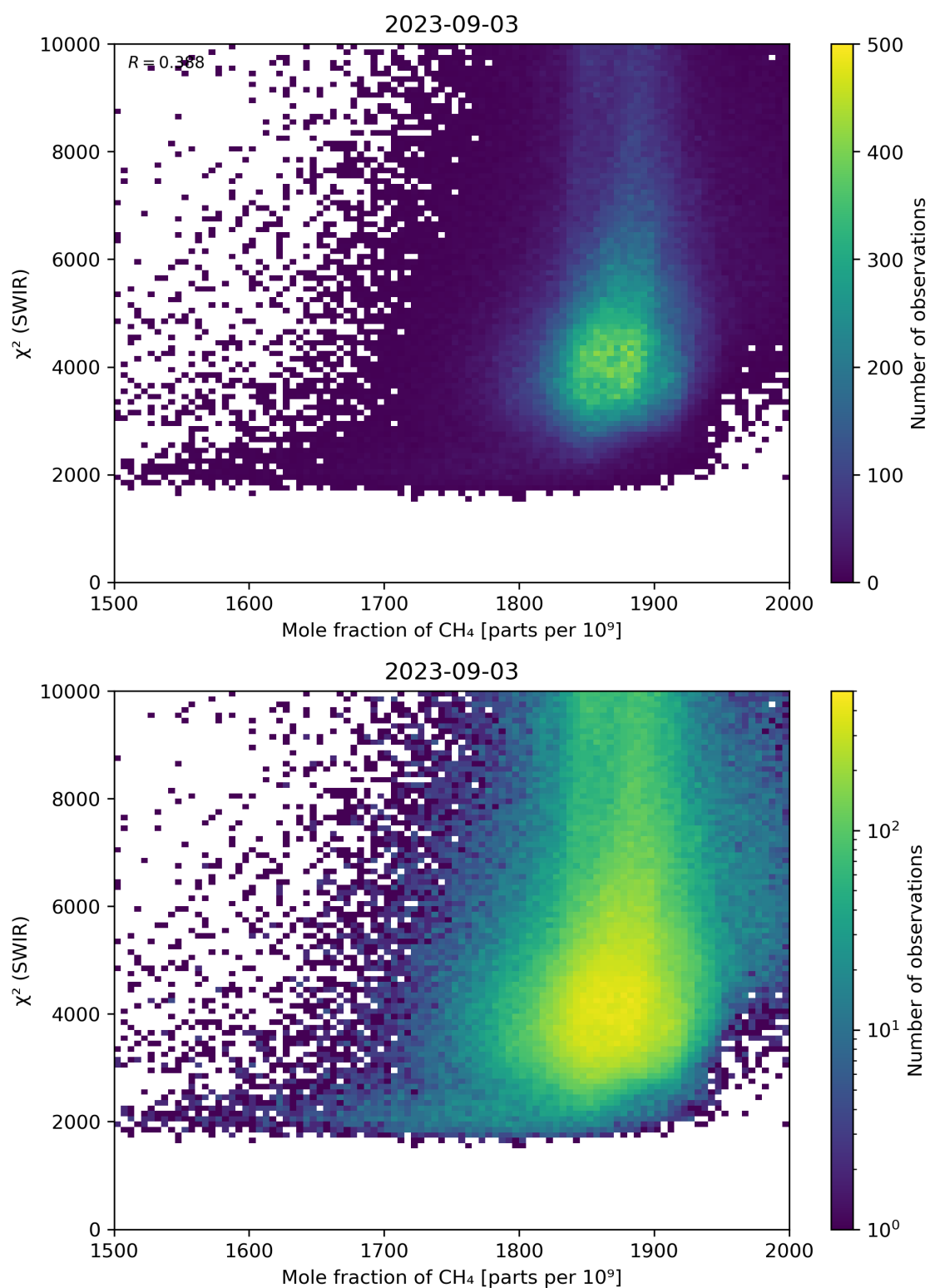
Figure 71: Scatter density plot of “Mole fraction of \text{CH}_4 ” against “ \chi^2 (SWIR)” for 2023-09-02 to 2023-09-04.
