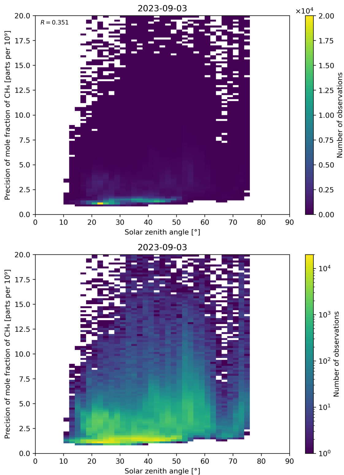
Figure 101: Scatter density plot of “Solar zenith angle” against “Precision of mole fraction of CH 4 ” for 2023-09-02 to 2023-09-04.
