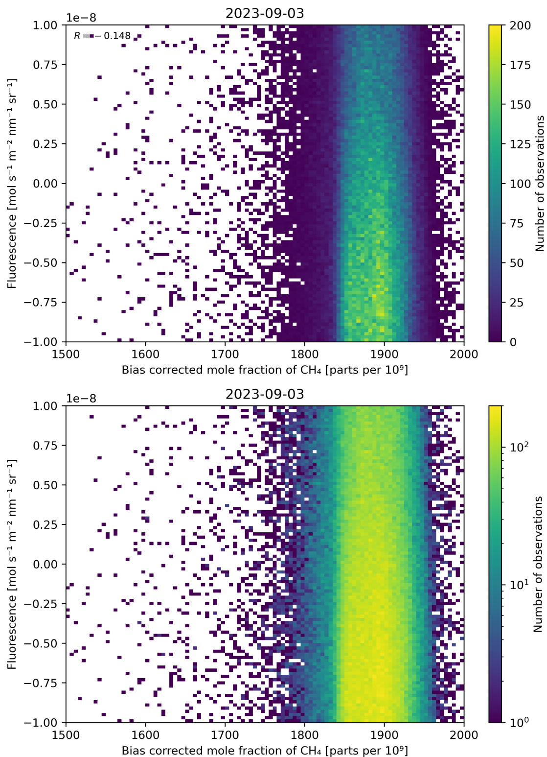
Figure 66: Scatter density plot of “Bias corrected mole fraction of \text{CH}_4 ” against “Fluorescence” for 2023-09-02 to 2023-09-04.
