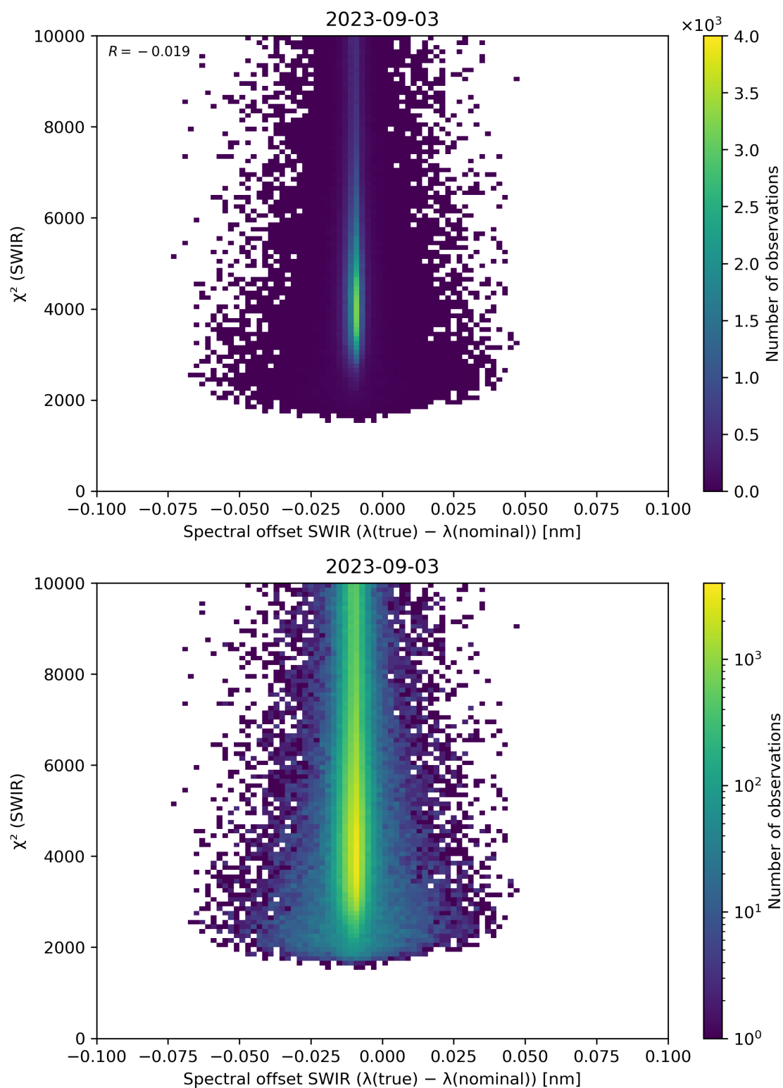
Figure 118: Scatter density plot of “Spectral offset SWIR ( \lambda(\text{true}) - \lambda(\text{nominal}) )” against “ \chi^2 (SWIR)” for 2023-09-02 to 2023-09-04.
