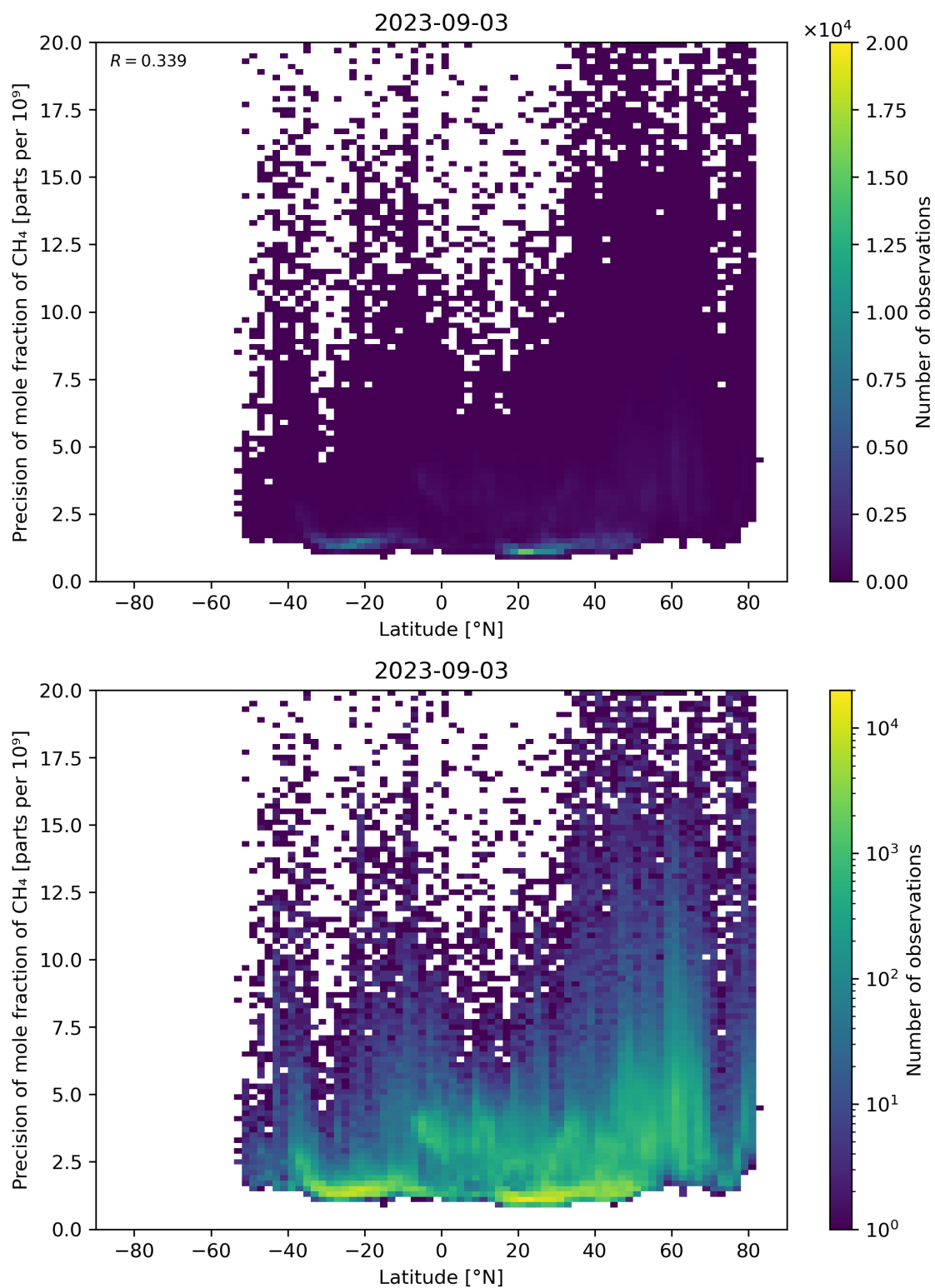
Figure 59: Scatter density plot of “Latitude” against “Precision of mole fraction of \text{CH}_4 ” for 2023-09-02 to 2023-09-04.
