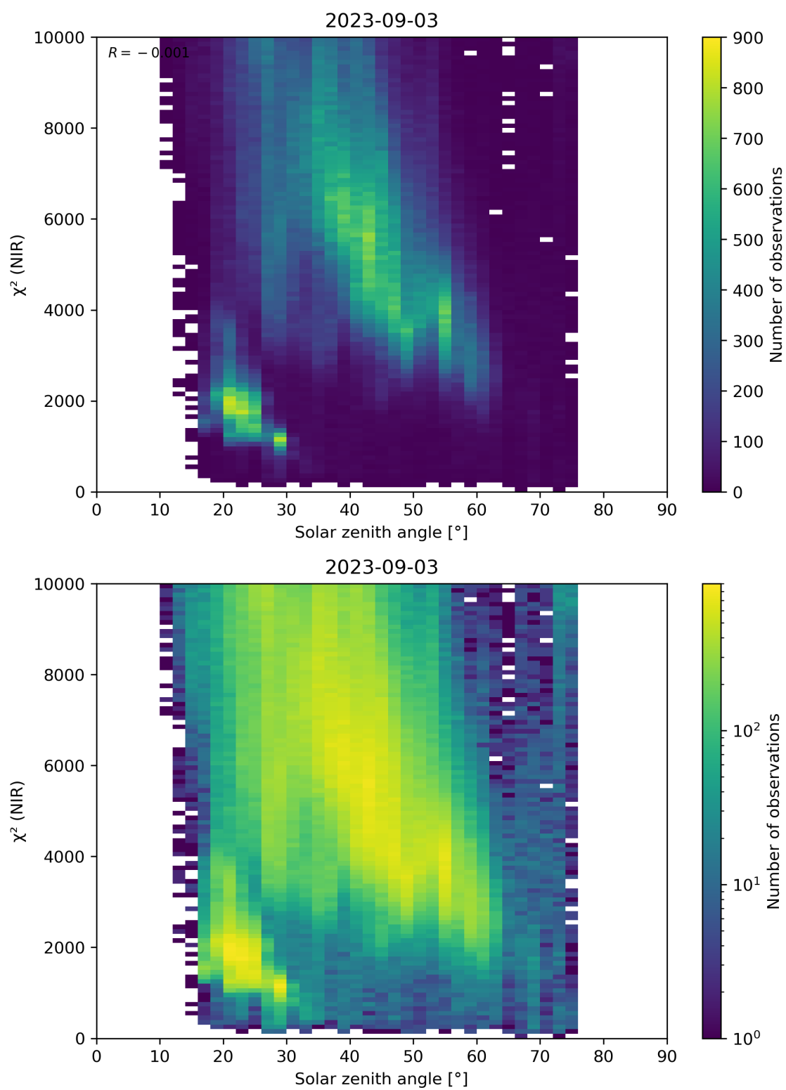
Figure 94: Scatter density plot of “Solar zenith angle” against “ \chi^2 (NIR)” for 2023-09-02 to 2023-09-04.
