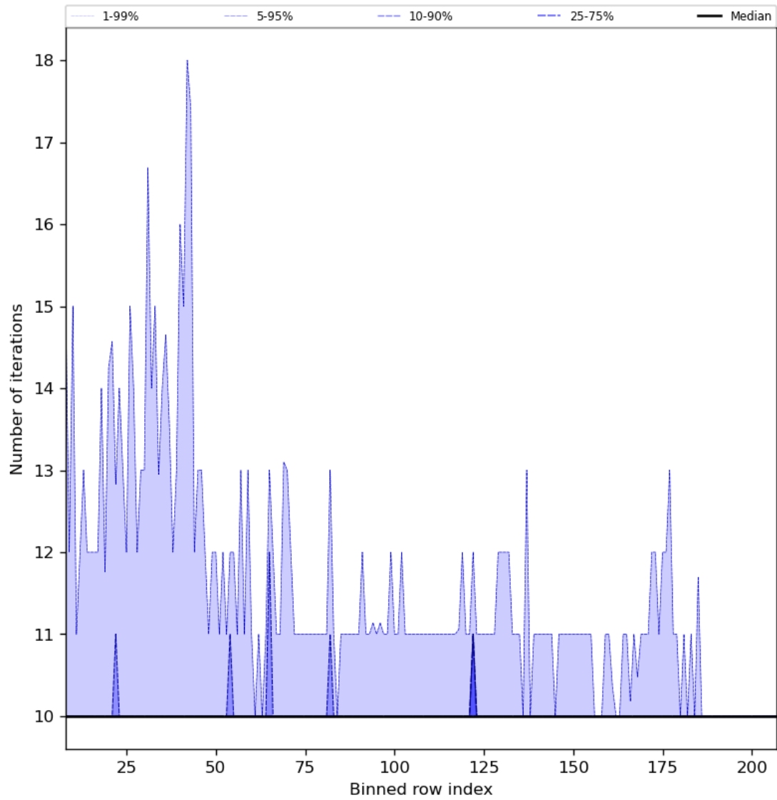
Figure 42: Along track statistics of “Number of iterations” for 2023-09-02 to 2023-09-04
