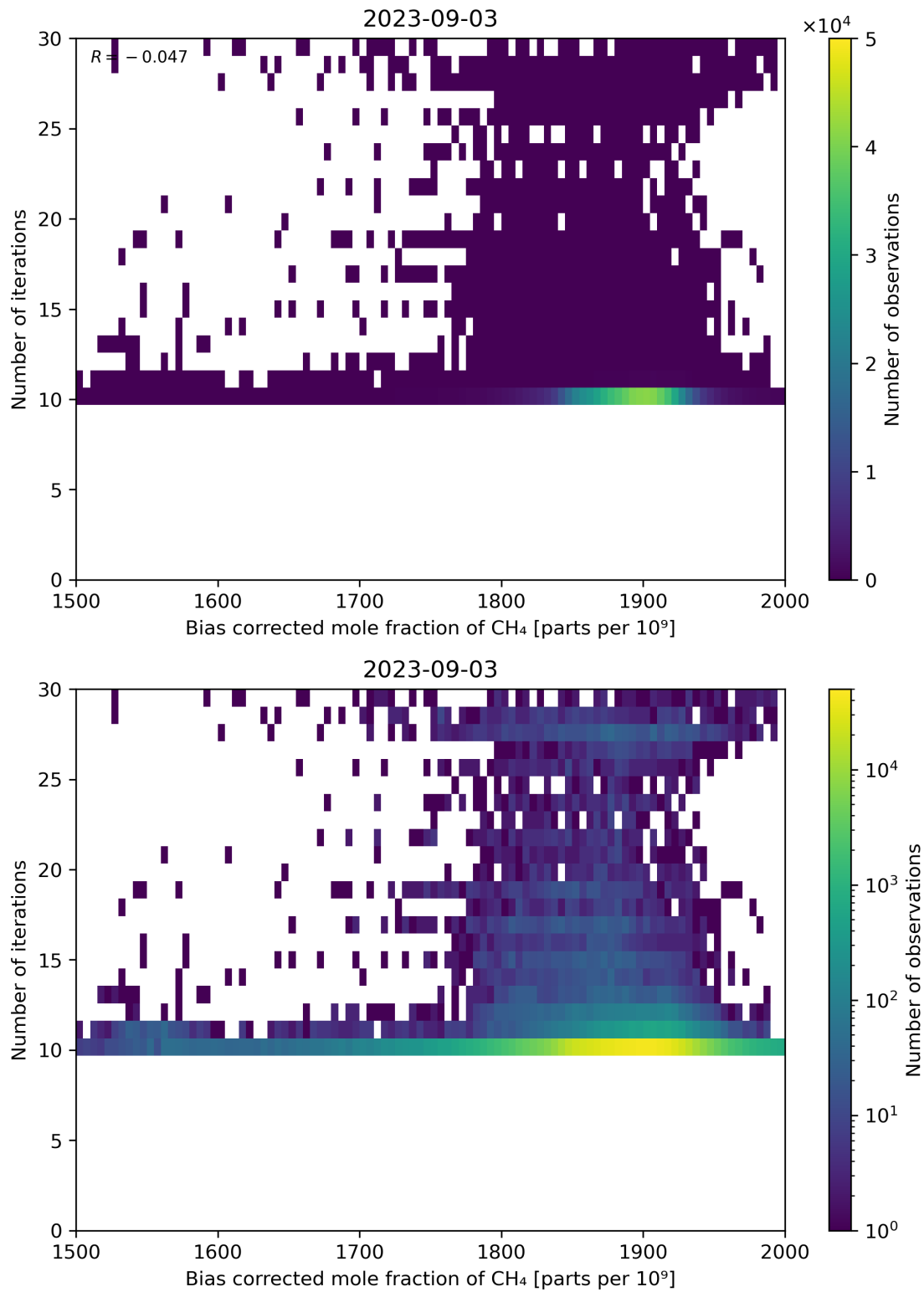
Figure 67: Scatter density plot of “Bias corrected mole fraction of CH 4 ” against “Number of iterations” for 2023-09-02 to 2023-09-04.
