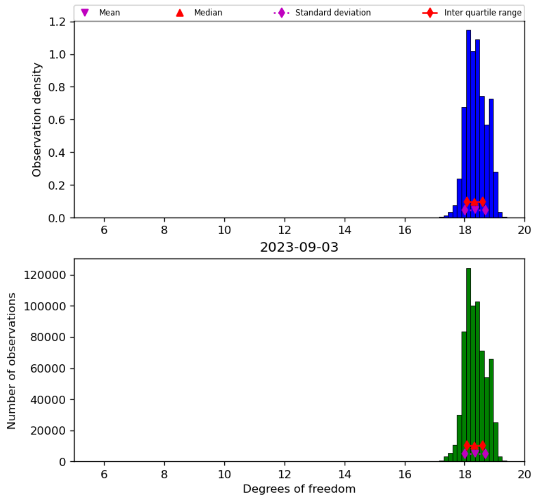
Figure 30: Histogram of “Degrees of freedom” for 2023-09-02 to 2023-09-04
