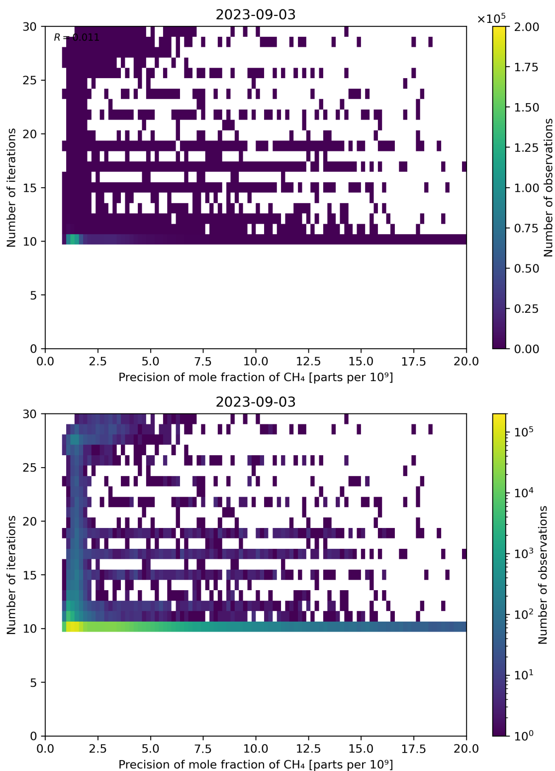
Figure 83: Scatter density plot of “Precision of mole fraction of CH 4 ” against “Number of iterations” for 2023-09-02 to 2023-09-04.
