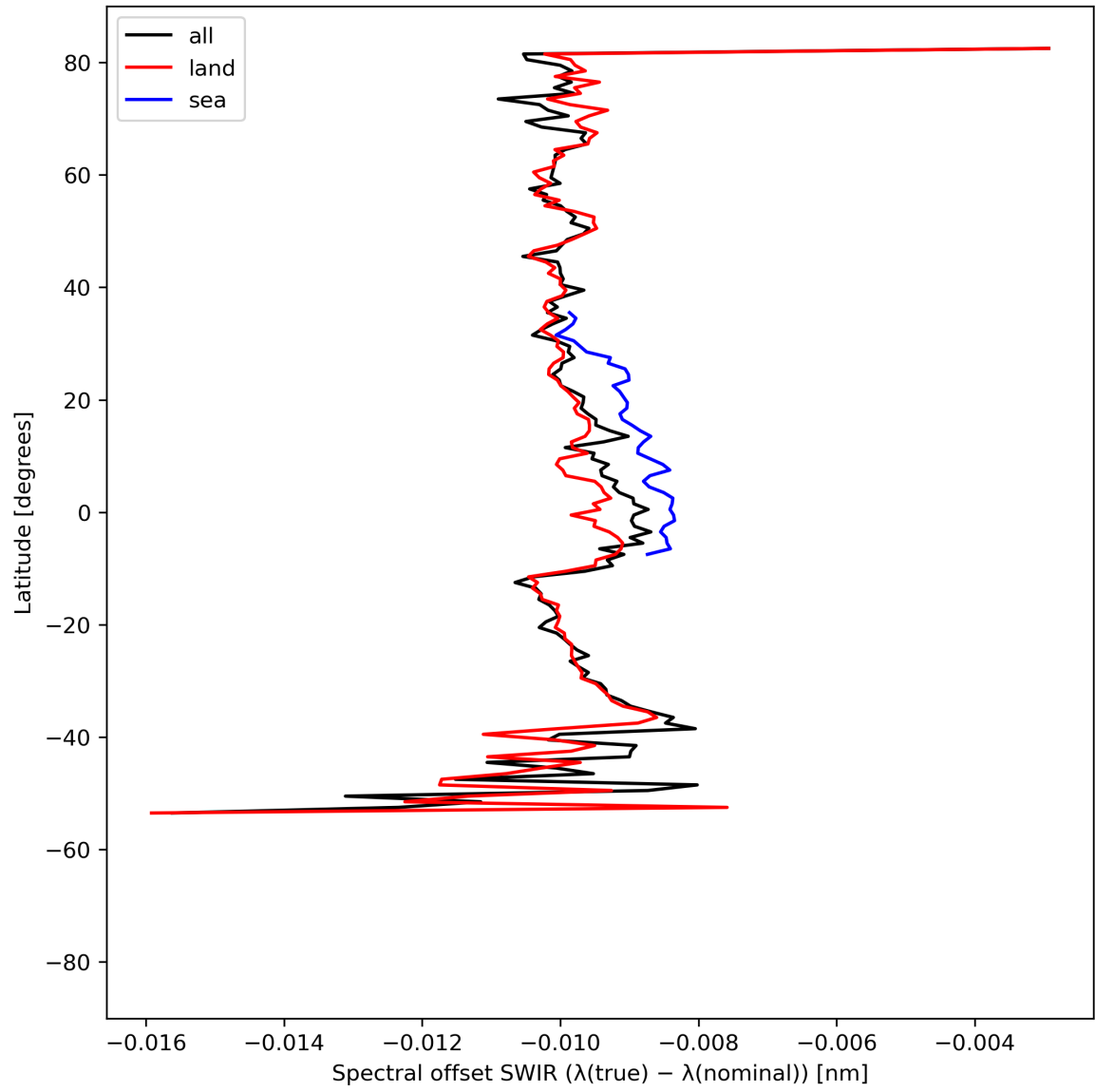
Figure 16: Zonal average of “Spectral offset SWIR ( \lambda(\text{true}) - \lambda(\text{nominal}) )” for 2023-09-02 to 2023-09-04.
