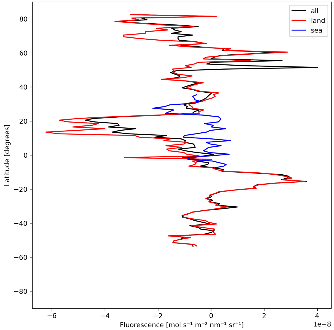
Figure 21: Zonal average of “Fluorescence” for 2023-09-02 to 2023-09-04.
