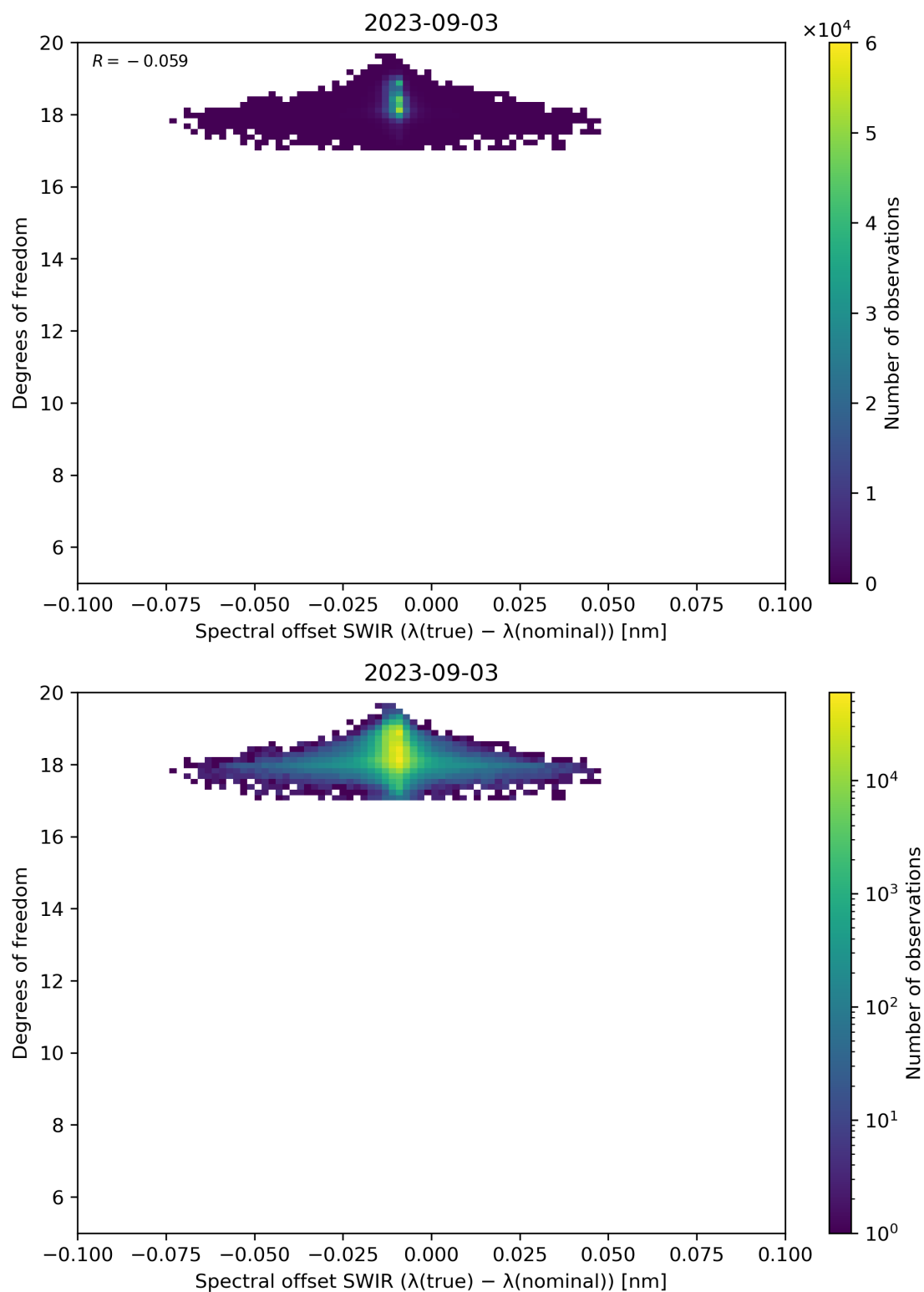
Figure 119: Scatter density plot of “Spectral offset SWIR ( \lambda(\text{true}) - \lambda(\text{nominal}) )” against “Degrees of freedom” for 2023-09-02 to 2023-09-04.
