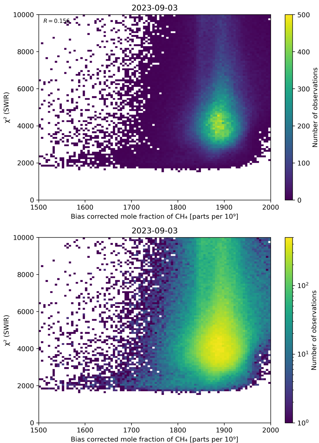
Figure 64: Scatter density plot of “Bias corrected mole fraction of \text{CH}_4 ” against “ \chi^2 (SWIR)” for 2023-09-02 to 2023-09-04.
