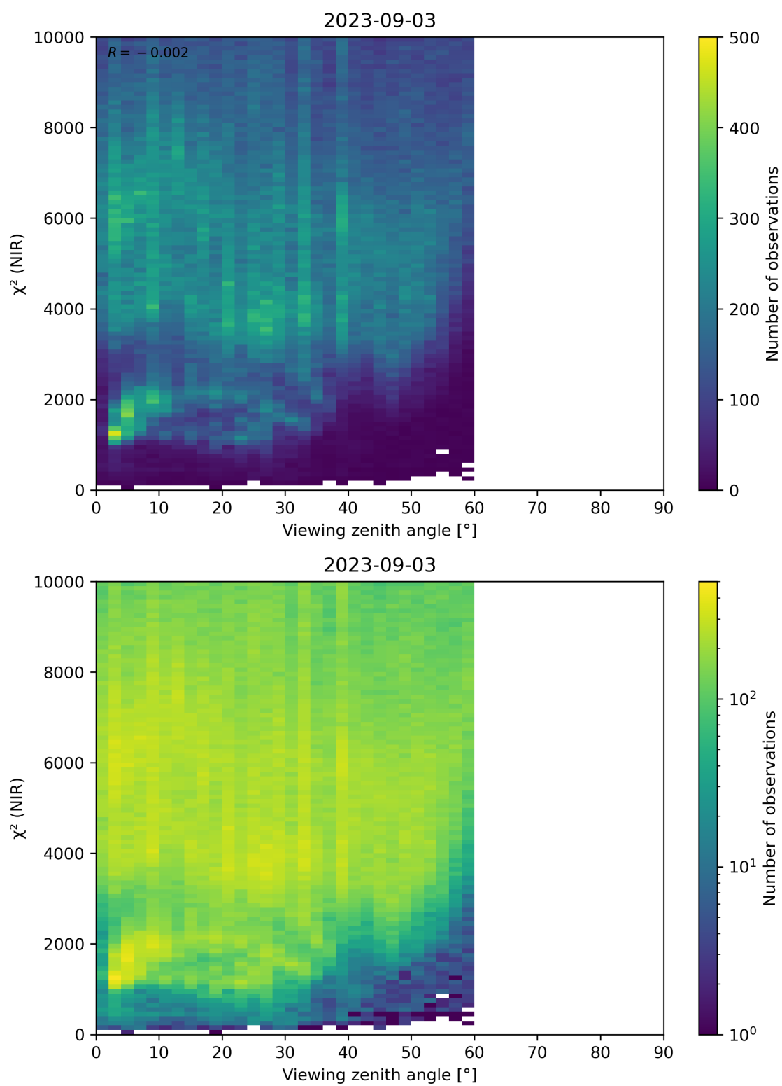
Figure 105: Scatter density plot of “Viewing zenith angle” against “ \chi^2 (NIR)” for 2023-09-02 to 2023-09-04.
