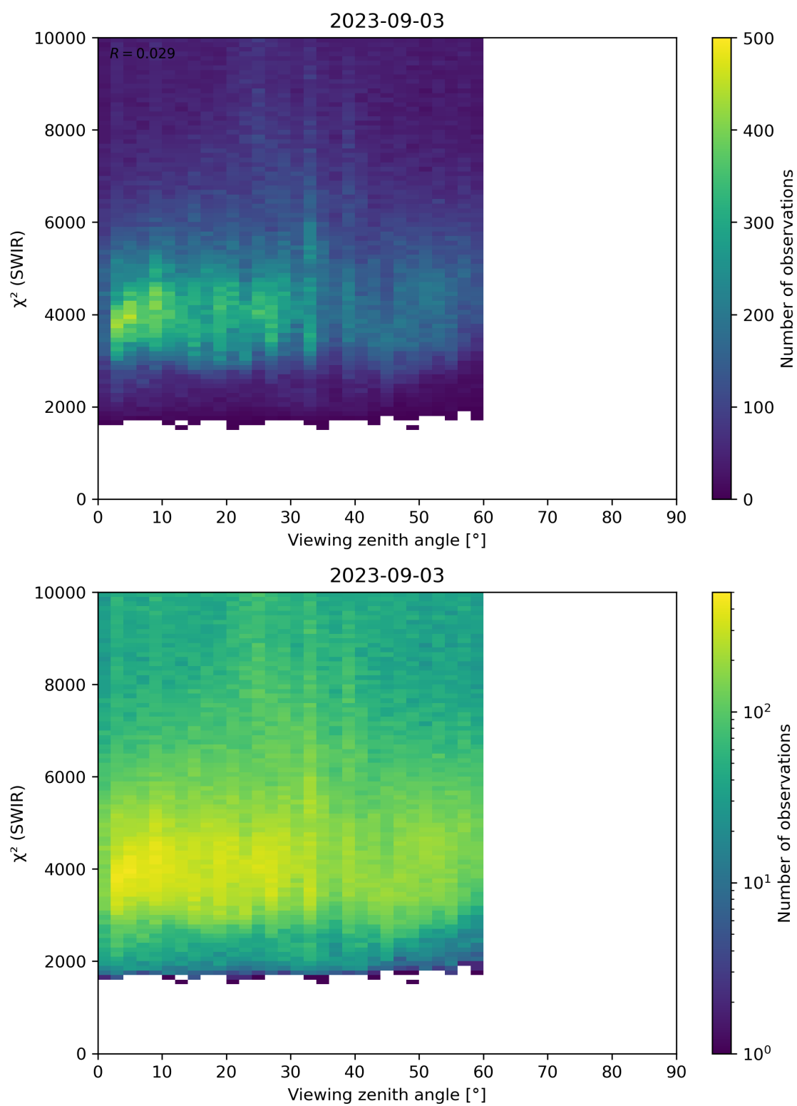
Figure 106: Scatter density plot of “Viewing zenith angle” against “ \chi^2 (SWIR)” for 2023-09-02 to 2023-09-04.
