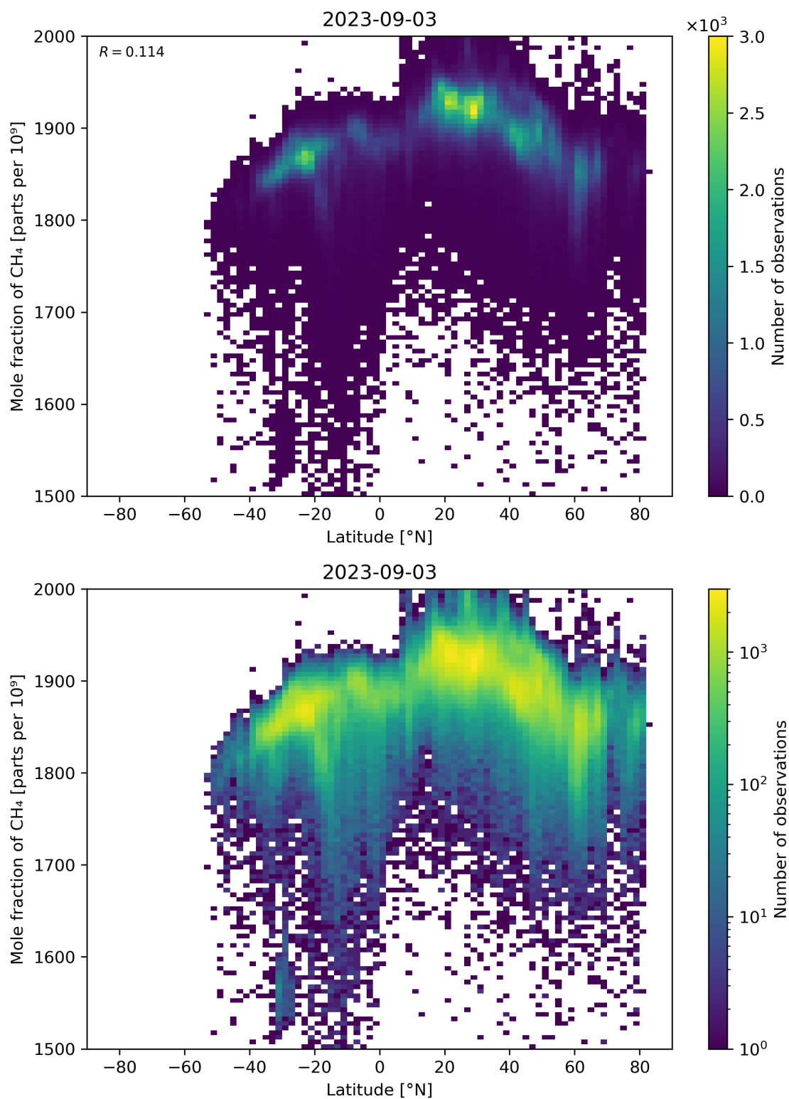
Figure 57: Scatter density plot of “Latitude” against “Mole fraction of \text{CH}_4 ” for 2023-09-02 to 2023-09-04.
