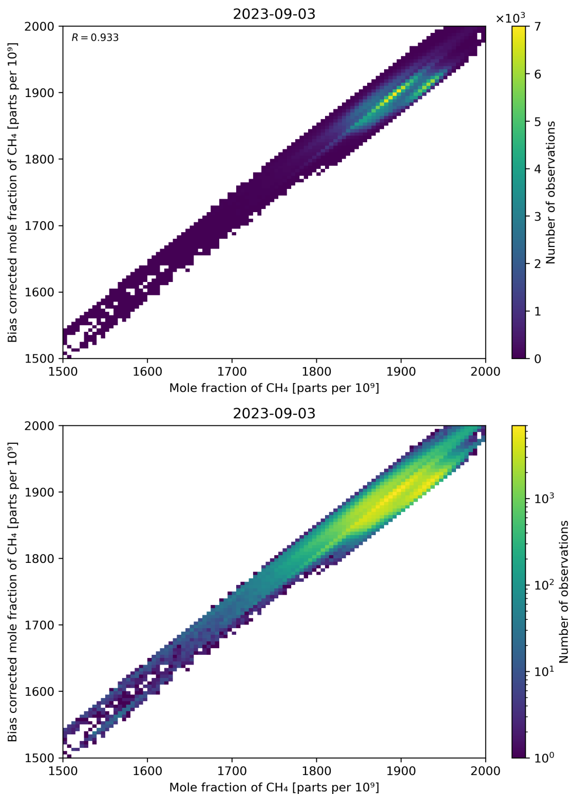
Figure 74: Scatter density plot of “Mole fraction of CH 4 ” against “Bias corrected mole fraction of CH 4 ” for 2023-09-02 to 2023-09-04.
