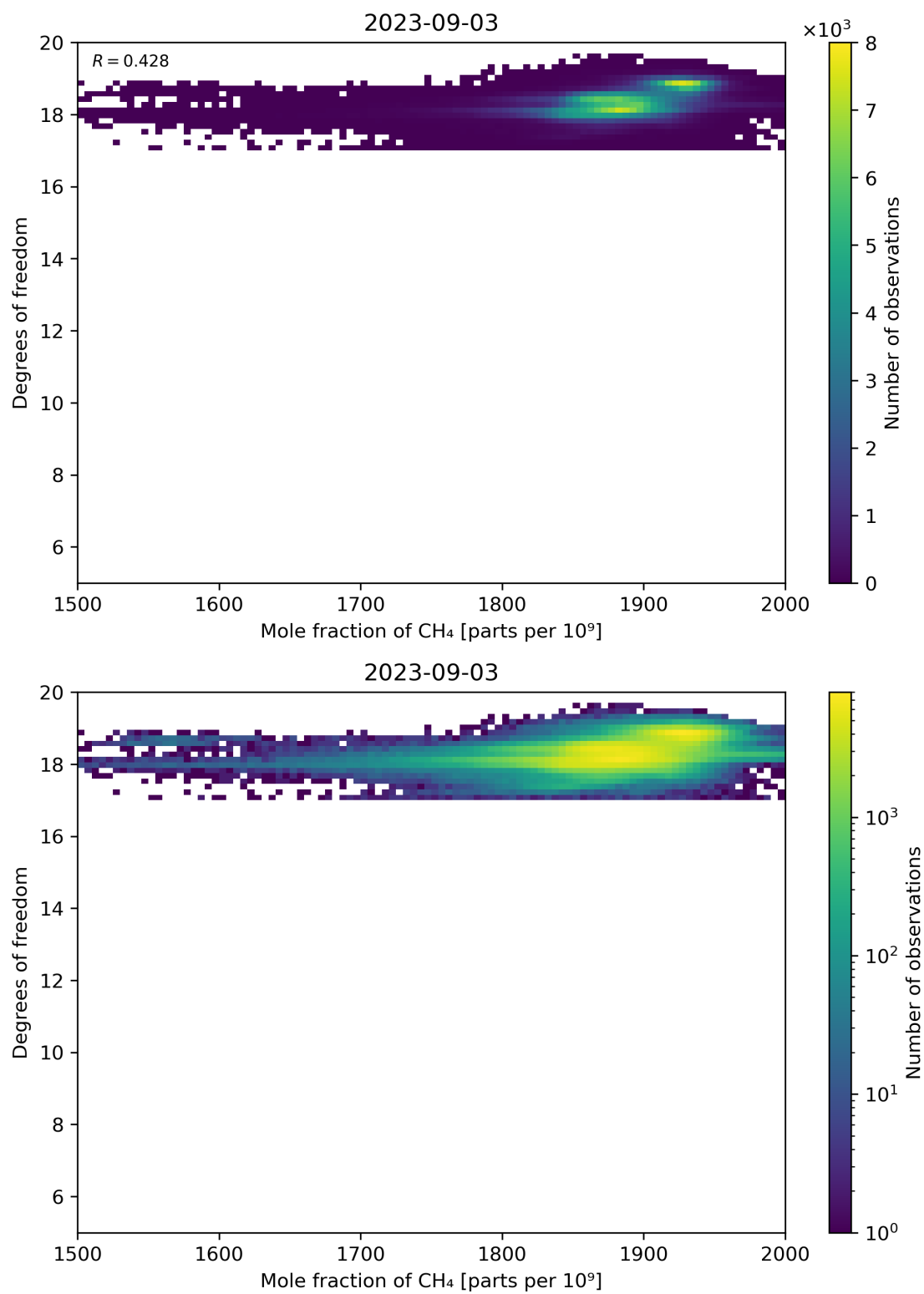
Figure 72: Scatter density plot of “Mole fraction of CH 4 ” against “Degrees of freedom” for 2023-09-02 to 2023-09-04.
