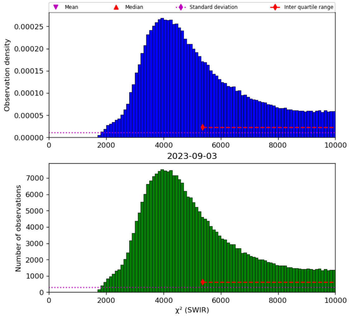
Figure 28: Histogram of “ \chi^2 (SWIR)” for 2023-09-02 to 2023-09-04
