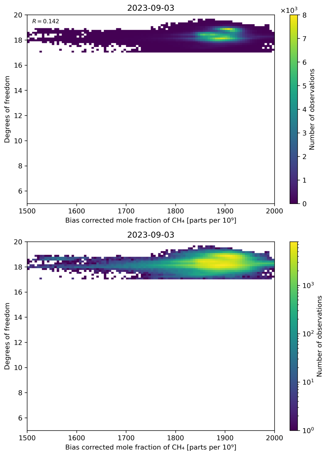
Figure 65: Scatter density plot of “Bias corrected mole fraction of CH 4 ” against “Degrees of freedom” for 2023-09-02 to 2023-09-04.
