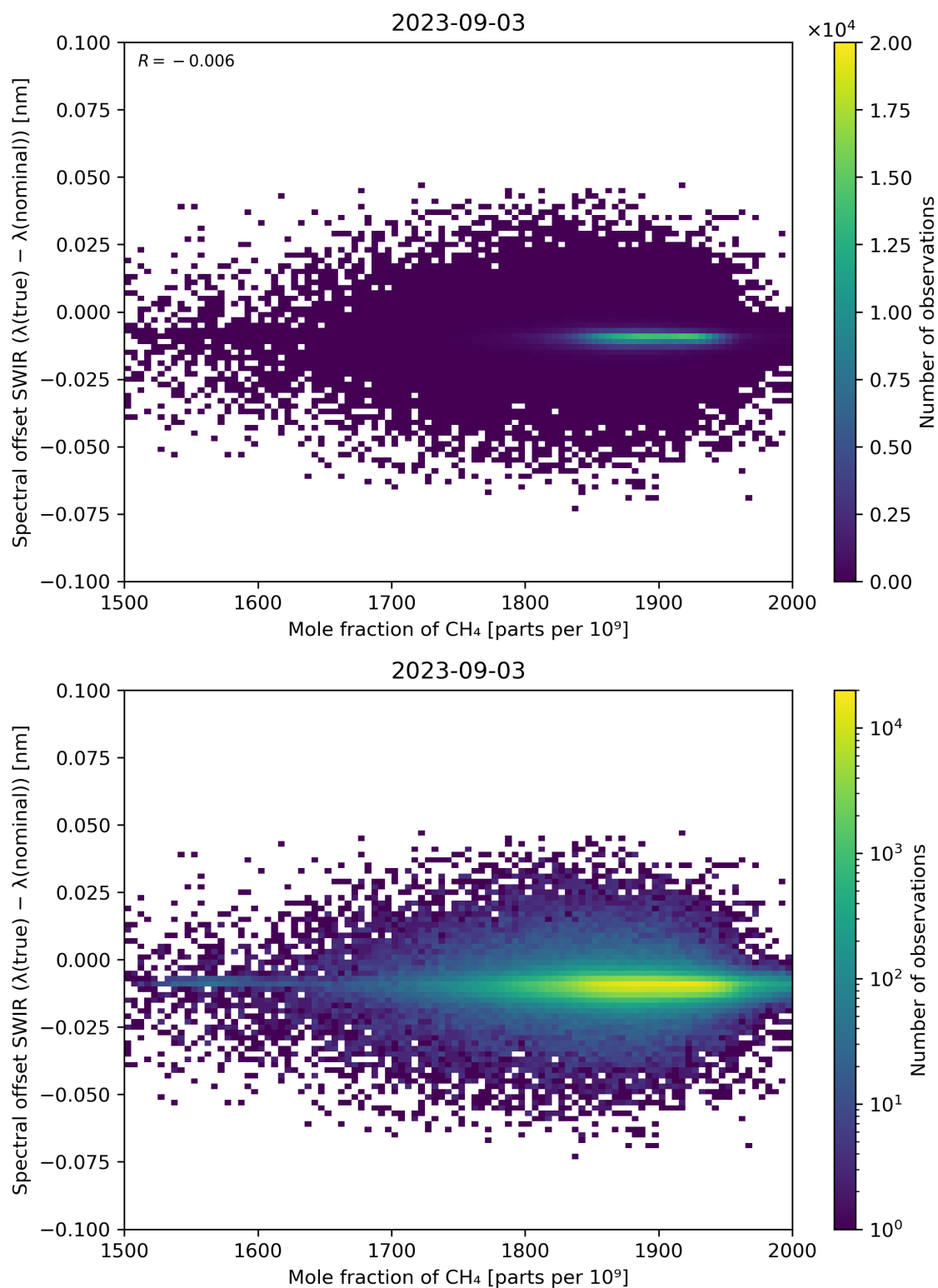
Figure 86: Scatter density plot of “Mole fraction of CH 4 ” against “Spectral offset SWIR ( \lambda(\text{true}) - \lambda(\text{nominal}) )” for 2023-09-02 to 2023-09-04.
