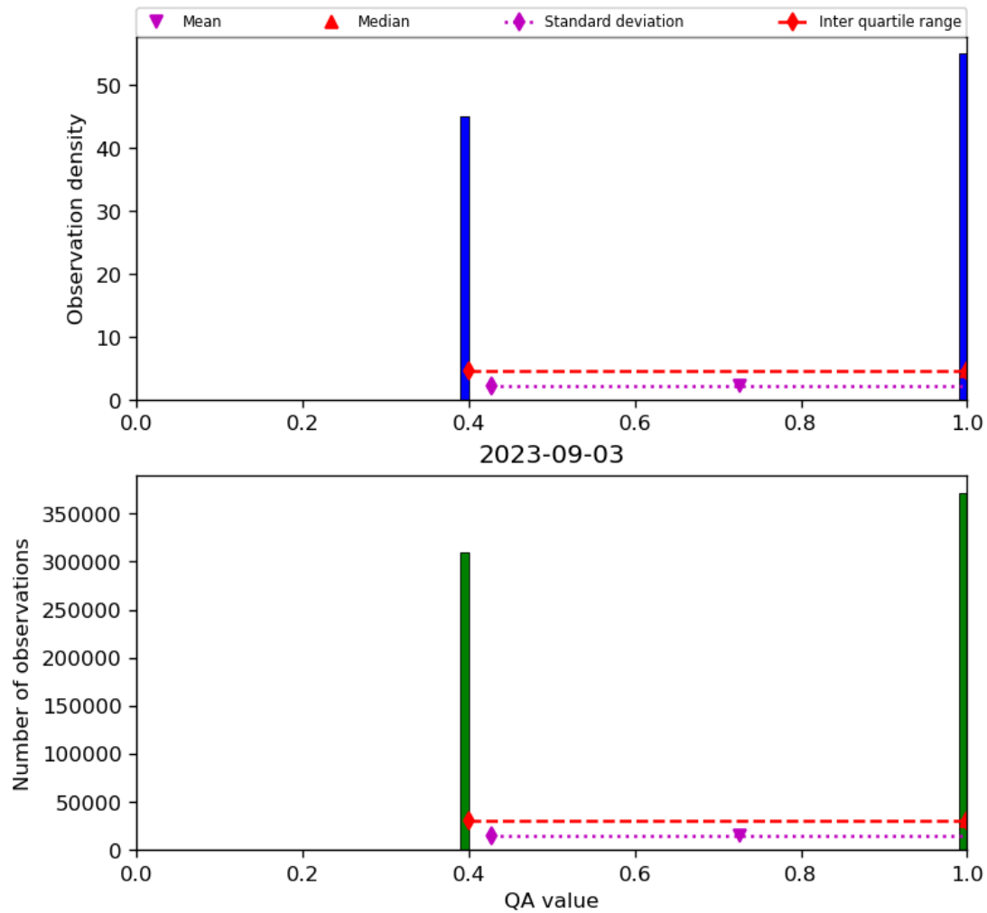
Figure 22: Histogram of “QA value” for 2023-09-02 to 2023-09-04
