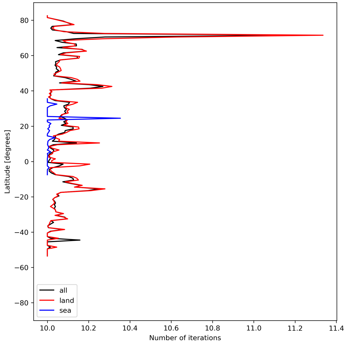
Figure 20: Zonal average of “Number of iterations” for 2023-09-02 to 2023-09-04.
