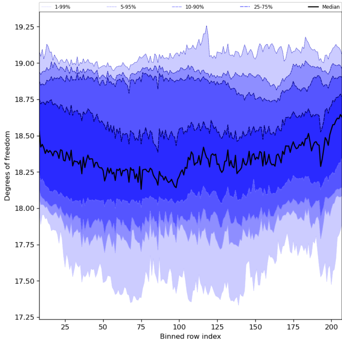
Figure 41: Along track statistics of “Degrees of freedom” for 2023-09-02 to 2023-09-04
