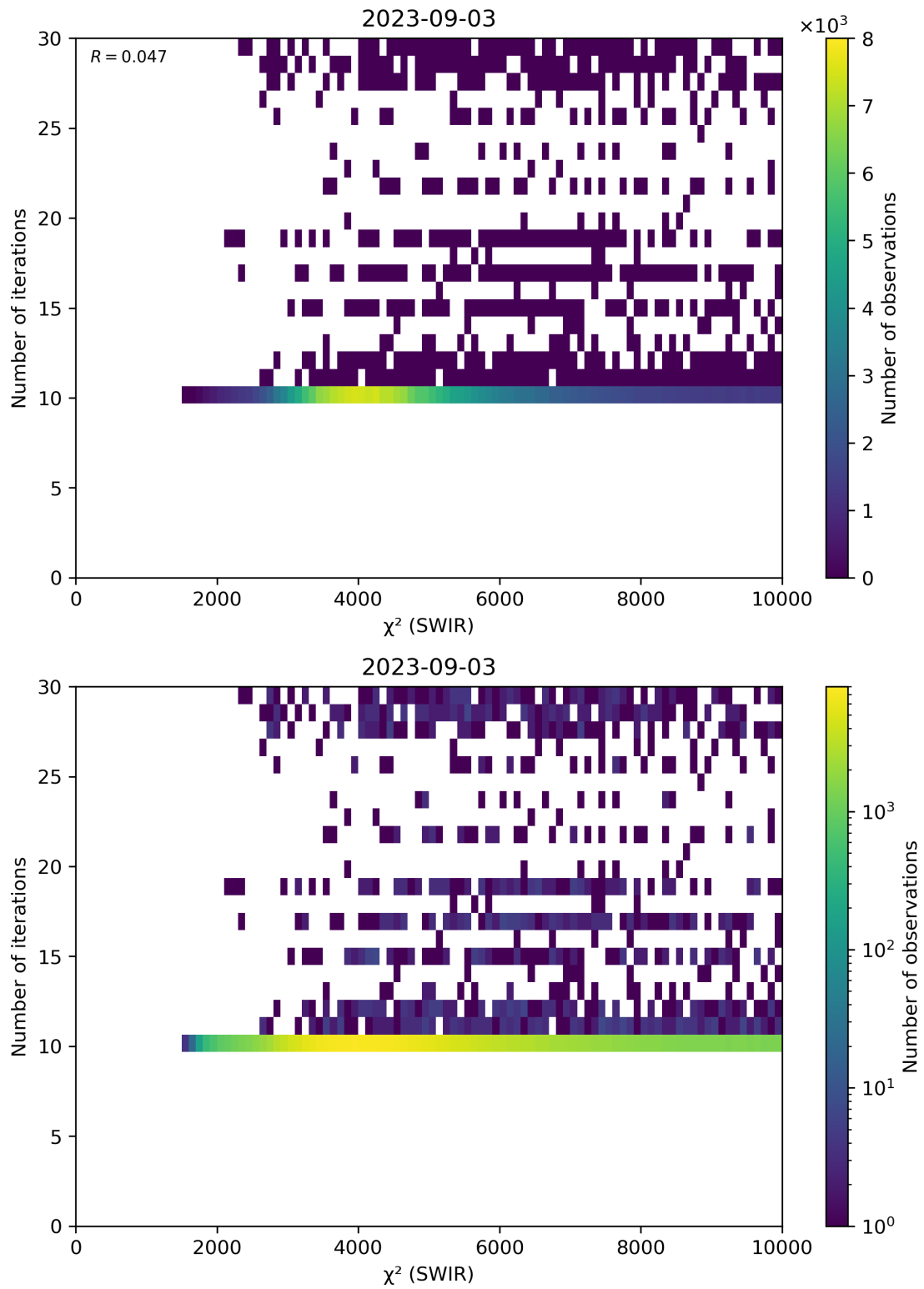
Figure 50: Scatter density plot of “ \chi^2 (SWIR)” against “Number of iterations” for 2023-09-02 to 2023-09-04.
