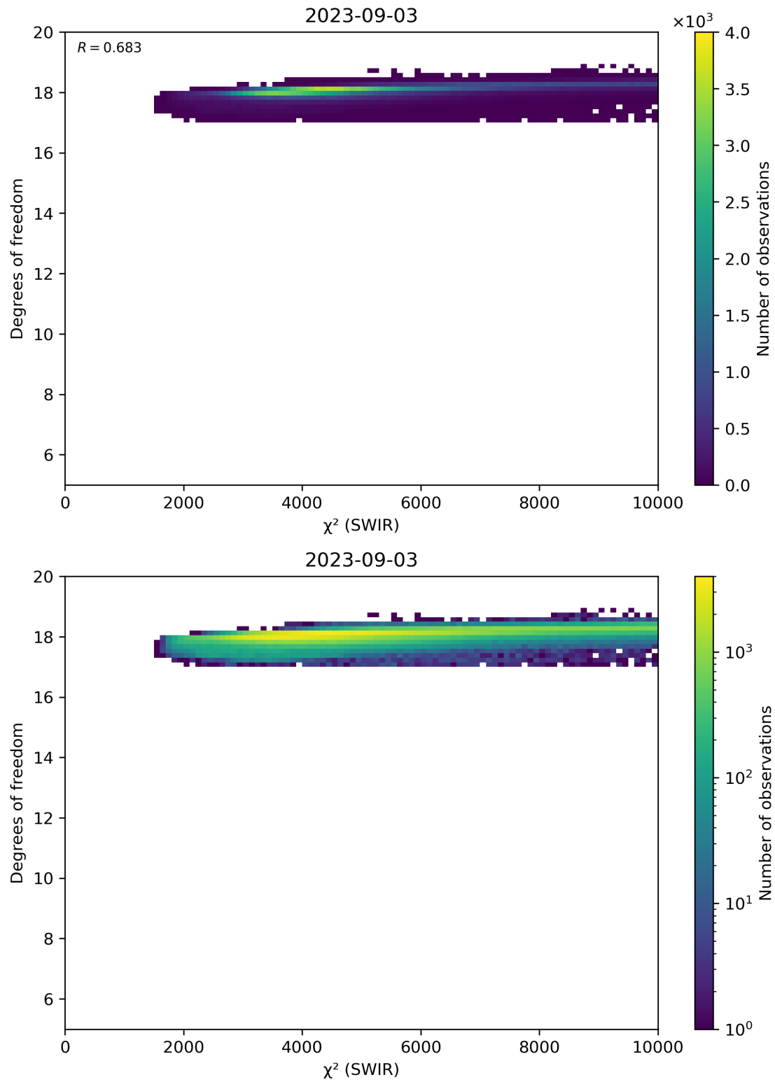
Figure 48: Scatter density plot of “ \chi^2 (SWIR)” against “Degrees of freedom” for 2023-09-02 to 2023-09-04.
