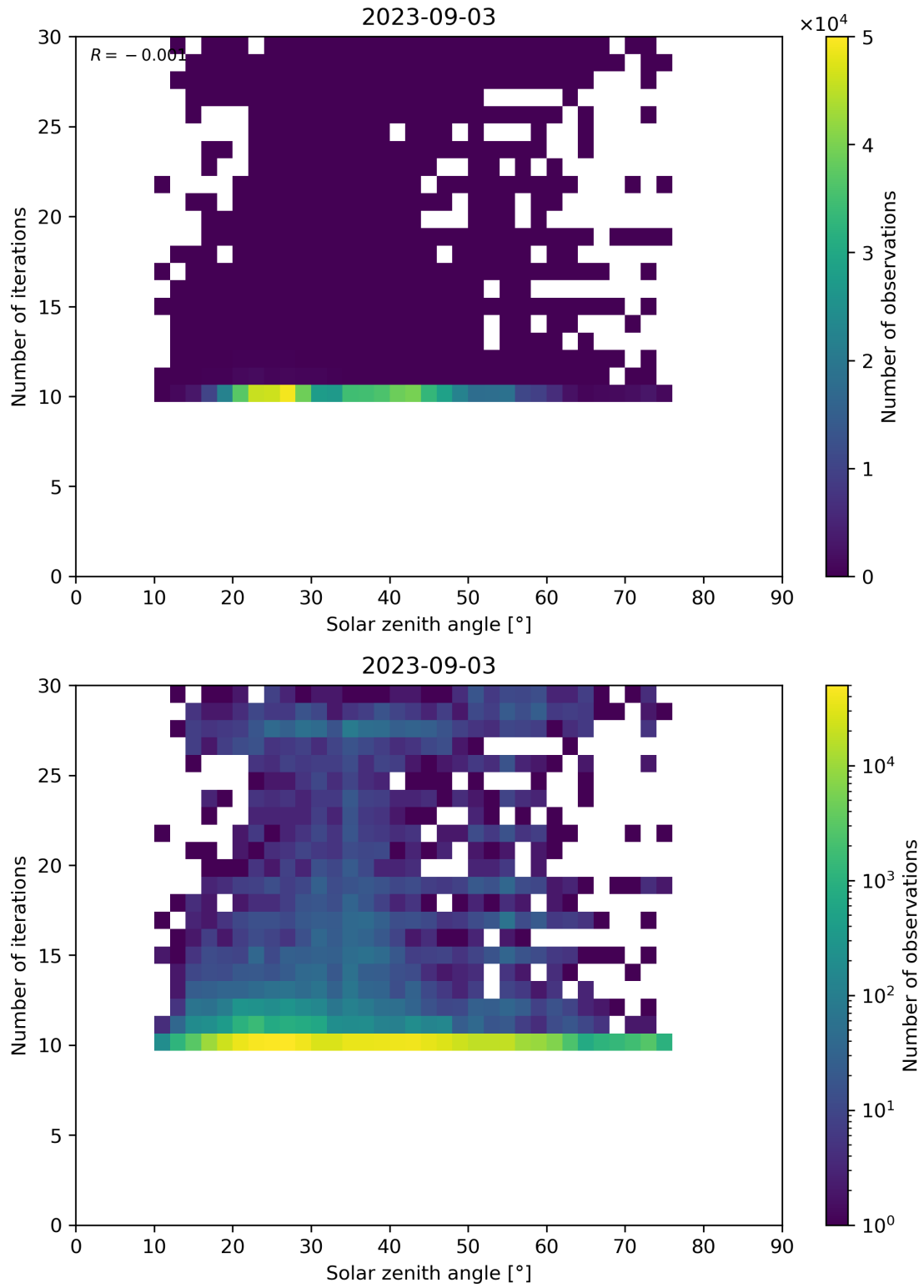
Figure 102: Scatter density plot of “Solar zenith angle” against “Number of iterations” for 2023-09-02 to 2023-09-04.
