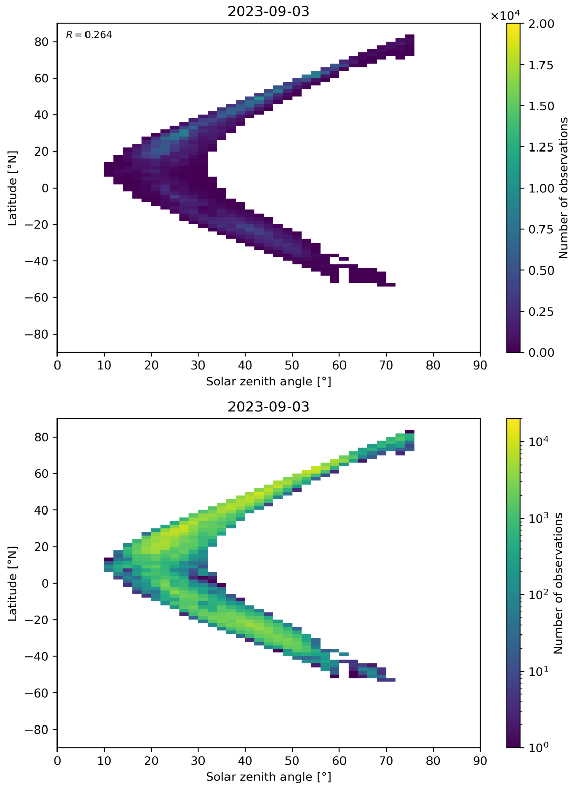
Figure 98: Scatter density plot of “Solar zenith angle” against “Latitude” for 2023-09-02 to 2023-09-04.
