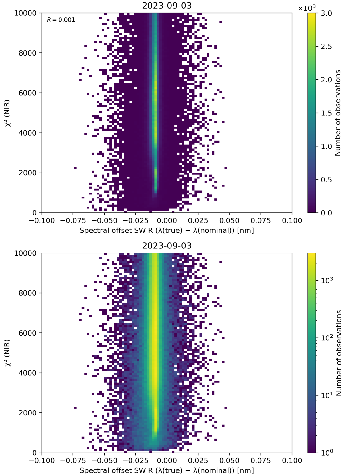
Figure 117: Scatter density plot of “Spectral offset SWIR ( \lambda(\text{true}) - \lambda(\text{nominal}) )” against “ \chi^2 (NIR)” for 2023-09-02 to 2023-09-04.
