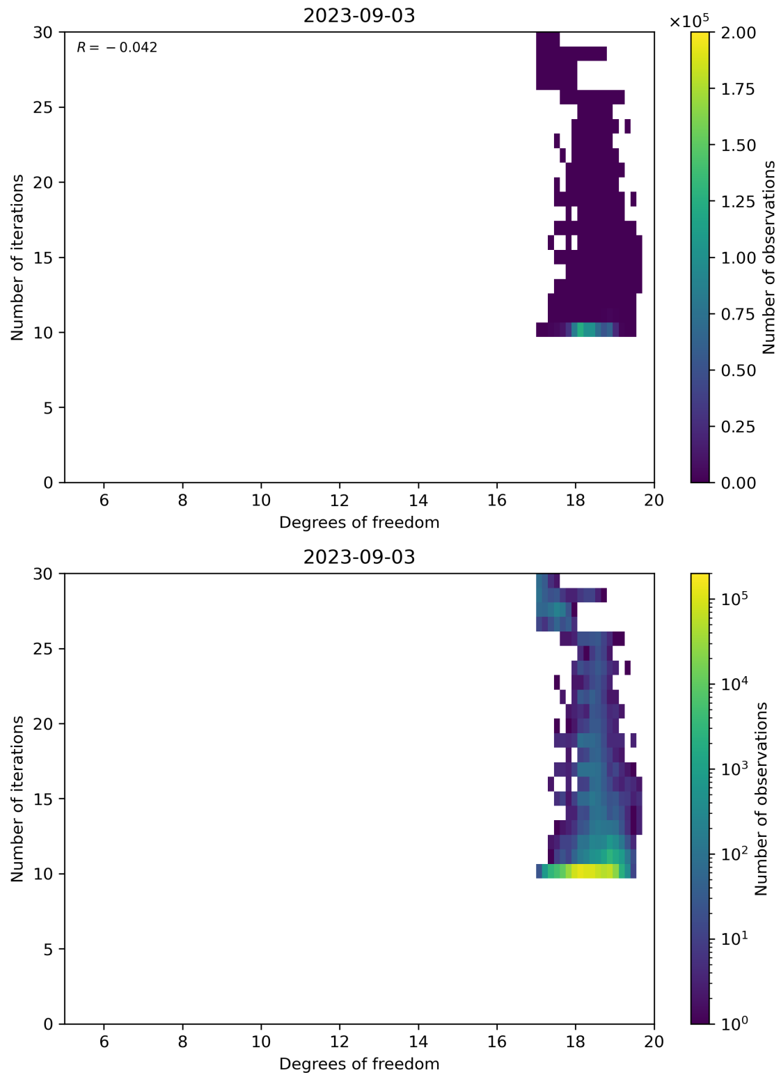
Figure 52: Scatter density plot of “Degrees of freedom” against “Number of iterations” for 2023-09-02 to 2023-09-04.
