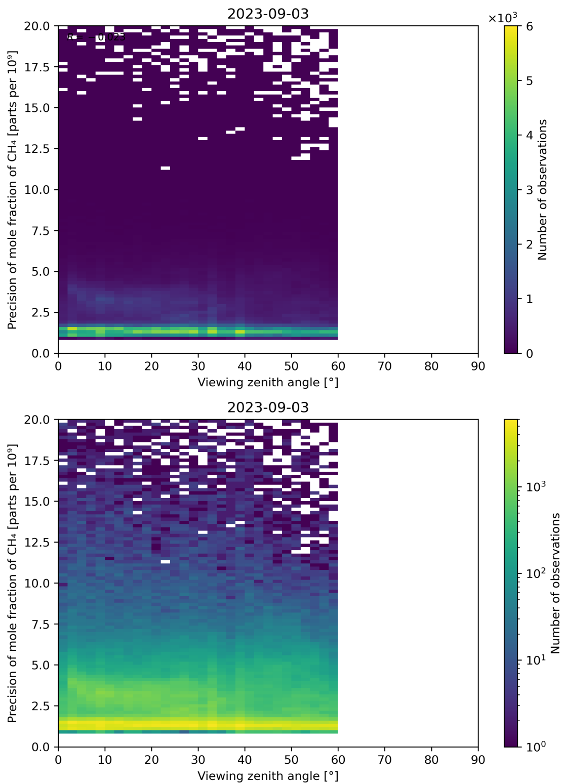
Figure 112: Scatter density plot of “Viewing zenith angle” against “Precision of mole fraction of CH 4 ” for 2023-09-02 to 2023-09-04.
