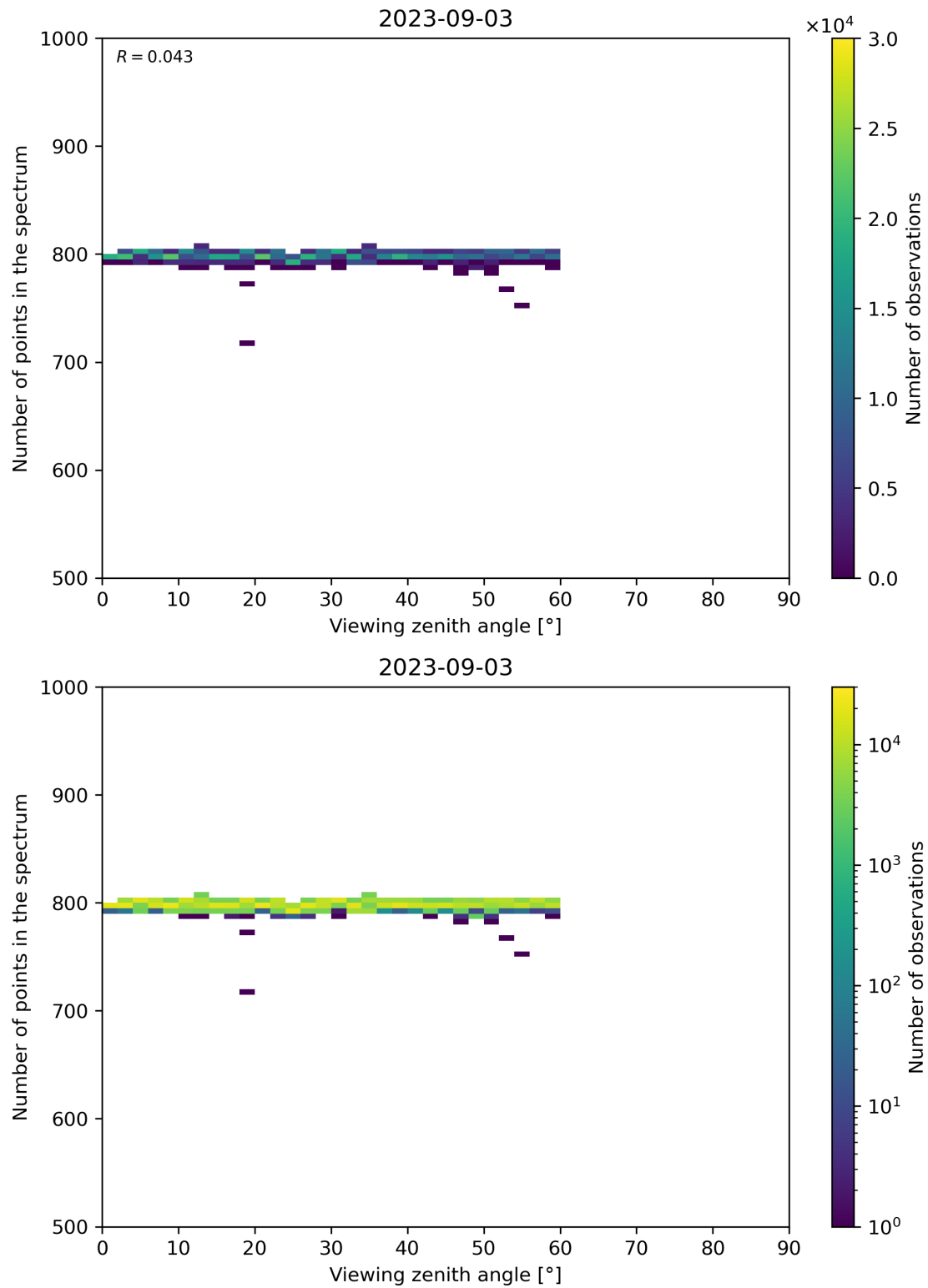
Figure 114: Scatter density plot of “Viewing zenith angle” against “Number of points in the spectrum” for 2023-09-02 to 2023-09-04.
