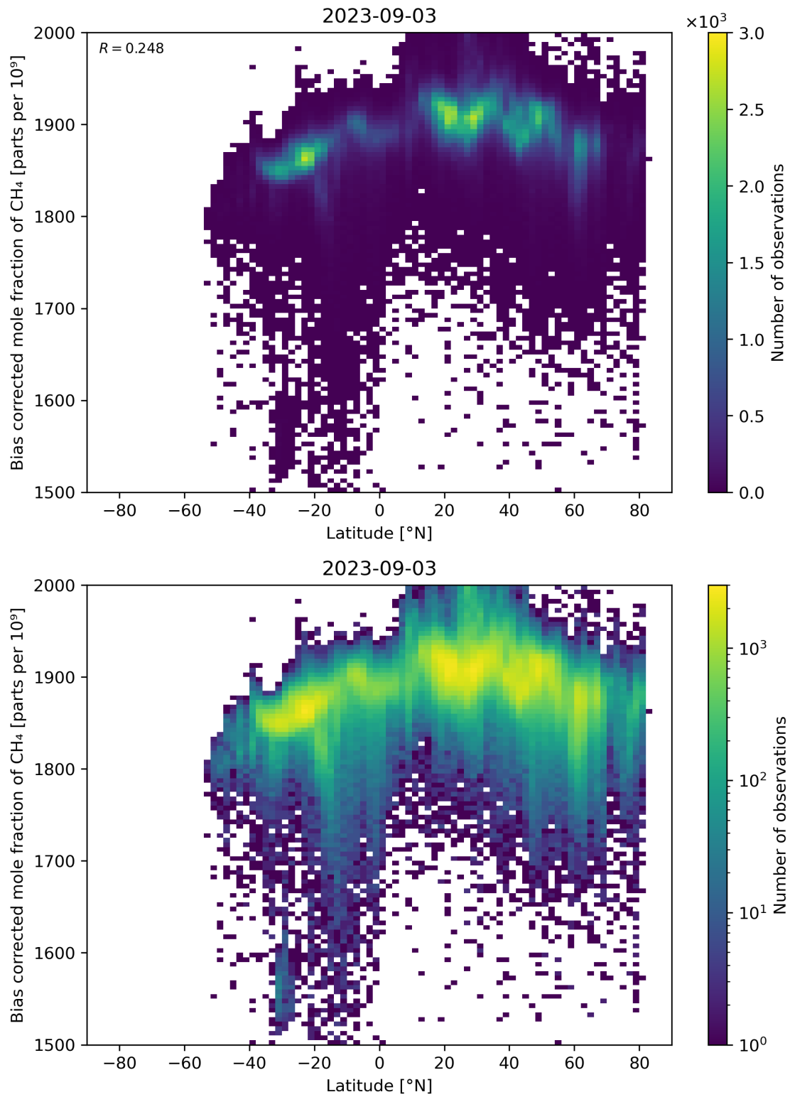
Figure 58: Scatter density plot of “Latitude” against “Bias corrected mole fraction of CH 4 ” for 2023-09-02 to 2023-09-04.
