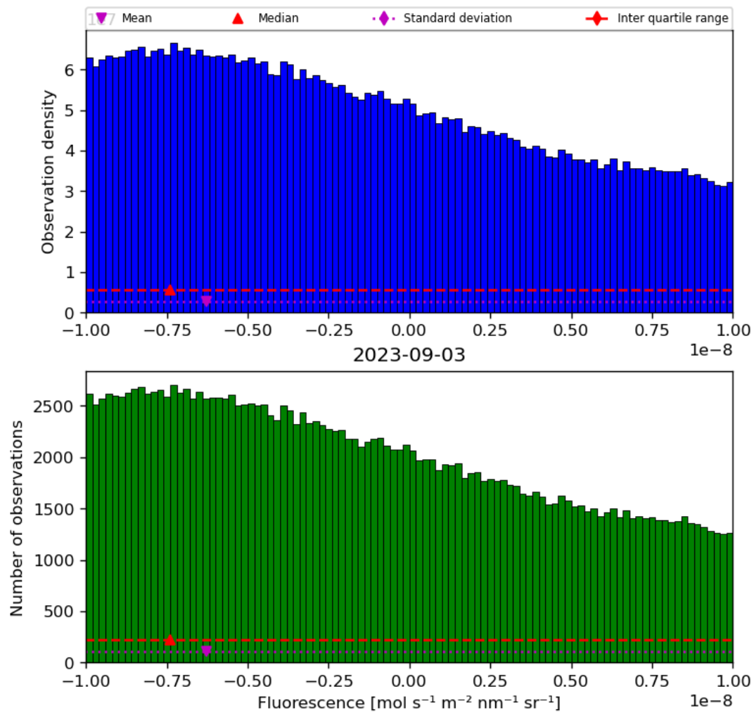
Figure 32: Histogram of “Fluorescence” for 2023-09-02 to 2023-09-04
