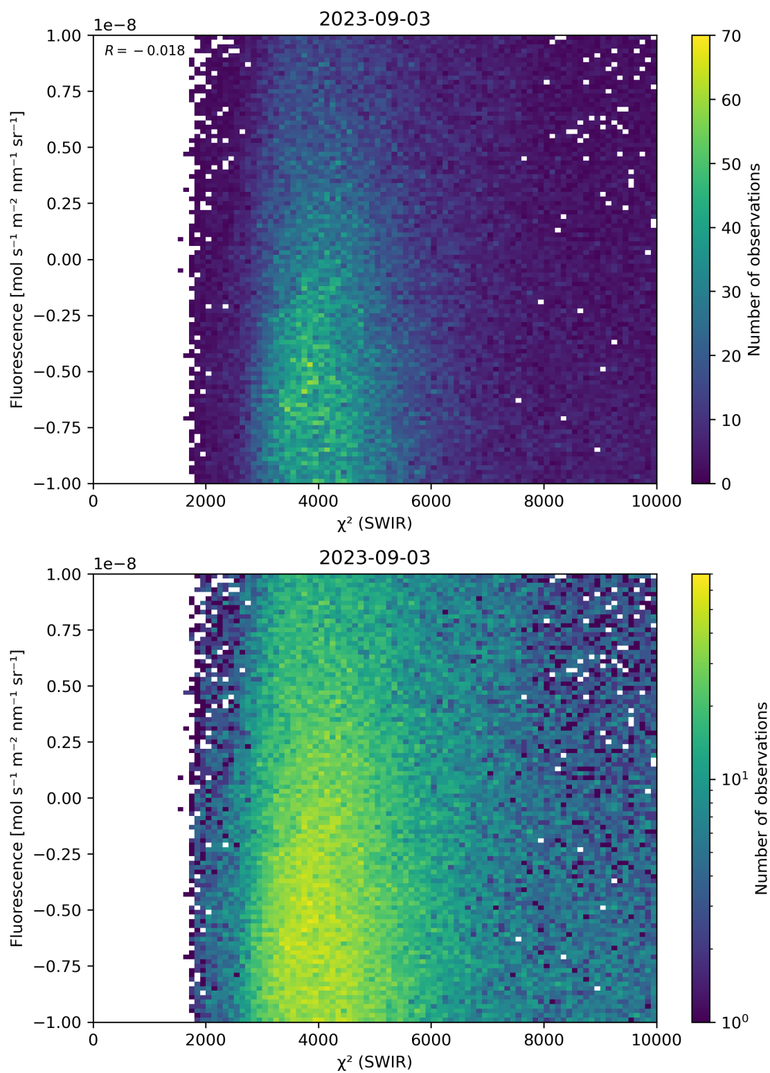
Figure 49: Scatter density plot of “ \chi^2 (SWIR)” against “Fluorescence” for 2023-09-02 to 2023-09-04.
