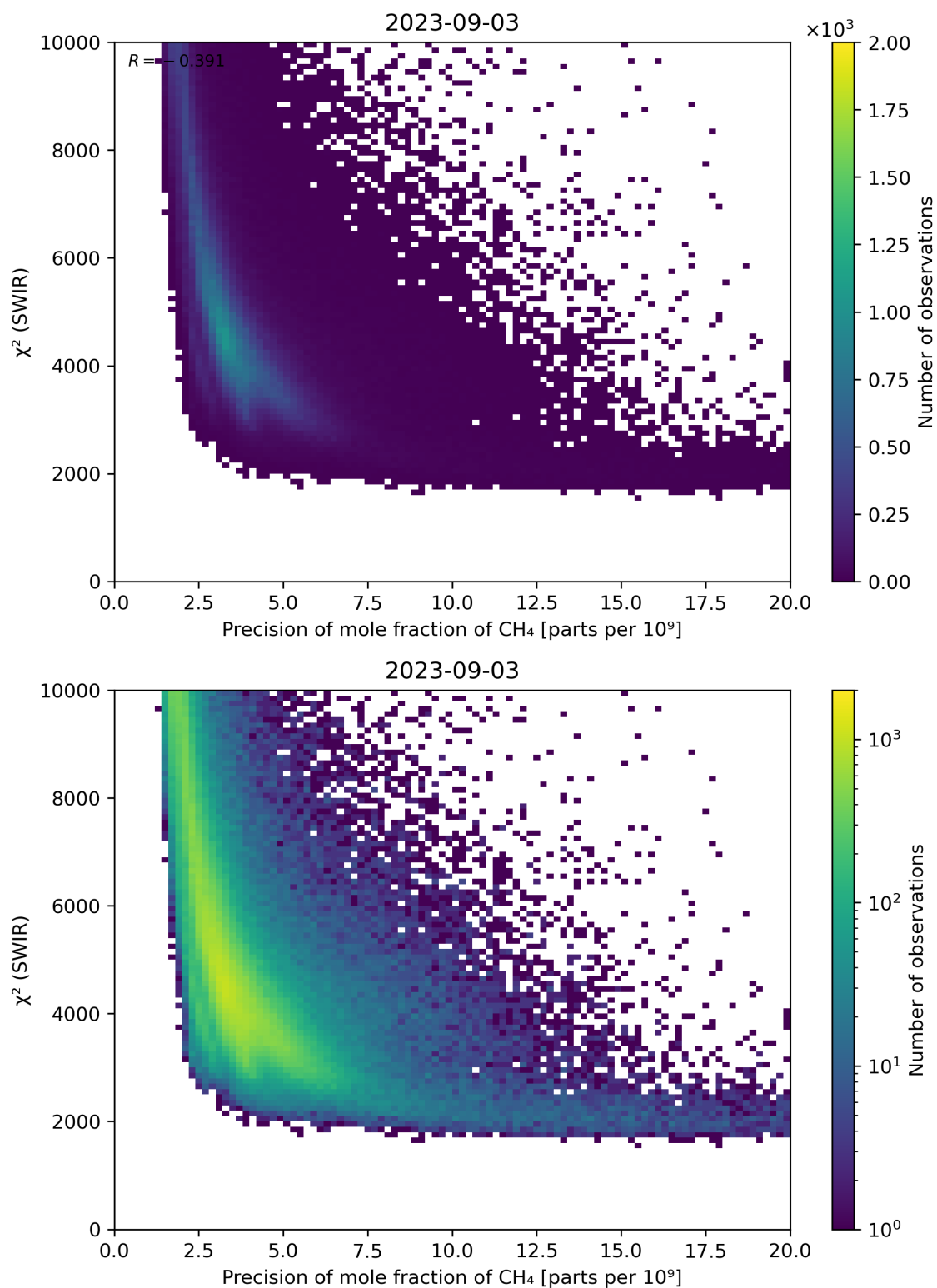
Figure 79: Scatter density plot of “Precision of mole fraction of \text{CH}_4 ” against “ \chi^2 (SWIR)” for 2023-09-02 to 2023-09-04.
