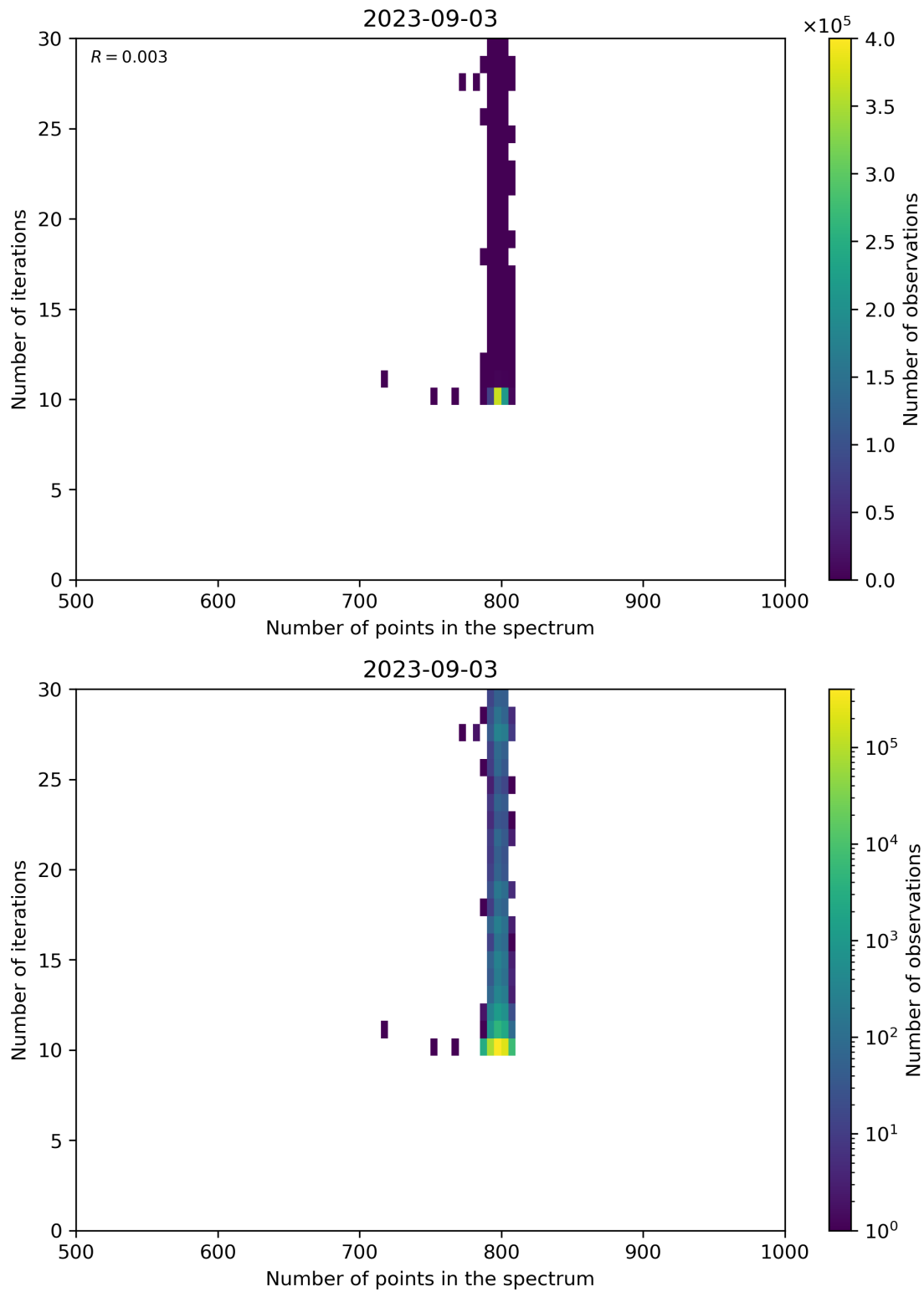
Figure 92: Scatter density plot of “Number of points in the spectrum” against “Number of iterations” for 2023-09-02 to 2023-09-04.
