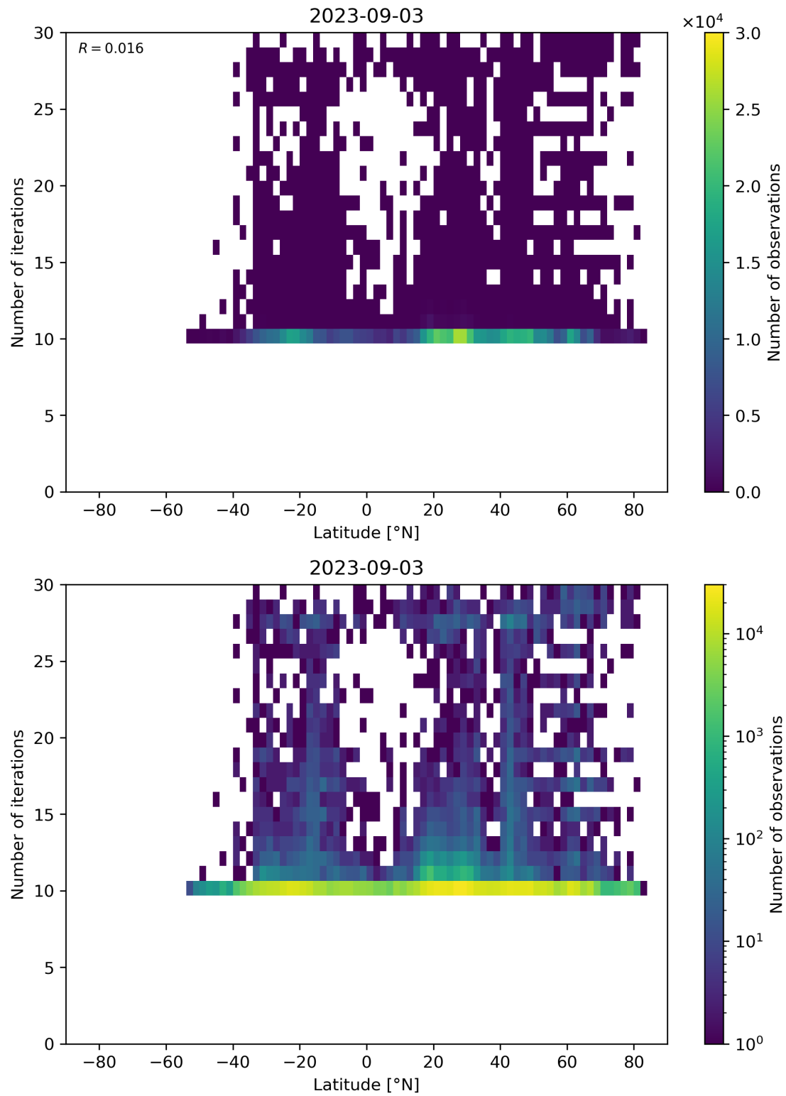
Figure 60: Scatter density plot of “Latitude” against “Number of iterations” for 2023-09-02 to 2023-09-04.
