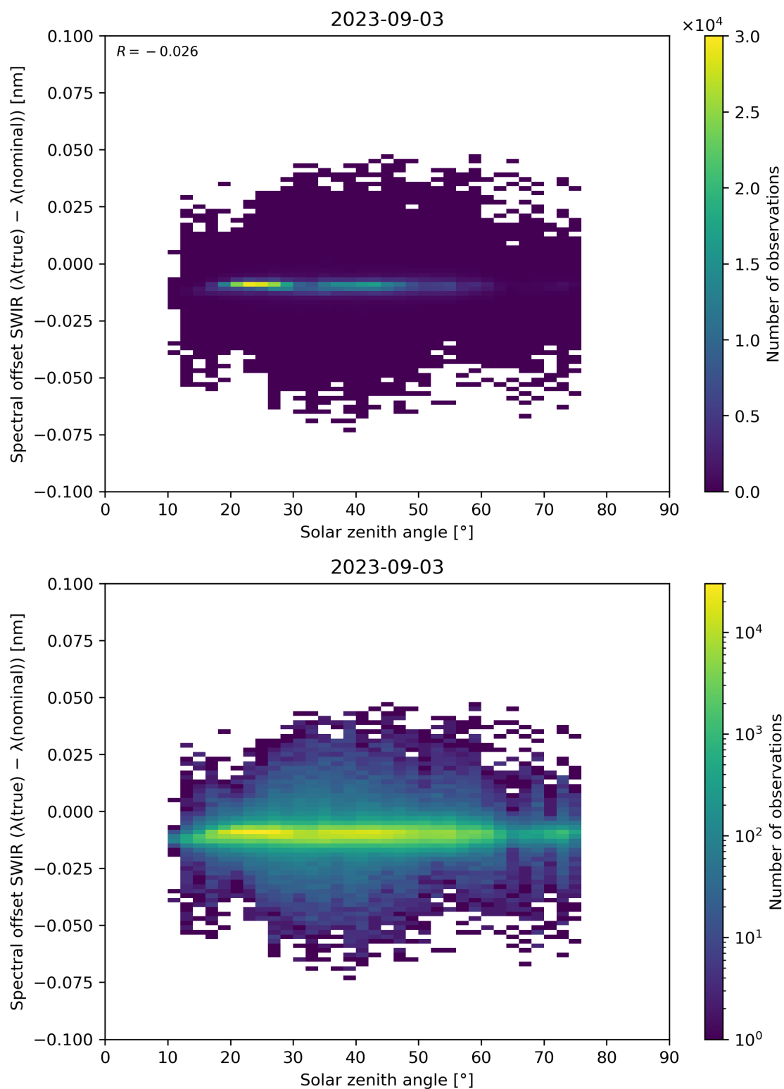
Figure 104: Scatter density plot of “Solar zenith angle” against “Spectral offset SWIR ( \lambda(\text{true}) - \lambda(\text{nominal}) )” for 2023-09-02 to 2023-09-04.
