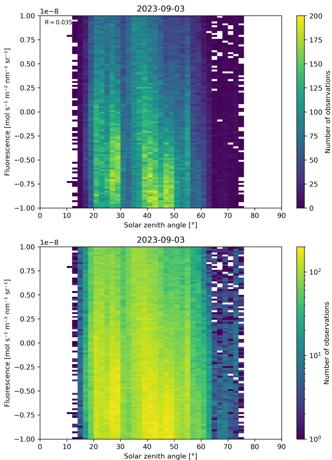
Figure 97: Scatter density plot of “Solar zenith angle” against “Fluorescence” for 2023-09-02 to 2023-09-04.
