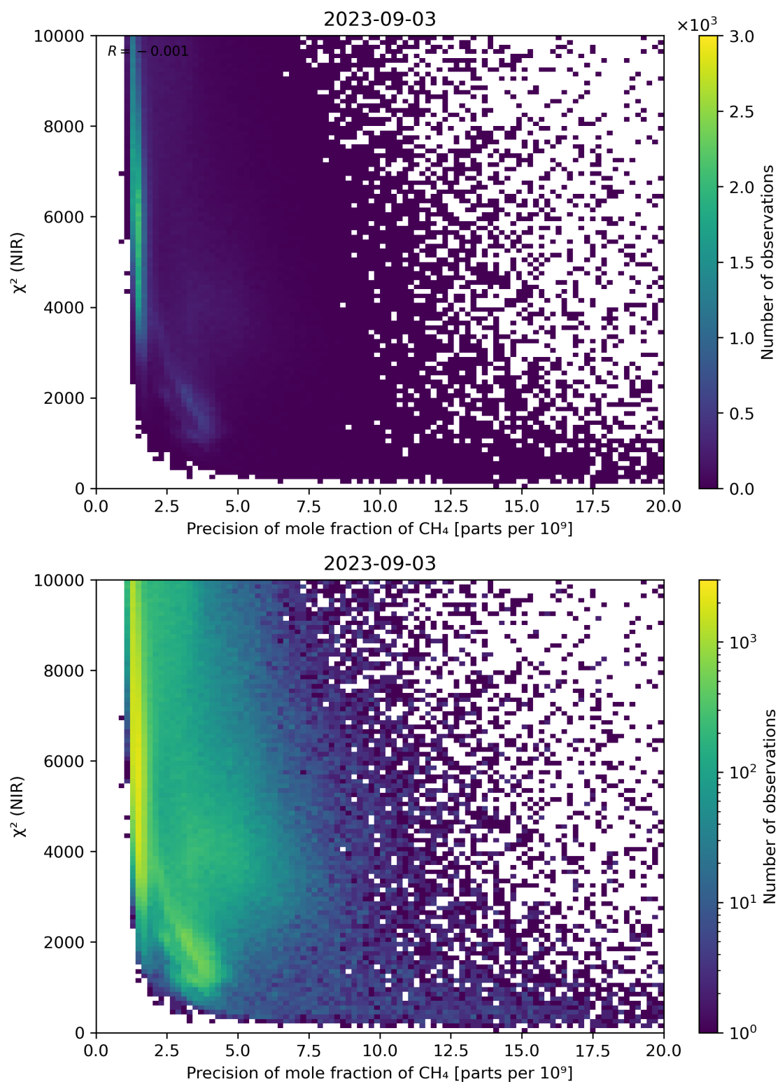
Figure 78: Scatter density plot of “Precision of mole fraction of CH 4 ” against “ \chi^2 (NIR)” for 2023-09-02 to 2023-09-04.
