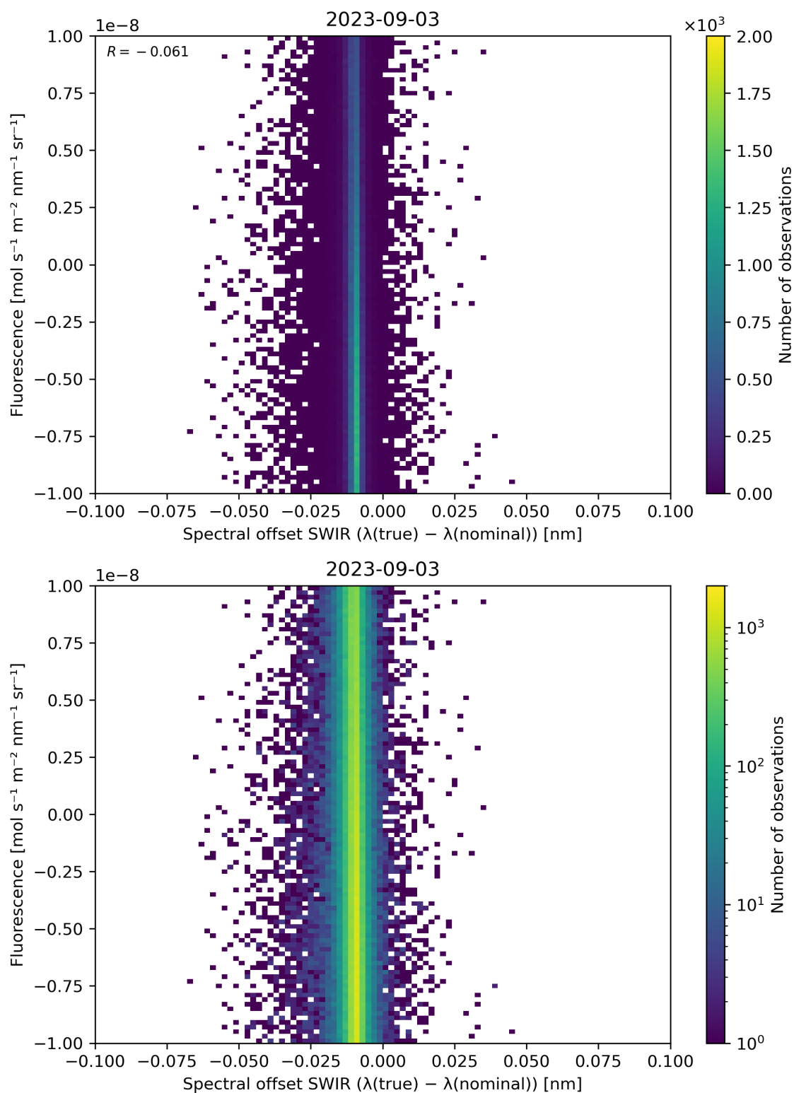
Figure 120: Scatter density plot of “Spectral offset SWIR ( \lambda(\text{true}) - \lambda(\text{nominal}) )” against “Fluorescence” for 2023-09-02 to 2023-09-04.
