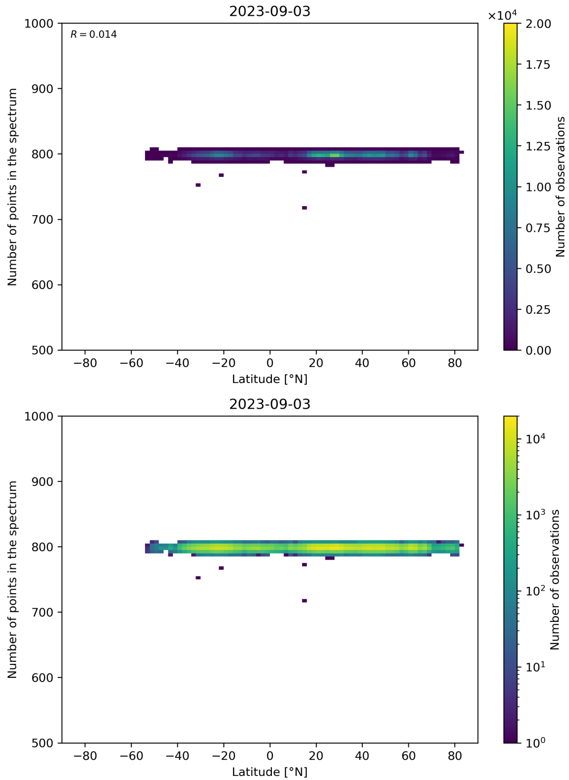
Figure 61: Scatter density plot of “Latitude” against “Number of points in the spectrum” for 2023-09-02 to 2023-09-04.
