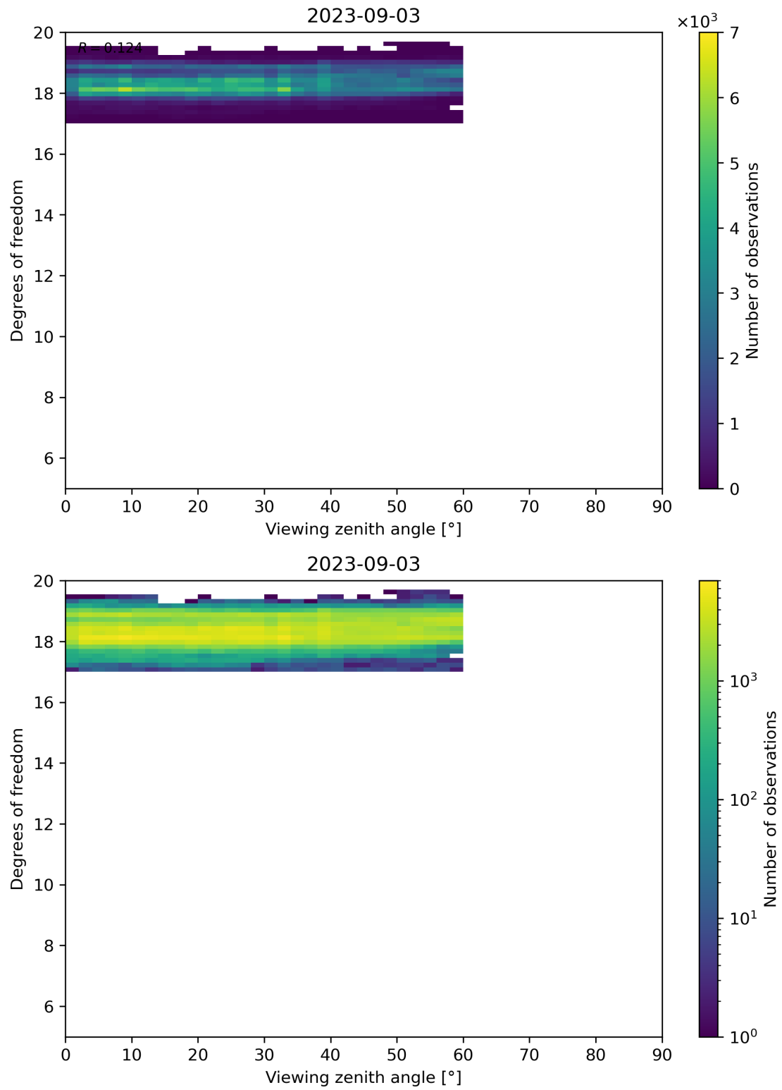
Figure 107: Scatter density plot of “Viewing zenith angle” against “Degrees of freedom” for 2023-09-02 to 2023-09-04.
