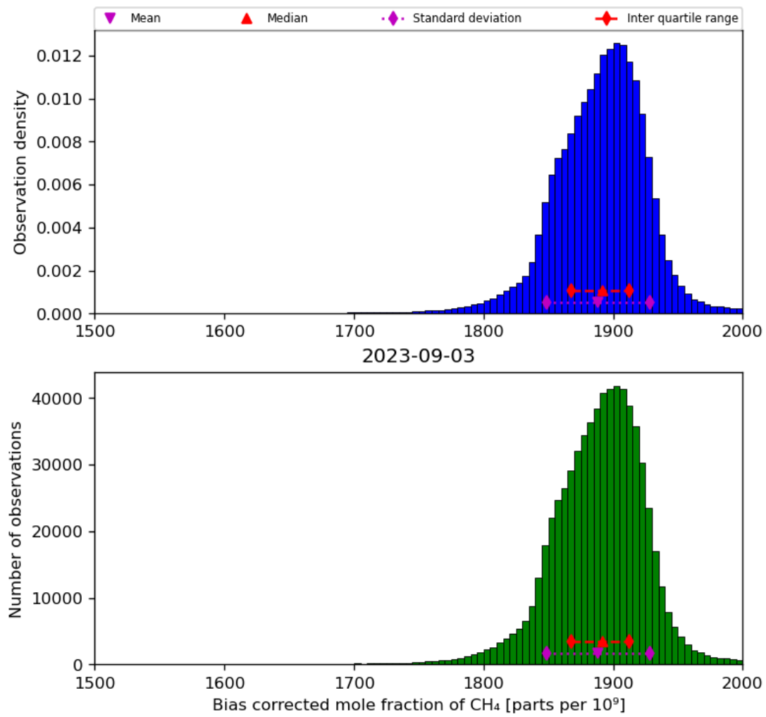
Figure 25: Histogram of “Bias corrected mole fraction of CH 4 ” for 2023-09-02 to 2023-09-04
