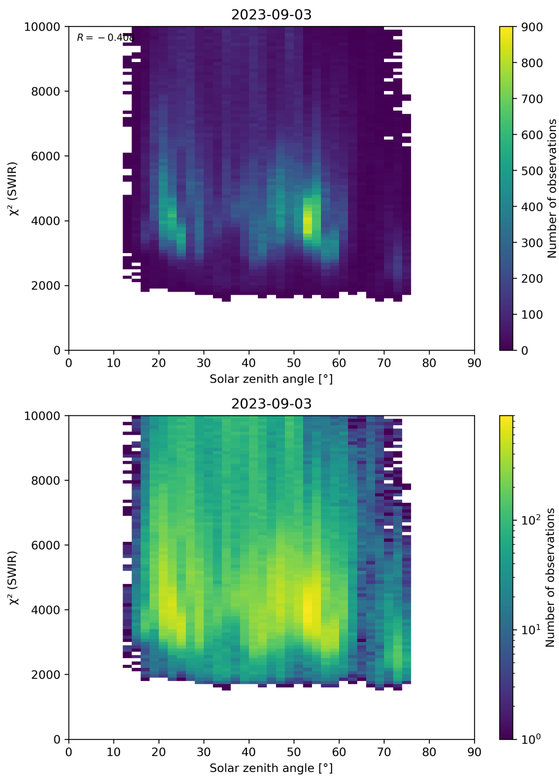
Figure 95: Scatter density plot of “Solar zenith angle” against “ \chi^2 (SWIR)” for 2023-09-02 to 2023-09-04.
