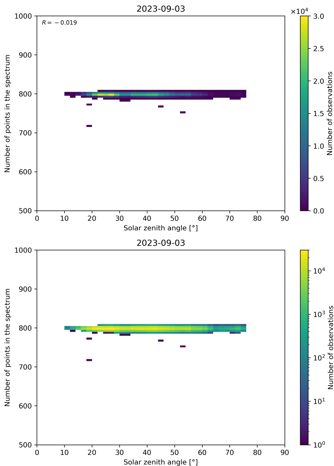
Figure 103: Scatter density plot of “Solar zenith angle” against “Number of points in the spectrum” for 2023-09-02 to 2023-09-04.
