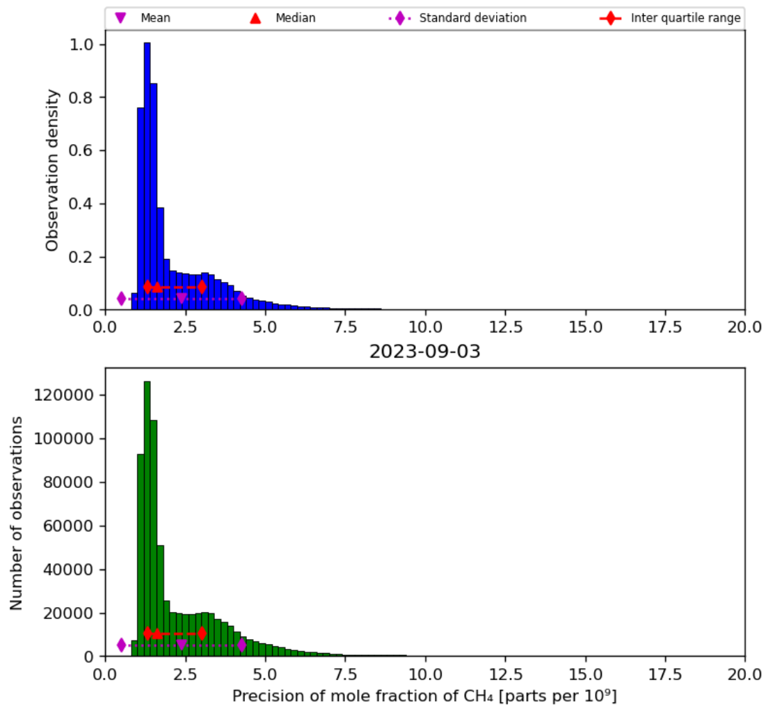
Figure 24: Histogram of “Precision of mole fraction of CH 4 ” for 2023-09-02 to 2023-09-04
