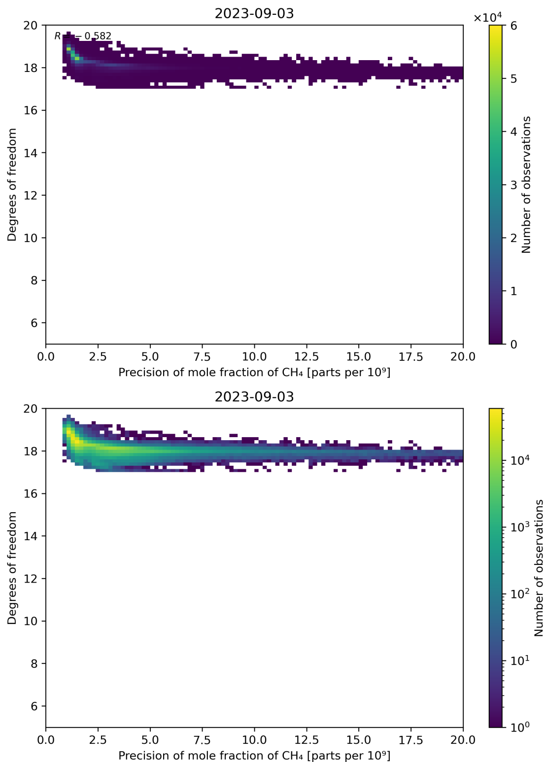
Figure 80: Scatter density plot of “Precision of mole fraction of CH 4 ” against “Degrees of freedom” for 2023-09-02 to 2023-09-04.
