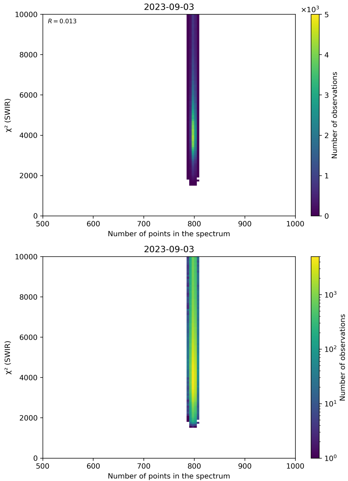
Figure 89: Scatter density plot of “Number of points in the spectrum” against “ \chi^2 (SWIR)” for 2023-09-02 to 2023-09-04.
