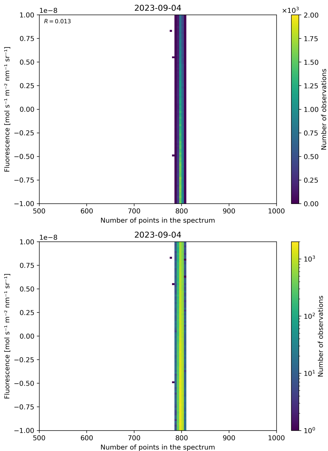
Figure 91: Scatter density plot of “Number of points in the spectrum” against “Fluorescence” for 2023-09-04 to 2023-09-05.
