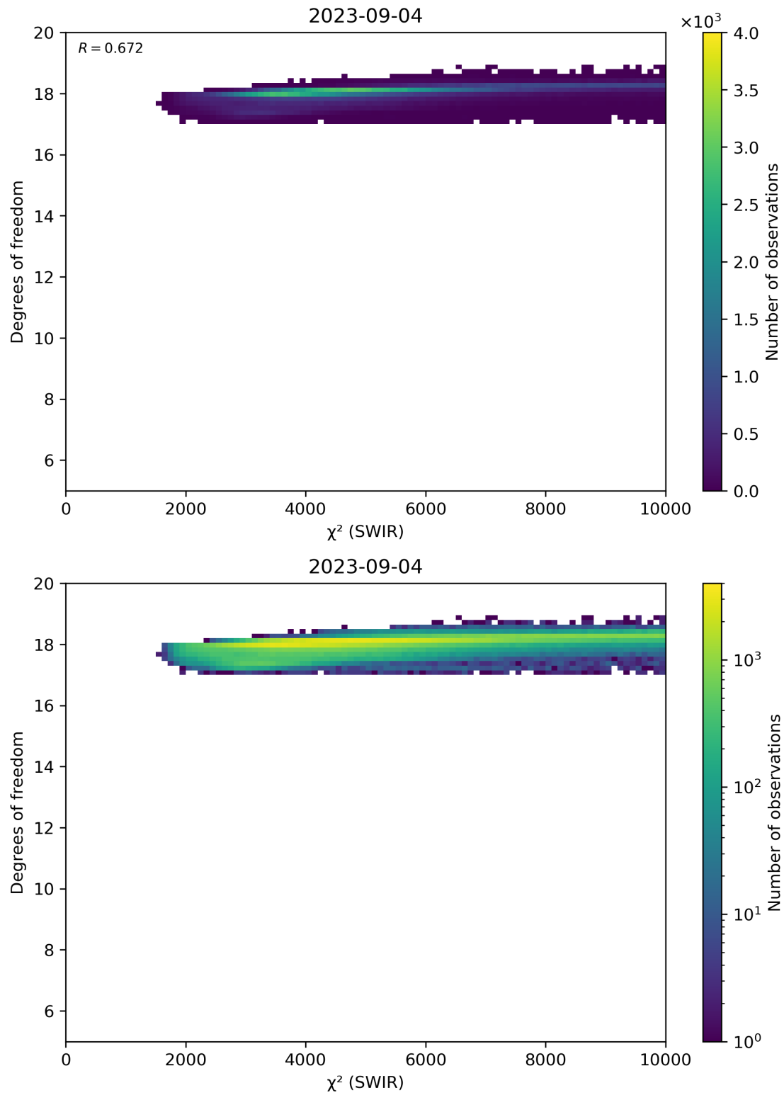
Figure 48: Scatter density plot of “ \chi^2 (SWIR)” against “Degrees of freedom” for 2023-09-04 to 2023-09-05.
