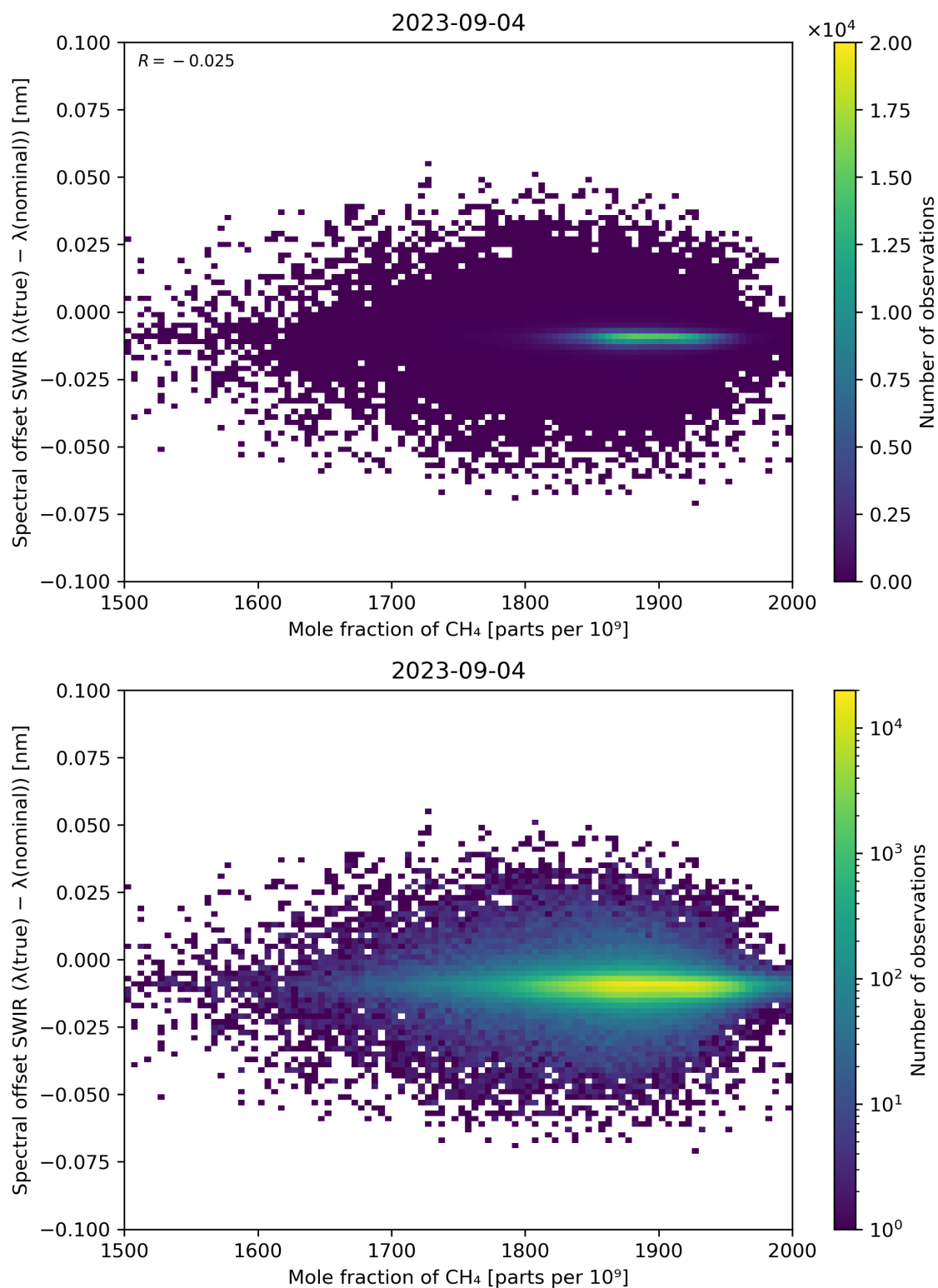
Figure 86: Scatter density plot of “Mole fraction of CH 4 ” against “Spectral offset SWIR ( \lambda(\text{true}) - \lambda(\text{nominal}) )” for 2023-09-04 to 2023-09-05.
