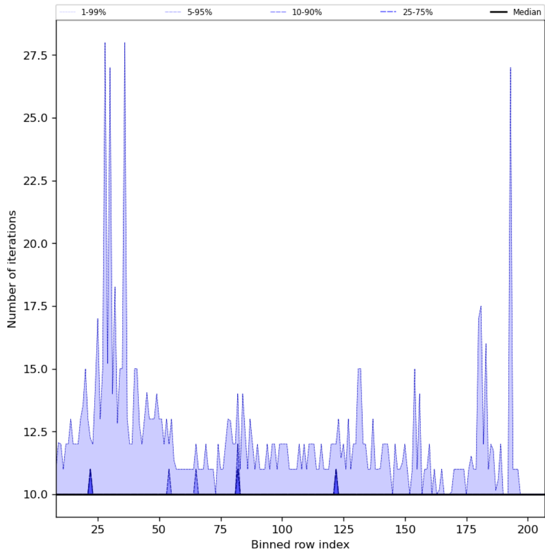
Figure 42: Along track statistics of “Number of iterations” for 2023-09-04 to 2023-09-05
