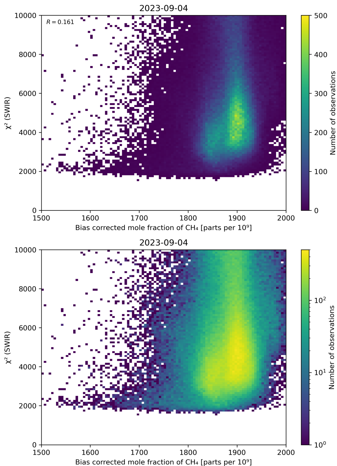
Figure 64: Scatter density plot of “Bias corrected mole fraction of \text{CH}_4 ” against “ \chi^2 (SWIR)” for 2023-09-04 to 2023-09-05.
