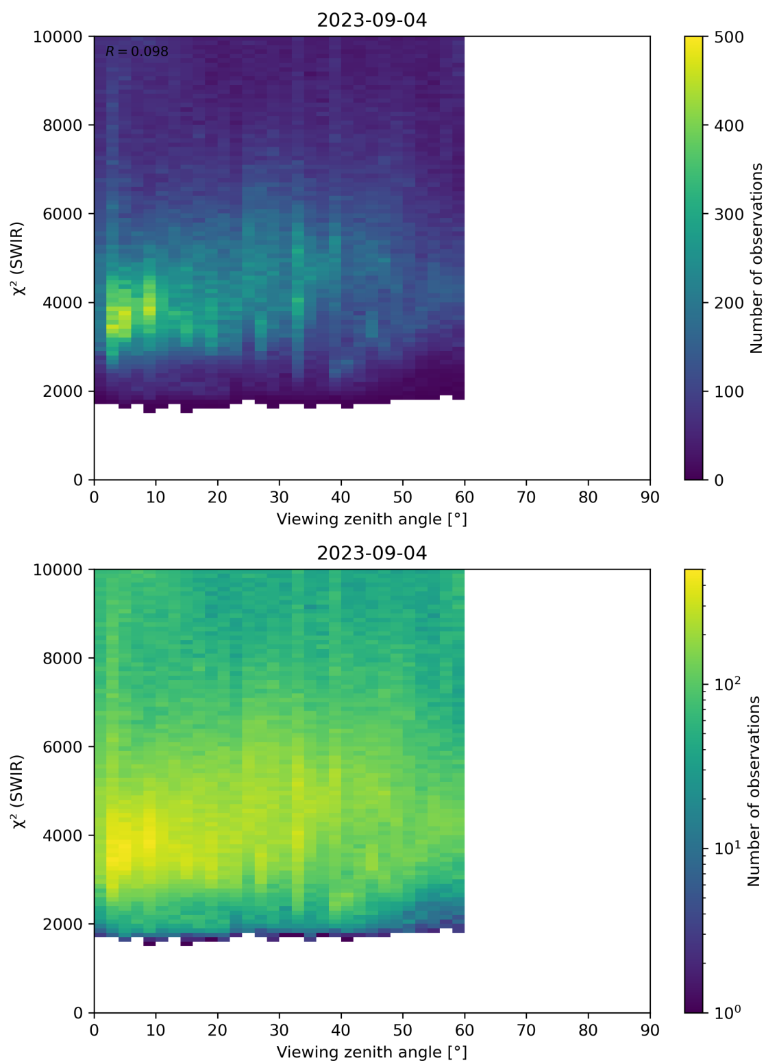
Figure 106: Scatter density plot of “Viewing zenith angle” against “ \chi^2 (SWIR)” for 2023-09-04 to 2023-09-05.
