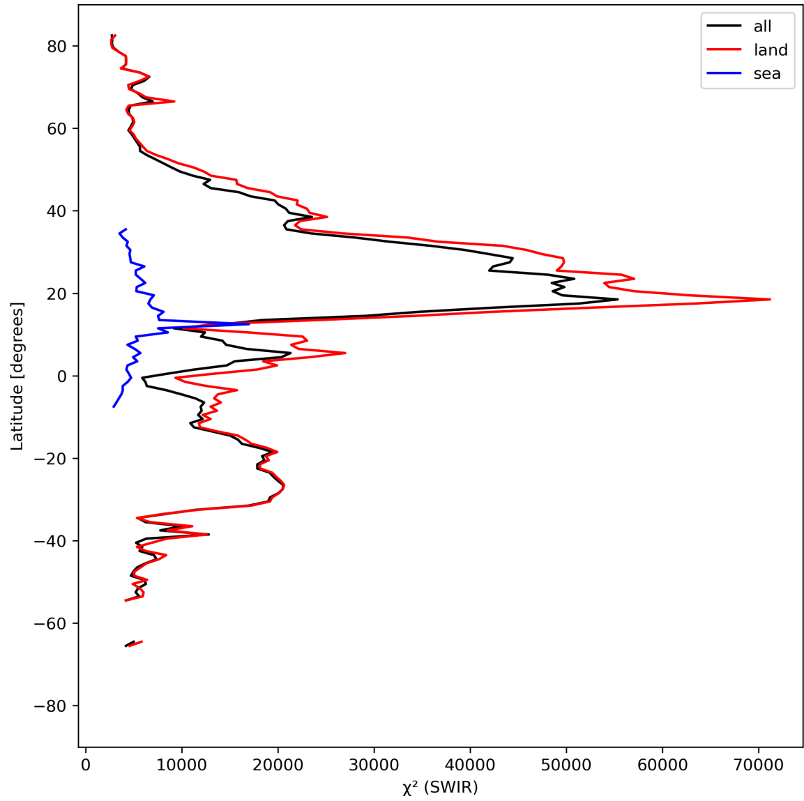
Figure 17: Zonal average of “ \chi^2 (SWIR)” for 2023-09-04 to 2023-09-05.
