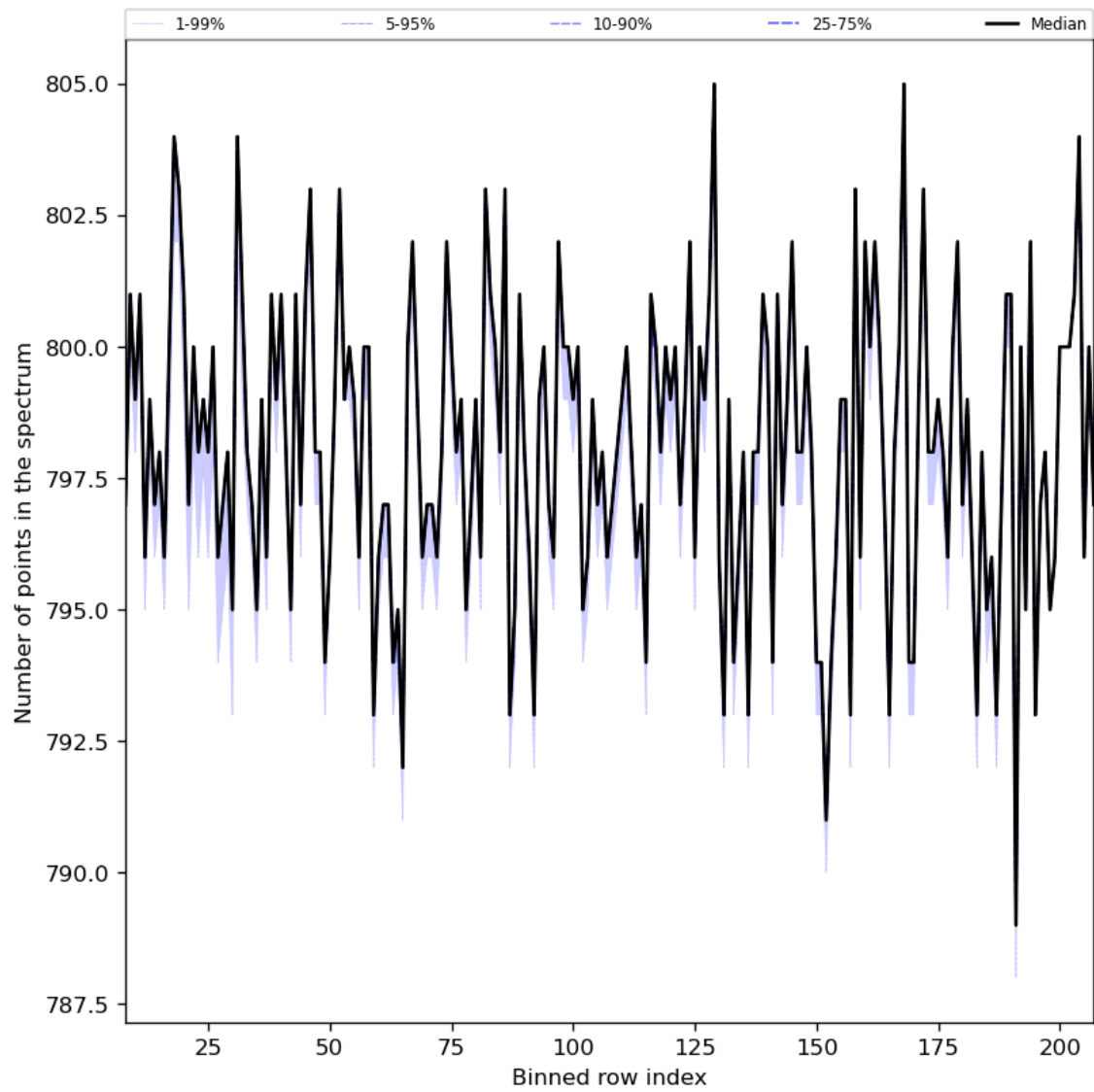
Figure 37: Along track statistics of “Number of points in the spectrum” for 2023-09-04 to 2023-09-05
