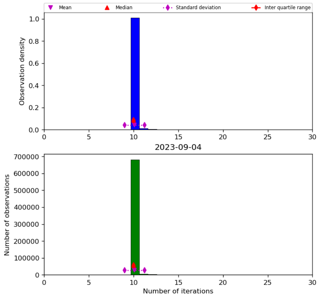
Figure 31: Histogram of “Number of iterations” for 2023-09-04 to 2023-09-05
