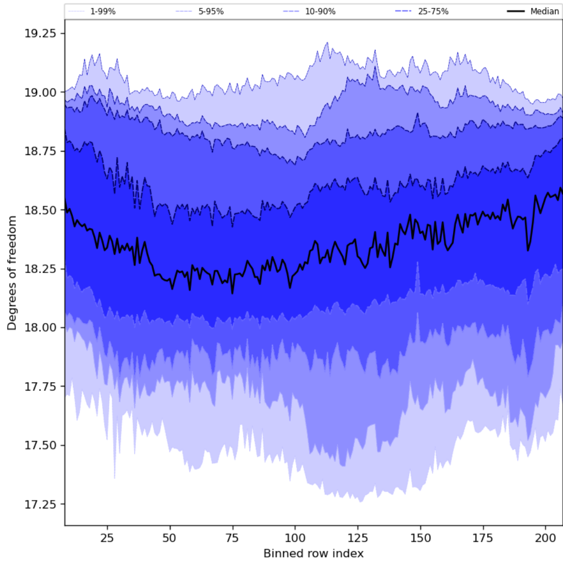
Figure 41: Along track statistics of “Degrees of freedom” for 2023-09-04 to 2023-09-05
