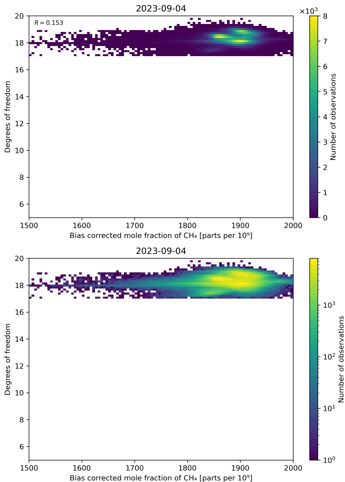
Figure 65: Scatter density plot of “Bias corrected mole fraction of CH 4 ” against “Degrees of freedom” for 2023-09-04 to 2023-09-05.
