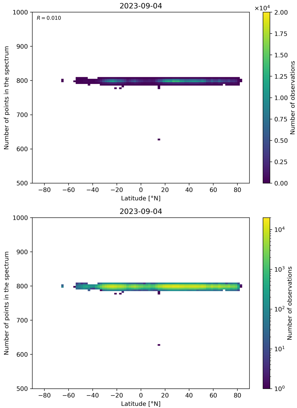
Figure 61: Scatter density plot of “Latitude” against “Number of points in the spectrum” for 2023-09-04 to 2023-09-05.
