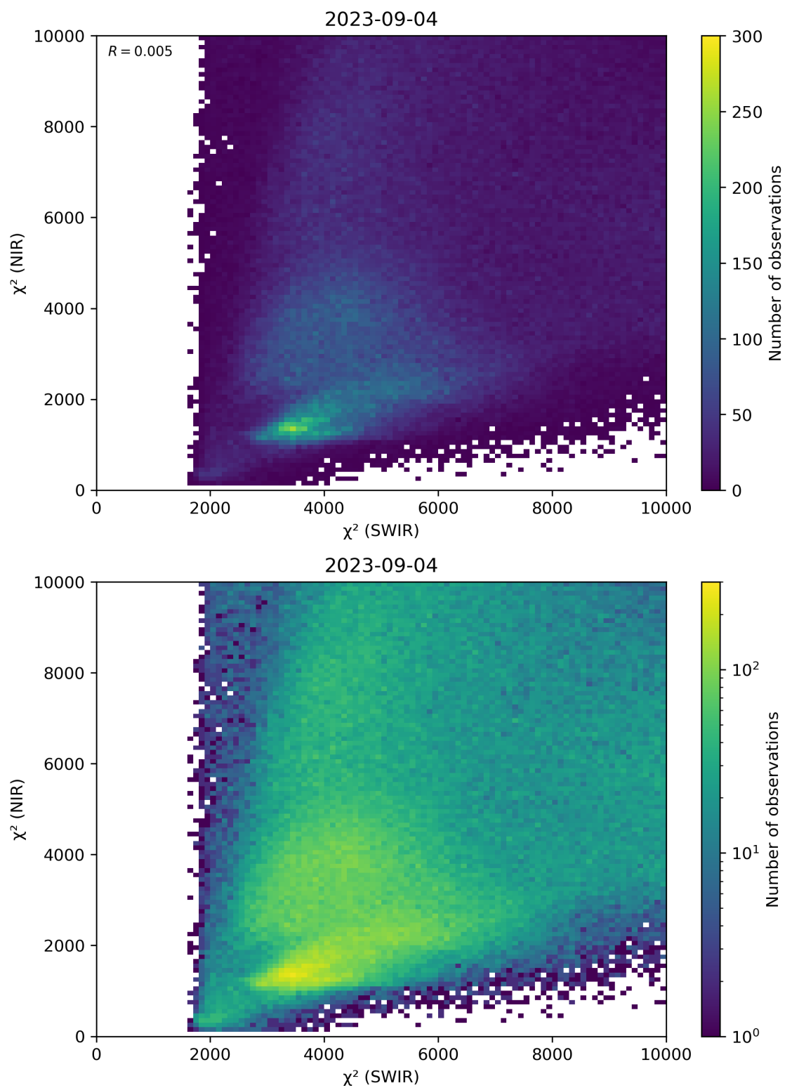
Figure 47: Scatter density plot of “ \chi^2 (SWIR)” against “ \chi^2 (NIR)” for 2023-09-04 to 2023-09-05.
