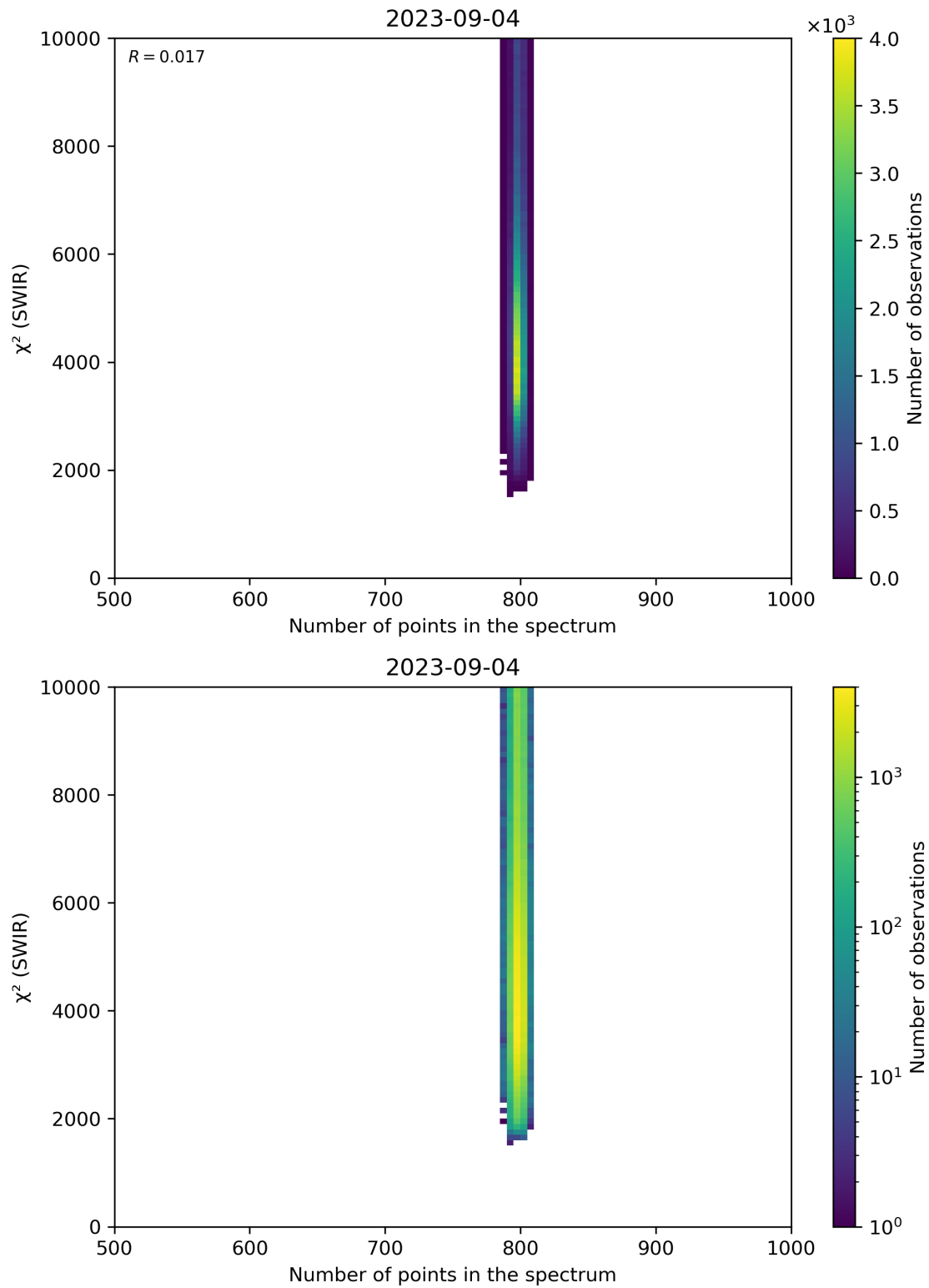
Figure 89: Scatter density plot of “Number of points in the spectrum” against “ \chi^2 (SWIR)” for 2023-09-04 to 2023-09-05.
