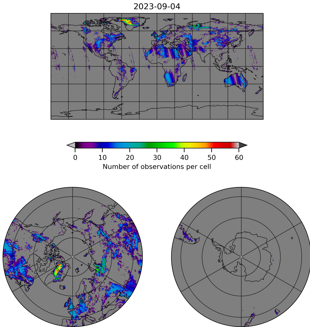
Figure 10: Map of the number of observations for 2023-09-04 to 2023-09-05
