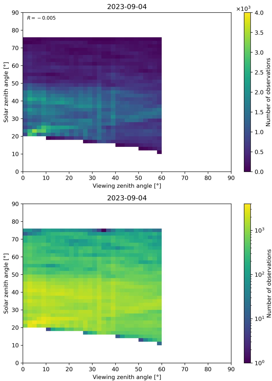
Figure 115: Scatter density plot of “Viewing zenith angle” against “Solar zenith angle” for 2023-09-04 to 2023-09-05.
