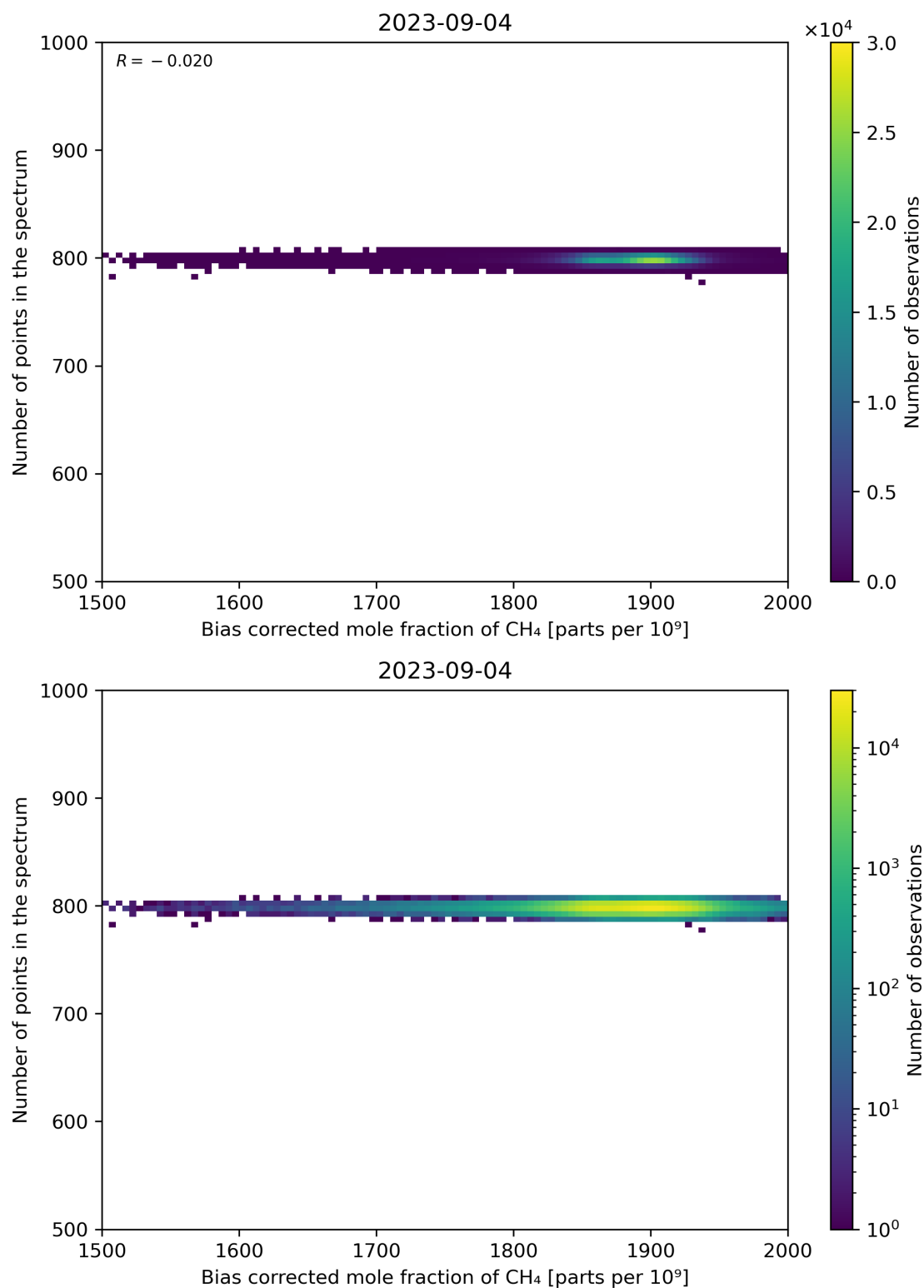
Figure 68: Scatter density plot of “Bias corrected mole fraction of CH 4 ” against “Number of points in the spectrum” for 2023-09-04 to 2023-09-05.
