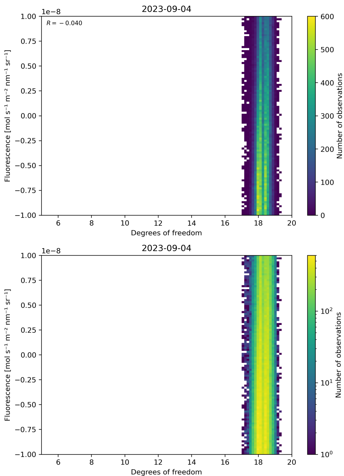
Figure 51: Scatter density plot of “Degrees of freedom” against “Fluorescence” for 2023-09-04 to 2023-09-05.
