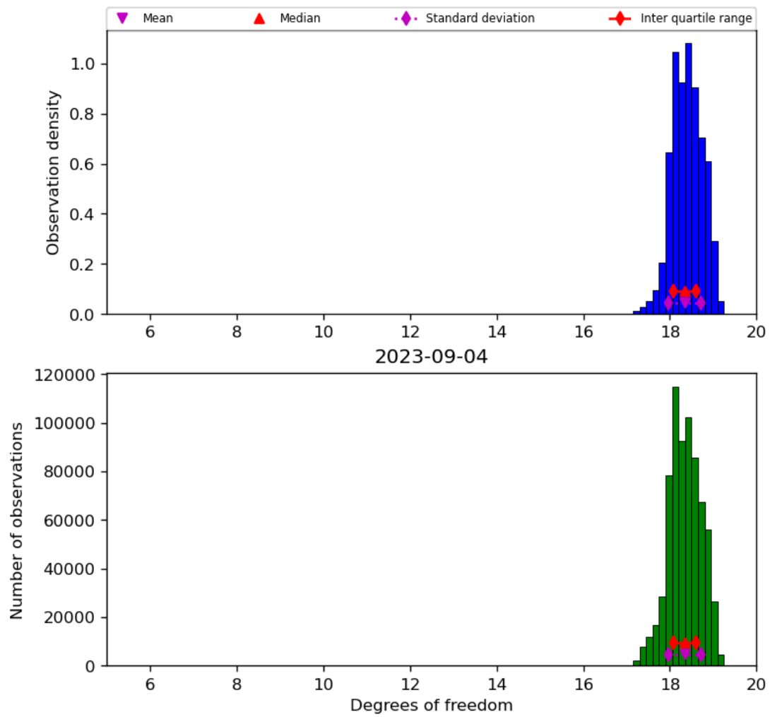
Figure 30: Histogram of “Degrees of freedom” for 2023-09-04 to 2023-09-05
