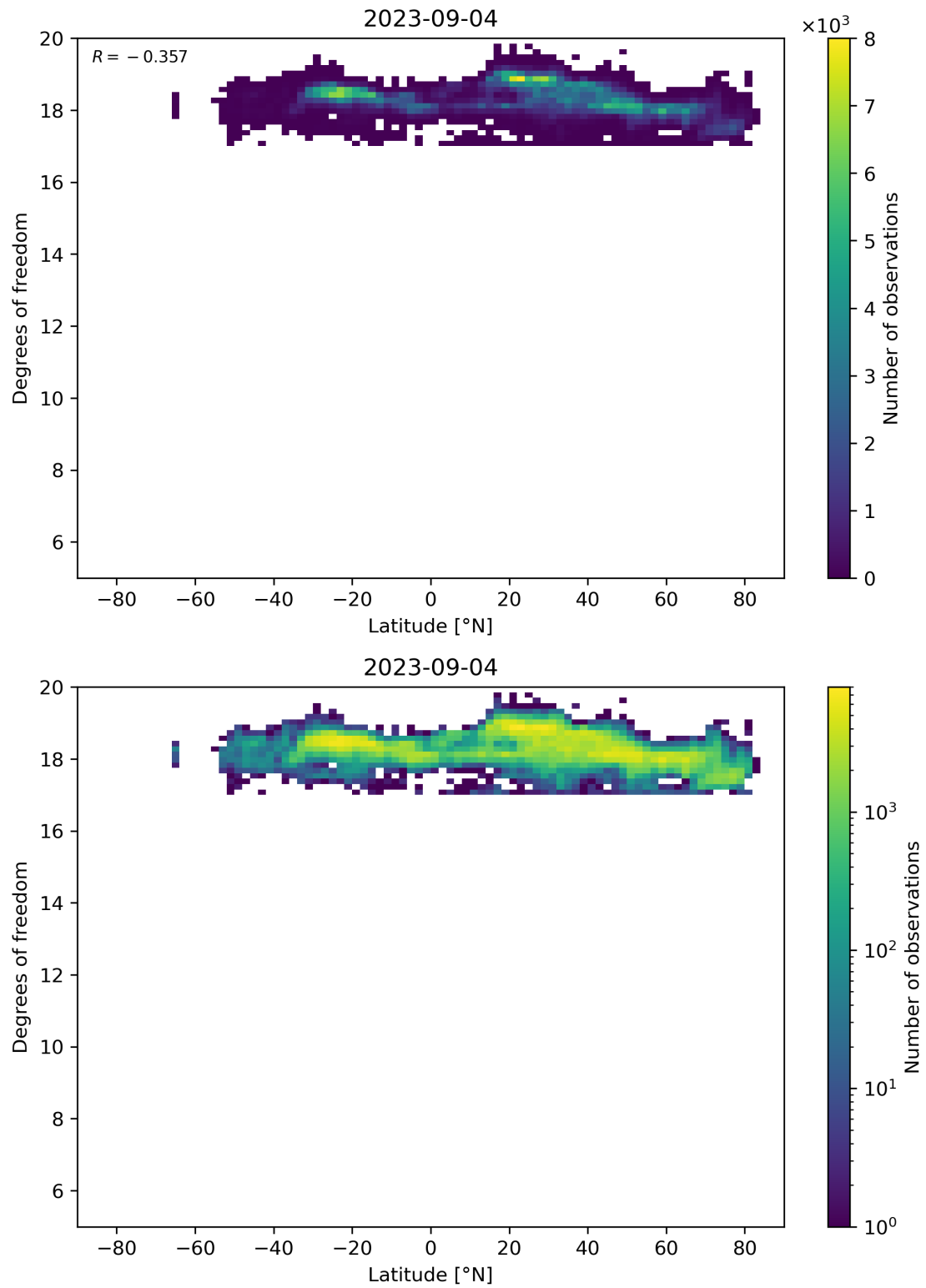
Figure 55: Scatter density plot of “Latitude” against “Degrees of freedom” for 2023-09-04 to 2023-09-05.
