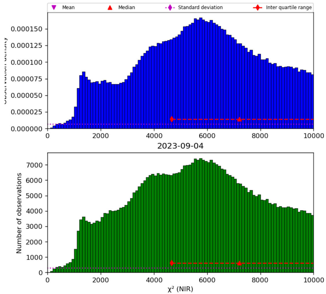
Figure 29: Histogram of “ \chi^2 (NIR)” for 2023-09-04 to 2023-09-05
