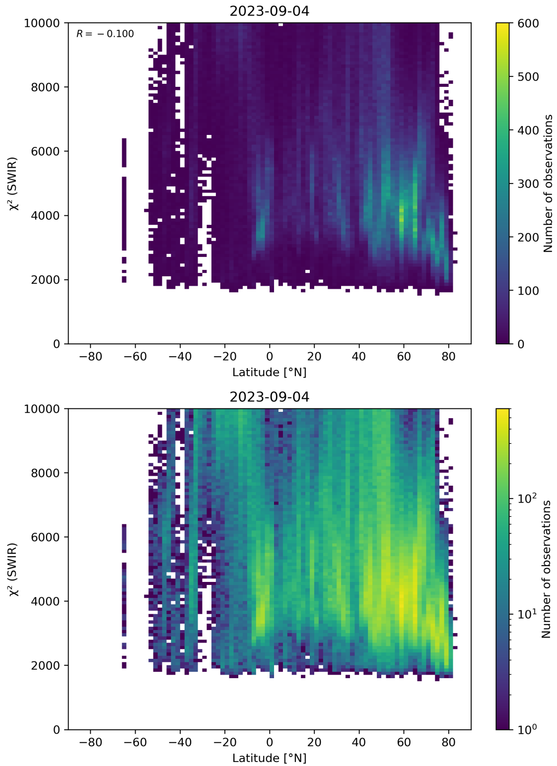
Figure 54: Scatter density plot of “Latitude” against “ \chi^2 (SWIR)” for 2023-09-04 to 2023-09-05.
