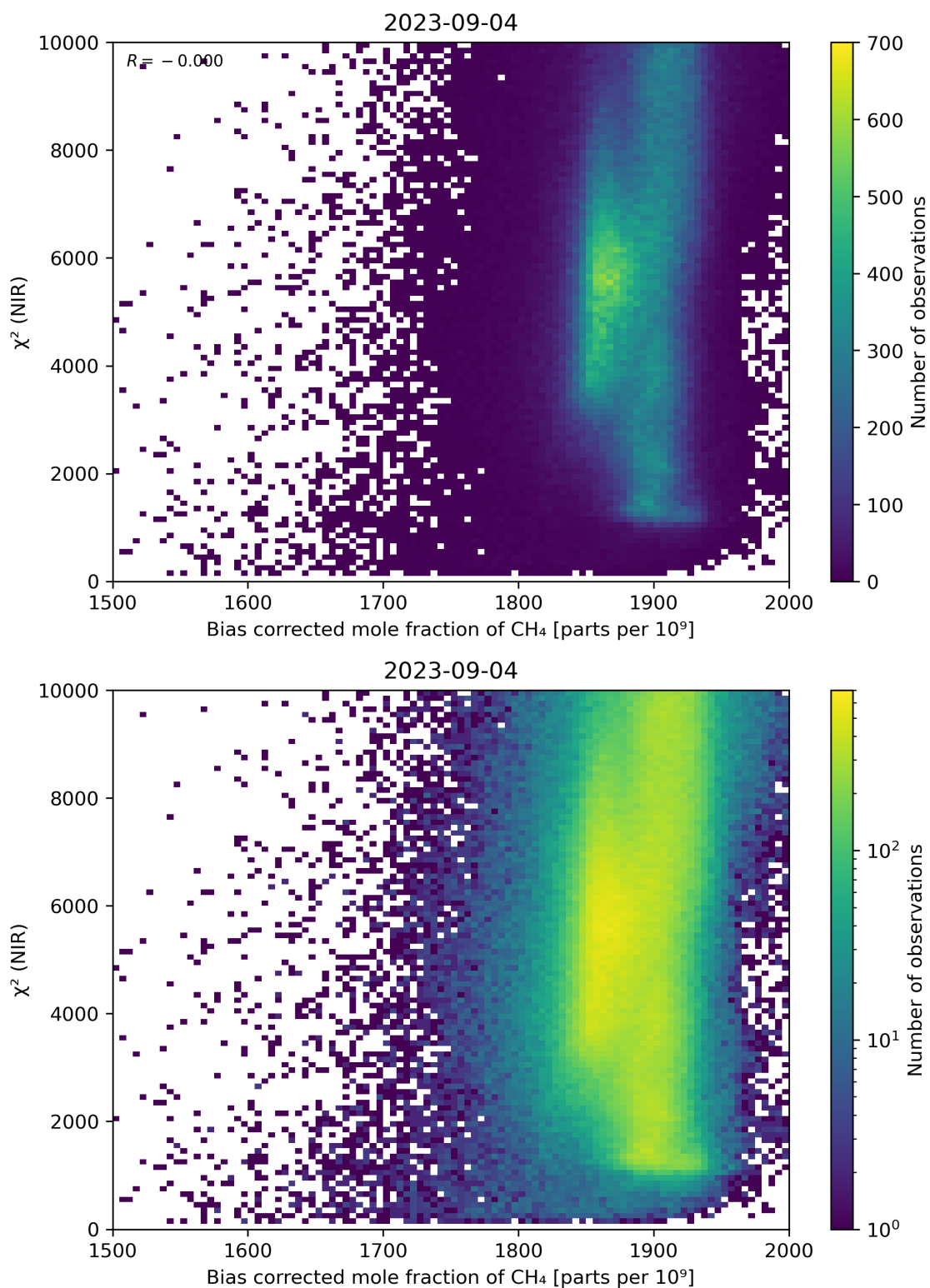
Figure 63: Scatter density plot of “Bias corrected mole fraction of CH 4 ” against “ \chi^2 (NIR)” for 2023-09-04 to 2023-09-05.
