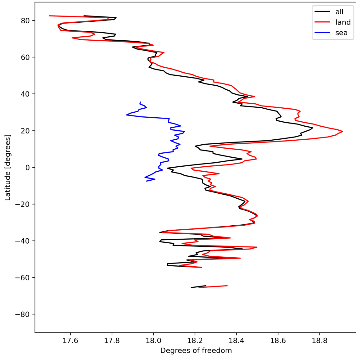
Figure 19: Zonal average of “Degrees of freedom” for 2023-09-04 to 2023-09-05.
