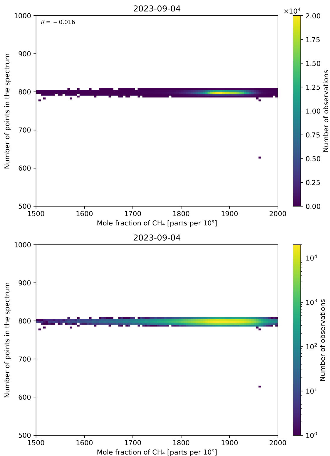
Figure 77: Scatter density plot of “Mole fraction of CH 4 ” against “Number of points in the spectrum” for 2023-09-04 to 2023-09-05.
