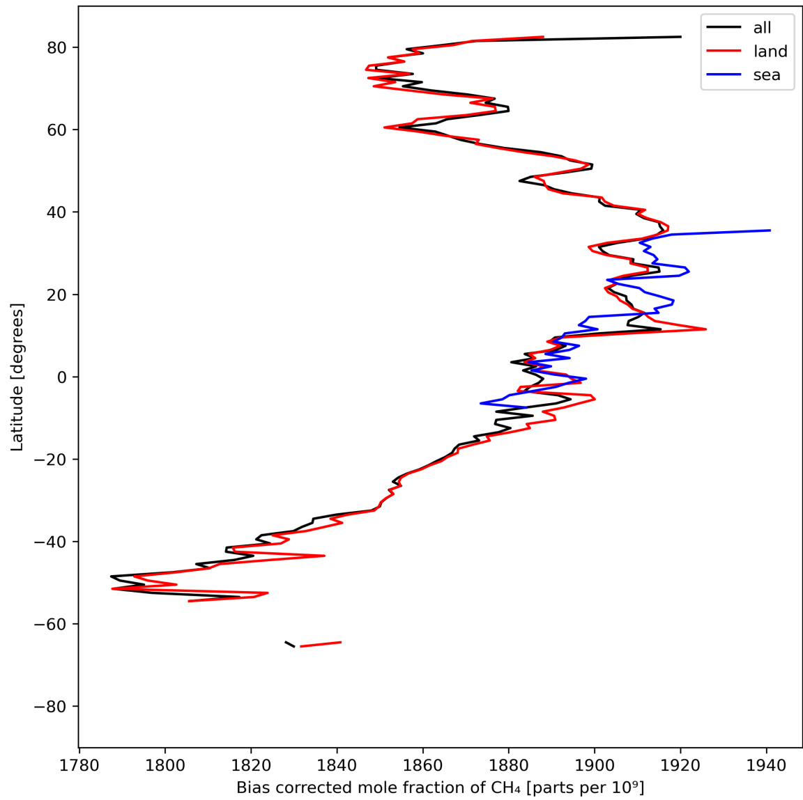
Figure 14: Zonal average of “Bias corrected mole fraction of CH 4 ” for 2023-09-04 to 2023-09-05.
