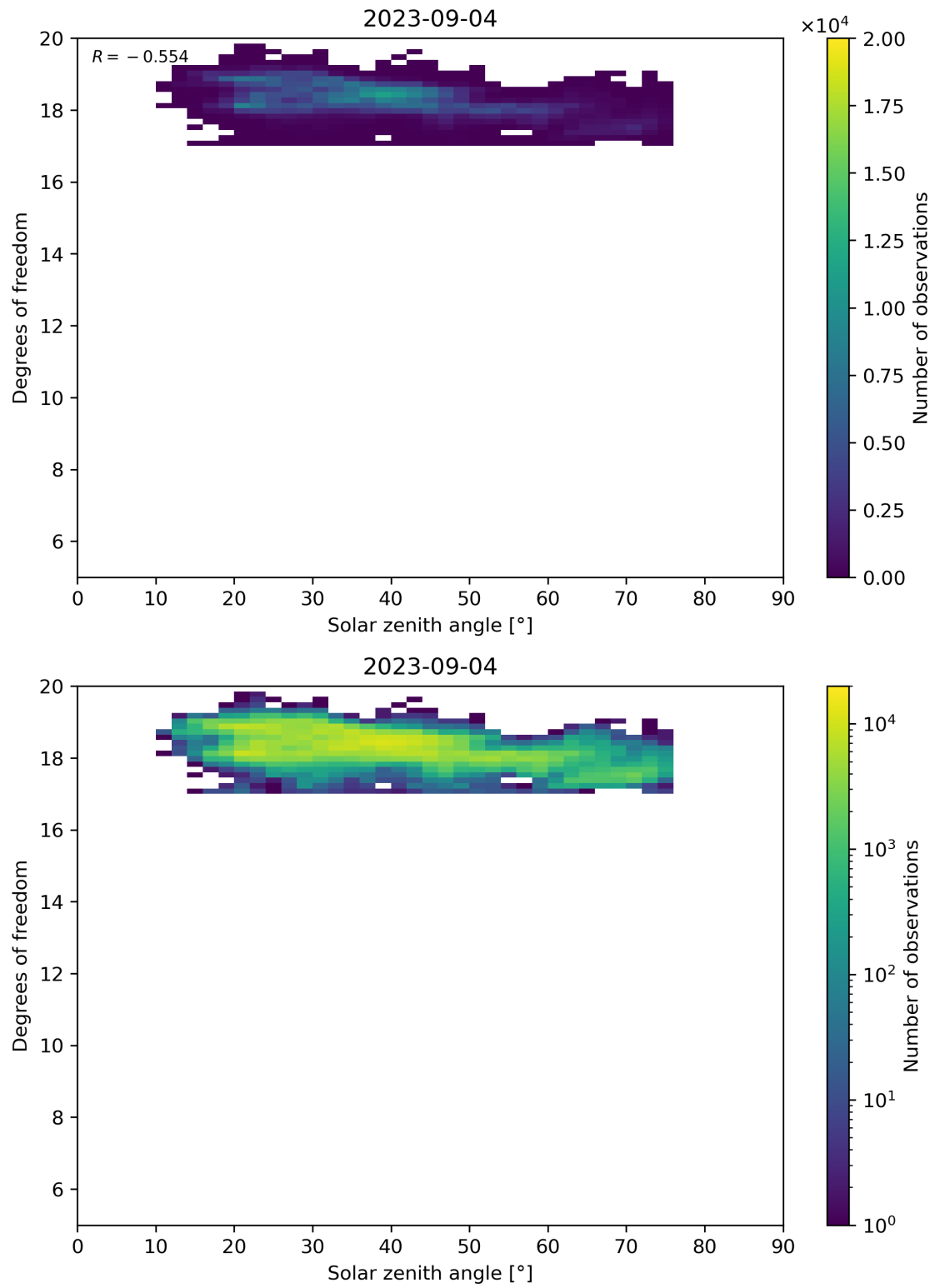
Figure 96: Scatter density plot of “Solar zenith angle” against “Degrees of freedom” for 2023-09-04 to 2023-09-05.
