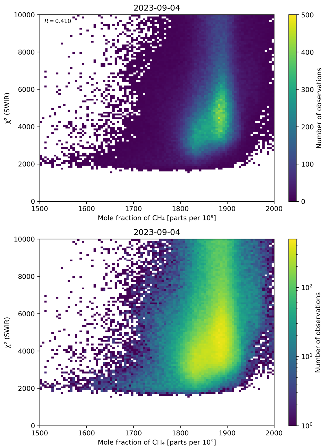
Figure 71: Scatter density plot of “Mole fraction of \text{CH}_4 ” against “ \chi^2 (SWIR)” for 2023-09-04 to 2023-09-05.
