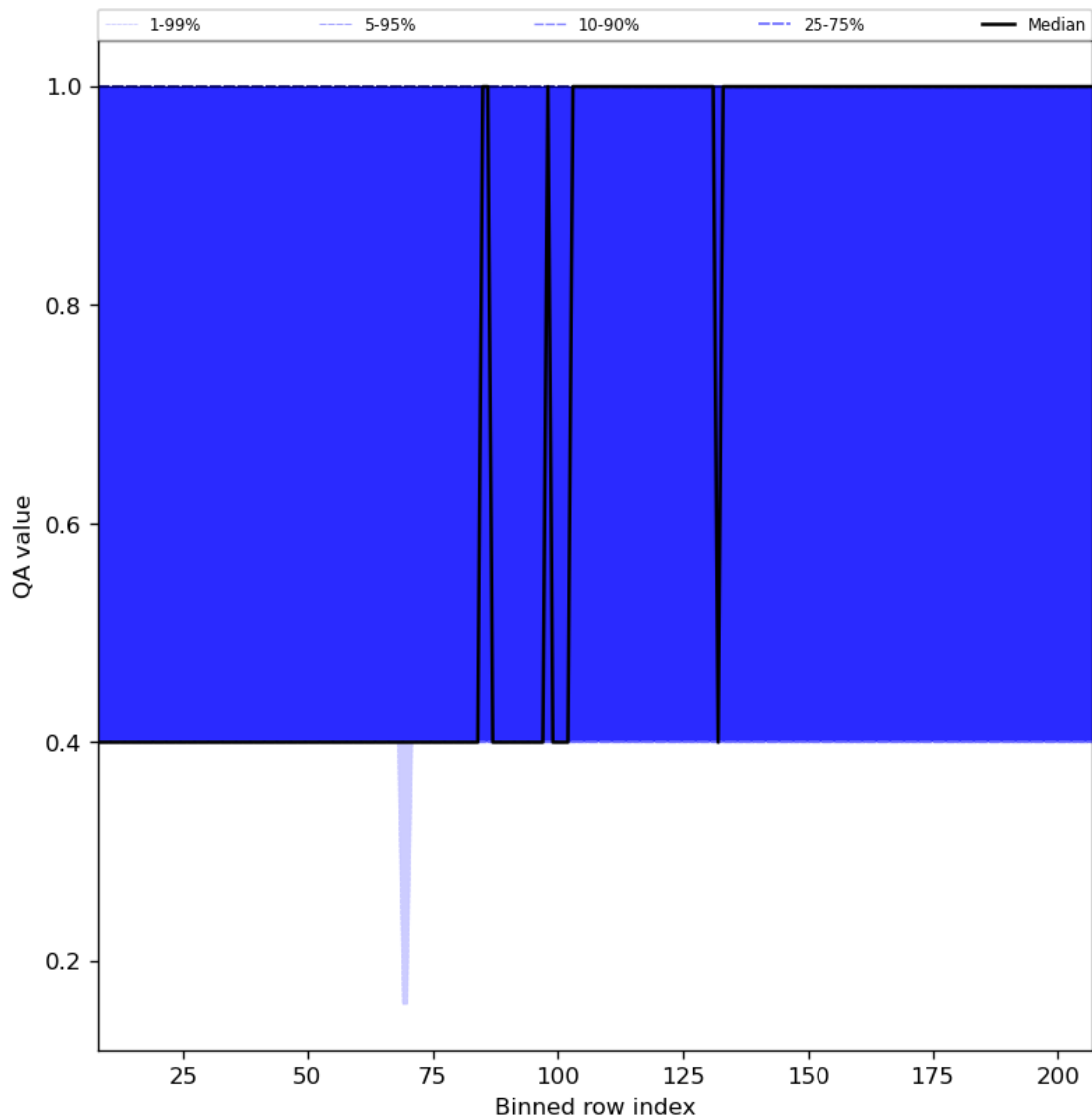
Figure 33: Along track statistics of “QA value” for 2023-09-04 to 2023-09-05
