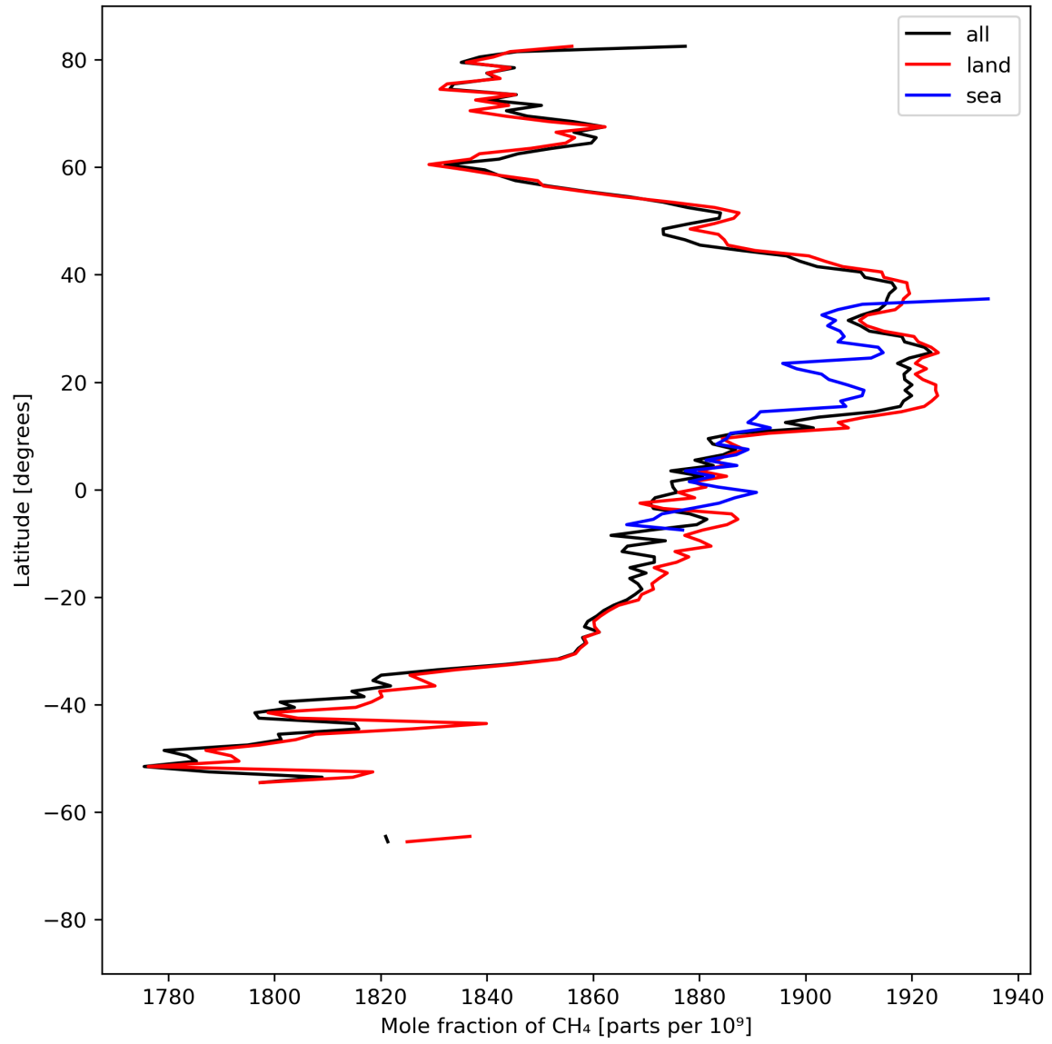
Figure 12: Zonal average of “Mole fraction of \text{CH}_4 ” for 2023-09-04 to 2023-09-05.
