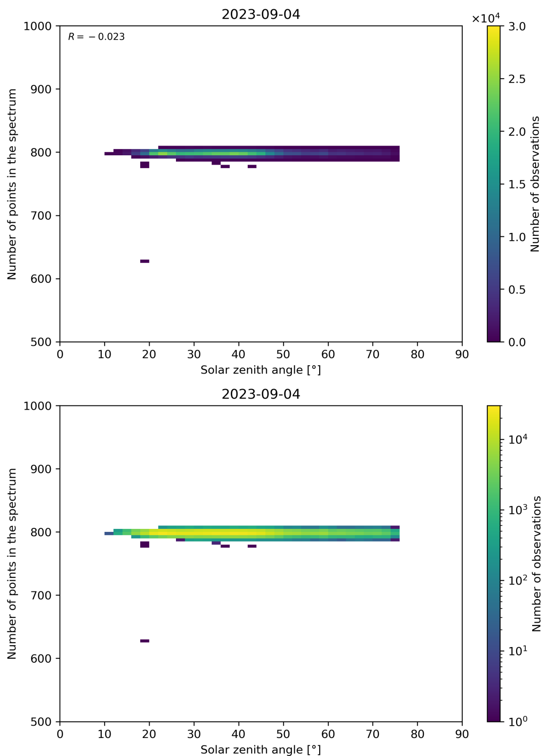
Figure 103: Scatter density plot of “Solar zenith angle” against “Number of points in the spectrum” for 2023-09-04 to 2023-09-05.
