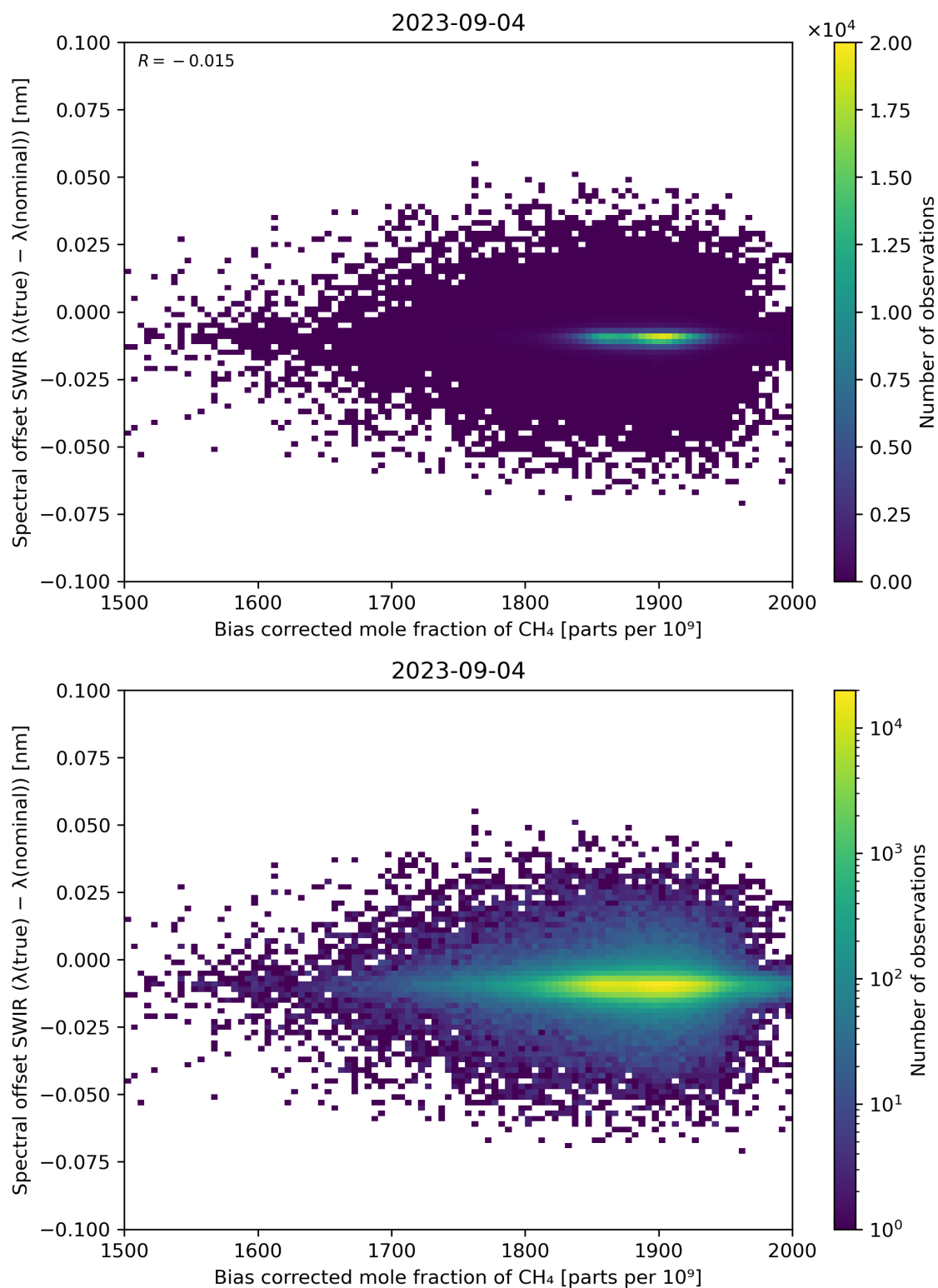
Figure 69: Scatter density plot of “Bias corrected mole fraction of \text{CH}_4 ” against “Spectral offset SWIR ( \lambda(\text{true}) - \lambda(\text{nominal}) )” for 2023-09-04 to 2023-09-05.
