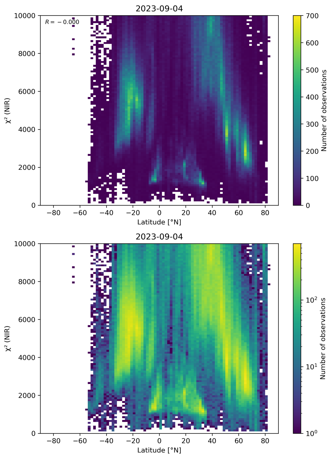
Figure 53: Scatter density plot of “Latitude” against “ \chi^2 (NIR)” for 2023-09-04 to 2023-09-05.
