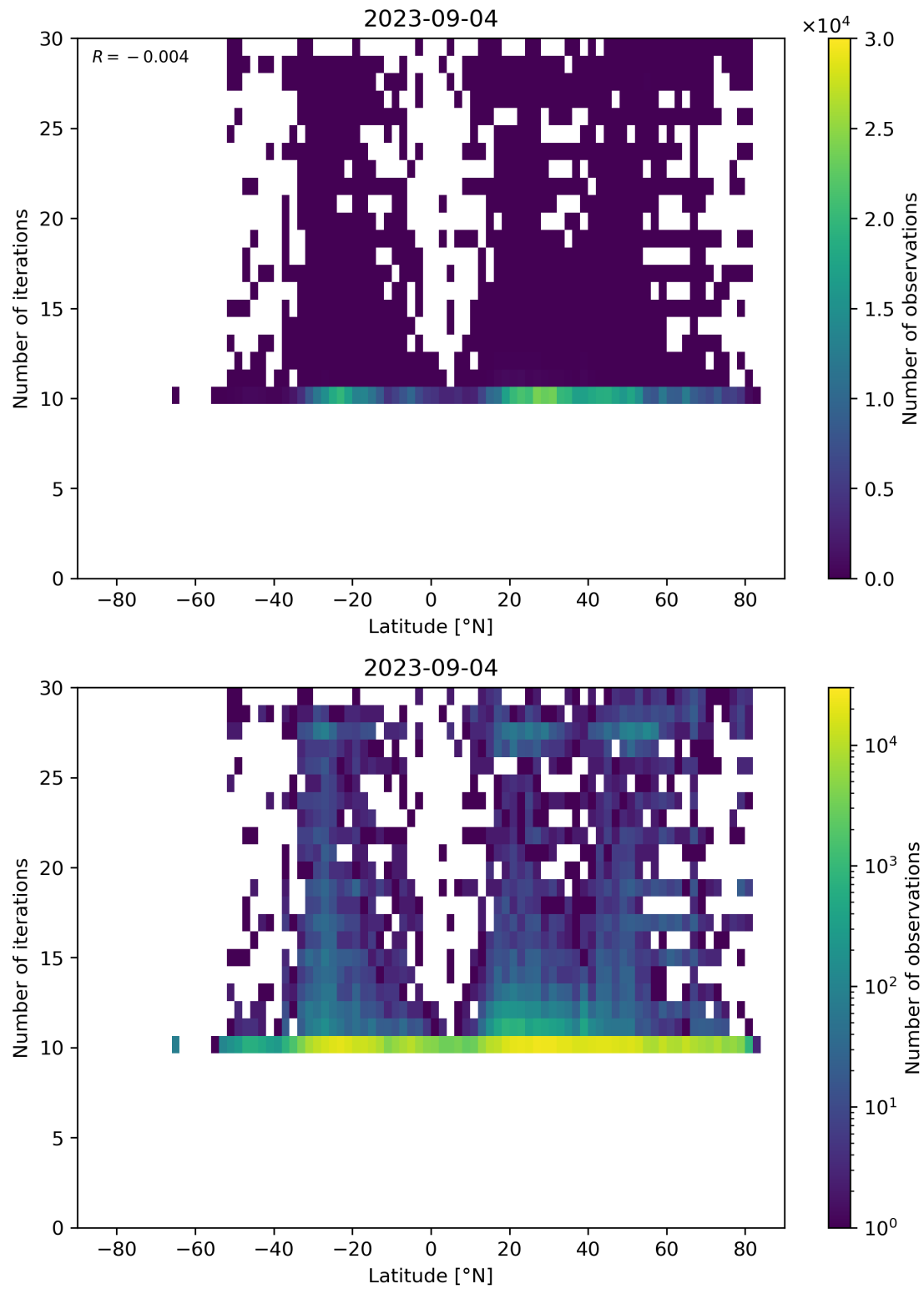
Figure 60: Scatter density plot of “Latitude” against “Number of iterations” for 2023-09-04 to 2023-09-05.
