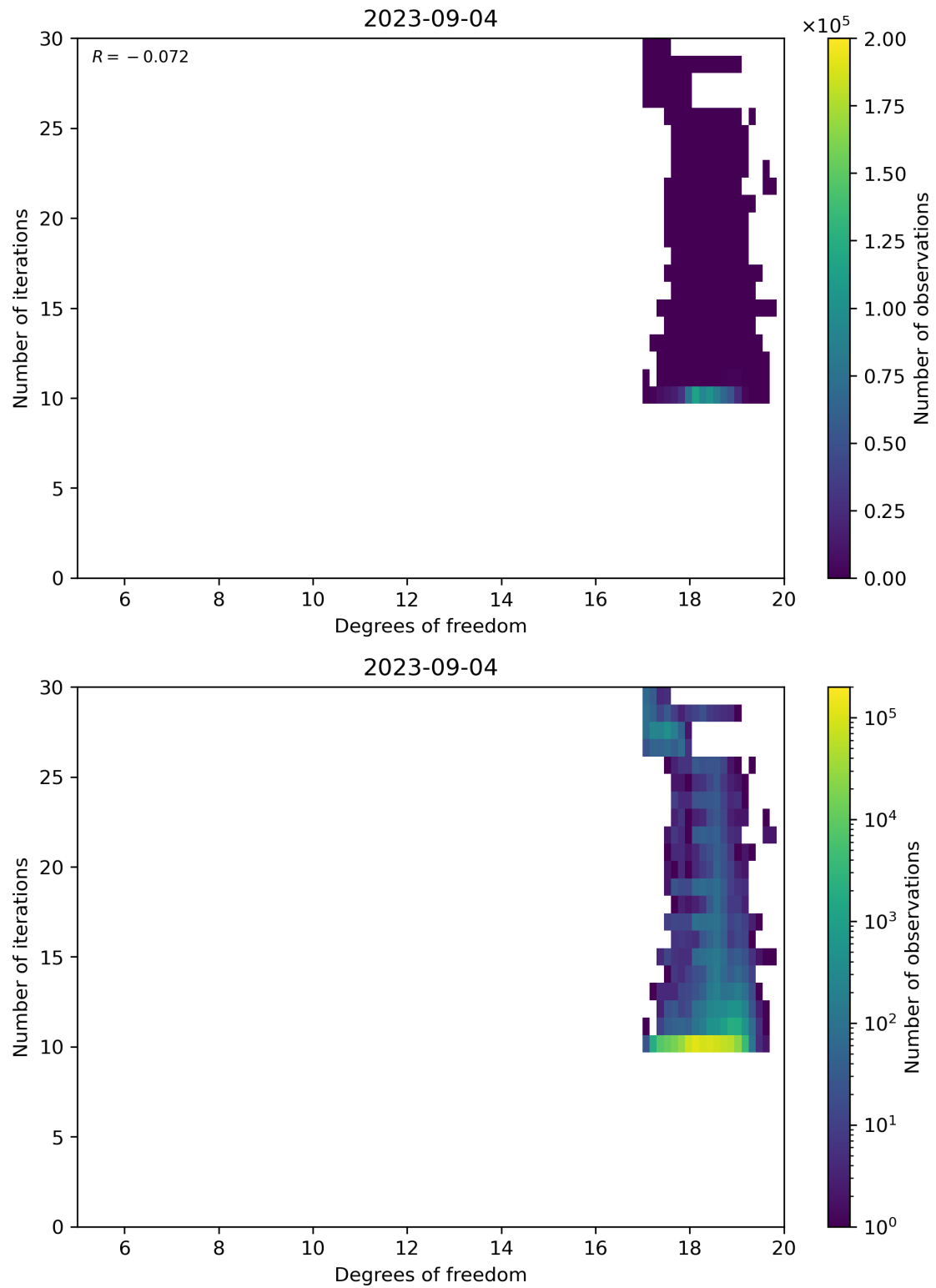
Figure 52: Scatter density plot of “Degrees of freedom” against “Number of iterations” for 2023-09-04 to 2023-09-05.
