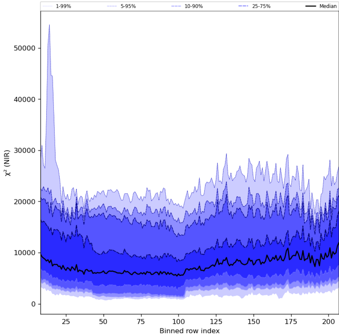
Figure 40: Along track statistics of “ \chi^2 (NIR)” for 2023-09-04 to 2023-09-05
