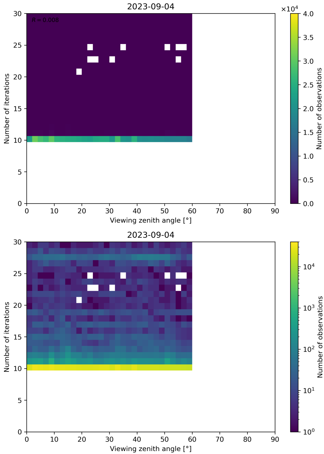
Figure 113: Scatter density plot of “Viewing zenith angle” against “Number of iterations” for 2023-09-04 to 2023-09-05.
