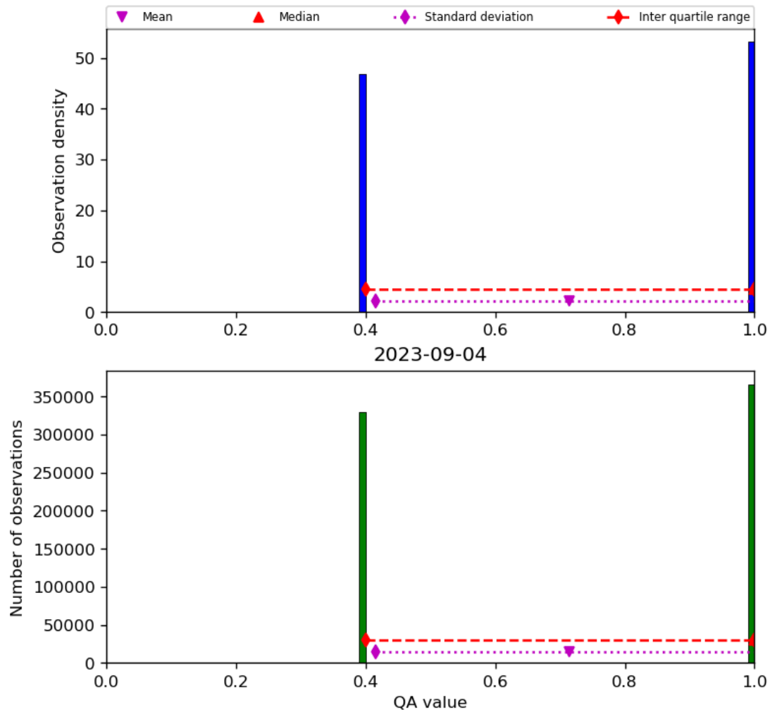
Figure 22: Histogram of "QA value" for 2023-09-04 to 2023-09-05
