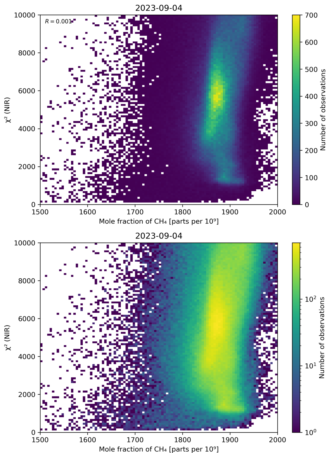
Figure 70: Scatter density plot of “Mole fraction of CH 4 ” against “ \chi^2 (NIR)” for 2023-09-04 to 2023-09-05.
