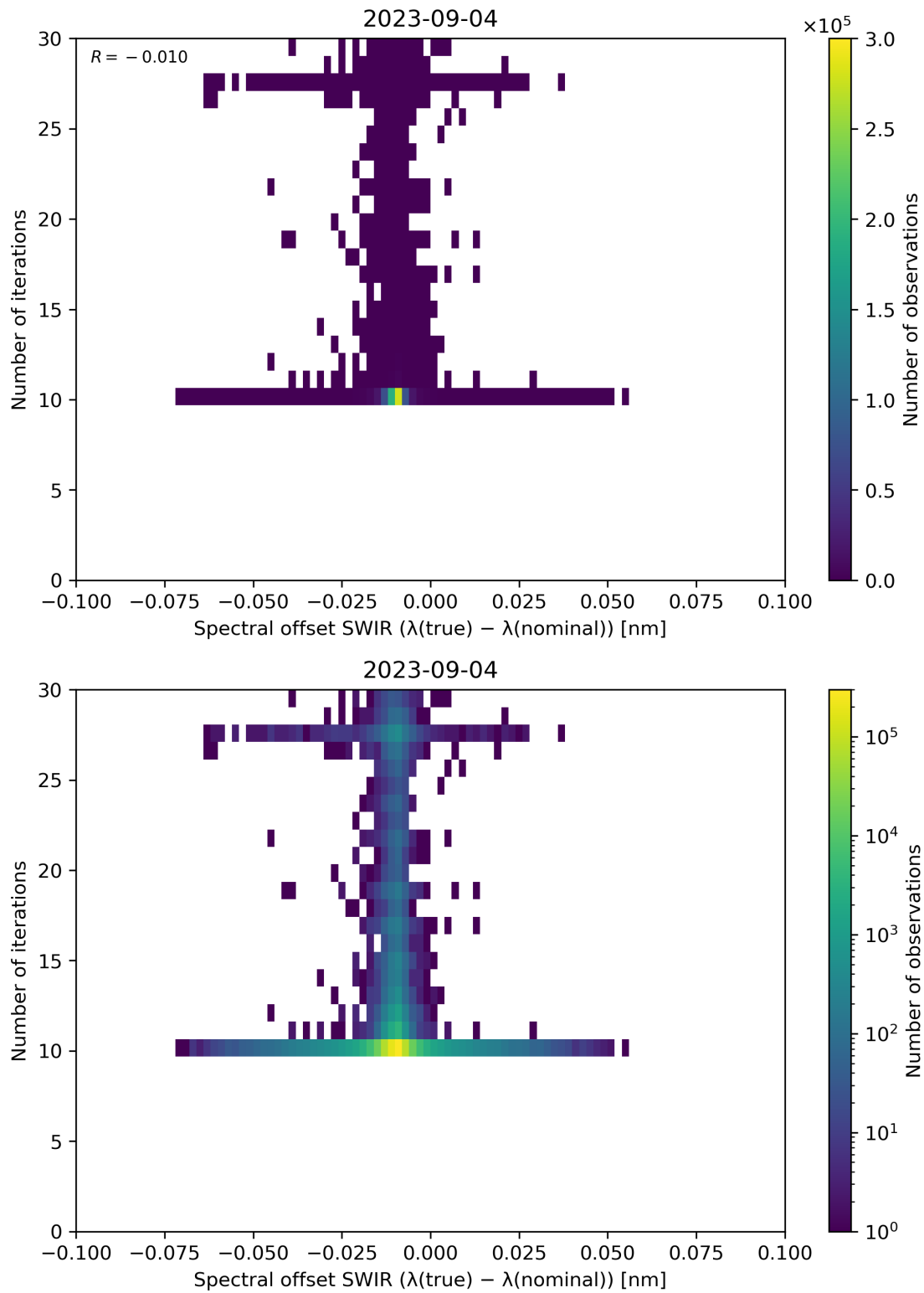
Figure 121: Scatter density plot of “Spectral offset SWIR ( \lambda(\text{true}) - \lambda(\text{nominal}) )” against “Number of iterations” for 2023-09-04 to 2023-09-05.
