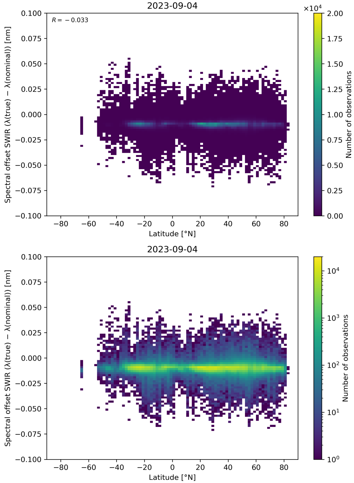
Figure 62: Scatter density plot of “Latitude” against “Spectral offset SWIR ( \lambda(\text{true}) - \lambda(\text{nominal}) )” for 2023-09-04 to 2023-09-05.
