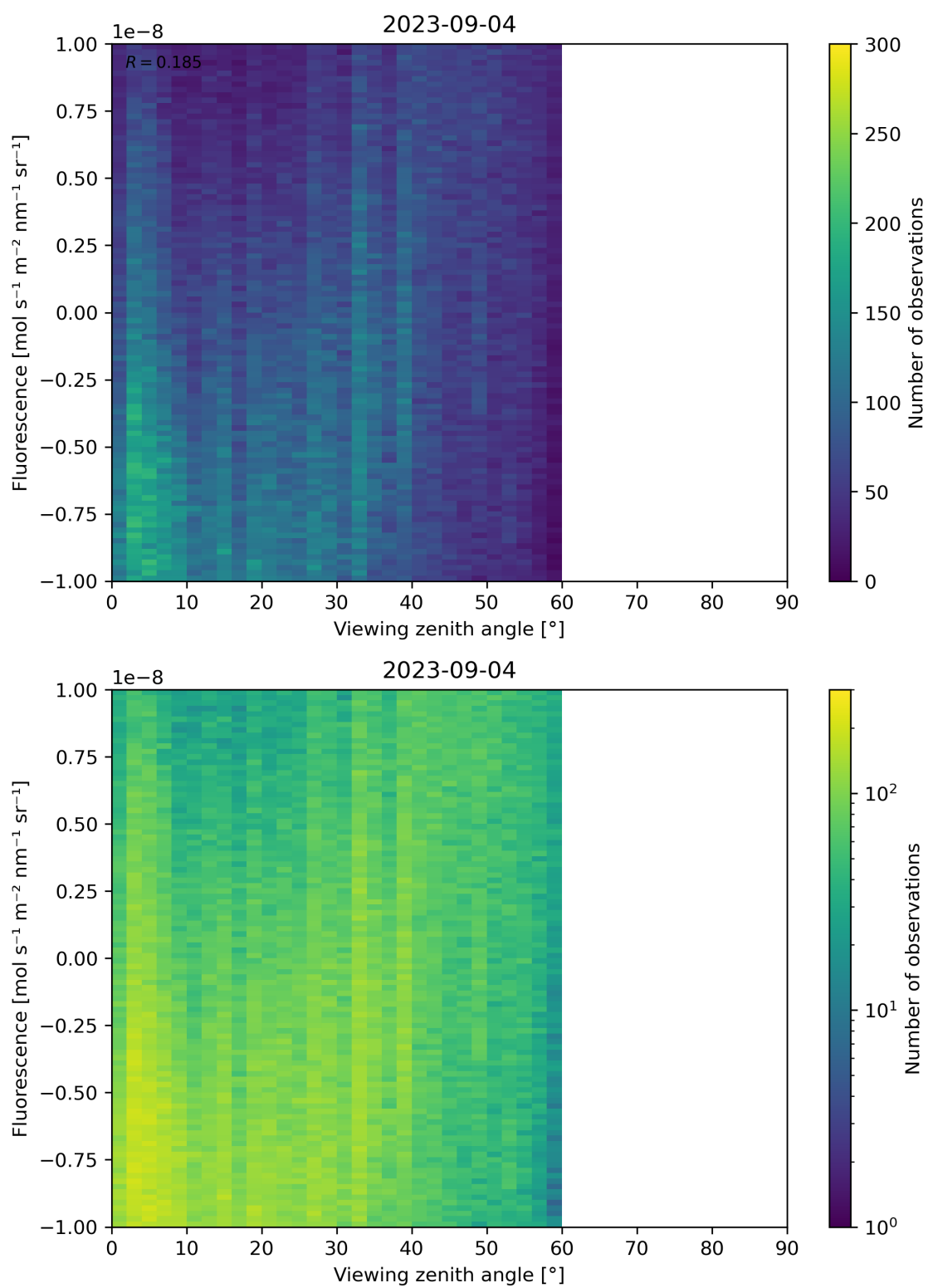
Figure 108: Scatter density plot of “Viewing zenith angle” against “Fluorescence” for 2023-09-04 to 2023-09-05.
