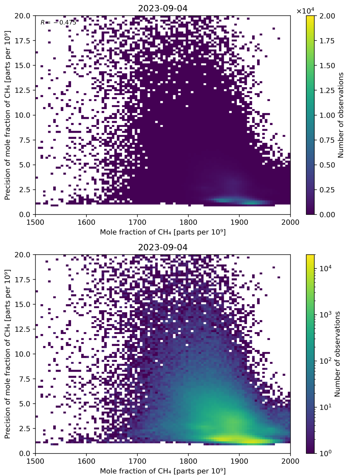
Figure 75: Scatter density plot of “Mole fraction of CH 4 ” against “Precision of mole fraction of CH 4 ” for 2023-09-04 to 2023-09-05.
