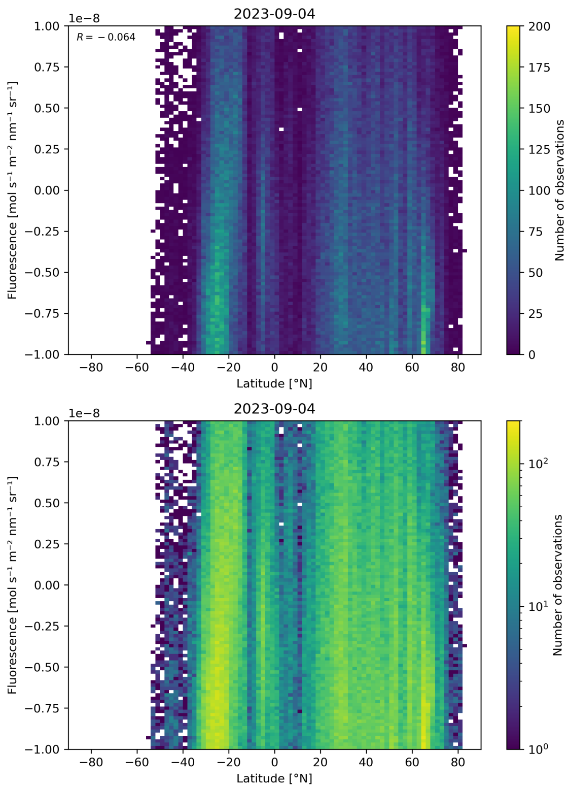
Figure 56: Scatter density plot of “Latitude” against “Fluorescence” for 2023-09-04 to 2023-09-05.
