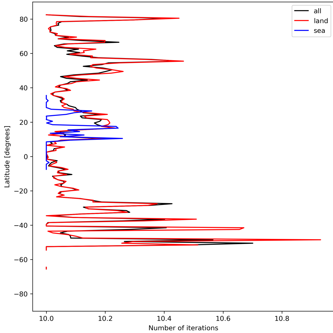
Figure 20: Zonal average of “Number of iterations” for 2023-09-04 to 2023-09-05.
