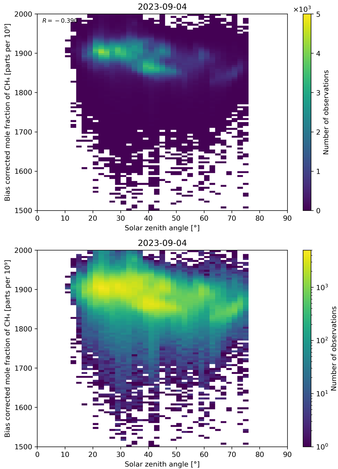
Figure 100: Scatter density plot of “Solar zenith angle” against “Bias corrected mole fraction of CH 4 ” for 2023-09-04 to 2023-09-05.
