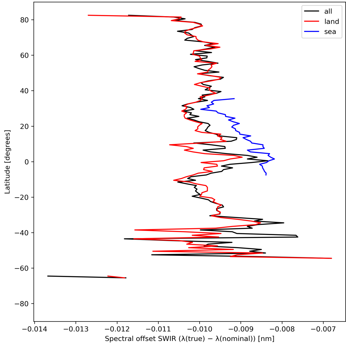
Figure 16: Zonal average of “Spectral offset SWIR ( \lambda(\text{true}) - \lambda(\text{nominal}) )” for 2023-09-04 to 2023-09-05.
