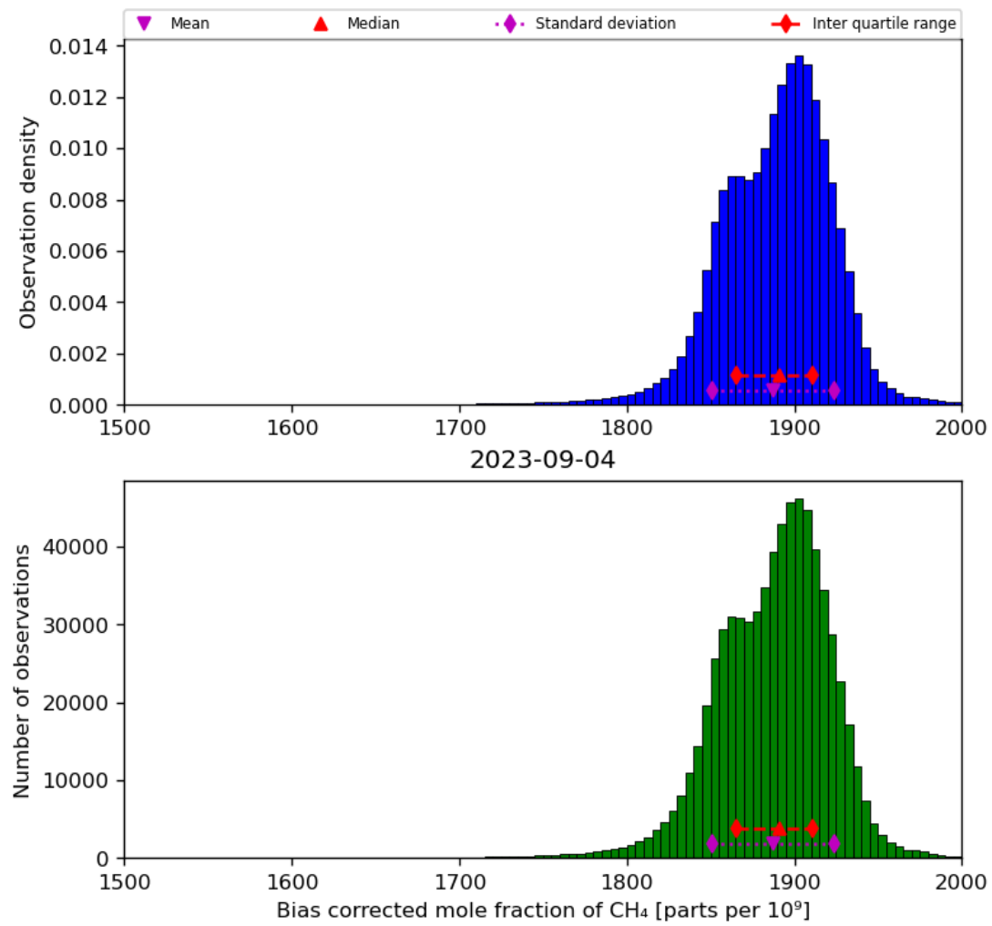
Figure 25: Histogram of “Bias corrected mole fraction of CH 4 ” for 2023-09-04 to 2023-09-05
