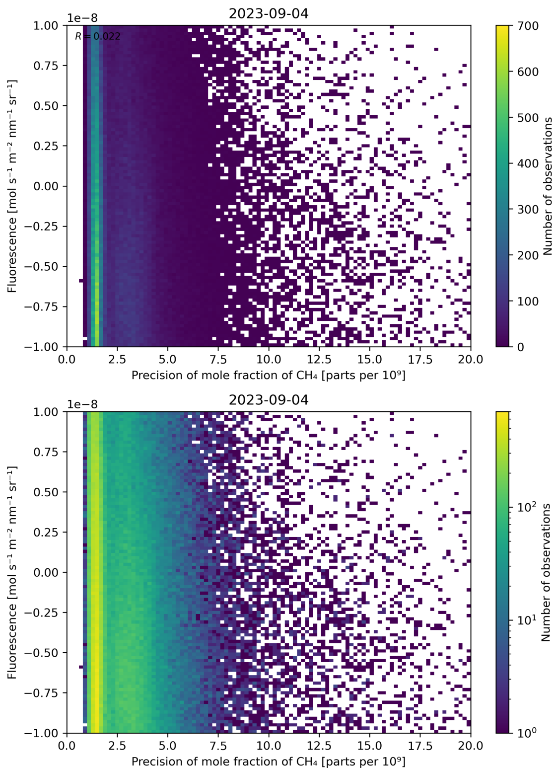
Figure 81: Scatter density plot of “Precision of mole fraction of \text{CH}_4 ” against “Fluorescence” for 2023-09-04 to 2023-09-05.
