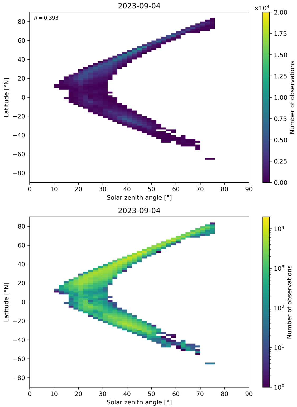
Figure 98: Scatter density plot of “Solar zenith angle” against “Latitude” for 2023-09-04 to 2023-09-05.
