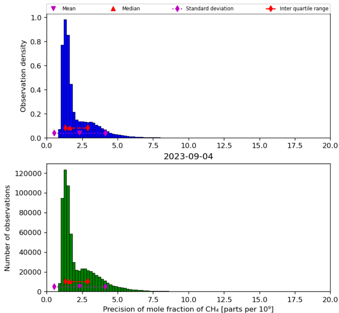
Figure 24: Histogram of “Precision of mole fraction of CH 4 ” for 2023-09-04 to 2023-09-05
