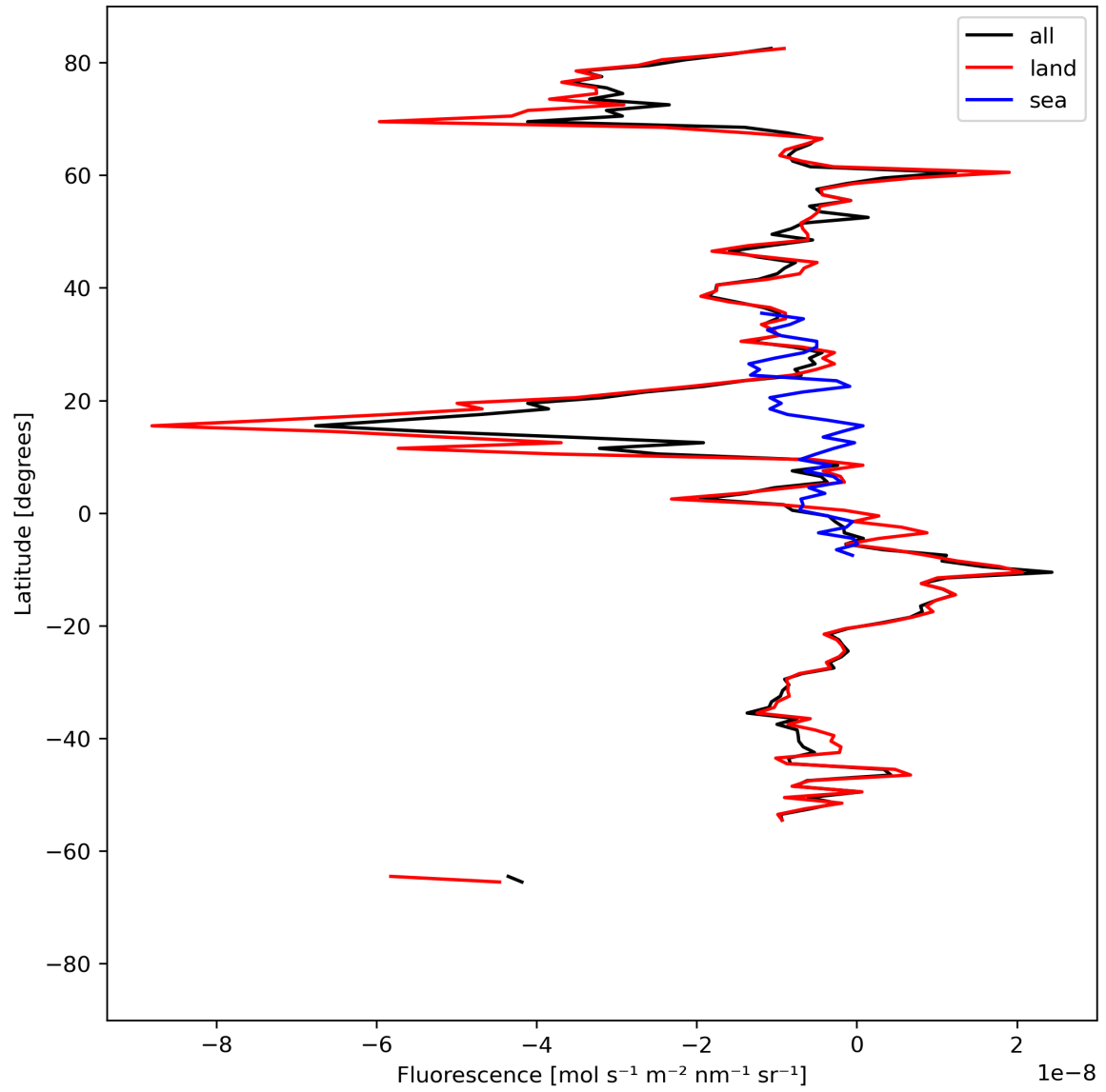
Figure 21: Zonal average of “Fluorescence” for 2023-09-04 to 2023-09-05.
