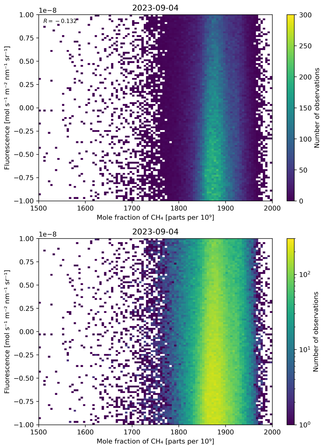
Figure 73: Scatter density plot of “Mole fraction of \text{CH}_4 ” against “Fluorescence” for 2023-09-04 to 2023-09-05.
