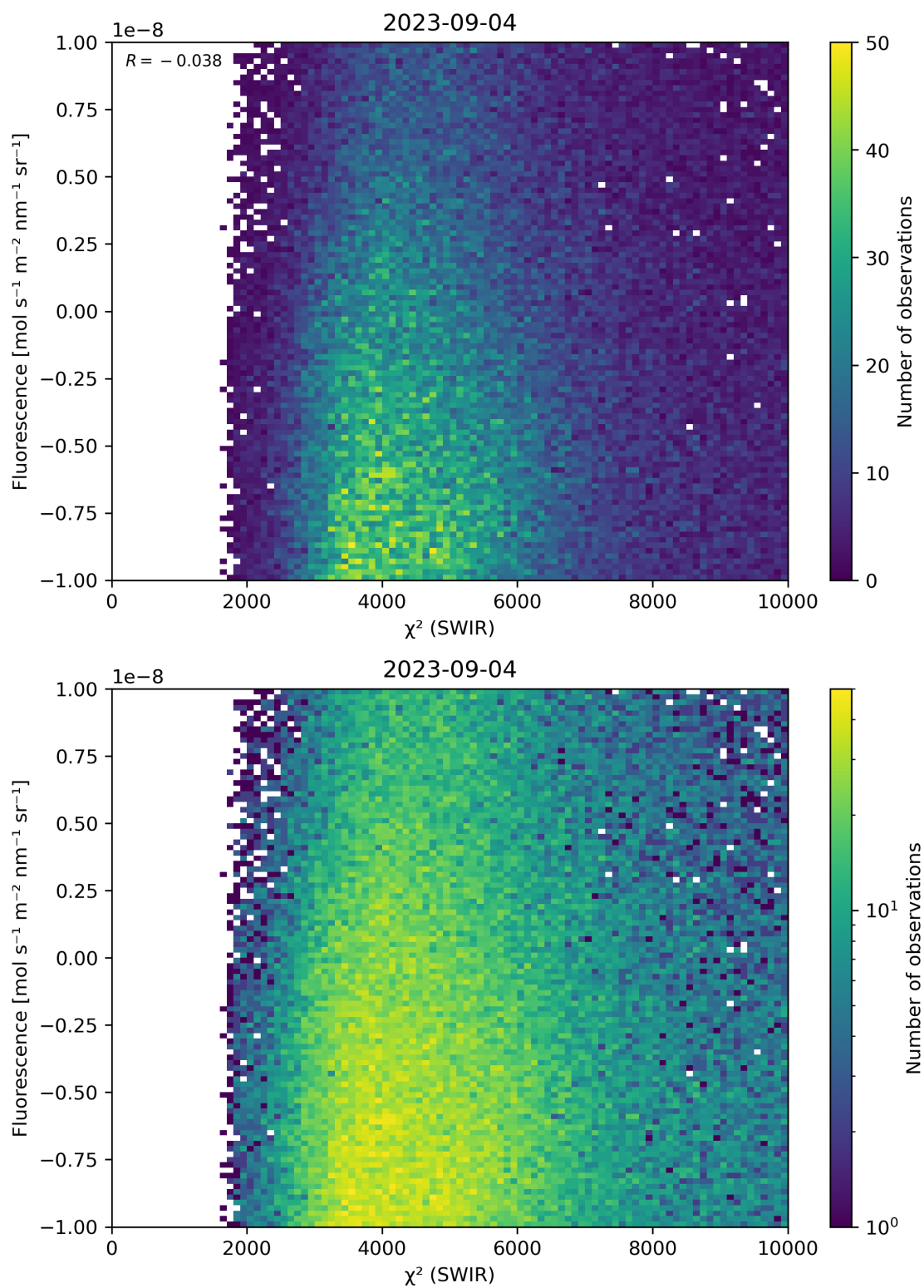
Figure 49: Scatter density plot of “ \chi^2 (SWIR)” against “Fluorescence” for 2023-09-04 to 2023-09-05.
