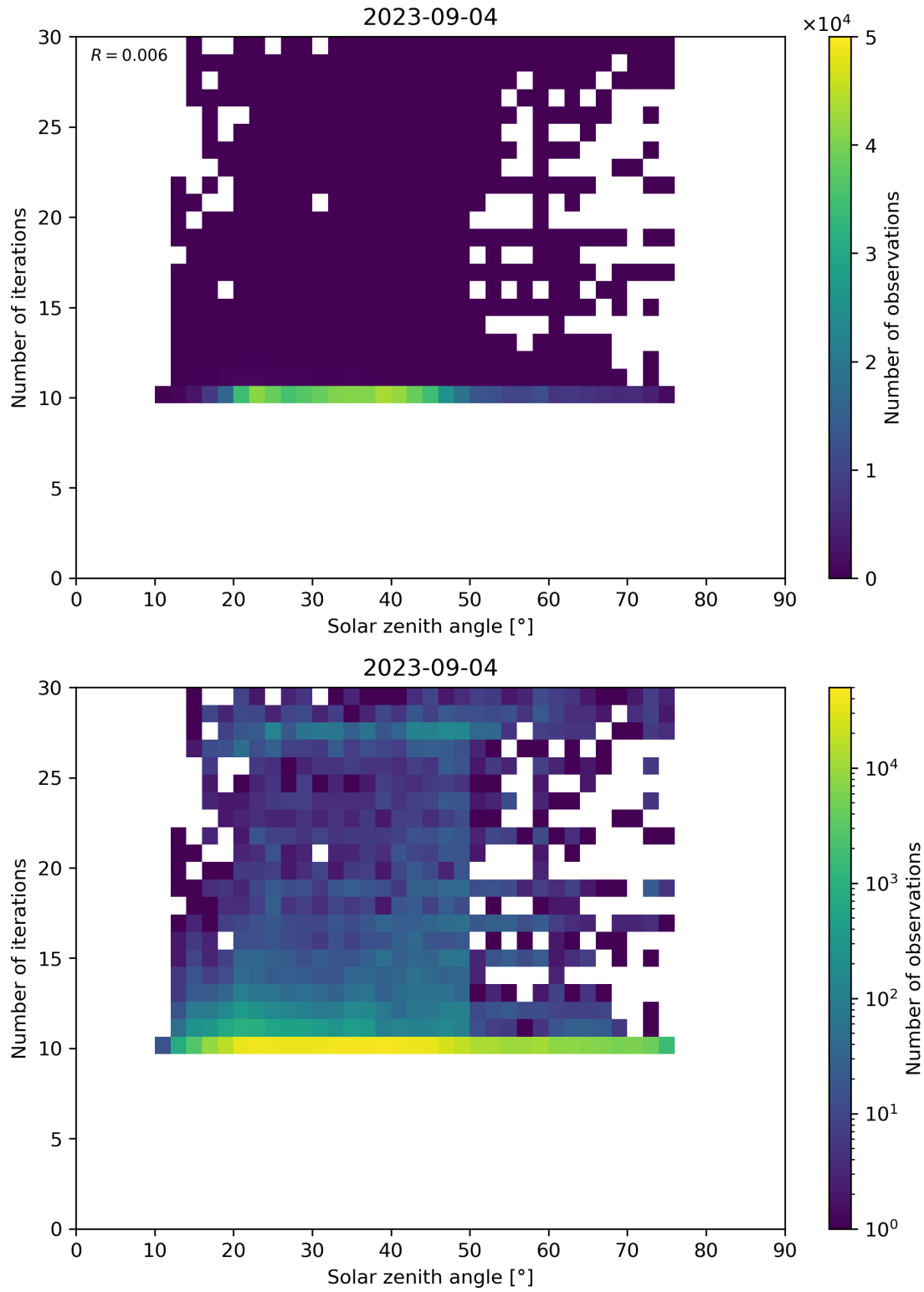
Figure 102: Scatter density plot of “Solar zenith angle” against “Number of iterations” for 2023-09-04 to 2023-09-05.
