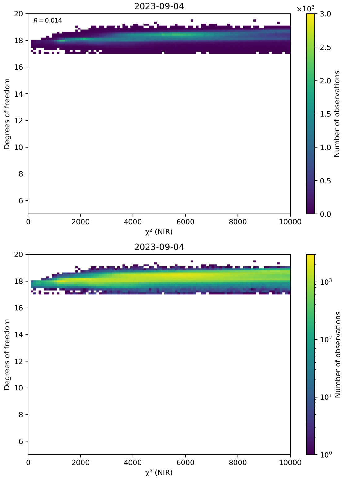
Figure 44: Scatter density plot of “ \chi^2 (NIR)” against “Degrees of freedom” for 2023-09-04 to 2023-09-05.
