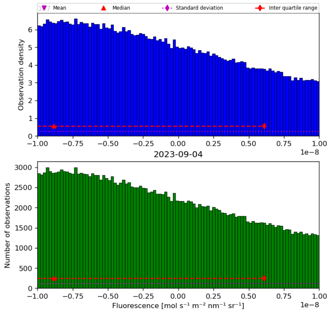
Figure 32: Histogram of “Fluorescence” for 2023-09-04 to 2023-09-05
