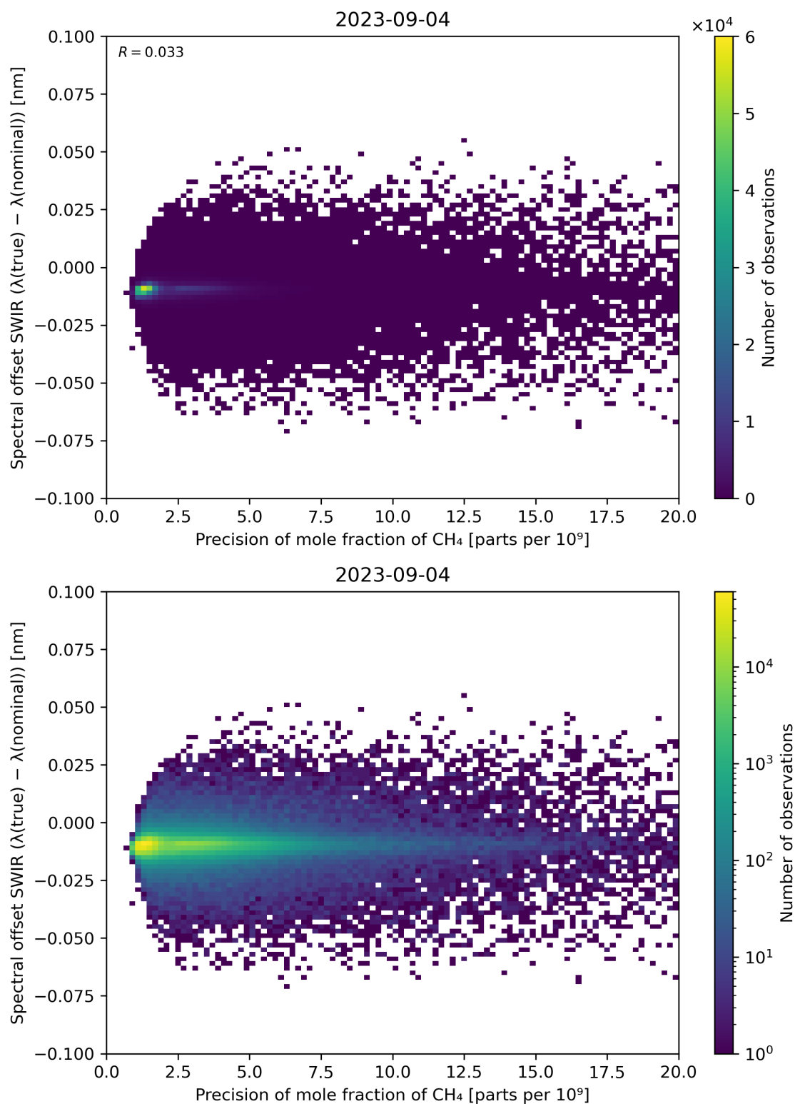
Figure 85: Scatter density plot of “Precision of mole fraction of CH 4 ” against “Spectral offset SWIR ( \lambda(\text{true}) - \lambda(\text{nominal}) )” for 2023-09-04 to 2023-09-05.
