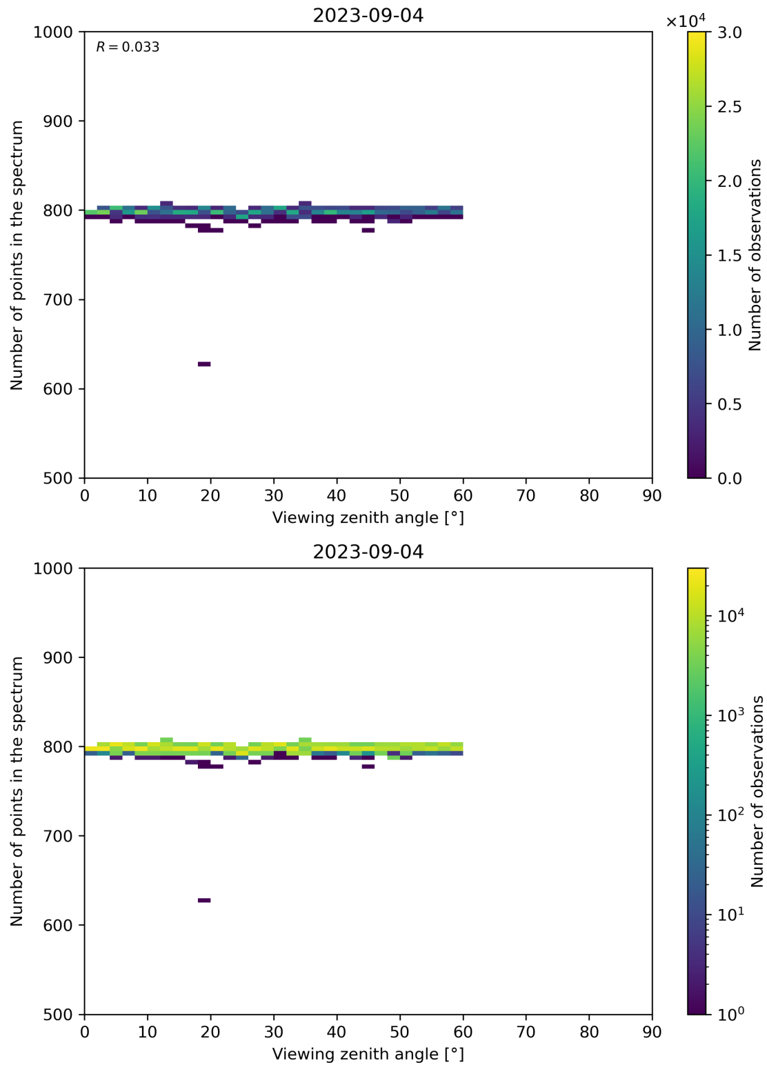
Figure 114: Scatter density plot of “Viewing zenith angle” against “Number of points in the spectrum” for 2023-09-04 to 2023-09-05.
