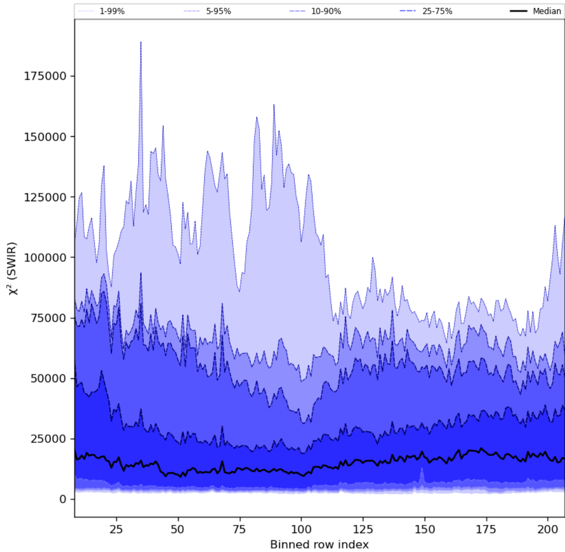
Figure 39: Along track statistics of " \chi^2 (SWIR)" for 2023-09-04 to 2023-09-05
