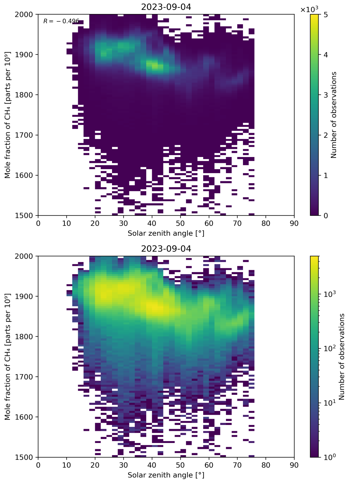
Figure 99: Scatter density plot of “Solar zenith angle” against “Mole fraction of CH 4 ” for 2023-09-04 to 2023-09-05.
