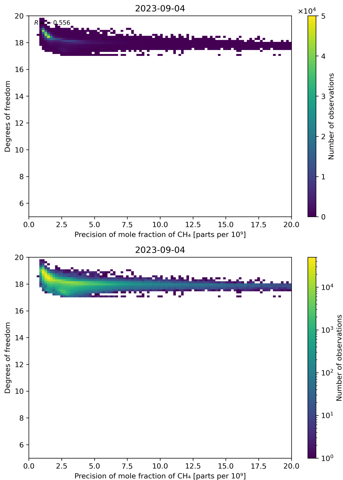
Figure 80: Scatter density plot of “Precision of mole fraction of CH 4 ” against “Degrees of freedom” for 2023-09-04 to 2023-09-05.
