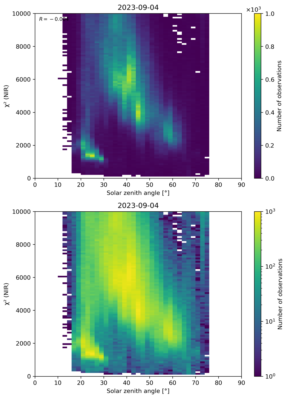
Figure 94: Scatter density plot of “Solar zenith angle” against “ \chi^2 (NIR)” for 2023-09-04 to 2023-09-05.
