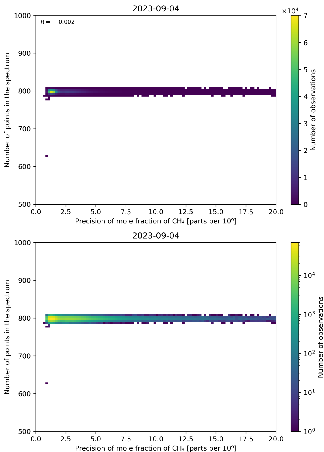
Figure 84: Scatter density plot of “Precision of mole fraction of CH 4 ” against “Number of points in the spectrum” for 2023-09-04 to 2023-09-05.
