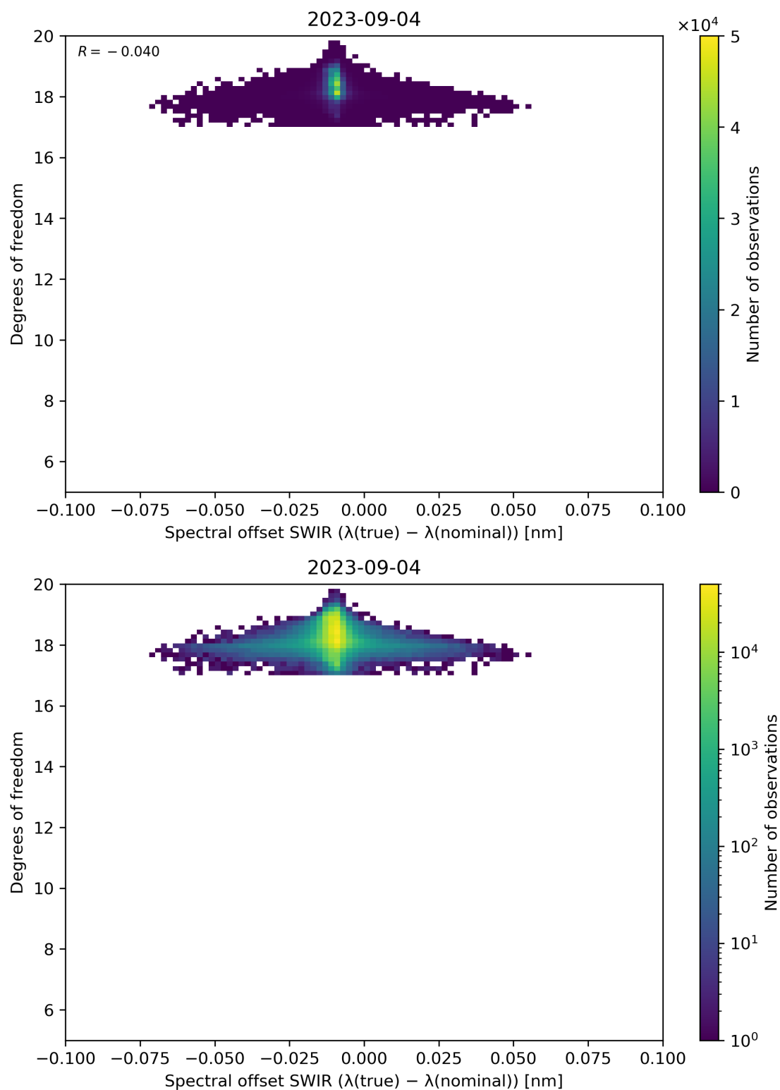
Figure 119: Scatter density plot of “Spectral offset SWIR ( \lambda(\text{true}) - \lambda(\text{nominal}) )” against “Degrees of freedom” for 2023-09-04 to 2023-09-05.
