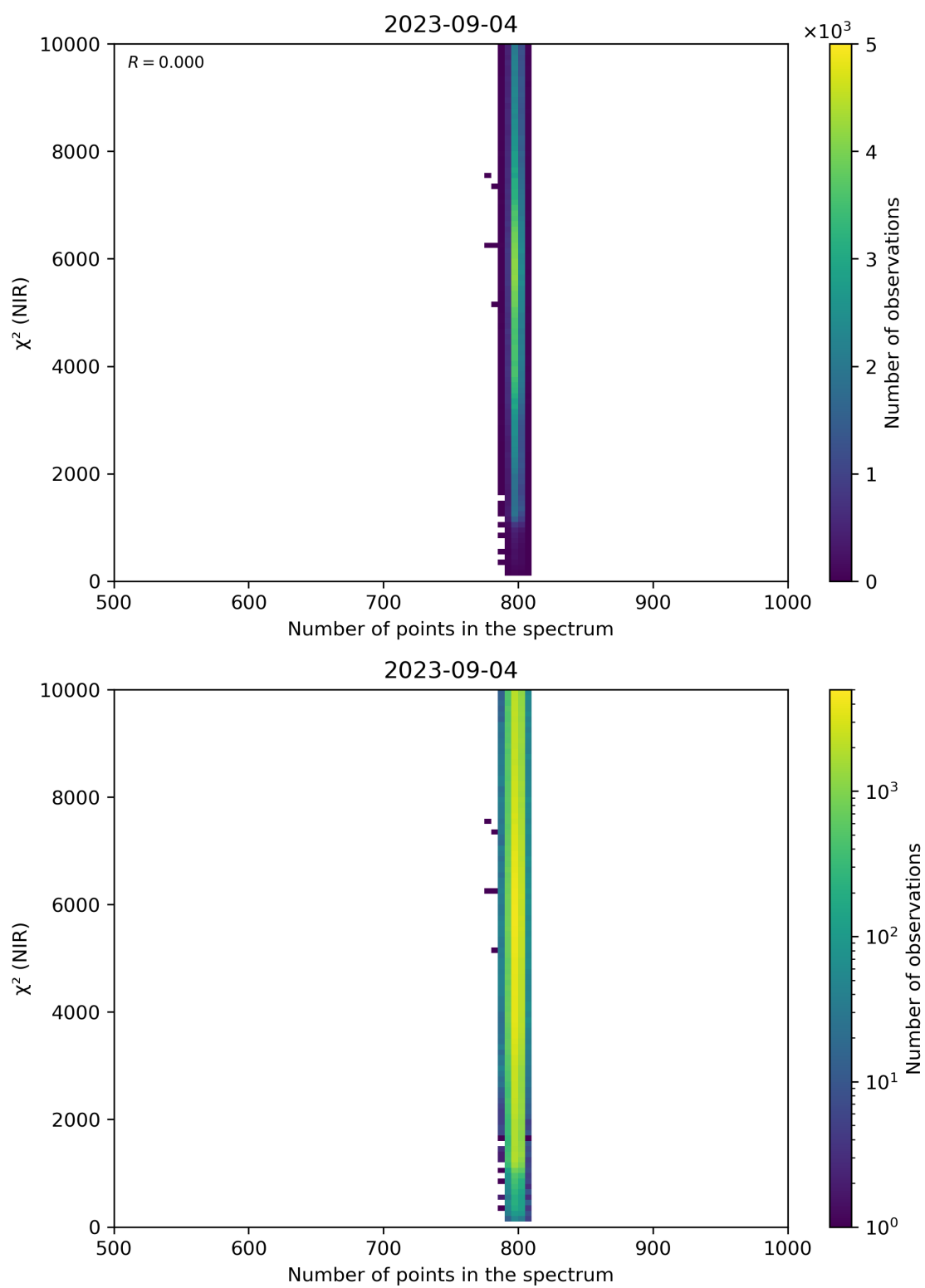
Figure 88: Scatter density plot of “Number of points in the spectrum” against “ \chi^2 (NIR)” for 2023-09-04 to 2023-09-05.
