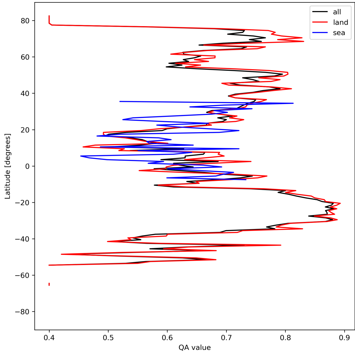
Figure 11: Zonal average of “QA value” for 2023-09-04 to 2023-09-05.
