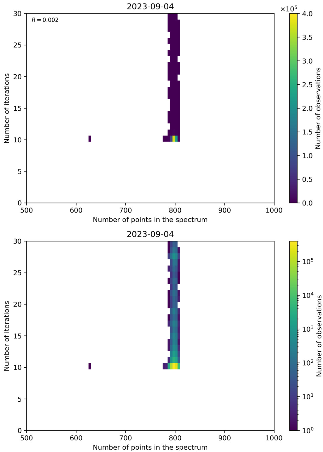
Figure 92: Scatter density plot of “Number of points in the spectrum” against “Number of iterations” for 2023-09-04 to 2023-09-05.
