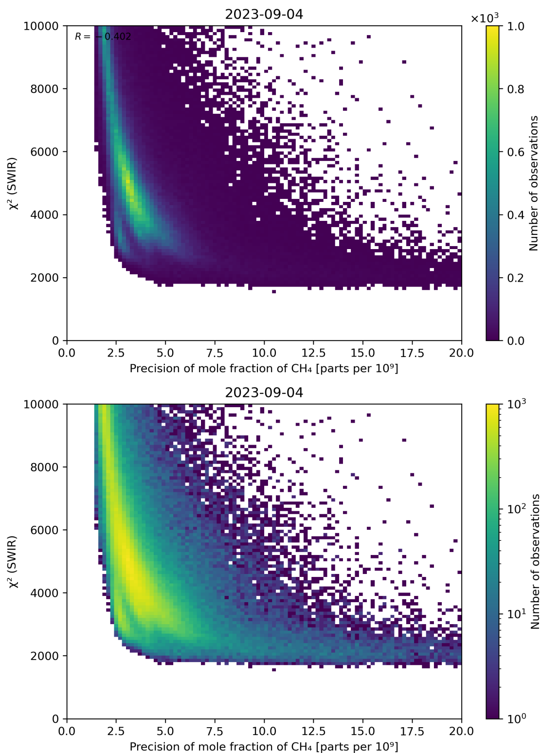
Figure 79: Scatter density plot of “Precision of mole fraction of \text{CH}_4 ” against “ \chi^2 (SWIR)” for 2023-09-04 to 2023-09-05.
