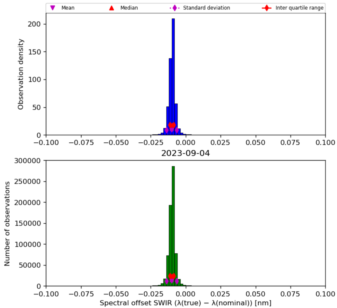
Figure 27: Histogram of “Spectral offset SWIR ( \lambda(\text{true}) - \lambda(\text{nominal}) )” for 2023-09-04 to 2023-09-05
