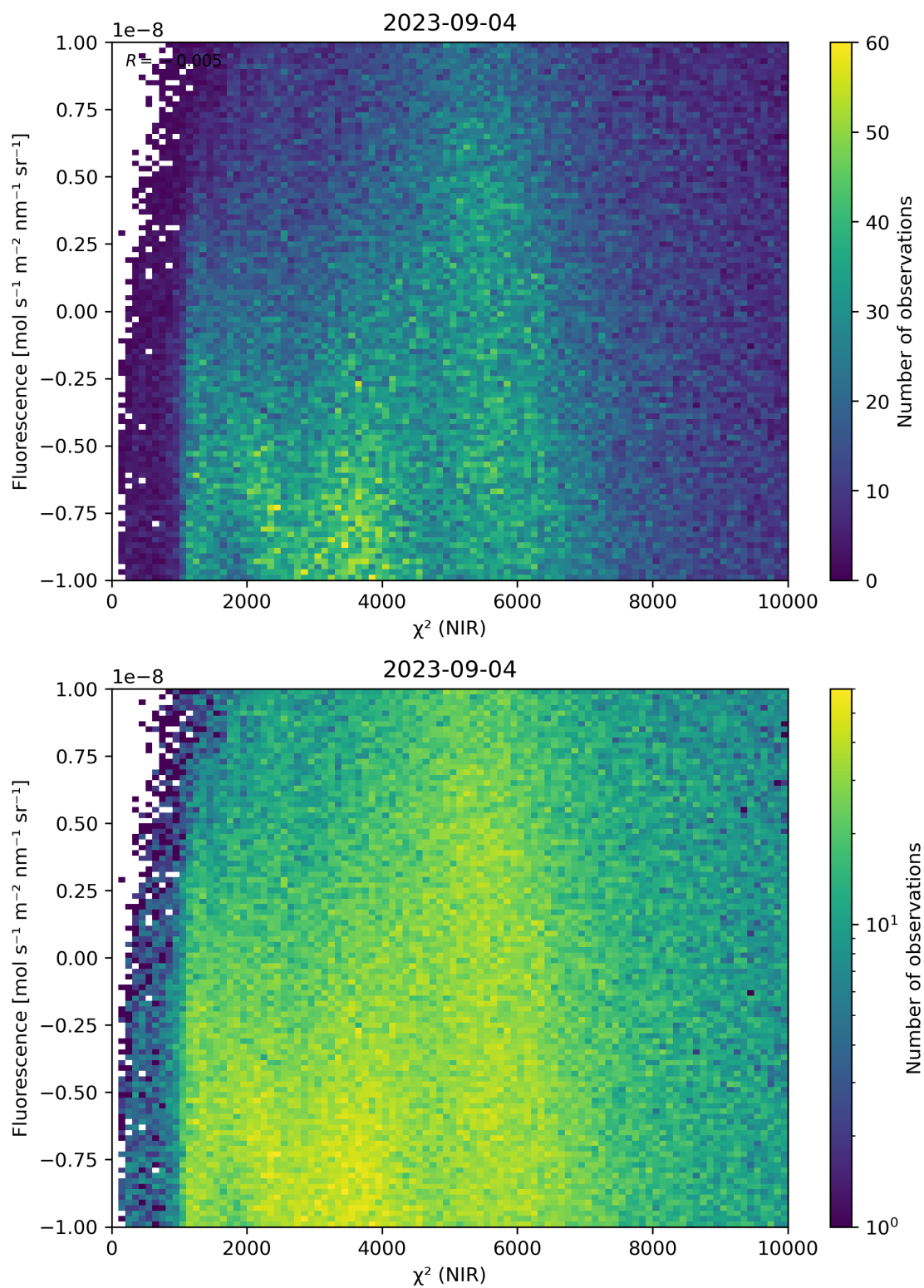
Figure 45: Scatter density plot of “ \chi^2 (NIR)” against “Fluorescence” for 2023-09-04 to 2023-09-05.
