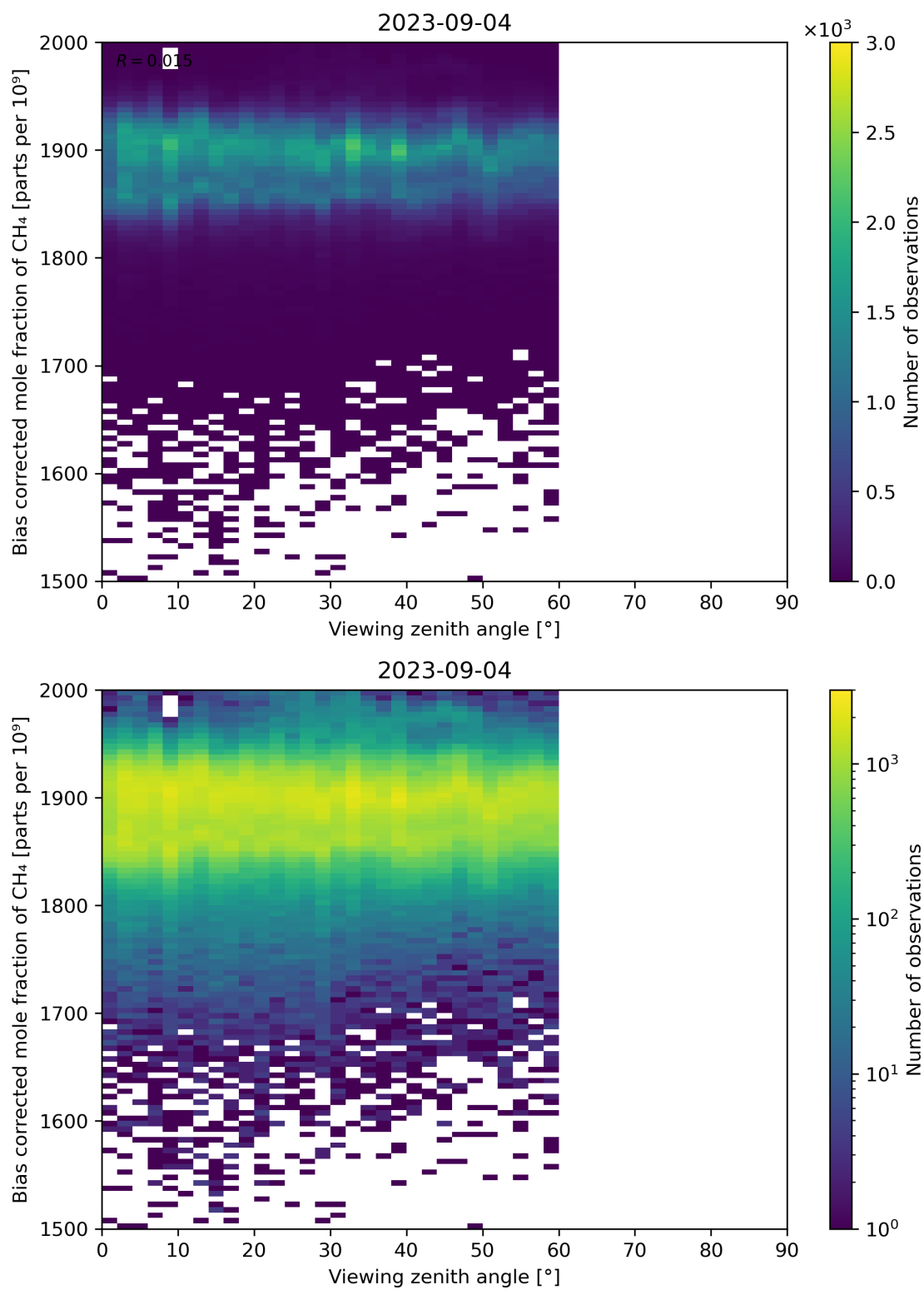
Figure 111: Scatter density plot of “Viewing zenith angle” against “Bias corrected mole fraction of CH 4 ” for 2023-09-04 to 2023-09-05.
