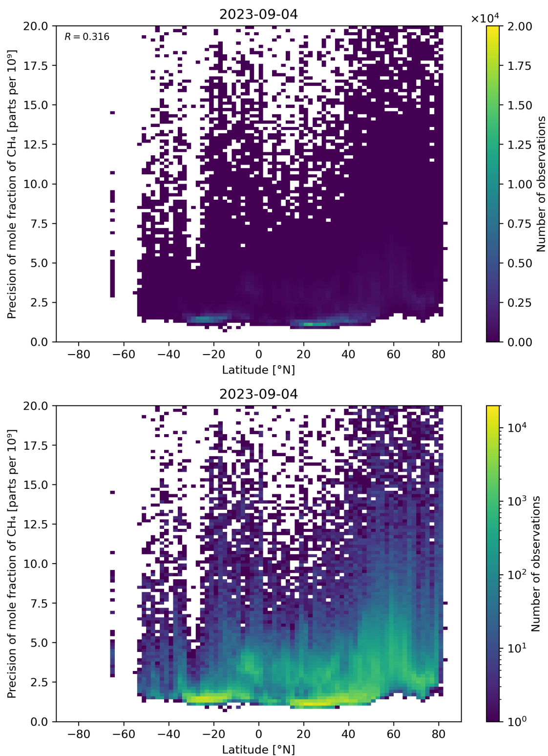
Figure 59: Scatter density plot of “Latitude” against “Precision of mole fraction of \text{CH}_4 ” for 2023-09-04 to 2023-09-05.
