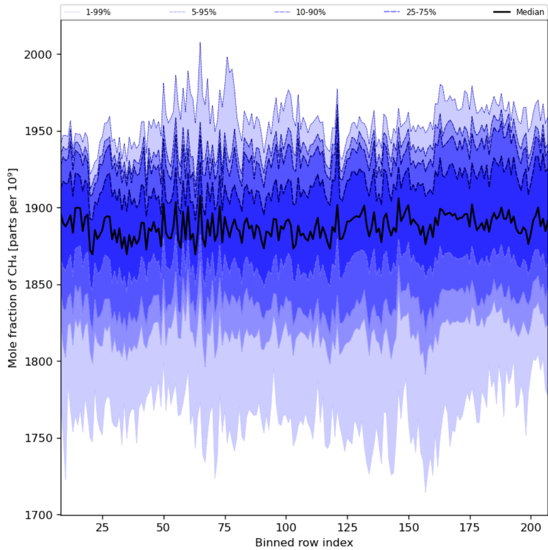
Figure 34: Along track statistics of “Mole fraction of CH 4 ” for 2023-09-04 to 2023-09-05
