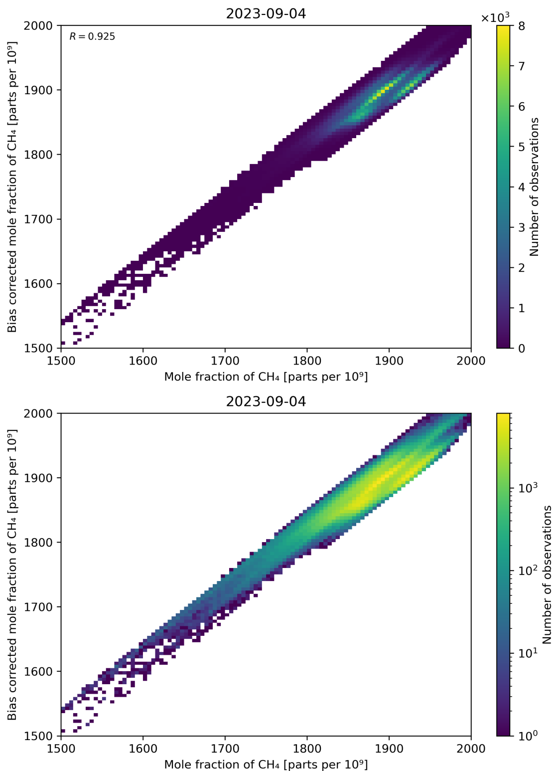
Figure 74: Scatter density plot of “Mole fraction of CH 4 ” against “Bias corrected mole fraction of CH 4 ” for 2023-09-04 to 2023-09-05.
