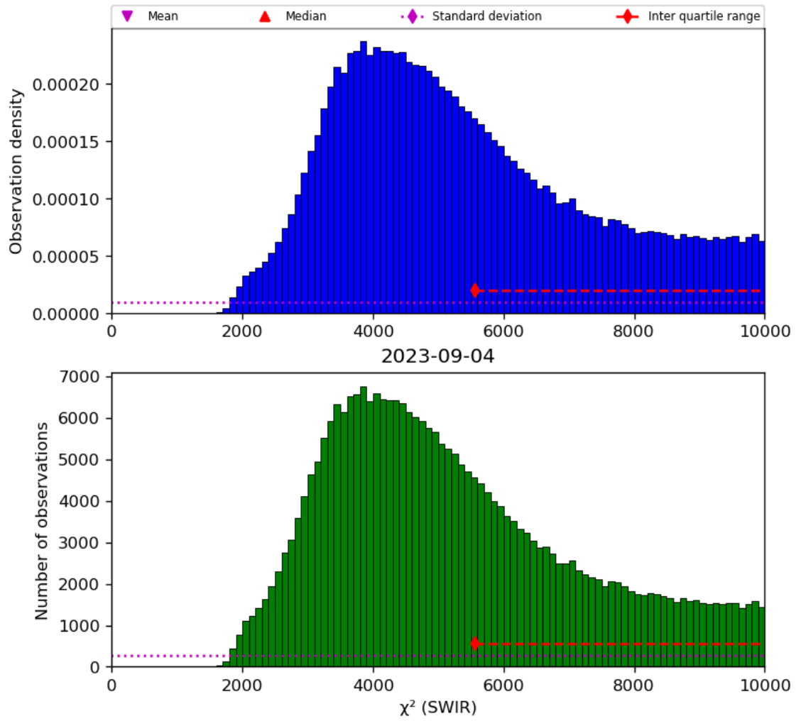
Figure 28: Histogram of “ \chi^2 (SWIR)” for 2023-09-04 to 2023-09-05
