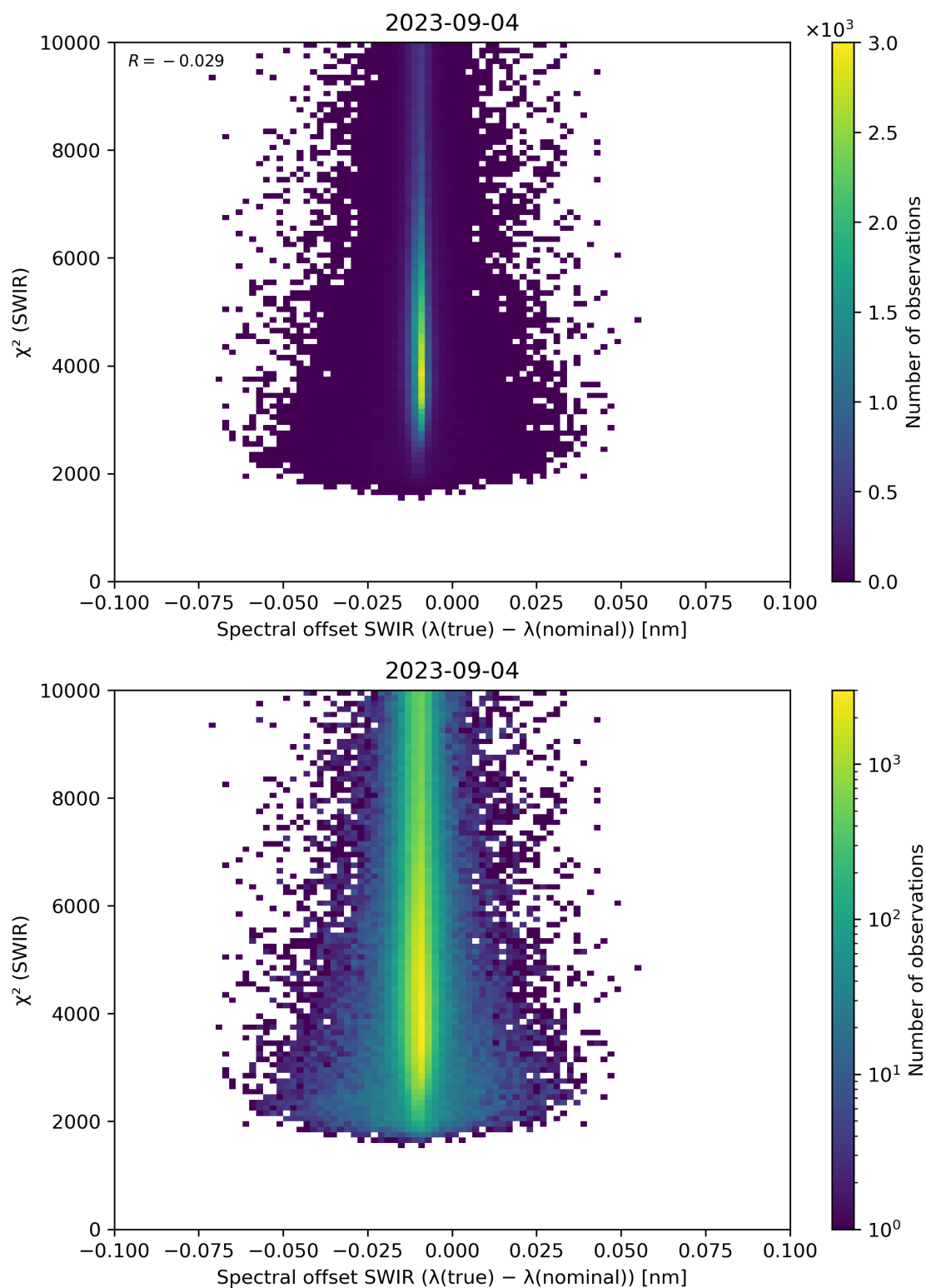
Figure 118: Scatter density plot of “Spectral offset SWIR ( \lambda(\text{true}) - \lambda(\text{nominal}) )” against “ \chi^2 (SWIR)” for 2023-09-04 to 2023-09-05.
