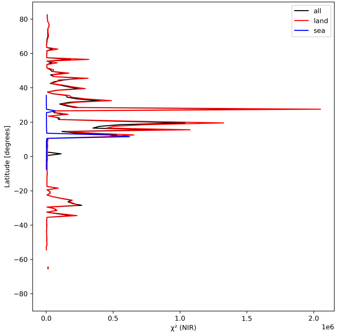
Figure 18: Zonal average of “ \chi^2 (NIR)” for 2023-09-04 to 2023-09-05.
