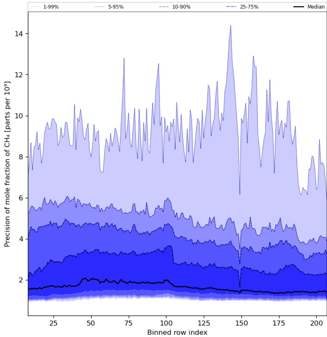
Figure 35: Along track statistics of “Precision of mole fraction of CH 4 ” for 2023-09-04 to 2023-09-05
