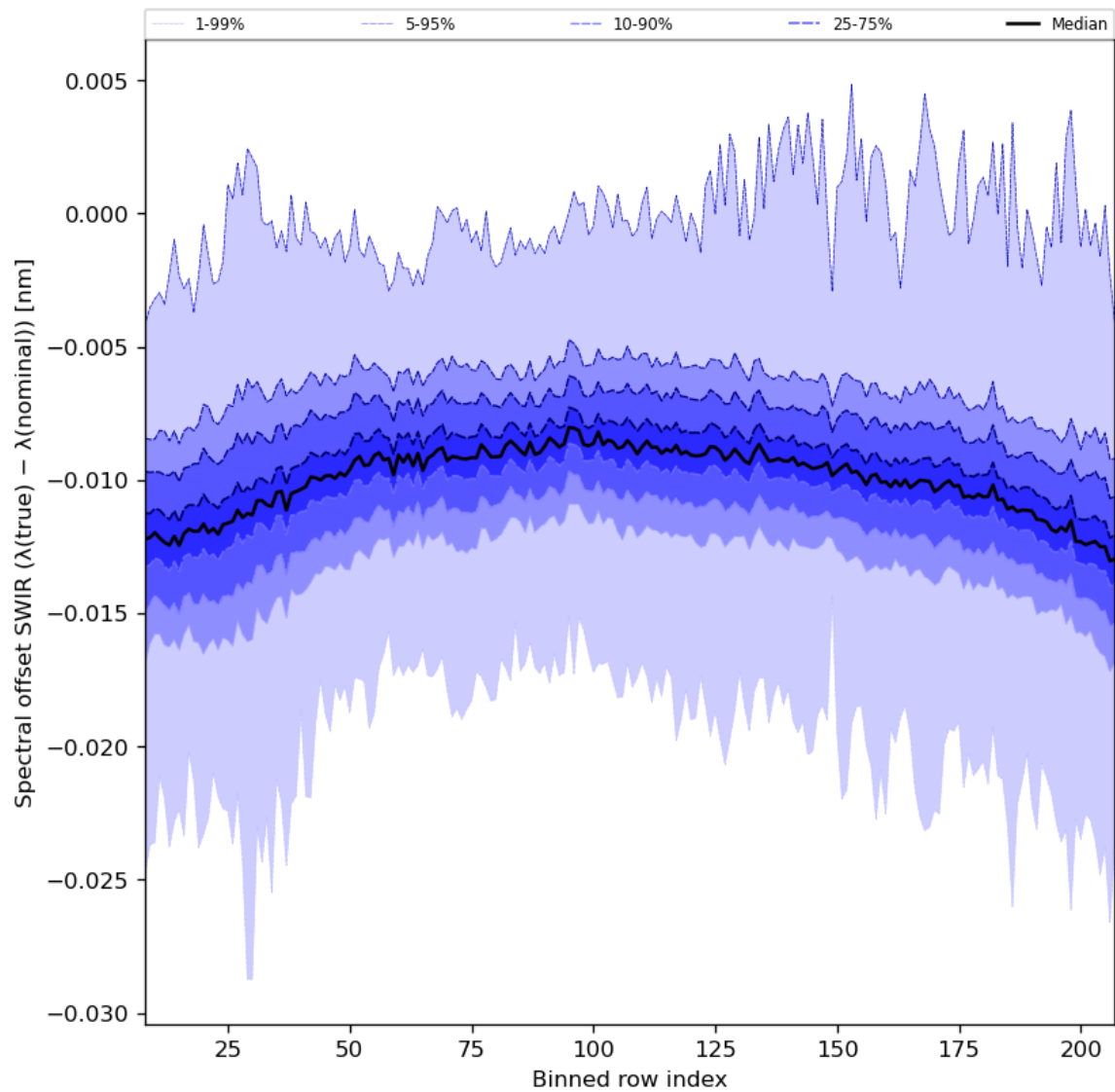
Figure 38: Along track statistics of “Spectral offset SWIR ( \lambda(\text{true}) - \lambda(\text{nominal}) )” for 2023-09-04 to 2023-09-05
