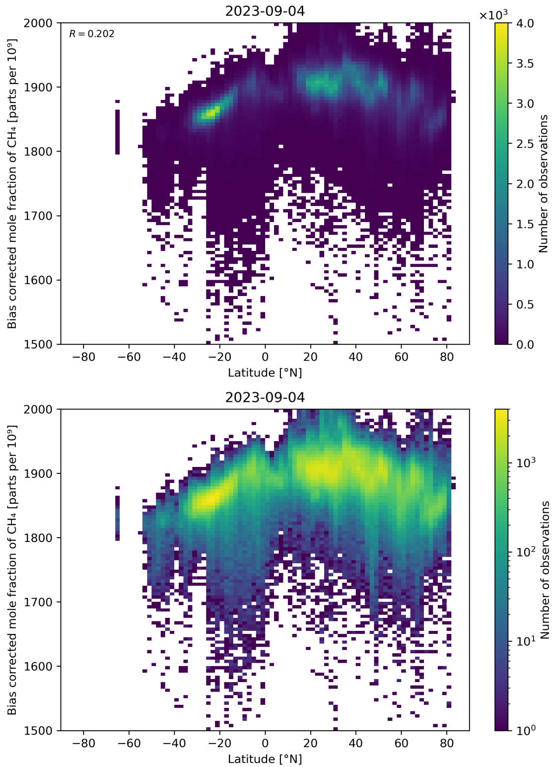
Figure 58: Scatter density plot of “Latitude” against “Bias corrected mole fraction of CH 4 ” for 2023-09-04 to 2023-09-05.
