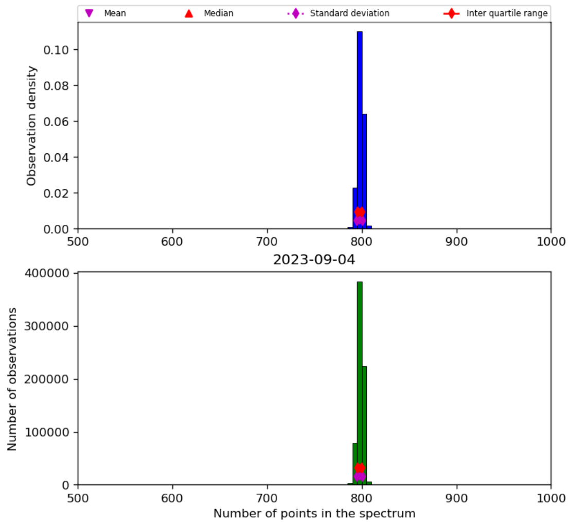
Figure 26: Histogram of “Number of points in the spectrum” for 2023-09-04 to 2023-09-05
