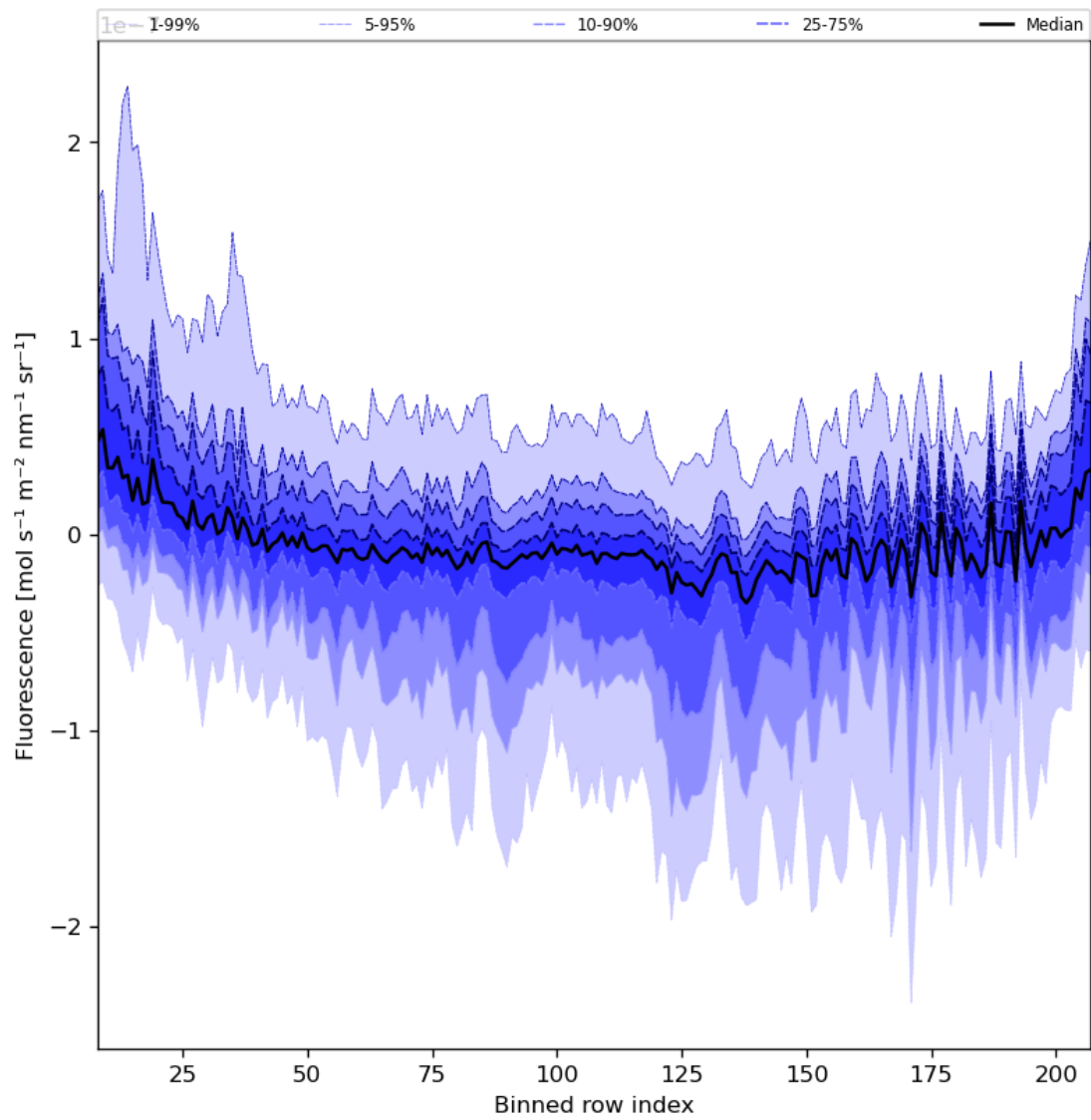
Figure 43: Along track statistics of “Fluorescence” for 2023-09-04 to 2023-09-05
