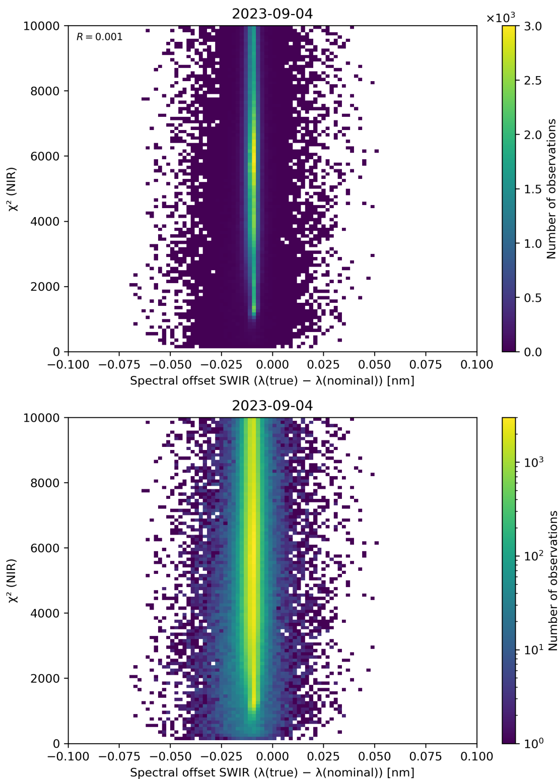
Figure 117: Scatter density plot of “Spectral offset SWIR ( \lambda(\text{true}) - \lambda(\text{nominal}) )” against “ \chi^2 (NIR)” for 2023-09-04 to 2023-09-05.
