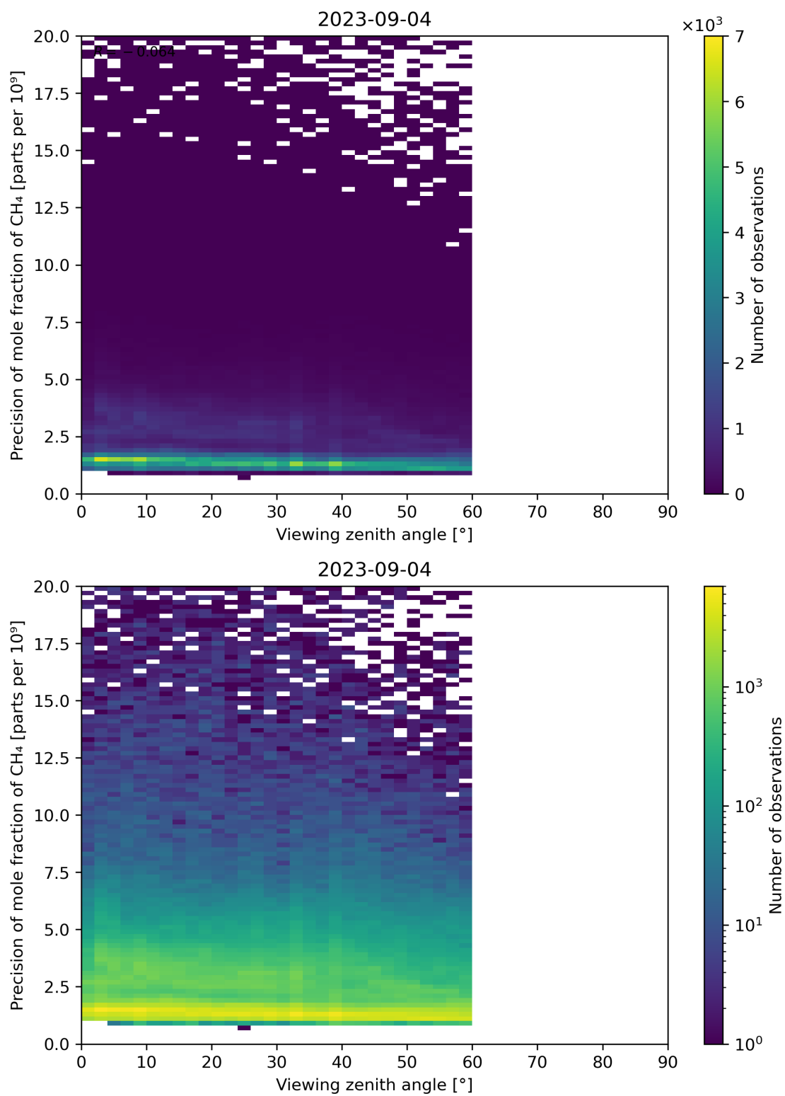
Figure 112: Scatter density plot of “Viewing zenith angle” against “Precision of mole fraction of CH 4 ” for 2023-09-04 to 2023-09-05.
