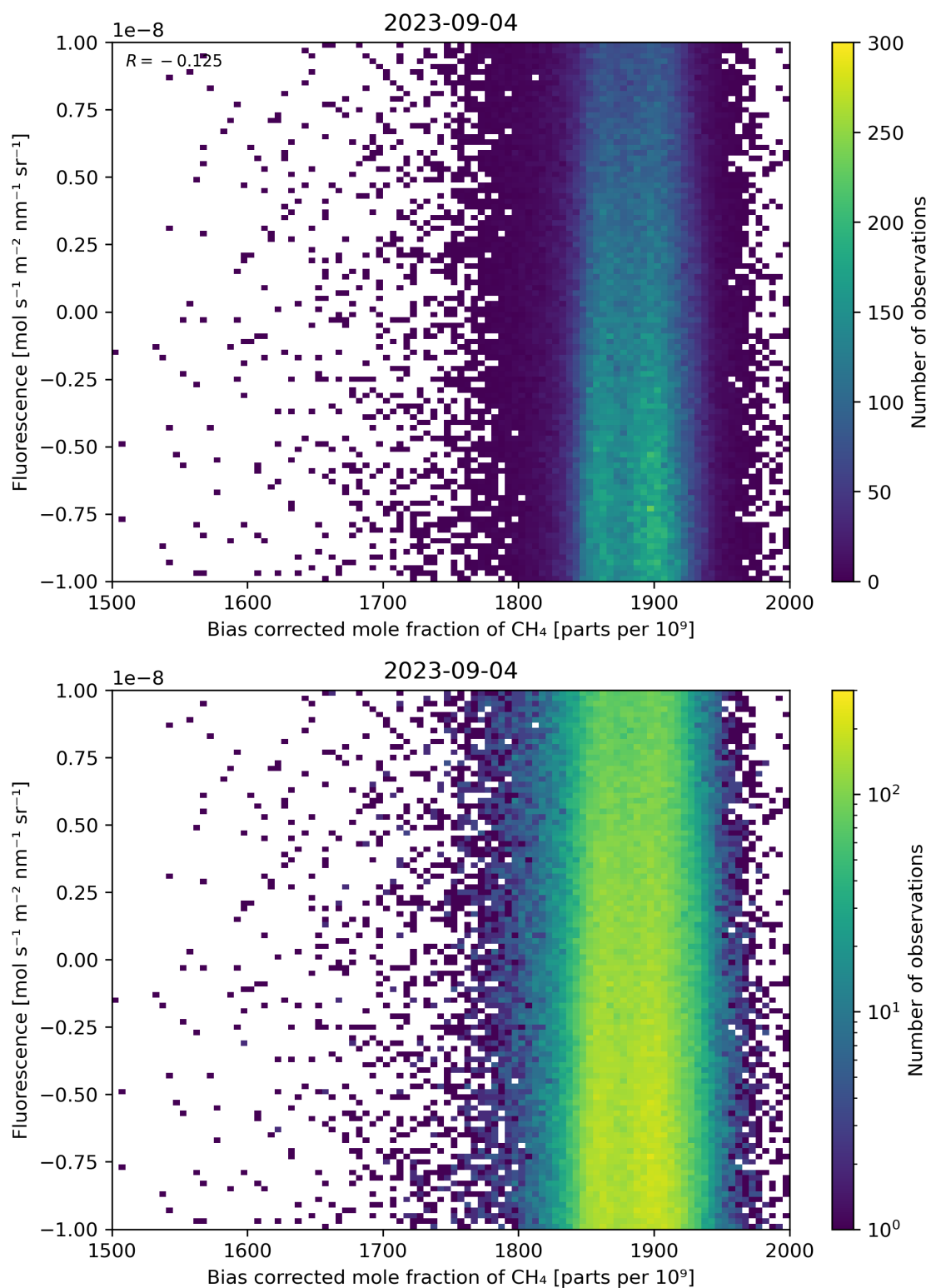
Figure 66: Scatter density plot of “Bias corrected mole fraction of \text{CH}_4 ” against “Fluorescence” for 2023-09-04 to 2023-09-05.
