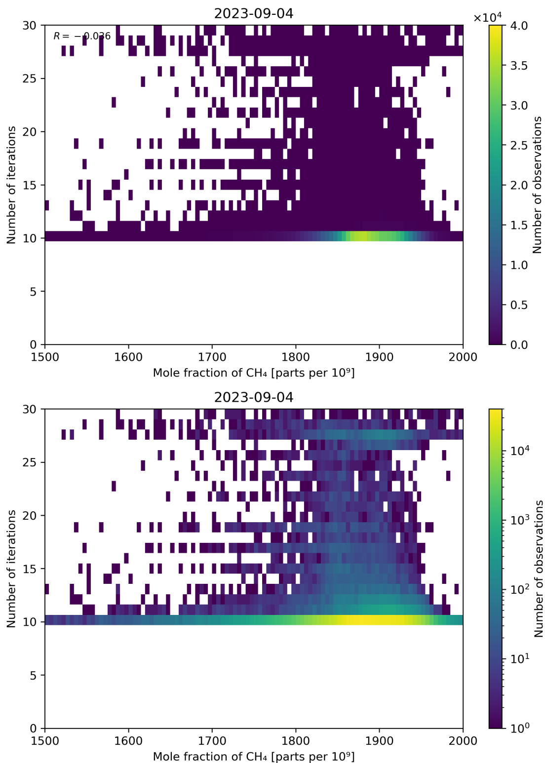
Figure 76: Scatter density plot of “Mole fraction of CH 4 ” against “Number of iterations” for 2023-09-04 to 2023-09-05.
