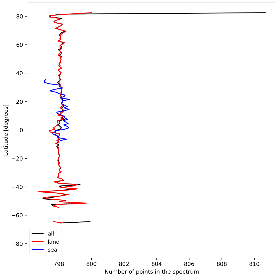
Figure 15: Zonal average of “Number of points in the spectrum” for 2023-09-04 to 2023-09-05.
