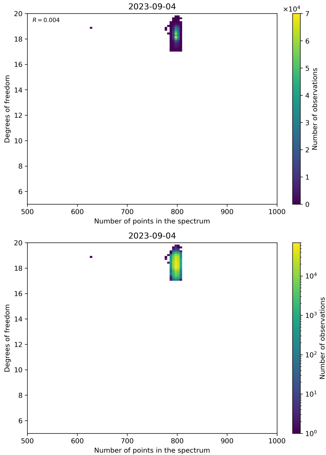
Figure 90: Scatter density plot of “Number of points in the spectrum” against “Degrees of freedom” for 2023-09-04 to 2023-09-05.
