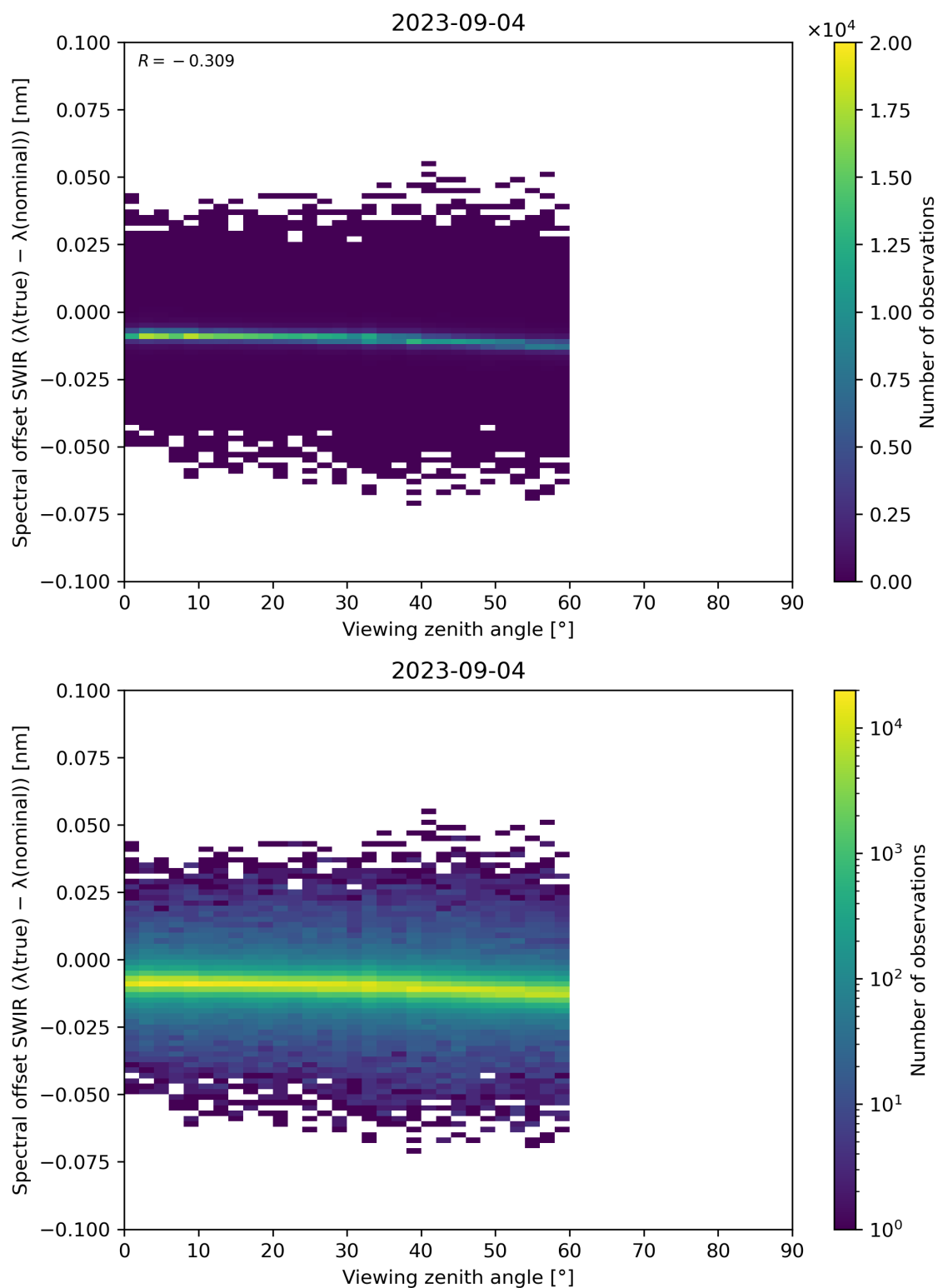
Figure 116: Scatter density plot of “Viewing zenith angle” against “Spectral offset SWIR ( \lambda(\text{true}) - \lambda(\text{nominal}) )” for 2023-09-04 to 2023-09-05.
