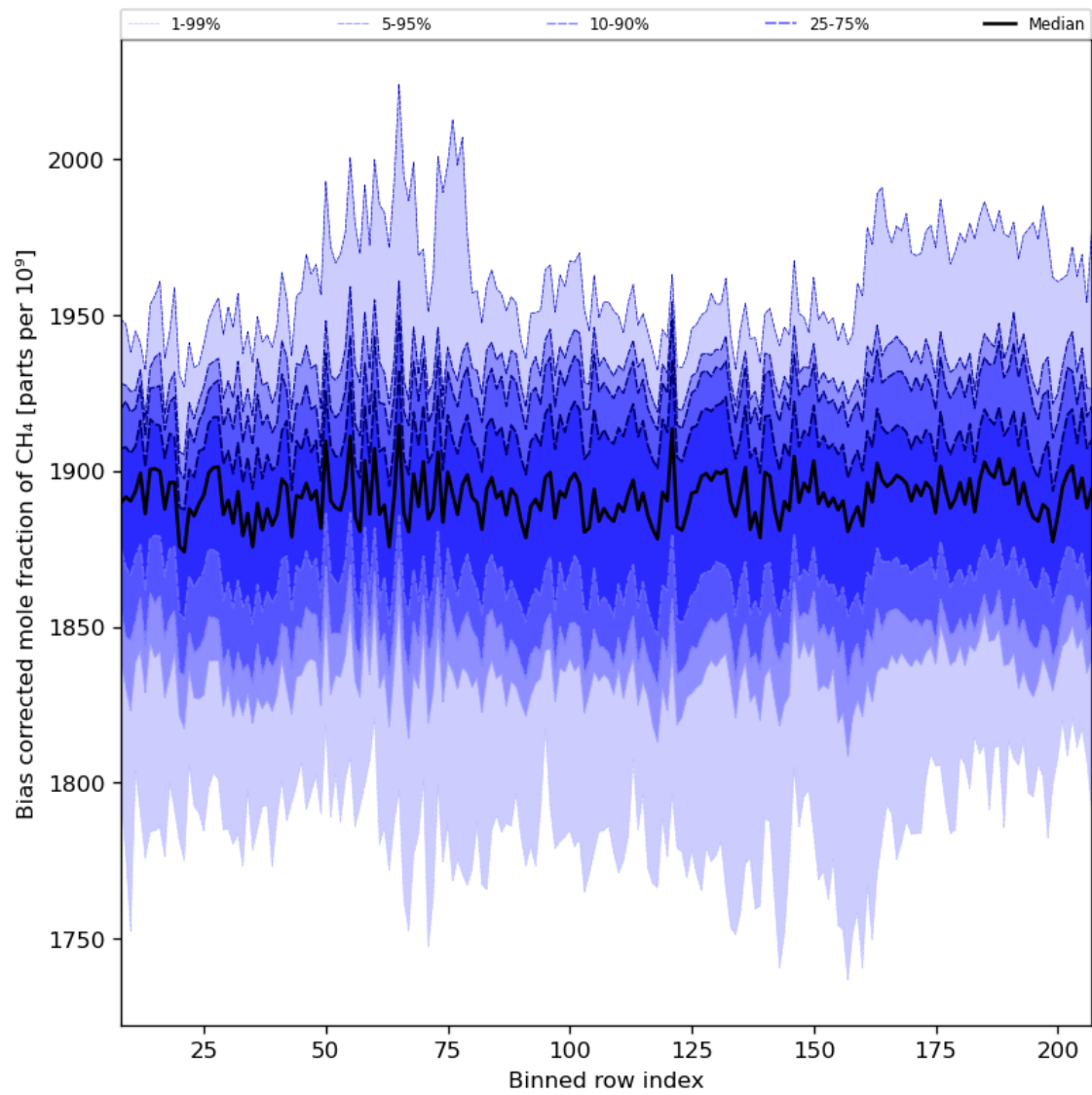
Figure 36: Along track statistics of “Bias corrected mole fraction of CH 4 ” for 2023-09-04 to 2023-09-05
