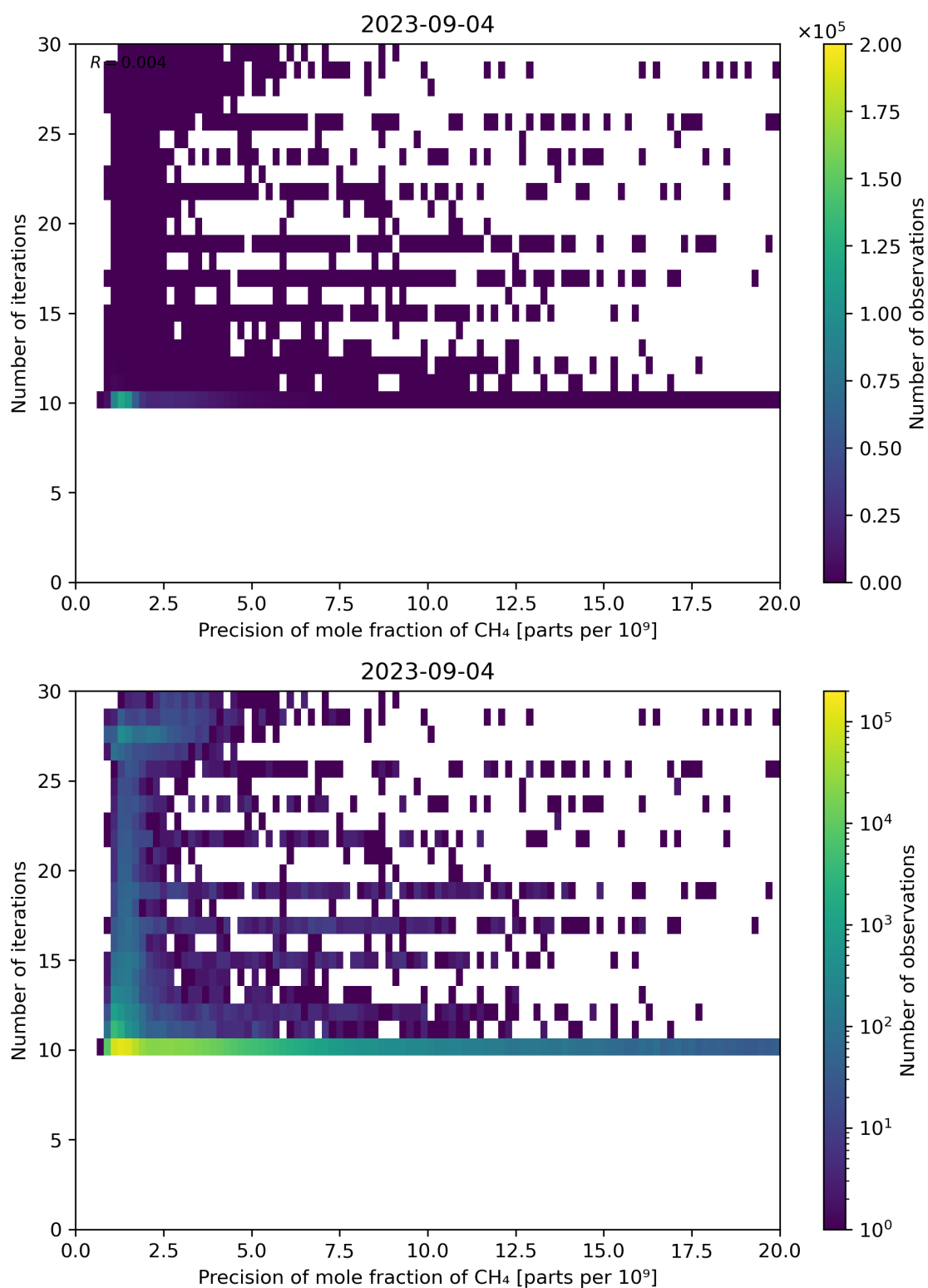
Figure 83: Scatter density plot of “Precision of mole fraction of CH 4 ” against “Number of iterations” for 2023-09-04 to 2023-09-05.
