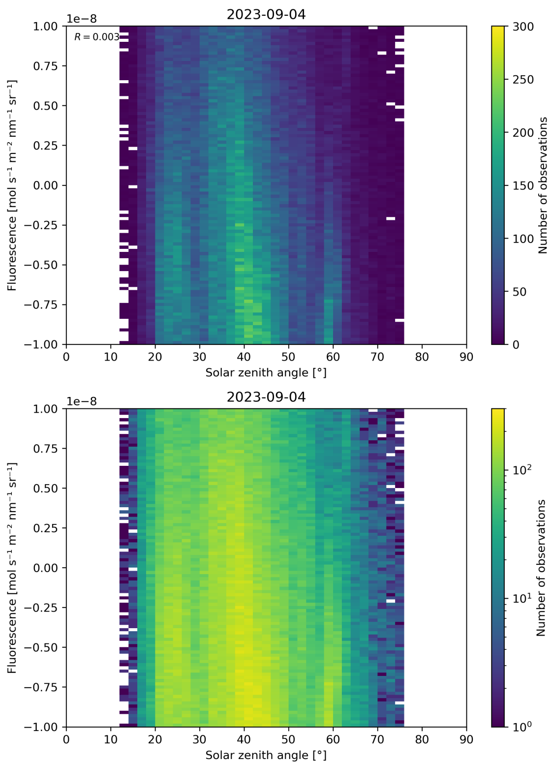
Figure 97: Scatter density plot of “Solar zenith angle” against “Fluorescence” for 2023-09-04 to 2023-09-05.
