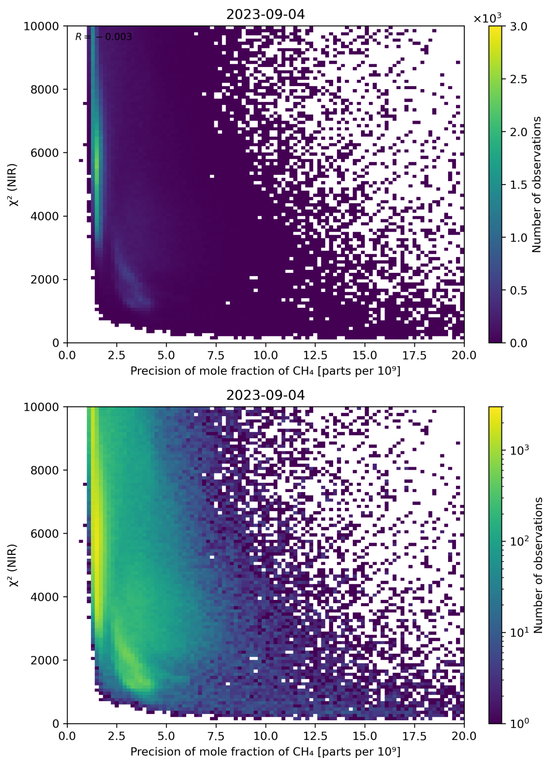
Figure 78: Scatter density plot of “Precision of mole fraction of \text{CH}_4 ” against “ \chi^2 (NIR)” for 2023-09-04 to 2023-09-05.
