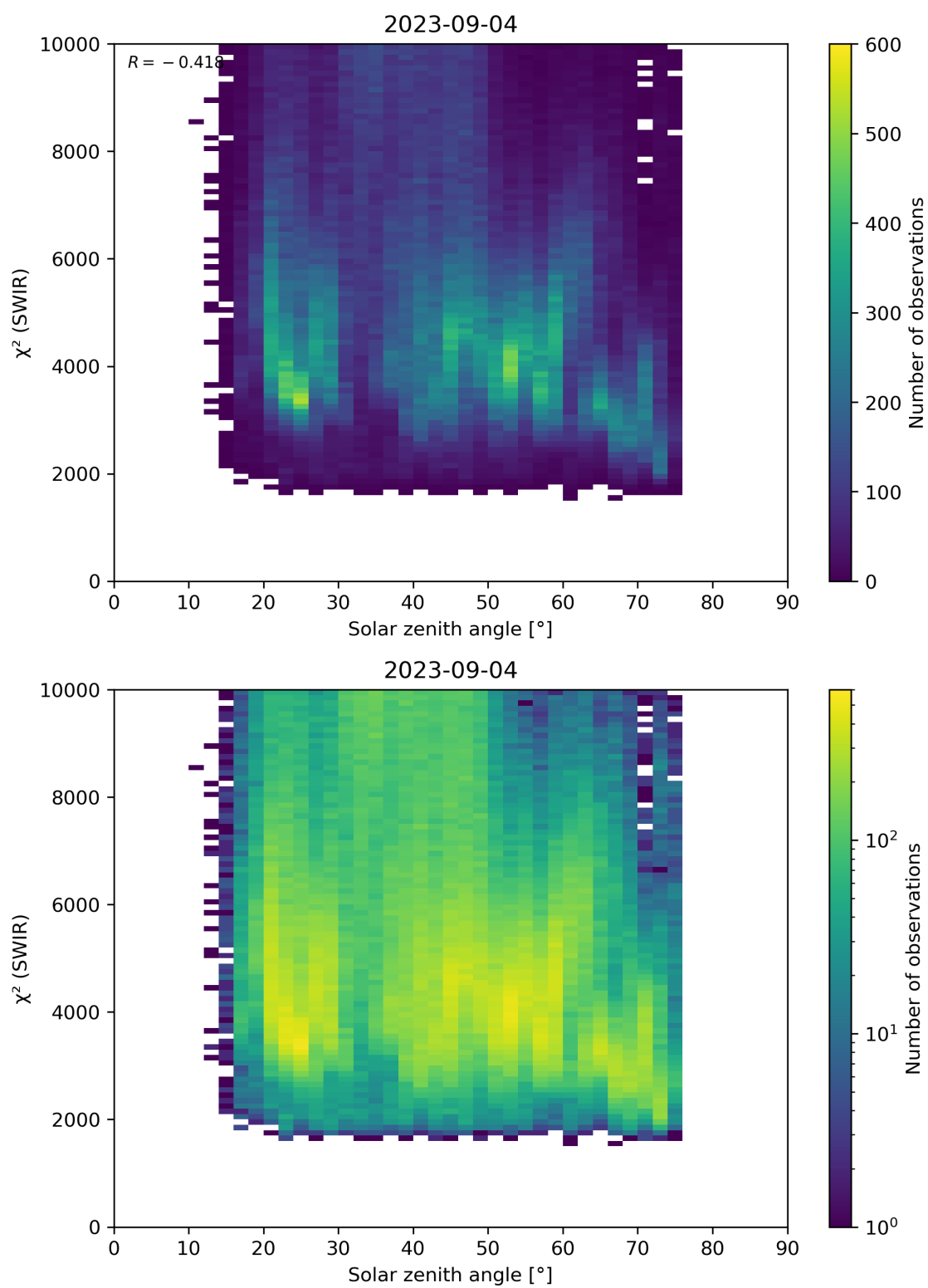
Figure 95: Scatter density plot of “Solar zenith angle” against “ \chi^2 (SWIR)” for 2023-09-04 to 2023-09-05.
