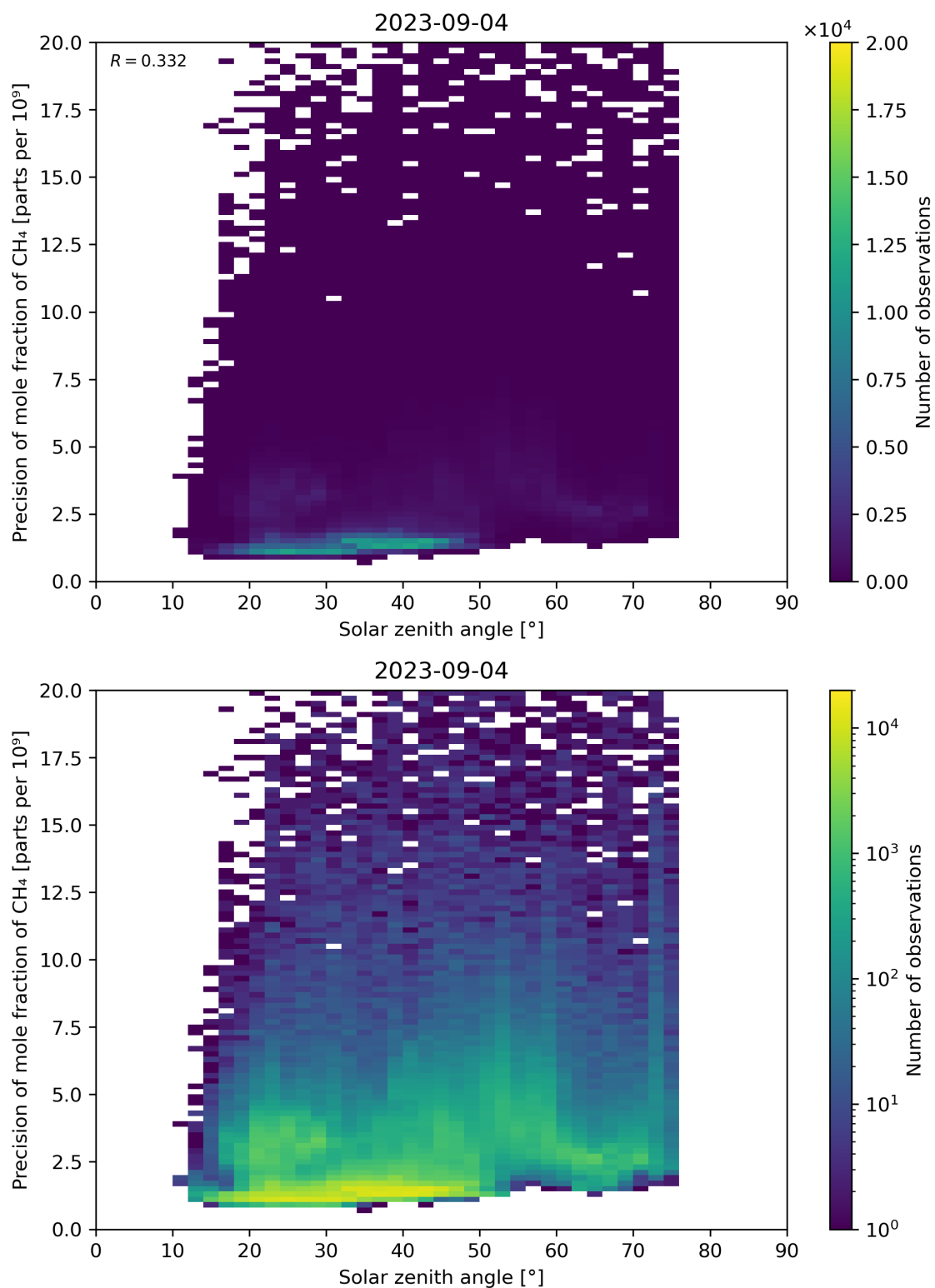
Figure 101: Scatter density plot of “Solar zenith angle” against “Precision of mole fraction of CH 4 ” for 2023-09-04 to 2023-09-05.
