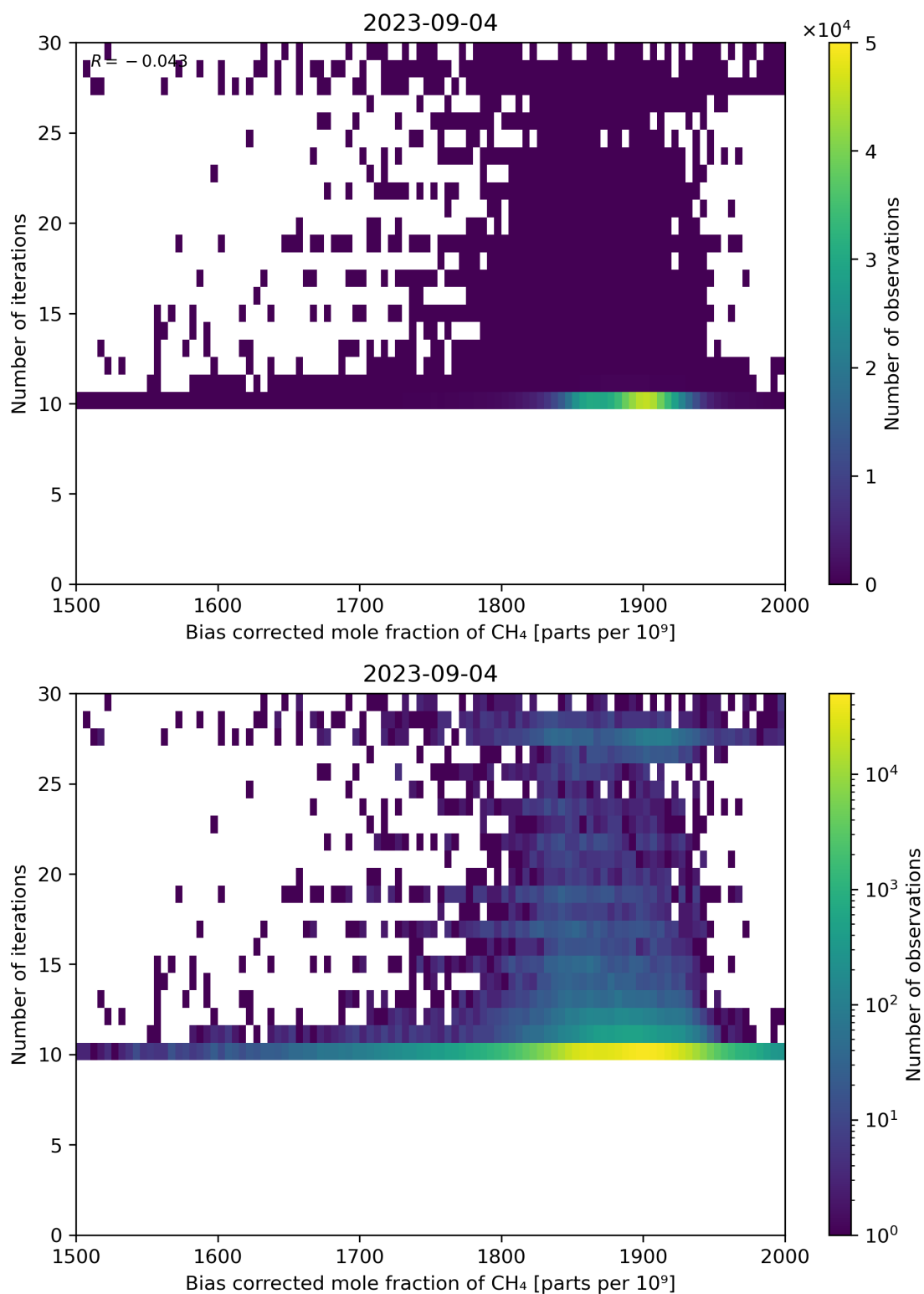
Figure 67: Scatter density plot of “Bias corrected mole fraction of CH 4 ” against “Number of iterations” for 2023-09-04 to 2023-09-05.
