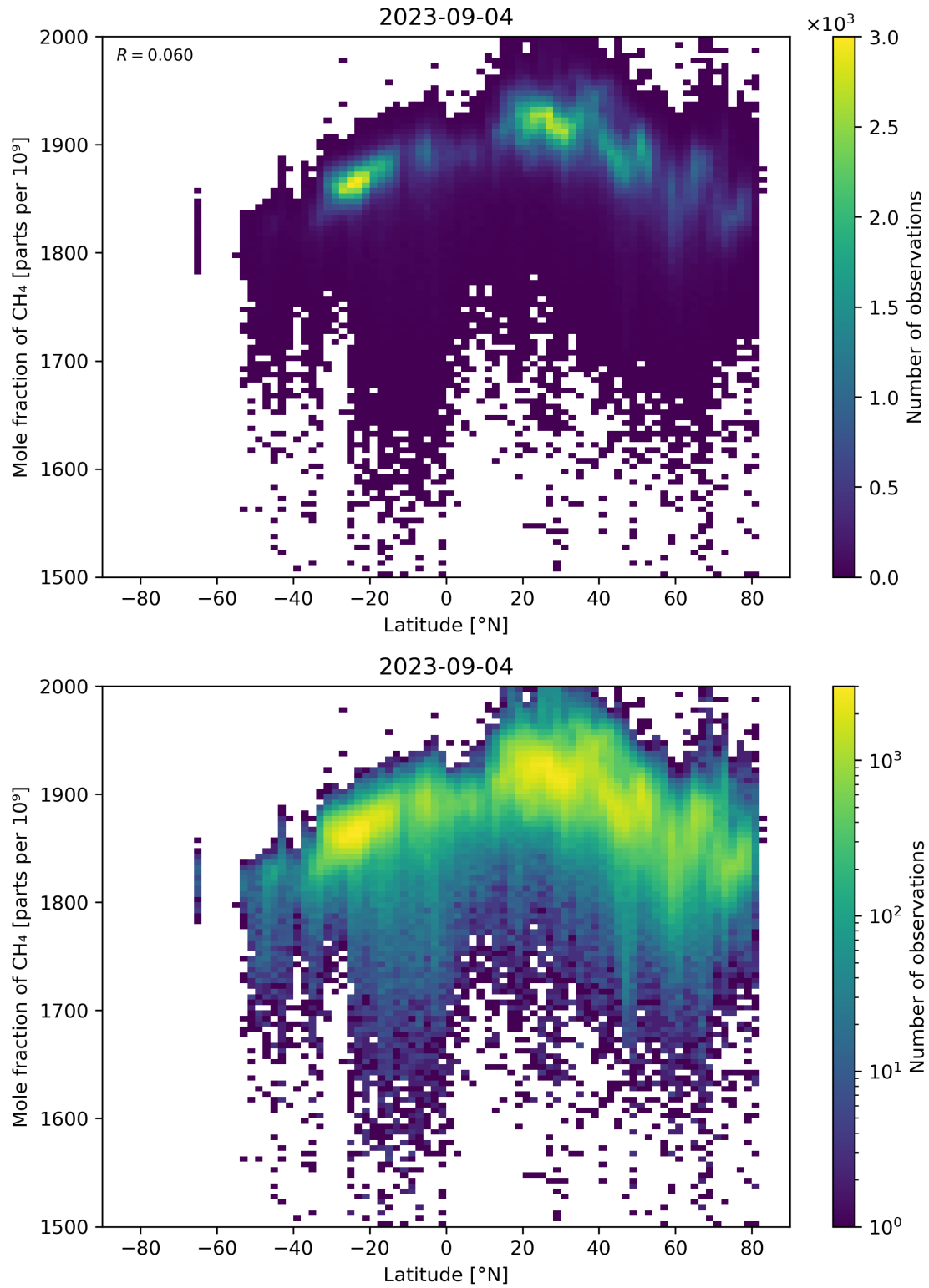
Figure 57: Scatter density plot of “Latitude” against “Mole fraction of \text{CH}_4 ” for 2023-09-04 to 2023-09-05.
