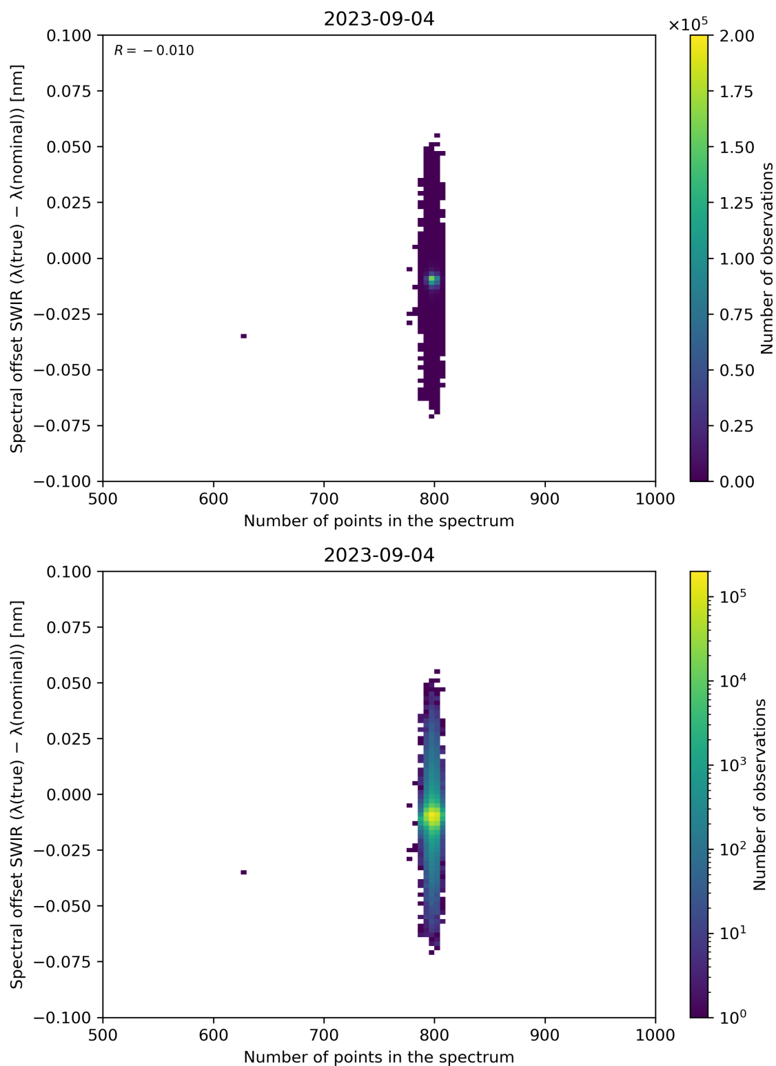
Figure 93: Scatter density plot of “Number of points in the spectrum” against “Spectral offset SWIR ( \lambda(\text{true}) - \lambda(\text{nominal}) )” for 2023-09-04 to 2023-09-05.
