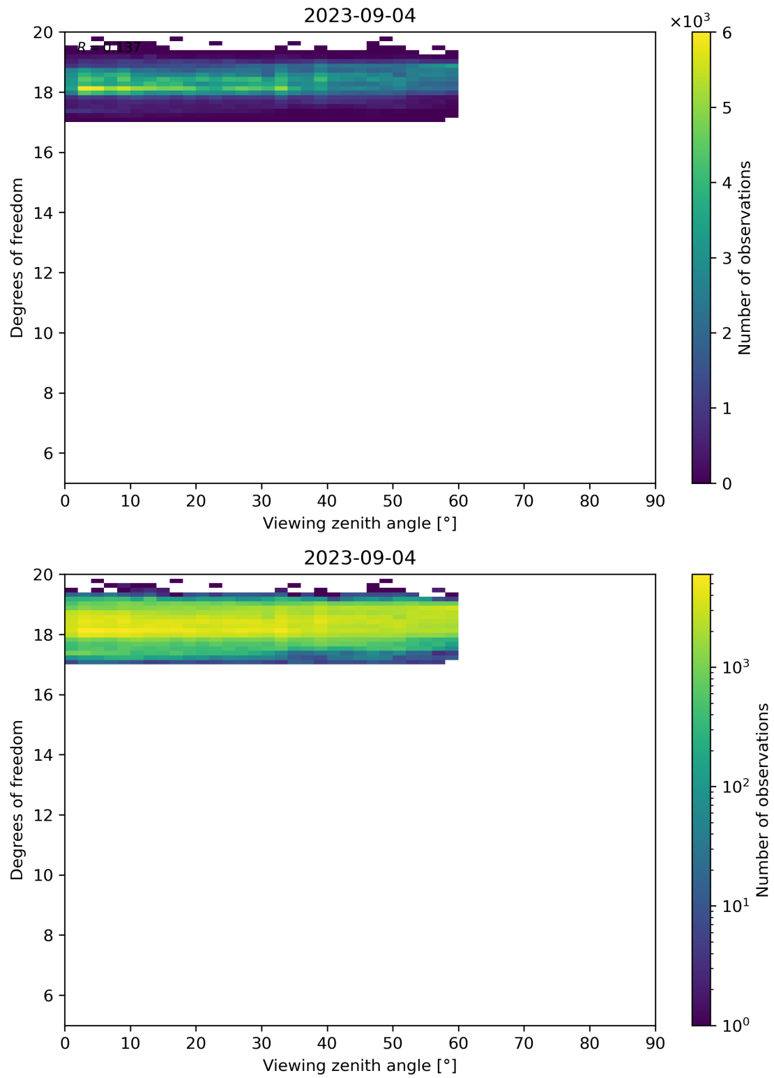
Figure 107: Scatter density plot of “Viewing zenith angle” against “Degrees of freedom” for 2023-09-04 to 2023-09-05.
