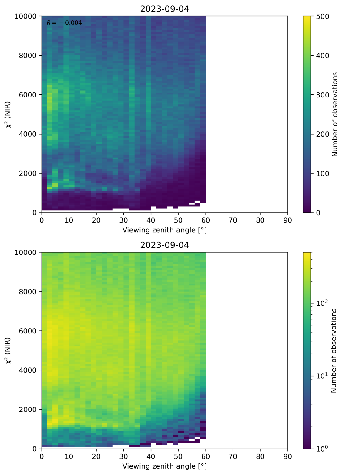
Figure 105: Scatter density plot of “Viewing zenith angle” against “ \chi^2 (NIR)” for 2023-09-04 to 2023-09-05.
