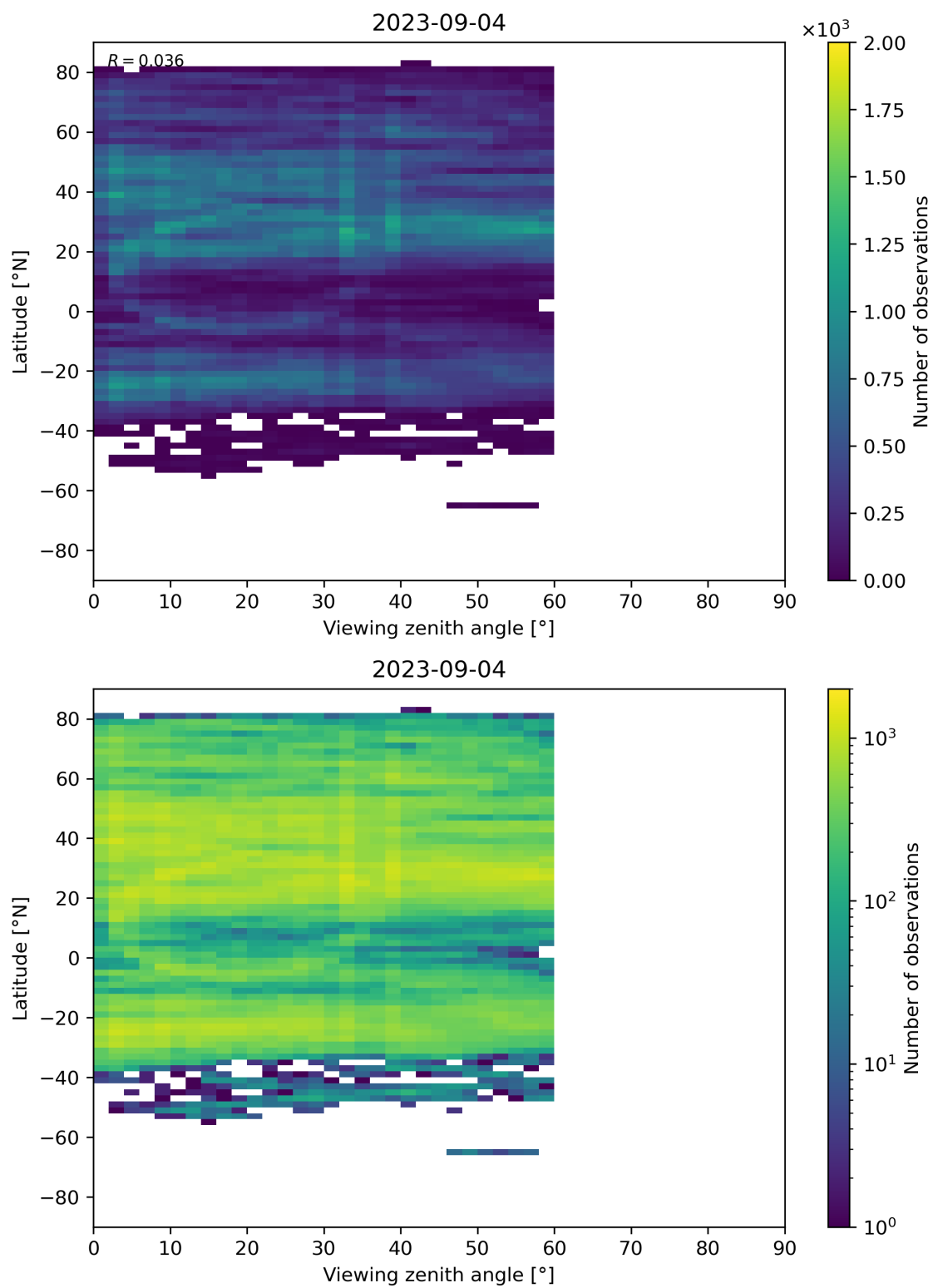
Figure 109: Scatter density plot of “Viewing zenith angle” against “Latitude” for 2023-09-04 to 2023-09-05.
