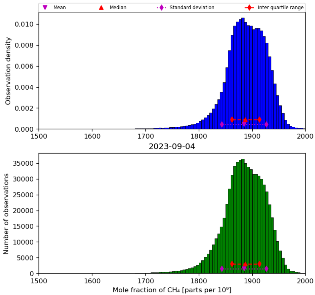
Figure 23: Histogram of “Mole fraction of CH 4 ” for 2023-09-04 to 2023-09-05
