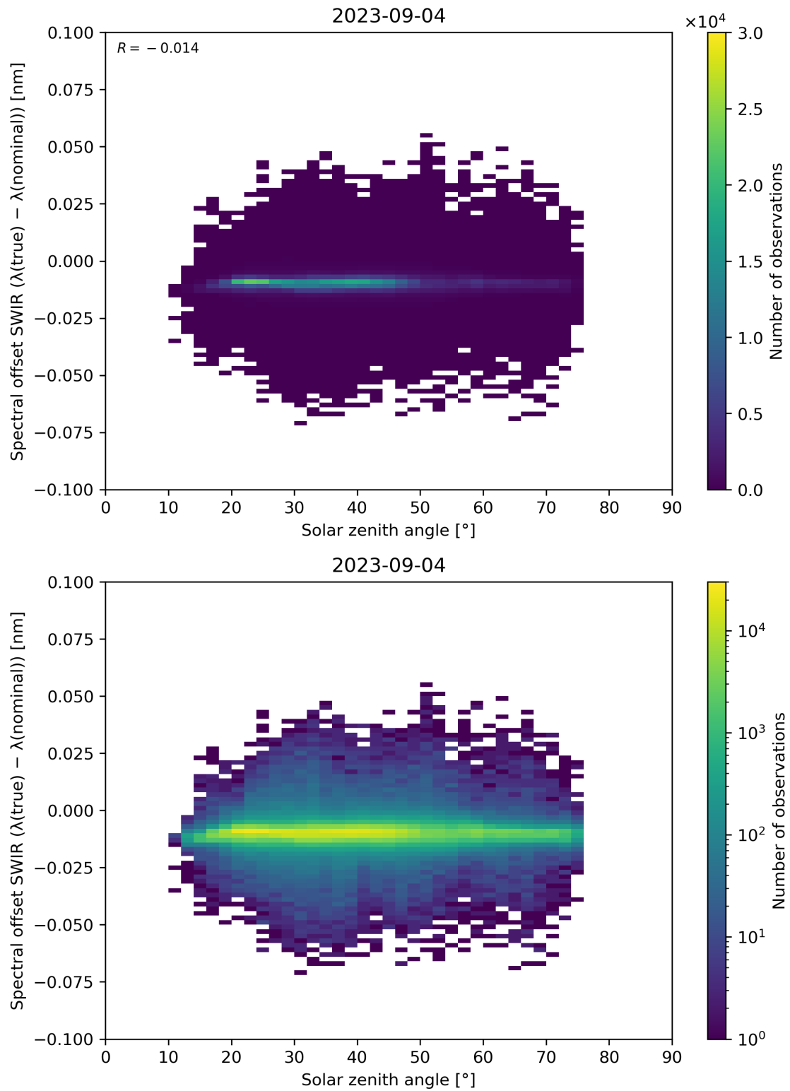
Figure 104: Scatter density plot of “Solar zenith angle” against “Spectral offset SWIR ( \lambda(\text{true}) - \lambda(\text{nominal}) )” for 2023-09-04 to 2023-09-05.
