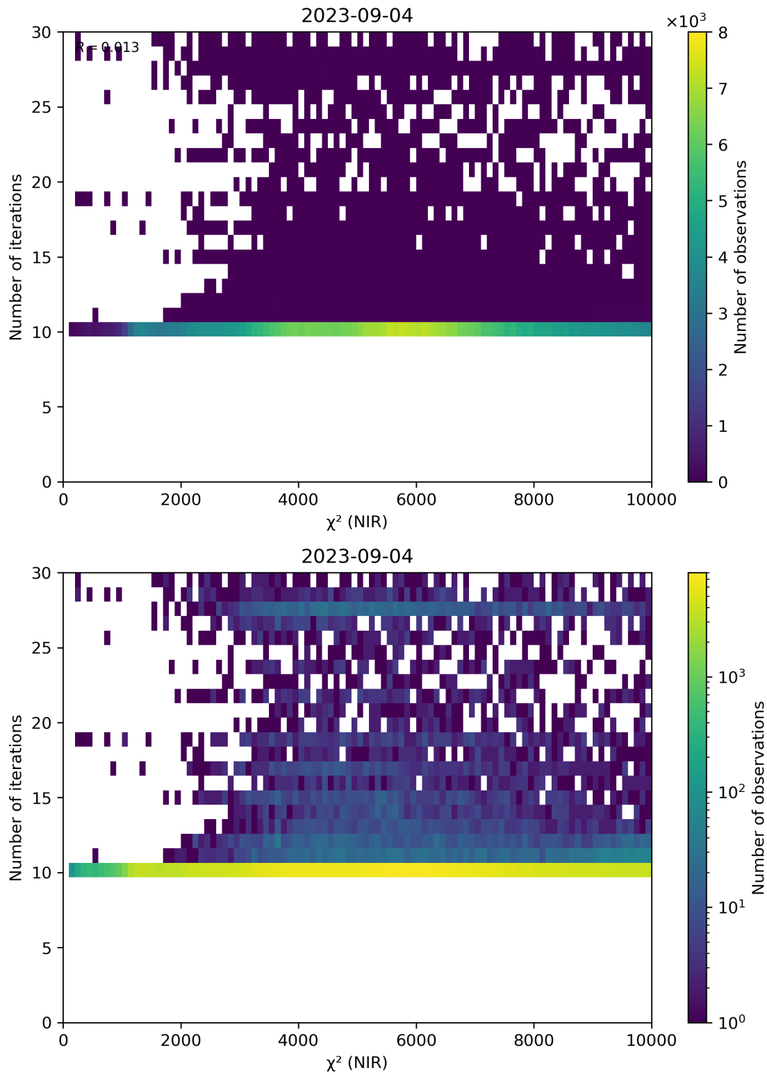
Figure 46: Scatter density plot of “ \chi^2 (NIR)” against “Number of iterations” for 2023-09-04 to 2023-09-05.
