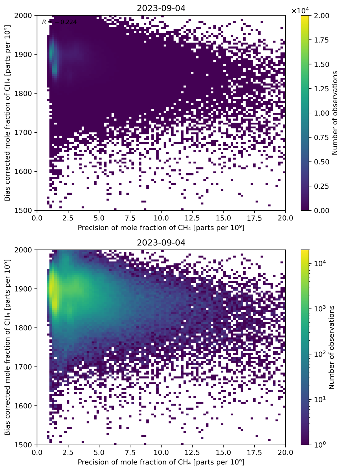
Figure 82: Scatter density plot of “Precision of mole fraction of \text{CH}_4 ” against “Bias corrected mole fraction of \text{CH}_4 ” for 2023-09-04 to 2023-09-05.
