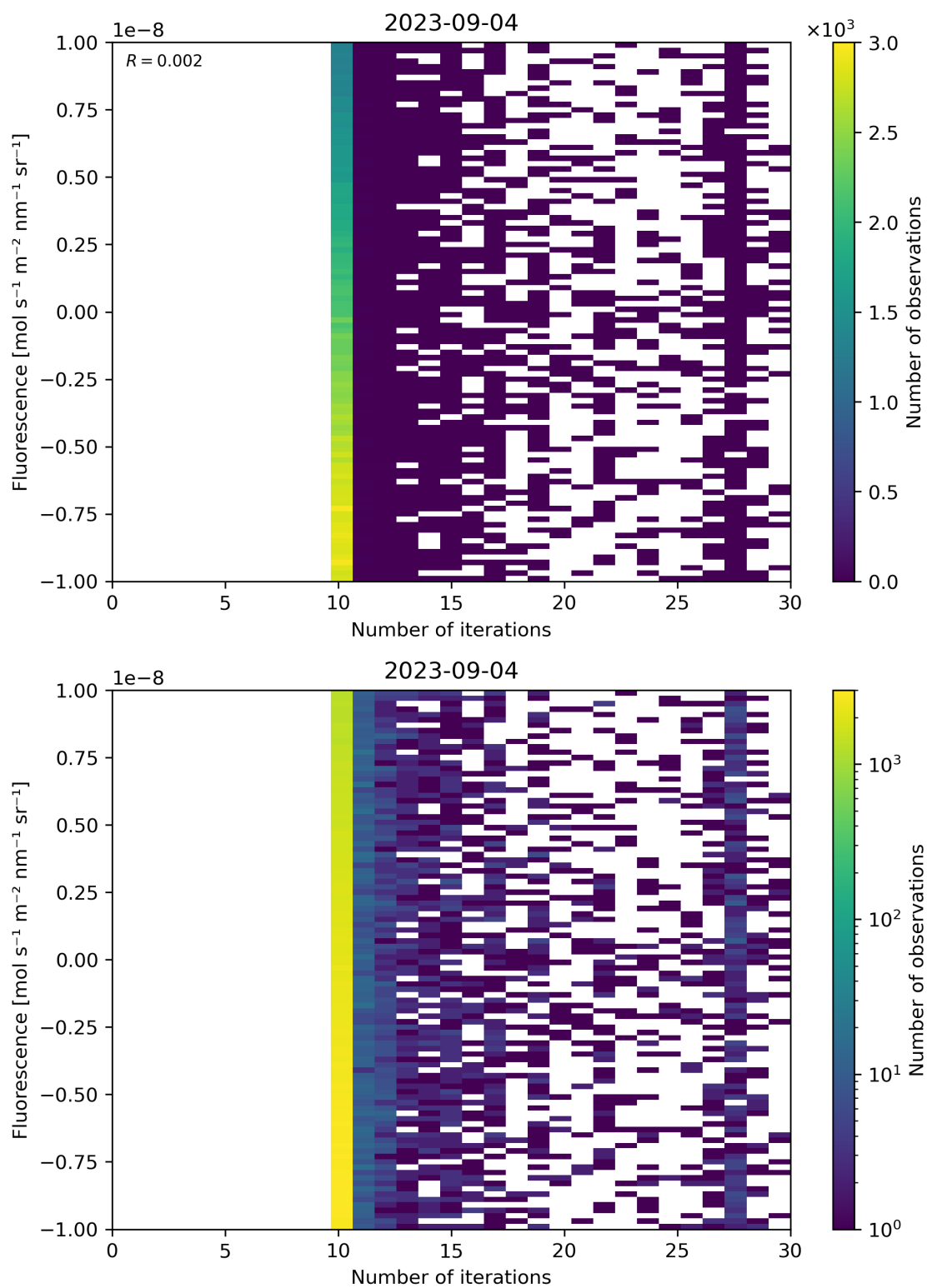
Figure 87: Scatter density plot of “Number of iterations” against “Fluorescence” for 2023-09-04 to 2023-09-05.
