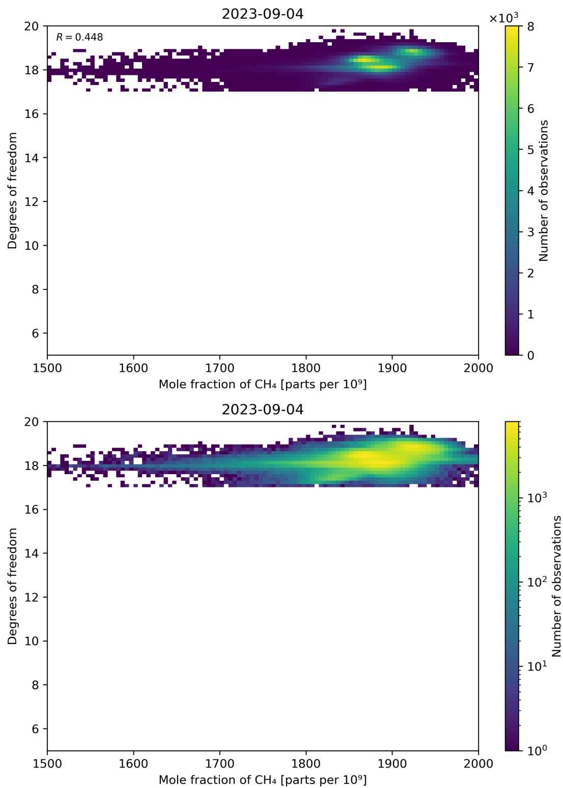
Figure 72: Scatter density plot of “Mole fraction of CH 4 ” against “Degrees of freedom” for 2023-09-04 to 2023-09-05.
