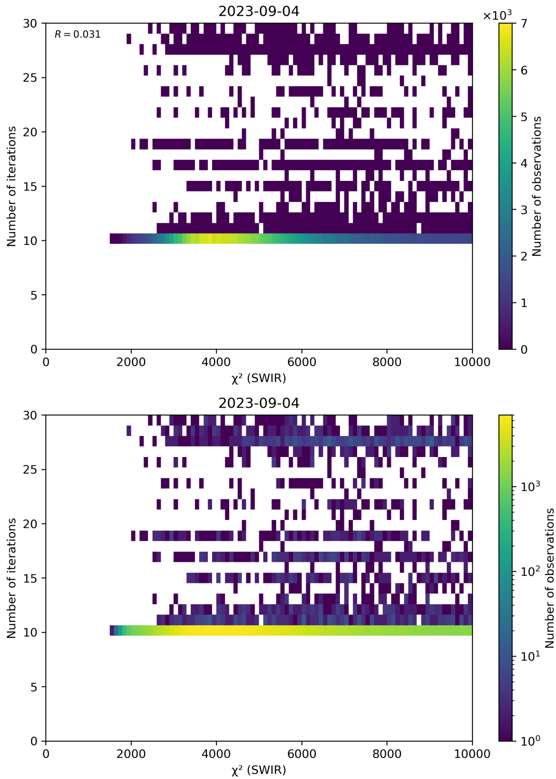
Figure 50: Scatter density plot of “ \chi^2 (SWIR)” against “Number of iterations” for 2023-09-04 to 2023-09-05.
