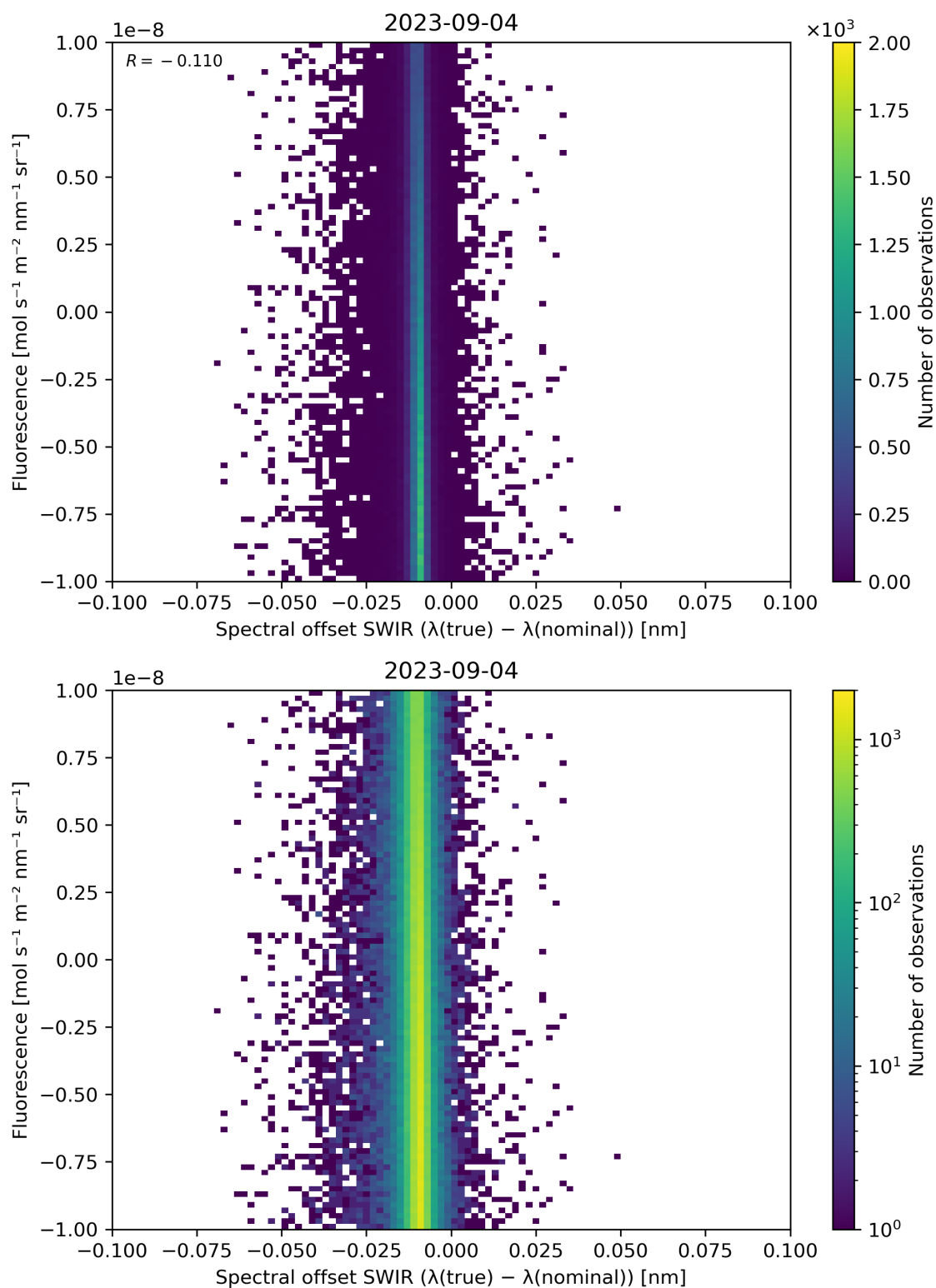
Figure 120: Scatter density plot of “Spectral offset SWIR ( \lambda(\text{true}) - \lambda(\text{nominal}) )” against “Fluorescence” for 2023-09-04 to 2023-09-05.
