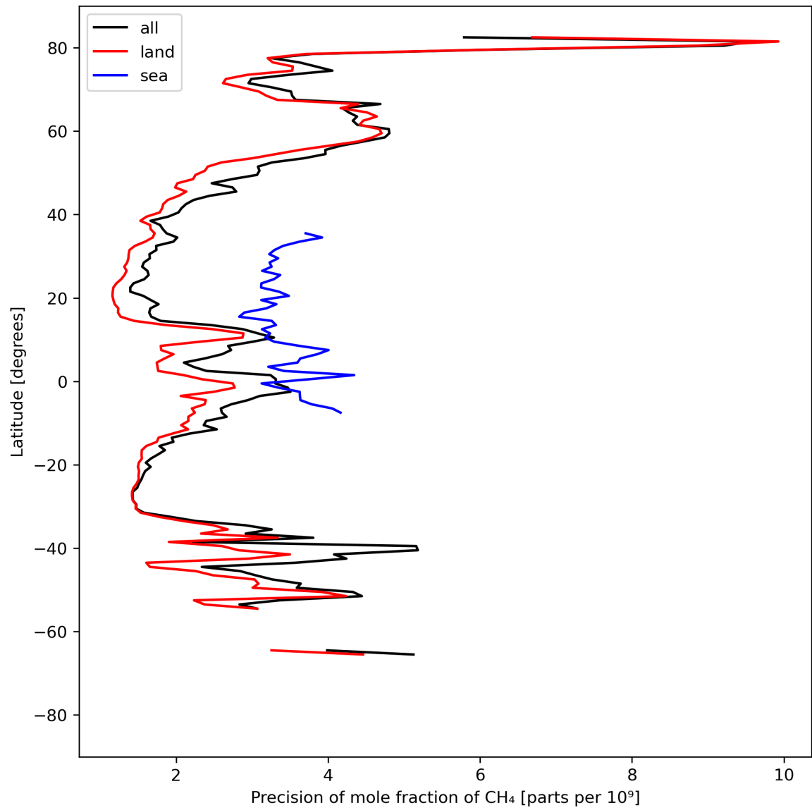
Figure 13: Zonal average of “Precision of mole fraction of CH 4 ” for 2023-09-04 to 2023-09-05.
