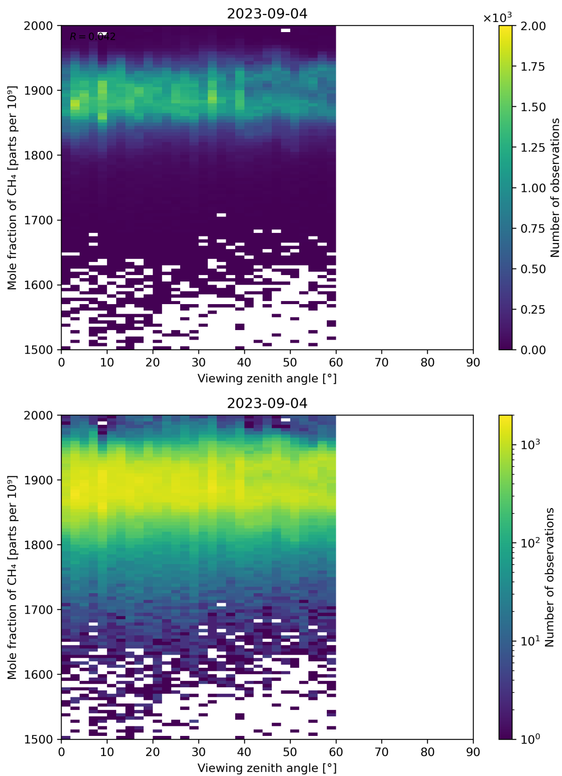
Figure 110: Scatter density plot of “Viewing zenith angle” against “Mole fraction of CH 4 ” for 2023-09-04 to 2023-09-05.
