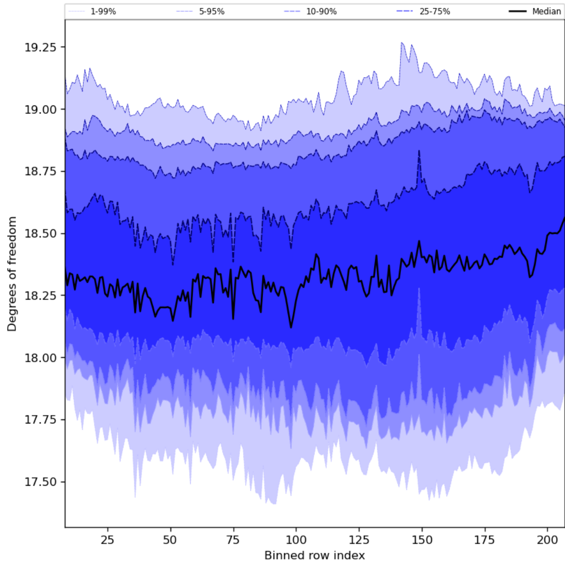
Figure 41: Along track statistics of “Degrees of freedom” for 2023-09-05 to 2023-09-07
