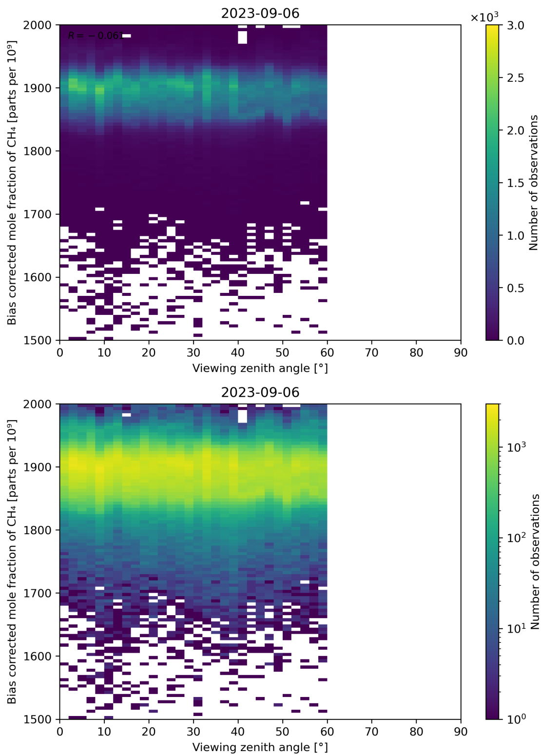
Figure 111: Scatter density plot of “Viewing zenith angle” against “Bias corrected mole fraction of CH 4 ” for 2023-09-05 to 2023-09-07.
