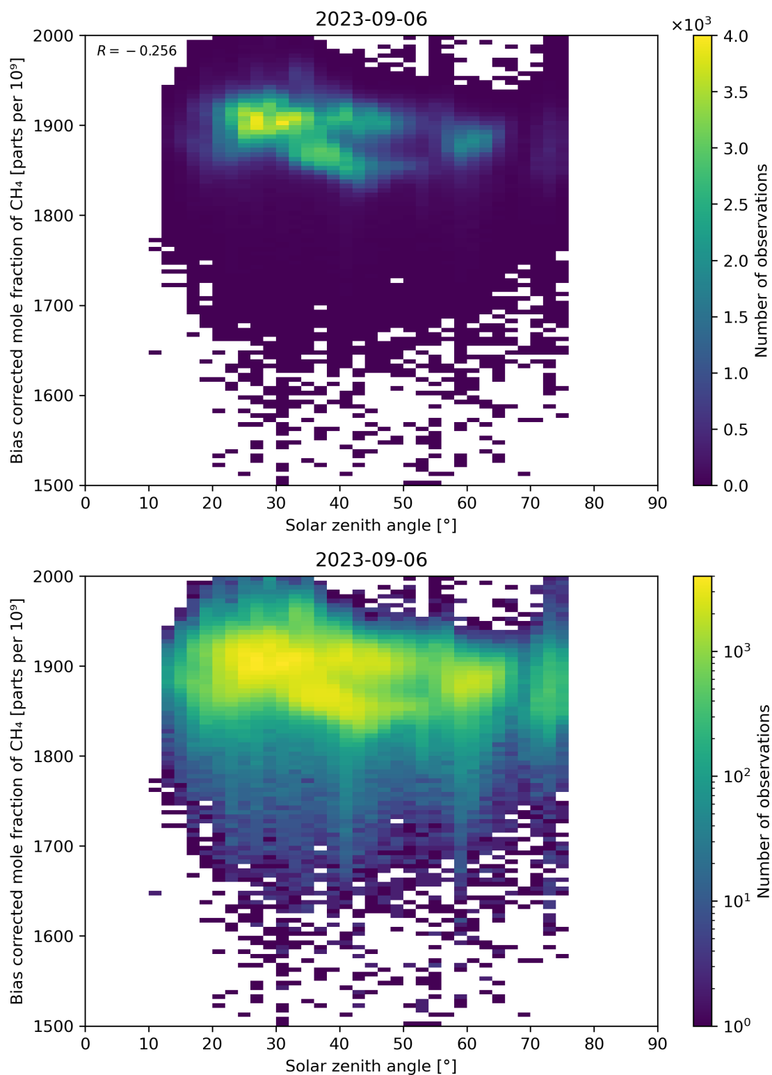
Figure 100: Scatter density plot of “Solar zenith angle” against “Bias corrected mole fraction of \text{CH}_4 ” for 2023-09-05 to 2023-09-07.
