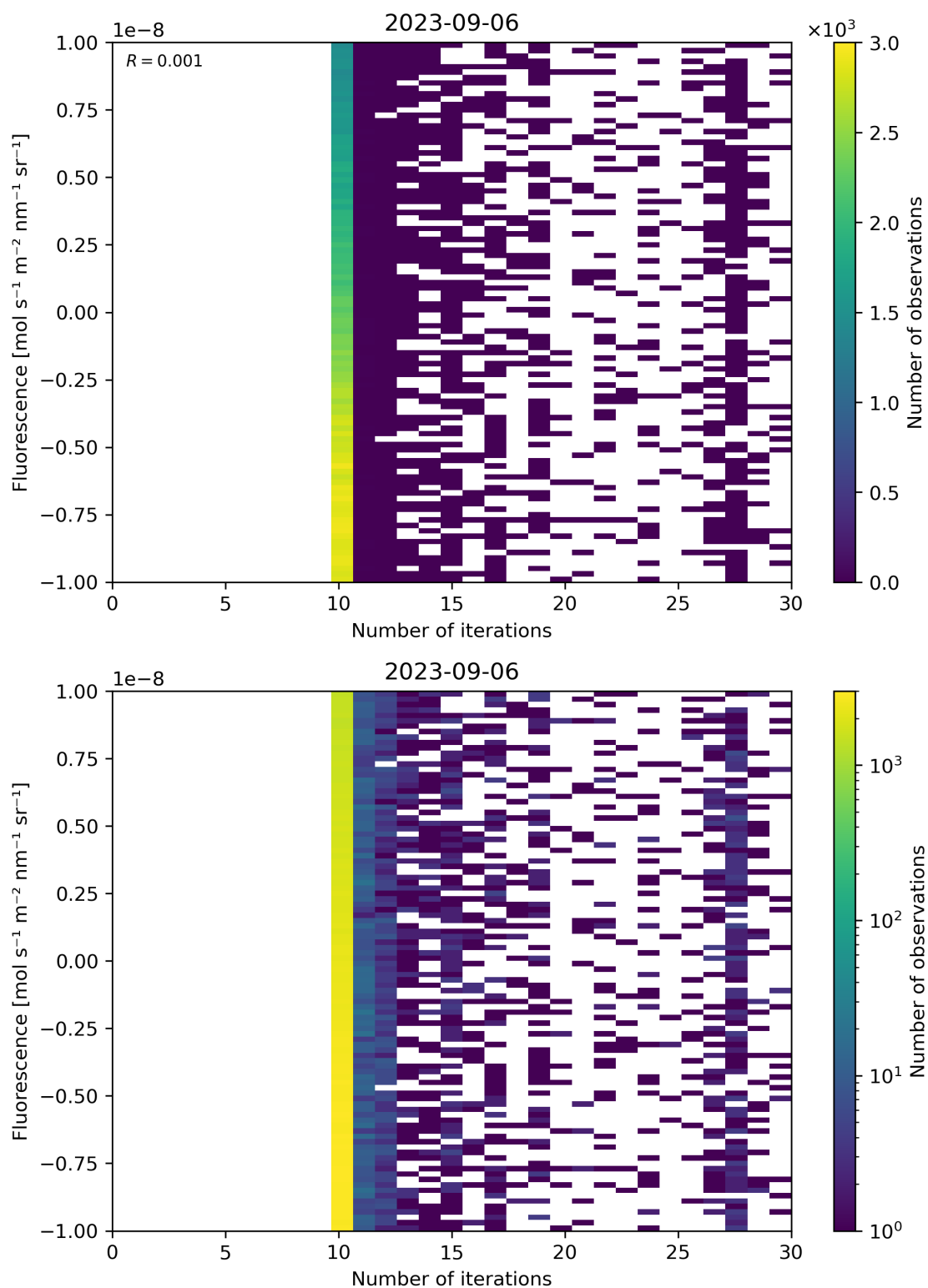
Figure 87: Scatter density plot of “Number of iterations” against “Fluorescence” for 2023-09-05 to 2023-09-07.
