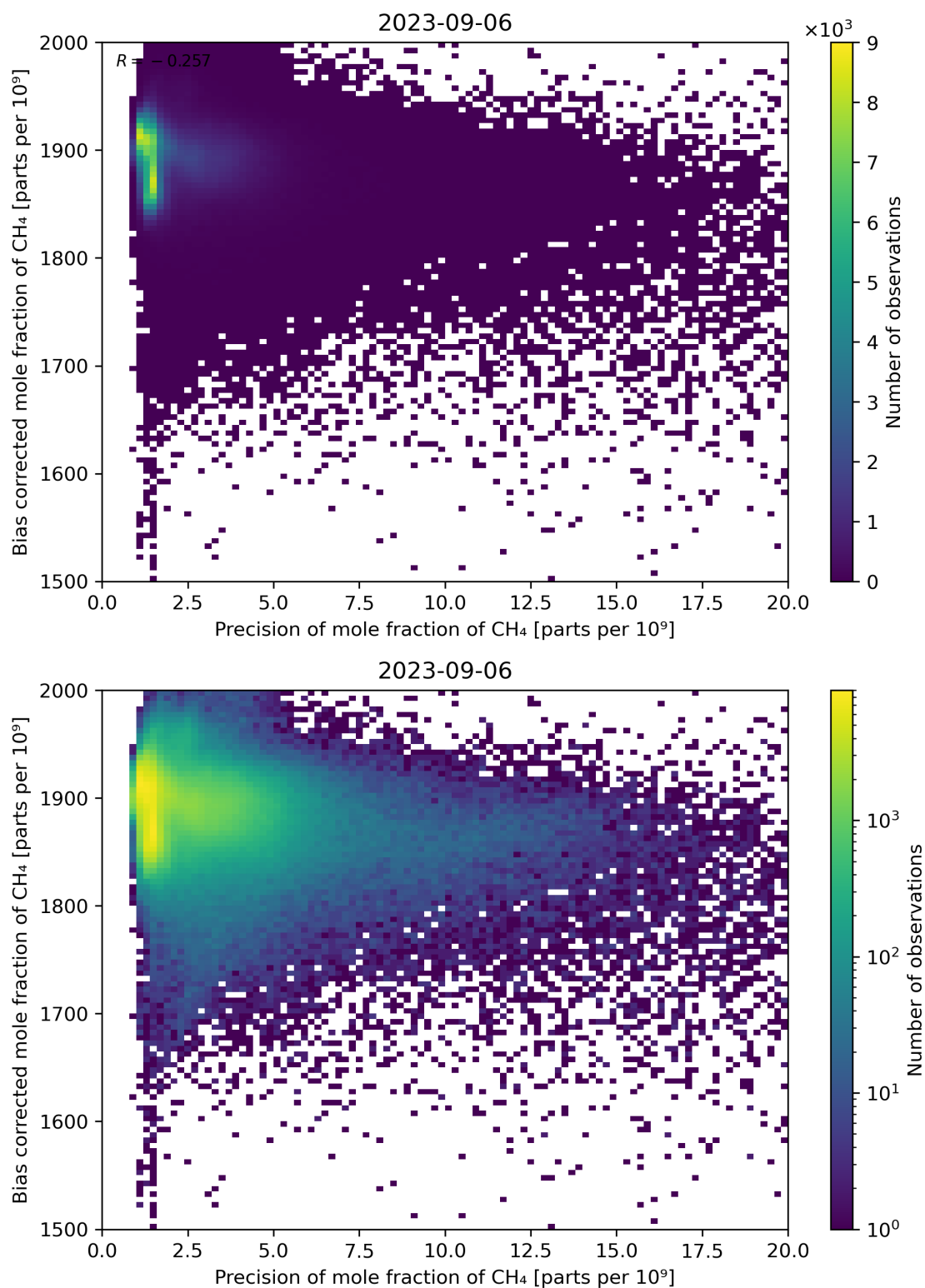
Figure 82: Scatter density plot of “Precision of mole fraction of CH 4 ” against “Bias corrected mole fraction of CH 4 ” for 2023-09-05 to 2023-09-07.
