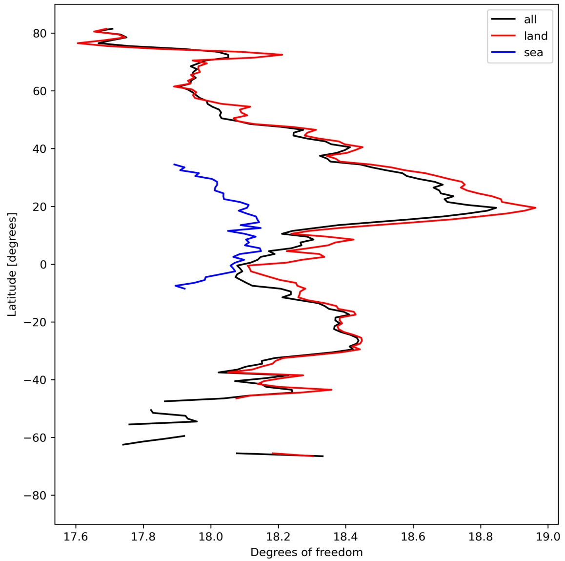
Figure 19: Zonal average of “Degrees of freedom” for 2023-09-05 to 2023-09-07.
