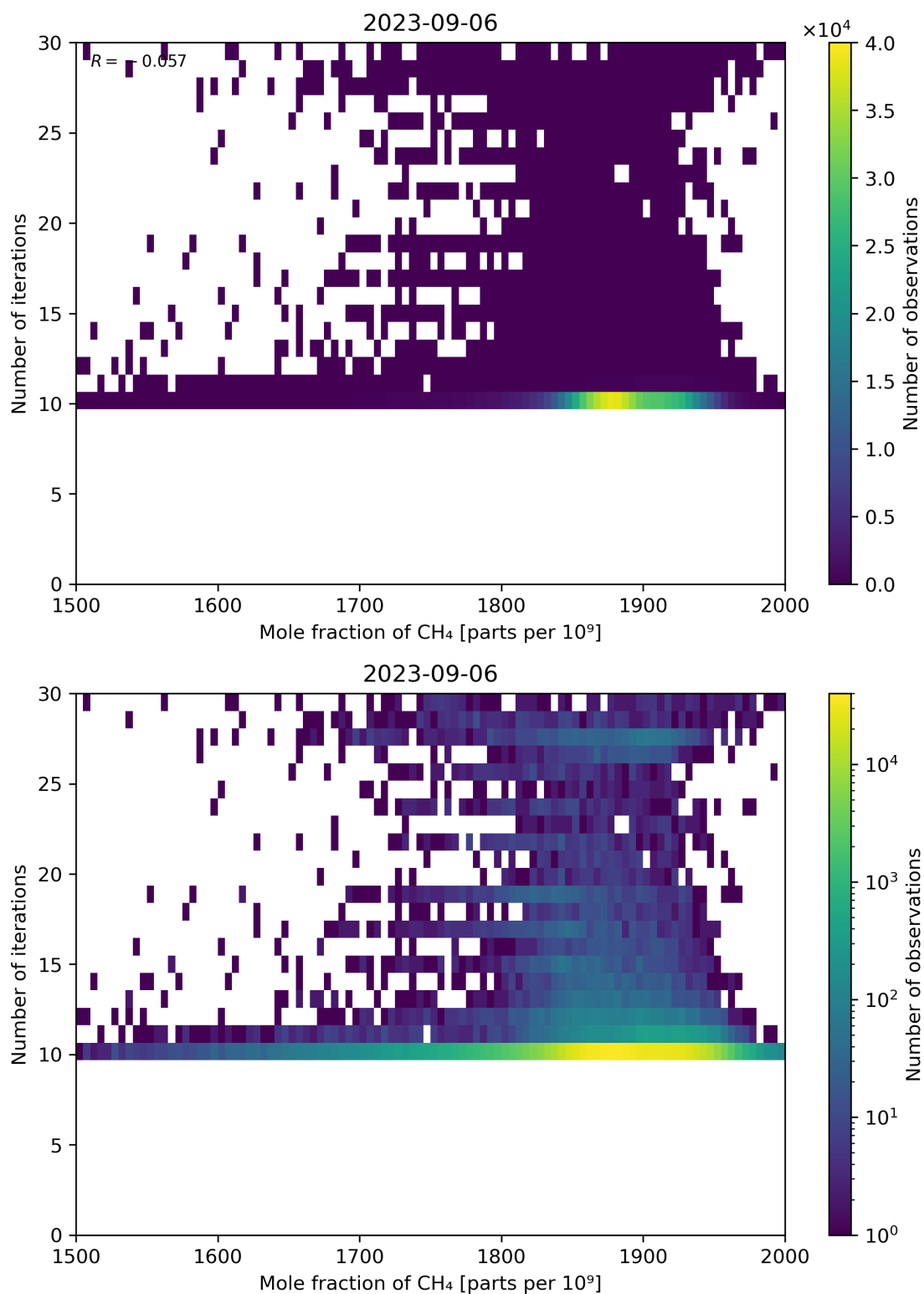
Figure 76: Scatter density plot of “Mole fraction of CH 4 ” against “Number of iterations” for 2023-09-05 to 2023-09-07.
