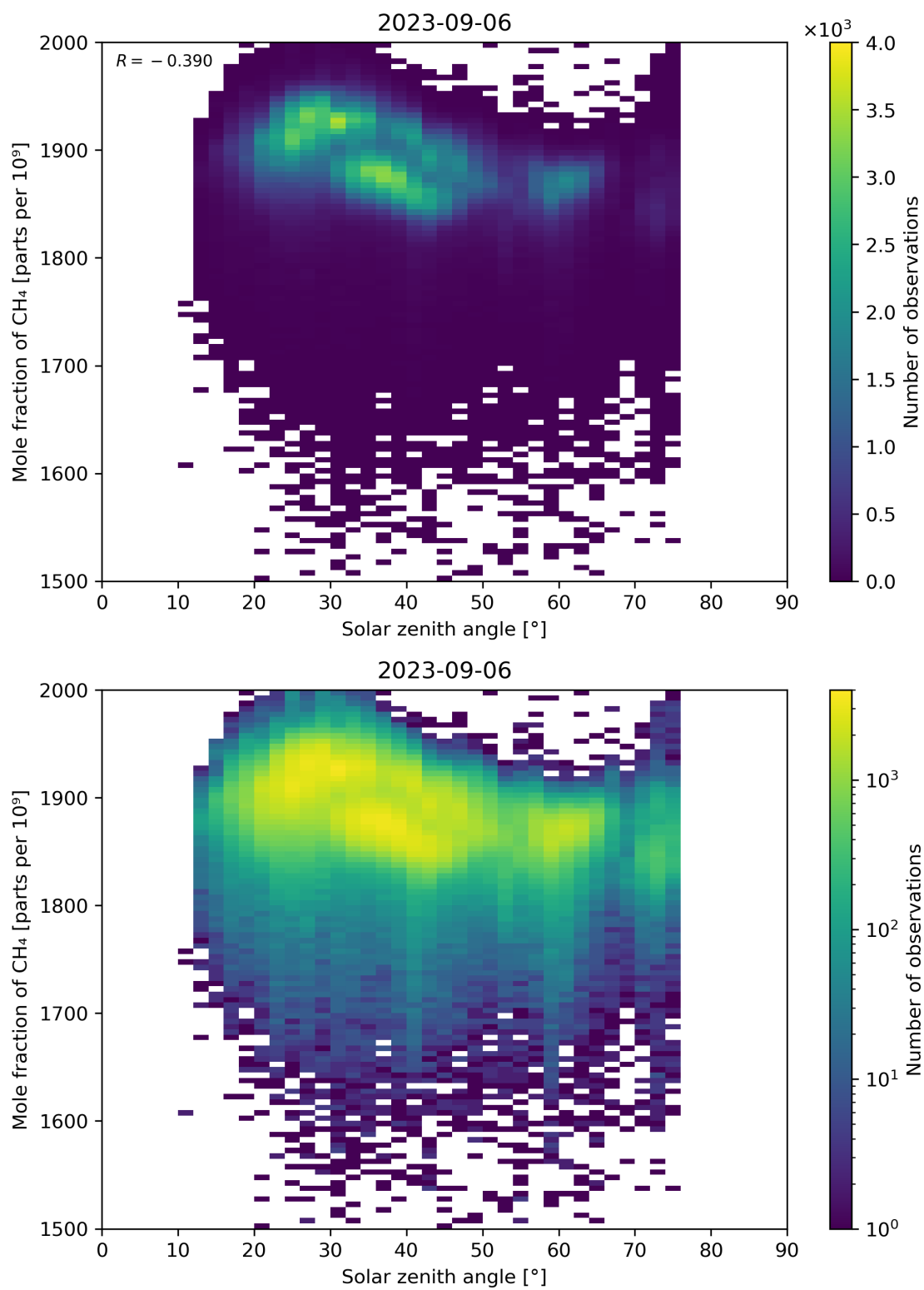
Figure 99: Scatter density plot of “Solar zenith angle” against “Mole fraction of CH 4 ” for 2023-09-05 to 2023-09-07.
