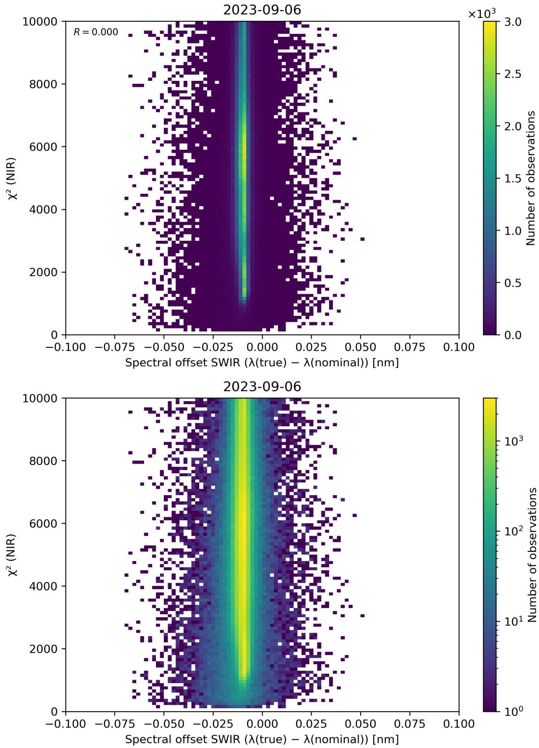
Figure 117: Scatter density plot of “Spectral offset SWIR ( \lambda(\text{true}) - \lambda(\text{nominal}) )” against “ \chi^2 (NIR)” for 2023-09-05 to 2023-09-07.
