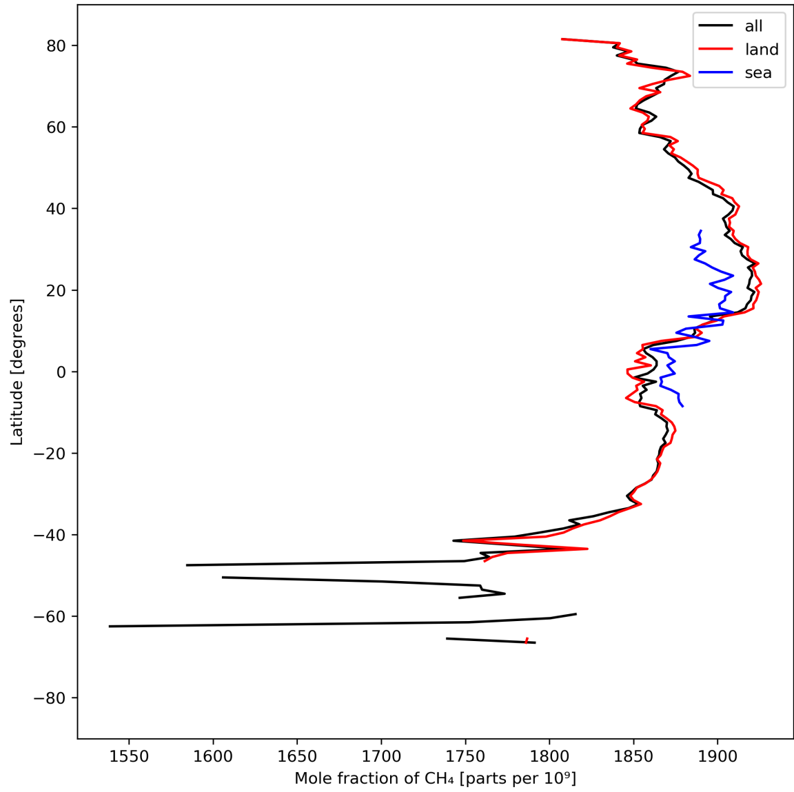
Figure 12: Zonal average of “Mole fraction of \text{CH}_4 ” for 2023-09-05 to 2023-09-07.
