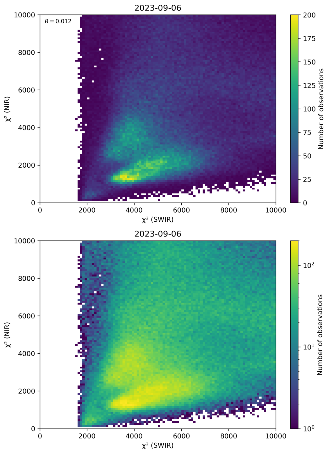
Figure 47: Scatter density plot of “ \chi^2 (SWIR)” against “ \chi^2 (NIR)” for 2023-09-05 to 2023-09-07.
