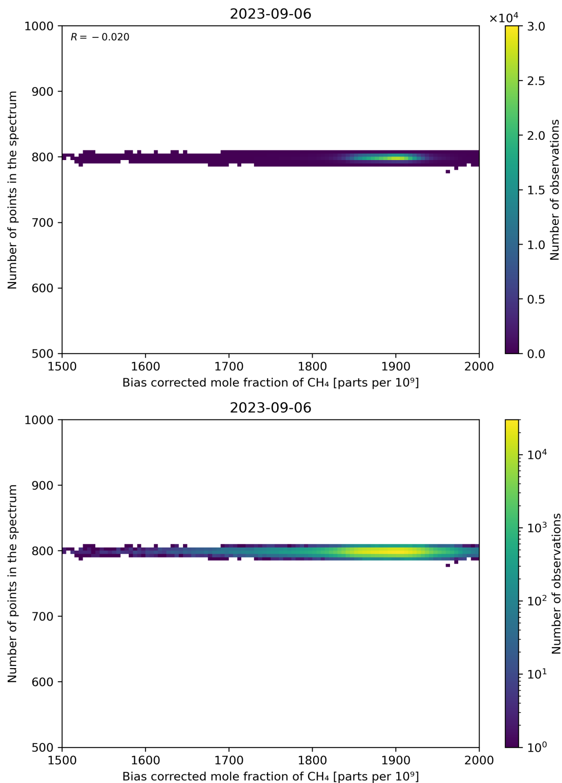
Figure 68: Scatter density plot of “Bias corrected mole fraction of CH 4 ” against “Number of points in the spectrum” for 2023-09-05 to 2023-09-07.
