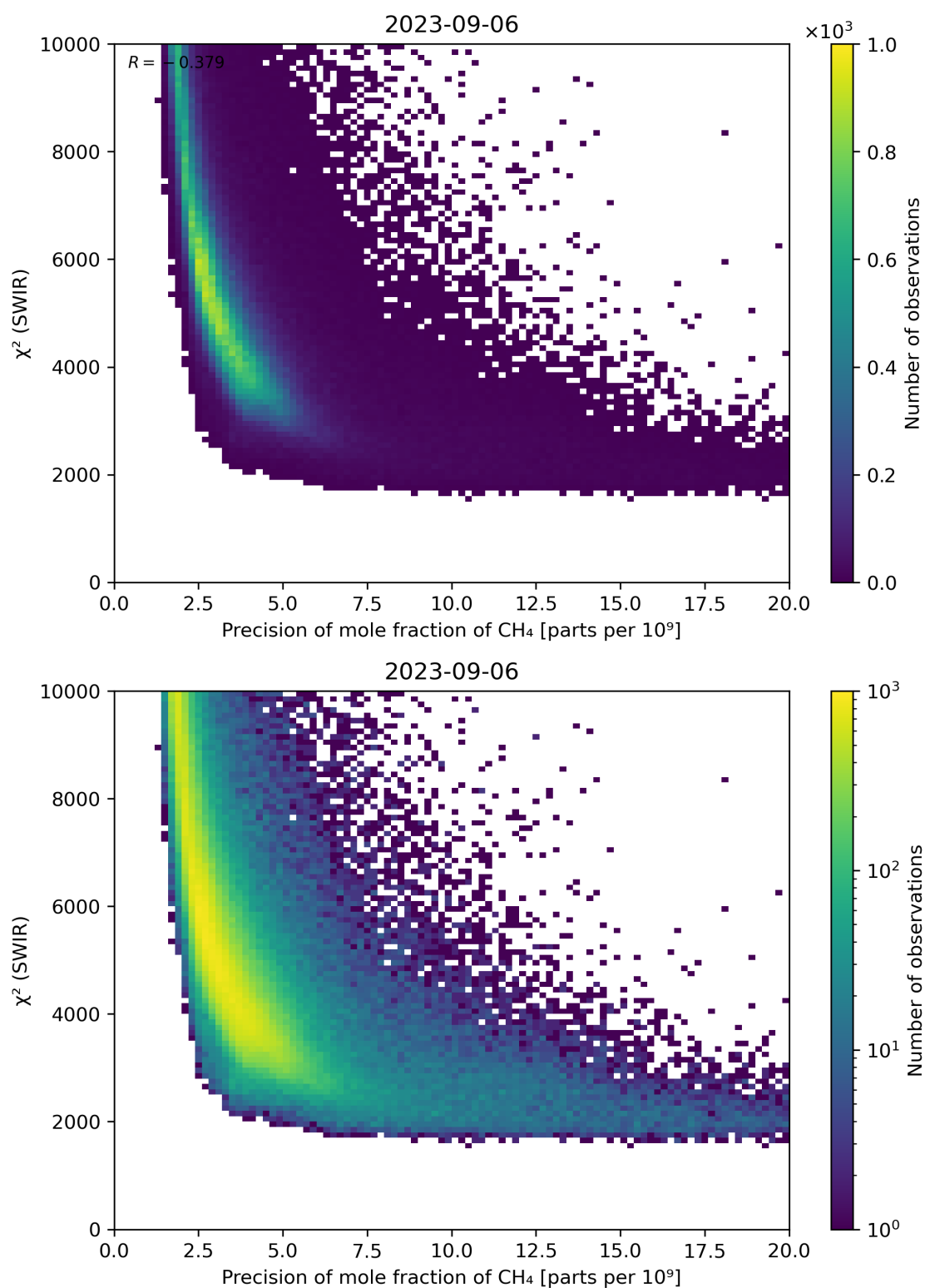
Figure 79: Scatter density plot of “Precision of mole fraction of \text{CH}_4 ” against “ \chi^2 (SWIR)” for 2023-09-05 to 2023-09-07.
