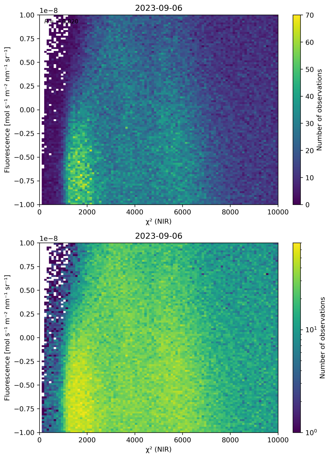
Figure 45: Scatter density plot of “ \chi^2 (NIR)” against “Fluorescence” for 2023-09-05 to 2023-09-07.
