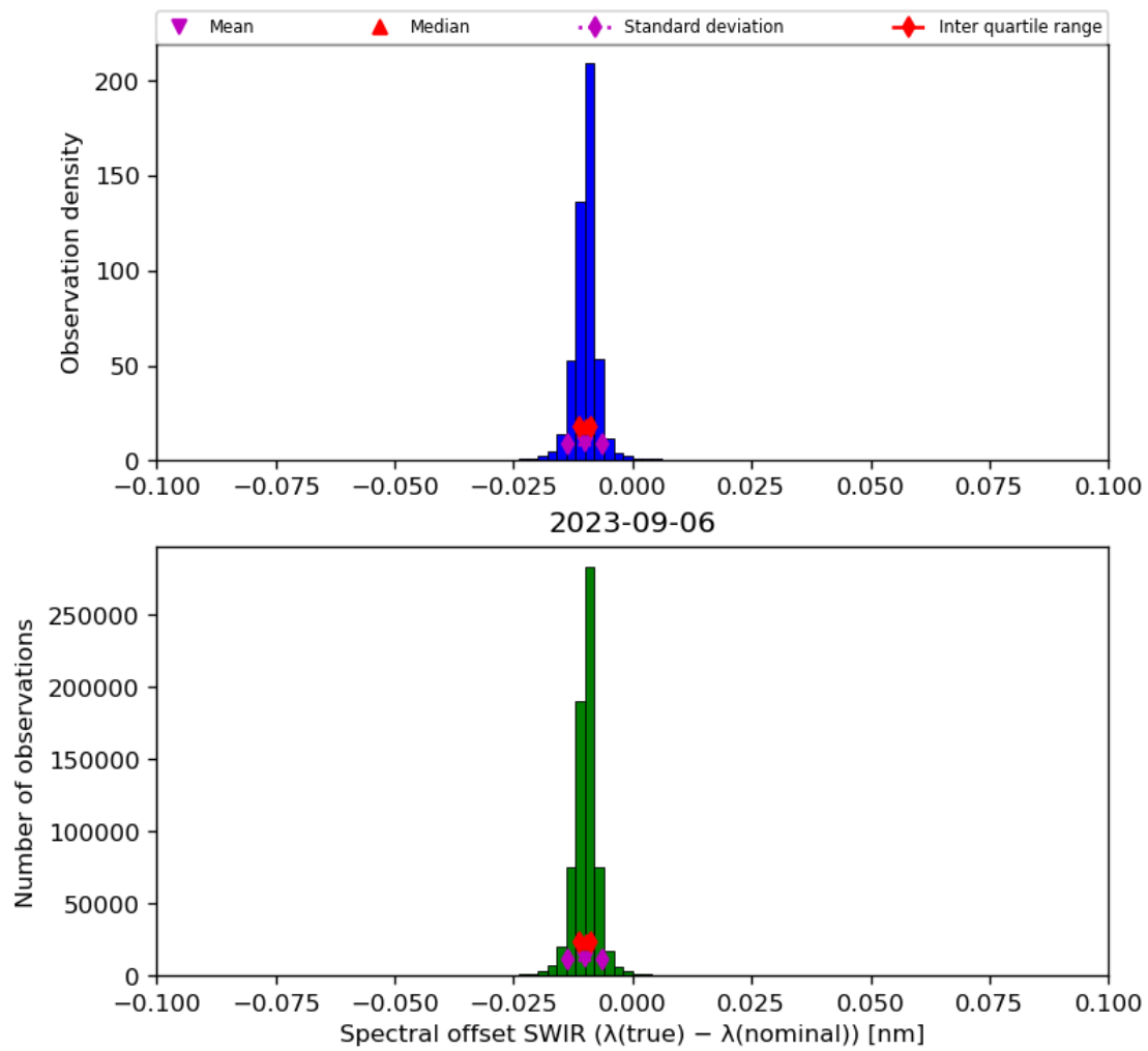
Figure 27: Histogram of “Spectral offset SWIR ( \lambda(\text{true}) - \lambda(\text{nominal}) )” for 2023-09-05 to 2023-09-07
