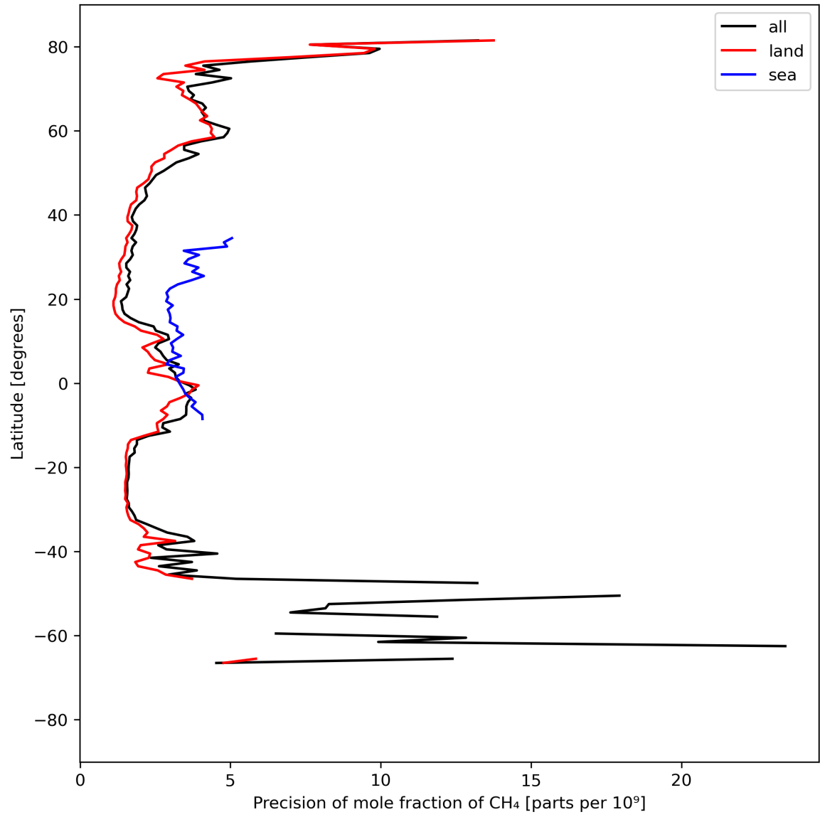
Figure 13: Zonal average of “Precision of mole fraction of CH 4 ” for 2023-09-05 to 2023-09-07.
