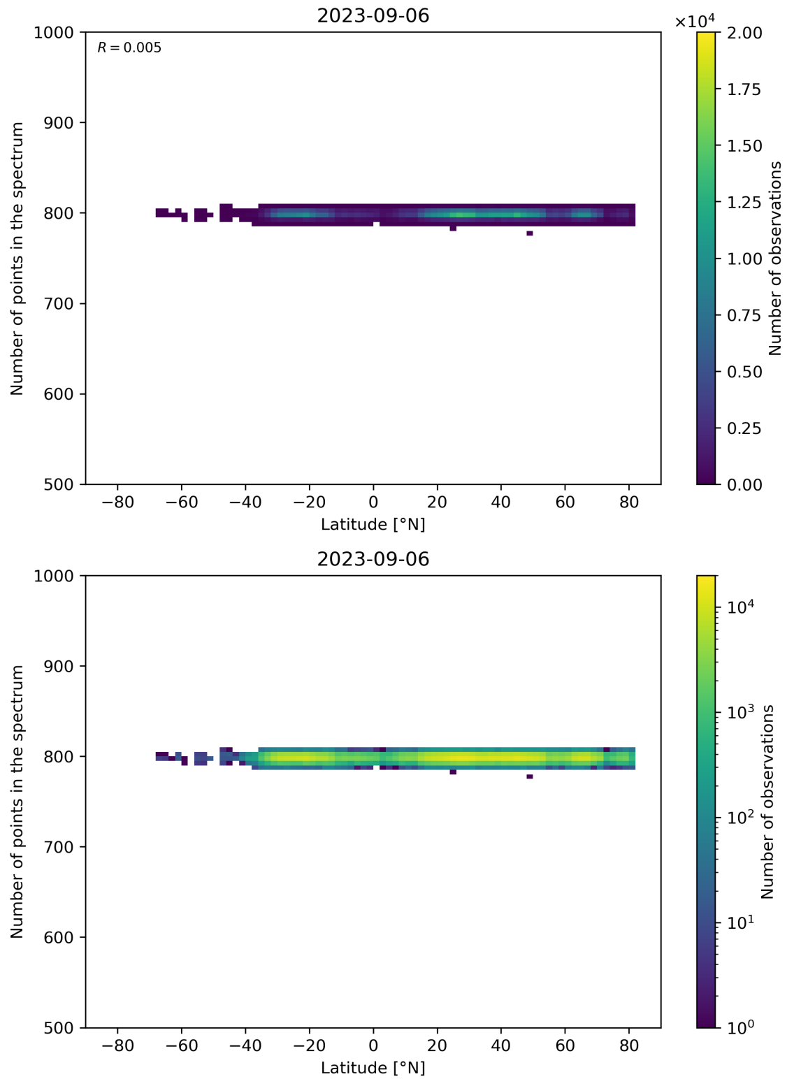
Figure 61: Scatter density plot of “Latitude” against “Number of points in the spectrum” for 2023-09-05 to 2023-09-07.
