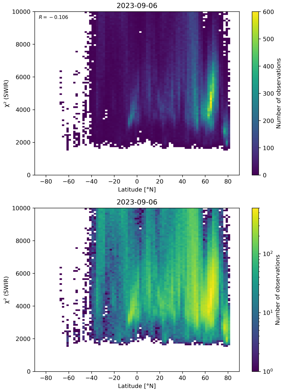
Figure 54: Scatter density plot of “Latitude” against “ \chi^2 (SWIR)” for 2023-09-05 to 2023-09-07.
