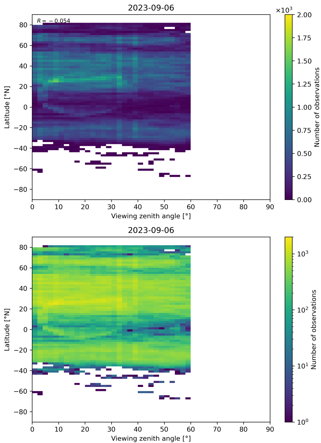
Figure 109: Scatter density plot of “Viewing zenith angle” against “Latitude” for 2023-09-05 to 2023-09-07.
