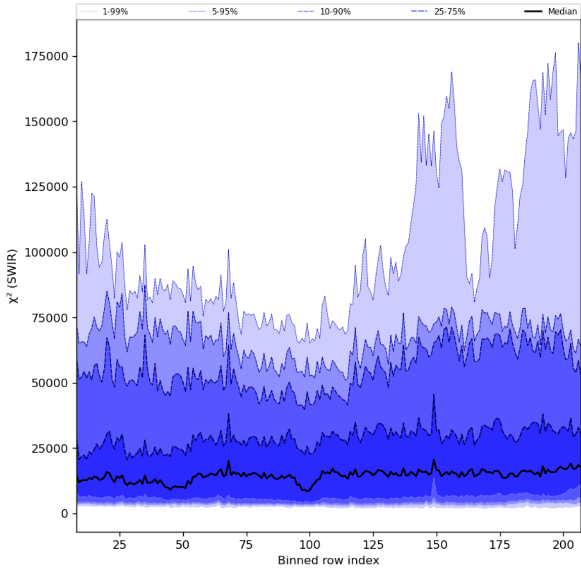
Figure 39: Along track statistics of " \chi^2 (SWIR)" for 2023-09-05 to 2023-09-07
