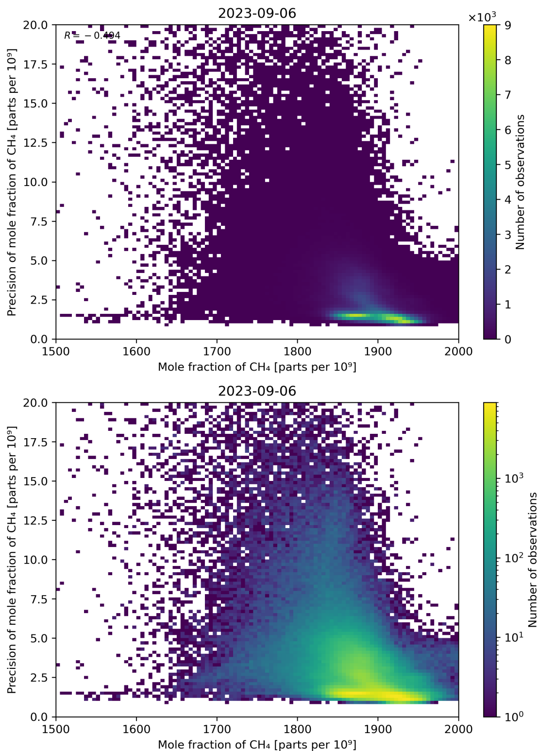
Figure 75: Scatter density plot of “Mole fraction of CH 4 ” against “Precision of mole fraction of CH 4 ” for 2023-09-05 to 2023-09-07.
