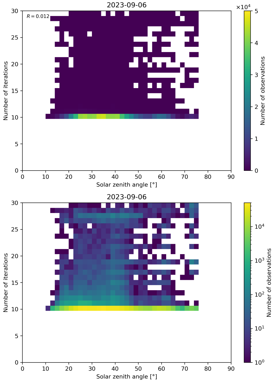
Figure 102: Scatter density plot of “Solar zenith angle” against “Number of iterations” for 2023-09-05 to 2023-09-07.
