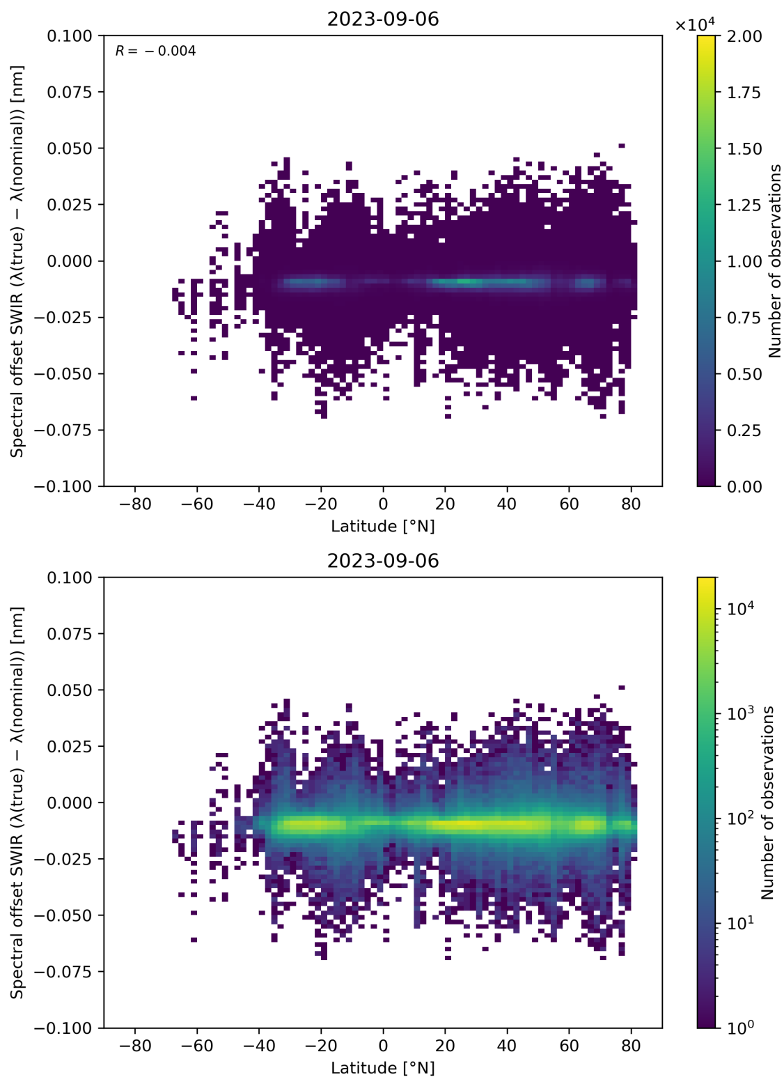
Figure 62: Scatter density plot of “Latitude” against “Spectral offset SWIR ( \lambda(\text{true}) - \lambda(\text{nominal}) )” for 2023-09-05 to 2023-09-07.
