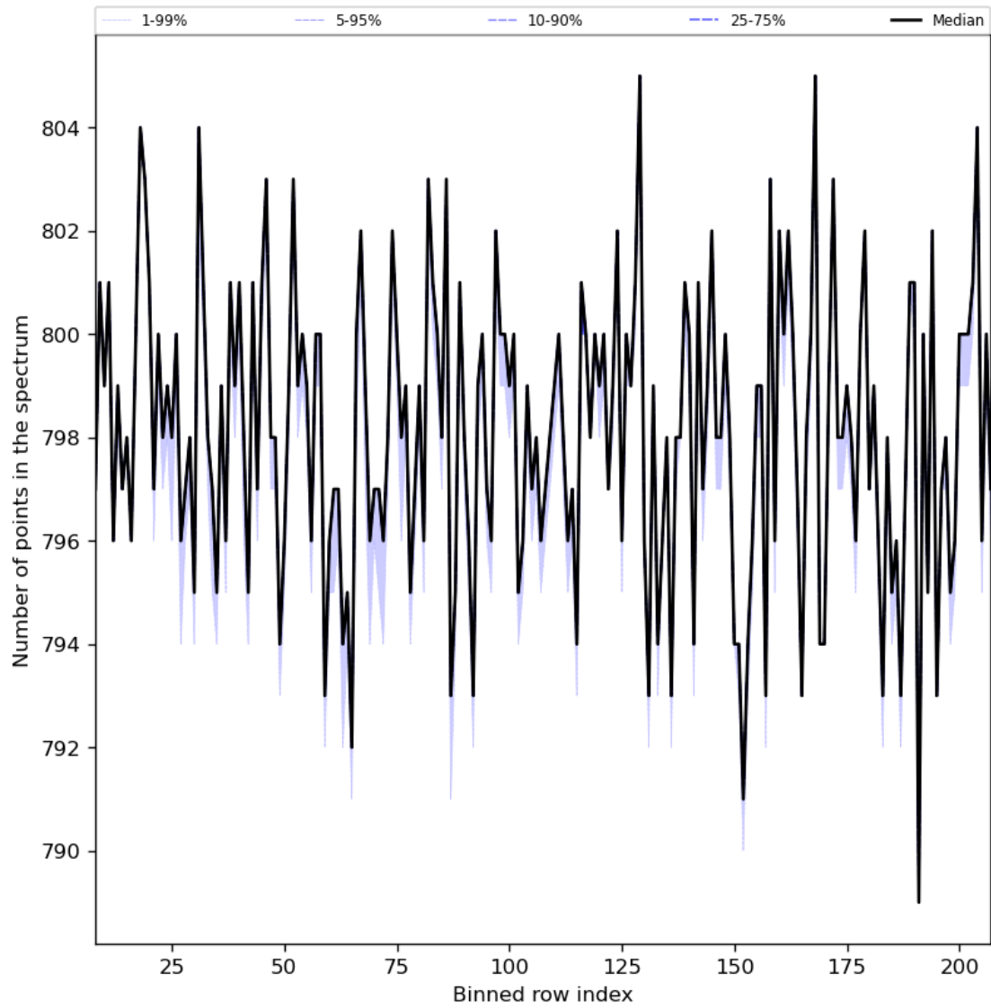
Figure 37: Along track statistics of “Number of points in the spectrum” for 2023-09-05 to 2023-09-07
