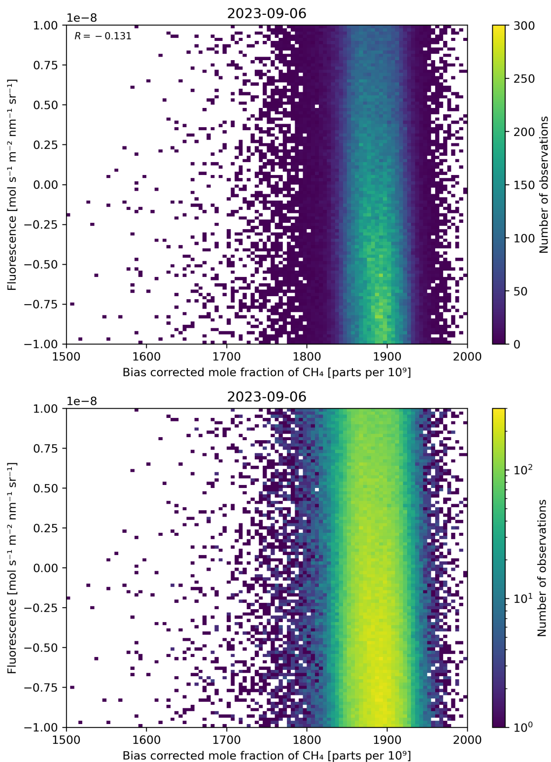
Figure 66: Scatter density plot of “Bias corrected mole fraction of \text{CH}_4 ” against “Fluorescence” for 2023-09-05 to 2023-09-07.
