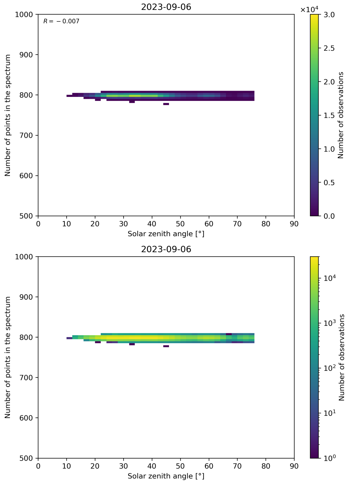
Figure 103: Scatter density plot of “Solar zenith angle” against “Number of points in the spectrum” for 2023-09-05 to 2023-09-07.
