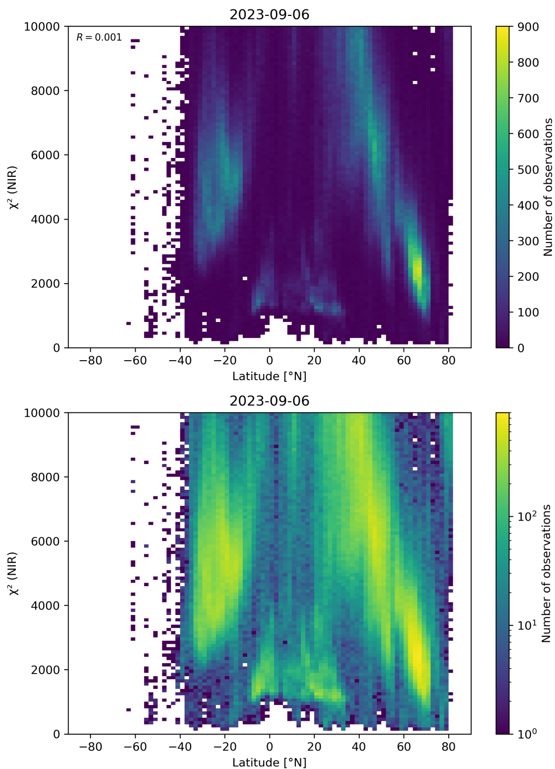
Figure 53: Scatter density plot of “Latitude” against “ \chi^2 (NIR)” for 2023-09-05 to 2023-09-07.
