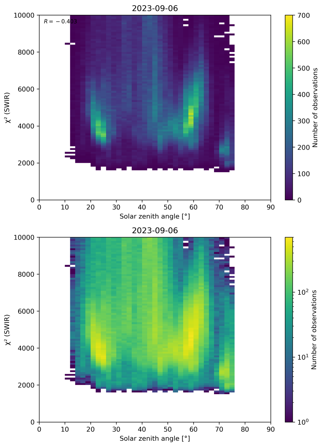
Figure 95: Scatter density plot of “Solar zenith angle” against “ \chi^2 (SWIR)” for 2023-09-05 to 2023-09-07.
