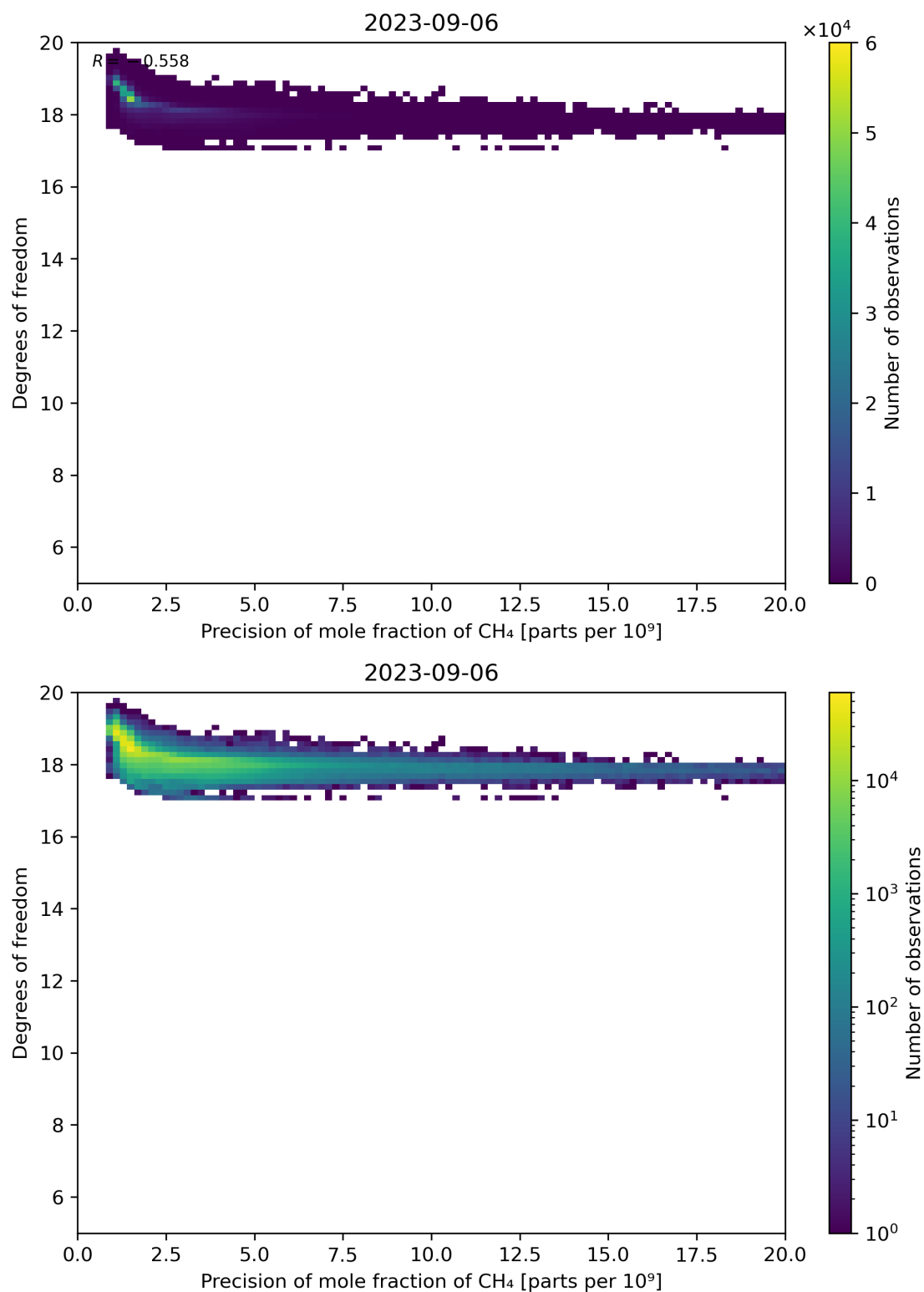
Figure 80: Scatter density plot of “Precision of mole fraction of CH 4 ” against “Degrees of freedom” for 2023-09-05 to 2023-09-07.
