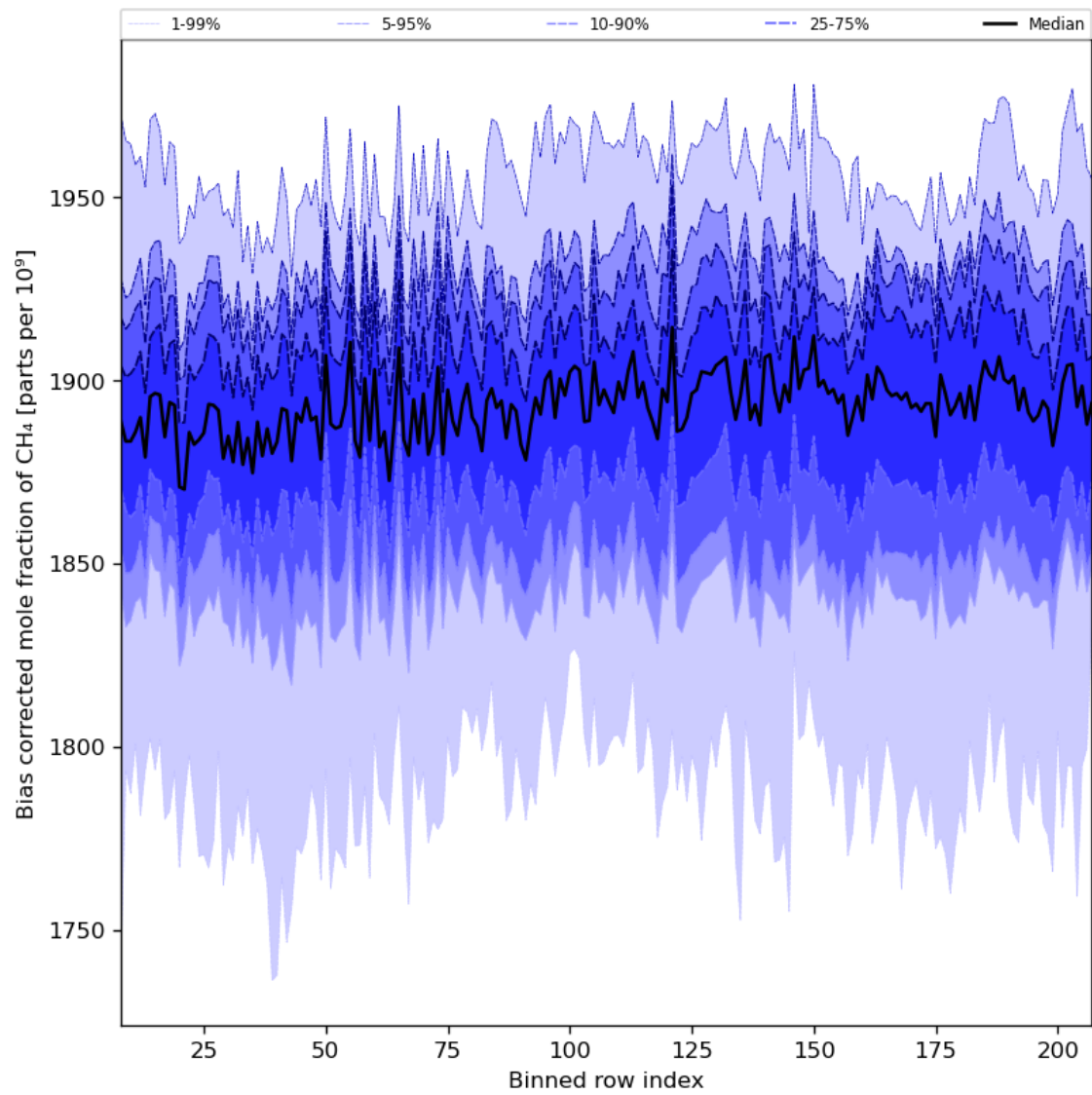
Figure 36: Along track statistics of “Bias corrected mole fraction of CH 4 ” for 2023-09-05 to 2023-09-07
