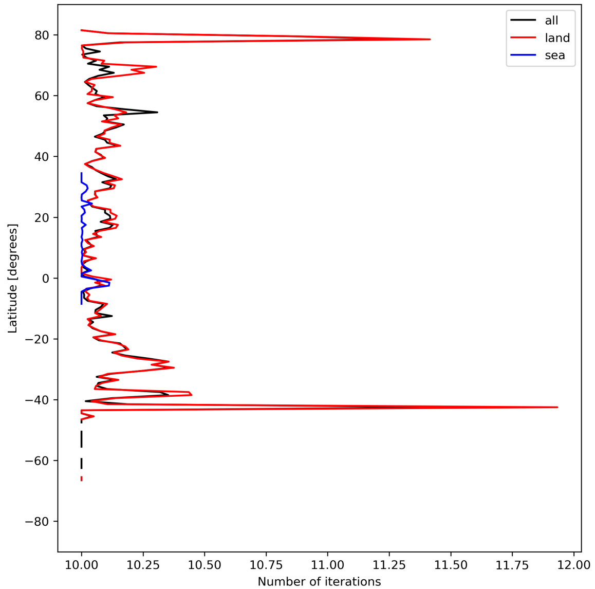
Figure 20: Zonal average of “Number of iterations” for 2023-09-05 to 2023-09-07.
