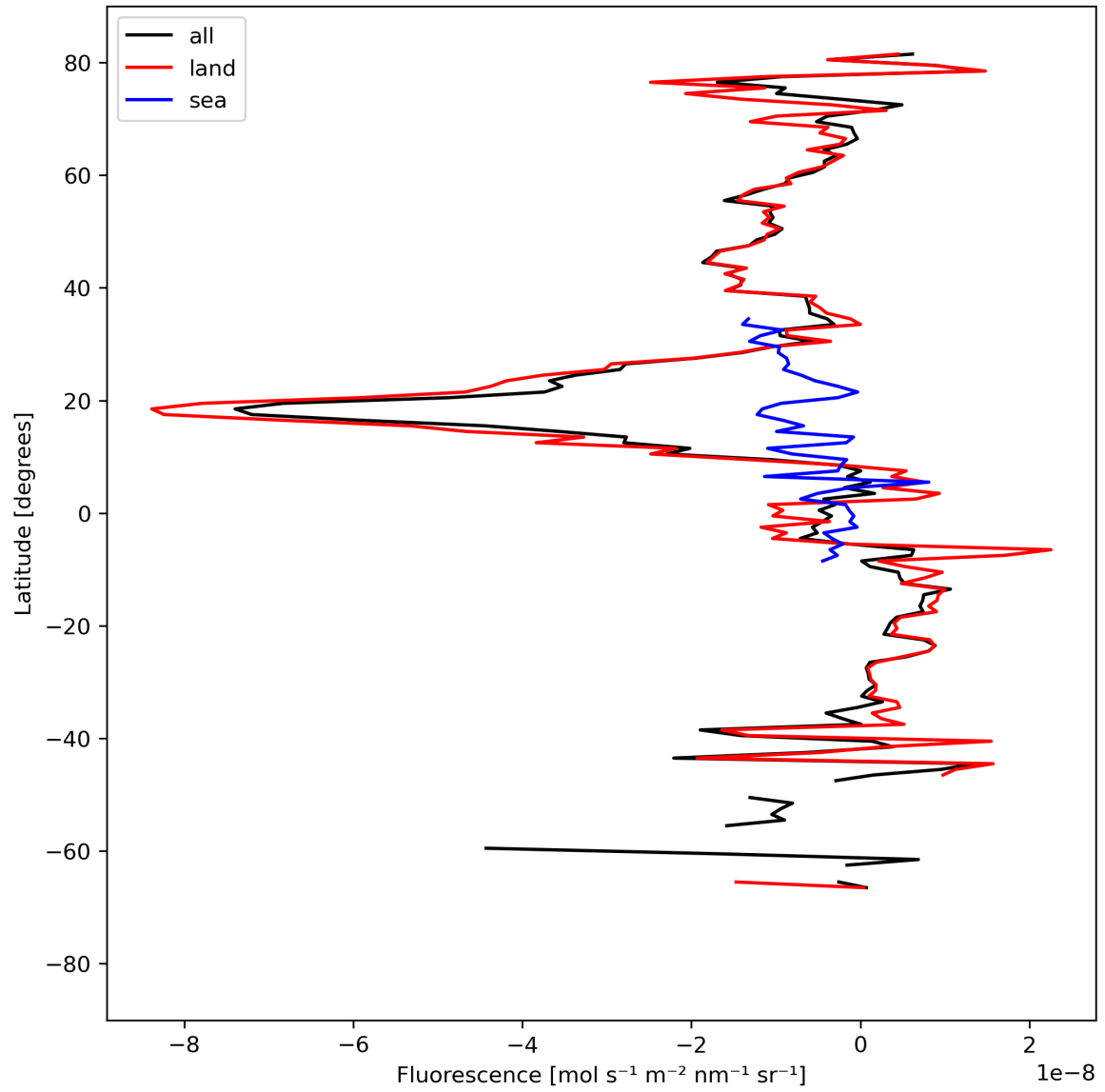
Figure 21: Zonal average of “Fluorescence” for 2023-09-05 to 2023-09-07.
