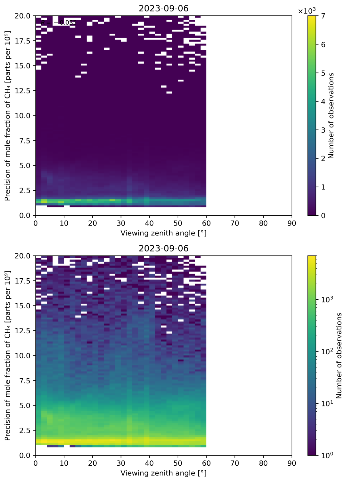
Figure 112: Scatter density plot of “Viewing zenith angle” against “Precision of mole fraction of CH 4 ” for 2023-09-05 to 2023-09-07.
