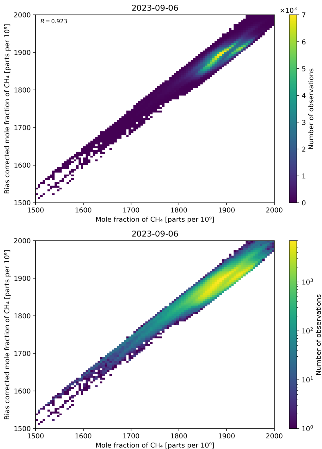
Figure 74: Scatter density plot of “Mole fraction of CH 4 ” against “Bias corrected mole fraction of CH 4 ” for 2023-09-05 to 2023-09-07.
