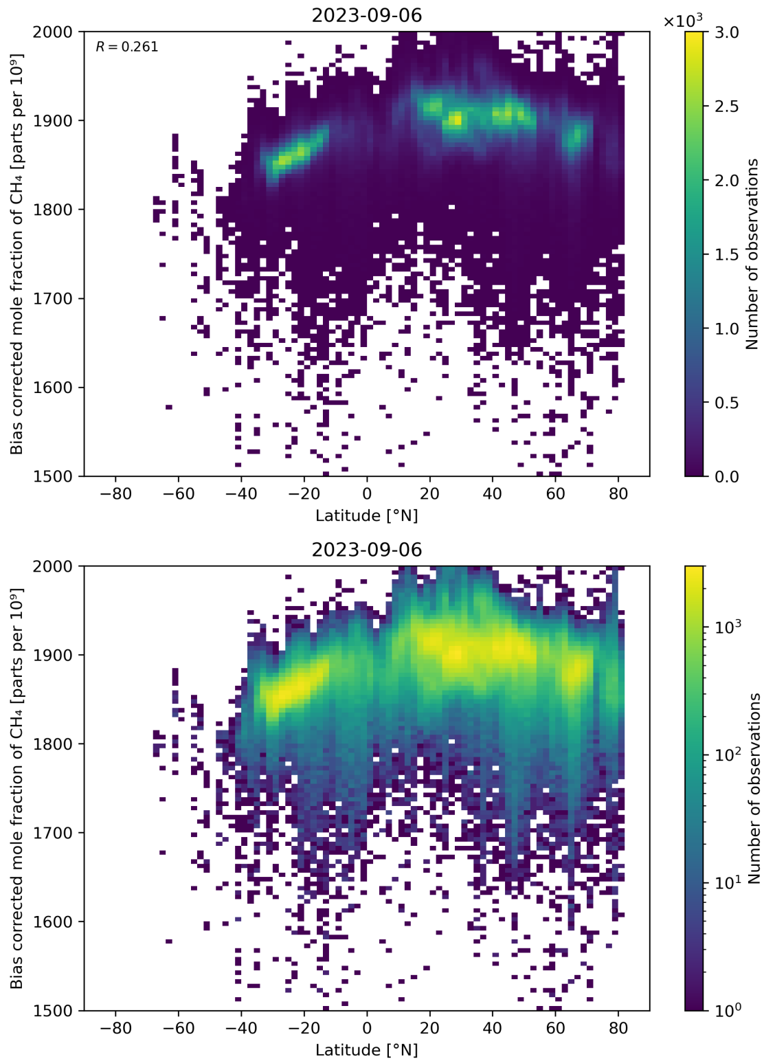
Figure 58: Scatter density plot of “Latitude” against “Bias corrected mole fraction of CH 4 ” for 2023-09-05 to 2023-09-07.
