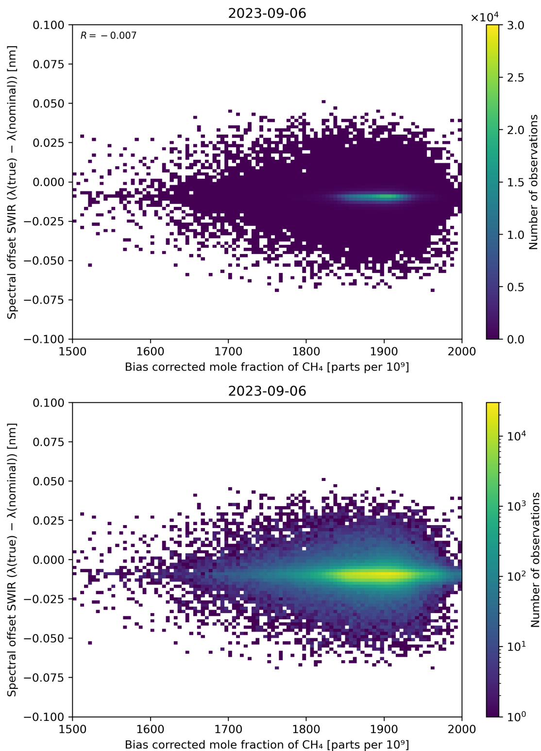
Figure 69: Scatter density plot of “Bias corrected mole fraction of \text{CH}_4 ” against “Spectral offset SWIR ( \lambda(\text{true}) - \lambda(\text{nominal}) )” for 2023-09-05 to 2023-09-07.
