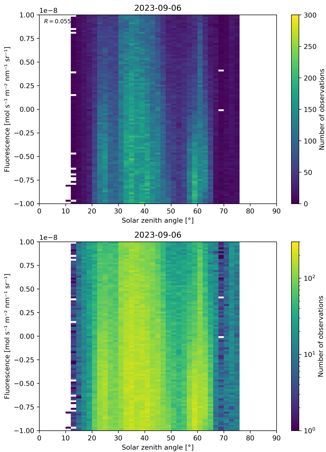
Figure 97: Scatter density plot of “Solar zenith angle” against “Fluorescence” for 2023-09-05 to 2023-09-07.
