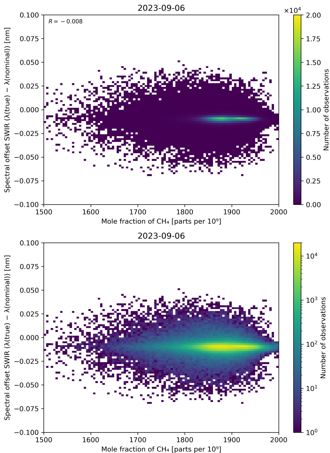
Figure 86: Scatter density plot of “Mole fraction of CH 4 ” against “Spectral offset SWIR ( \lambda(\text{true}) - \lambda(\text{nominal}) )” for 2023-09-05 to 2023-09-07.
