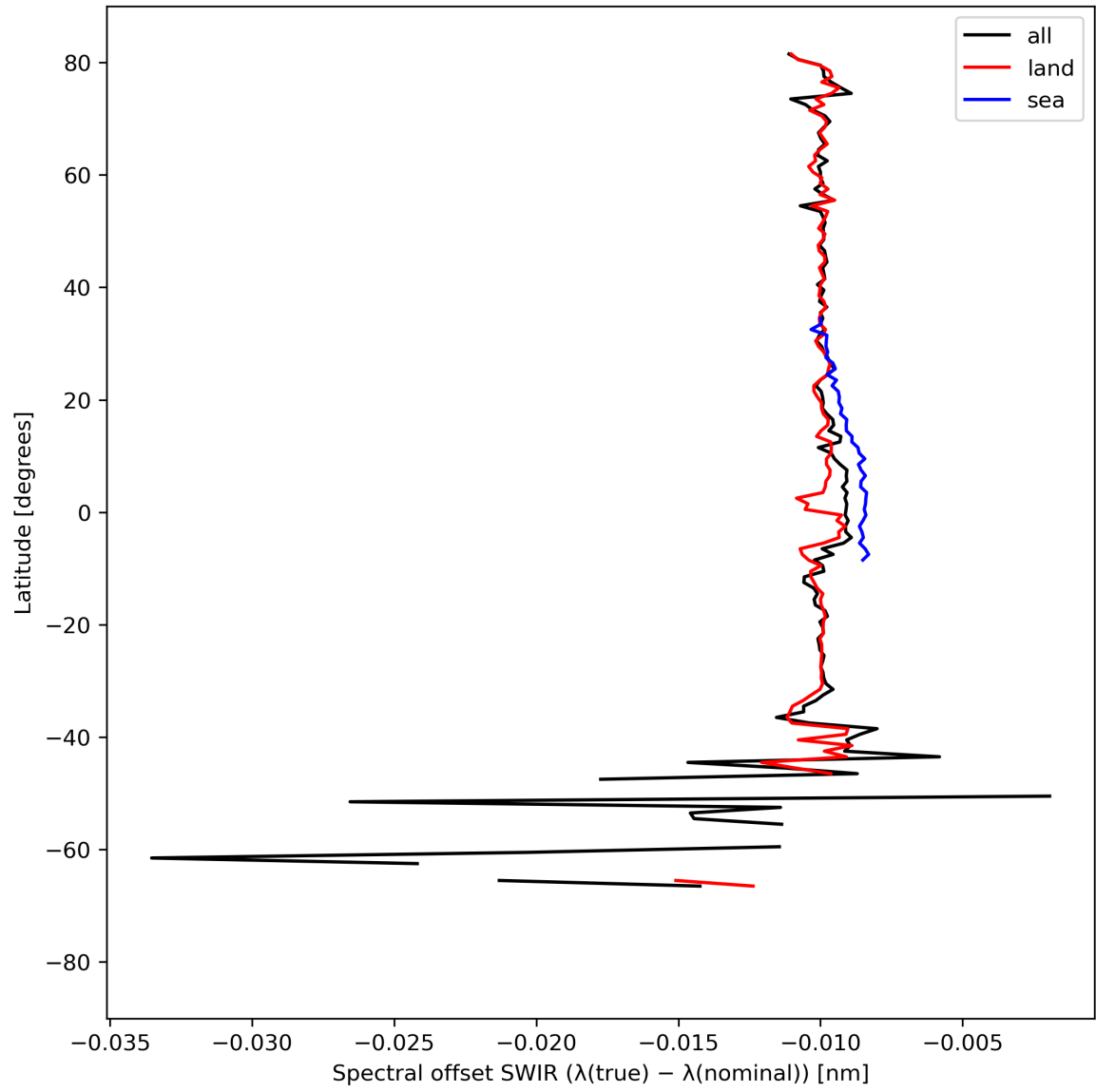
Figure 16: Zonal average of “Spectral offset SWIR ( \lambda(\text{true}) - \lambda(\text{nominal}) )” for 2023-09-05 to 2023-09-07.
