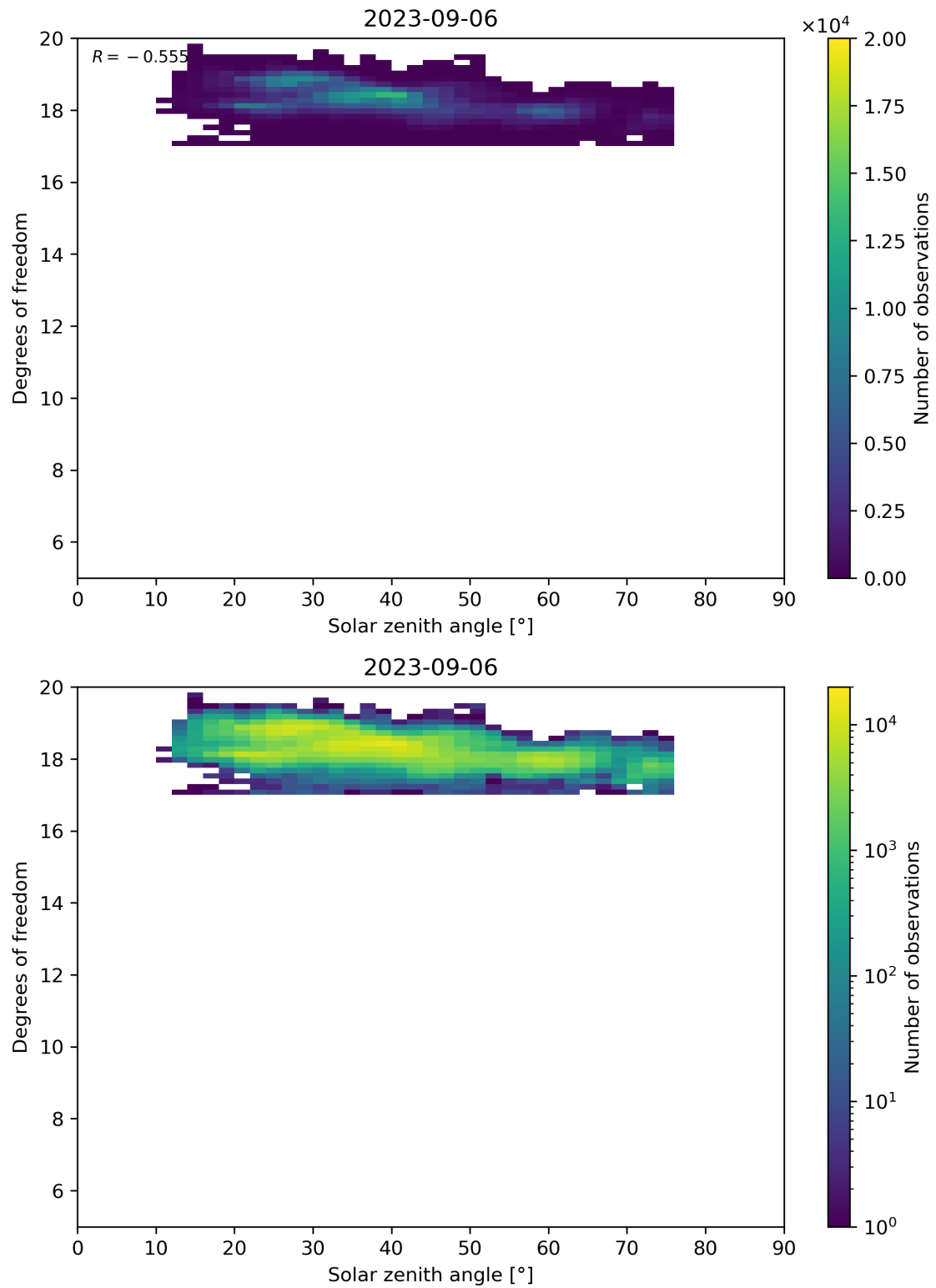
Figure 96: Scatter density plot of “Solar zenith angle” against “Degrees of freedom” for 2023-09-05 to 2023-09-07.
