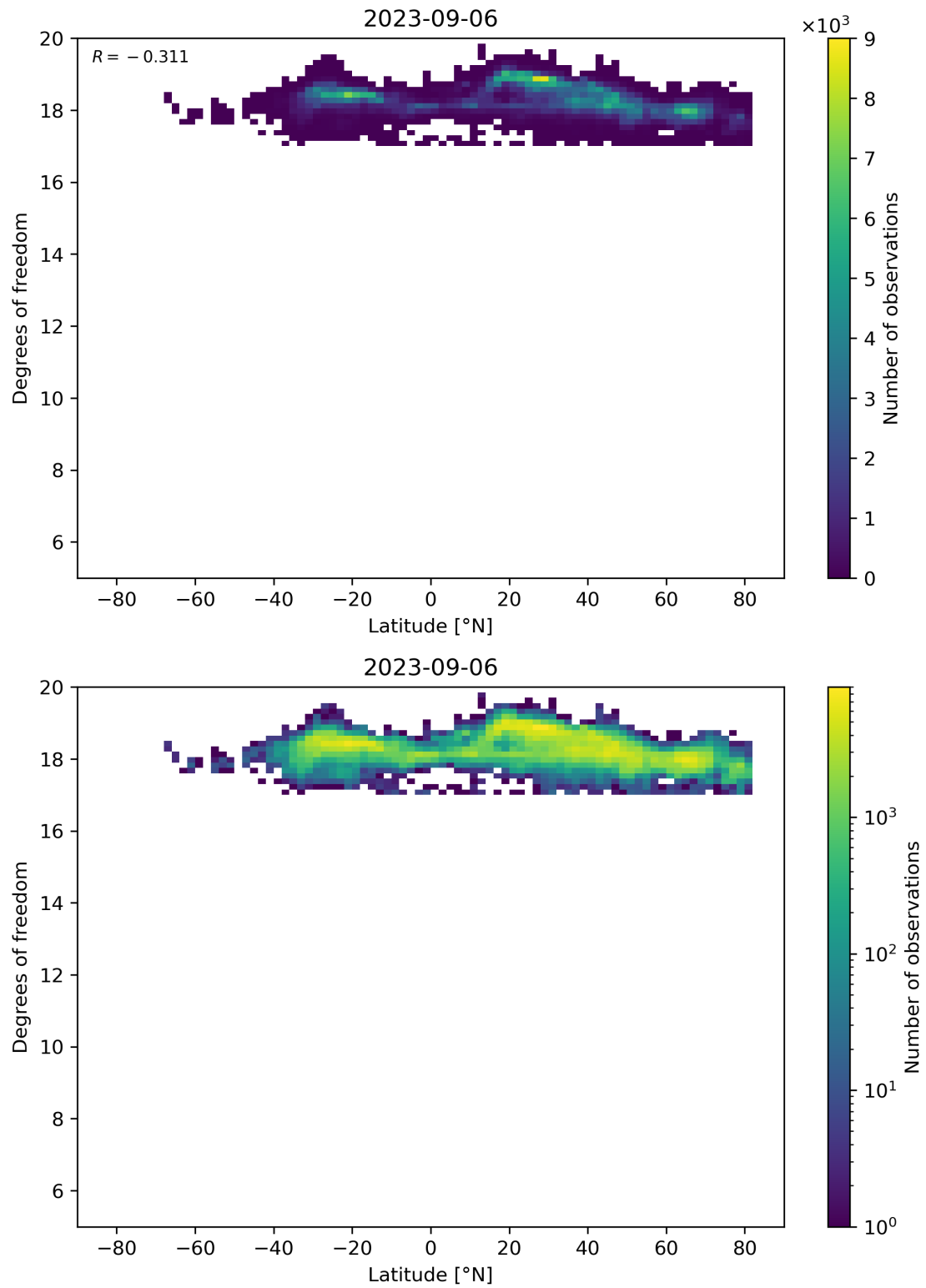
Figure 55: Scatter density plot of “Latitude” against “Degrees of freedom” for 2023-09-05 to 2023-09-07.
