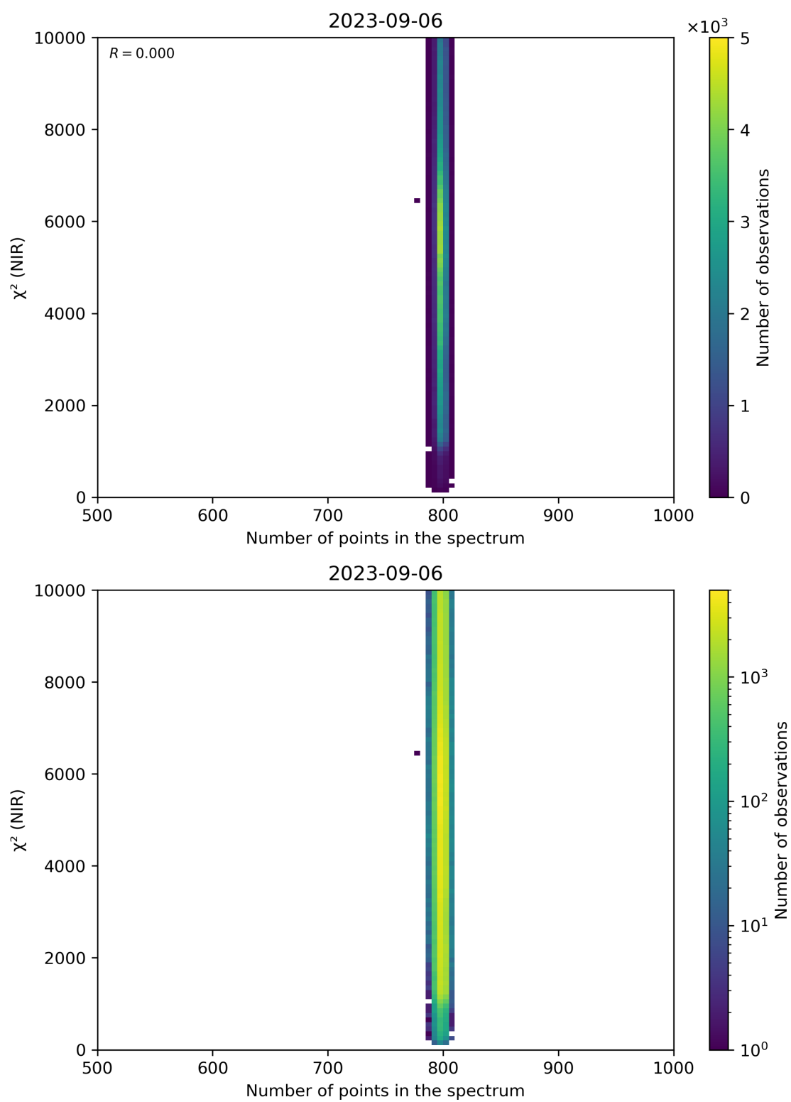
Figure 88: Scatter density plot of “Number of points in the spectrum” against “ \chi^2 (NIR)” for 2023-09-05 to 2023-09-07.
