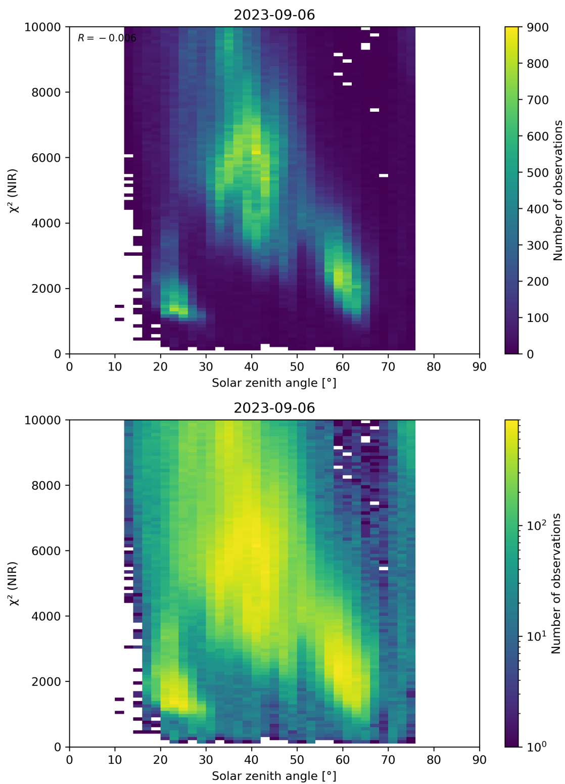
Figure 94: Scatter density plot of “Solar zenith angle” against “ \chi^2 (NIR)” for 2023-09-05 to 2023-09-07.
