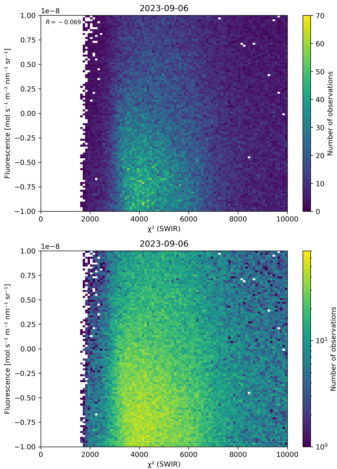
Figure 49: Scatter density plot of “ \chi^2 (SWIR)” against “Fluorescence” for 2023-09-05 to 2023-09-07.
