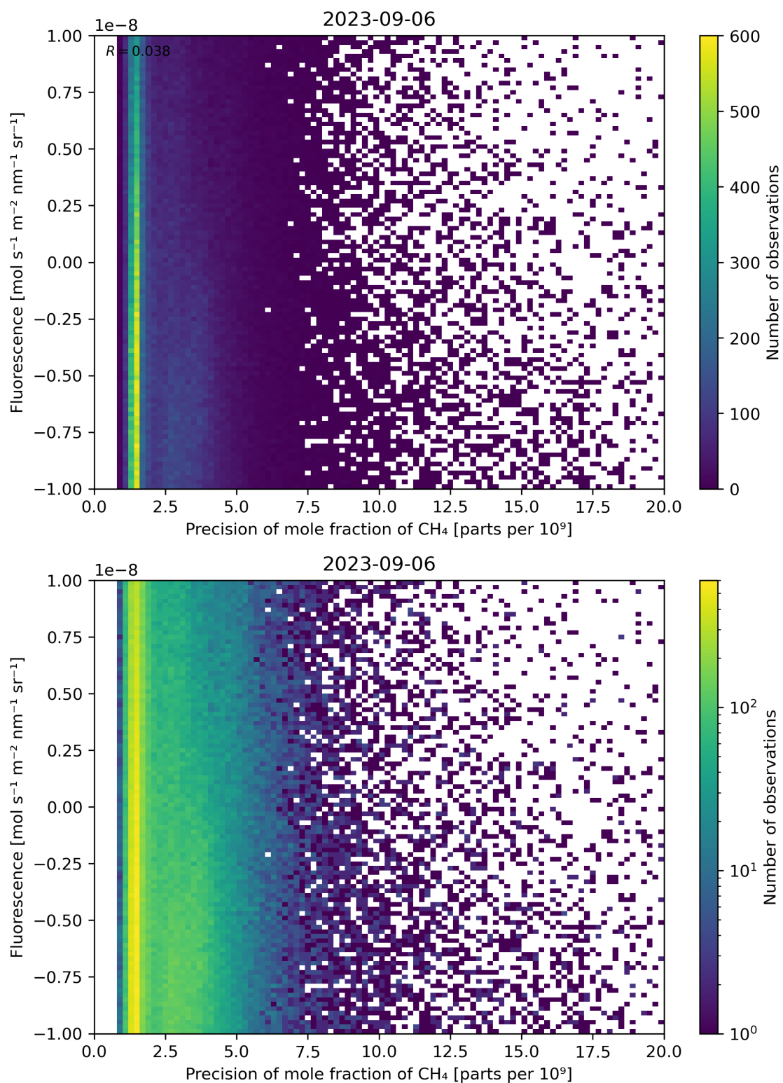
Figure 81: Scatter density plot of “Precision of mole fraction of \text{CH}_4 ” against “Fluorescence” for 2023-09-05 to 2023-09-07.
