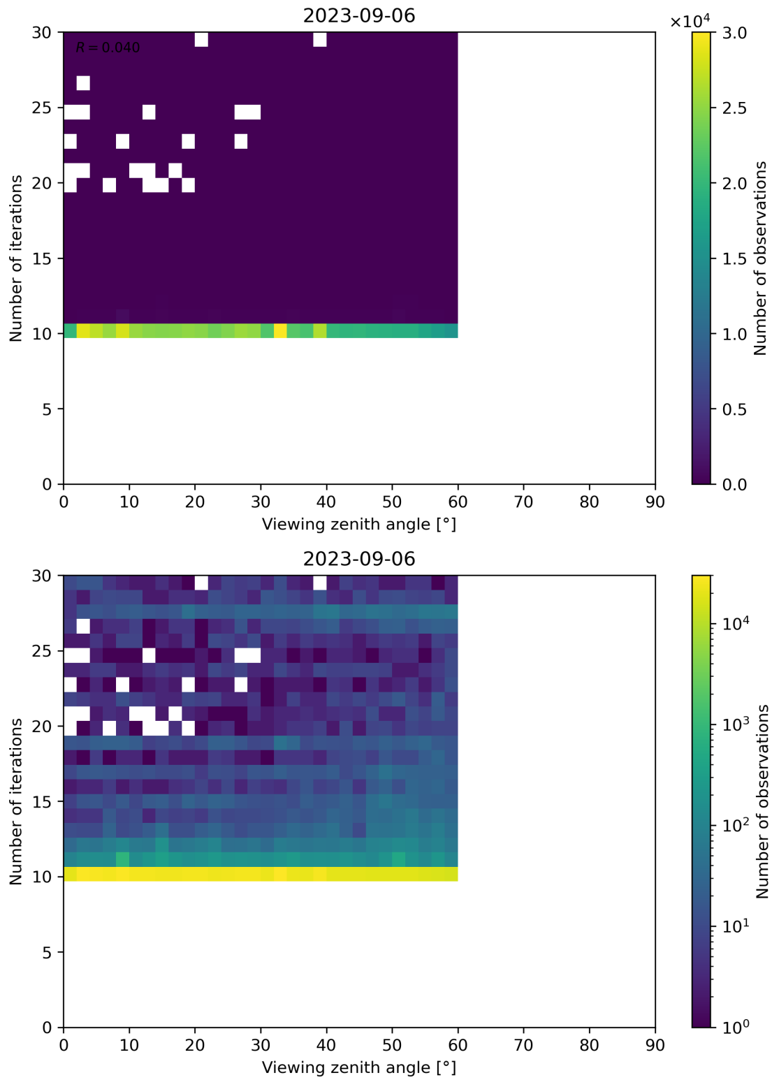
Figure 113: Scatter density plot of “Viewing zenith angle” against “Number of iterations” for 2023-09-05 to 2023-09-07.
