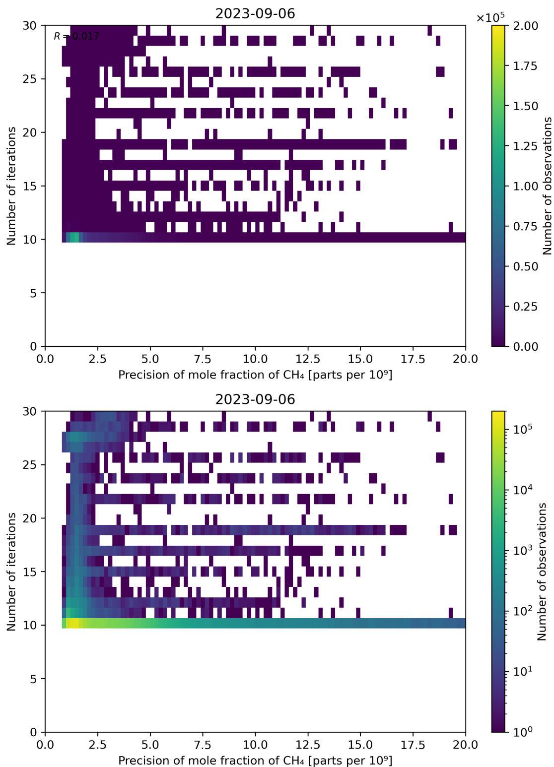
Figure 83: Scatter density plot of “Precision of mole fraction of CH 4 ” against “Number of iterations” for 2023-09-05 to 2023-09-07.
