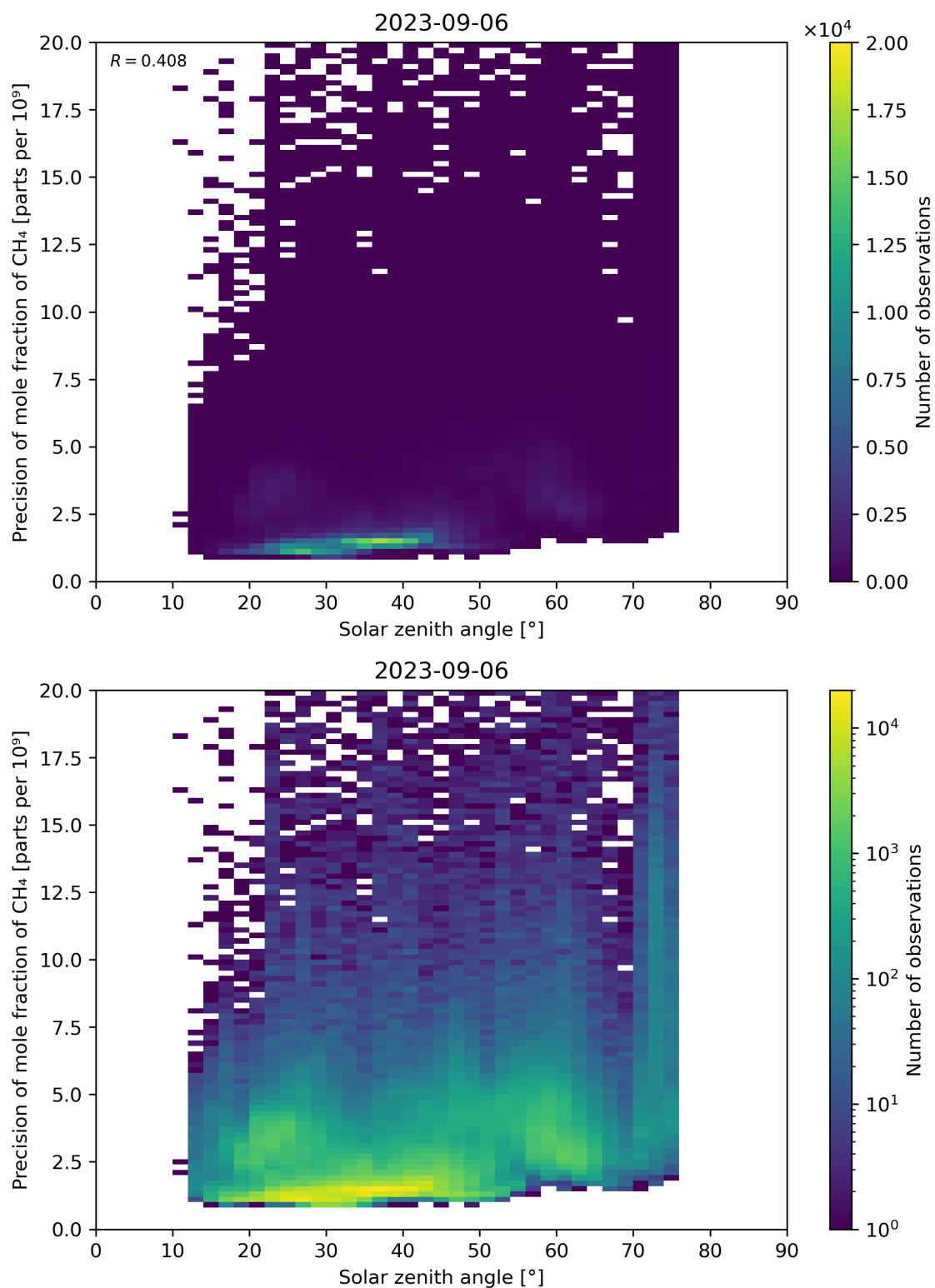
Figure 101: Scatter density plot of “Solar zenith angle” against “Precision of mole fraction of CH 4 ” for 2023-09-05 to 2023-09-07.
