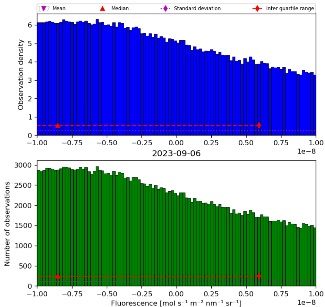
Figure 32: Histogram of “Fluorescence” for 2023-09-05 to 2023-09-07
