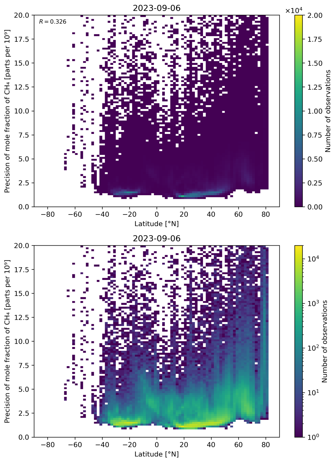
Figure 59: Scatter density plot of “Latitude” against “Precision of mole fraction of \text{CH}_4 ” for 2023-09-05 to 2023-09-07.
