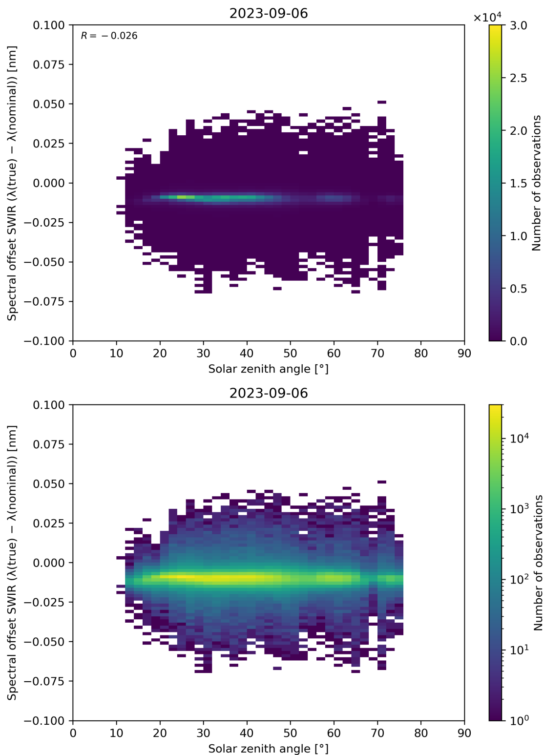
Figure 104: Scatter density plot of “Solar zenith angle” against “Spectral offset SWIR ( \lambda(\text{true}) - \lambda(\text{nominal}) )” for 2023-09-05 to 2023-09-07.
