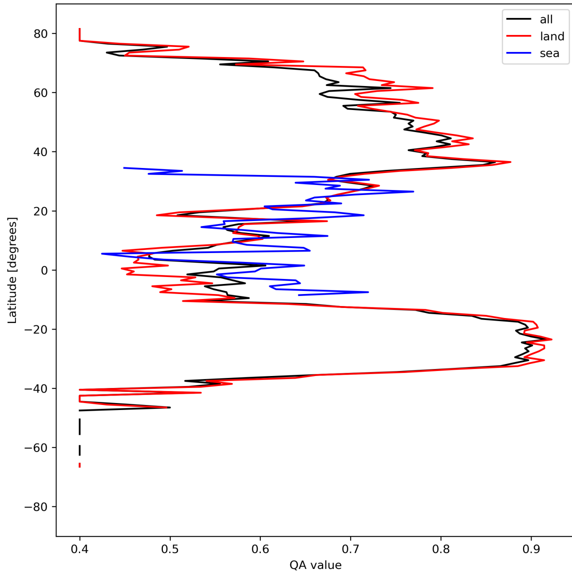
Figure 11: Zonal average of “QA value” for 2023-09-05 to 2023-09-07.
