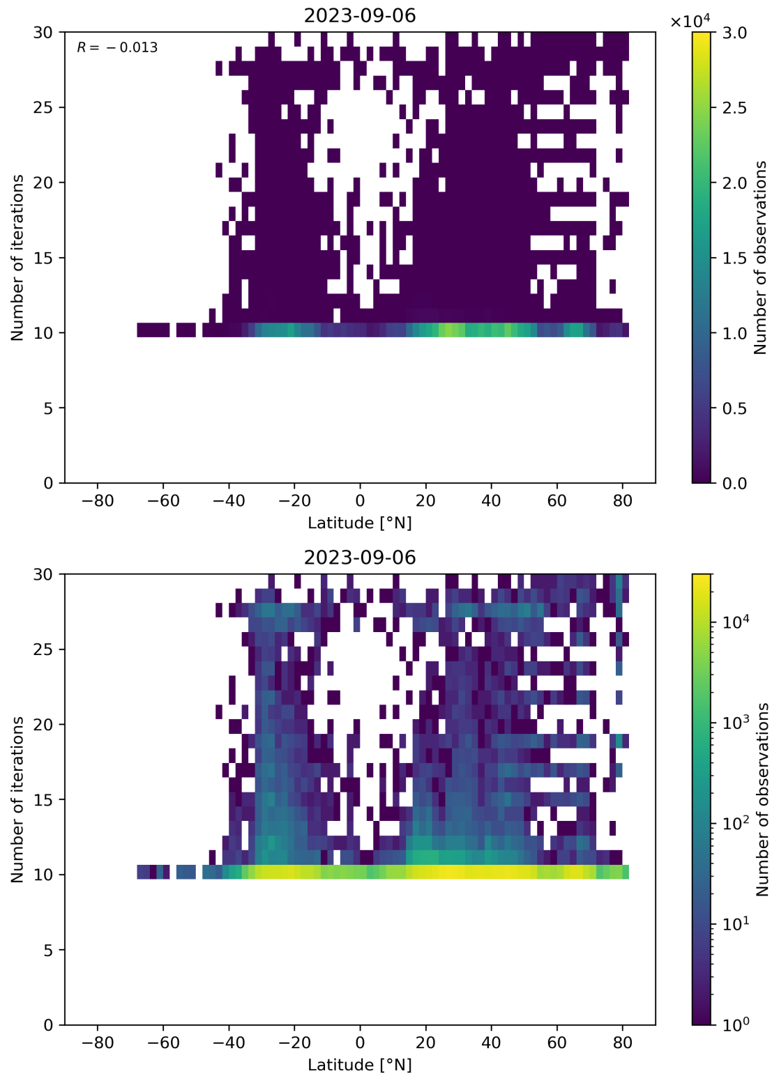
Figure 60: Scatter density plot of “Latitude” against “Number of iterations” for 2023-09-05 to 2023-09-07.
