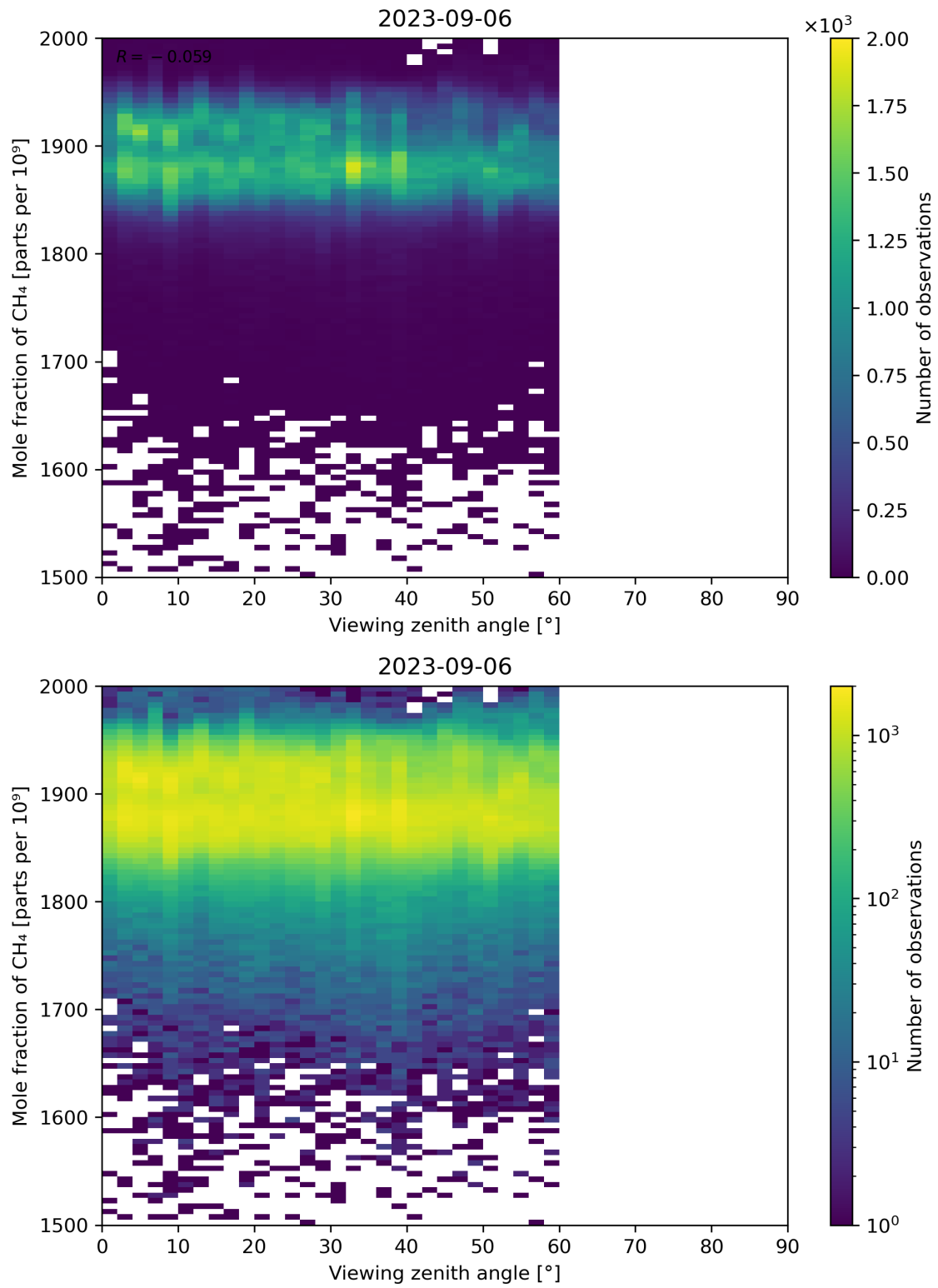
Figure 110: Scatter density plot of “Viewing zenith angle” against “Mole fraction of CH 4 ” for 2023-09-05 to 2023-09-07.
