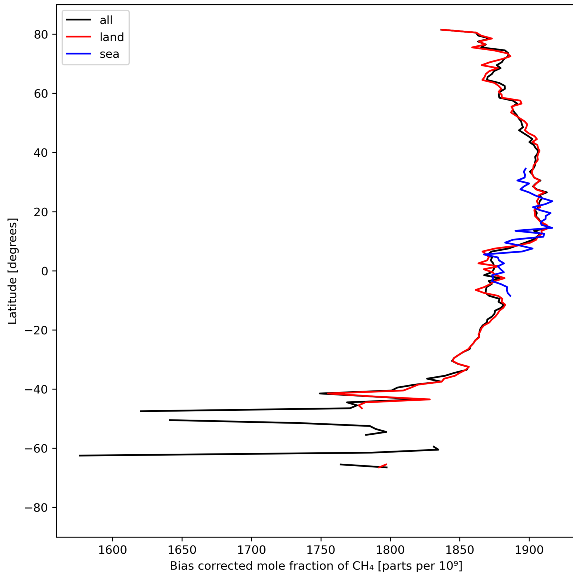
Figure 14: Zonal average of “Bias corrected mole fraction of CH 4 ” for 2023-09-05 to 2023-09-07.
