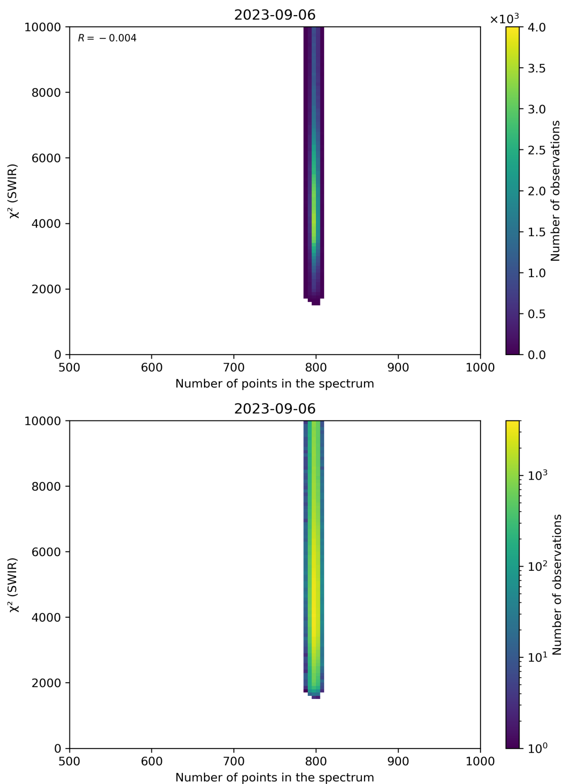
Figure 89: Scatter density plot of “Number of points in the spectrum” against “ \chi^2 (SWIR)” for 2023-09-05 to 2023-09-07.
