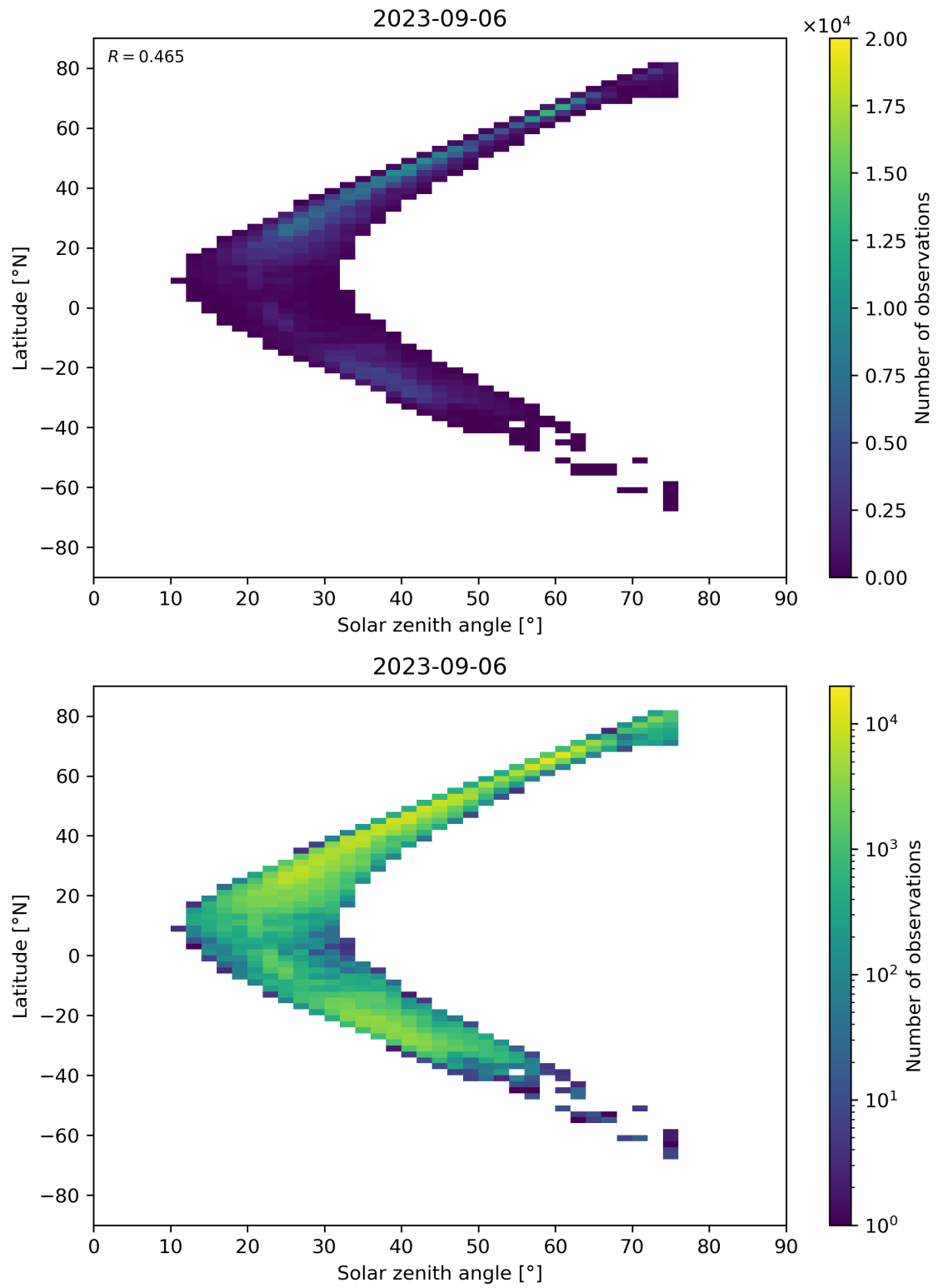
Figure 98: Scatter density plot of “Solar zenith angle” against “Latitude” for 2023-09-05 to 2023-09-07.
