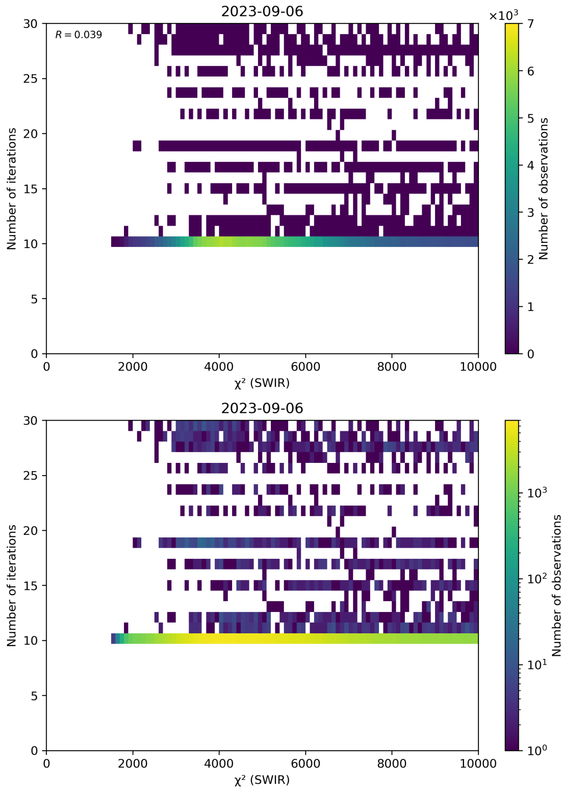
Figure 50: Scatter density plot of “ \chi^2 (SWIR)” against “Number of iterations” for 2023-09-05 to 2023-09-07.
