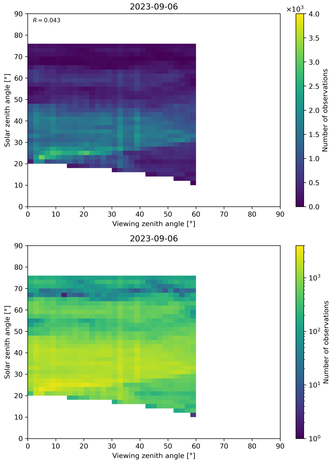
Figure 115: Scatter density plot of “Viewing zenith angle” against “Solar zenith angle” for 2023-09-05 to 2023-09-07.
