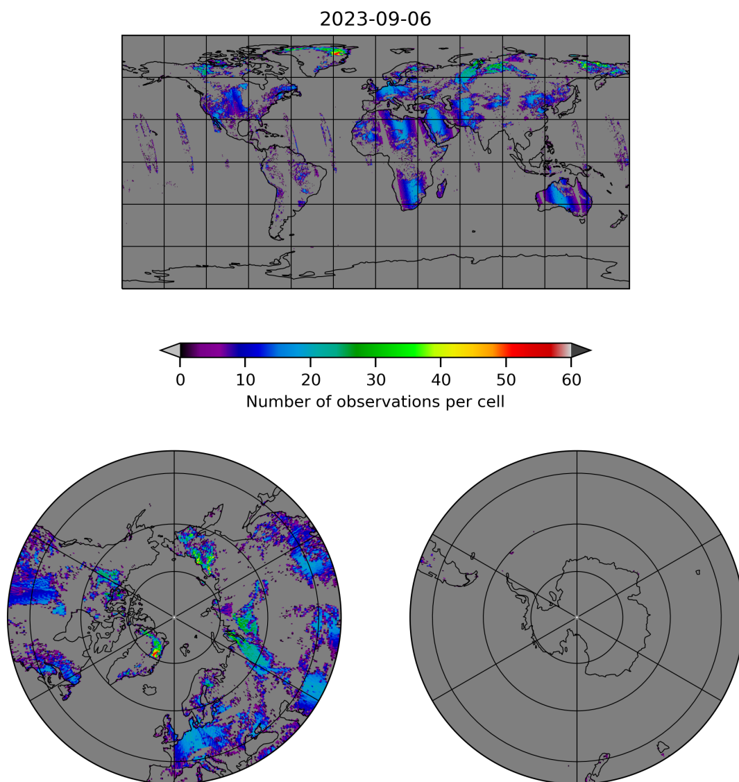
Figure 10: Map of the number of observations for 2023-09-05 to 2023-09-07
