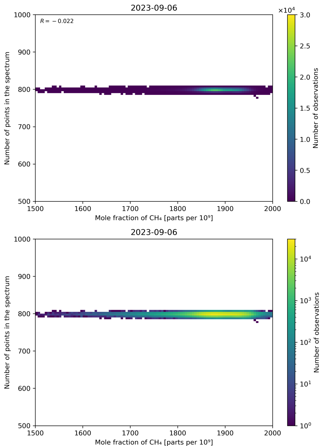
Figure 77: Scatter density plot of “Mole fraction of CH 4 ” against “Number of points in the spectrum” for 2023-09-05 to 2023-09-07.
