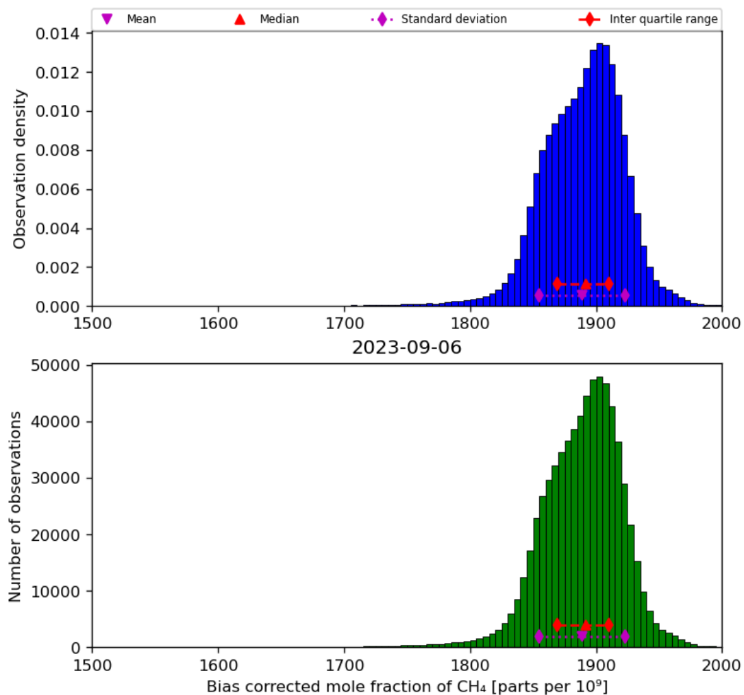
Figure 25: Histogram of “Bias corrected mole fraction of CH 4 ” for 2023-09-05 to 2023-09-07
