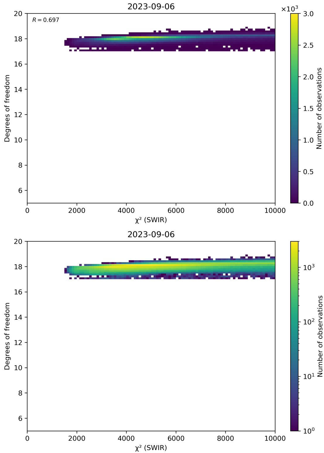
Figure 48: Scatter density plot of “ \chi^2 (SWIR)” against “Degrees of freedom” for 2023-09-05 to 2023-09-07.
