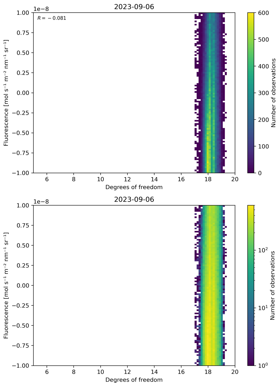
Figure 51: Scatter density plot of “Degrees of freedom” against “Fluorescence” for 2023-09-05 to 2023-09-07.
