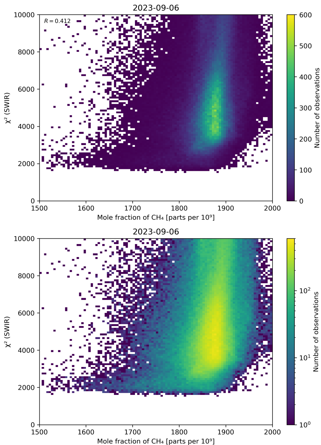
Figure 71: Scatter density plot of “Mole fraction of \text{CH}_4 ” against “ \chi^2 (SWIR)” for 2023-09-05 to 2023-09-07.
