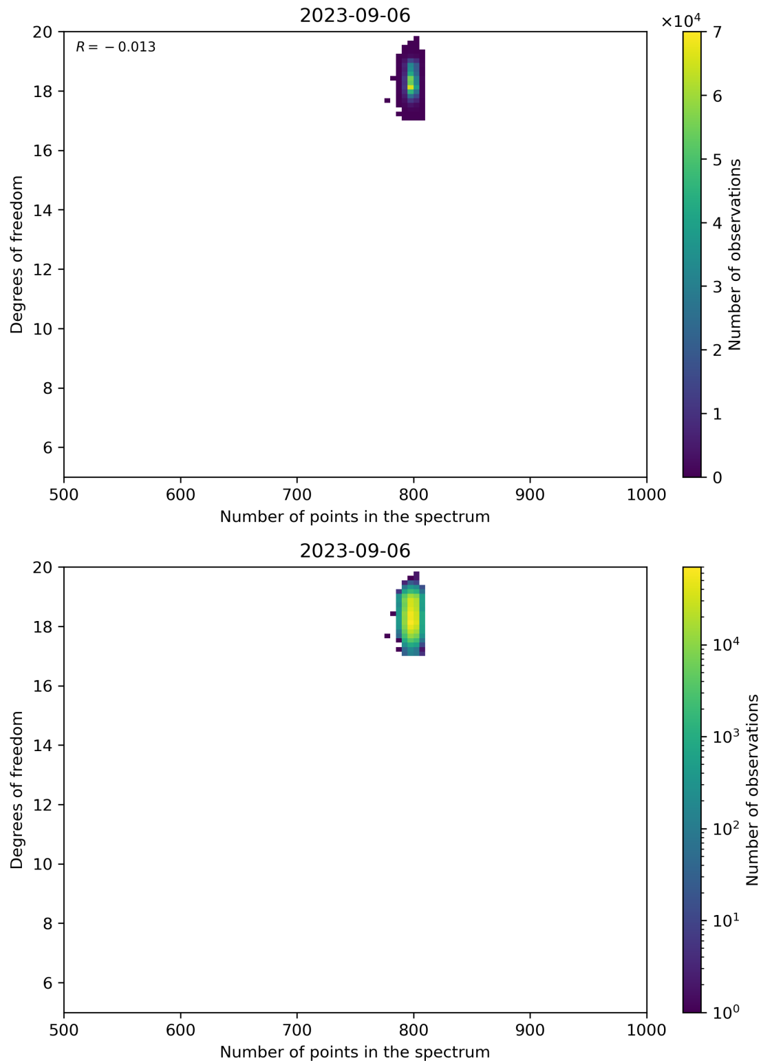
Figure 90: Scatter density plot of “Number of points in the spectrum” against “Degrees of freedom” for 2023-09-05 to 2023-09-07.
