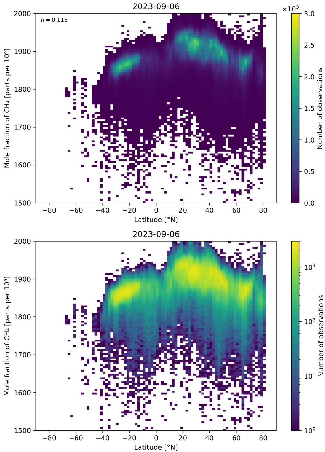
Figure 57: Scatter density plot of “Latitude” against “Mole fraction of CH 4 ” for 2023-09-05 to 2023-09-07.
