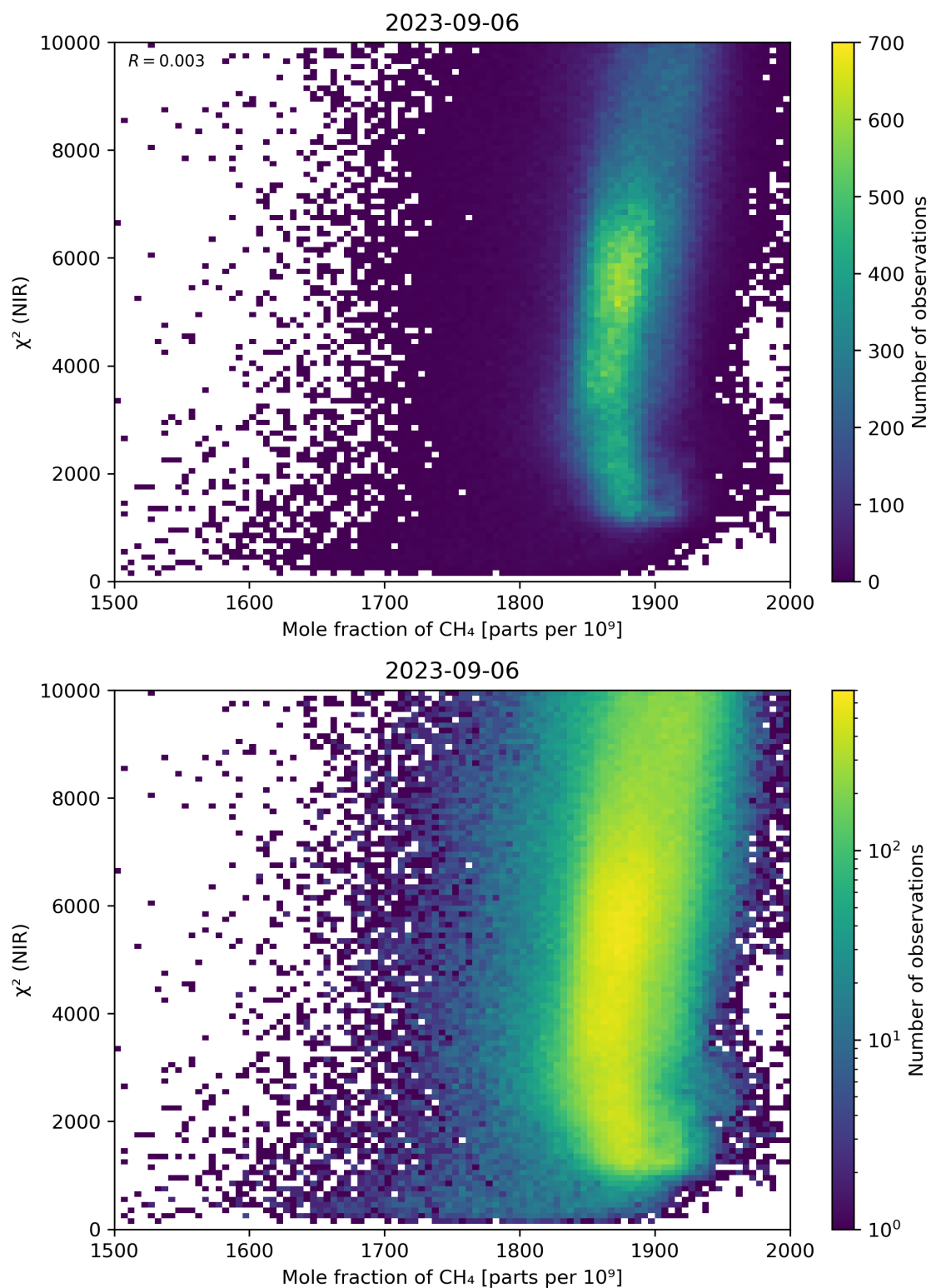
Figure 70: Scatter density plot of “Mole fraction of CH 4 ” against “ \chi^2 (NIR)” for 2023-09-05 to 2023-09-07.
