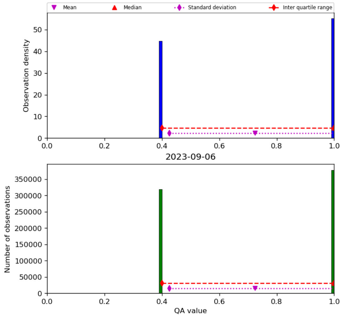
Figure 22: Histogram of “QA value” for 2023-09-05 to 2023-09-07
