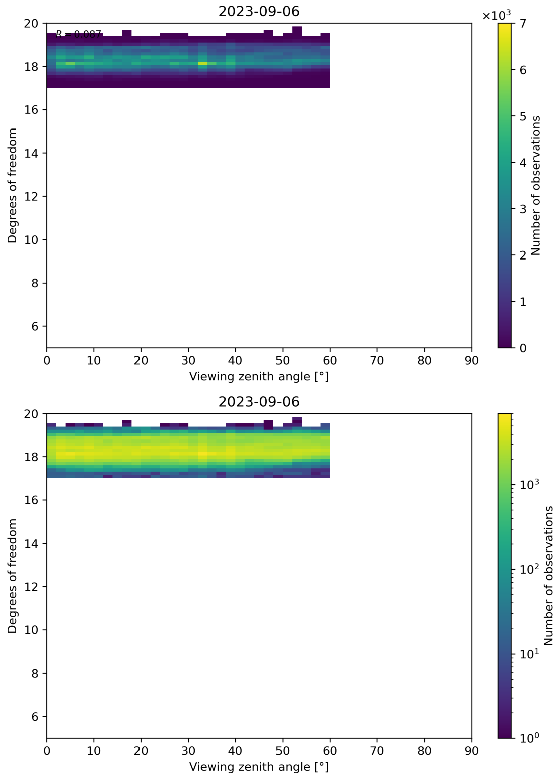
Figure 107: Scatter density plot of “Viewing zenith angle” against “Degrees of freedom” for 2023-09-05 to 2023-09-07.
