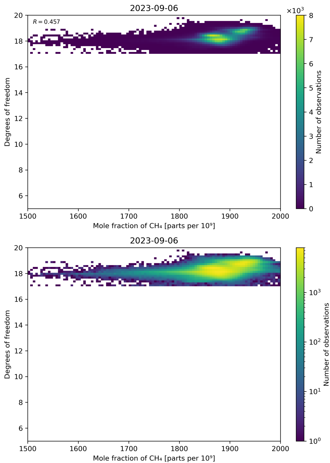
Figure 72: Scatter density plot of “Mole fraction of CH 4 ” against “Degrees of freedom” for 2023-09-05 to 2023-09-07.
