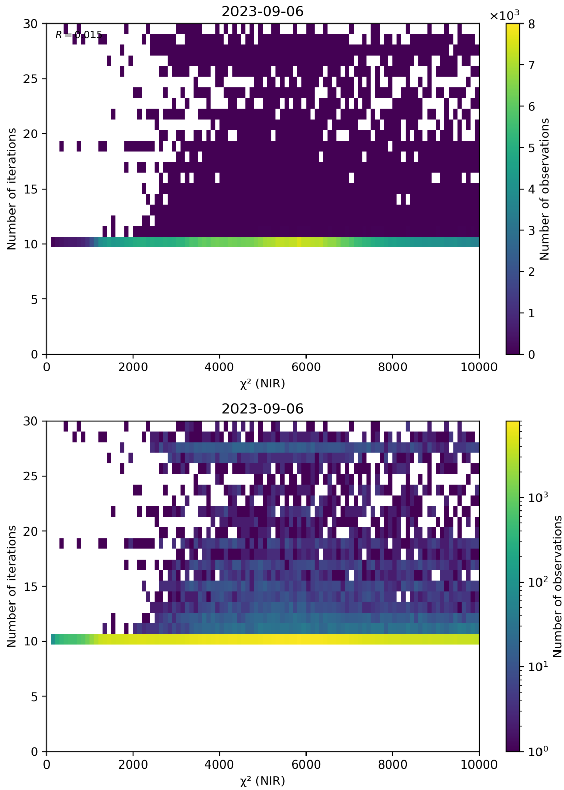
Figure 46: Scatter density plot of “ \chi^2 (NIR)” against “Number of iterations” for 2023-09-05 to 2023-09-07.
