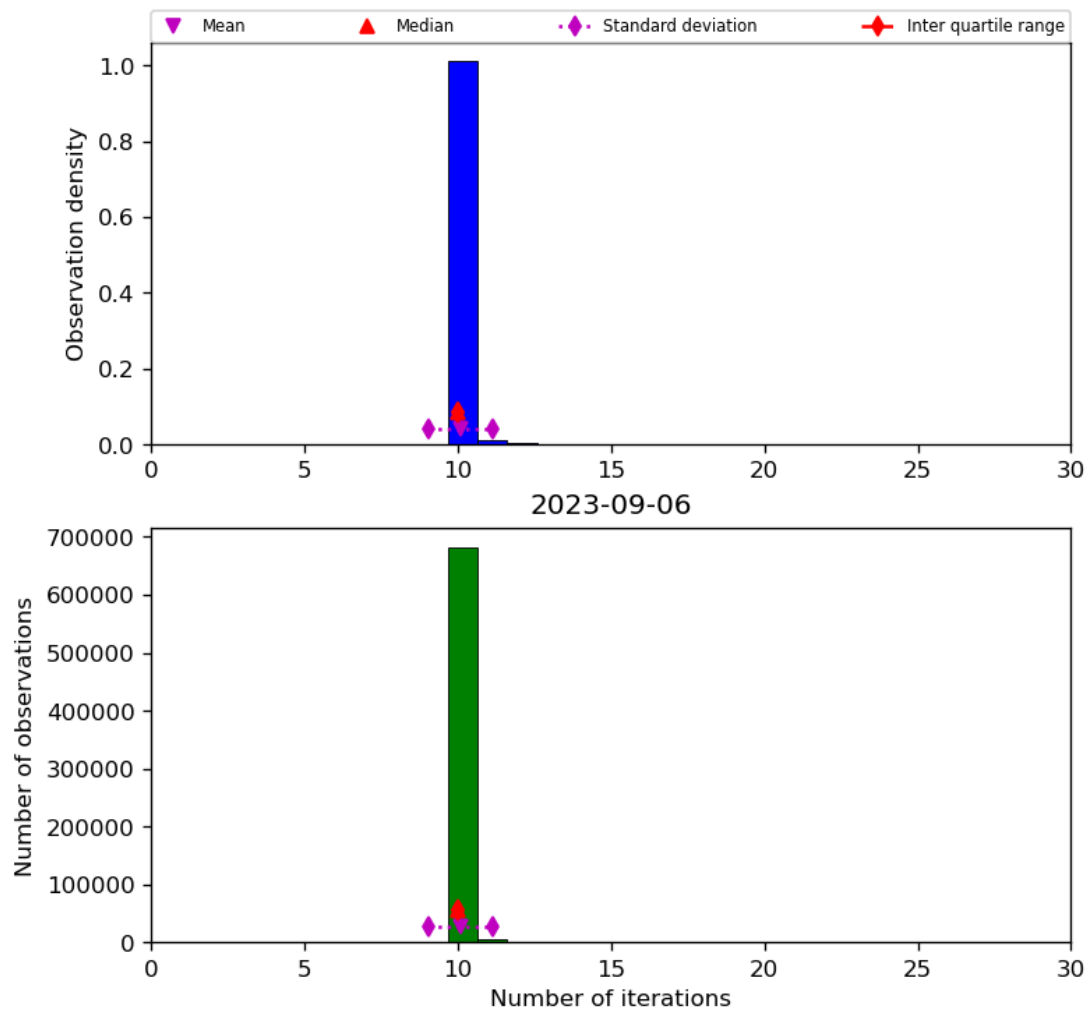
Figure 31: Histogram of “Number of iterations” for 2023-09-05 to 2023-09-07
