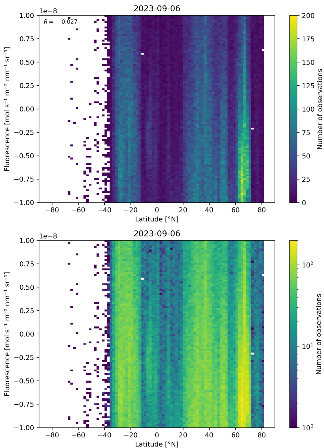
Figure 56: Scatter density plot of “Latitude” against “Fluorescence” for 2023-09-05 to 2023-09-07.
