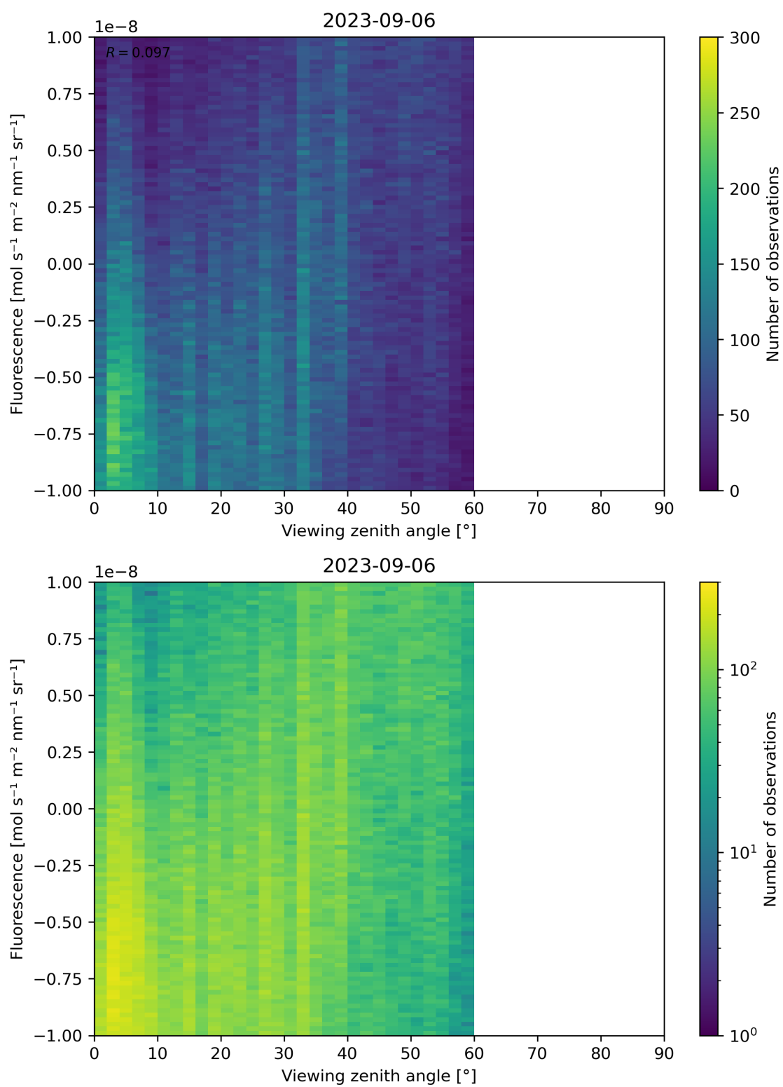
Figure 108: Scatter density plot of “Viewing zenith angle” against “Fluorescence” for 2023-09-05 to 2023-09-07.
