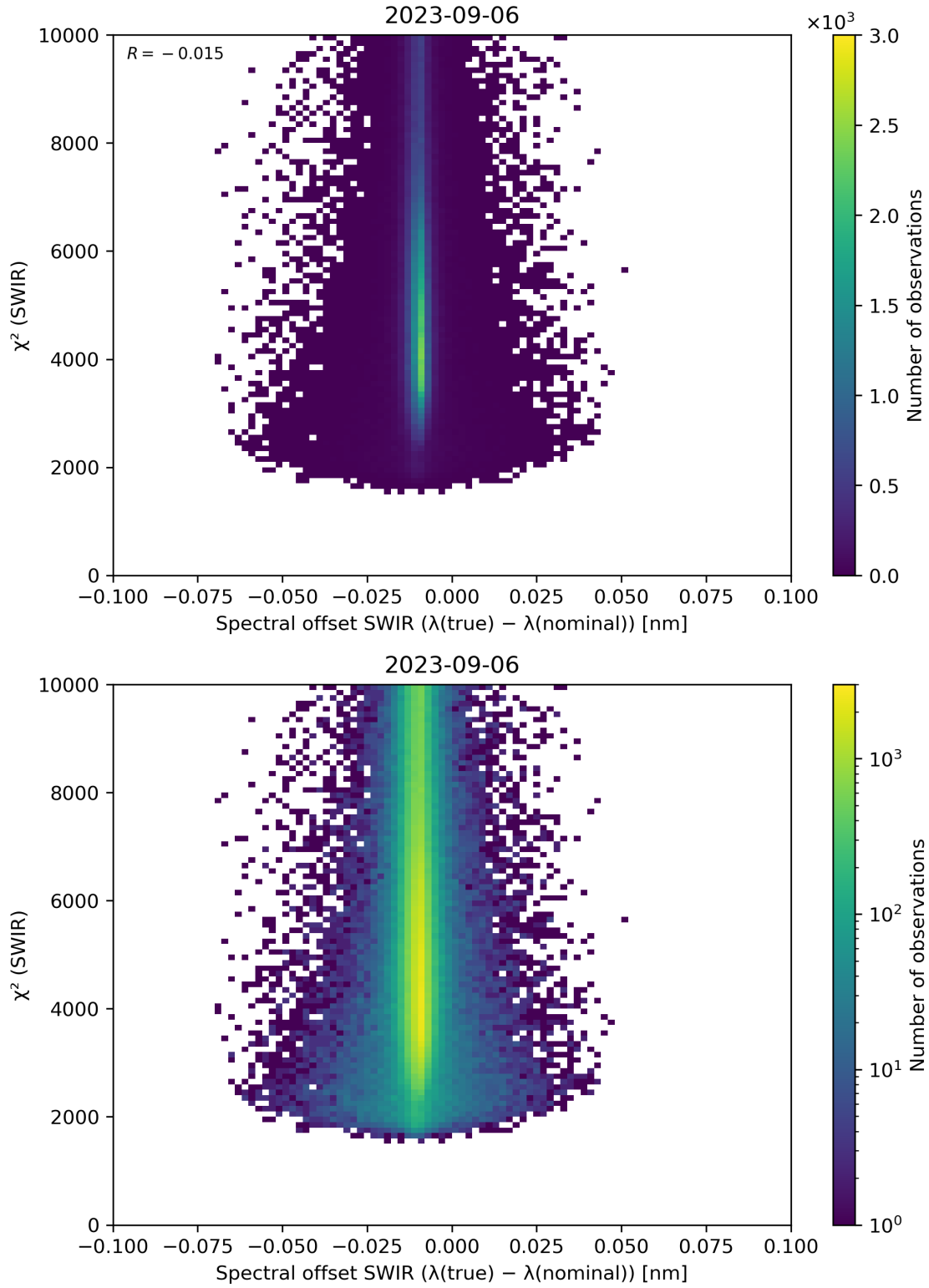
Figure 118: Scatter density plot of “Spectral offset SWIR ( \lambda(\text{true}) - \lambda(\text{nominal}) )” against “ \chi^2 (SWIR)” for 2023-09-05 to 2023-09-07.
