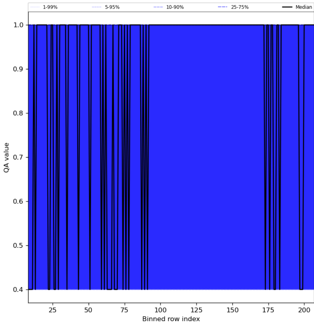
Figure 33: Along track statistics of “QA value” for 2023-09-05 to 2023-09-07
