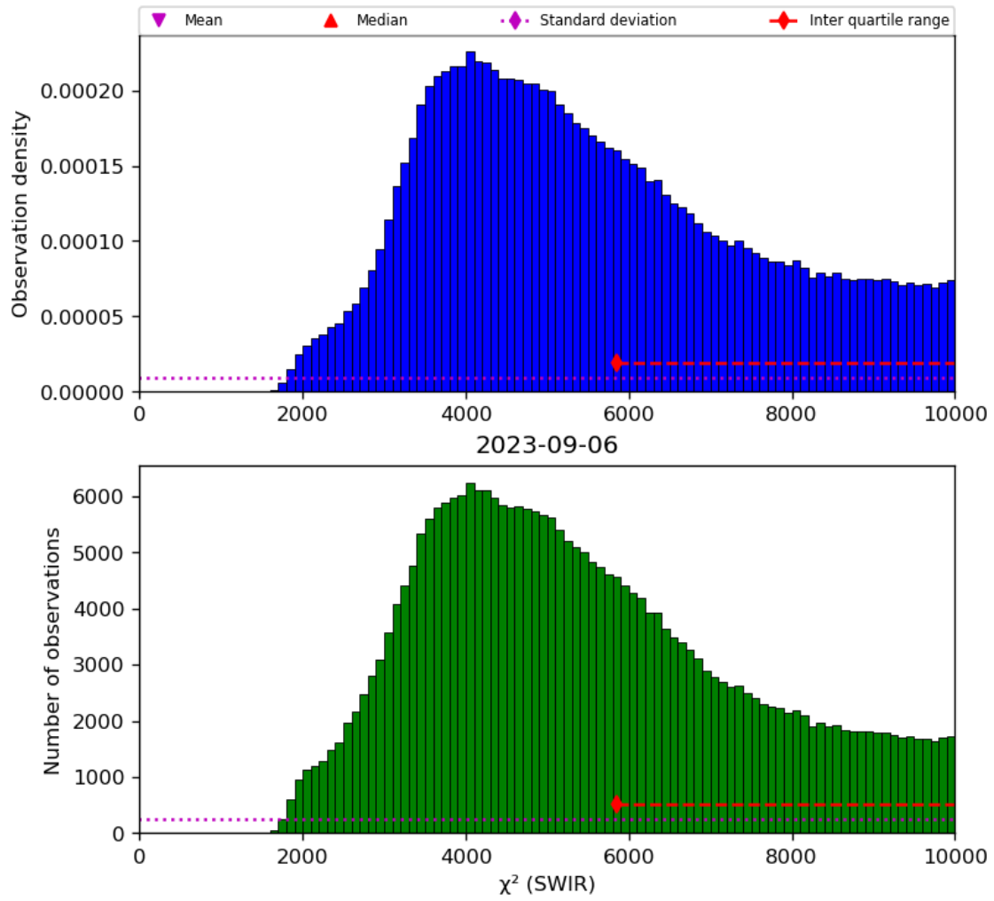
Figure 28: Histogram of “ \chi^2 (SWIR)” for 2023-09-05 to 2023-09-07
