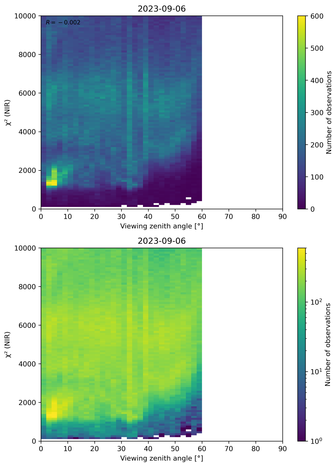
Figure 105: Scatter density plot of “Viewing zenith angle” against “ \chi^2 (NIR)” for 2023-09-05 to 2023-09-07.
