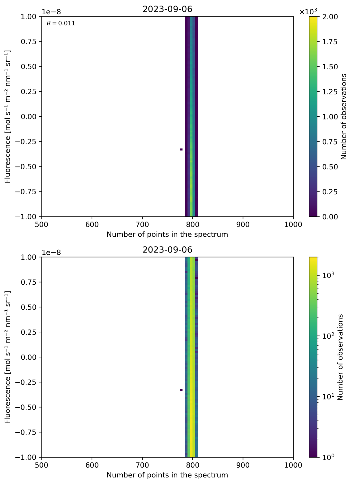
Figure 91: Scatter density plot of “Number of points in the spectrum” against “Fluorescence” for 2023-09-05 to 2023-09-07.
