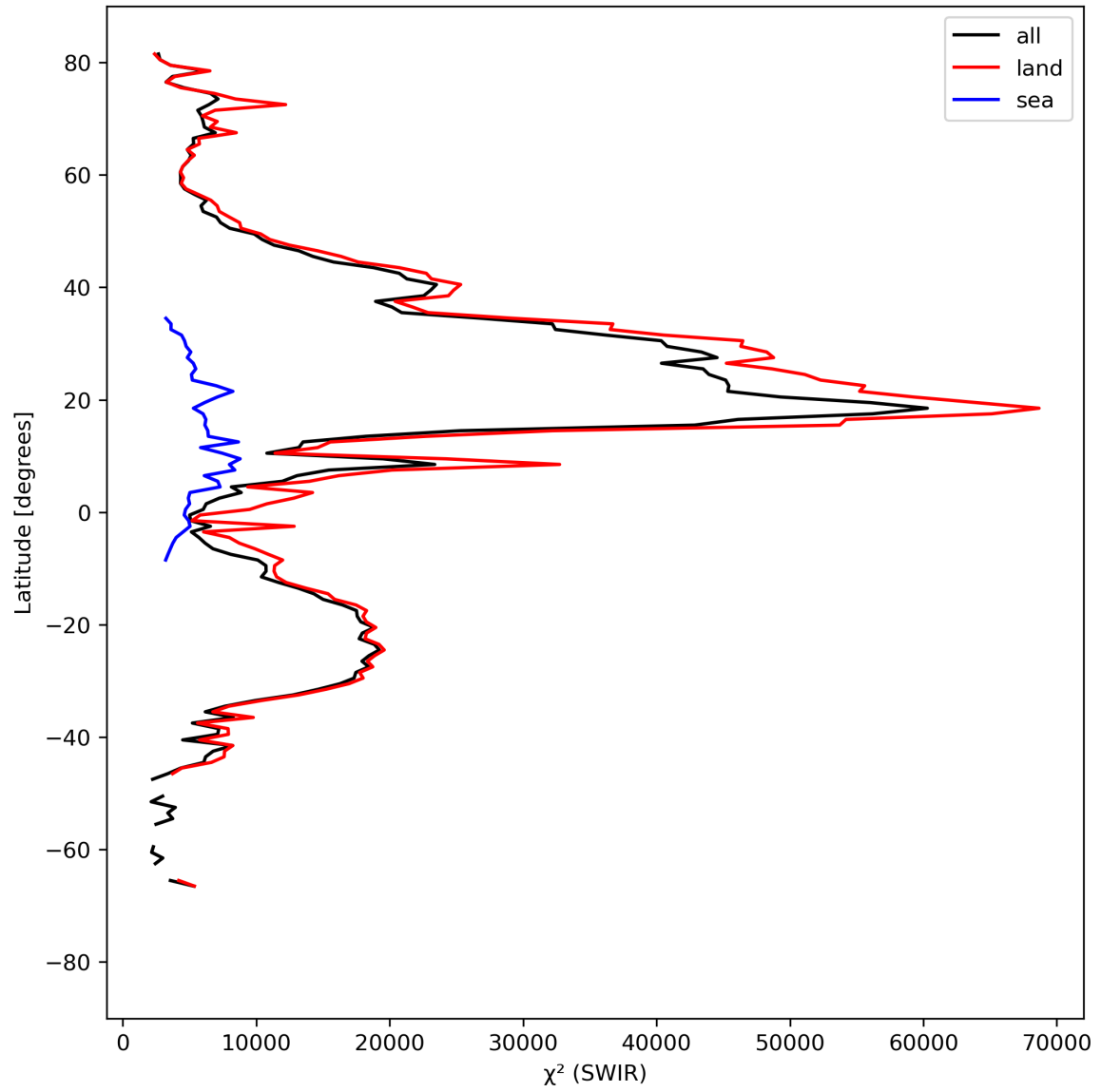
Figure 17: Zonal average of “ \chi^2 (SWIR)” for 2023-09-05 to 2023-09-07.
