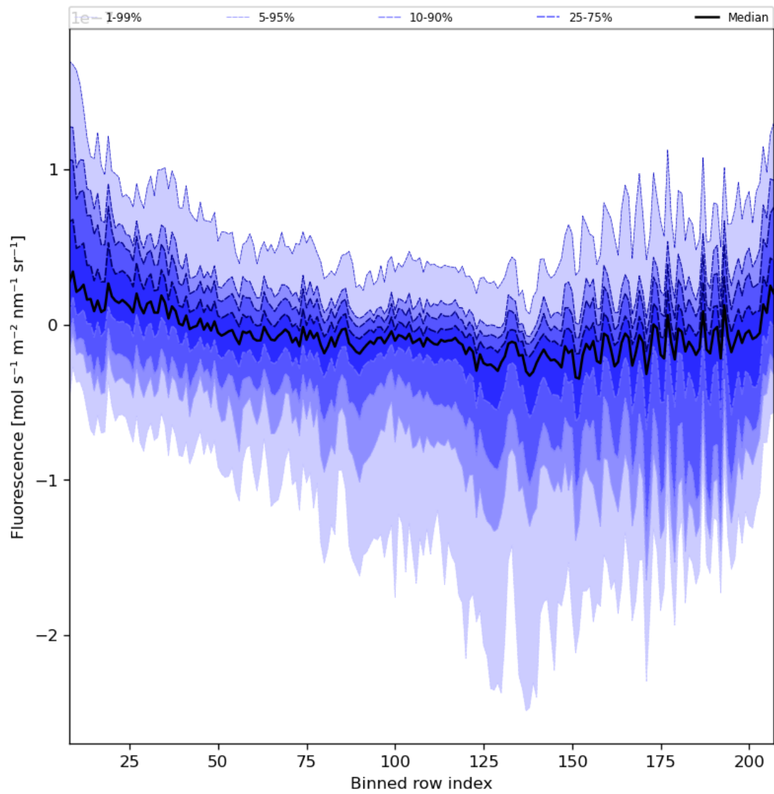
Figure 43: Along track statistics of “Fluorescence” for 2023-09-05 to 2023-09-07
