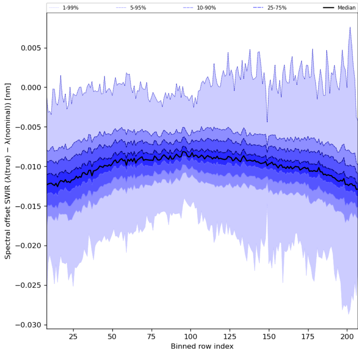
Figure 38: Along track statistics of “Spectral offset SWIR ( \lambda(\text{true}) - \lambda(\text{nominal}) )” for 2023-09-05 to 2023-09-07
