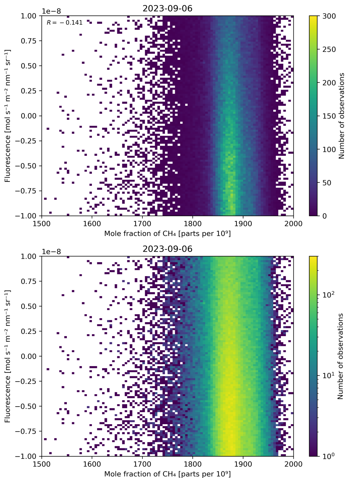
Figure 73: Scatter density plot of “Mole fraction of \text{CH}_4 ” against “Fluorescence” for 2023-09-05 to 2023-09-07.
