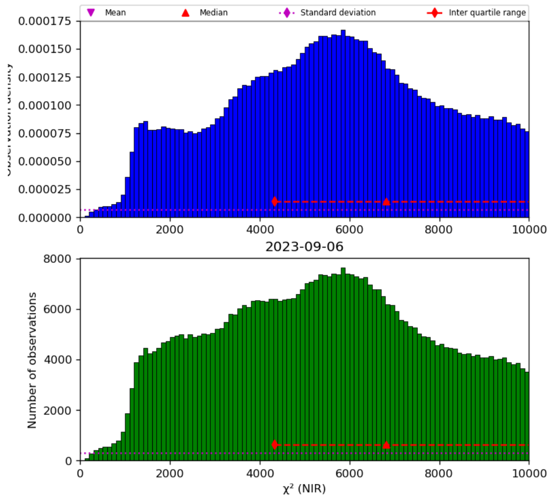
Figure 29: Histogram of “ \chi^2 (NIR)” for 2023-09-05 to 2023-09-07
