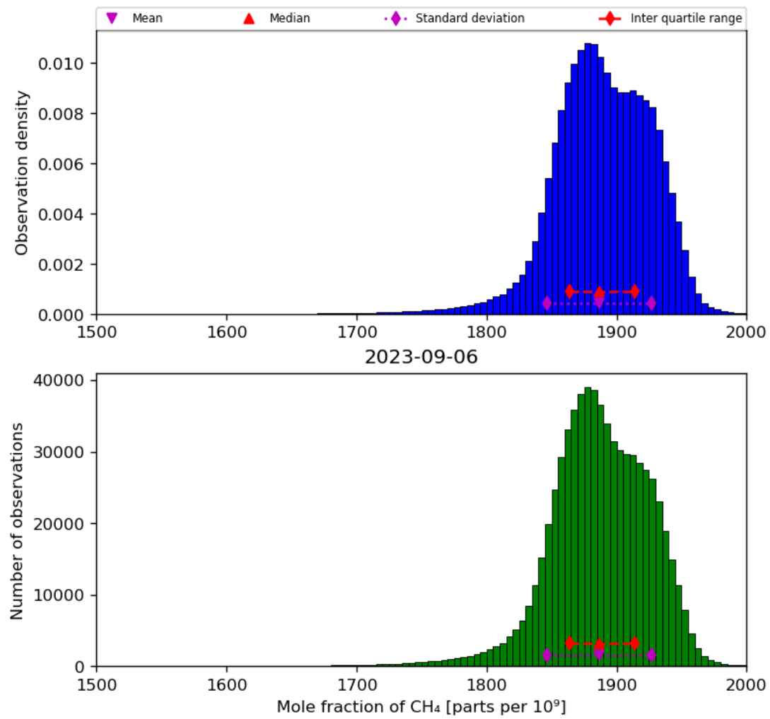
Figure 23: Histogram of “Mole fraction of CH 4 ” for 2023-09-05 to 2023-09-07
