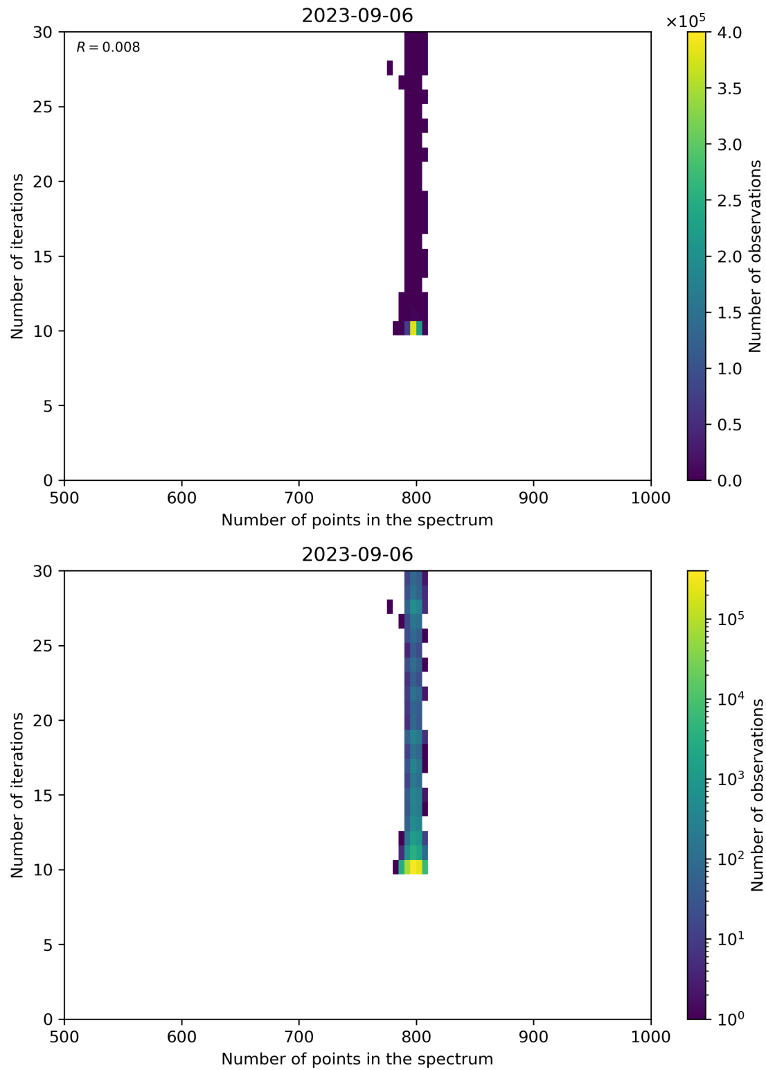
Figure 92: Scatter density plot of “Number of points in the spectrum” against “Number of iterations” for 2023-09-05 to 2023-09-07.
