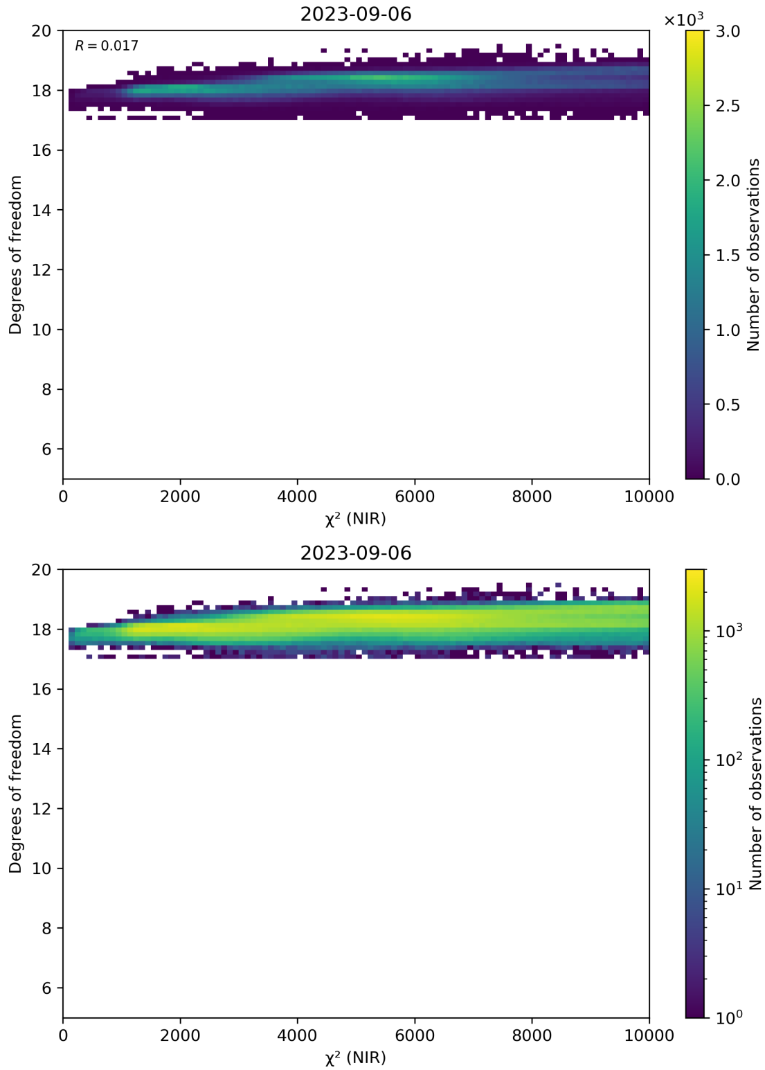
Figure 44: Scatter density plot of “ \chi^2 (NIR)” against “Degrees of freedom” for 2023-09-05 to 2023-09-07.
