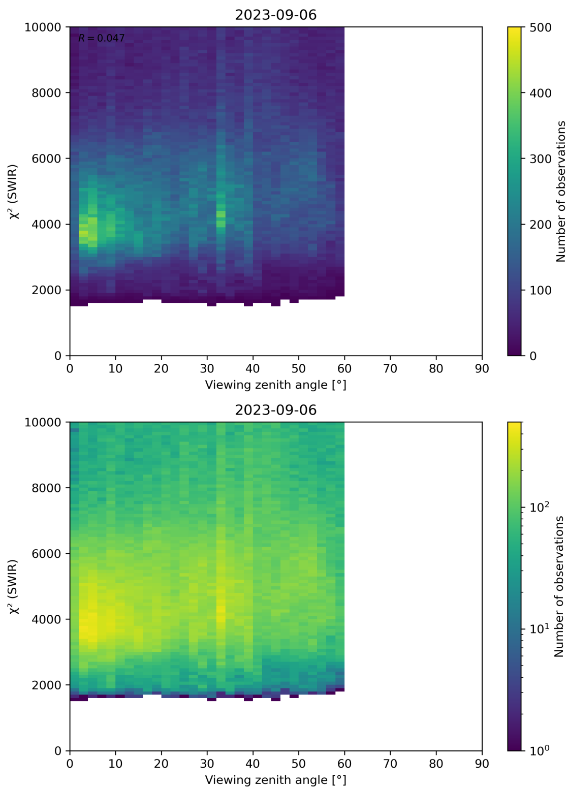
Figure 106: Scatter density plot of “Viewing zenith angle” against “ \chi^2 (SWIR)” for 2023-09-05 to 2023-09-07.
