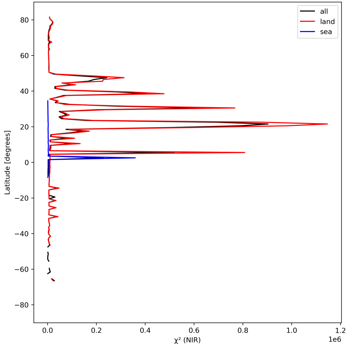
Figure 18: Zonal average of “ \chi^2 (NIR)” for 2023-09-05 to 2023-09-07.
