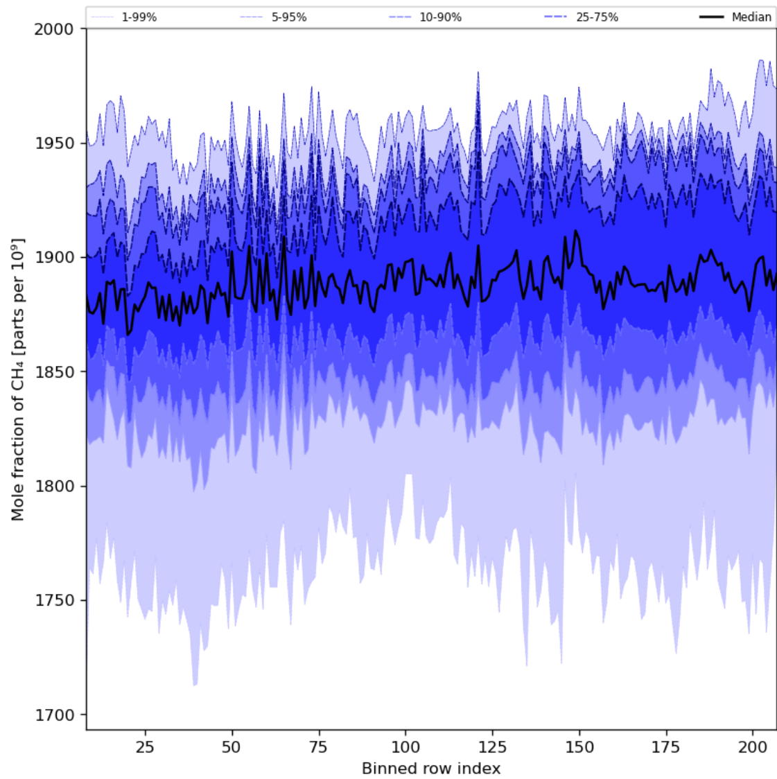
Figure 34: Along track statistics of “Mole fraction of CH 4 ” for 2023-09-05 to 2023-09-07
