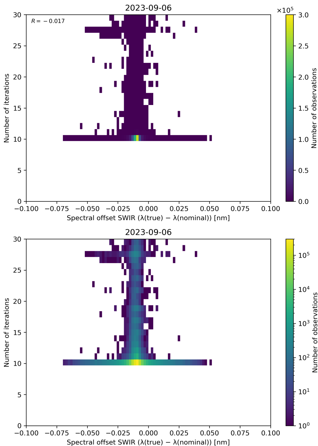
Figure 121: Scatter density plot of “Spectral offset SWIR ( \lambda(\text{true}) - \lambda(\text{nominal}) )” against “Number of iterations” for 2023-09-05 to 2023-09-07.
