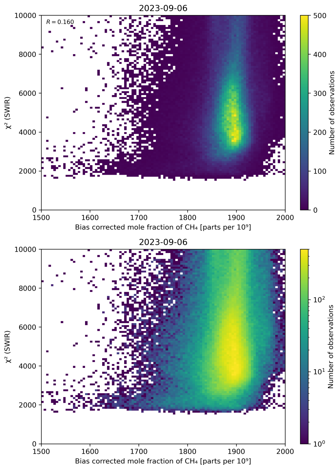
Figure 64: Scatter density plot of “Bias corrected mole fraction of CH 4 ” against “ \chi^2 (SWIR)” for 2023-09-05 to 2023-09-07.
