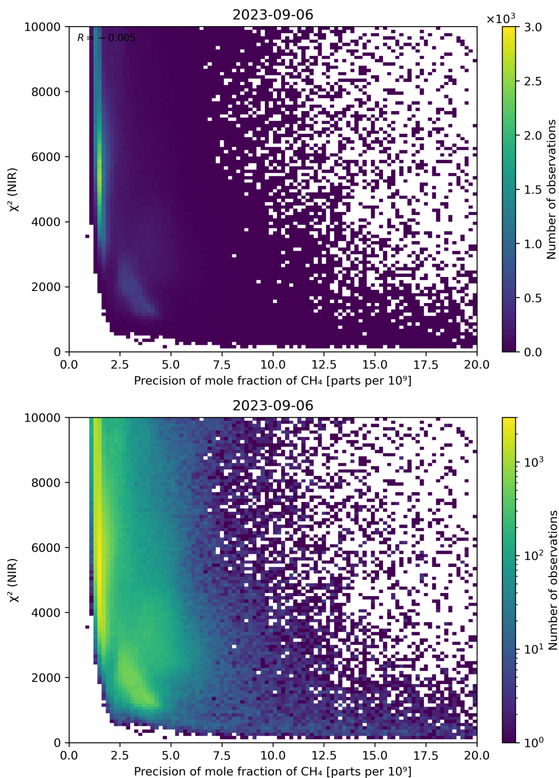
Figure 78: Scatter density plot of “Precision of mole fraction of CH 4 ” against “ \chi^2 (NIR)” for 2023-09-05 to 2023-09-07.
