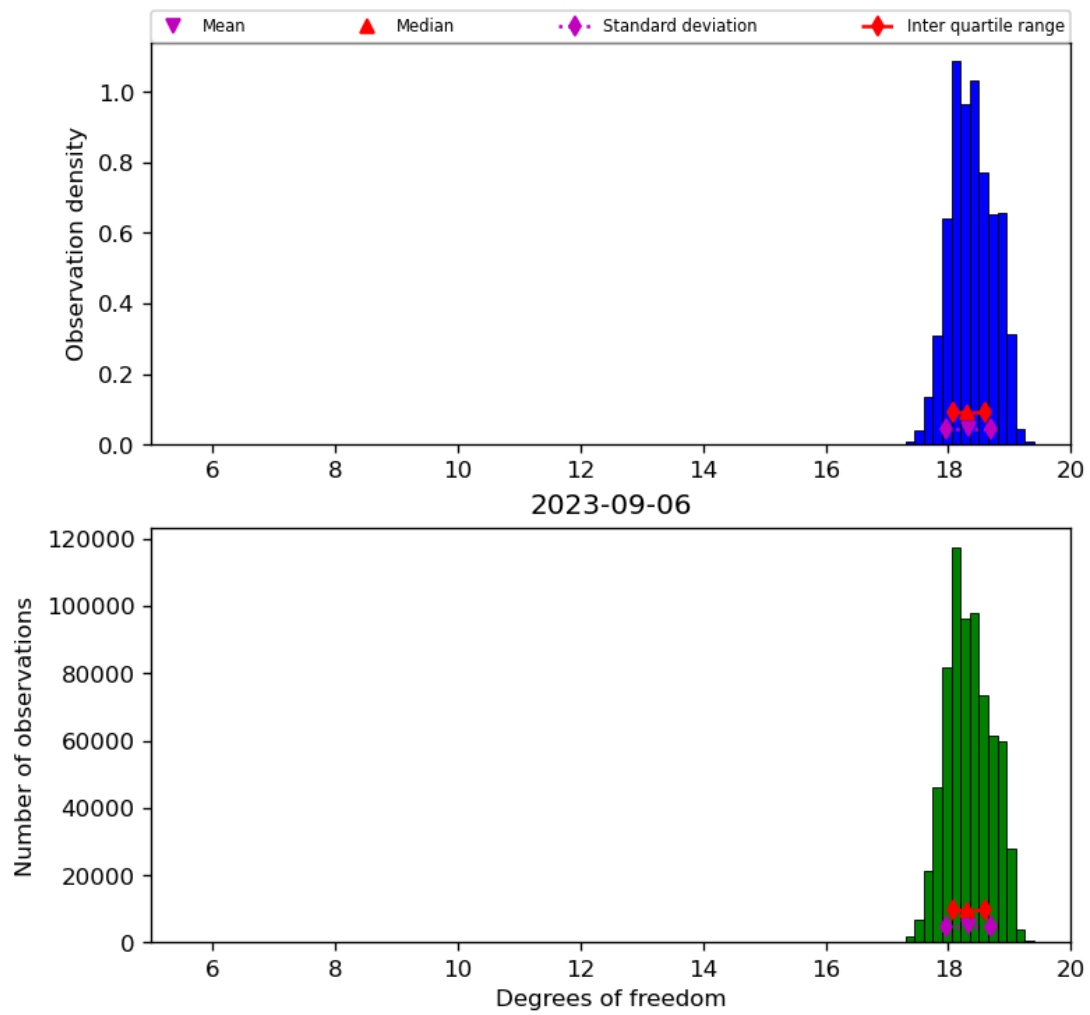
Figure 30: Histogram of “Degrees of freedom” for 2023-09-05 to 2023-09-07
