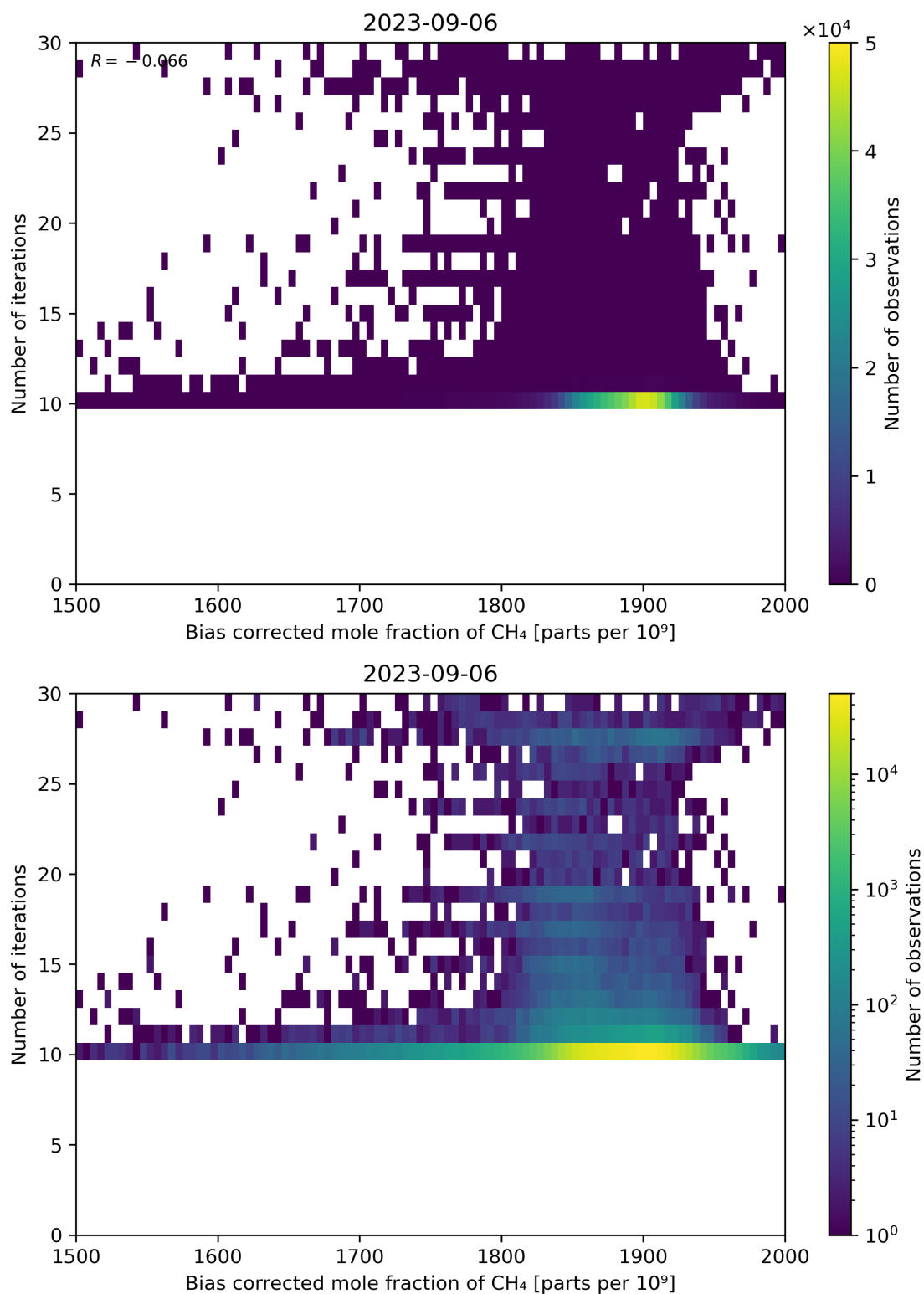
Figure 67: Scatter density plot of “Bias corrected mole fraction of CH 4 ” against “Number of iterations” for 2023-09-05 to 2023-09-07.
