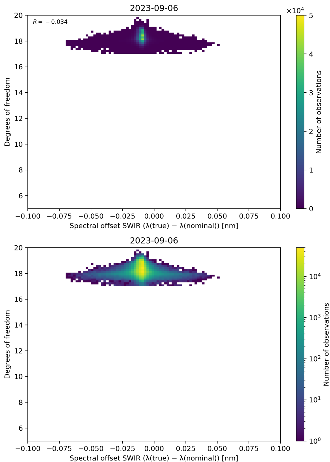
Figure 119: Scatter density plot of “Spectral offset SWIR ( \lambda(\text{true}) - \lambda(\text{nominal}) )” against “Degrees of freedom” for 2023-09-05 to 2023-09-07.
