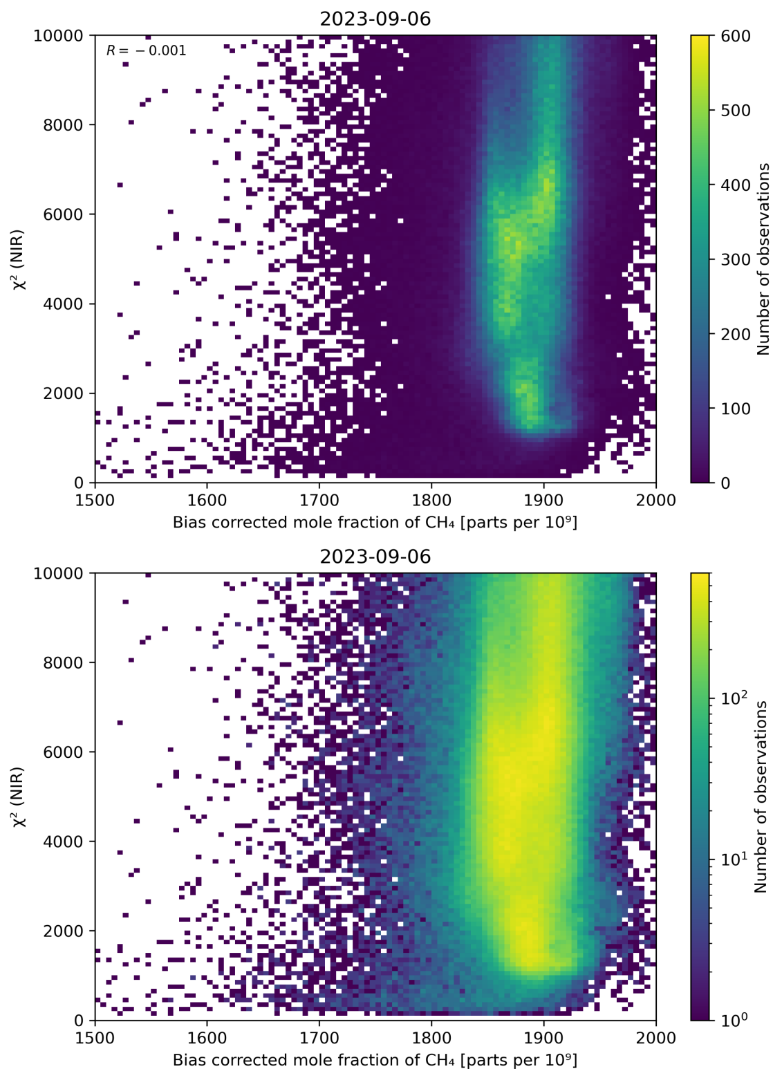
Figure 63: Scatter density plot of “Bias corrected mole fraction of CH 4 ” against “ \chi^2 (NIR)” for 2023-09-05 to 2023-09-07.
