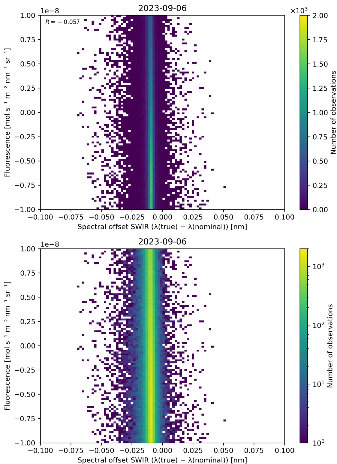
Figure 120: Scatter density plot of “Spectral offset SWIR ( \lambda(\text{true}) - \lambda(\text{nominal}) )” against “Fluorescence” for 2023-09-05 to 2023-09-07.
