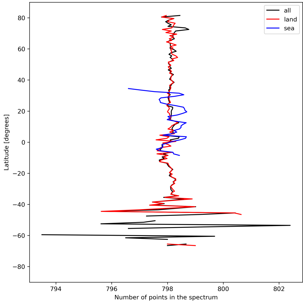
Figure 15: Zonal average of “Number of points in the spectrum” for 2023-09-05 to 2023-09-07.
