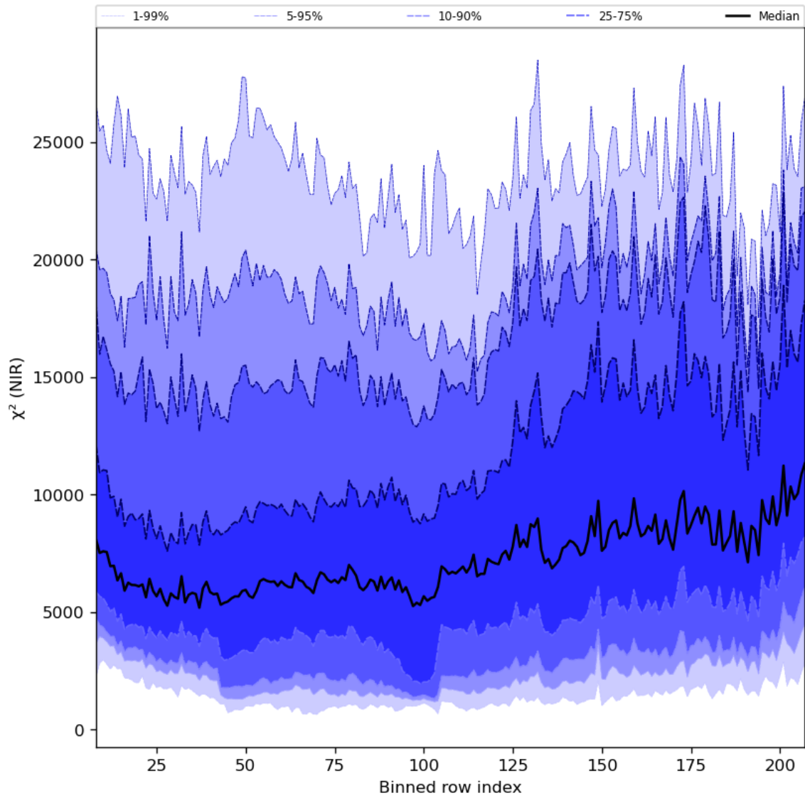
Figure 40: Along track statistics of “ \chi^2 (NIR)” for 2023-09-05 to 2023-09-07
