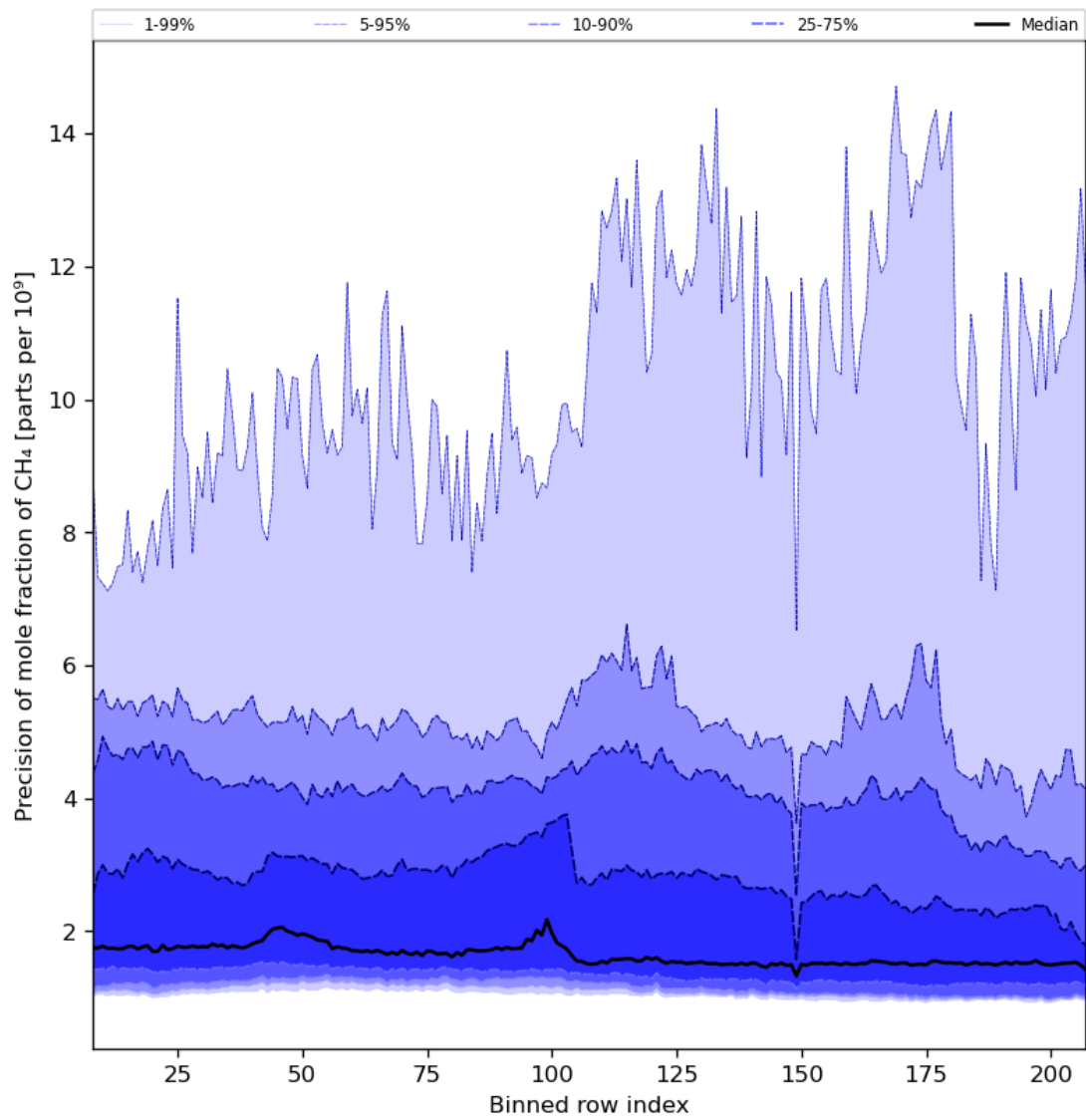
Figure 35: Along track statistics of “Precision of mole fraction of CH 4 ” for 2023-09-05 to 2023-09-07
