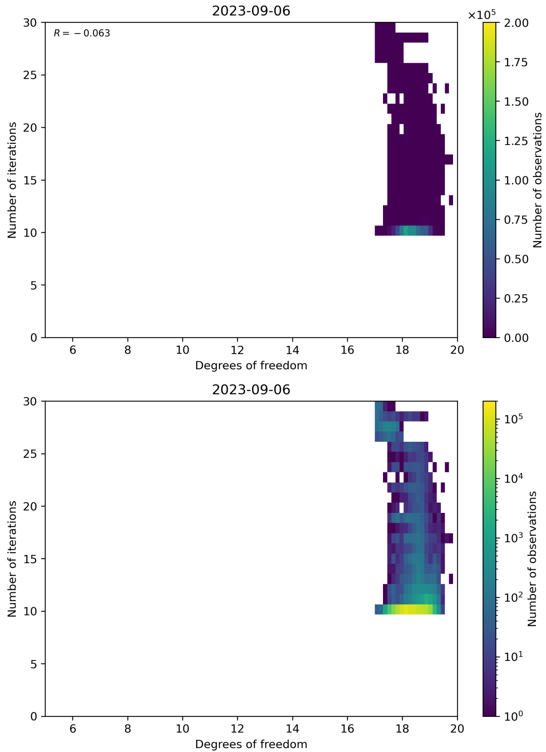
Figure 52: Scatter density plot of “Degrees of freedom” against “Number of iterations” for 2023-09-05 to 2023-09-07.
