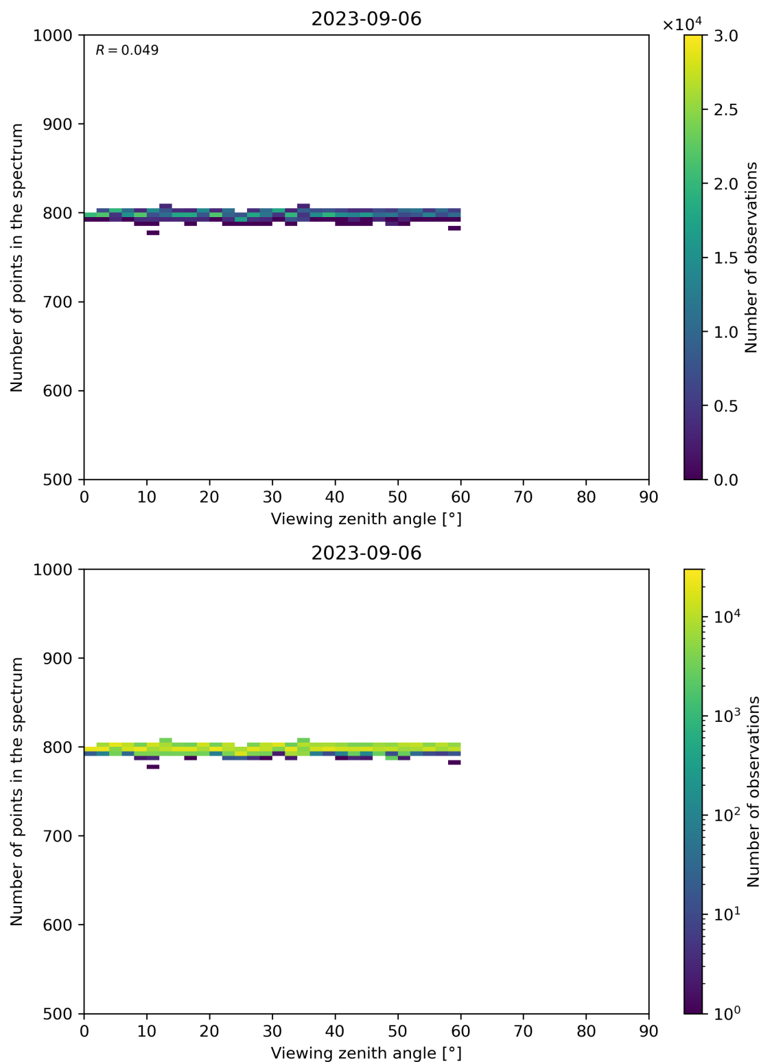
Figure 114: Scatter density plot of “Viewing zenith angle” against “Number of points in the spectrum” for 2023-09-05 to 2023-09-07.
