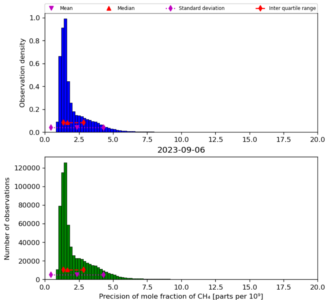
Figure 24: Histogram of “Precision of mole fraction of CH 4 ” for 2023-09-05 to 2023-09-07
