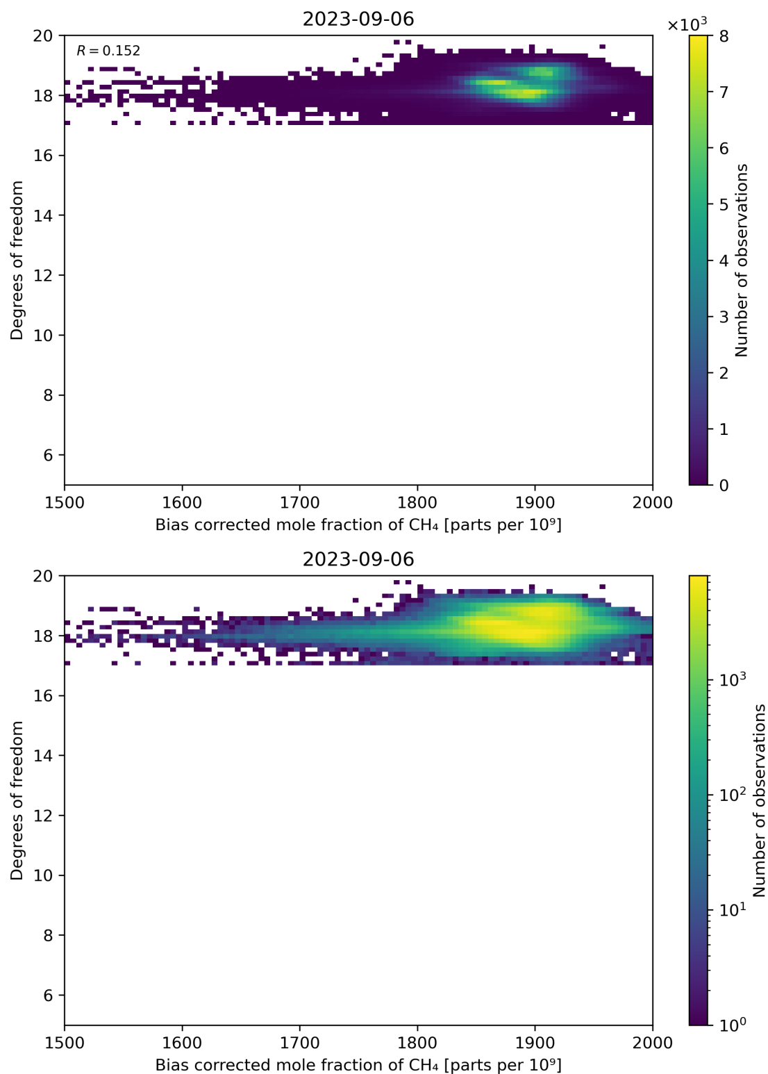
Figure 65: Scatter density plot of “Bias corrected mole fraction of CH 4 ” against “Degrees of freedom” for 2023-09-05 to 2023-09-07.
