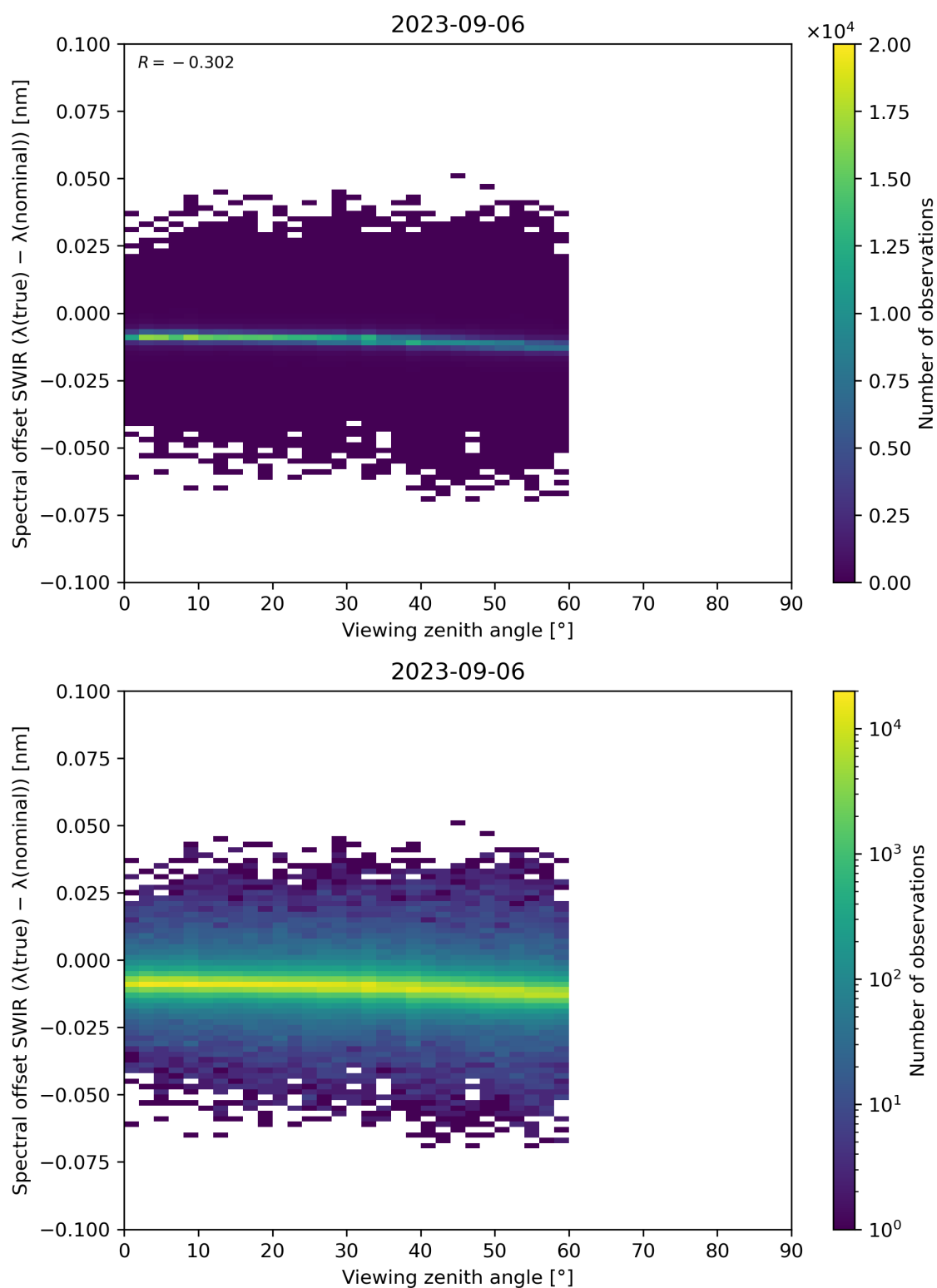
Figure 116: Scatter density plot of “Viewing zenith angle” against “Spectral offset SWIR ( \lambda(\text{true}) - \lambda(\text{nominal}) )” for 2023-09-05 to 2023-09-07.
