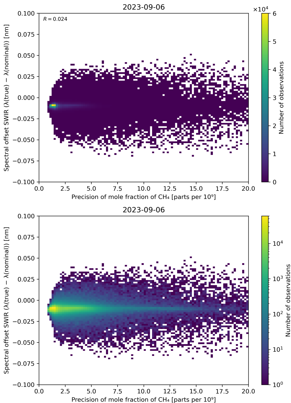
Figure 85: Scatter density plot of “Precision of mole fraction of CH 4 ” against “Spectral offset SWIR ( \lambda(\text{true}) - \lambda(\text{nominal}) )” for 2023-09-05 to 2023-09-07.
