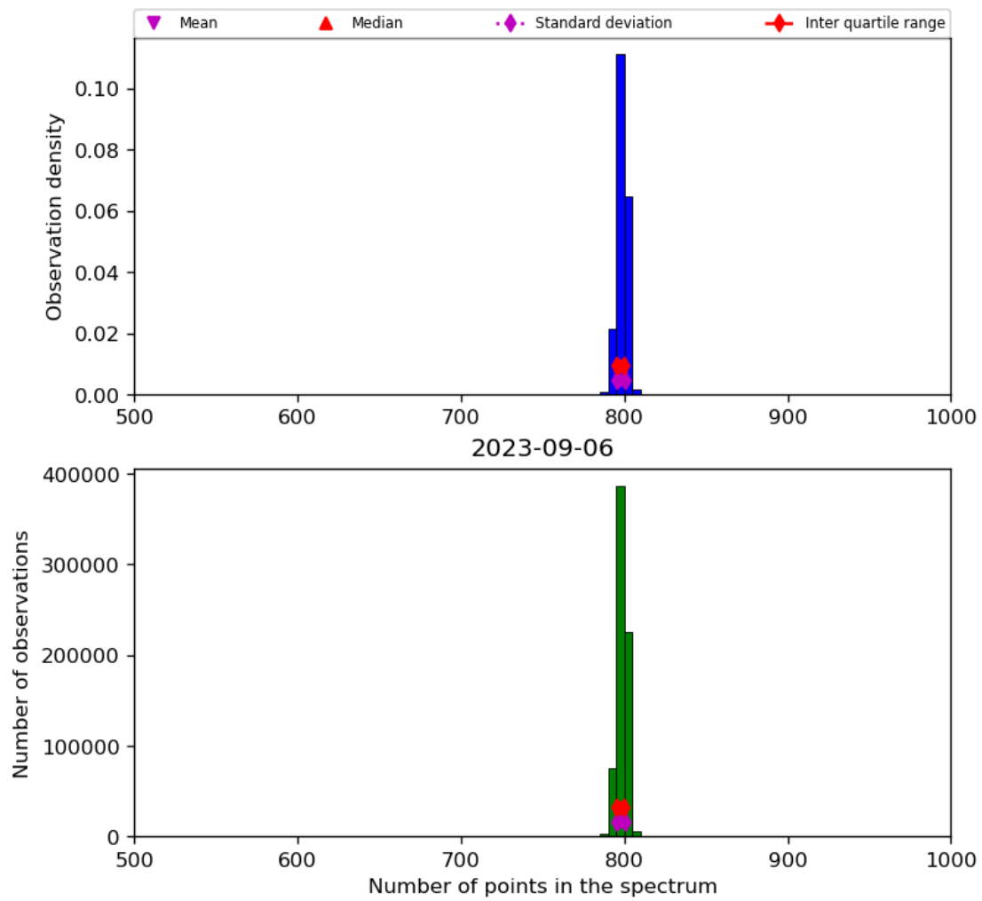
Figure 26: Histogram of “Number of points in the spectrum” for 2023-09-05 to 2023-09-07
