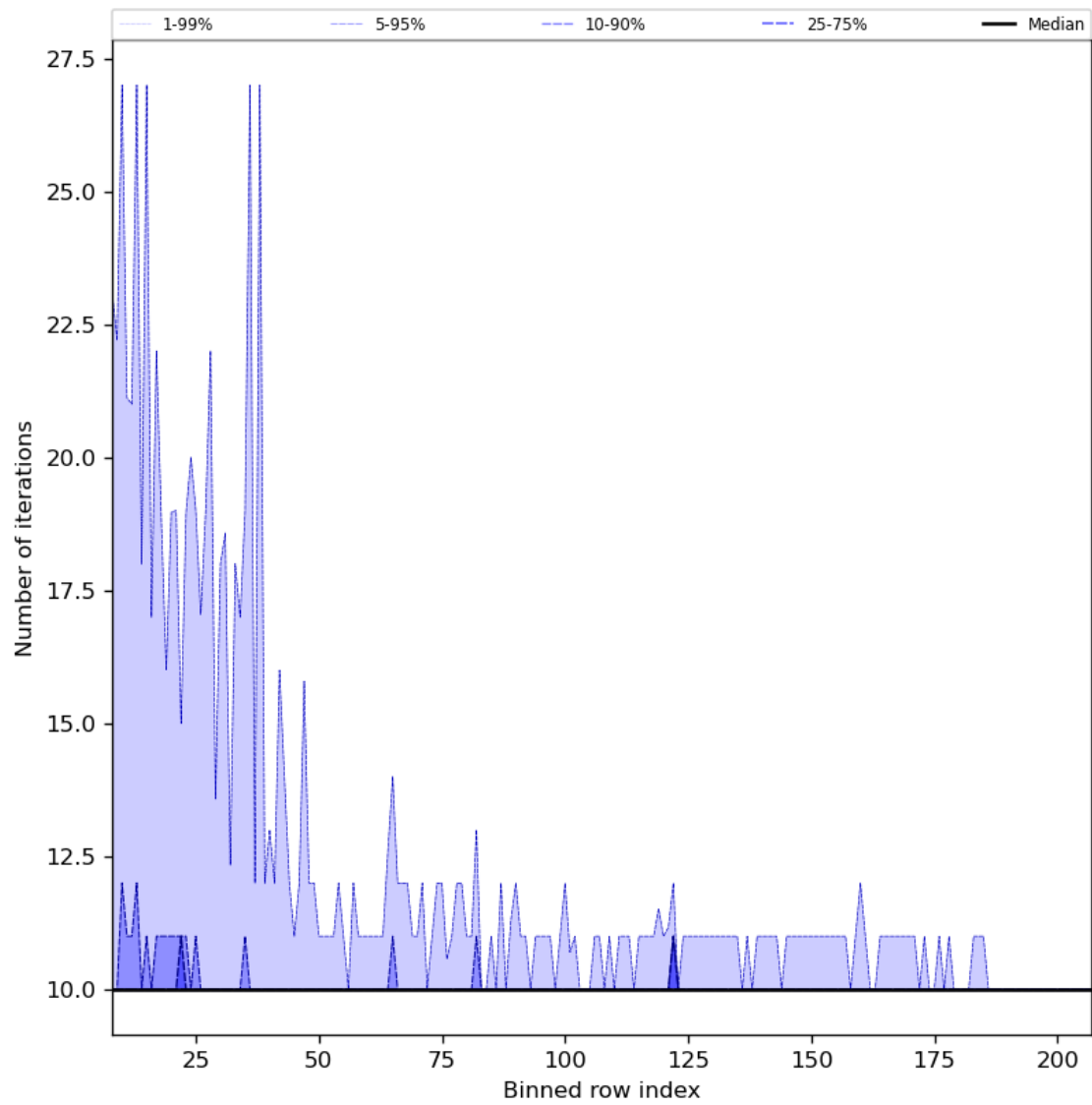
Figure 42: Along track statistics of “Number of iterations” for 2023-09-05 to 2023-09-07
