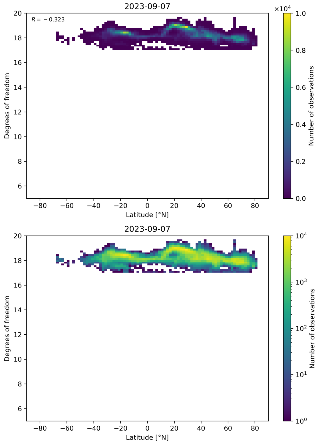
Figure 55: Scatter density plot of “Latitude” against “Degrees of freedom” for 2023-09-06 to 2023-09-08.
