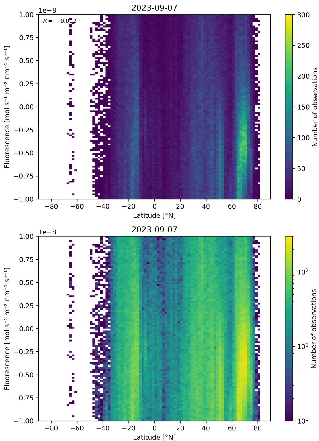
Figure 56: Scatter density plot of “Latitude” against “Fluorescence” for 2023-09-06 to 2023-09-08.
