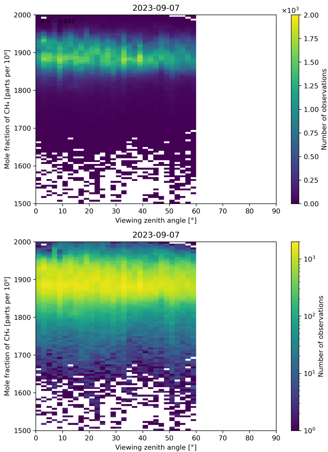
Figure 110: Scatter density plot of “Viewing zenith angle” against “Mole fraction of CH 4 ” for 2023-09-06 to 2023-09-08.
