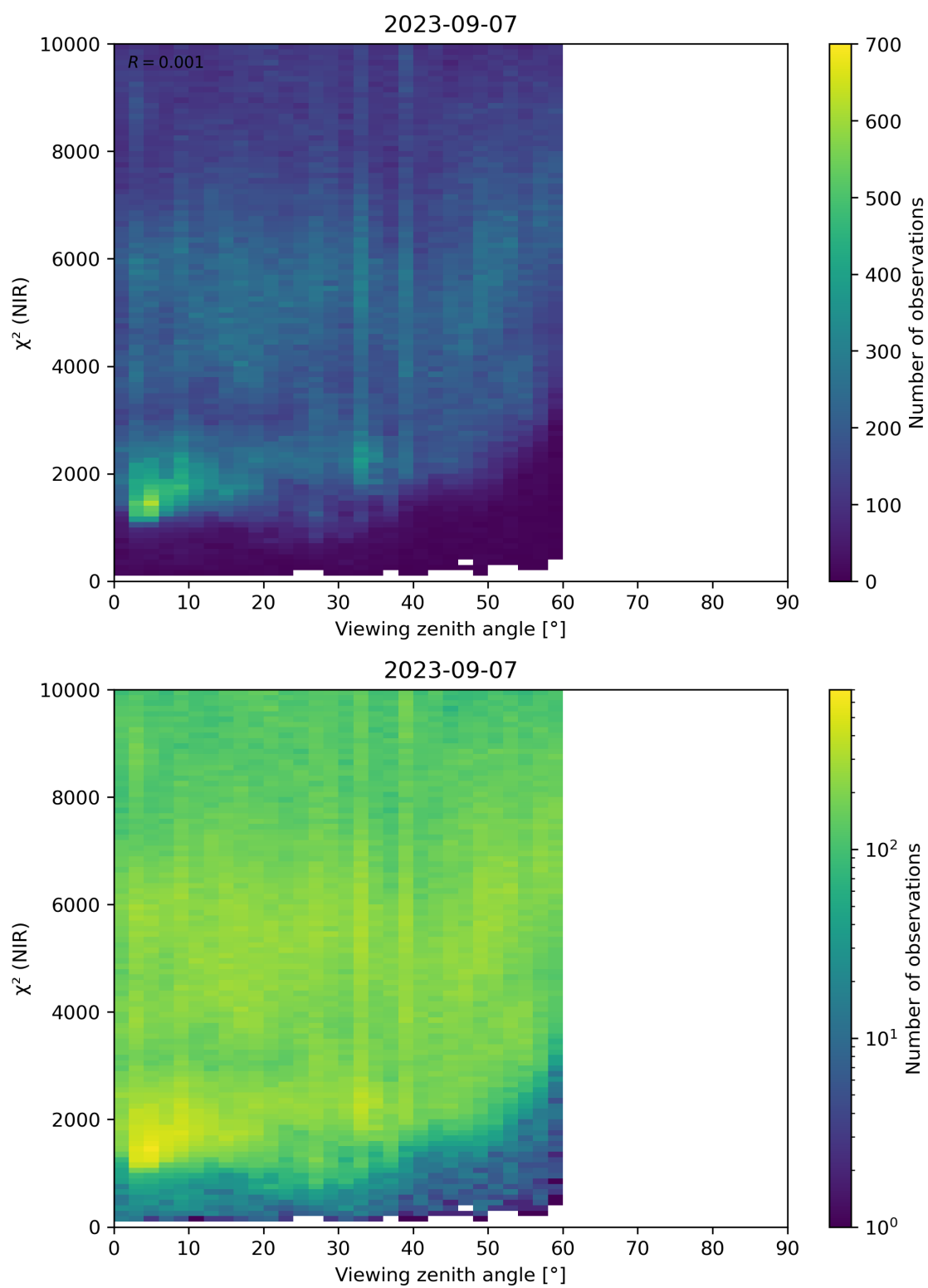
Figure 105: Scatter density plot of “Viewing zenith angle” against “ \chi^2 (NIR)” for 2023-09-06 to 2023-09-08.
