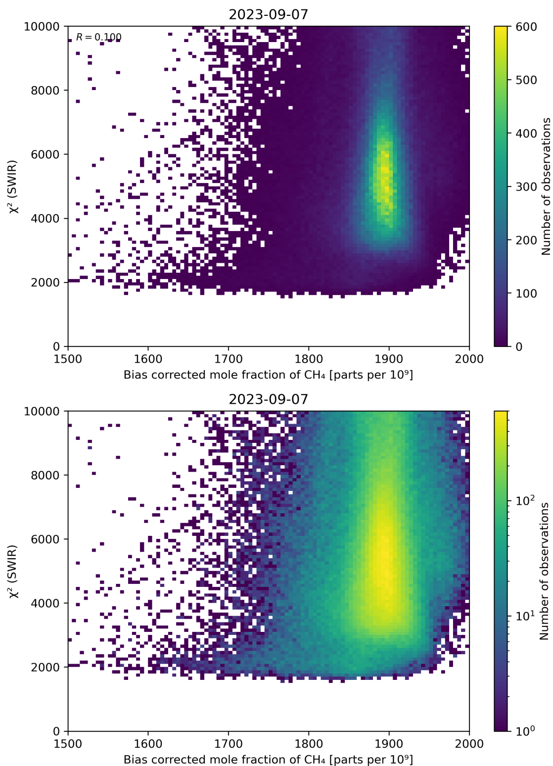
Figure 64: Scatter density plot of “Bias corrected mole fraction of CH 4 ” against “ \chi^2 (SWIR)” for 2023-09-06 to 2023-09-08.
