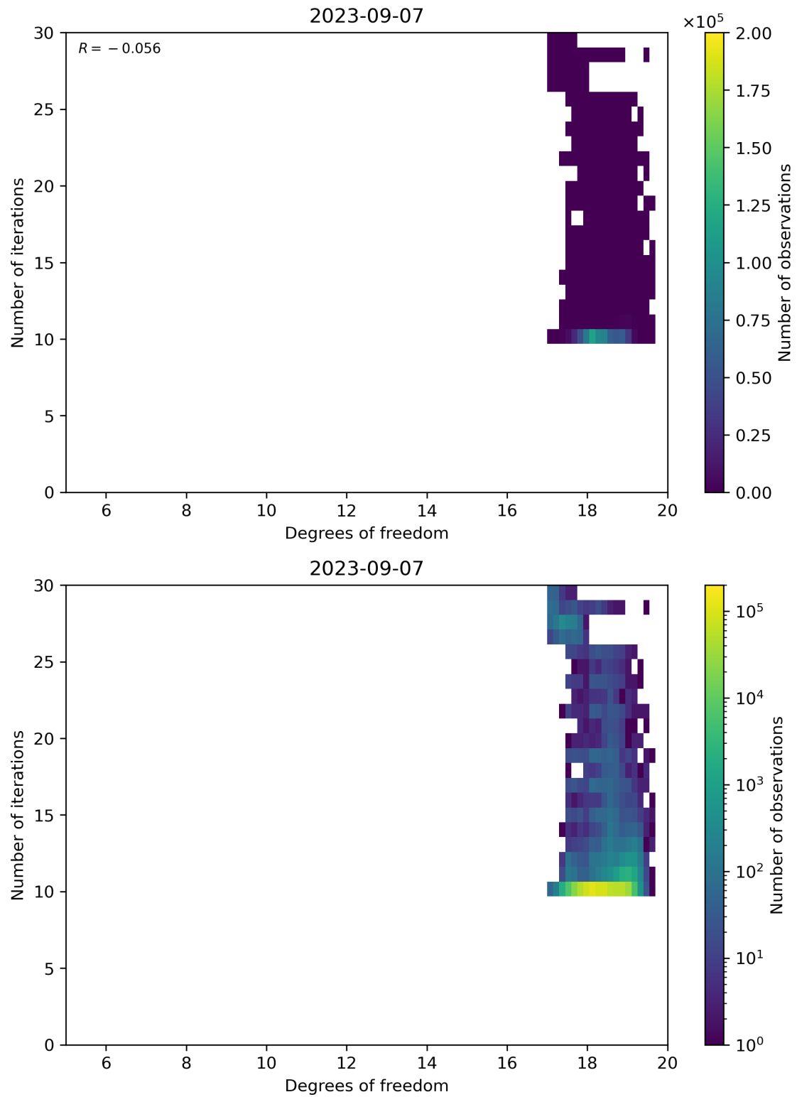
Figure 52: Scatter density plot of “Degrees of freedom” against “Number of iterations” for 2023-09-06 to 2023-09-08.
