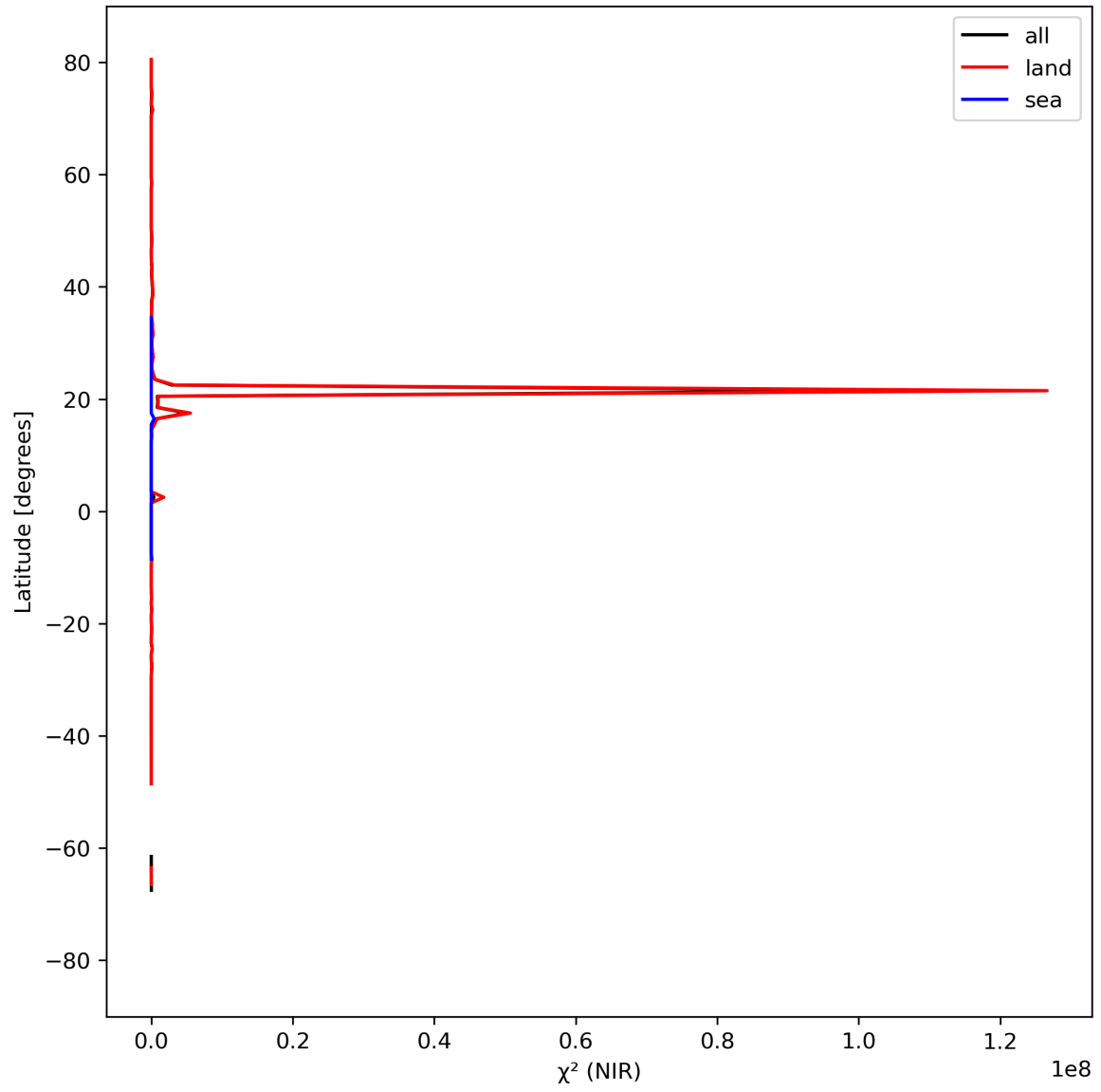
Figure 18: Zonal average of “ \chi^2 (NIR)” for 2023-09-06 to 2023-09-08.
