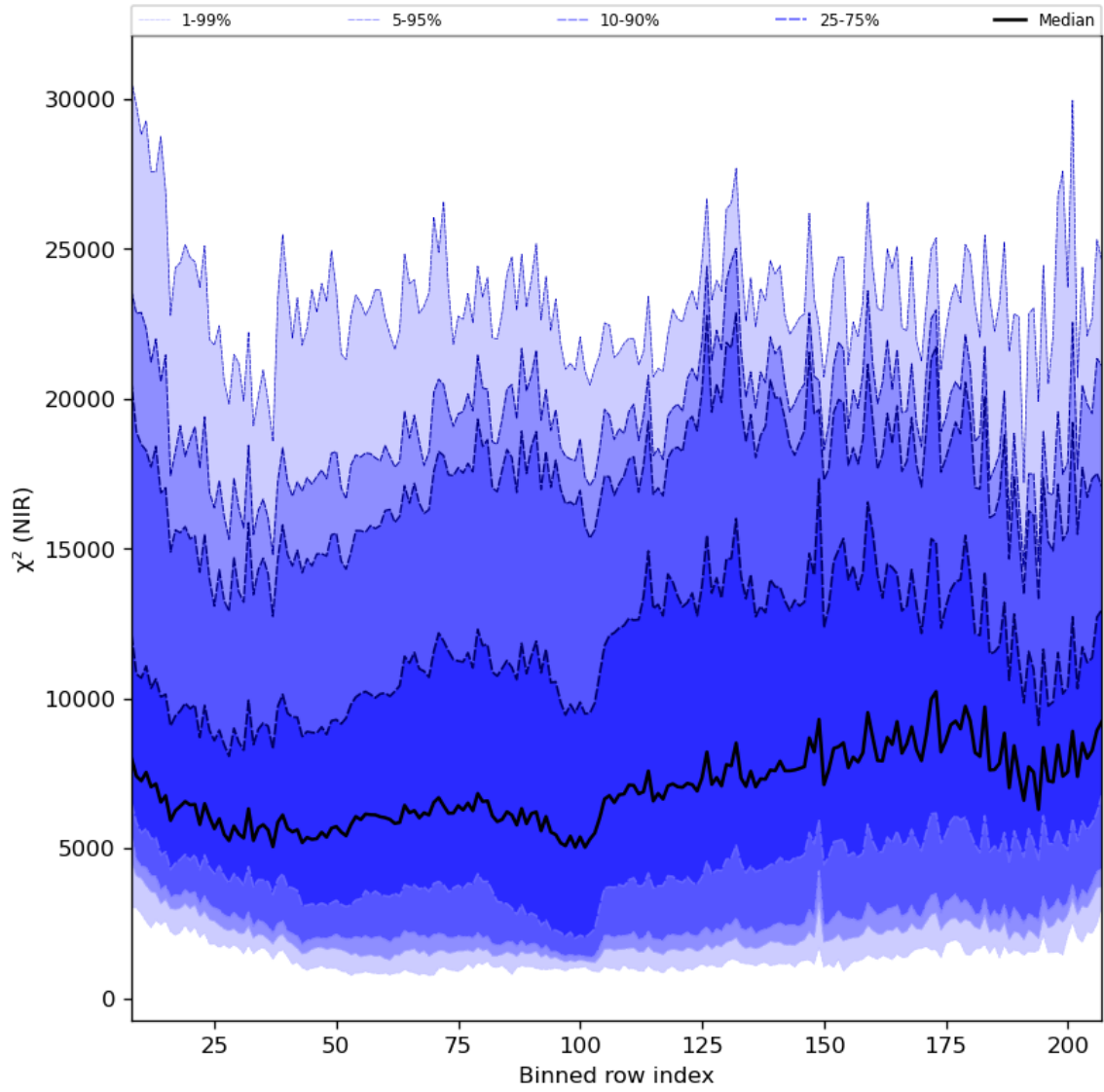
Figure 40: Along track statistics of " \chi^2 (NIR)" for 2023-09-06 to 2023-09-08
