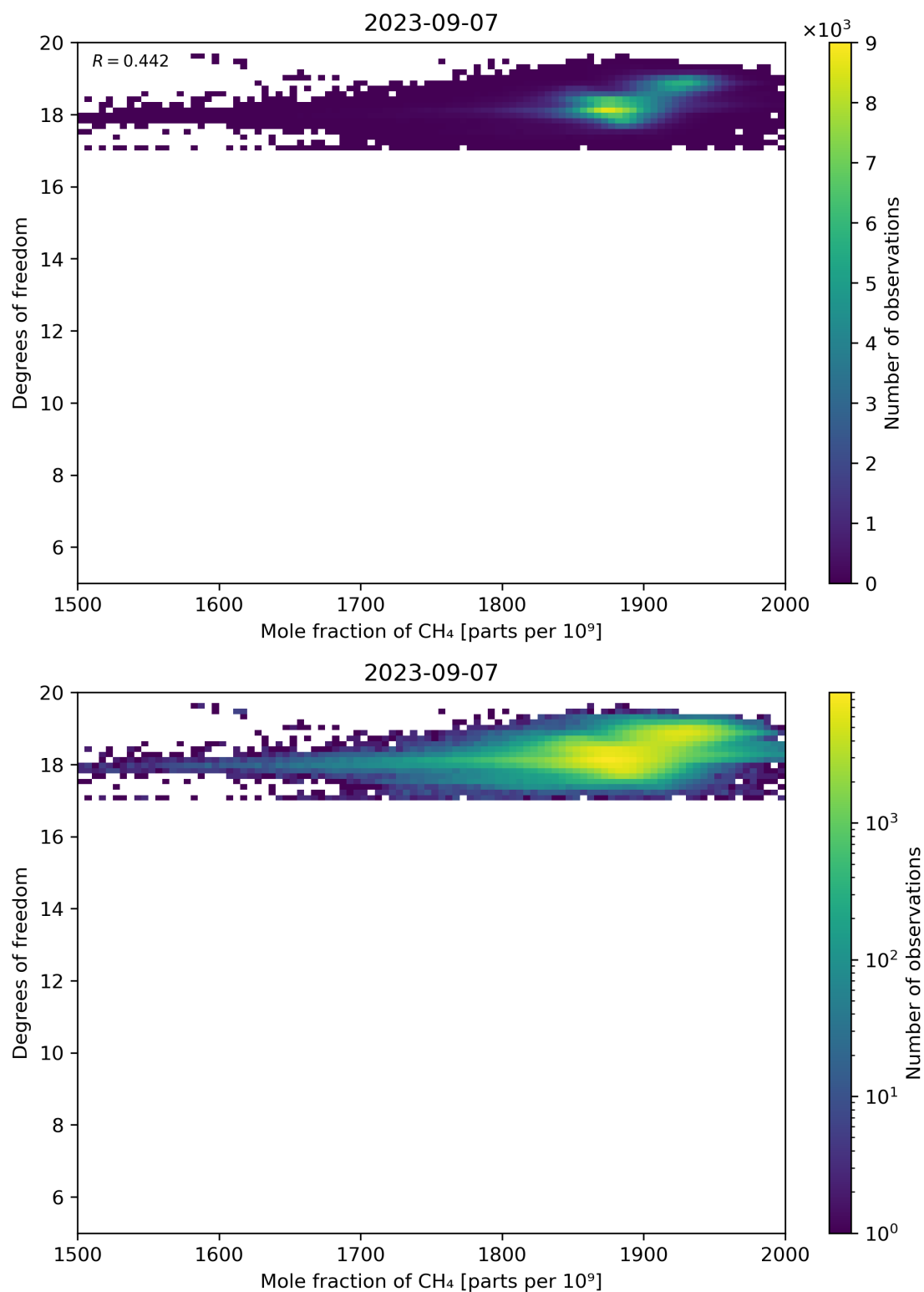
Figure 72: Scatter density plot of “Mole fraction of CH 4 ” against “Degrees of freedom” for 2023-09-06 to 2023-09-08.
