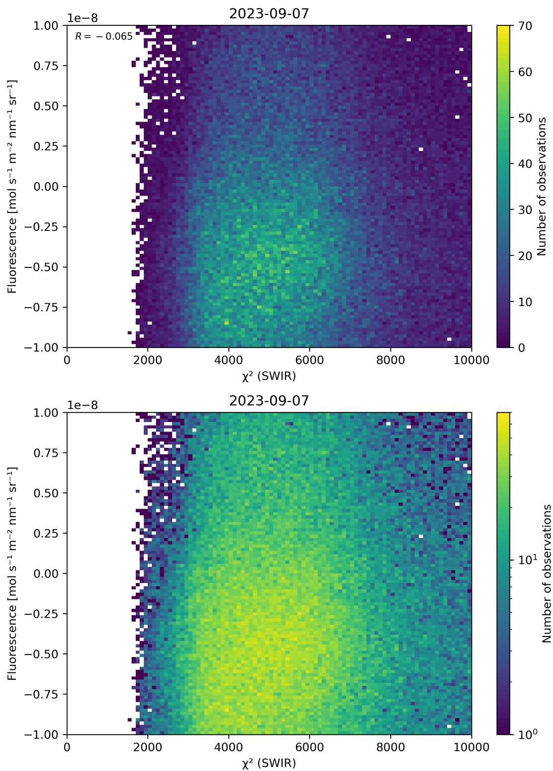
Figure 49: Scatter density plot of “ \chi^2 (SWIR)” against “Fluorescence” for 2023-09-06 to 2023-09-08.
