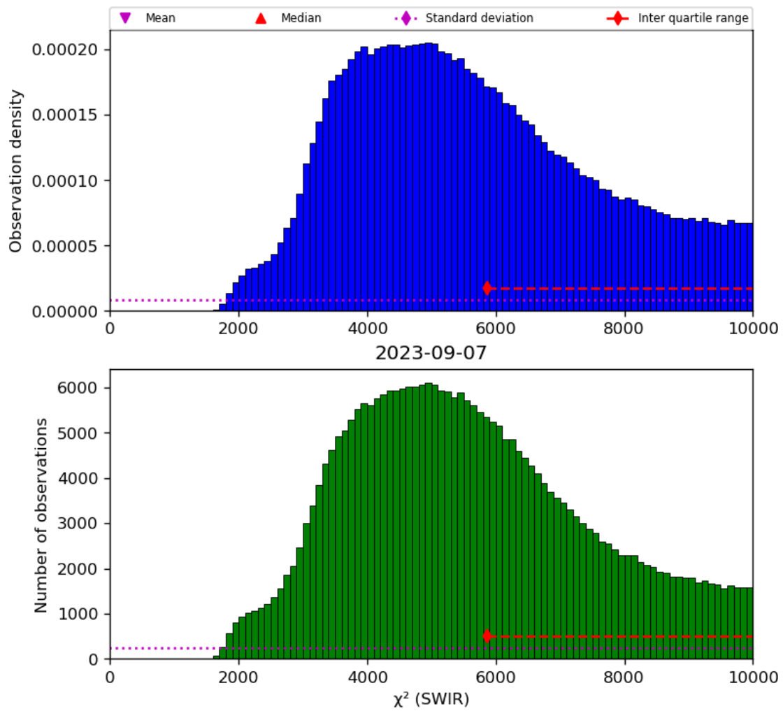
Figure 28: Histogram of “ \chi^2 (SWIR)” for 2023-09-06 to 2023-09-08
