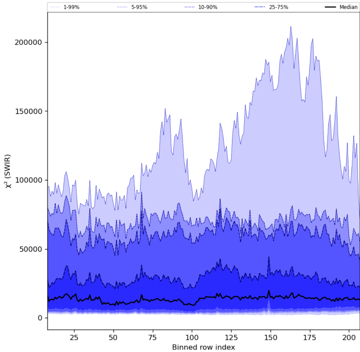
Figure 39: Along track statistics of “ \chi^2 (SWIR)” for 2023-09-06 to 2023-09-08
