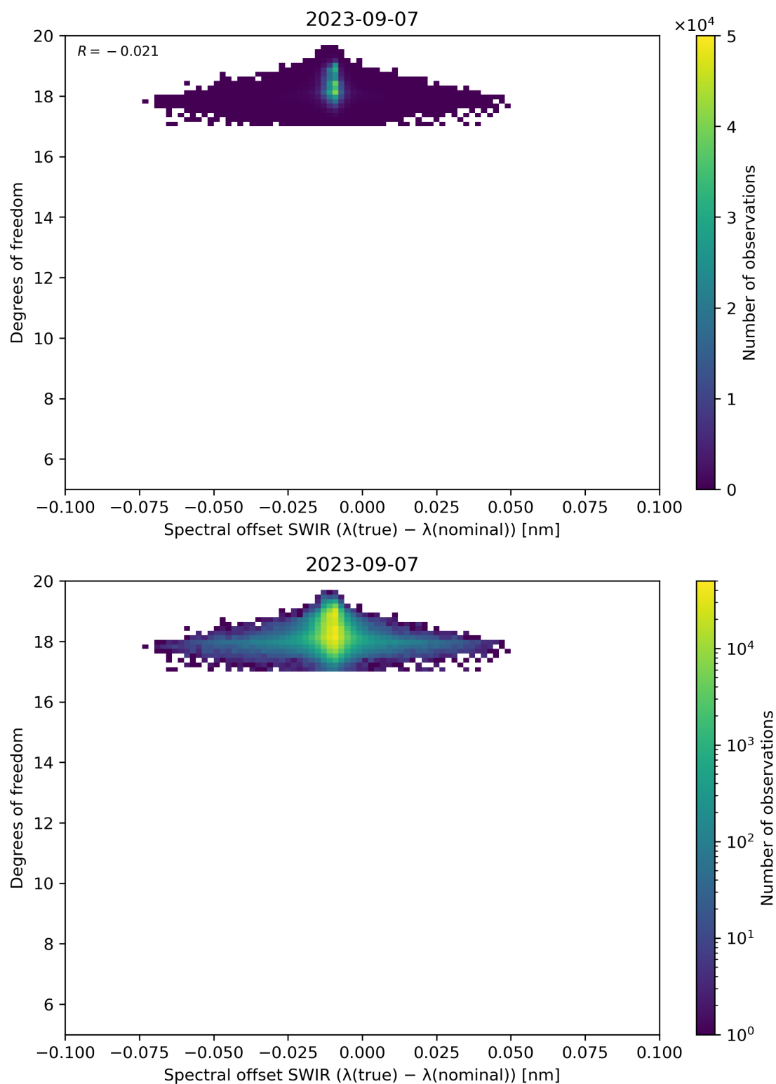
Figure 119: Scatter density plot of “Spectral offset SWIR ( \lambda(\text{true}) - \lambda(\text{nominal}) )” against “Degrees of freedom” for 2023-09-06 to 2023-09-08.
