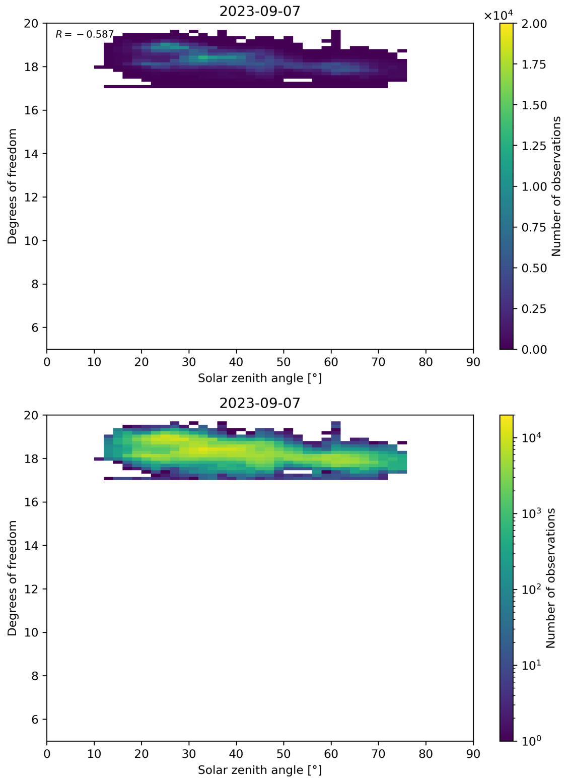
Figure 96: Scatter density plot of “Solar zenith angle” against “Degrees of freedom” for 2023-09-06 to 2023-09-08.
