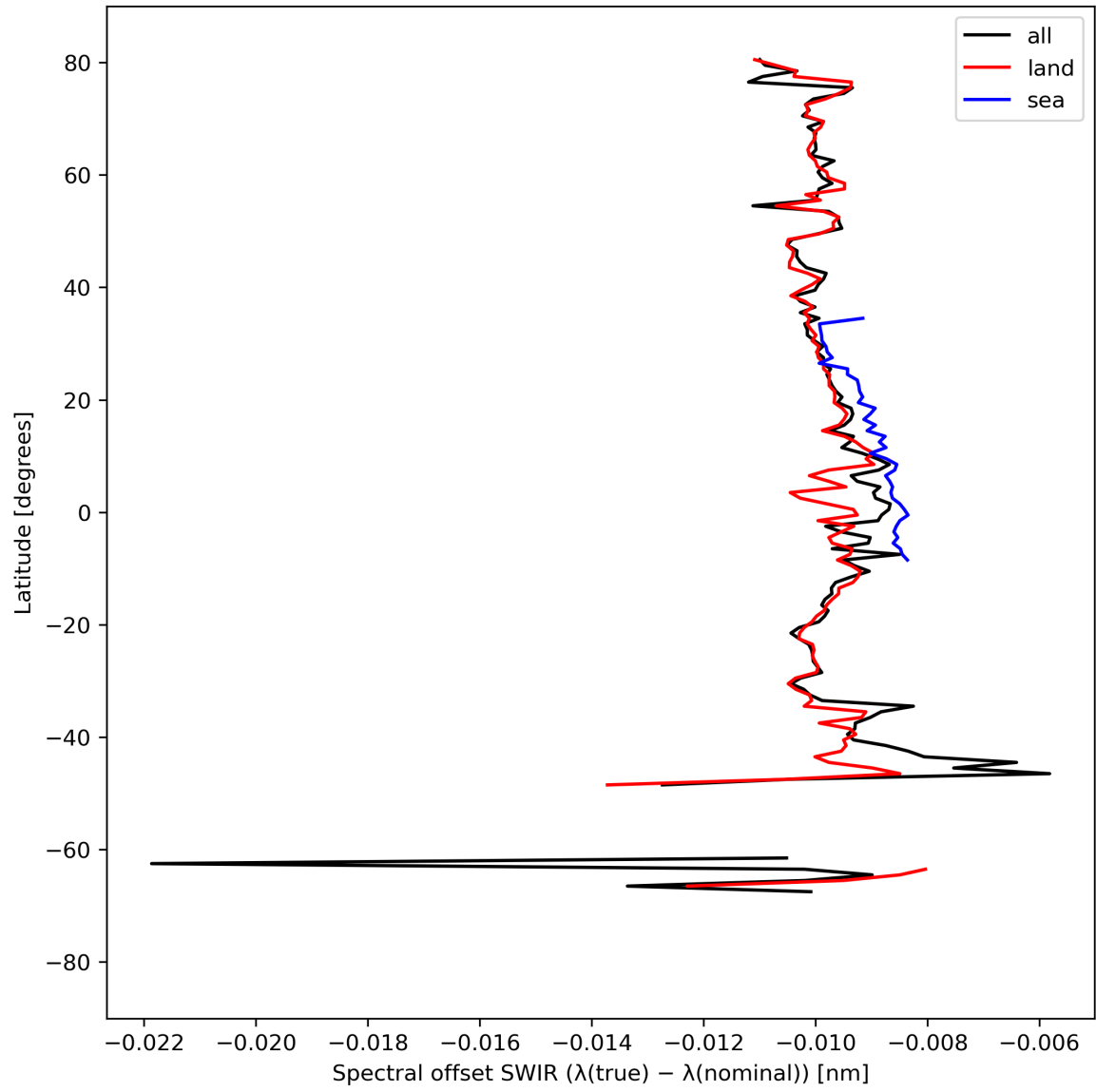
Figure 16: Zonal average of “Spectral offset SWIR ( \lambda(\text{true}) - \lambda(\text{nominal}) )” for 2023-09-06 to 2023-09-08.
