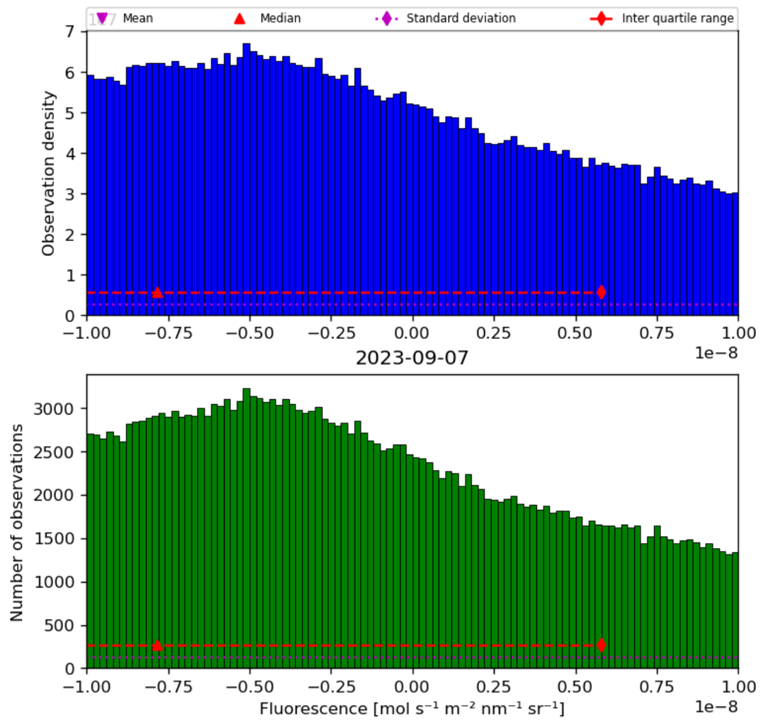
Figure 32: Histogram of “Fluorescence” for 2023-09-06 to 2023-09-08
