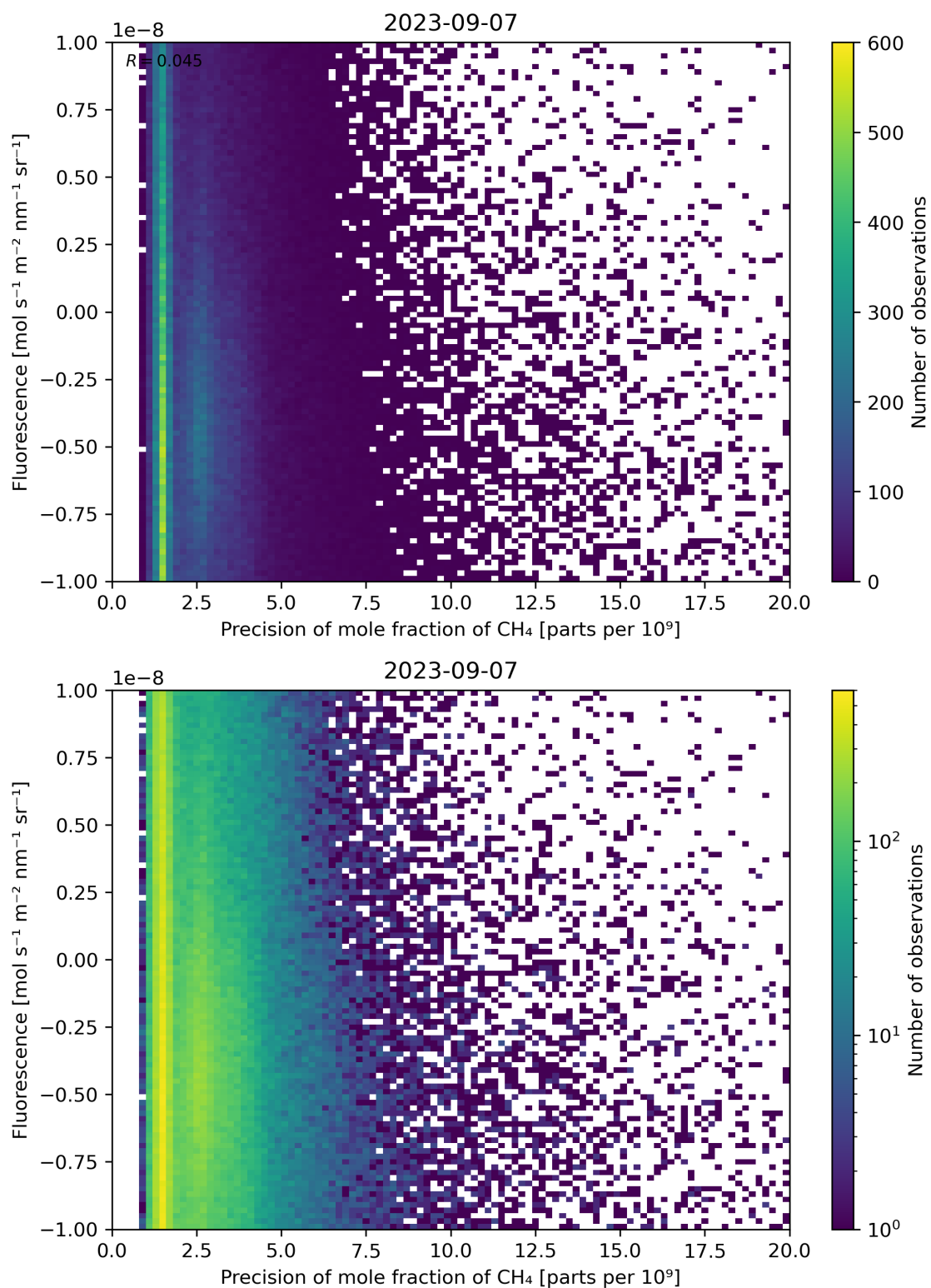
Figure 81: Scatter density plot of “Precision of mole fraction of \text{CH}_4 ” against “Fluorescence” for 2023-09-06 to 2023-09-08.
