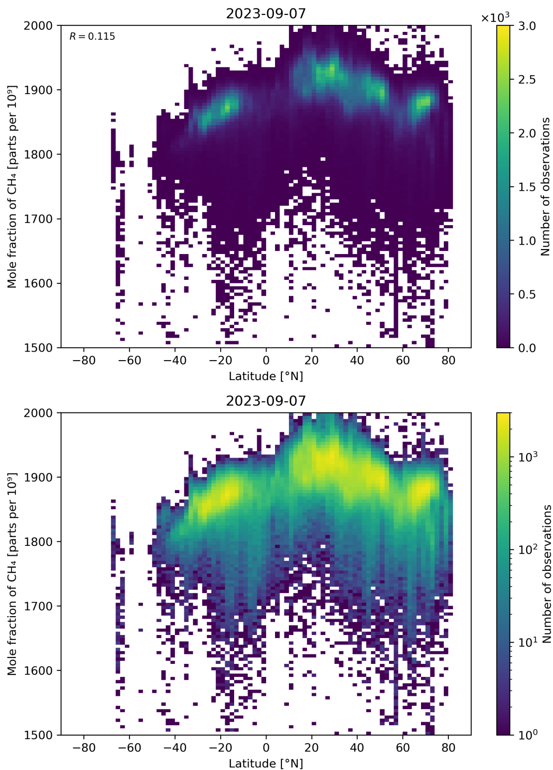
Figure 57: Scatter density plot of “Latitude” against “Mole fraction of CH 4 ” for 2023-09-06 to 2023-09-08.
