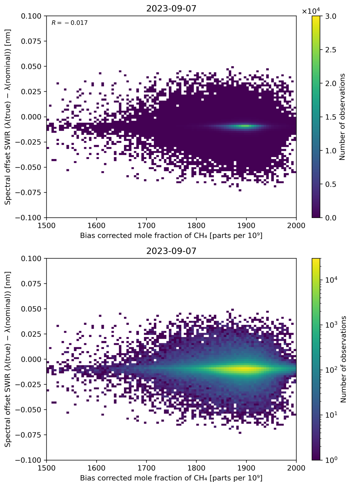
Figure 69: Scatter density plot of “Bias corrected mole fraction of \text{CH}_4 ” against “Spectral offset SWIR ( \lambda(\text{true}) - \lambda(\text{nominal}) )” for 2023-09-06 to 2023-09-08.
