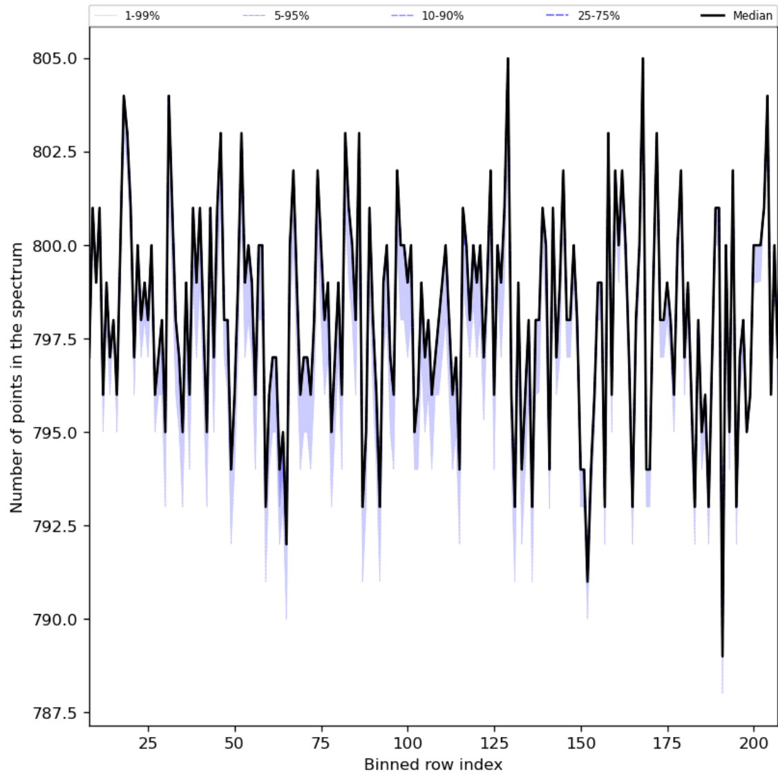
Figure 37: Along track statistics of “Number of points in the spectrum” for 2023-09-06 to 2023-09-08
