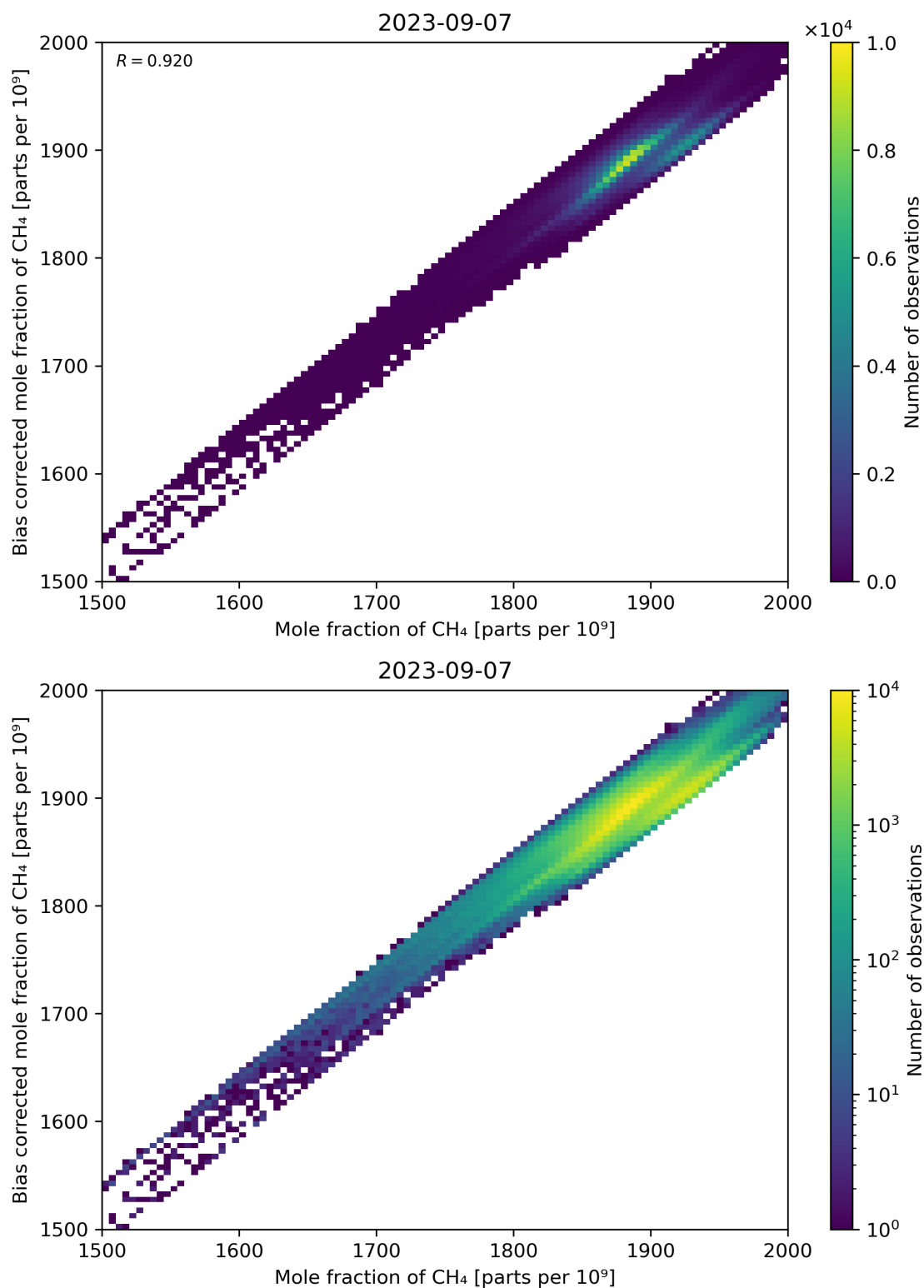
Figure 74: Scatter density plot of “Mole fraction of CH 4 ” against “Bias corrected mole fraction of CH 4 ” for 2023-09-06 to 2023-09-08.
