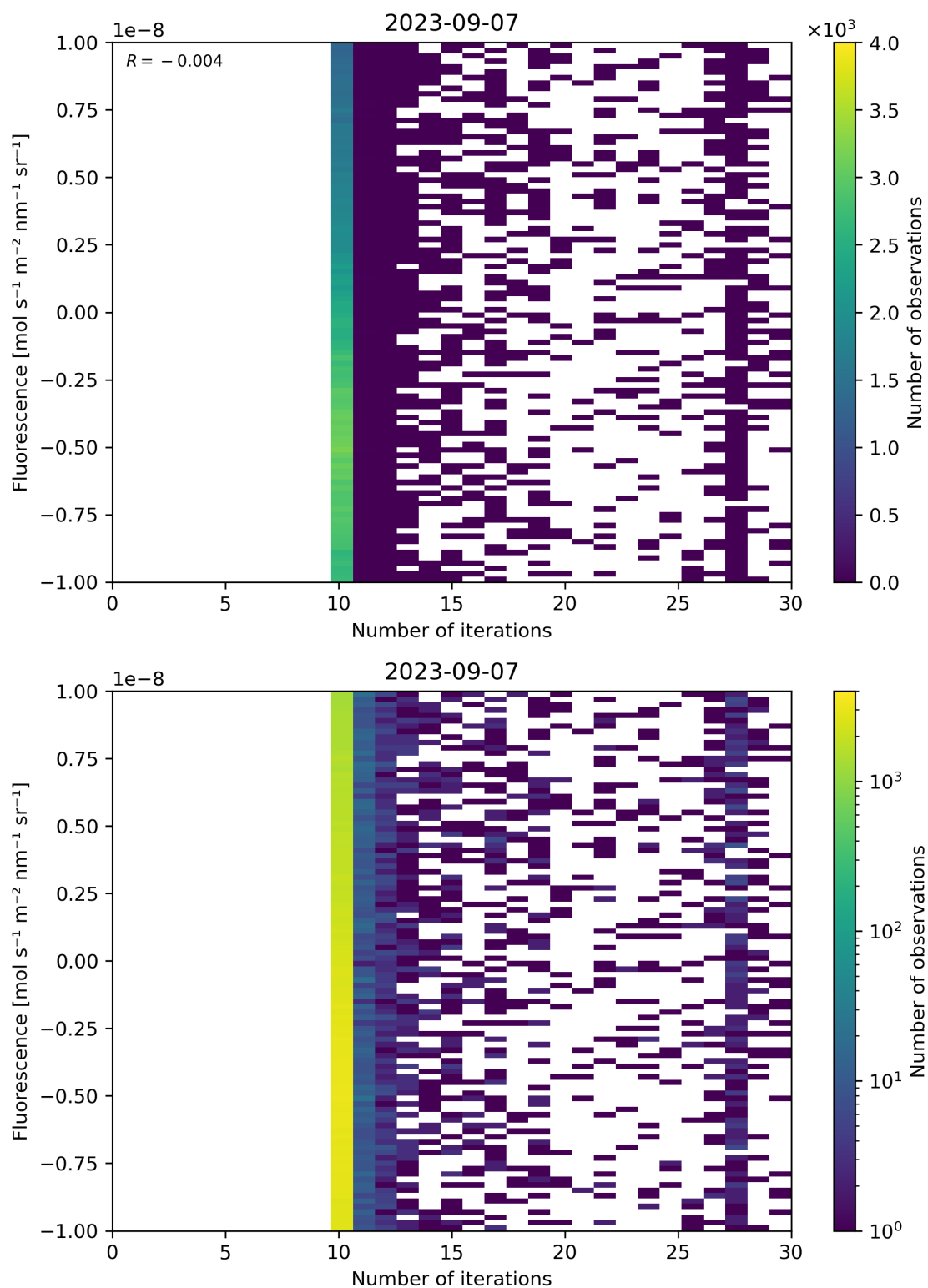
Figure 87: Scatter density plot of “Number of iterations” against “Fluorescence” for 2023-09-06 to 2023-09-08.
