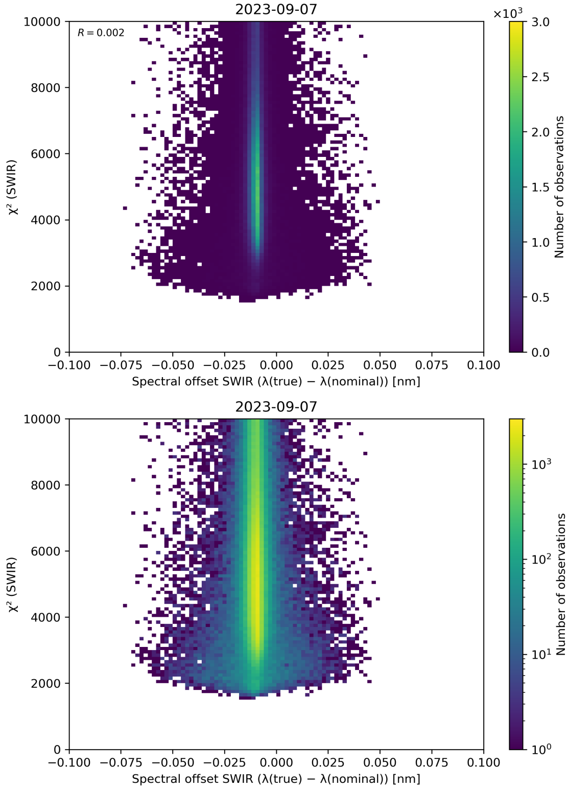
Figure 118: Scatter density plot of “Spectral offset SWIR ( \lambda(\text{true}) - \lambda(\text{nominal}) )” against “ \chi^2 (SWIR)” for 2023-09-06 to 2023-09-08.
