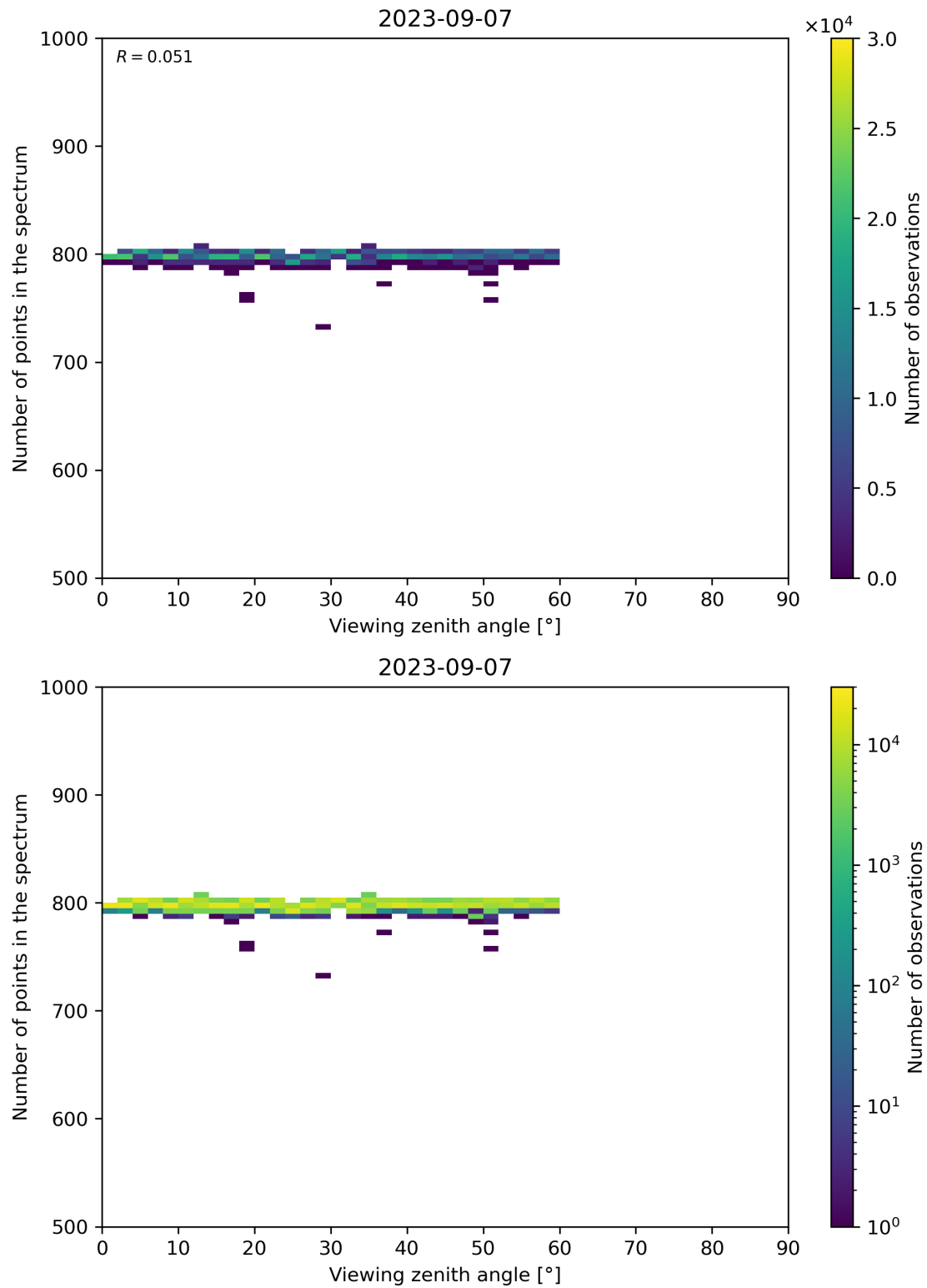
Figure 114: Scatter density plot of “Viewing zenith angle” against “Number of points in the spectrum” for 2023-09-06 to 2023-09-08.
