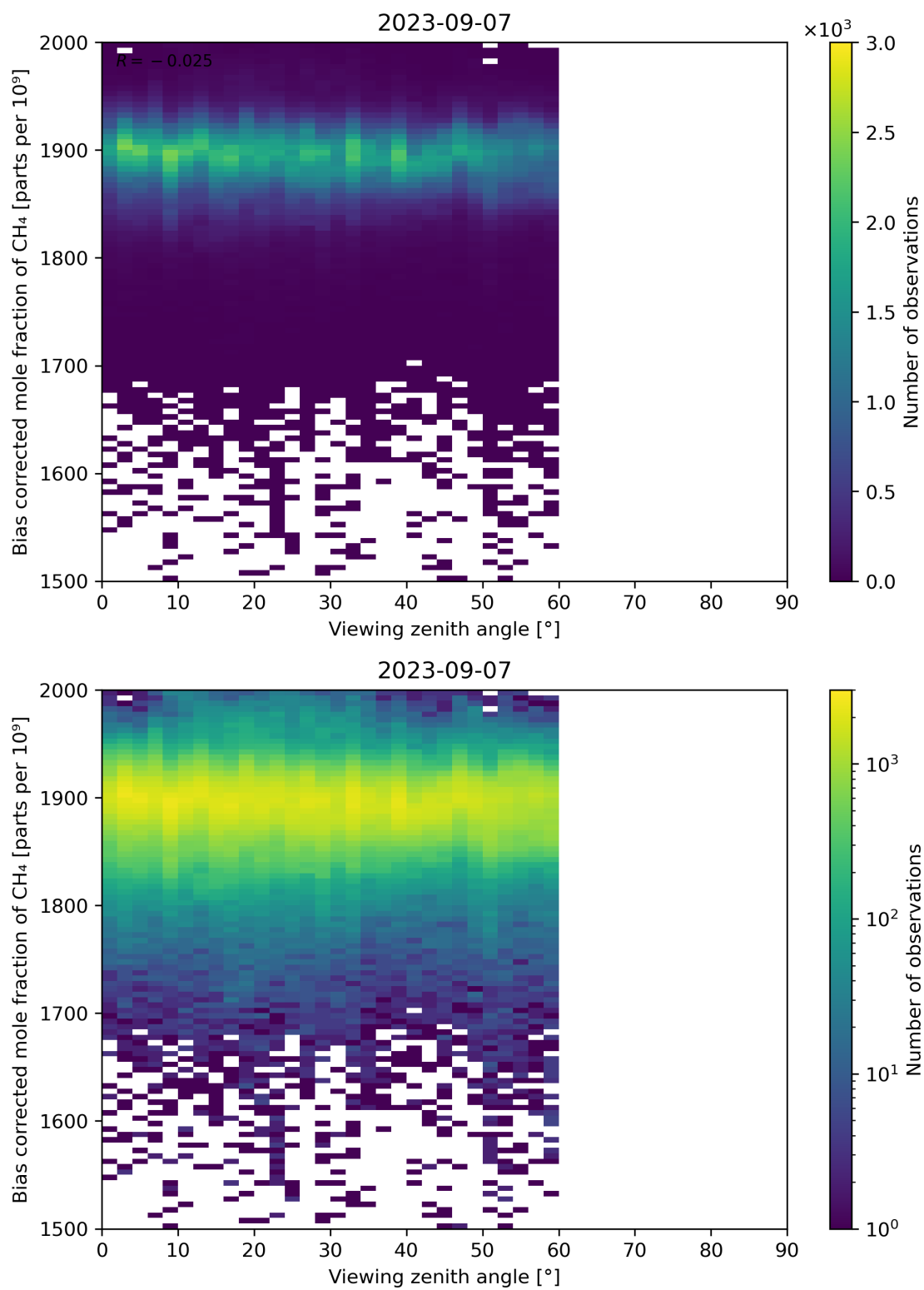
Figure 111: Scatter density plot of “Viewing zenith angle” against “Bias corrected mole fraction of CH 4 ” for 2023-09-06 to 2023-09-08.
