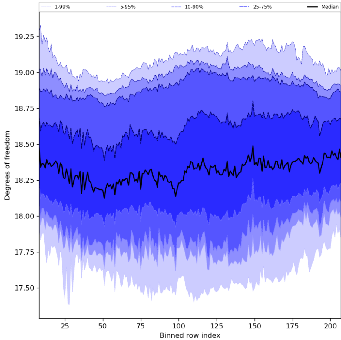
Figure 41: Along track statistics of “Degrees of freedom” for 2023-09-06 to 2023-09-08
