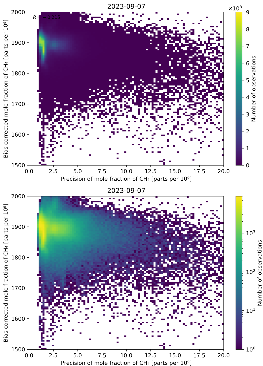
Figure 82: Scatter density plot of “Precision of mole fraction of CH 4 ” against “Bias corrected mole fraction of CH 4 ” for 2023-09-06 to 2023-09-08.
