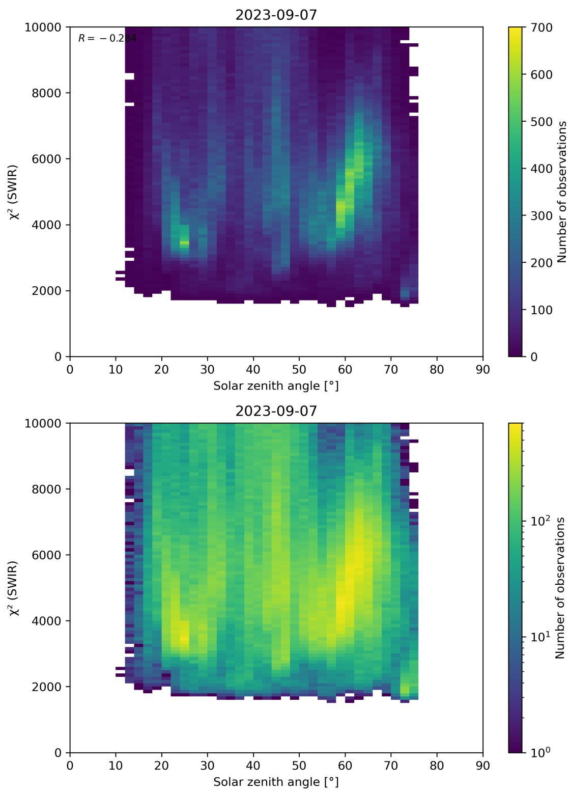
Figure 95: Scatter density plot of “Solar zenith angle” against “ \chi^2 (SWIR)” for 2023-09-06 to 2023-09-08.
