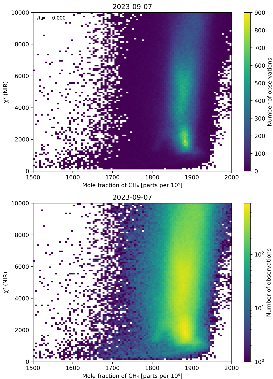
Figure 70: Scatter density plot of “Mole fraction of CH 4 ” against “ \chi^2 (NIR)” for 2023-09-06 to 2023-09-08.
