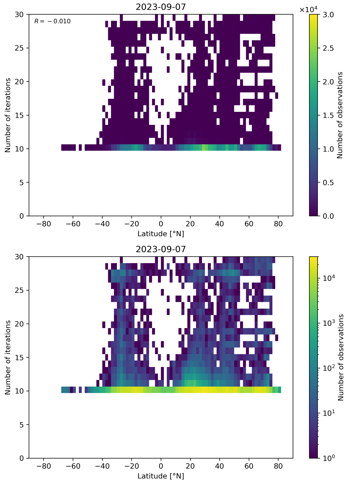
Figure 60: Scatter density plot of “Latitude” against “Number of iterations” for 2023-09-06 to 2023-09-08.
