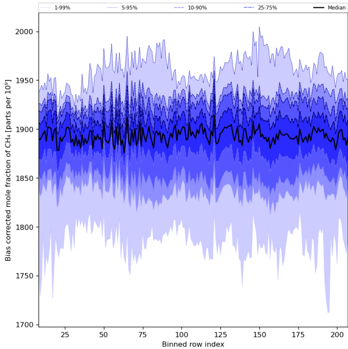
Figure 36: Along track statistics of “Bias corrected mole fraction of CH 4 ” for 2023-09-06 to 2023-09-08
