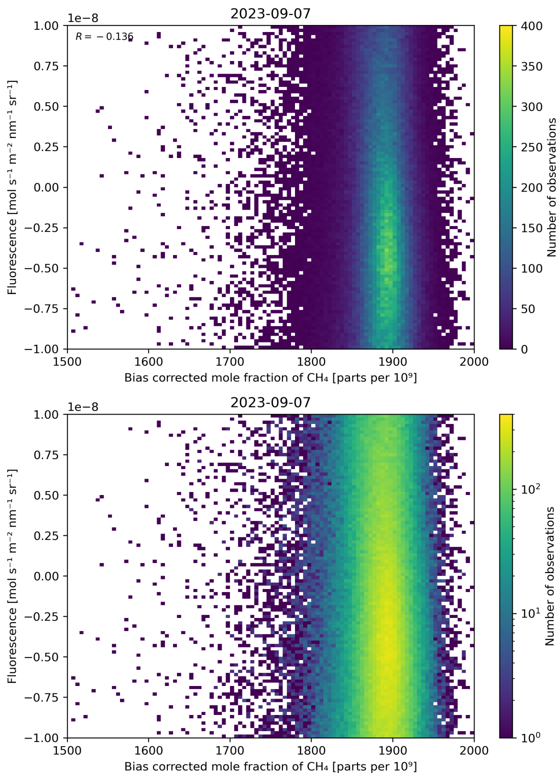
Figure 66: Scatter density plot of “Bias corrected mole fraction of \text{CH}_4 ” against “Fluorescence” for 2023-09-06 to 2023-09-08.
