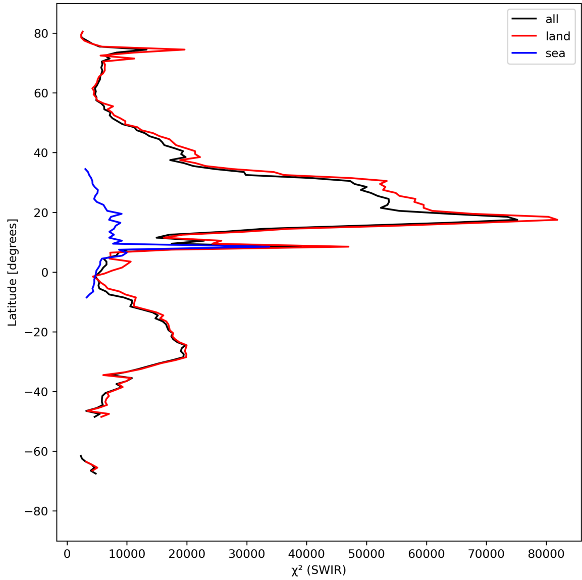
Figure 17: Zonal average of “ \chi^2 (SWIR)” for 2023-09-06 to 2023-09-08.
