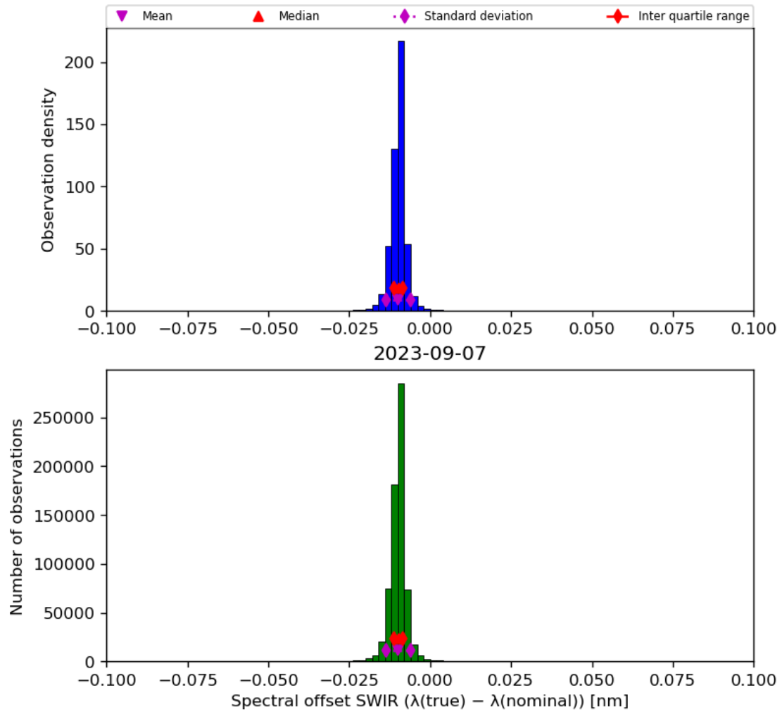
Figure 27: Histogram of “Spectral offset SWIR ( \lambda(\text{true}) - \lambda(\text{nominal}) )” for 2023-09-06 to 2023-09-08
