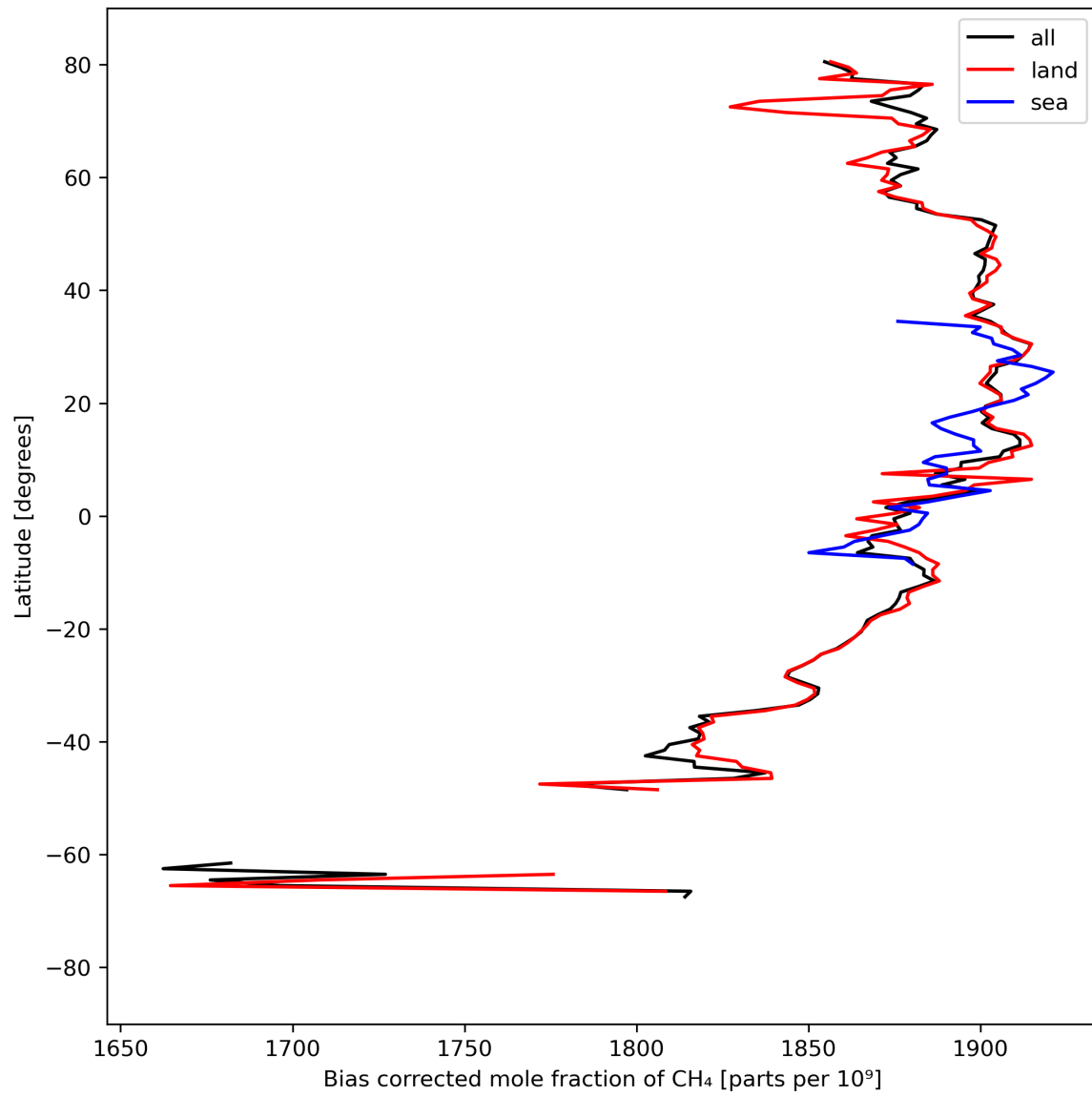
Figure 14: Zonal average of “Bias corrected mole fraction of CH 4 ” for 2023-09-06 to 2023-09-08.
