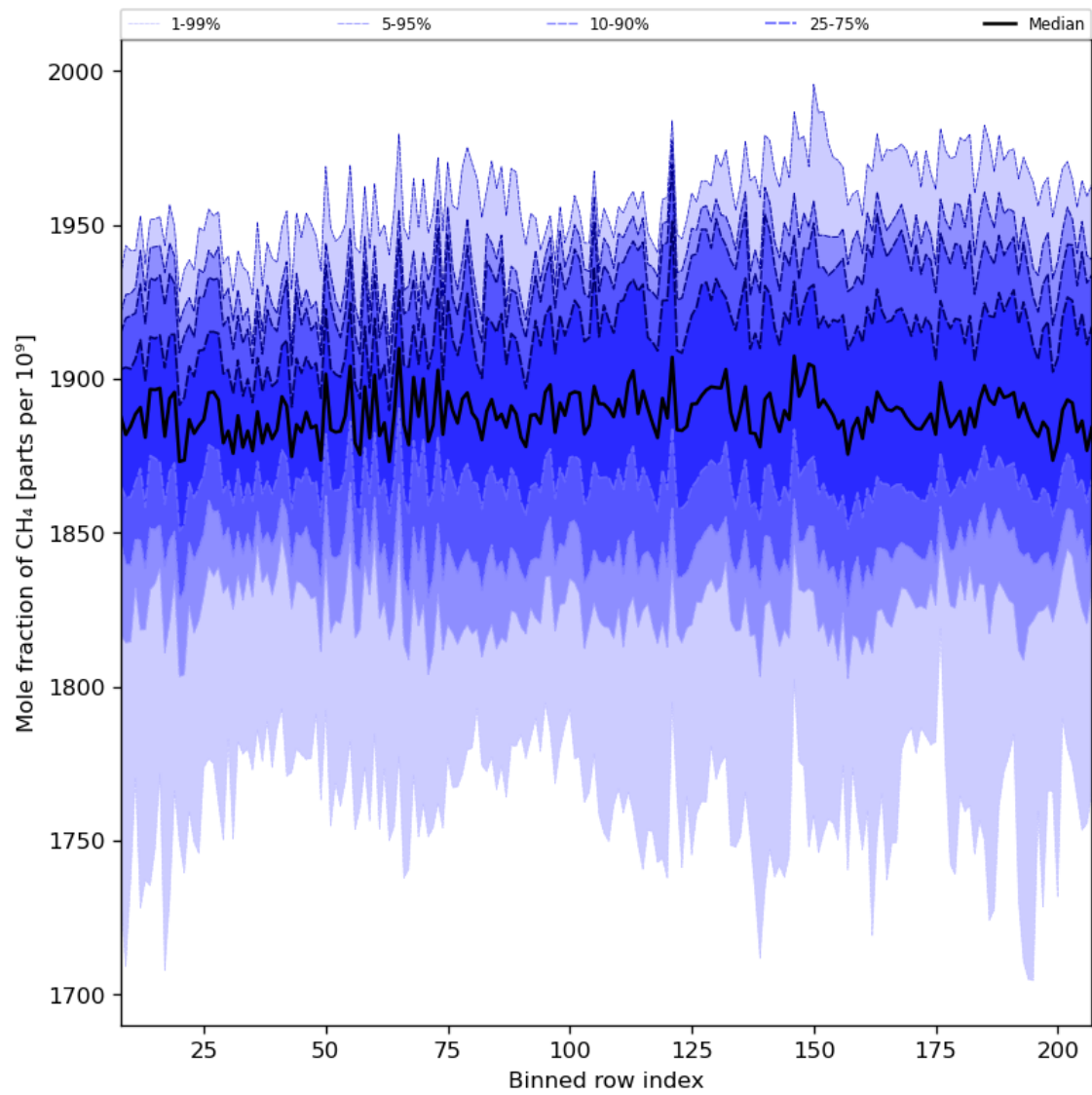
Figure 34: Along track statistics of “Mole fraction of CH 4 ” for 2023-09-06 to 2023-09-08
