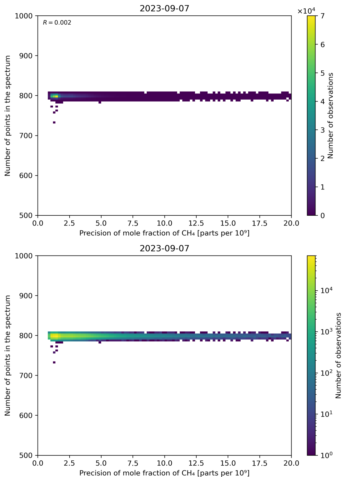
Figure 84: Scatter density plot of “Precision of mole fraction of CH 4 ” against “Number of points in the spectrum” for 2023-09-06 to 2023-09-08.
