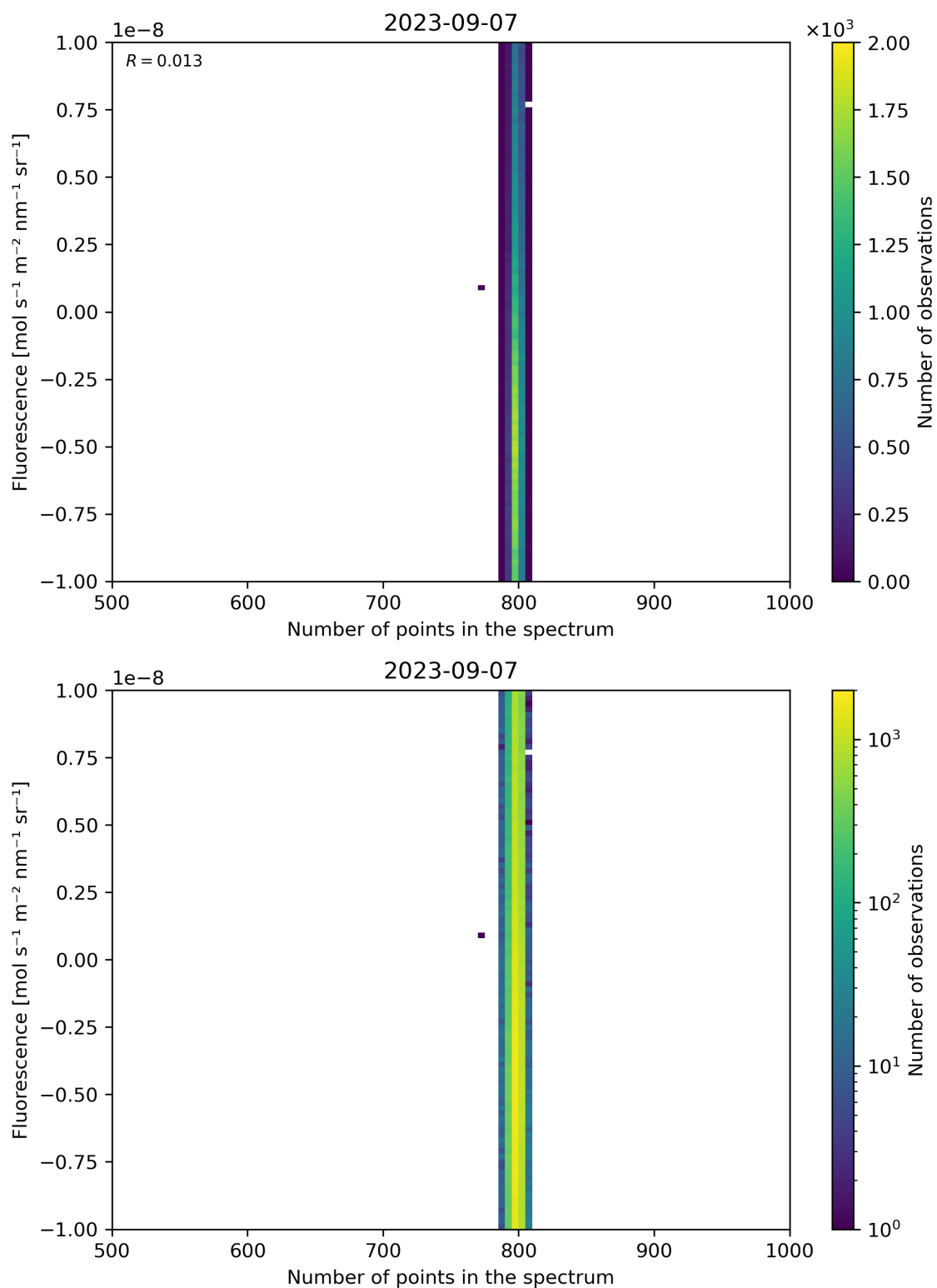
Figure 91: Scatter density plot of “Number of points in the spectrum” against “Fluorescence” for 2023-09-06 to 2023-09-08.
