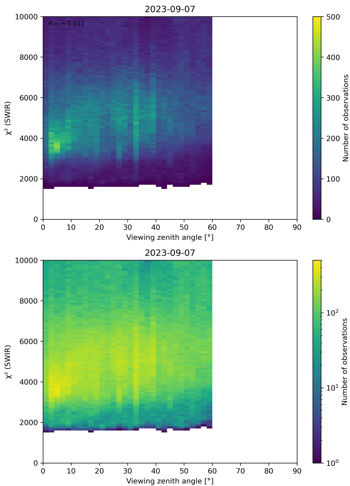
Figure 106: Scatter density plot of “Viewing zenith angle” against “ \chi^2 (SWIR)” for 2023-09-06 to 2023-09-08.
