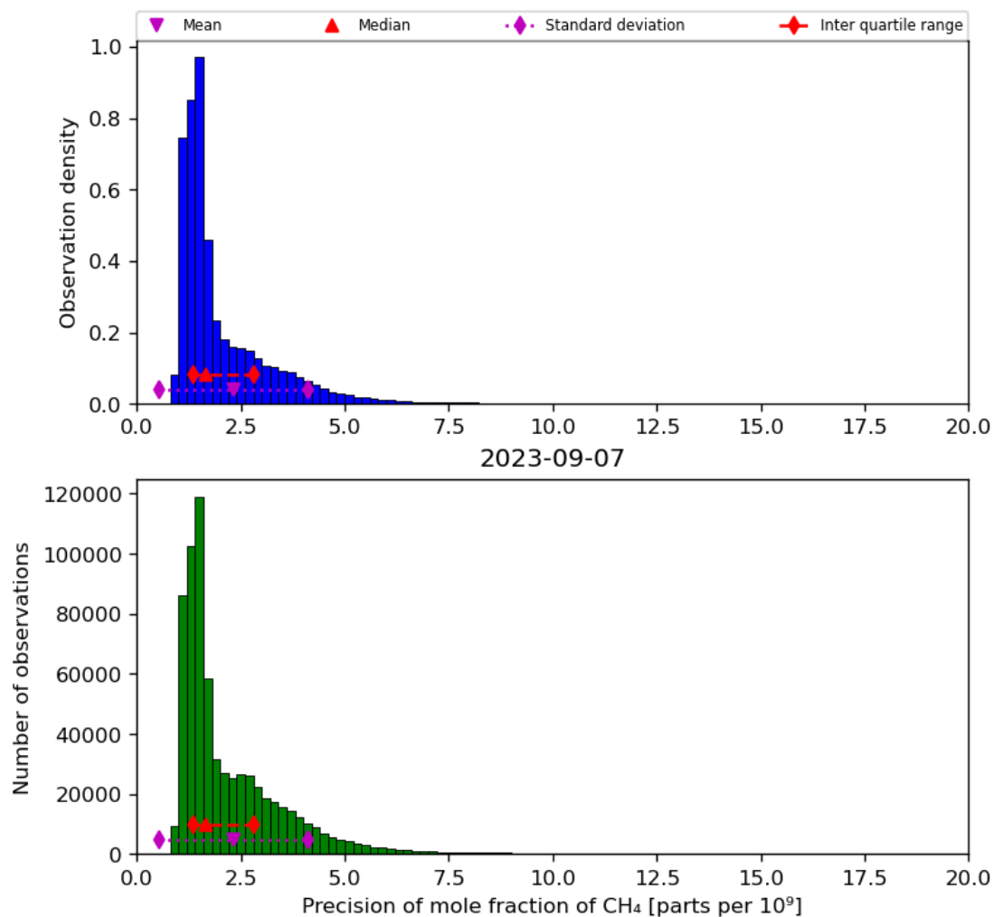
Figure 24: Histogram of “Precision of mole fraction of CH 4 ” for 2023-09-06 to 2023-09-08
