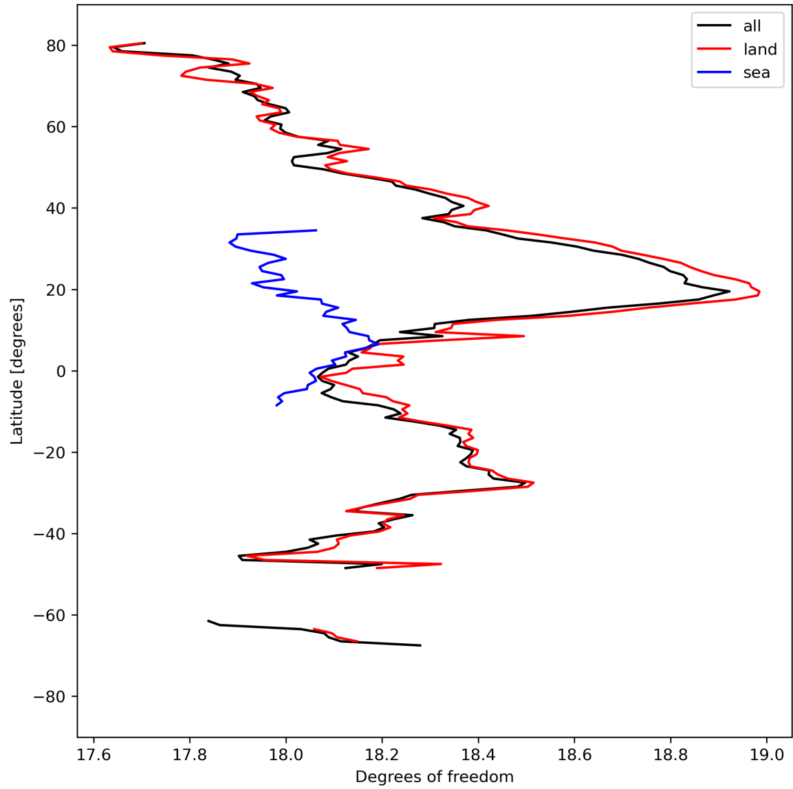
Figure 19: Zonal average of “Degrees of freedom” for 2023-09-06 to 2023-09-08.
