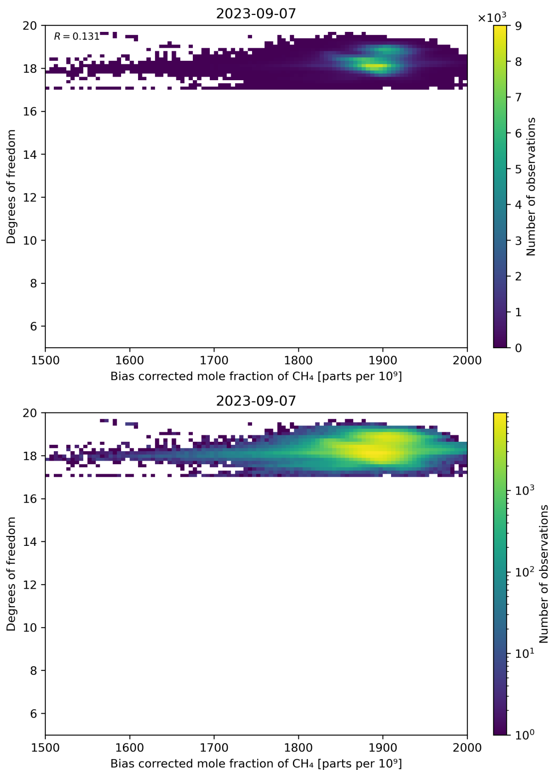
Figure 65: Scatter density plot of “Bias corrected mole fraction of CH 4 ” against “Degrees of freedom” for 2023-09-06 to 2023-09-08.
