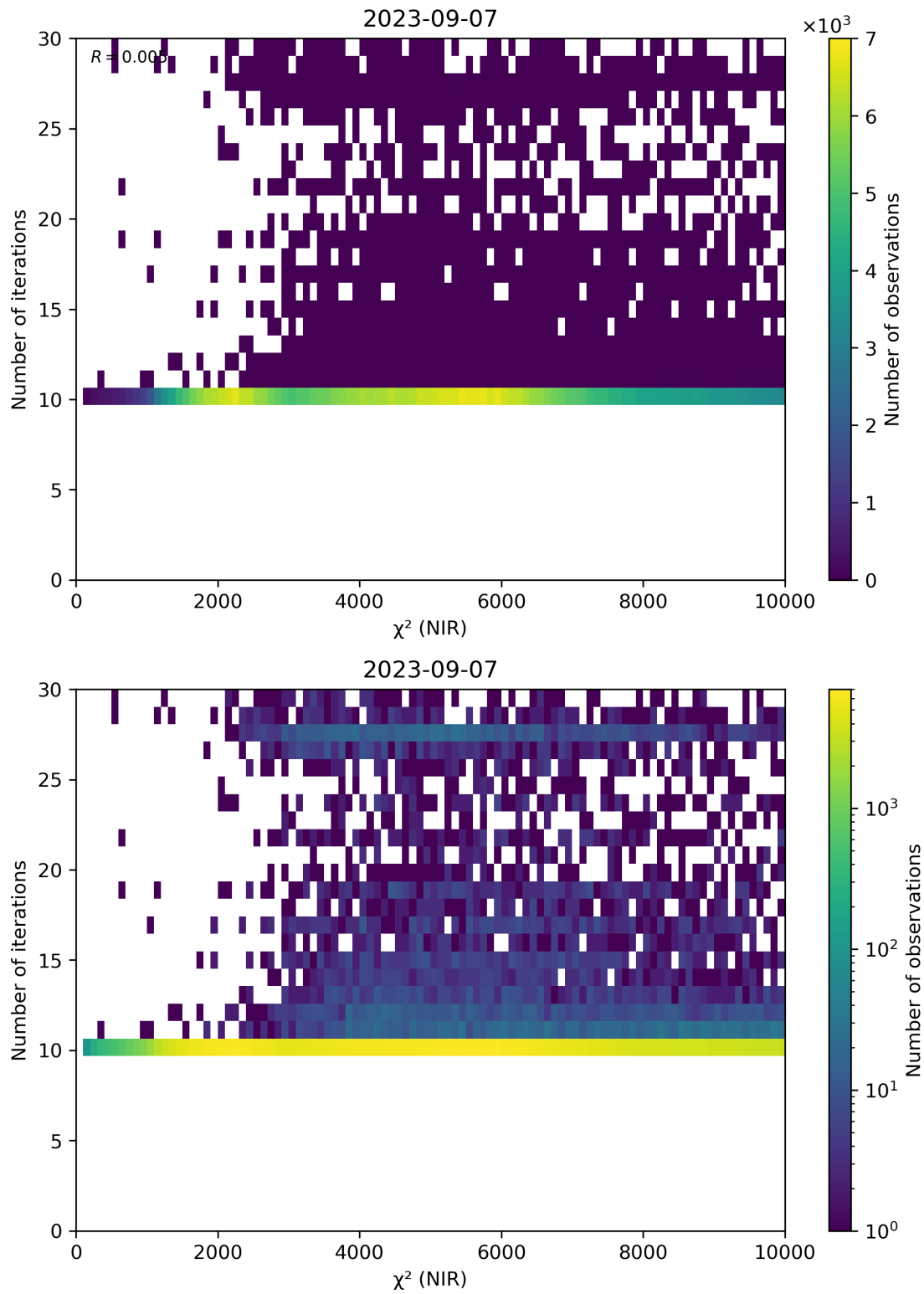
Figure 46: Scatter density plot of “ \chi^2 (NIR)” against “Number of iterations” for 2023-09-06 to 2023-09-08.
