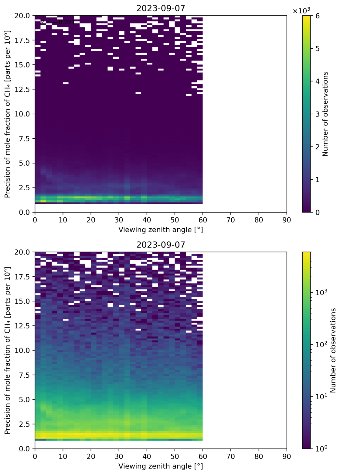
Figure 112: Scatter density plot of “Viewing zenith angle” against “Precision of mole fraction of CH 4 ” for 2023-09-06 to 2023-09-08.
