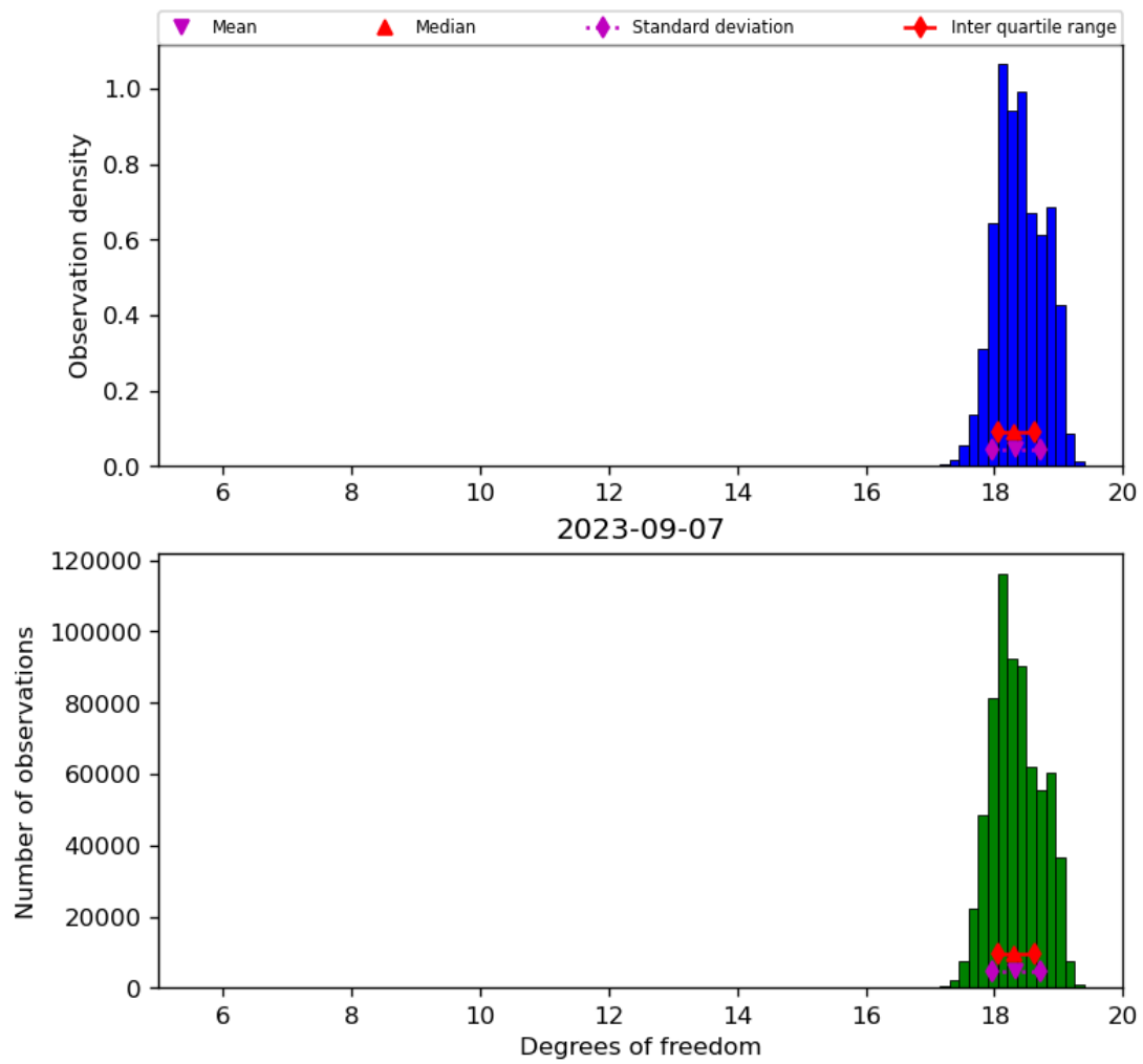
Figure 30: Histogram of “Degrees of freedom” for 2023-09-06 to 2023-09-08
