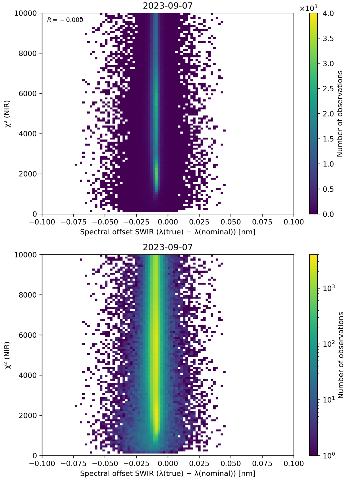
Figure 117: Scatter density plot of “Spectral offset SWIR ( \lambda(\text{true}) - \lambda(\text{nominal}) )” against “ \chi^2 (NIR)” for 2023-09-06 to 2023-09-08.
