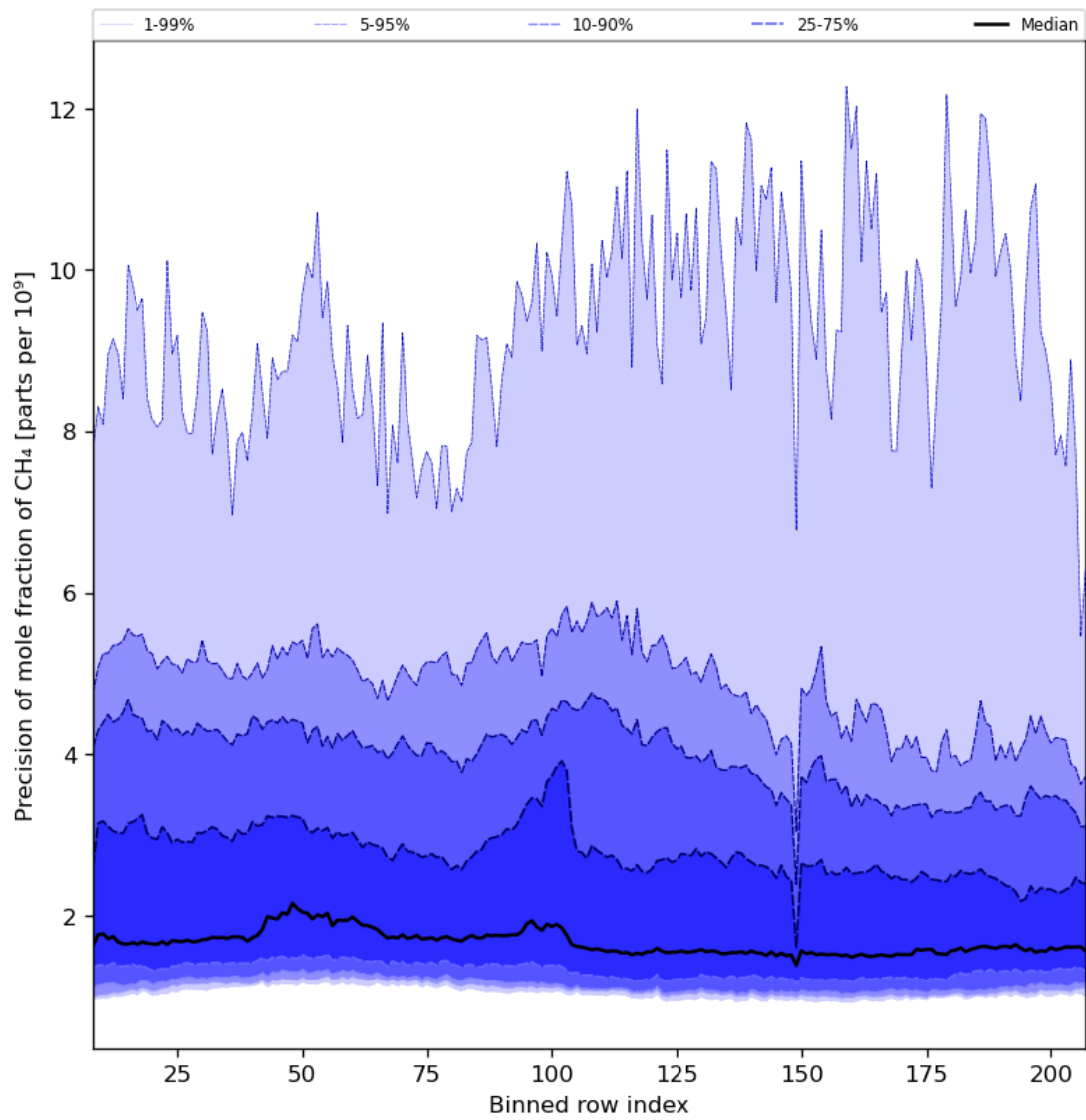
Figure 35: Along track statistics of “Precision of mole fraction of CH 4 ” for 2023-09-06 to 2023-09-08
