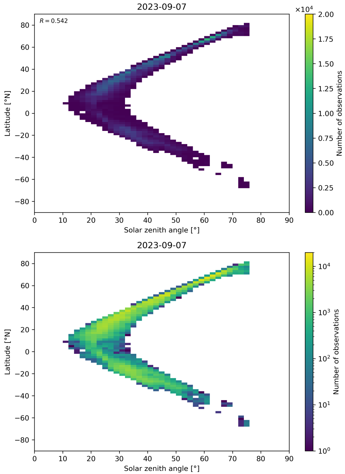
Figure 98: Scatter density plot of “Solar zenith angle” against “Latitude” for 2023-09-06 to 2023-09-08.
