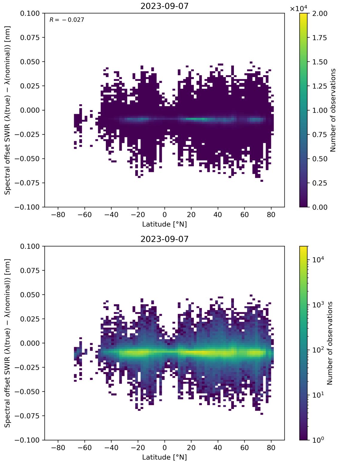
Figure 62: Scatter density plot of “Latitude” against “Spectral offset SWIR ( \lambda(\text{true}) - \lambda(\text{nominal}) )” for 2023-09-06 to 2023-09-08.
