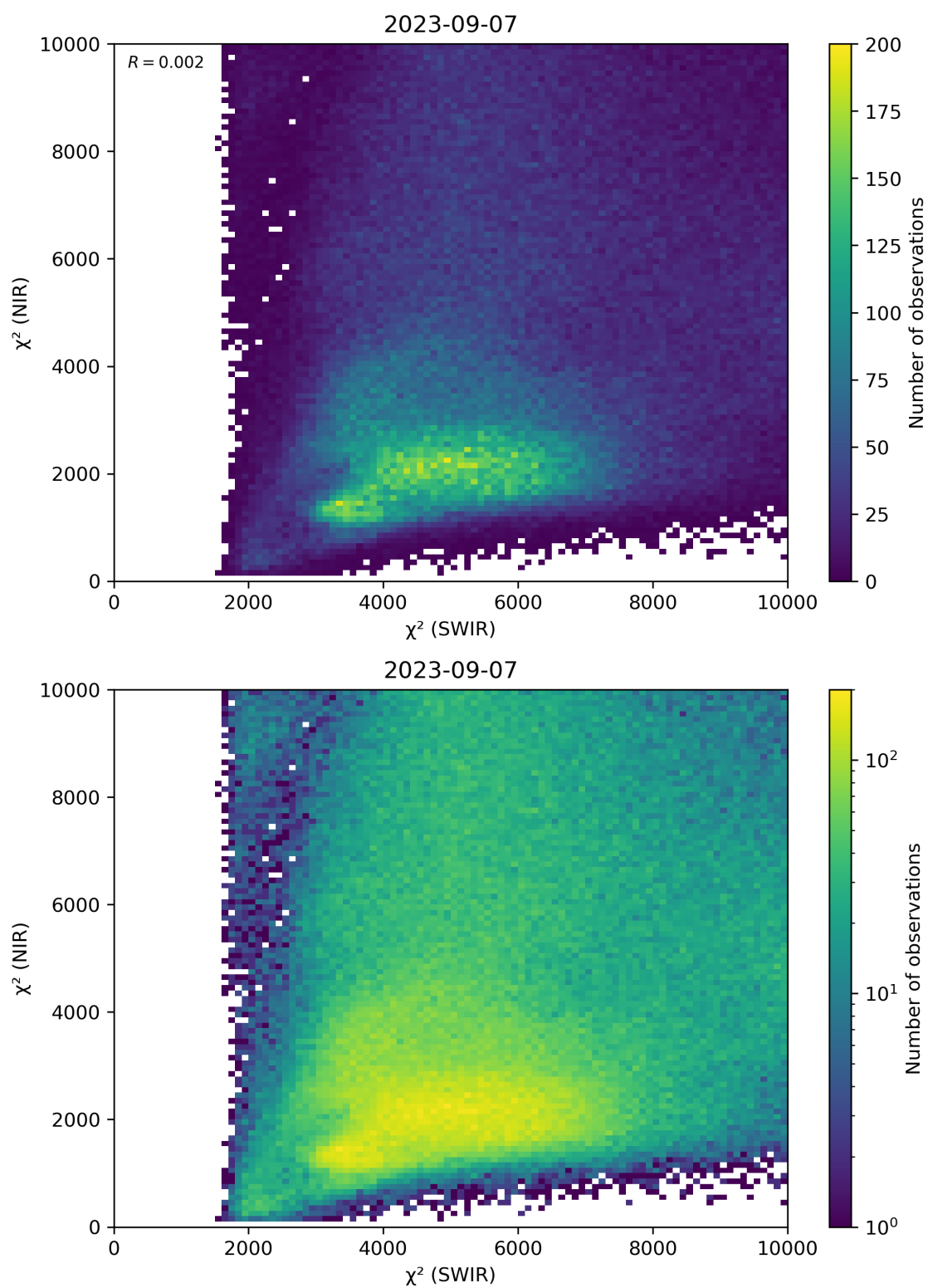
Figure 47: Scatter density plot of “ \chi^2 (SWIR)” against “ \chi^2 (NIR)” for 2023-09-06 to 2023-09-08.
