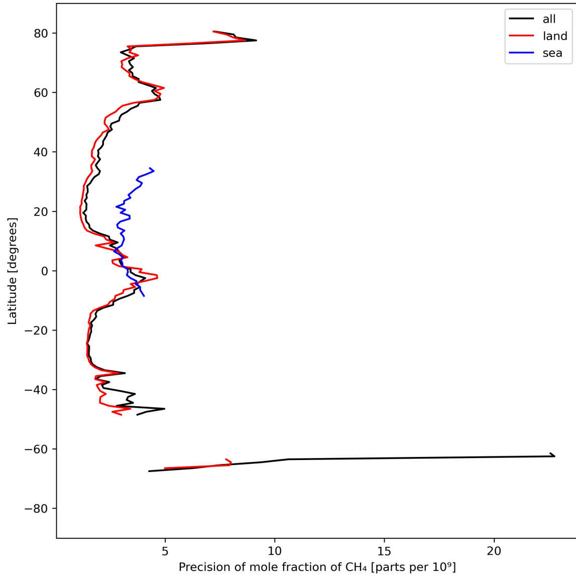
Figure 13: Zonal average of “Precision of mole fraction of CH 4 ” for 2023-09-06 to 2023-09-08.
