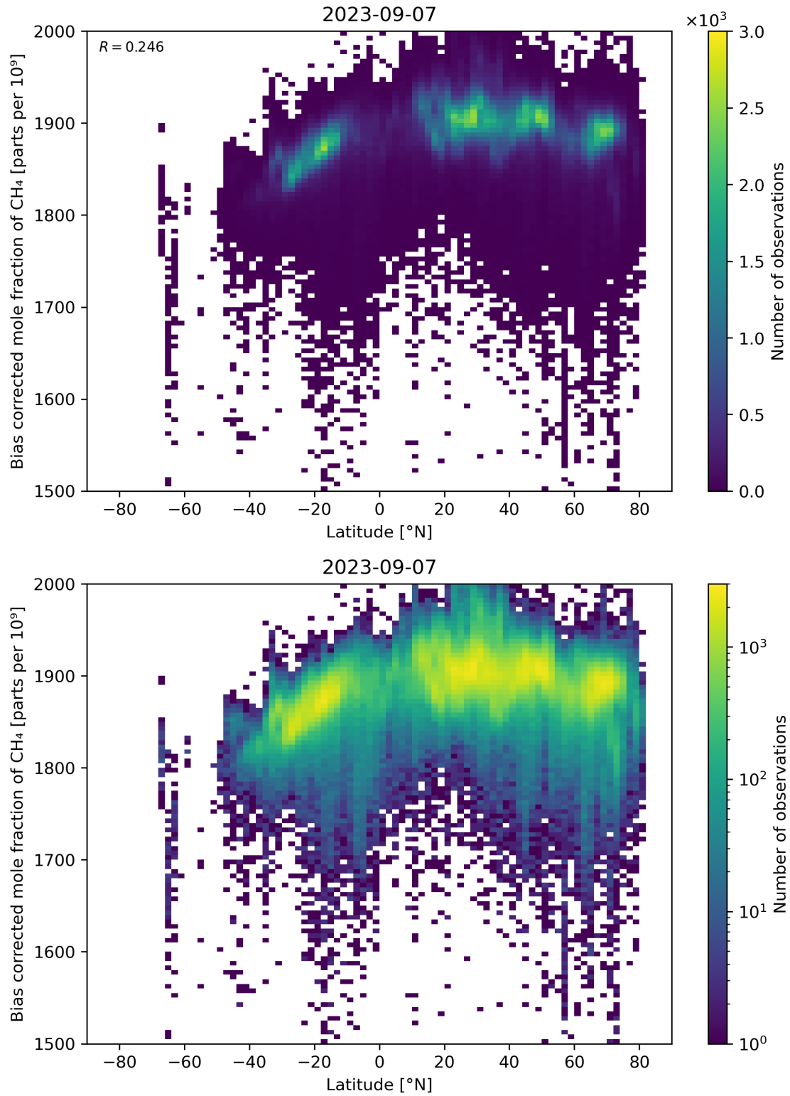
Figure 58: Scatter density plot of “Latitude” against “Bias corrected mole fraction of CH 4 ” for 2023-09-06 to 2023-09-08.
