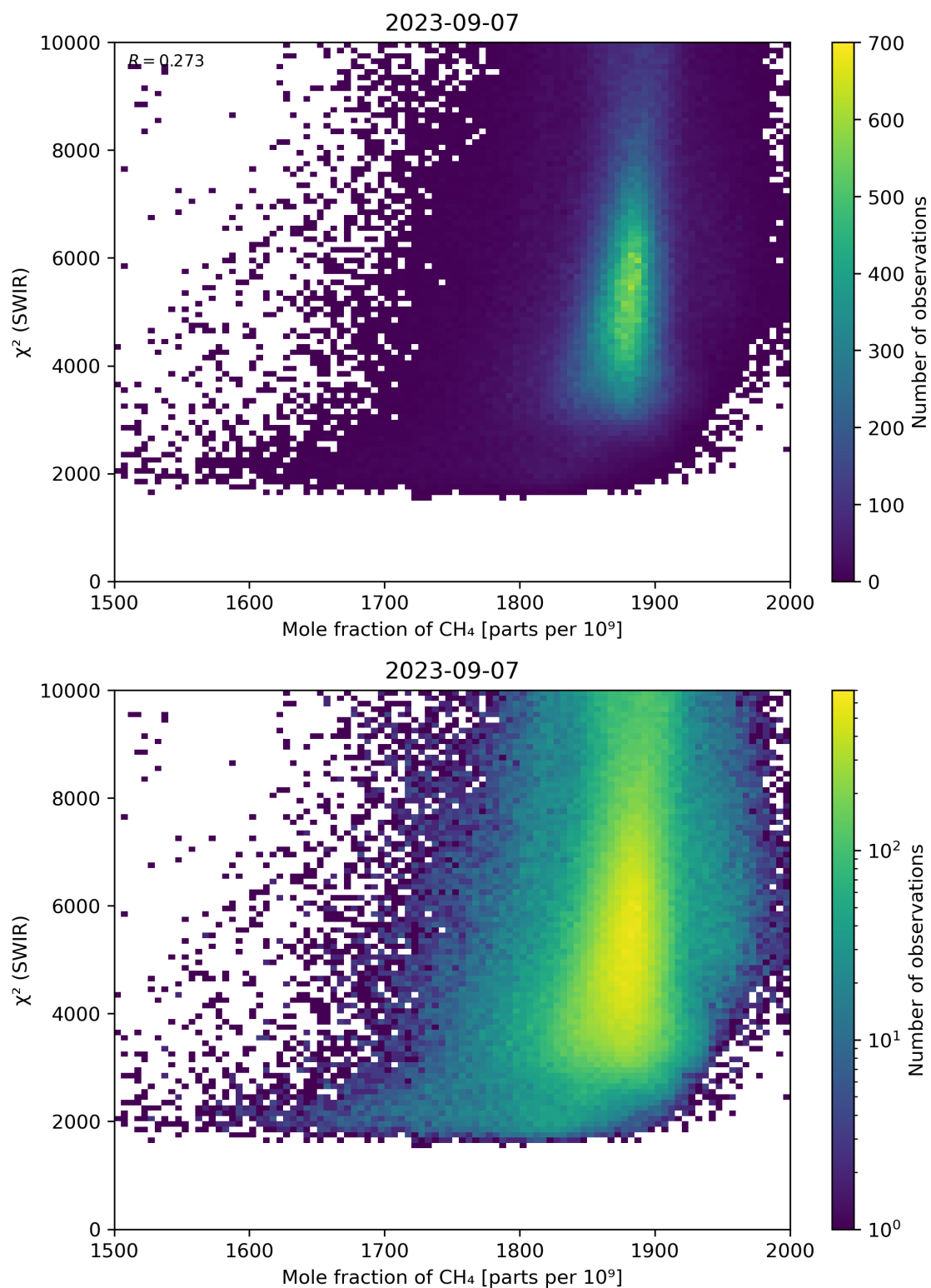
Figure 71: Scatter density plot of “Mole fraction of CH 4 ” against “ \chi^2 (SWIR)” for 2023-09-06 to 2023-09-08.
