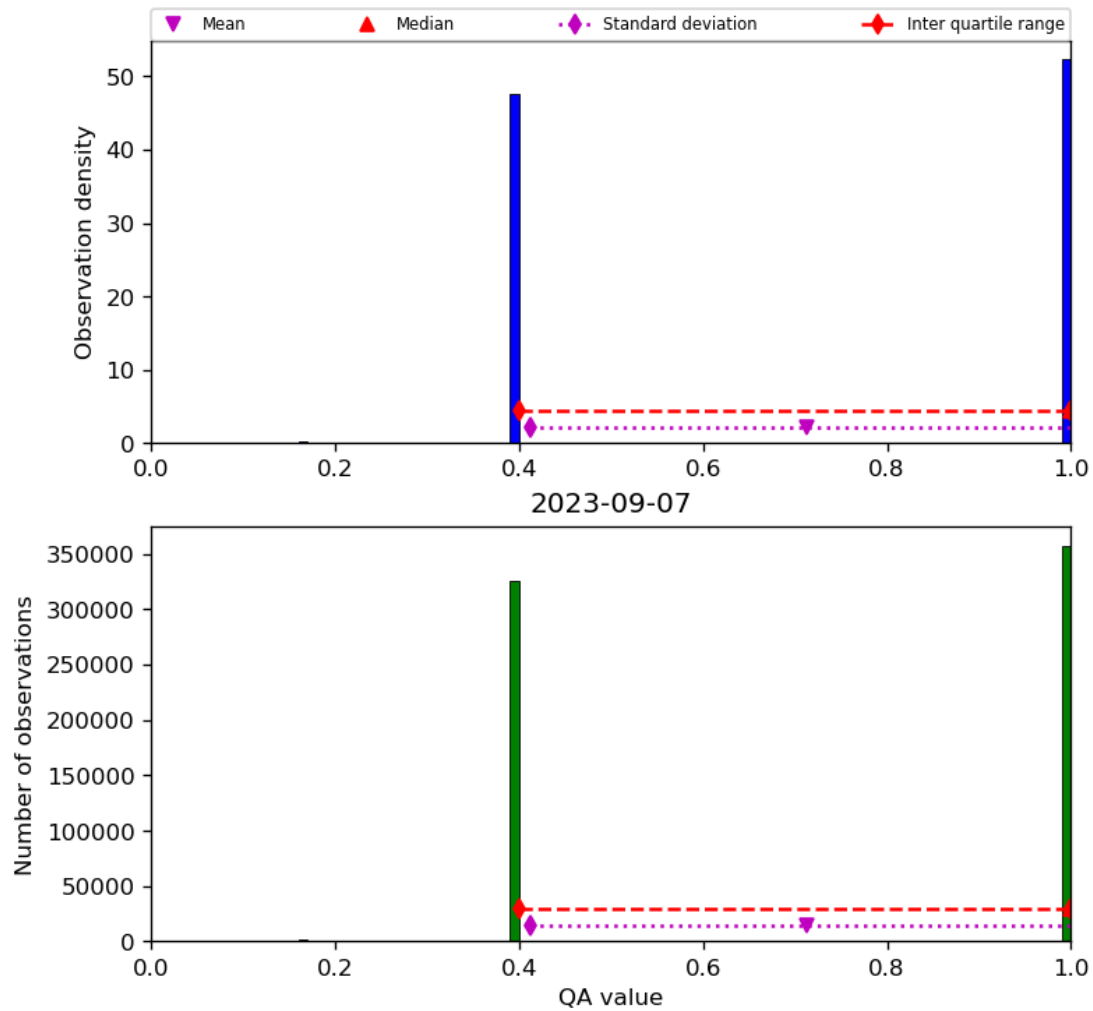
Figure 22: Histogram of “QA value” for 2023-09-06 to 2023-09-08
