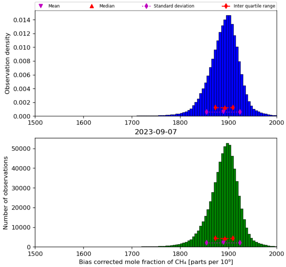
Figure 25: Histogram of “Bias corrected mole fraction of CH 4 ” for 2023-09-06 to 2023-09-08
