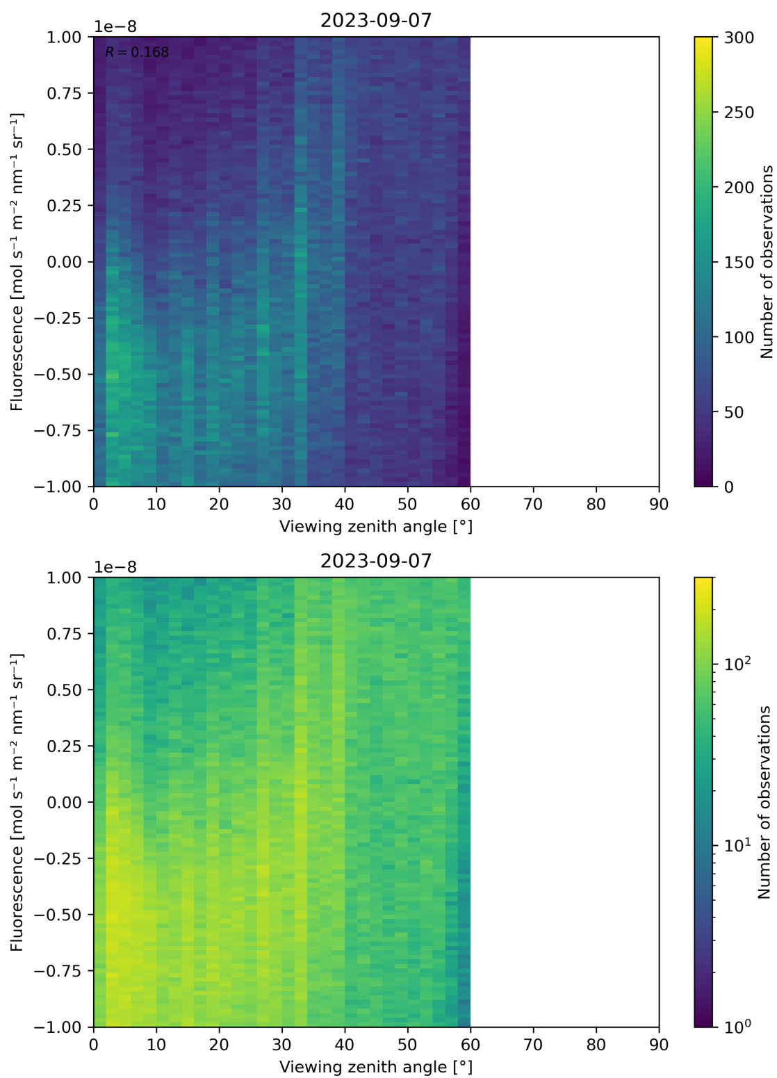
Figure 108: Scatter density plot of “Viewing zenith angle” against “Fluorescence” for 2023-09-06 to 2023-09-08.
