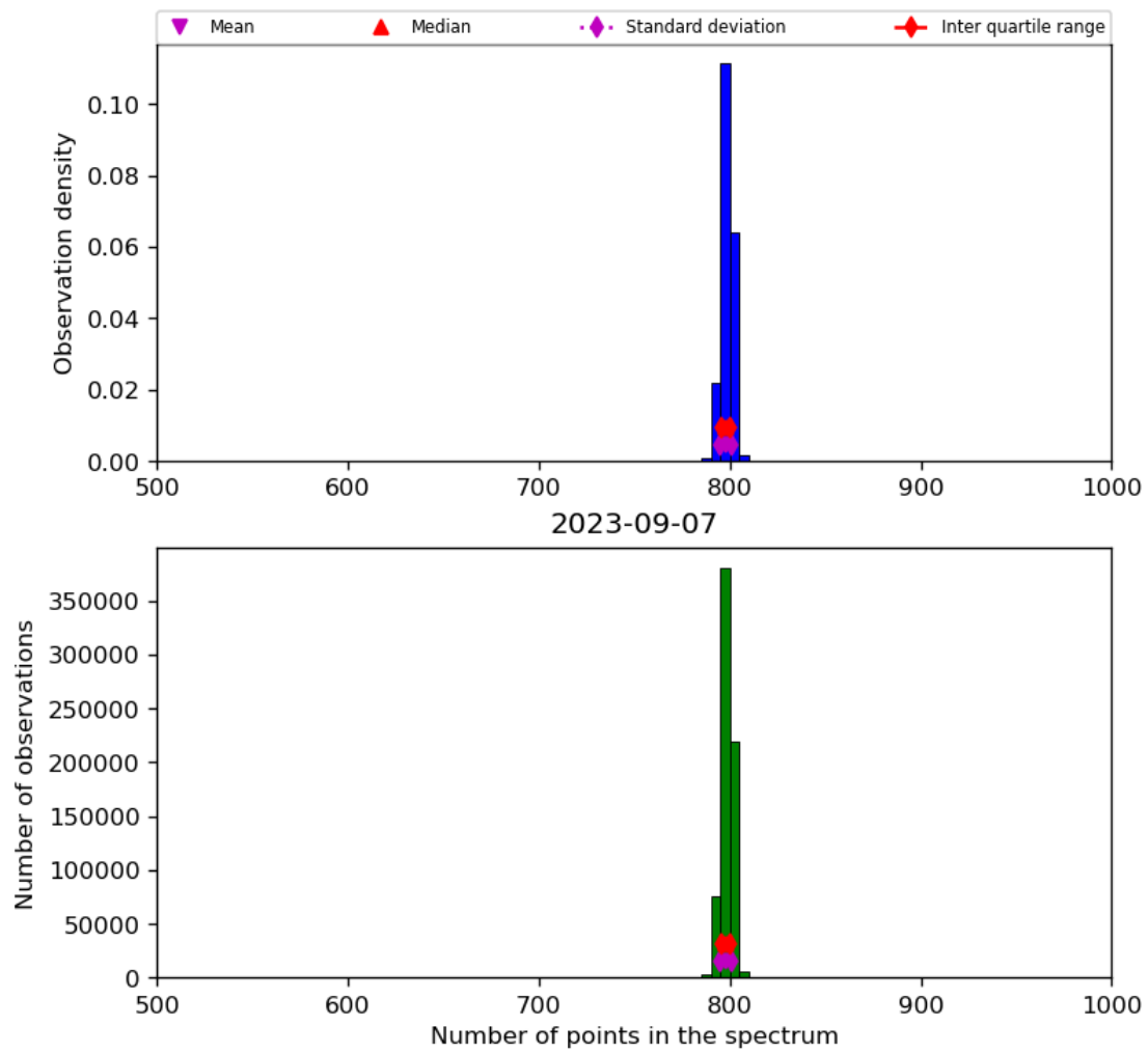
Figure 26: Histogram of “Number of points in the spectrum” for 2023-09-06 to 2023-09-08
