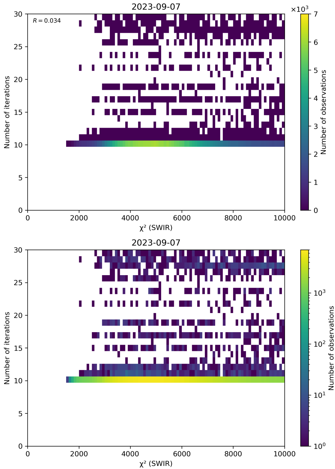
Figure 50: Scatter density plot of “ \chi^2 (SWIR)” against “Number of iterations” for 2023-09-06 to 2023-09-08.
