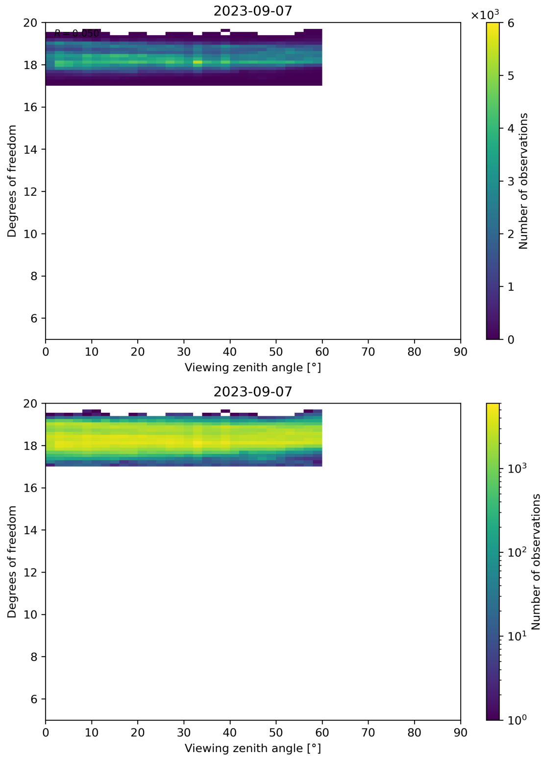
Figure 107: Scatter density plot of “Viewing zenith angle” against “Degrees of freedom” for 2023-09-06 to 2023-09-08.
