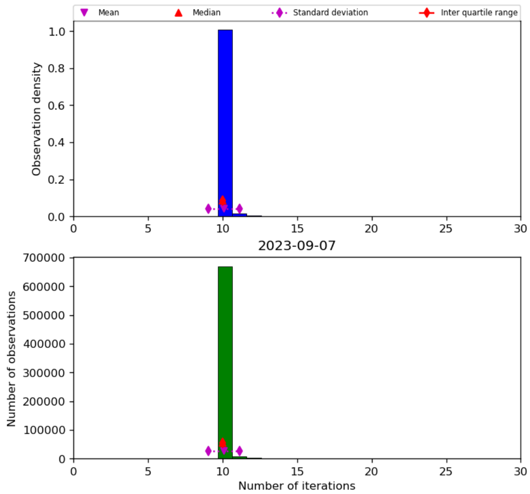
Figure 31: Histogram of “Number of iterations” for 2023-09-06 to 2023-09-08
