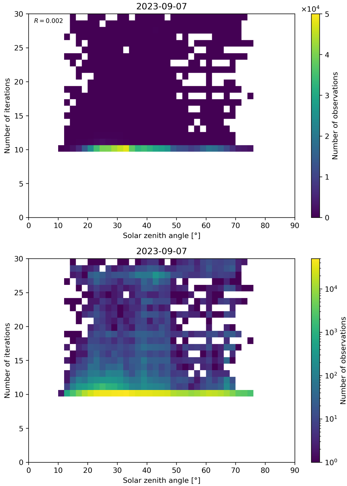
Figure 102: Scatter density plot of “Solar zenith angle” against “Number of iterations” for 2023-09-06 to 2023-09-08.
