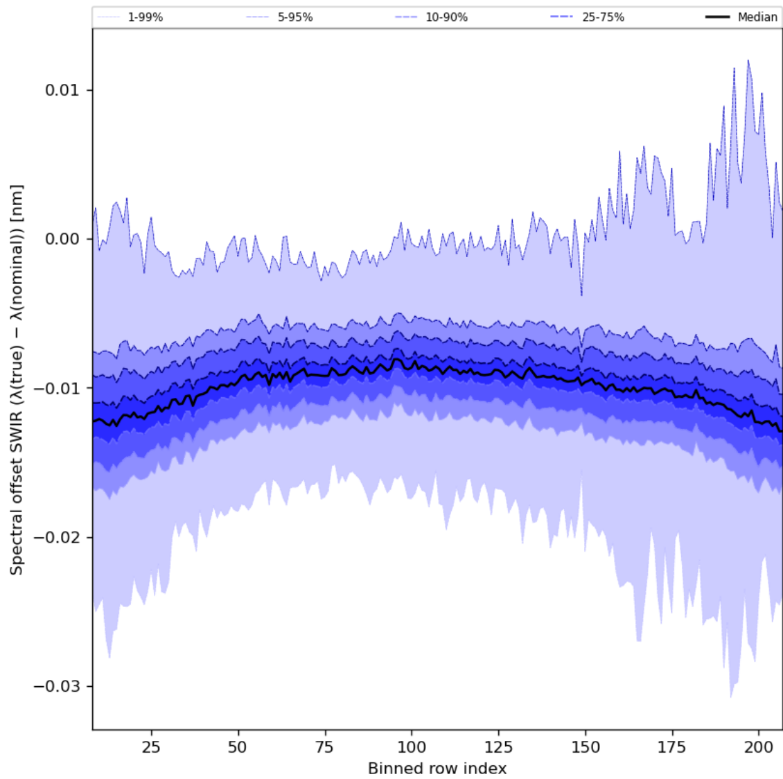
Figure 38: Along track statistics of “Spectral offset SWIR ( \lambda(\text{true}) - \lambda(\text{nominal}) )” for 2023-09-06 to 2023-09-08
