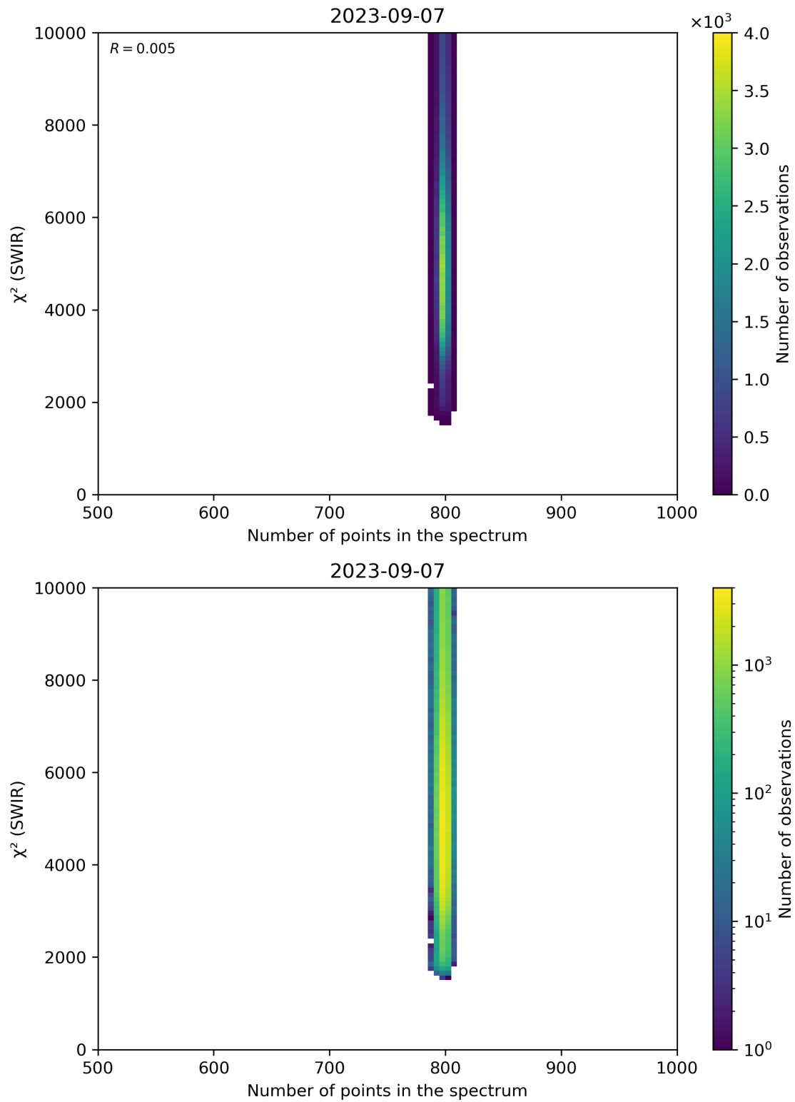
Figure 89: Scatter density plot of “Number of points in the spectrum” against “ \chi^2 (SWIR)” for 2023-09-06 to 2023-09-08.
