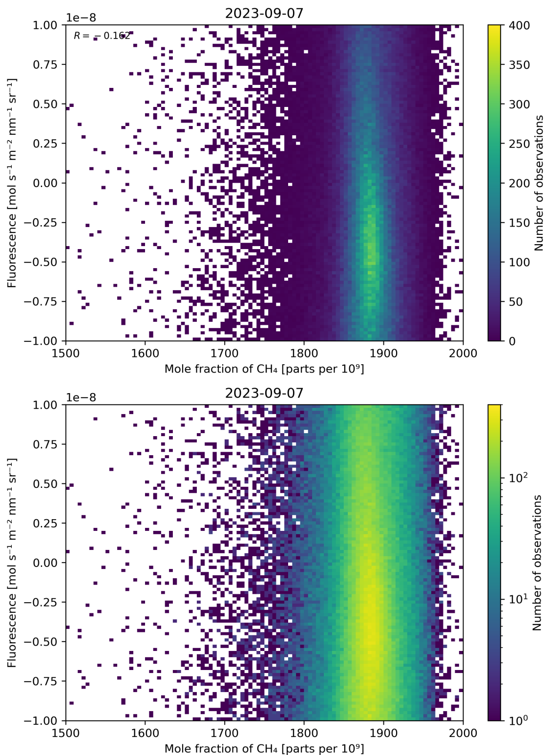
Figure 73: Scatter density plot of “Mole fraction of \text{CH}_4 ” against “Fluorescence” for 2023-09-06 to 2023-09-08.
