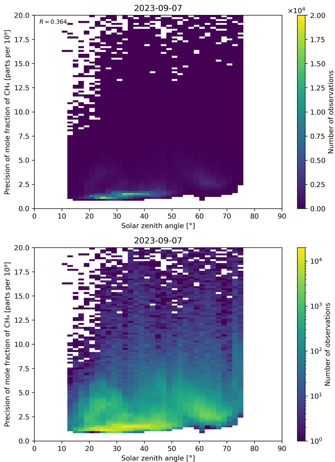
Figure 101: Scatter density plot of “Solar zenith angle” against “Precision of mole fraction of CH 4 ” for 2023-09-06 to 2023-09-08.
