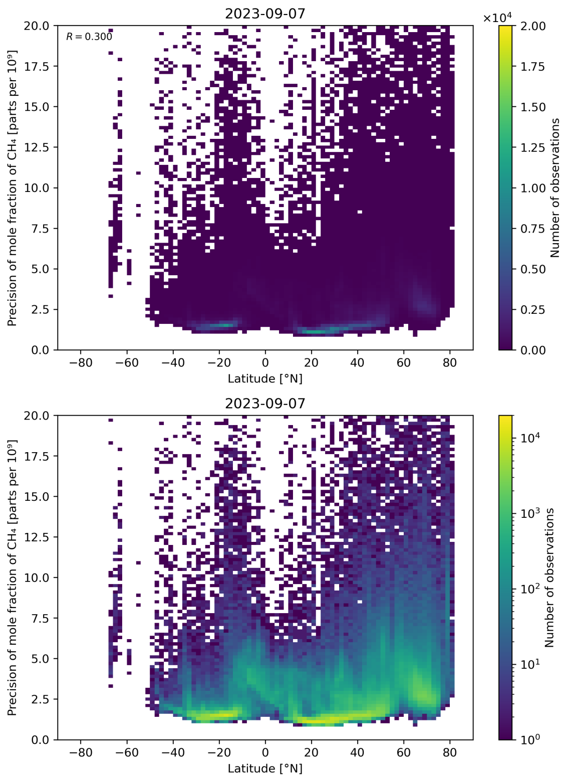
Figure 59: Scatter density plot of “Latitude” against “Precision of mole fraction of \text{CH}_4 ” for 2023-09-06 to 2023-09-08.
