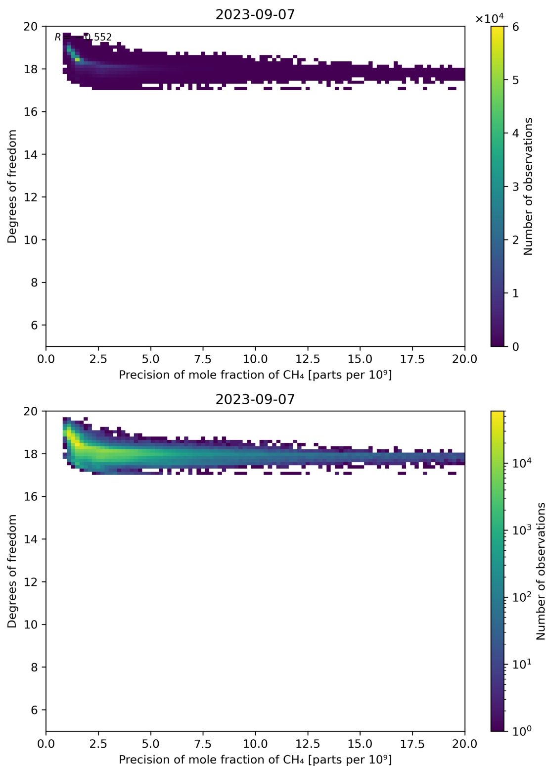
Figure 80: Scatter density plot of “Precision of mole fraction of CH 4 ” against “Degrees of freedom” for 2023-09-06 to 2023-09-08.
