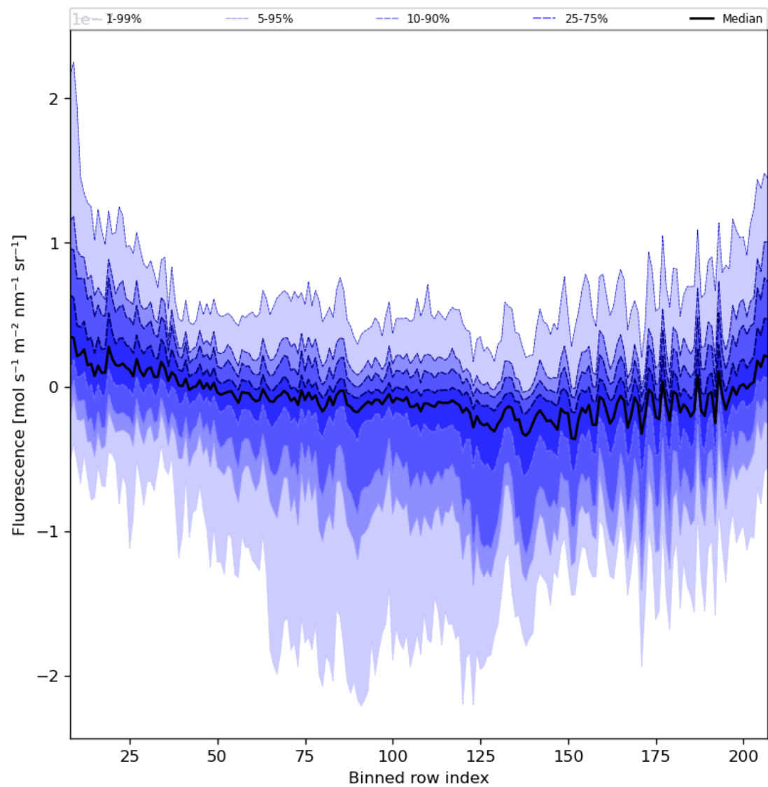
Figure 43: Along track statistics of “Fluorescence” for 2023-09-06 to 2023-09-08
