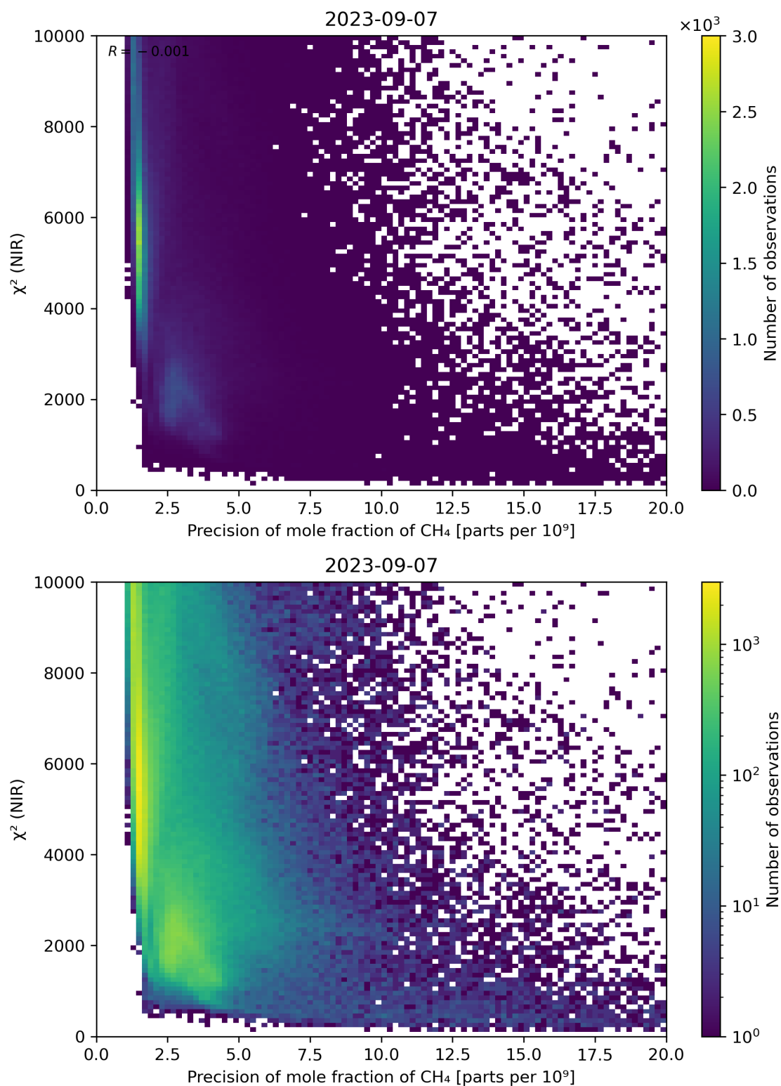
Figure 78: Scatter density plot of “Precision of mole fraction of CH 4 ” against “ \chi^2 (NIR)” for 2023-09-06 to 2023-09-08.
