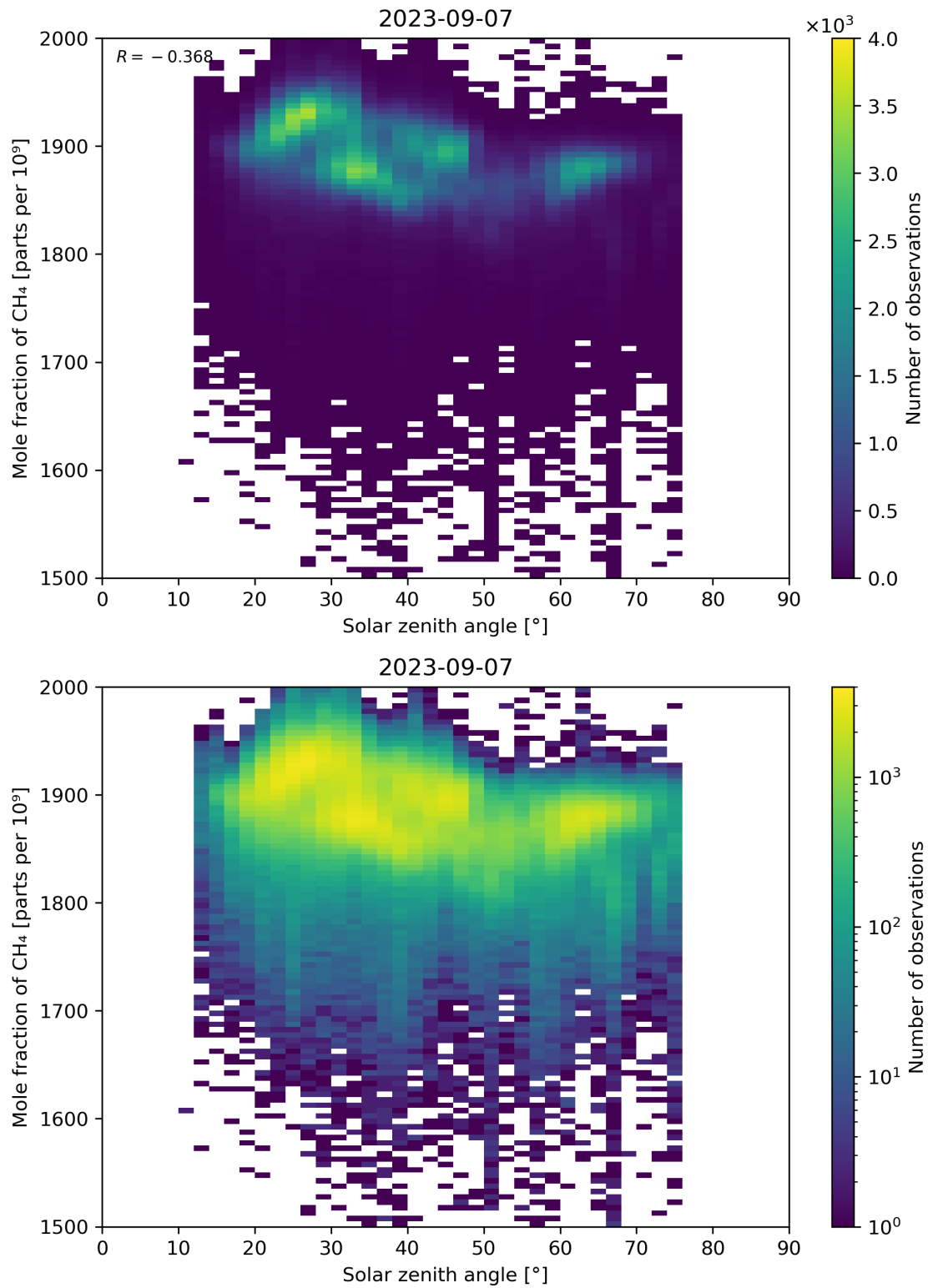
Figure 99: Scatter density plot of “Solar zenith angle” against “Mole fraction of CH 4 ” for 2023-09-06 to 2023-09-08.
