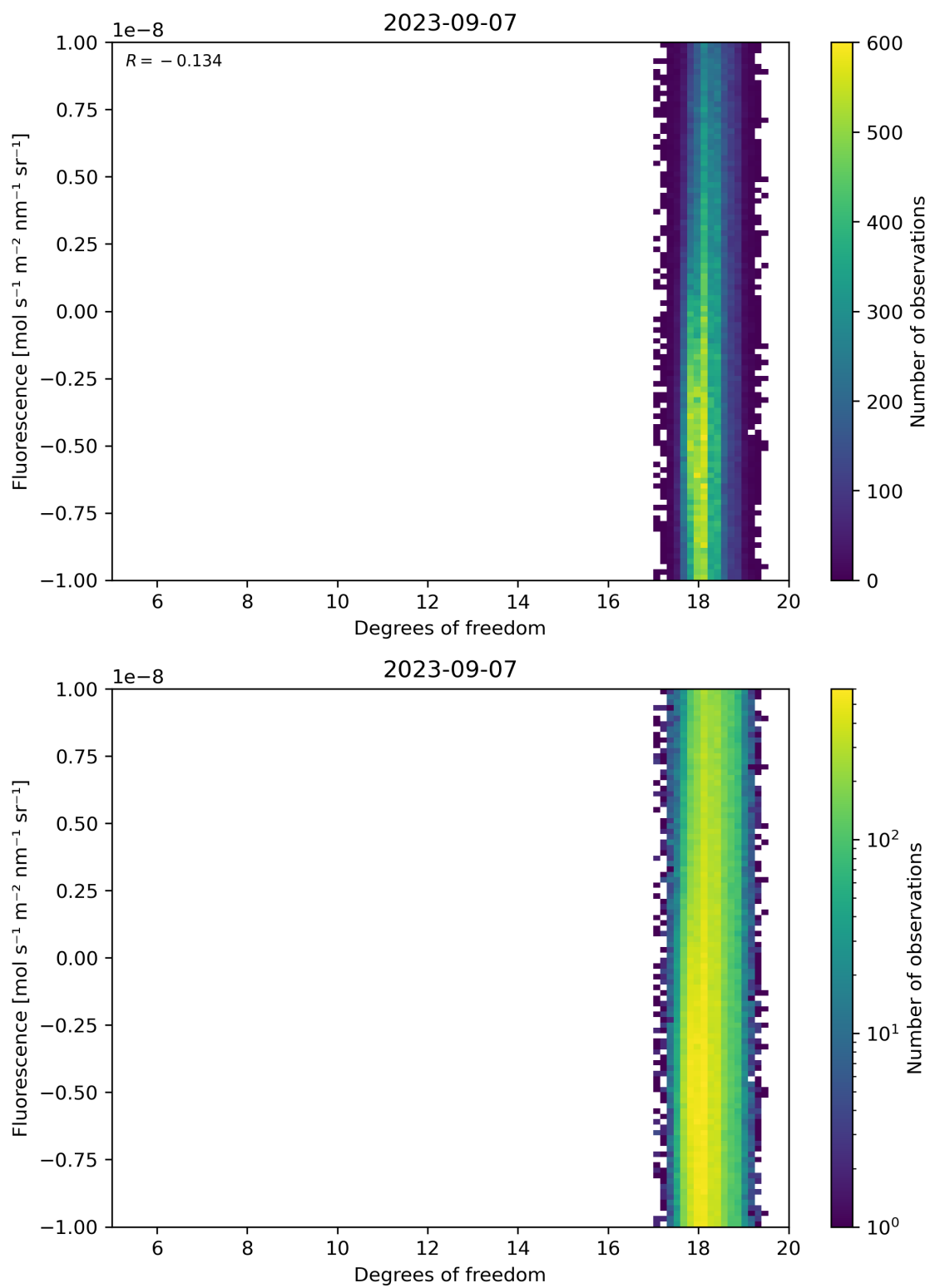
Figure 51: Scatter density plot of “Degrees of freedom” against “Fluorescence” for 2023-09-06 to 2023-09-08.
