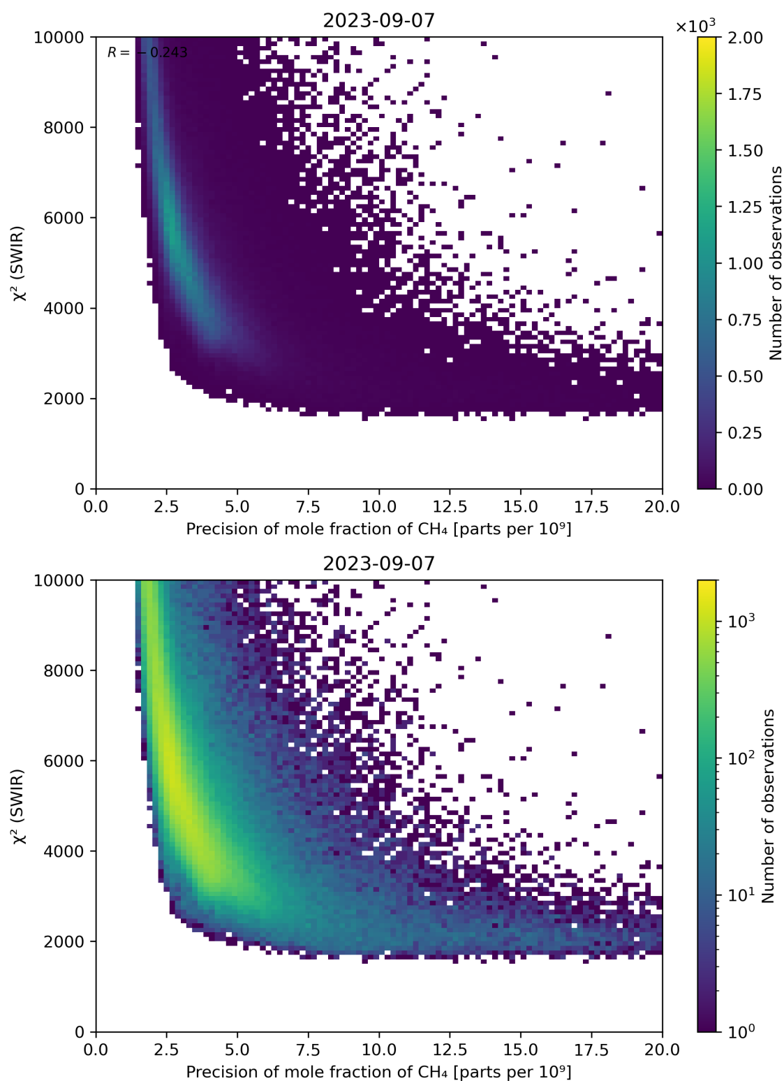
Figure 79: Scatter density plot of “Precision of mole fraction of \text{CH}_4 ” against “ \chi^2 (SWIR)” for 2023-09-06 to 2023-09-08.
