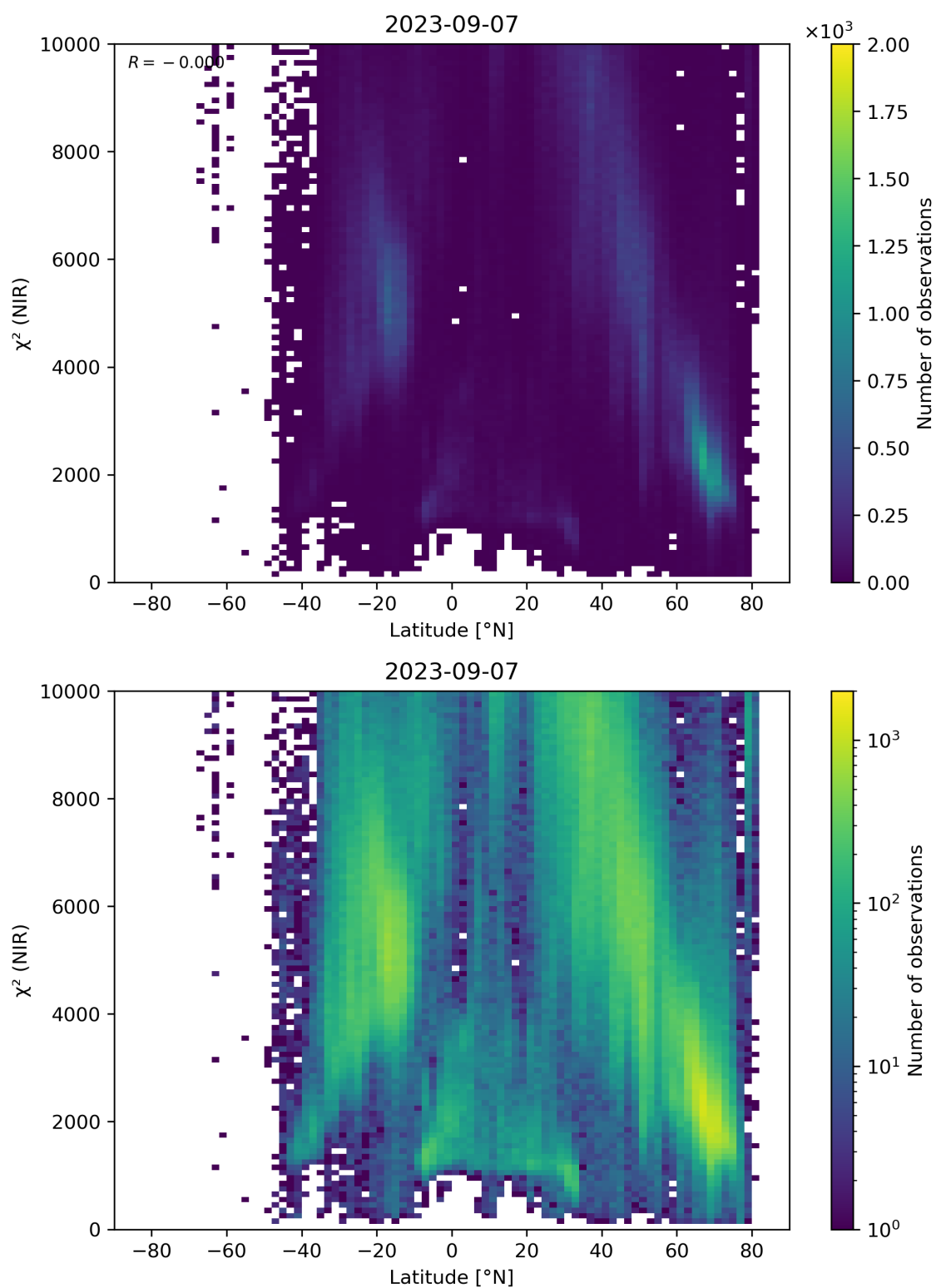
Figure 53: Scatter density plot of “Latitude” against “ \chi^2 (NIR)” for 2023-09-06 to 2023-09-08.
