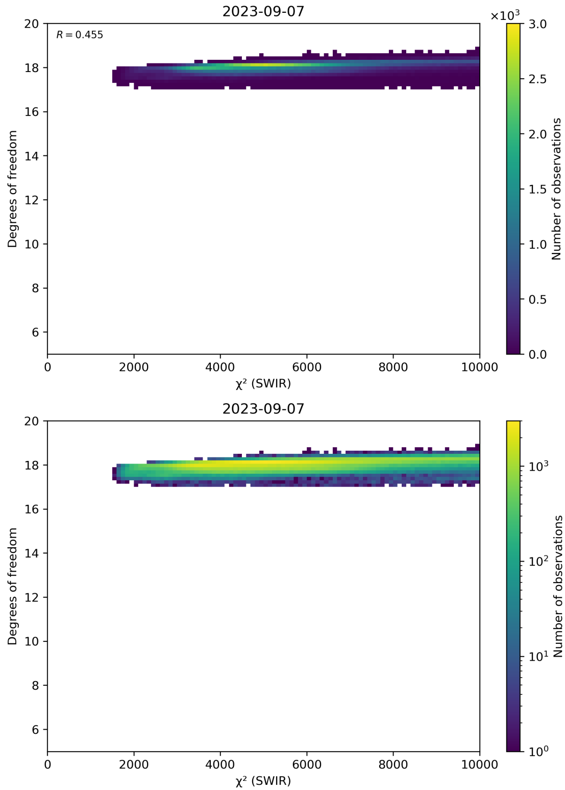
Figure 48: Scatter density plot of “ \chi^2 (SWIR)” against “Degrees of freedom” for 2023-09-06 to 2023-09-08.
