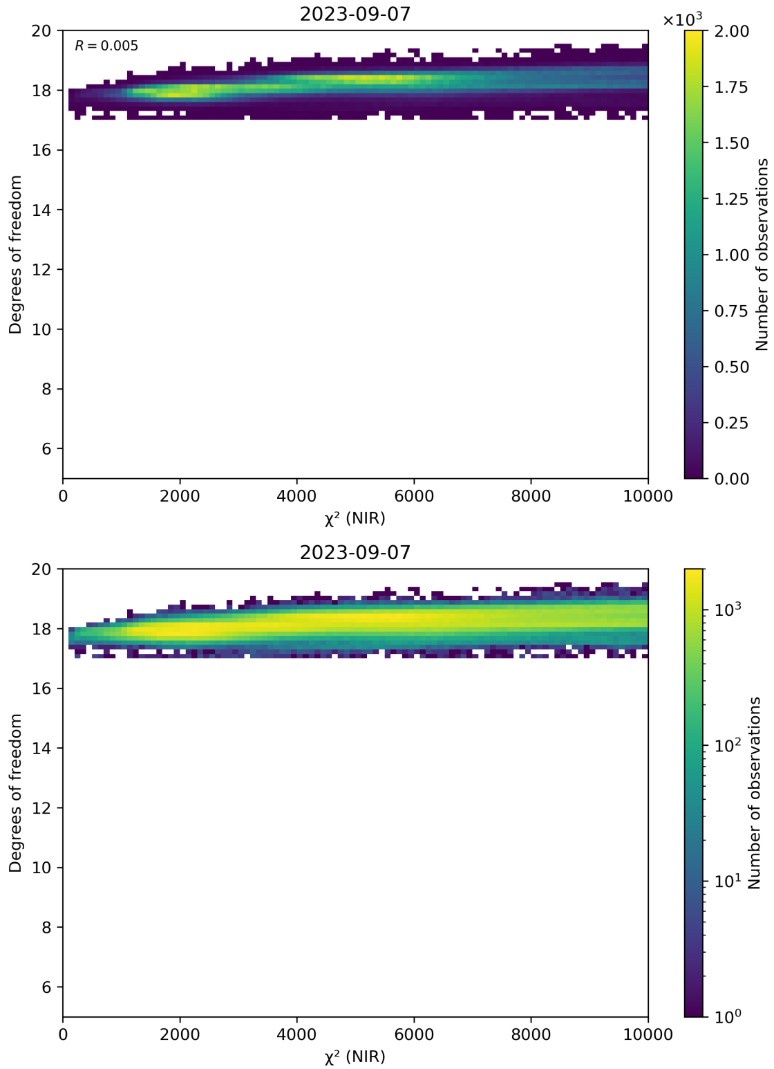
Figure 44: Scatter density plot of “ \chi^2 (NIR)” against “Degrees of freedom” for 2023-09-06 to 2023-09-08.
