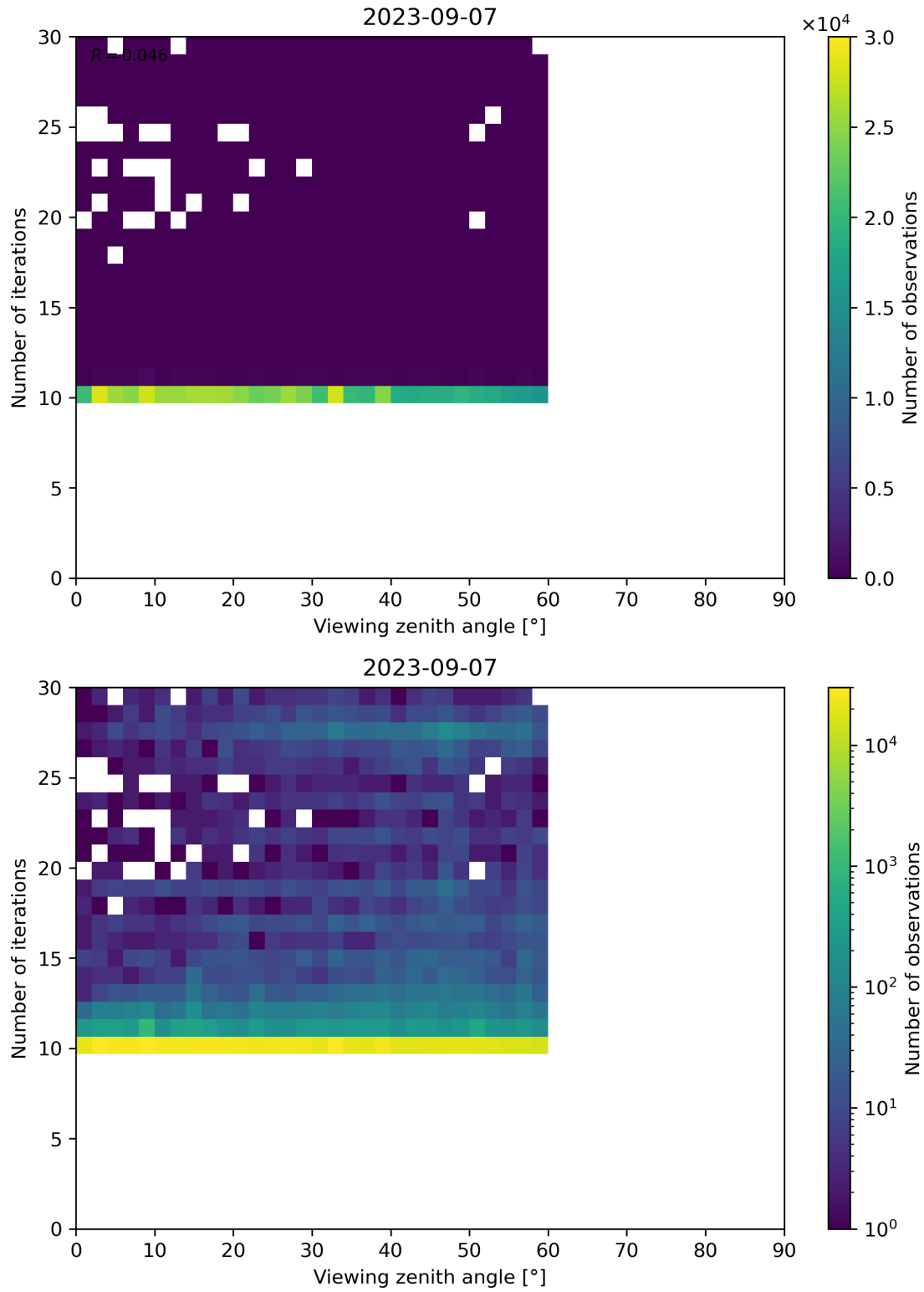
Figure 113: Scatter density plot of “Viewing zenith angle” against “Number of iterations” for 2023-09-06 to 2023-09-08.
