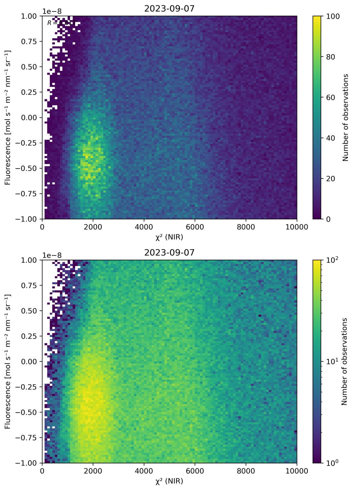
Figure 45: Scatter density plot of “ \chi^2 (NIR)” against “Fluorescence” for 2023-09-06 to 2023-09-08.
