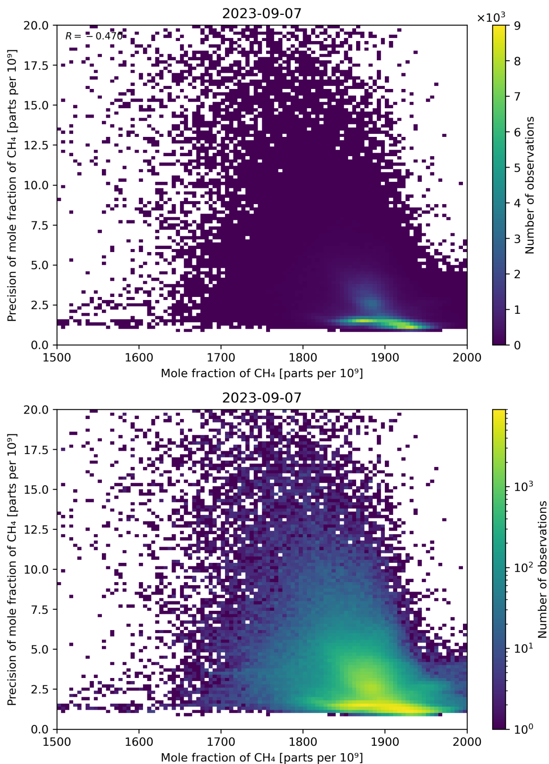
Figure 75: Scatter density plot of “Mole fraction of CH 4 ” against “Precision of mole fraction of CH 4 ” for 2023-09-06 to 2023-09-08.
