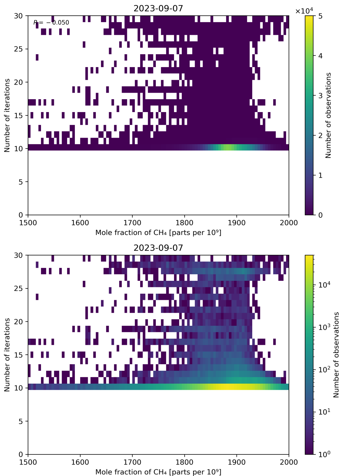
Figure 76: Scatter density plot of “Mole fraction of CH 4 ” against “Number of iterations” for 2023-09-06 to 2023-09-08.
