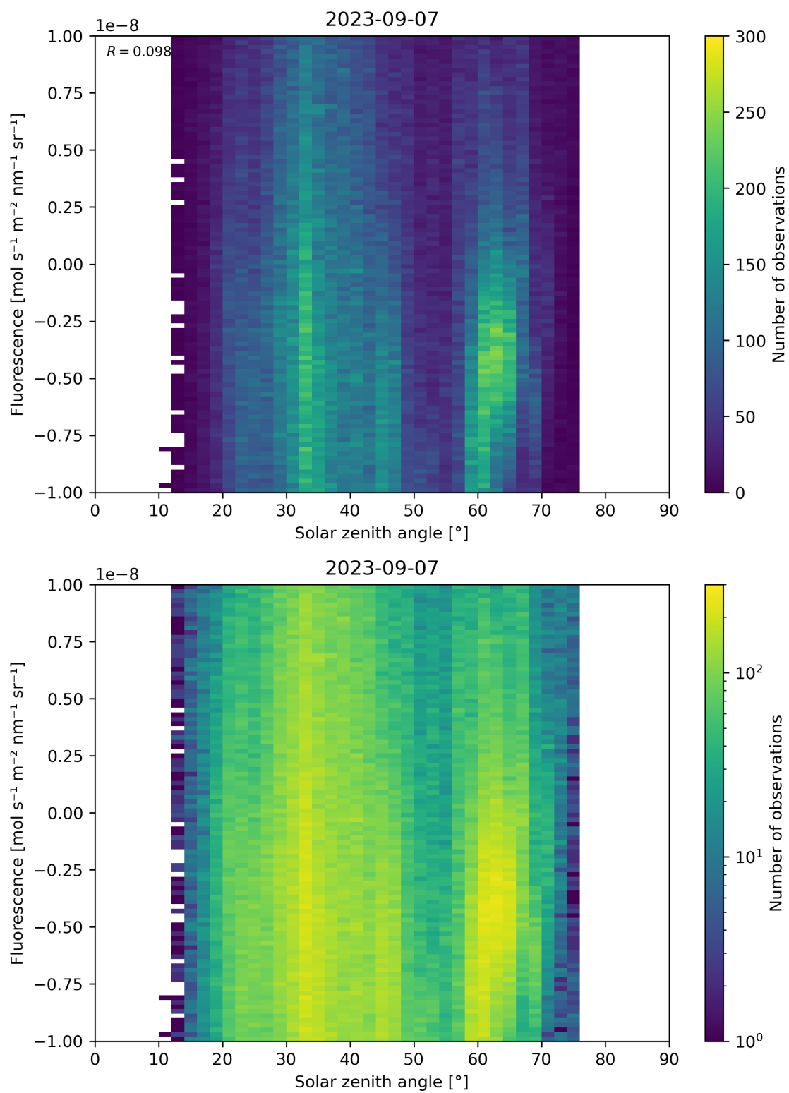
Figure 97: Scatter density plot of “Solar zenith angle” against “Fluorescence” for 2023-09-06 to 2023-09-08.
