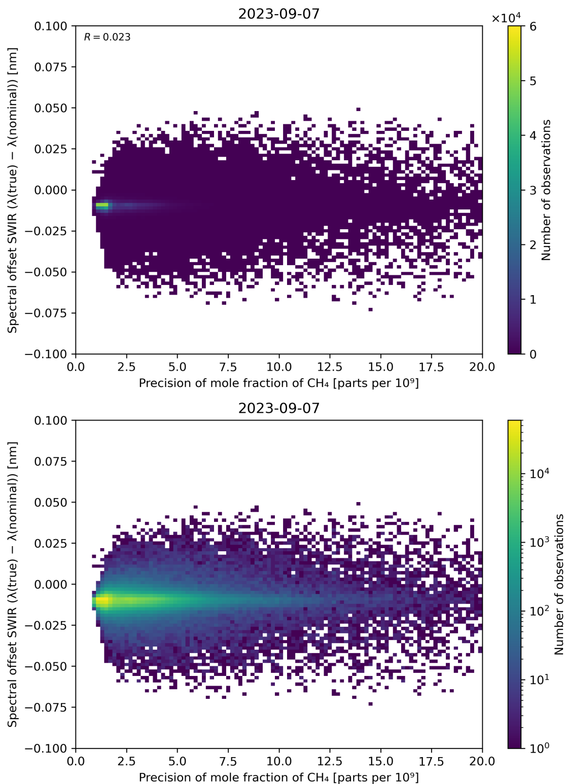
Figure 85: Scatter density plot of “Precision of mole fraction of CH 4 ” against “Spectral offset SWIR ( \lambda(\text{true}) - \lambda(\text{nominal}) )” for 2023-09-06 to 2023-09-08.
