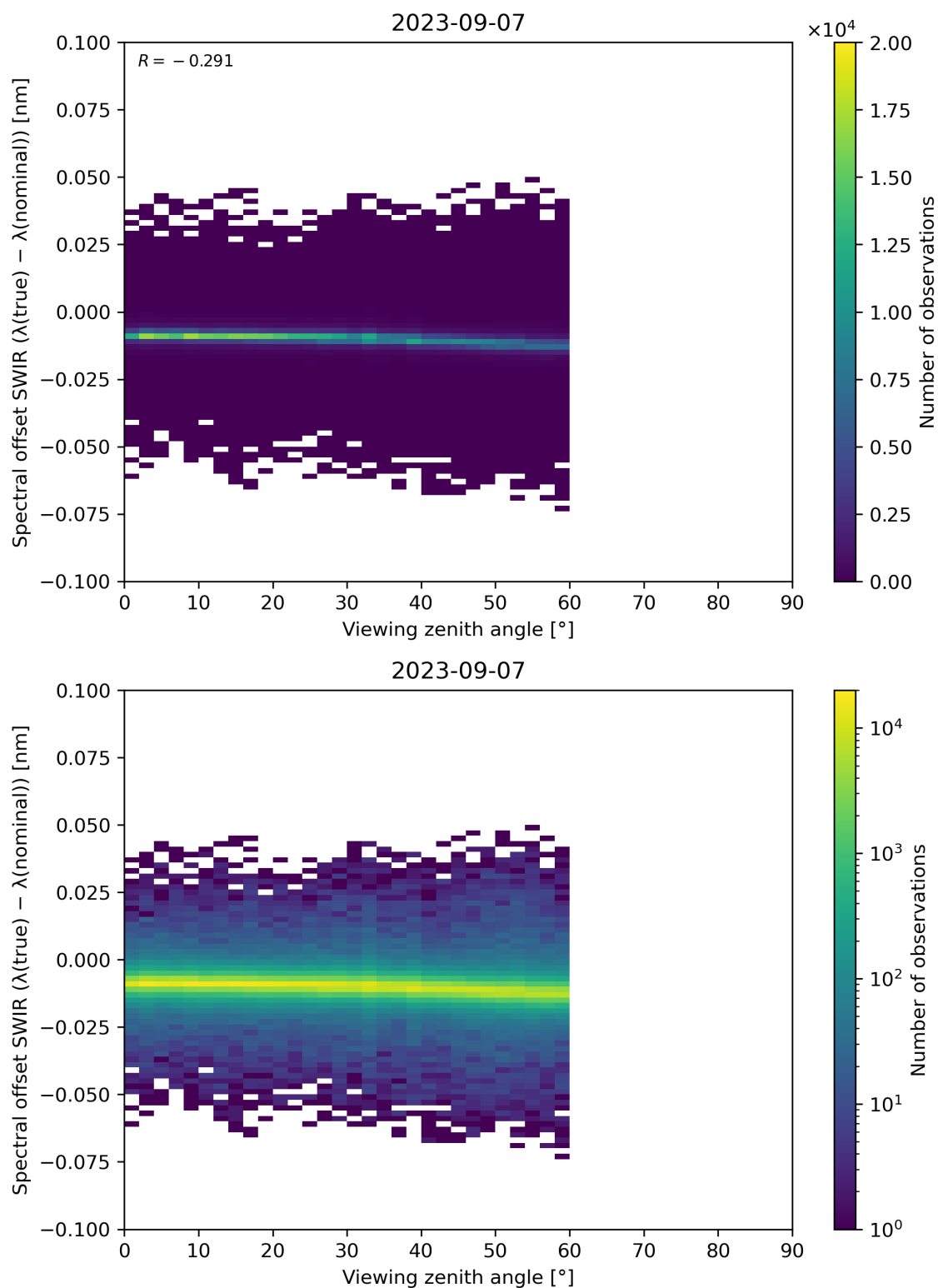
Figure 116: Scatter density plot of “Viewing zenith angle” against “Spectral offset SWIR ( \lambda(\text{true}) - \lambda(\text{nominal}) )” for 2023-09-06 to 2023-09-08.
