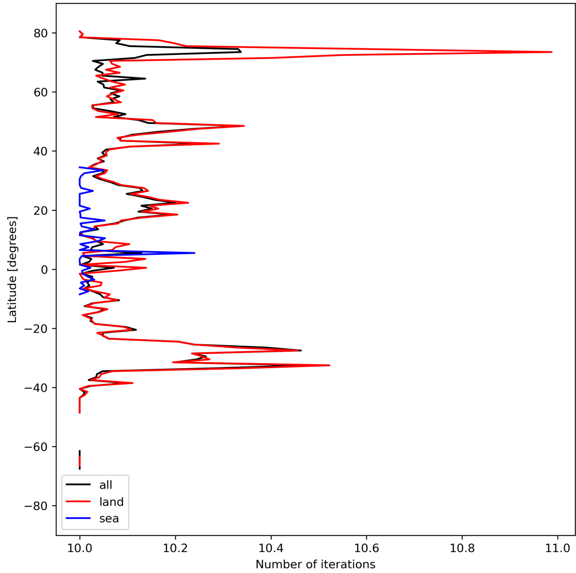
Figure 20: Zonal average of “Number of iterations” for 2023-09-06 to 2023-09-08.
