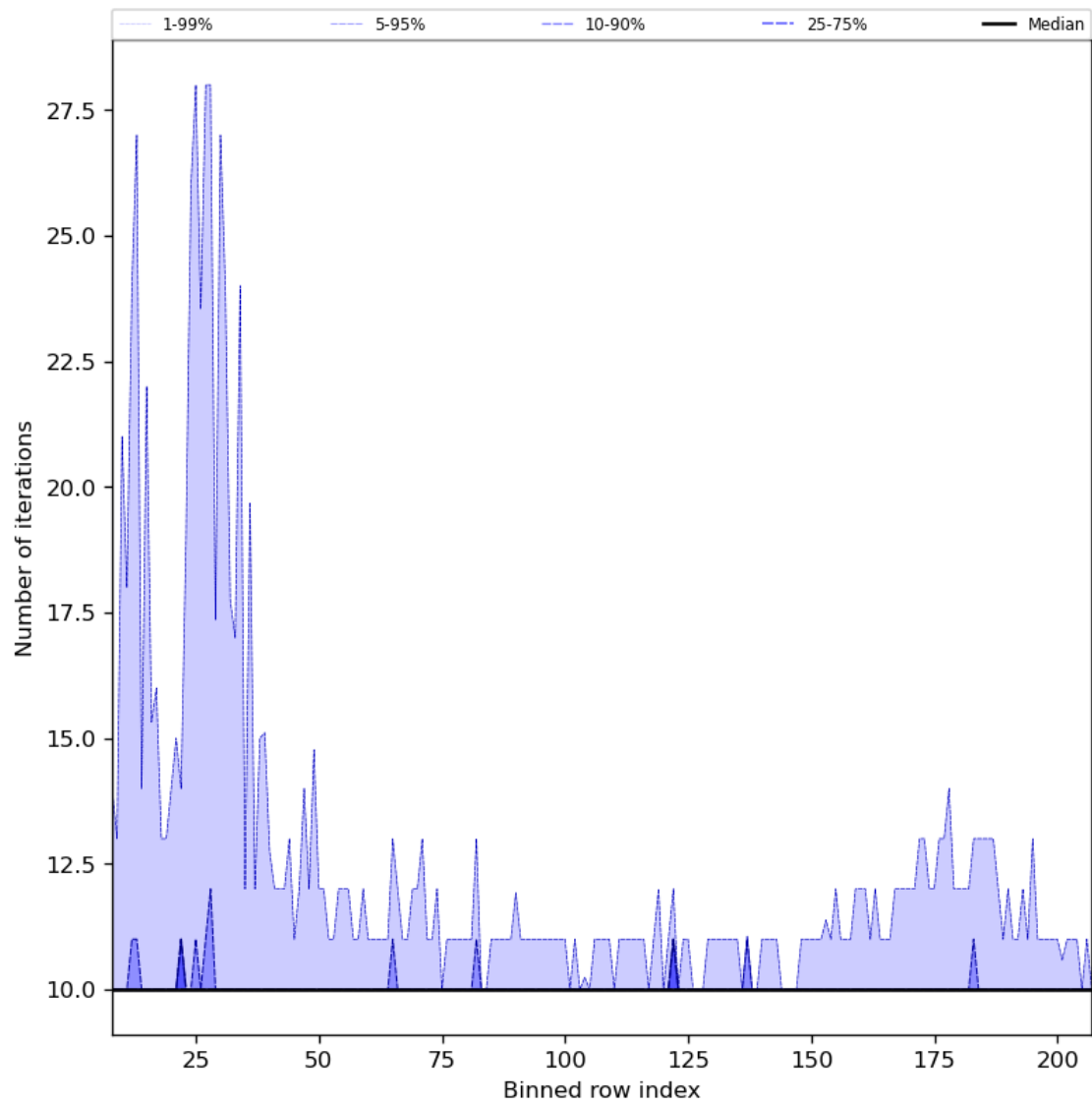
Figure 42: Along track statistics of “Number of iterations” for 2023-09-06 to 2023-09-08
