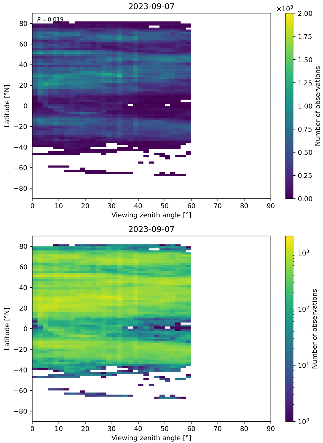
Figure 109: Scatter density plot of “Viewing zenith angle” against “Latitude” for 2023-09-06 to 2023-09-08.
