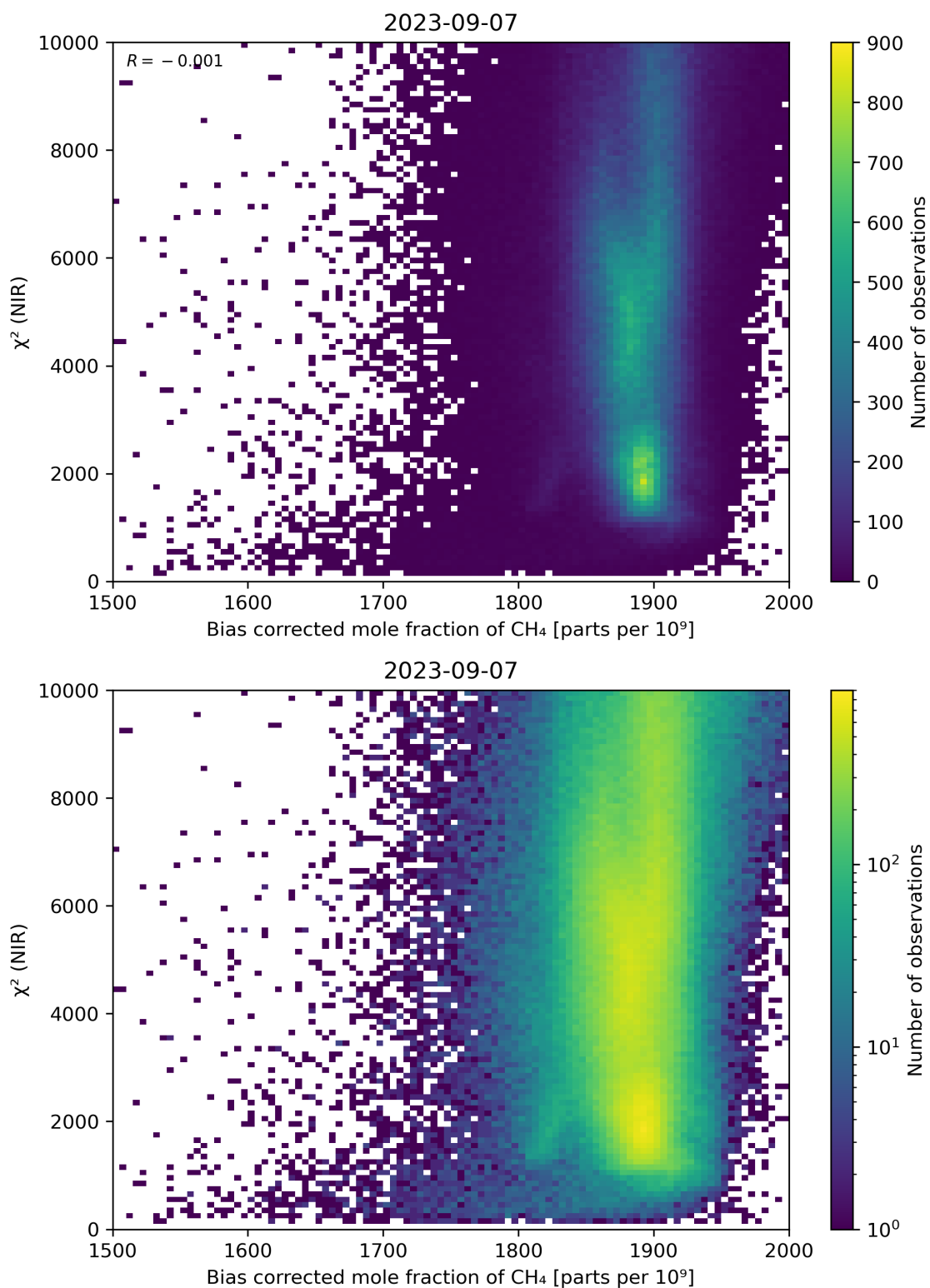
Figure 63: Scatter density plot of “Bias corrected mole fraction of CH 4 ” against “ \chi^2 (NIR)” for 2023-09-06 to 2023-09-08.
