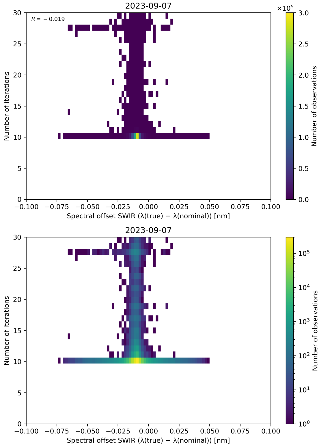
Figure 121: Scatter density plot of “Spectral offset SWIR ( \lambda(\text{true}) - \lambda(\text{nominal}) )” against “Number of iterations” for 2023-09-06 to 2023-09-08.
