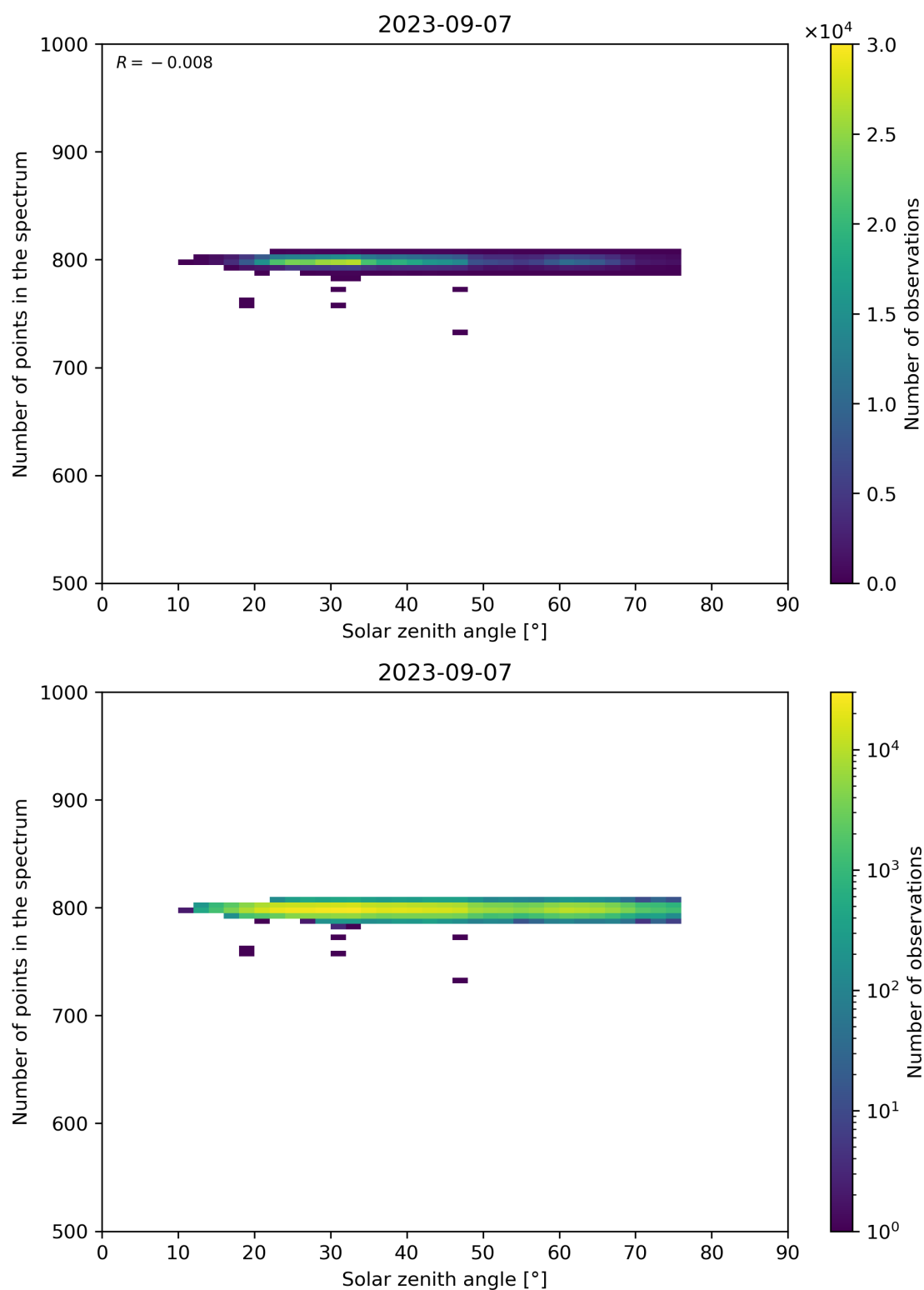
Figure 103: Scatter density plot of “Solar zenith angle” against “Number of points in the spectrum” for 2023-09-06 to 2023-09-08.
