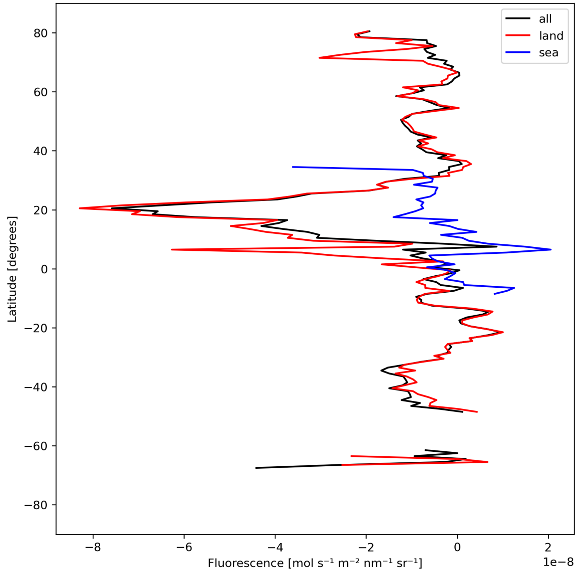
Figure 21: Zonal average of “Fluorescence” for 2023-09-06 to 2023-09-08.
