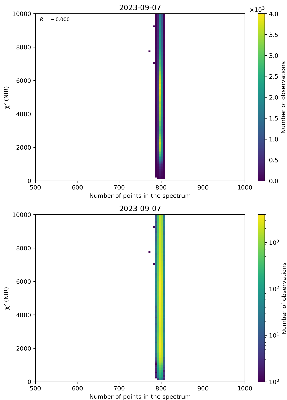
Figure 88: Scatter density plot of “Number of points in the spectrum” against “ \chi^2 (NIR)” for 2023-09-06 to 2023-09-08.
