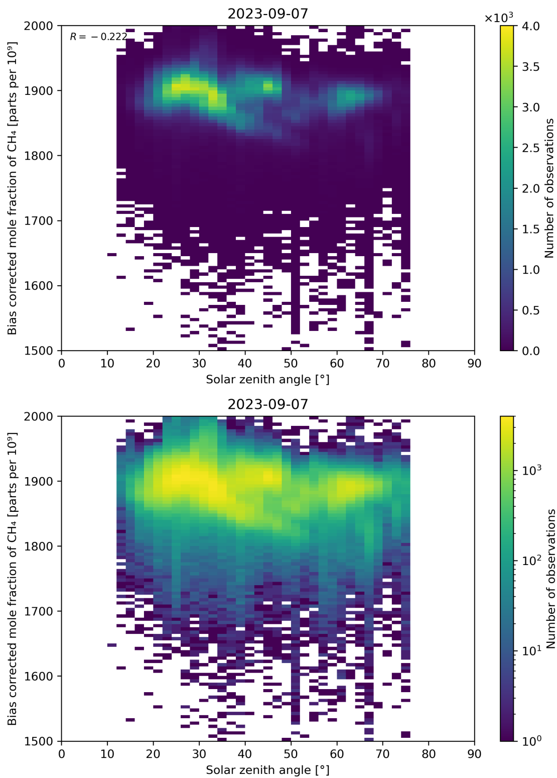
Figure 100: Scatter density plot of “Solar zenith angle” against “Bias corrected mole fraction of CH 4 ” for 2023-09-06 to 2023-09-08.
