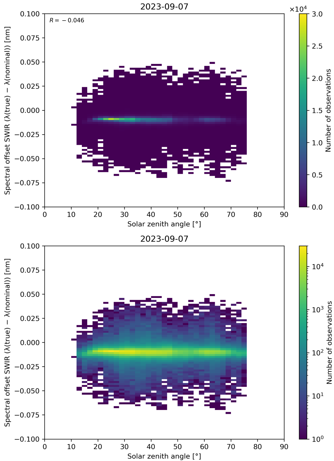
Figure 104: Scatter density plot of “Solar zenith angle” against “Spectral offset SWIR ( \lambda(\text{true}) - \lambda(\text{nominal}) )” for 2023-09-06 to 2023-09-08.
