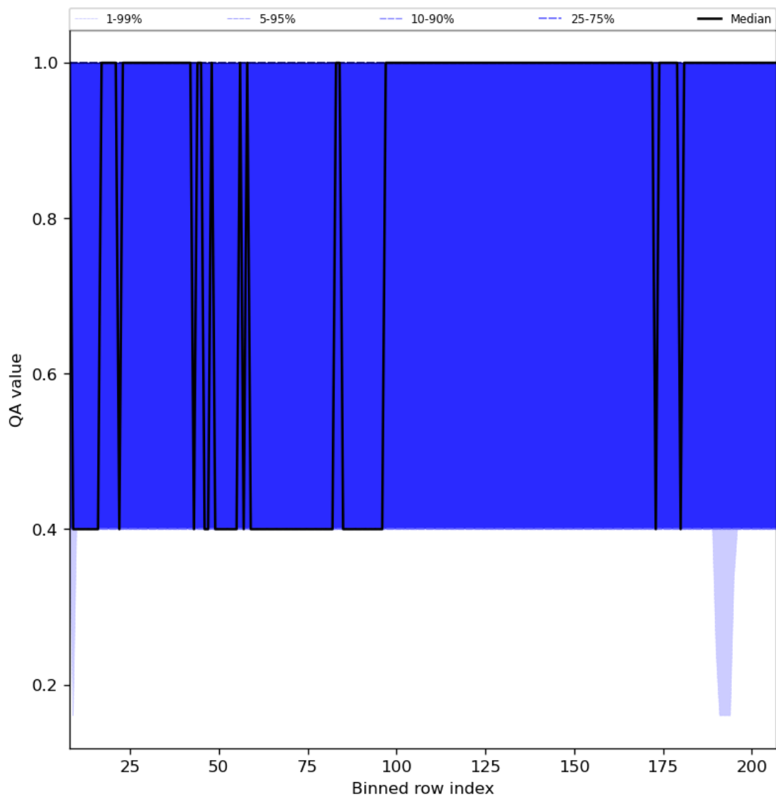
Figure 33: Along track statistics of “QA value” for 2023-09-06 to 2023-09-08
