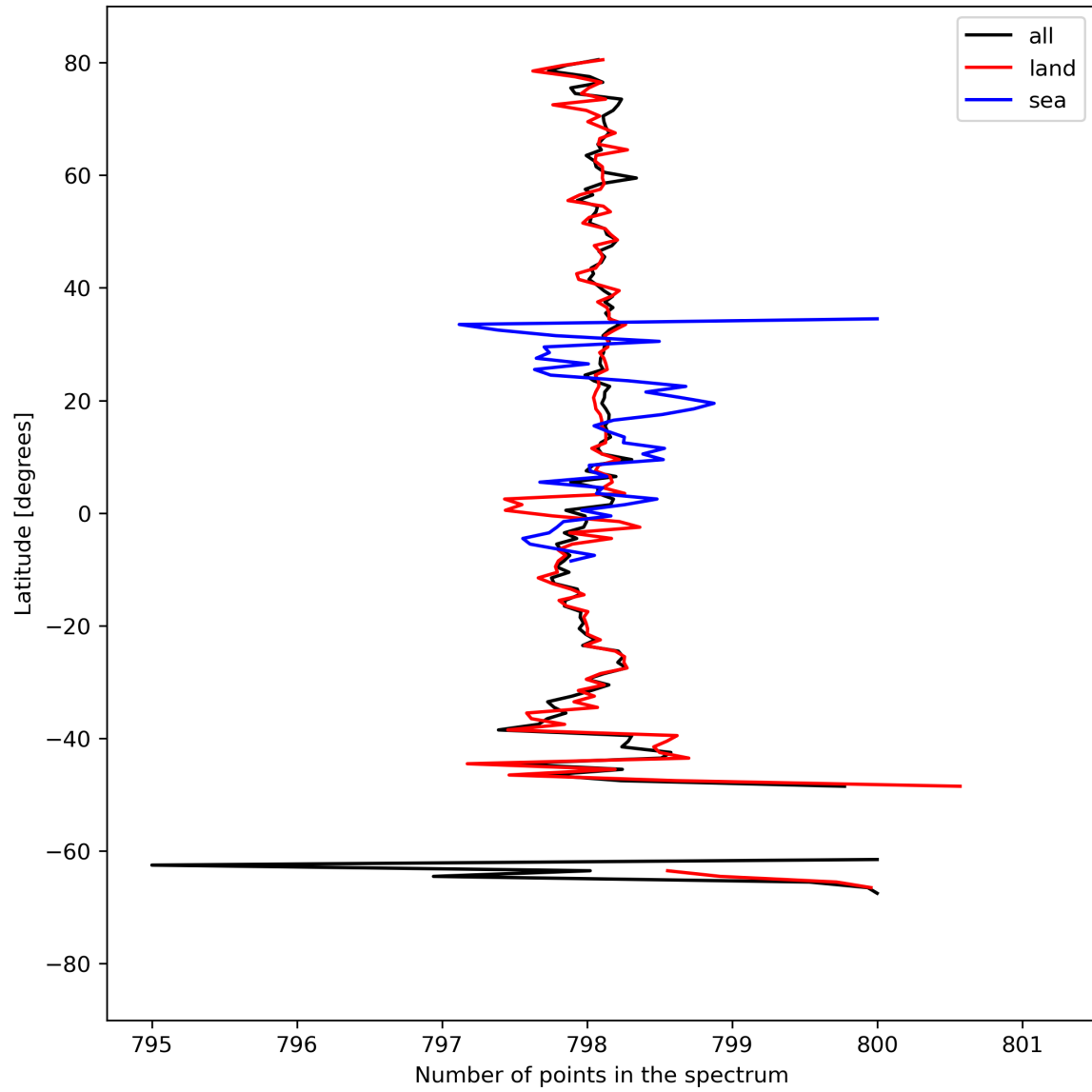
Figure 15: Zonal average of “Number of points in the spectrum” for 2023-09-06 to 2023-09-08.
