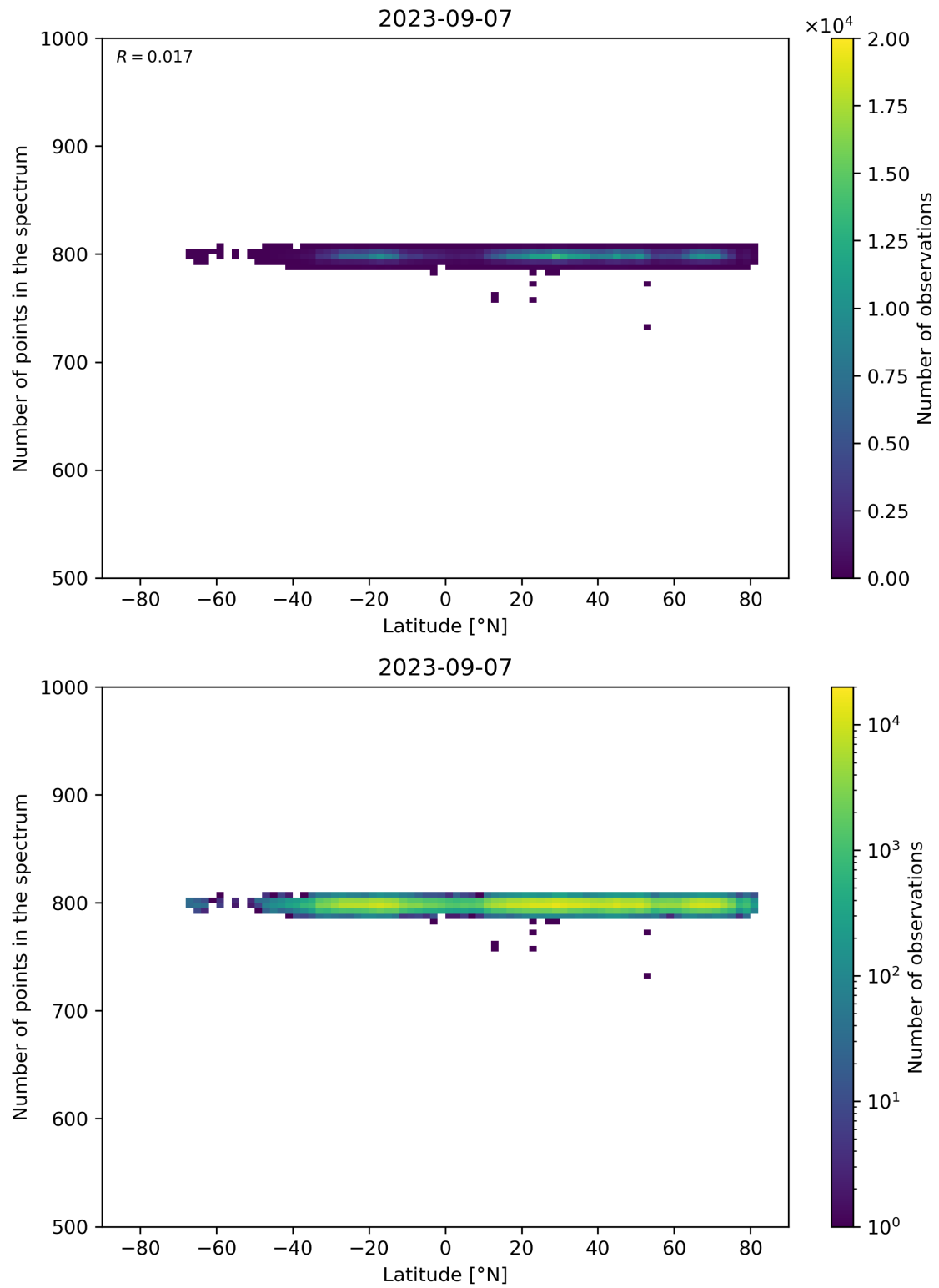
Figure 61: Scatter density plot of “Latitude” against “Number of points in the spectrum” for 2023-09-06 to 2023-09-08.
