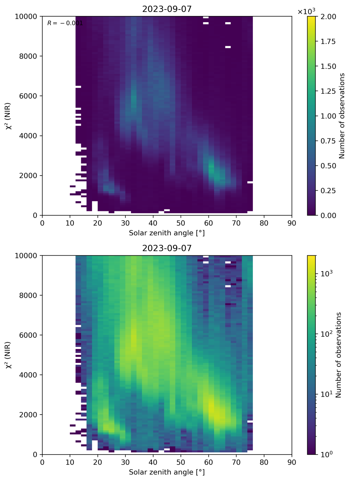
Figure 94: Scatter density plot of “Solar zenith angle” against “ \chi^2 (NIR)” for 2023-09-06 to 2023-09-08.
