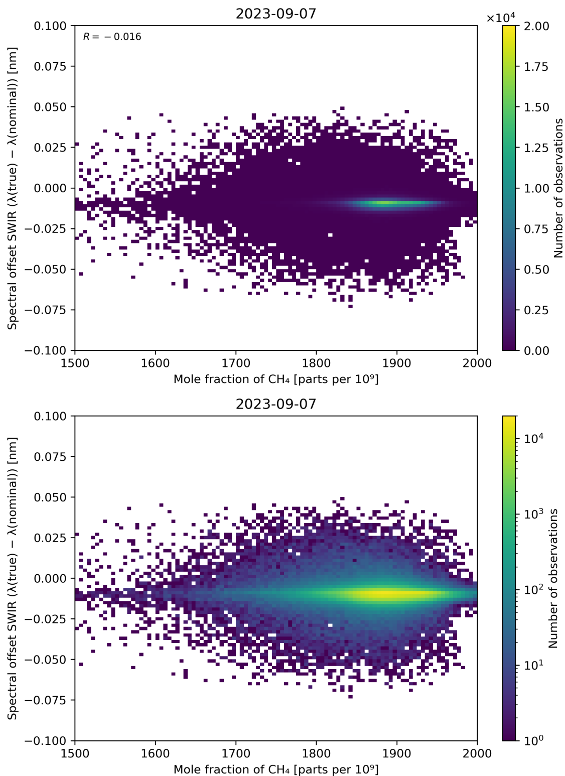
Figure 86: Scatter density plot of “Mole fraction of CH 4 ” against “Spectral offset SWIR ( \lambda(\text{true}) - \lambda(\text{nominal}) )” for 2023-09-06 to 2023-09-08.
