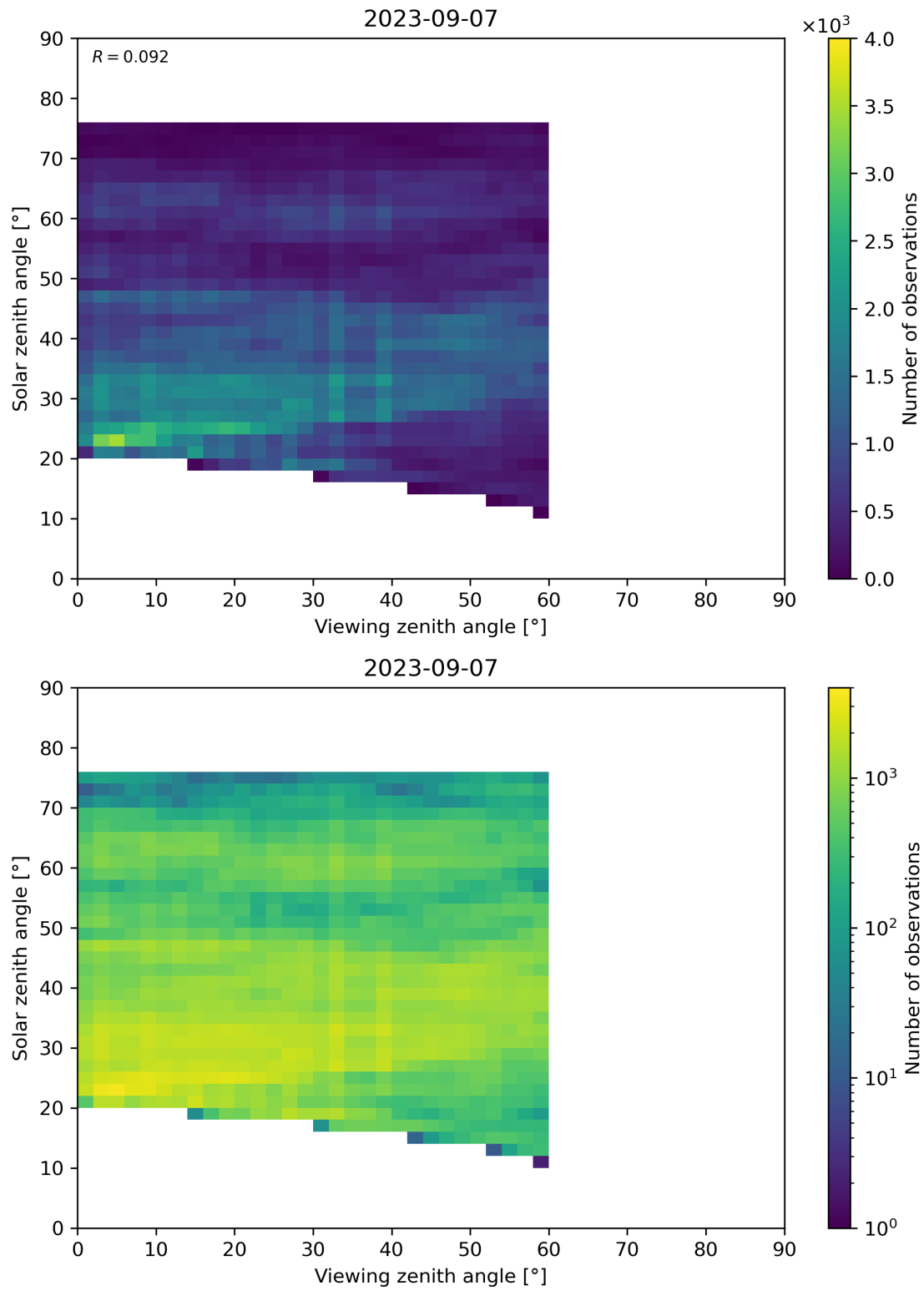
Figure 115: Scatter density plot of “Viewing zenith angle” against “Solar zenith angle” for 2023-09-06 to 2023-09-08.
