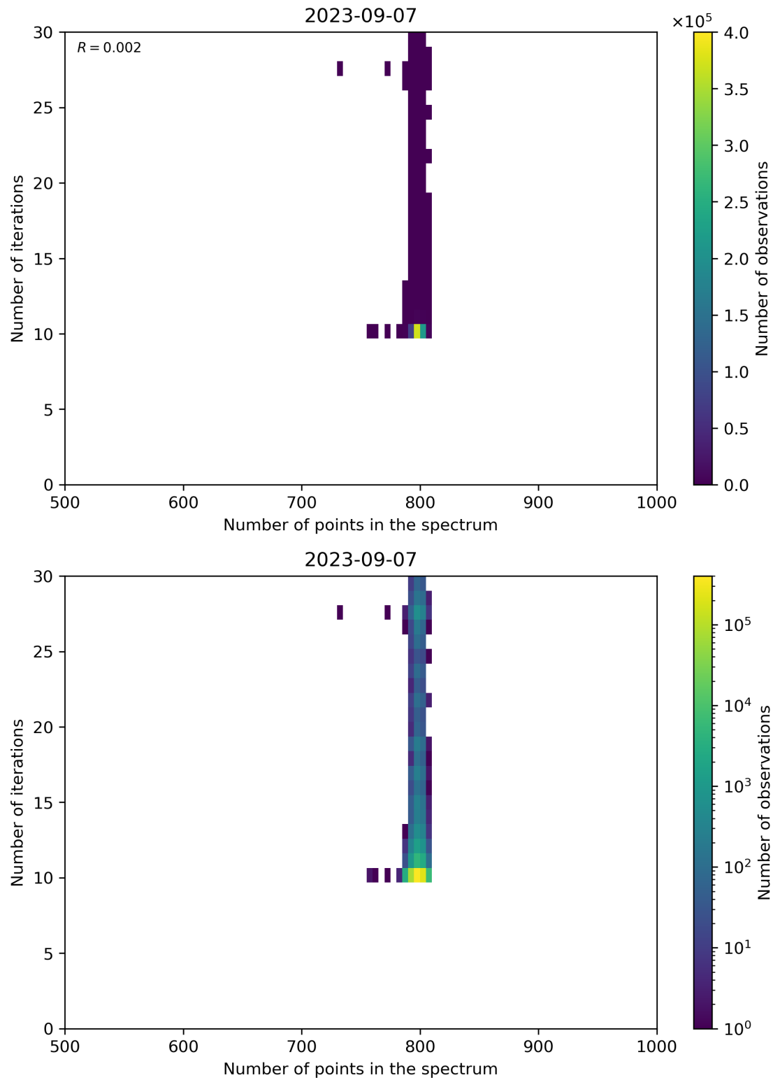
Figure 92: Scatter density plot of “Number of points in the spectrum” against “Number of iterations” for 2023-09-06 to 2023-09-08.
