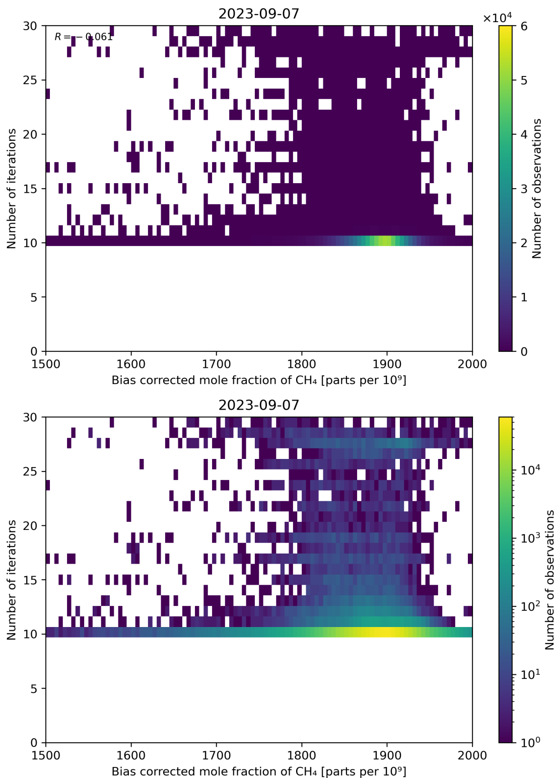
Figure 67: Scatter density plot of “Bias corrected mole fraction of CH 4 ” against “Number of iterations” for 2023-09-06 to 2023-09-08.
