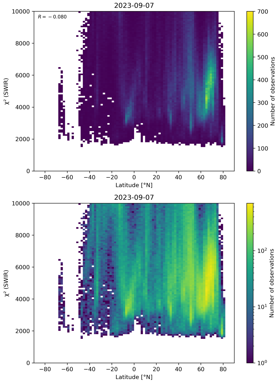
Figure 54: Scatter density plot of “Latitude” against “ \chi^2 (SWIR)” for 2023-09-06 to 2023-09-08.
