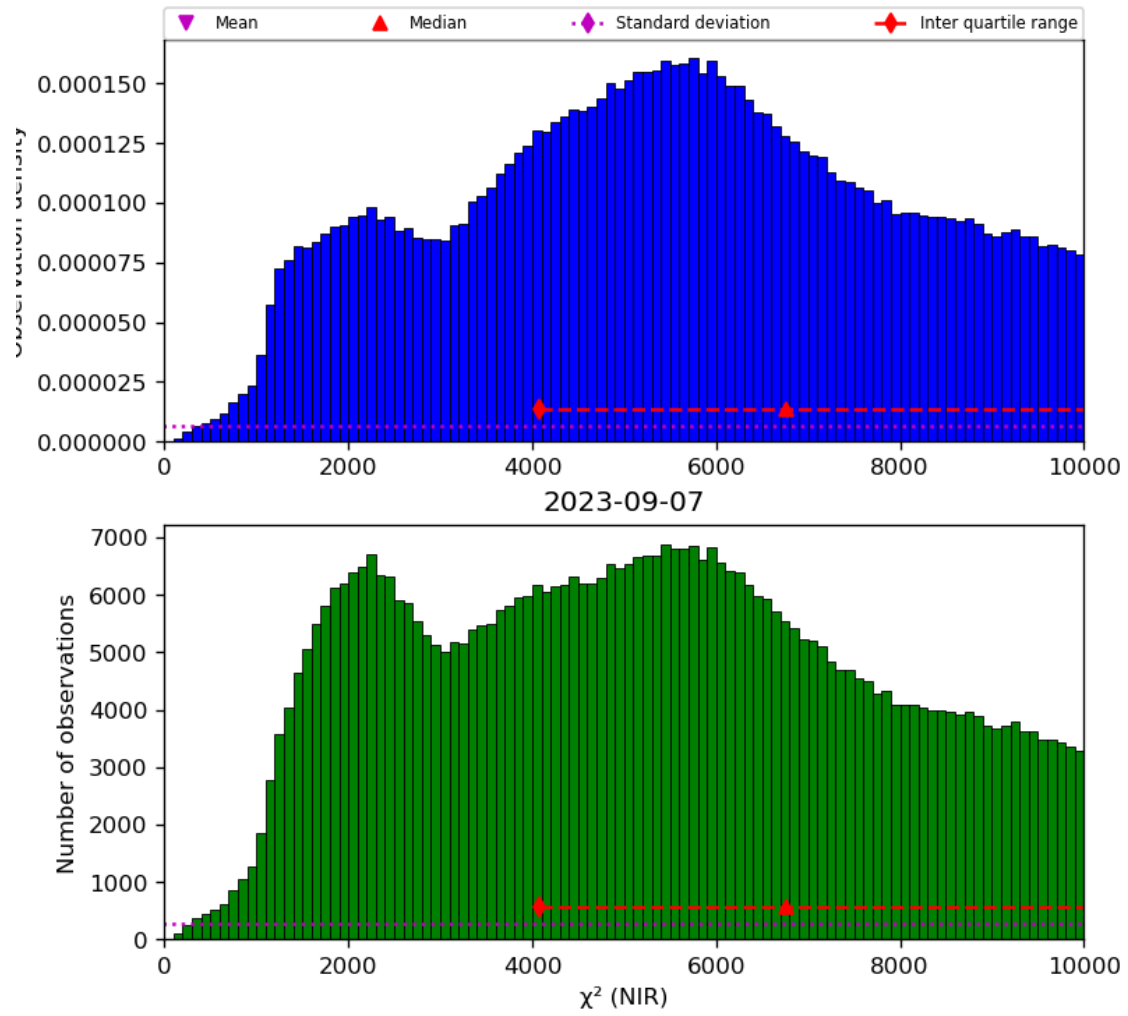
Figure 29: Histogram of “ \chi^2 (NIR)” for 2023-09-06 to 2023-09-08
