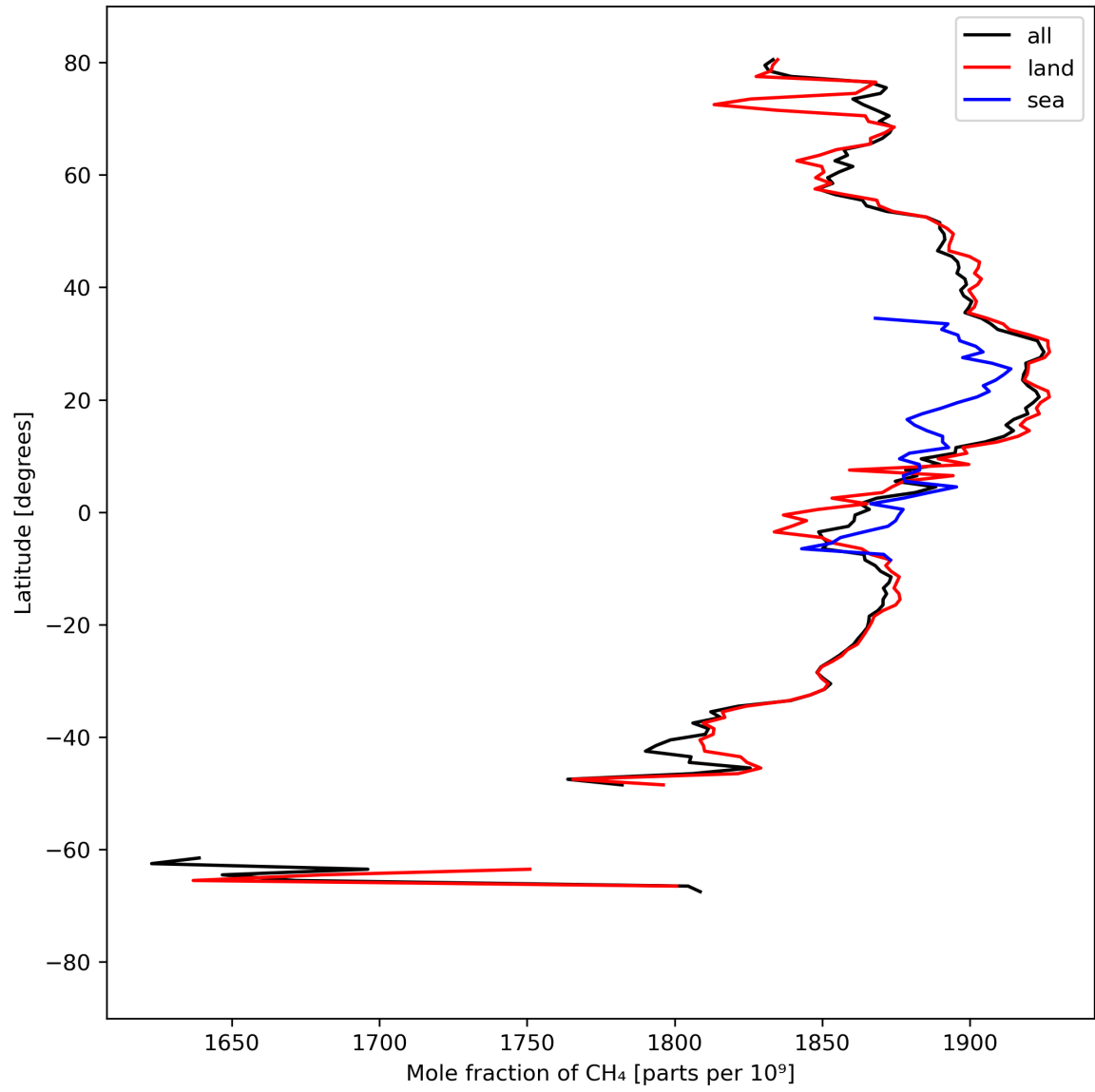
Figure 12: Zonal average of “Mole fraction of CH 4 ” for 2023-09-06 to 2023-09-08.
