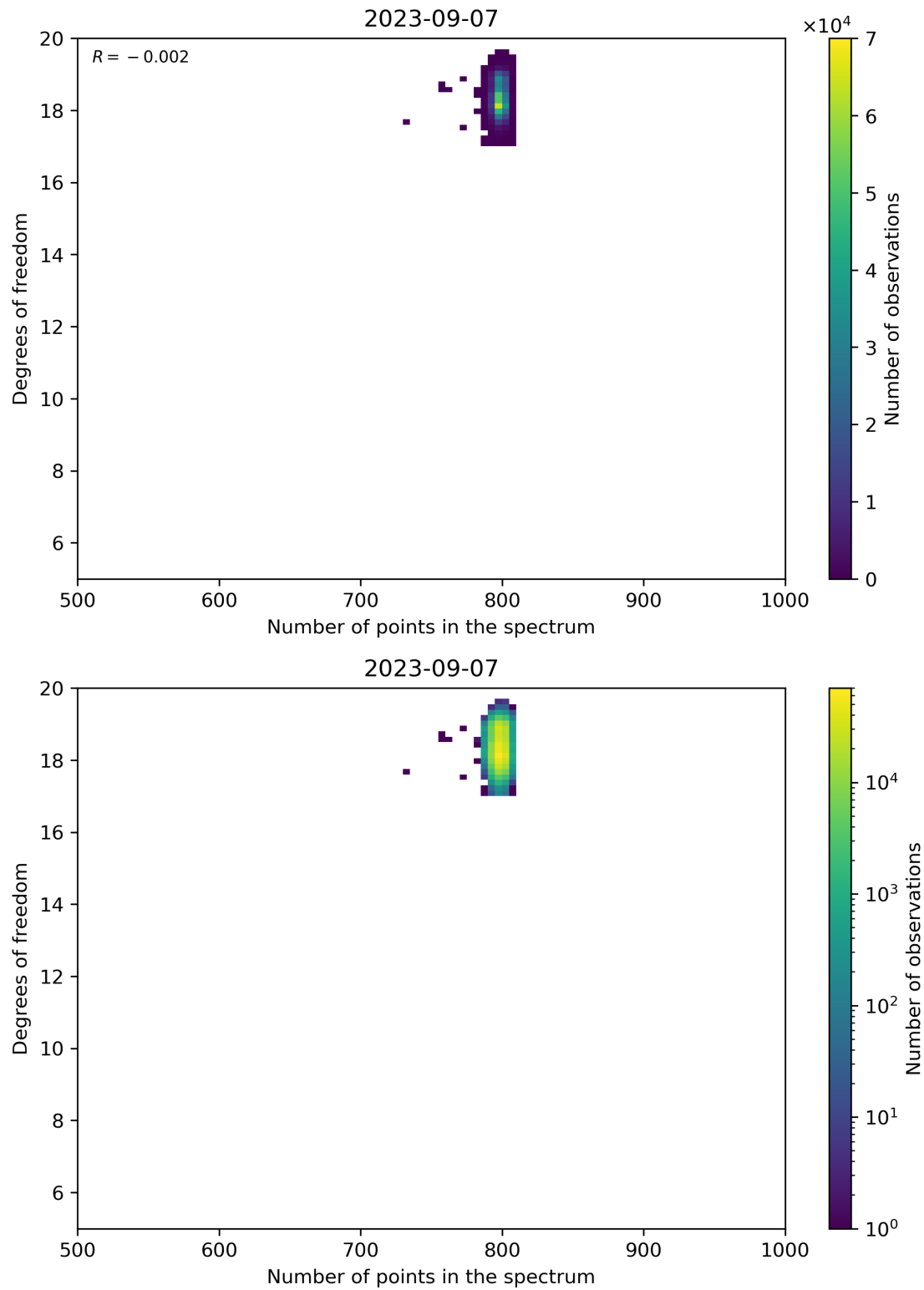
Figure 90: Scatter density plot of “Number of points in the spectrum” against “Degrees of freedom” for 2023-09-06 to 2023-09-08.
