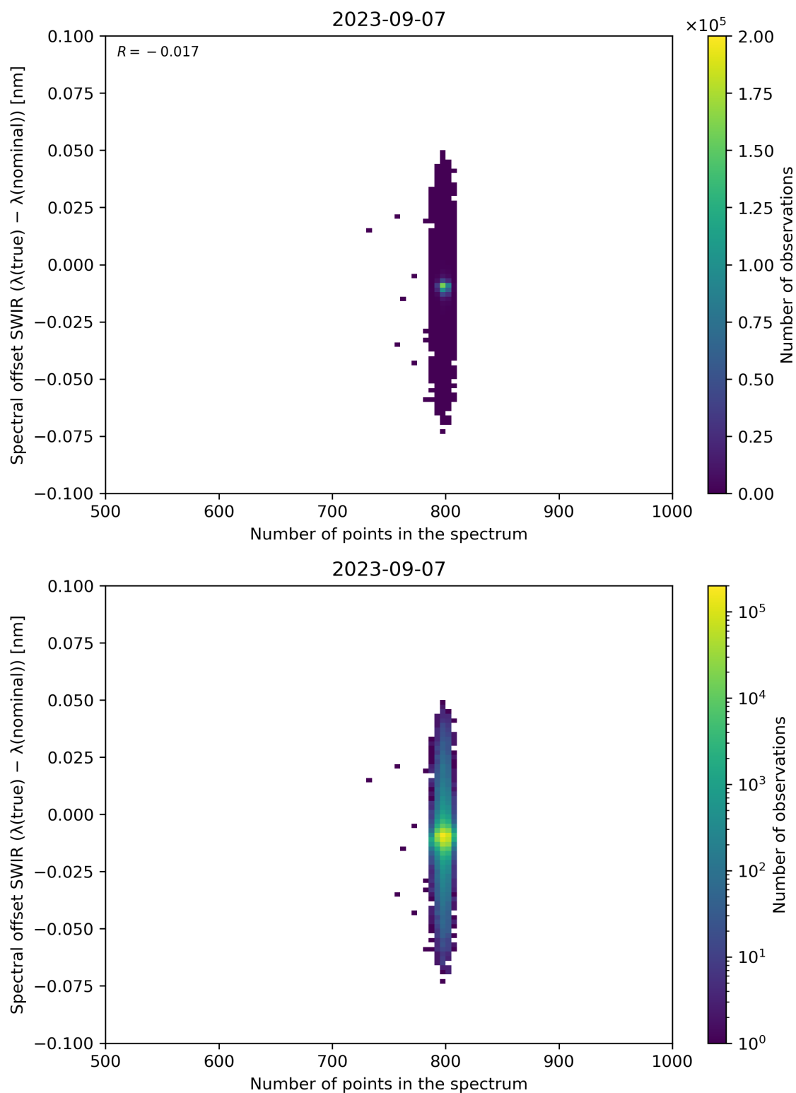
Figure 93: Scatter density plot of “Number of points in the spectrum” against “Spectral offset SWIR ( \lambda(\text{true}) - \lambda(\text{nominal}) )” for 2023-09-06 to 2023-09-08.
