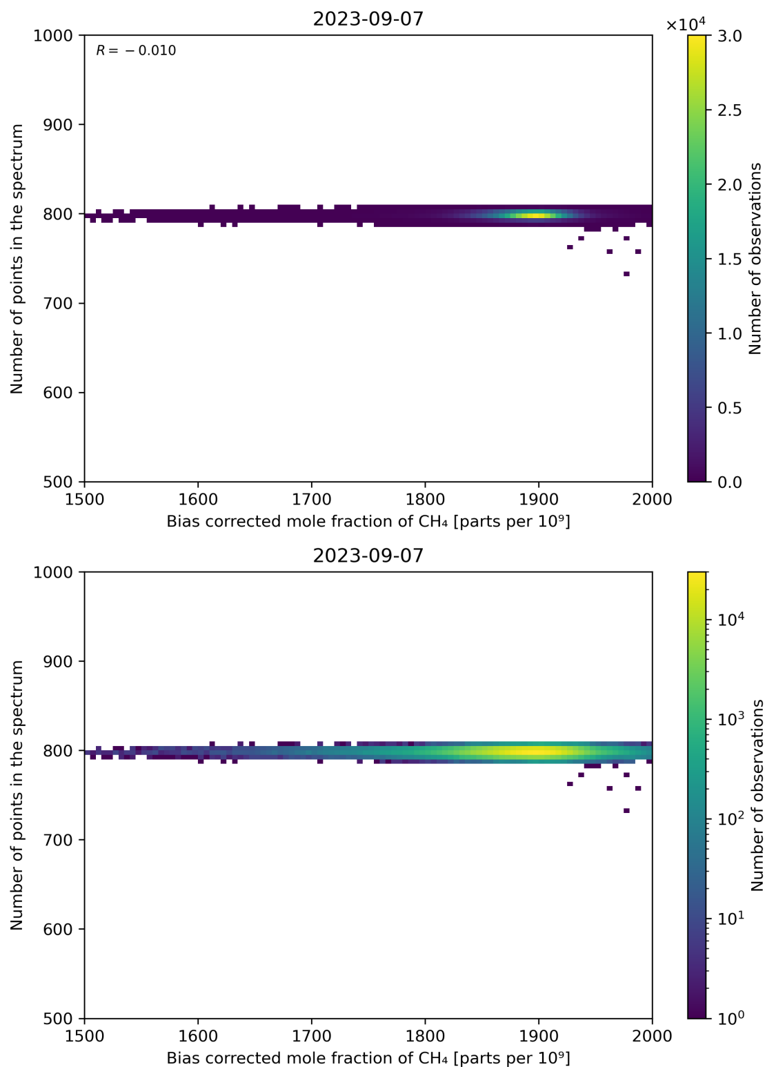
Figure 68: Scatter density plot of “Bias corrected mole fraction of CH 4 ” against “Number of points in the spectrum” for 2023-09-06 to 2023-09-08.
