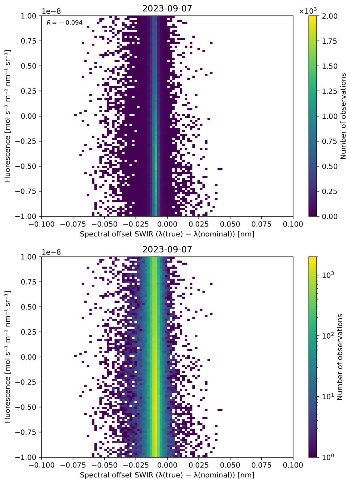
Figure 120: Scatter density plot of “Spectral offset SWIR ( \lambda(\text{true}) - \lambda(\text{nominal}) )” against “Fluorescence” for 2023-09-06 to 2023-09-08.
