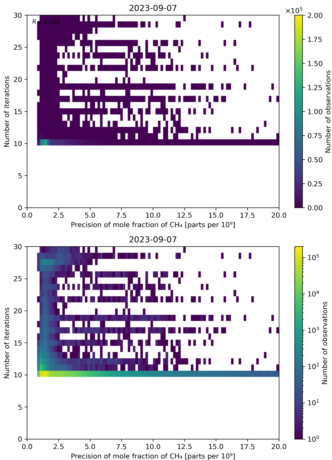
Figure 83: Scatter density plot of “Precision of mole fraction of CH 4 ” against “Number of iterations” for 2023-09-06 to 2023-09-08.
