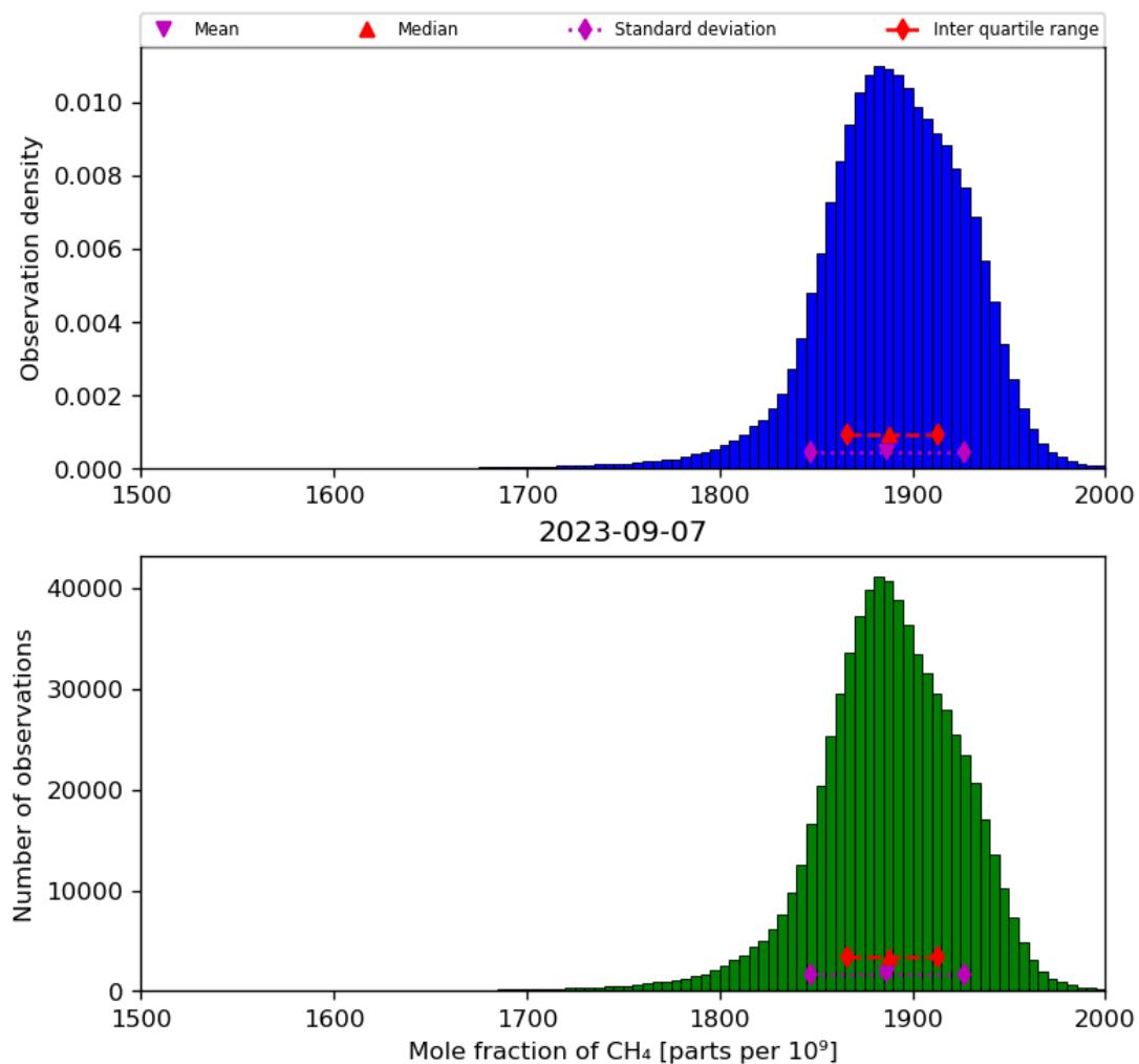
Figure 23: Histogram of “Mole fraction of CH 4 ” for 2023-09-06 to 2023-09-08
