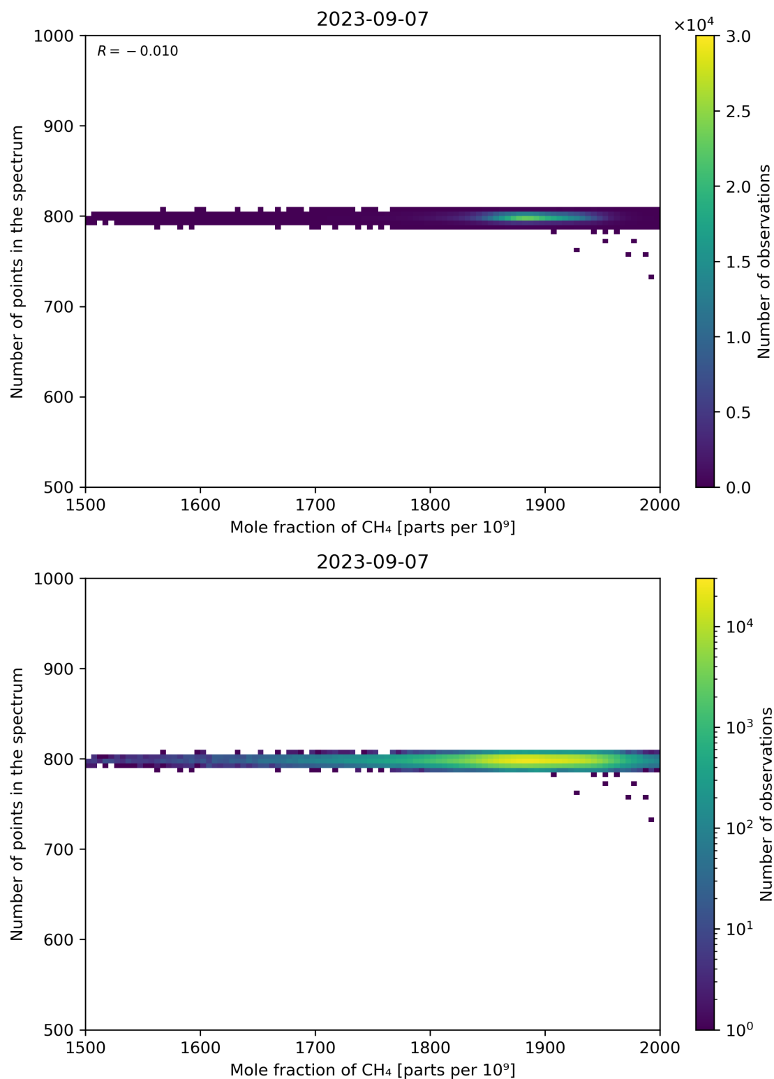
Figure 77: Scatter density plot of “Mole fraction of CH 4 ” against “Number of points in the spectrum” for 2023-09-06 to 2023-09-08.
