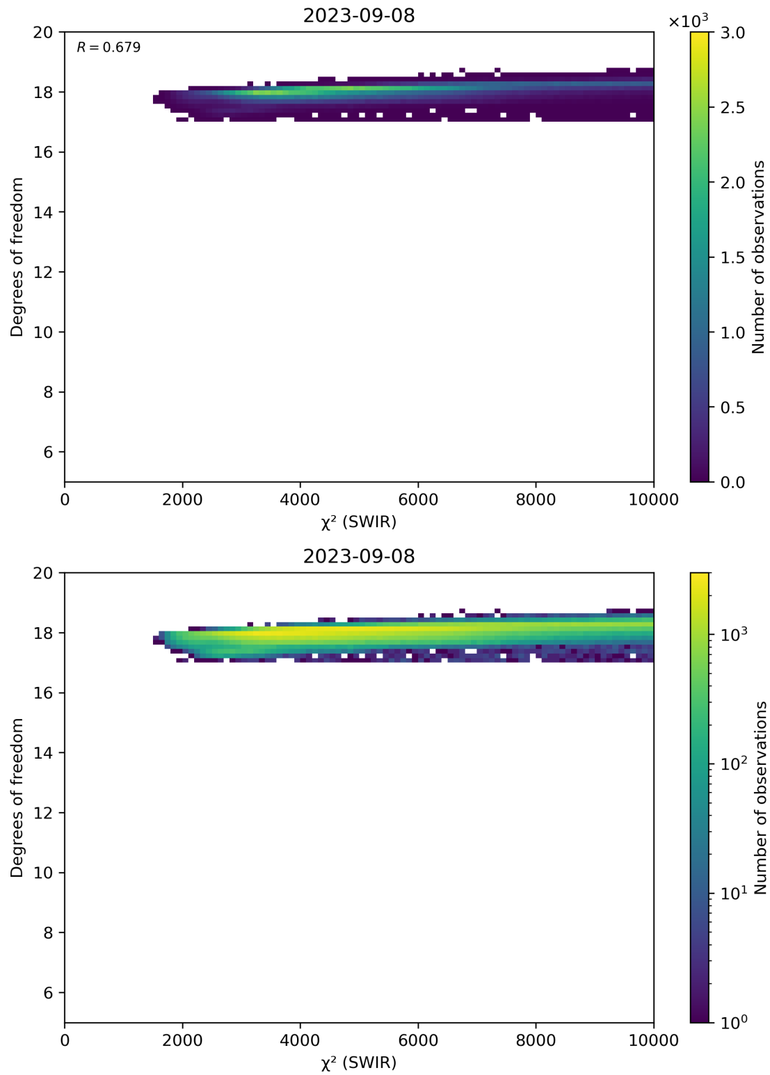
Figure 48: Scatter density plot of “ \chi^2 (SWIR)” against “Degrees of freedom” for 2023-09-07 to 2023-09-09.
