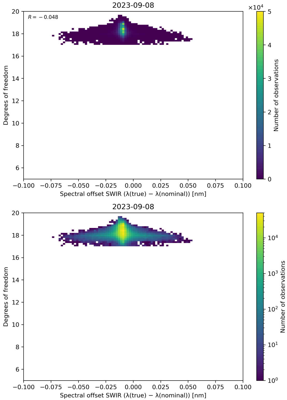
Figure 119: Scatter density plot of “Spectral offset SWIR ( \lambda(\text{true}) - \lambda(\text{nominal}) )” against “Degrees of freedom” for 2023-09-07 to 2023-09-09.
