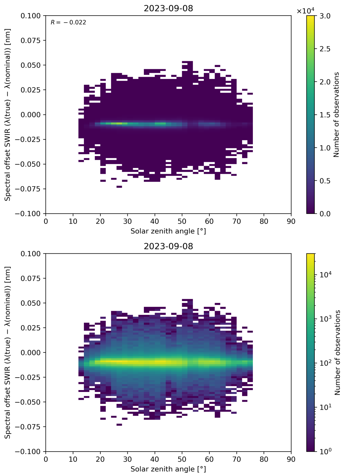
Figure 104: Scatter density plot of “Solar zenith angle” against “Spectral offset SWIR ( \lambda(\text{true}) - \lambda(\text{nominal}) )” for 2023-09-07 to 2023-09-09.
