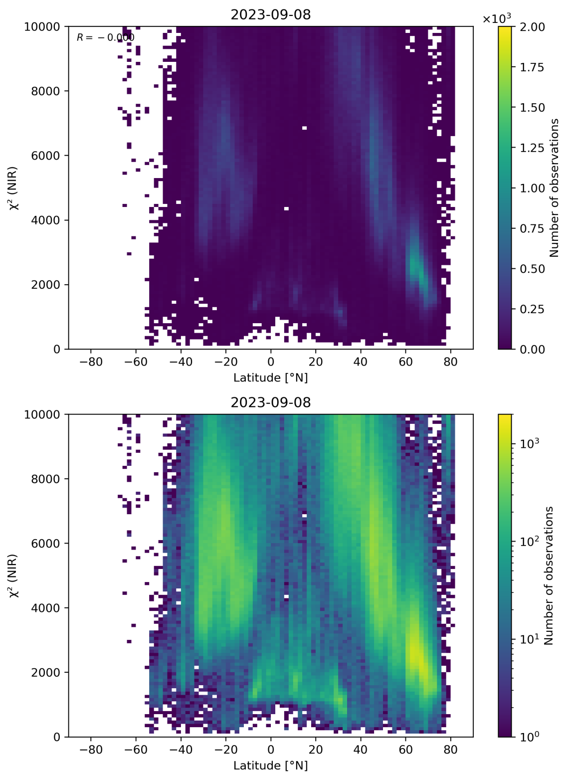
Figure 53: Scatter density plot of “Latitude” against “ \chi^2 (NIR)” for 2023-09-07 to 2023-09-09.
