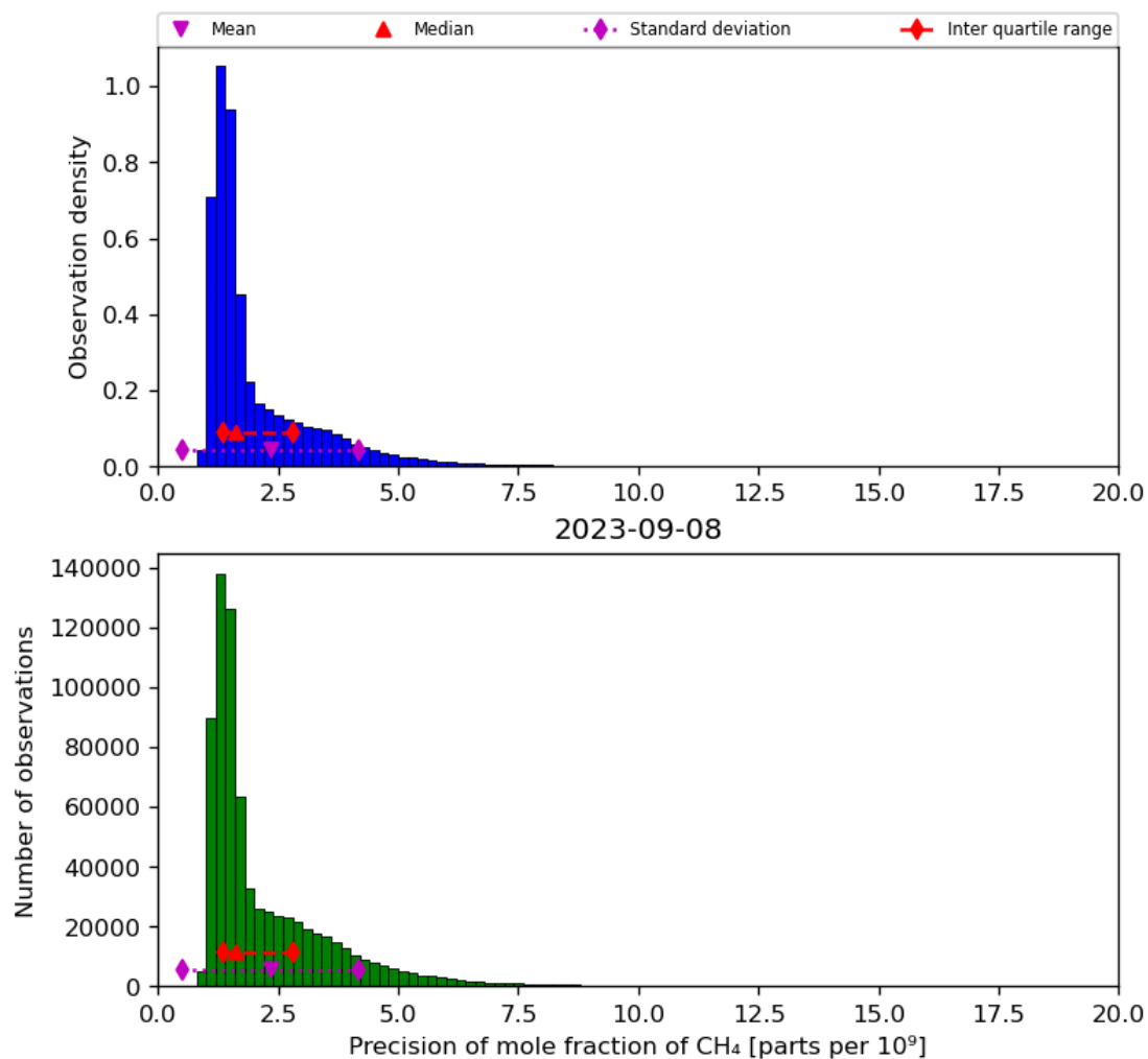
Figure 24: Histogram of “Precision of mole fraction of CH 4 ” for 2023-09-07 to 2023-09-09
