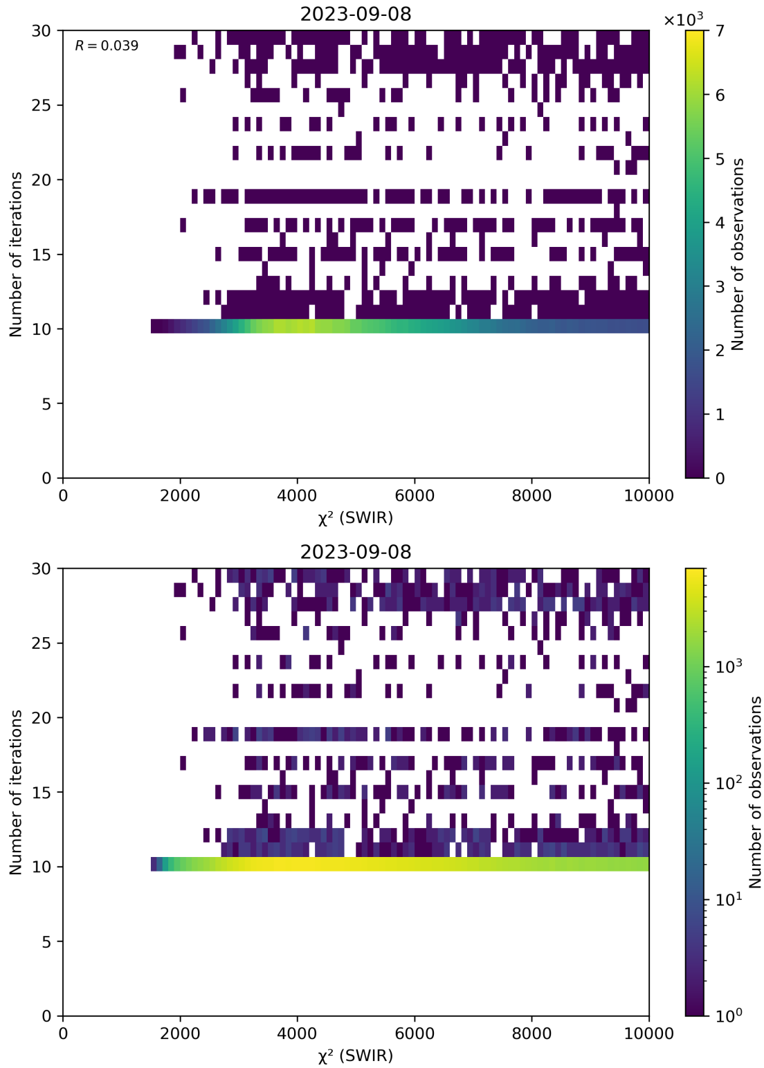
Figure 50: Scatter density plot of “ \chi^2 (SWIR)” against “Number of iterations” for 2023-09-07 to 2023-09-09.
