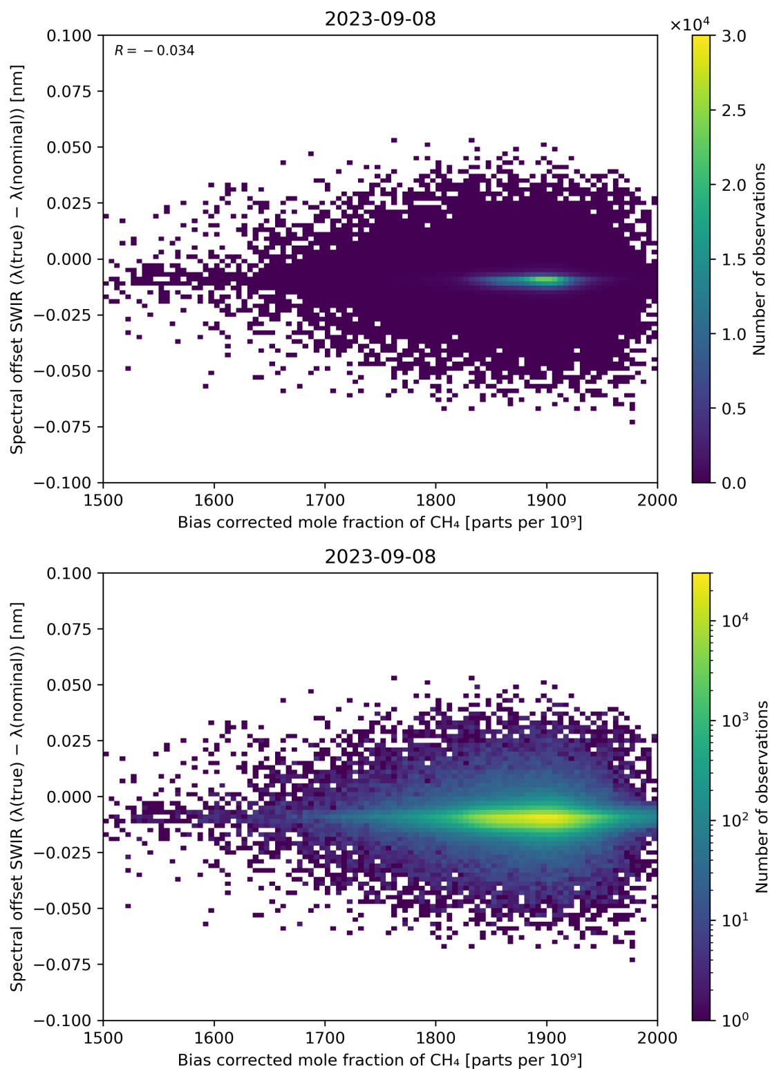
Figure 69: Scatter density plot of “Bias corrected mole fraction of CH 4 ” against “Spectral offset SWIR ( \lambda(\text{true}) - \lambda(\text{nominal}) )” for 2023-09-07 to 2023-09-09.
