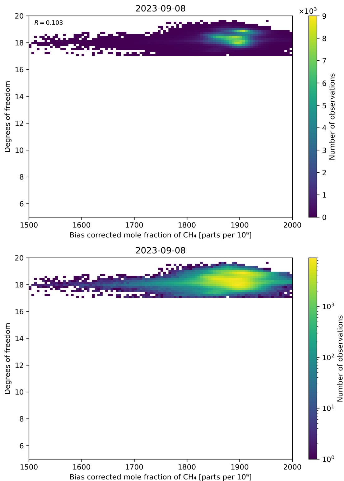
Figure 65: Scatter density plot of “Bias corrected mole fraction of CH 4 ” against “Degrees of freedom” for 2023-09-07 to 2023-09-09.
