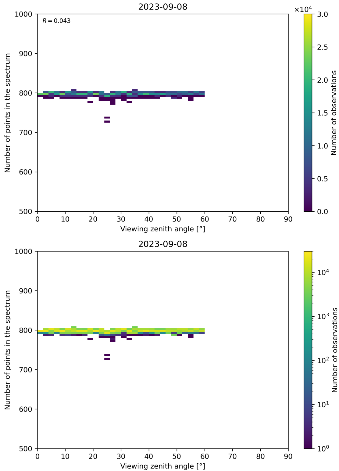
Figure 114: Scatter density plot of “Viewing zenith angle” against “Number of points in the spectrum” for 2023-09-07 to 2023-09-09.
