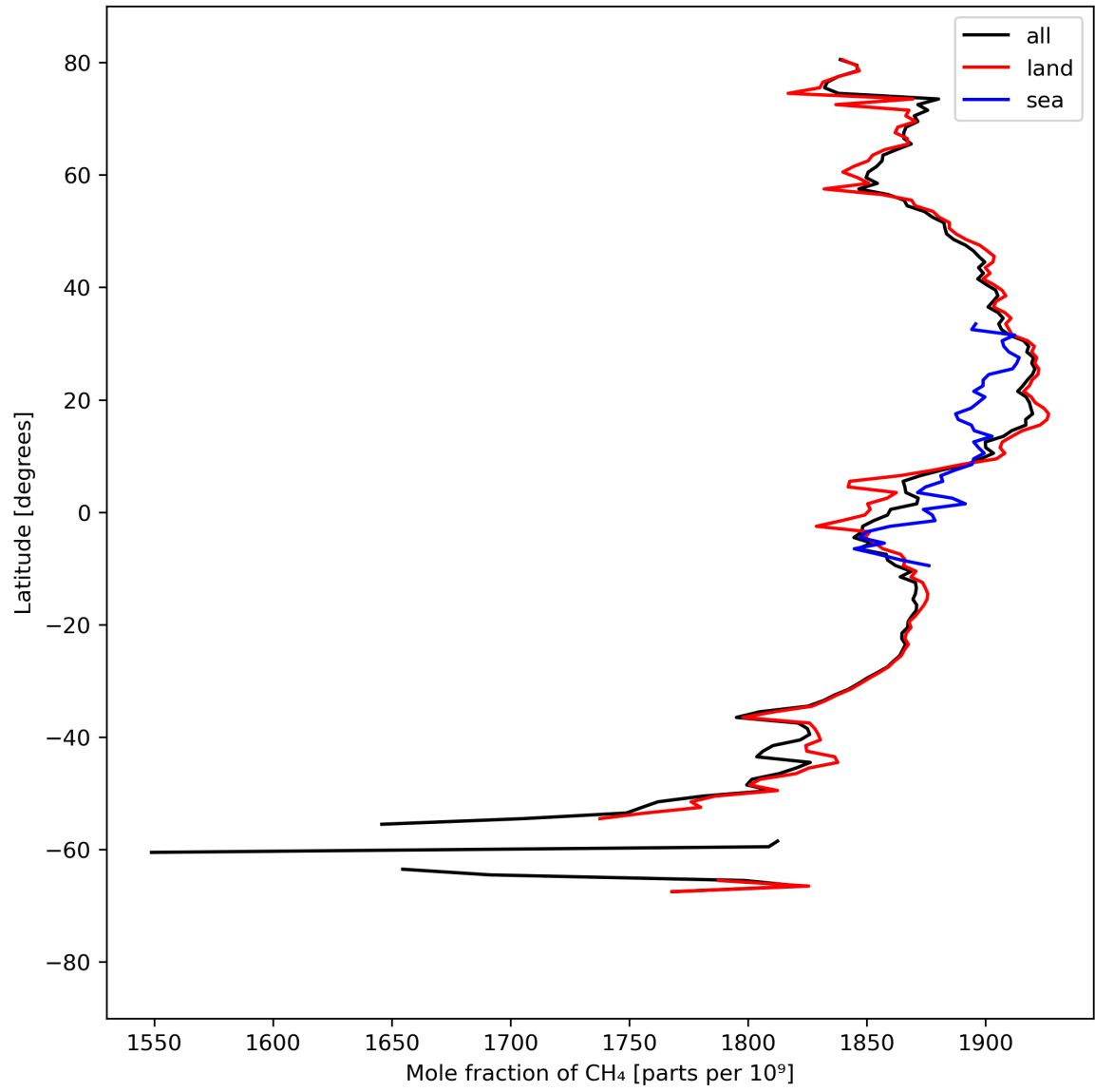
Figure 12: Zonal average of “Mole fraction of \text{CH}_4 ” for 2023-09-07 to 2023-09-09.
