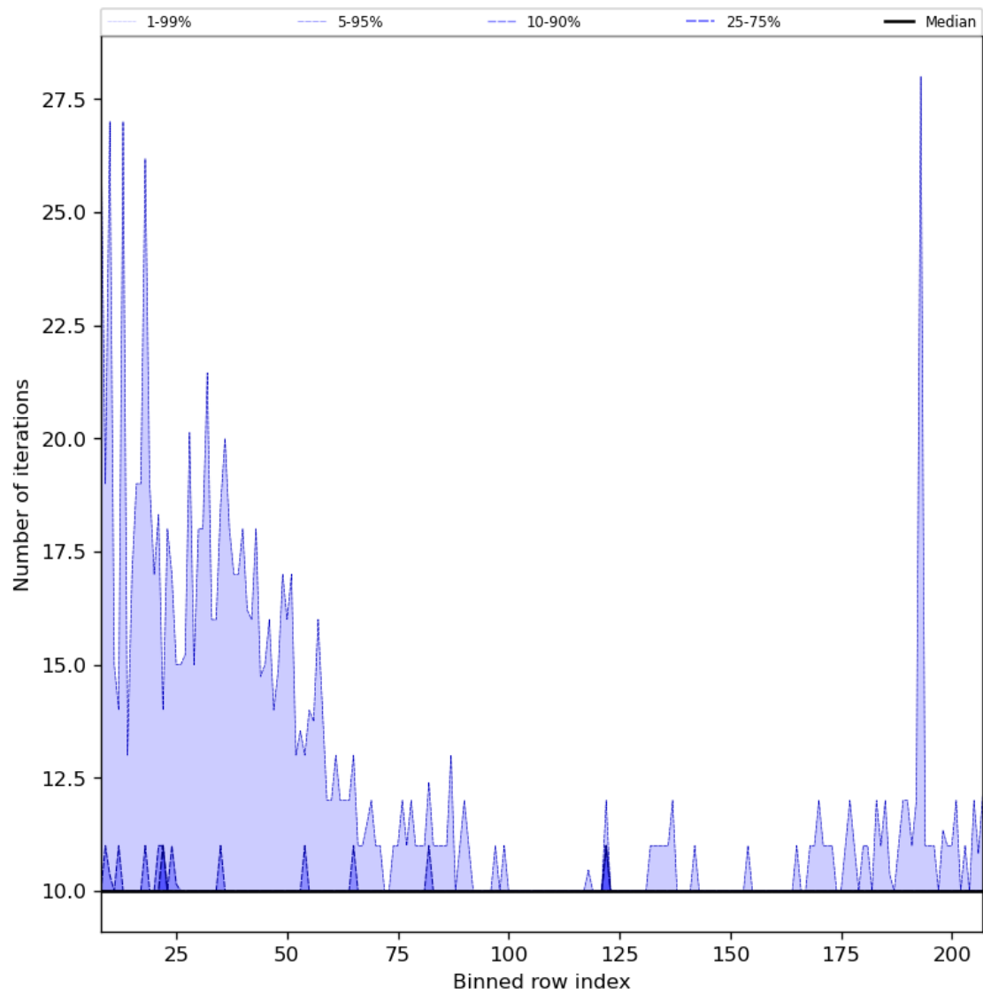
Figure 42: Along track statistics of “Number of iterations” for 2023-09-07 to 2023-09-09
