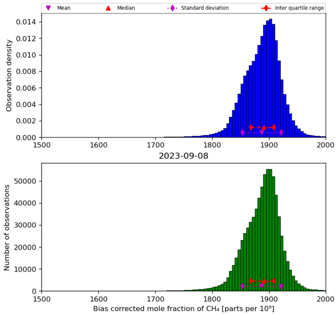
Figure 25: Histogram of “Bias corrected mole fraction of CH 4 ” for 2023-09-07 to 2023-09-09
