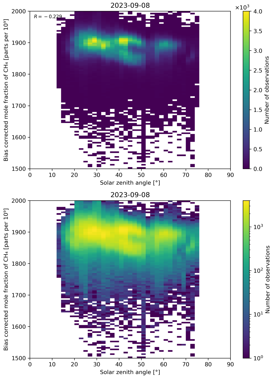
Figure 100: Scatter density plot of “Solar zenith angle” against “Bias corrected mole fraction of CH 4 ” for 2023-09-07 to 2023-09-09.
