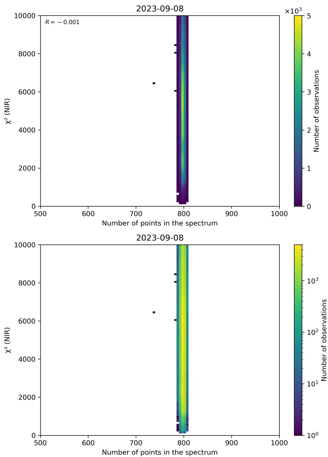
Figure 88: Scatter density plot of “Number of points in the spectrum” against “ \chi^2 (NIR)” for 2023-09-07 to 2023-09-09.
