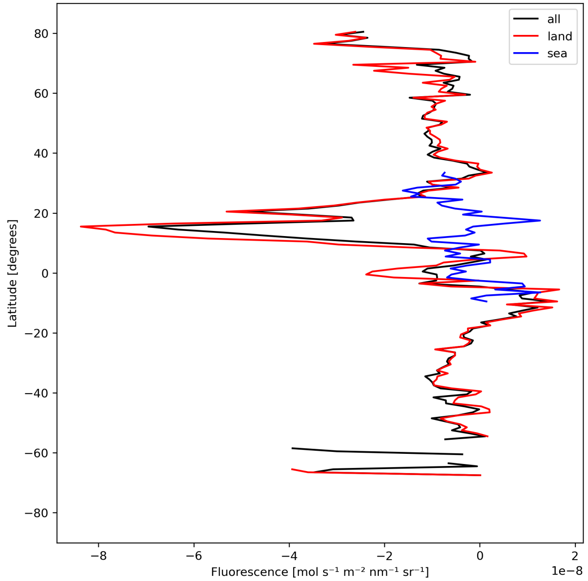
Figure 21: Zonal average of “Fluorescence” for 2023-09-07 to 2023-09-09.
