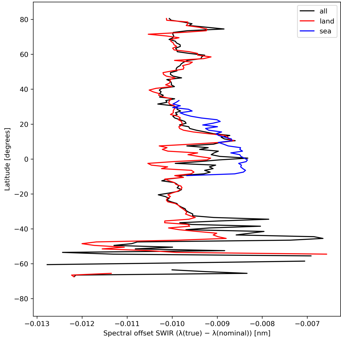
Figure 16: Zonal average of “Spectral offset SWIR ( \lambda(\text{true}) - \lambda(\text{nominal}) )” for 2023-09-07 to 2023-09-09.
