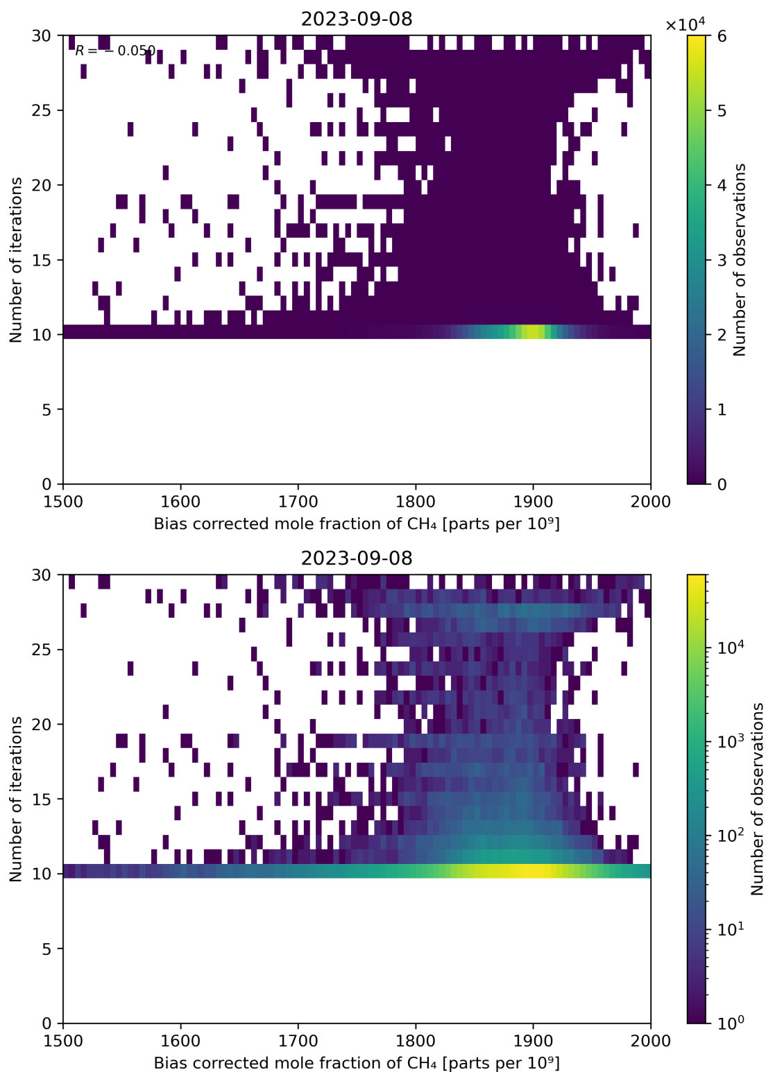
Figure 67: Scatter density plot of “Bias corrected mole fraction of CH 4 ” against “Number of iterations” for 2023-09-07 to 2023-09-09.
