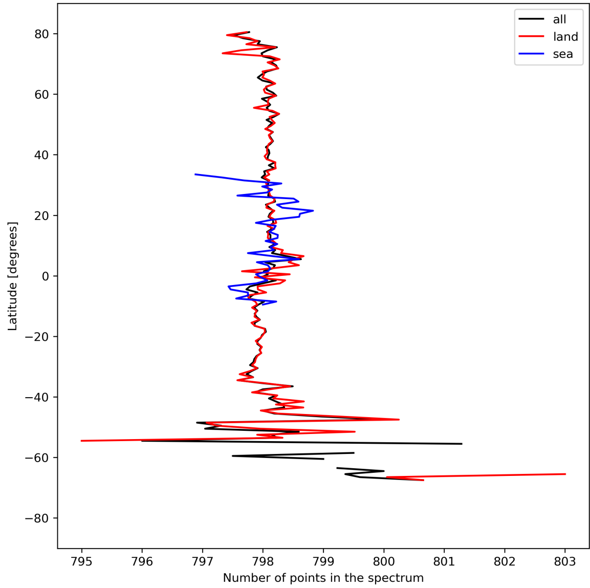
Figure 15: Zonal average of “Number of points in the spectrum” for 2023-09-07 to 2023-09-09.
