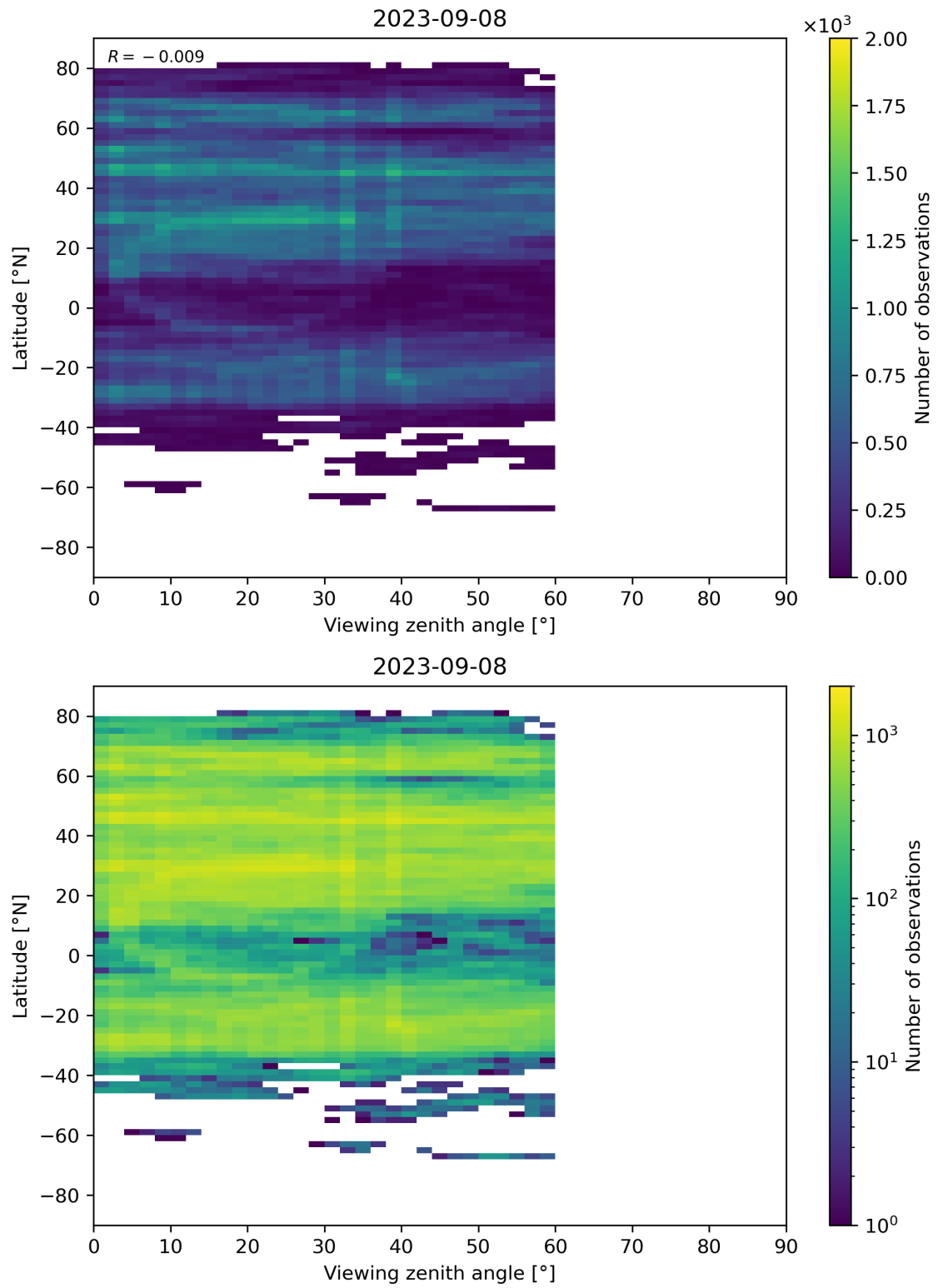
Figure 109: Scatter density plot of “Viewing zenith angle” against “Latitude” for 2023-09-07 to 2023-09-09.
