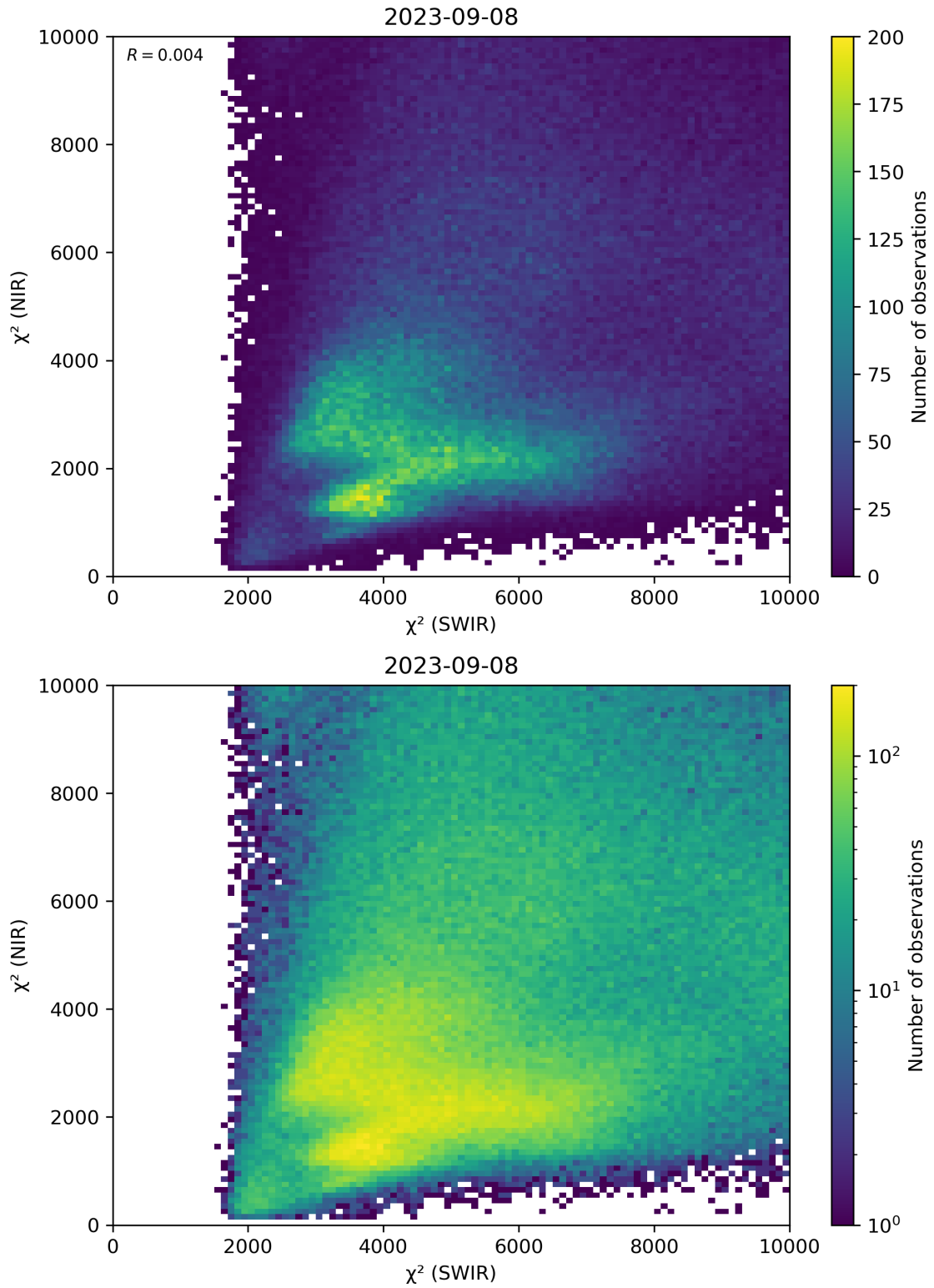
Figure 47: Scatter density plot of “ \chi^2 (SWIR)” against “ \chi^2 (NIR)” for 2023-09-07 to 2023-09-09.
