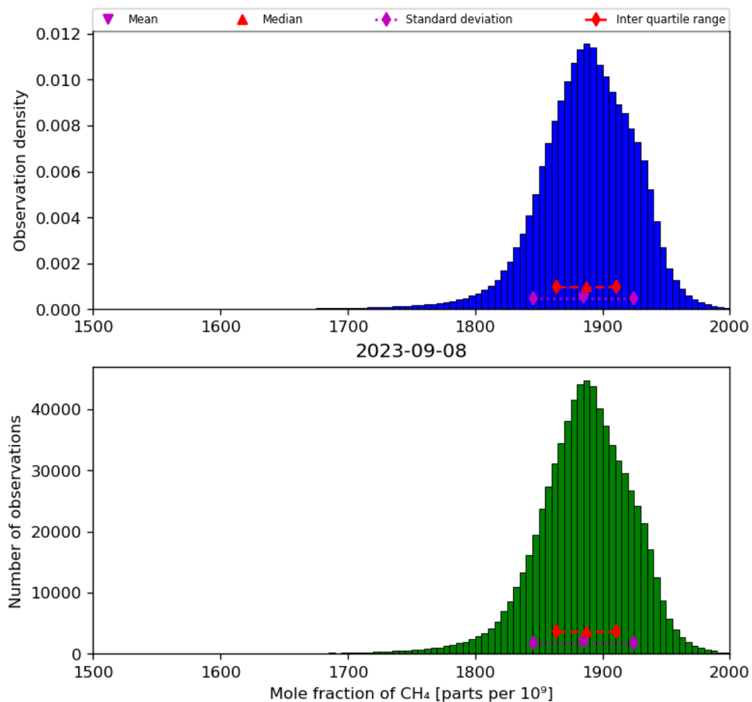
Figure 23: Histogram of “Mole fraction of CH 4 ” for 2023-09-07 to 2023-09-09
