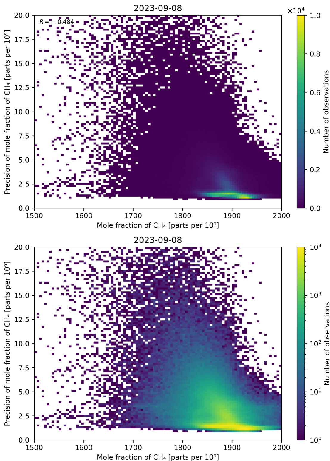
Figure 75: Scatter density plot of “Mole fraction of CH 4 ” against “Precision of mole fraction of CH 4 ” for 2023-09-07 to 2023-09-09.
