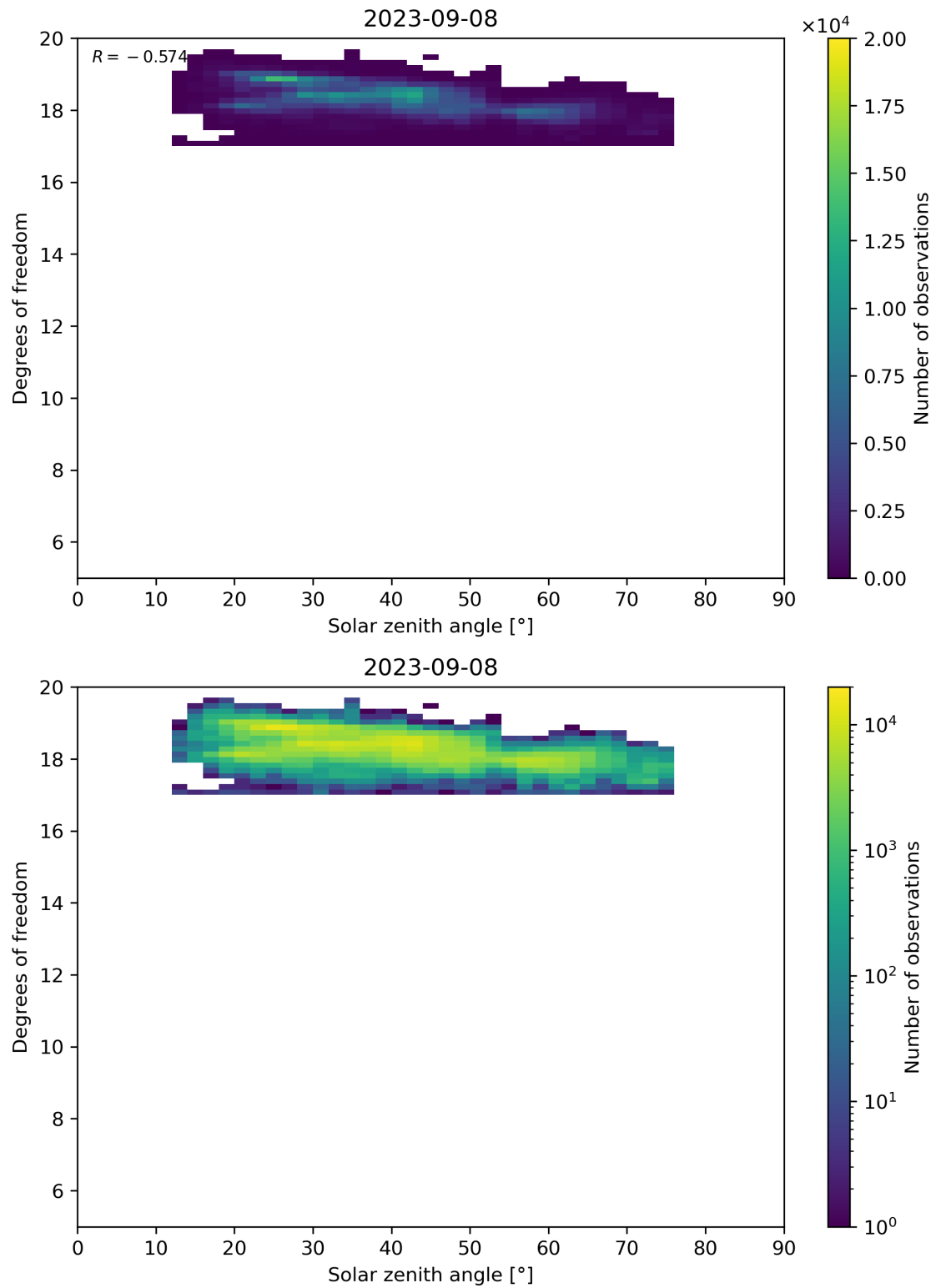
Figure 96: Scatter density plot of “Solar zenith angle” against “Degrees of freedom” for 2023-09-07 to 2023-09-09.
