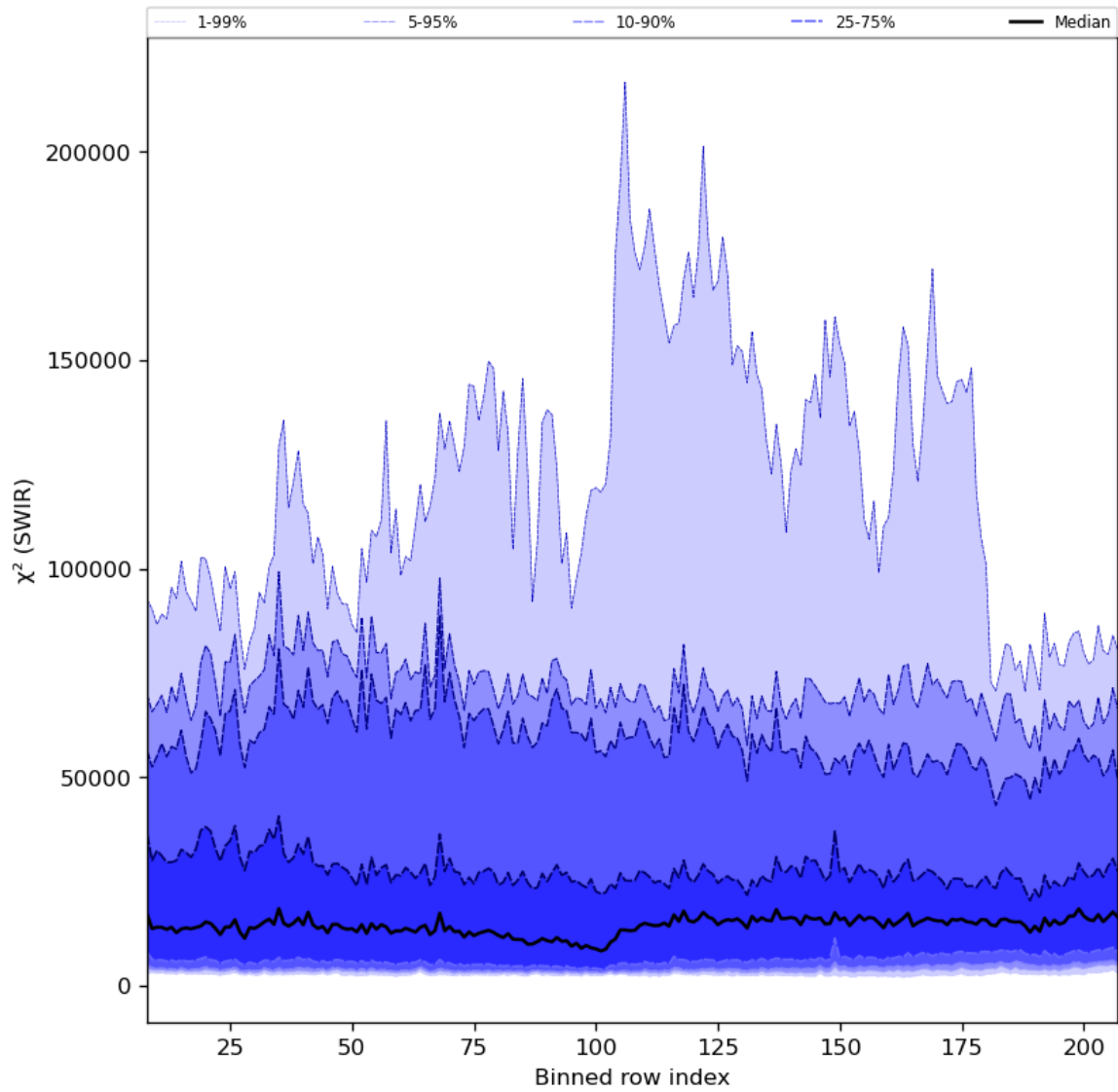
Figure 39: Along track statistics of " \chi^2 (SWIR)" for 2023-09-07 to 2023-09-09
