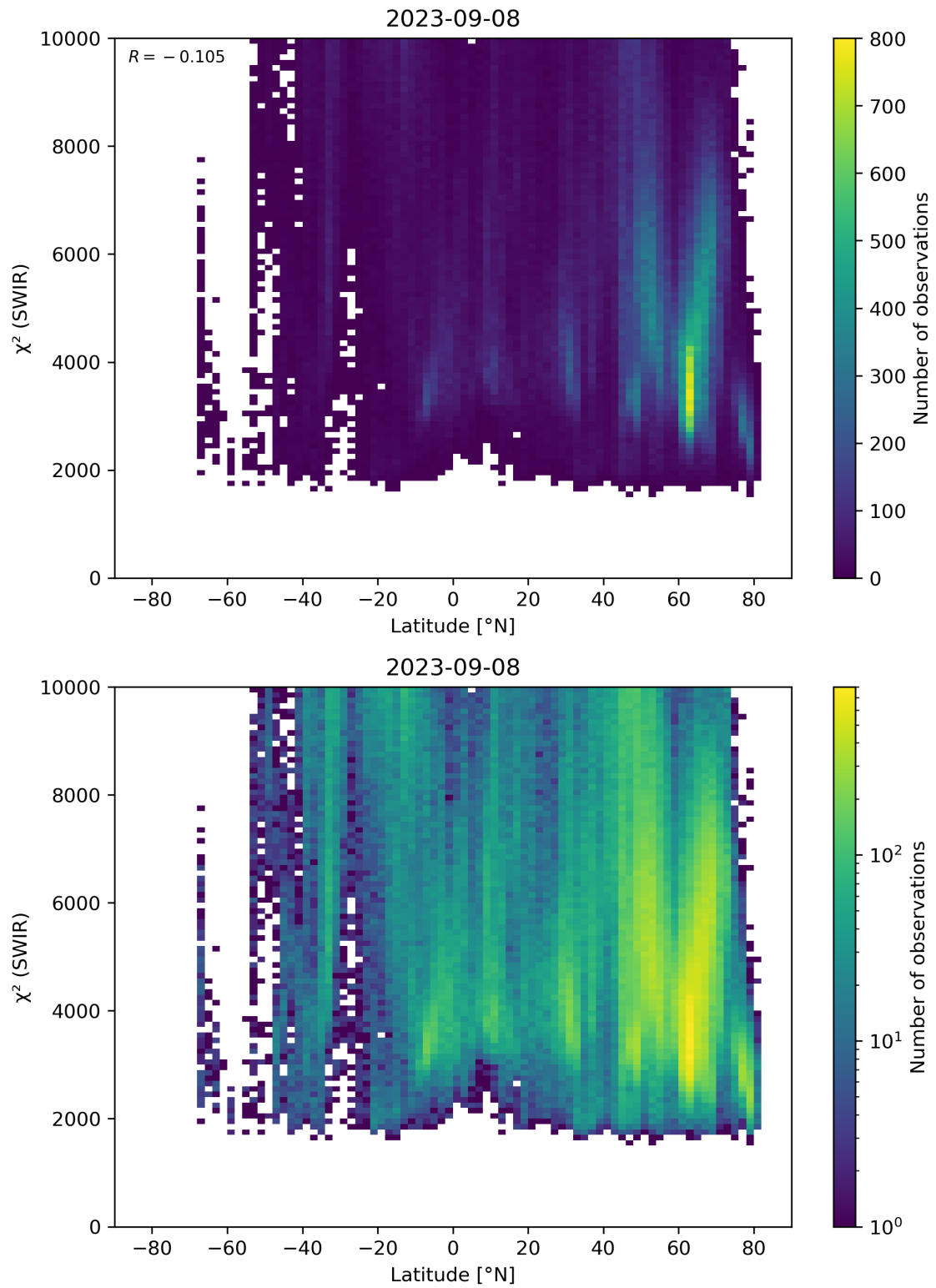
Figure 54: Scatter density plot of “Latitude” against “ \chi^2 (SWIR)” for 2023-09-07 to 2023-09-09.
