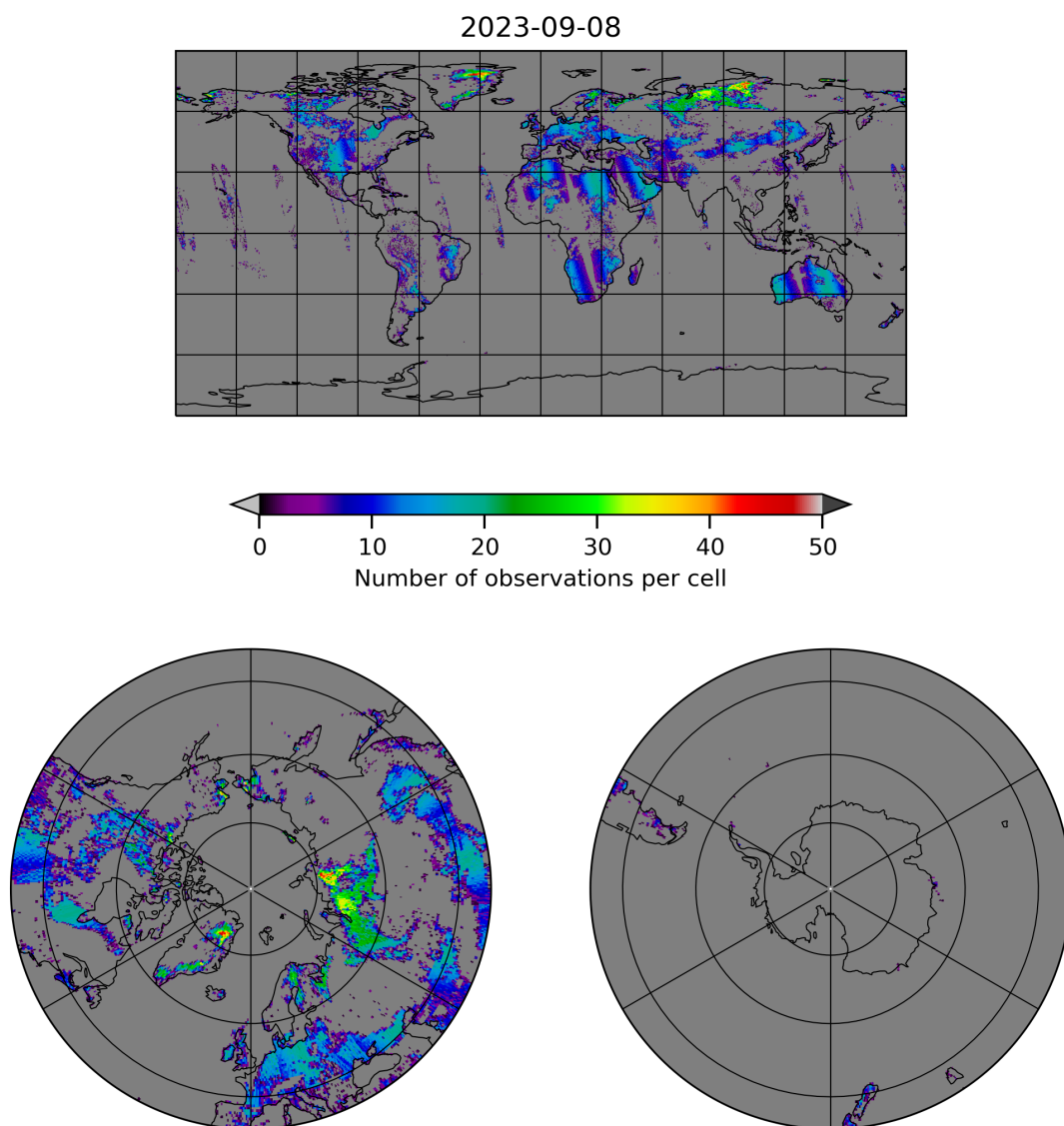
Figure 10: Map of the number of observations for 2023-09-07 to 2023-09-09
