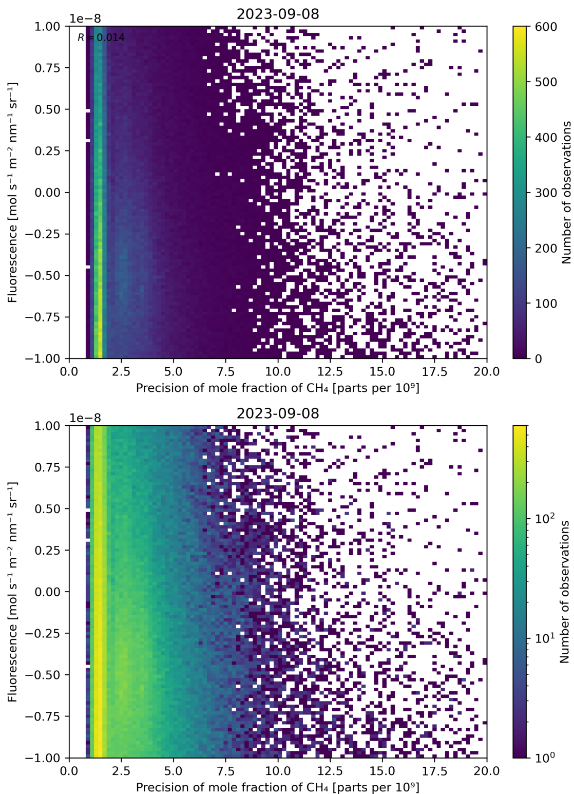
Figure 81: Scatter density plot of “Precision of mole fraction of \text{CH}_4 ” against “Fluorescence” for 2023-09-07 to 2023-09-09.
