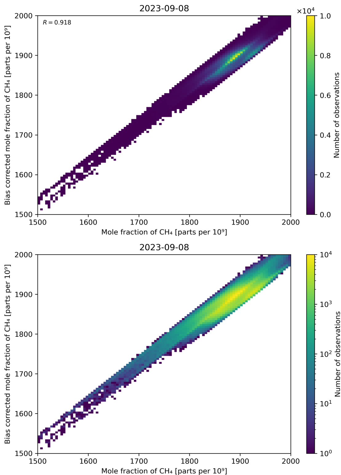
Figure 74: Scatter density plot of “Mole fraction of CH 4 ” against “Bias corrected mole fraction of CH 4 ” for 2023-09-07 to 2023-09-09.
