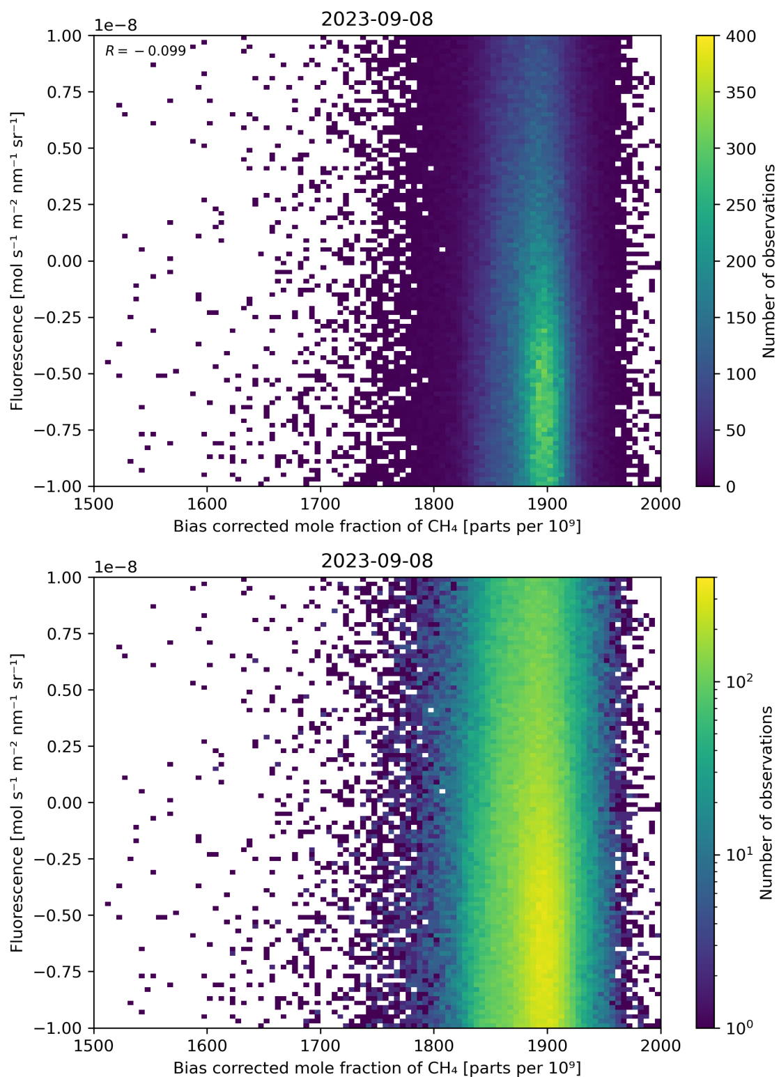
Figure 66: Scatter density plot of “Bias corrected mole fraction of \text{CH}_4 ” against “Fluorescence” for 2023-09-07 to 2023-09-09.
