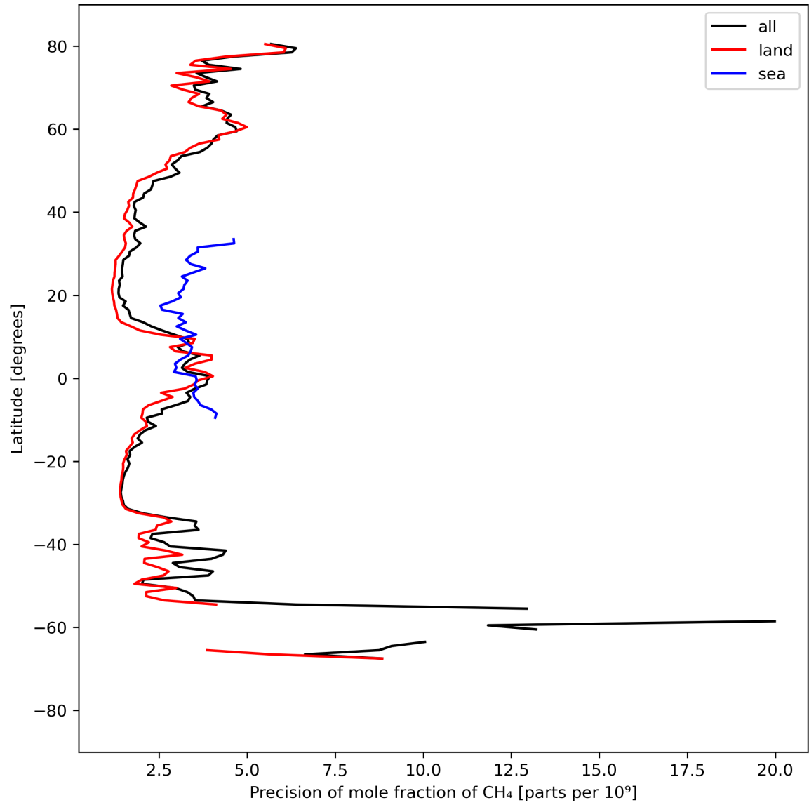
Figure 13: Zonal average of “Precision of mole fraction of CH 4 ” for 2023-09-07 to 2023-09-09.
