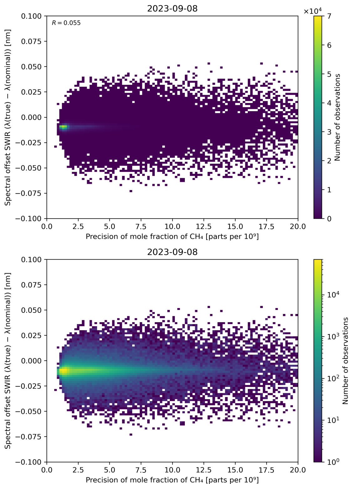
Figure 85: Scatter density plot of “Precision of mole fraction of CH 4 ” against “Spectral offset SWIR ( \lambda(\text{true}) - \lambda(\text{nominal}) )” for 2023-09-07 to 2023-09-09.
