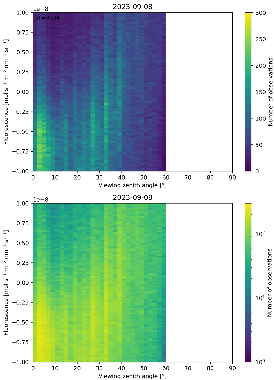
Figure 108: Scatter density plot of “Viewing zenith angle” against “Fluorescence” for 2023-09-07 to 2023-09-09.
