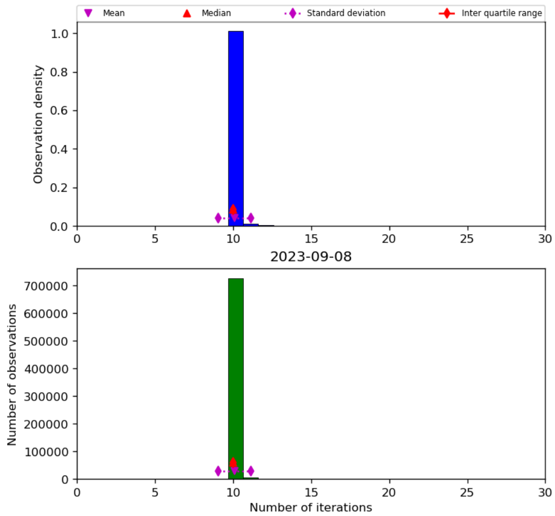
Figure 31: Histogram of “Number of iterations” for 2023-09-07 to 2023-09-09
