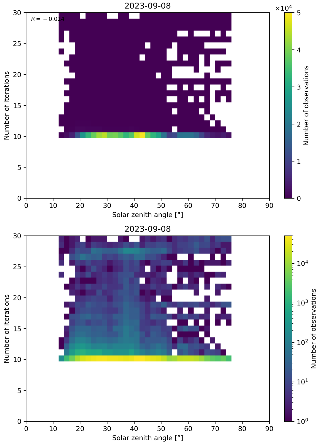
Figure 102: Scatter density plot of “Solar zenith angle” against “Number of iterations” for 2023-09-07 to 2023-09-09.
