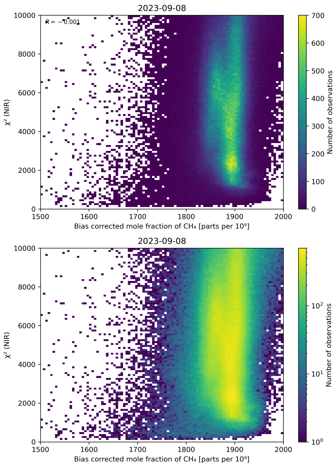
Figure 63: Scatter density plot of “Bias corrected mole fraction of CH 4 ” against “ \chi^2 (NIR)” for 2023-09-07 to 2023-09-09.
