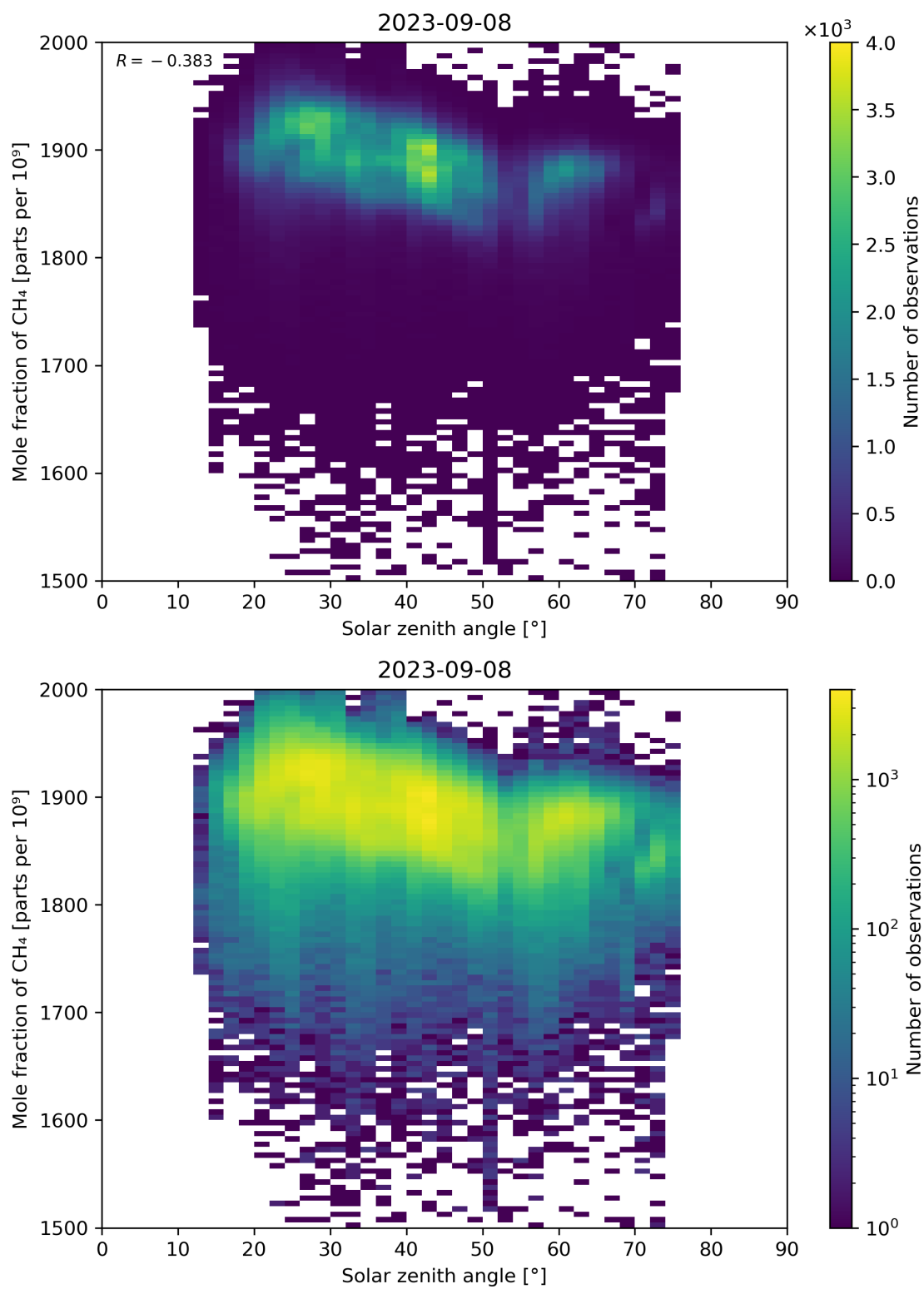
Figure 99: Scatter density plot of “Solar zenith angle” against “Mole fraction of CH 4 ” for 2023-09-07 to 2023-09-09.
