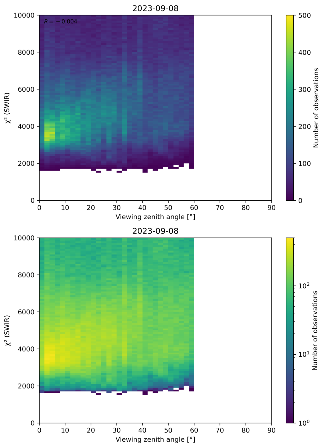
Figure 106: Scatter density plot of “Viewing zenith angle” against “ \chi^2 (SWIR)” for 2023-09-07 to 2023-09-09.
