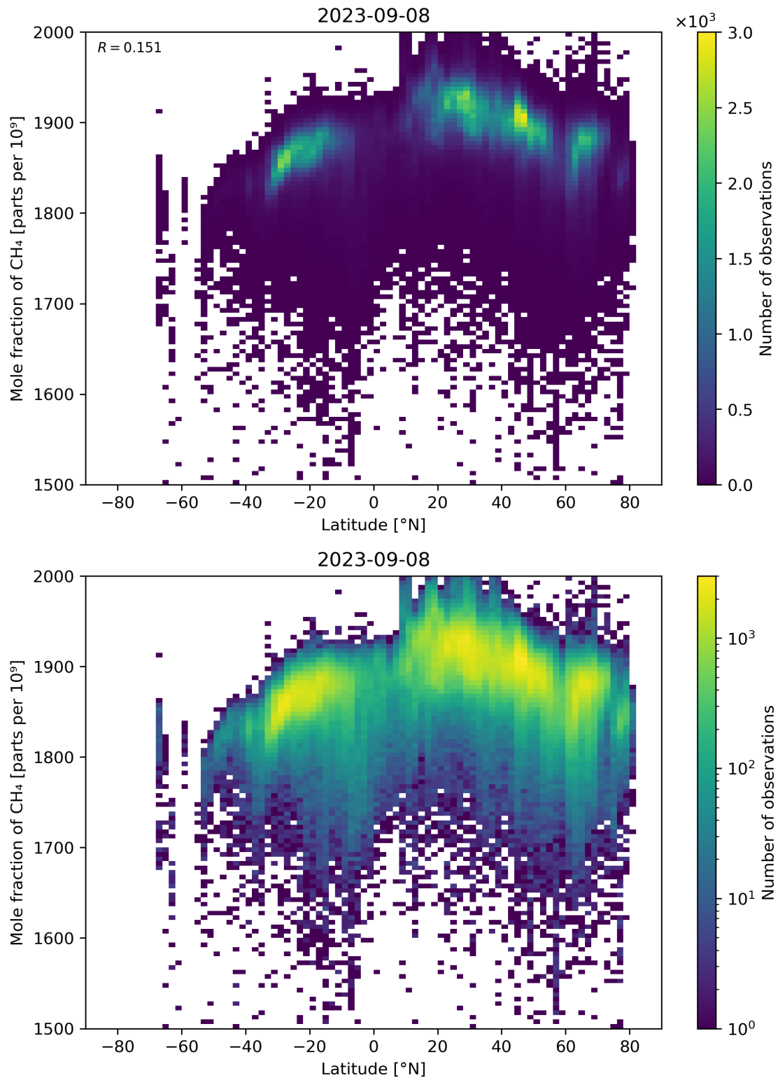
Figure 57: Scatter density plot of “Latitude” against “Mole fraction of \text{CH}_4 ” for 2023-09-07 to 2023-09-09.
