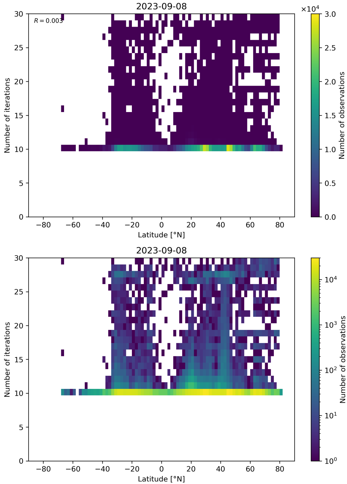
Figure 60: Scatter density plot of “Latitude” against “Number of iterations” for 2023-09-07 to 2023-09-09.
