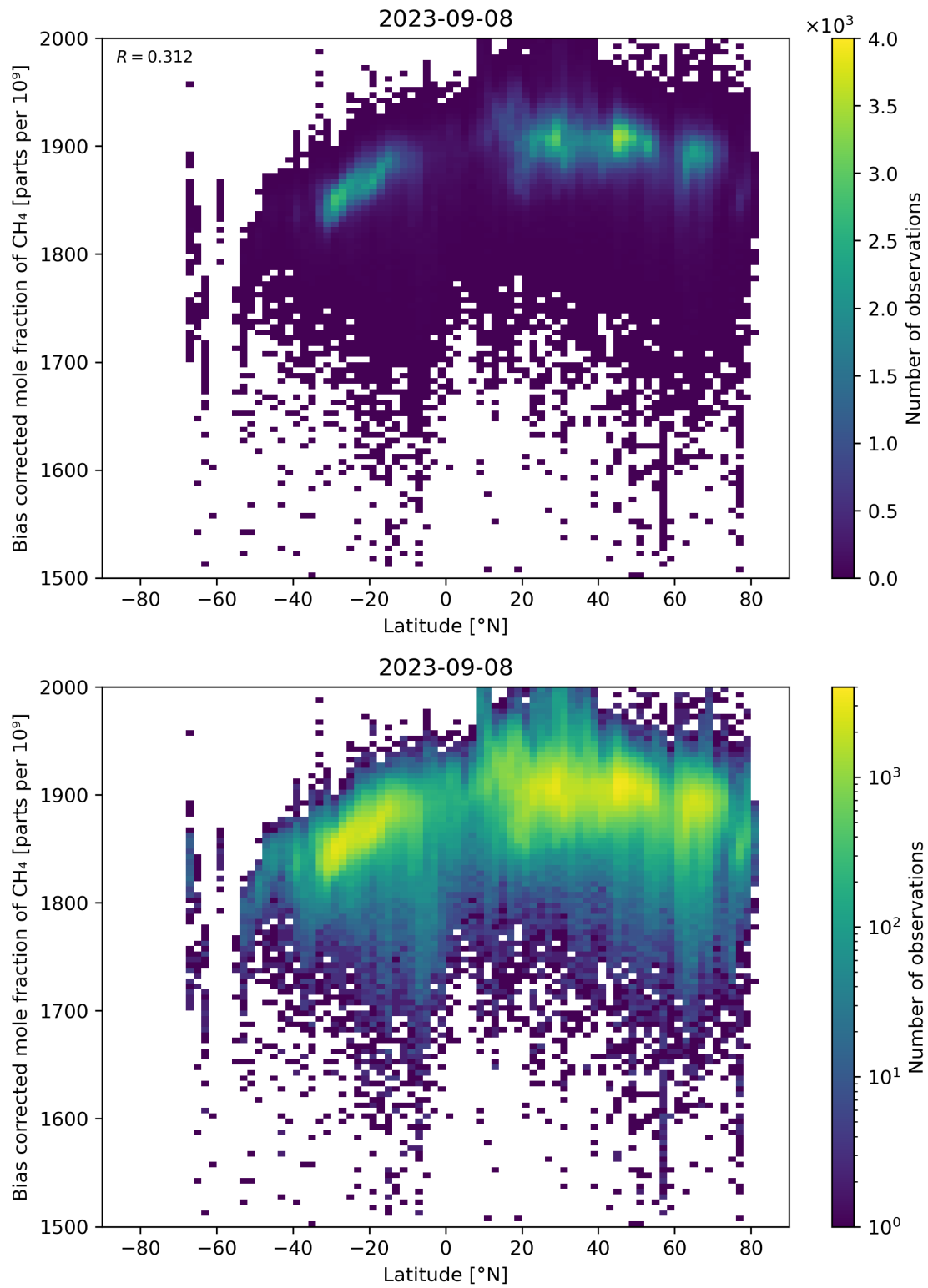
Figure 58: Scatter density plot of “Latitude” against “Bias corrected mole fraction of \text{CH}_4 ” for 2023-09-07 to 2023-09-09.
