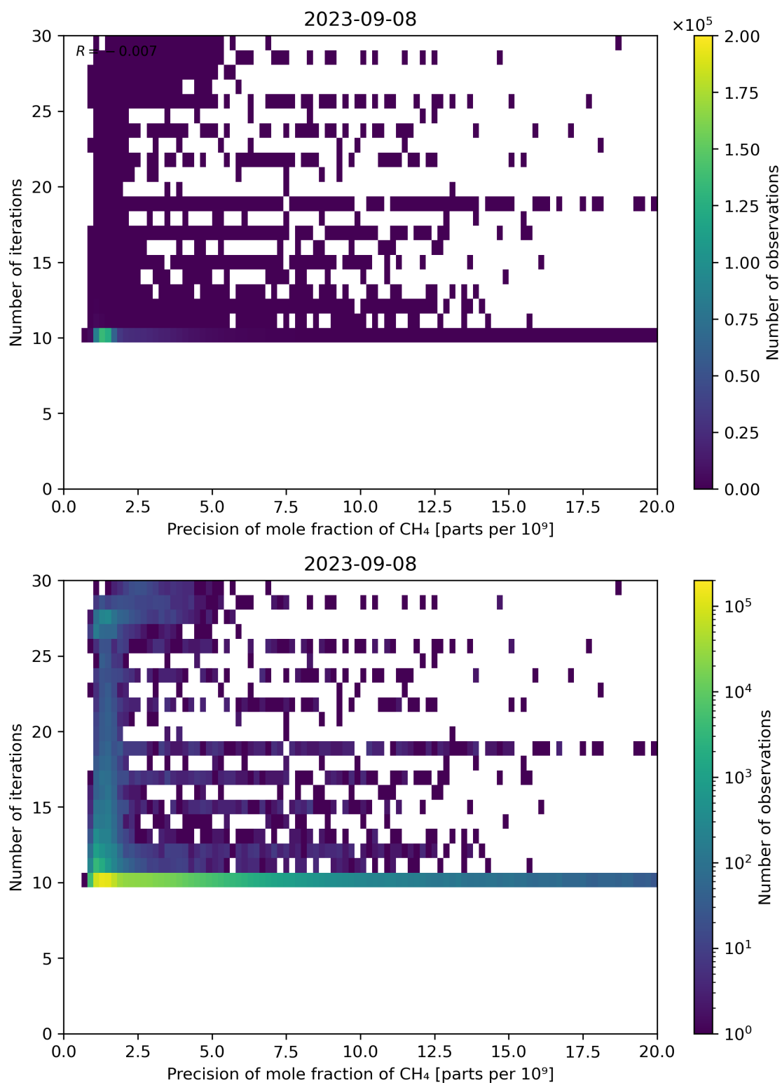
Figure 83: Scatter density plot of “Precision of mole fraction of CH 4 ” against “Number of iterations” for 2023-09-07 to 2023-09-09.
