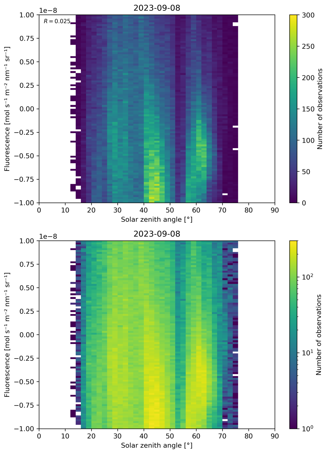
Figure 97: Scatter density plot of “Solar zenith angle” against “Fluorescence” for 2023-09-07 to 2023-09-09.
