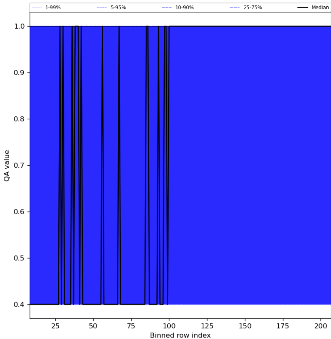
Figure 33: Along track statistics of “QA value” for 2023-09-07 to 2023-09-09
