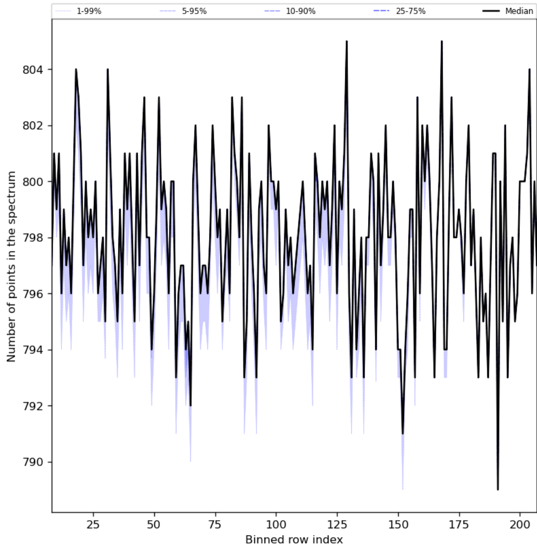
Figure 37: Along track statistics of “Number of points in the spectrum” for 2023-09-07 to 2023-09-09
