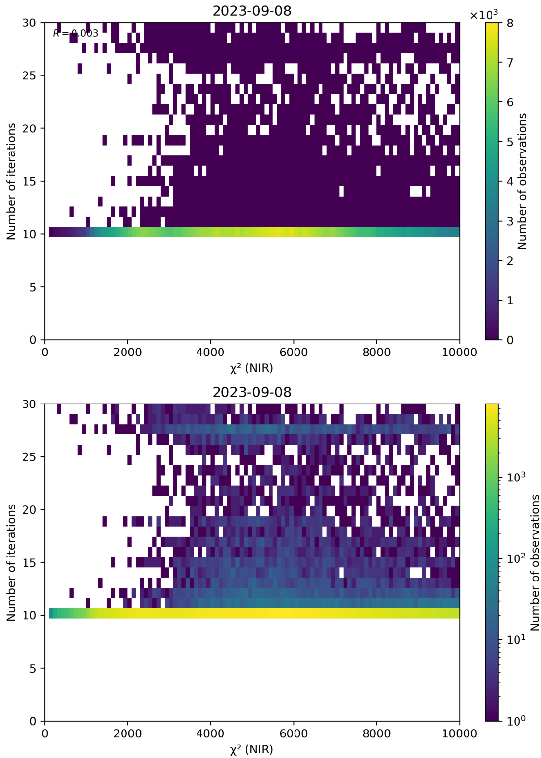
Figure 46: Scatter density plot of “ \chi^2 (NIR)” against “Number of iterations” for 2023-09-07 to 2023-09-09.
