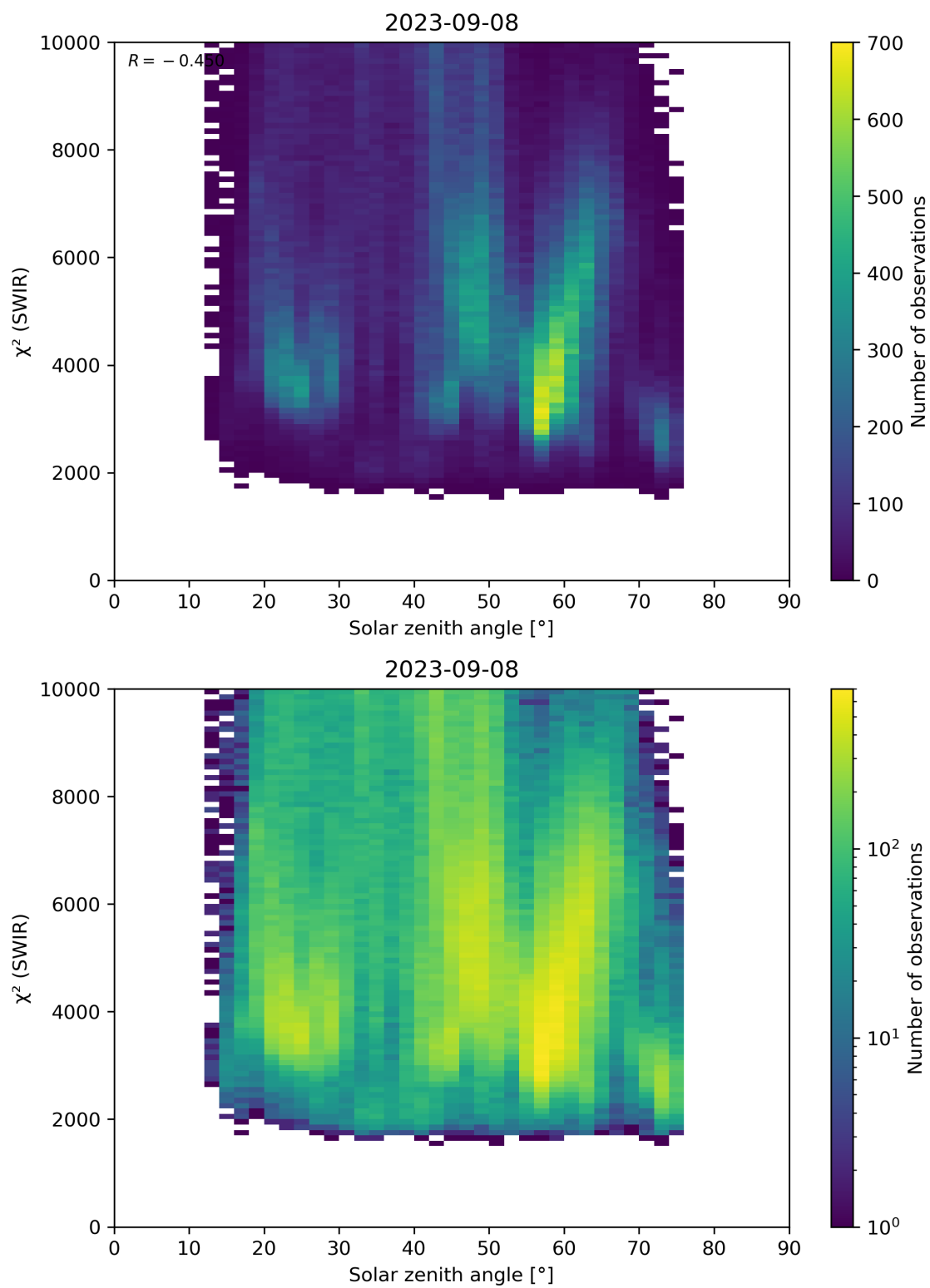
Figure 95: Scatter density plot of “Solar zenith angle” against “ \chi^2 (SWIR)” for 2023-09-07 to 2023-09-09.
