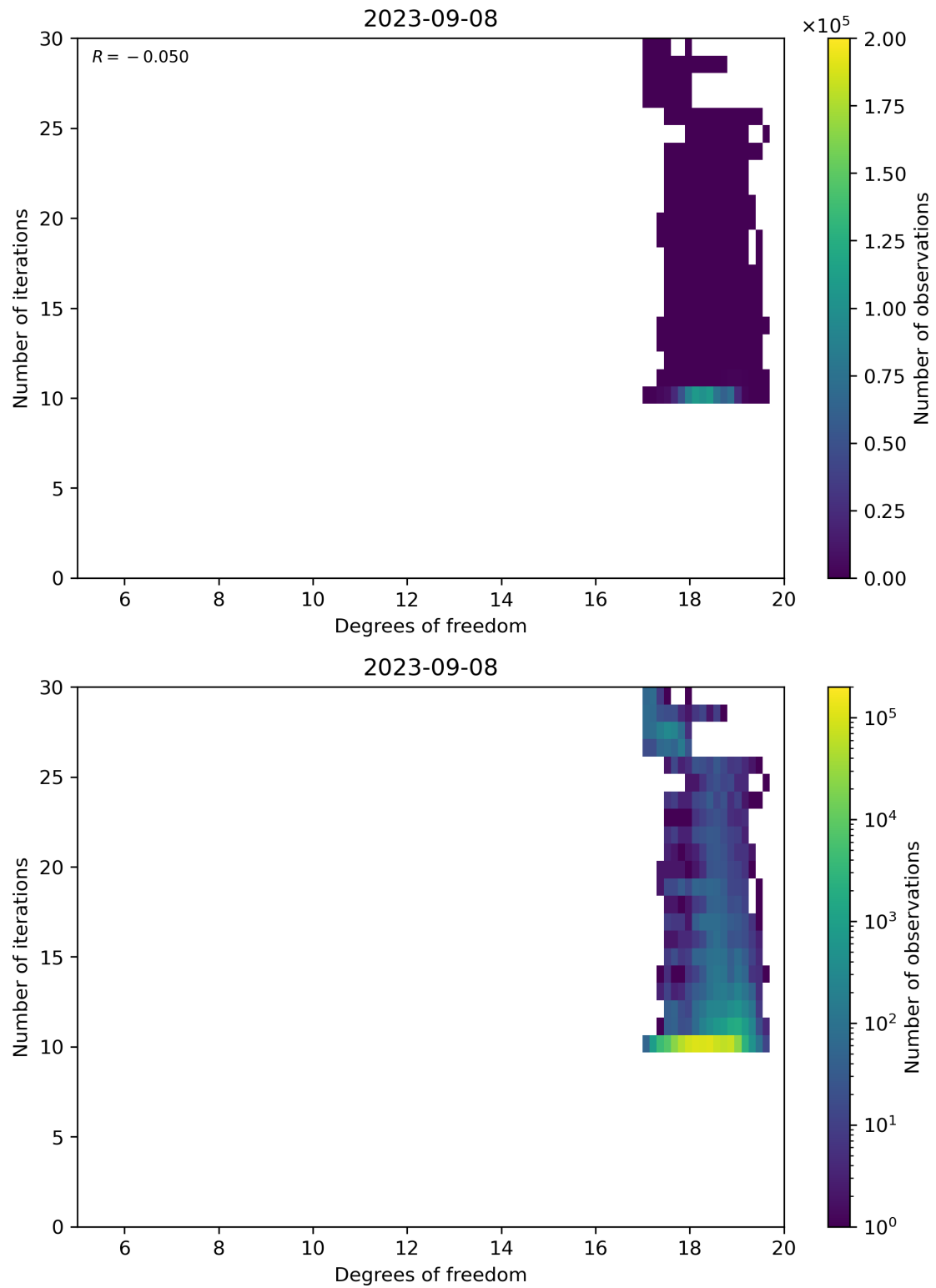
Figure 52: Scatter density plot of “Degrees of freedom” against “Number of iterations” for 2023-09-07 to 2023-09-09.
