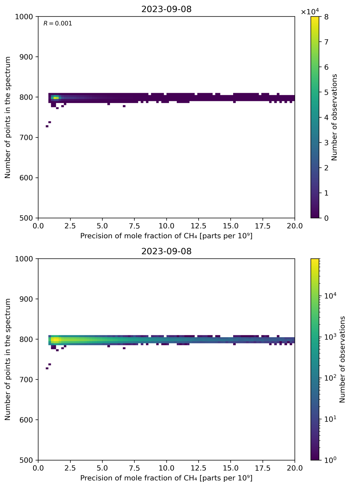
Figure 84: Scatter density plot of “Precision of mole fraction of CH 4 ” against “Number of points in the spectrum” for 2023-09-07 to 2023-09-09.
