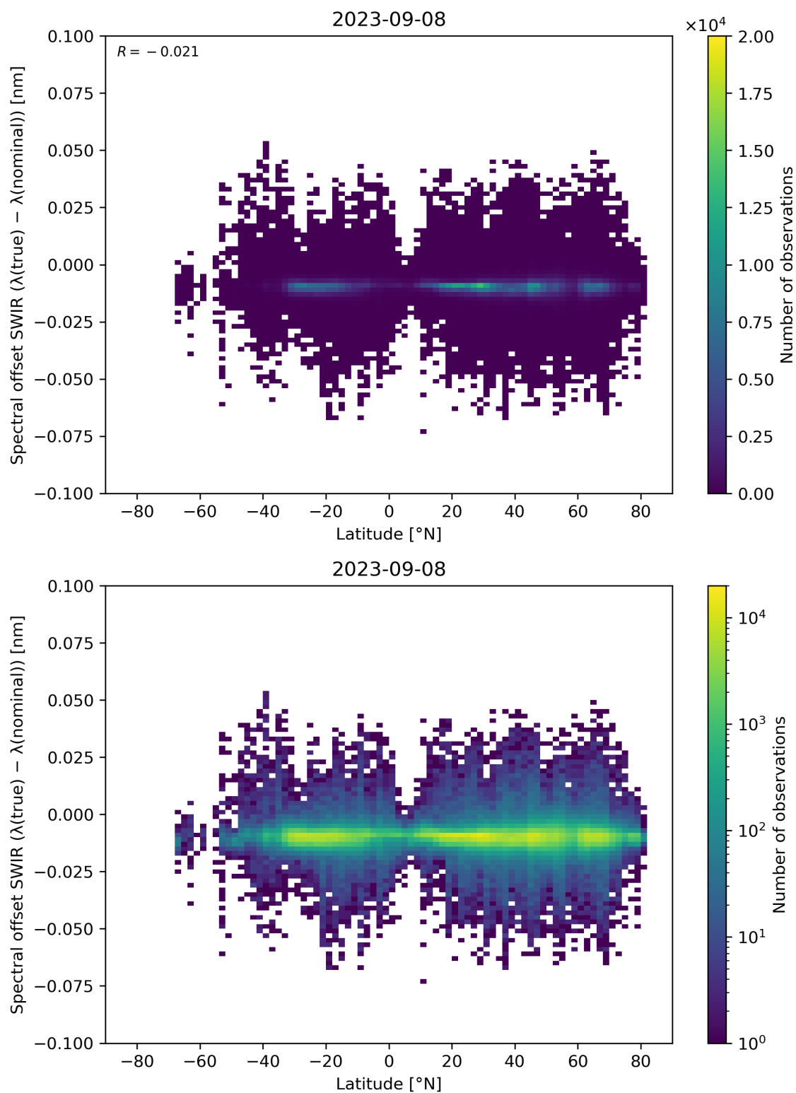
Figure 62: Scatter density plot of “Latitude” against “Spectral offset SWIR ( \lambda(\text{true}) - \lambda(\text{nominal}) )” for 2023-09-07 to 2023-09-09.
