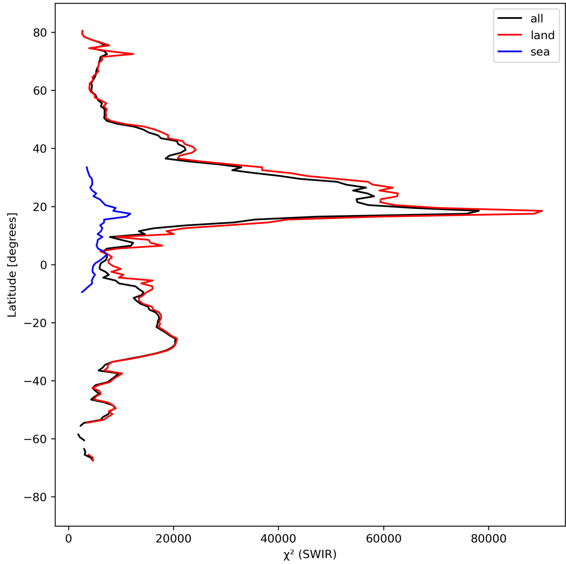
Figure 17: Zonal average of “ \chi^2 (SWIR)” for 2023-09-07 to 2023-09-09.
