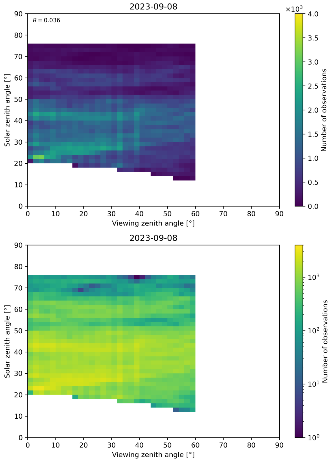
Figure 115: Scatter density plot of “Viewing zenith angle” against “Solar zenith angle” for 2023-09-07 to 2023-09-09.
