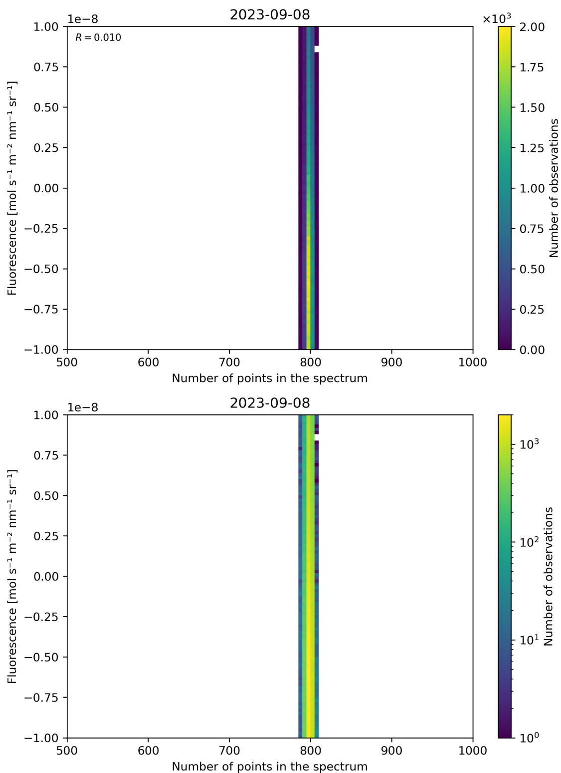
Figure 91: Scatter density plot of “Number of points in the spectrum” against “Fluorescence” for 2023-09-07 to 2023-09-09.
