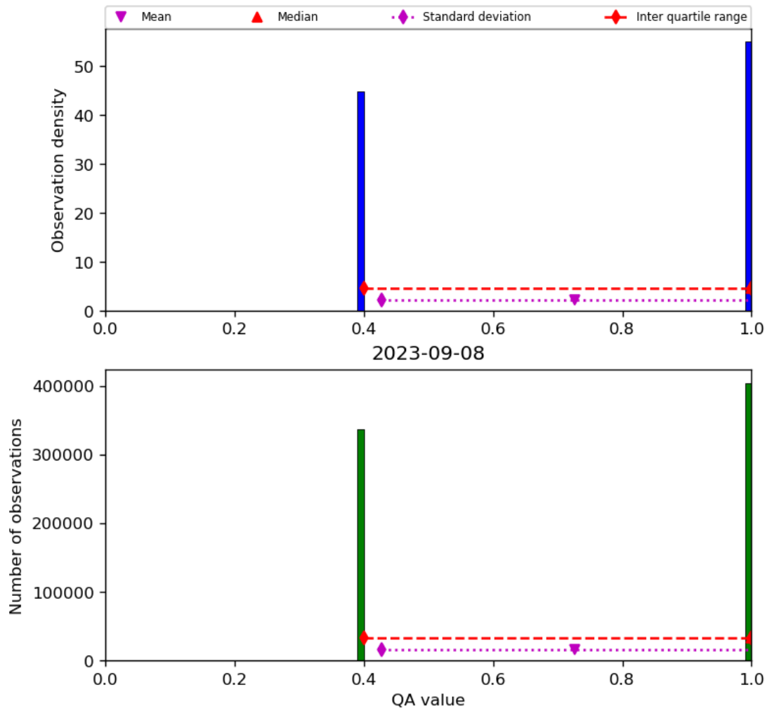
Figure 22: Histogram of “QA value” for 2023-09-07 to 2023-09-09
