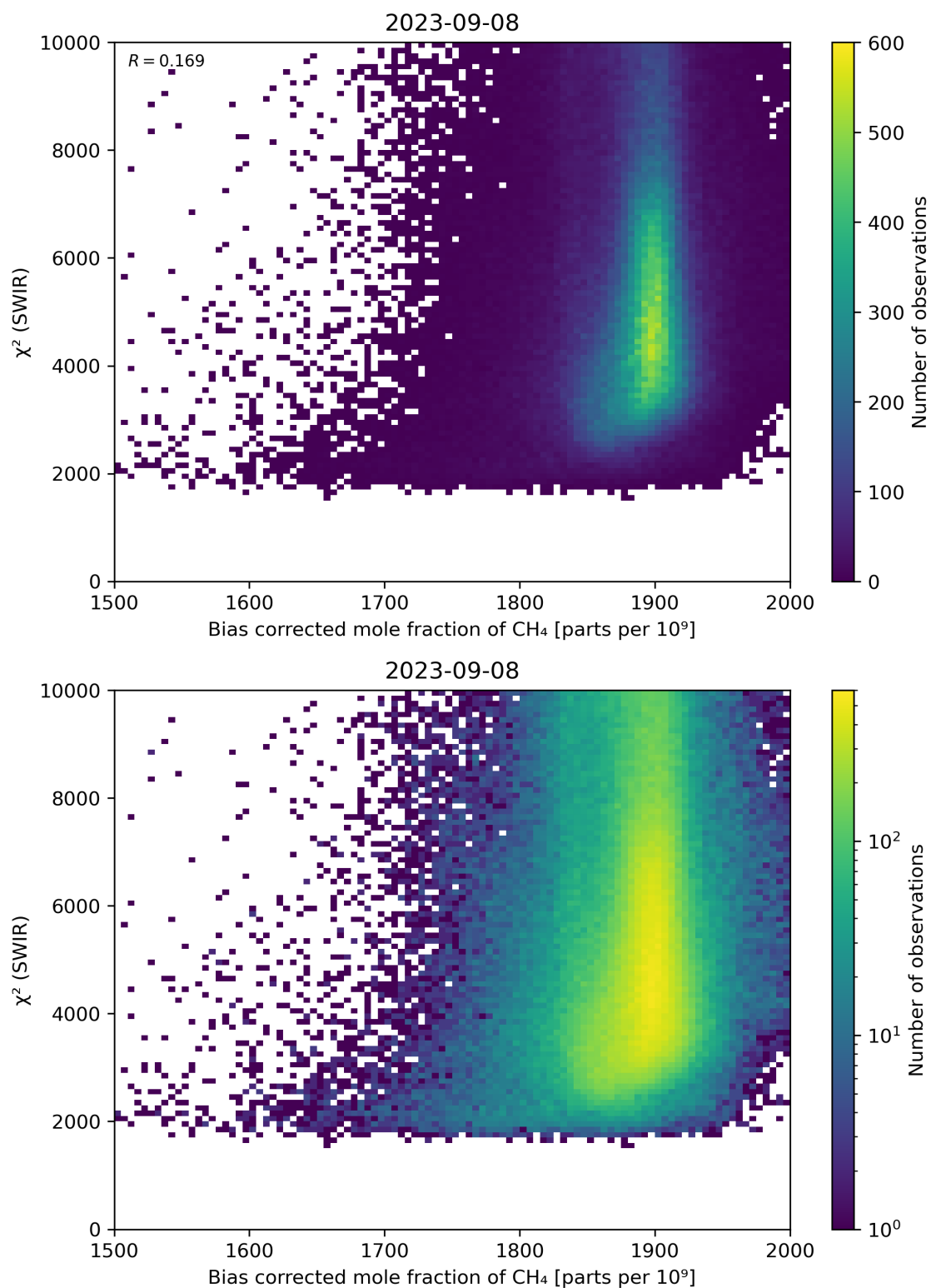
Figure 64: Scatter density plot of “Bias corrected mole fraction of \text{CH}_4 ” against “ \chi^2 (SWIR)” for 2023-09-07 to 2023-09-09.
