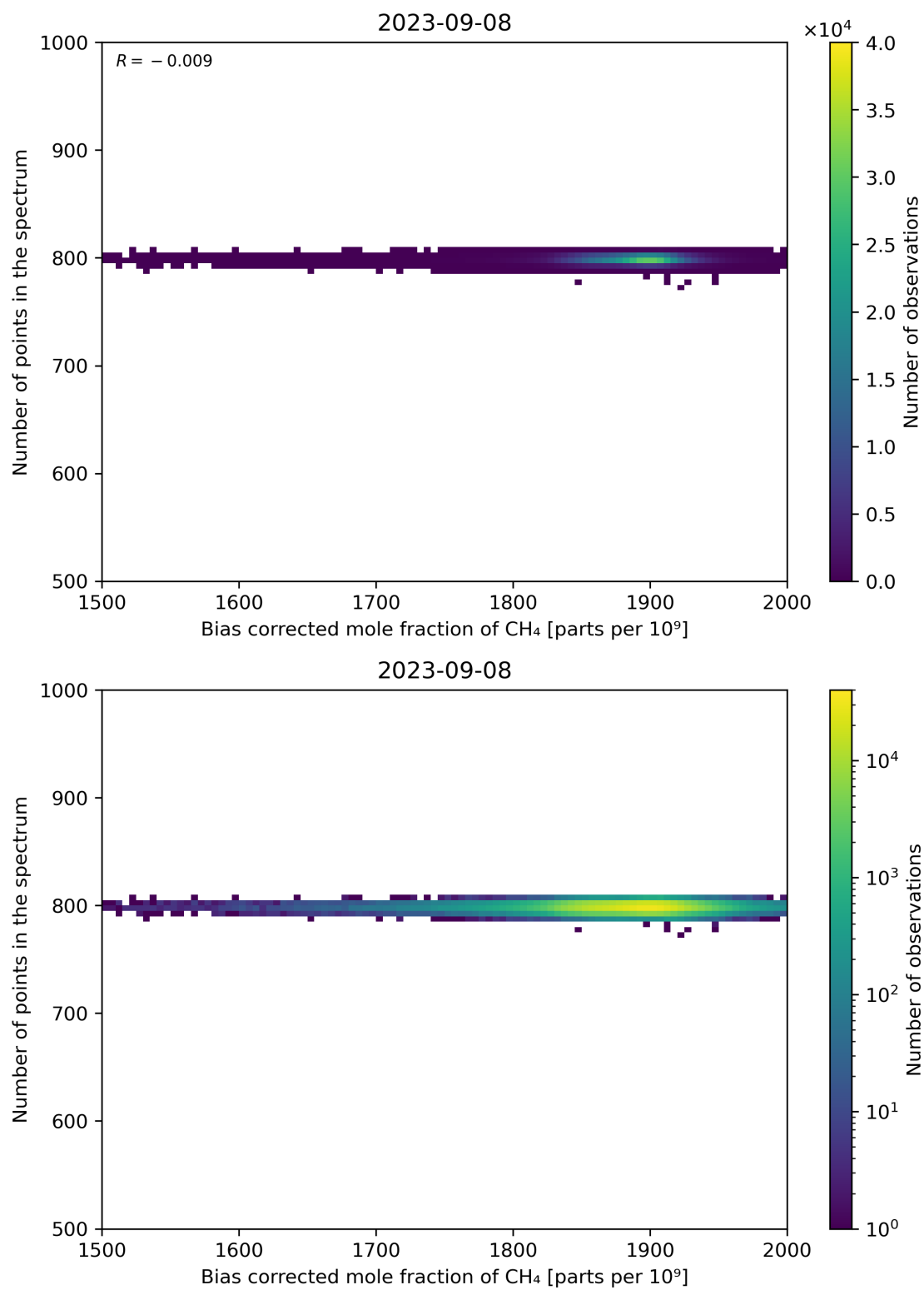
Figure 68: Scatter density plot of “Bias corrected mole fraction of CH 4 ” against “Number of points in the spectrum” for 2023-09-07 to 2023-09-09.
