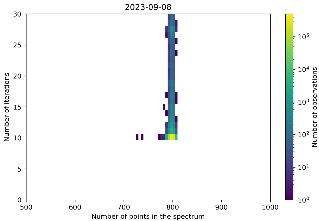
Figure 92: Scatter density plot of “Number of points in the spectrum” against “Number of iterations” for 2023-09-07 to 2023-09-09.
