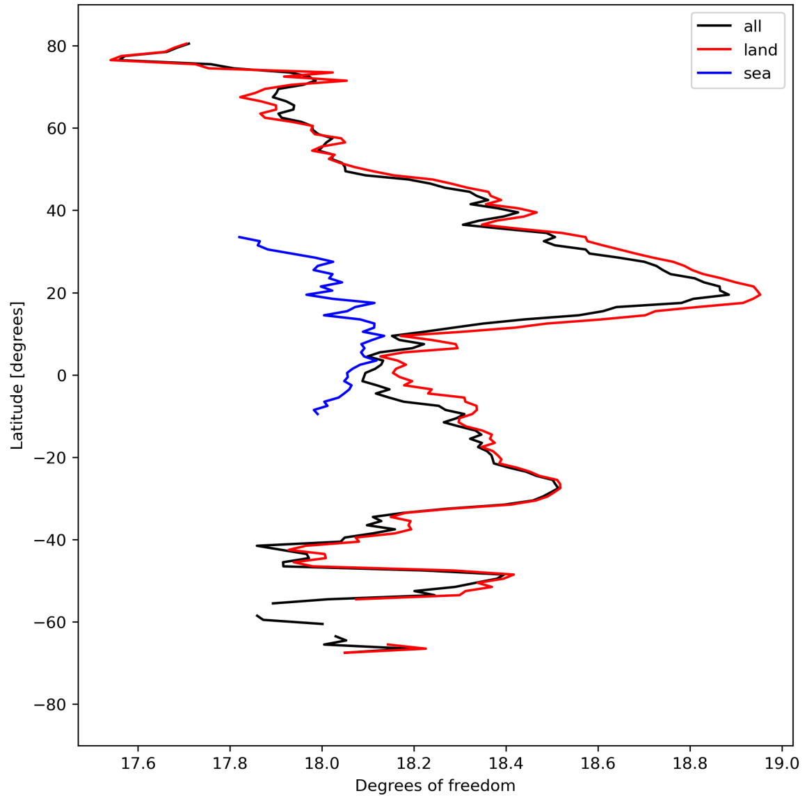
Figure 19: Zonal average of “Degrees of freedom” for 2023-09-07 to 2023-09-09.
