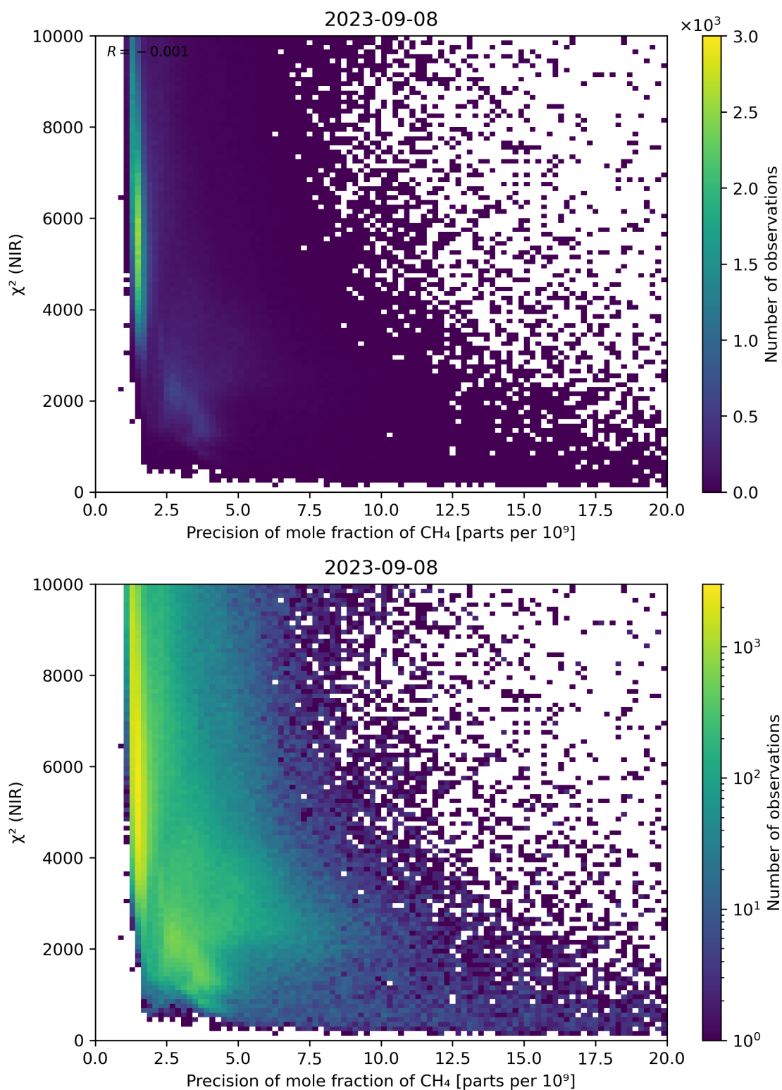
Figure 78: Scatter density plot of “Precision of mole fraction of CH 4 ” against “ \chi^2 (NIR)” for 2023-09-07 to 2023-09-09.
