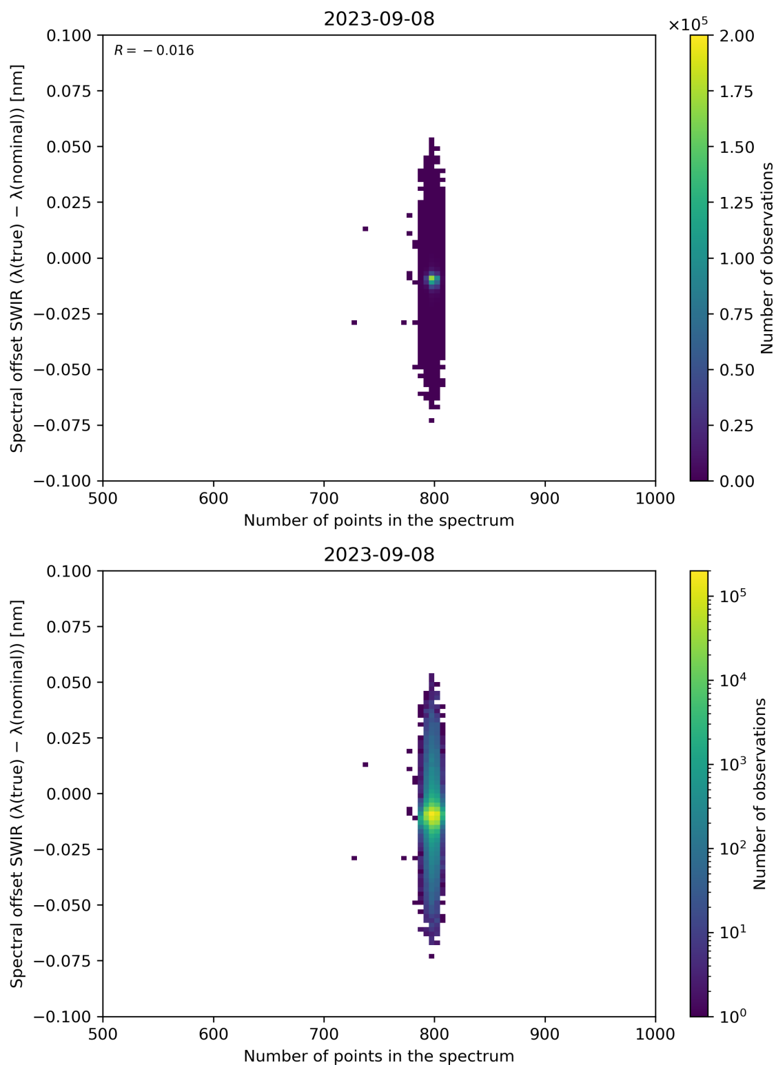
Figure 93: Scatter density plot of “Number of points in the spectrum” against “Spectral offset SWIR ( \lambda(\text{true}) - \lambda(\text{nominal}) )” for 2023-09-07 to 2023-09-09.
