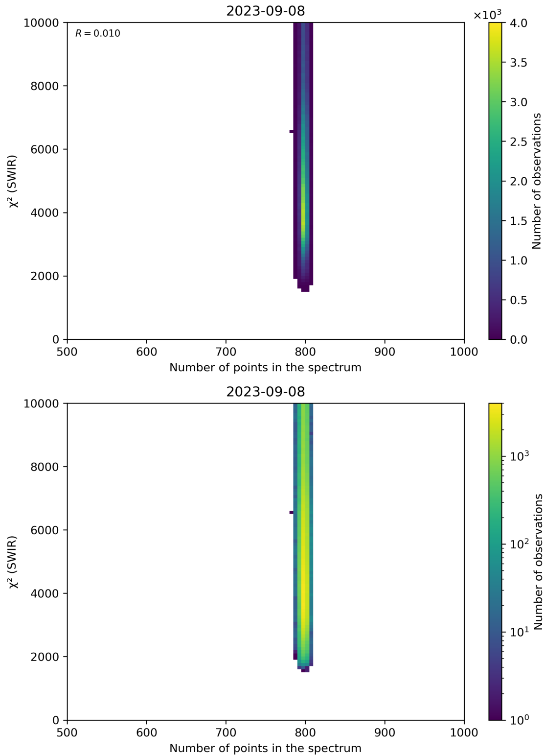
Figure 89: Scatter density plot of “Number of points in the spectrum” against “ \chi^2 (SWIR)” for 2023-09-07 to 2023-09-09.
