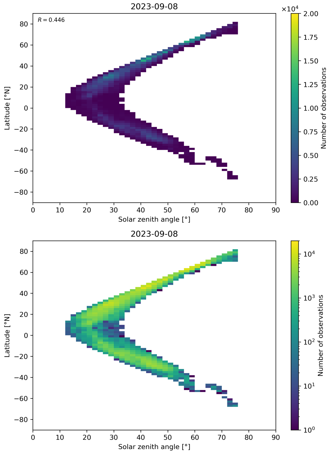
Figure 98: Scatter density plot of “Solar zenith angle” against “Latitude” for 2023-09-07 to 2023-09-09.
