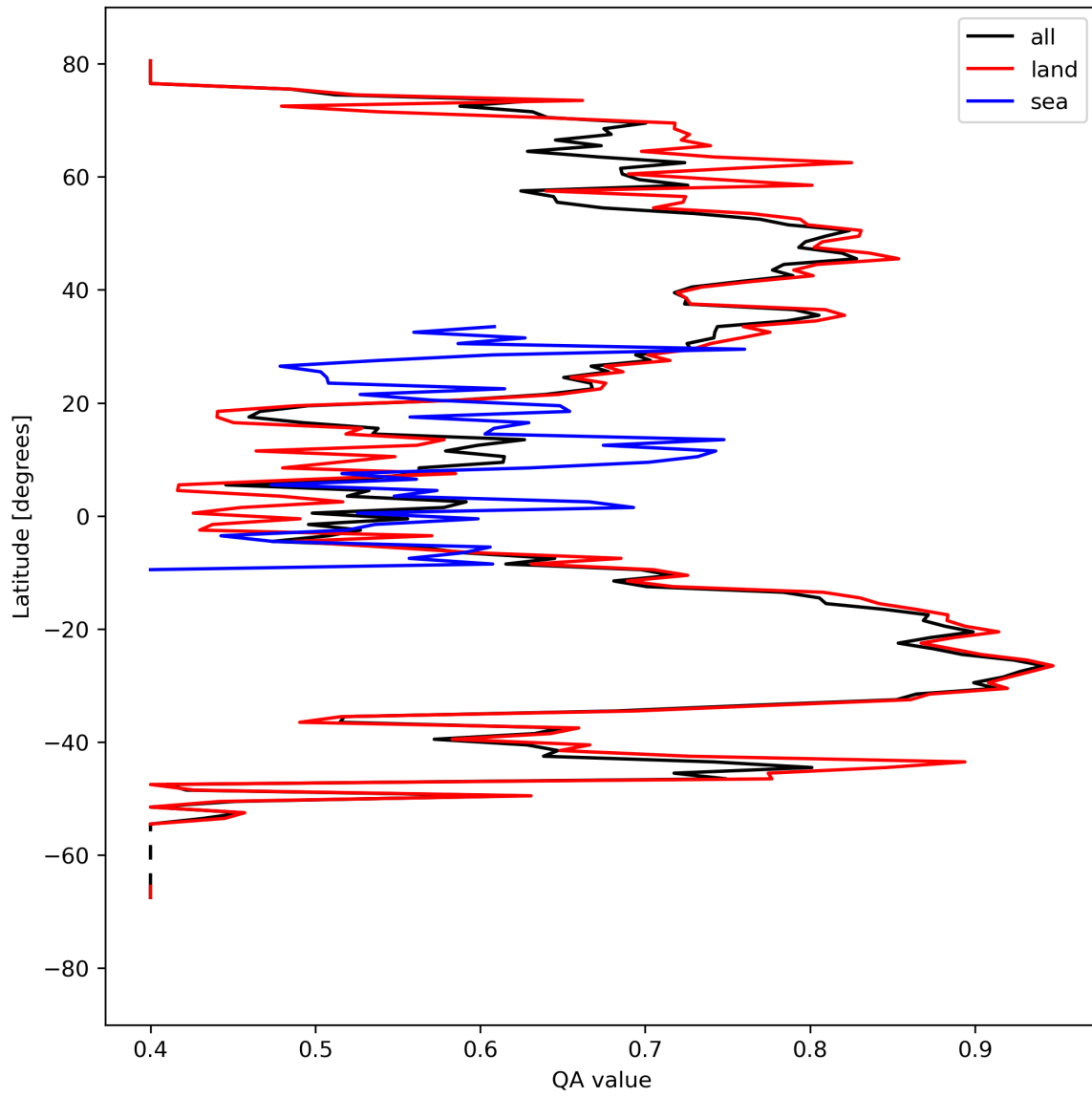
Figure 11: Zonal average of “QA value” for 2023-09-07 to 2023-09-09.
