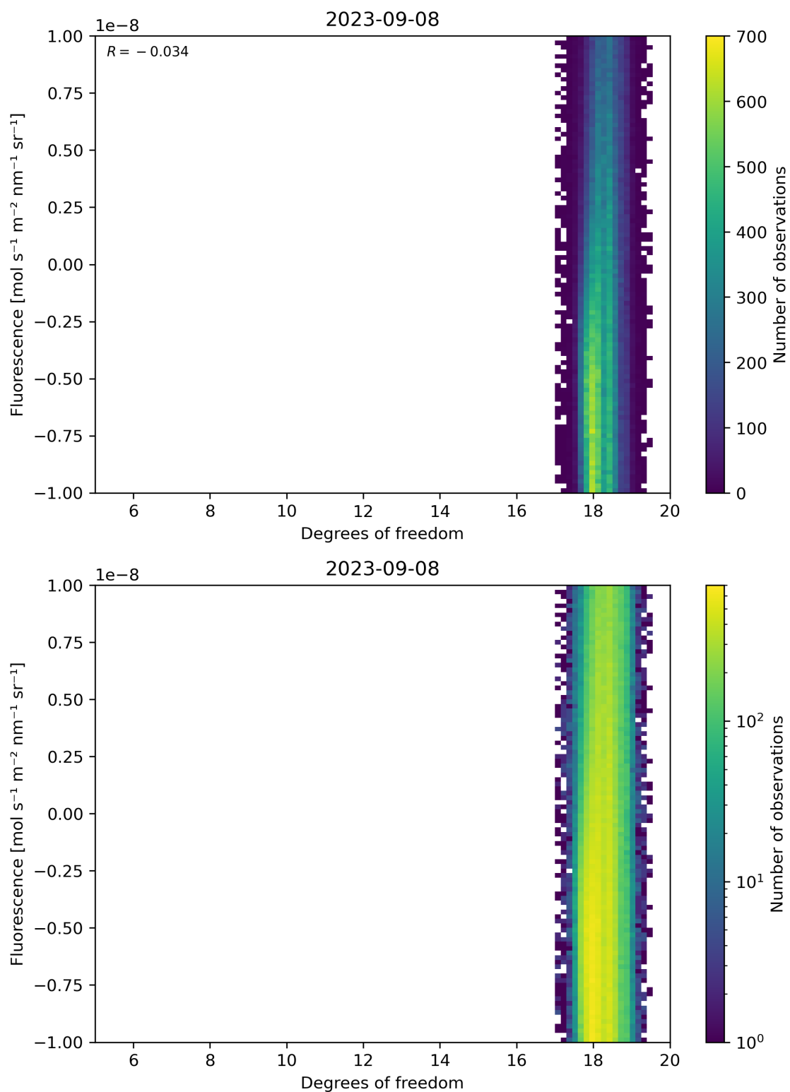
Figure 51: Scatter density plot of “Degrees of freedom” against “Fluorescence” for 2023-09-07 to 2023-09-09.
