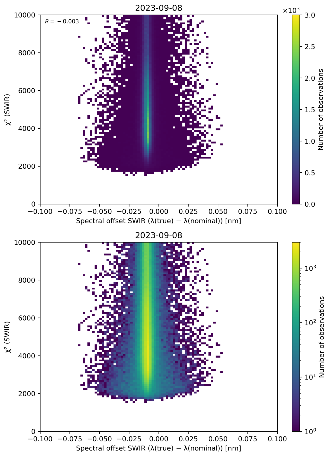
Figure 118: Scatter density plot of “Spectral offset SWIR ( \lambda(\text{true}) - \lambda(\text{nominal}) )” against “ \chi^2 (SWIR)” for 2023-09-07 to 2023-09-09.
