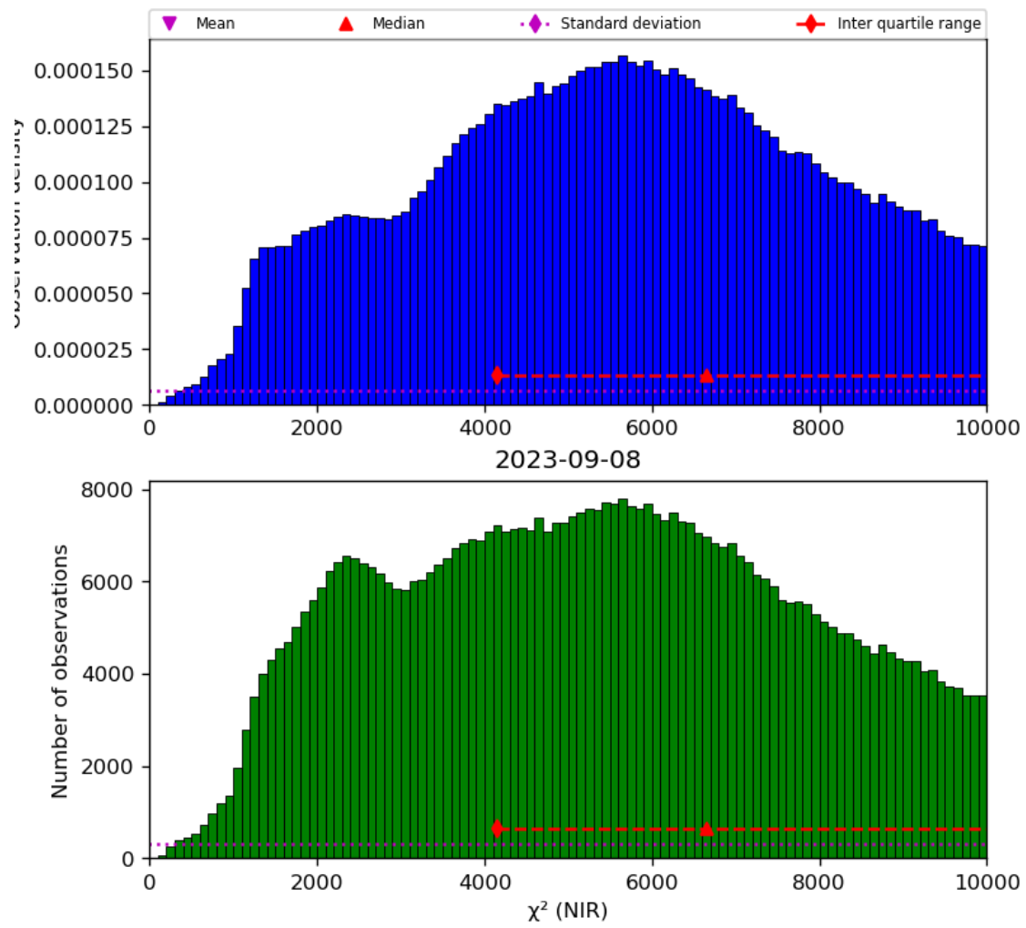
Figure 29: Histogram of “ \chi^2 (NIR)” for 2023-09-07 to 2023-09-09
