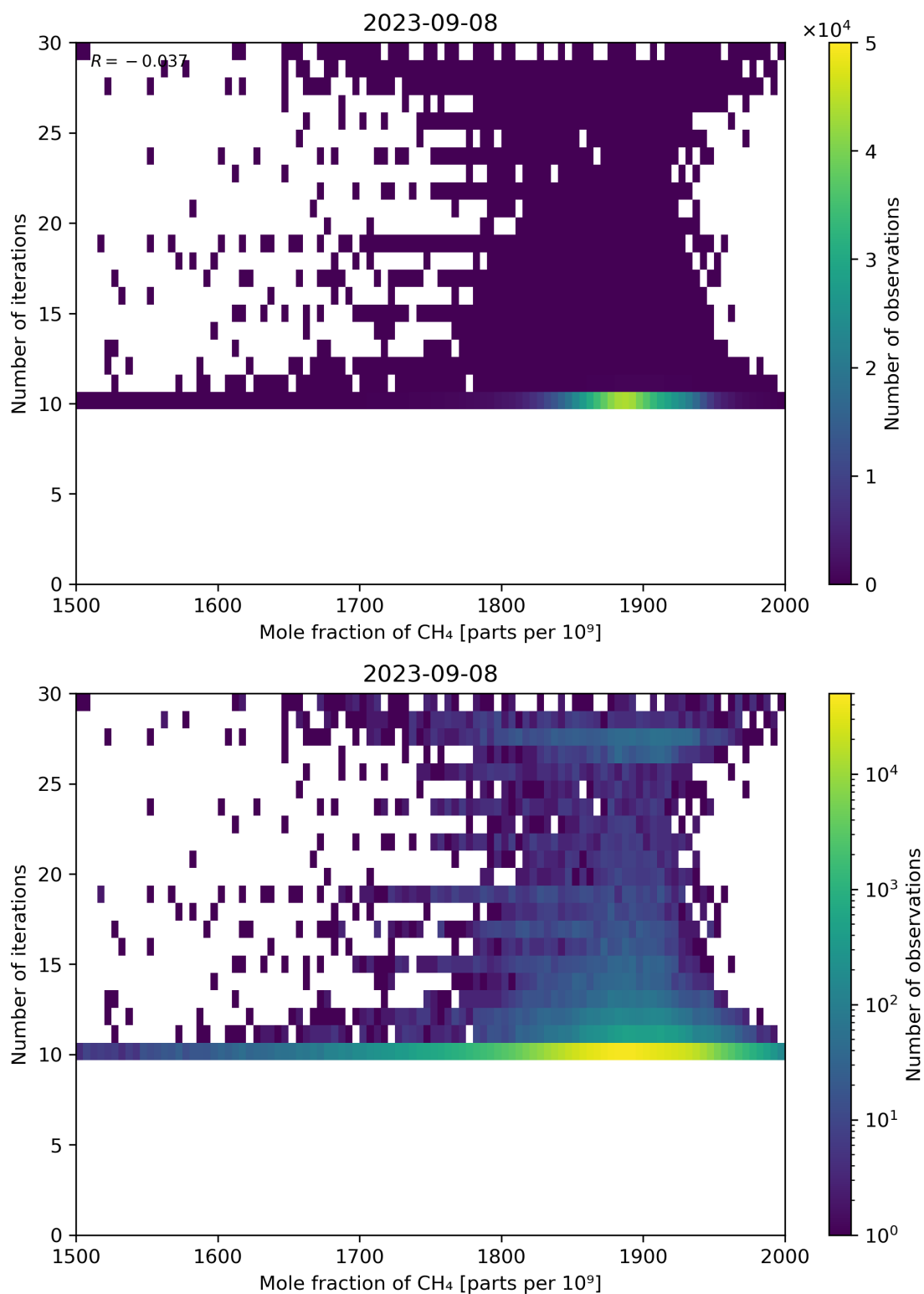
Figure 76: Scatter density plot of “Mole fraction of CH 4 ” against “Number of iterations” for 2023-09-07 to 2023-09-09.
