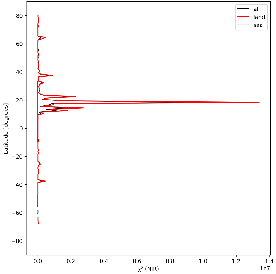
Figure 18: Zonal average of “ \chi^2 (NIR)” for 2023-09-07 to 2023-09-09.
