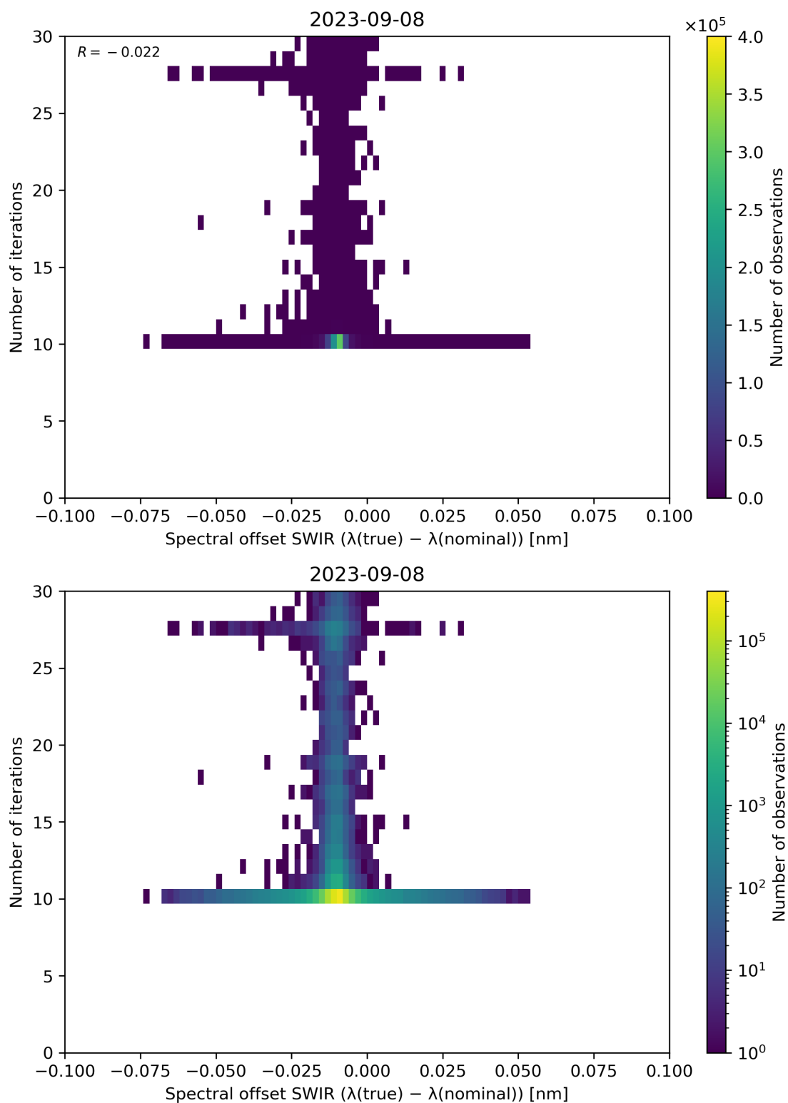
Figure 121: Scatter density plot of “Spectral offset SWIR ( \lambda(\text{true}) - \lambda(\text{nominal}) )” against “Number of iterations” for 2023-09-07 to 2023-09-09.
