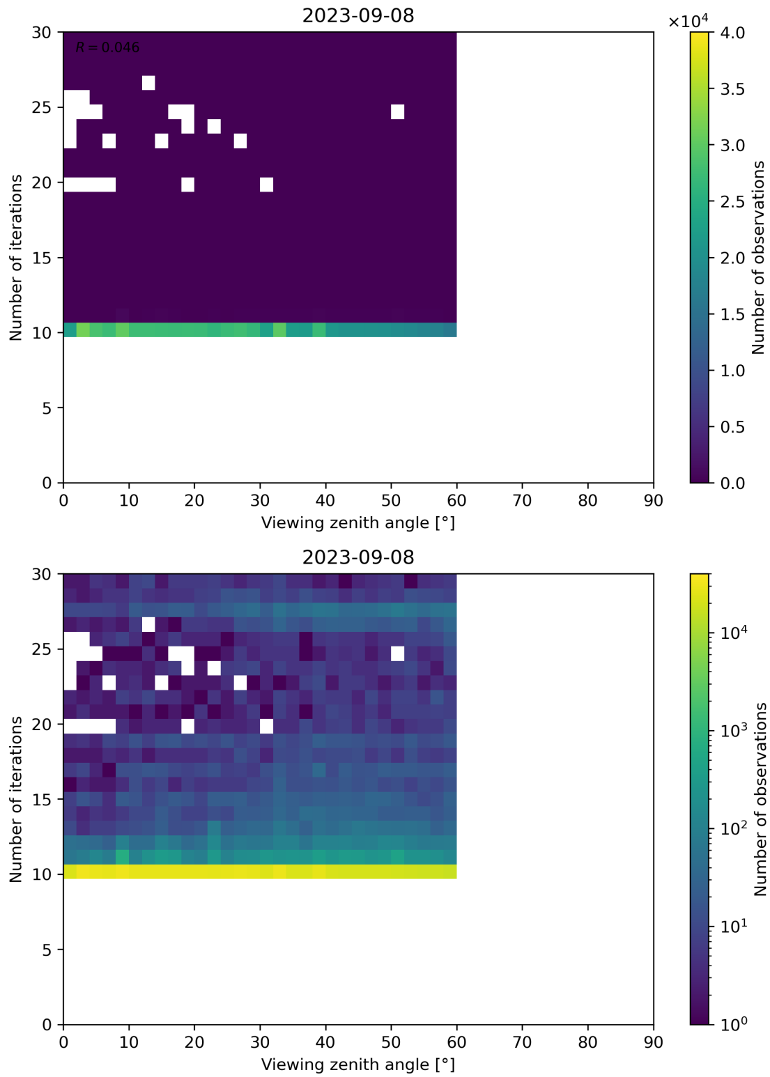
Figure 113: Scatter density plot of “Viewing zenith angle” against “Number of iterations” for 2023-09-07 to 2023-09-09.
