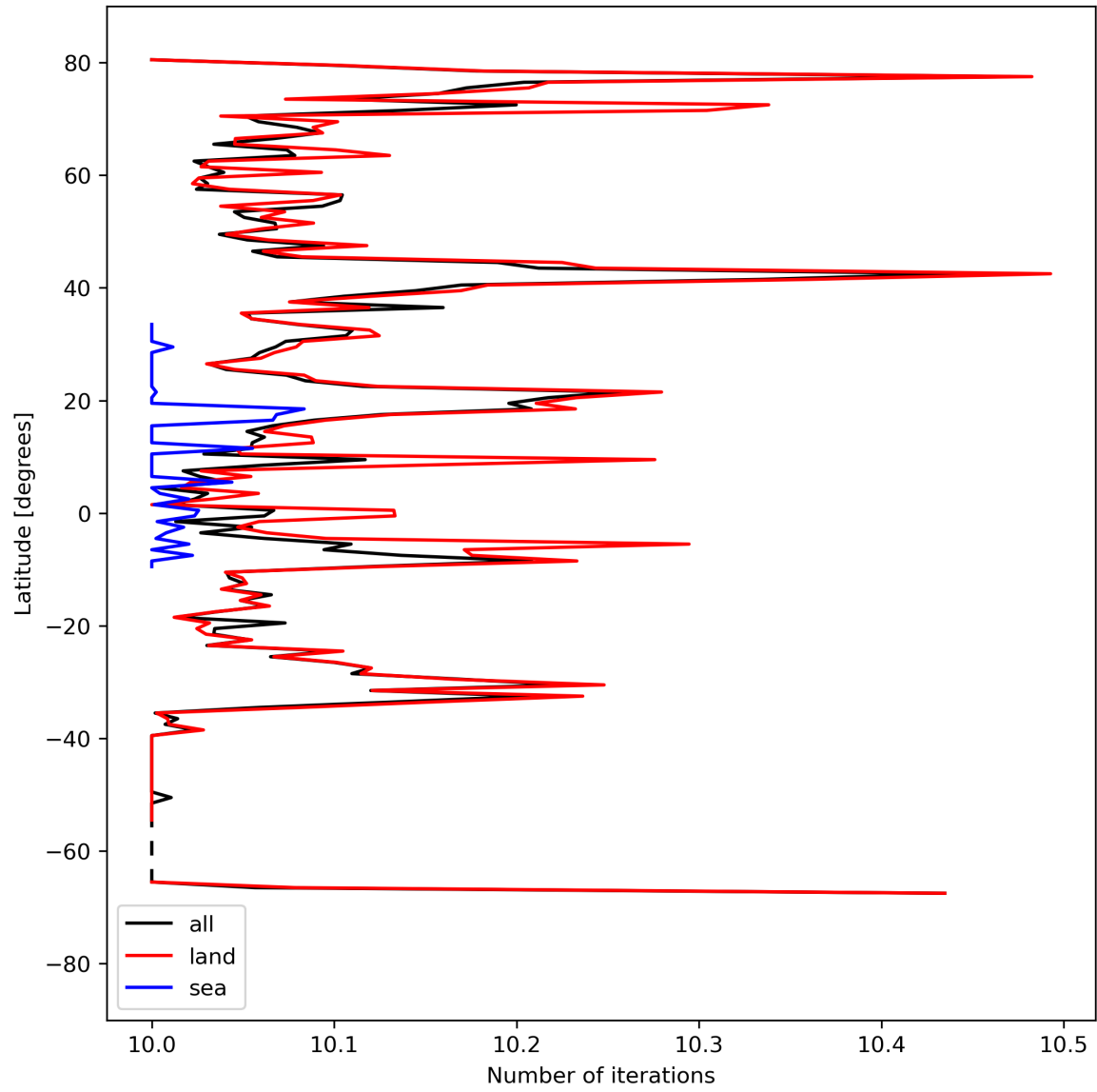
Figure 20: Zonal average of “Number of iterations” for 2023-09-07 to 2023-09-09.
