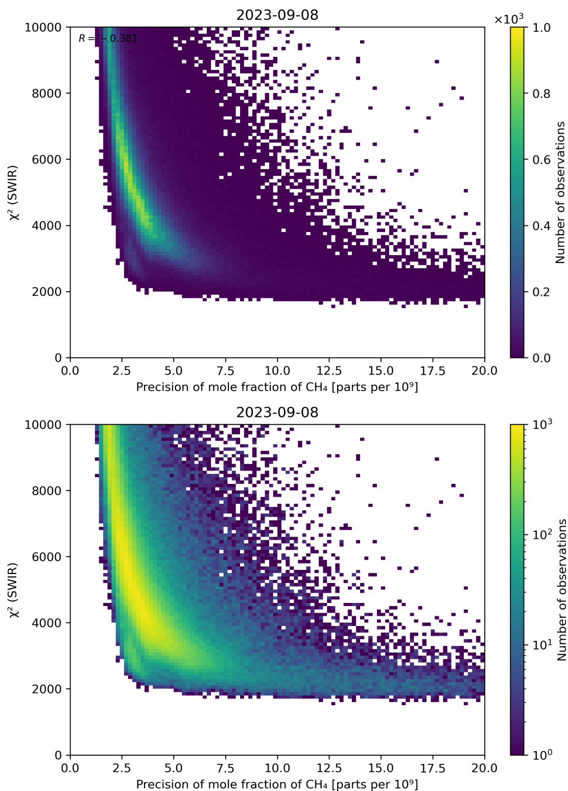
Figure 79: Scatter density plot of “Precision of mole fraction of CH 4 ” against “ \chi^2 (SWIR)” for 2023-09-07 to 2023-09-09.
