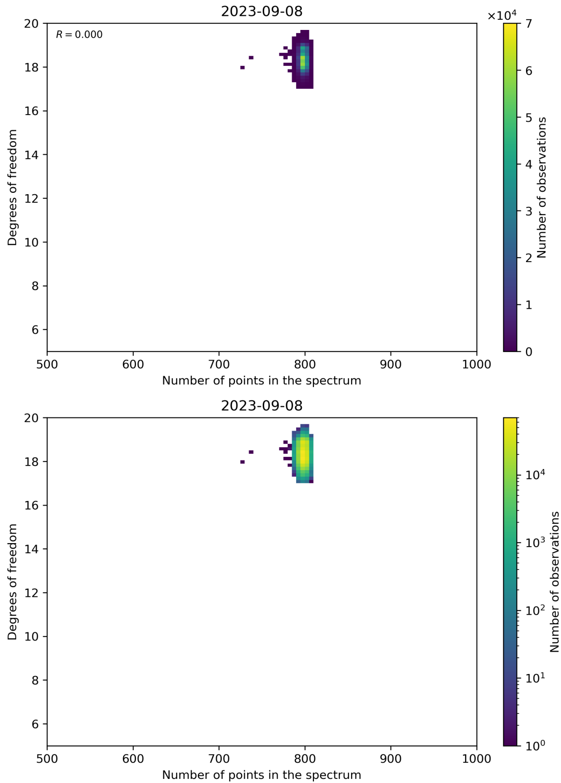
Figure 90: Scatter density plot of “Number of points in the spectrum” against “Degrees of freedom” for 2023-09-07 to 2023-09-09.
