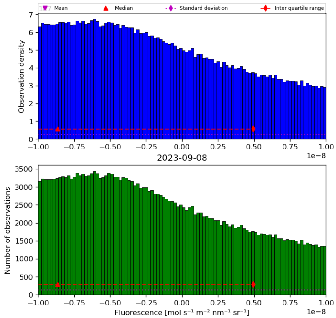
Figure 32: Histogram of “Fluorescence” for 2023-09-07 to 2023-09-09
