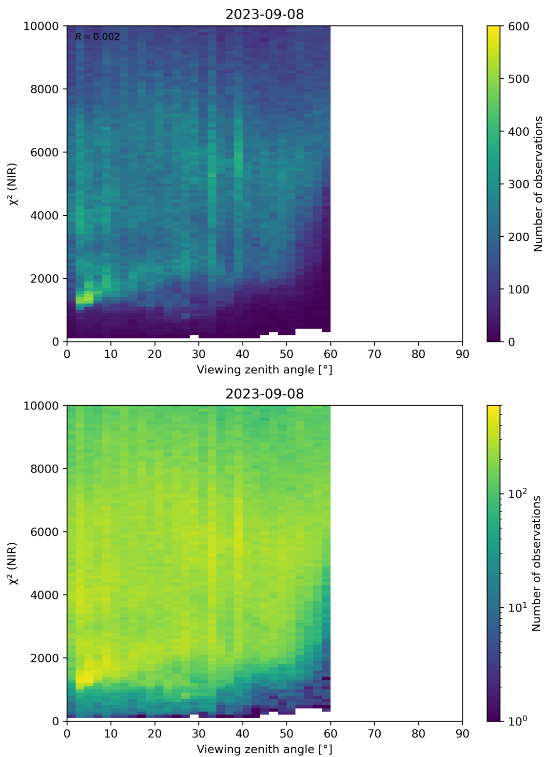
Figure 105: Scatter density plot of “Viewing zenith angle” against “ \chi^2 (NIR)” for 2023-09-07 to 2023-09-09.
