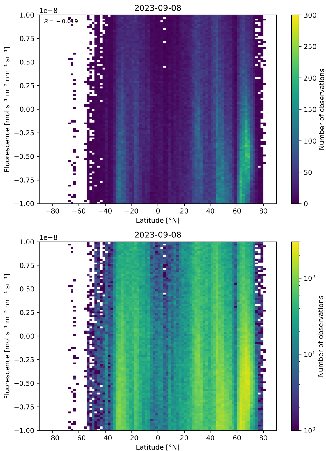
Figure 56: Scatter density plot of “Latitude” against “Fluorescence” for 2023-09-07 to 2023-09-09.
