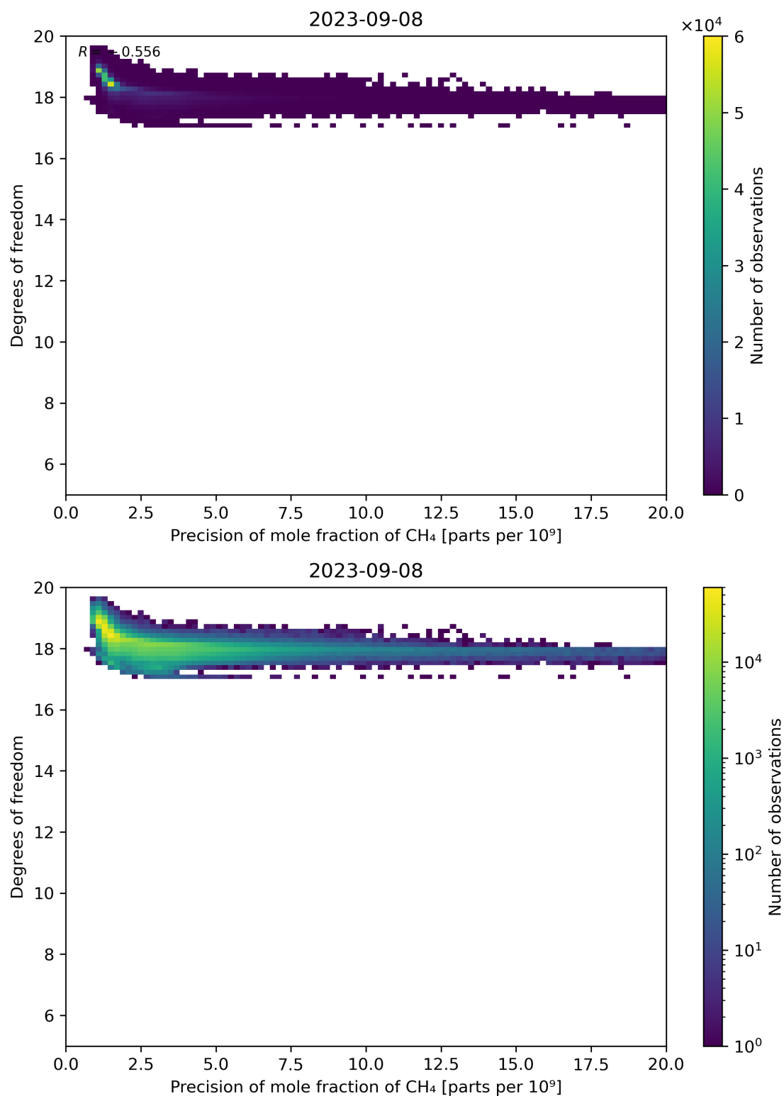
Figure 80: Scatter density plot of “Precision of mole fraction of CH 4 ” against “Degrees of freedom” for 2023-09-07 to 2023-09-09.
