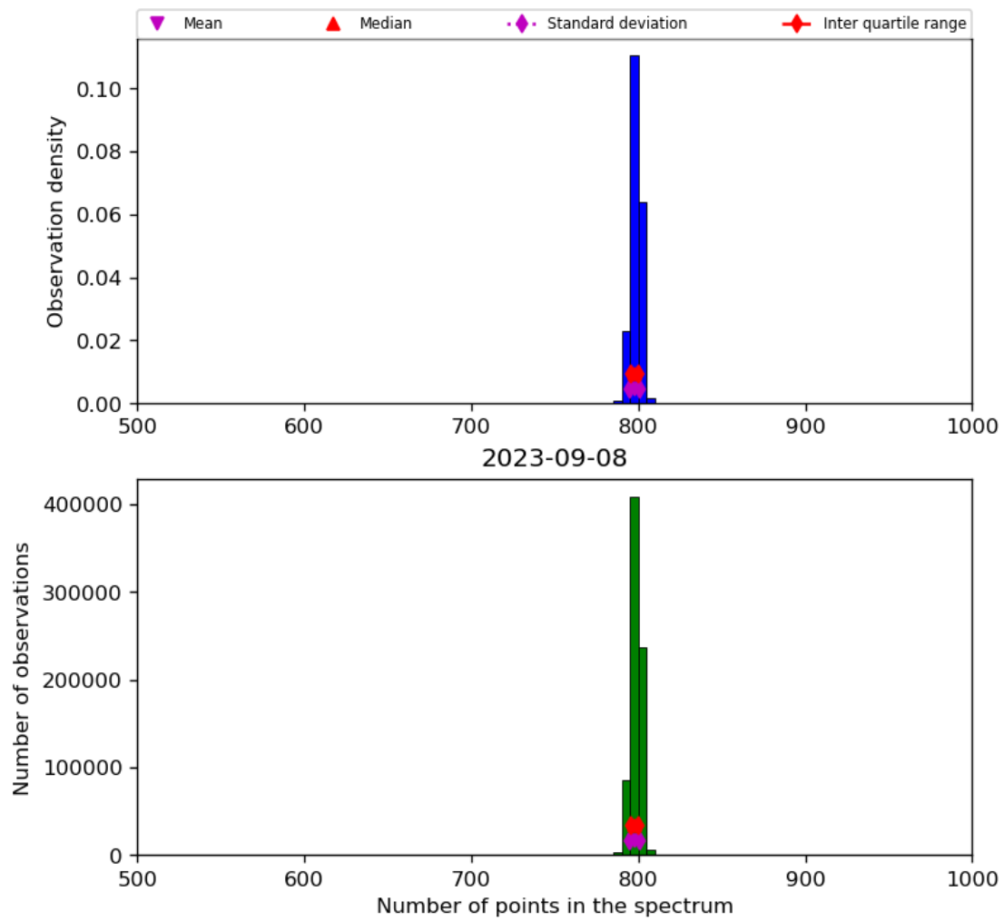
Figure 26: Histogram of “Number of points in the spectrum” for 2023-09-07 to 2023-09-09
