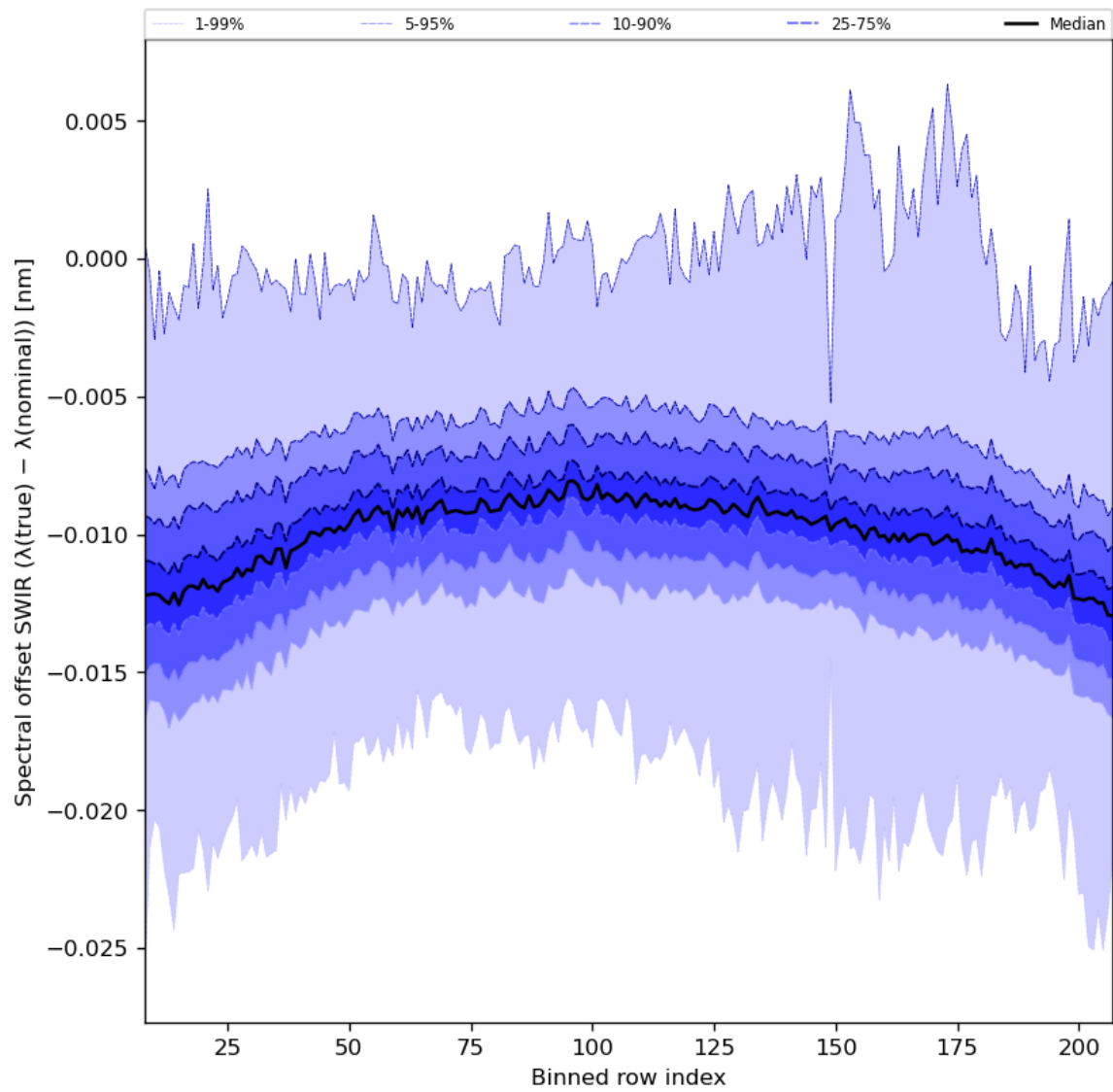
Figure 38: Along track statistics of “Spectral offset SWIR ( \lambda(\text{true}) - \lambda(\text{nominal}) )” for 2023-09-07 to 2023-09-09
