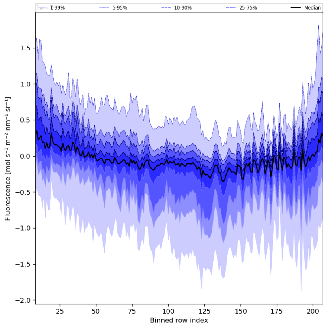
Figure 43: Along track statistics of “Fluorescence” for 2023-09-07 to 2023-09-09
