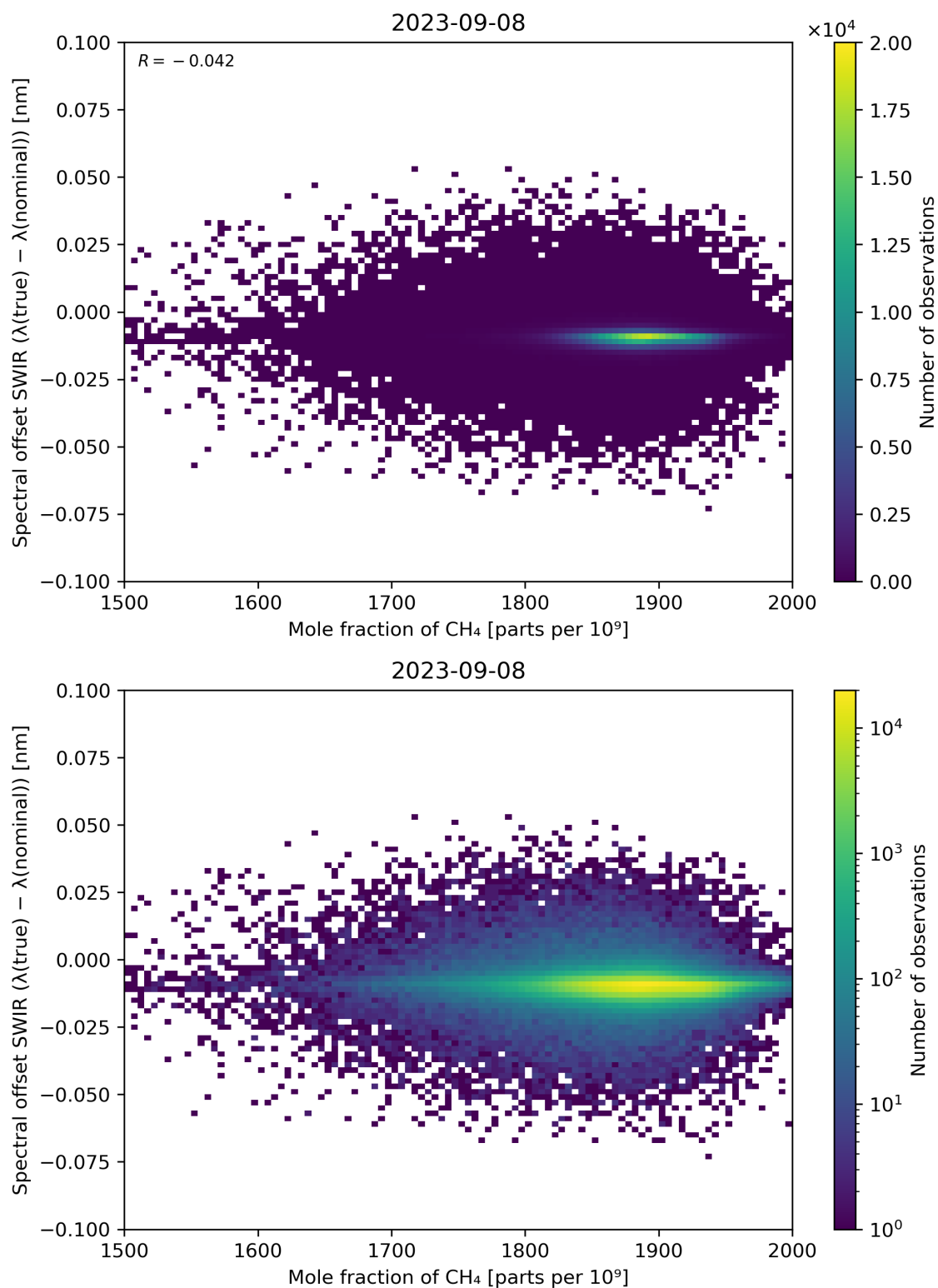
Figure 86: Scatter density plot of “Mole fraction of CH 4 ” against “Spectral offset SWIR ( \lambda(\text{true}) - \lambda(\text{nominal}) )” for 2023-09-07 to 2023-09-09.
