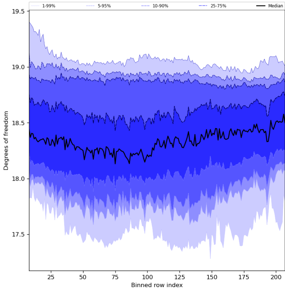
Figure 41: Along track statistics of “Degrees of freedom” for 2023-09-07 to 2023-09-09
