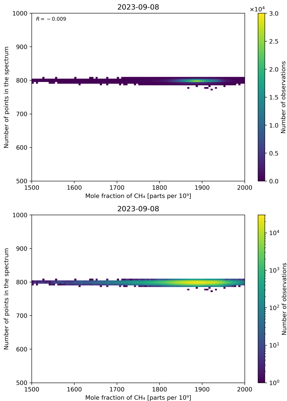
Figure 77: Scatter density plot of “Mole fraction of CH 4 ” against “Number of points in the spectrum” for 2023-09-07 to 2023-09-09.
