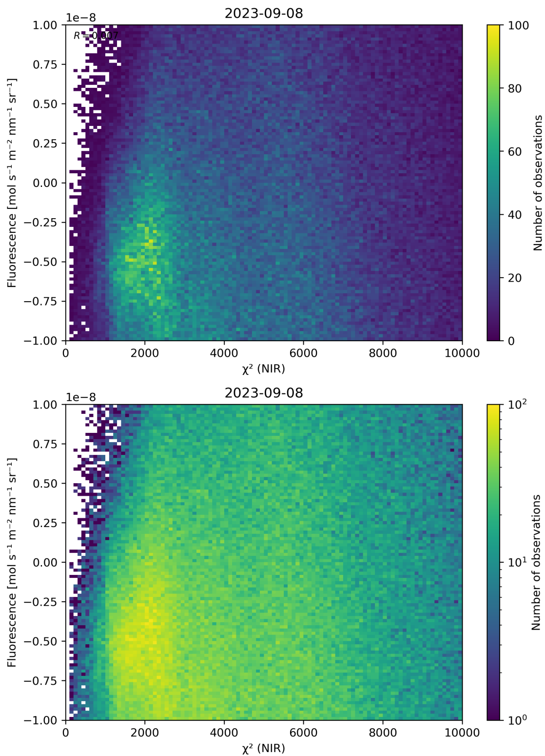
Figure 45: Scatter density plot of “ \chi^2 (NIR)” against “Fluorescence” for 2023-09-07 to 2023-09-09.
