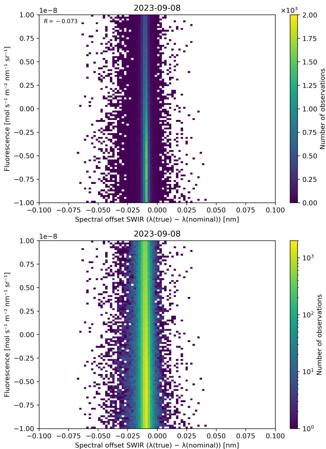
Figure 120: Scatter density plot of “Spectral offset SWIR ( \lambda(\text{true}) - \lambda(\text{nominal}) )” against “Fluorescence” for 2023-09-07 to 2023-09-09.
