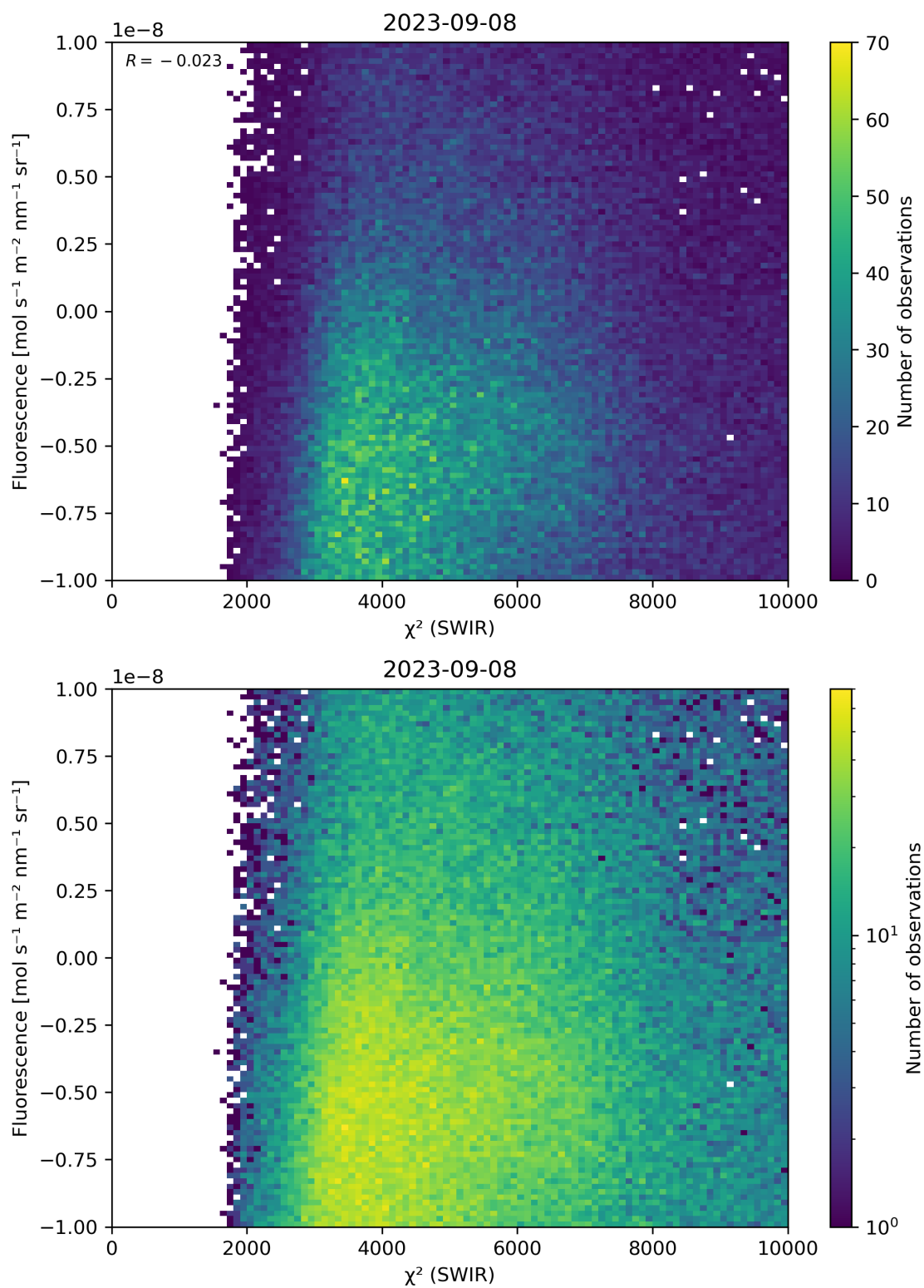
Figure 49: Scatter density plot of “ \chi^2 (SWIR)” against “Fluorescence” for 2023-09-07 to 2023-09-09.
