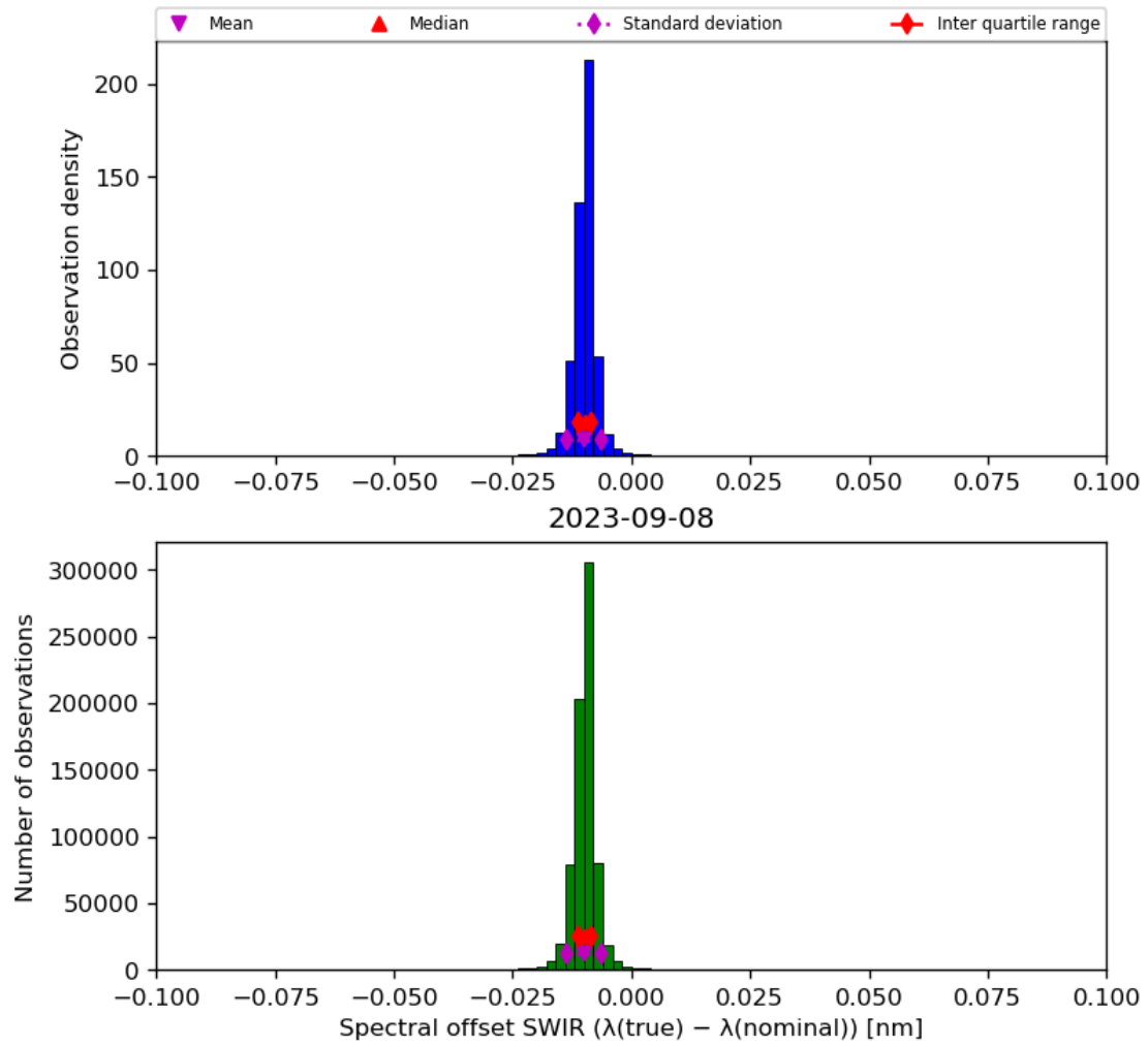
Figure 27: Histogram of “Spectral offset SWIR ( \lambda(\text{true}) - \lambda(\text{nominal}) )” for 2023-09-07 to 2023-09-09
