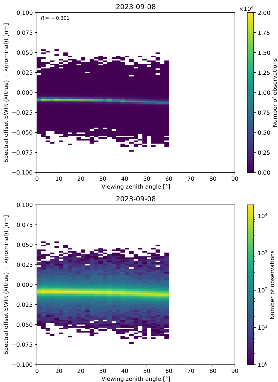
Figure 116: Scatter density plot of “Viewing zenith angle” against “Spectral offset SWIR ( \lambda(\text{true}) - \lambda(\text{nominal}) )” for 2023-09-07 to 2023-09-09.
