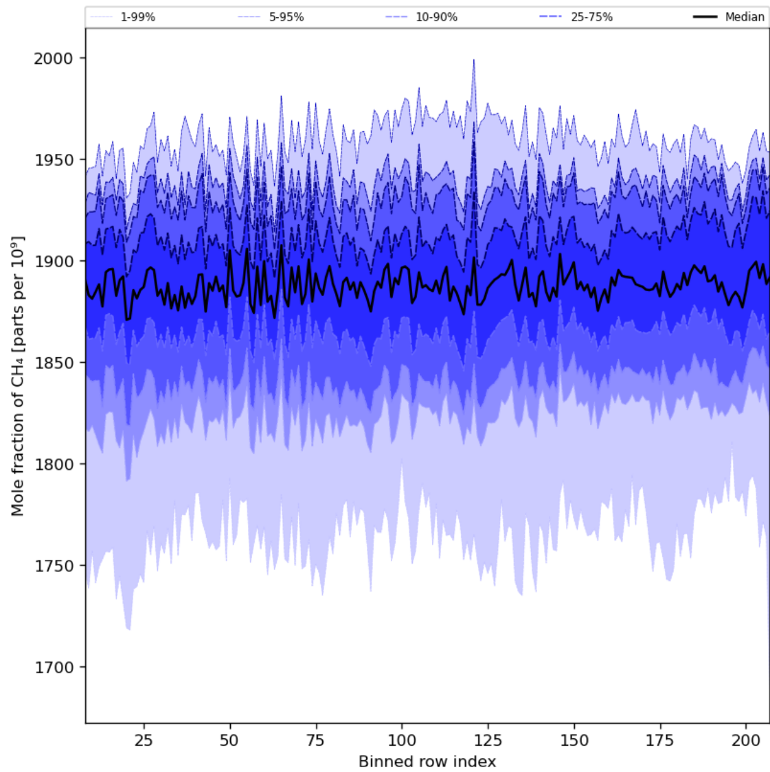
Figure 34: Along track statistics of “Mole fraction of CH 4 ” for 2023-09-07 to 2023-09-09
