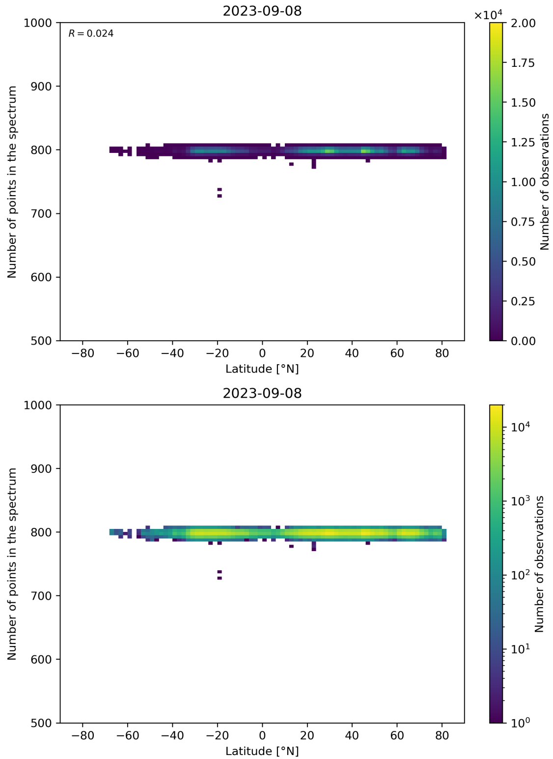
Figure 61: Scatter density plot of “Latitude” against “Number of points in the spectrum” for 2023-09-07 to 2023-09-09.
