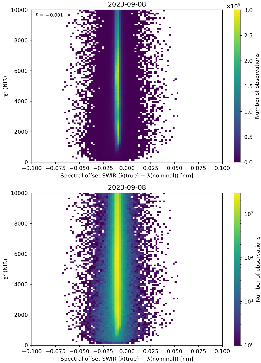
Figure 117: Scatter density plot of “Spectral offset SWIR ( \lambda(\text{true}) - \lambda(\text{nominal}) )” against “ \chi^2 (NIR)” for 2023-09-07 to 2023-09-09.
