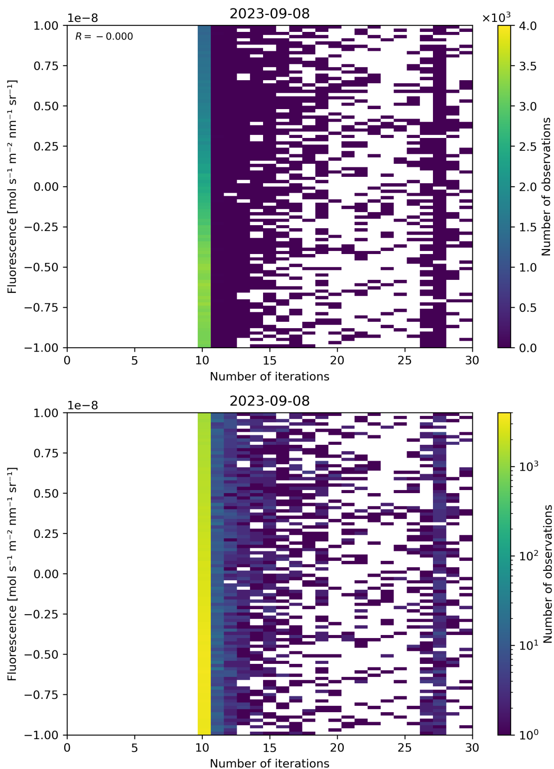
Figure 87: Scatter density plot of “Number of iterations” against “Fluorescence” for 2023-09-07 to 2023-09-09.
