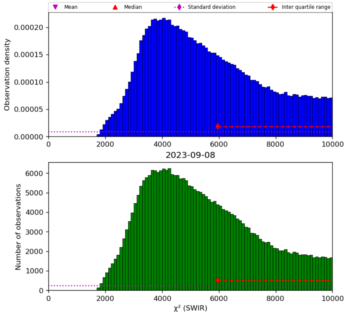
Figure 28: Histogram of " \chi^2 (SWIR)" for 2023-09-07 to 2023-09-09
