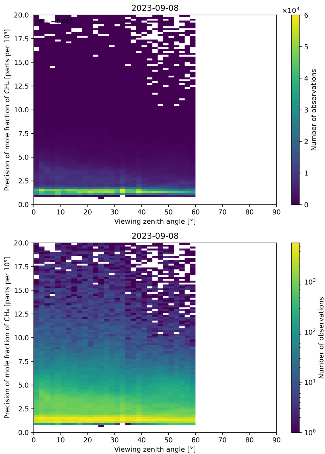
Figure 112: Scatter density plot of “Viewing zenith angle” against “Precision of mole fraction of CH 4 ” for 2023-09-07 to 2023-09-09.
