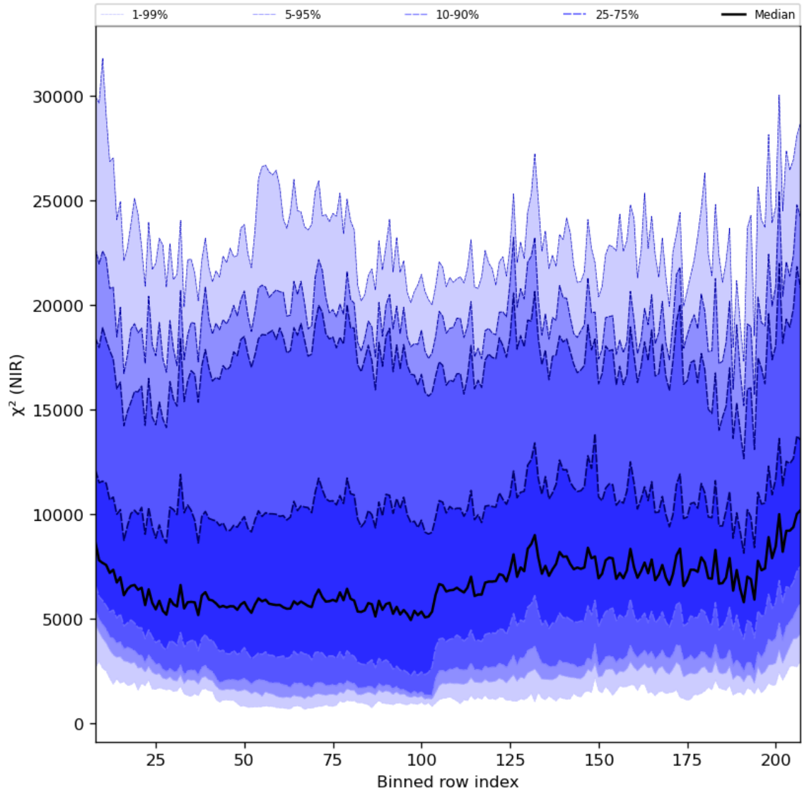
Figure 40: Along track statistics of “ \chi^2 (NIR)” for 2023-09-07 to 2023-09-09
