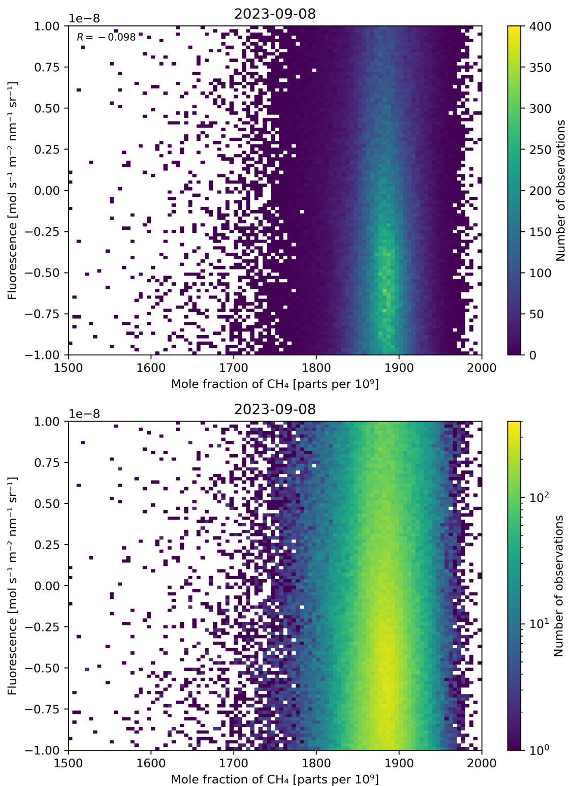
Figure 73: Scatter density plot of “Mole fraction of CH 4 ” against “Fluorescence” for 2023-09-07 to 2023-09-09.
