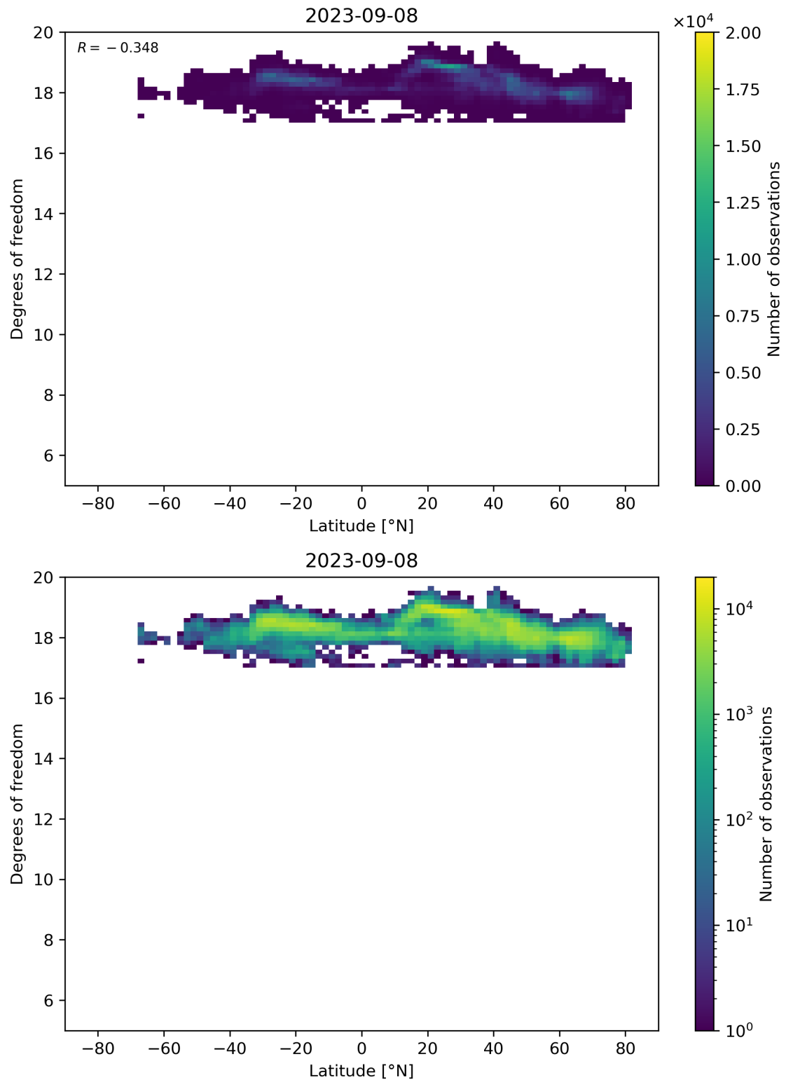
Figure 55: Scatter density plot of “Latitude” against “Degrees of freedom” for 2023-09-07 to 2023-09-09.
