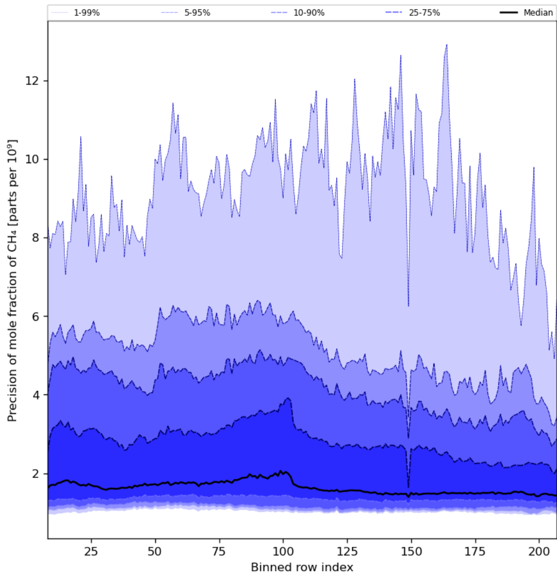
Figure 35: Along track statistics of "Precision of mole fraction of CH 4 " for 2023-09-07 to 2023-09-09
