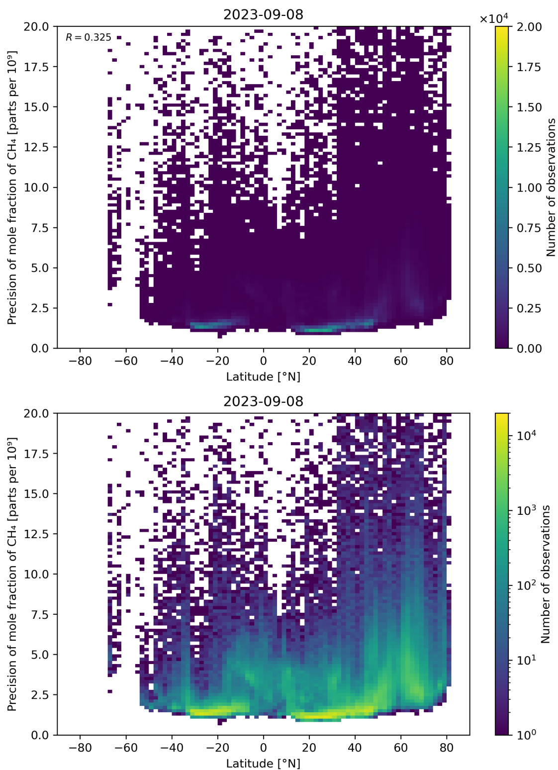
Figure 59: Scatter density plot of “Latitude” against “Precision of mole fraction of \text{CH}_4 ” for 2023-09-07 to 2023-09-09.
