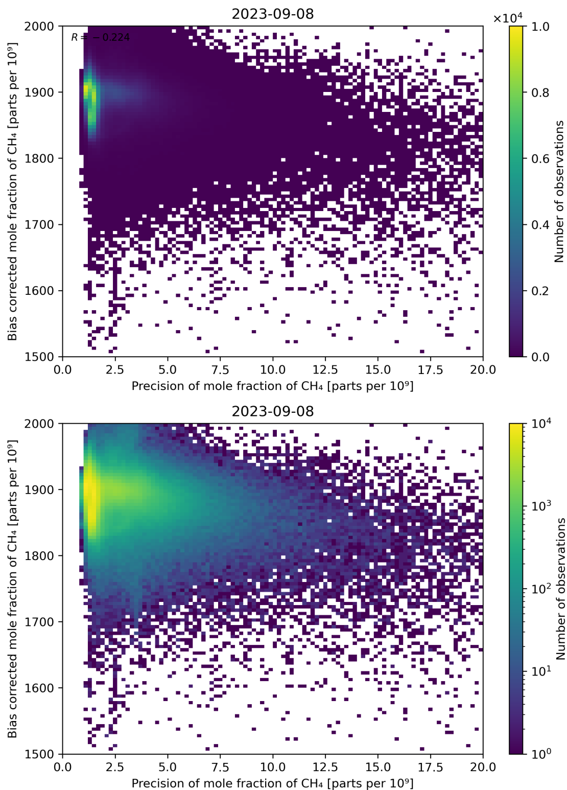
Figure 82: Scatter density plot of “Precision of mole fraction of \text{CH}_4 ” against “Bias corrected mole fraction of \text{CH}_4 ” for 2023-09-07 to 2023-09-09.
