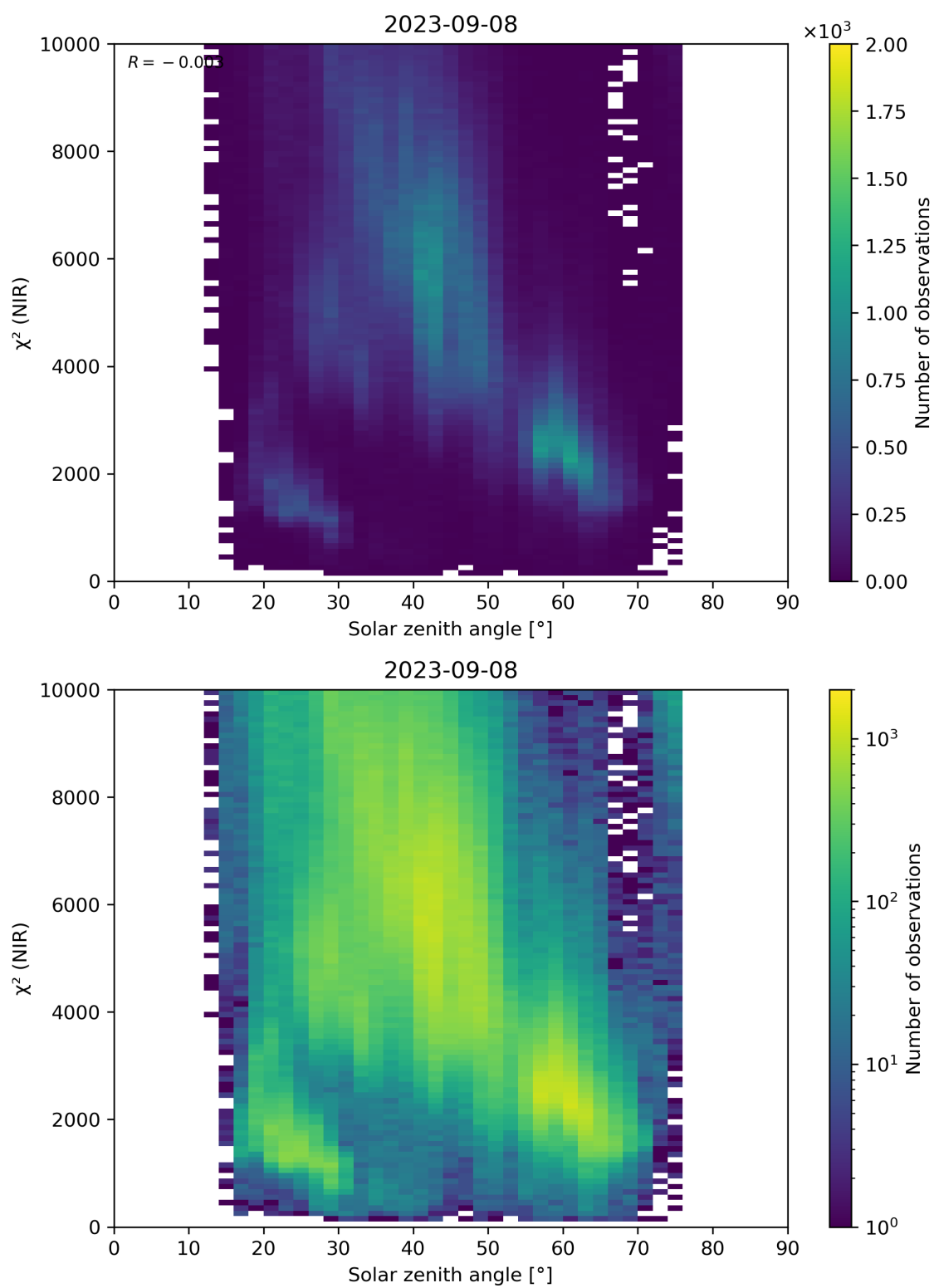
Figure 94: Scatter density plot of “Solar zenith angle” against “ \chi^2 (NIR)” for 2023-09-07 to 2023-09-09.
