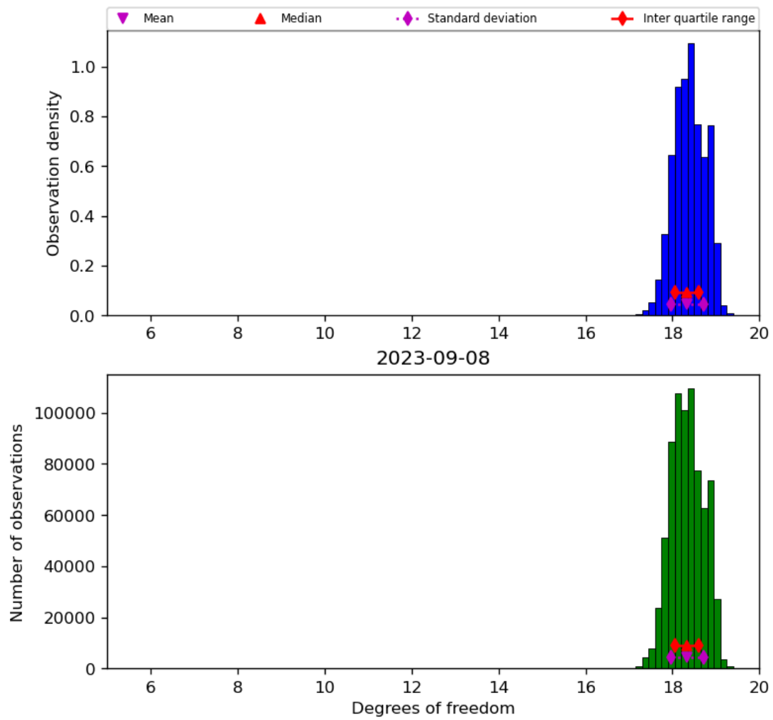
Figure 30: Histogram of “Degrees of freedom” for 2023-09-07 to 2023-09-09
