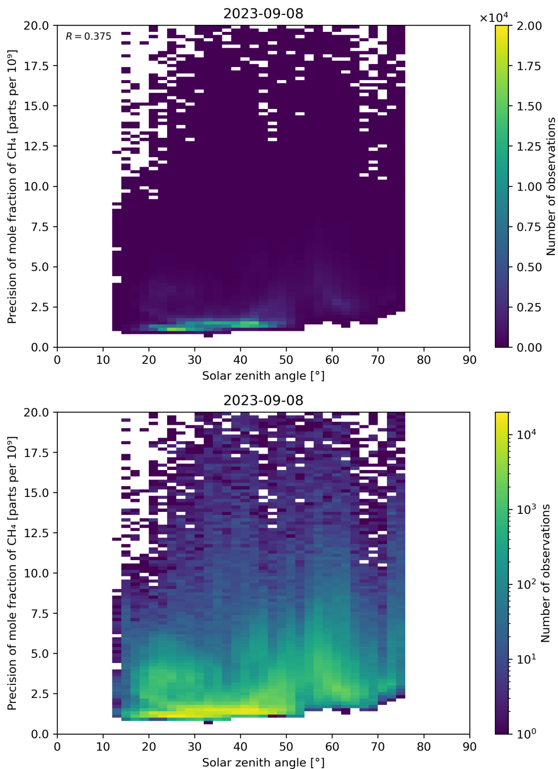
Figure 101: Scatter density plot of “Solar zenith angle” against “Precision of mole fraction of \text{CH}_4 ” for 2023-09-07 to 2023-09-09.
