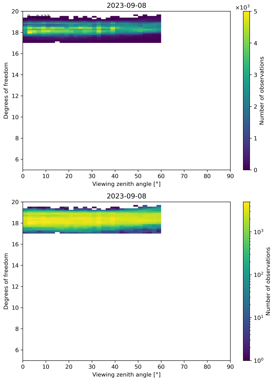
Figure 107: Scatter density plot of “Viewing zenith angle” against “Degrees of freedom” for 2023-09-07 to 2023-09-09.
