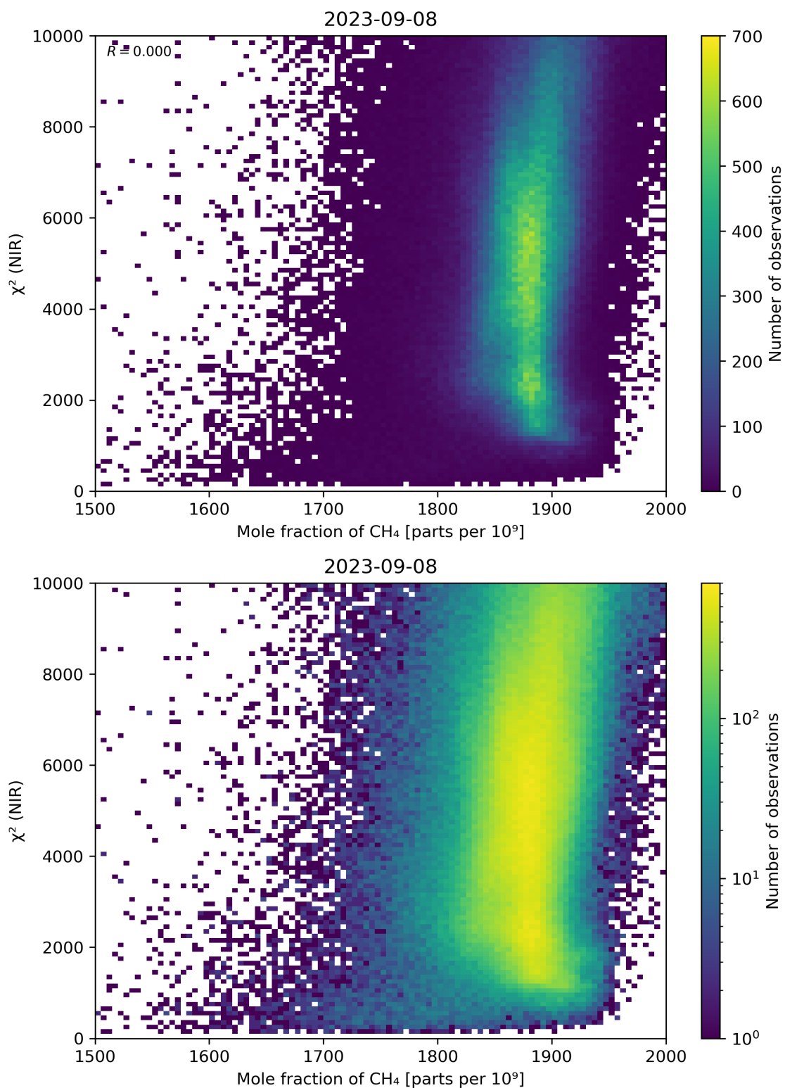
Figure 70: Scatter density plot of “Mole fraction of CH 4 ” against “ \chi^2 (NIR)” for 2023-09-07 to 2023-09-09.
