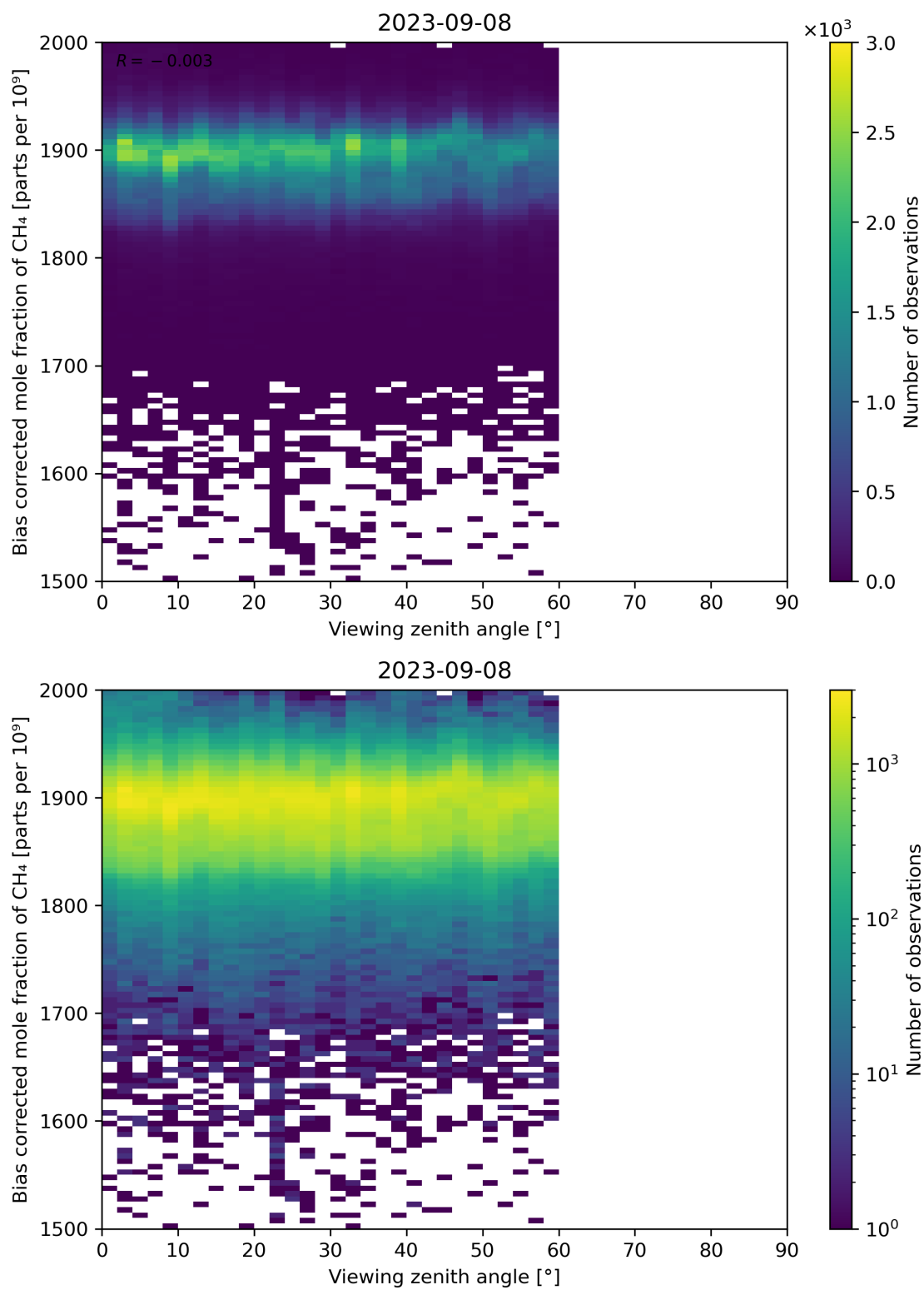
Figure 111: Scatter density plot of “Viewing zenith angle” against “Bias corrected mole fraction of CH 4 ” for 2023-09-07 to 2023-09-09.
