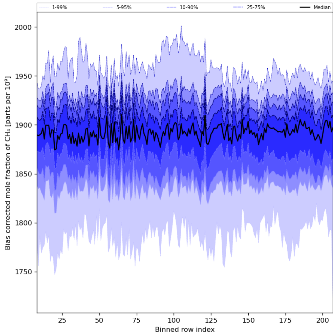
Figure 36: Along track statistics of “Bias corrected mole fraction of CH 4 ” for 2023-09-07 to 2023-09-09
