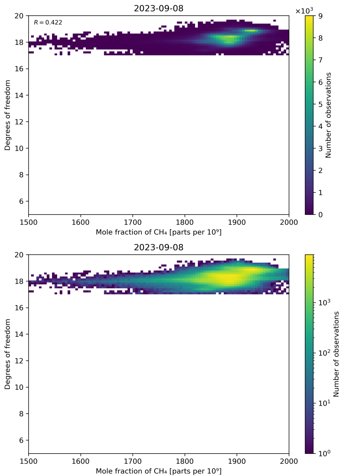
Figure 72: Scatter density plot of “Mole fraction of CH 4 ” against “Degrees of freedom” for 2023-09-07 to 2023-09-09.
