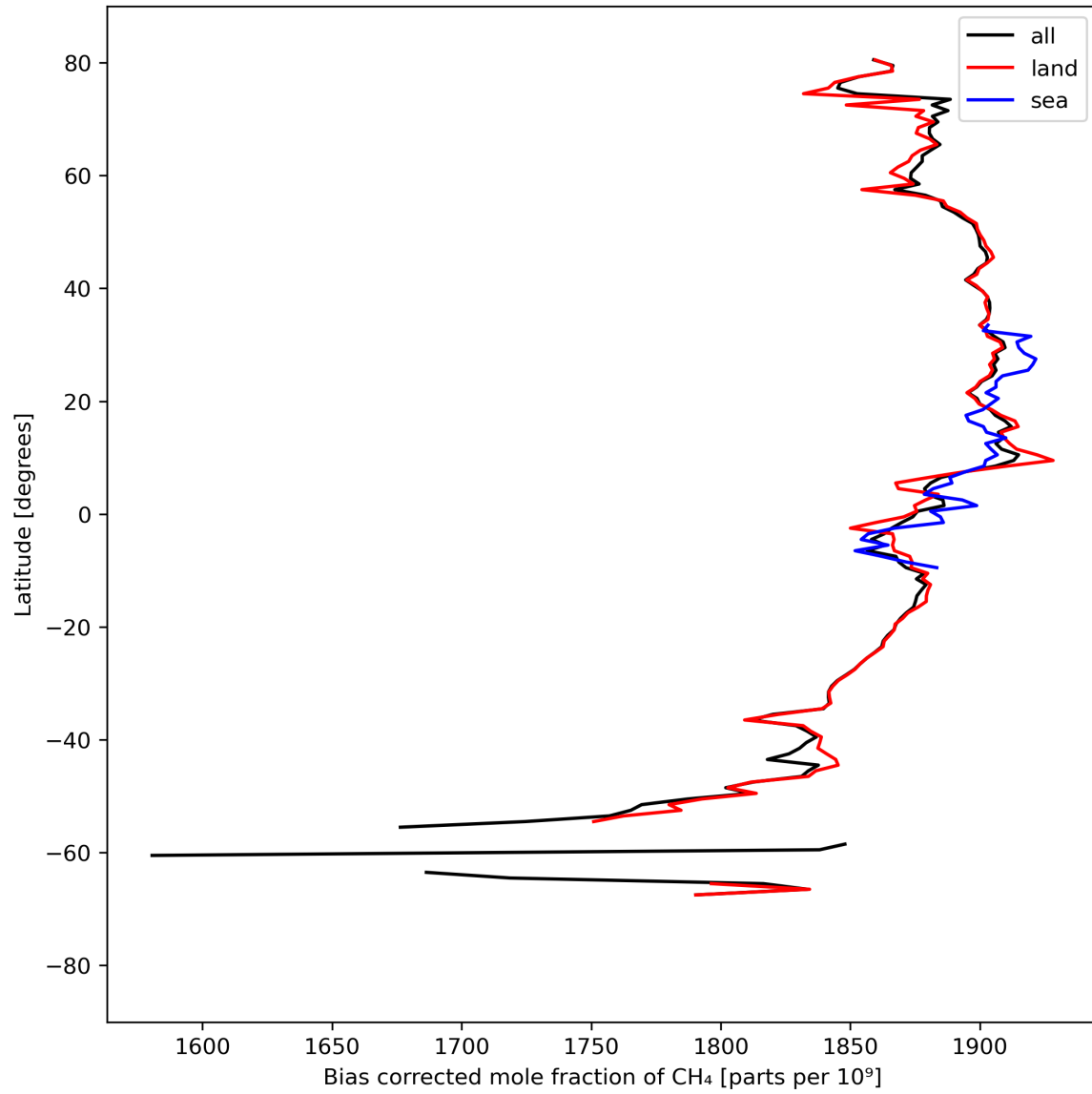
Figure 14: Zonal average of “Bias corrected mole fraction of CH 4 ” for 2023-09-07 to 2023-09-09.
