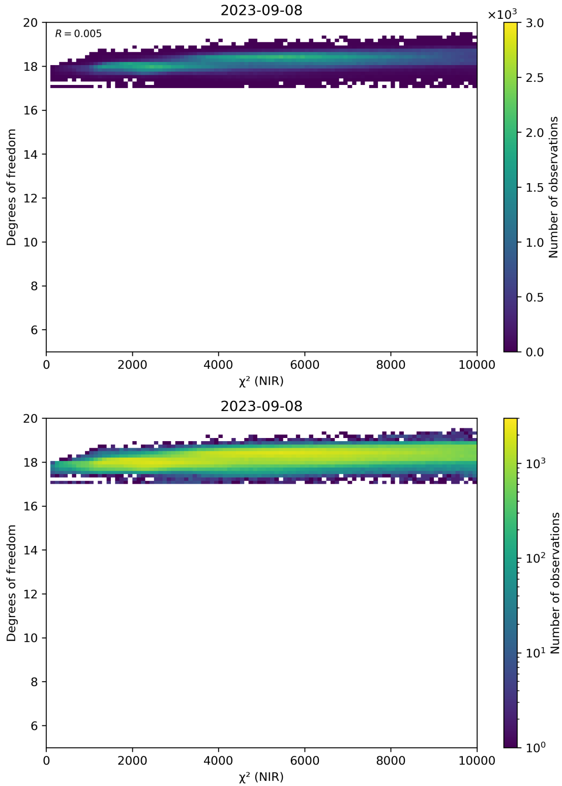
Figure 44: Scatter density plot of “ \chi^2 (NIR)” against “Degrees of freedom” for 2023-09-07 to 2023-09-09.
