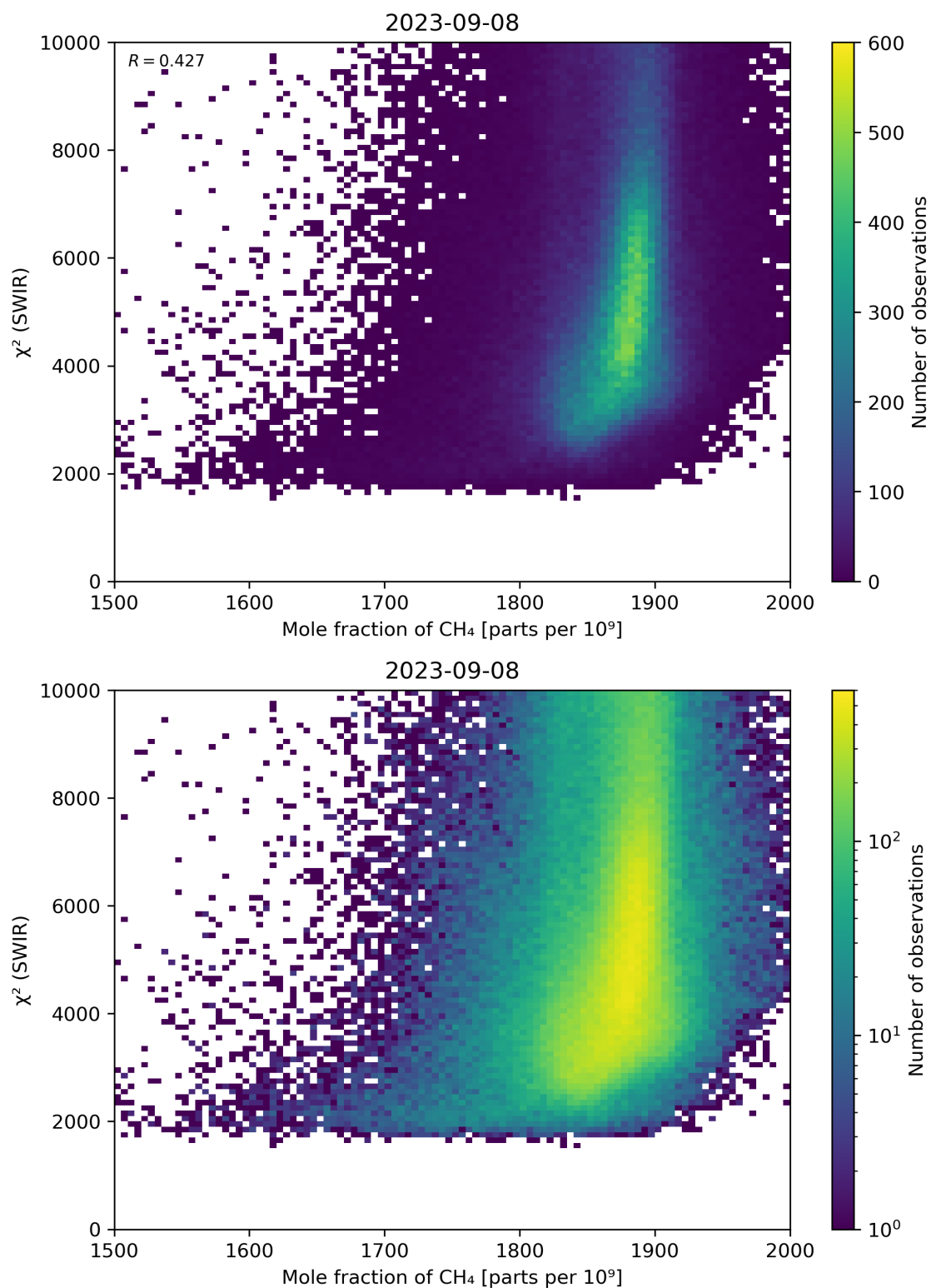
Figure 71: Scatter density plot of “Mole fraction of \text{CH}_4 ” against “ \chi^2 (SWIR)” for 2023-09-07 to 2023-09-09.
