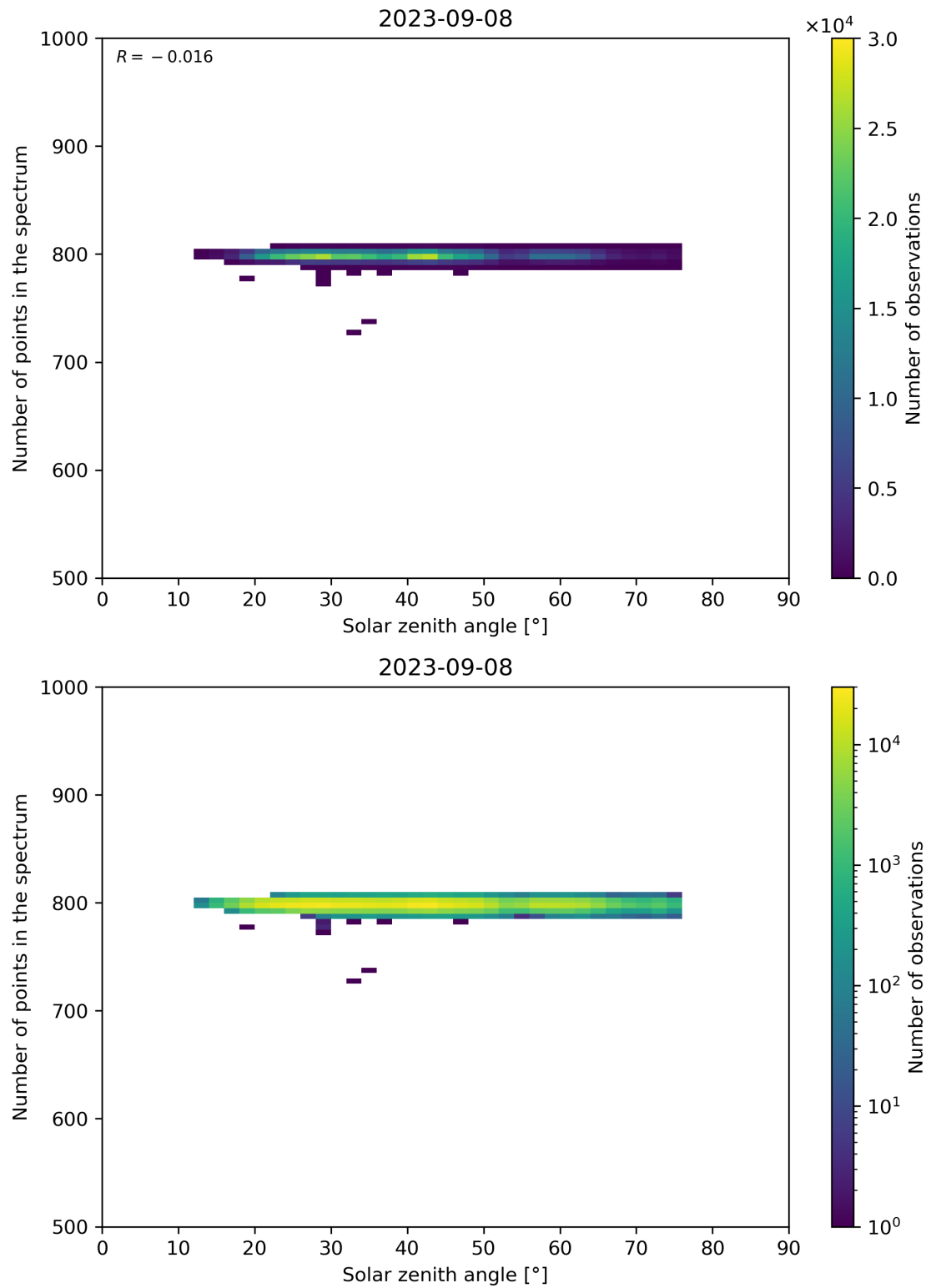
Figure 103: Scatter density plot of “Solar zenith angle” against “Number of points in the spectrum” for 2023-09-07 to 2023-09-09.
