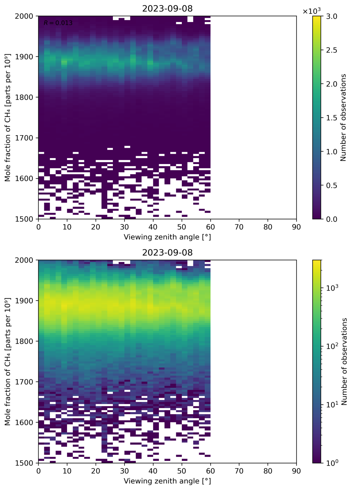
Figure 110: Scatter density plot of “Viewing zenith angle” against “Mole fraction of CH 4 ” for 2023-09-07 to 2023-09-09.
