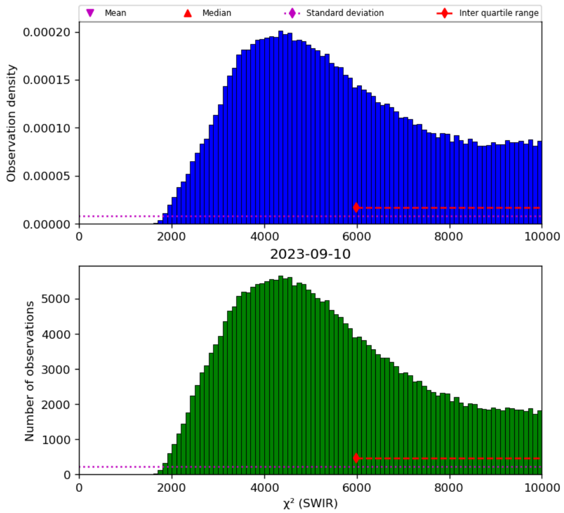
Figure 28: Histogram of “ \chi^2 (SWIR)” for 2023-09-10 to 2023-09-11
