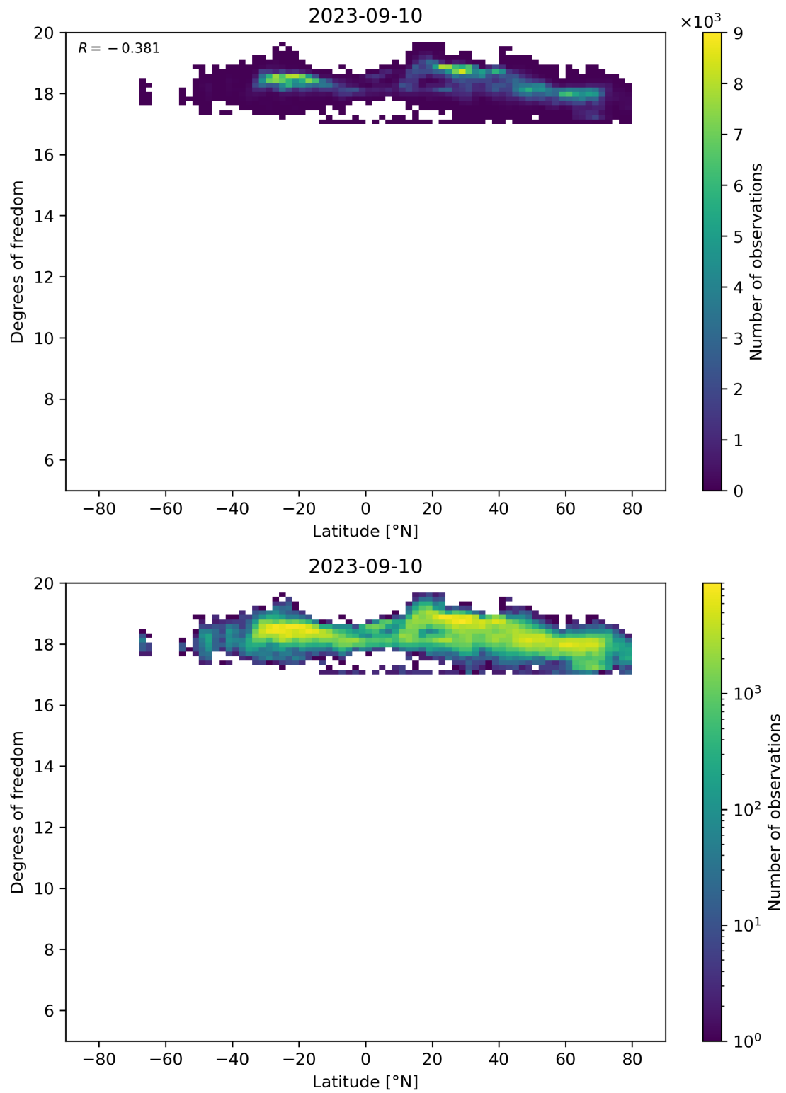
Figure 55: Scatter density plot of “Latitude” against “Degrees of freedom” for 2023-09-10 to 2023-09-11.
