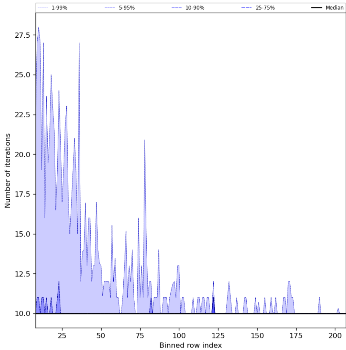
Figure 42: Along track statistics of “Number of iterations” for 2023-09-10 to 2023-09-11
