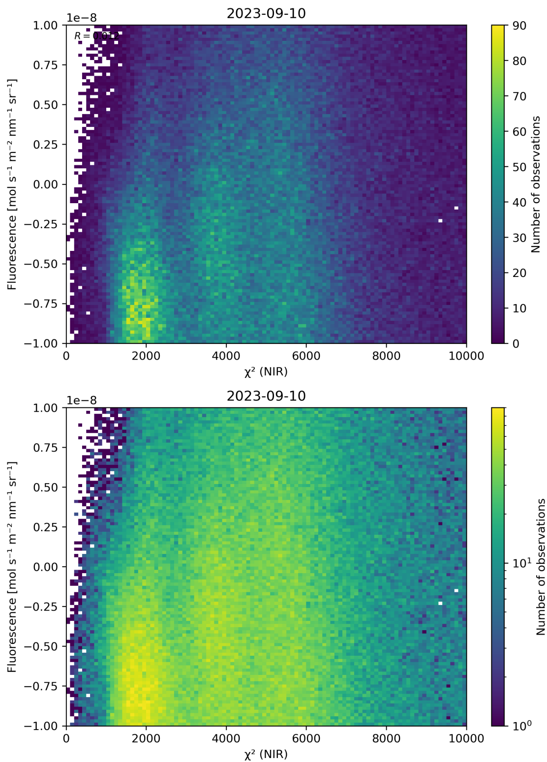
Figure 45: Scatter density plot of “ \chi^2 (NIR)” against “Fluorescence” for 2023-09-10 to 2023-09-11.
