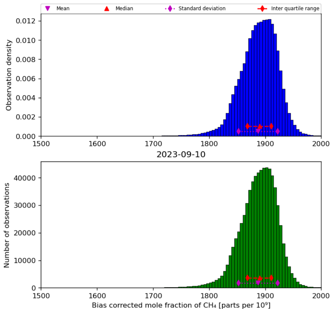
Figure 25: Histogram of “Bias corrected mole fraction of CH 4 ” for 2023-09-10 to 2023-09-11
