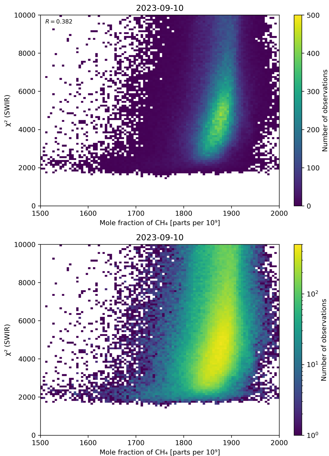
Figure 71: Scatter density plot of “Mole fraction of \text{CH}_4 ” against “ \chi^2 (SWIR)” for 2023-09-10 to 2023-09-11.
