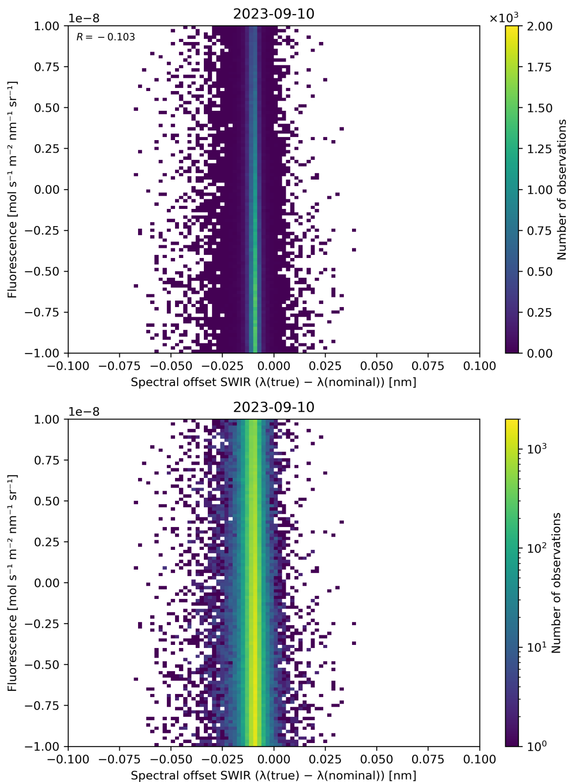
Figure 120: Scatter density plot of “Spectral offset SWIR ( \lambda(\text{true}) - \lambda(\text{nominal}) )” against “Fluorescence” for 2023-09-10 to 2023-09-11.
