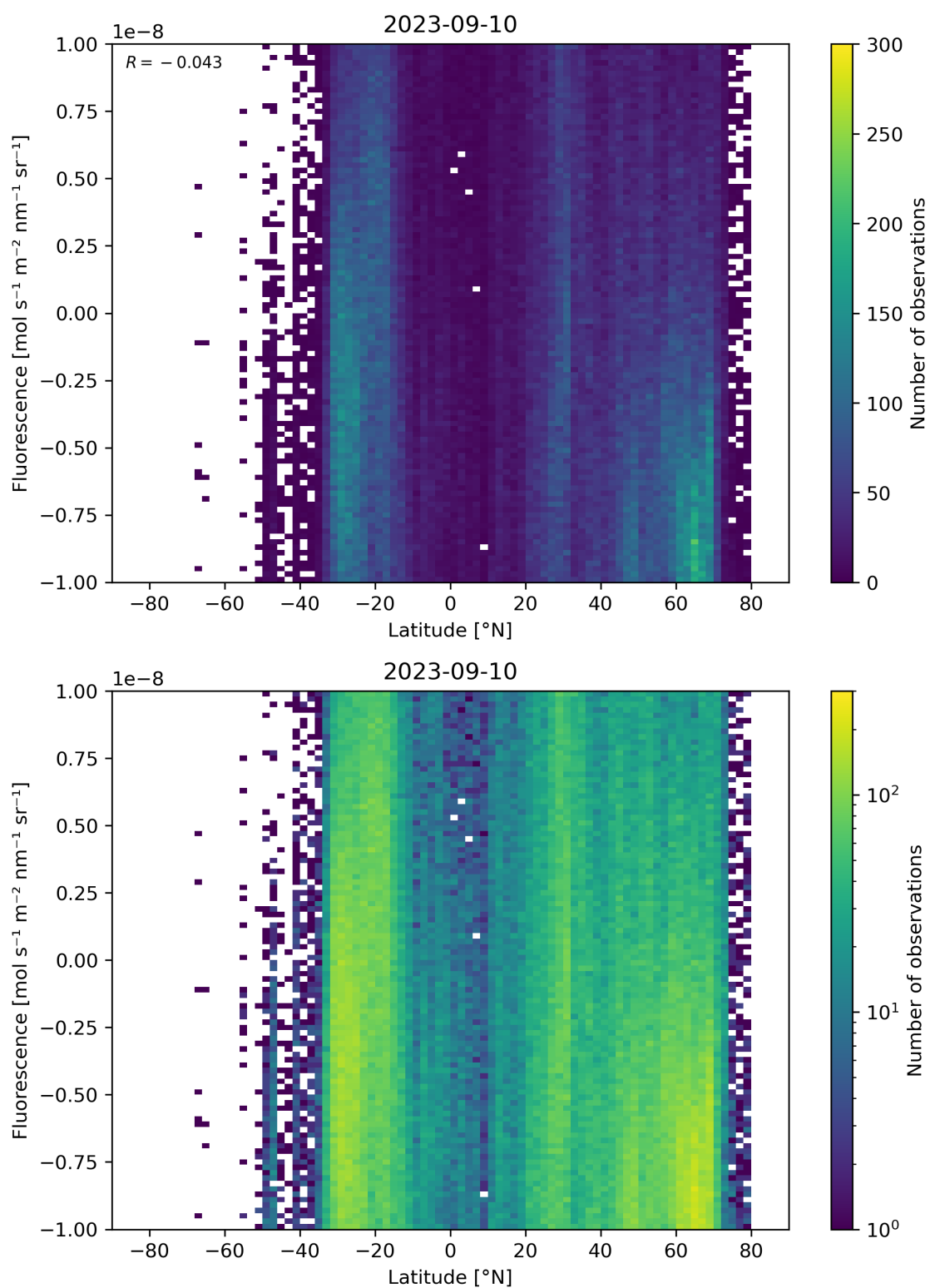
Figure 56: Scatter density plot of “Latitude” against “Fluorescence” for 2023-09-10 to 2023-09-11.
