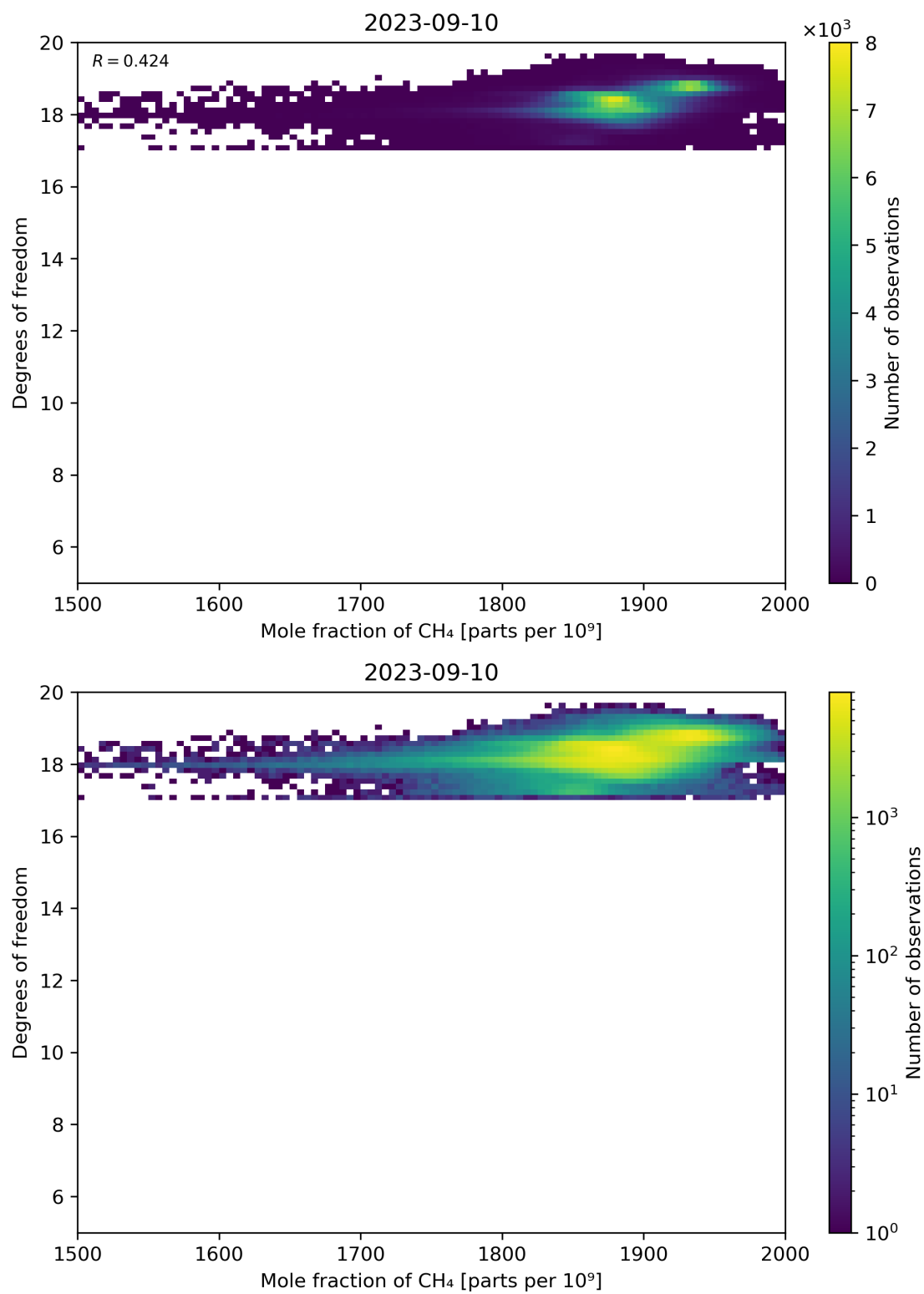
Figure 72: Scatter density plot of “Mole fraction of CH 4 ” against “Degrees of freedom” for 2023-09-10 to 2023-09-11.
