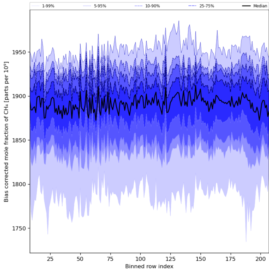
Figure 36: Along track statistics of “Bias corrected mole fraction of CH 4 ” for 2023-09-10 to 2023-09-11
