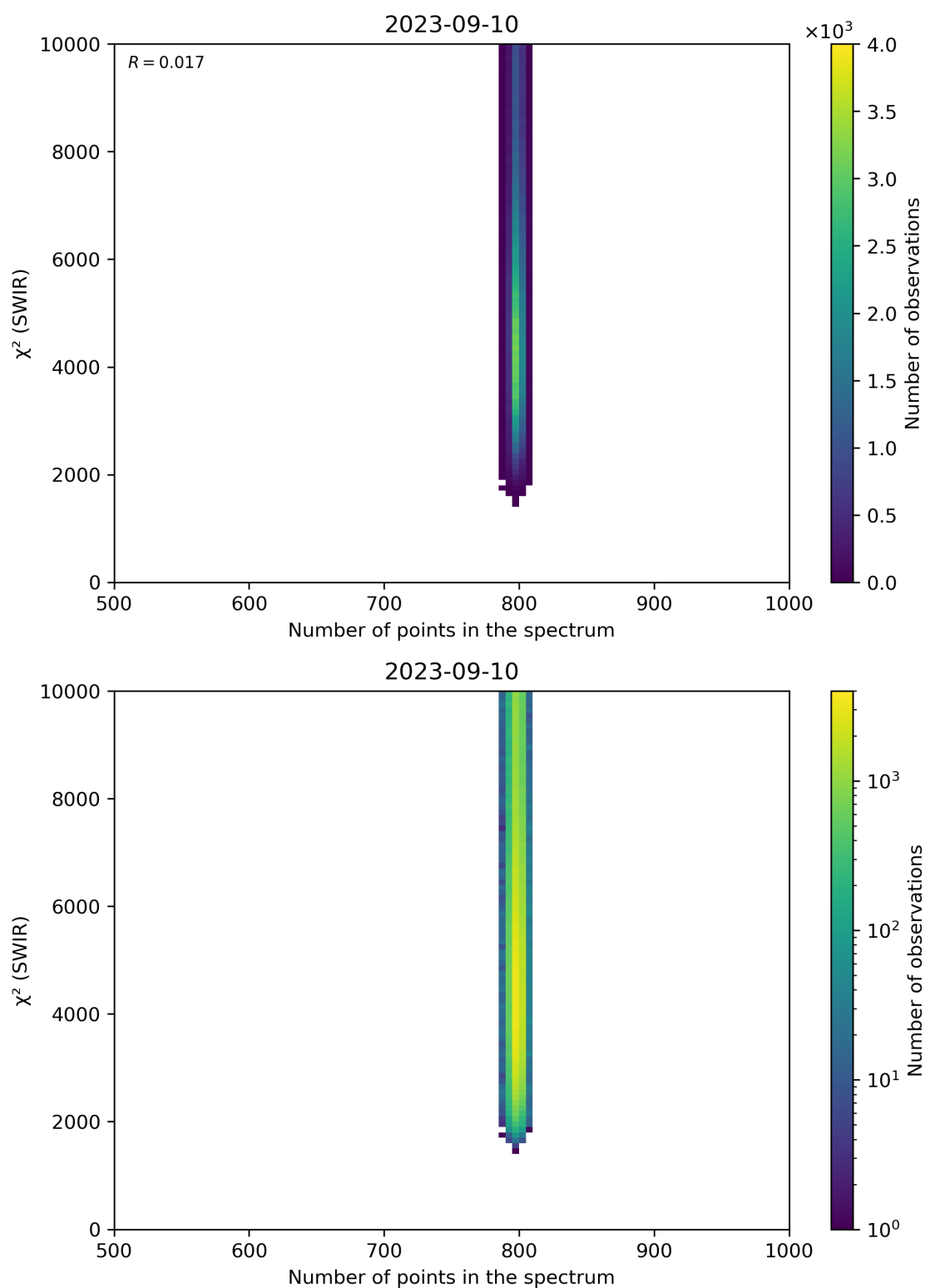
Figure 89: Scatter density plot of “Number of points in the spectrum” against “ \chi^2 (SWIR)” for 2023-09-10 to 2023-09-11.
