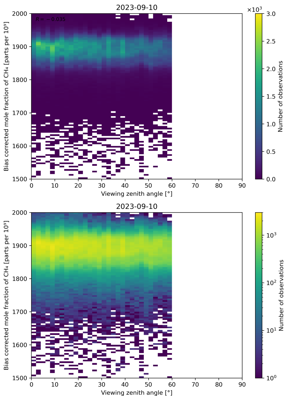
Figure 111: Scatter density plot of “Viewing zenith angle” against “Bias corrected mole fraction of CH 4 ” for 2023-09-10 to 2023-09-11.
