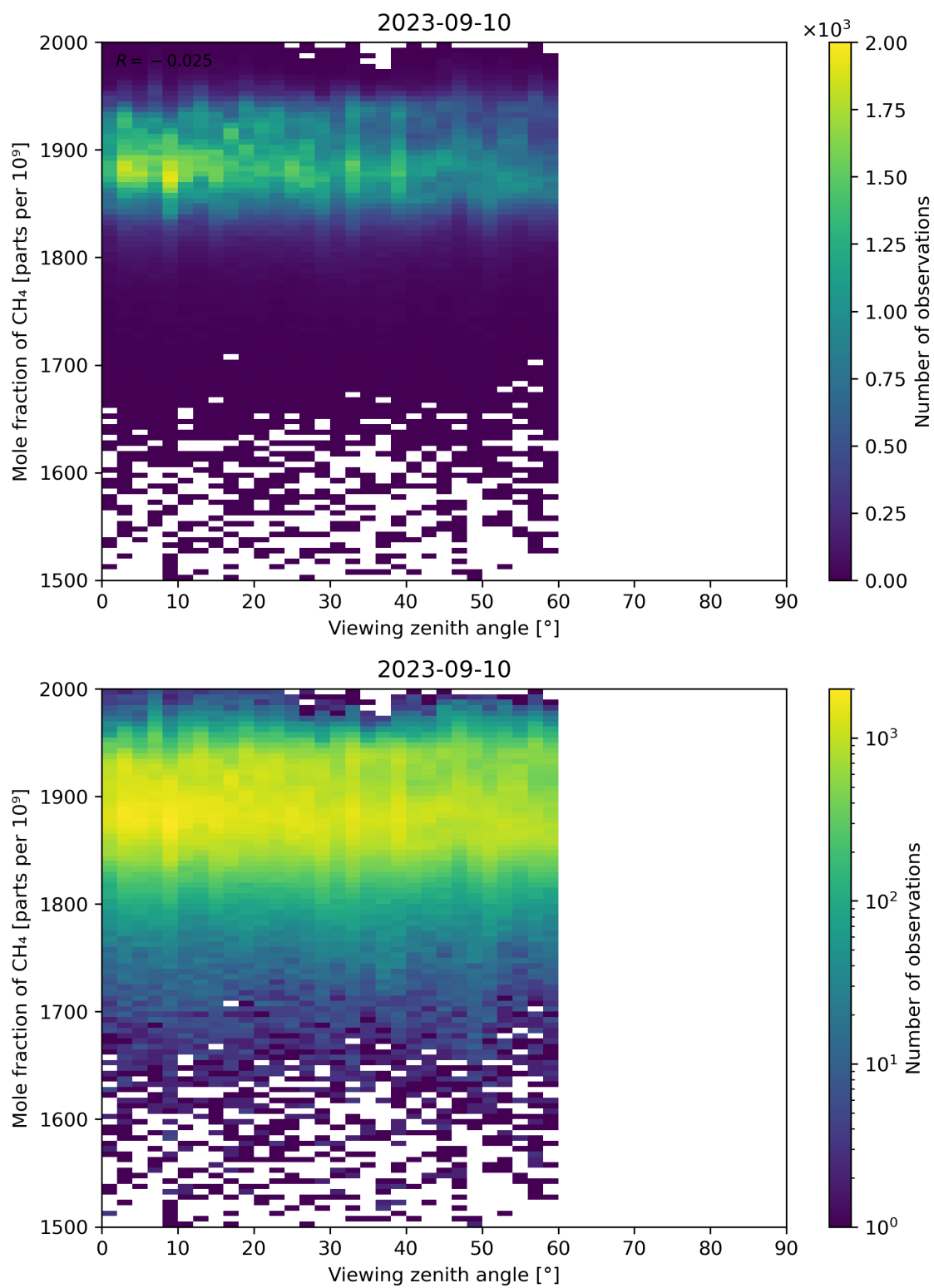
Figure 110: Scatter density plot of “Viewing zenith angle” against “Mole fraction of CH 4 ” for 2023-09-10 to 2023-09-11.
