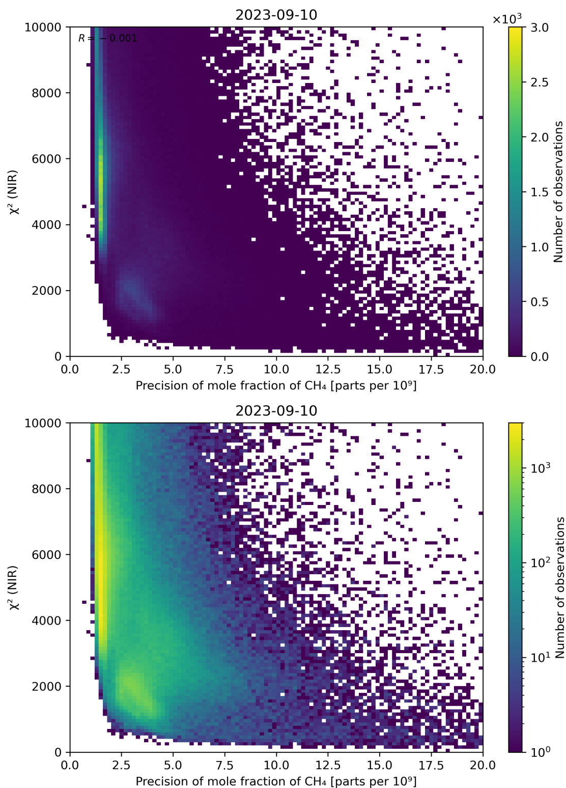
Figure 78: Scatter density plot of “Precision of mole fraction of CH 4 ” against “ \chi^2 (NIR)” for 2023-09-10 to 2023-09-11.
