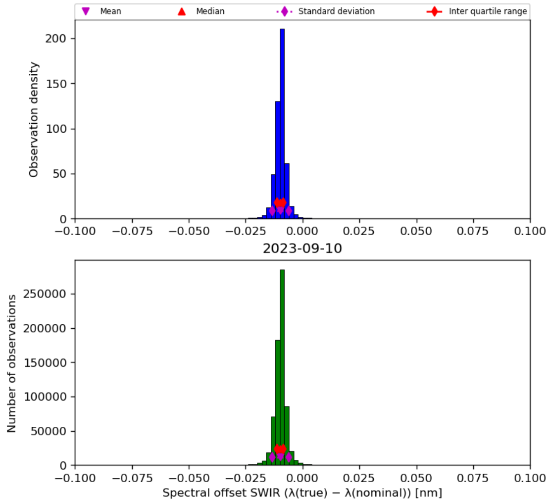
Figure 27: Histogram of “Spectral offset SWIR ( \lambda(\text{true}) - \lambda(\text{nominal}) )” for 2023-09-10 to 2023-09-11
