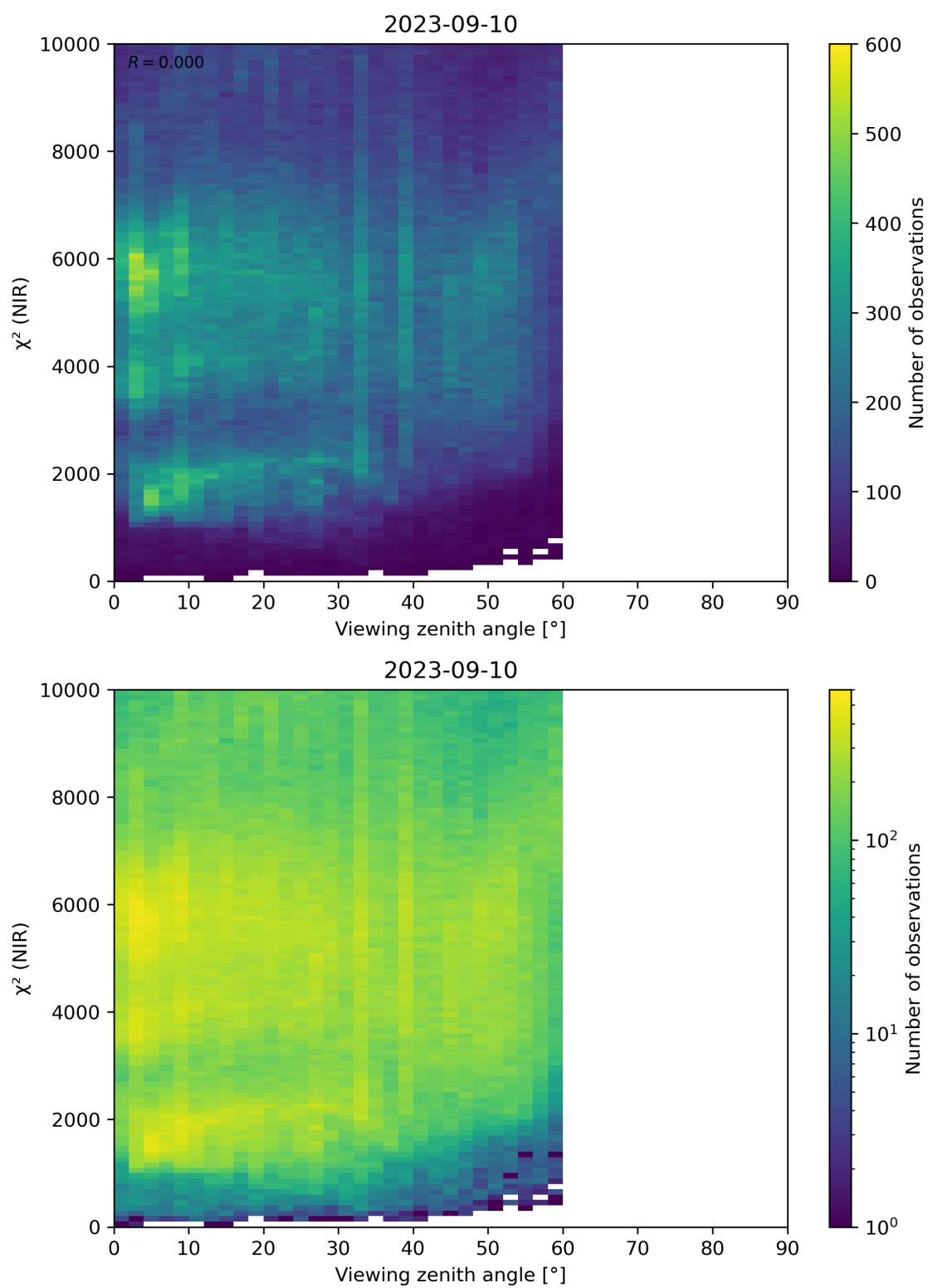
Figure 105: Scatter density plot of “Viewing zenith angle” against “ \chi^2 (NIR)” for 2023-09-10 to 2023-09-11.
