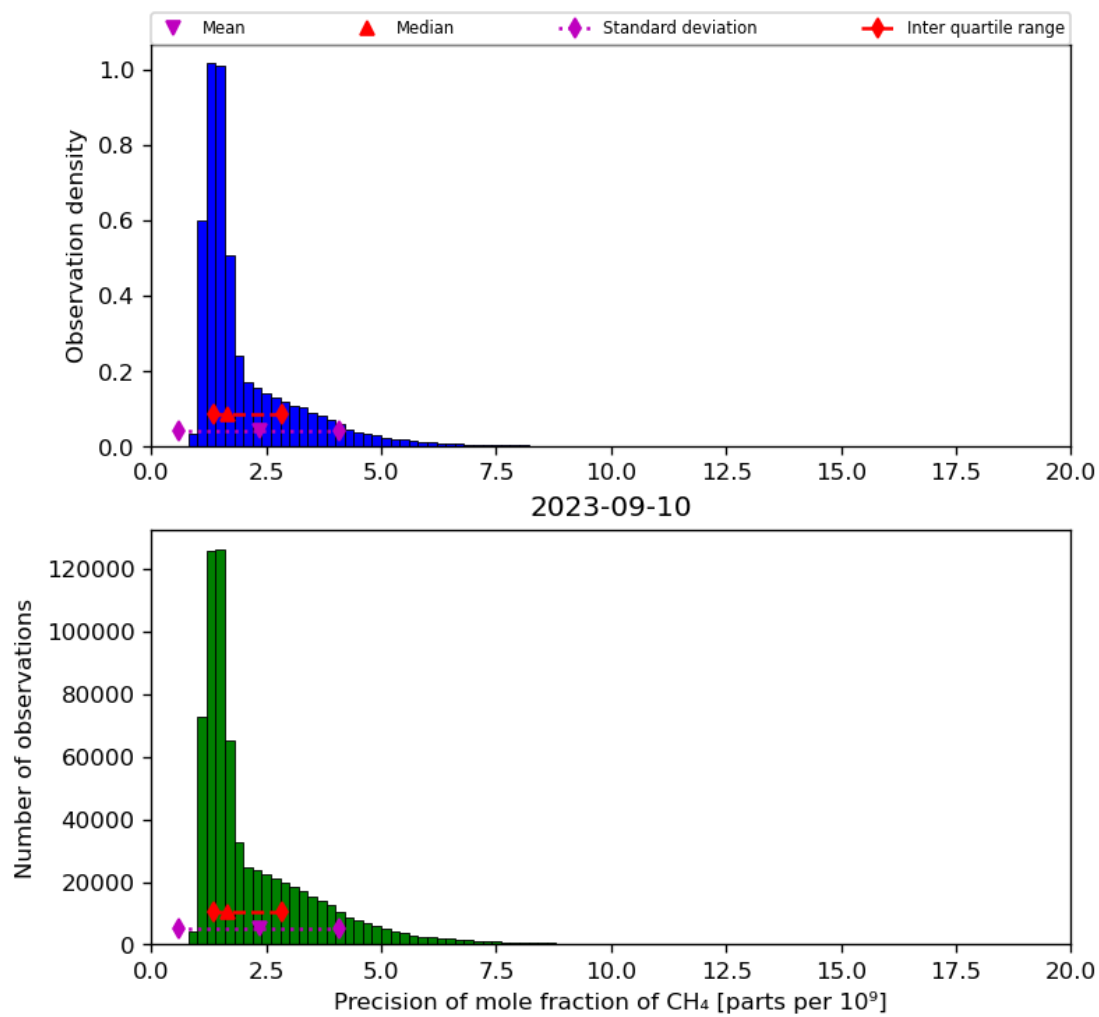
Figure 24: Histogram of “Precision of mole fraction of CH 4 ” for 2023-09-10 to 2023-09-11
