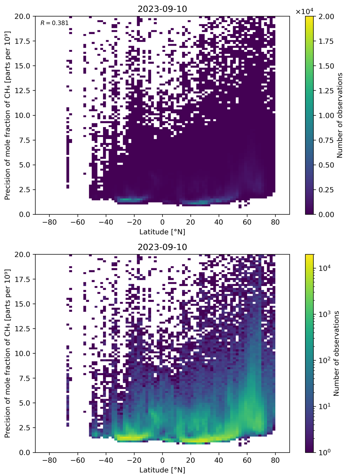
Figure 59: Scatter density plot of “Latitude” against “Precision of mole fraction of \text{CH}_4 ” for 2023-09-10 to 2023-09-11.
