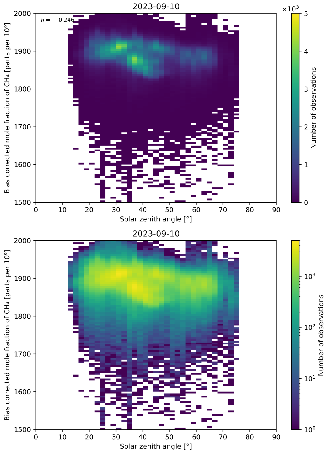
Figure 100: Scatter density plot of “Solar zenith angle” against “Bias corrected mole fraction of CH 4 ” for 2023-09-10 to 2023-09-11.
