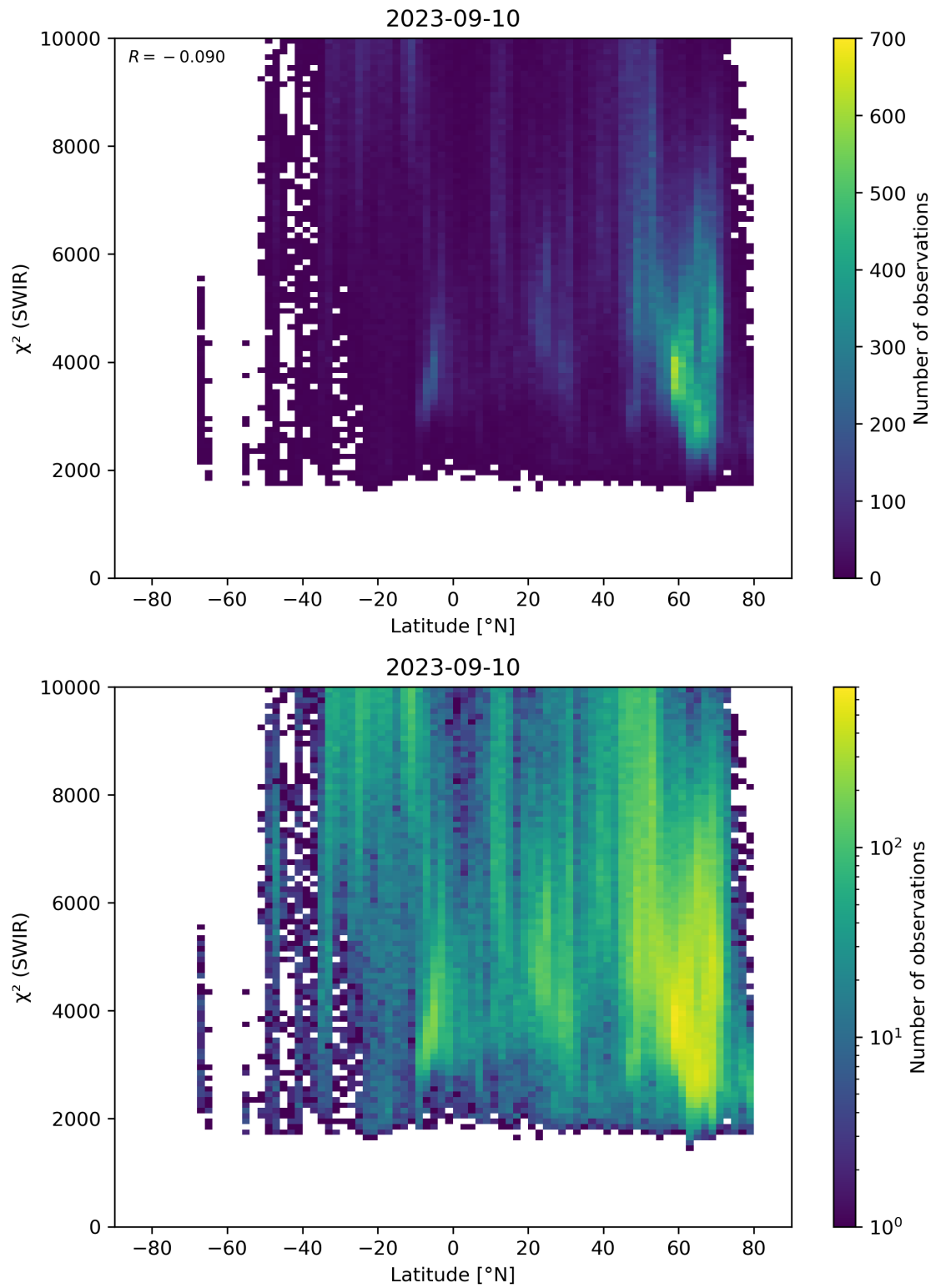
Figure 54: Scatter density plot of “Latitude” against “ \chi^2 (SWIR)” for 2023-09-10 to 2023-09-11.
