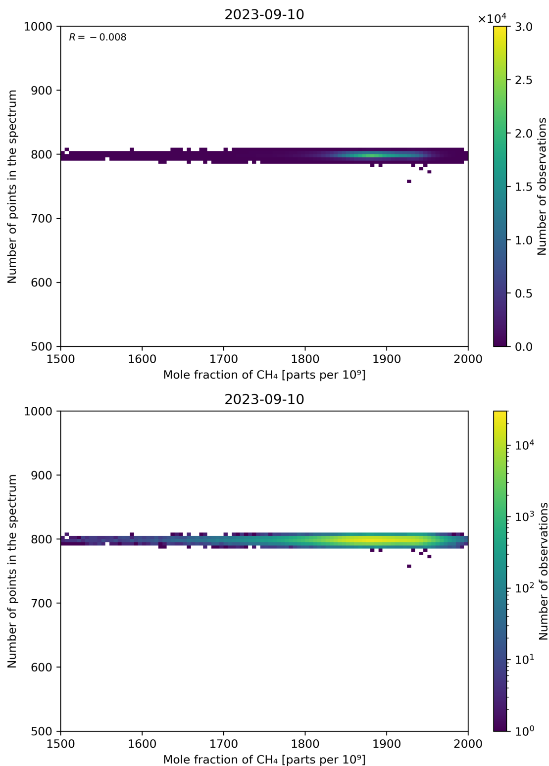
Figure 77: Scatter density plot of “Mole fraction of CH 4 ” against “Number of points in the spectrum” for 2023-09-10 to 2023-09-11.
