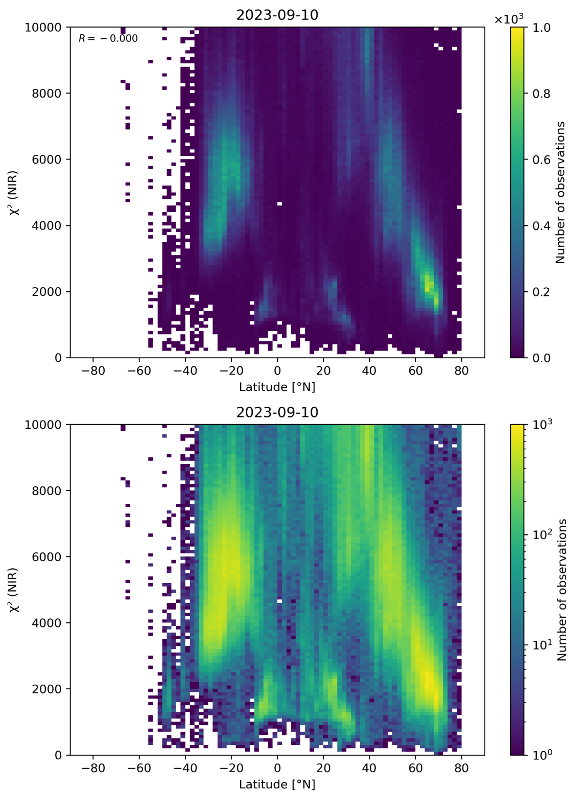
Figure 53: Scatter density plot of “Latitude” against “ \chi^2 (NIR)” for 2023-09-10 to 2023-09-11.
