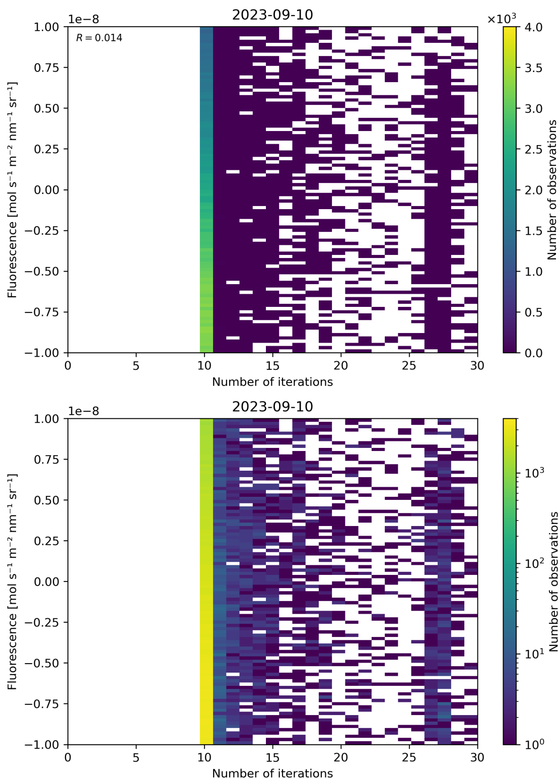
Figure 87: Scatter density plot of “Number of iterations” against “Fluorescence” for 2023-09-10 to 2023-09-11.
