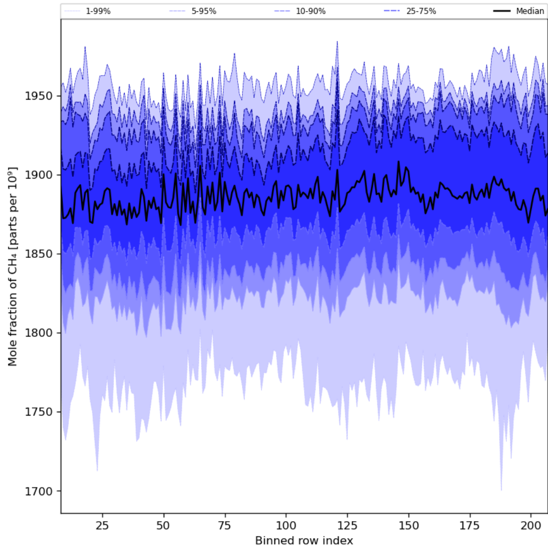
Figure 34: Along track statistics of “Mole fraction of CH 4 ” for 2023-09-10 to 2023-09-11
