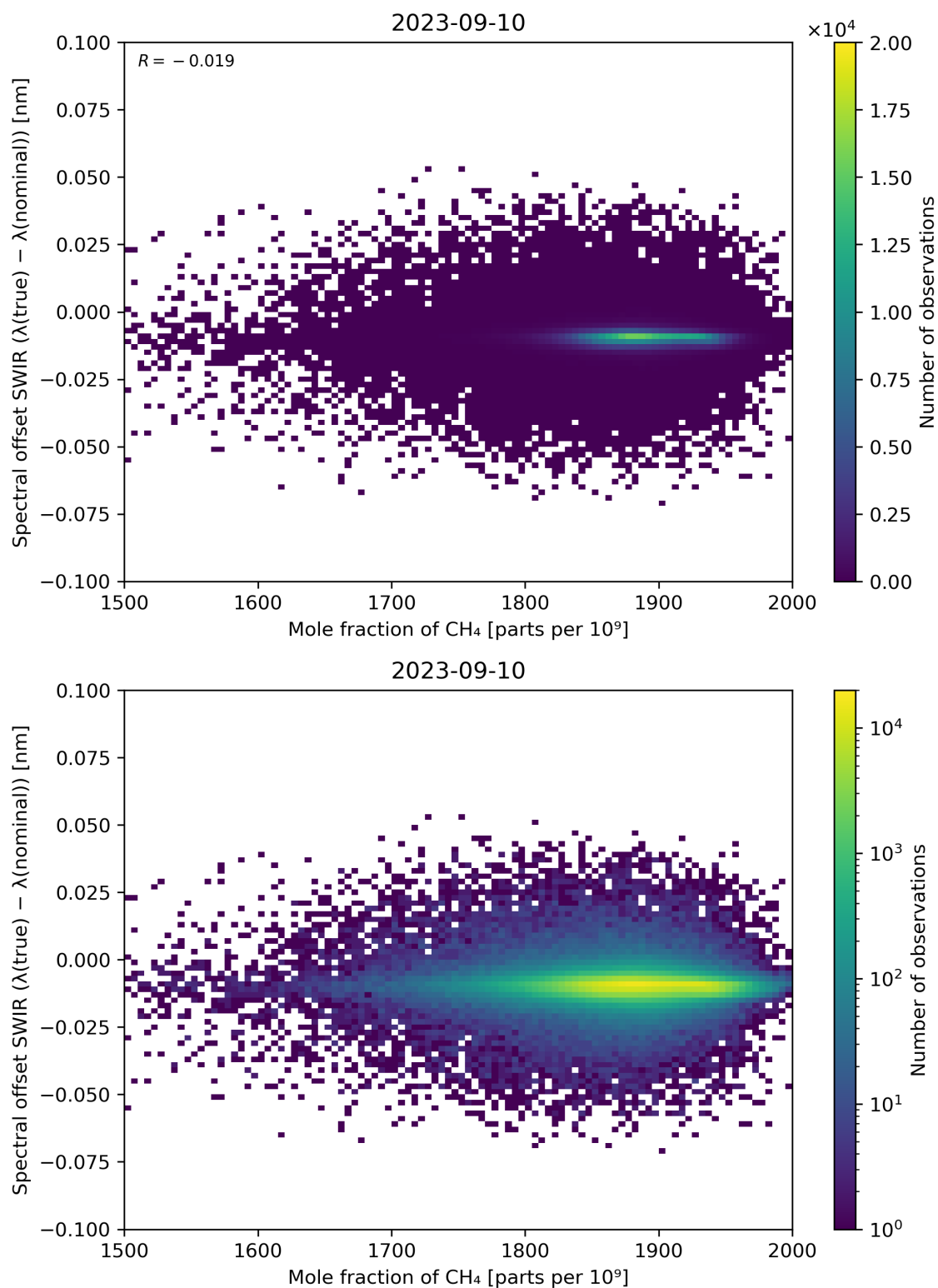
Figure 86: Scatter density plot of “Mole fraction of CH 4 ” against “Spectral offset SWIR ( \lambda(\text{true}) - \lambda(\text{nominal}) )” for 2023-09-10 to 2023-09-11.
