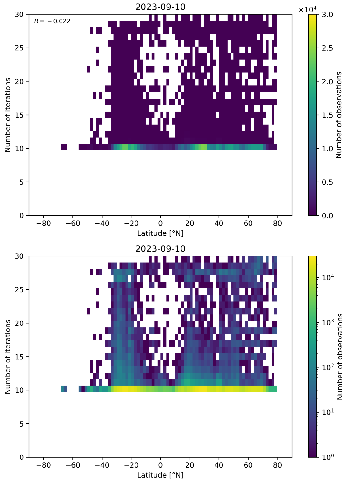
Figure 60: Scatter density plot of “Latitude” against “Number of iterations” for 2023-09-10 to 2023-09-11.
