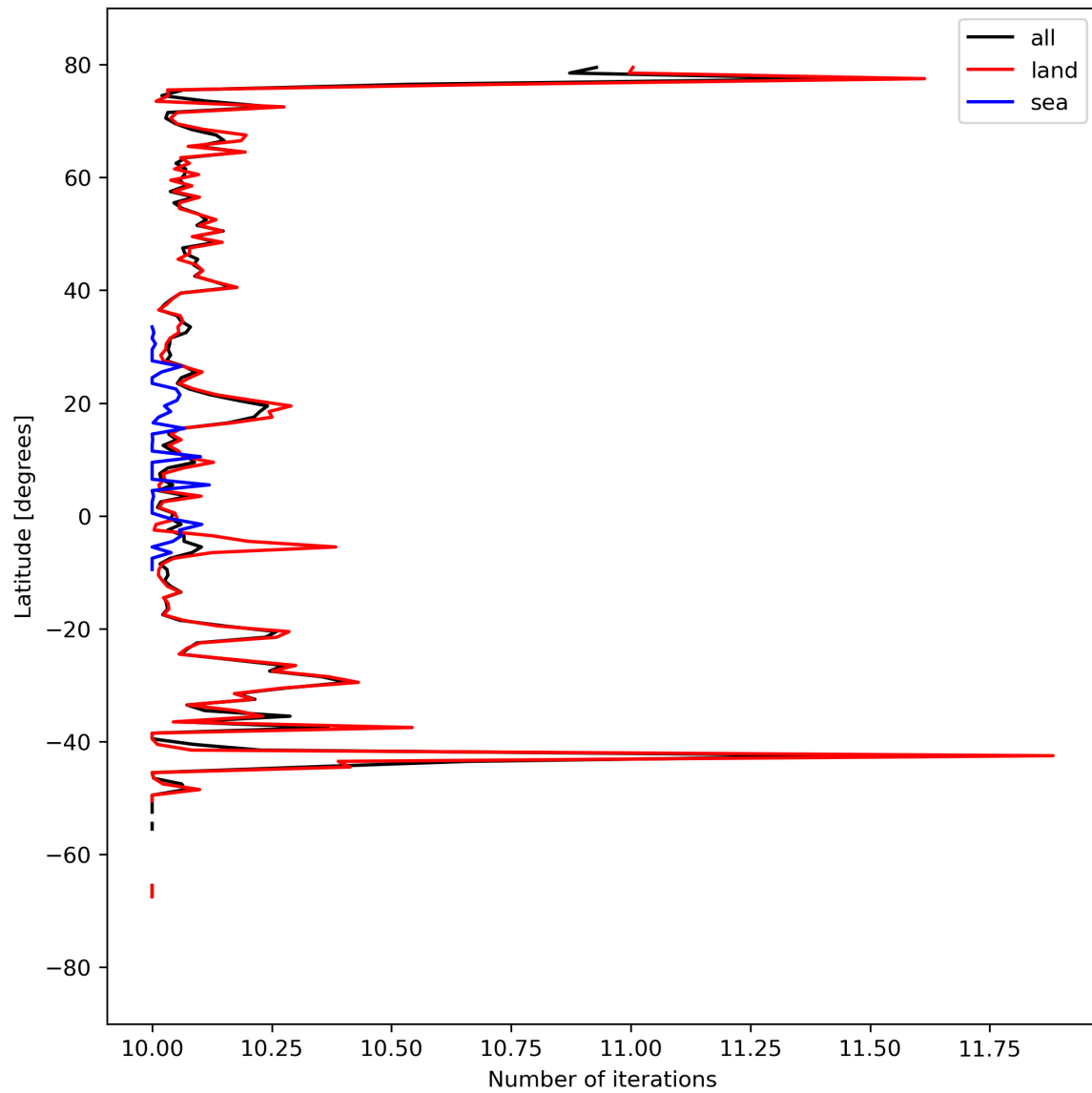
Figure 20: Zonal average of “Number of iterations” for 2023-09-10 to 2023-09-11.
