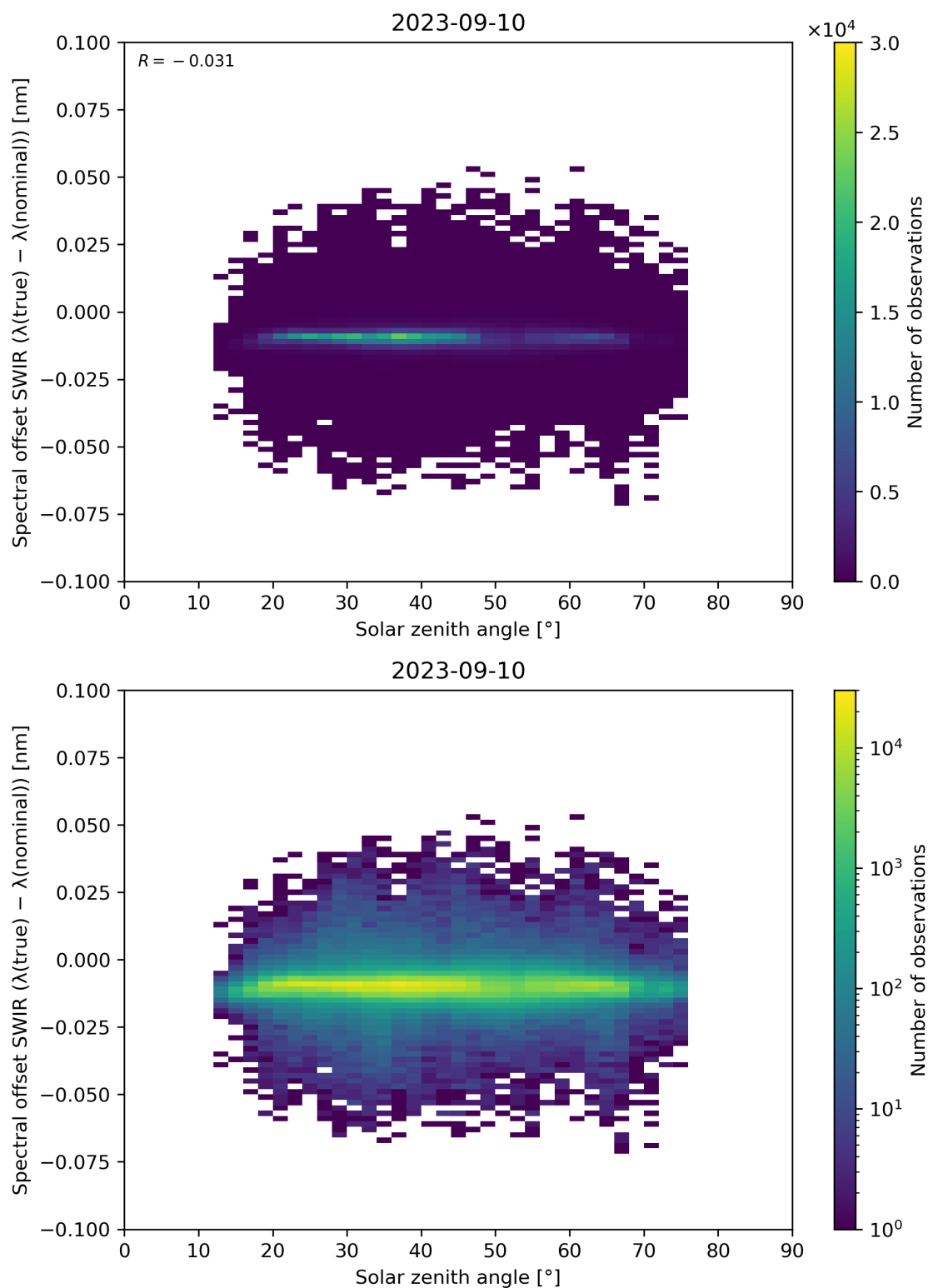
Figure 104: Scatter density plot of “Solar zenith angle” against “Spectral offset SWIR ( \lambda(\text{true}) - \lambda(\text{nominal}) )” for 2023-09-10 to 2023-09-11.
