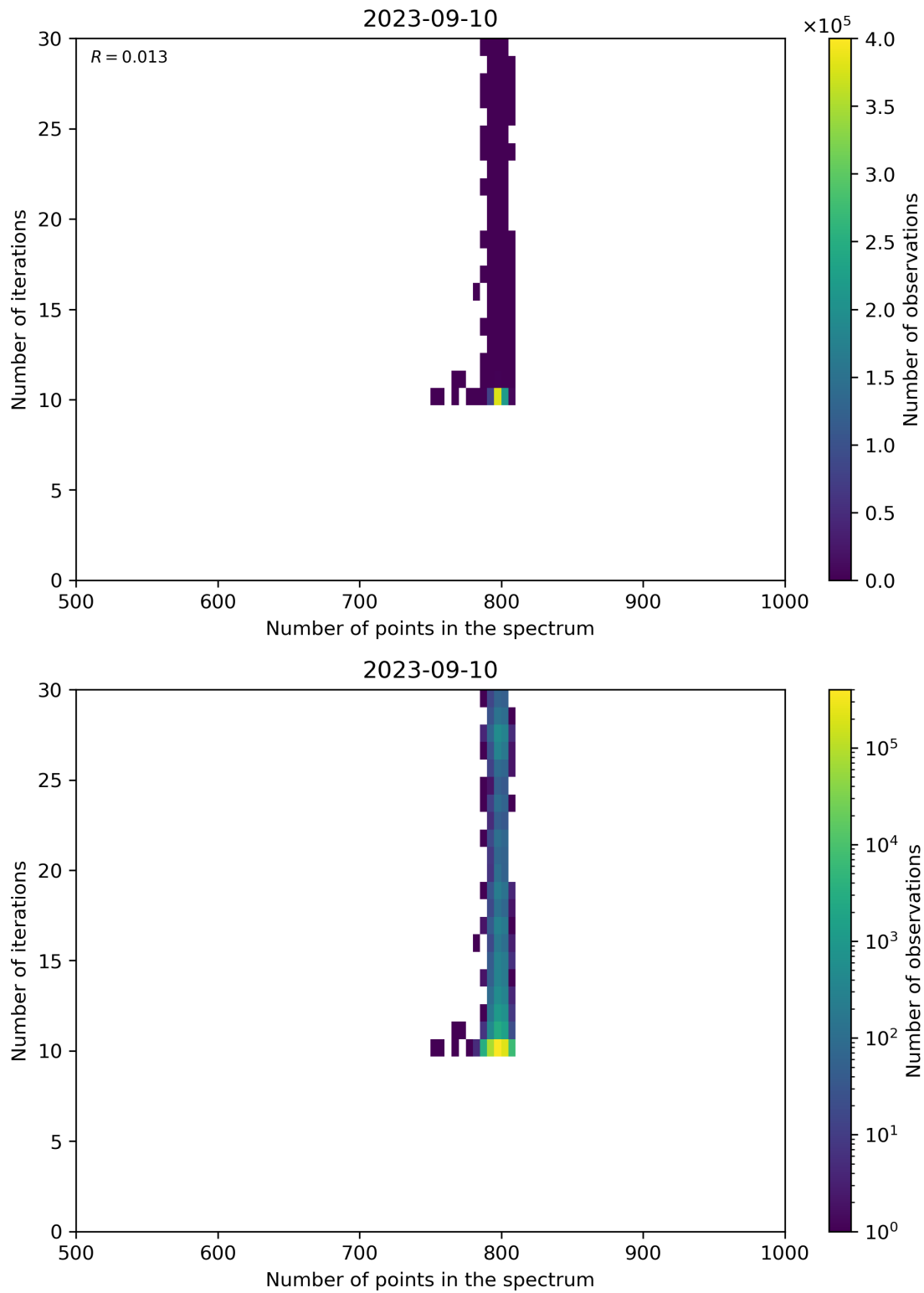
Figure 92: Scatter density plot of “Number of points in the spectrum” against “Number of iterations” for 2023-09-10 to 2023-09-11.
