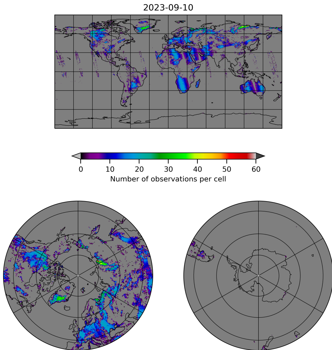
Figure 10: Map of the number of observations for 2023-09-10 to 2023-09-11
