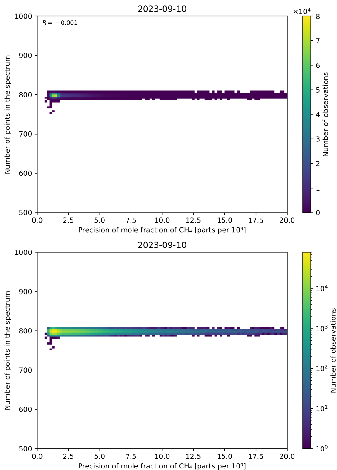
Figure 84: Scatter density plot of “Precision of mole fraction of CH 4 ” against “Number of points in the spectrum” for 2023-09-10 to 2023-09-11.
