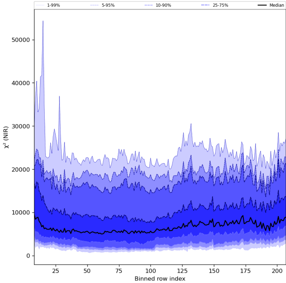
Figure 40: Along track statistics of “ \chi^2 (NIR)” for 2023-09-10 to 2023-09-11
