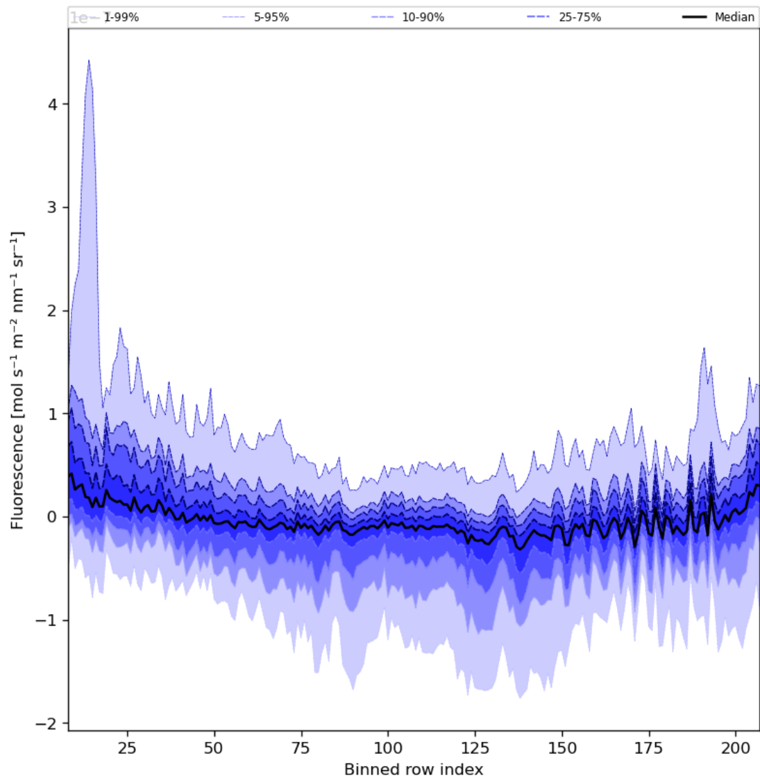
Figure 43: Along track statistics of “Fluorescence” for 2023-09-10 to 2023-09-11
