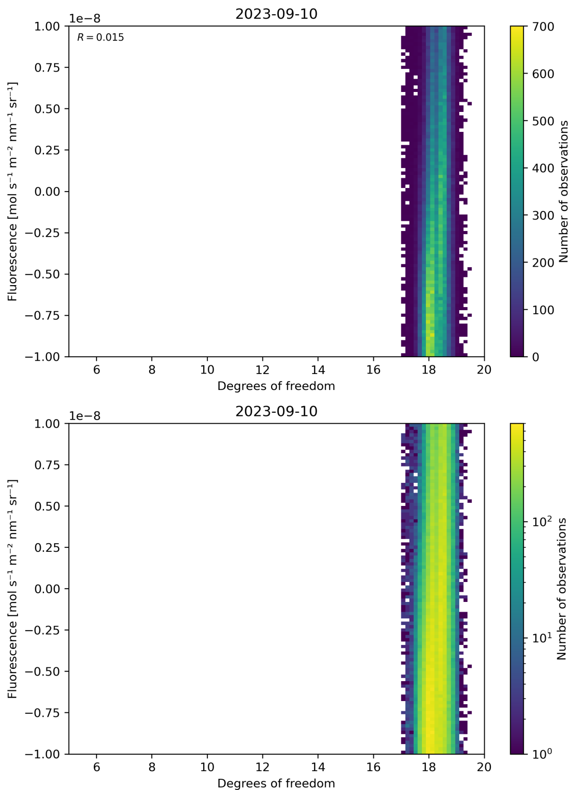
Figure 51: Scatter density plot of “Degrees of freedom” against “Fluorescence” for 2023-09-10 to 2023-09-11.
