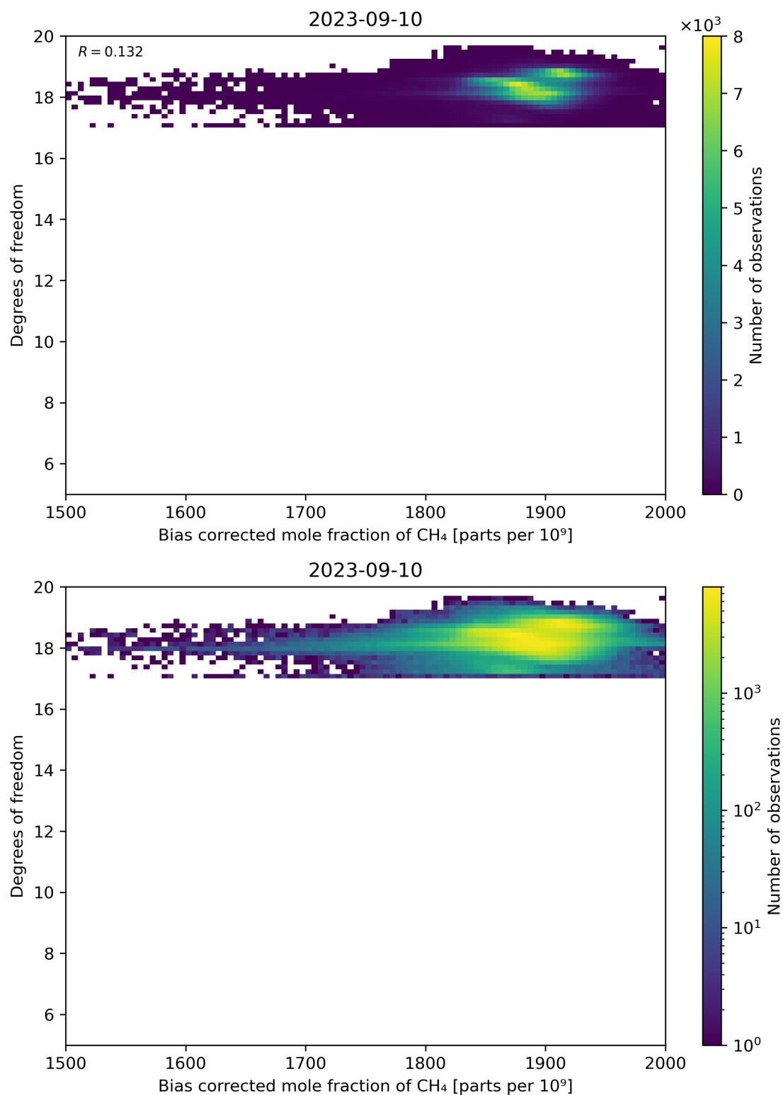
Figure 65: Scatter density plot of “Bias corrected mole fraction of CH 4 ” against “Degrees of freedom” for 2023-09-10 to 2023-09-11.
