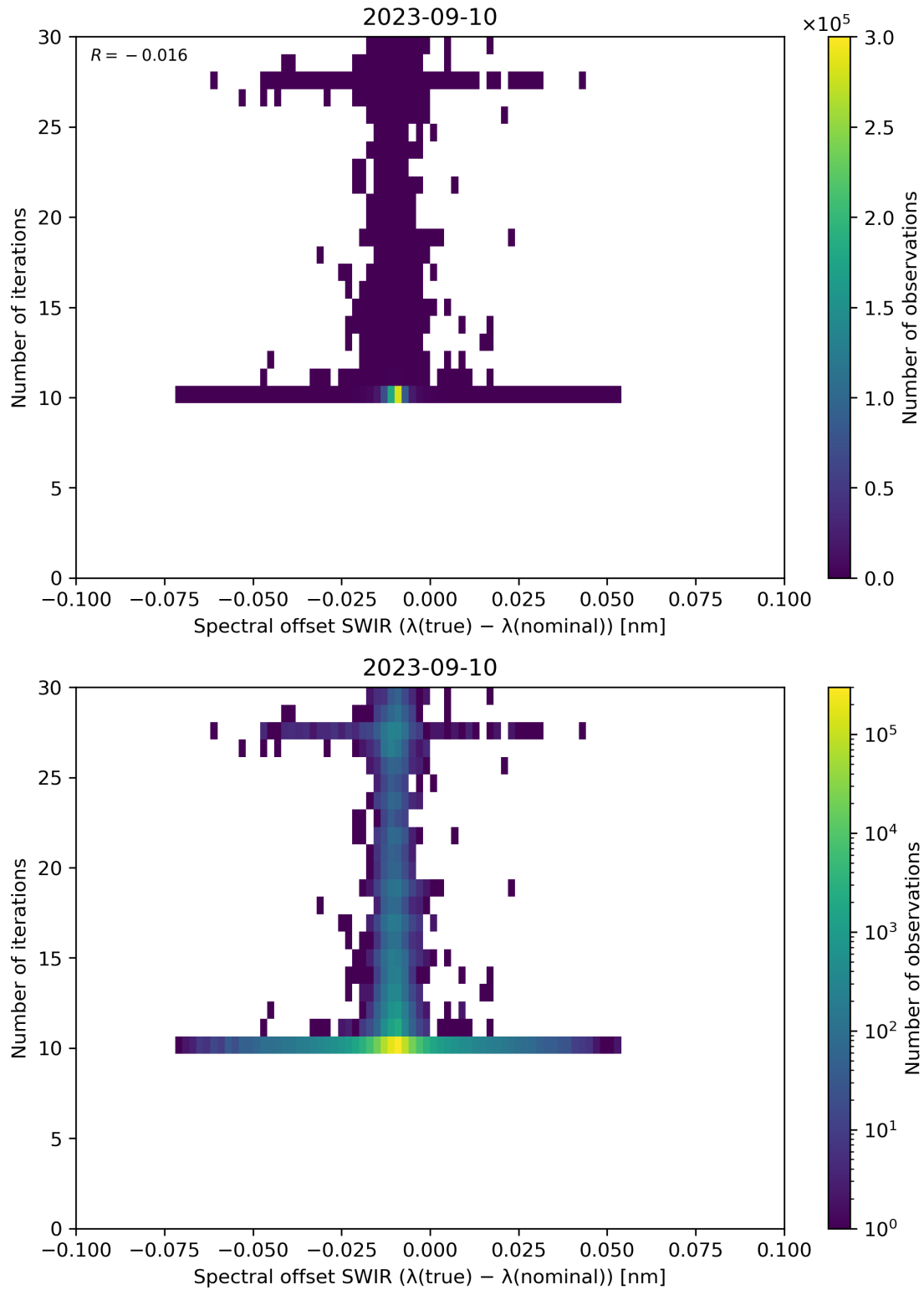
Figure 121: Scatter density plot of “Spectral offset SWIR ( \lambda(\text{true}) - \lambda(\text{nominal}) )” against “Number of iterations” for 2023-09-10 to 2023-09-11.
