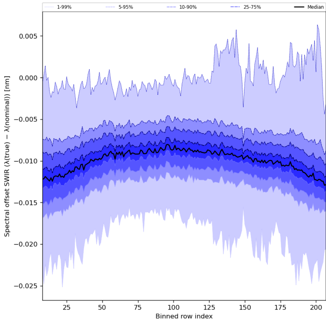
Figure 38: Along track statistics of “Spectral offset SWIR ( \lambda(\text{true}) - \lambda(\text{nominal}) )” for 2023-09-10 to 2023-09-11
