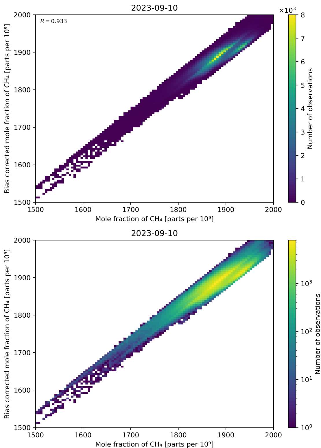
Figure 74: Scatter density plot of “Mole fraction of CH 4 ” against “Bias corrected mole fraction of CH 4 ” for 2023-09-10 to 2023-09-11.
