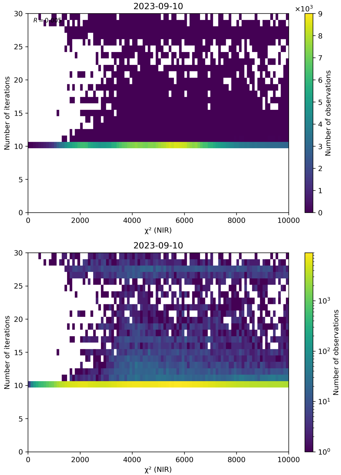
Figure 46: Scatter density plot of “ \chi^2 (NIR)” against “Number of iterations” for 2023-09-10 to 2023-09-11.
