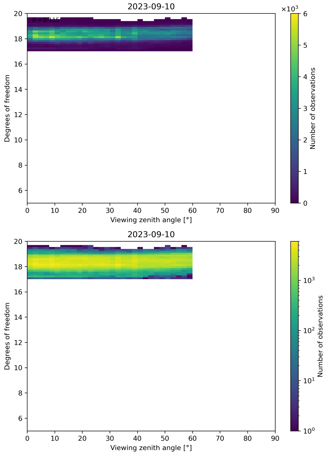
Figure 107: Scatter density plot of “Viewing zenith angle” against “Degrees of freedom” for 2023-09-10 to 2023-09-11.
