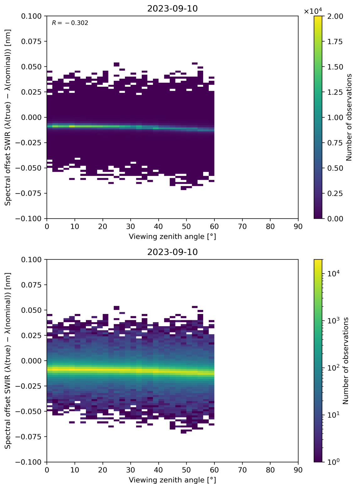
Figure 116: Scatter density plot of “Viewing zenith angle” against “Spectral offset SWIR ( \lambda(\text{true}) - \lambda(\text{nominal}) )” for 2023-09-10 to 2023-09-11.
