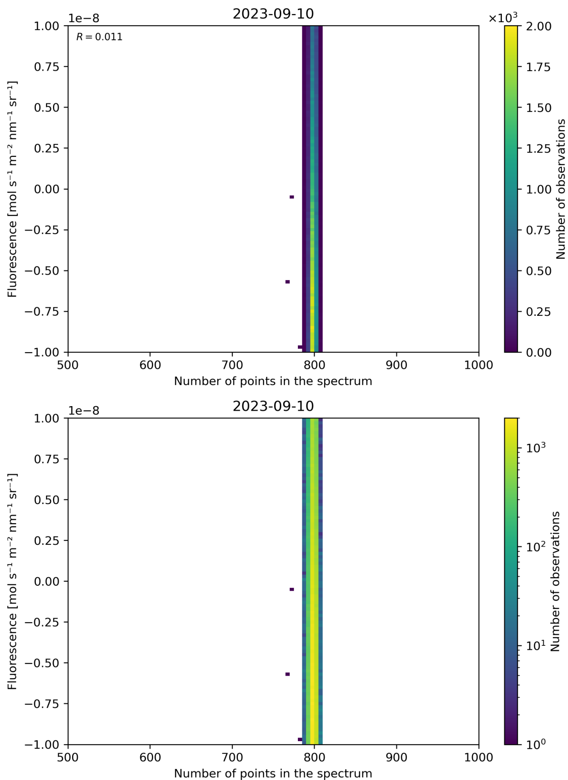
Figure 91: Scatter density plot of “Number of points in the spectrum” against “Fluorescence” for 2023-09-10 to 2023-09-11.
