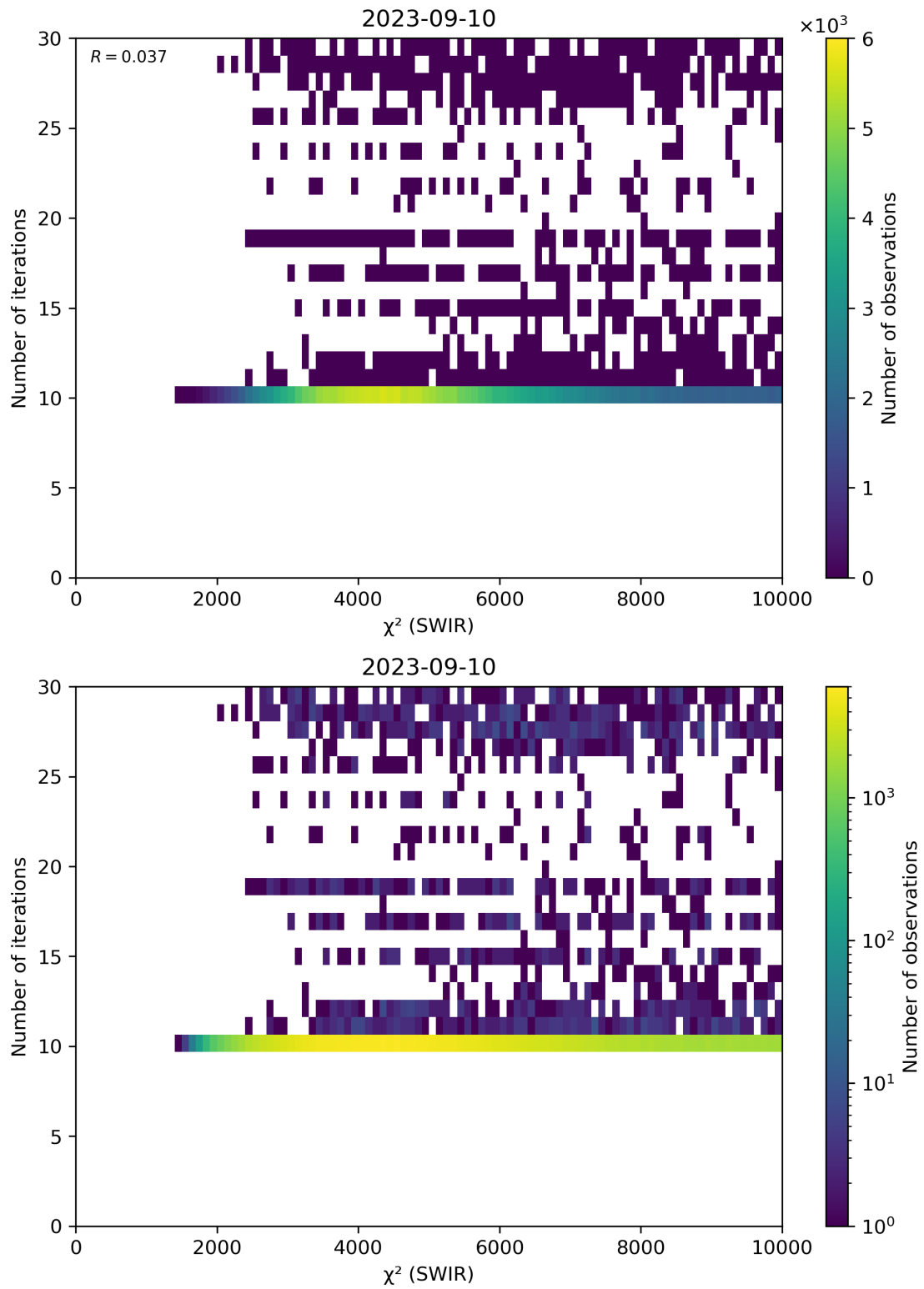
Figure 50: Scatter density plot of “ \chi^2 (SWIR)” against “Number of iterations” for 2023-09-10 to 2023-09-11.
