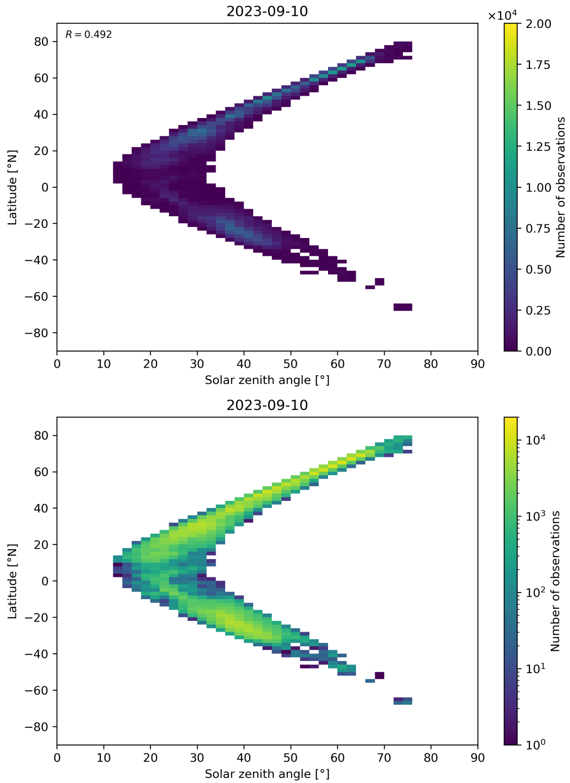
Figure 98: Scatter density plot of “Solar zenith angle” against “Latitude” for 2023-09-10 to 2023-09-11.
