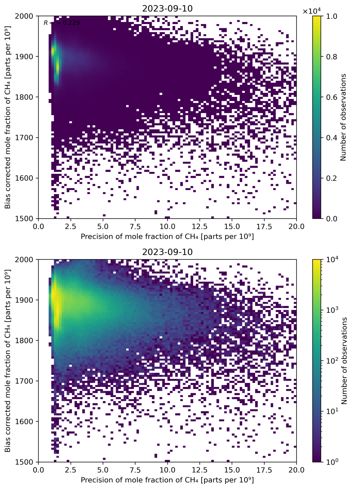
Figure 82: Scatter density plot of “Precision of mole fraction of CH 4 ” against “Bias corrected mole fraction of CH 4 ” for 2023-09-10 to 2023-09-11.
