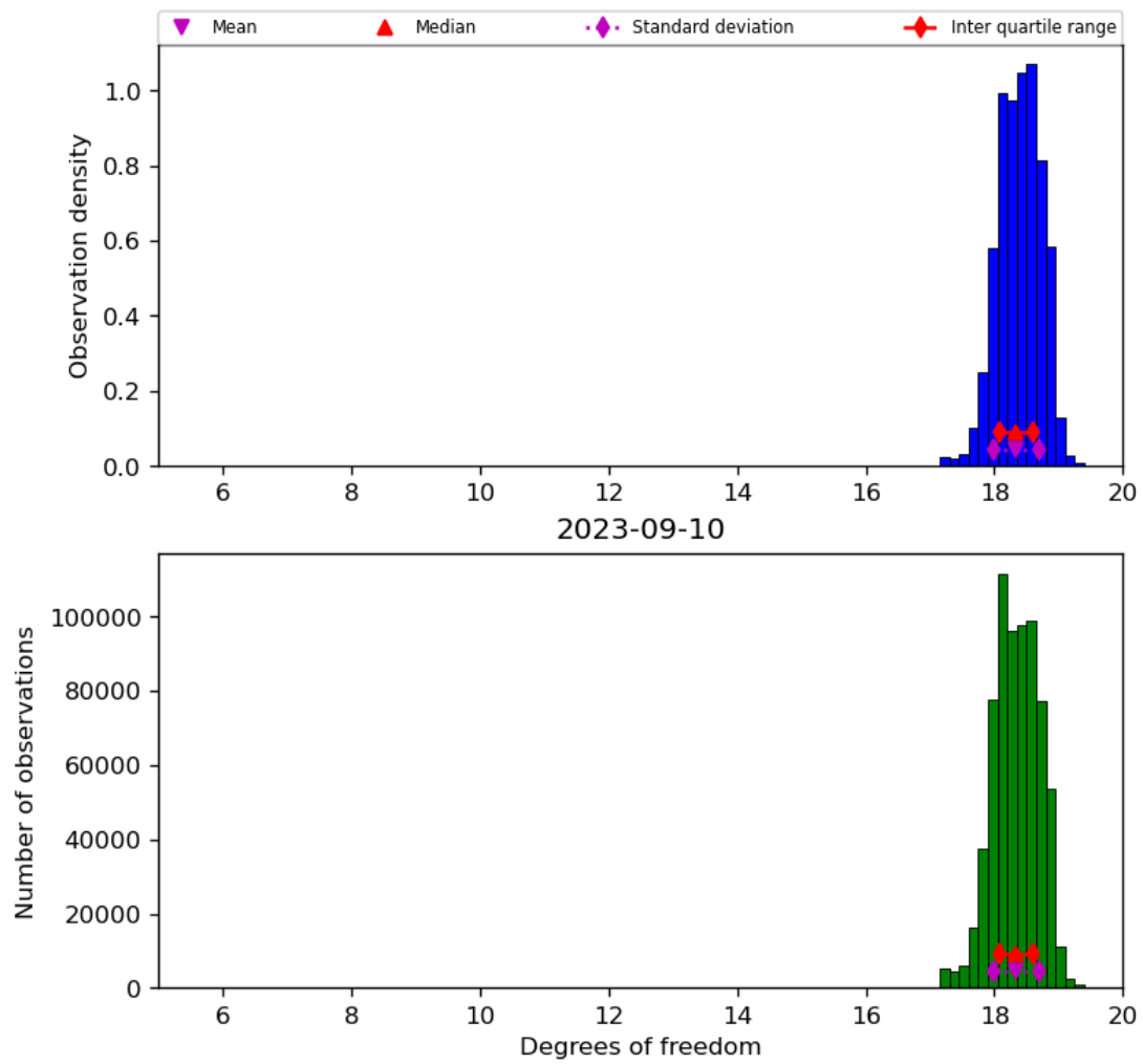
Figure 30: Histogram of “Degrees of freedom” for 2023-09-10 to 2023-09-11
