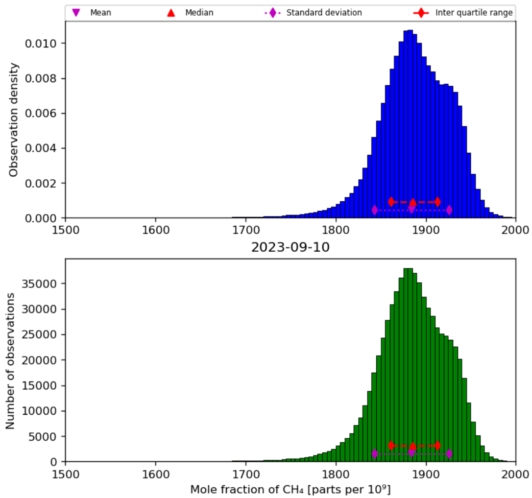
Figure 23: Histogram of “Mole fraction of CH 4 ” for 2023-09-10 to 2023-09-11
