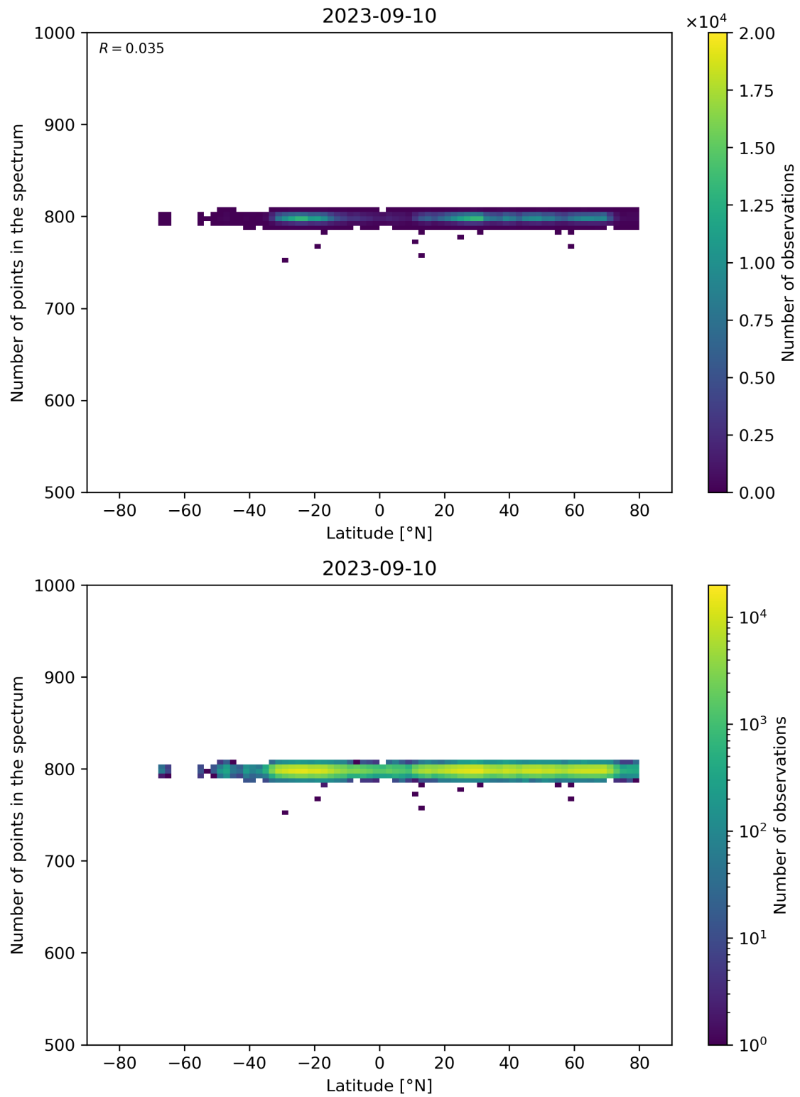
Figure 61: Scatter density plot of “Latitude” against “Number of points in the spectrum” for 2023-09-10 to 2023-09-11.
