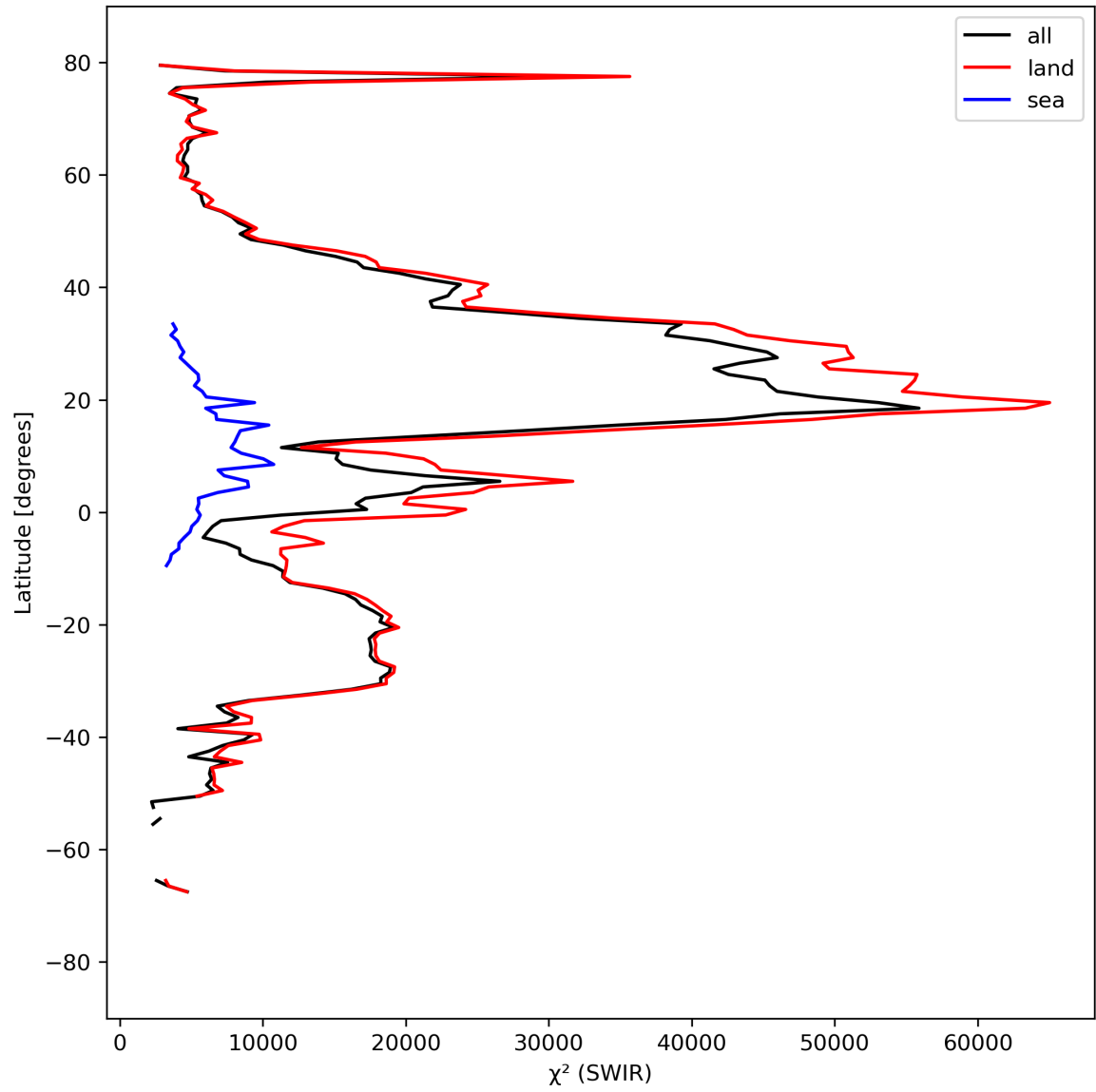
Figure 17: Zonal average of “ \chi^2 (SWIR)” for 2023-09-10 to 2023-09-11.
