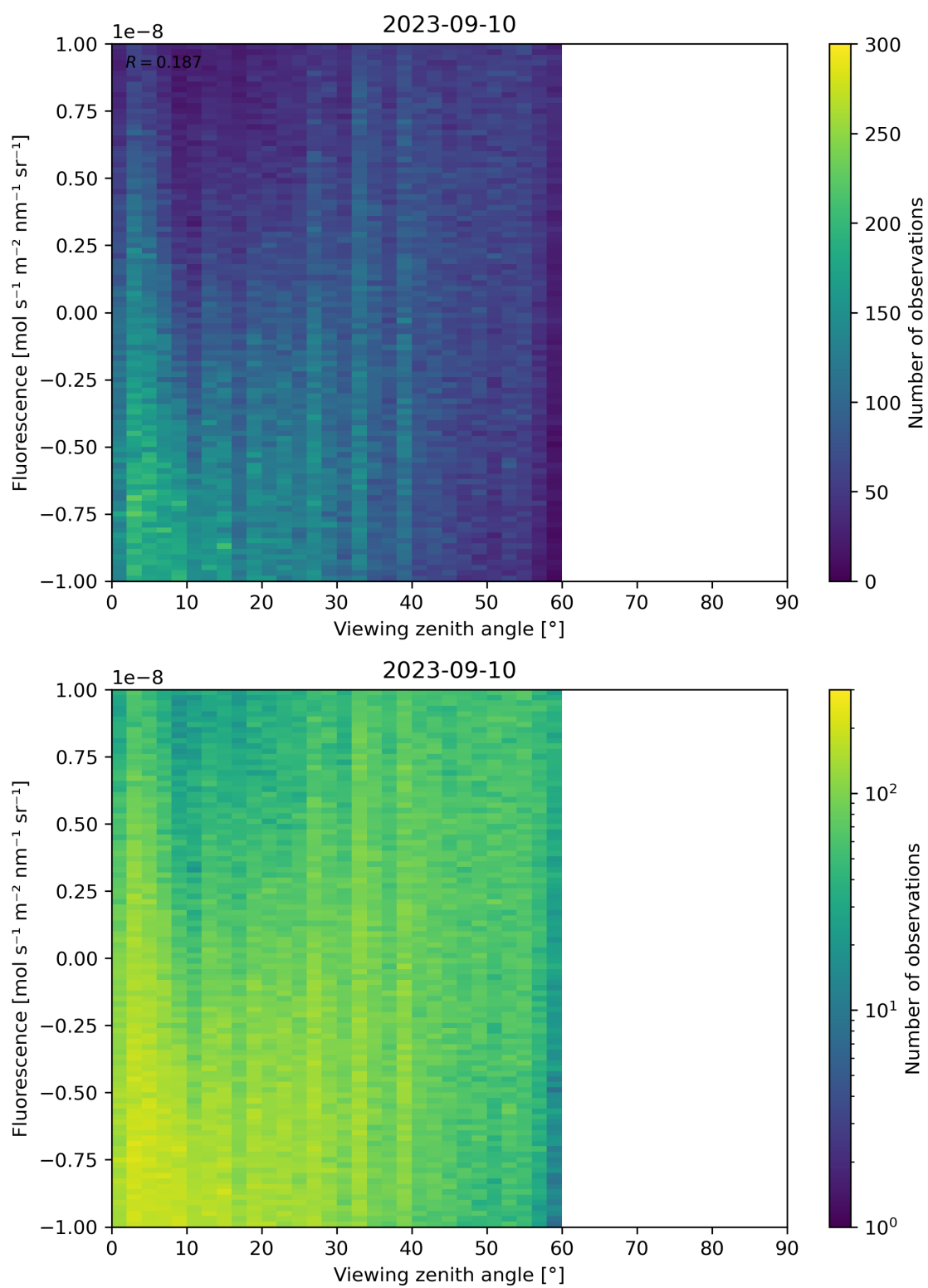
Figure 108: Scatter density plot of “Viewing zenith angle” against “Fluorescence” for 2023-09-10 to 2023-09-11.
