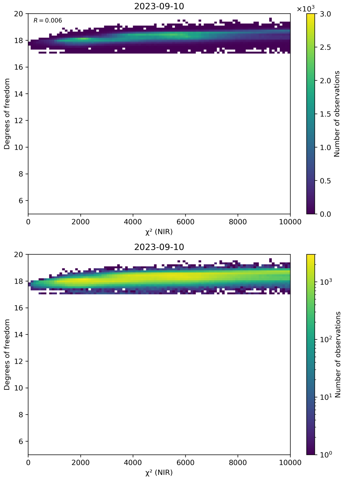
Figure 44: Scatter density plot of “ \chi^2 (NIR)” against “Degrees of freedom” for 2023-09-10 to 2023-09-11.
