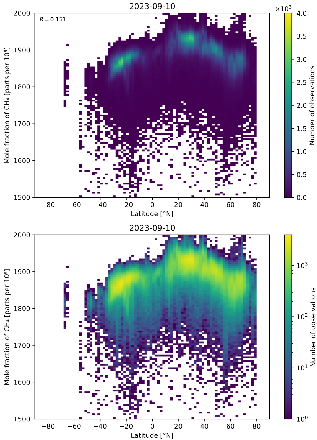
Figure 57: Scatter density plot of “Latitude” against “Mole fraction of \text{CH}_4 ” for 2023-09-10 to 2023-09-11.
