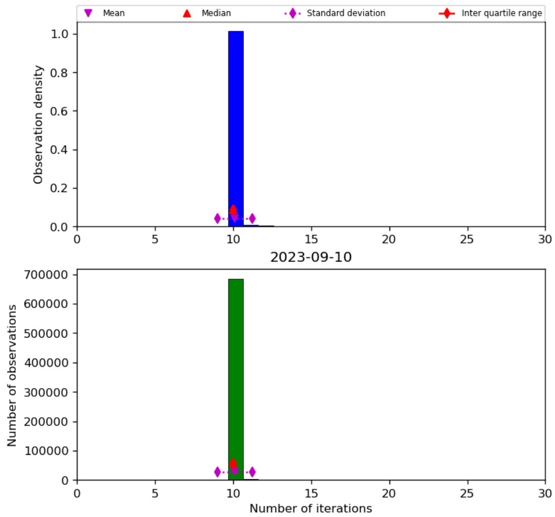
Figure 31: Histogram of “Number of iterations” for 2023-09-10 to 2023-09-11
