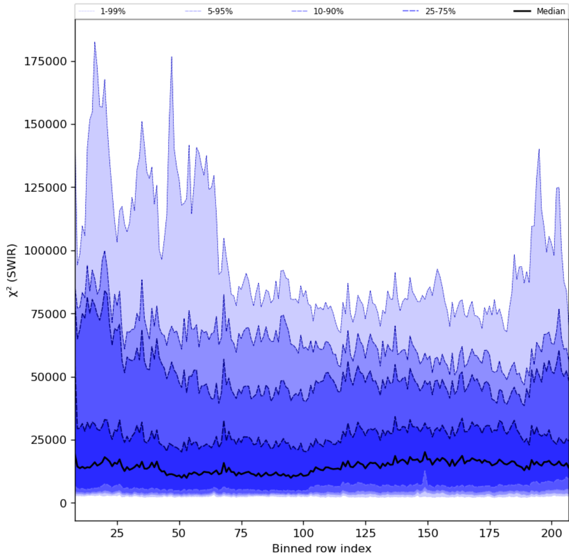
Figure 39: Along track statistics of “ \chi^2 (SWIR)” for 2023-09-10 to 2023-09-11
