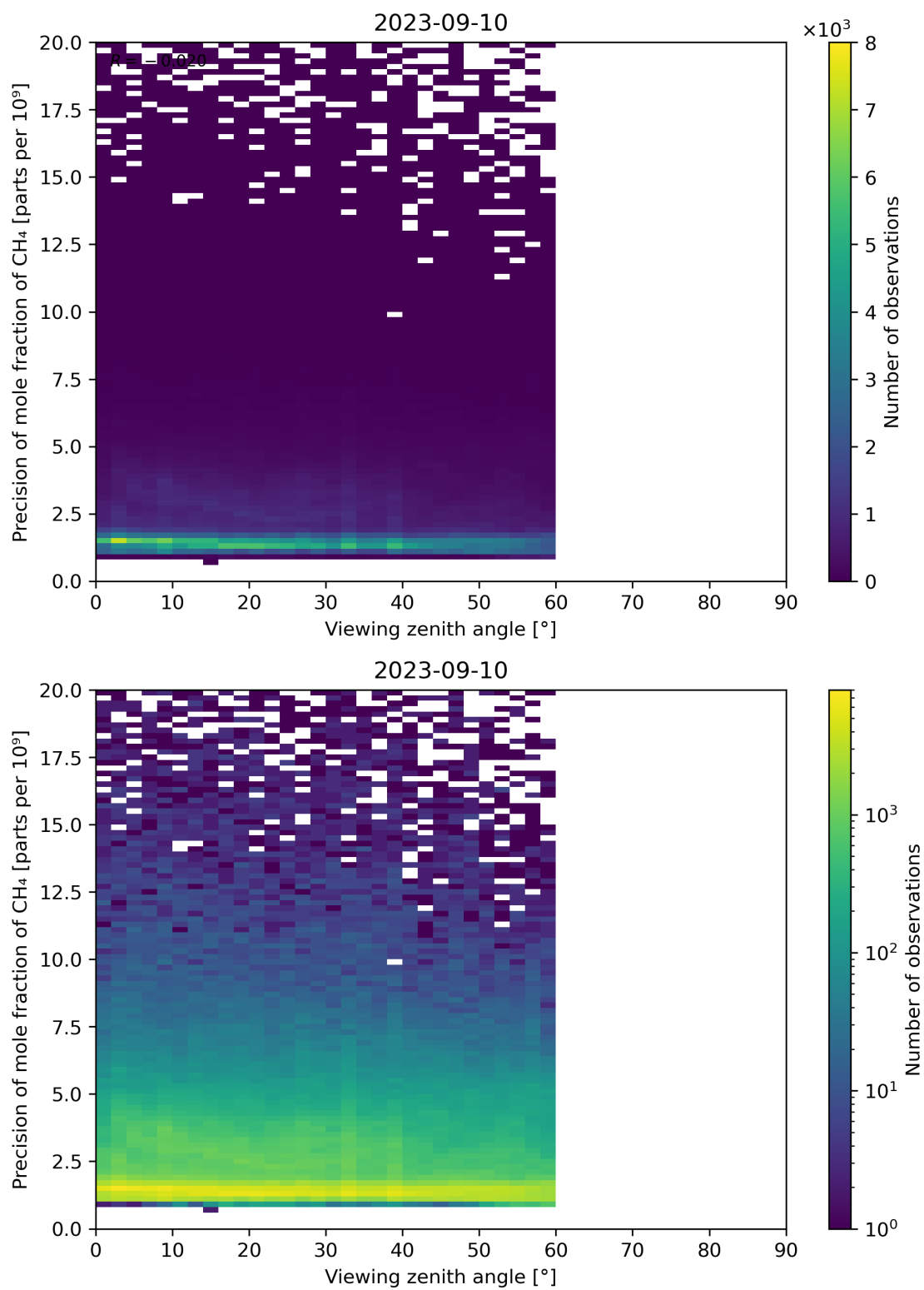
Figure 112: Scatter density plot of “Viewing zenith angle” against “Precision of mole fraction of CH 4 ” for 2023-09-10 to 2023-09-11.
