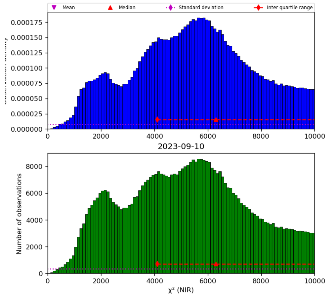
Figure 29: Histogram of “ \chi^2 (NIR)” for 2023-09-10 to 2023-09-11
