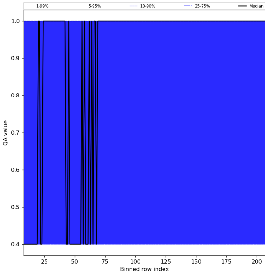
Figure 33: Along track statistics of “QA value” for 2023-09-10 to 2023-09-11
