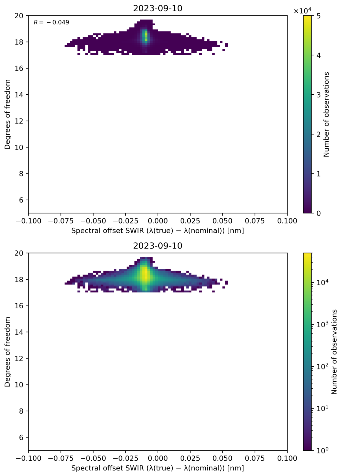
Figure 119: Scatter density plot of “Spectral offset SWIR ( \lambda(\text{true}) - \lambda(\text{nominal}) )” against “Degrees of freedom” for 2023-09-10 to 2023-09-11.
