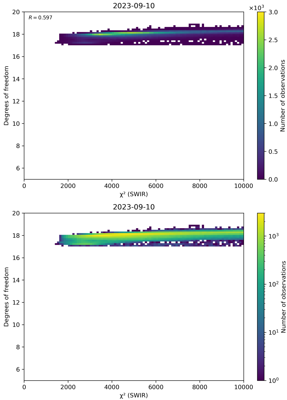
Figure 48: Scatter density plot of “ \chi^2 (SWIR)” against “Degrees of freedom” for 2023-09-10 to 2023-09-11.
