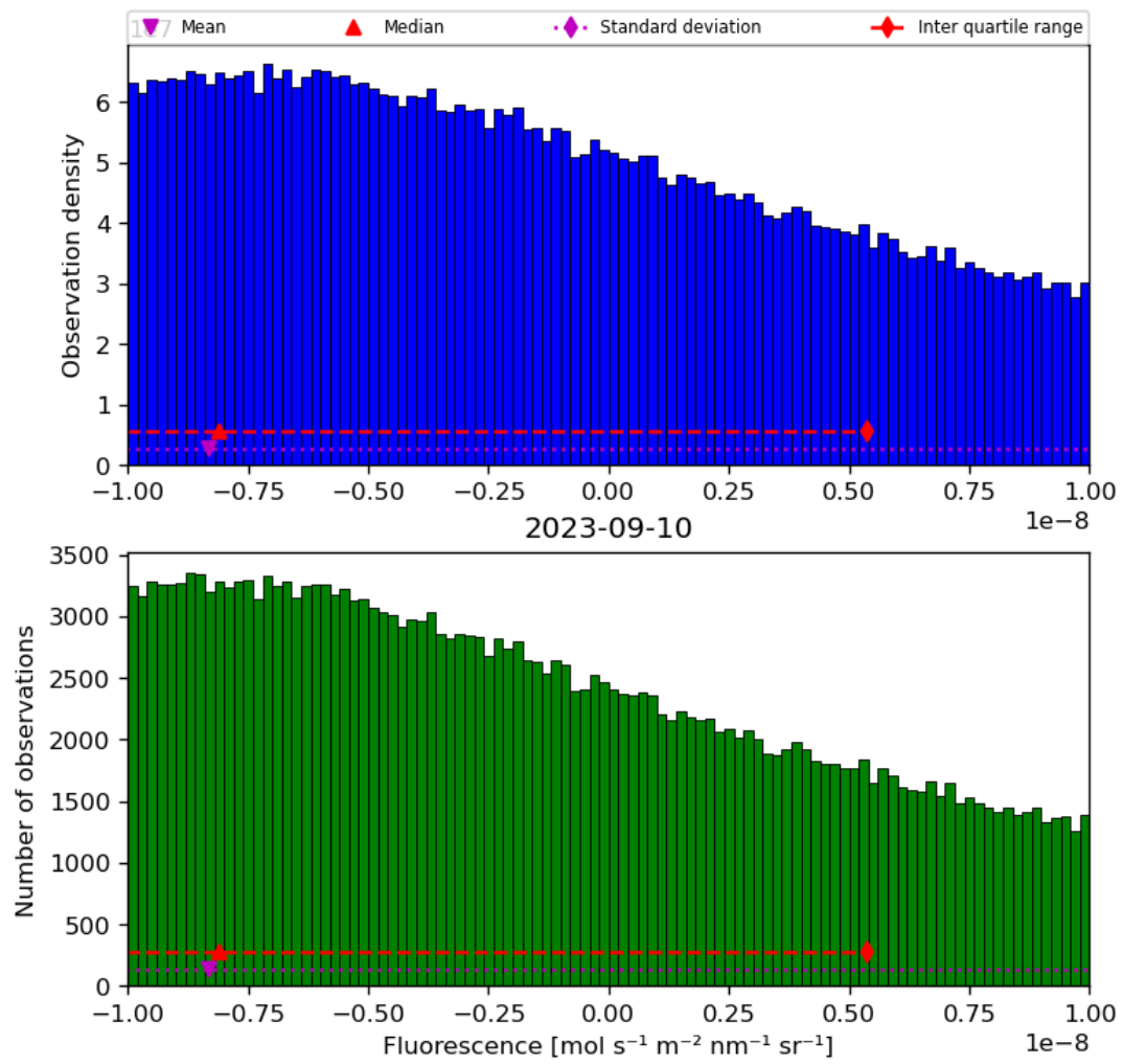
Figure 32: Histogram of “Fluorescence” for 2023-09-10 to 2023-09-11
