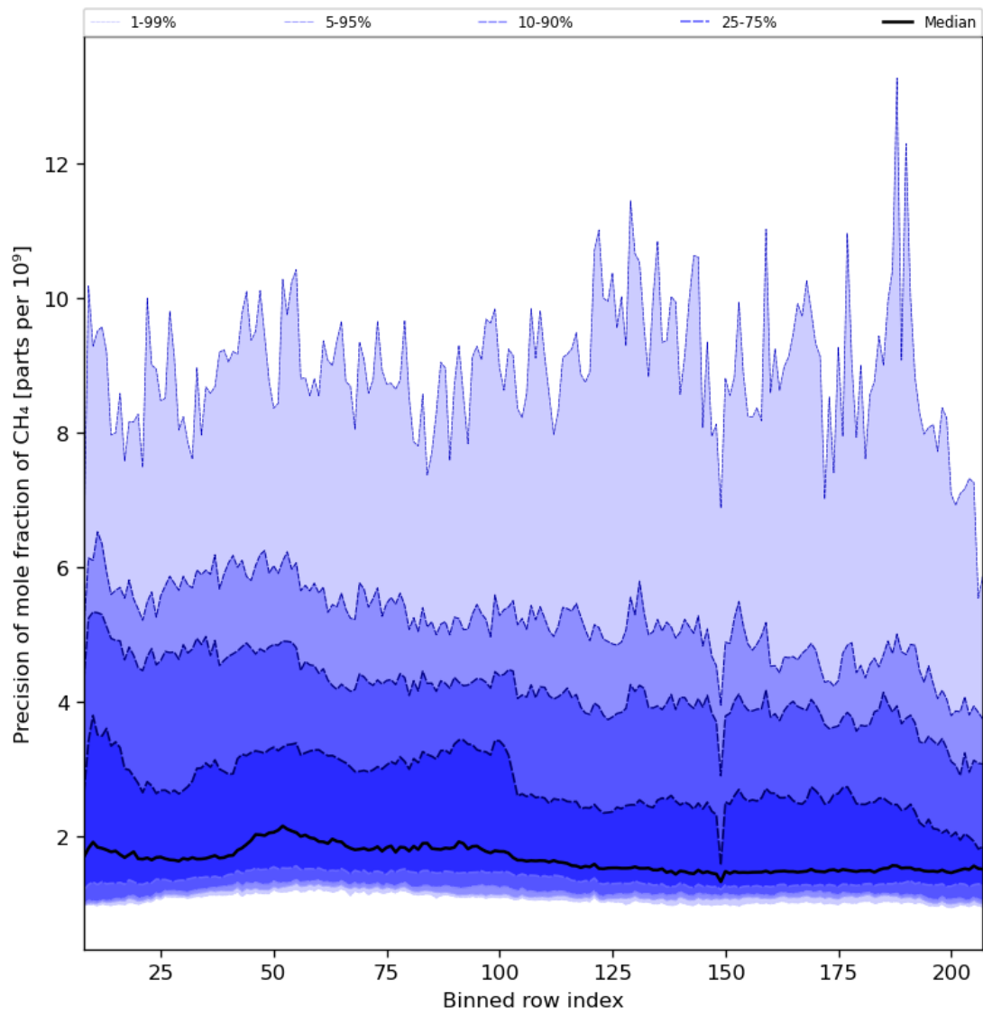
Figure 35: Along track statistics of “Precision of mole fraction of CH 4 ” for 2023-09-10 to 2023-09-11
