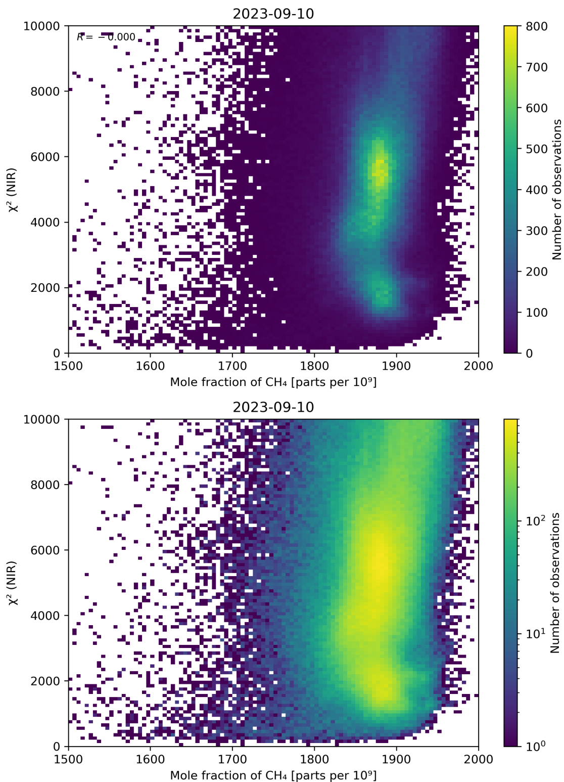
Figure 70: Scatter density plot of “Mole fraction of CH 4 ” against “ \chi^2 (NIR)” for 2023-09-10 to 2023-09-11.
