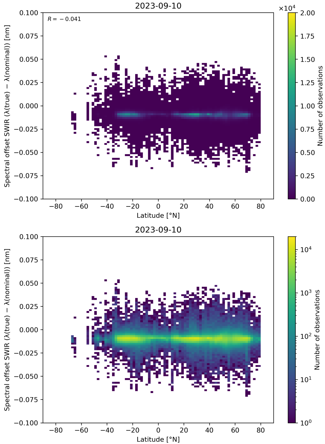
Figure 62: Scatter density plot of “Latitude” against “Spectral offset SWIR ( \lambda(\text{true}) - \lambda(\text{nominal}) )” for 2023-09-10 to 2023-09-11.
