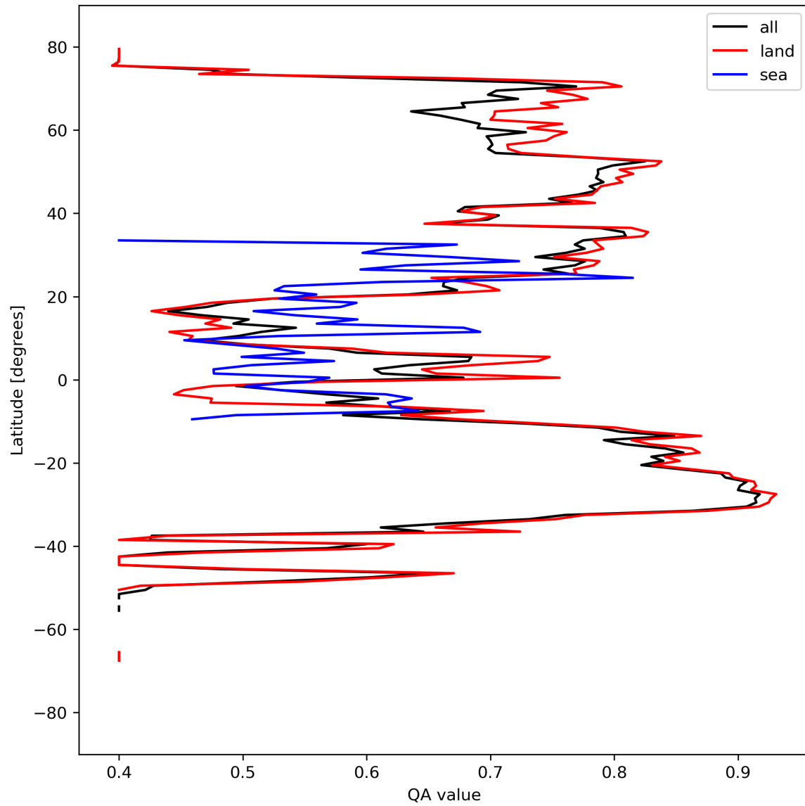
Figure 11: Zonal average of “QA value” for 2023-09-10 to 2023-09-11.
