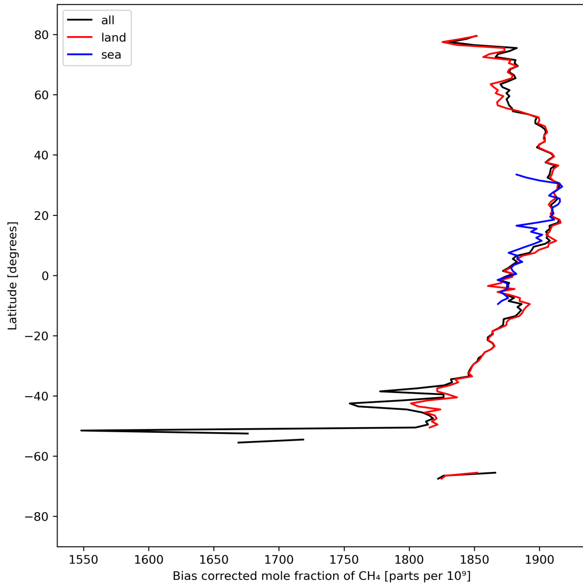
Figure 14: Zonal average of “Bias corrected mole fraction of CH 4 ” for 2023-09-10 to 2023-09-11.
