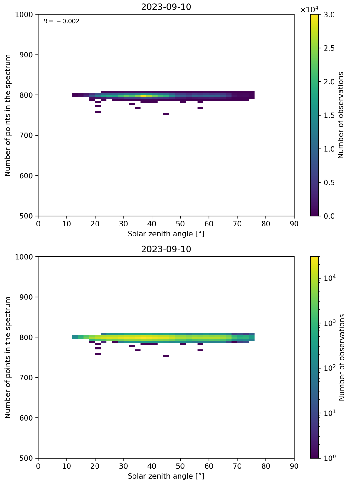
Figure 103: Scatter density plot of “Solar zenith angle” against “Number of points in the spectrum” for 2023-09-10 to 2023-09-11.
