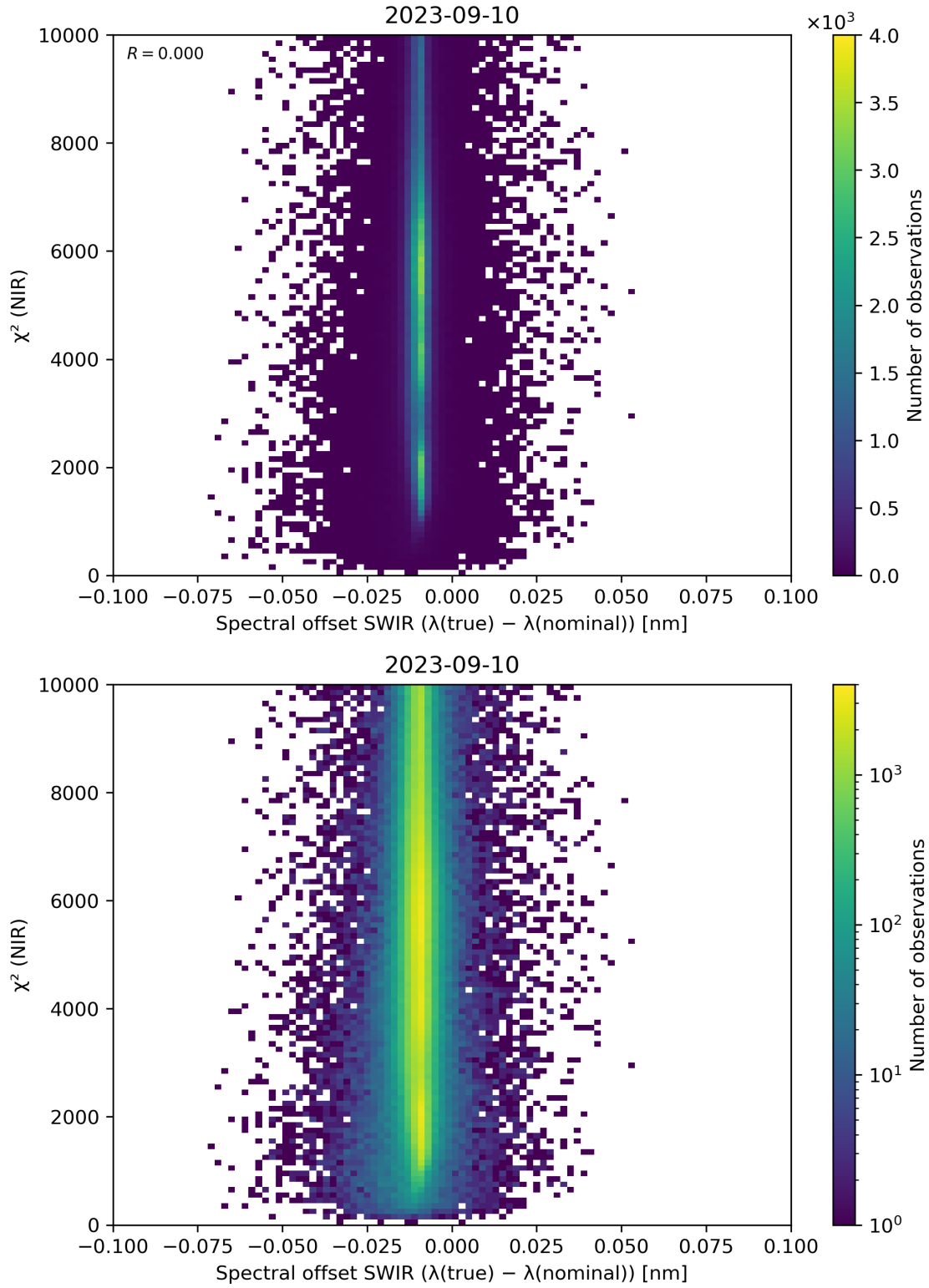
Figure 117: Scatter density plot of “Spectral offset SWIR ( \lambda(\text{true}) - \lambda(\text{nominal}) )” against “ \chi^2 (NIR)” for 2023-09-10 to 2023-09-11.
