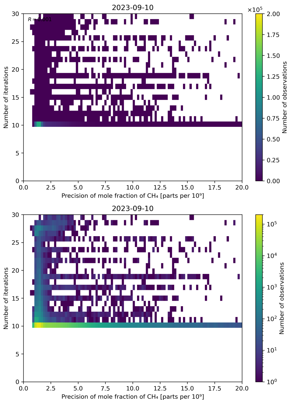
Figure 83: Scatter density plot of “Precision of mole fraction of CH 4 ” against “Number of iterations” for 2023-09-10 to 2023-09-11.
