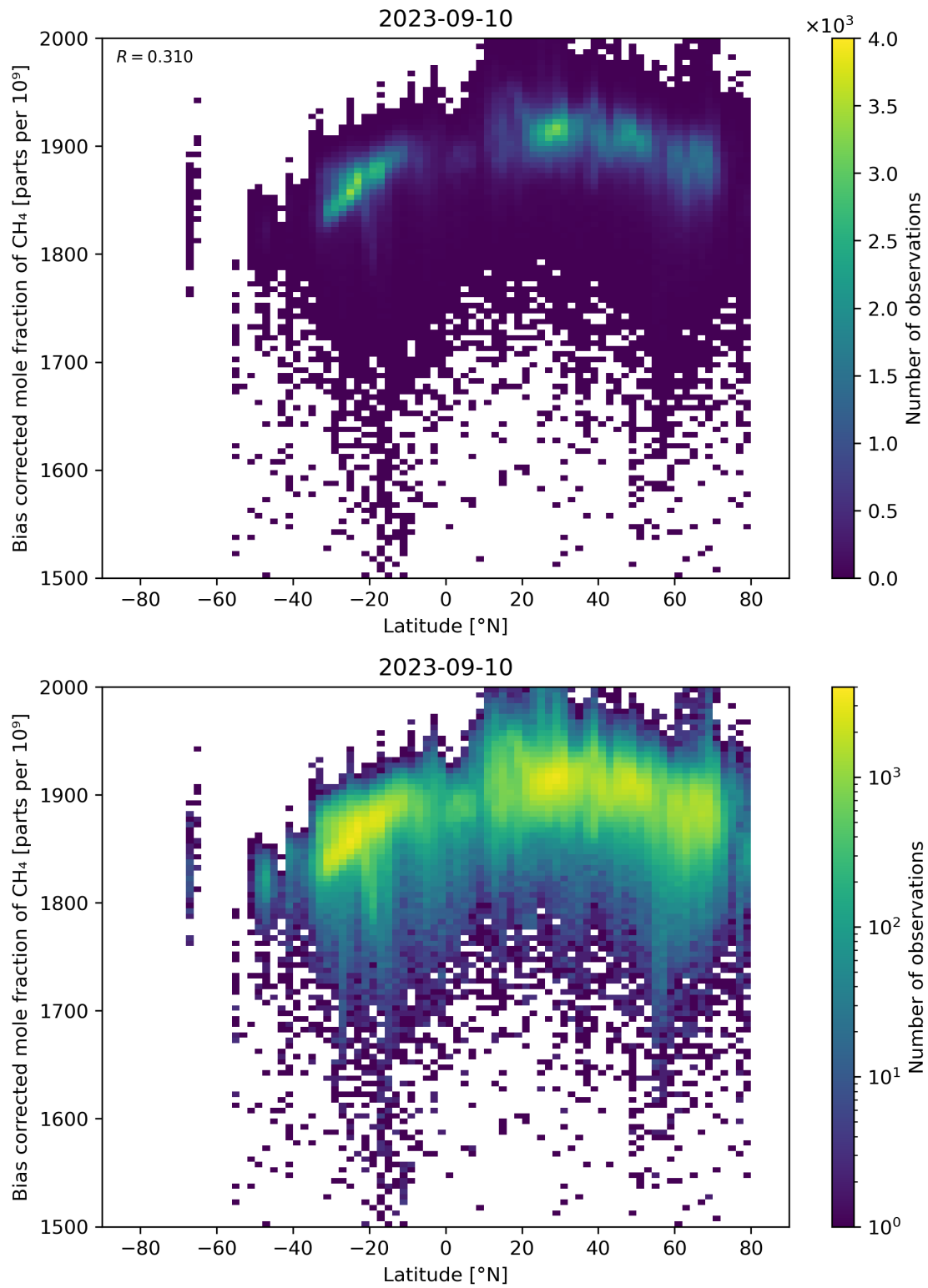
Figure 58: Scatter density plot of “Latitude” against “Bias corrected mole fraction of CH 4 ” for 2023-09-10 to 2023-09-11.
