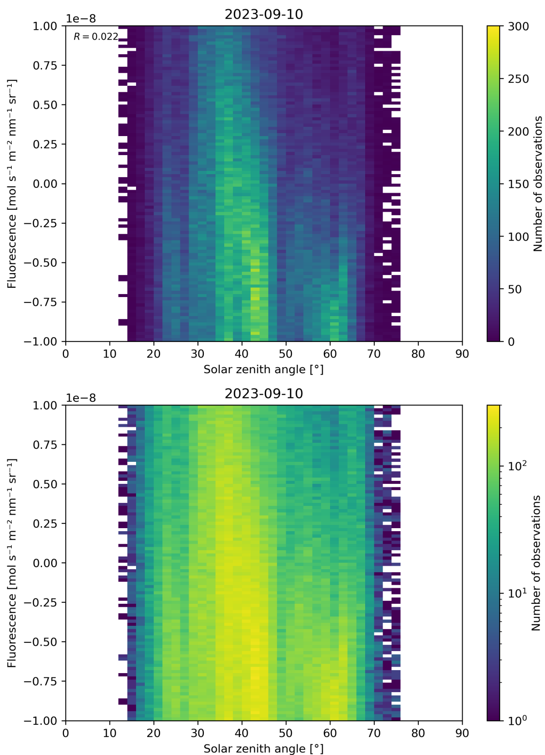
Figure 97: Scatter density plot of “Solar zenith angle” against “Fluorescence” for 2023-09-10 to 2023-09-11.
