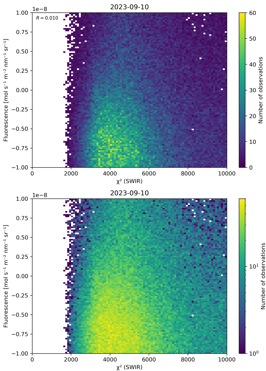
Figure 49: Scatter density plot of “ \chi^2 (SWIR)” against “Fluorescence” for 2023-09-10 to 2023-09-11.
