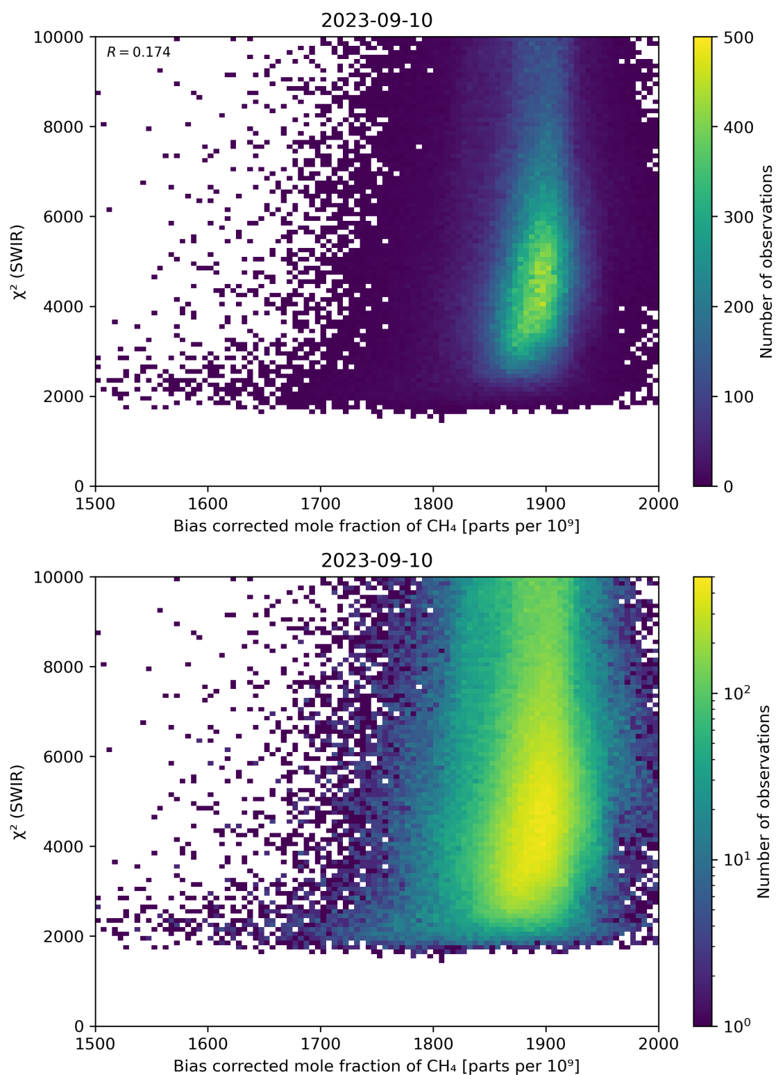
Figure 64: Scatter density plot of “Bias corrected mole fraction of CH 4 ” against “ \chi^2 (SWIR)” for 2023-09-10 to 2023-09-11.
