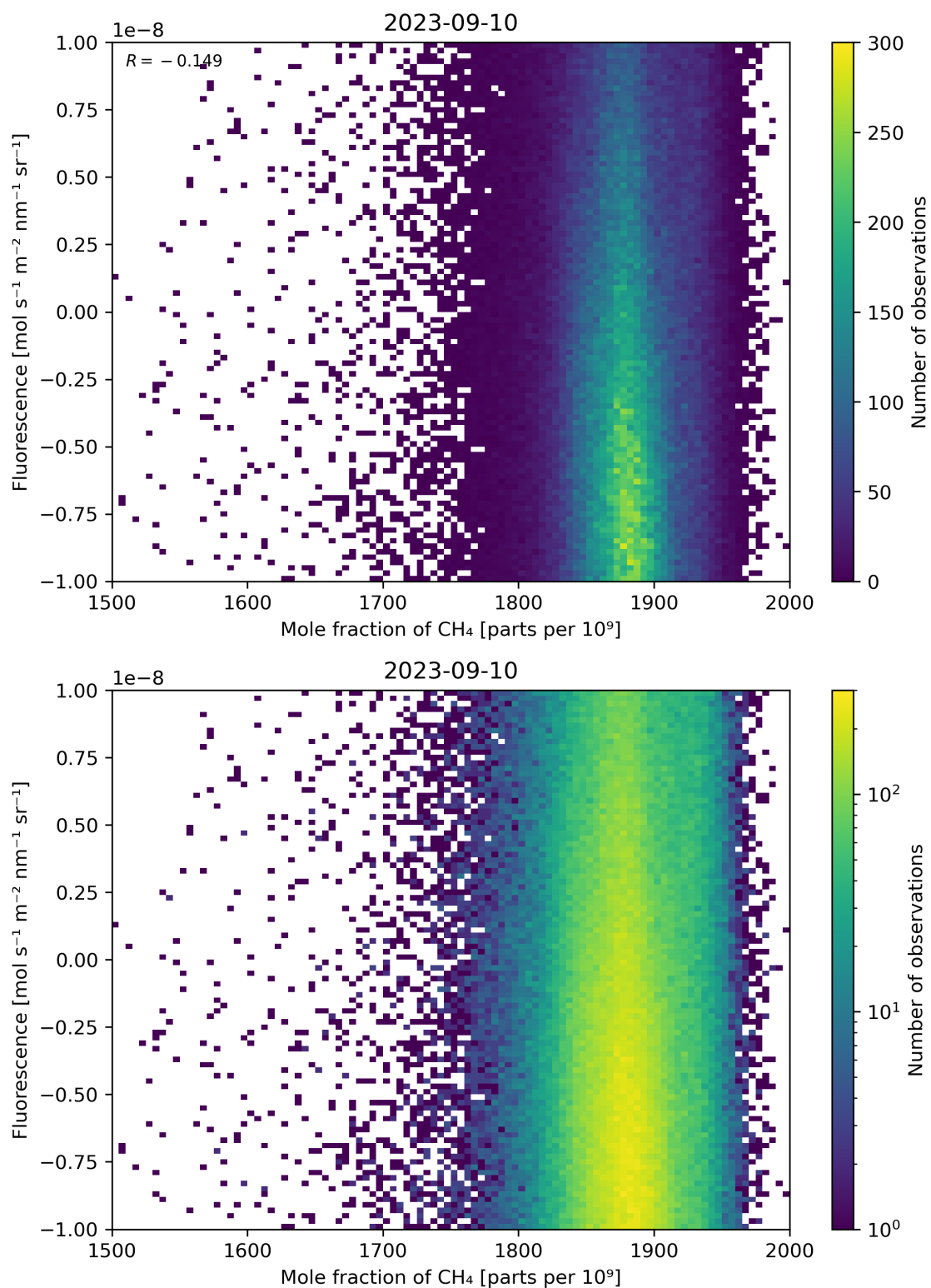
Figure 73: Scatter density plot of “Mole fraction of \text{CH}_4 ” against “Fluorescence” for 2023-09-10 to 2023-09-11.
