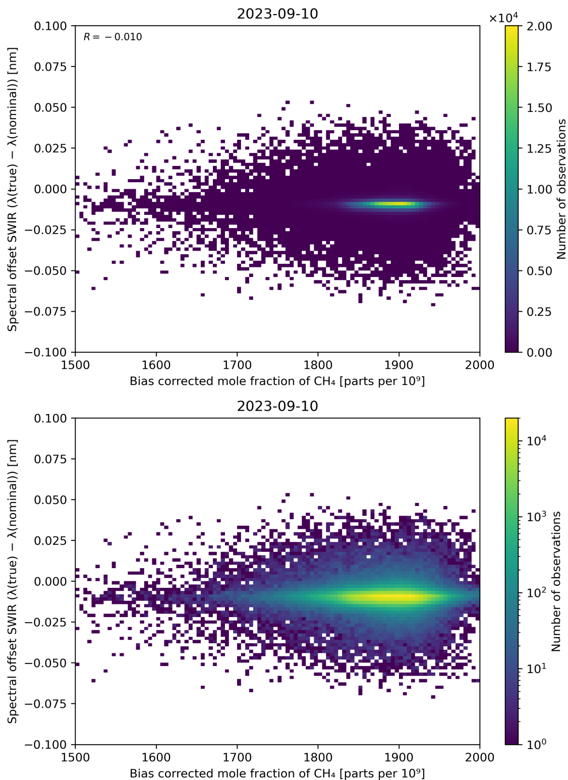
Figure 69: Scatter density plot of “Bias corrected mole fraction of \text{CH}_4 ” against “Spectral offset SWIR ( \lambda(\text{true}) - \lambda(\text{nominal}) )” for 2023-09-10 to 2023-09-11.
