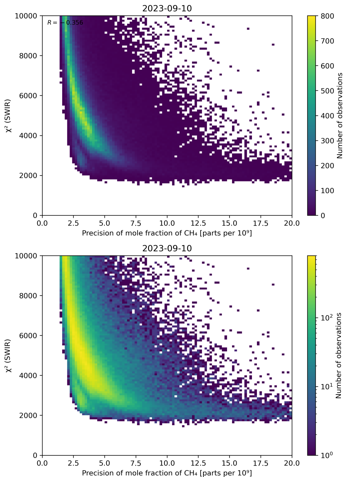
Figure 79: Scatter density plot of “Precision of mole fraction of CH 4 ” against “ \chi^2 (SWIR)” for 2023-09-10 to 2023-09-11.
