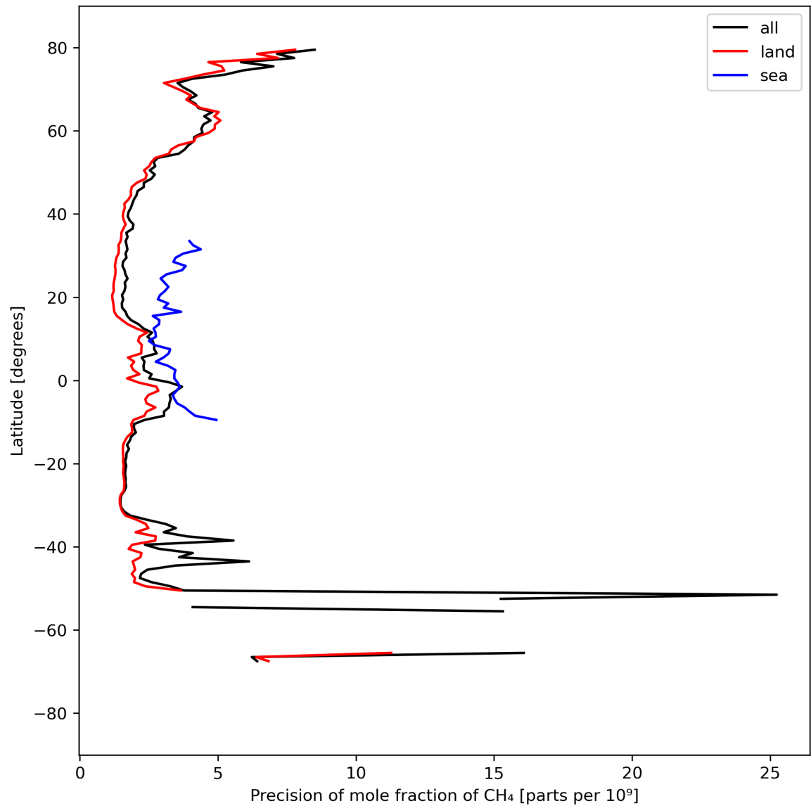
Figure 13: Zonal average of “Precision of mole fraction of CH 4 ” for 2023-09-10 to 2023-09-11.
