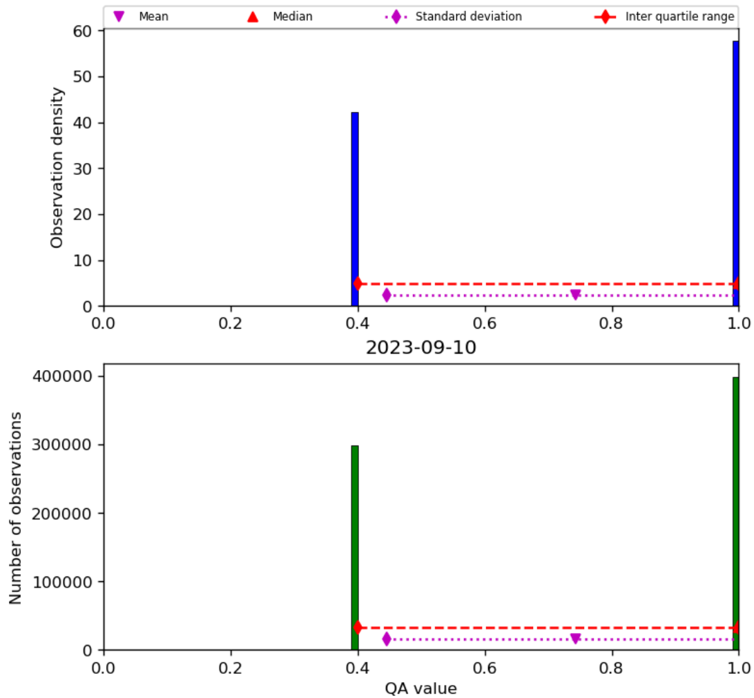
Figure 22: Histogram of “QA value” for 2023-09-10 to 2023-09-11
