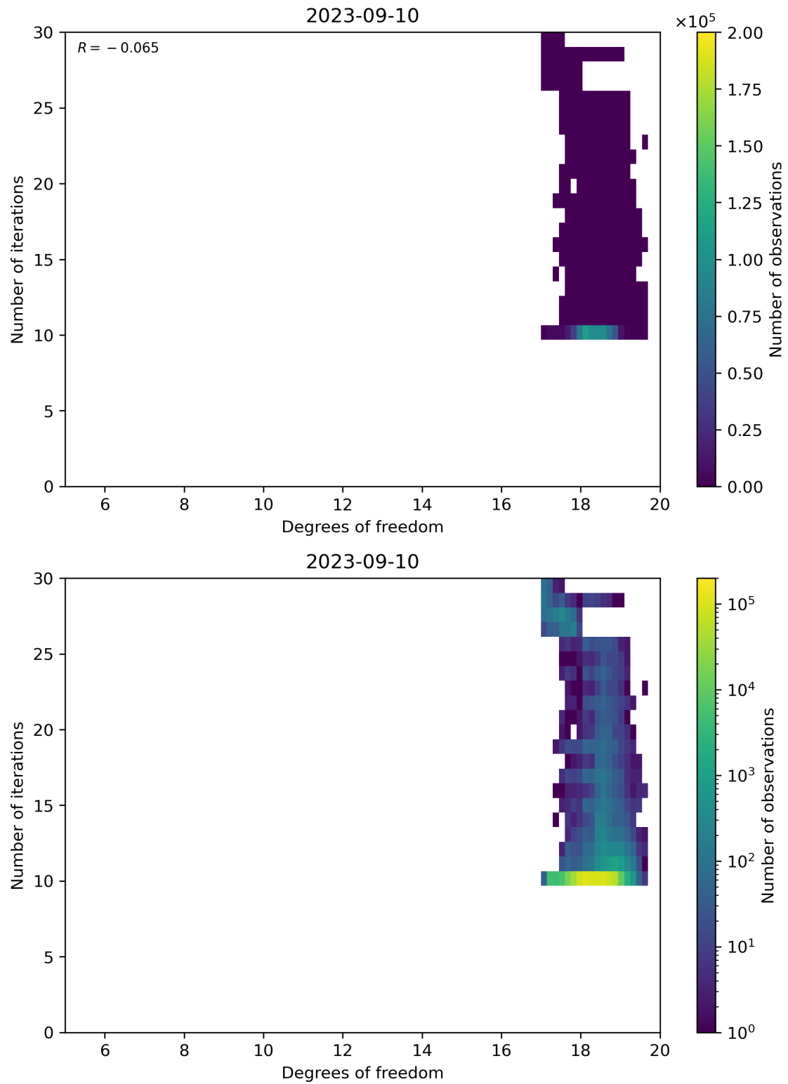
Figure 52: Scatter density plot of “Degrees of freedom” against “Number of iterations” for 2023-09-10 to 2023-09-11.
