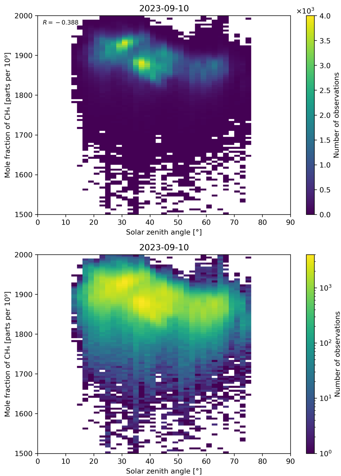
Figure 99: Scatter density plot of “Solar zenith angle” against “Mole fraction of CH 4 ” for 2023-09-10 to 2023-09-11.
