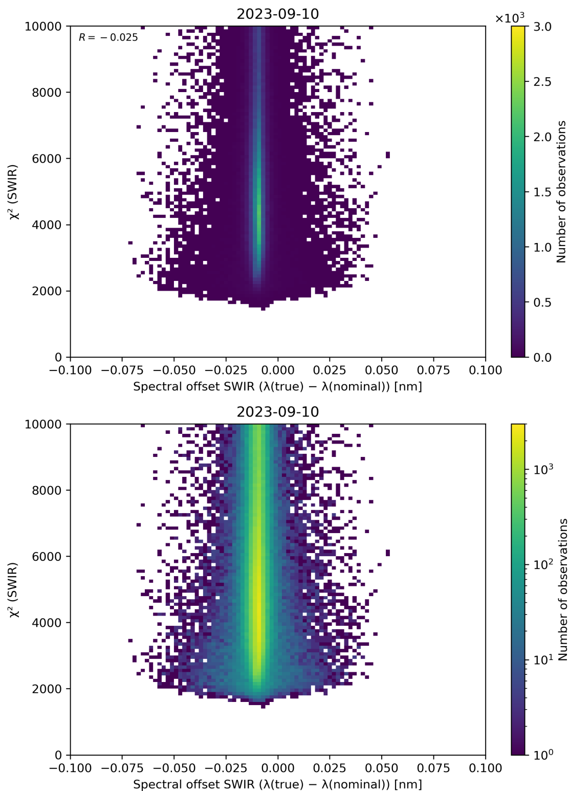
Figure 118: Scatter density plot of “Spectral offset SWIR ( \lambda(\text{true}) - \lambda(\text{nominal}) )” against “ \chi^2 (SWIR)” for 2023-09-10 to 2023-09-11.
