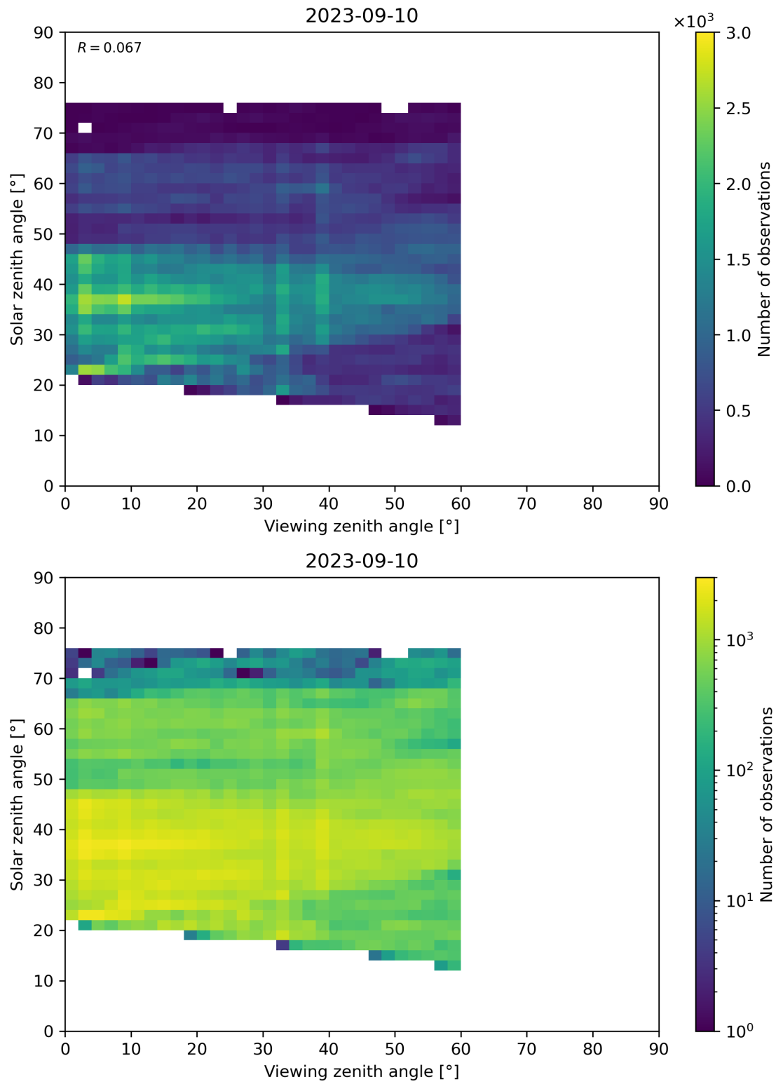
Figure 115: Scatter density plot of “Viewing zenith angle” against “Solar zenith angle” for 2023-09-10 to 2023-09-11.
