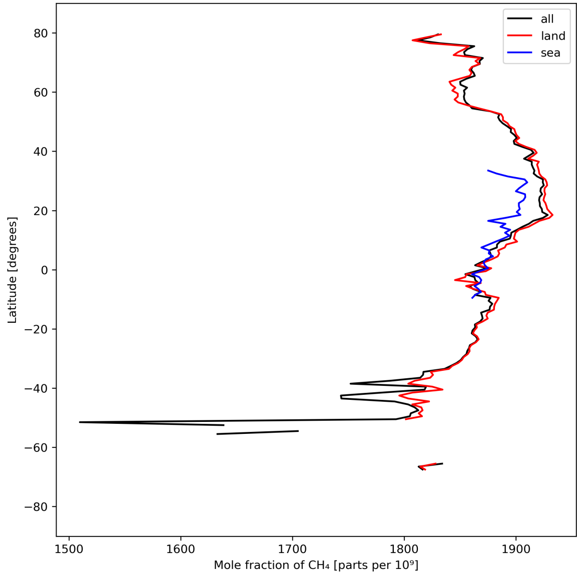
Figure 12: Zonal average of “Mole fraction of CH 4 ” for 2023-09-10 to 2023-09-11.
