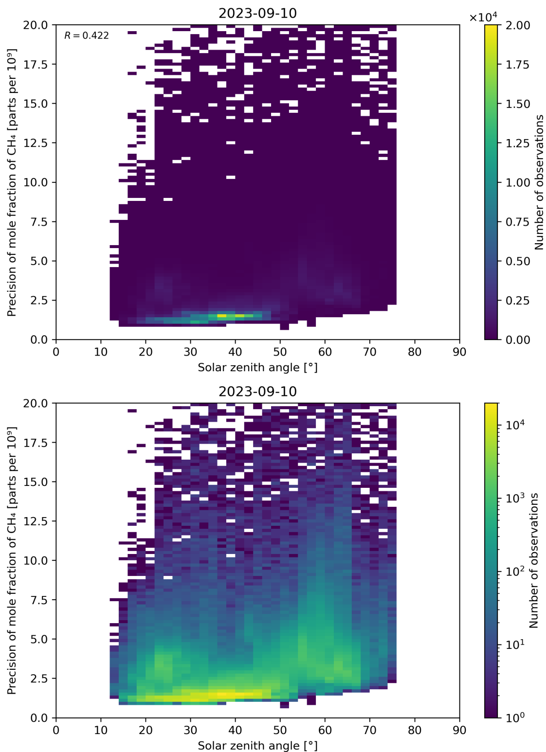
Figure 101: Scatter density plot of “Solar zenith angle” against “Precision of mole fraction of \text{CH}_4 ” for 2023-09-10 to 2023-09-11.
