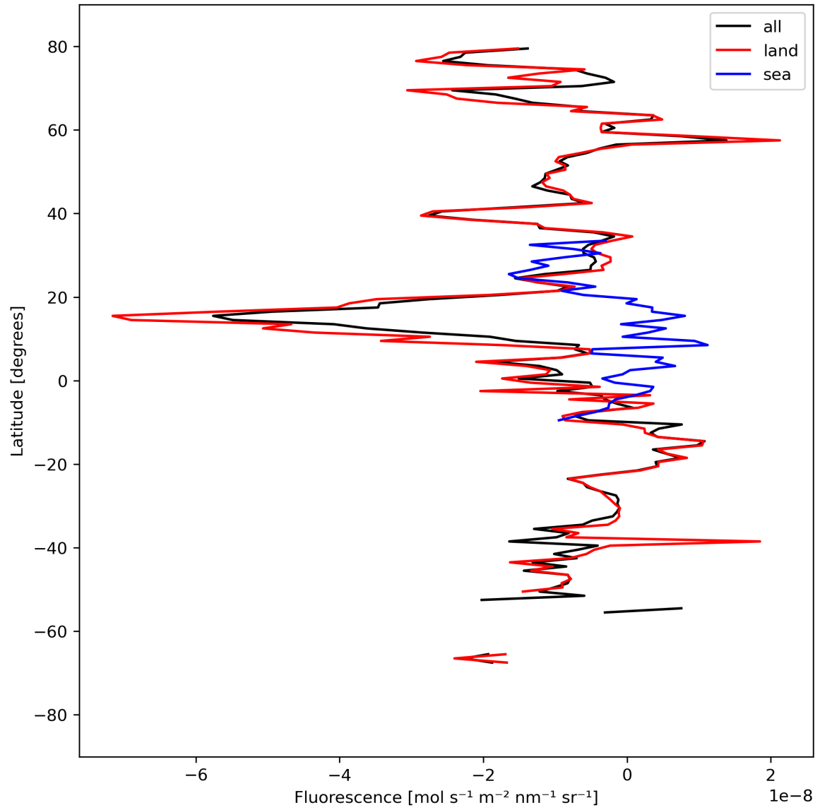
Figure 21: Zonal average of “Fluorescence” for 2023-09-10 to 2023-09-11.
