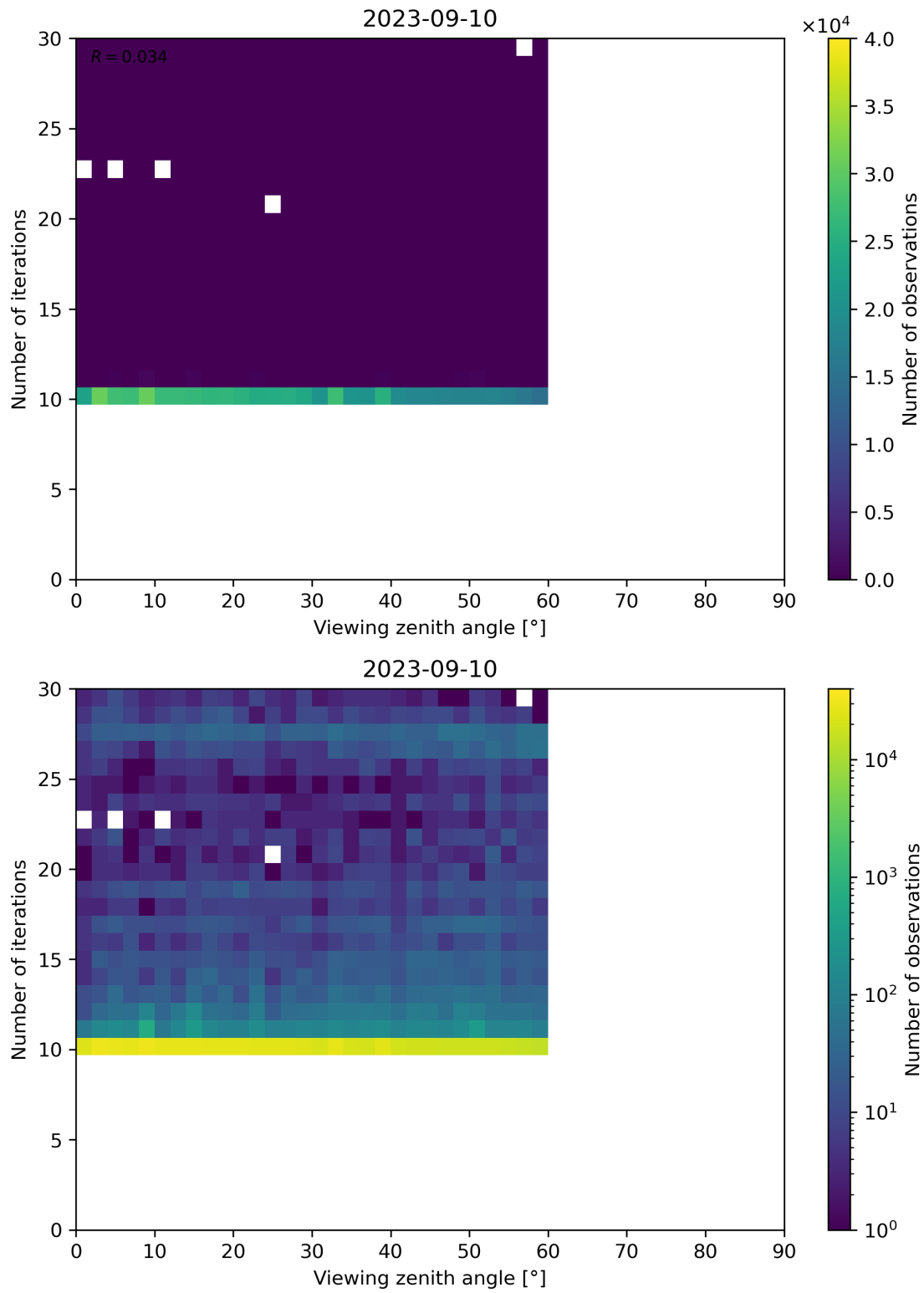
Figure 113: Scatter density plot of “Viewing zenith angle” against “Number of iterations” for 2023-09-10 to 2023-09-11.
