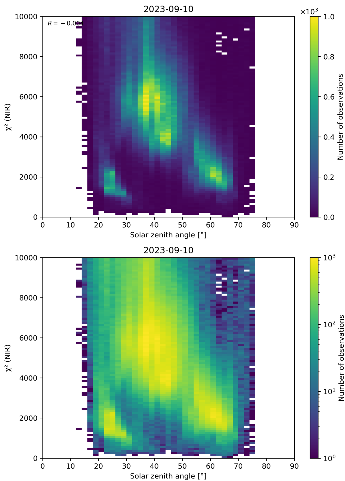
Figure 94: Scatter density plot of “Solar zenith angle” against “ \chi^2 (NIR)” for 2023-09-10 to 2023-09-11.
