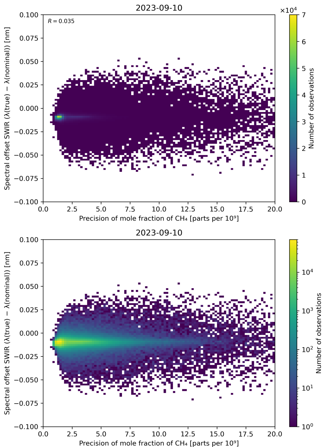
Figure 85: Scatter density plot of “Precision of mole fraction of CH 4 ” against “Spectral offset SWIR ( \lambda(\text{true}) - \lambda(\text{nominal}) )” for 2023-09-10 to 2023-09-11.
