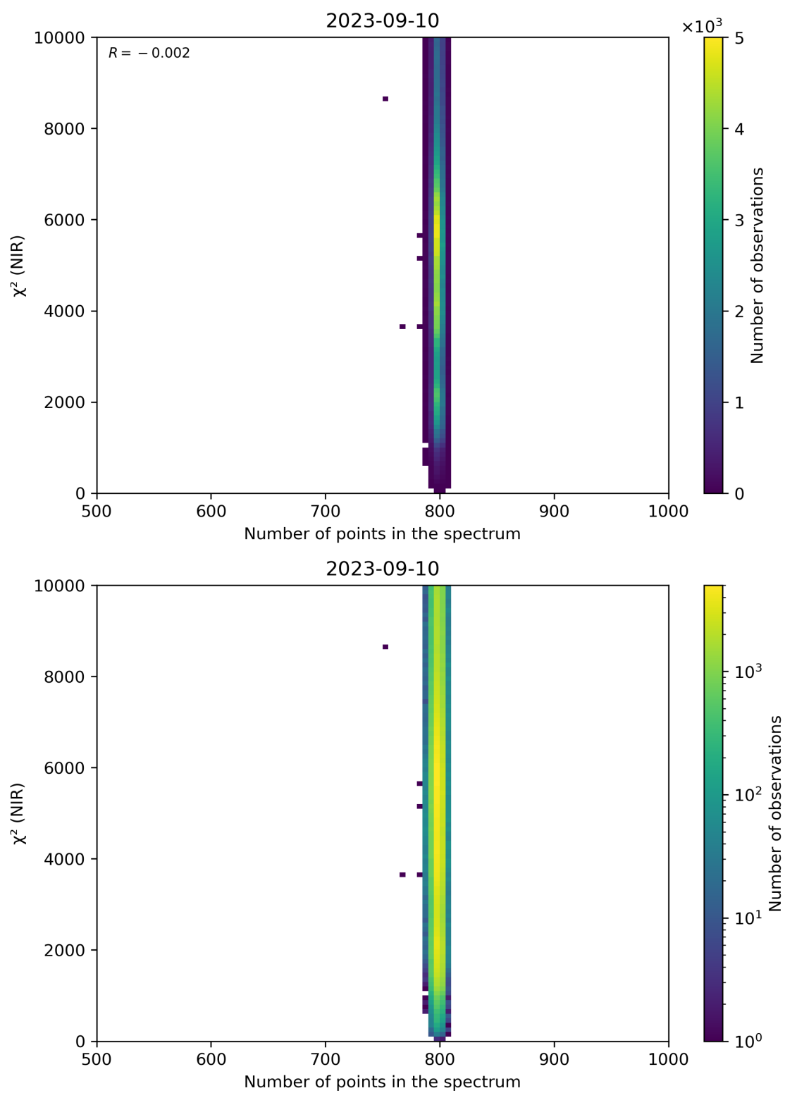
Figure 88: Scatter density plot of “Number of points in the spectrum” against “ \chi^2 (NIR)” for 2023-09-10 to 2023-09-11.
