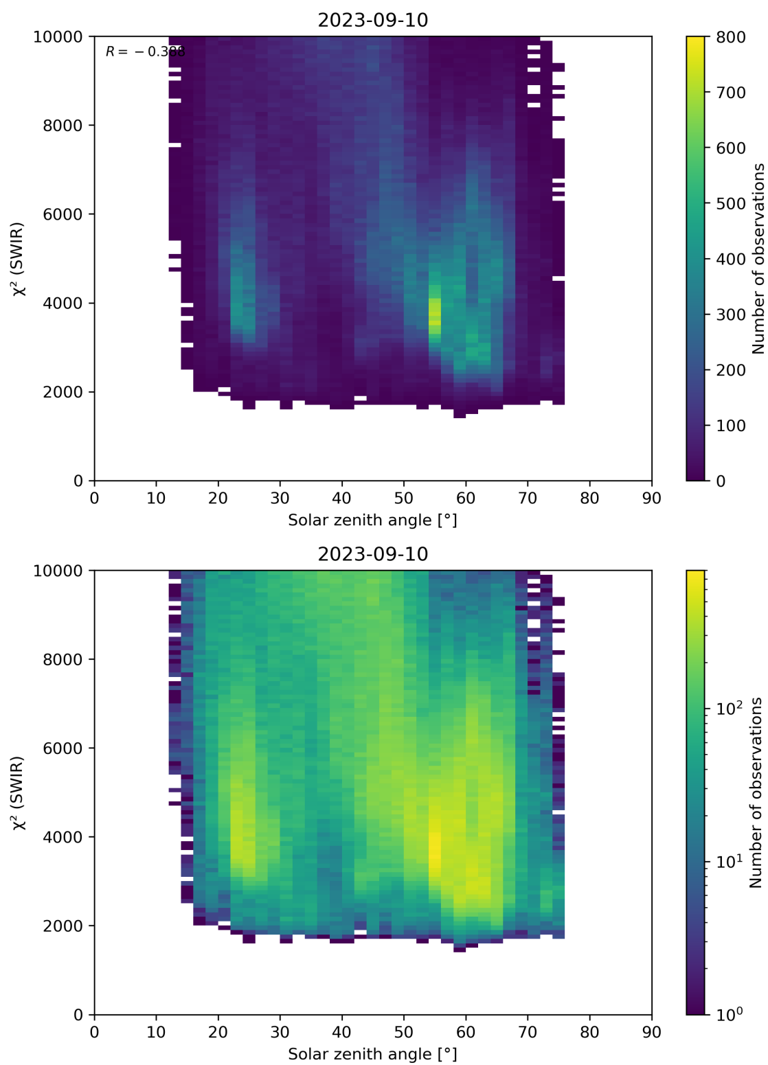
Figure 95: Scatter density plot of “Solar zenith angle” against “ \chi^2 (SWIR)” for 2023-09-10 to 2023-09-11.
