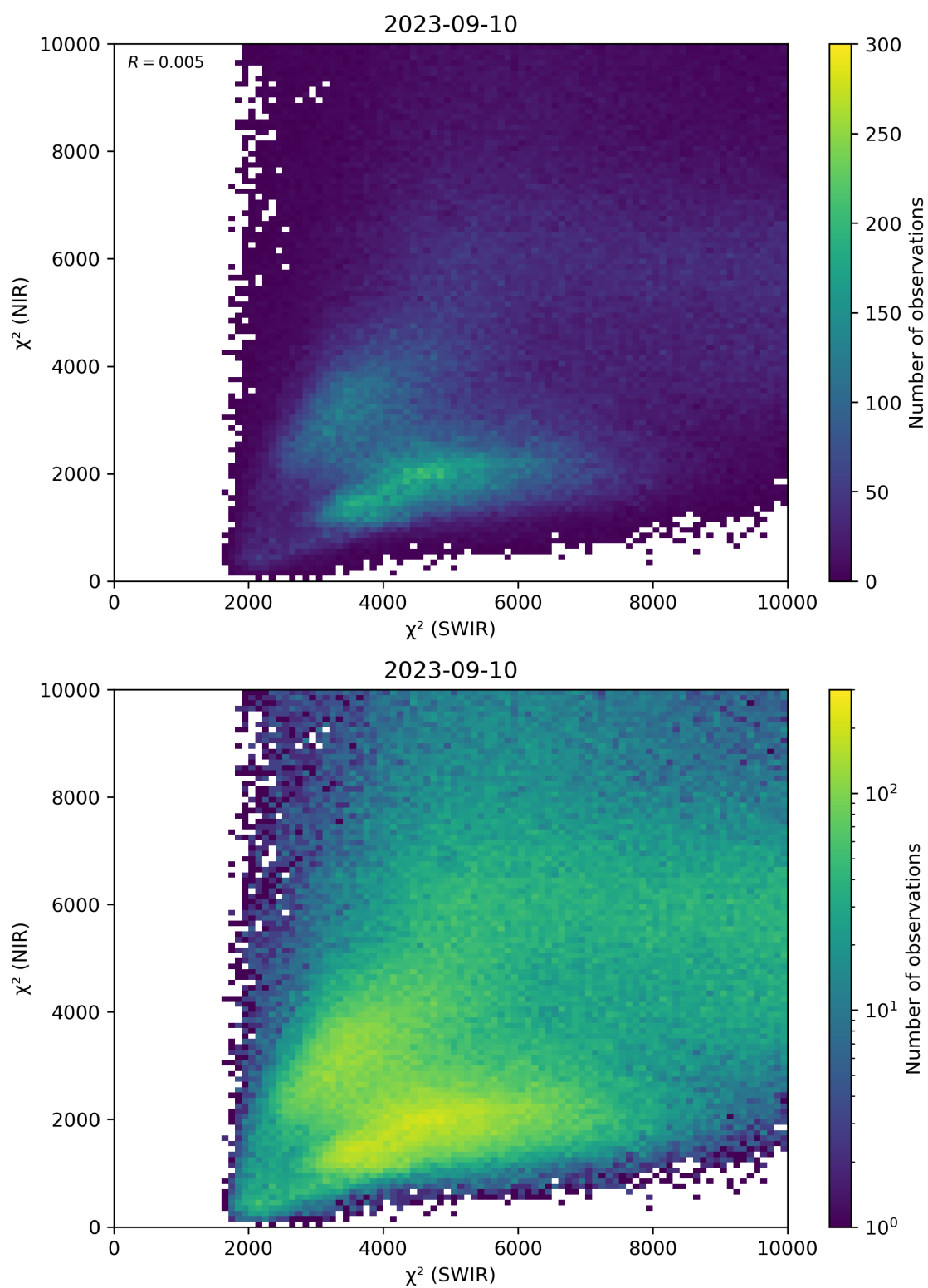
Figure 47: Scatter density plot of “ \chi^2 (SWIR)” against “ \chi^2 (NIR)” for 2023-09-10 to 2023-09-11.
