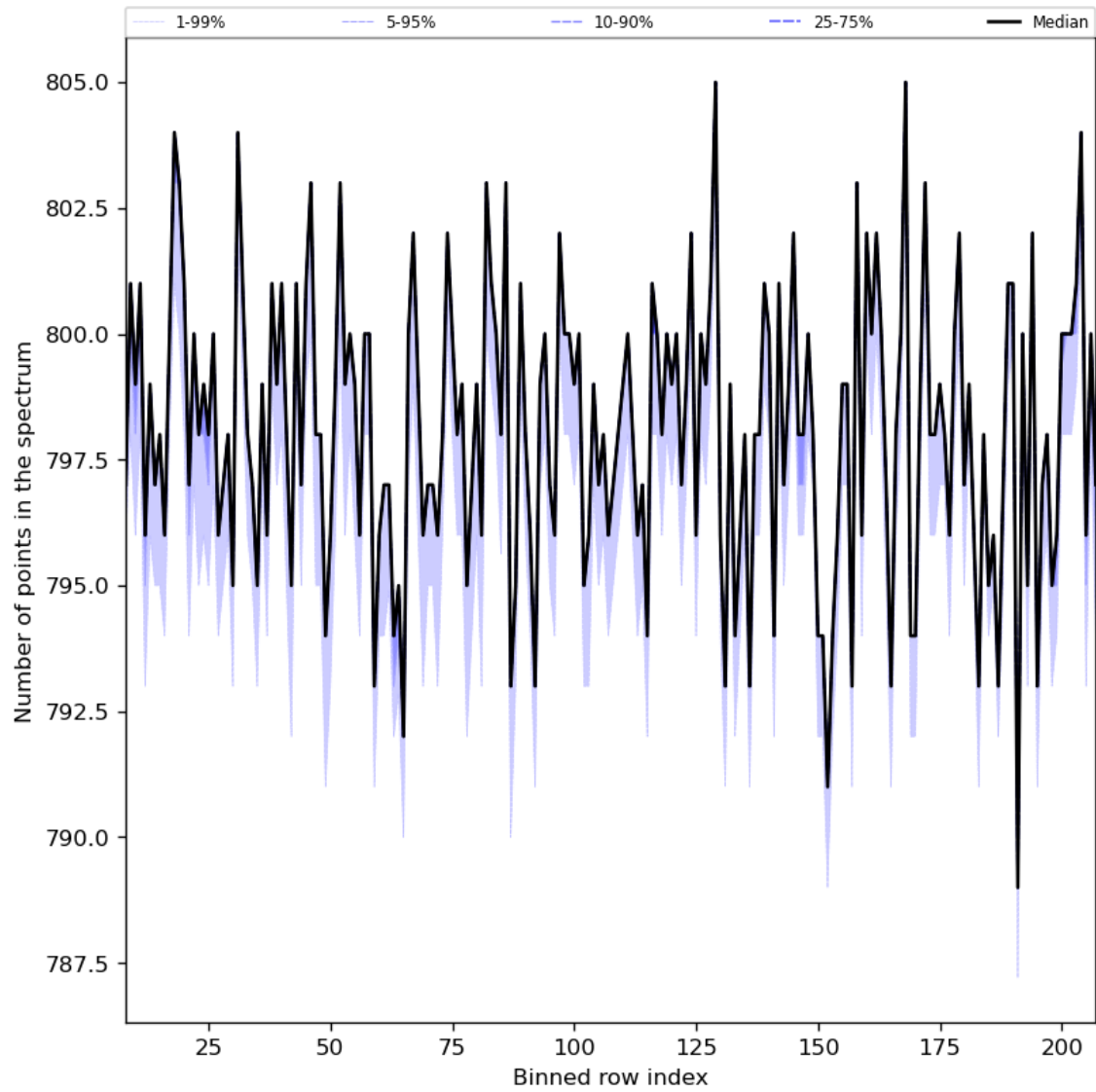
Figure 37: Along track statistics of “Number of points in the spectrum” for 2023-09-10 to 2023-09-11
