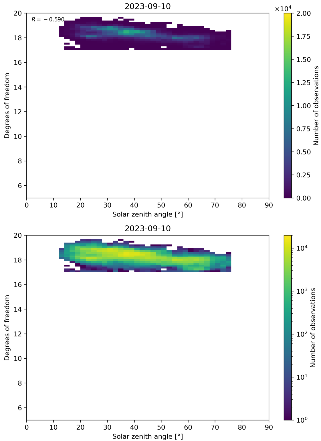
Figure 96: Scatter density plot of “Solar zenith angle” against “Degrees of freedom” for 2023-09-10 to 2023-09-11.
