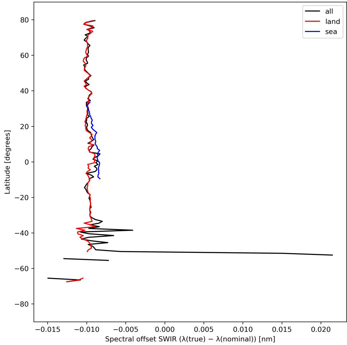
Figure 16: Zonal average of “Spectral offset SWIR ( \lambda(\text{true}) - \lambda(\text{nominal}) )” for 2023-09-10 to 2023-09-11.
