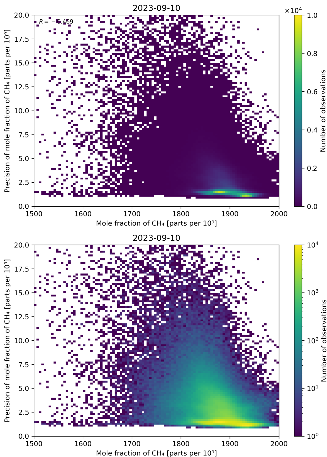
Figure 75: Scatter density plot of “Mole fraction of CH 4 ” against “Precision of mole fraction of CH 4 ” for 2023-09-10 to 2023-09-11.
