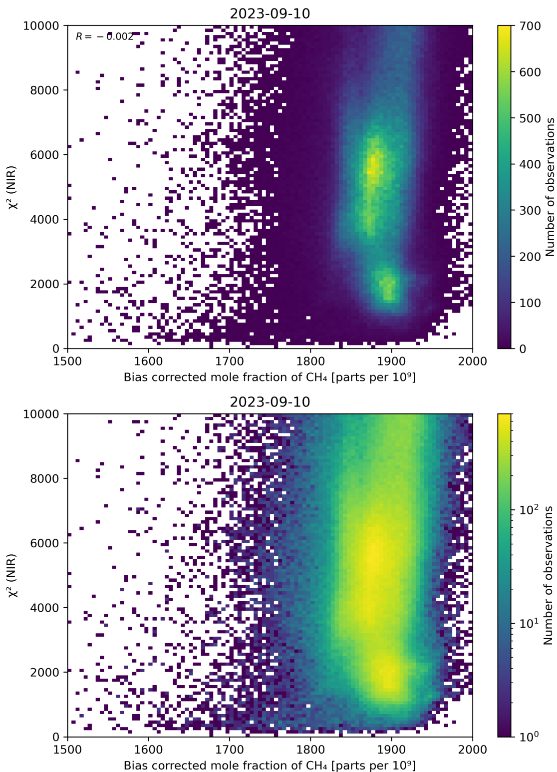
Figure 63: Scatter density plot of “Bias corrected mole fraction of CH 4 ” against “ \chi^2 (NIR)” for 2023-09-10 to 2023-09-11.
