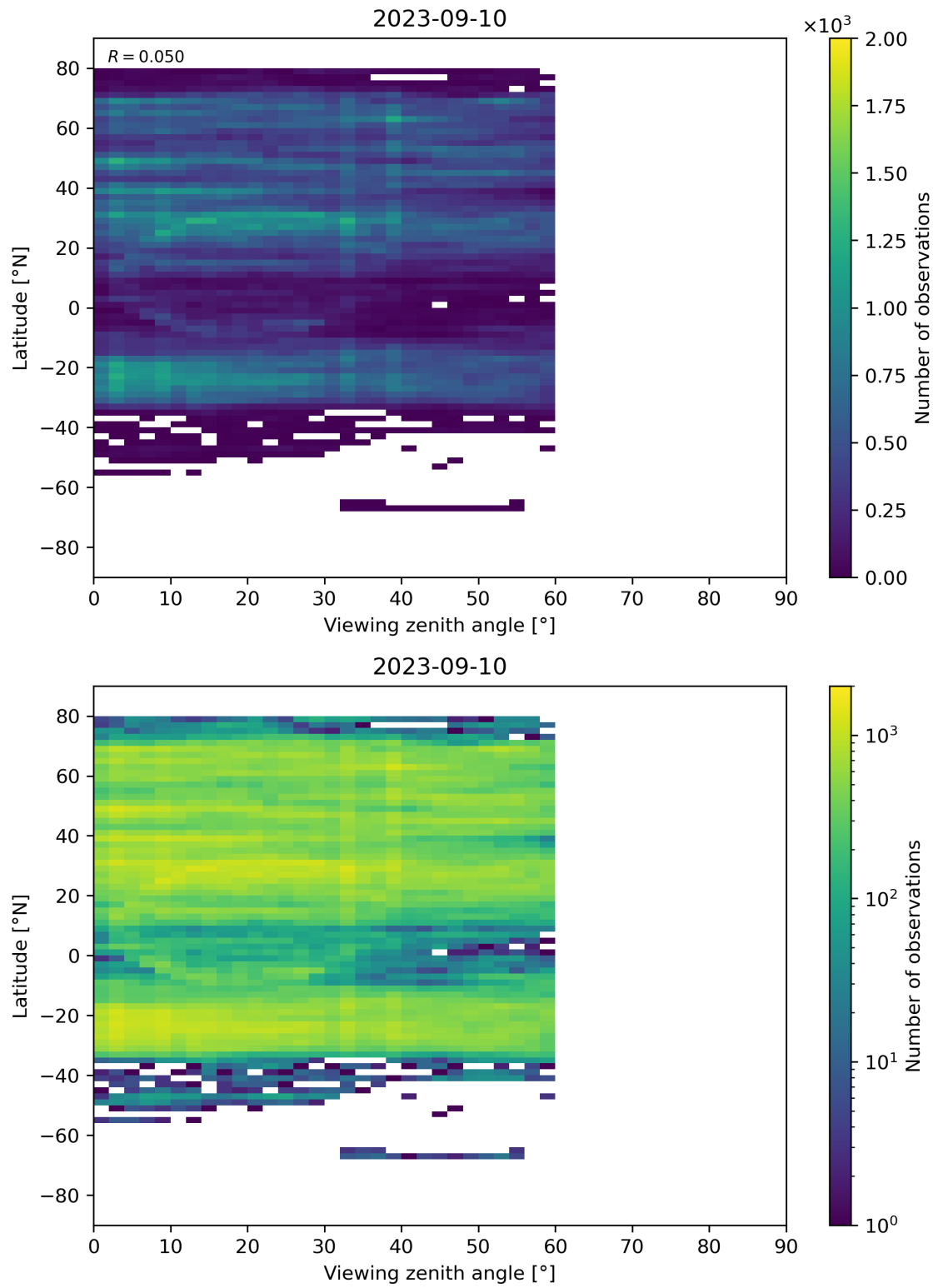
Figure 109: Scatter density plot of “Viewing zenith angle” against “Latitude” for 2023-09-10 to 2023-09-11.
