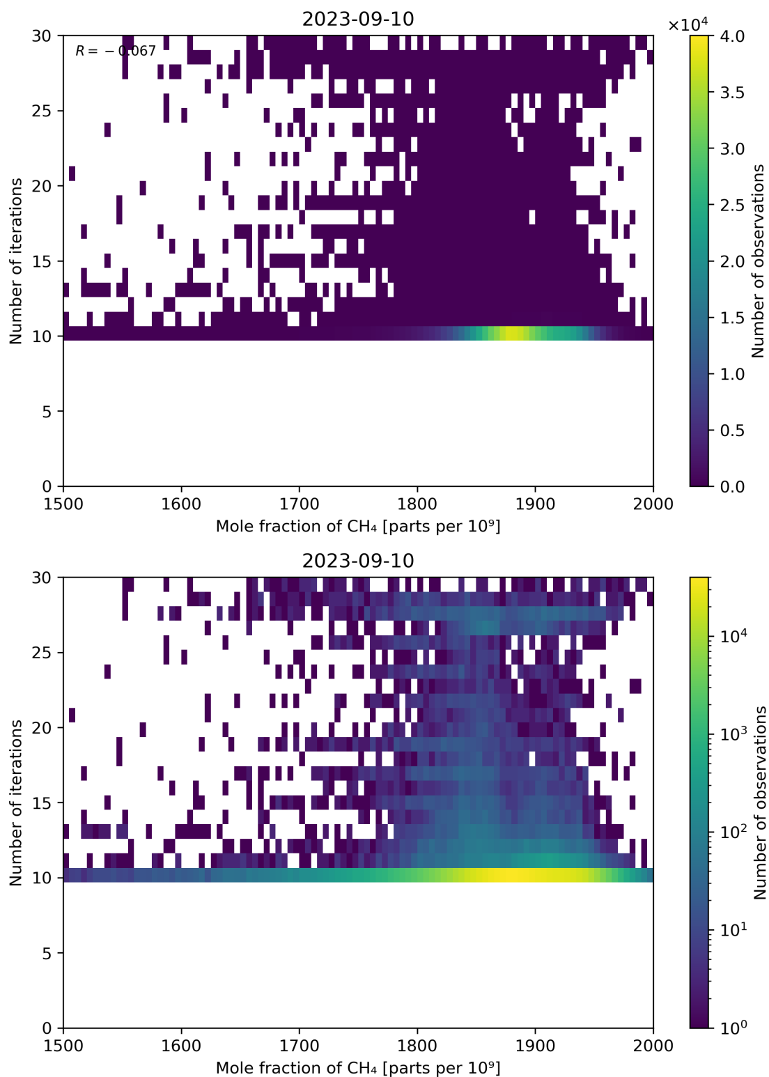
Figure 76: Scatter density plot of “Mole fraction of CH 4 ” against “Number of iterations” for 2023-09-10 to 2023-09-11.
