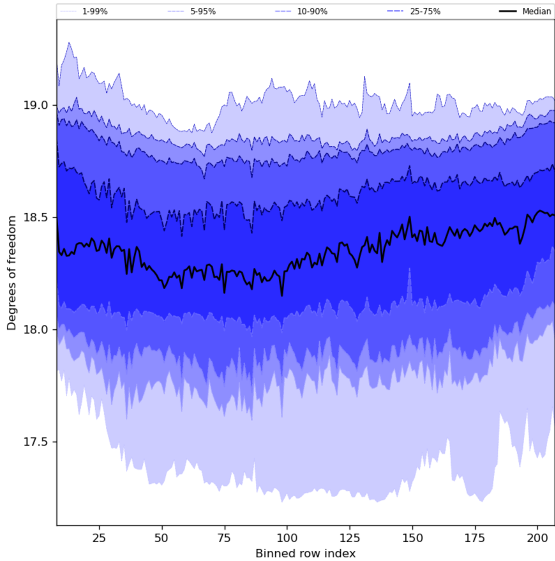
Figure 41: Along track statistics of “Degrees of freedom” for 2023-09-10 to 2023-09-11
