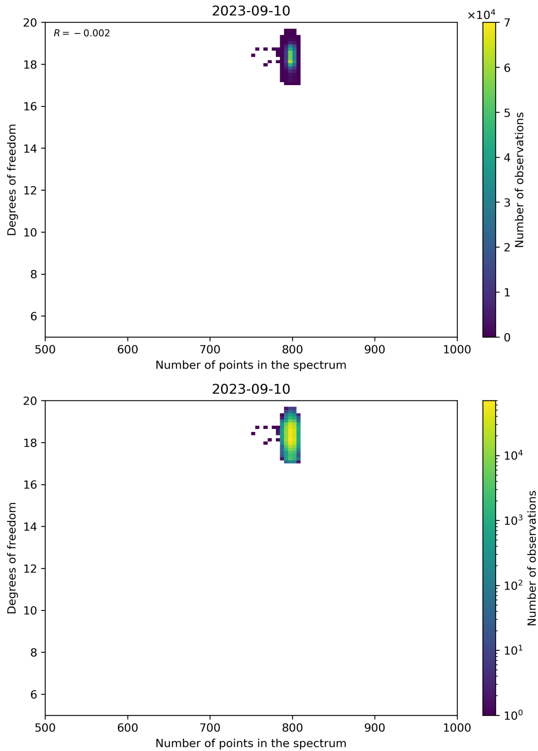
Figure 90: Scatter density plot of “Number of points in the spectrum” against “Degrees of freedom” for 2023-09-10 to 2023-09-11.
