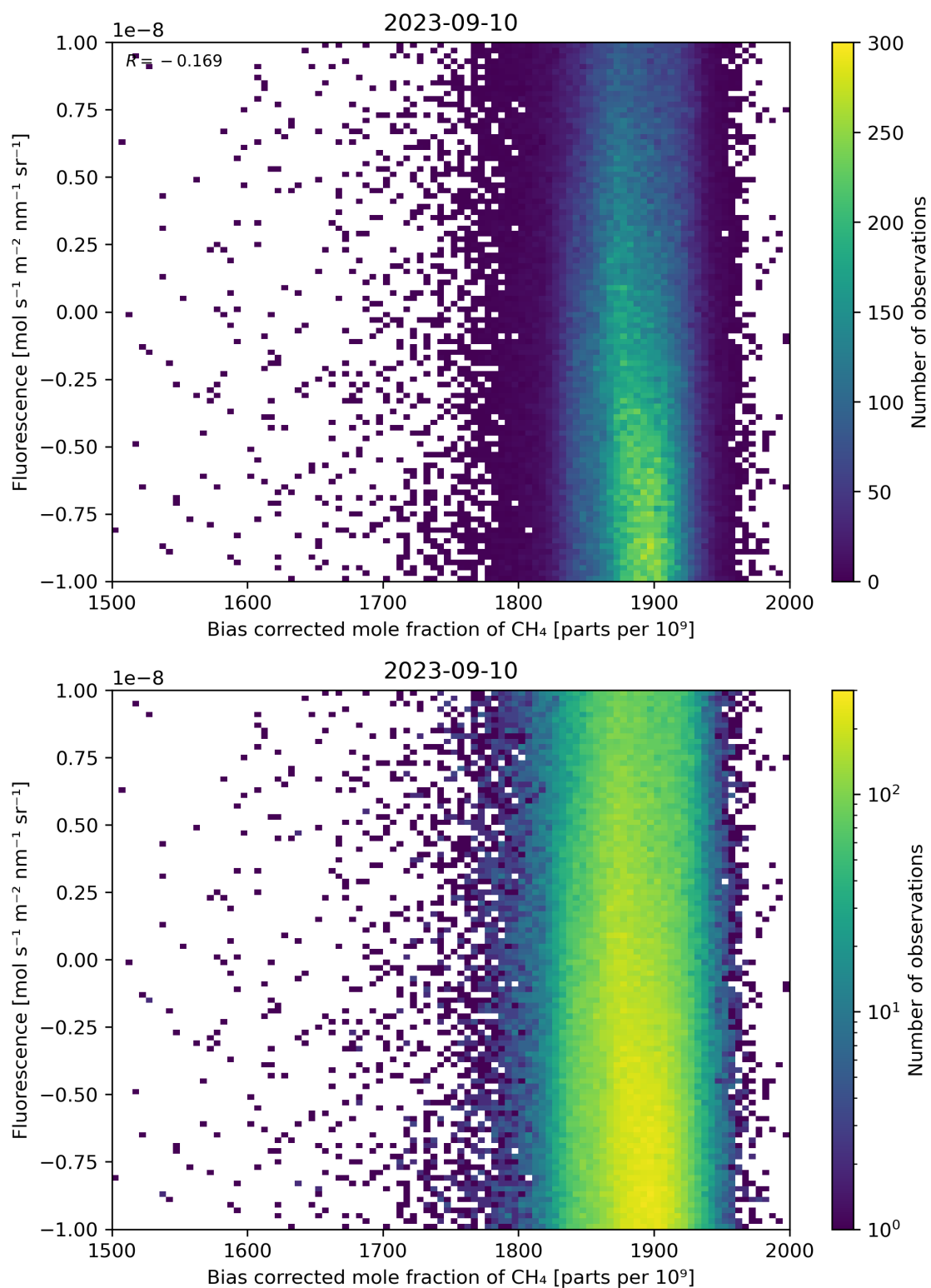
Figure 66: Scatter density plot of “Bias corrected mole fraction of CH 4 ” against “Fluorescence” for 2023-09-10 to 2023-09-11.
