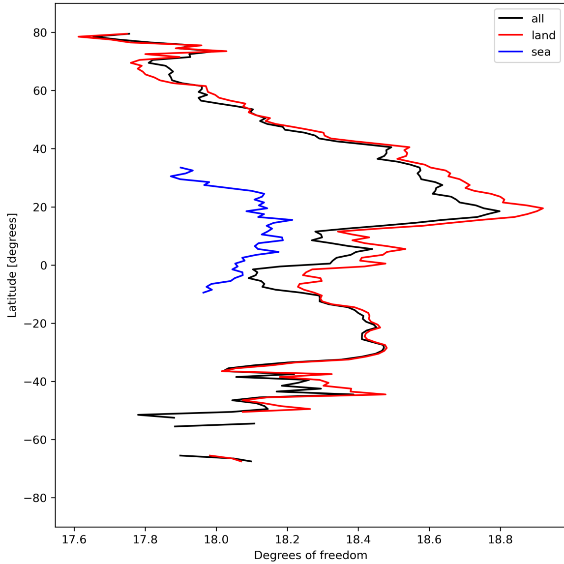
Figure 19: Zonal average of “Degrees of freedom” for 2023-09-10 to 2023-09-11.
