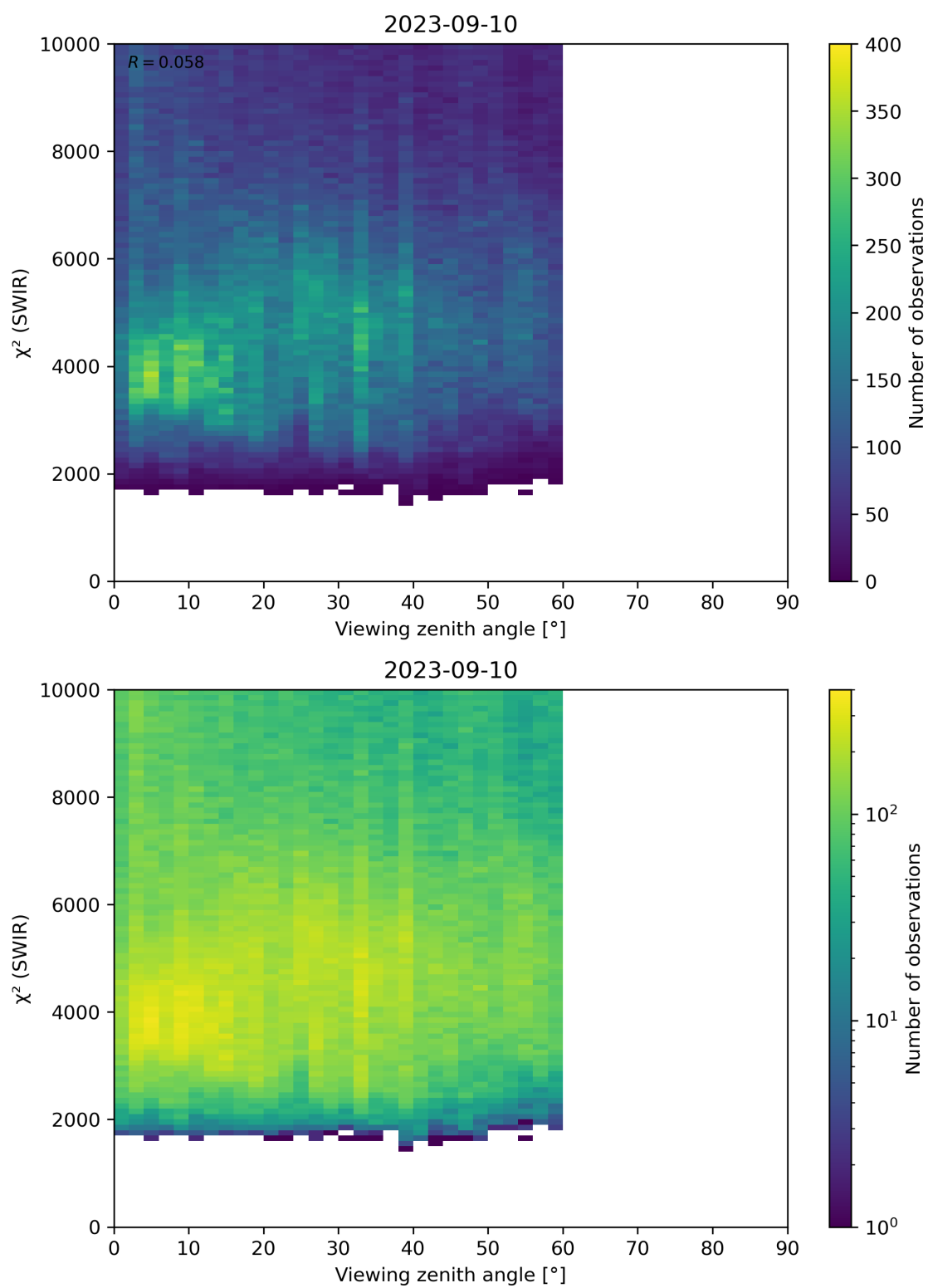
Figure 106: Scatter density plot of “Viewing zenith angle” against “ \chi^2 (SWIR)” for 2023-09-10 to 2023-09-11.
