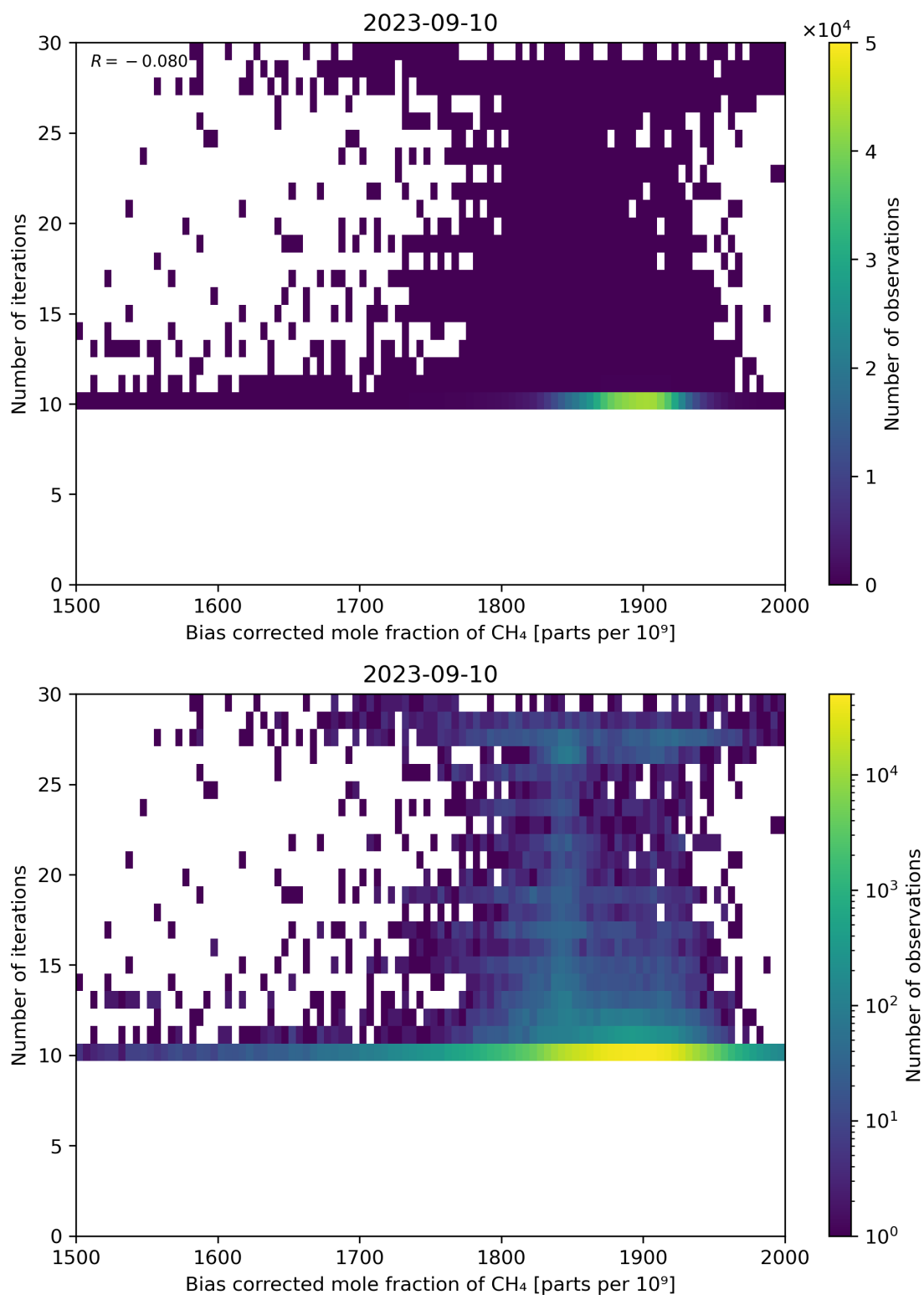
Figure 67: Scatter density plot of “Bias corrected mole fraction of \text{CH}_4 ” against “Number of iterations” for 2023-09-10 to 2023-09-11.
