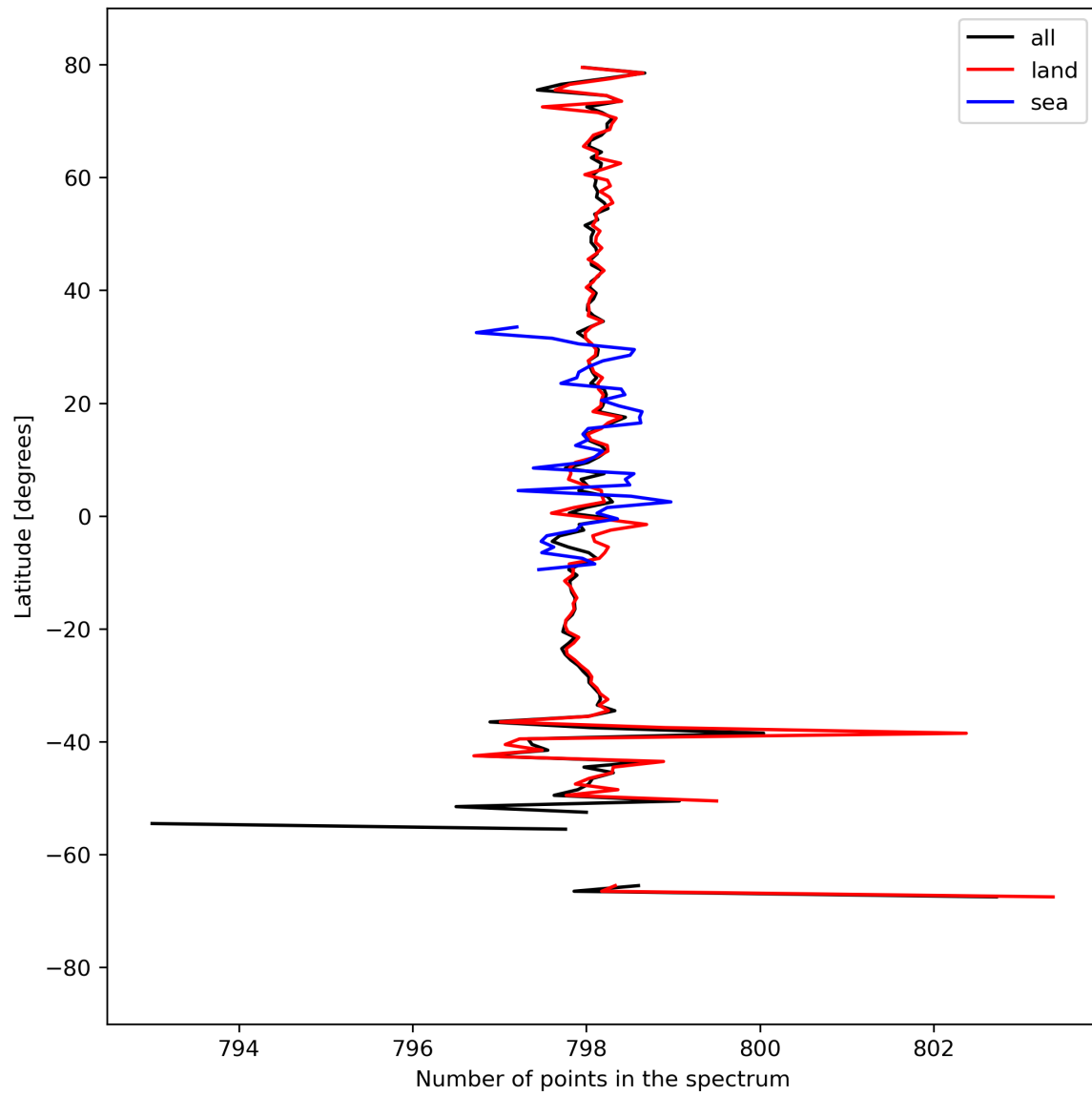
Figure 15: Zonal average of “Number of points in the spectrum” for 2023-09-10 to 2023-09-11.
