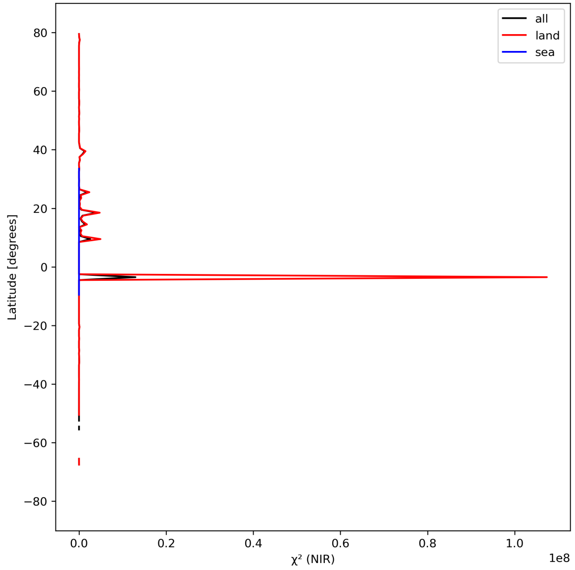
Figure 18: Zonal average of “ \chi^2 (NIR)” for 2023-09-10 to 2023-09-11.
