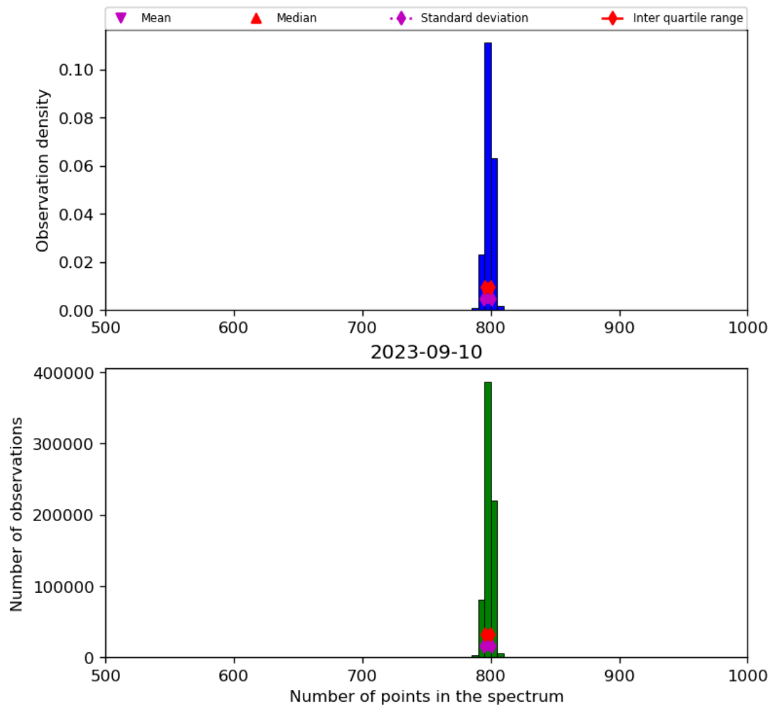
Figure 26: Histogram of “Number of points in the spectrum” for 2023-09-10 to 2023-09-11
