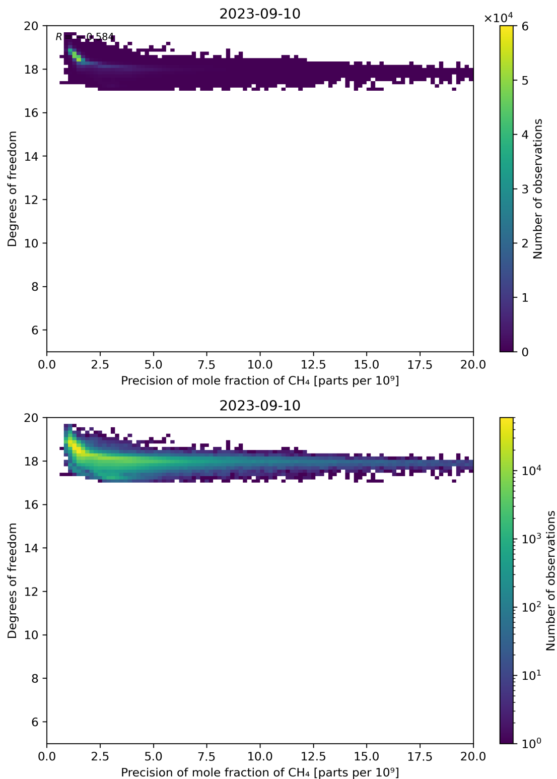
Figure 80: Scatter density plot of “Precision of mole fraction of CH 4 ” against “Degrees of freedom” for 2023-09-10 to 2023-09-11.
