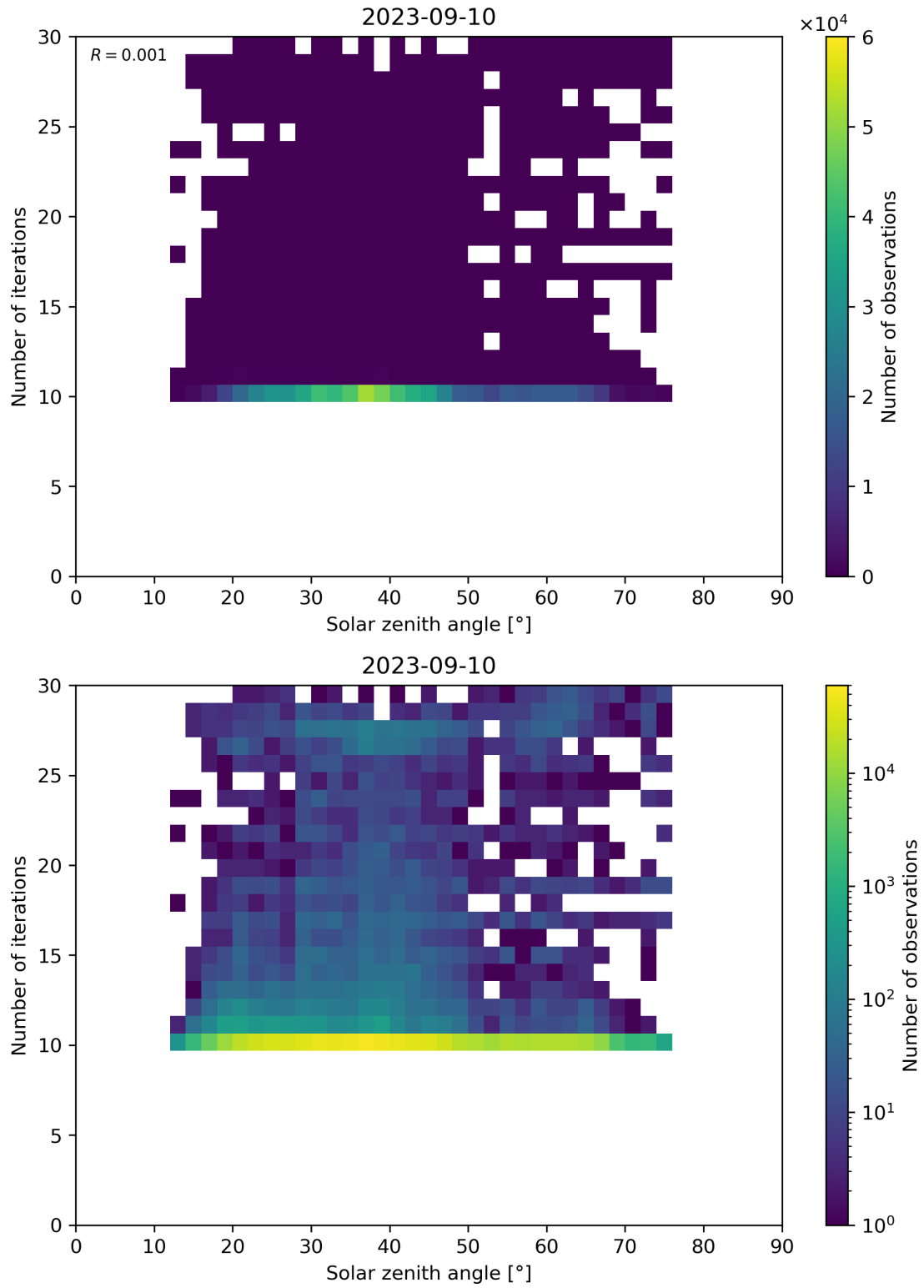
Figure 102: Scatter density plot of “Solar zenith angle” against “Number of iterations” for 2023-09-10 to 2023-09-11.
