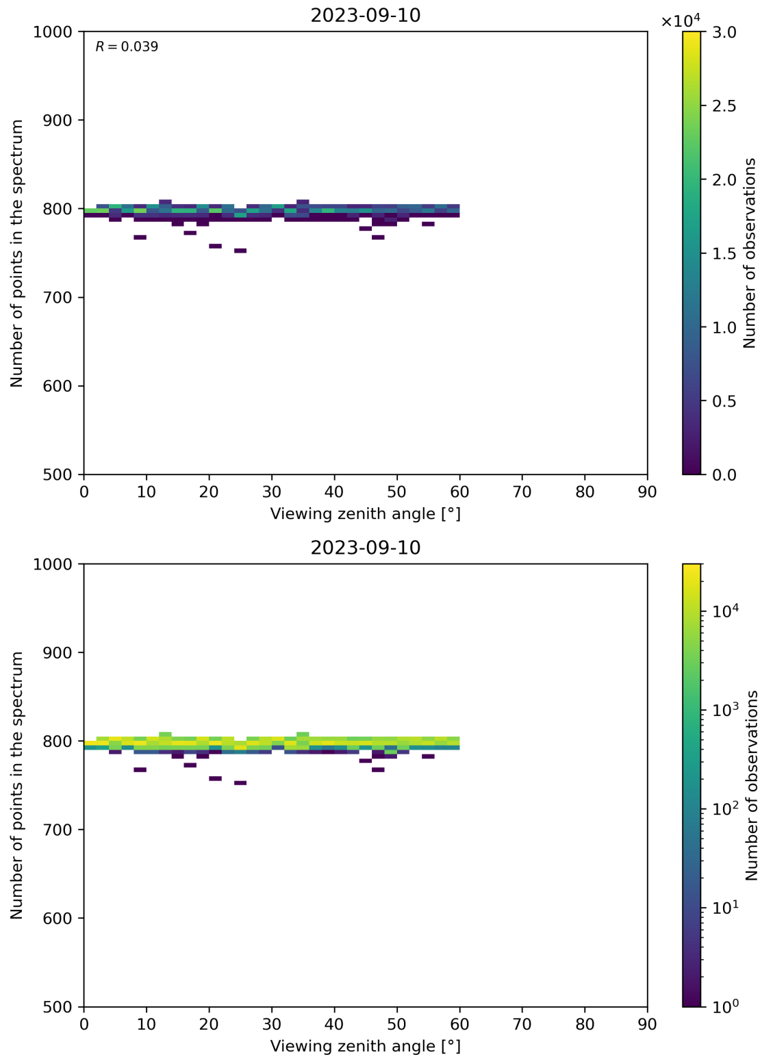
Figure 114: Scatter density plot of “Viewing zenith angle” against “Number of points in the spectrum” for 2023-09-10 to 2023-09-11.
