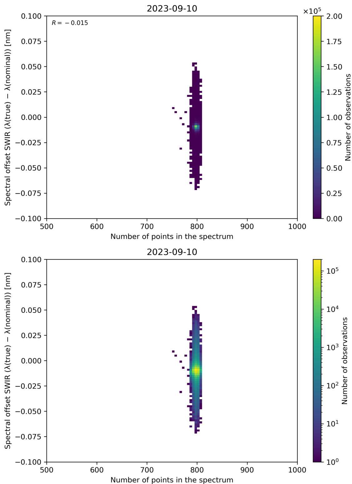
Figure 93: Scatter density plot of “Number of points in the spectrum” against “Spectral offset SWIR ( \lambda(\text{true}) - \lambda(\text{nominal}) )” for 2023-09-10 to 2023-09-11.
