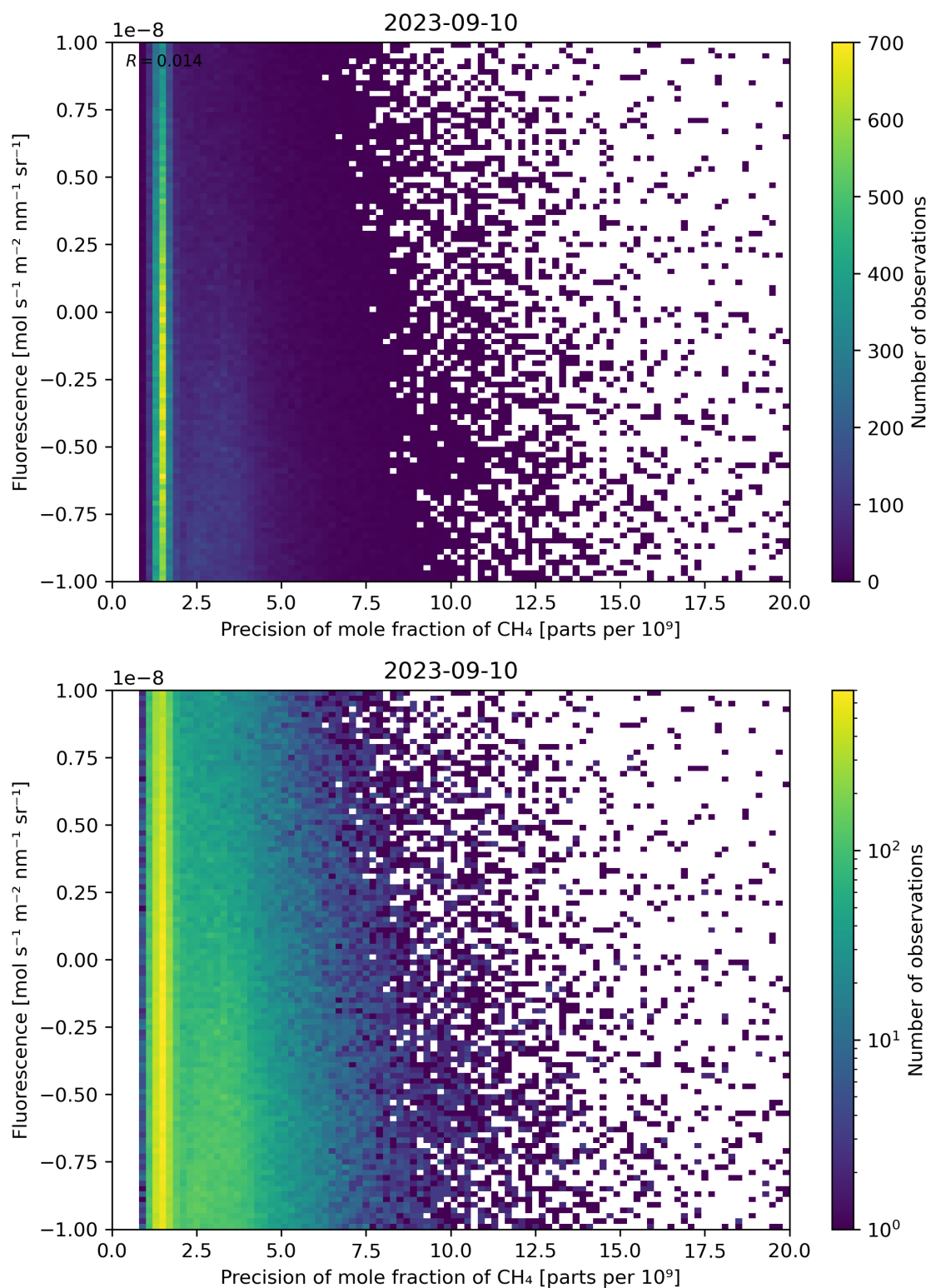
Figure 81: Scatter density plot of “Precision of mole fraction of \text{CH}_4 ” against “Fluorescence” for 2023-09-10 to 2023-09-11.
