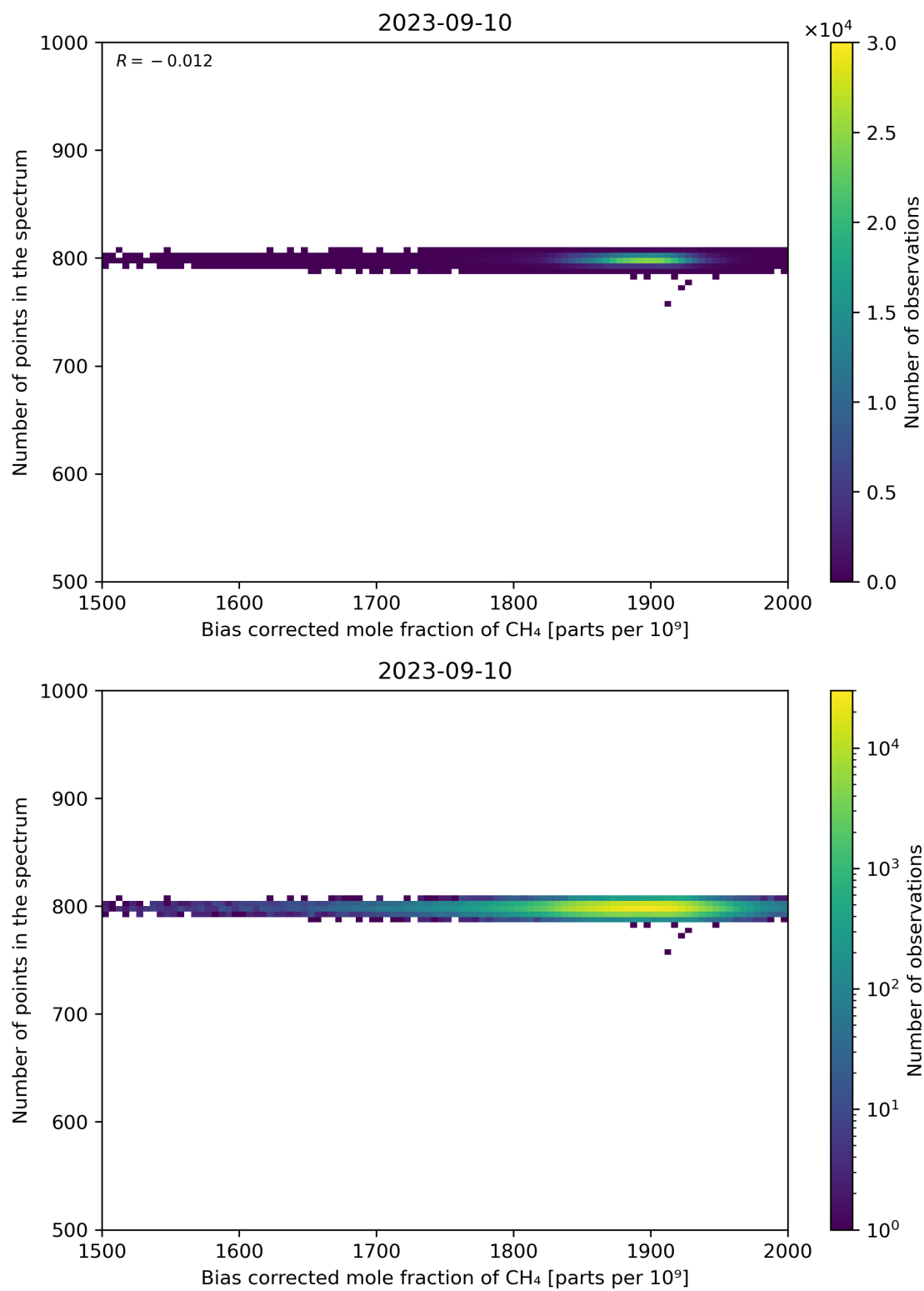
Figure 68: Scatter density plot of “Bias corrected mole fraction of CH 4 ” against “Number of points in the spectrum” for 2023-09-10 to 2023-09-11.
