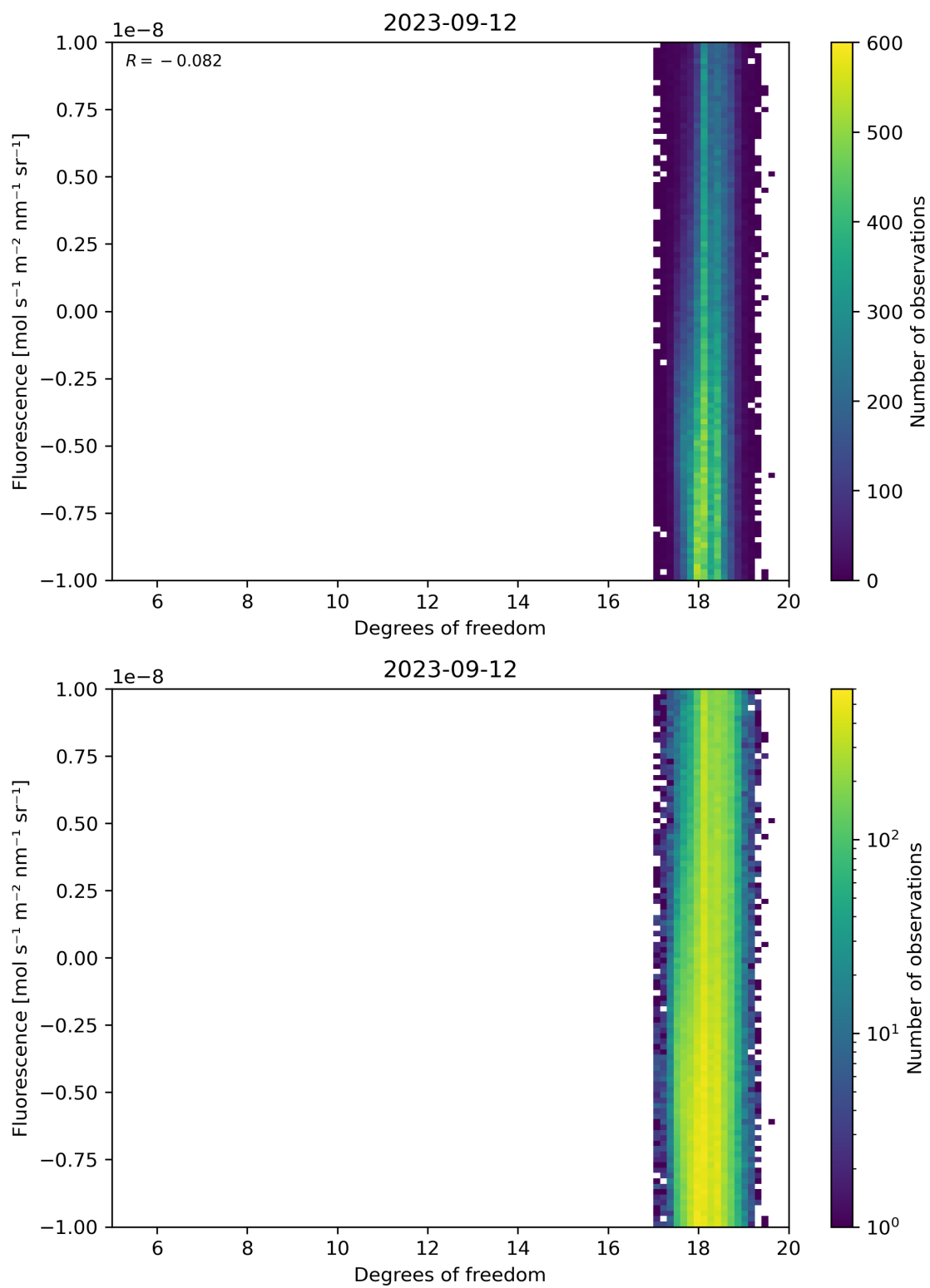
Figure 51: Scatter density plot of “Degrees of freedom” against “Fluorescence” for 2023-09-11 to 2023-09-13.
