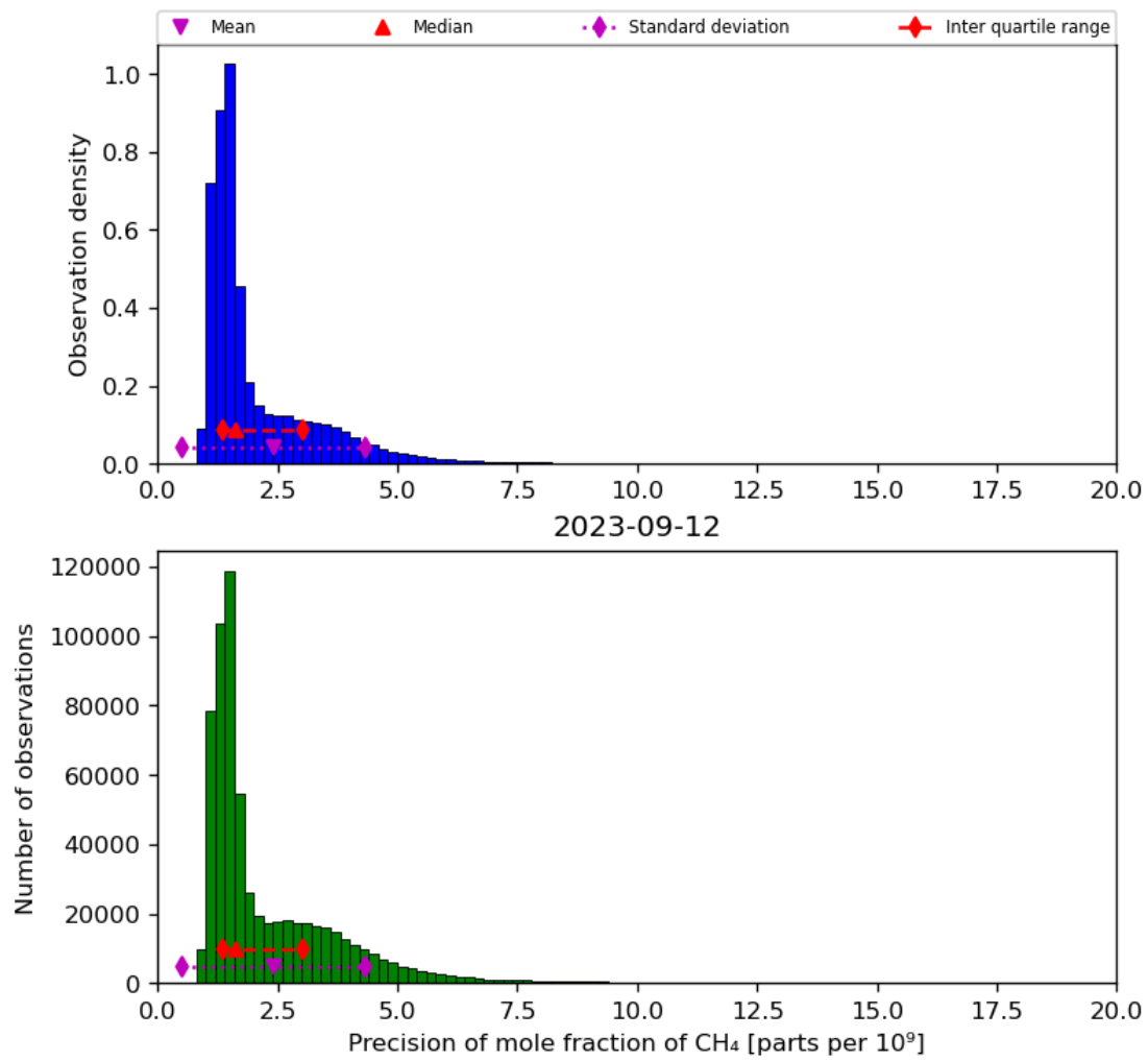
Figure 24: Histogram of “Precision of mole fraction of CH 4 ” for 2023-09-11 to 2023-09-13
