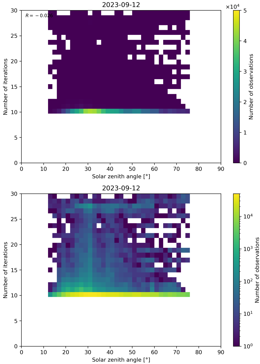
Figure 102: Scatter density plot of “Solar zenith angle” against “Number of iterations” for 2023-09-11 to 2023-09-13.
