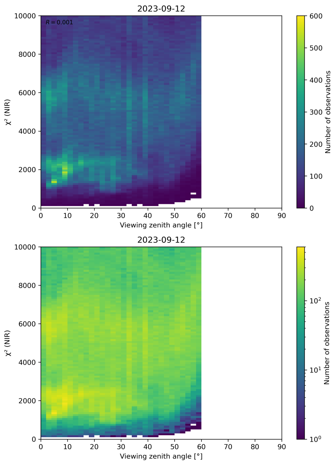
Figure 105: Scatter density plot of “Viewing zenith angle” against “ \chi^2 (NIR)” for 2023-09-11 to 2023-09-13.
