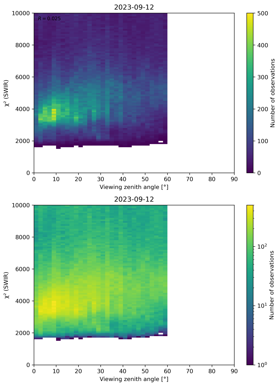
Figure 106: Scatter density plot of “Viewing zenith angle” against “ \chi^2 (SWIR)” for 2023-09-11 to 2023-09-13.
