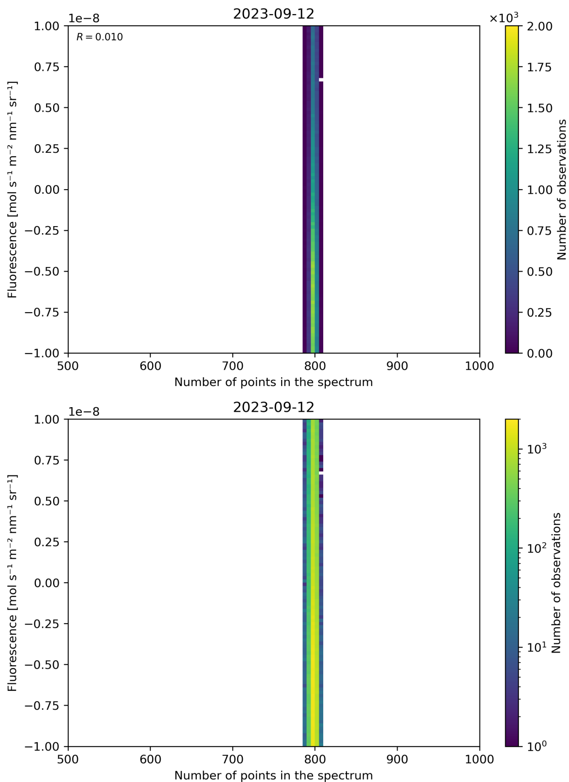
Figure 91: Scatter density plot of “Number of points in the spectrum” against “Fluorescence” for 2023-09-11 to 2023-09-13.
