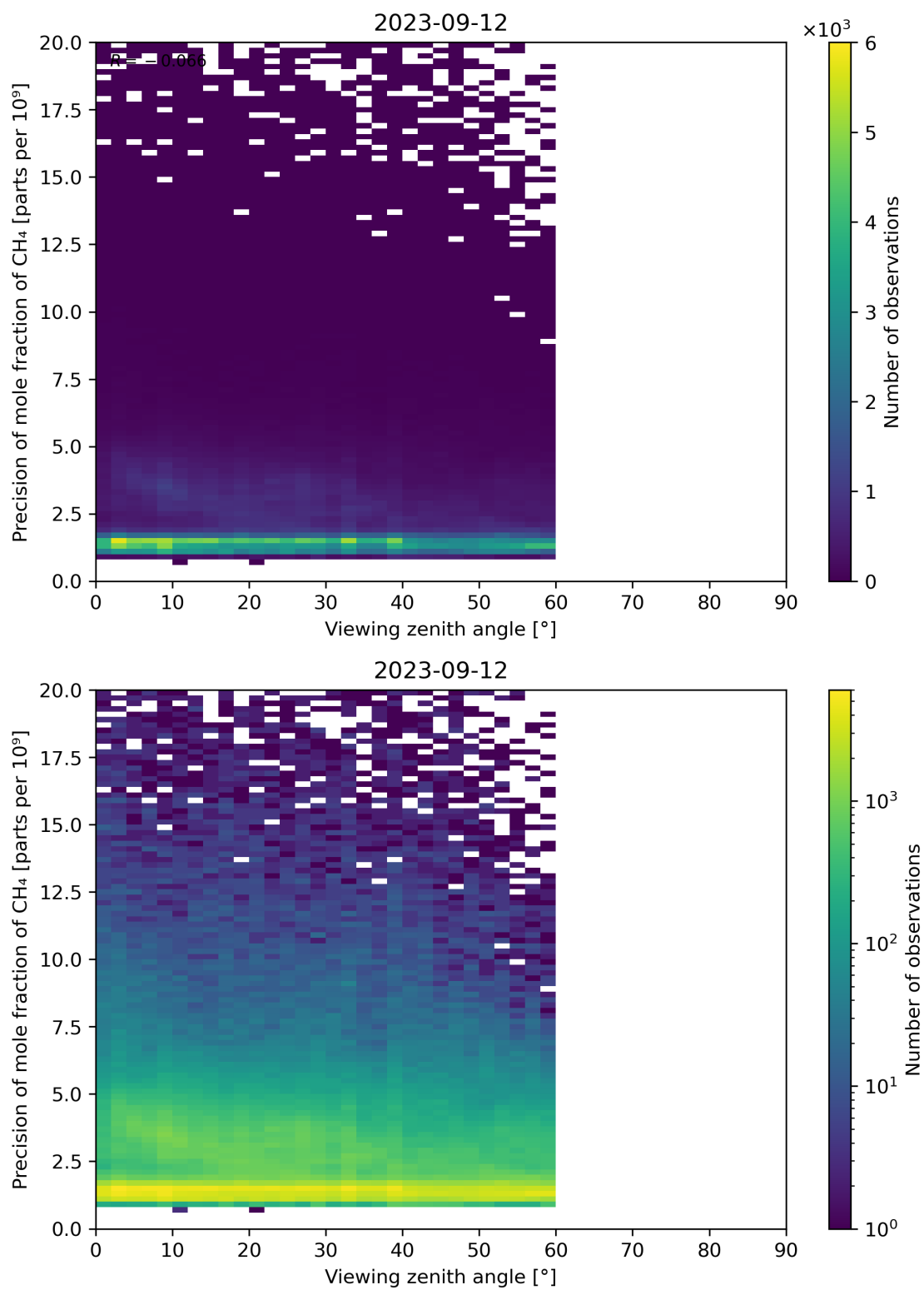
Figure 112: Scatter density plot of “Viewing zenith angle” against “Precision of mole fraction of CH 4 ” for 2023-09-11 to 2023-09-13.
