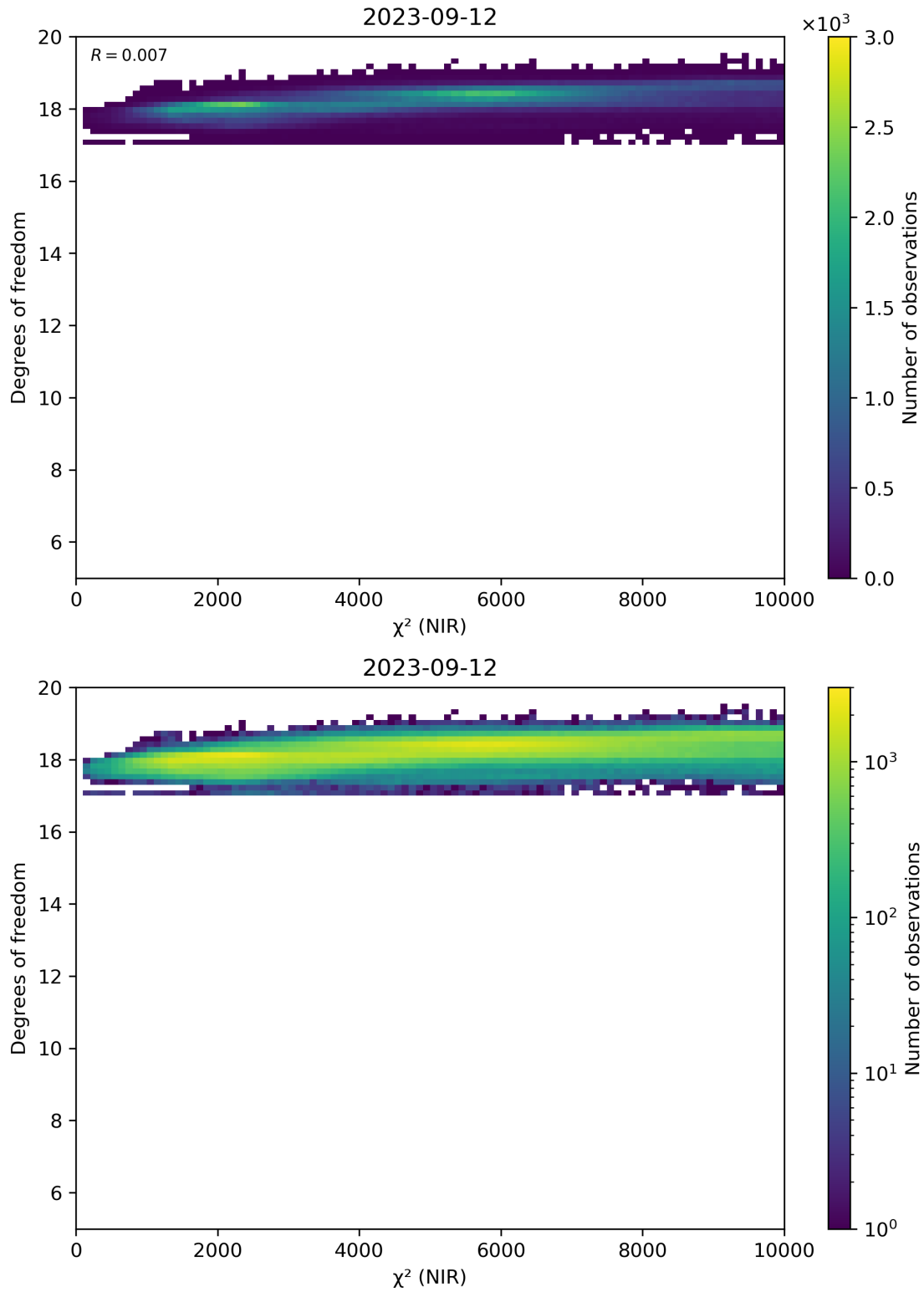
Figure 44: Scatter density plot of “ \chi^2 (NIR)” against “Degrees of freedom” for 2023-09-11 to 2023-09-13.
