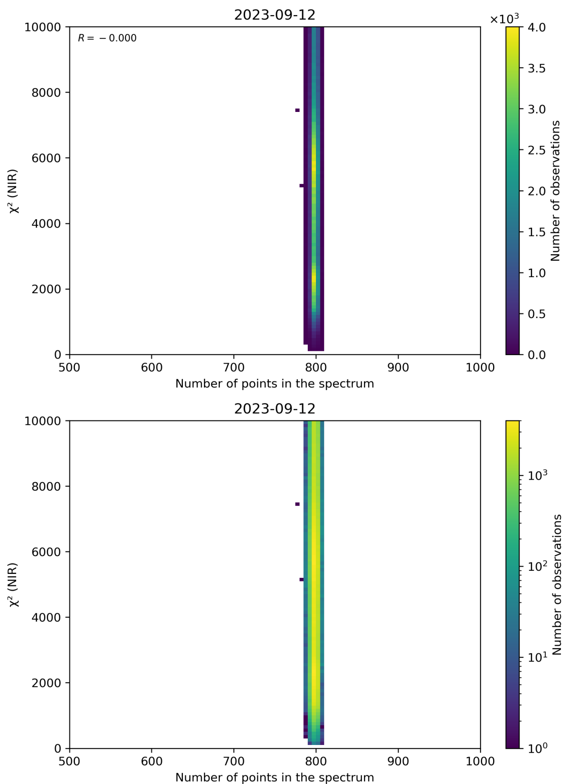
Figure 88: Scatter density plot of “Number of points in the spectrum” against “ \chi^2 (NIR)” for 2023-09-11 to 2023-09-13.
