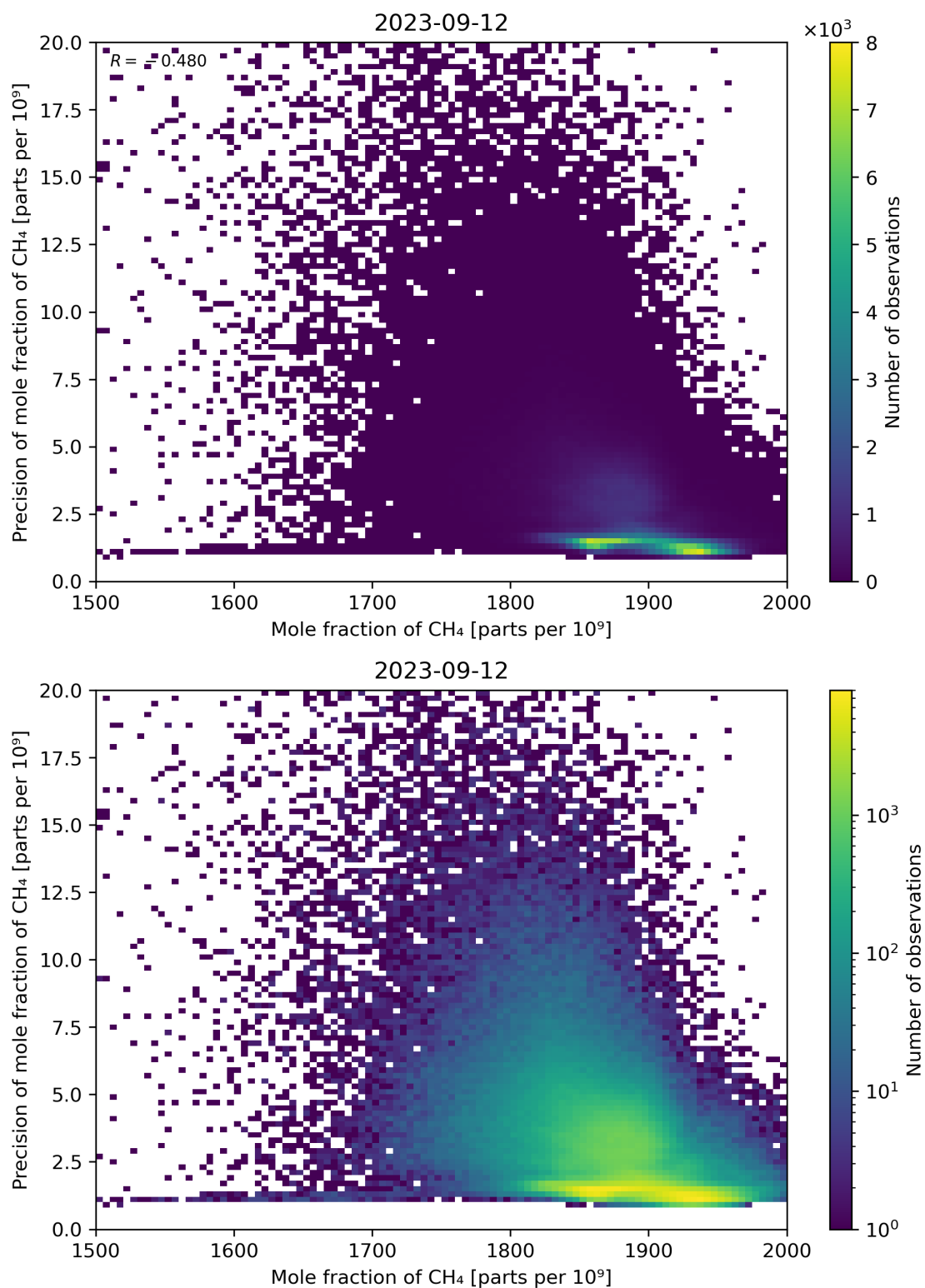
Figure 75: Scatter density plot of “Mole fraction of CH 4 ” against “Precision of mole fraction of CH 4 ” for 2023-09-11 to 2023-09-13.
