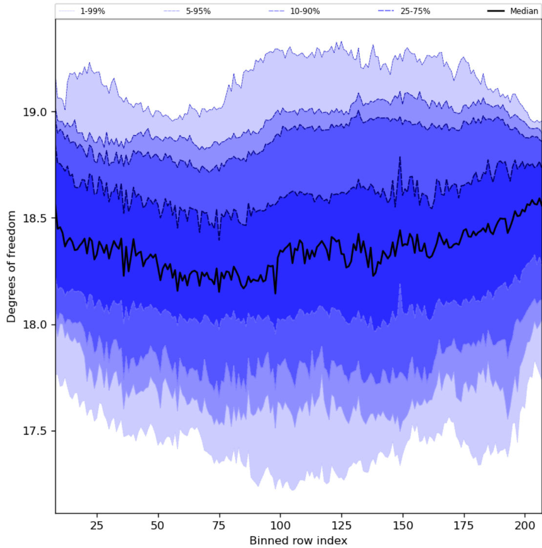
Figure 41: Along track statistics of “Degrees of freedom” for 2023-09-11 to 2023-09-13
