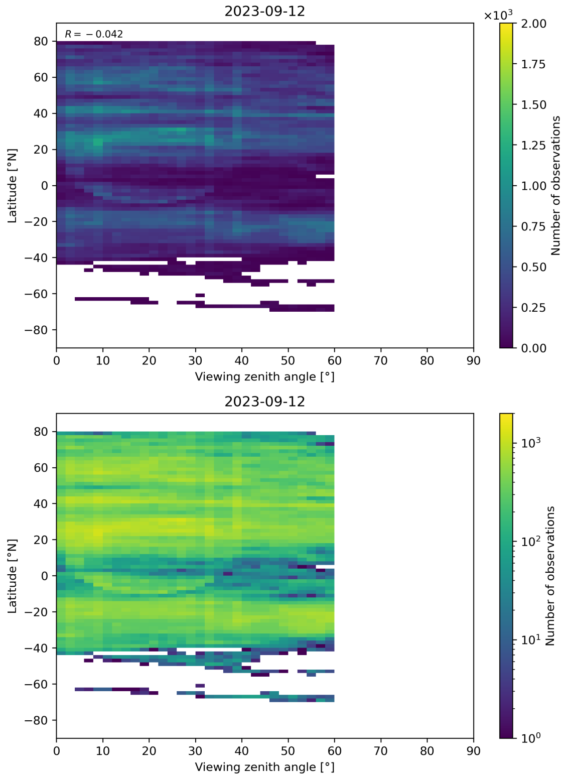
Figure 109: Scatter density plot of “Viewing zenith angle” against “Latitude” for 2023-09-11 to 2023-09-13.
