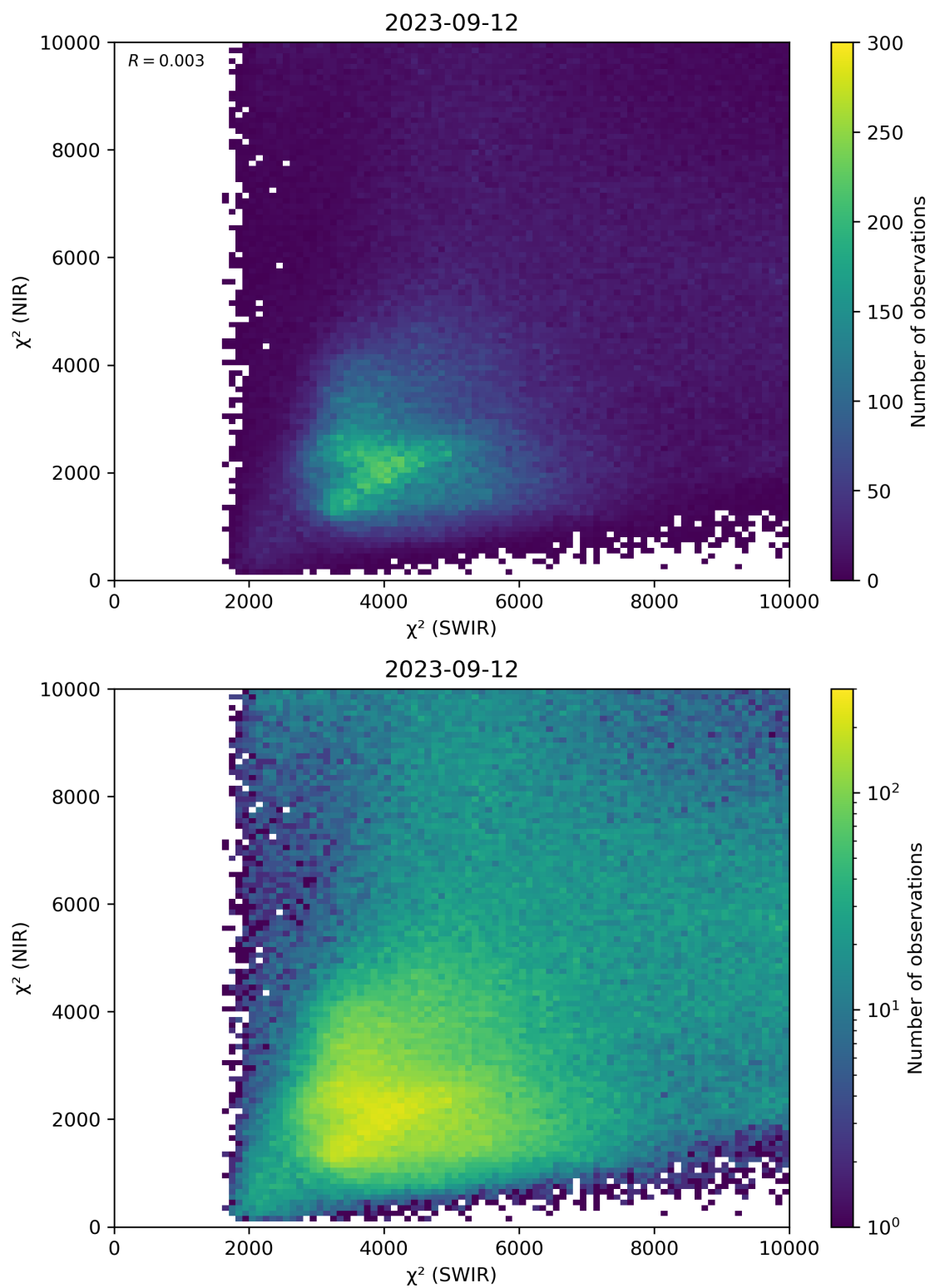
Figure 47: Scatter density plot of “ \chi^2 (SWIR)” against “ \chi^2 (NIR)” for 2023-09-11 to 2023-09-13.
