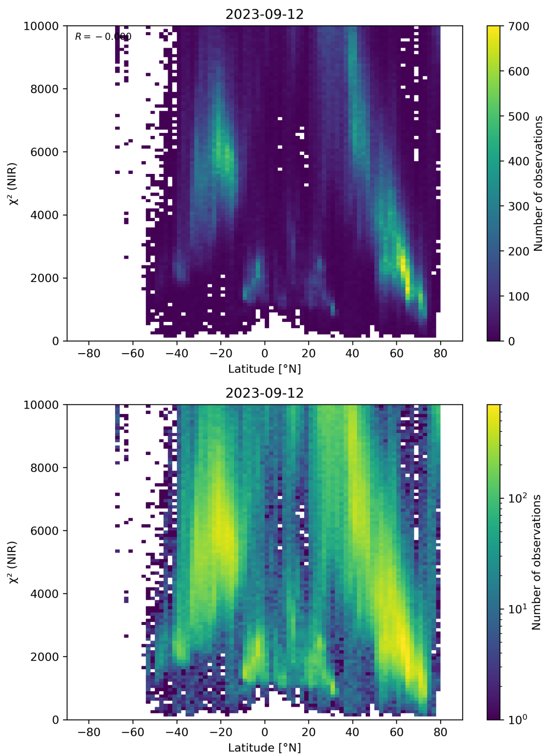
Figure 53: Scatter density plot of “Latitude” against “ \chi^2 (NIR)” for 2023-09-11 to 2023-09-13.
