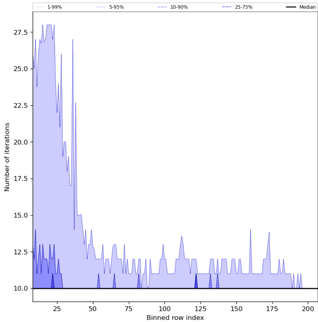
Figure 42: Along track statistics of “Number of iterations” for 2023-09-11 to 2023-09-13
