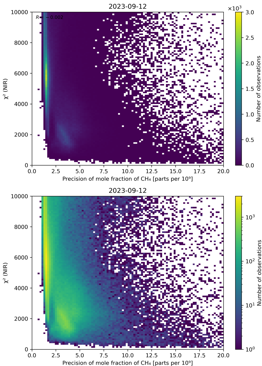
Figure 78: Scatter density plot of “Precision of mole fraction of CH 4 ” against “ \chi^2 (NIR)” for 2023-09-11 to 2023-09-13.
