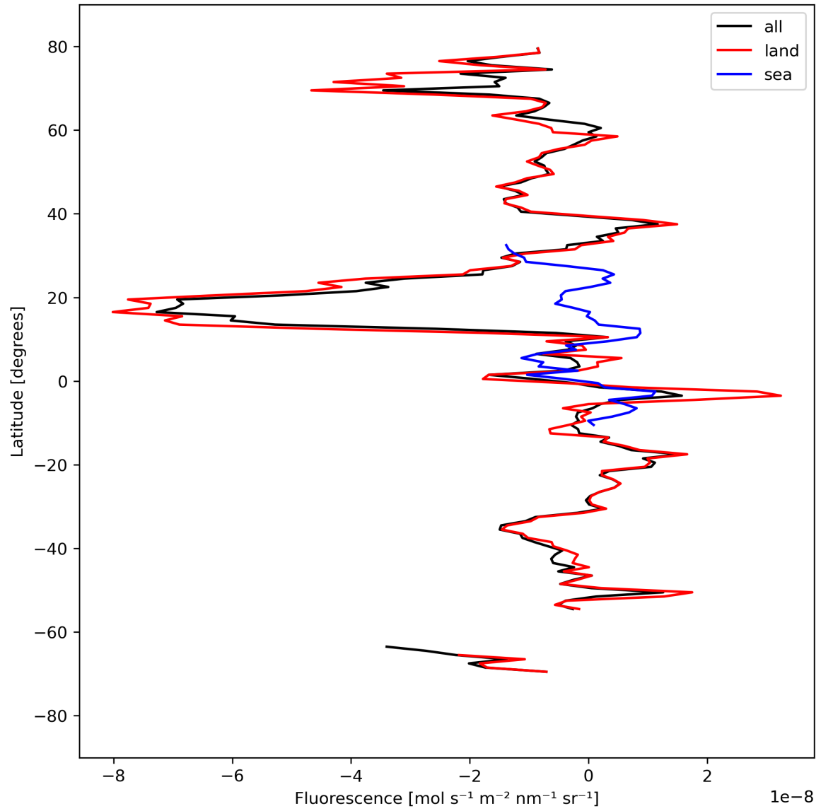
Figure 21: Zonal average of “Fluorescence” for 2023-09-11 to 2023-09-13.
