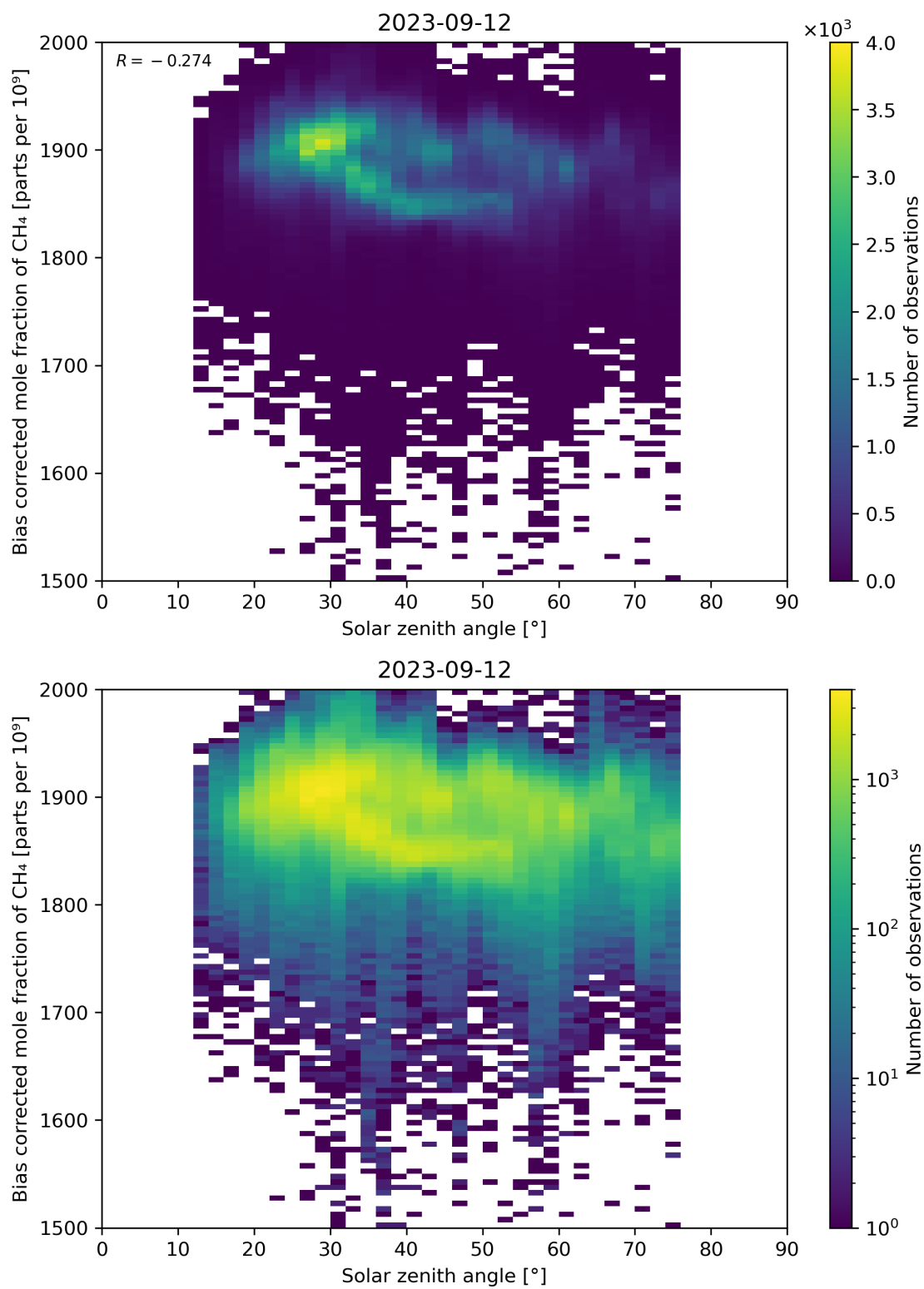
Figure 100: Scatter density plot of “Solar zenith angle” against “Bias corrected mole fraction of CH 4 ” for 2023-09-11 to 2023-09-13.
