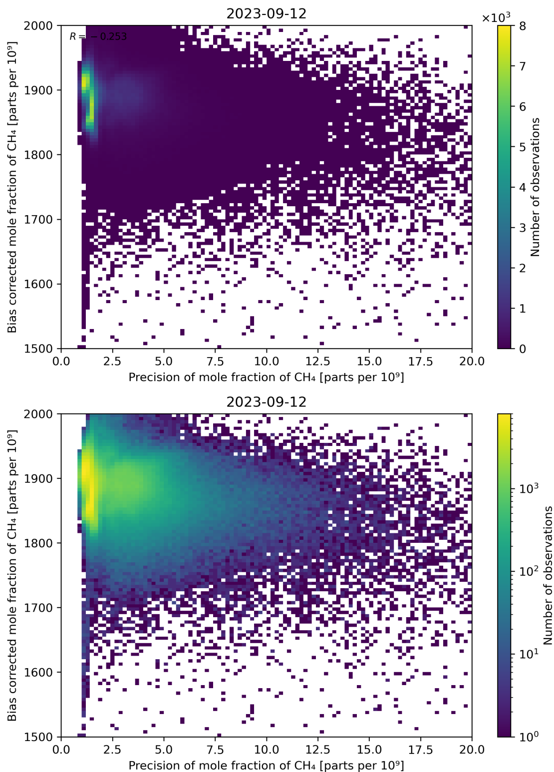
Figure 82: Scatter density plot of “Precision of mole fraction of CH 4 ” against “Bias corrected mole fraction of CH 4 ” for 2023-09-11 to 2023-09-13.
