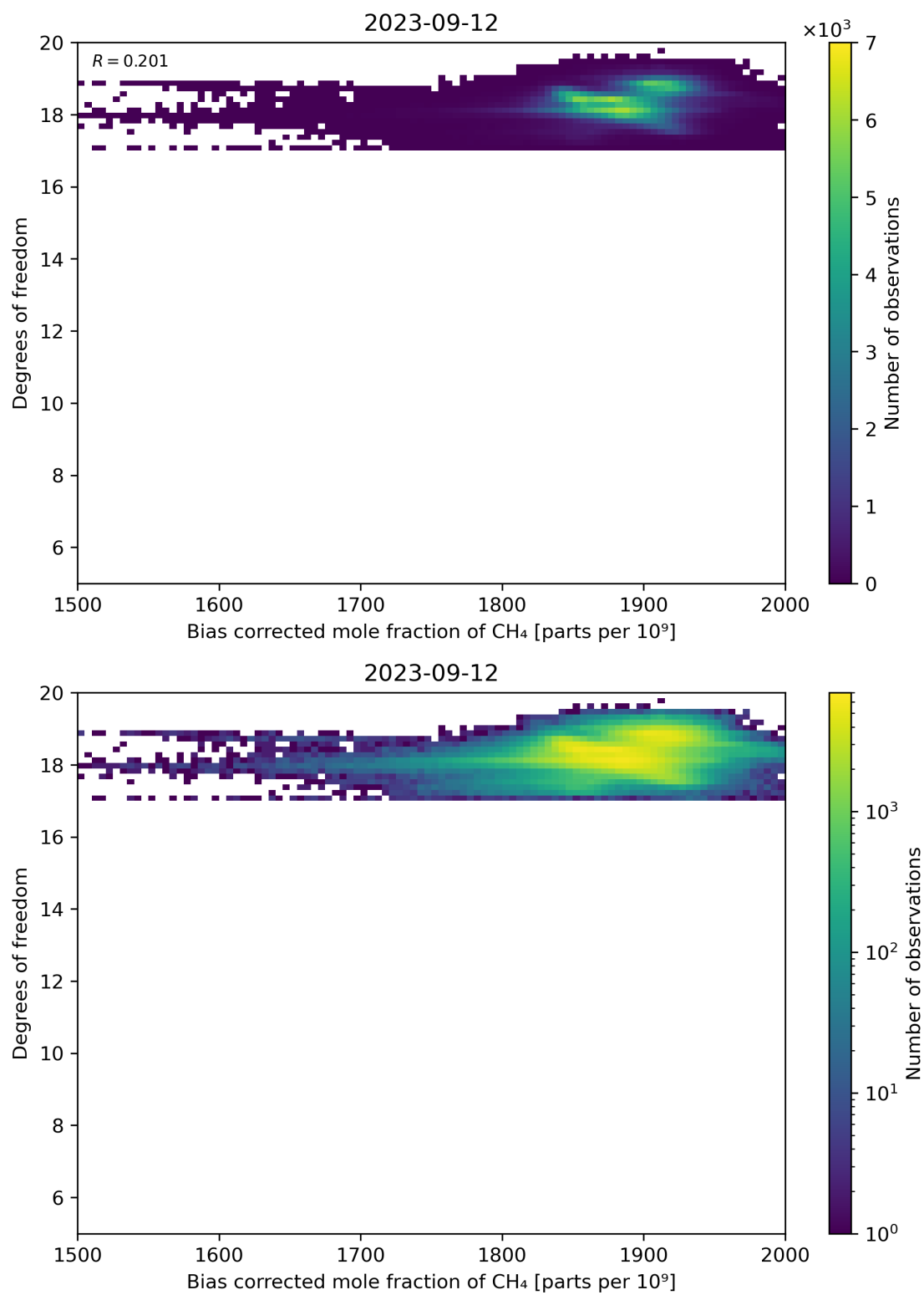
Figure 65: Scatter density plot of “Bias corrected mole fraction of CH 4 ” against “Degrees of freedom” for 2023-09-11 to 2023-09-13.
