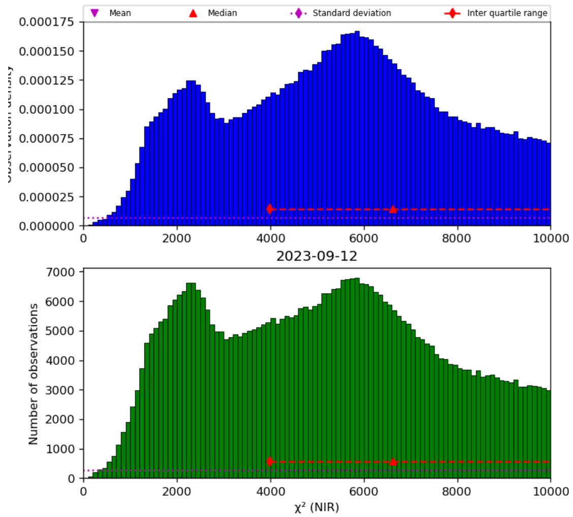
Figure 29: Histogram of “ \chi^2 (NIR)” for 2023-09-11 to 2023-09-13
