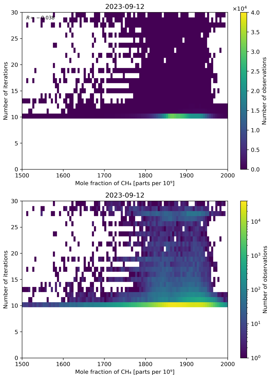
Figure 76: Scatter density plot of “Mole fraction of CH 4 ” against “Number of iterations” for 2023-09-11 to 2023-09-13.
