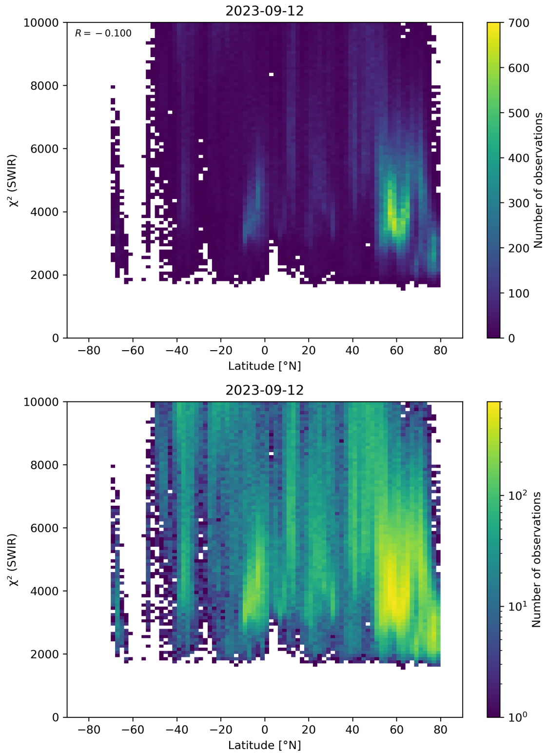
Figure 54: Scatter density plot of “Latitude” against “ \chi^2 (SWIR)” for 2023-09-11 to 2023-09-13.
