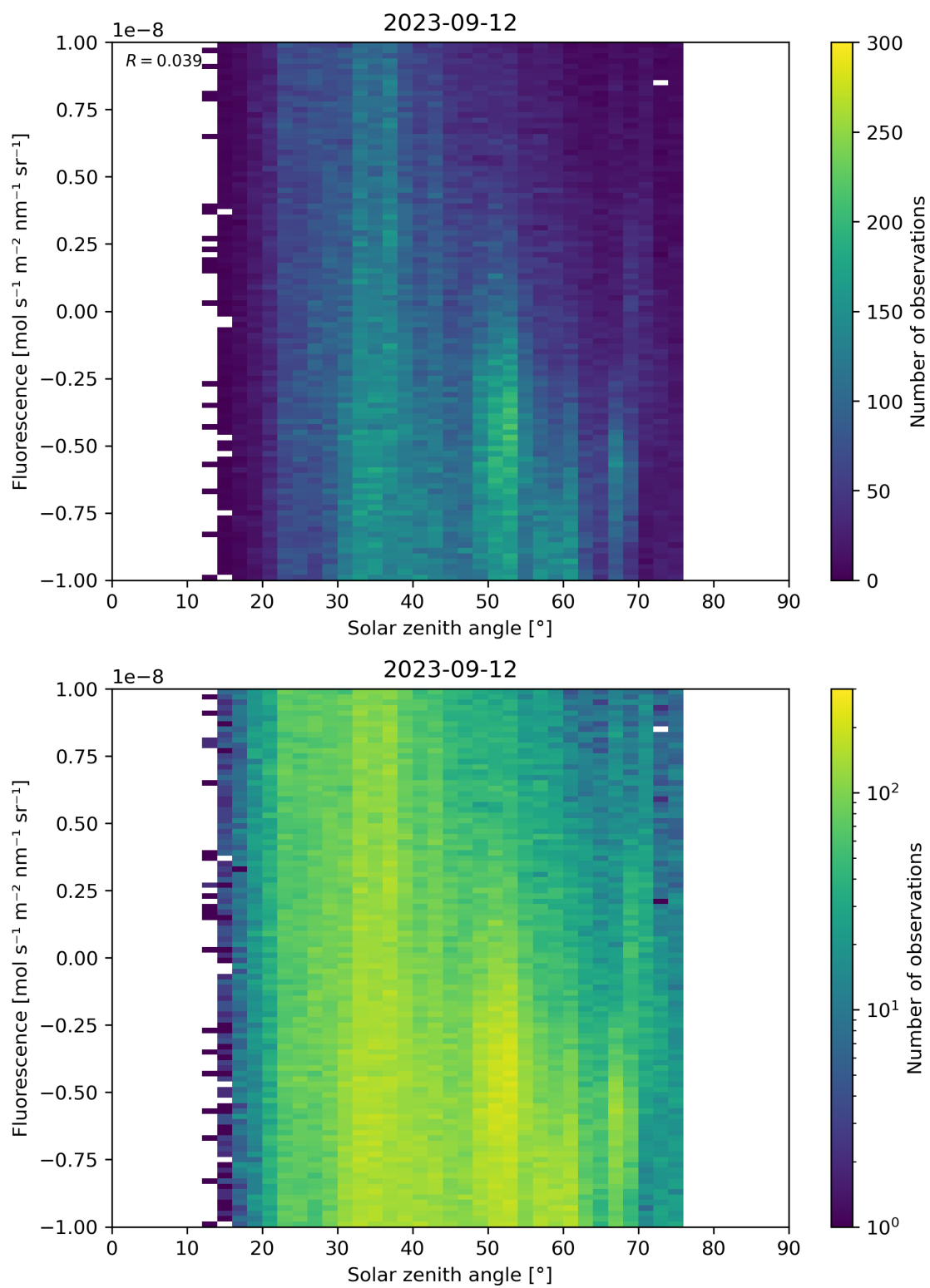
Figure 97: Scatter density plot of “Solar zenith angle” against “Fluorescence” for 2023-09-11 to 2023-09-13.
