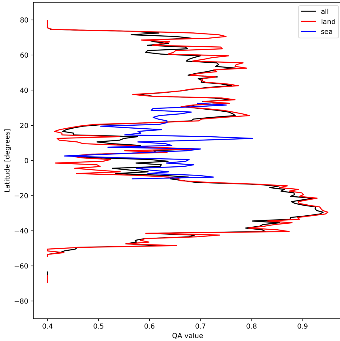
Figure 11: Zonal average of “QA value” for 2023-09-11 to 2023-09-13.
