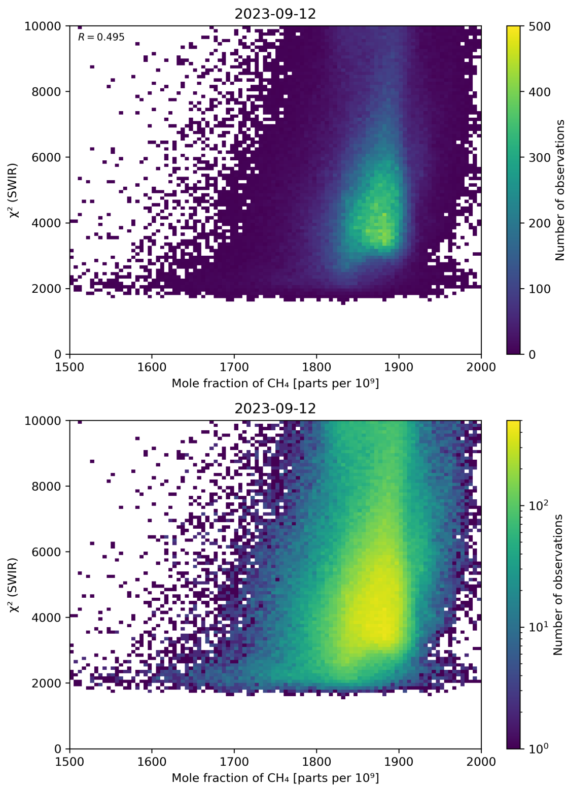
Figure 71: Scatter density plot of “Mole fraction of \text{CH}_4 ” against “ \chi^2 (SWIR)” for 2023-09-11 to 2023-09-13.
