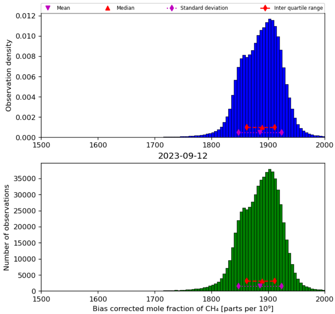
Figure 25: Histogram of “Bias corrected mole fraction of CH 4 ” for 2023-09-11 to 2023-09-13
