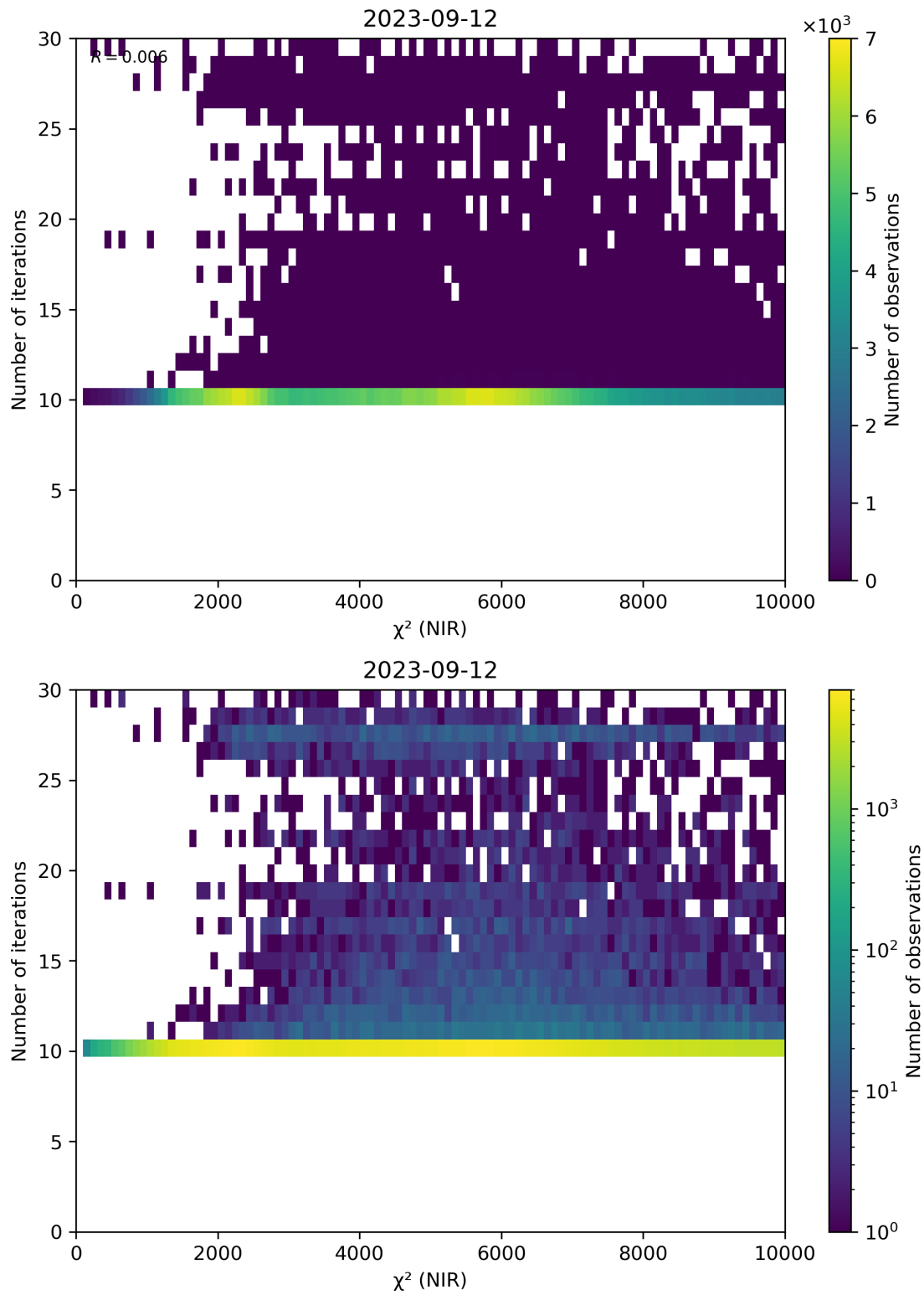
Figure 46: Scatter density plot of “ \chi^2 (NIR)” against “Number of iterations” for 2023-09-11 to 2023-09-13.
