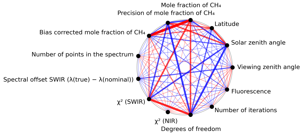
Figure 1: Map of correlation graph for 2023-09-11 to 2023-09-13.
