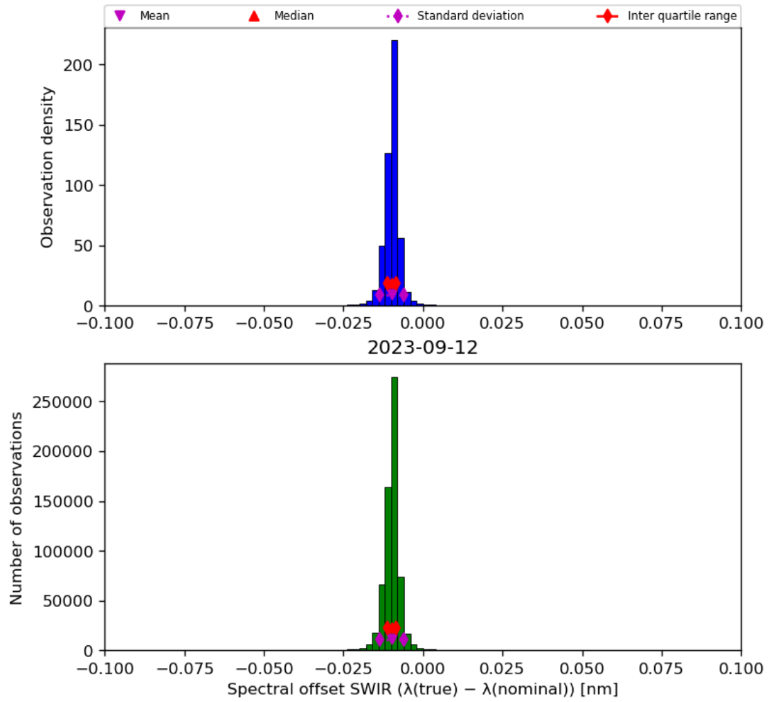
Figure 27: Histogram of “Spectral offset SWIR ( \lambda(\text{true}) - \lambda(\text{nominal}) )” for 2023-09-11 to 2023-09-13
