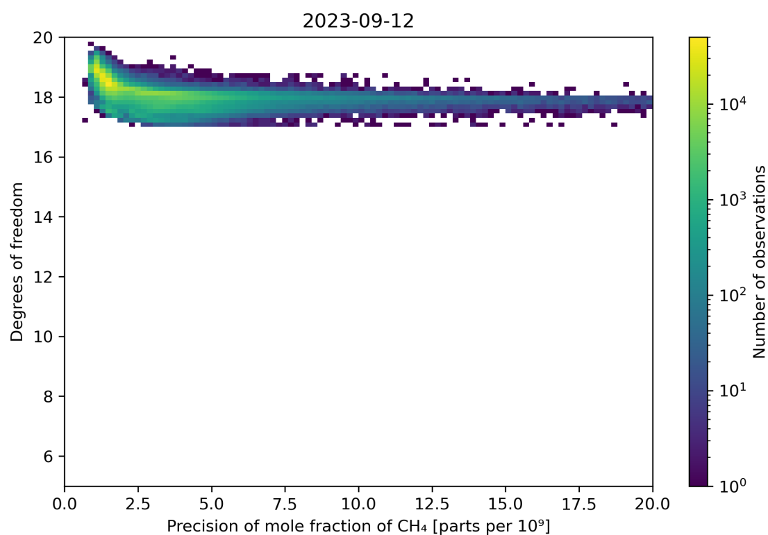
Figure 80: Scatter density plot of “Precision of mole fraction of CH 4 ” against “Degrees of freedom” for 2023-09-11 to 2023-09-13.
