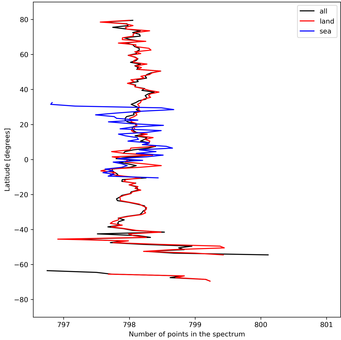
Figure 15: Zonal average of “Number of points in the spectrum” for 2023-09-11 to 2023-09-13.
