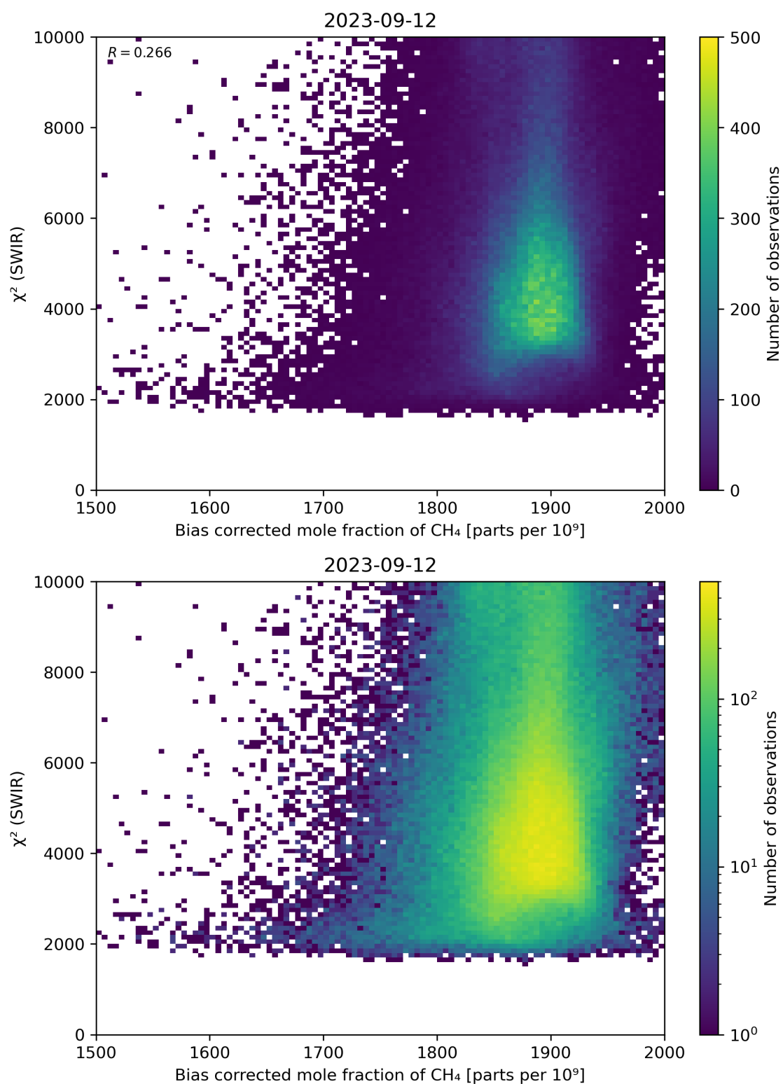
Figure 64: Scatter density plot of “Bias corrected mole fraction of CH 4 ” against “ \chi^2 (SWIR)” for 2023-09-11 to 2023-09-13.
