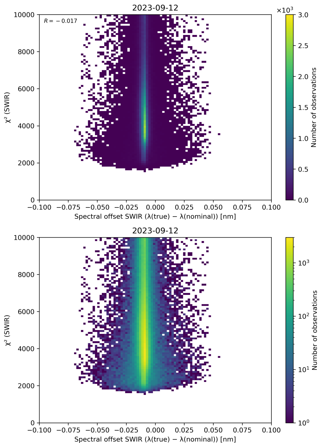
Figure 118: Scatter density plot of “Spectral offset SWIR ( \lambda(\text{true}) - \lambda(\text{nominal}) )” against “ \chi^2 (SWIR)” for 2023-09-11 to 2023-09-13.
