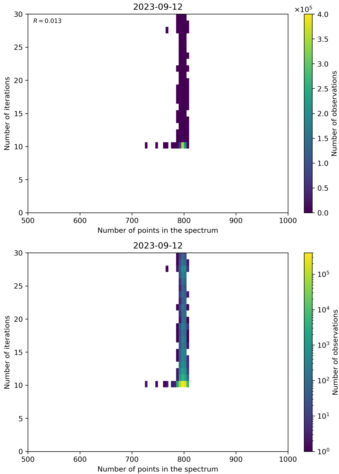
Figure 92: Scatter density plot of “Number of points in the spectrum” against “Number of iterations” for 2023-09-11 to 2023-09-13.
