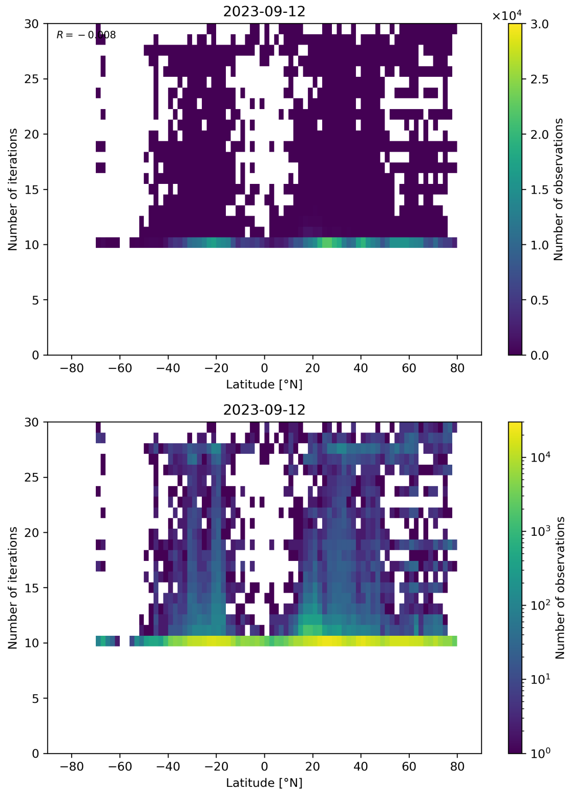
Figure 60: Scatter density plot of “Latitude” against “Number of iterations” for 2023-09-11 to 2023-09-13.
