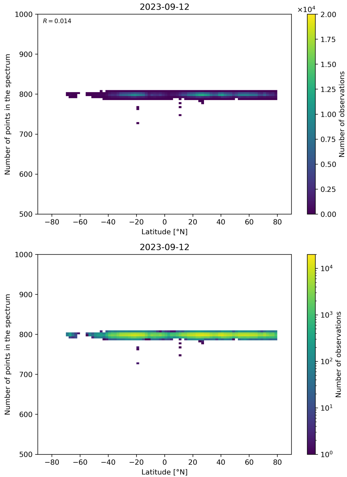
Figure 61: Scatter density plot of “Latitude” against “Number of points in the spectrum” for 2023-09-11 to 2023-09-13.
