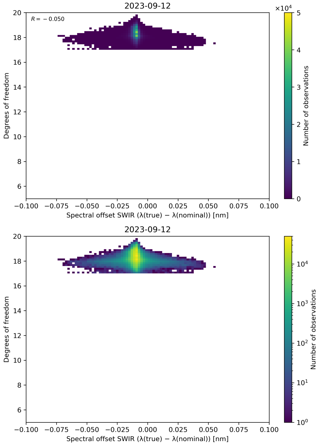
Figure 119: Scatter density plot of “Spectral offset SWIR ( \lambda(\text{true}) - \lambda(\text{nominal}) )” against “Degrees of freedom” for 2023-09-11 to 2023-09-13.
