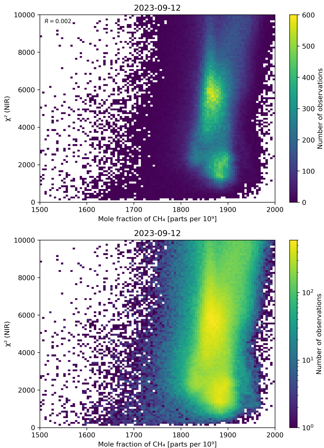
Figure 70: Scatter density plot of “Mole fraction of CH 4 ” against “ \chi^2 (NIR)” for 2023-09-11 to 2023-09-13.
