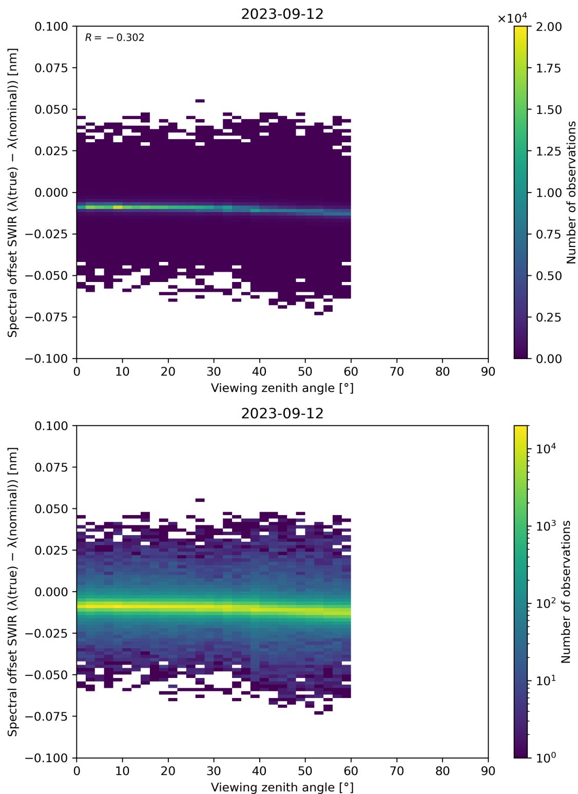
Figure 116: Scatter density plot of “Viewing zenith angle” against “Spectral offset SWIR ( \lambda(\text{true}) - \lambda(\text{nominal}) )” for 2023-09-11 to 2023-09-13.
