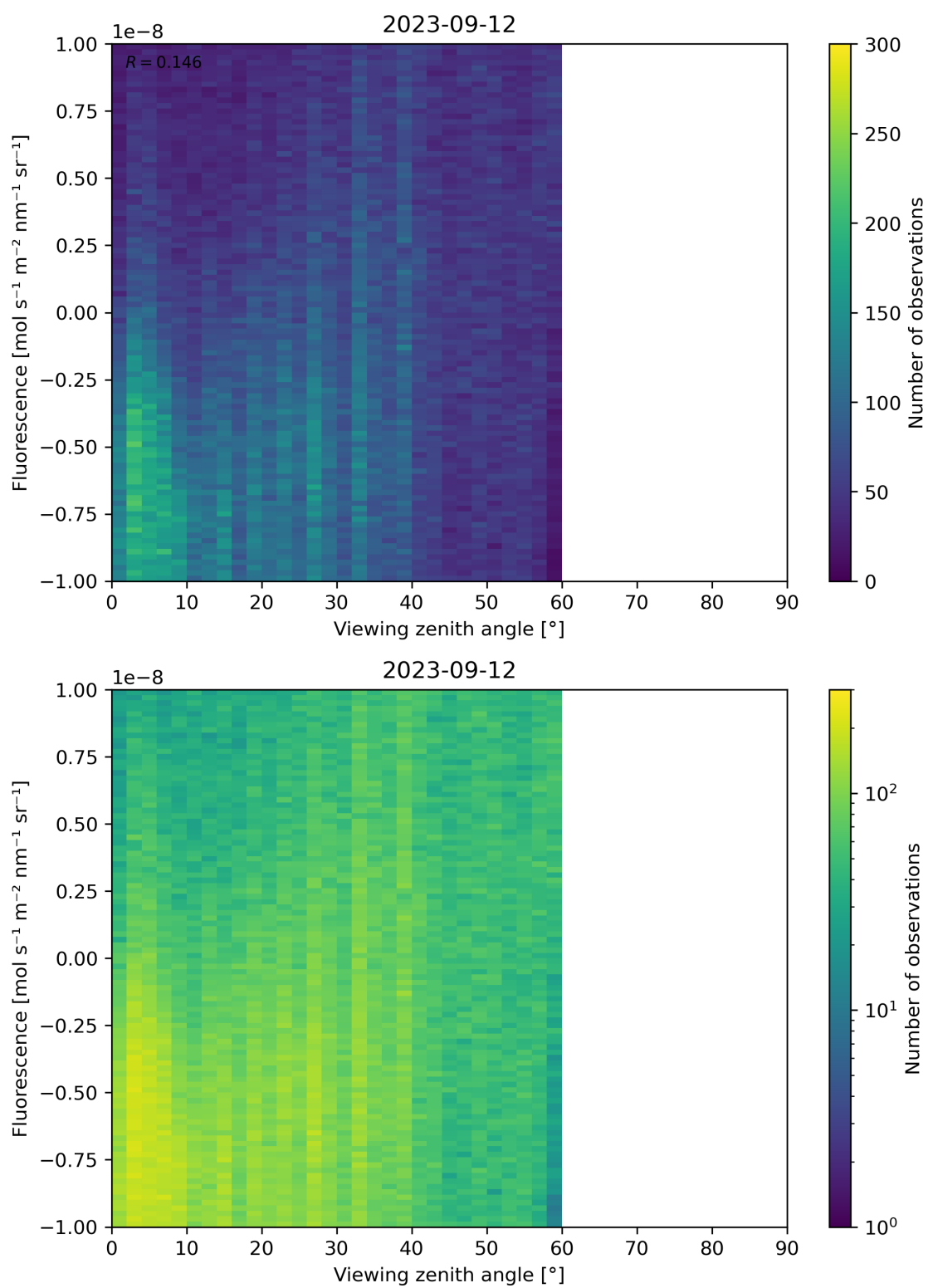
Figure 108: Scatter density plot of “Viewing zenith angle” against “Fluorescence” for 2023-09-11 to 2023-09-13.
