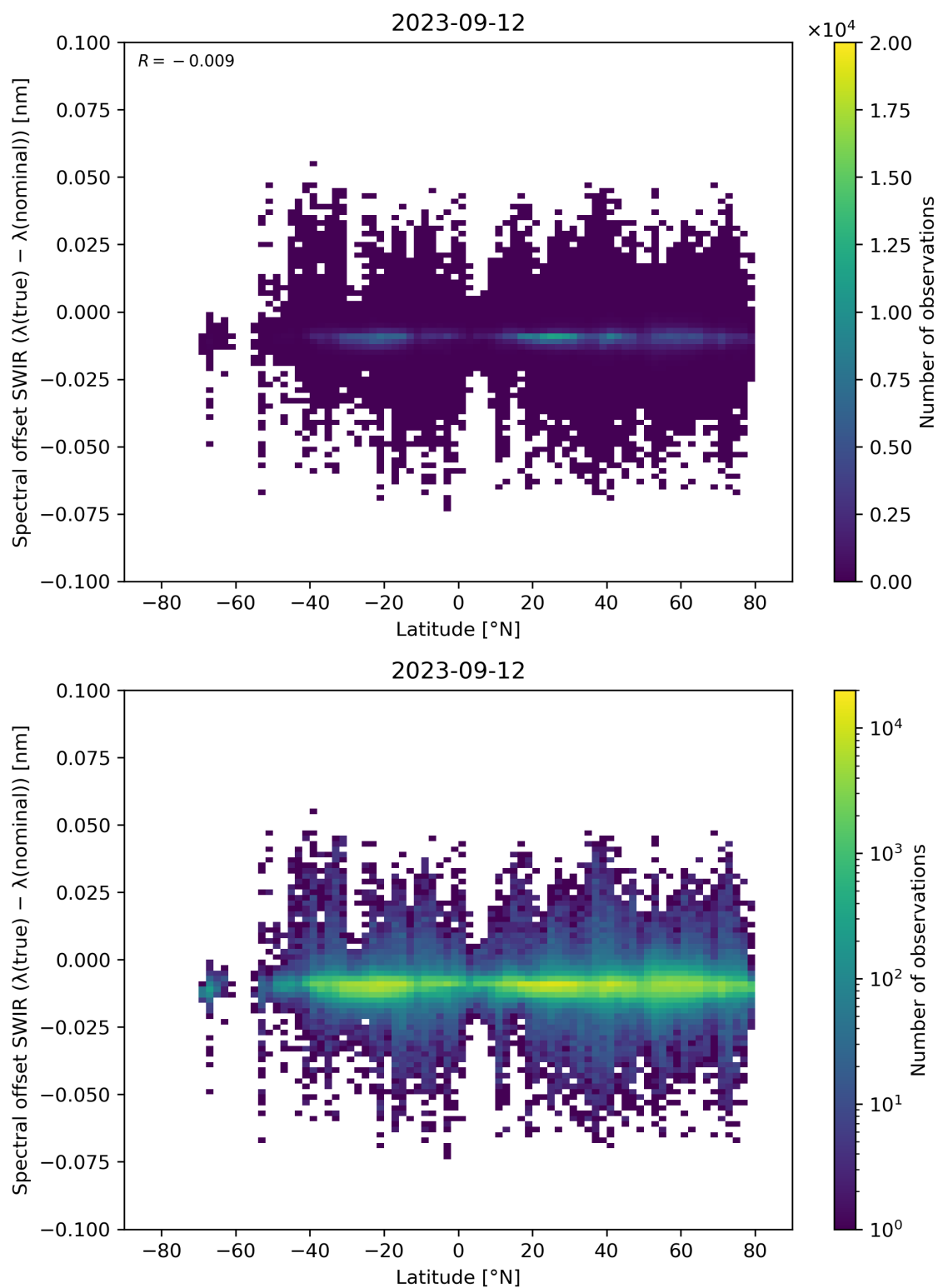
Figure 62: Scatter density plot of “Latitude” against “Spectral offset SWIR ( \lambda(\text{true}) - \lambda(\text{nominal}) )” for 2023-09-11 to 2023-09-13.
