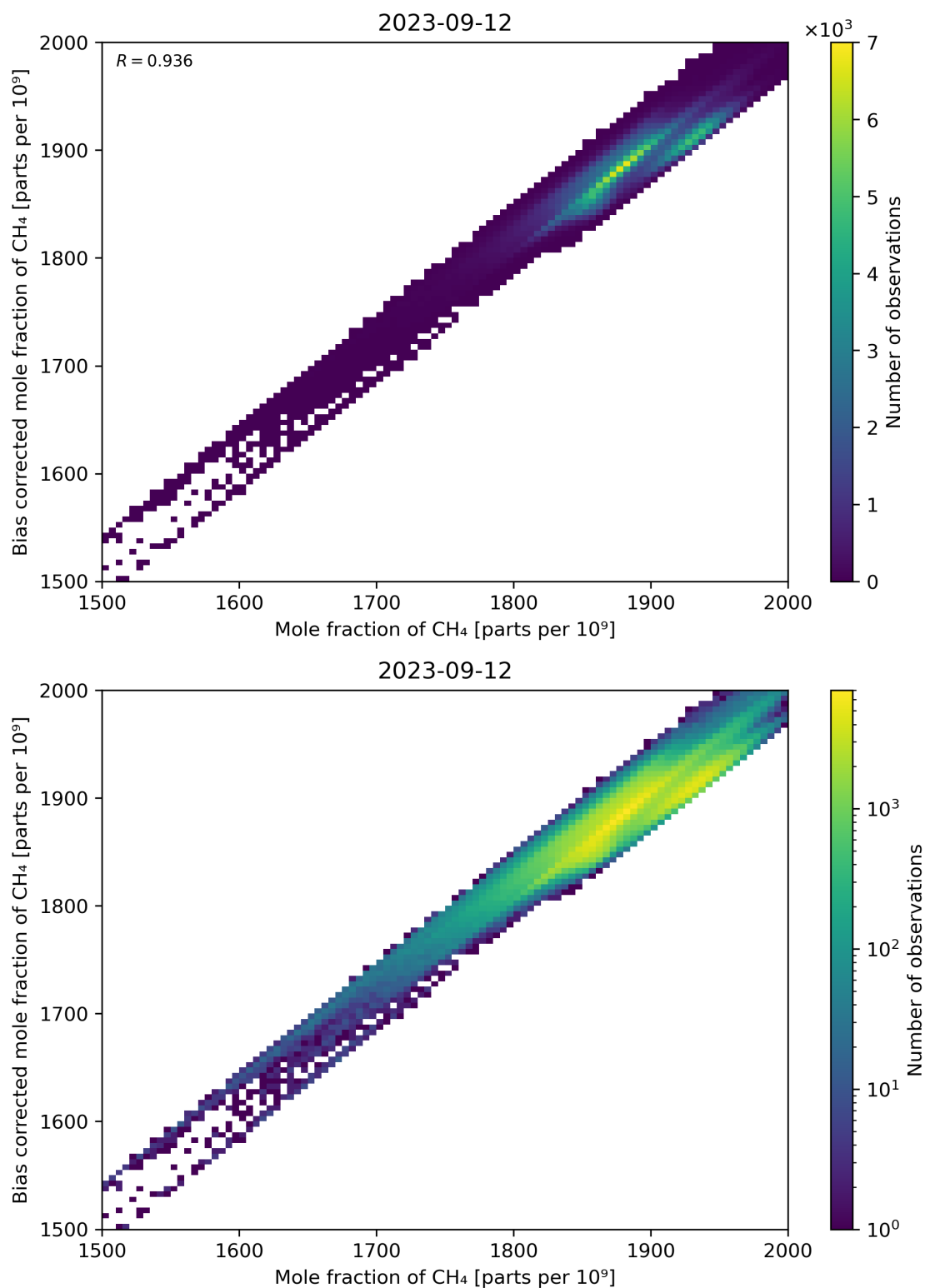
Figure 74: Scatter density plot of “Mole fraction of CH 4 ” against “Bias corrected mole fraction of CH 4 ” for 2023-09-11 to 2023-09-13.
