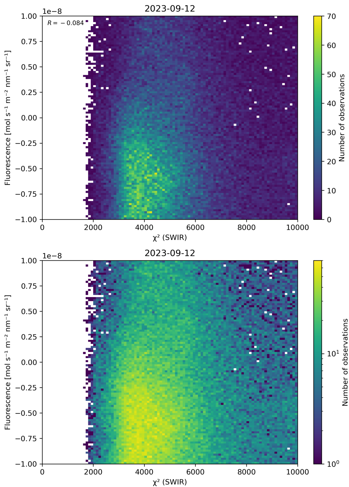
Figure 49: Scatter density plot of “ \chi^2 (SWIR)” against “Fluorescence” for 2023-09-11 to 2023-09-13.
