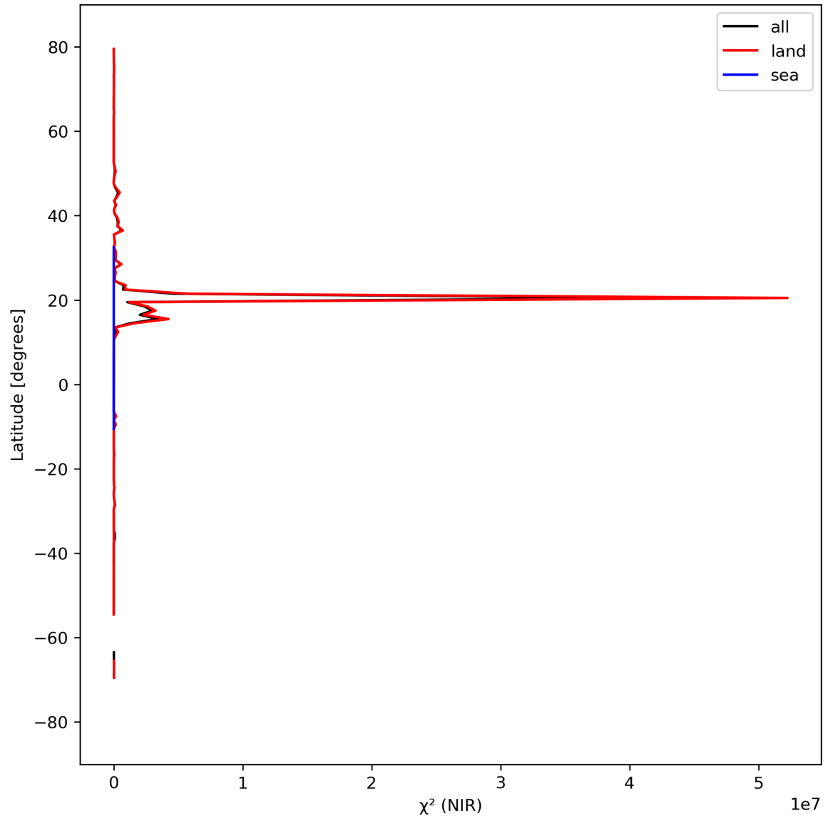
Figure 18: Zonal average of “ \chi^2 (NIR)” for 2023-09-11 to 2023-09-13.
