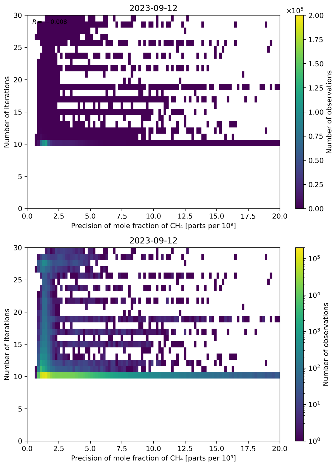
Figure 83: Scatter density plot of “Precision of mole fraction of CH 4 ” against “Number of iterations” for 2023-09-11 to 2023-09-13.
