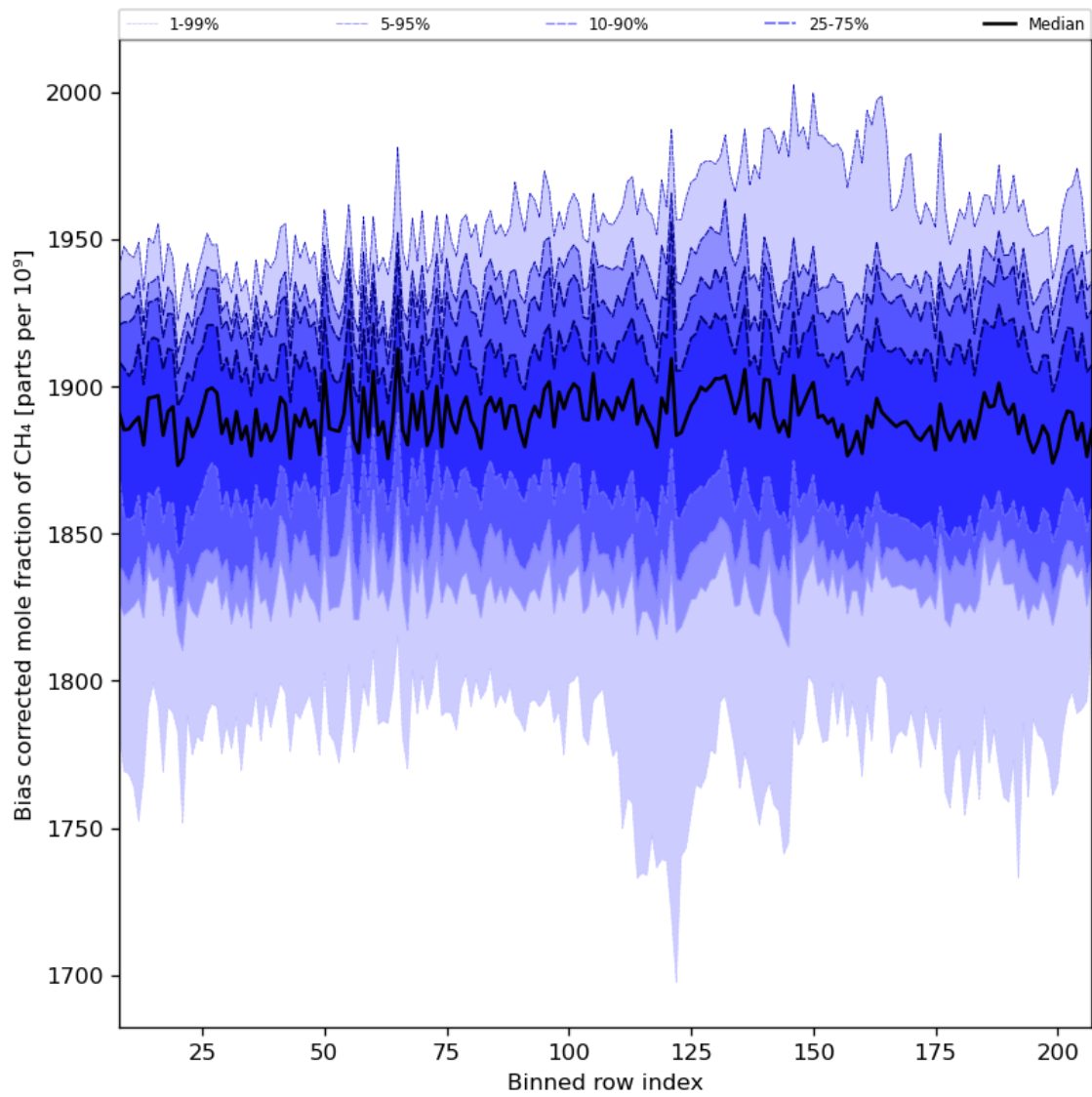
Figure 36: Along track statistics of “Bias corrected mole fraction of CH 4 ” for 2023-09-11 to 2023-09-13
