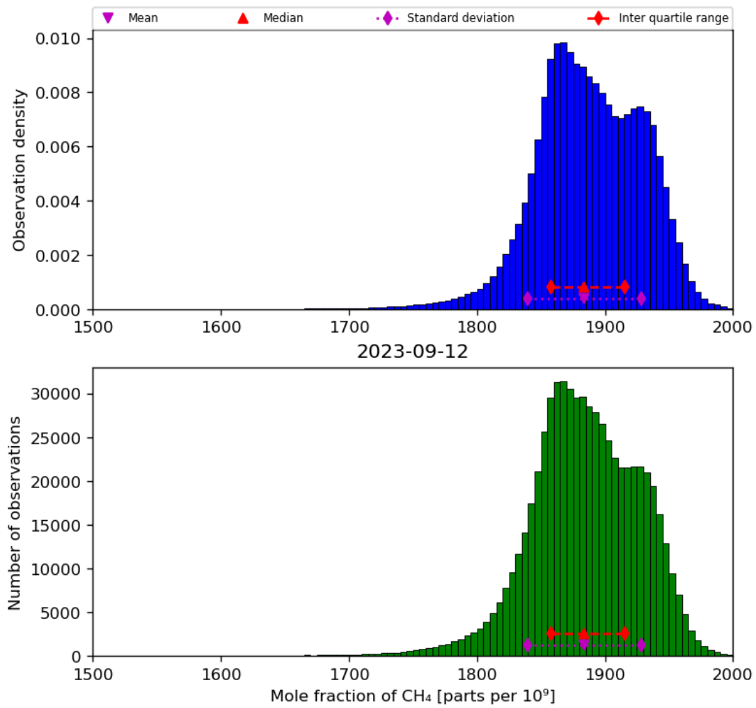
Figure 23: Histogram of “Mole fraction of CH 4 ” for 2023-09-11 to 2023-09-13
