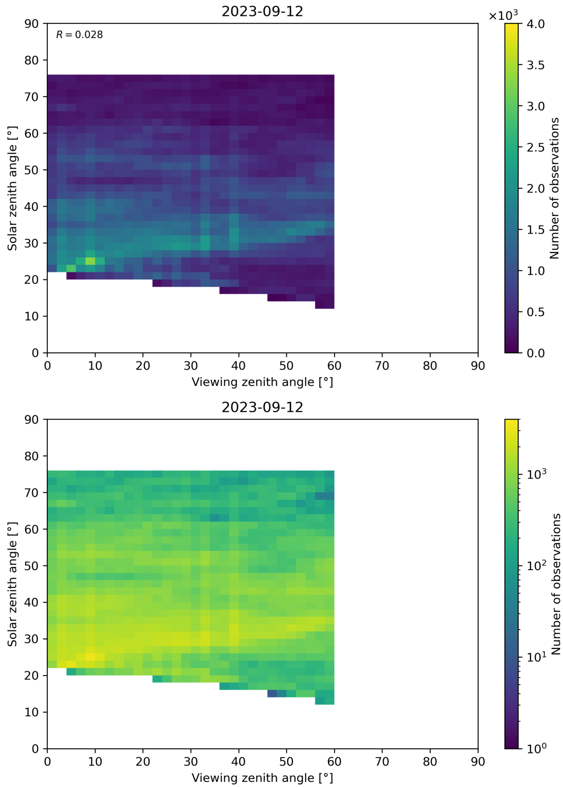
Figure 115: Scatter density plot of “Viewing zenith angle” against “Solar zenith angle” for 2023-09-11 to 2023-09-13.
