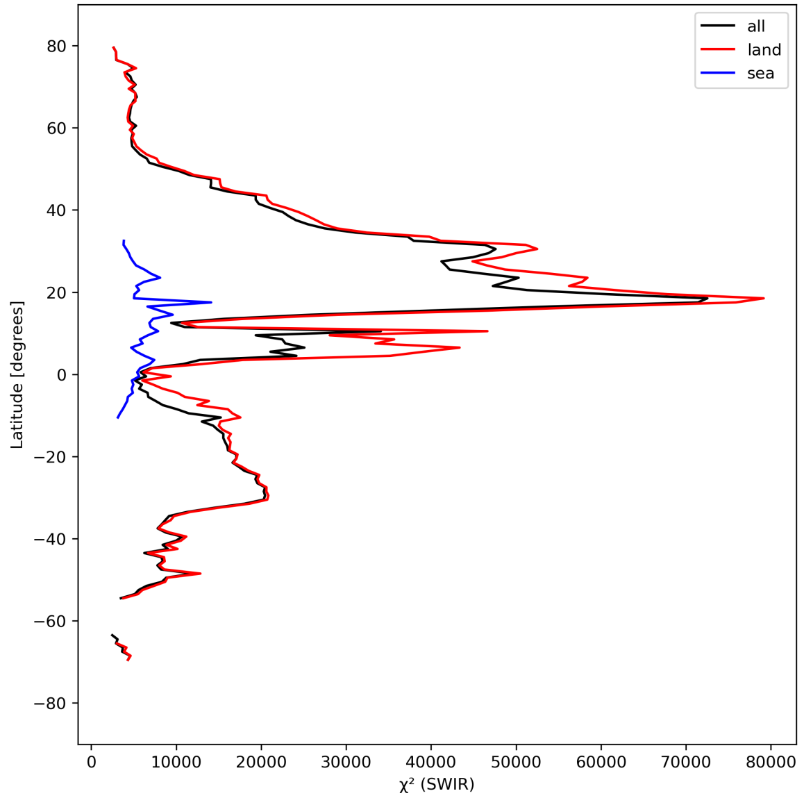
Figure 17: Zonal average of “ \chi^2 (SWIR)” for 2023-09-11 to 2023-09-13.
