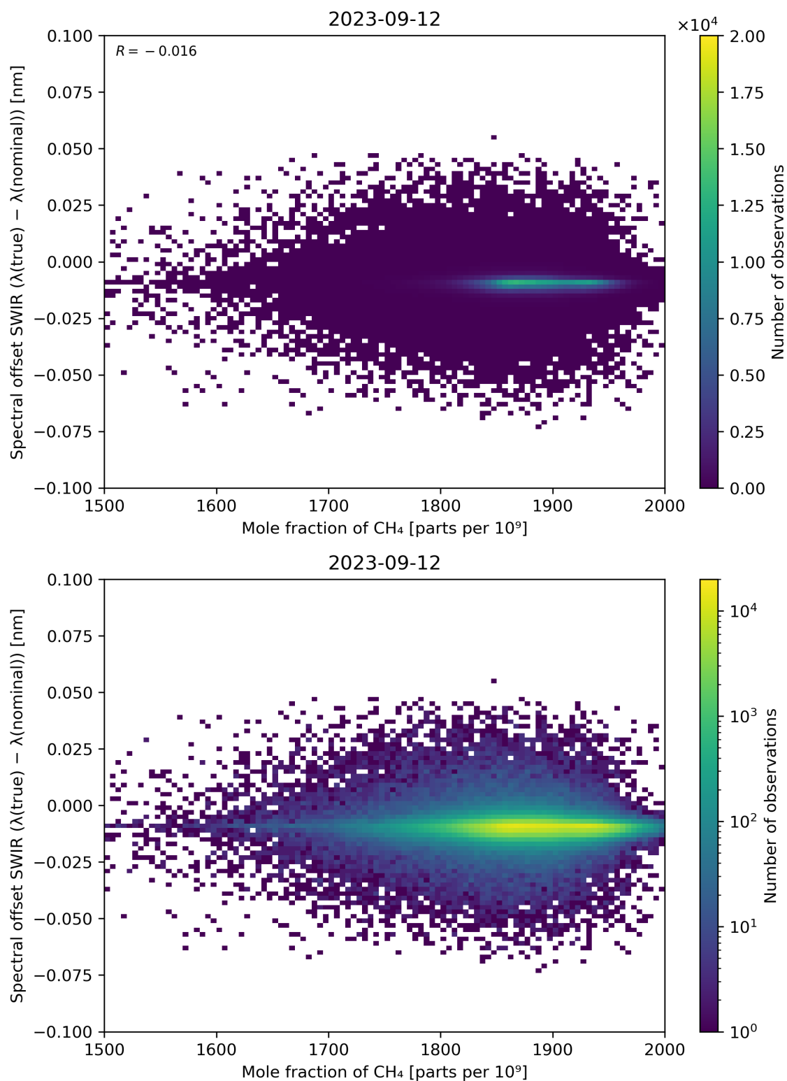
Figure 86: Scatter density plot of “Mole fraction of CH 4 ” against “Spectral offset SWIR ( \lambda(\text{true}) - \lambda(\text{nominal}) )” for 2023-09-11 to 2023-09-13.
