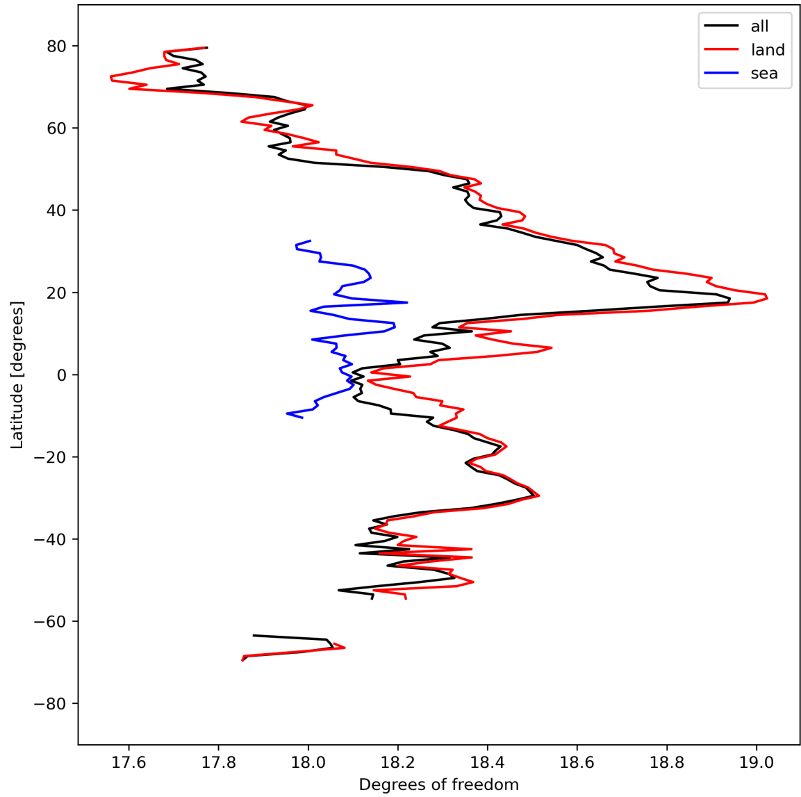
Figure 19: Zonal average of “Degrees of freedom” for 2023-09-11 to 2023-09-13.
