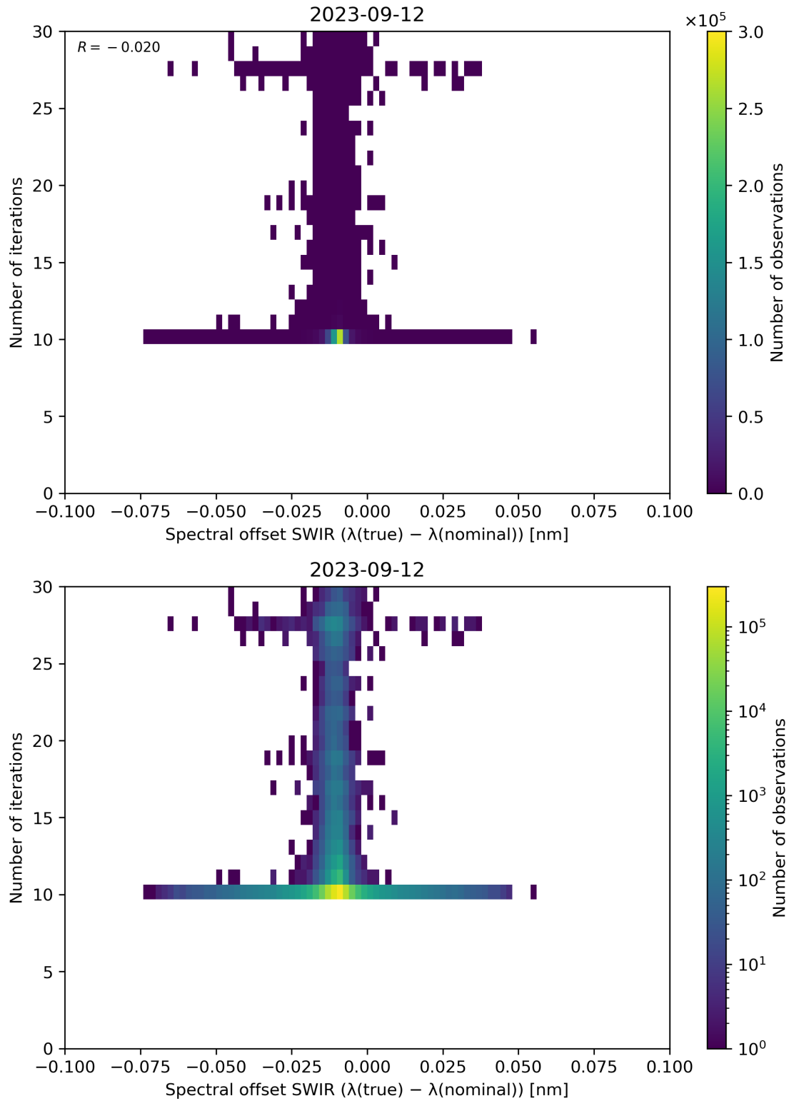
Figure 121: Scatter density plot of “Spectral offset SWIR ( \lambda(\text{true}) - \lambda(\text{nominal}) )” against “Number of iterations” for 2023-09-11 to 2023-09-13.
