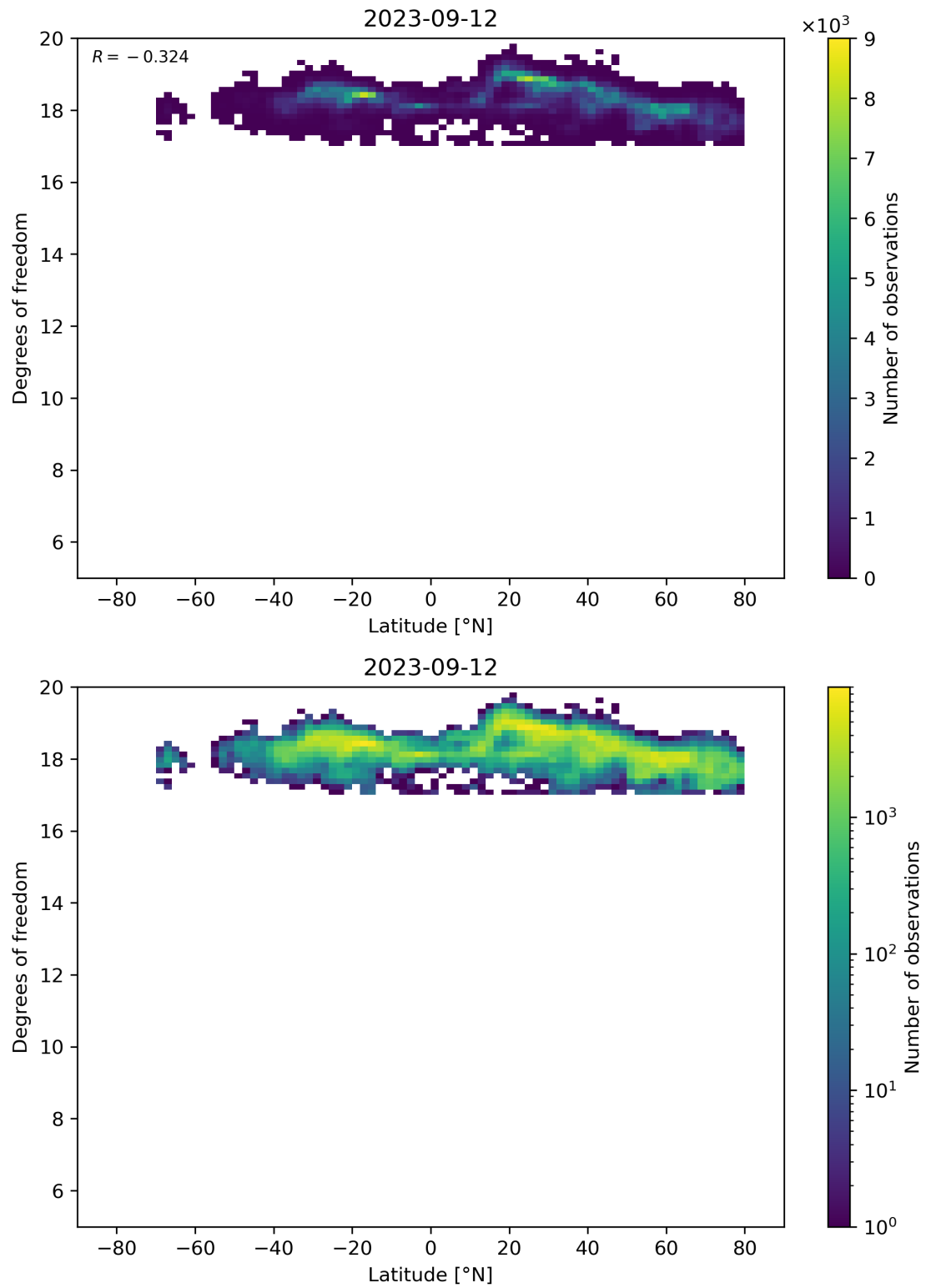
Figure 55: Scatter density plot of “Latitude” against “Degrees of freedom” for 2023-09-11 to 2023-09-13.
