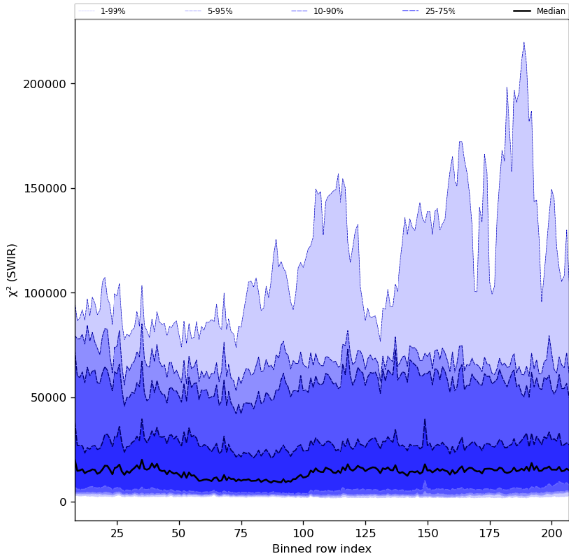
Figure 39: Along track statistics of “ \chi^2 (SWIR)” for 2023-09-11 to 2023-09-13
