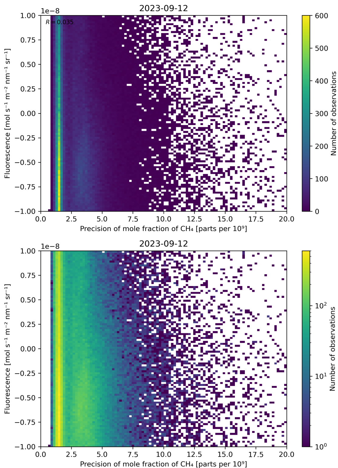
Figure 81: Scatter density plot of “Precision of mole fraction of \text{CH}_4 ” against “Fluorescence” for 2023-09-11 to 2023-09-13.
