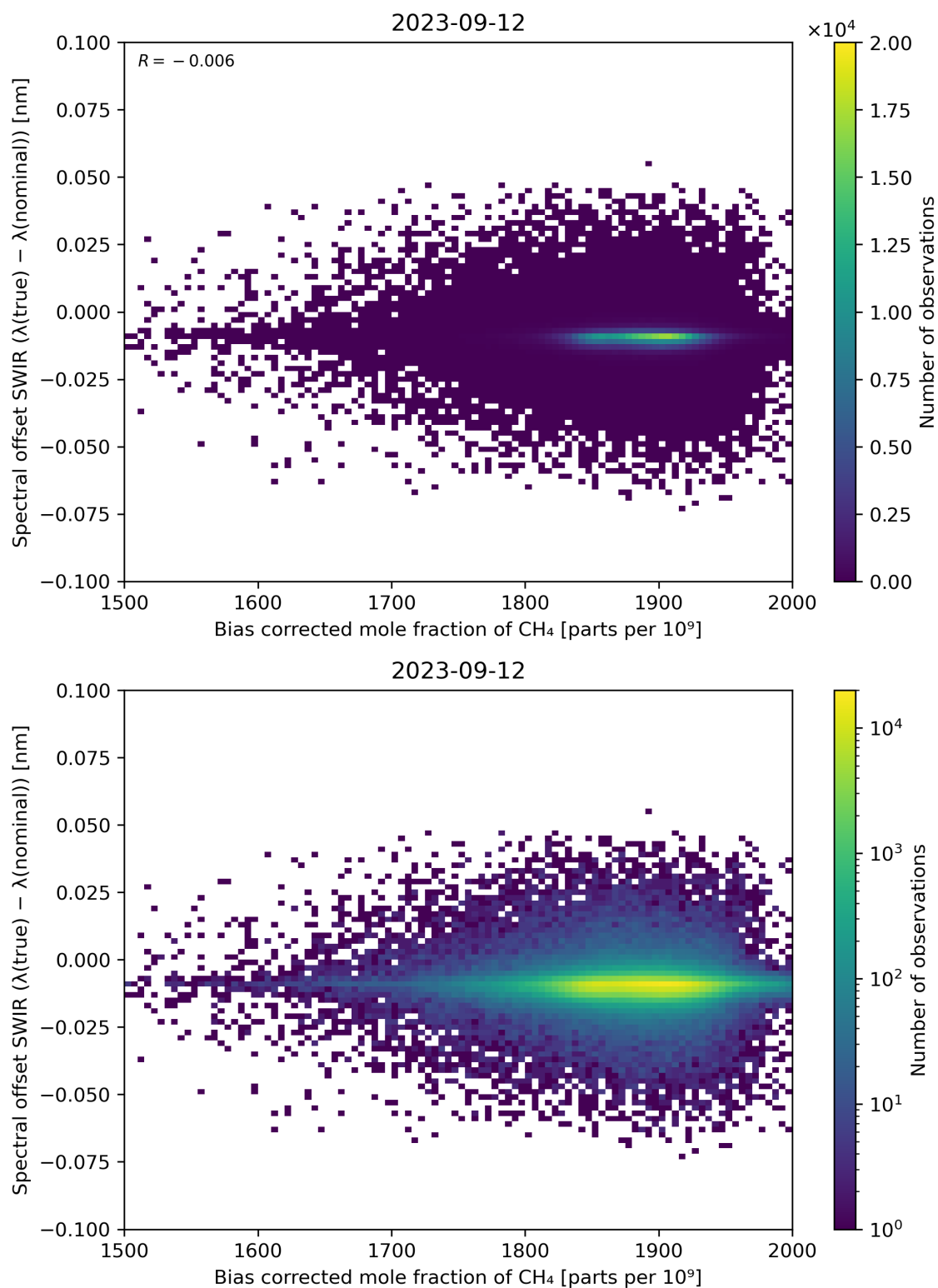
Figure 69: Scatter density plot of “Bias corrected mole fraction of \text{CH}_4 ” against “Spectral offset SWIR ( \lambda(\text{true}) - \lambda(\text{nominal}) )” for 2023-09-11 to 2023-09-13.
