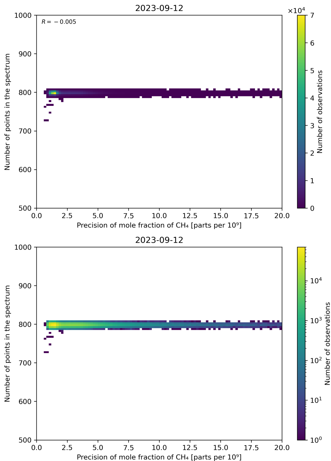
Figure 84: Scatter density plot of “Precision of mole fraction of CH 4 ” against “Number of points in the spectrum” for 2023-09-11 to 2023-09-13.
