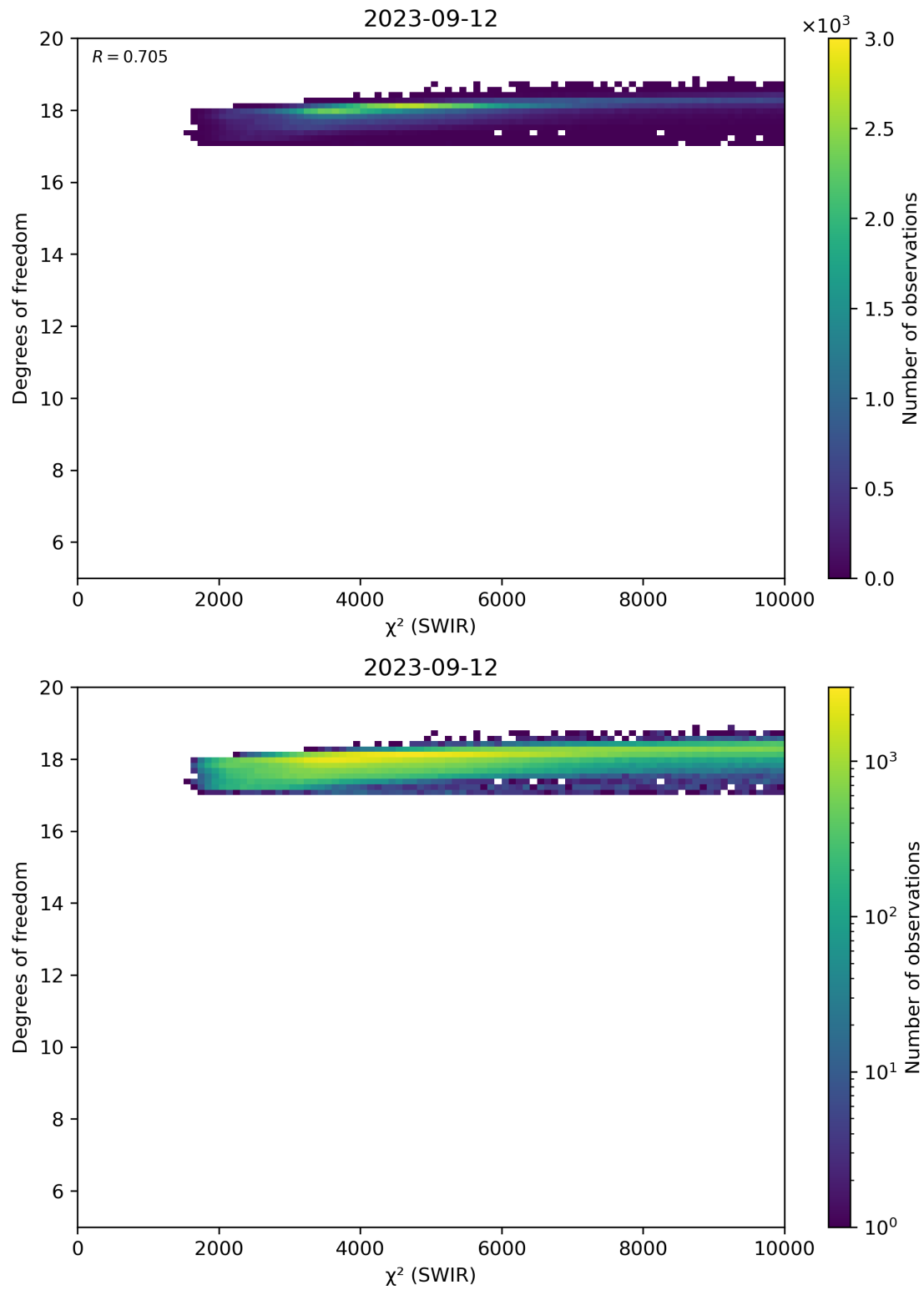
Figure 48: Scatter density plot of “ \chi^2 (SWIR)” against “Degrees of freedom” for 2023-09-11 to 2023-09-13.
