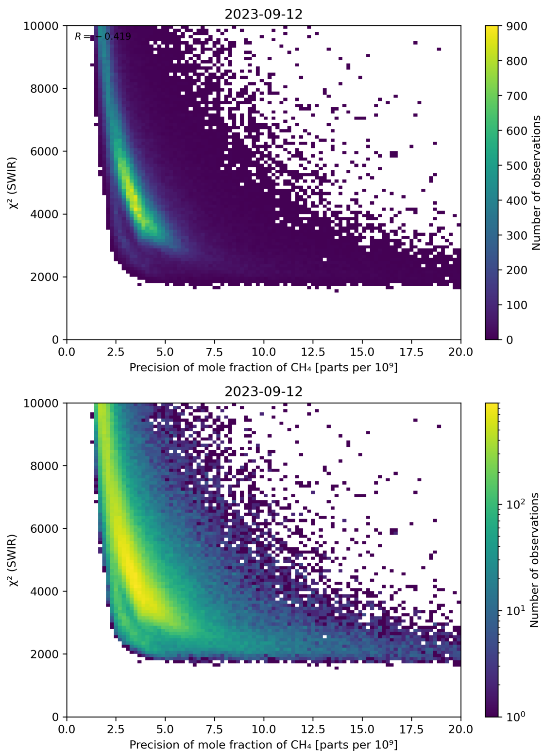
Figure 79: Scatter density plot of “Precision of mole fraction of CH 4 ” against “ \chi^2 (SWIR)” for 2023-09-11 to 2023-09-13.
