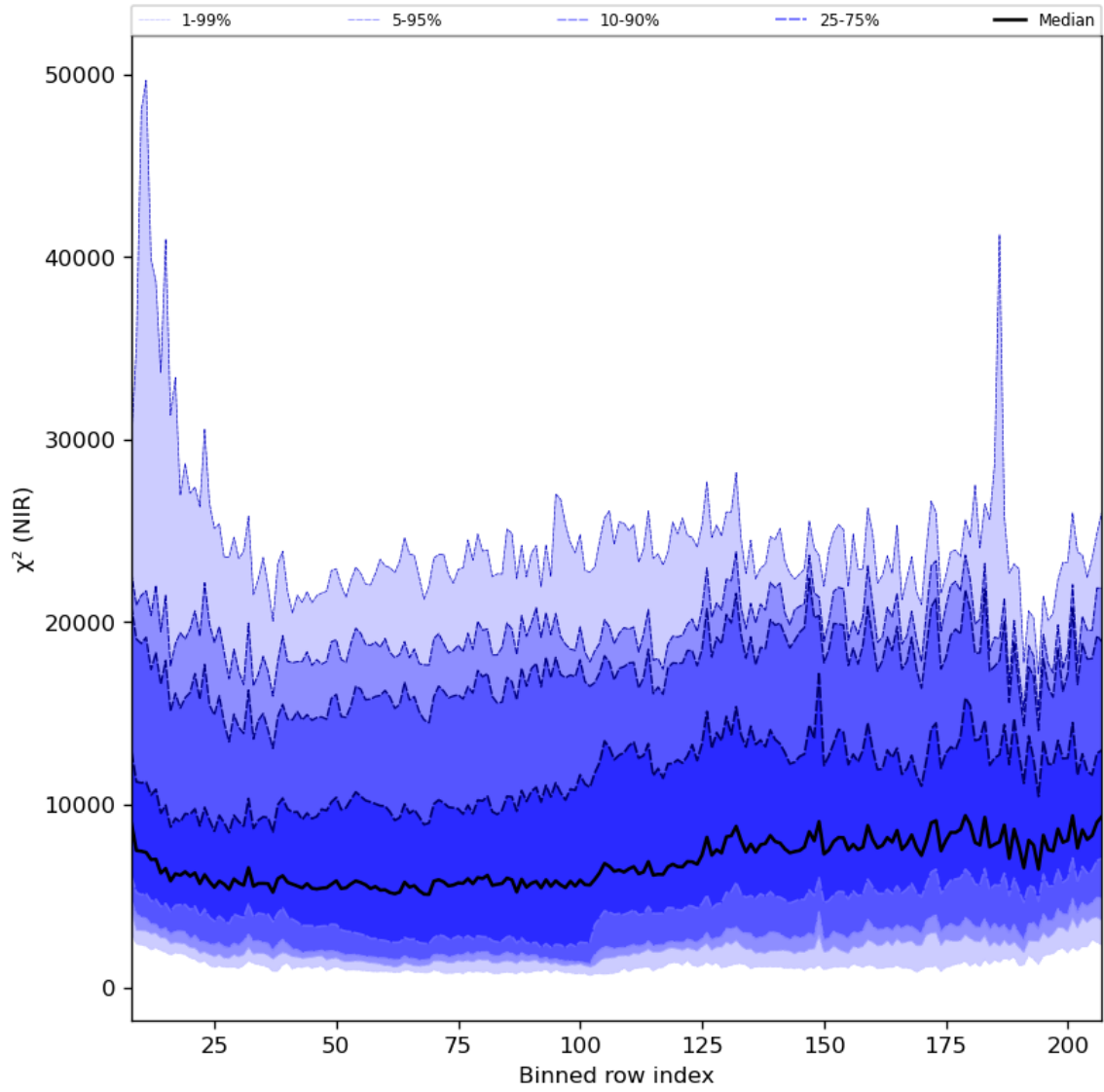
Figure 40: Along track statistics of “ \chi^2 (NIR)” for 2023-09-11 to 2023-09-13
