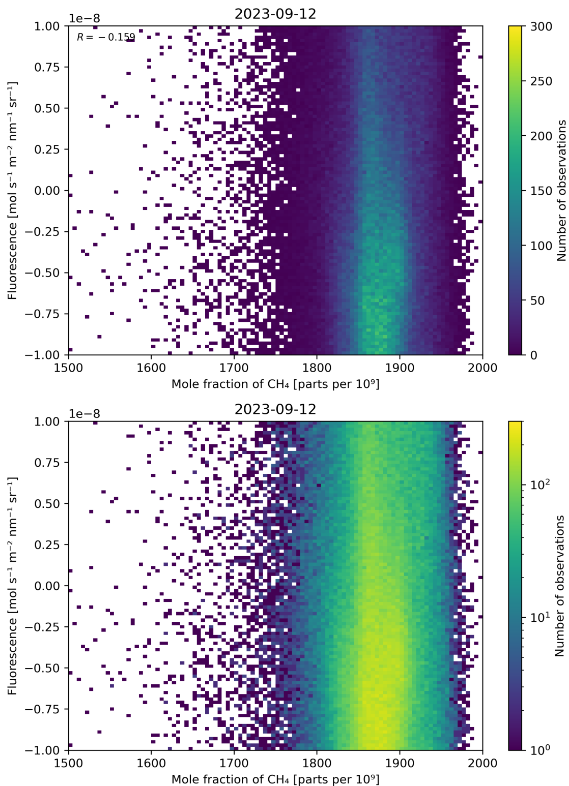
Figure 73: Scatter density plot of “Mole fraction of \text{CH}_4 ” against “Fluorescence” for 2023-09-11 to 2023-09-13.
