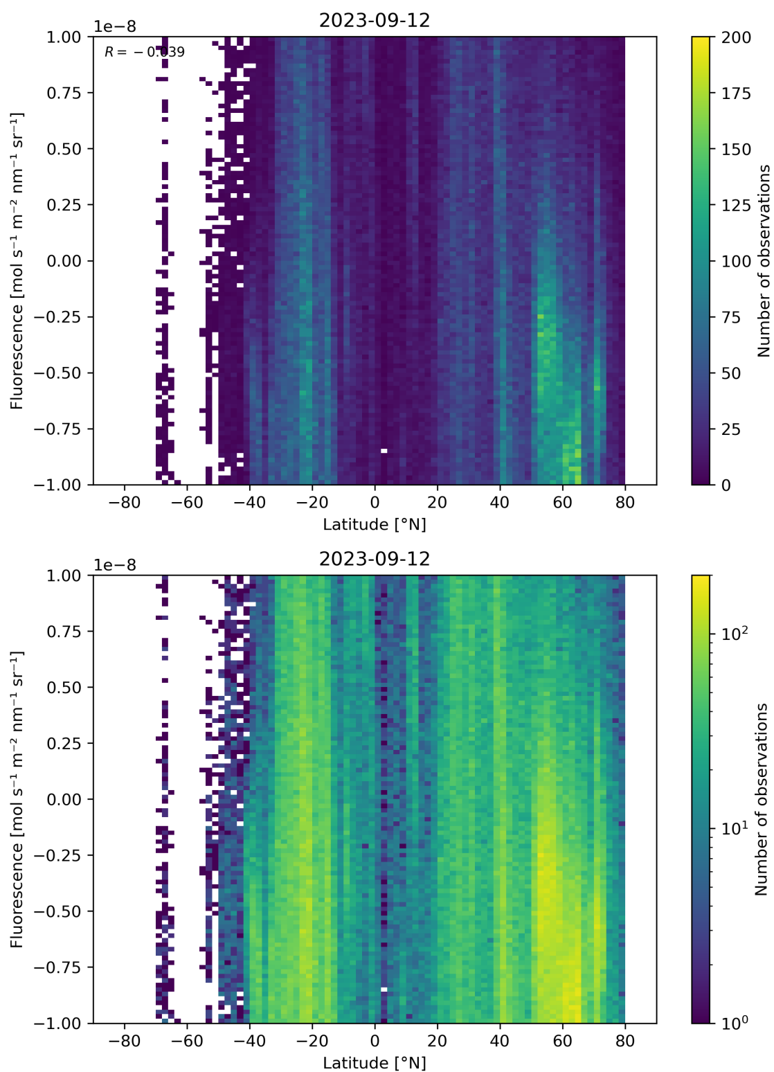
Figure 56: Scatter density plot of “Latitude” against “Fluorescence” for 2023-09-11 to 2023-09-13.
