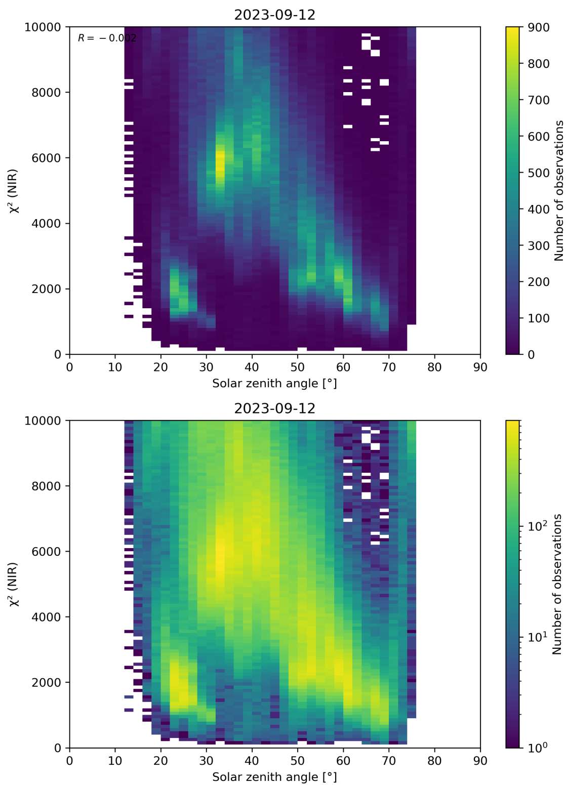
Figure 94: Scatter density plot of “Solar zenith angle” against “ \chi^2 (NIR)” for 2023-09-11 to 2023-09-13.
