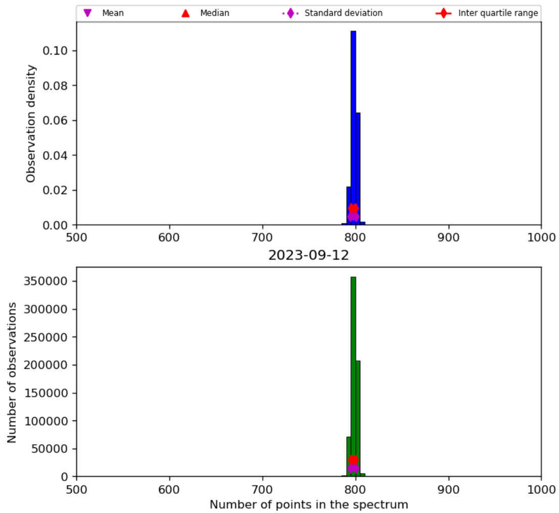
Figure 26: Histogram of “Number of points in the spectrum” for 2023-09-11 to 2023-09-13
