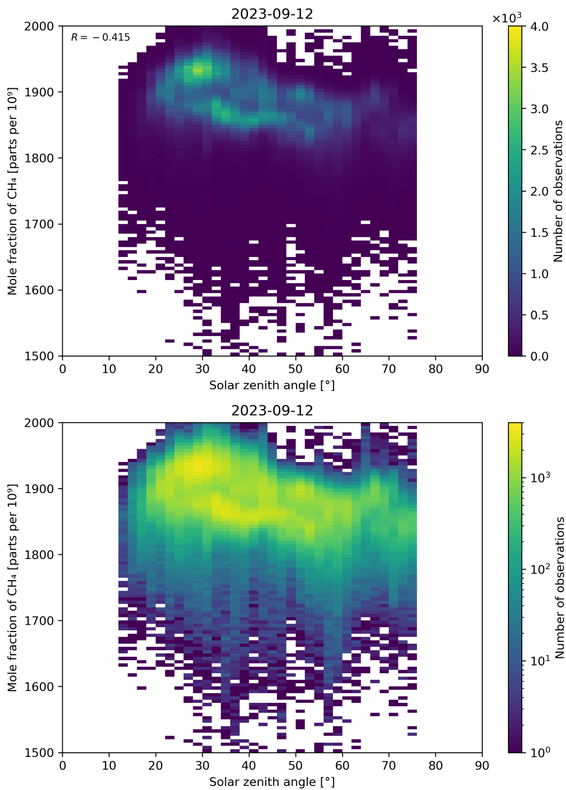
Figure 99: Scatter density plot of “Solar zenith angle” against “Mole fraction of CH 4 ” for 2023-09-11 to 2023-09-13.
