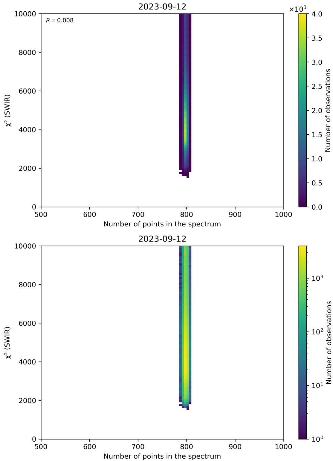
Figure 89: Scatter density plot of “Number of points in the spectrum” against “ \chi^2 (SWIR)” for 2023-09-11 to 2023-09-13.
