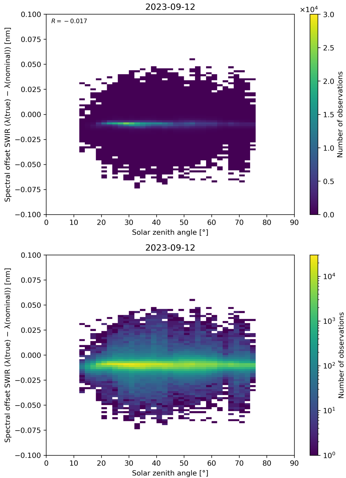
Figure 104: Scatter density plot of “Solar zenith angle” against “Spectral offset SWIR ( \lambda(\text{true}) - \lambda(\text{nominal}) )” for 2023-09-11 to 2023-09-13.
