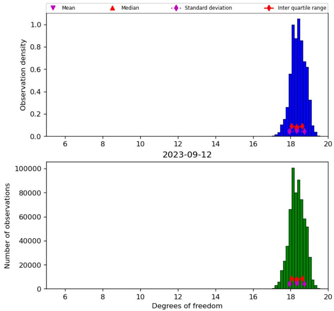
Figure 30: Histogram of “Degrees of freedom” for 2023-09-11 to 2023-09-13
