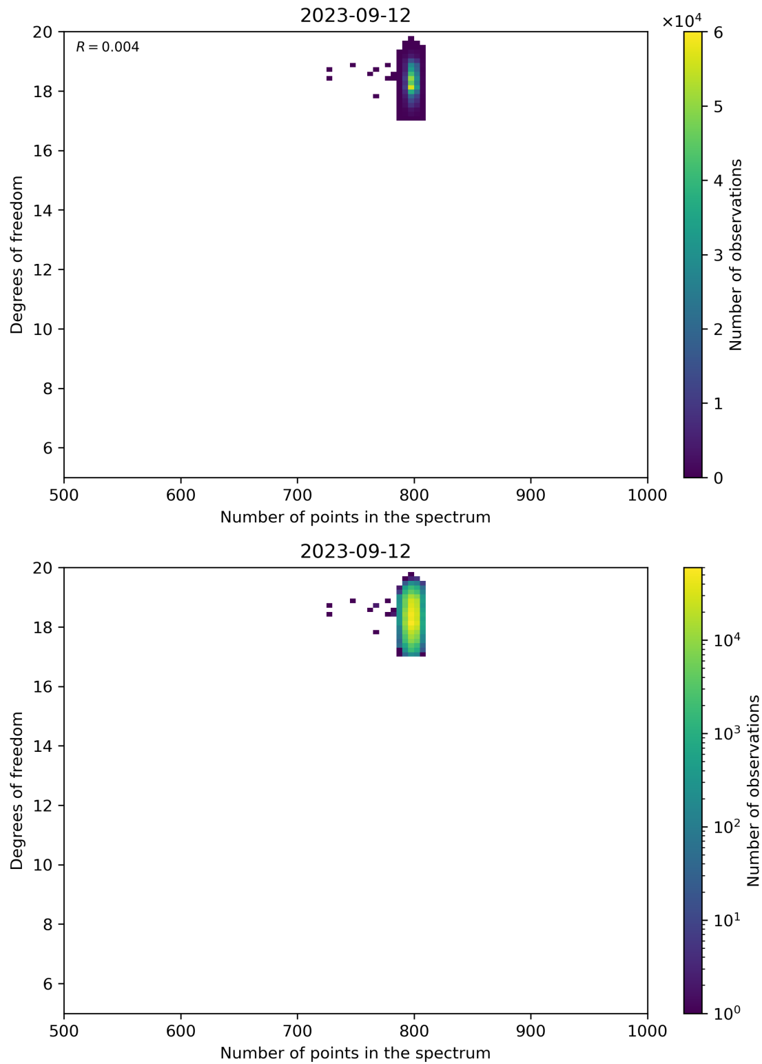
Figure 90: Scatter density plot of “Number of points in the spectrum” against “Degrees of freedom” for 2023-09-11 to 2023-09-13.
