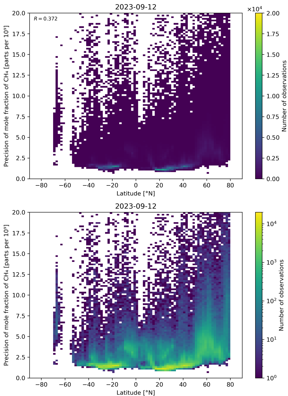
Figure 59: Scatter density plot of “Latitude” against “Precision of mole fraction of \text{CH}_4 ” for 2023-09-11 to 2023-09-13.
