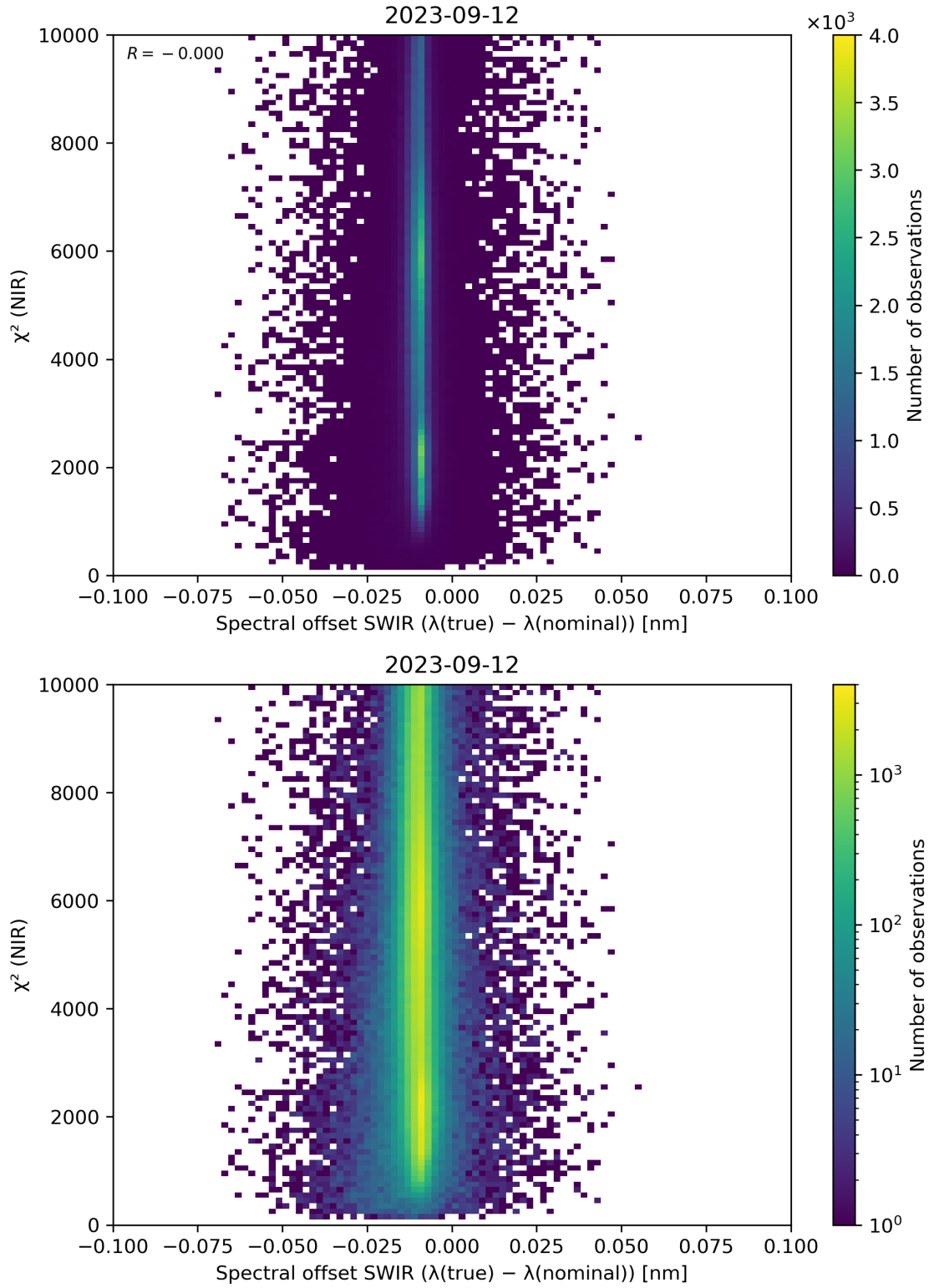
Figure 117: Scatter density plot of “Spectral offset SWIR ( \lambda(\text{true}) - \lambda(\text{nominal}) )” against “ \chi^2 (NIR)” for 2023-09-11 to 2023-09-13.
