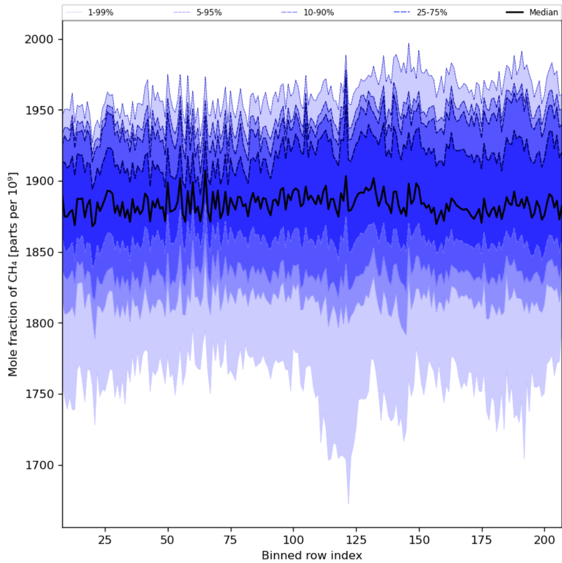
Figure 34: Along track statistics of “Mole fraction of CH 4 ” for 2023-09-11 to 2023-09-13
