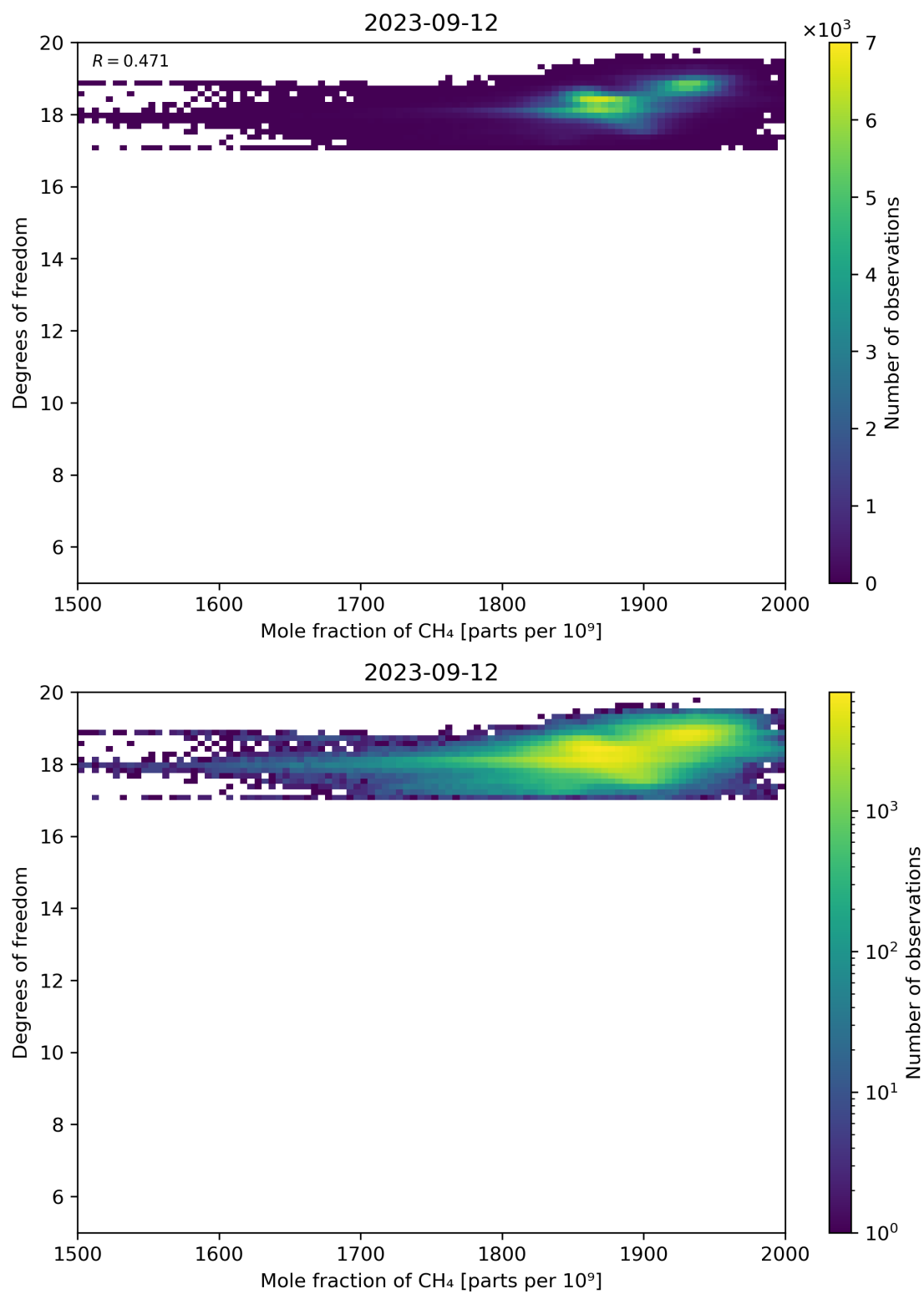
Figure 72: Scatter density plot of “Mole fraction of CH 4 ” against “Degrees of freedom” for 2023-09-11 to 2023-09-13.
