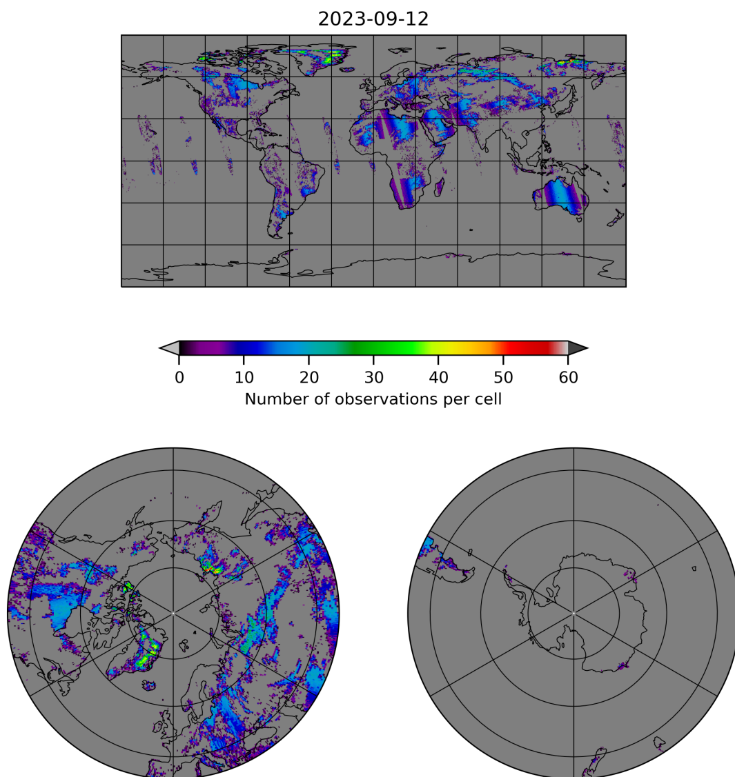
Figure 10: Map of the number of observations for 2023-09-11 to 2023-09-13
