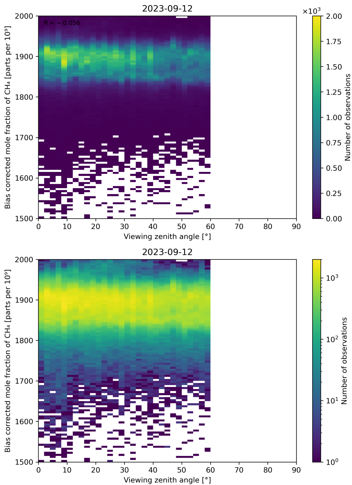
Figure 111: Scatter density plot of “Viewing zenith angle” against “Bias corrected mole fraction of CH 4 ” for 2023-09-11 to 2023-09-13.
