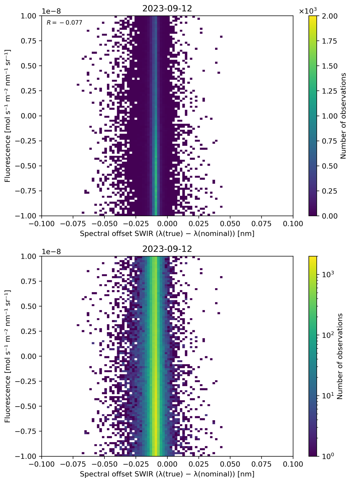
Figure 120: Scatter density plot of “Spectral offset SWIR ( \lambda(\text{true}) - \lambda(\text{nominal}) )” against “Fluorescence” for 2023-09-11 to 2023-09-13.
