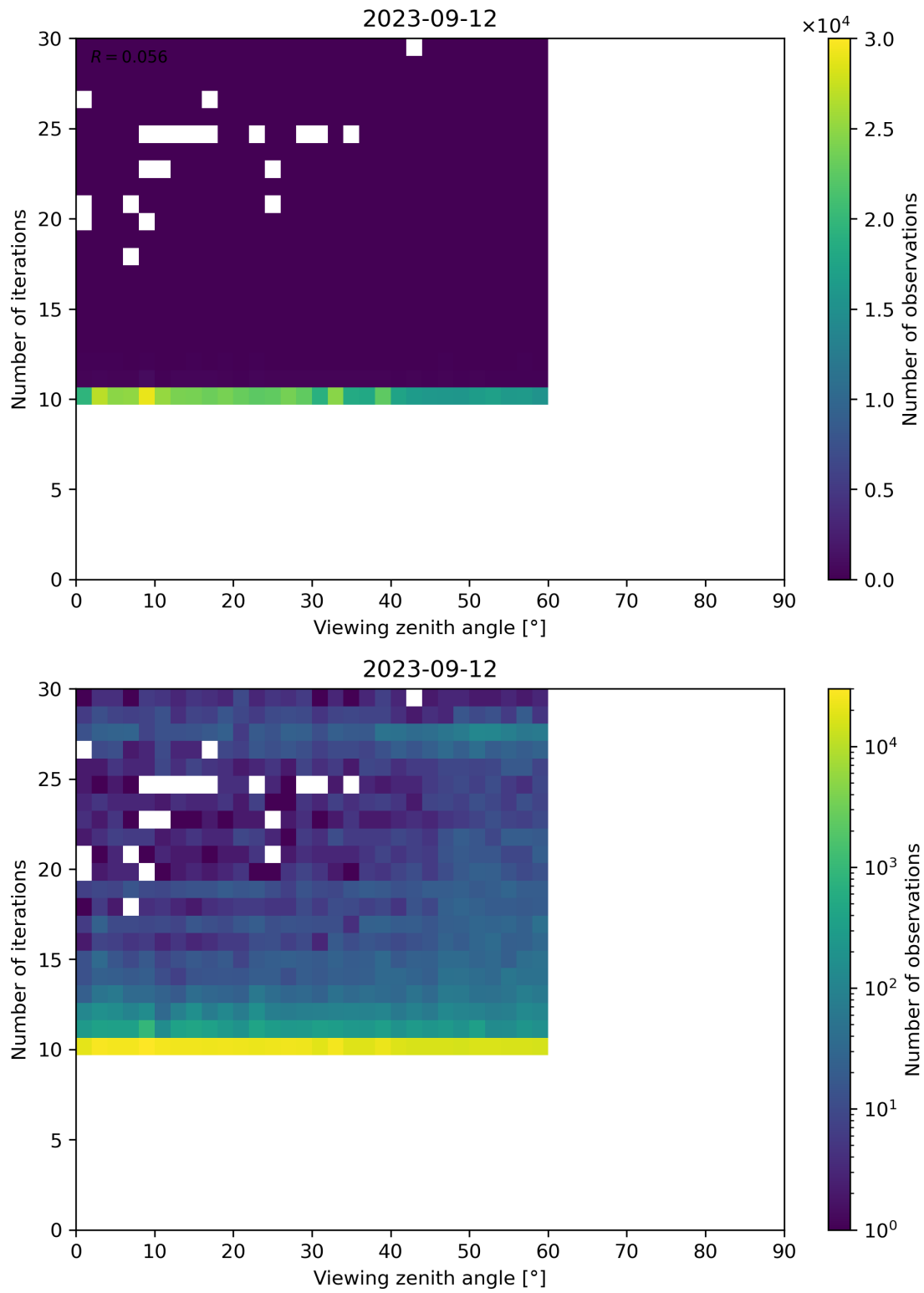
Figure 113: Scatter density plot of “Viewing zenith angle” against “Number of iterations” for 2023-09-11 to 2023-09-13.
