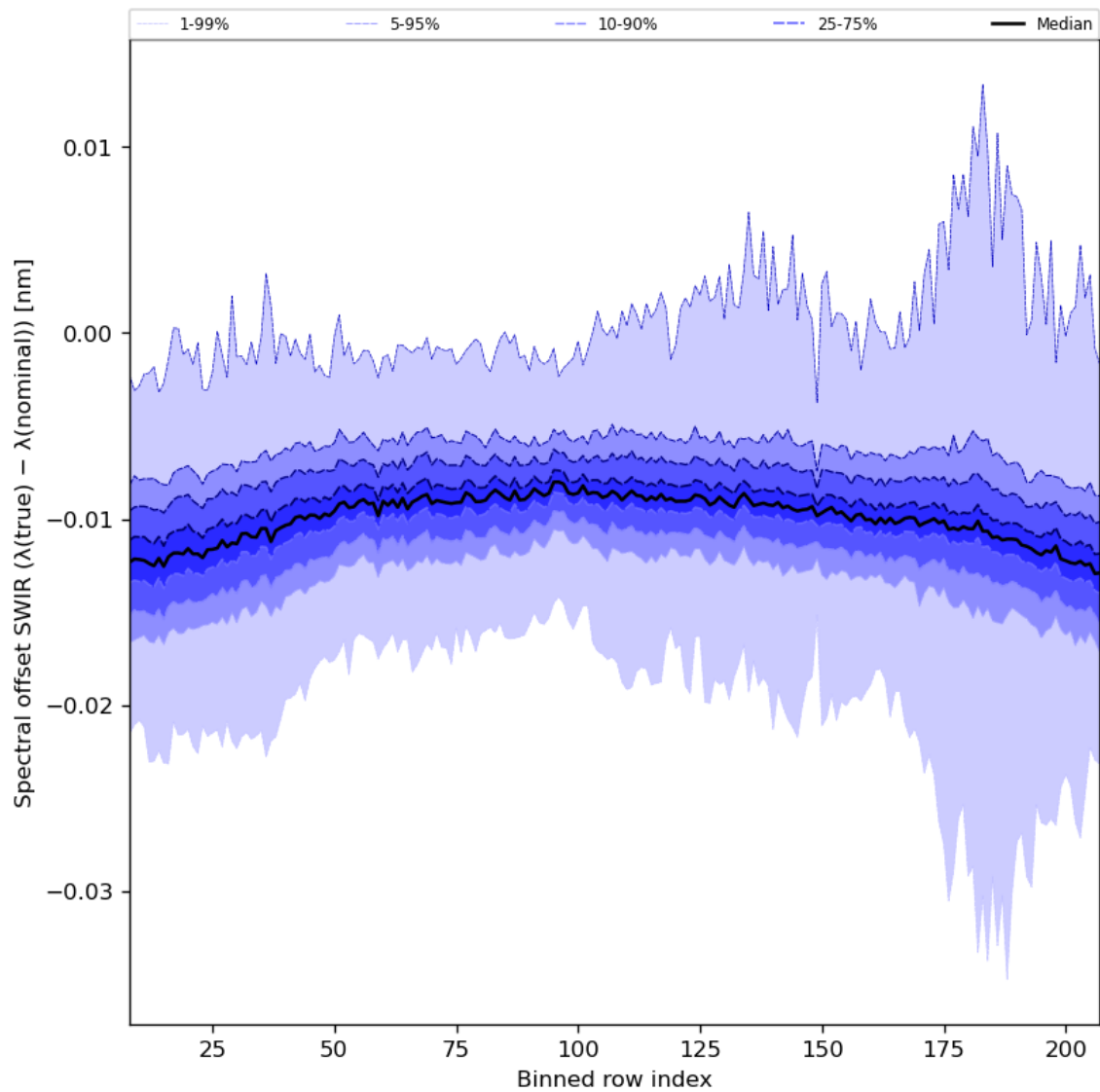
Figure 38: Along track statistics of “Spectral offset SWIR ( \lambda(\text{true}) - \lambda(\text{nominal}) )” for 2023-09-11 to 2023-09-13
