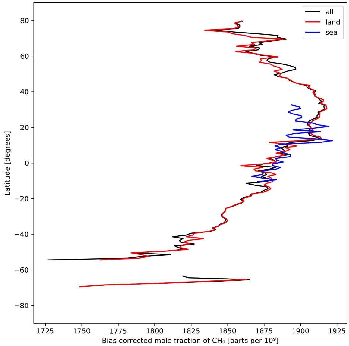
Figure 14: Zonal average of “Bias corrected mole fraction of CH 4 ” for 2023-09-11 to 2023-09-13.
