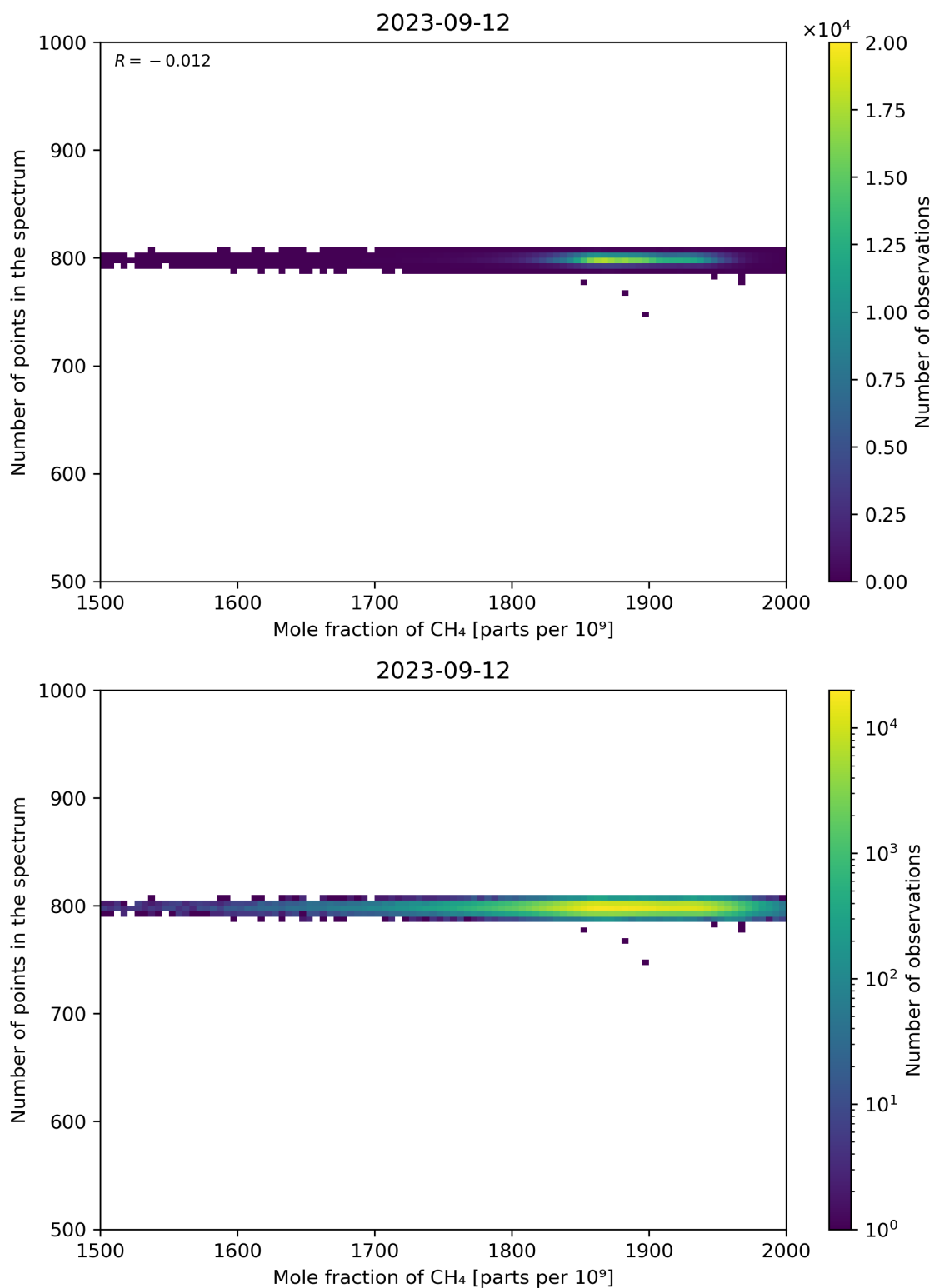
Figure 77: Scatter density plot of “Mole fraction of CH 4 ” against “Number of points in the spectrum” for 2023-09-11 to 2023-09-13.
