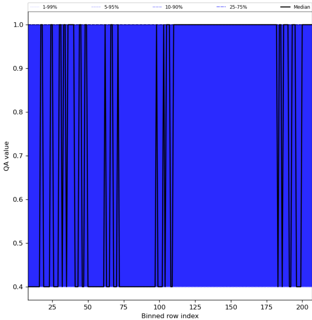
Figure 33: Along track statistics of “QA value” for 2023-09-11 to 2023-09-13
