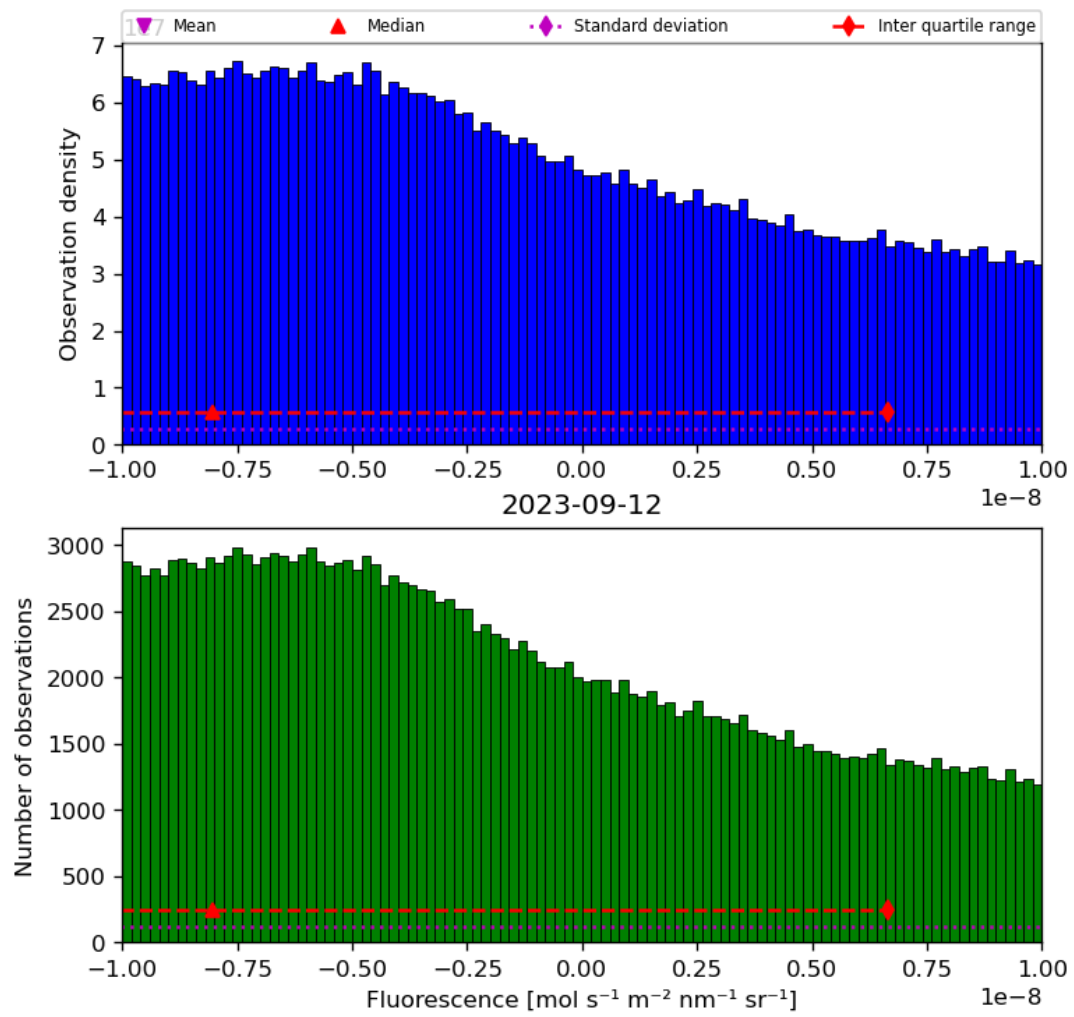
Figure 32: Histogram of “Fluorescence” for 2023-09-11 to 2023-09-13
