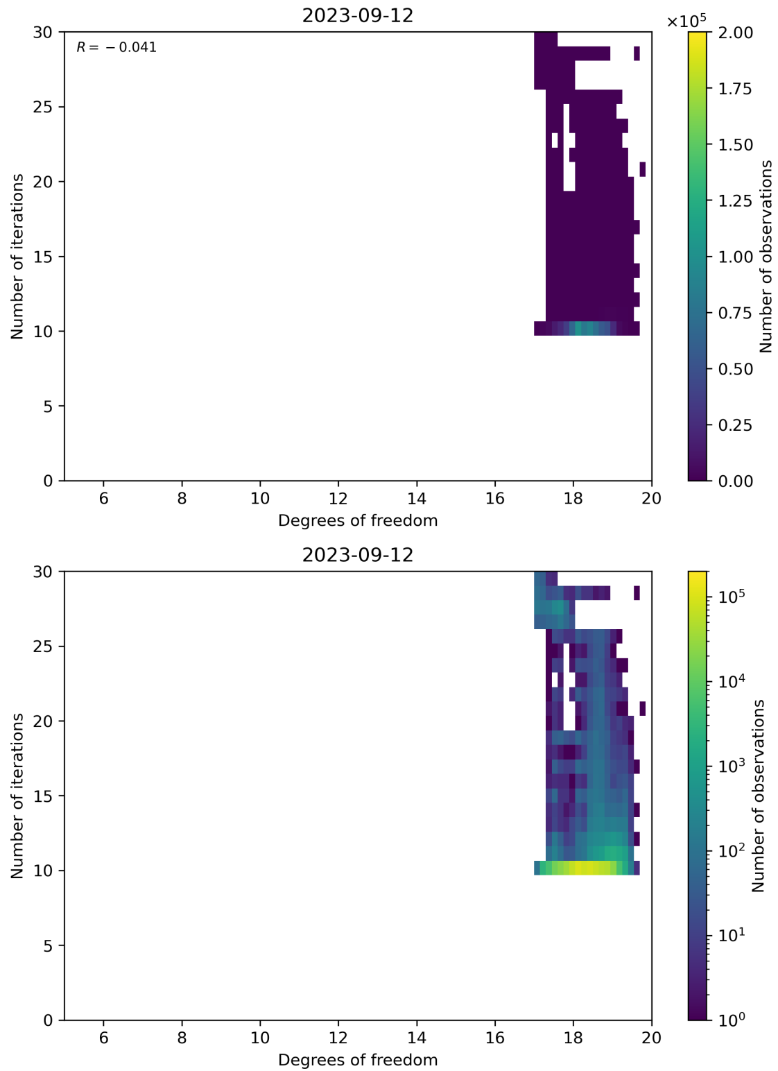
Figure 52: Scatter density plot of “Degrees of freedom” against “Number of iterations” for 2023-09-11 to 2023-09-13.
