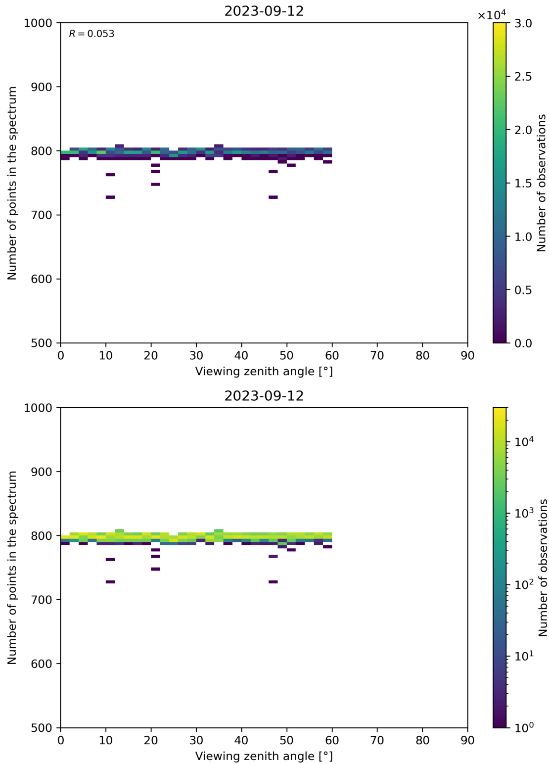
Figure 114: Scatter density plot of “Viewing zenith angle” against “Number of points in the spectrum” for 2023-09-11 to 2023-09-13.
