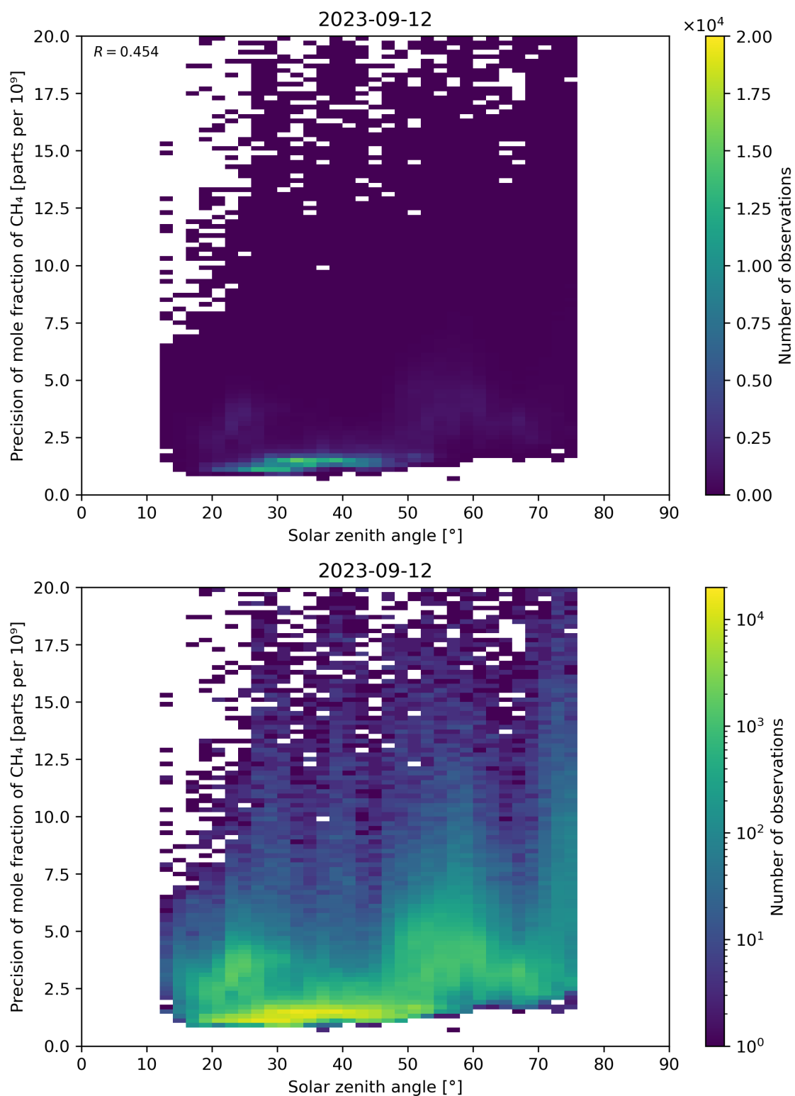
Figure 101: Scatter density plot of “Solar zenith angle” against “Precision of mole fraction of CH 4 ” for 2023-09-11 to 2023-09-13.
