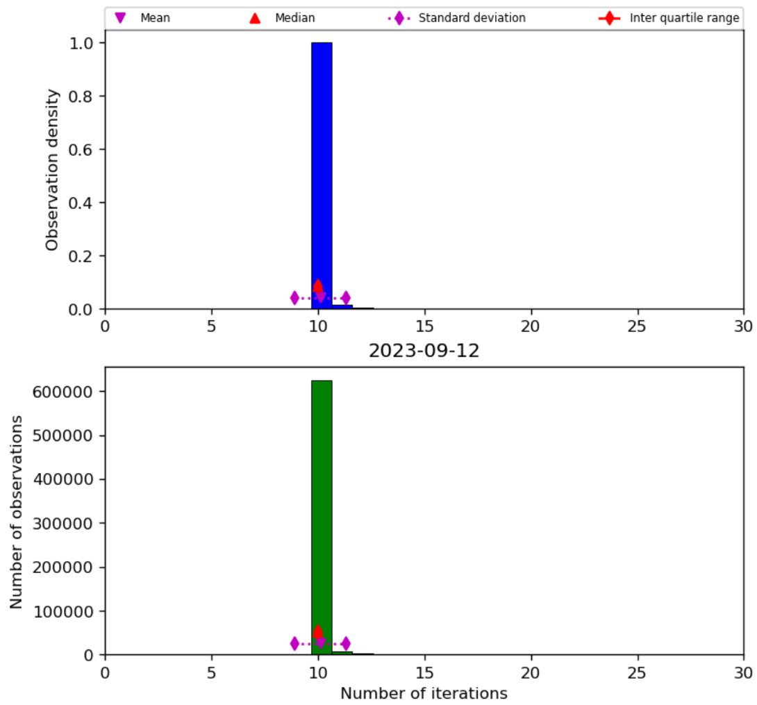
Figure 31: Histogram of “Number of iterations” for 2023-09-11 to 2023-09-13
