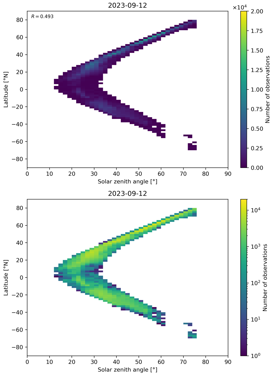
Figure 98: Scatter density plot of “Solar zenith angle” against “Latitude” for 2023-09-11 to 2023-09-13.
