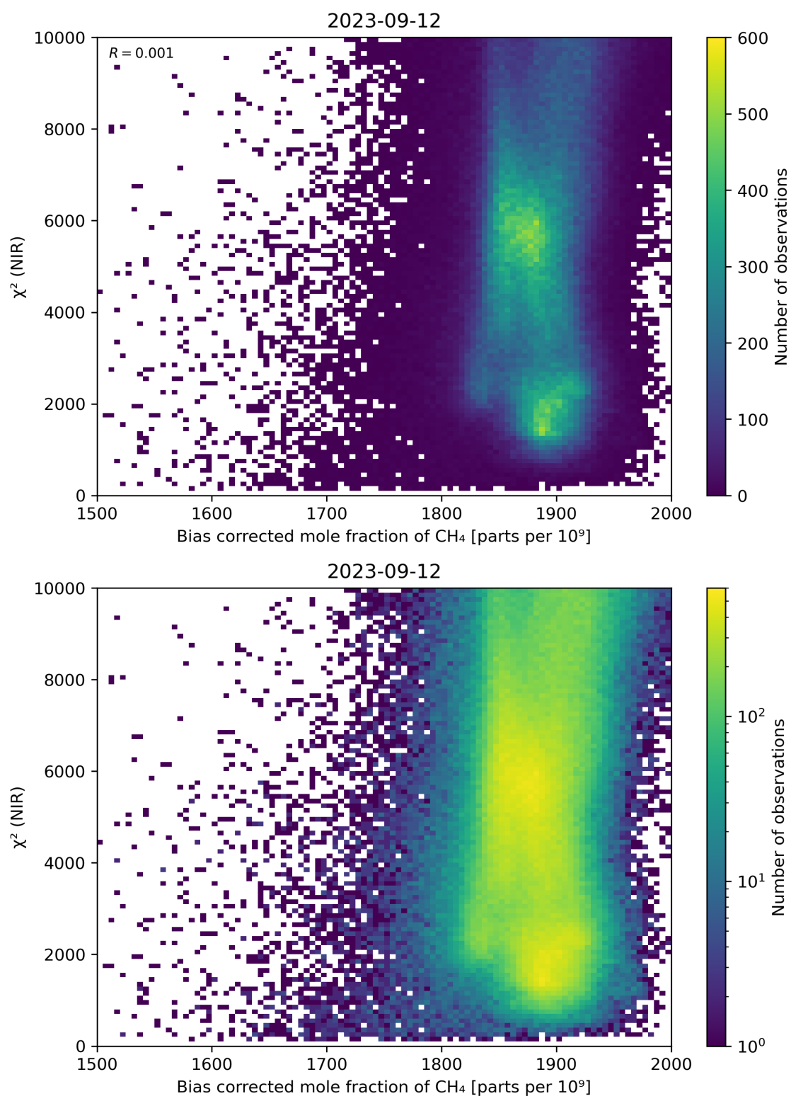
Figure 63: Scatter density plot of “Bias corrected mole fraction of \text{CH}_4 ” against “ \chi^2 (NIR)” for 2023-09-11 to 2023-09-13.
