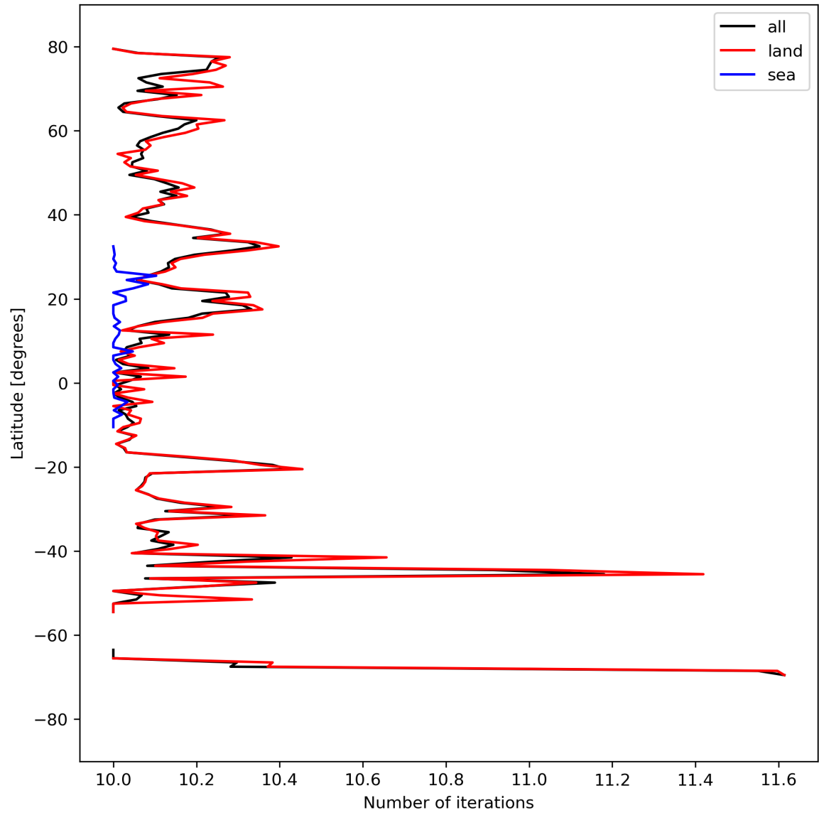
Figure 20: Zonal average of “Number of iterations” for 2023-09-11 to 2023-09-13.
