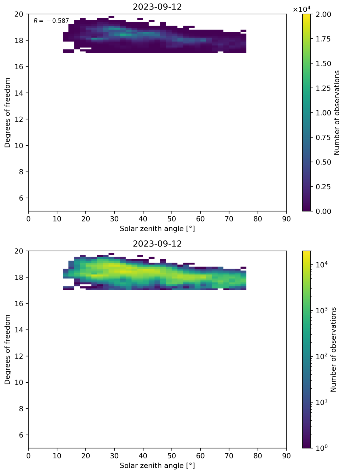
Figure 96: Scatter density plot of “Solar zenith angle” against “Degrees of freedom” for 2023-09-11 to 2023-09-13.
