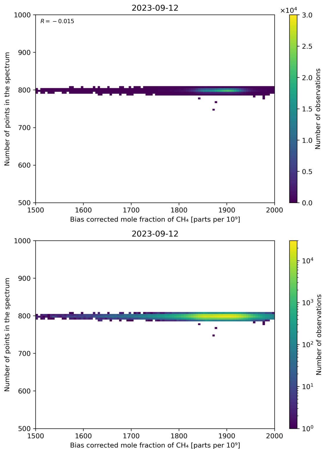
Figure 68: Scatter density plot of “Bias corrected mole fraction of CH 4 ” against “Number of points in the spectrum” for 2023-09-11 to 2023-09-13.
