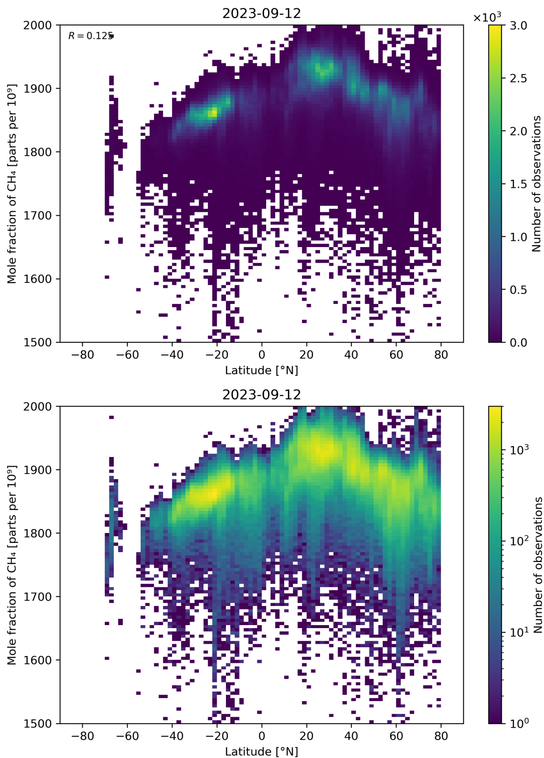
Figure 57: Scatter density plot of “Latitude” against “Mole fraction of CH 4 ” for 2023-09-11 to 2023-09-13.
