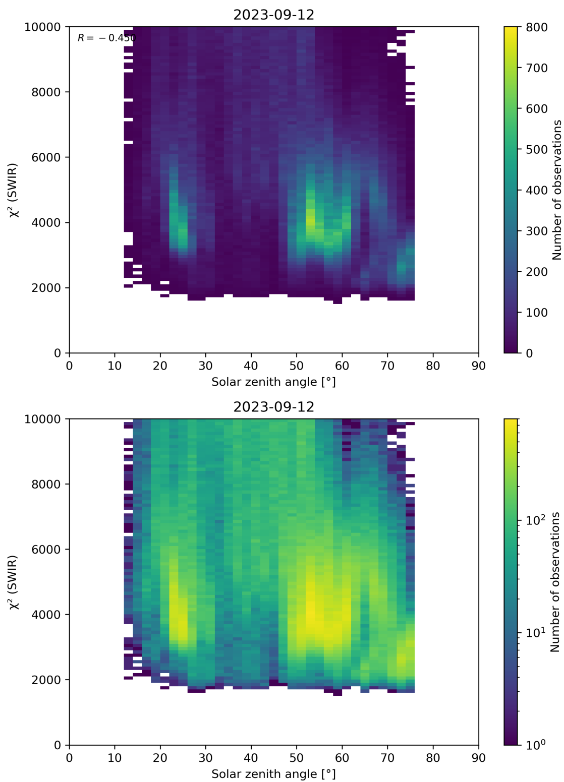
Figure 95: Scatter density plot of “Solar zenith angle” against “ \chi^2 (SWIR)” for 2023-09-11 to 2023-09-13.
