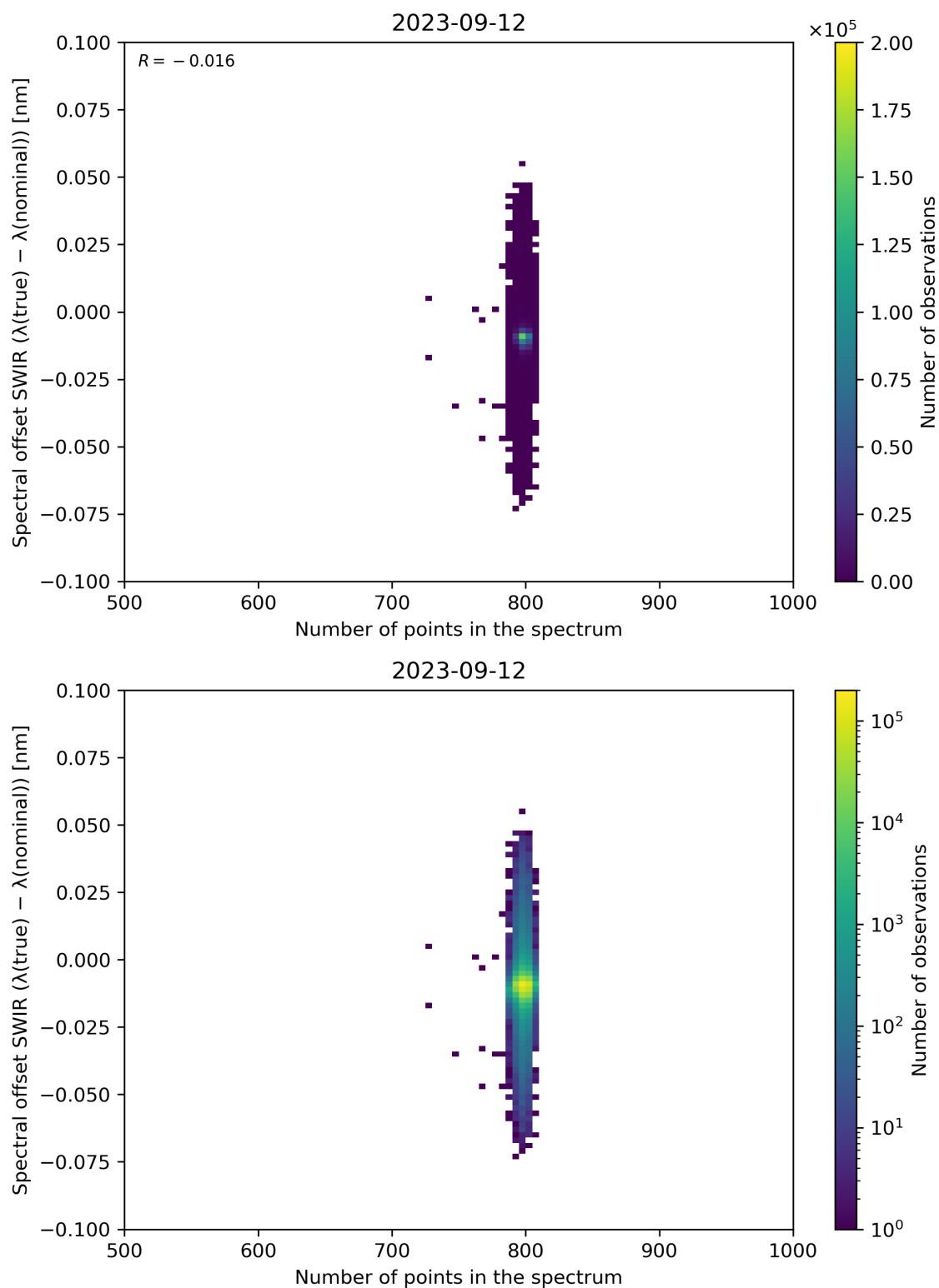
Figure 93: Scatter density plot of “Number of points in the spectrum” against “Spectral offset SWIR ( \lambda(\text{true}) - \lambda(\text{nominal}) )” for 2023-09-11 to 2023-09-13.
