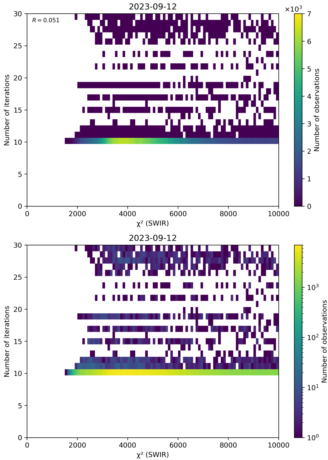
Figure 50: Scatter density plot of “ \chi^2 (SWIR)” against “Number of iterations” for 2023-09-11 to 2023-09-13.
