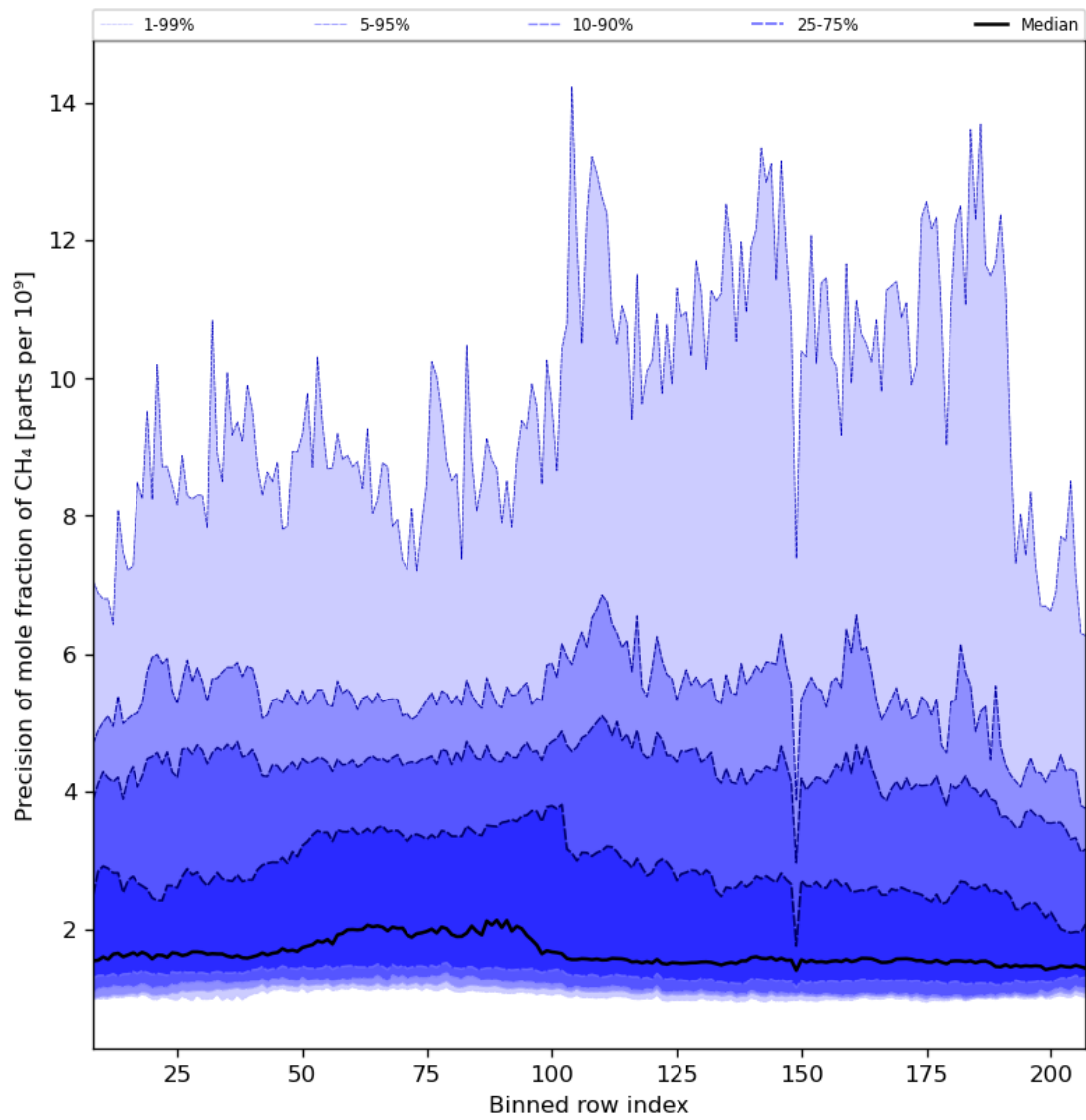
Figure 35: Along track statistics of “Precision of mole fraction of CH 4 ” for 2023-09-11 to 2023-09-13
