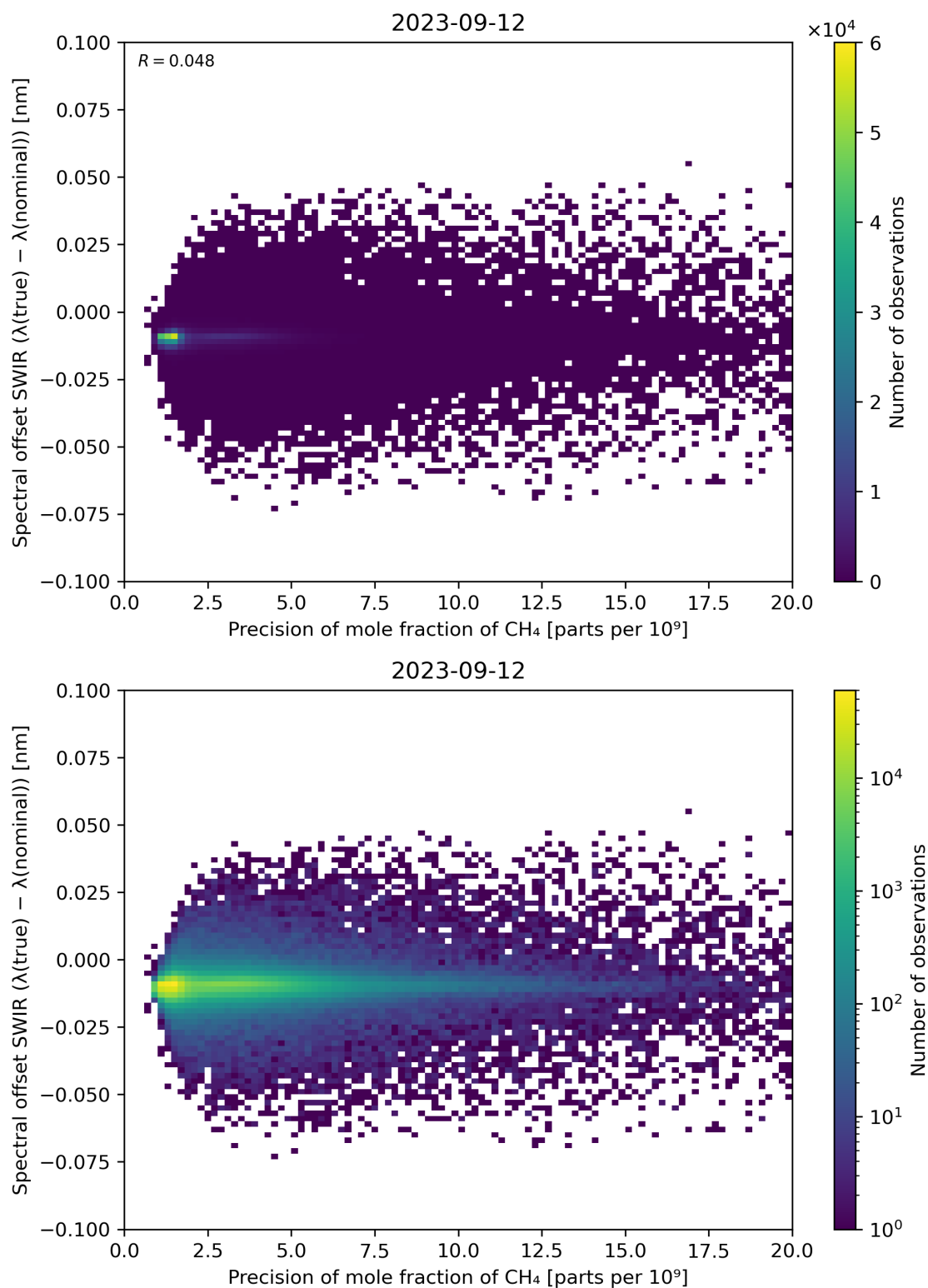
Figure 85: Scatter density plot of “Precision of mole fraction of CH 4 ” against “Spectral offset SWIR ( \lambda(\text{true}) - \lambda(\text{nominal}) )” for 2023-09-11 to 2023-09-13.
