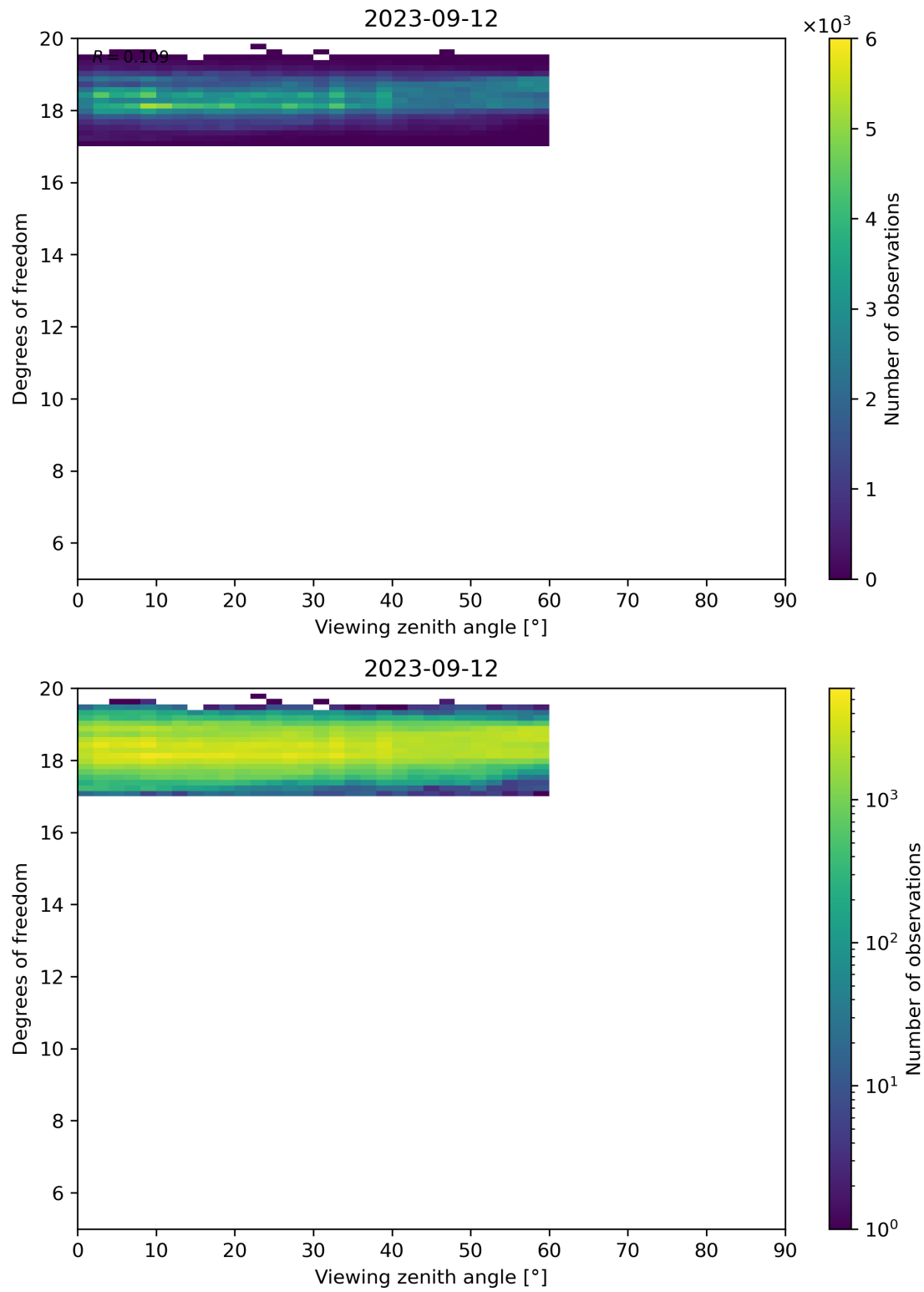
Figure 107: Scatter density plot of “Viewing zenith angle” against “Degrees of freedom” for 2023-09-11 to 2023-09-13.
