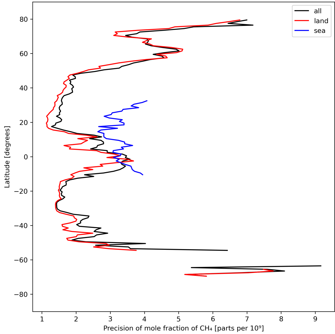
Figure 13: Zonal average of “Precision of mole fraction of CH 4 ” for 2023-09-11 to 2023-09-13.
