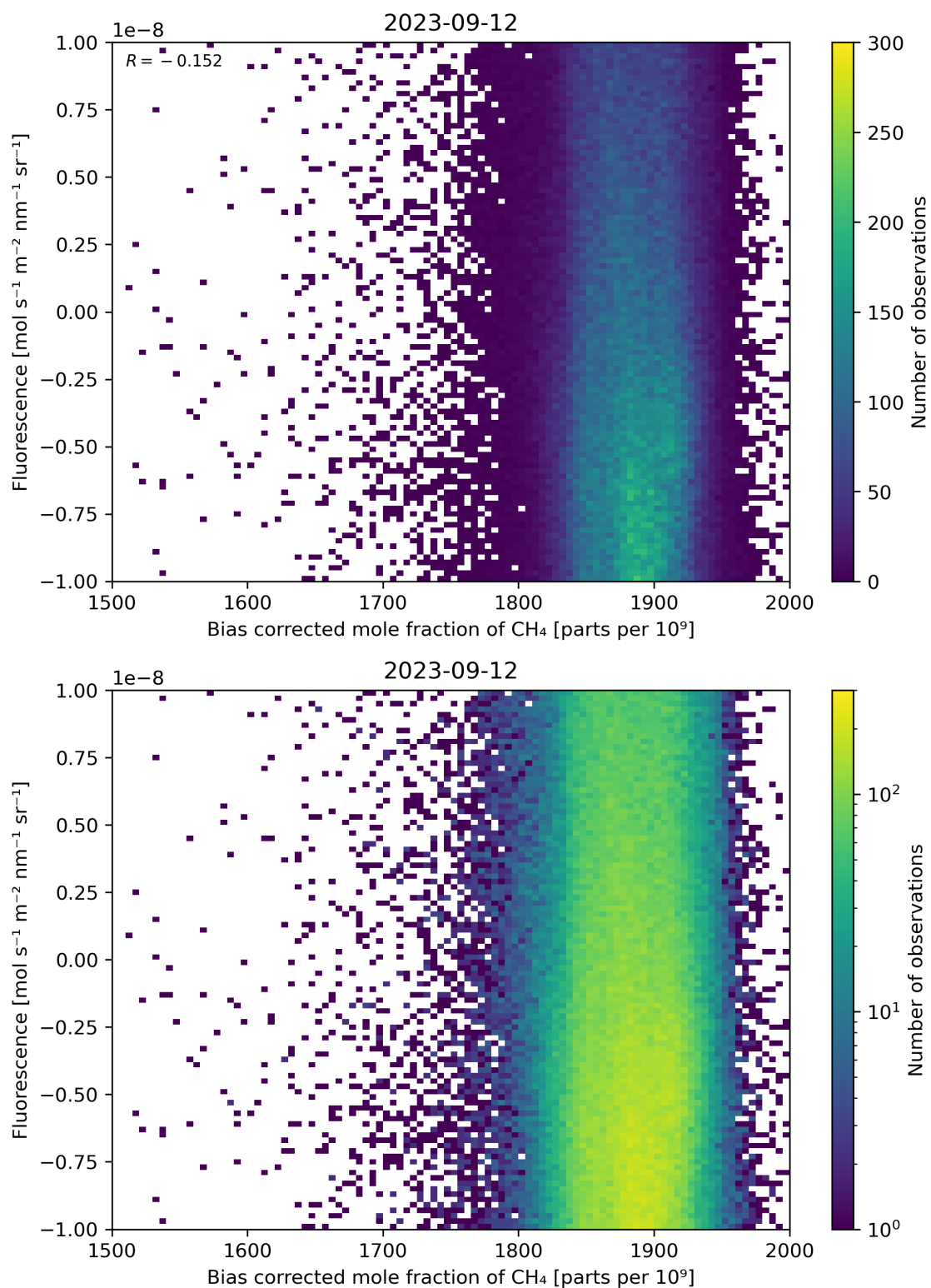
Figure 66: Scatter density plot of “Bias corrected mole fraction of \text{CH}_4 ” against “Fluorescence” for 2023-09-11 to 2023-09-13.
