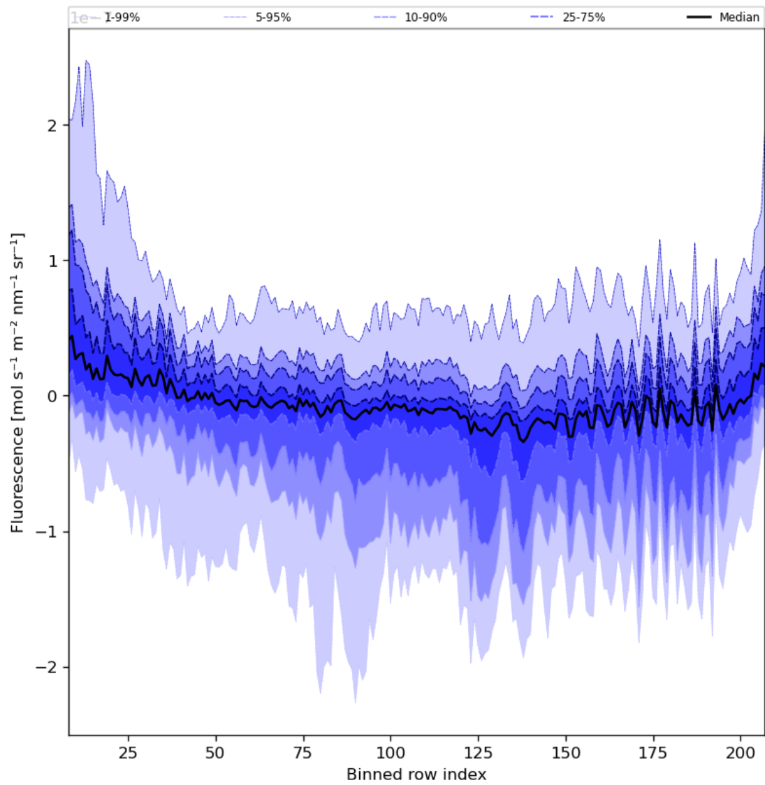
Figure 43: Along track statistics of “Fluorescence” for 2023-09-11 to 2023-09-13
