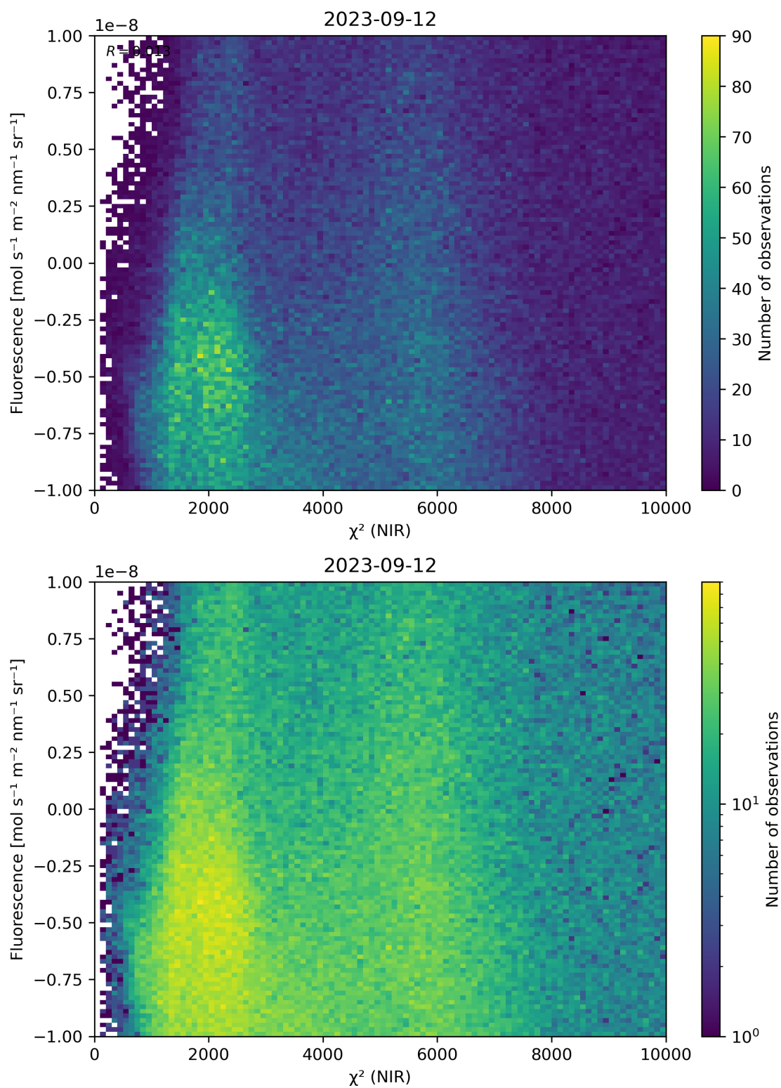
Figure 45: Scatter density plot of “ \chi^2 (NIR)” against “Fluorescence” for 2023-09-11 to 2023-09-13.
