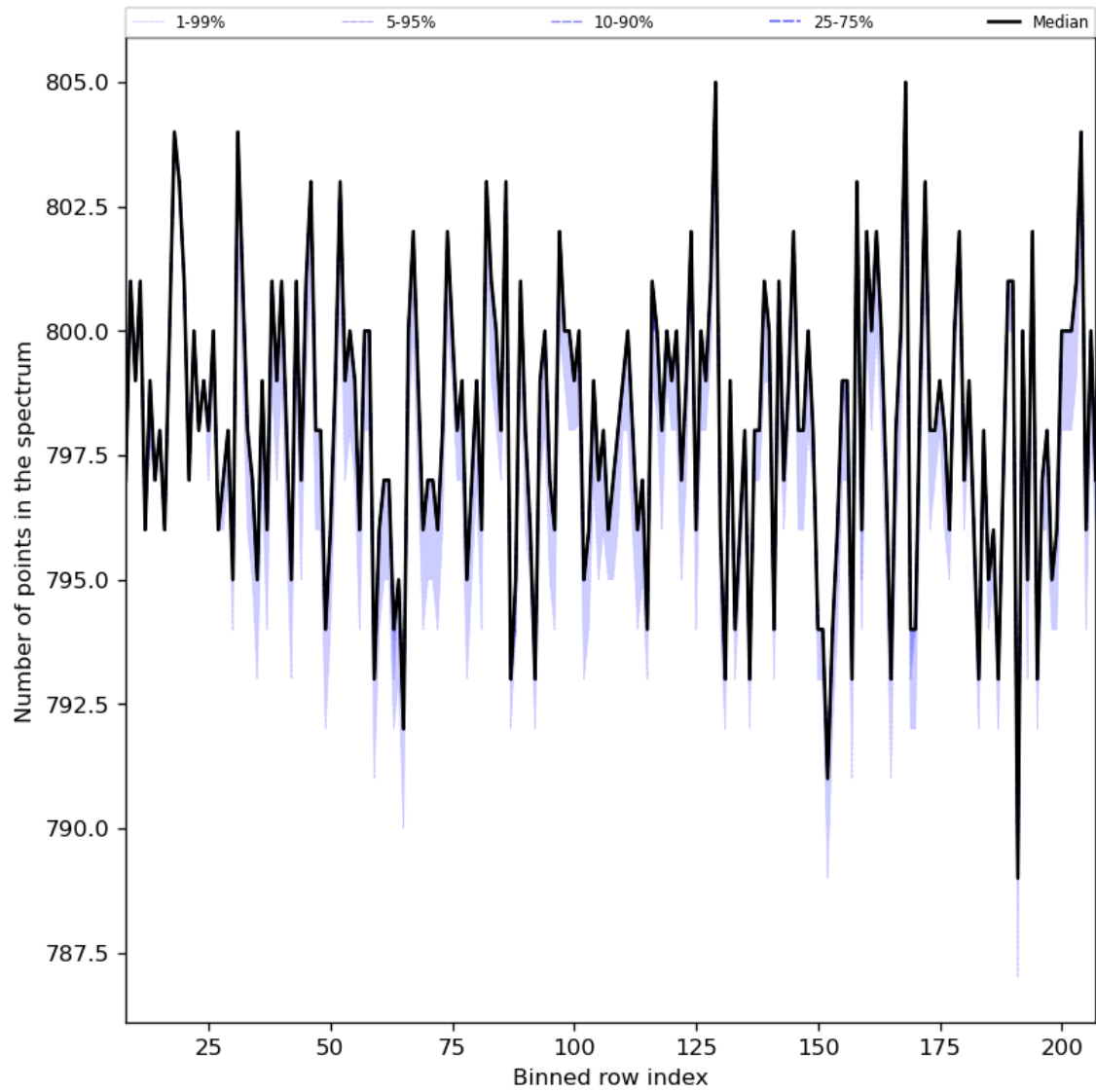
Figure 37: Along track statistics of “Number of points in the spectrum” for 2023-09-11 to 2023-09-13
