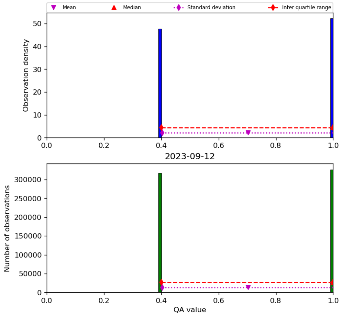
Figure 22: Histogram of “QA value” for 2023-09-11 to 2023-09-13
