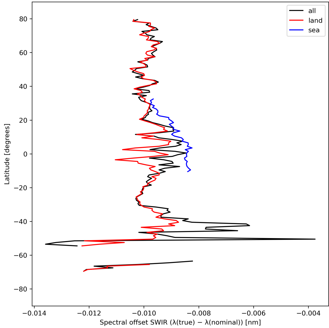
Figure 16: Zonal average of “Spectral offset SWIR ( \lambda(\text{true}) - \lambda(\text{nominal}) )” for 2023-09-11 to 2023-09-13.
