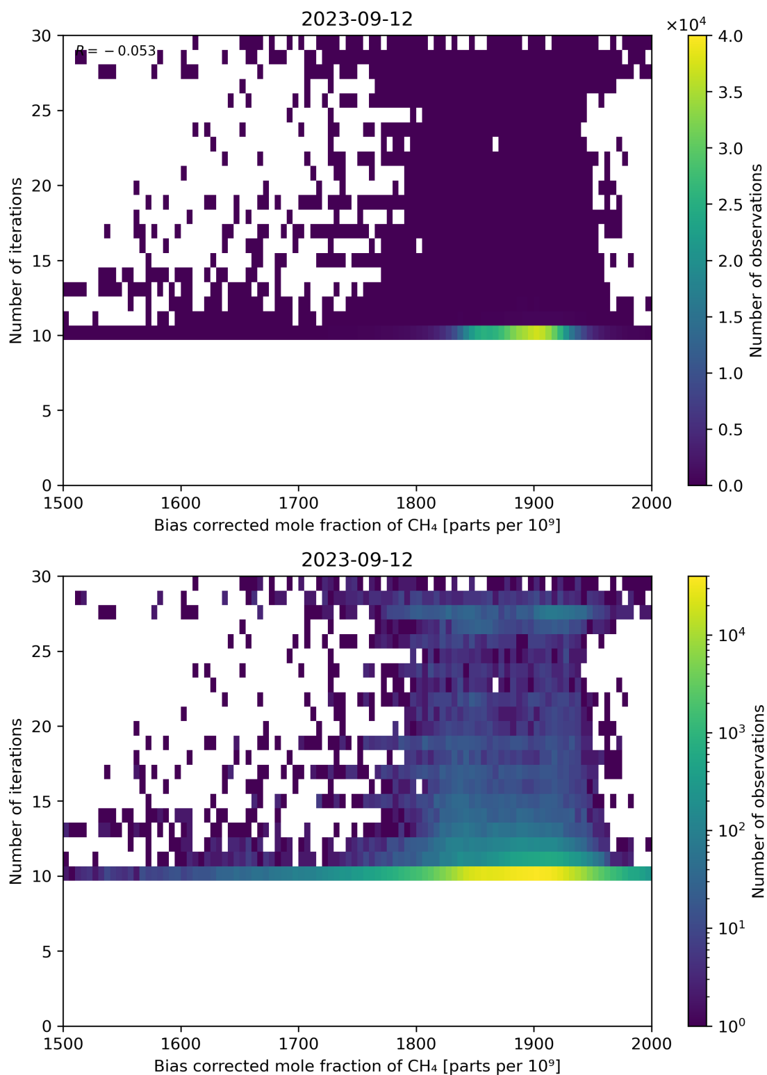
Figure 67: Scatter density plot of “Bias corrected mole fraction of CH 4 ” against “Number of iterations” for 2023-09-11 to 2023-09-13.
