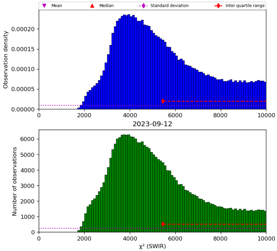
Figure 28: Histogram of “ \chi^2 (SWIR)” for 2023-09-11 to 2023-09-13
