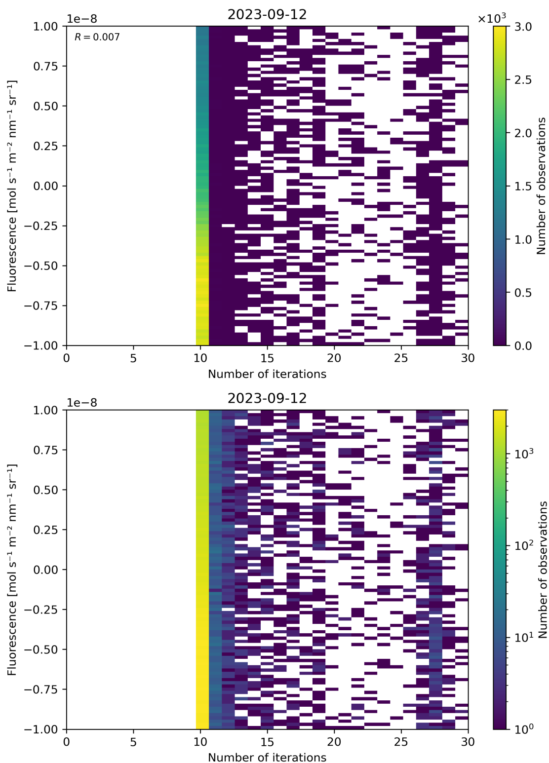
Figure 87: Scatter density plot of “Number of iterations” against “Fluorescence” for 2023-09-11 to 2023-09-13.
