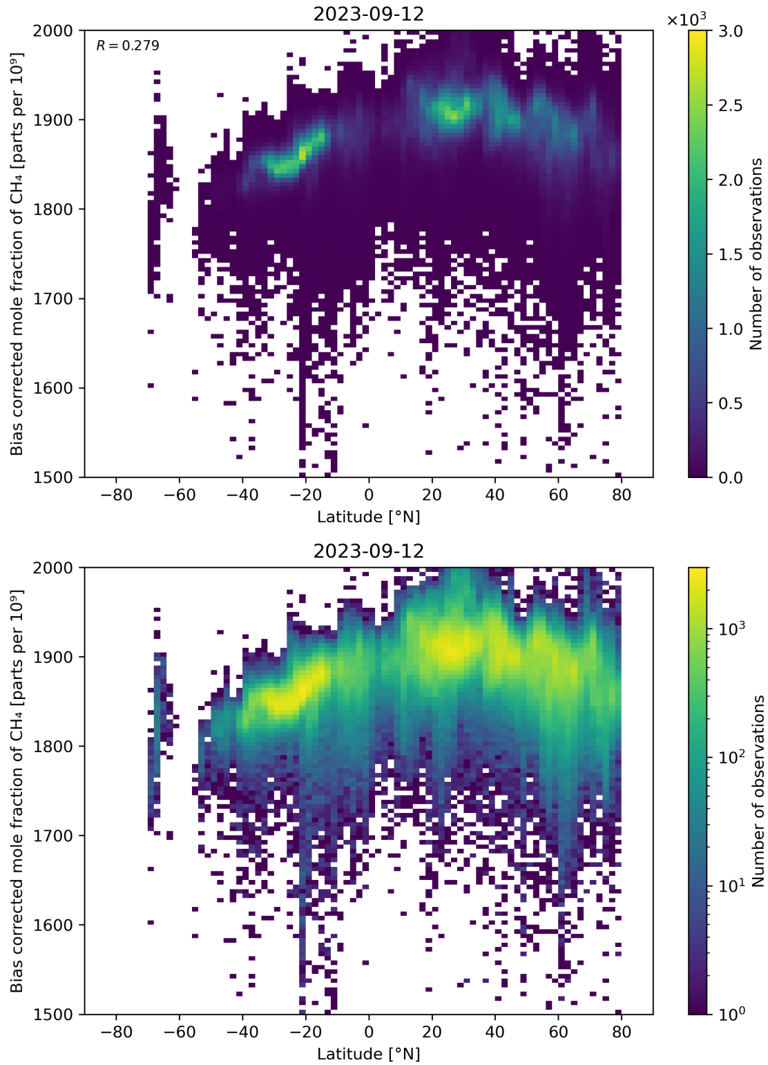
Figure 58: Scatter density plot of “Latitude” against “Bias corrected mole fraction of \text{CH}_4 ” for 2023-09-11 to 2023-09-13.
