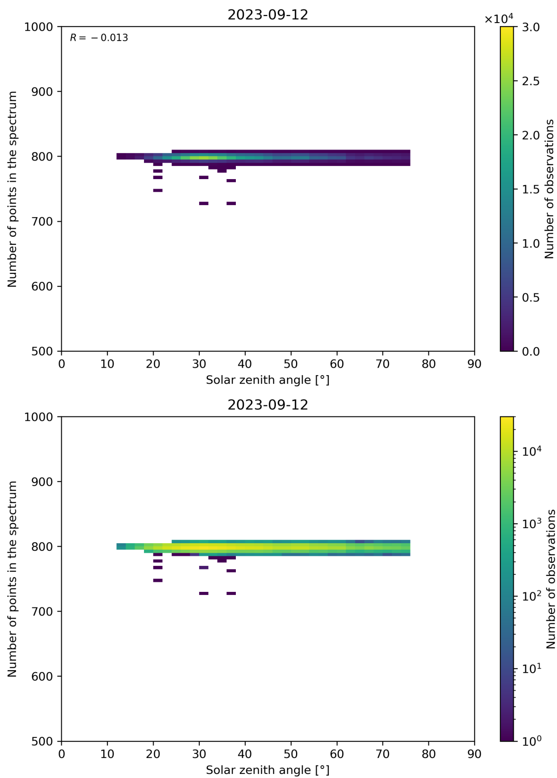
Figure 103: Scatter density plot of “Solar zenith angle” against “Number of points in the spectrum” for 2023-09-11 to 2023-09-13.
