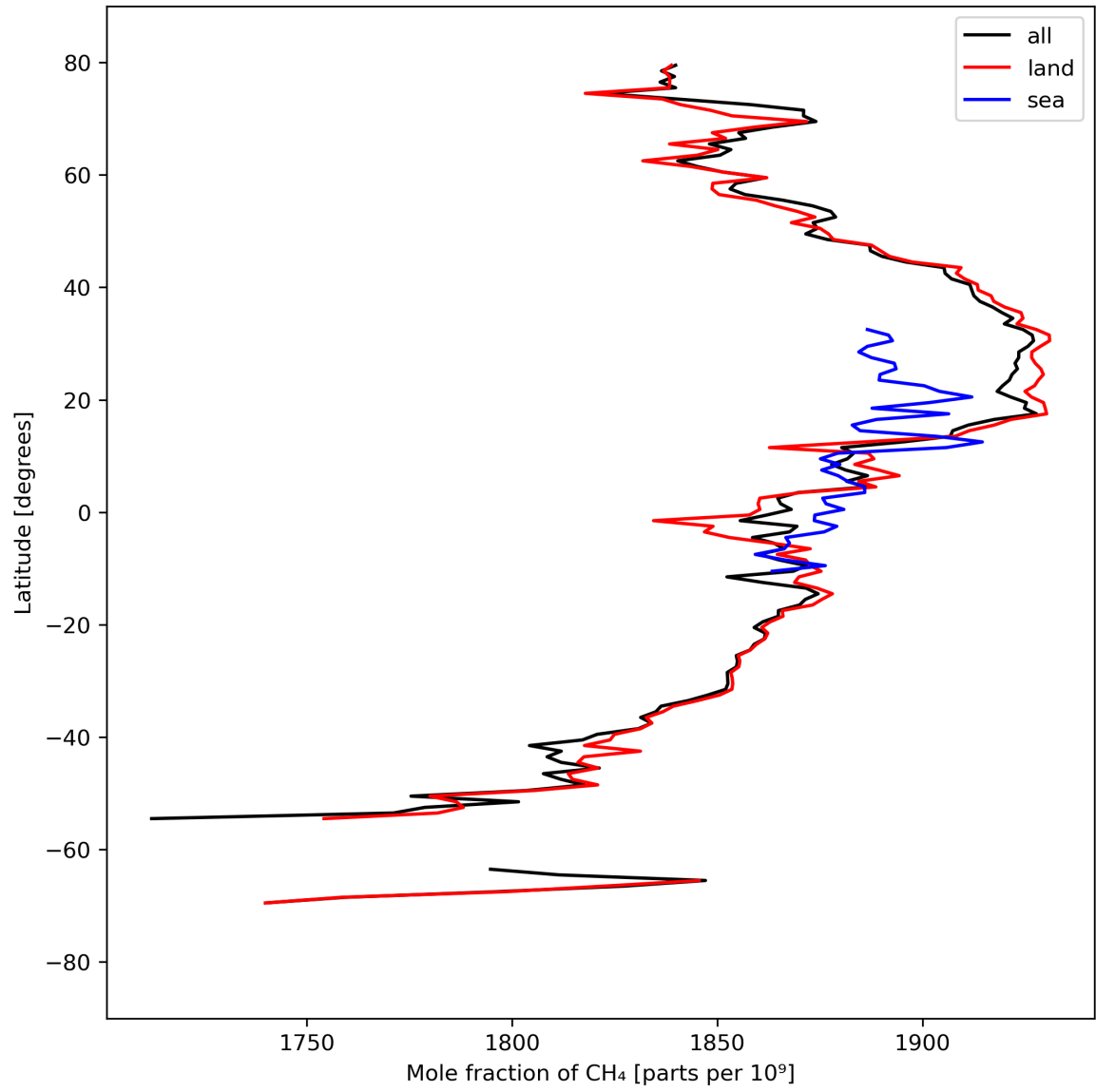
Figure 12: Zonal average of “Mole fraction of \text{CH}_4 ” for 2023-09-11 to 2023-09-13.
