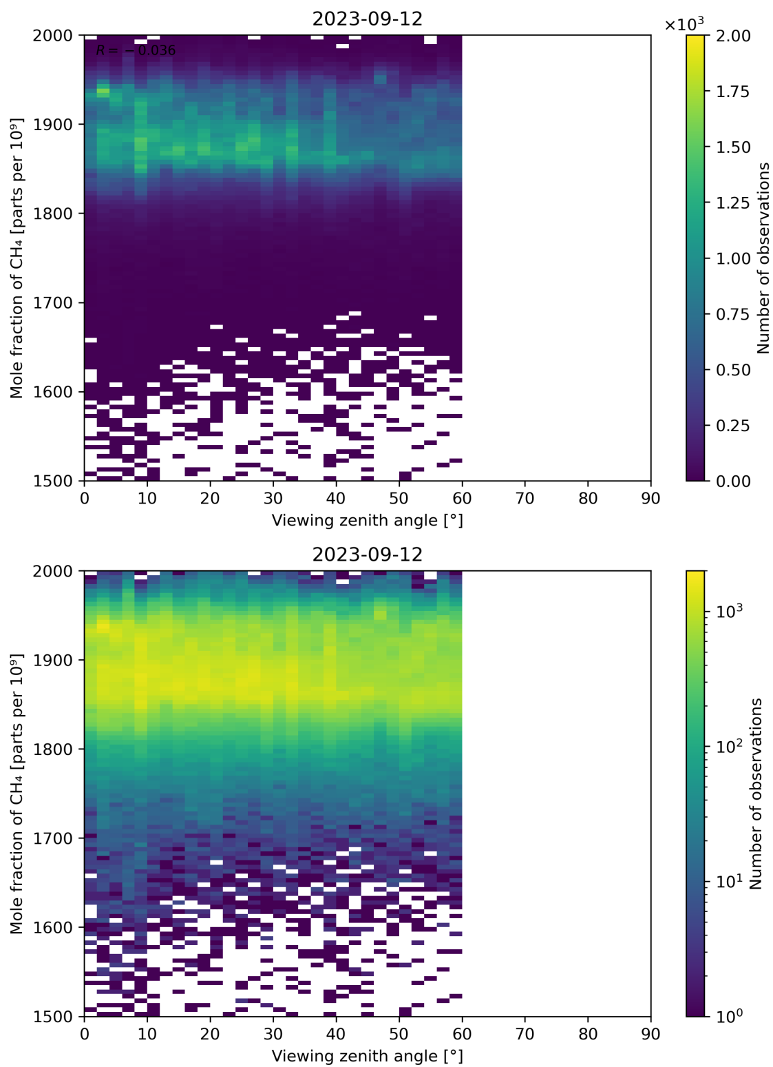
Figure 110: Scatter density plot of “Viewing zenith angle” against “Mole fraction of CH 4 ” for 2023-09-11 to 2023-09-13.
