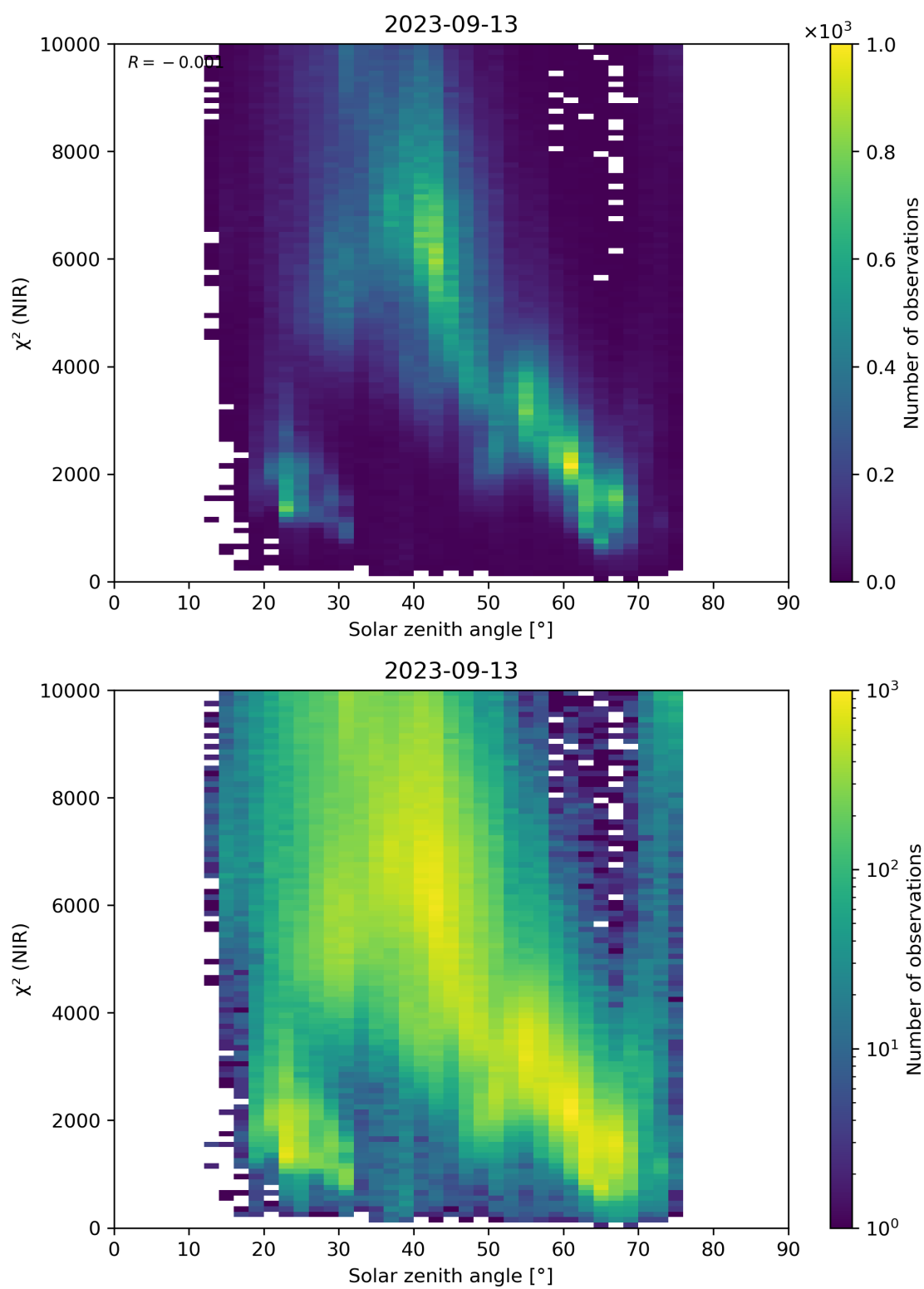
Figure 94: Scatter density plot of “Solar zenith angle” against “ \chi^2 (NIR)” for 2023-09-12 to 2023-09-14.
