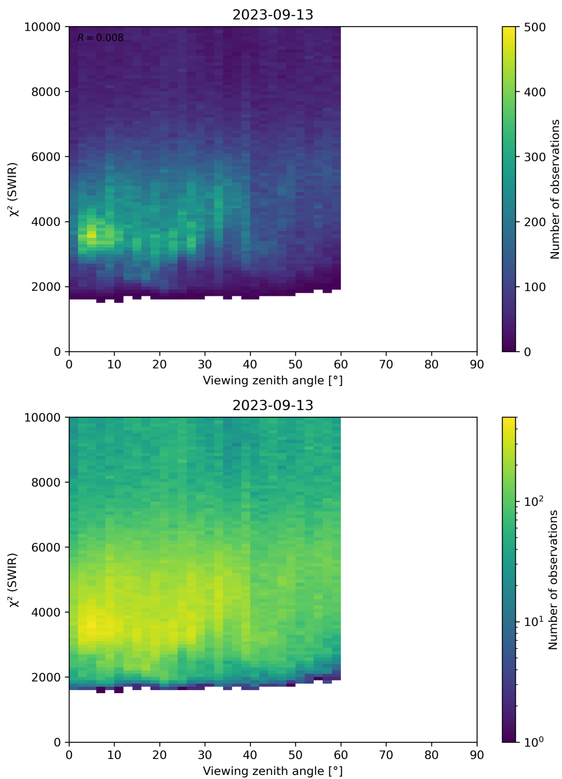
Figure 106: Scatter density plot of “Viewing zenith angle” against “ \chi^2 (SWIR)” for 2023-09-12 to 2023-09-14.
