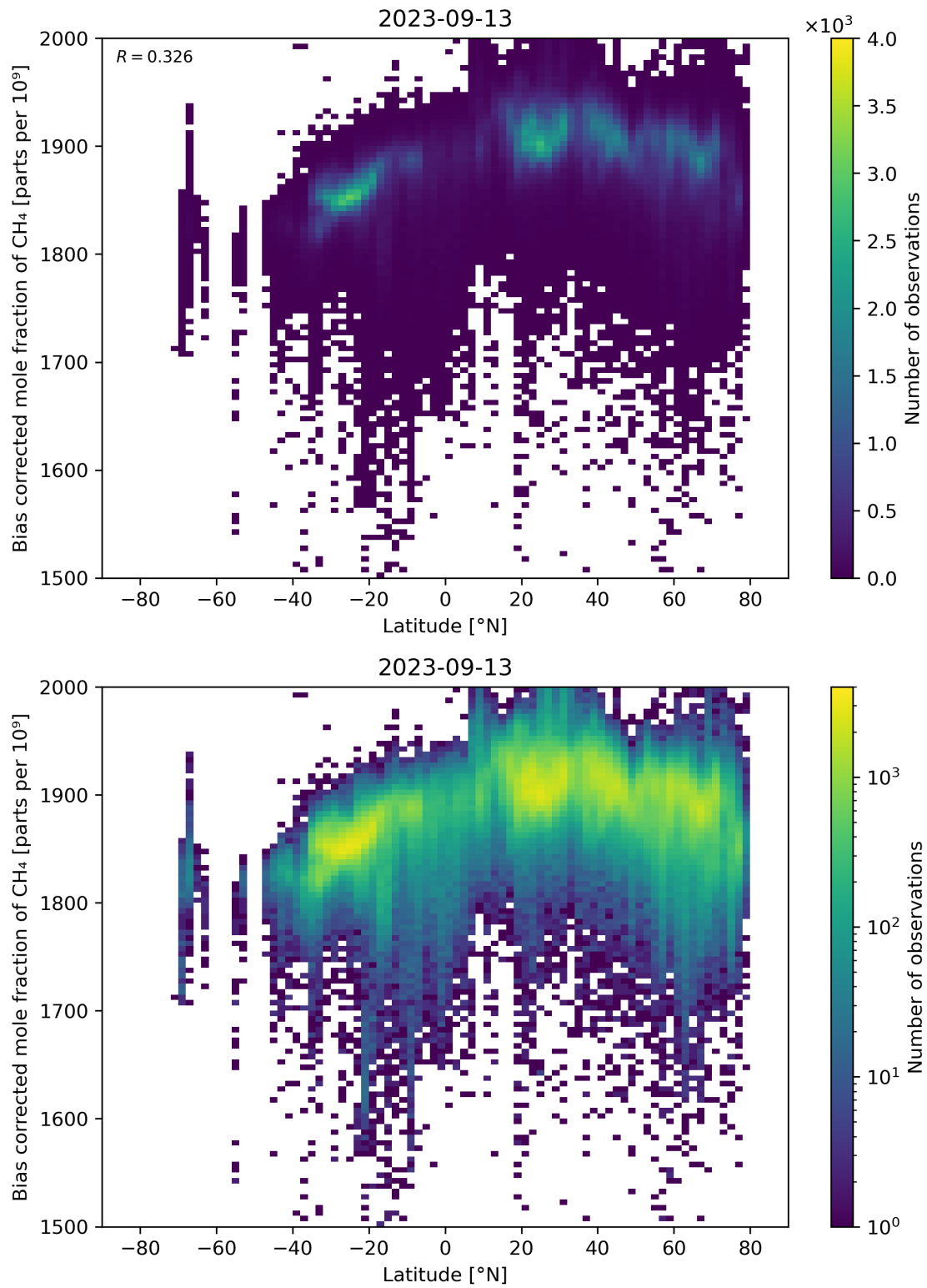
Figure 58: Scatter density plot of “Latitude” against “Bias corrected mole fraction of CH 4 ” for 2023-09-12 to 2023-09-14.
