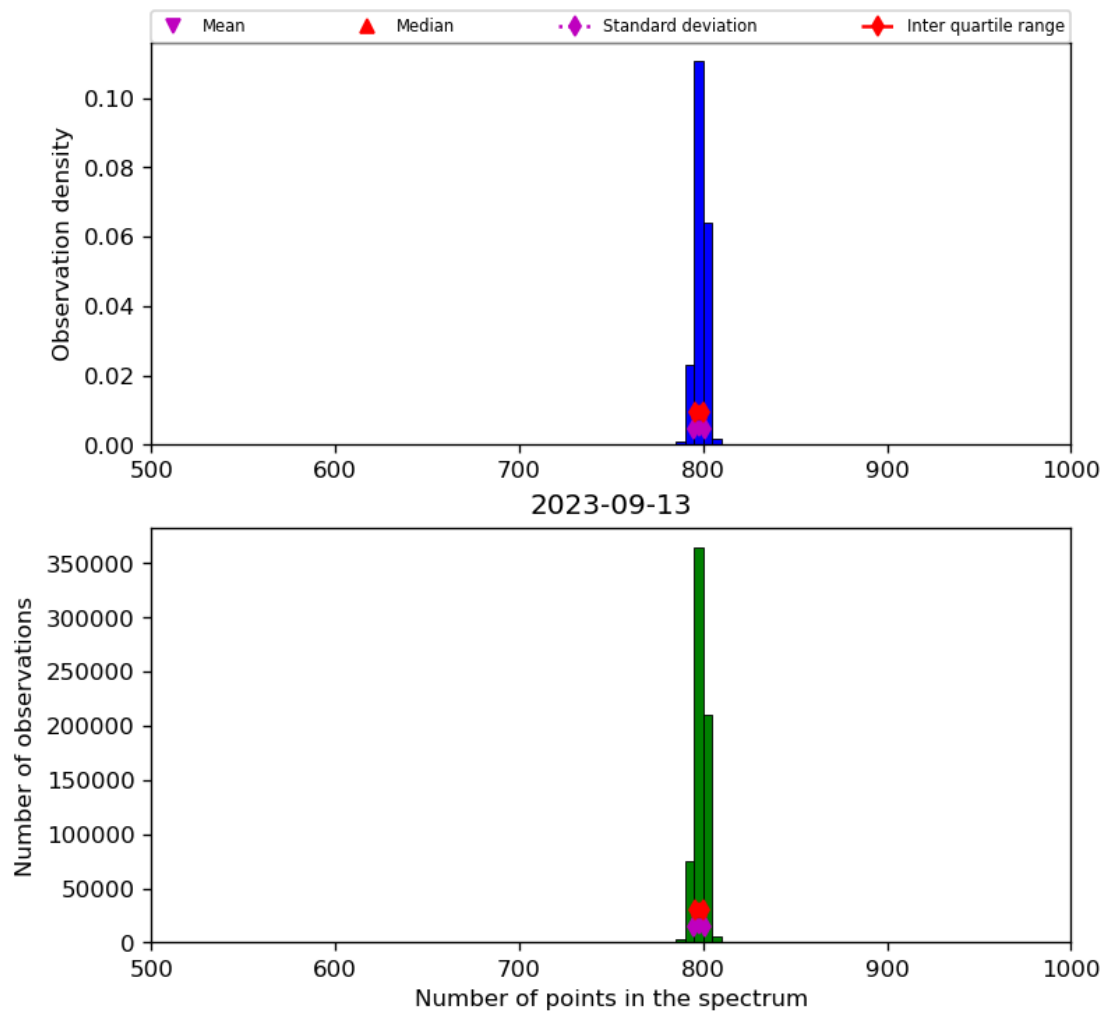
Figure 26: Histogram of “Number of points in the spectrum” for 2023-09-12 to 2023-09-14
