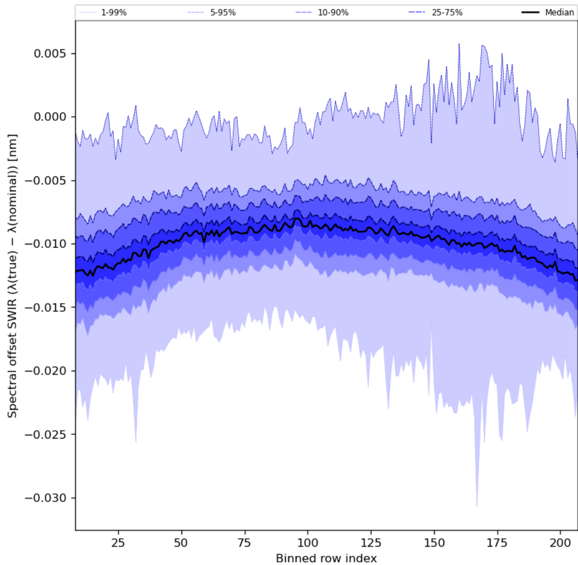
Figure 38: Along track statistics of “Spectral offset SWIR ( \lambda(\text{true}) - \lambda(\text{nominal}) )” for 2023-09-12 to 2023-09-14
