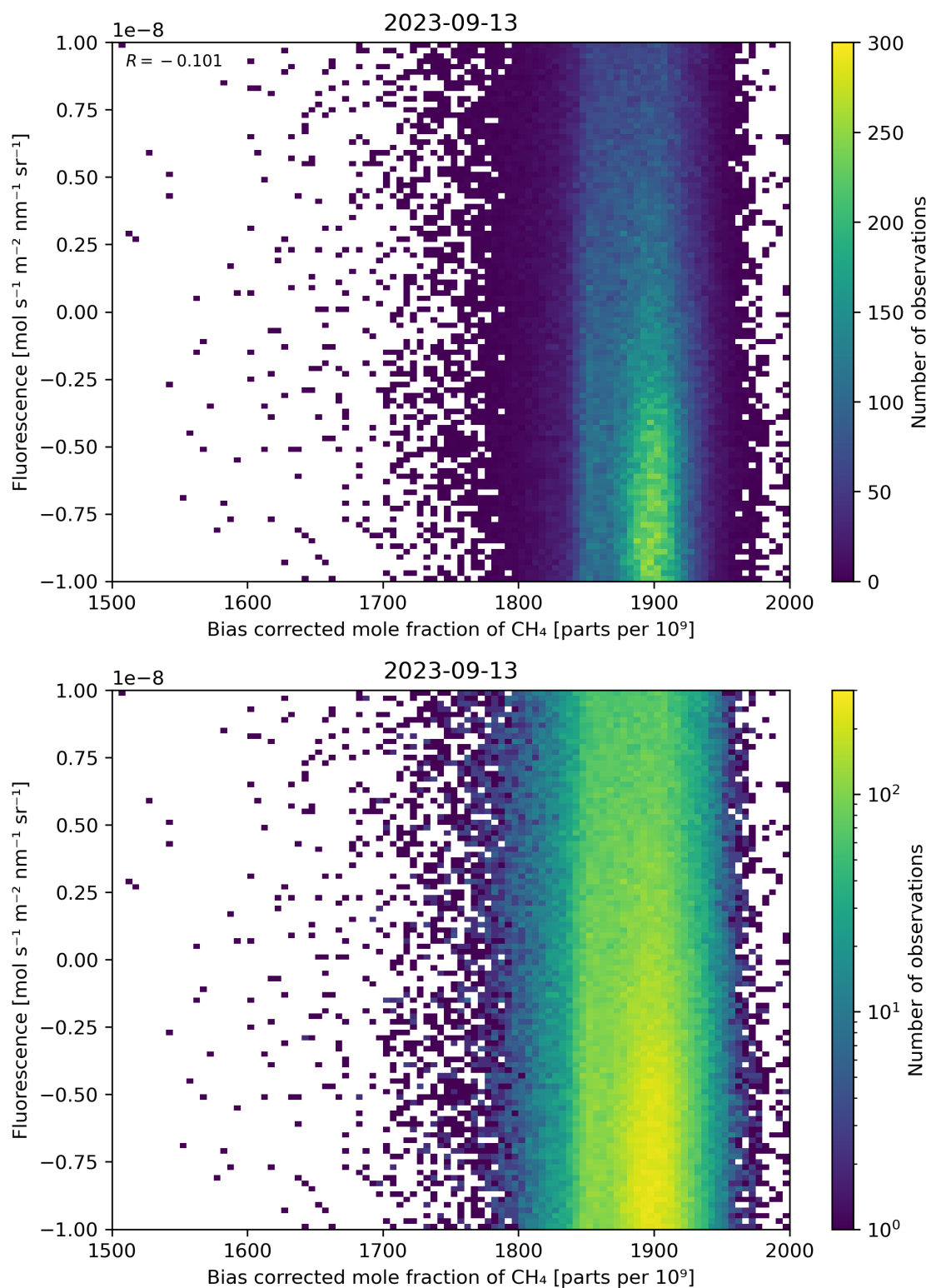
Figure 66: Scatter density plot of “Bias corrected mole fraction of \text{CH}_4 ” against “Fluorescence” for 2023-09-12 to 2023-09-14.
