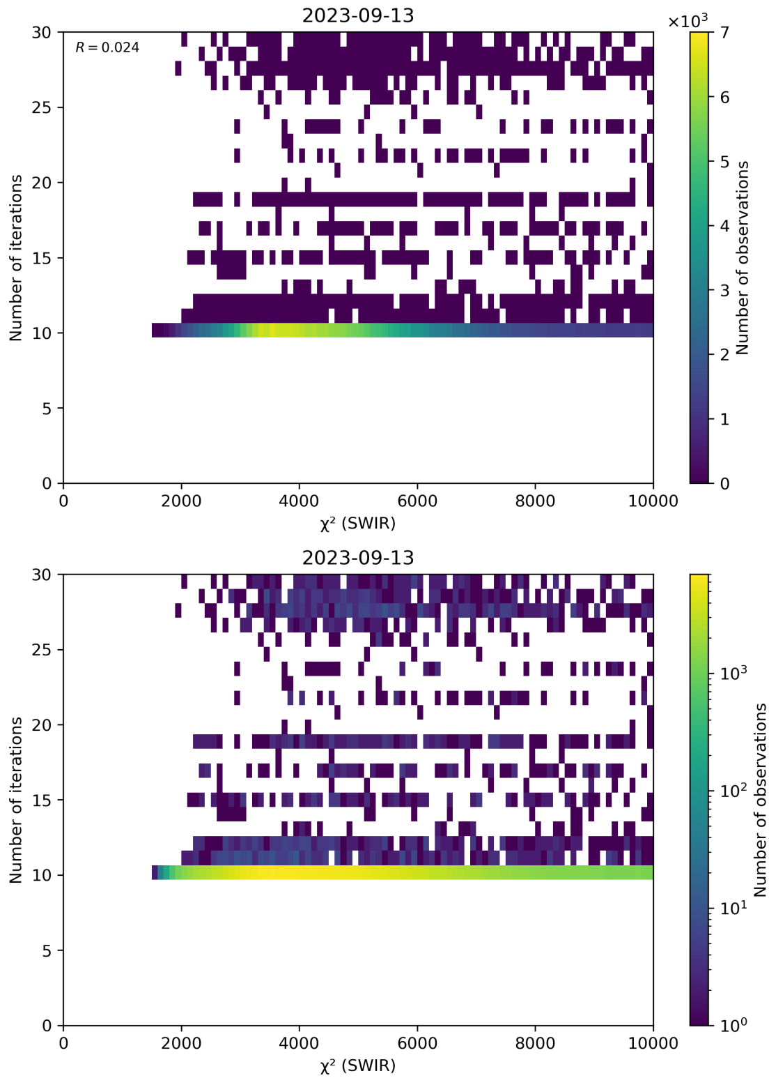
Figure 50: Scatter density plot of " \chi^2 (SWIR)" against "Number of iterations" for 2023-09-12 to 2023-09-14.
