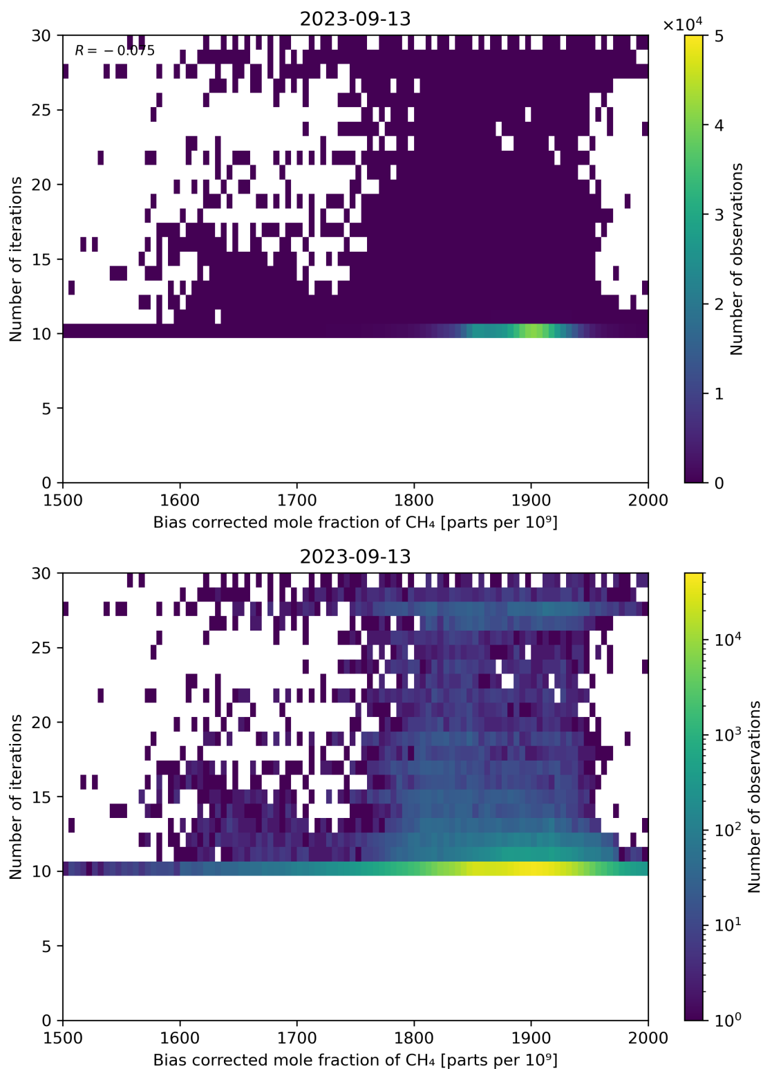
Figure 67: Scatter density plot of “Bias corrected mole fraction of CH 4 ” against “Number of iterations” for 2023-09-12 to 2023-09-14.
