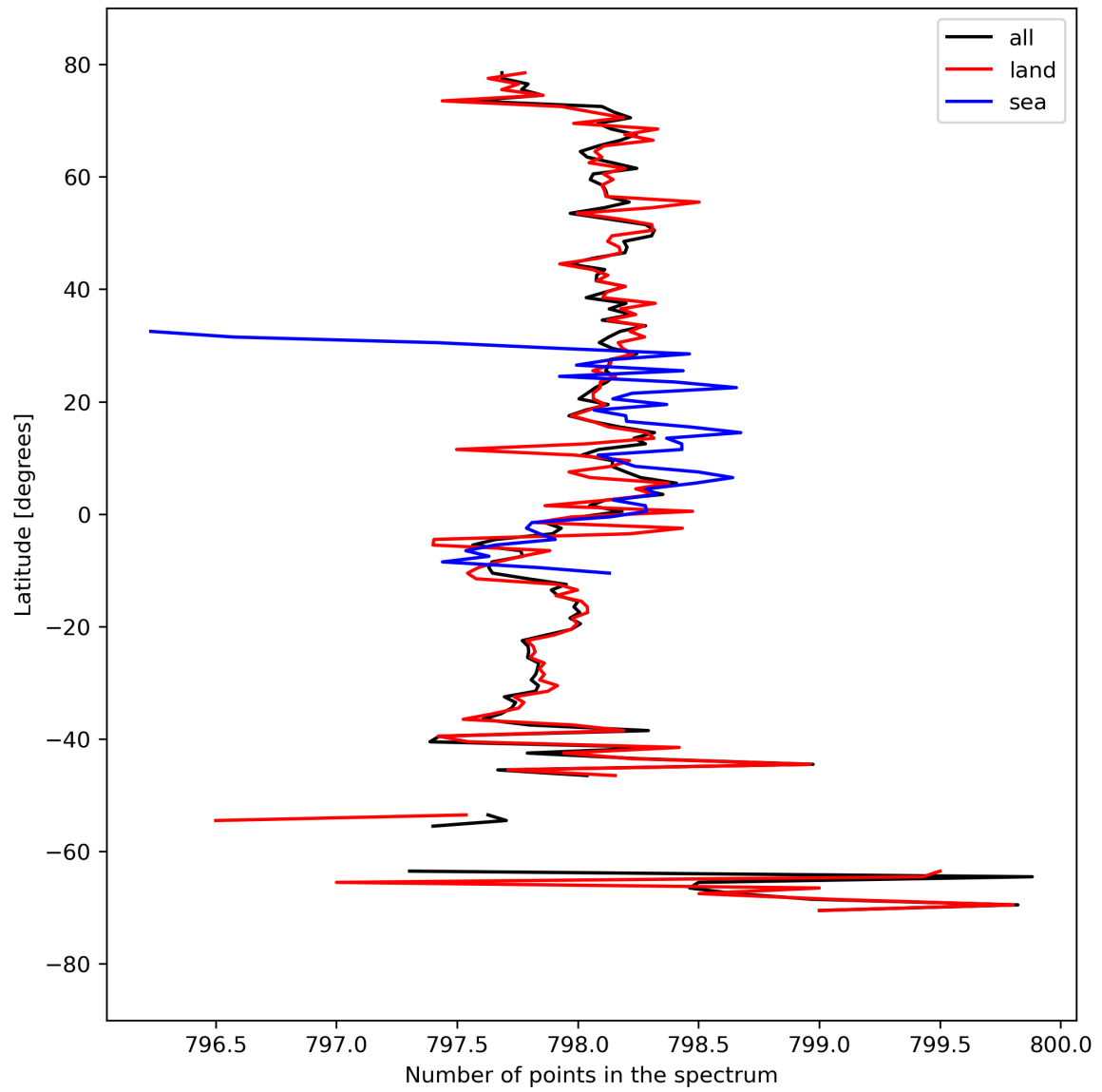
Figure 15: Zonal average of “Number of points in the spectrum” for 2023-09-12 to 2023-09-14.
