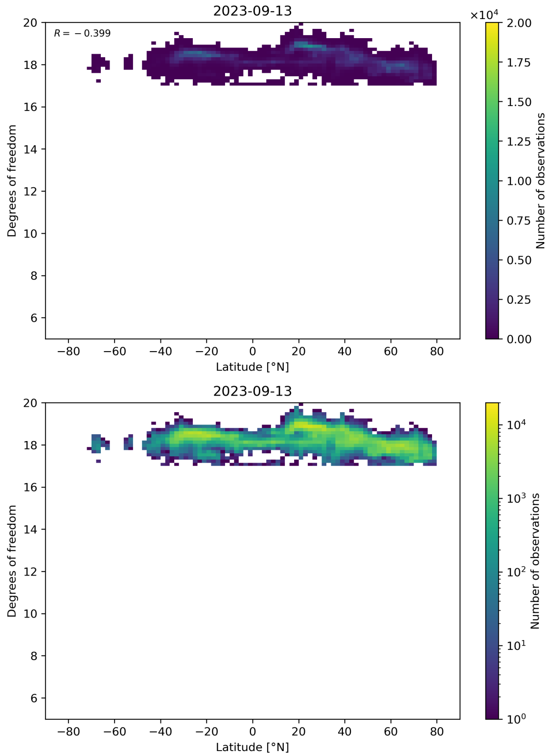
Figure 55: Scatter density plot of “Latitude” against “Degrees of freedom” for 2023-09-12 to 2023-09-14.
