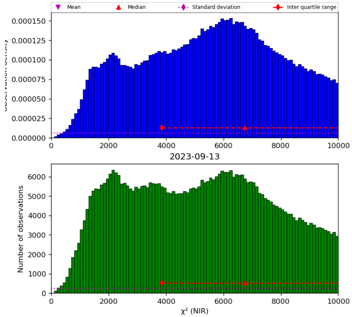
Figure 29: Histogram of “ \chi^2 (NIR)” for 2023-09-12 to 2023-09-14
