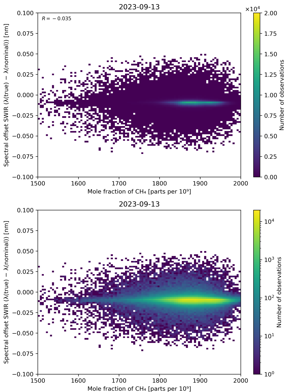
Figure 86: Scatter density plot of “Mole fraction of CH 4 ” against “Spectral offset SWIR ( \lambda(\text{true}) - \lambda(\text{nominal}) )” for 2023-09-12 to 2023-09-14.
