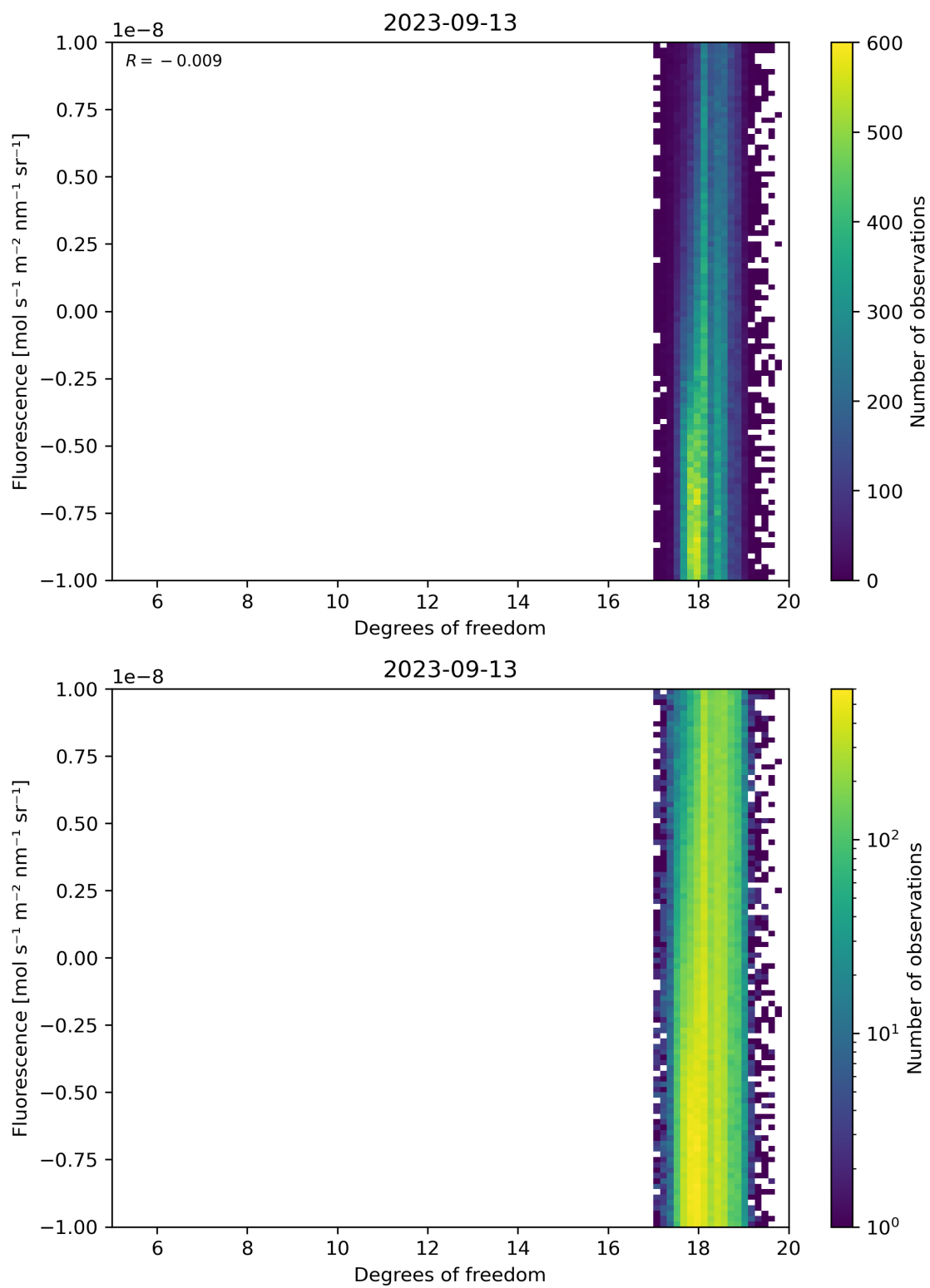
Figure 51: Scatter density plot of “Degrees of freedom” against “Fluorescence” for 2023-09-12 to 2023-09-14.
