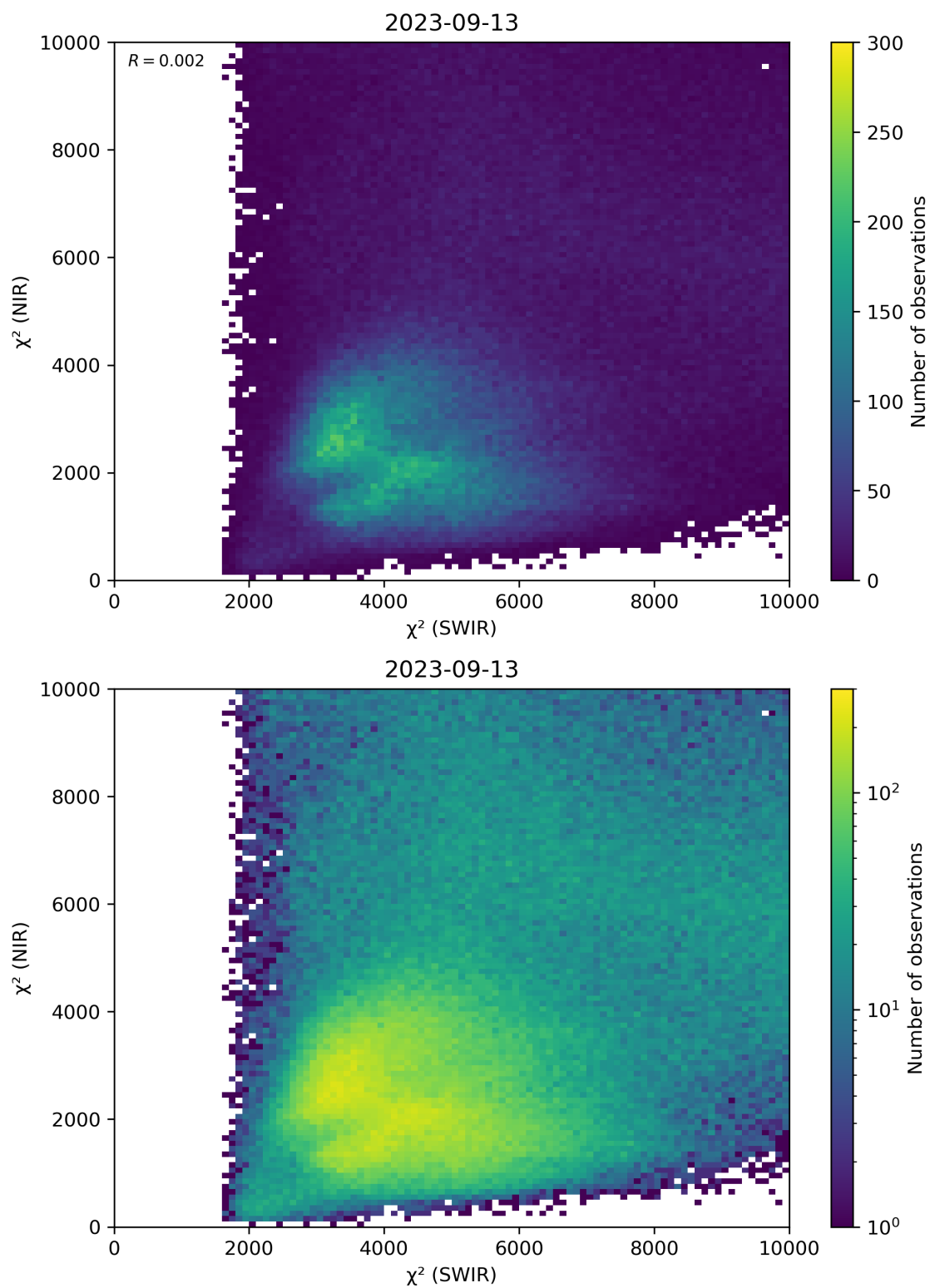
Figure 47: Scatter density plot of “ \chi^2 (SWIR)” against “ \chi^2 (NIR)” for 2023-09-12 to 2023-09-14.
