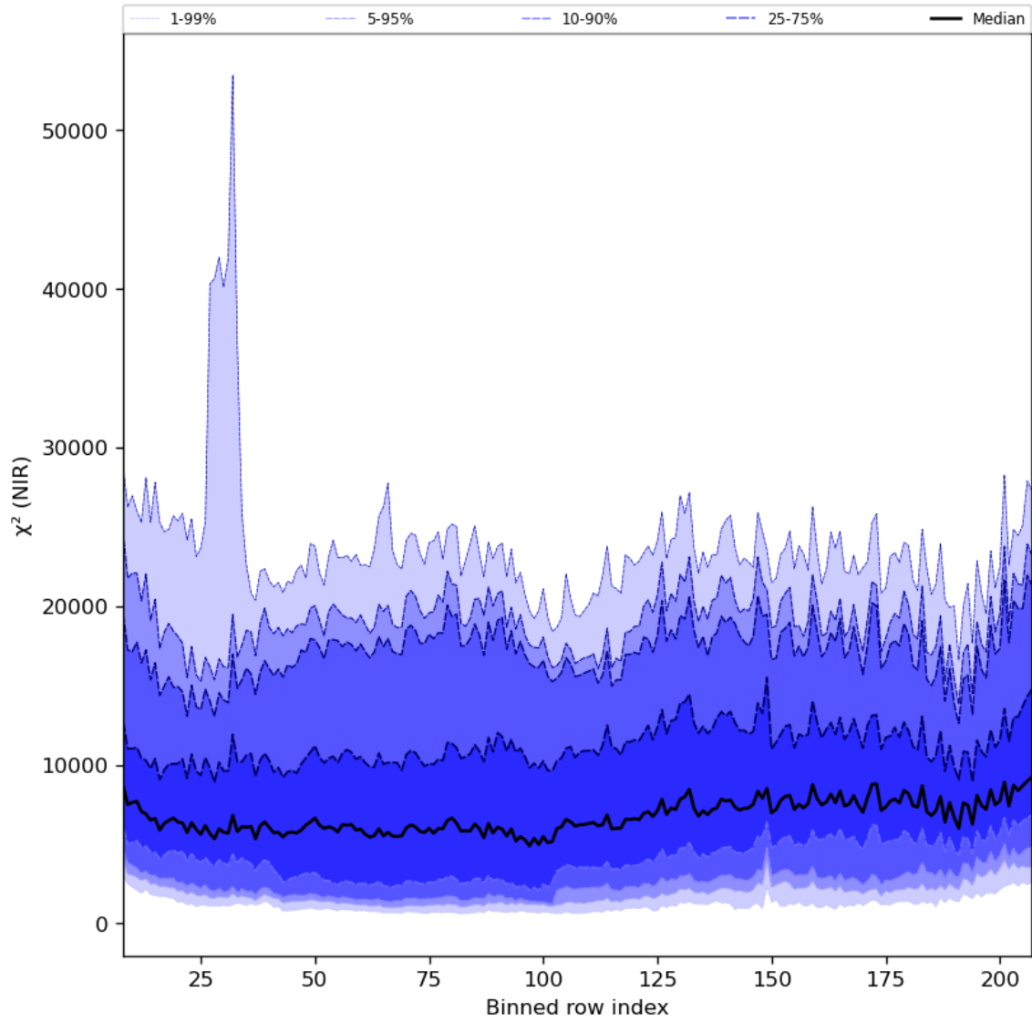
Figure 40: Along track statistics of “ \chi^2 (NIR)” for 2023-09-12 to 2023-09-14
