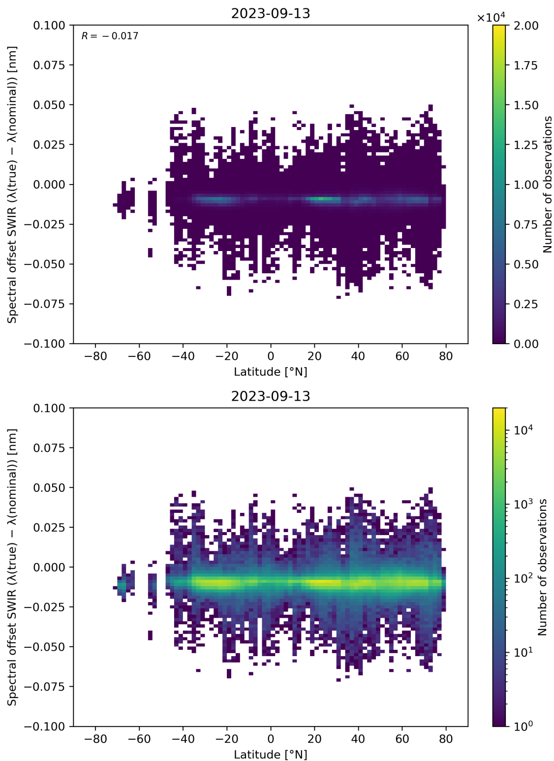
Figure 62: Scatter density plot of “Latitude” against “Spectral offset SWIR ( \lambda(\text{true}) - \lambda(\text{nominal}) )” for 2023-09-12 to 2023-09-14.
