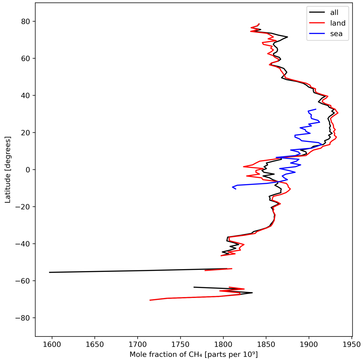
Figure 12: Zonal average of “Mole fraction of \text{CH}_4 ” for 2023-09-12 to 2023-09-14.
