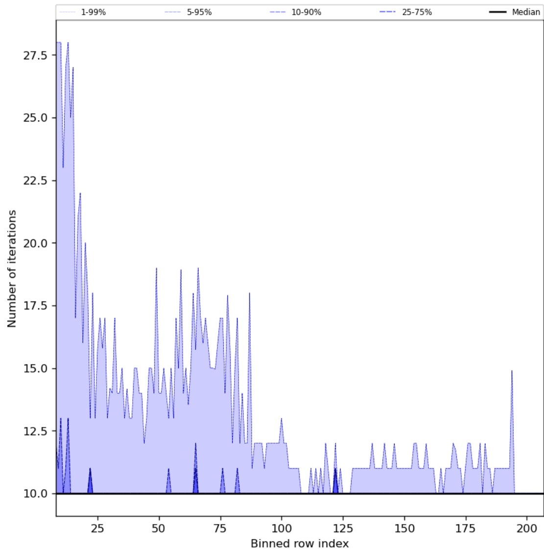
Figure 42: Along track statistics of “Number of iterations” for 2023-09-12 to 2023-09-14
