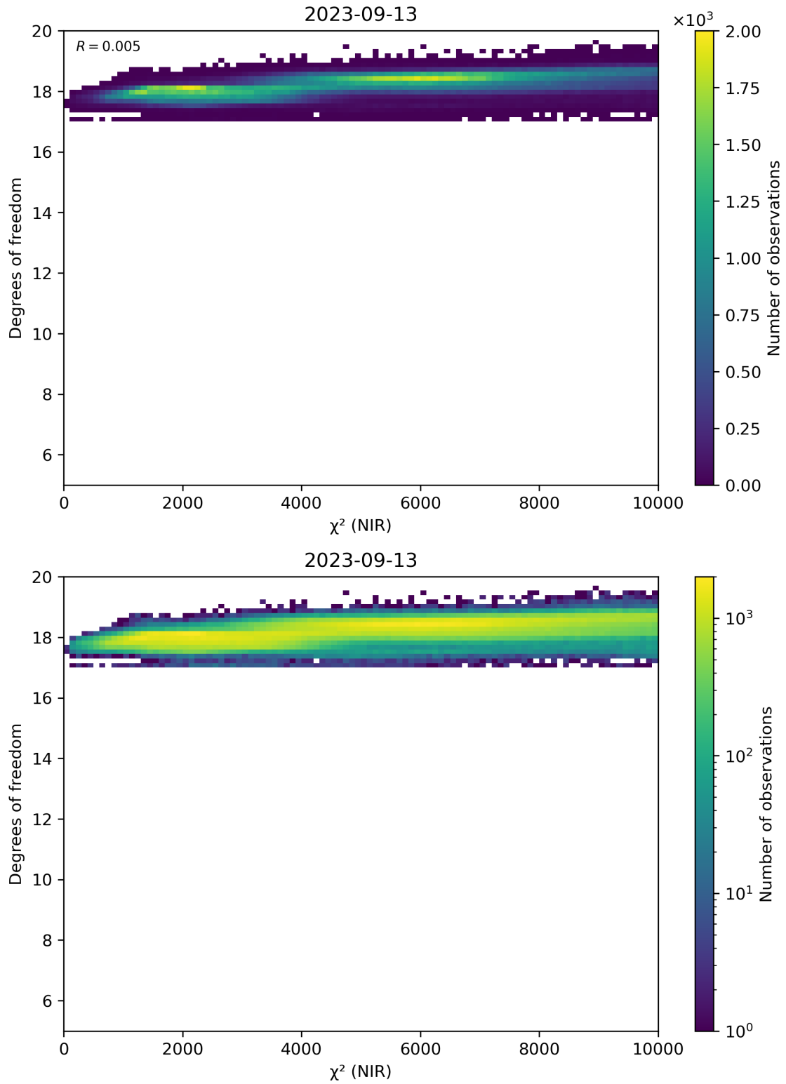
Figure 44: Scatter density plot of “ \chi^2 (NIR)” against “Degrees of freedom” for 2023-09-12 to 2023-09-14.
