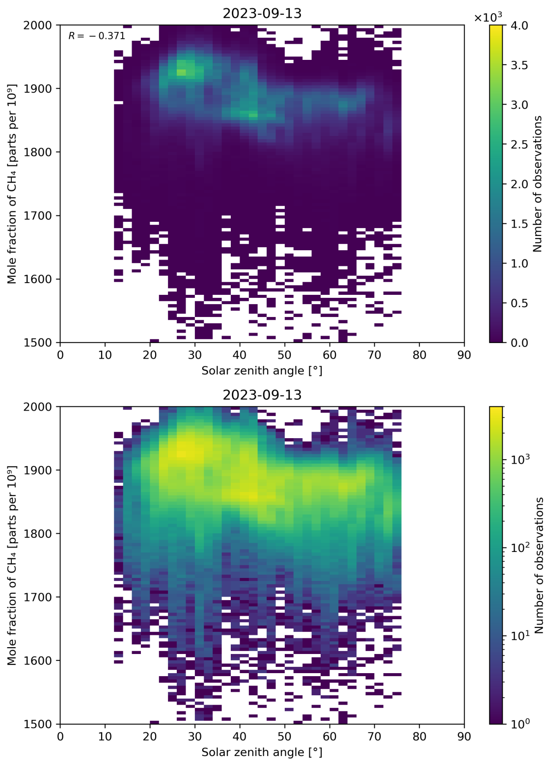
Figure 99: Scatter density plot of “Solar zenith angle” against “Mole fraction of CH 4 ” for 2023-09-12 to 2023-09-14.
