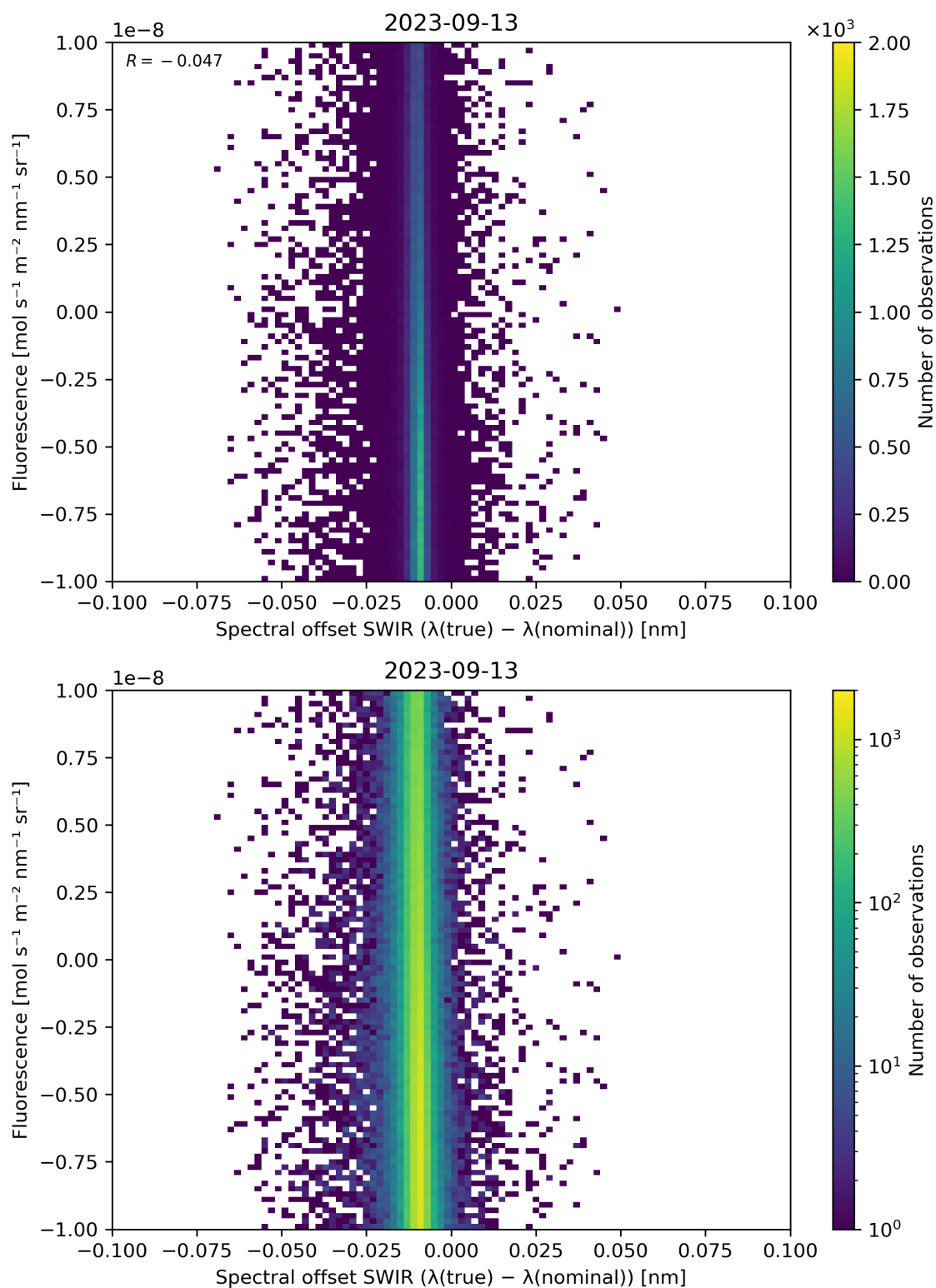
Figure 120: Scatter density plot of “Spectral offset SWIR ( \lambda(\text{true}) - \lambda(\text{nominal}) )” against “Fluorescence” for 2023-09-12 to 2023-09-14.
