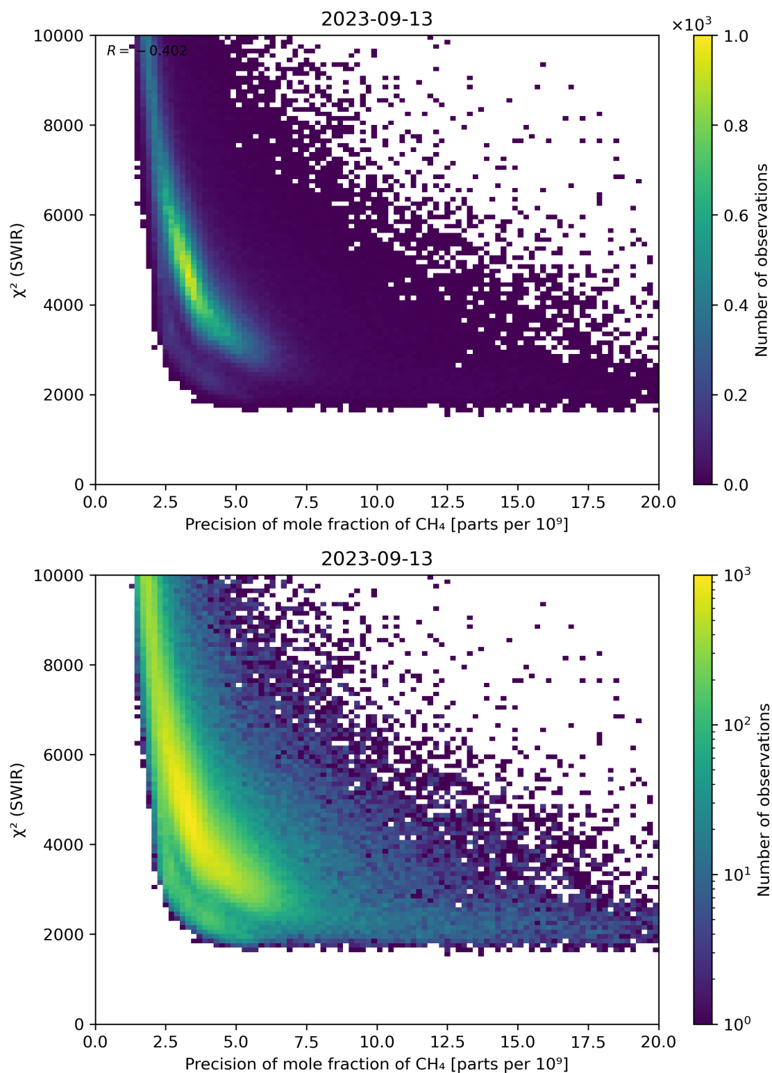
Figure 79: Scatter density plot of “Precision of mole fraction of CH 4 ” against “ \chi^2 (SWIR)” for 2023-09-12 to 2023-09-14.
