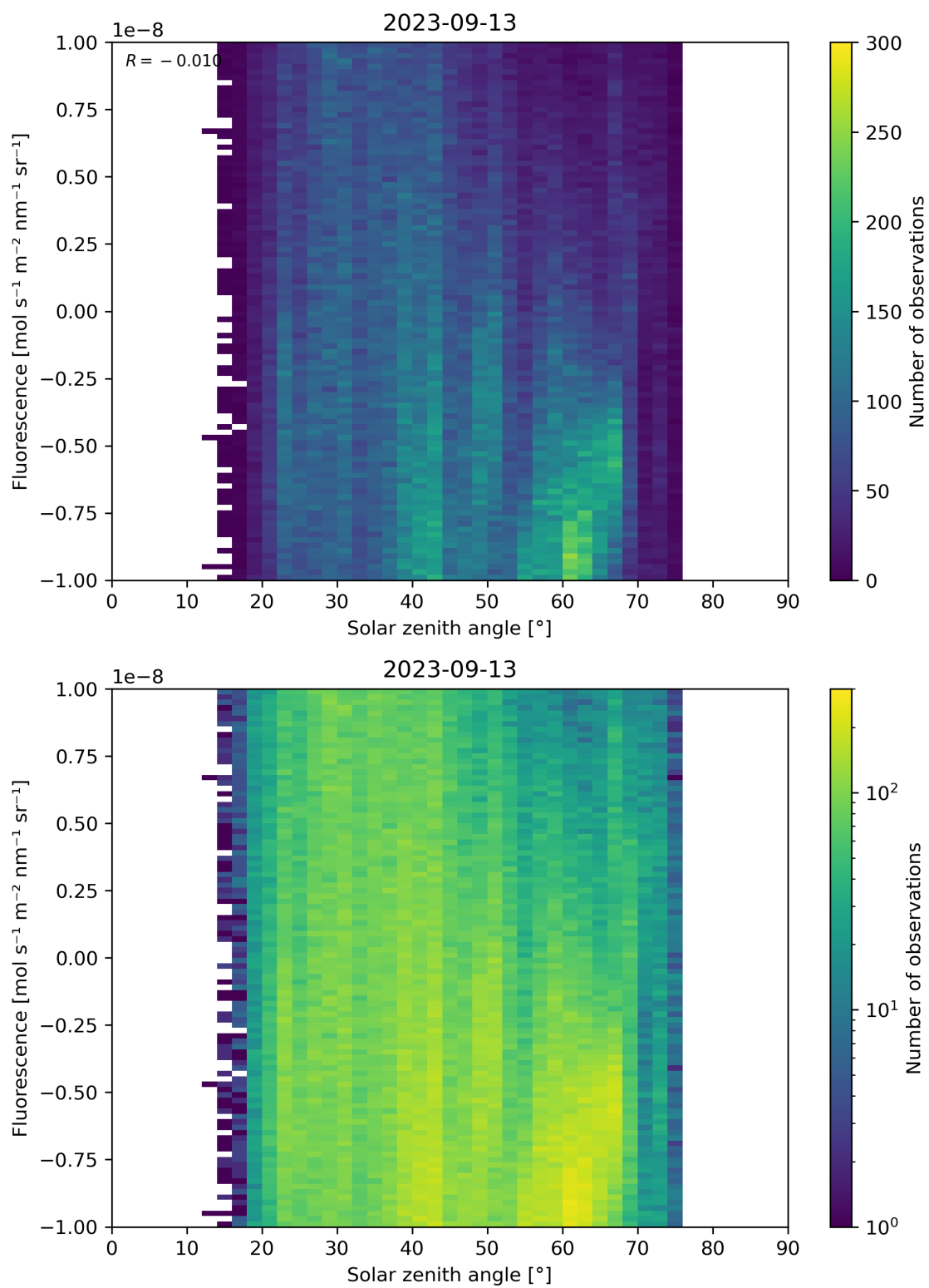
Figure 97: Scatter density plot of “Solar zenith angle” against “Fluorescence” for 2023-09-12 to 2023-09-14.
