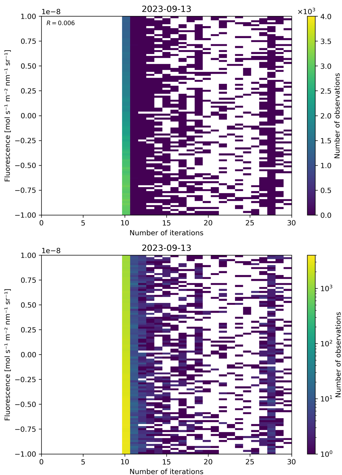
Figure 87: Scatter density plot of “Number of iterations” against “Fluorescence” for 2023-09-12 to 2023-09-14.
