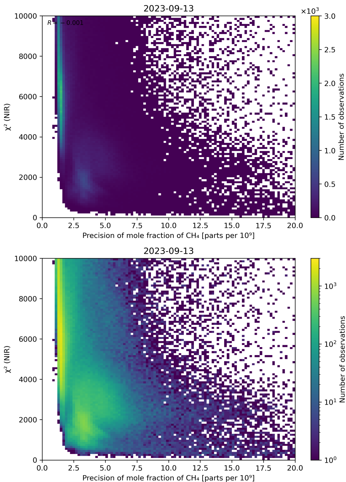
Figure 78: Scatter density plot of “Precision of mole fraction of CH 4 ” against “ \chi^2 (NIR)” for 2023-09-12 to 2023-09-14.
