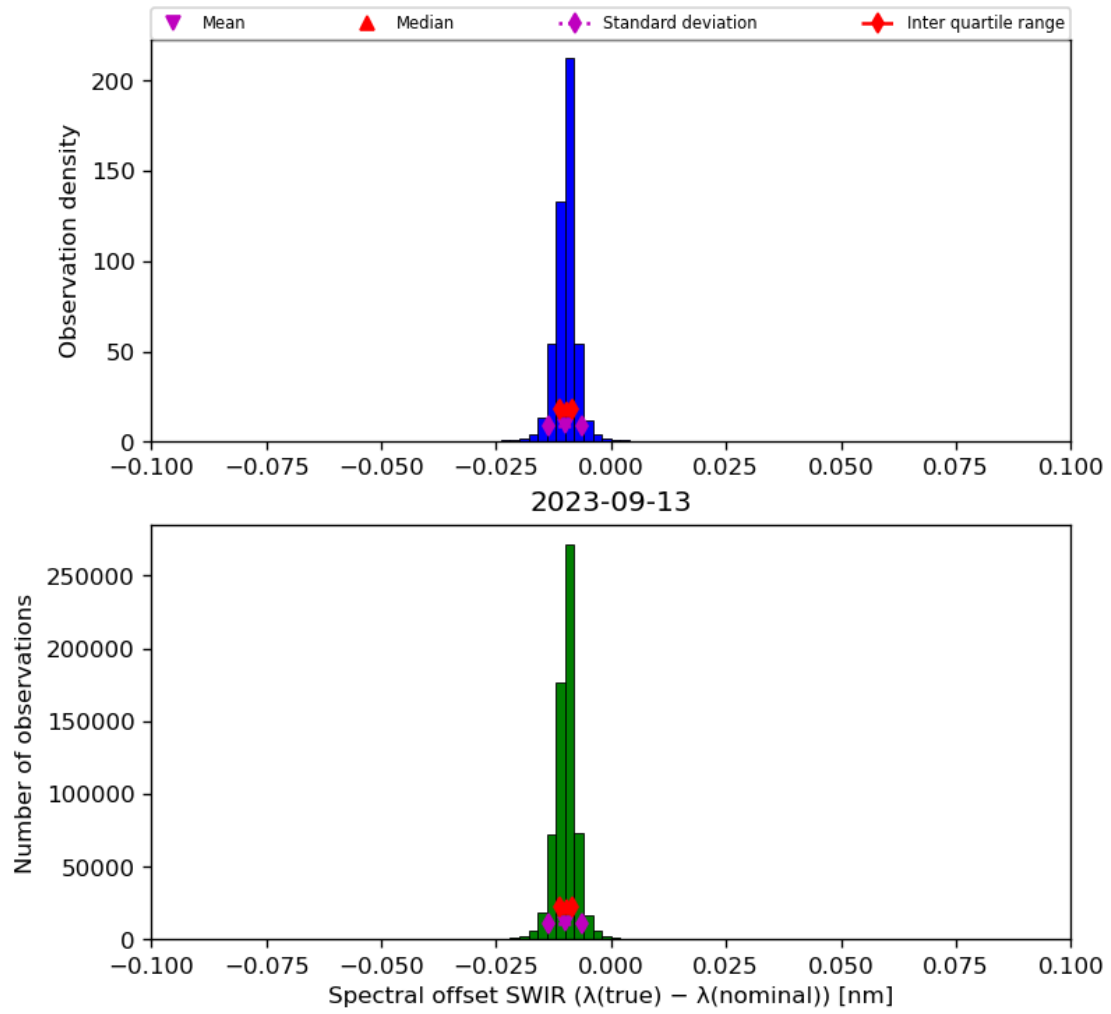
Figure 27: Histogram of “Spectral offset SWIR ( \lambda(\text{true}) - \lambda(\text{nominal}) )” for 2023-09-12 to 2023-09-14
