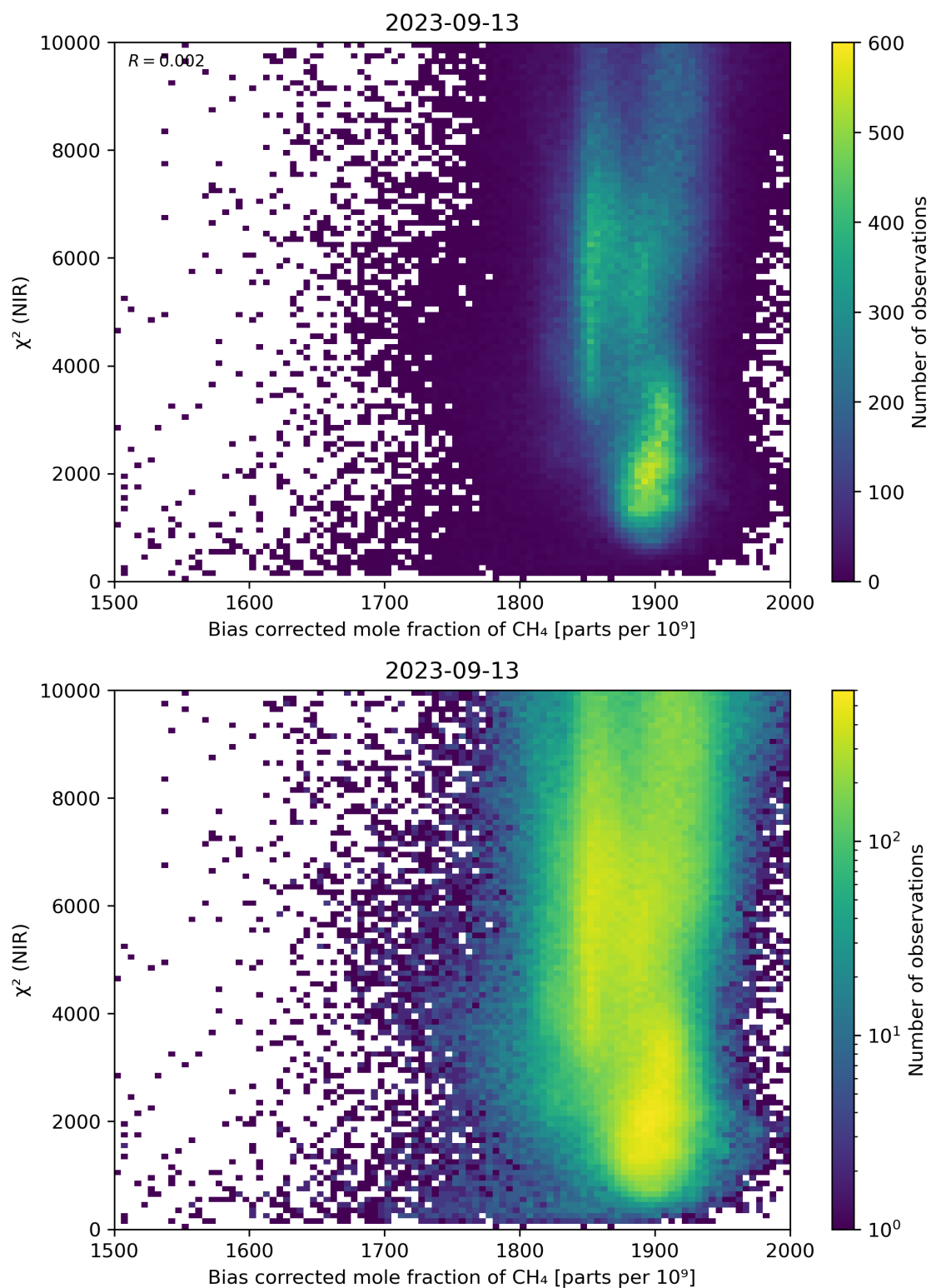
Figure 63: Scatter density plot of “Bias corrected mole fraction of \text{CH}_4 ” against “ \chi^2 (NIR)” for 2023-09-12 to 2023-09-14.
