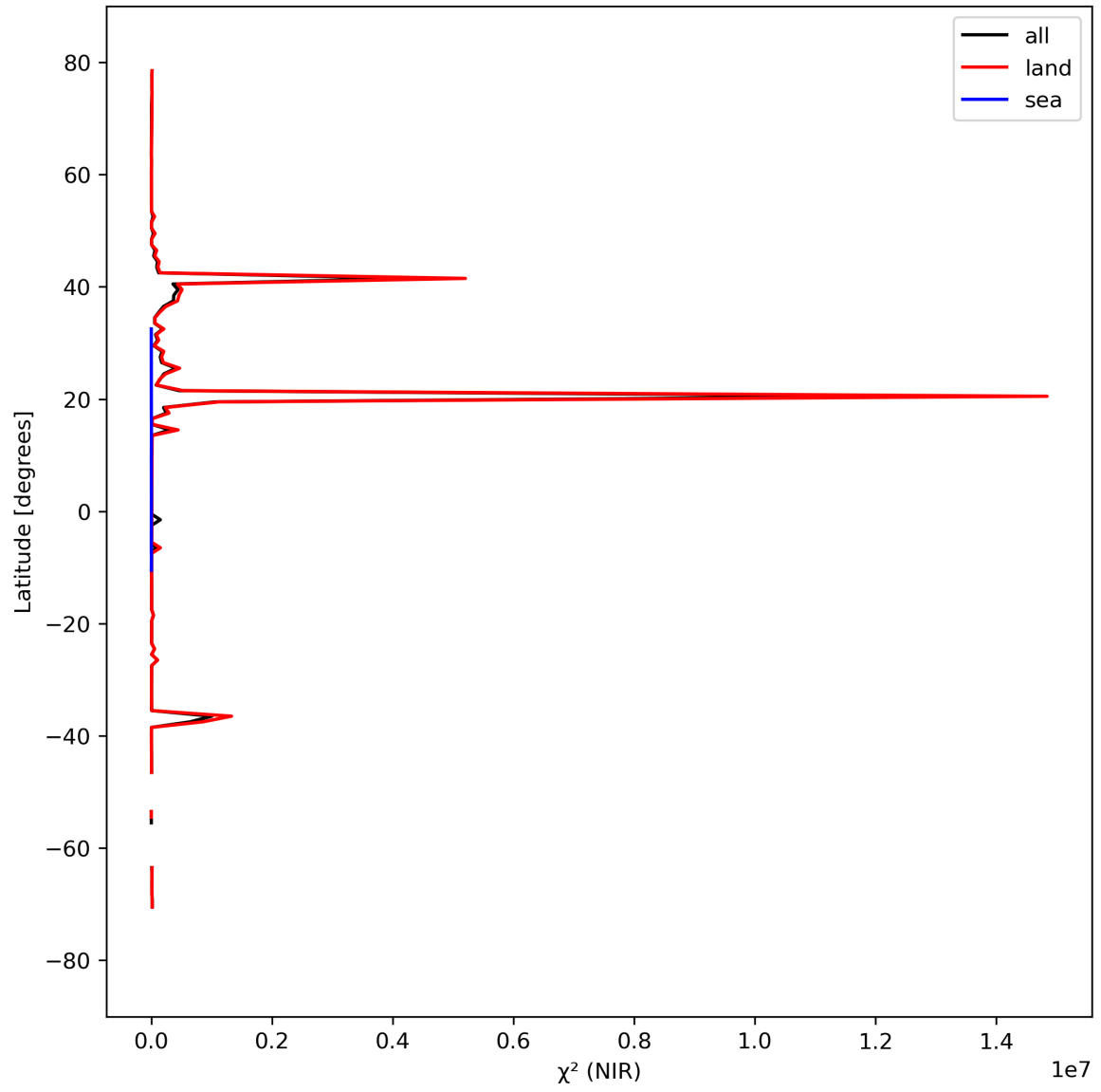
Figure 18: Zonal average of “ \chi^2 (NIR)” for 2023-09-12 to 2023-09-14.
