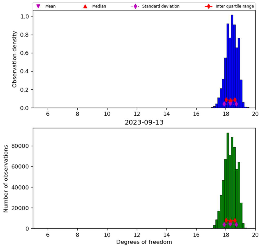
Figure 30: Histogram of “Degrees of freedom” for 2023-09-12 to 2023-09-14
