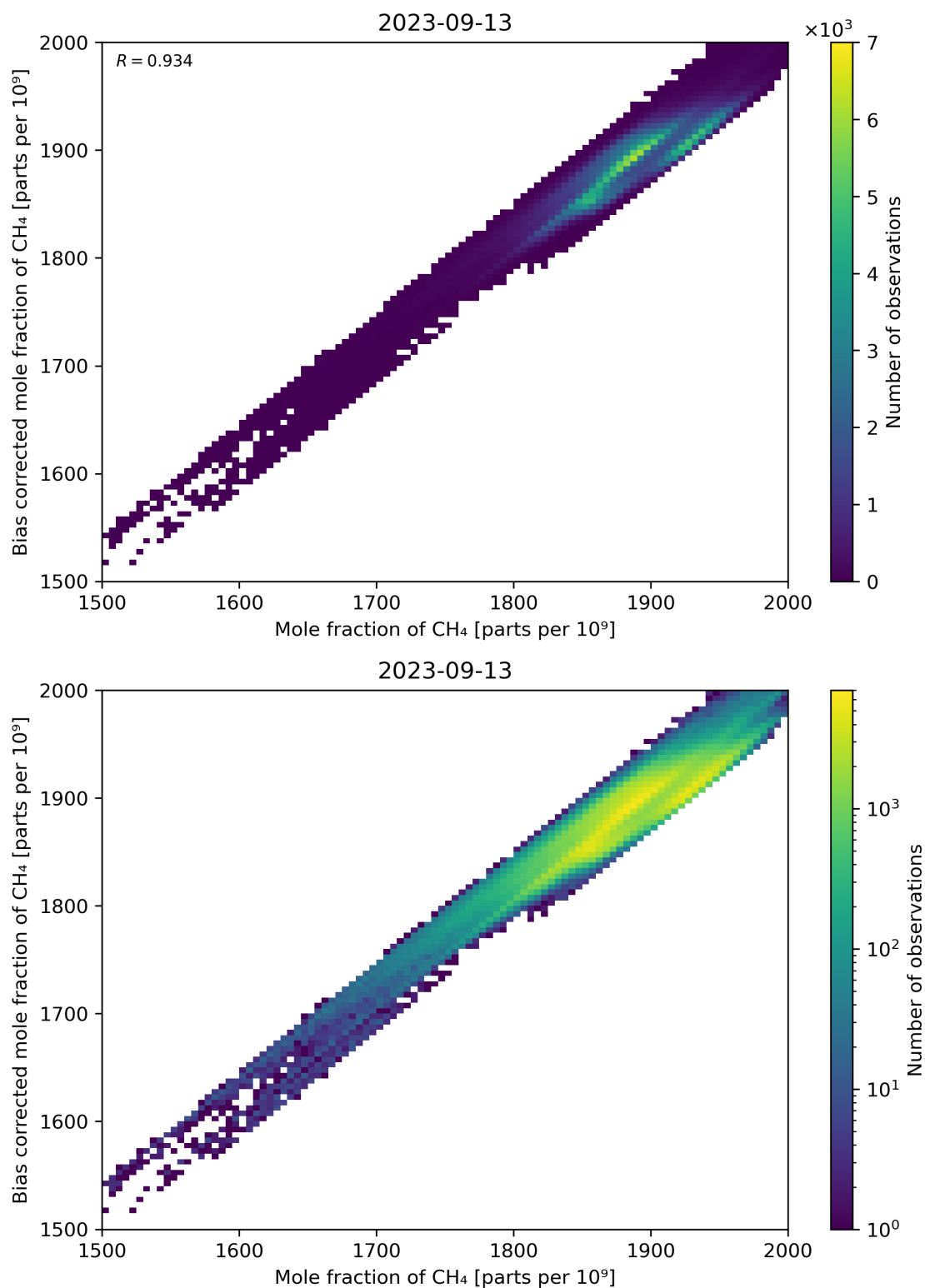
Figure 74: Scatter density plot of “Mole fraction of CH 4 ” against “Bias corrected mole fraction of CH 4 ” for 2023-09-12 to 2023-09-14.
