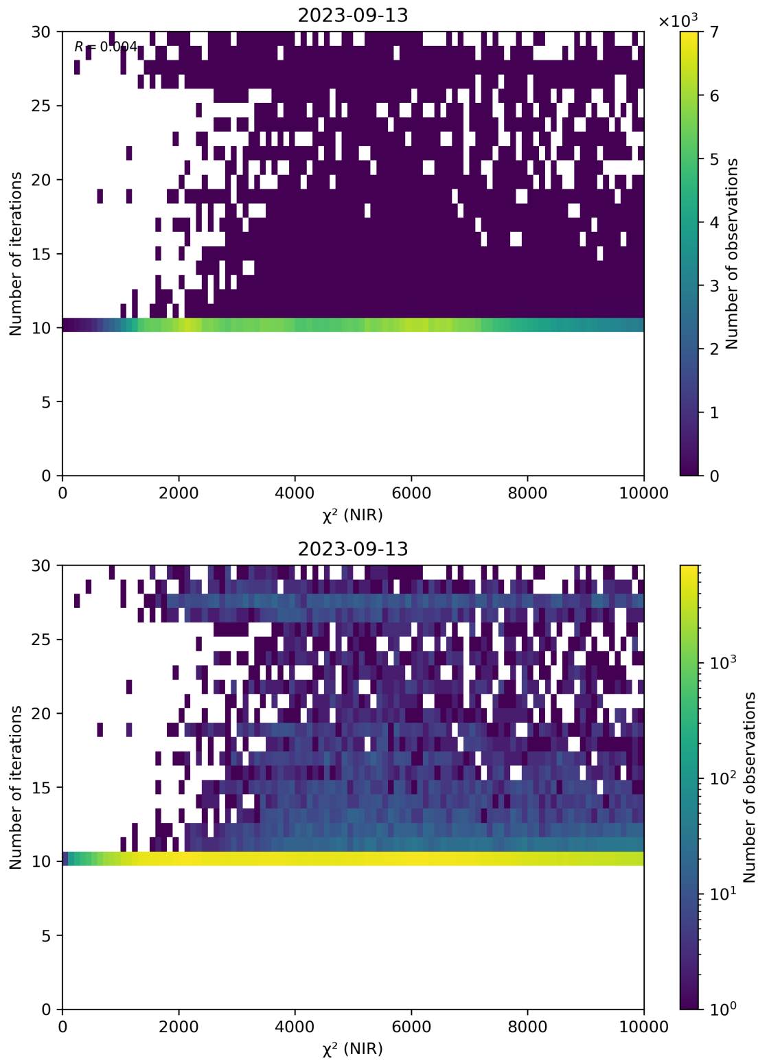
Figure 46: Scatter density plot of “ \chi^2 (NIR)” against “Number of iterations” for 2023-09-12 to 2023-09-14.
