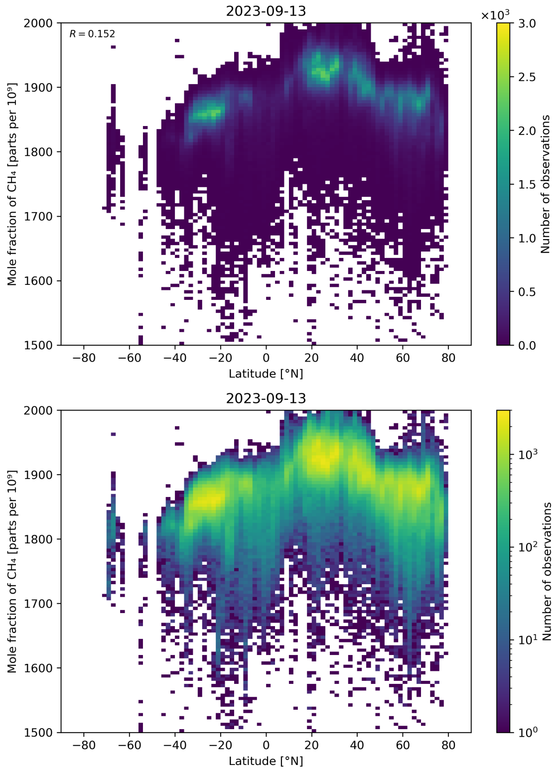
Figure 57: Scatter density plot of “Latitude” against “Mole fraction of \text{CH}_4 ” for 2023-09-12 to 2023-09-14.
