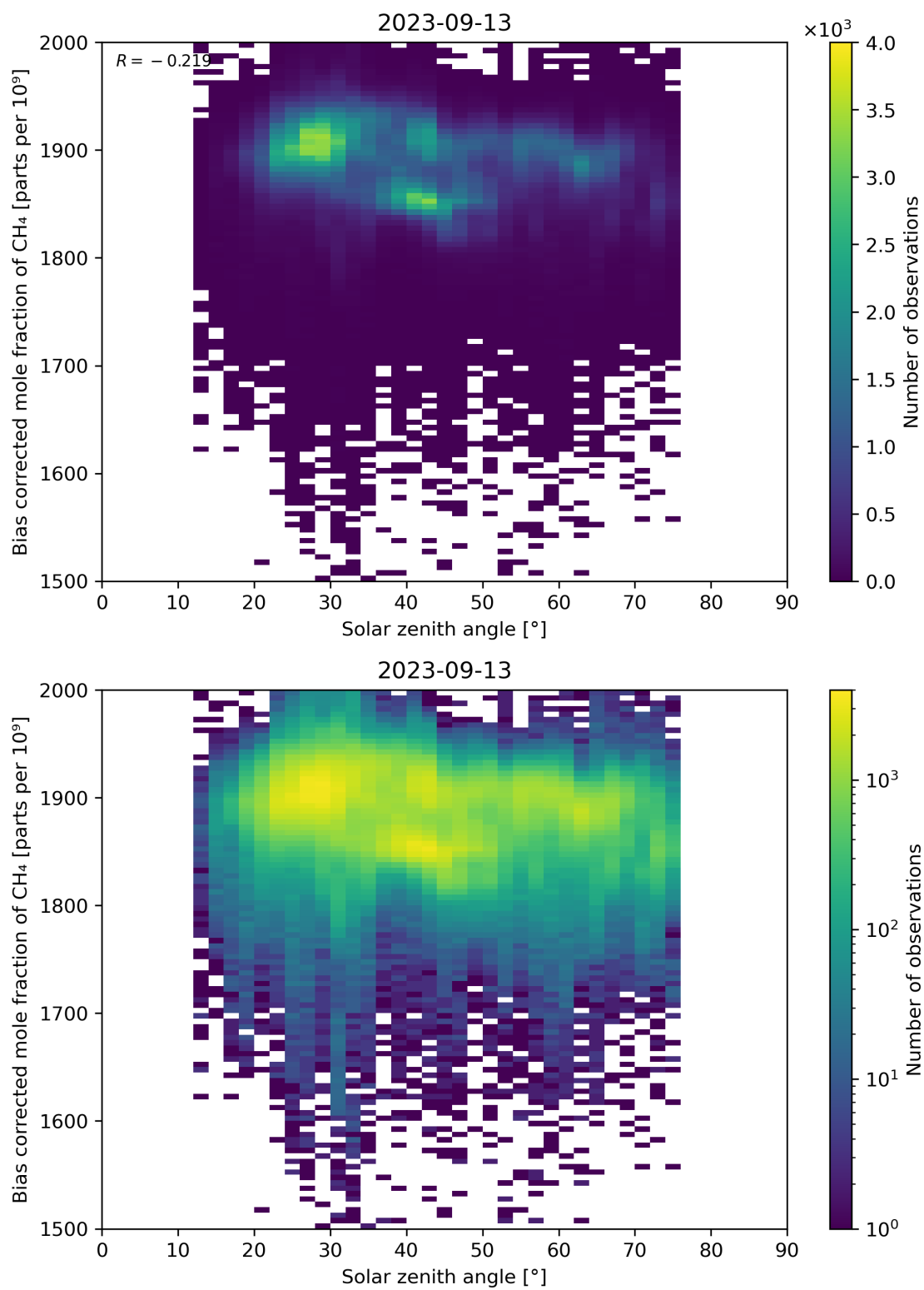
Figure 100: Scatter density plot of “Solar zenith angle” against “Bias corrected mole fraction of \text{CH}_4 ” for 2023-09-12 to 2023-09-14.
