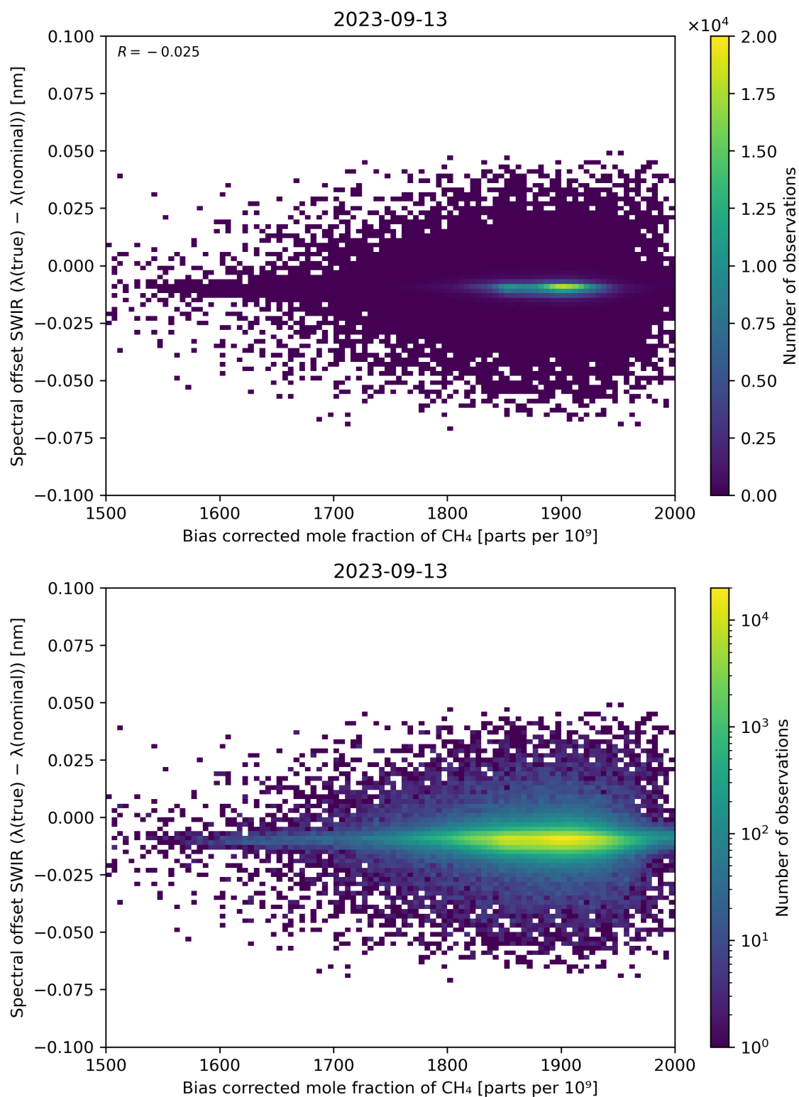
Figure 69: Scatter density plot of “Bias corrected mole fraction of \text{CH}_4 ” against “Spectral offset SWIR ( \lambda(\text{true}) - \lambda(\text{nominal}) )” for 2023-09-12 to 2023-09-14.
