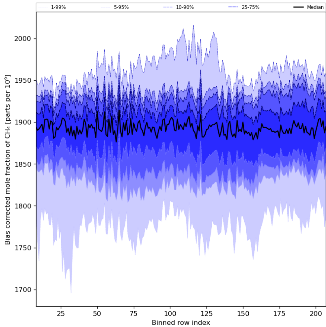
Figure 36: Along track statistics of “Bias corrected mole fraction of CH 4 ” for 2023-09-12 to 2023-09-14
