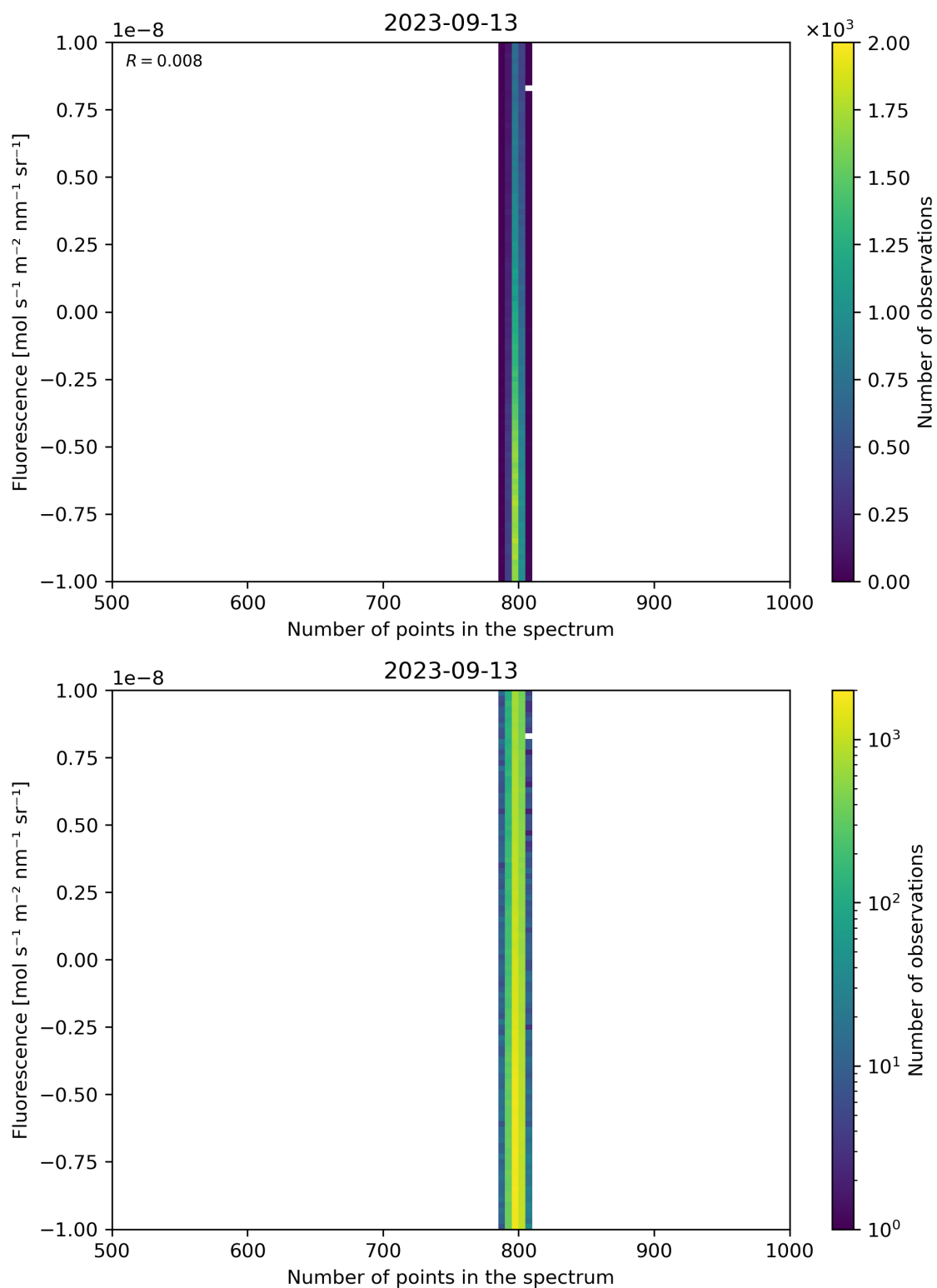
Figure 91: Scatter density plot of “Number of points in the spectrum” against “Fluorescence” for 2023-09-12 to 2023-09-14.
