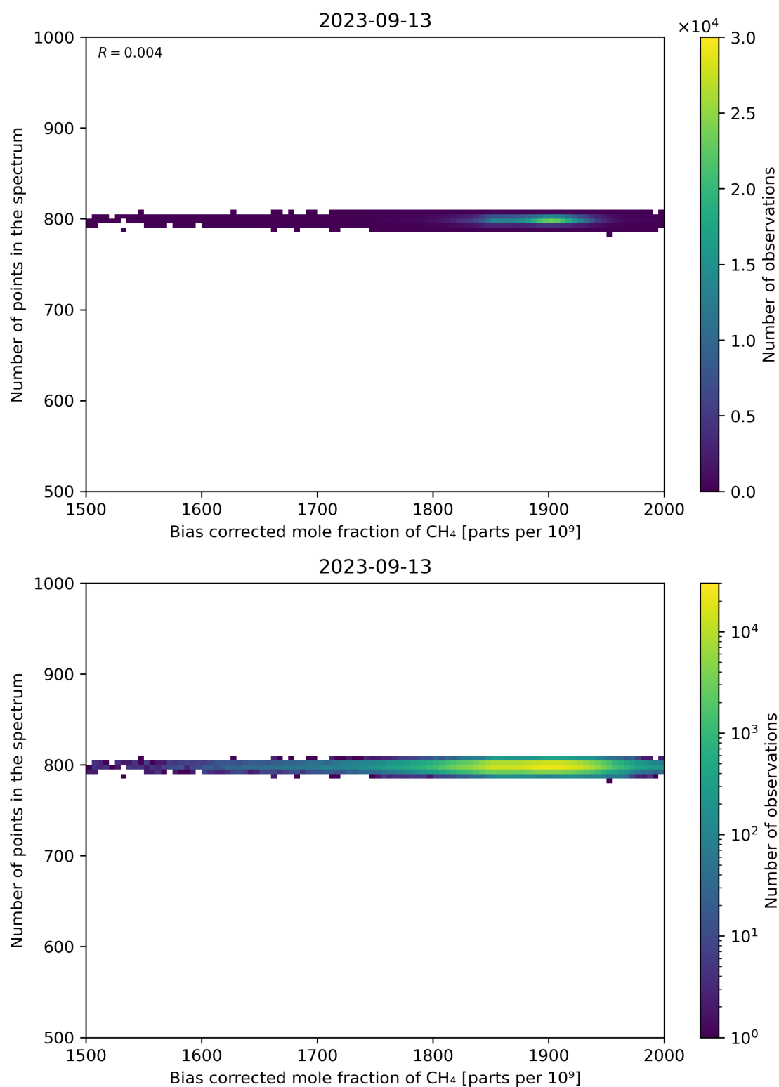
Figure 68: Scatter density plot of “Bias corrected mole fraction of CH 4 ” against “Number of points in the spectrum” for 2023-09-12 to 2023-09-14.
