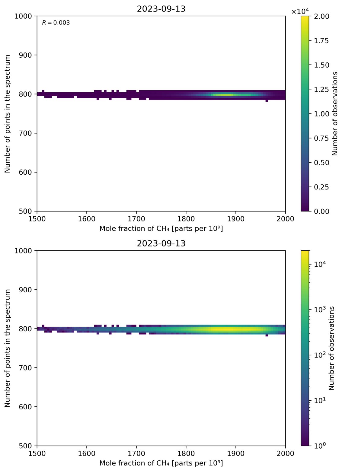
Figure 77: Scatter density plot of “Mole fraction of CH 4 ” against “Number of points in the spectrum” for 2023-09-12 to 2023-09-14.
