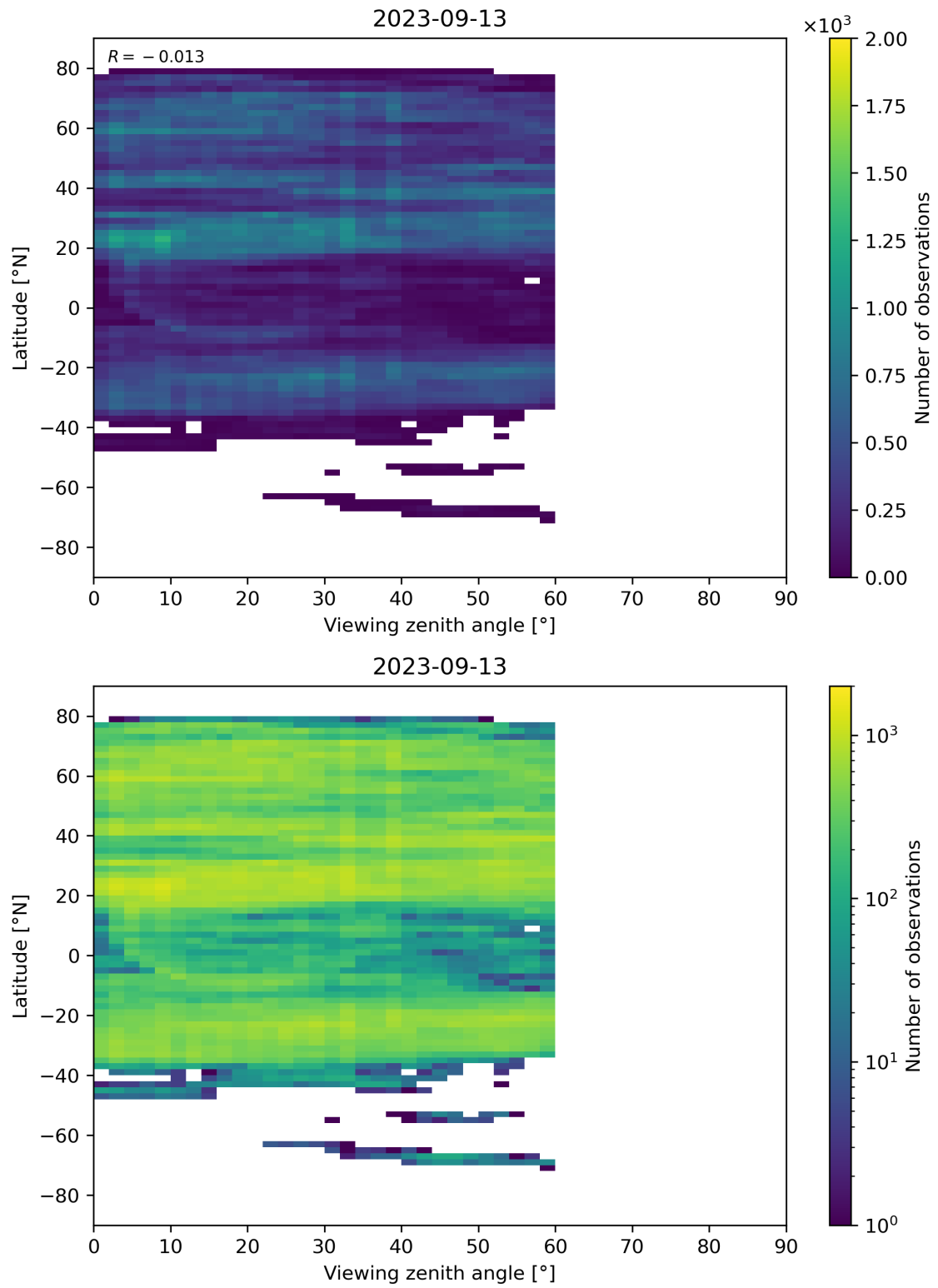
Figure 109: Scatter density plot of “Viewing zenith angle” against “Latitude” for 2023-09-12 to 2023-09-14.
