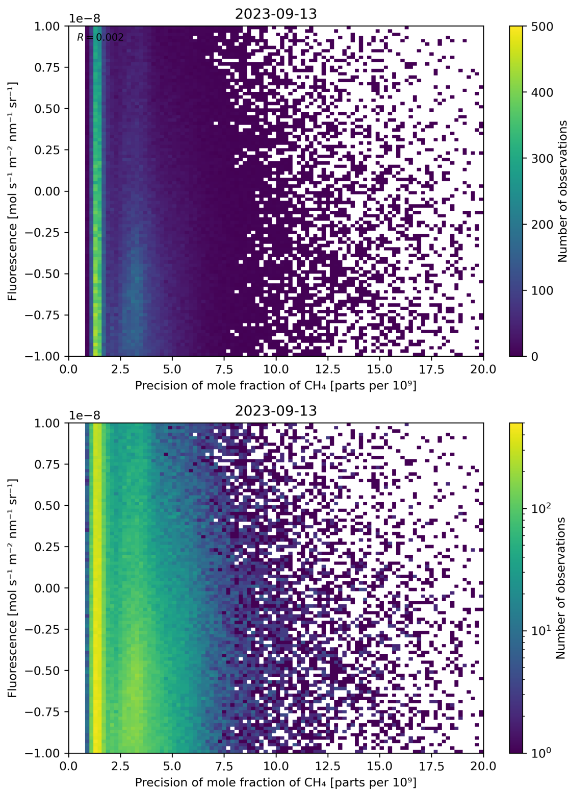
Figure 81: Scatter density plot of “Precision of mole fraction of \text{CH}_4 ” against “Fluorescence” for 2023-09-12 to 2023-09-14.
