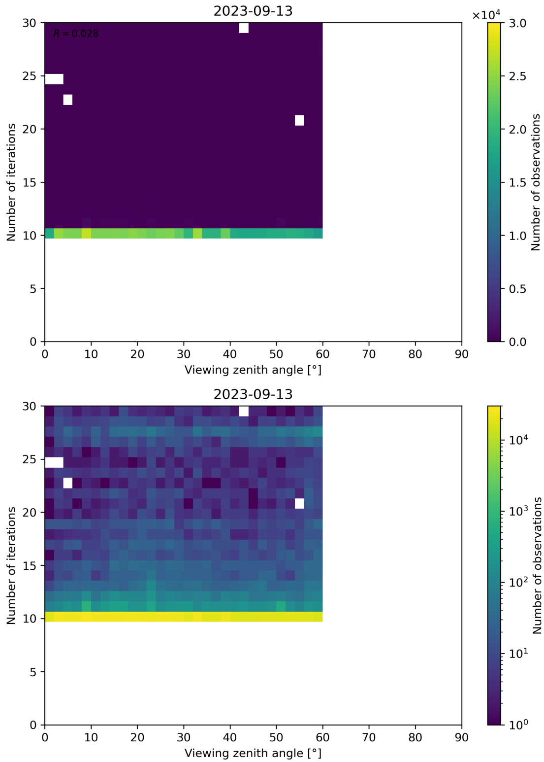
Figure 113: Scatter density plot of “Viewing zenith angle” against “Number of iterations” for 2023-09-12 to 2023-09-14.
