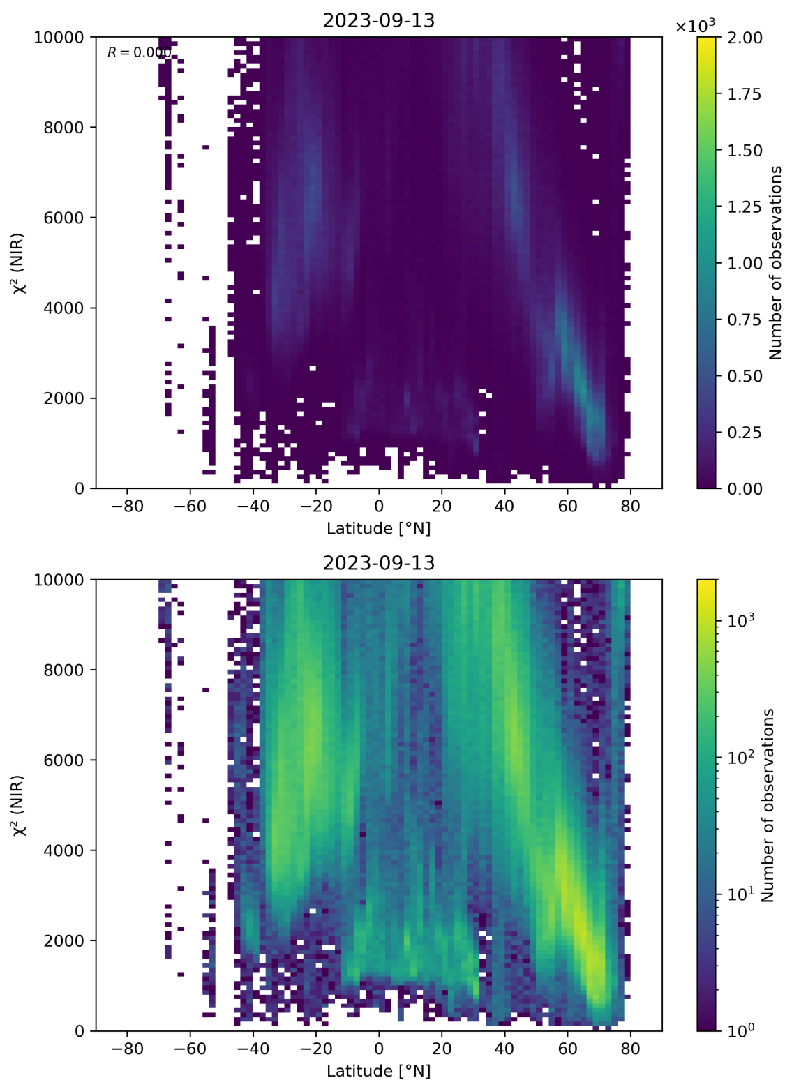
Figure 53: Scatter density plot of “Latitude” against “ \chi^2 (NIR)” for 2023-09-12 to 2023-09-14.
