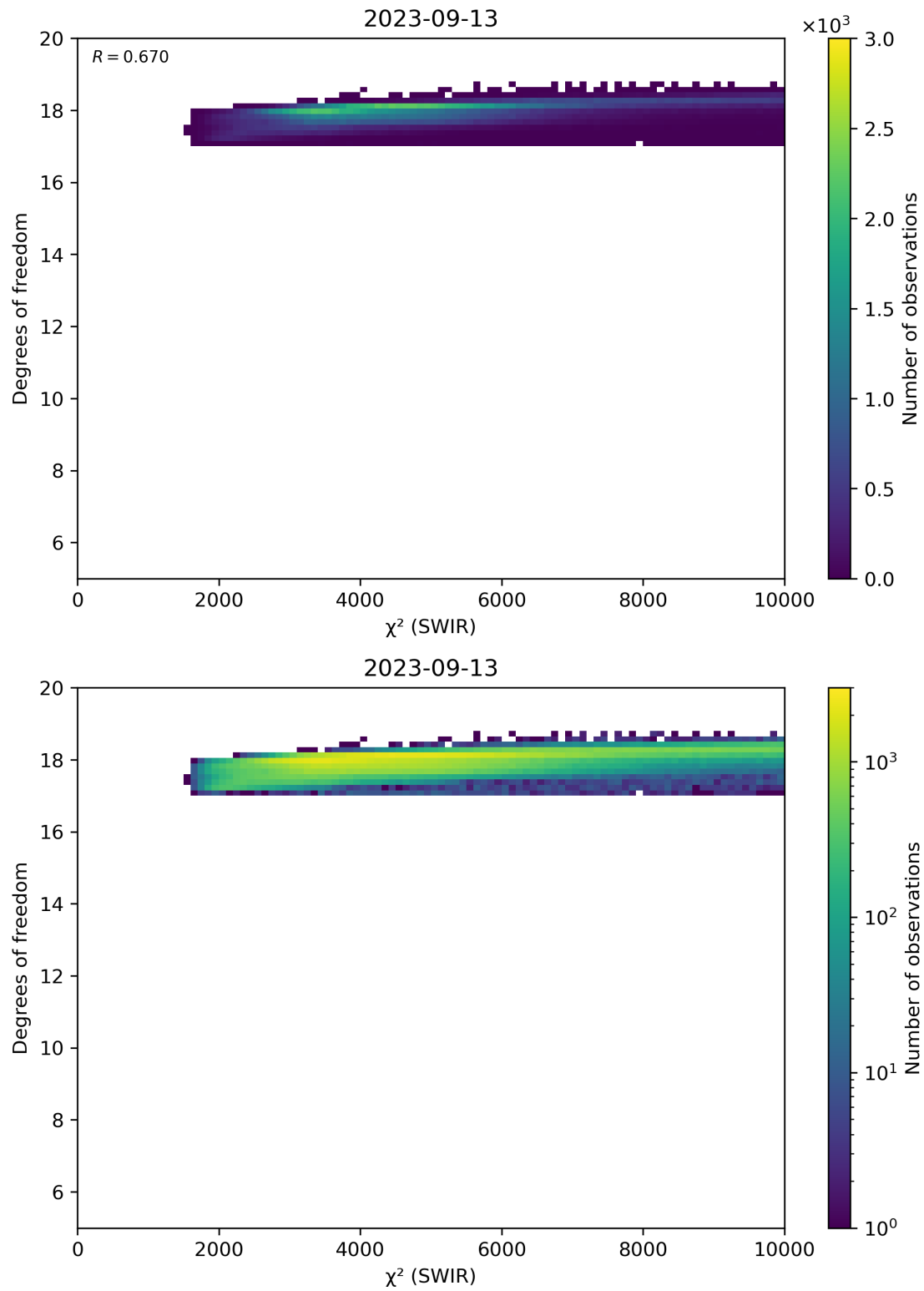
Figure 48: Scatter density plot of “ \chi^2 (SWIR)” against “Degrees of freedom” for 2023-09-12 to 2023-09-14.
