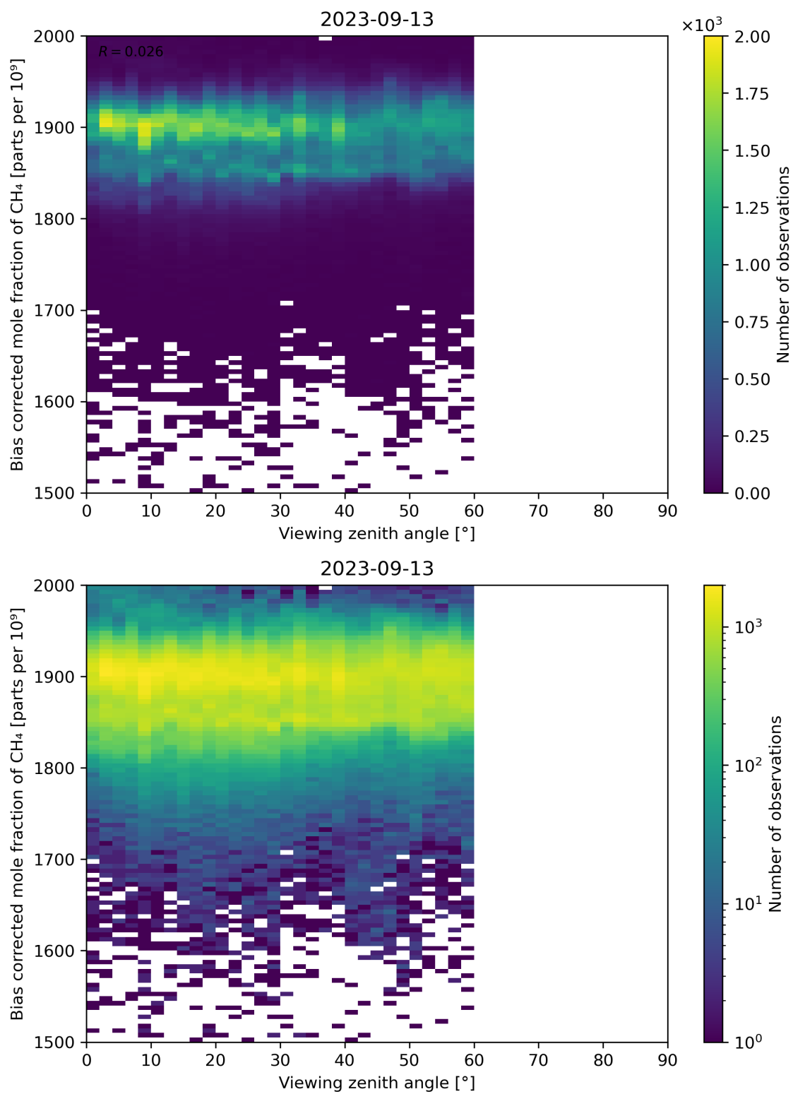
Figure 111: Scatter density plot of “Viewing zenith angle” against “Bias corrected mole fraction of CH 4 ” for 2023-09-12 to 2023-09-14.
