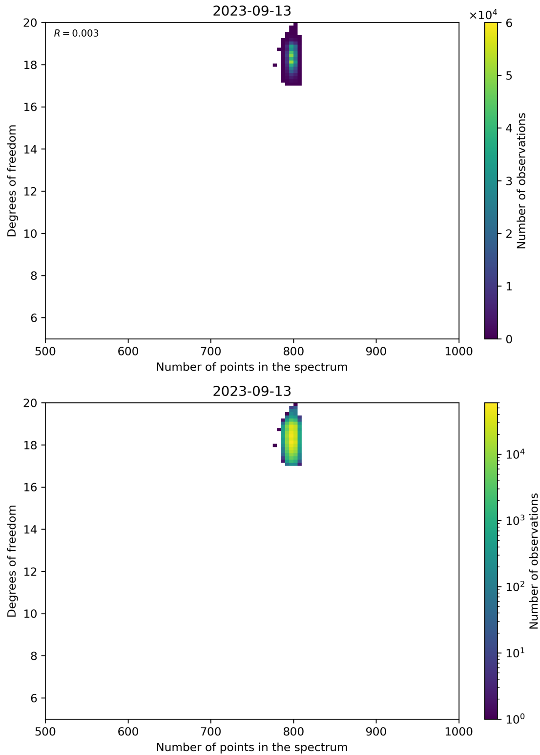
Figure 90: Scatter density plot of “Number of points in the spectrum” against “Degrees of freedom” for 2023-09-12 to 2023-09-14.
