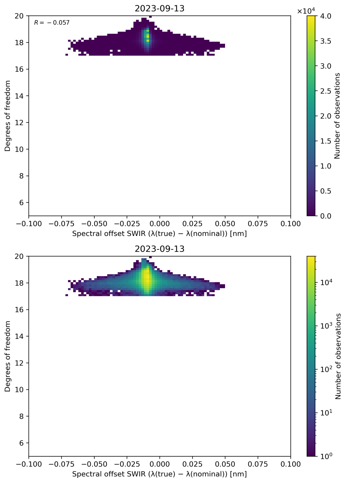
Figure 119: Scatter density plot of “Spectral offset SWIR ( \lambda(\text{true}) - \lambda(\text{nominal}) )” against “Degrees of freedom” for 2023-09-12 to 2023-09-14.
