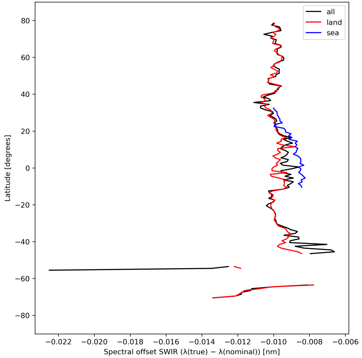
Figure 16: Zonal average of “Spectral offset SWIR ( \lambda(\text{true}) - \lambda(\text{nominal}) )” for 2023-09-12 to 2023-09-14.
