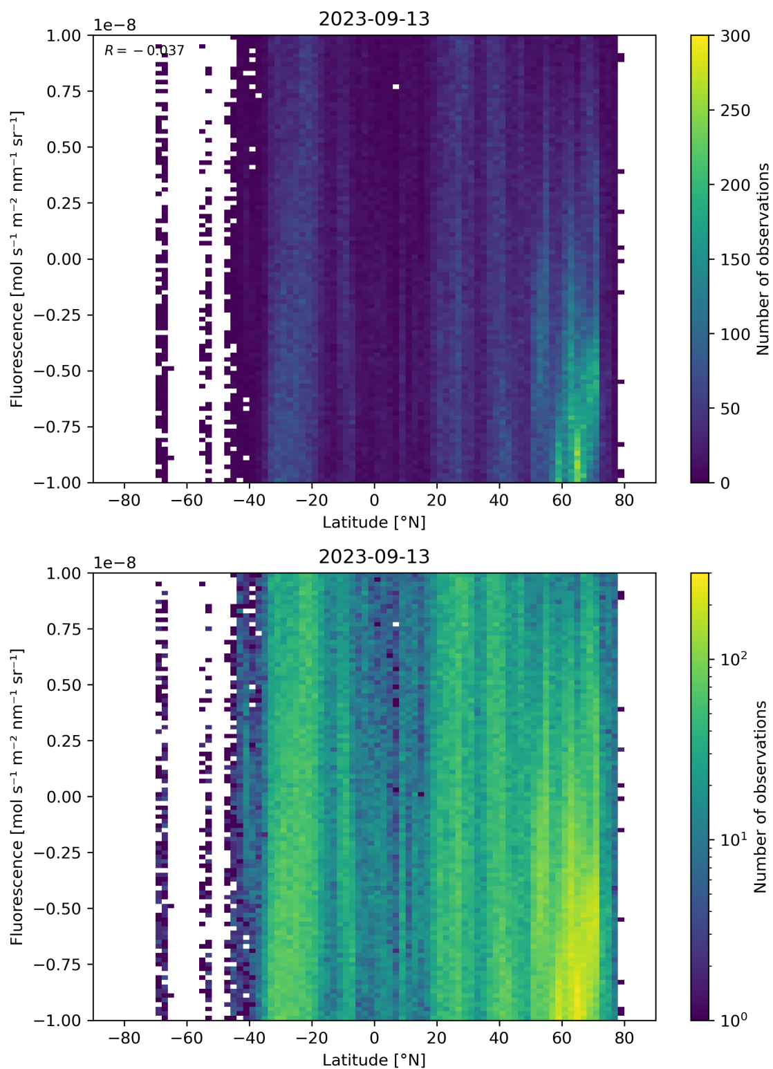
Figure 56: Scatter density plot of “Latitude” against “Fluorescence” for 2023-09-12 to 2023-09-14.
