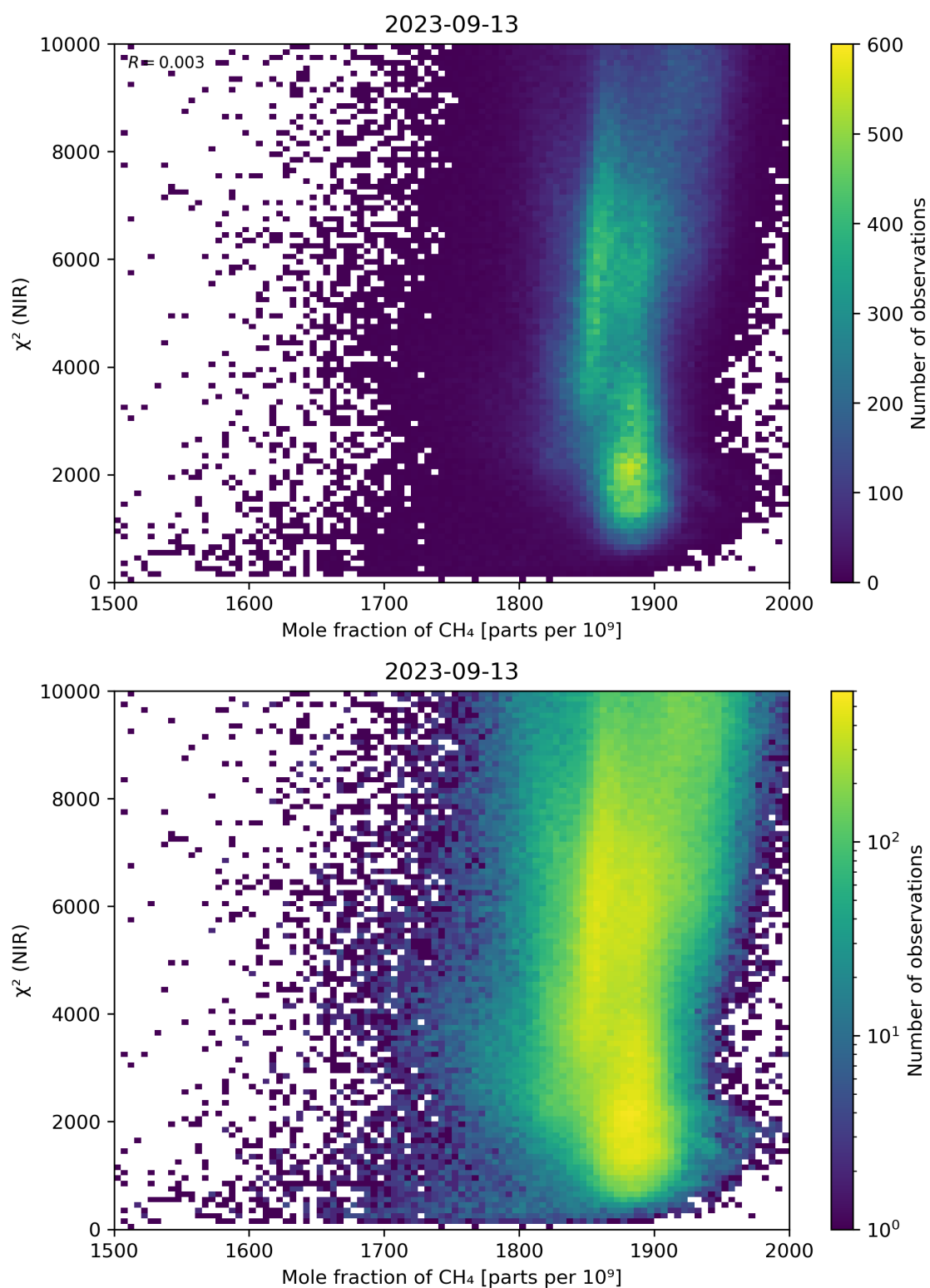
Figure 70: Scatter density plot of “Mole fraction of CH 4 ” against “ \chi^2 (NIR)” for 2023-09-12 to 2023-09-14.
