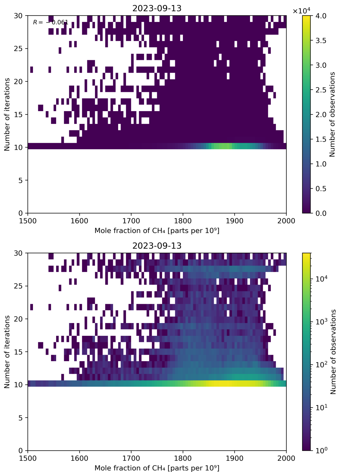
Figure 76: Scatter density plot of “Mole fraction of CH 4 ” against “Number of iterations” for 2023-09-12 to 2023-09-14.
