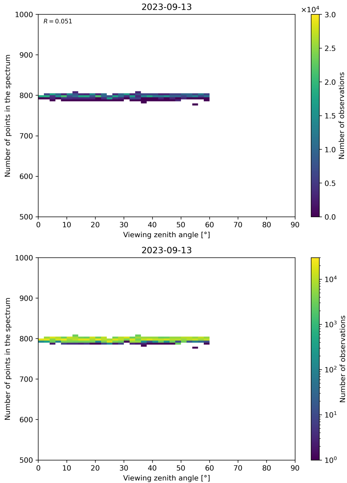
Figure 114: Scatter density plot of “Viewing zenith angle” against “Number of points in the spectrum” for 2023-09-12 to 2023-09-14.
