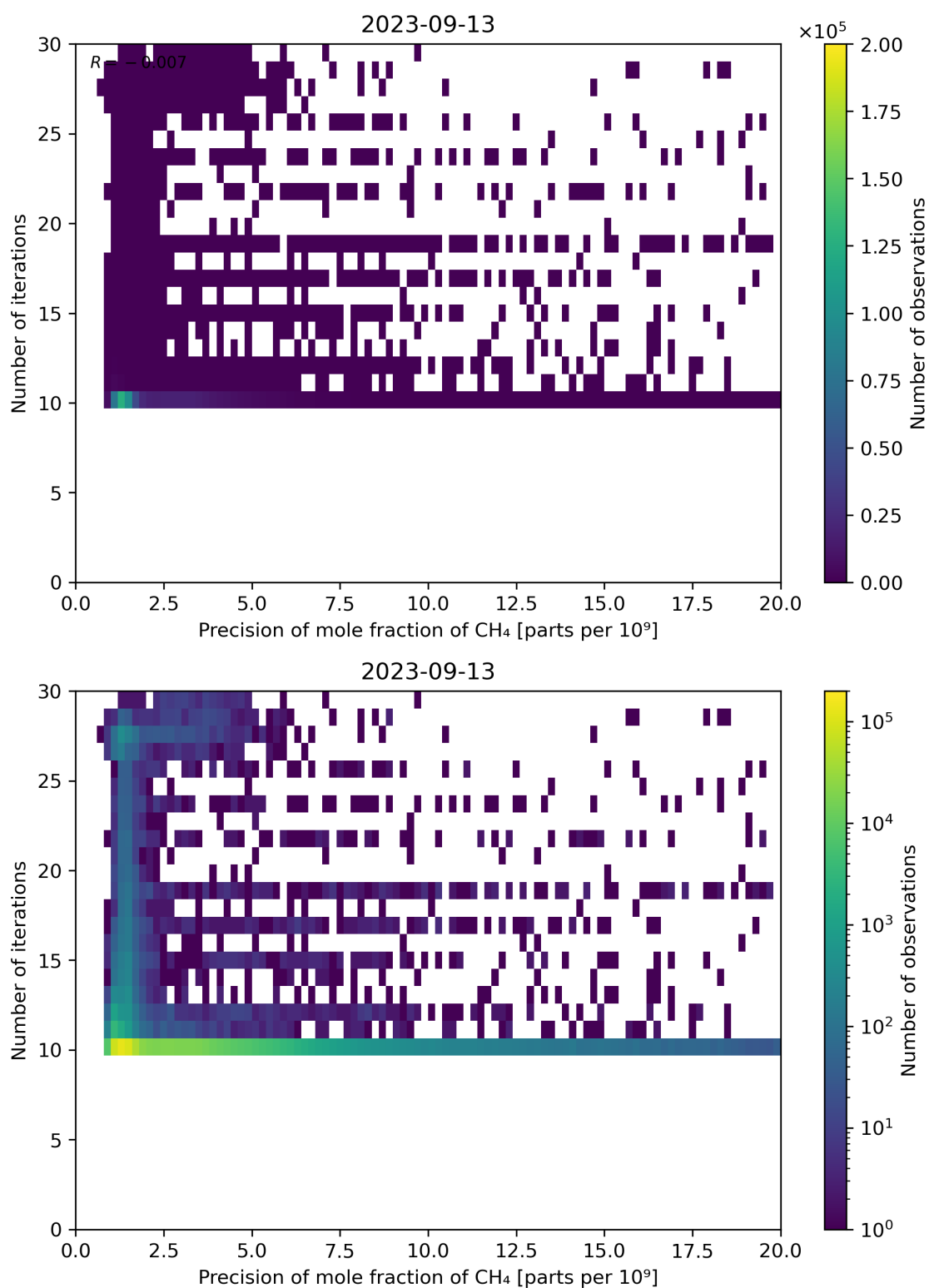
Figure 83: Scatter density plot of “Precision of mole fraction of CH 4 ” against “Number of iterations” for 2023-09-12 to 2023-09-14.
