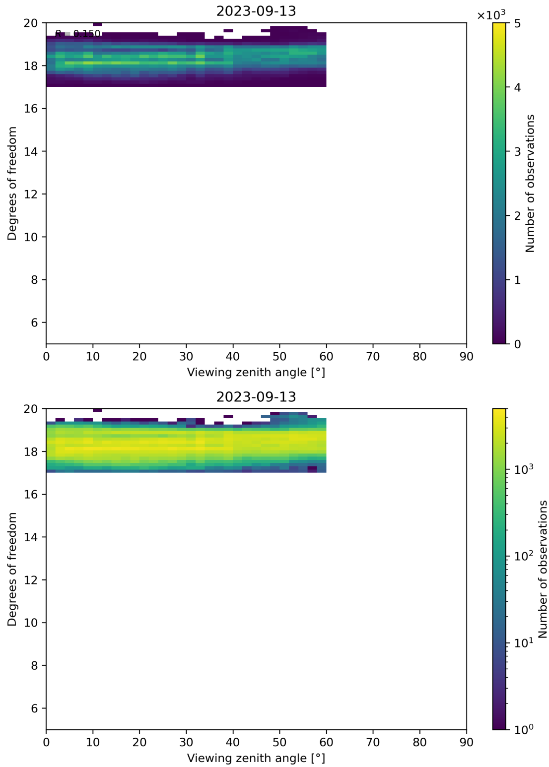
Figure 107: Scatter density plot of “Viewing zenith angle” against “Degrees of freedom” for 2023-09-12 to 2023-09-14.
