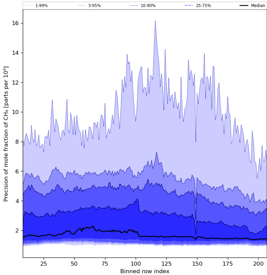
Figure 35: Along track statistics of “Precision of mole fraction of CH 4 ” for 2023-09-12 to 2023-09-14
