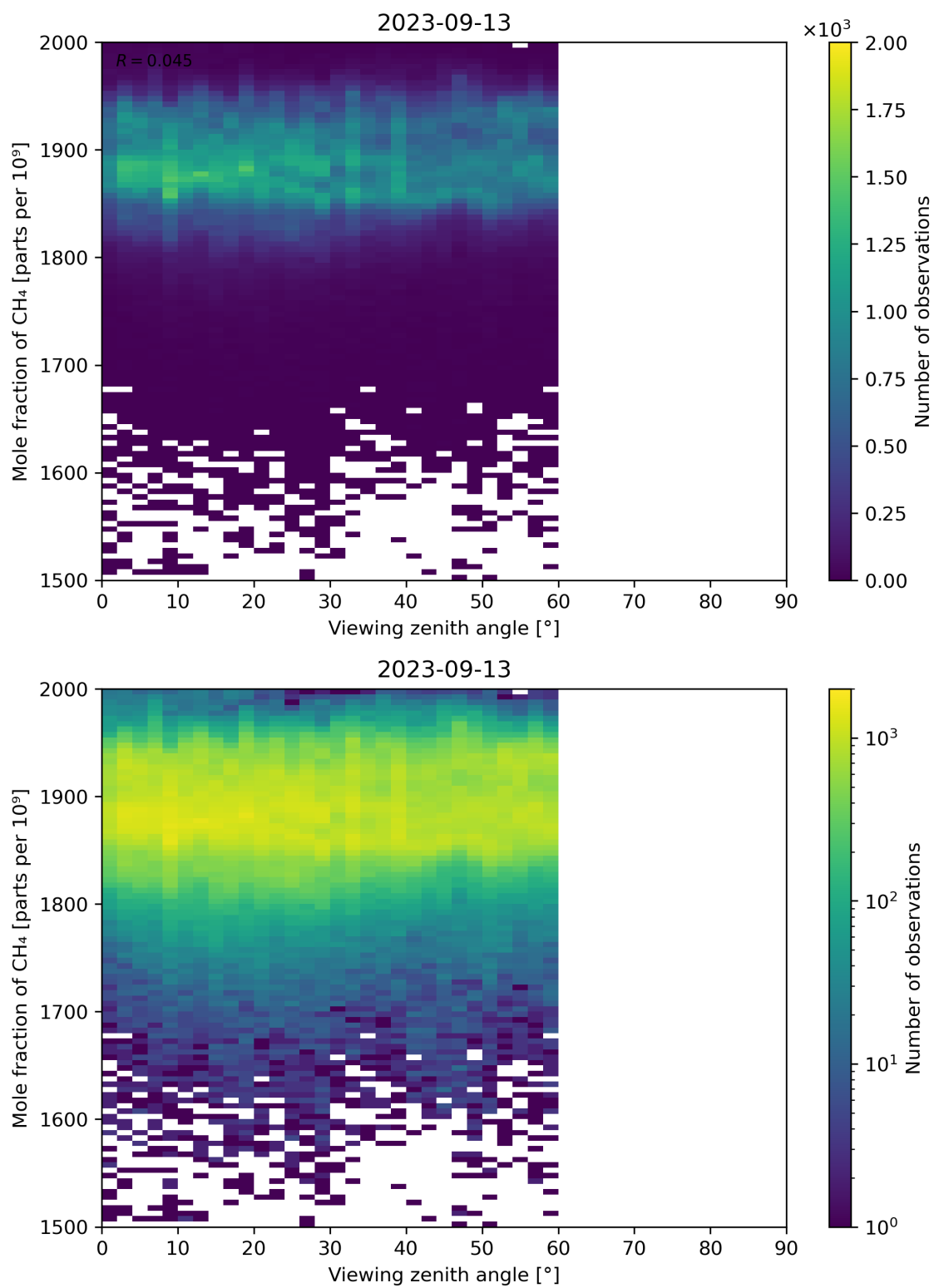
Figure 110: Scatter density plot of “Viewing zenith angle” against “Mole fraction of CH 4 ” for 2023-09-12 to 2023-09-14.
