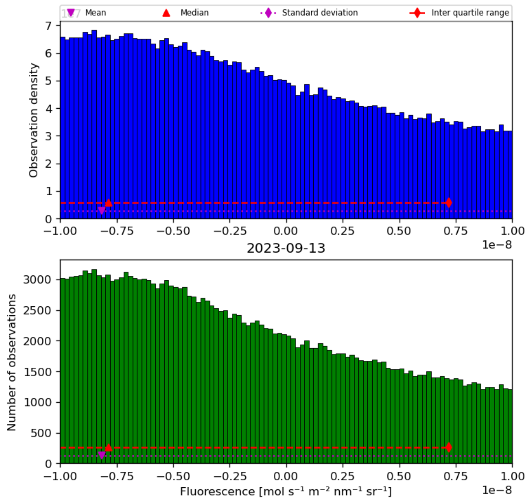
Figure 32: Histogram of “Fluorescence” for 2023-09-12 to 2023-09-14
