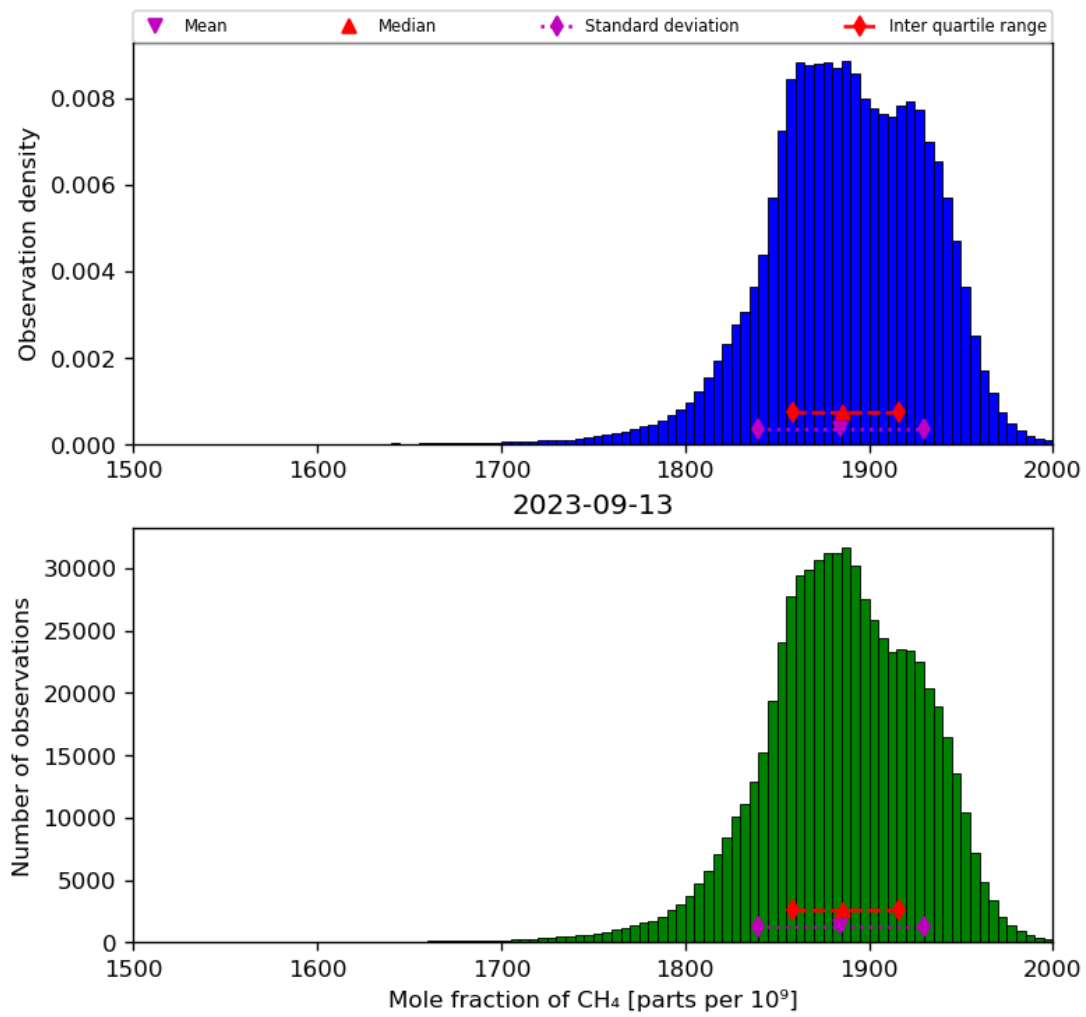
Figure 23: Histogram of “Mole fraction of CH 4 ” for 2023-09-12 to 2023-09-14
