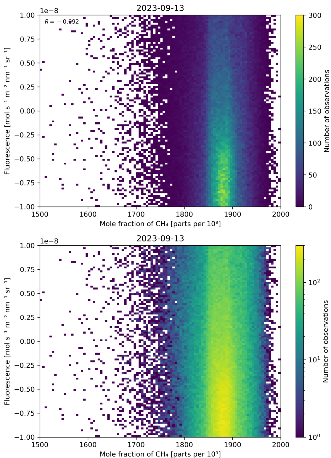
Figure 73: Scatter density plot of “Mole fraction of \text{CH}_4 ” against “Fluorescence” for 2023-09-12 to 2023-09-14.
