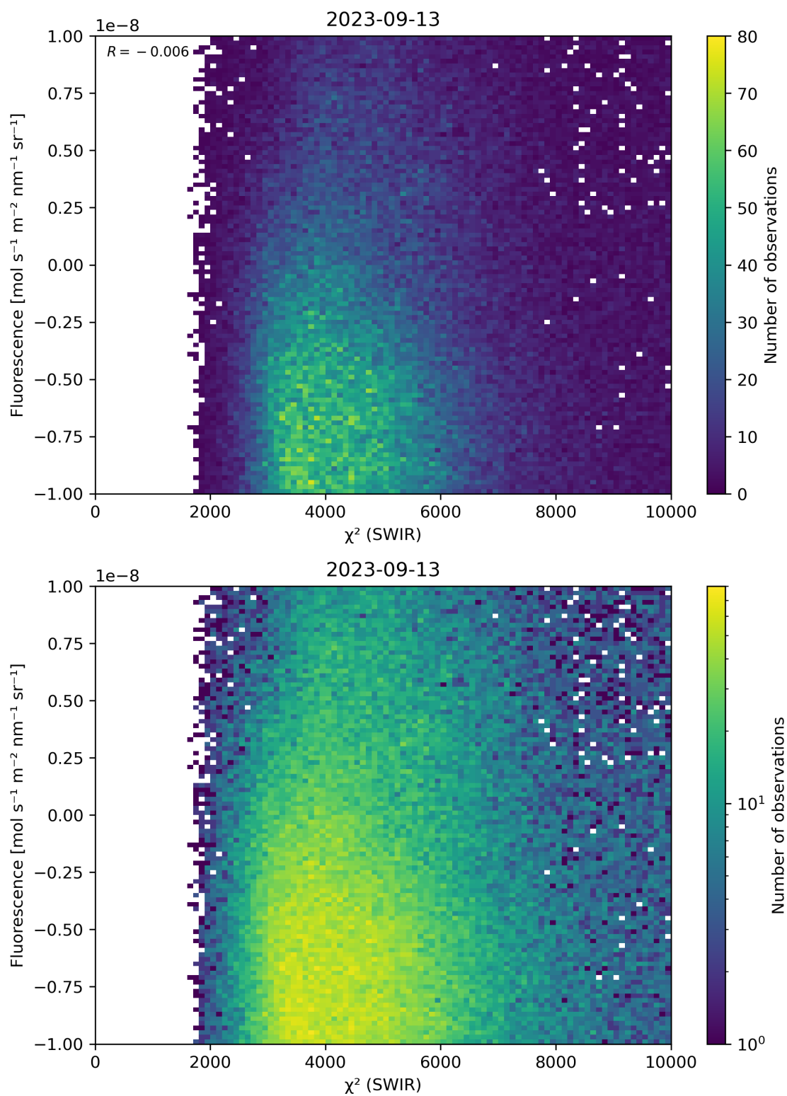
Figure 49: Scatter density plot of “ \chi^2 (SWIR)” against “Fluorescence” for 2023-09-12 to 2023-09-14.
