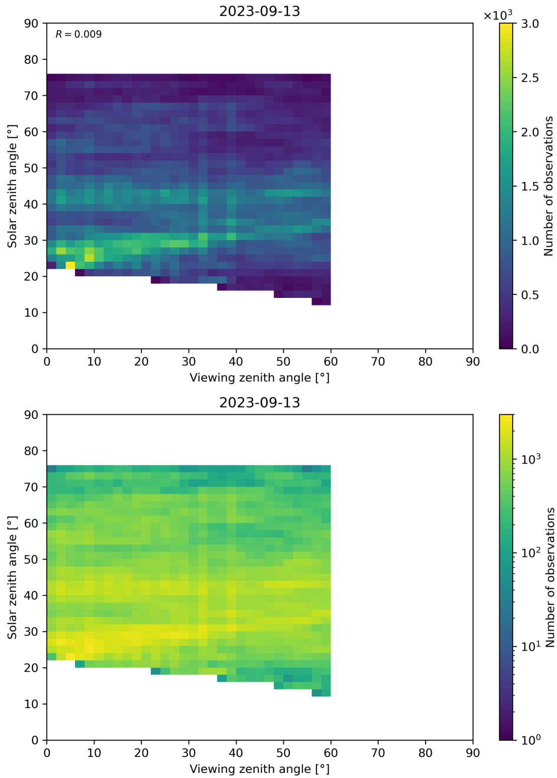
Figure 115: Scatter density plot of “Viewing zenith angle” against “Solar zenith angle” for 2023-09-12 to 2023-09-14.
