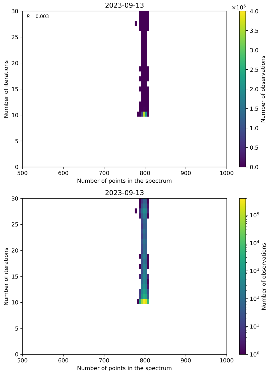
Figure 92: Scatter density plot of “Number of points in the spectrum” against “Number of iterations” for 2023-09-12 to 2023-09-14.
