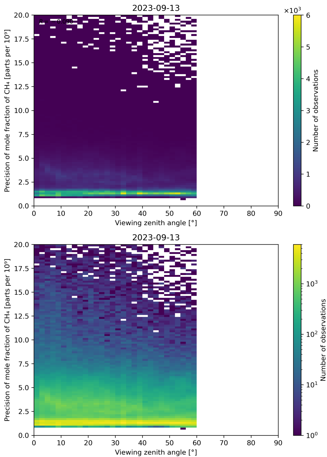
Figure 112: Scatter density plot of “Viewing zenith angle” against “Precision of mole fraction of CH 4 ” for 2023-09-12 to 2023-09-14.
