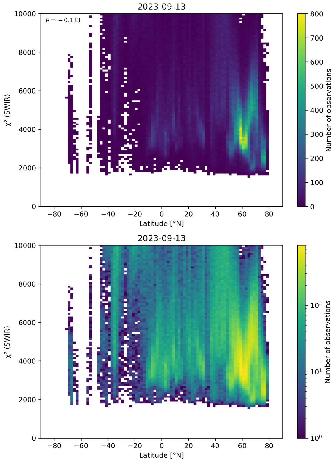
Figure 54: Scatter density plot of “Latitude” against “ \chi^2 (SWIR)” for 2023-09-12 to 2023-09-14.
