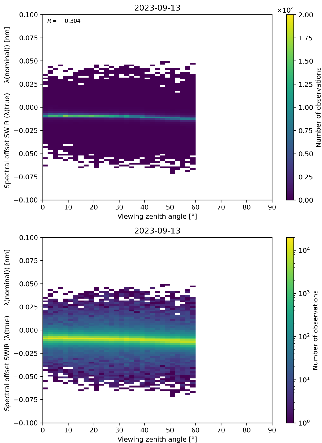
Figure 116: Scatter density plot of “Viewing zenith angle” against “Spectral offset SWIR ( \lambda(\text{true}) - \lambda(\text{nominal}) )” for 2023-09-12 to 2023-09-14.
