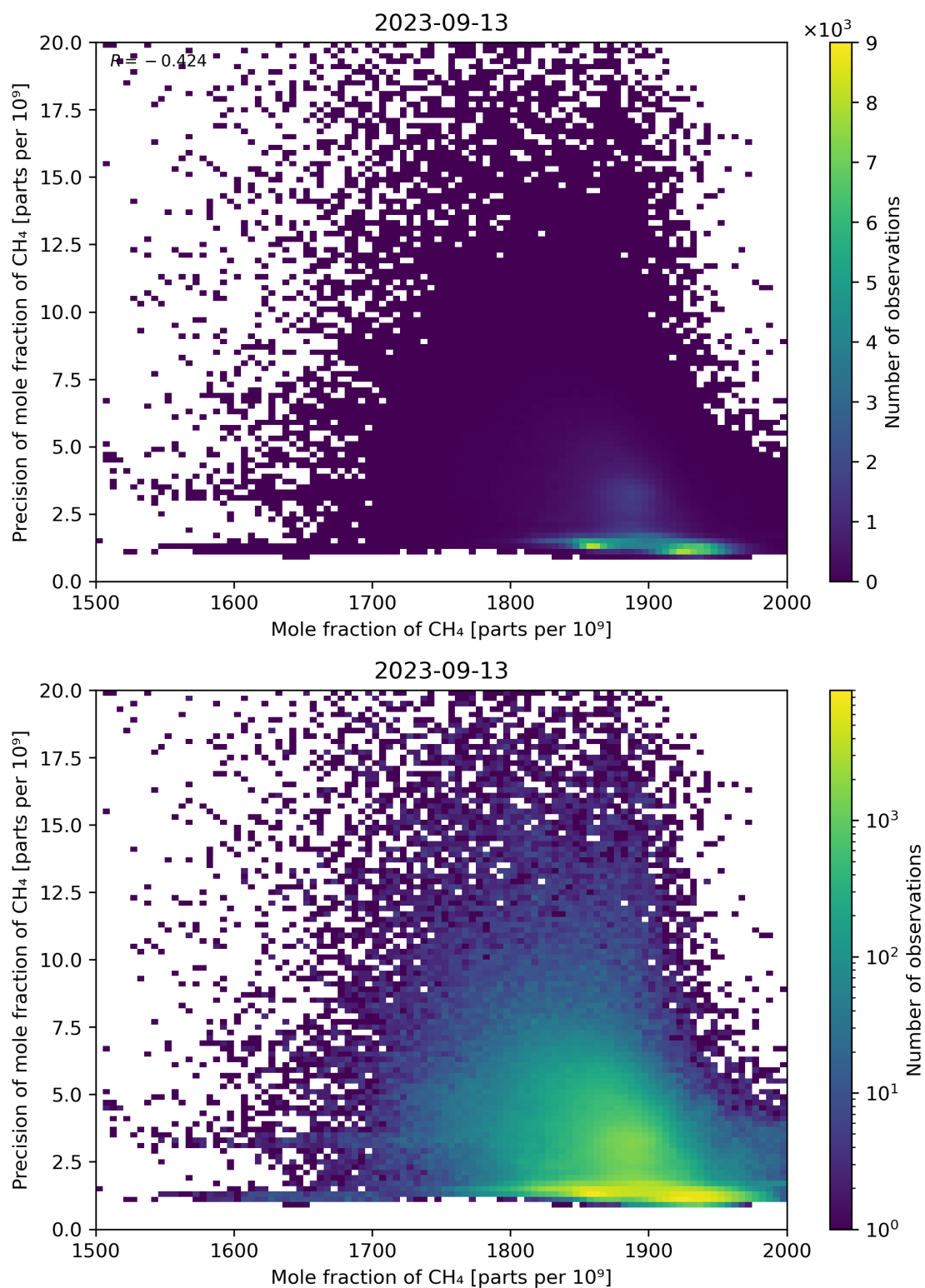
Figure 75: Scatter density plot of “Mole fraction of CH 4 ” against “Precision of mole fraction of CH 4 ” for 2023-09-12 to 2023-09-14.
