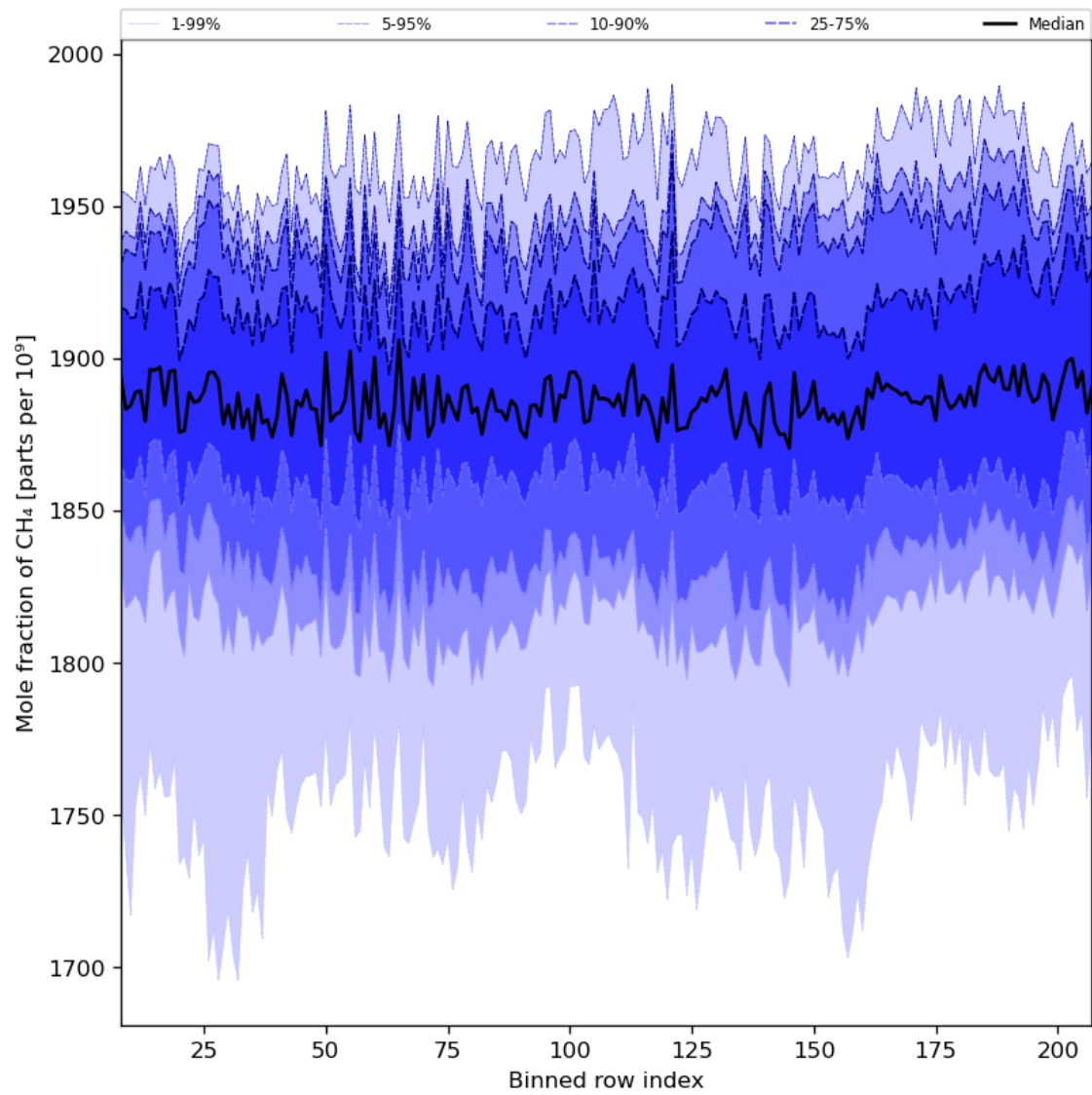
Figure 34: Along track statistics of “Mole fraction of CH 4 ” for 2023-09-12 to 2023-09-14
