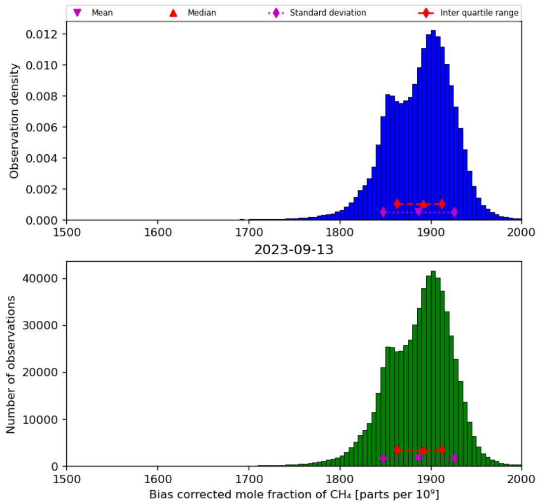
Figure 25: Histogram of “Bias corrected mole fraction of CH 4 ” for 2023-09-12 to 2023-09-14
