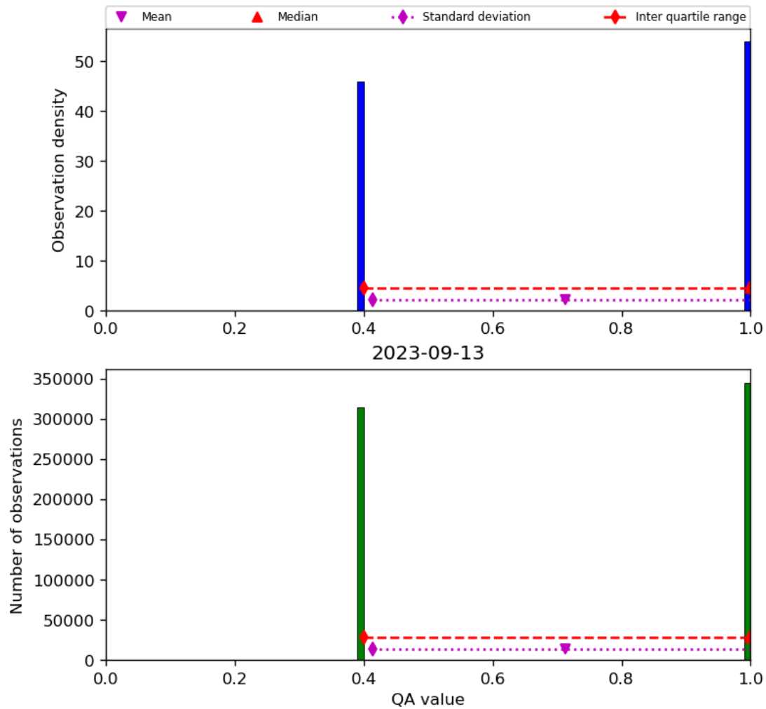
Figure 22: Histogram of “QA value” for 2023-09-12 to 2023-09-14
