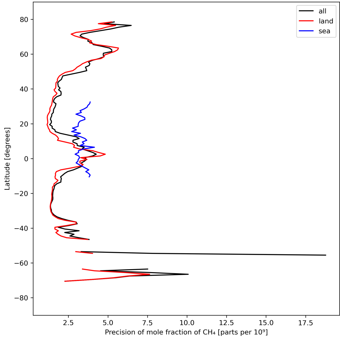
Figure 13: Zonal average of “Precision of mole fraction of CH 4 ” for 2023-09-12 to 2023-09-14.
