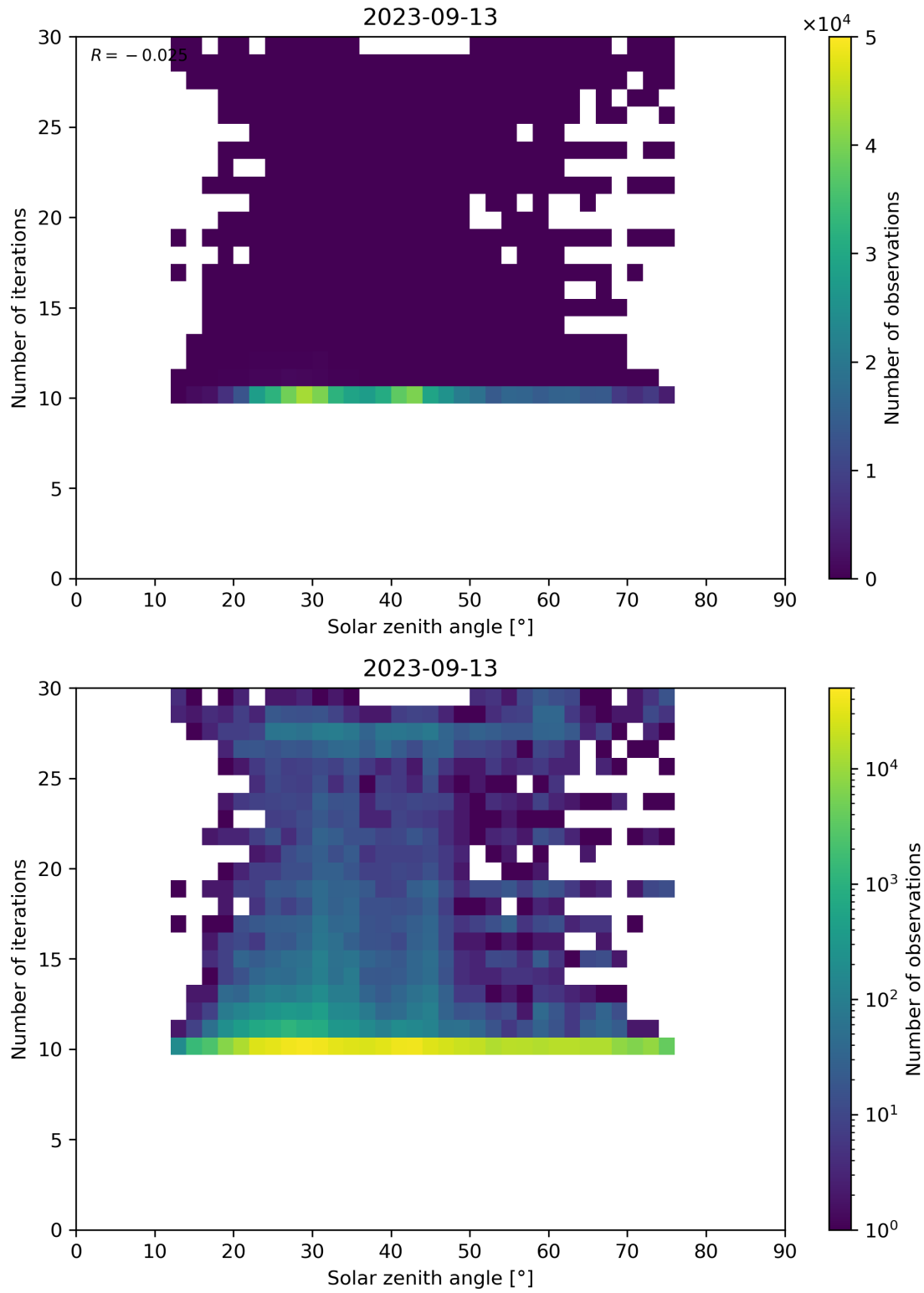
Figure 102: Scatter density plot of “Solar zenith angle” against “Number of iterations” for 2023-09-12 to 2023-09-14.
