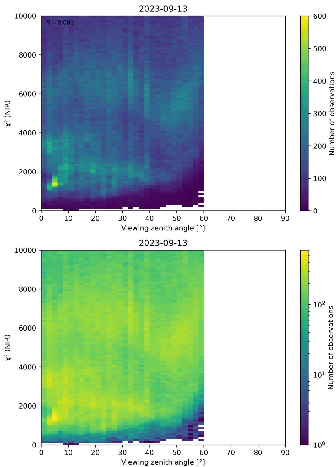
Figure 105: Scatter density plot of “Viewing zenith angle” against “ \chi^2 (NIR)” for 2023-09-12 to 2023-09-14.
