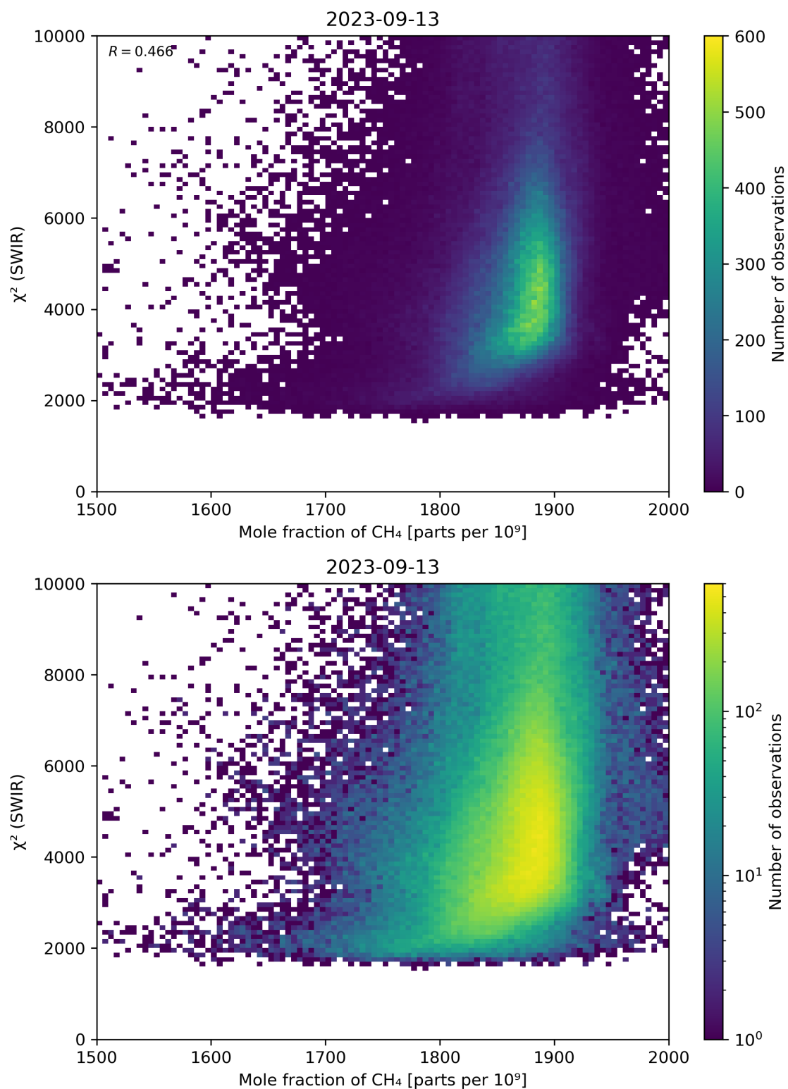
Figure 71: Scatter density plot of “Mole fraction of CH 4 ” against “ \chi^2 (SWIR)” for 2023-09-12 to 2023-09-14.
