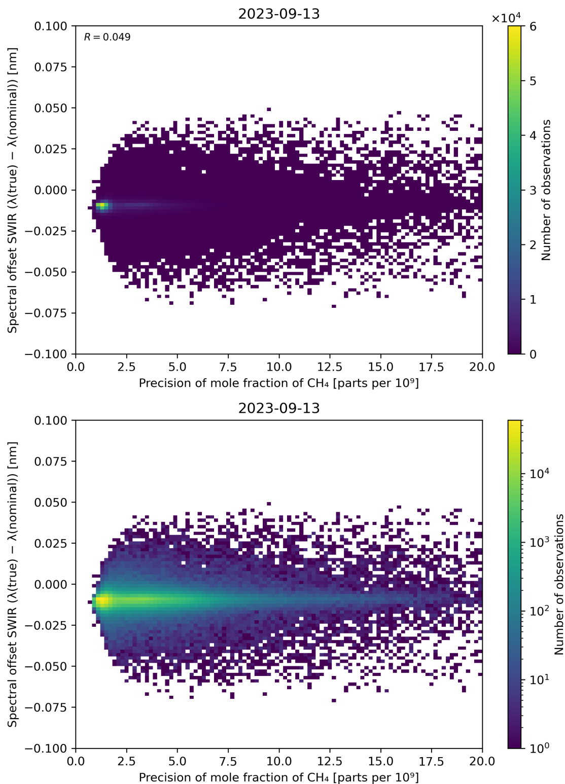
Figure 85: Scatter density plot of “Precision of mole fraction of CH 4 ” against “Spectral offset SWIR ( \lambda(\text{true}) - \lambda(\text{nominal}) )” for 2023-09-12 to 2023-09-14.
