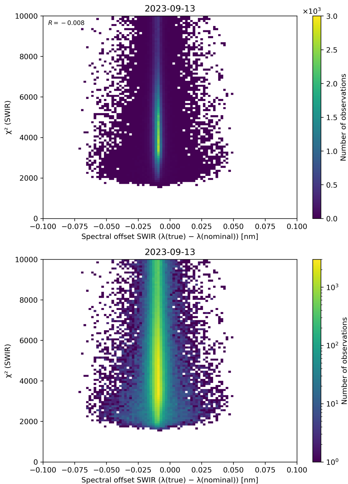
Figure 118: Scatter density plot of “Spectral offset SWIR ( \lambda(\text{true}) - \lambda(\text{nominal}) )” against “ \chi^2 (SWIR)” for 2023-09-12 to 2023-09-14.
