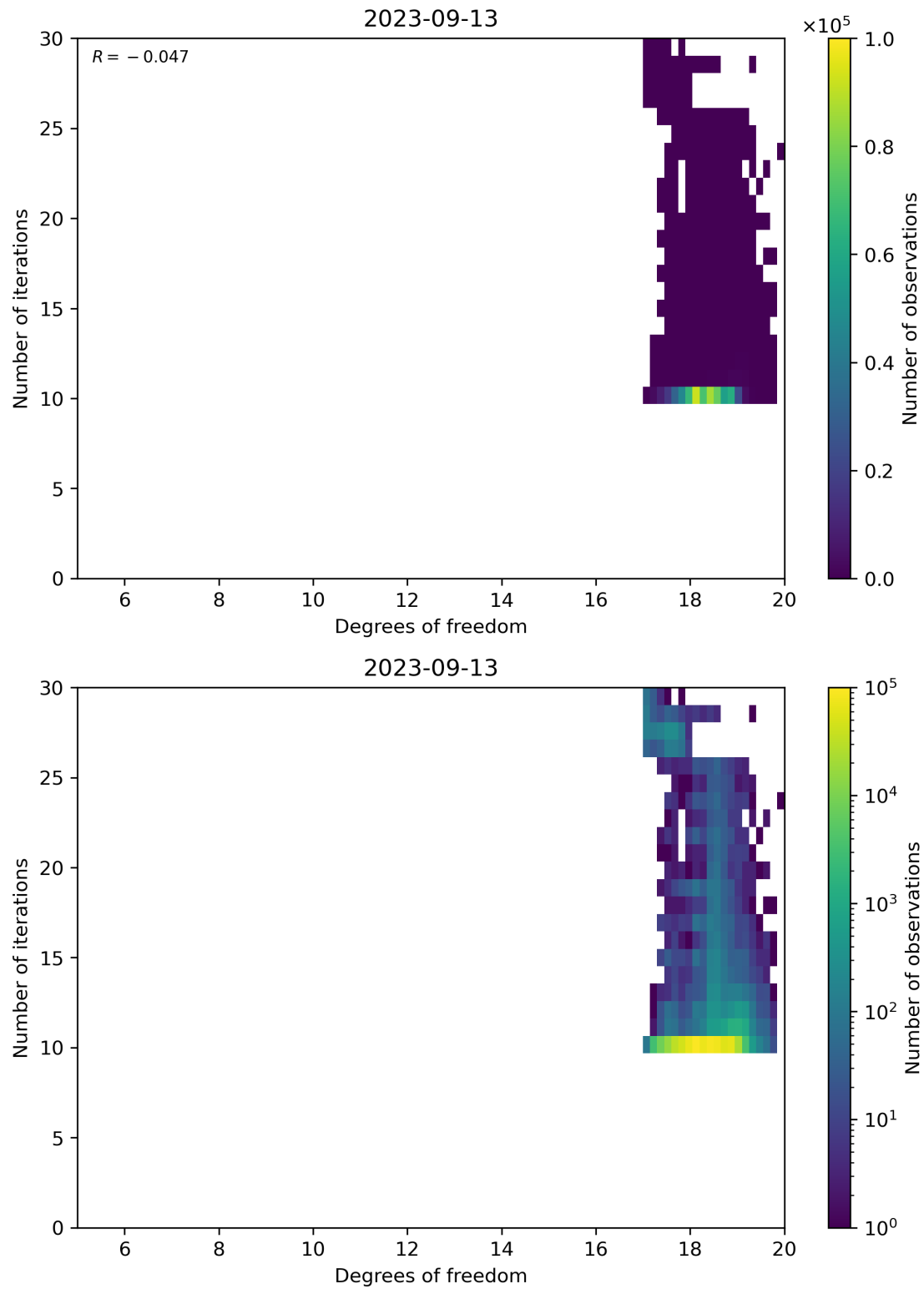
Figure 52: Scatter density plot of “Degrees of freedom” against “Number of iterations” for 2023-09-12 to 2023-09-14.
