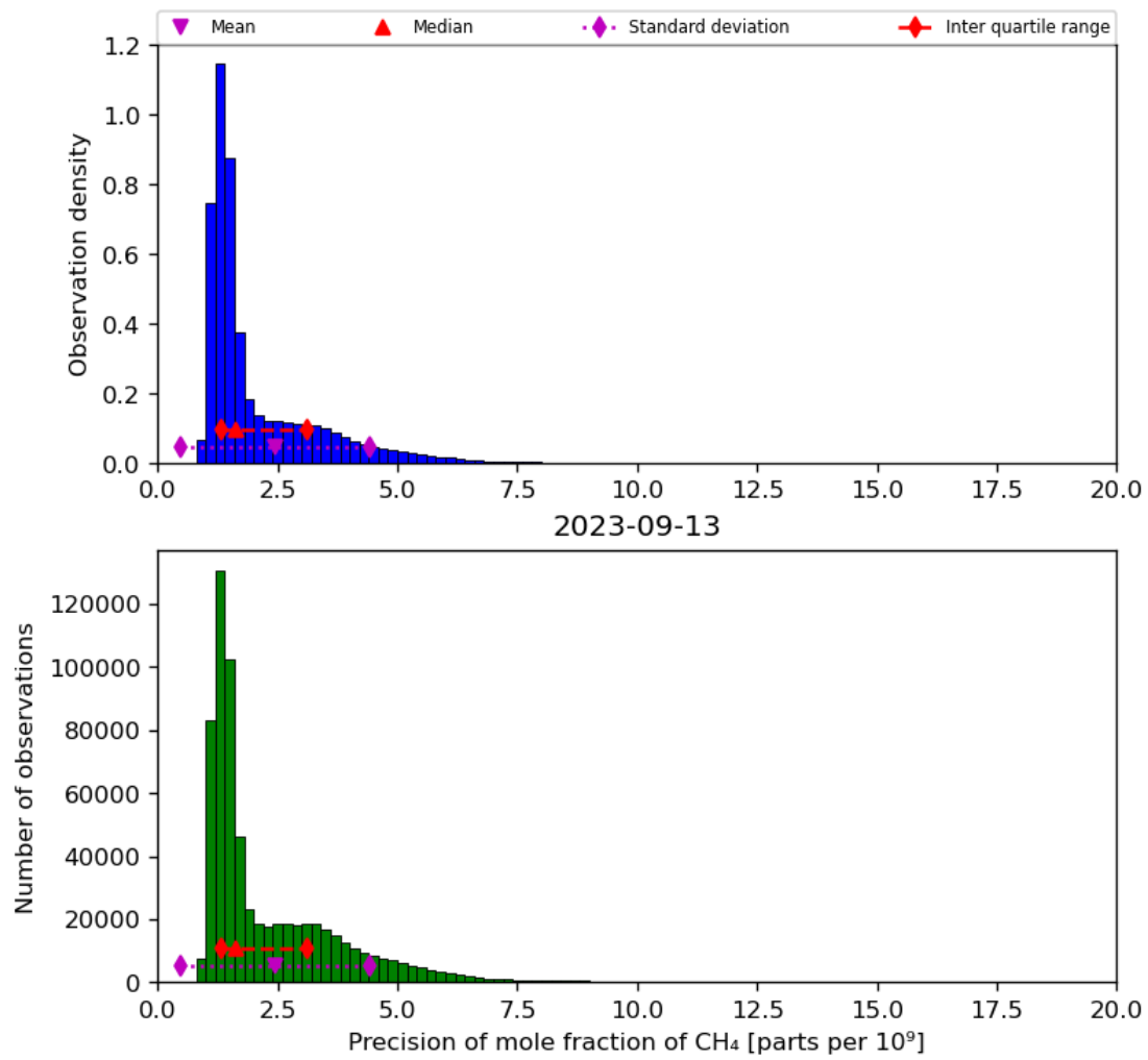
Figure 24: Histogram of “Precision of mole fraction of CH 4 ” for 2023-09-12 to 2023-09-14
