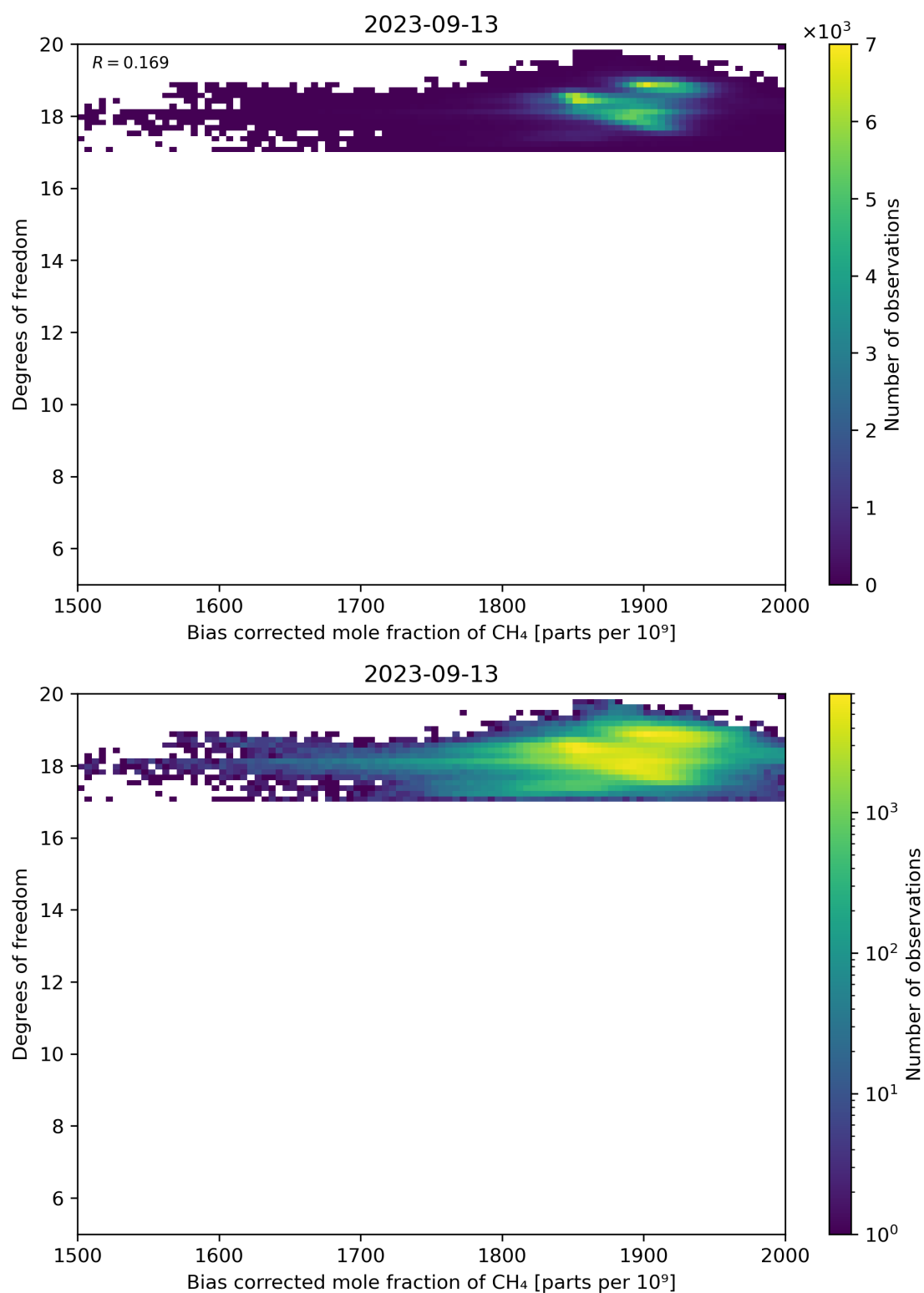
Figure 65: Scatter density plot of “Bias corrected mole fraction of CH 4 ” against “Degrees of freedom” for 2023-09-12 to 2023-09-14.
