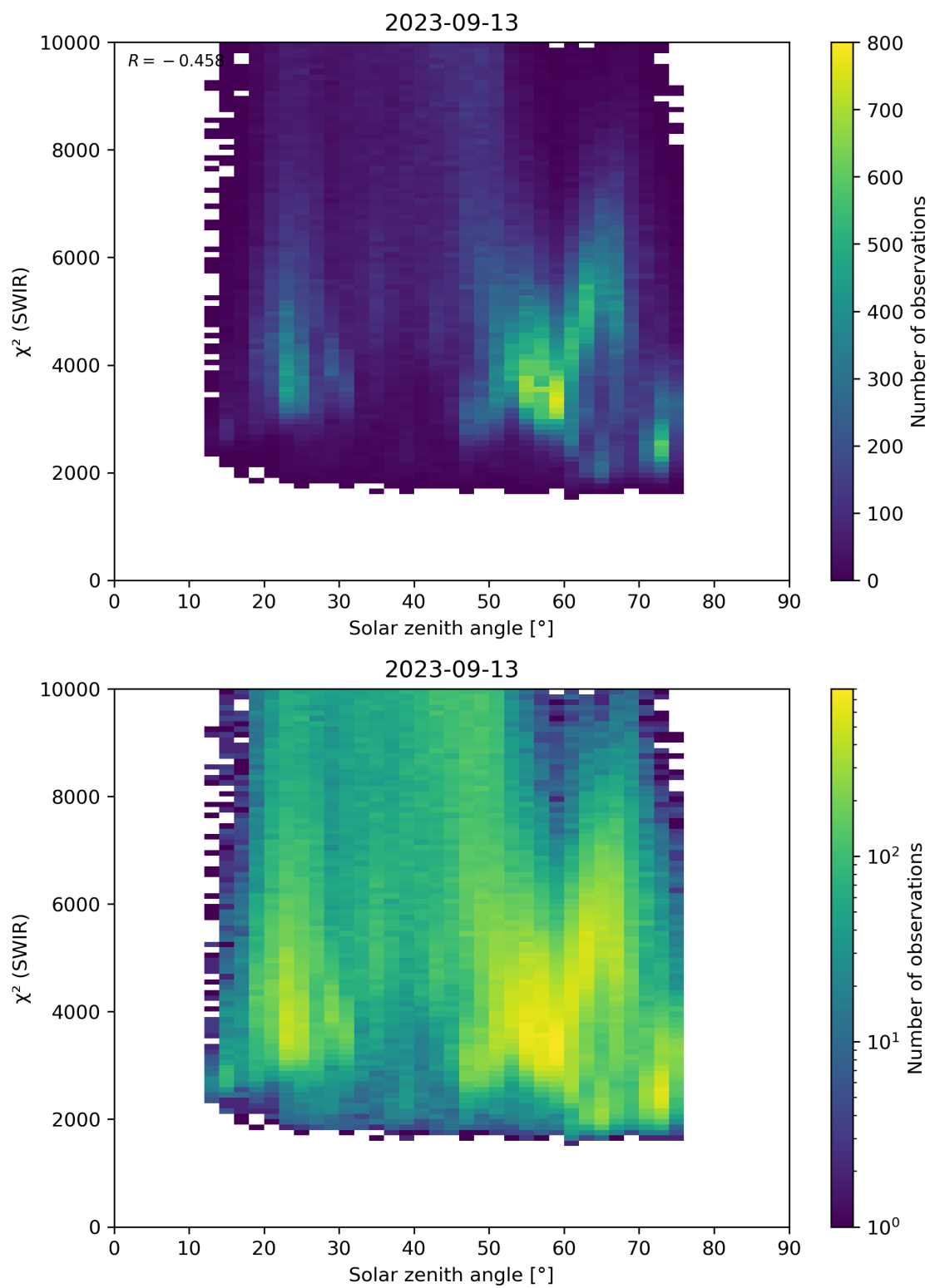
Figure 95: Scatter density plot of “Solar zenith angle” against “ \chi^2 (SWIR)” for 2023-09-12 to 2023-09-14.
