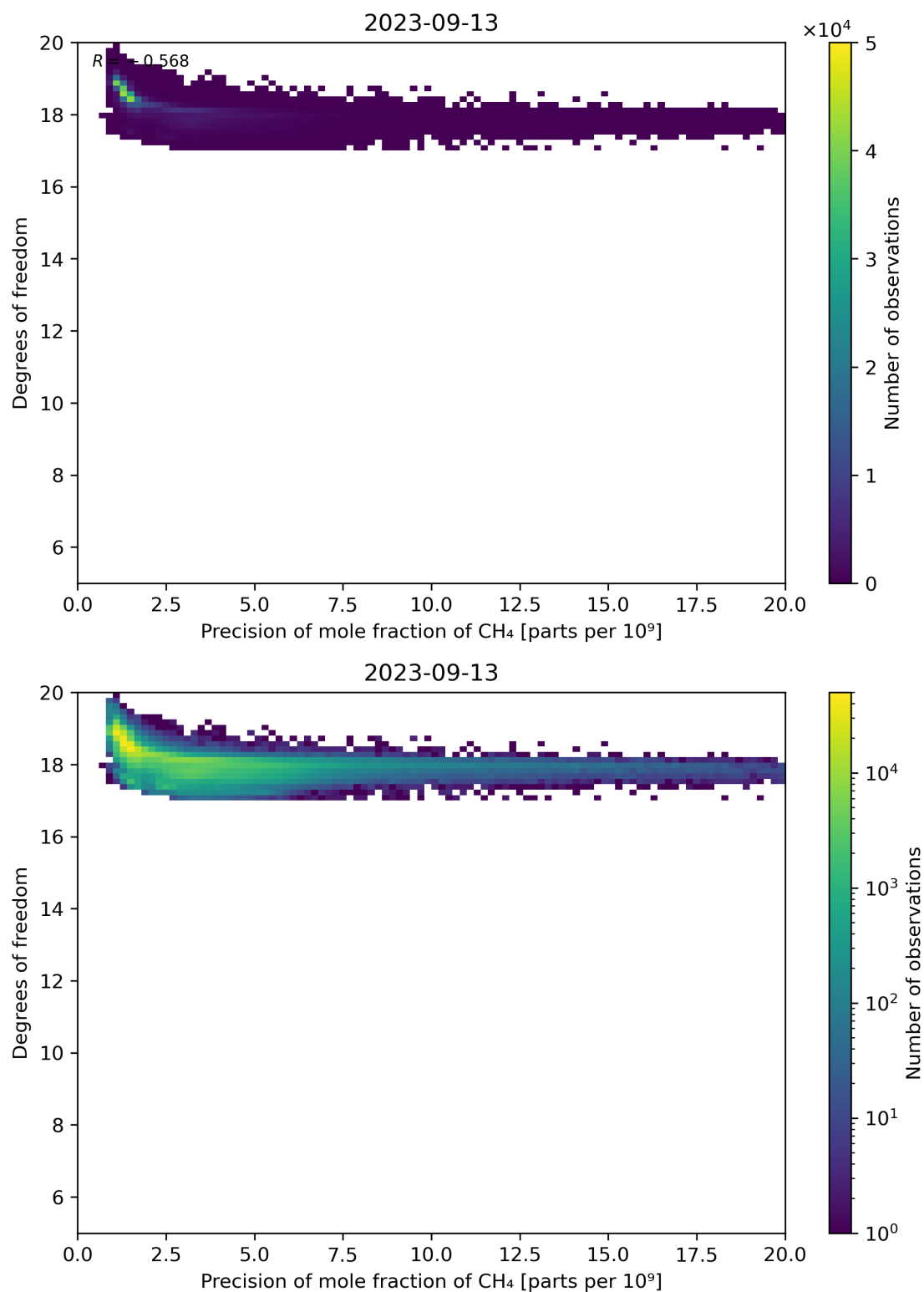
Figure 80: Scatter density plot of “Precision of mole fraction of CH 4 ” against “Degrees of freedom” for 2023-09-12 to 2023-09-14.
