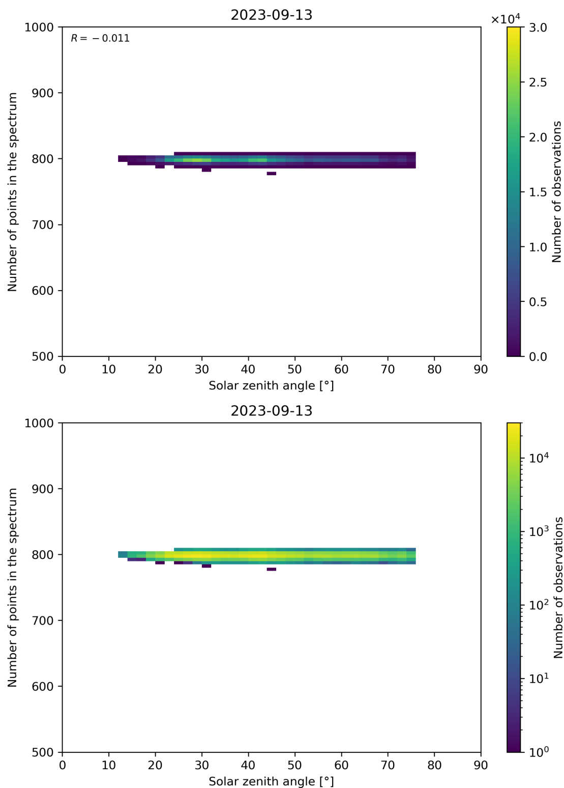
Figure 103: Scatter density plot of “Solar zenith angle” against “Number of points in the spectrum” for 2023-09-12 to 2023-09-14.
