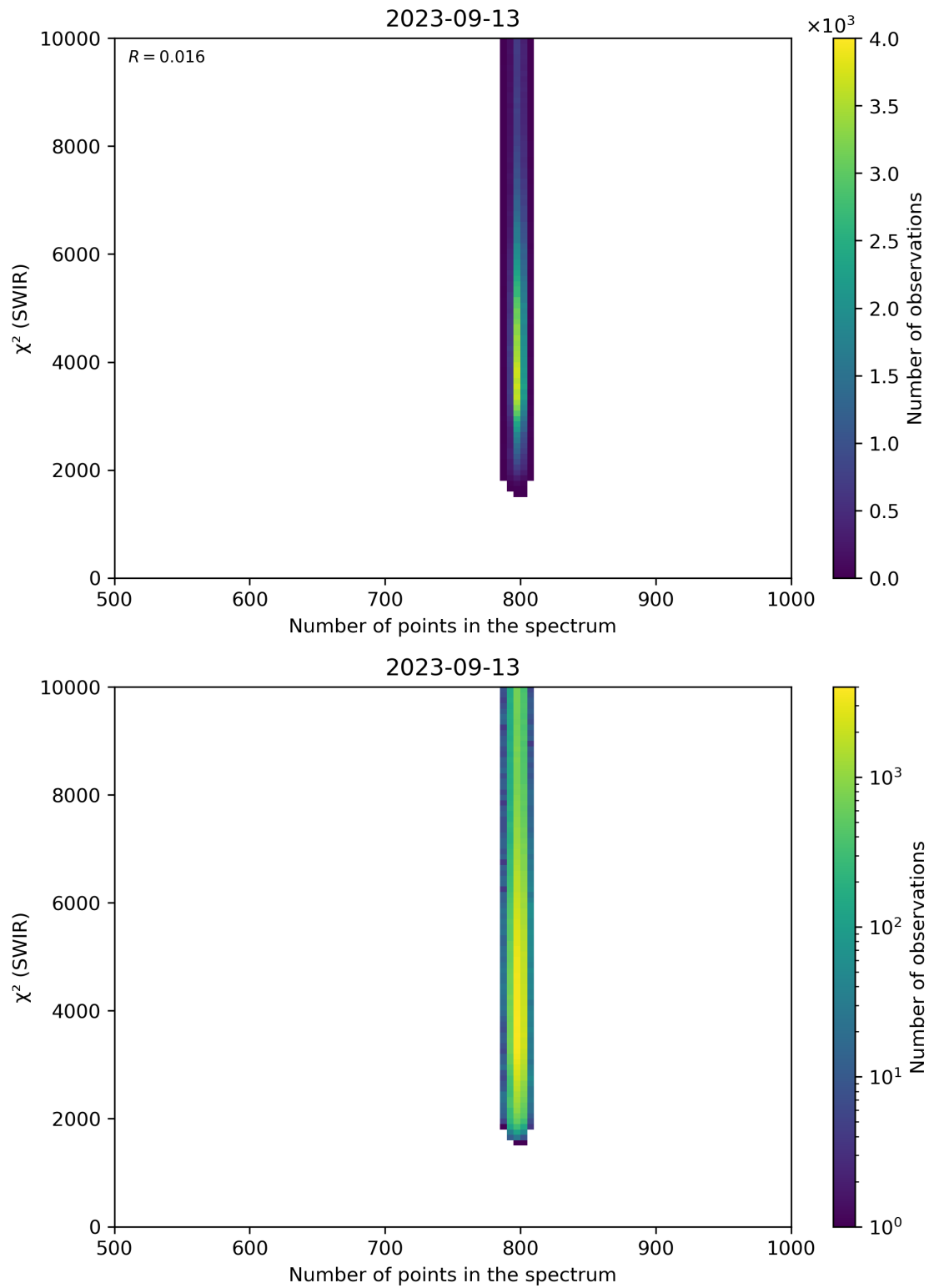
Figure 89: Scatter density plot of “Number of points in the spectrum” against “ \chi^2 (SWIR)” for 2023-09-12 to 2023-09-14.
