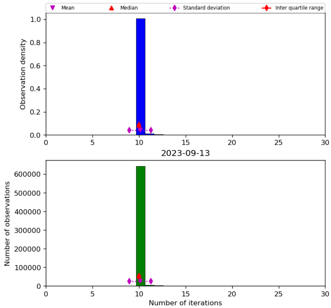
Figure 31: Histogram of “Number of iterations” for 2023-09-12 to 2023-09-14
