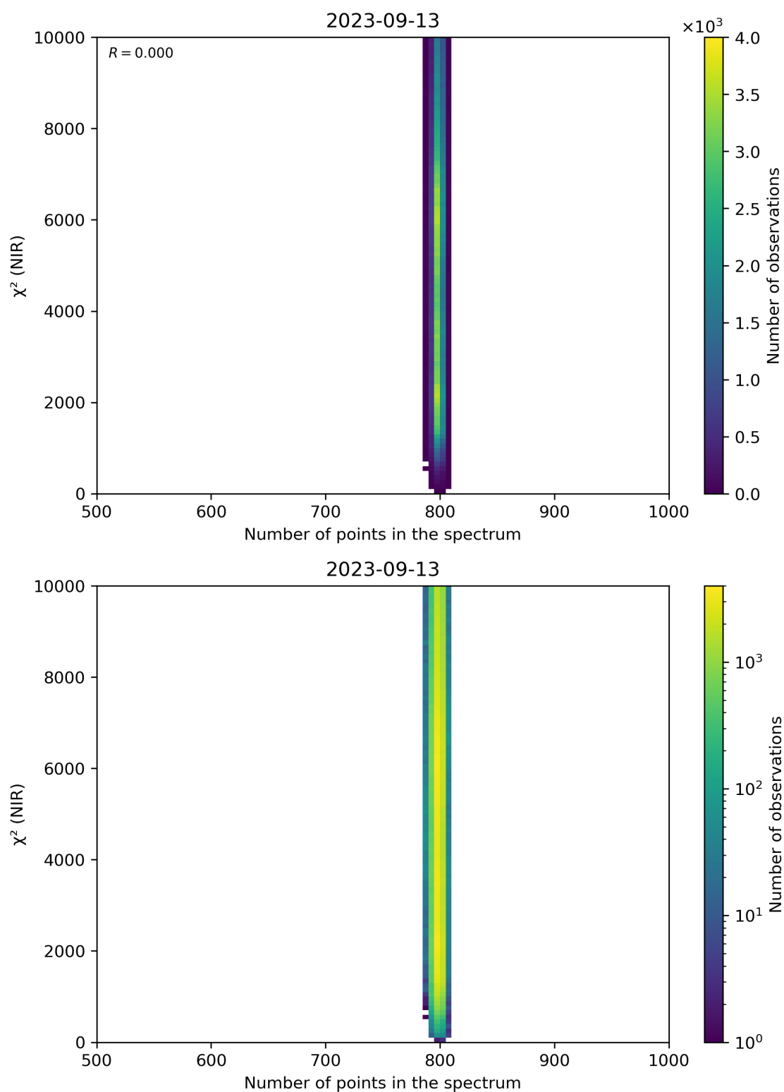
Figure 88: Scatter density plot of “Number of points in the spectrum” against “ \chi^2 (NIR)” for 2023-09-12 to 2023-09-14.
