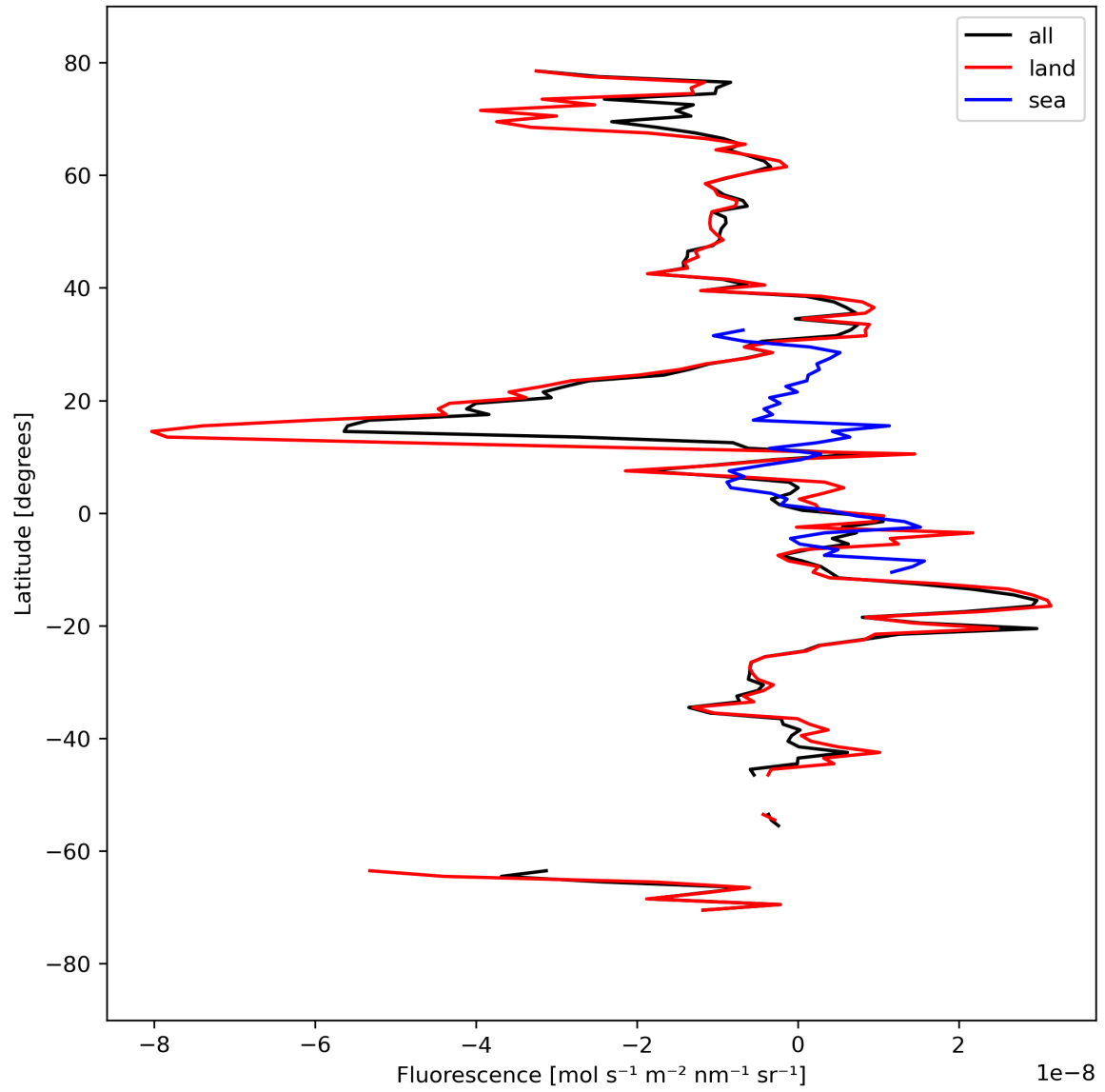
Figure 21: Zonal average of “Fluorescence” for 2023-09-12 to 2023-09-14.
