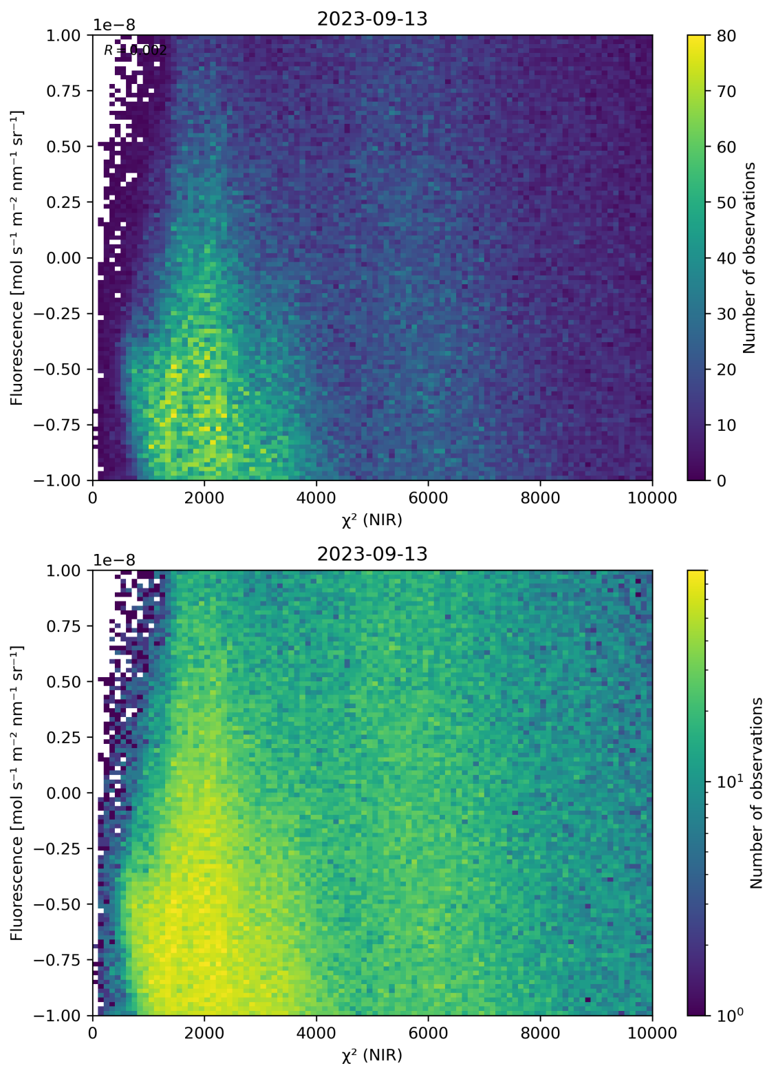
Figure 45: Scatter density plot of “ \chi^2 (NIR)” against “Fluorescence” for 2023-09-12 to 2023-09-14.
