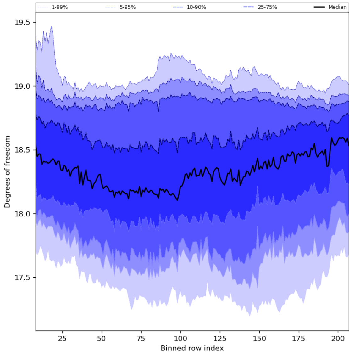
Figure 41: Along track statistics of “Degrees of freedom” for 2023-09-12 to 2023-09-14
