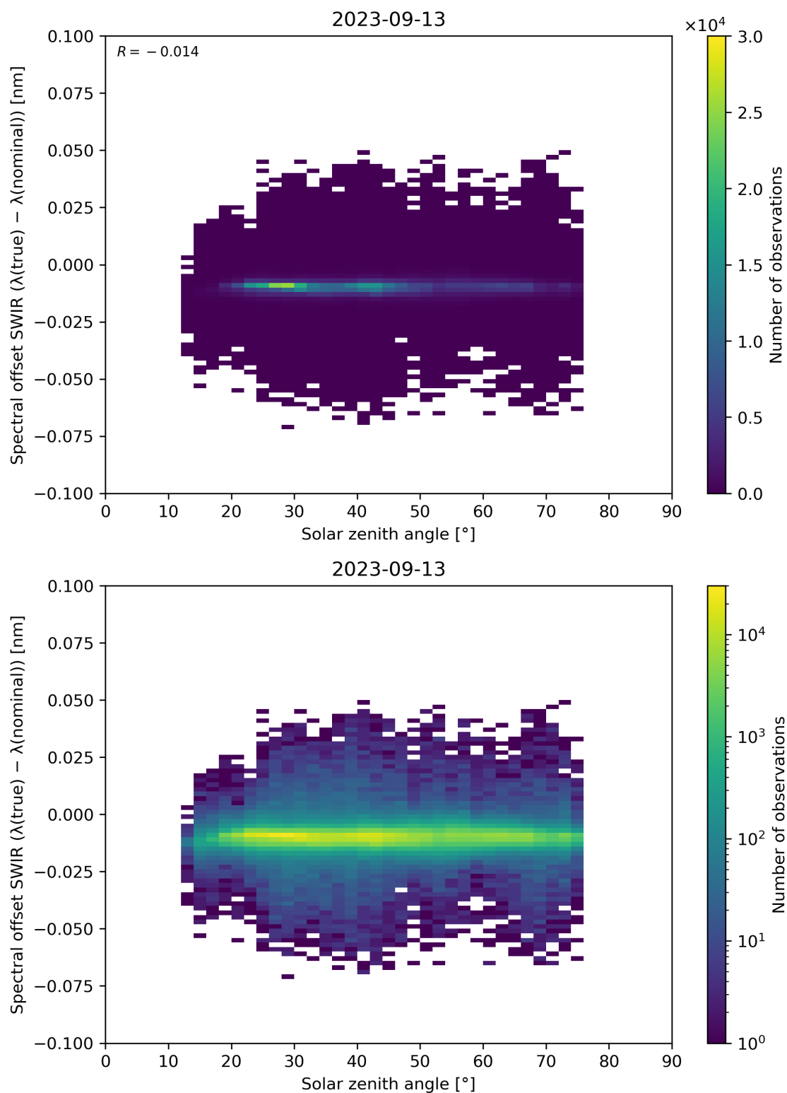
Figure 104: Scatter density plot of “Solar zenith angle” against “Spectral offset SWIR ( \lambda(\text{true}) - \lambda(\text{nominal}) )” for 2023-09-12 to 2023-09-14.
