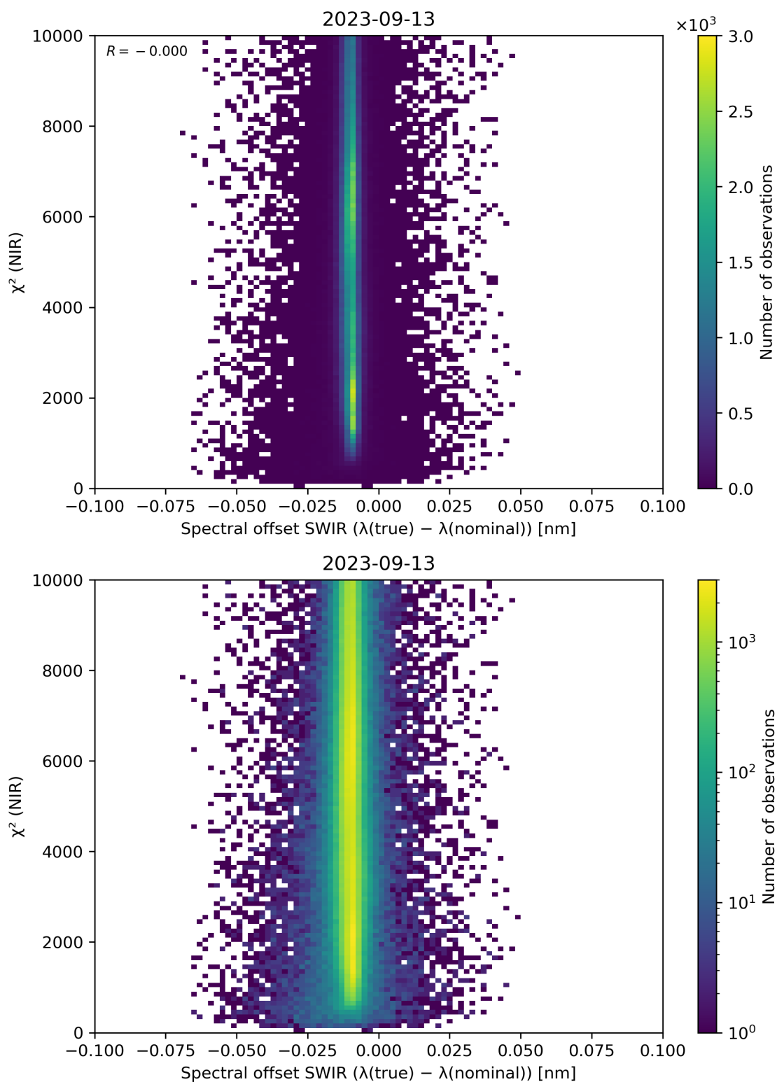
Figure 117: Scatter density plot of “Spectral offset SWIR ( \lambda(\text{true}) - \lambda(\text{nominal}) )” against “ \chi^2 (NIR)” for 2023-09-12 to 2023-09-14.
