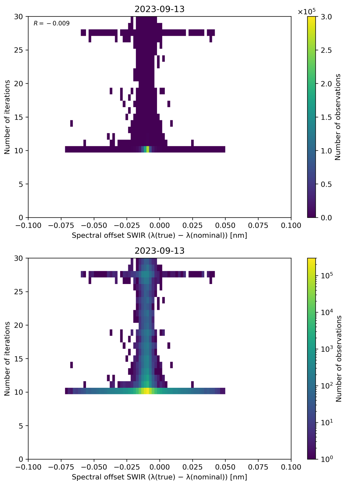
Figure 121: Scatter density plot of “Spectral offset SWIR ( \lambda(\text{true}) - \lambda(\text{nominal}) )” against “Number of iterations” for 2023-09-12 to 2023-09-14.
