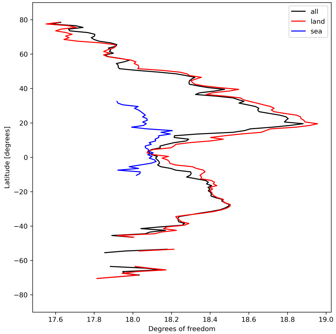
Figure 19: Zonal average of “Degrees of freedom” for 2023-09-12 to 2023-09-14.
