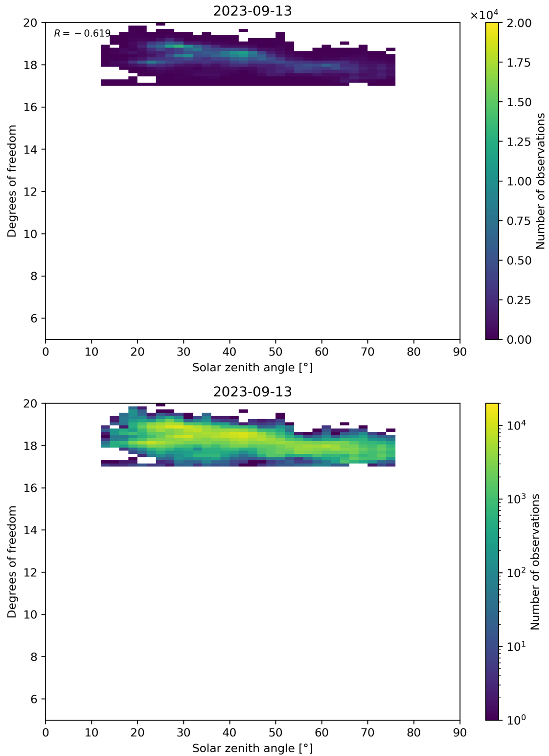
Figure 96: Scatter density plot of “Solar zenith angle” against “Degrees of freedom” for 2023-09-12 to 2023-09-14.
