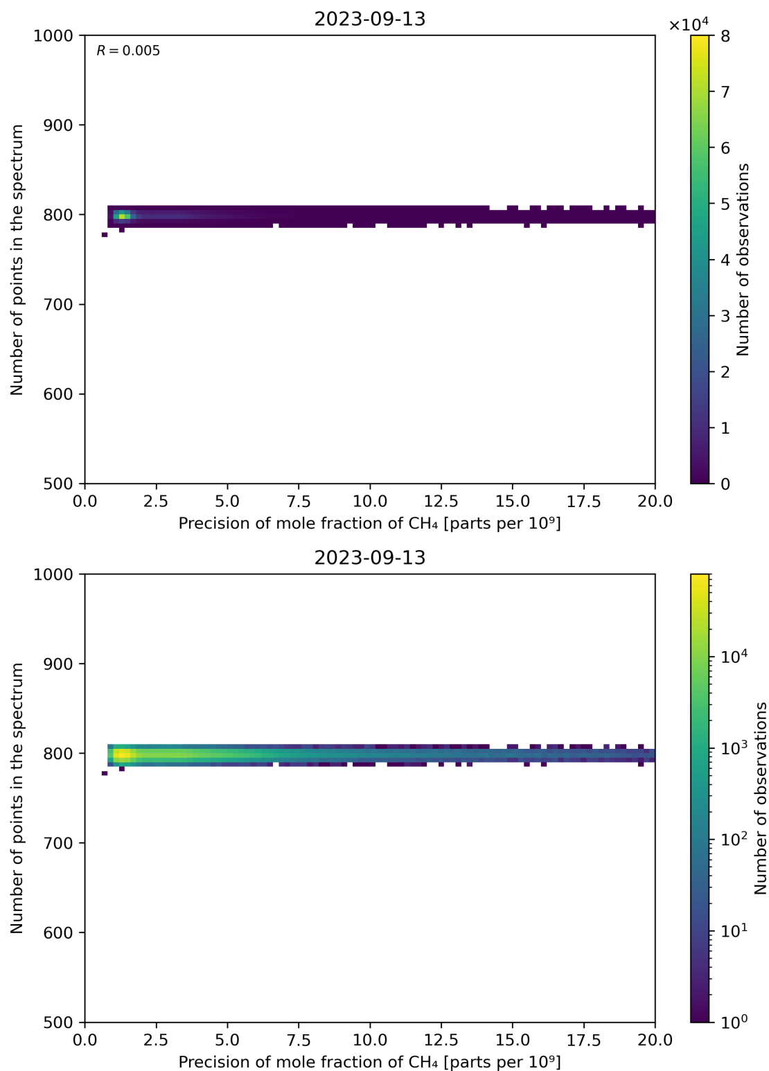
Figure 84: Scatter density plot of “Precision of mole fraction of \text{CH}_4 ” against “Number of points in the spectrum” for 2023-09-12 to 2023-09-14.
