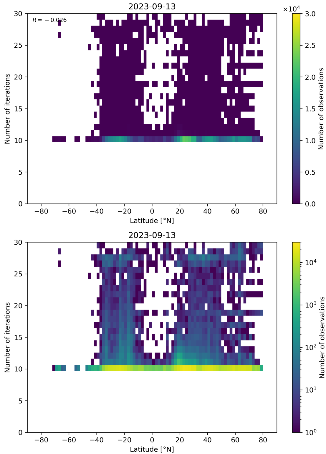
Figure 60: Scatter density plot of “Latitude” against “Number of iterations” for 2023-09-12 to 2023-09-14.
