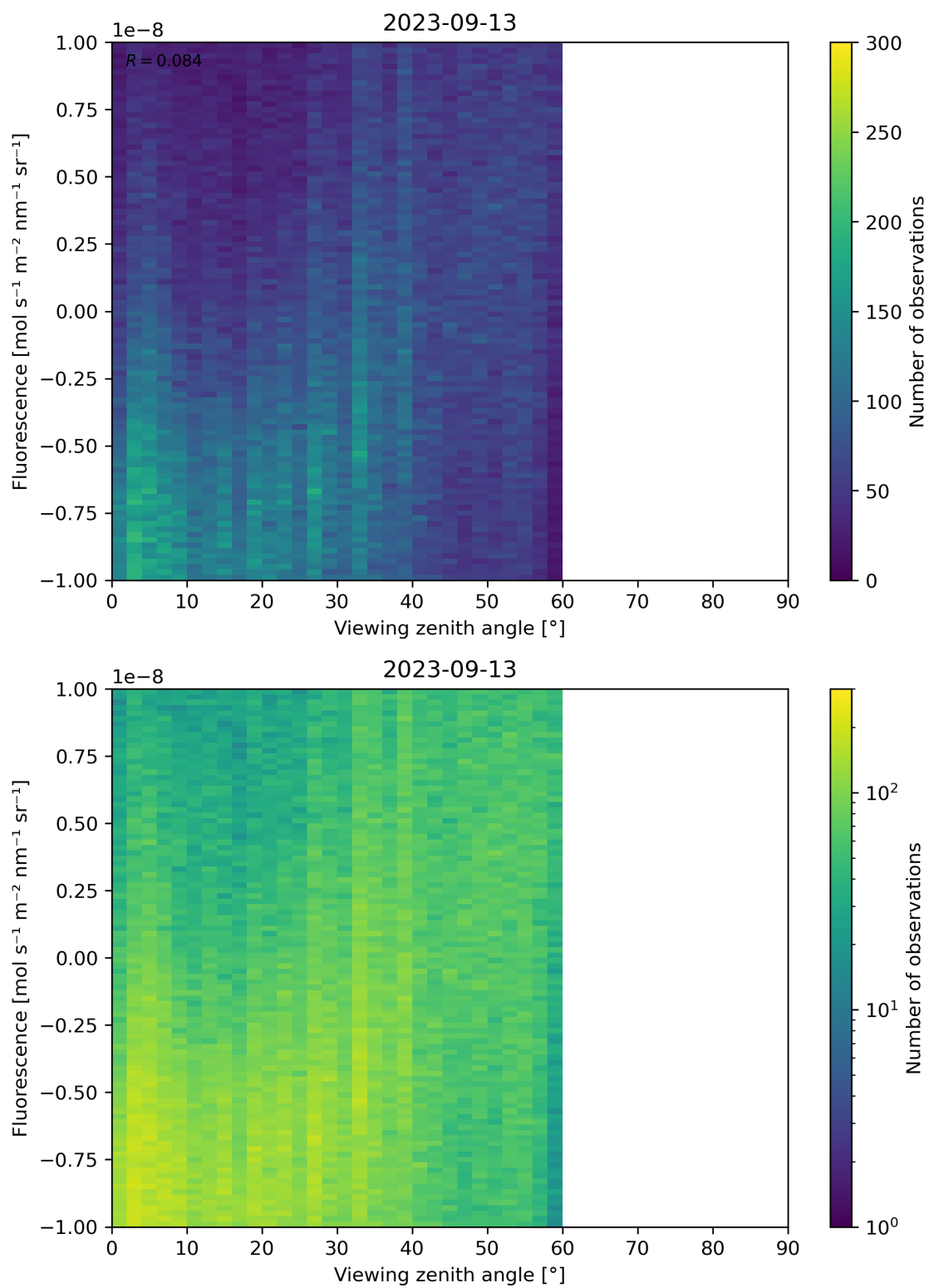
Figure 108: Scatter density plot of “Viewing zenith angle” against “Fluorescence” for 2023-09-12 to 2023-09-14.
