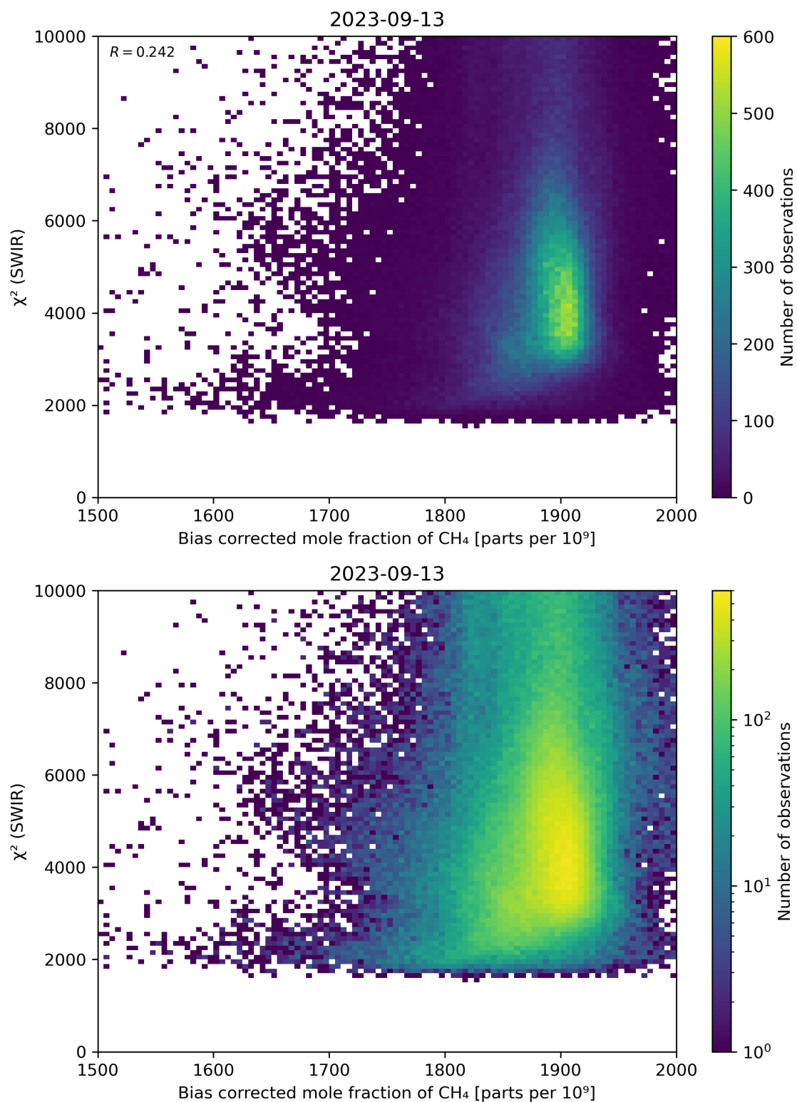
Figure 64: Scatter density plot of “Bias corrected mole fraction of CH 4 ” against “ \chi^2 (SWIR)” for 2023-09-12 to 2023-09-14.
