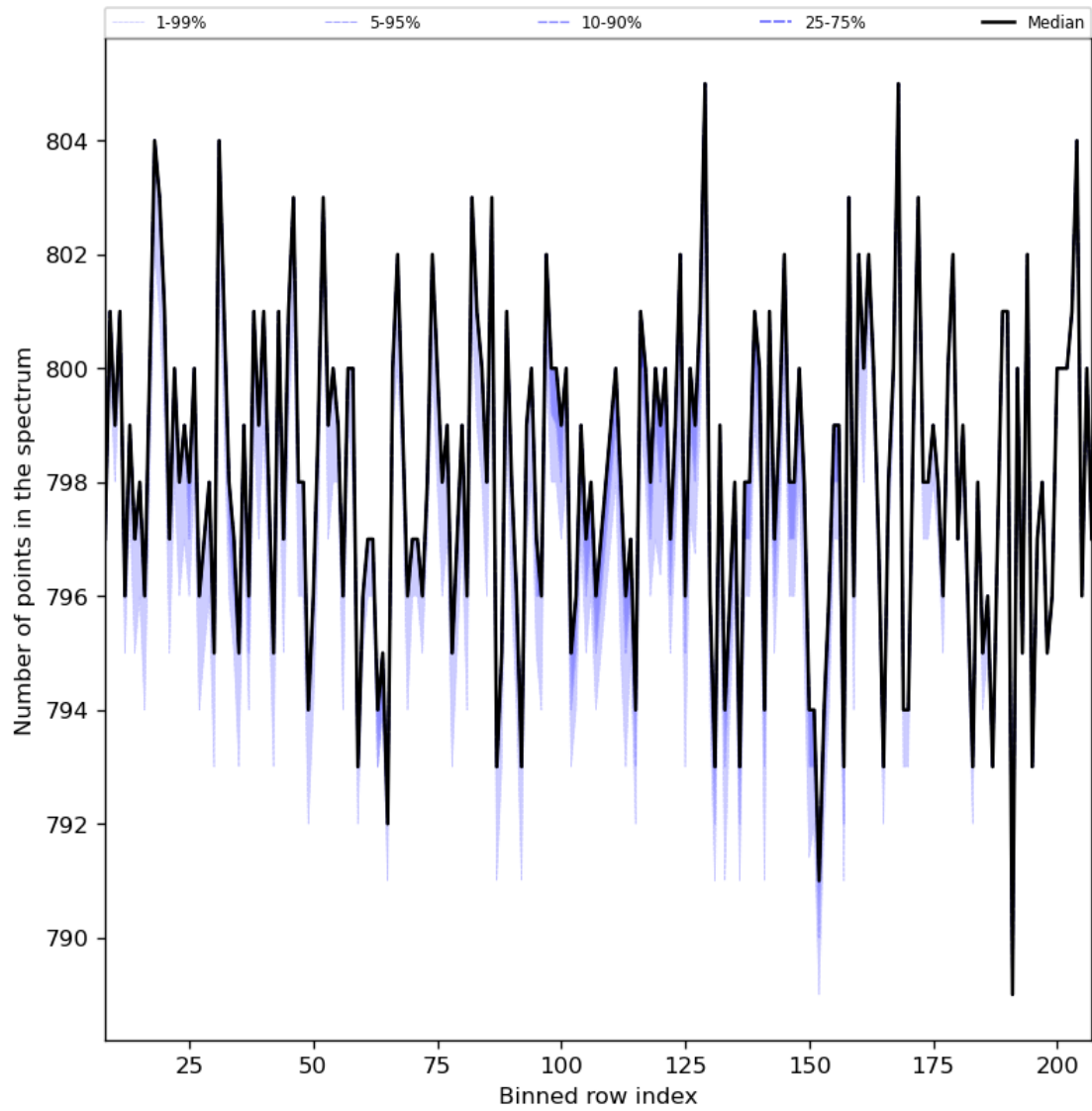
Figure 37: Along track statistics of “Number of points in the spectrum” for 2023-09-12 to 2023-09-14
