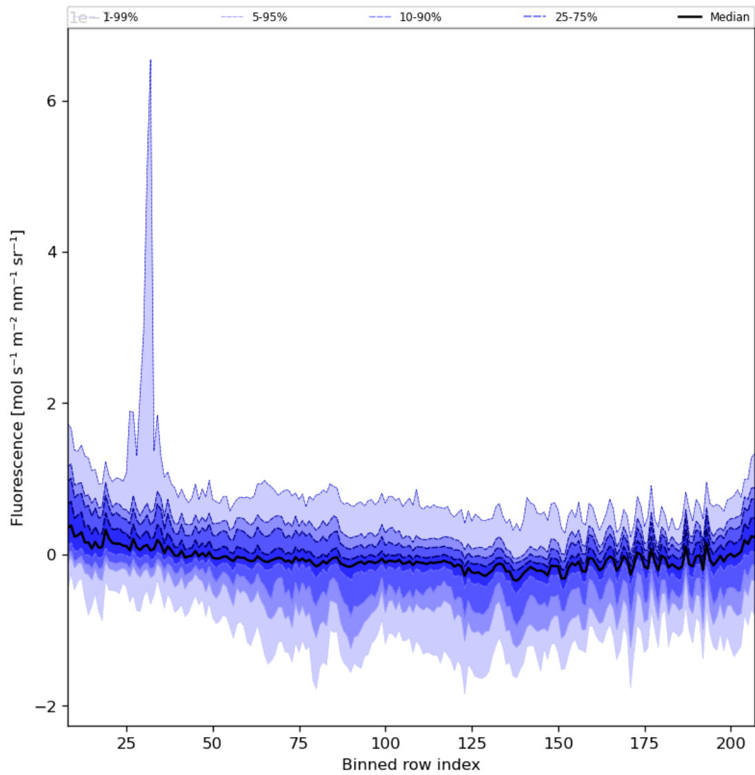
Figure 43: Along track statistics of “Fluorescence” for 2023-09-12 to 2023-09-14
