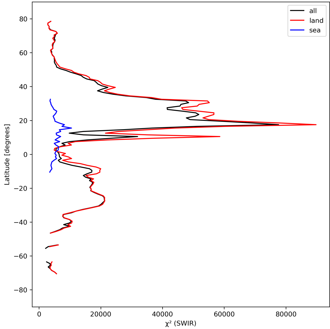
Figure 17: Zonal average of “ \chi^2 (SWIR)” for 2023-09-12 to 2023-09-14.
