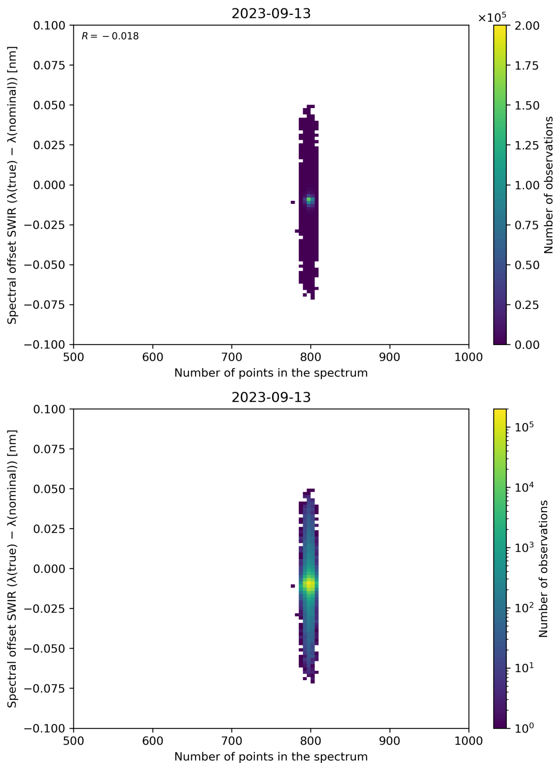
Figure 93: Scatter density plot of “Number of points in the spectrum” against “Spectral offset SWIR ( \lambda(\text{true}) - \lambda(\text{nominal}) )” for 2023-09-12 to 2023-09-14.
