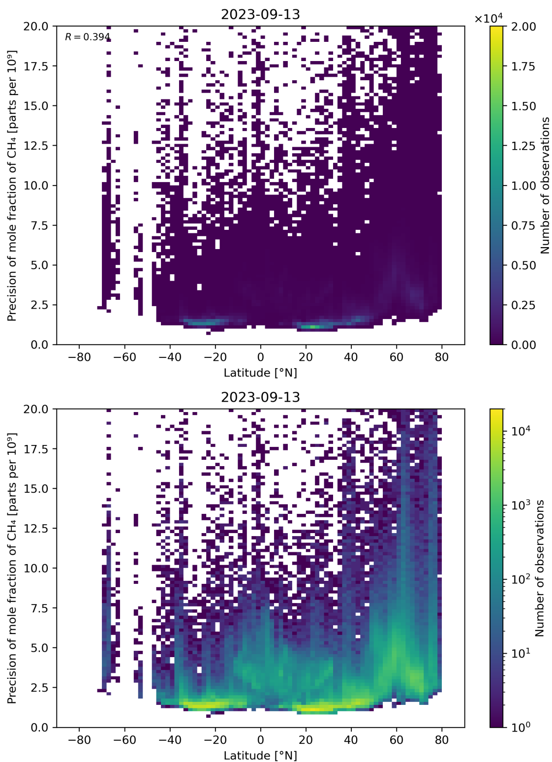
Figure 59: Scatter density plot of “Latitude” against “Precision of mole fraction of \text{CH}_4 ” for 2023-09-12 to 2023-09-14.
