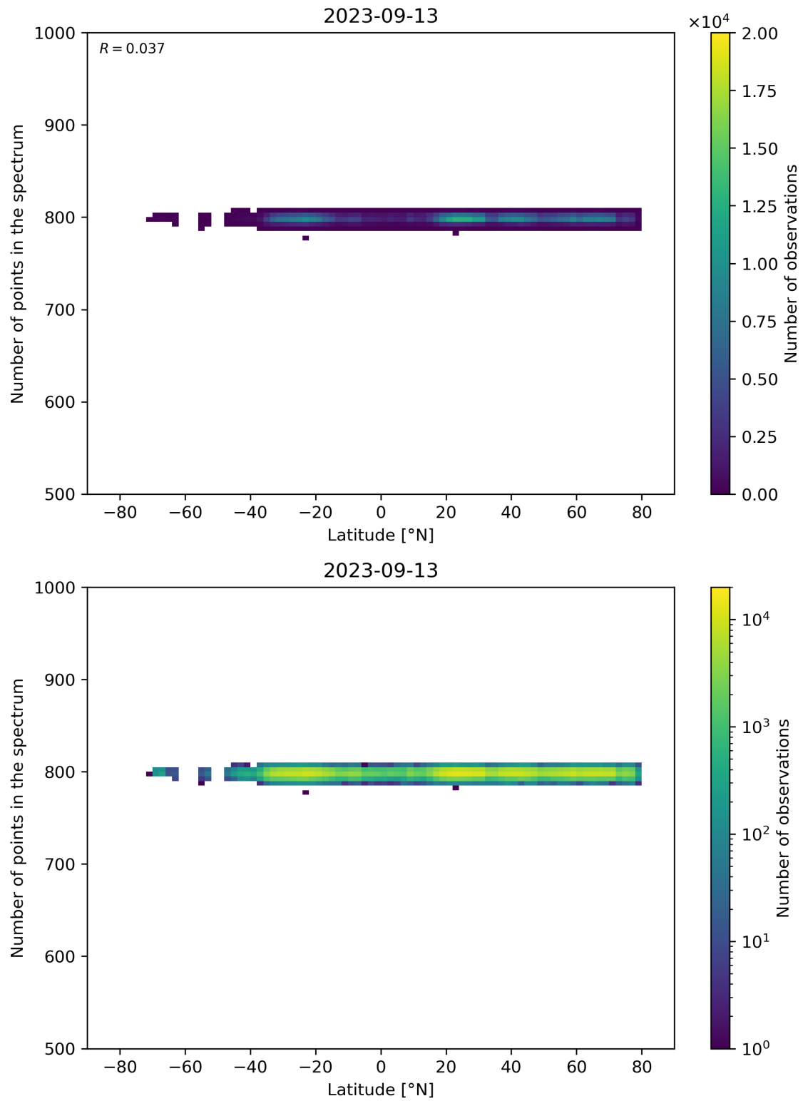
Figure 61: Scatter density plot of “Latitude” against “Number of points in the spectrum” for 2023-09-12 to 2023-09-14.
