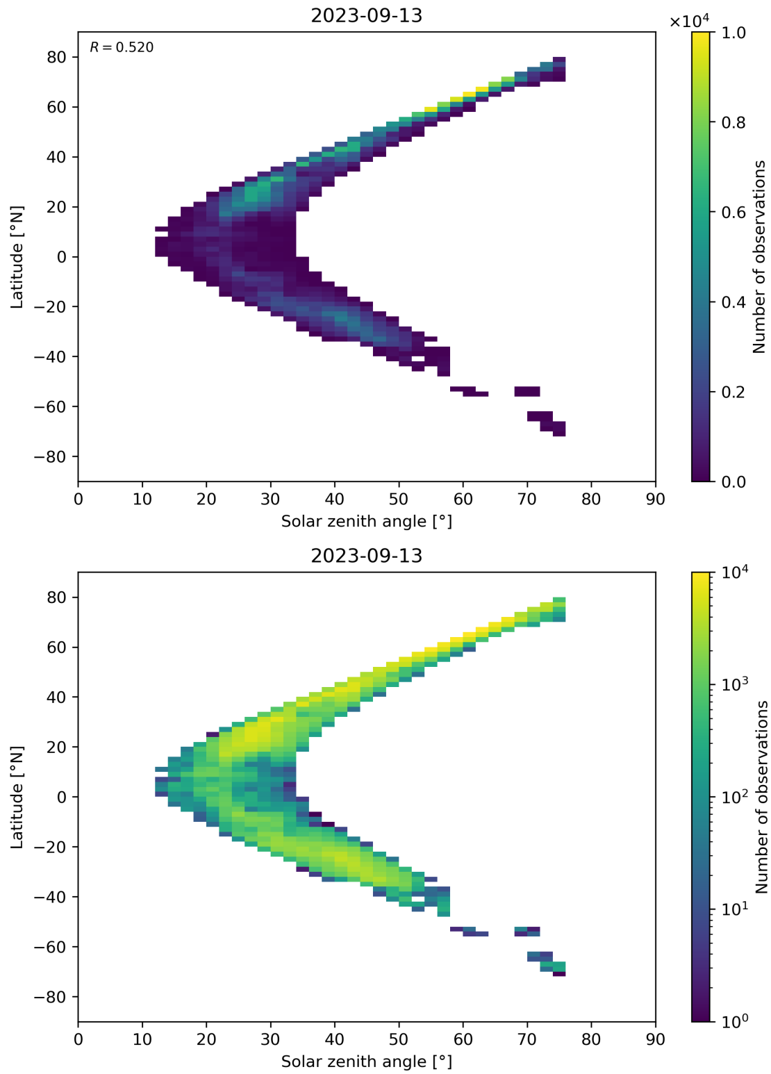
Figure 98: Scatter density plot of “Solar zenith angle” against “Latitude” for 2023-09-12 to 2023-09-14.
