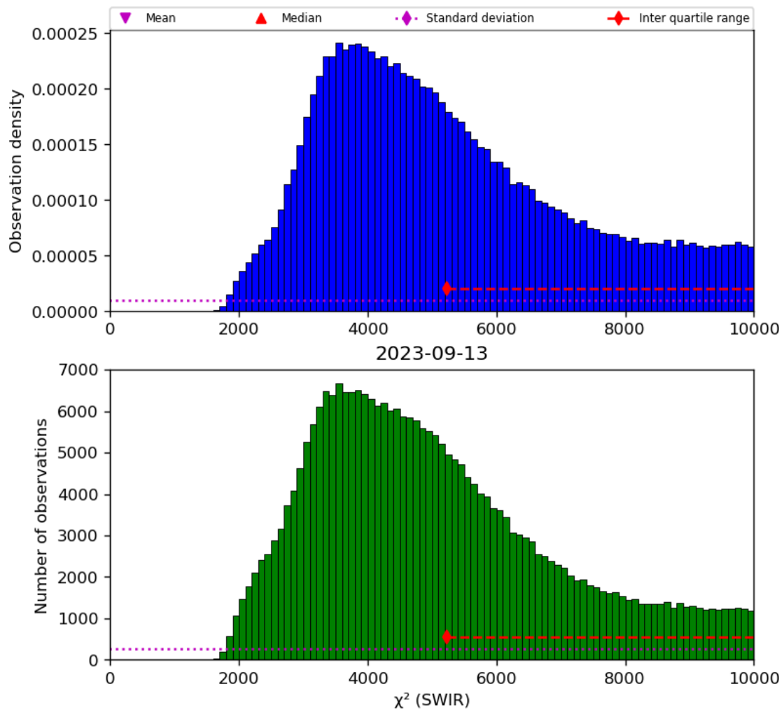
Figure 28: Histogram of “ \chi^2 (SWIR)” for 2023-09-12 to 2023-09-14
