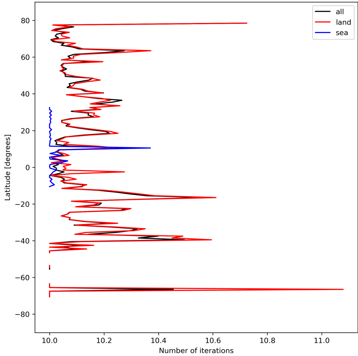
Figure 20: Zonal average of “Number of iterations” for 2023-09-12 to 2023-09-14.
