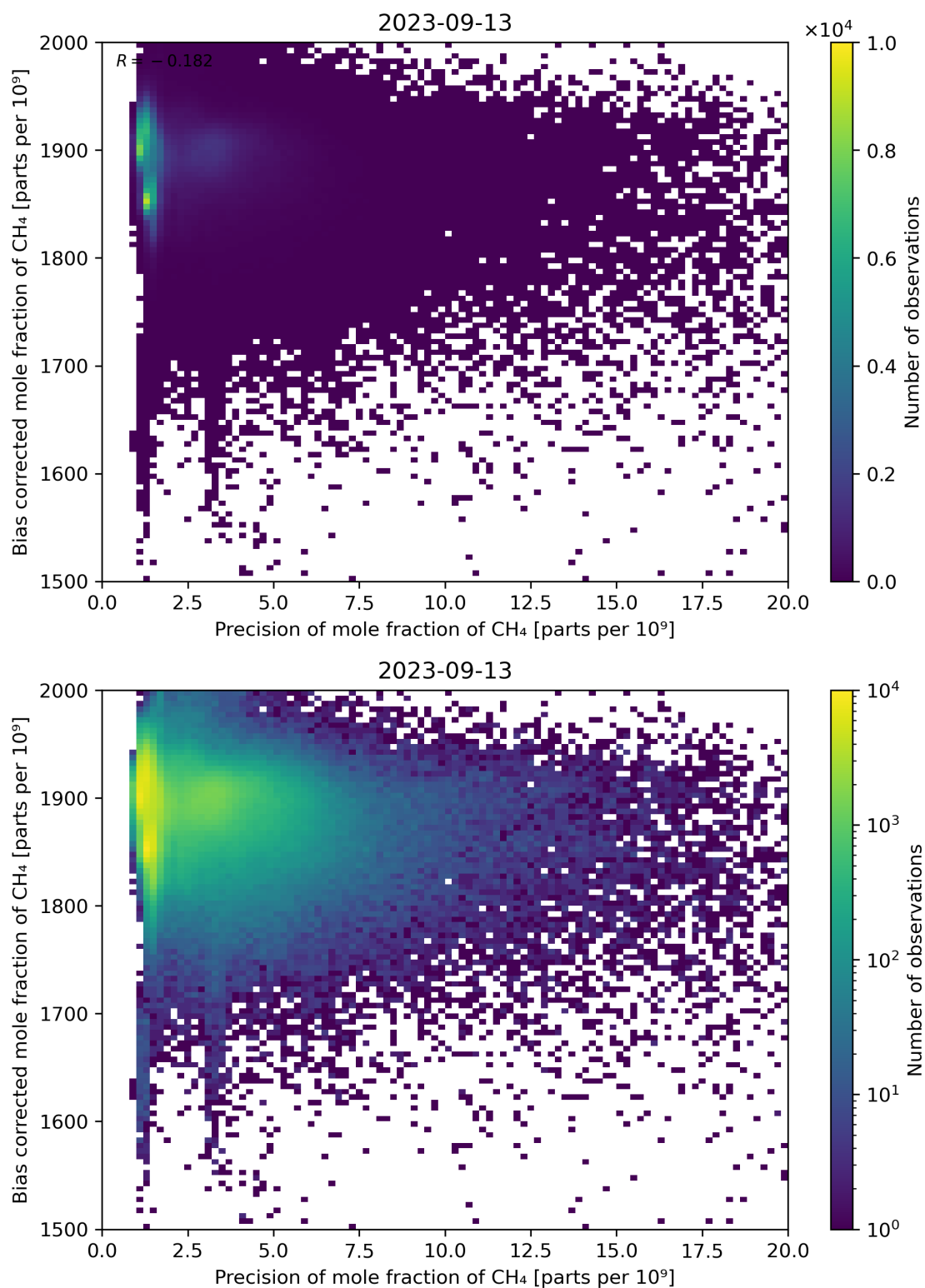
Figure 82: Scatter density plot of “Precision of mole fraction of CH 4 ” against “Bias corrected mole fraction of CH 4 ” for 2023-09-12 to 2023-09-14.
