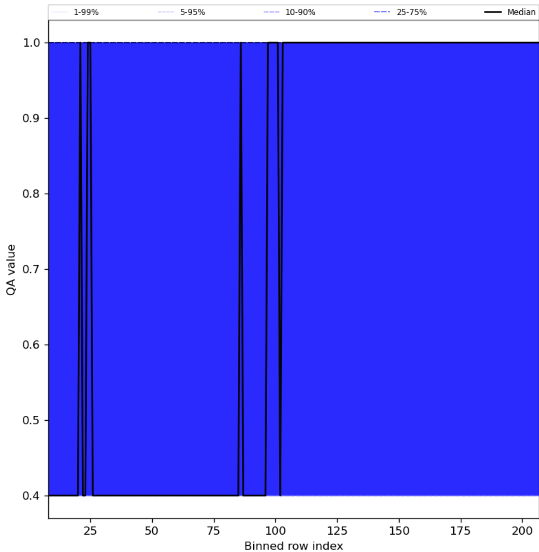
Figure 33: Along track statistics of “QA value” for 2023-09-12 to 2023-09-14
