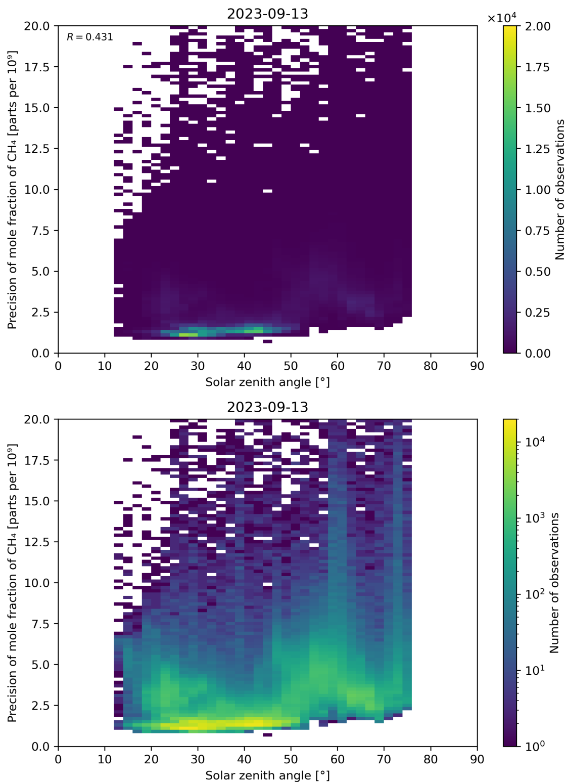
Figure 101: Scatter density plot of “Solar zenith angle” against “Precision of mole fraction of CH 4 ” for 2023-09-12 to 2023-09-14.
