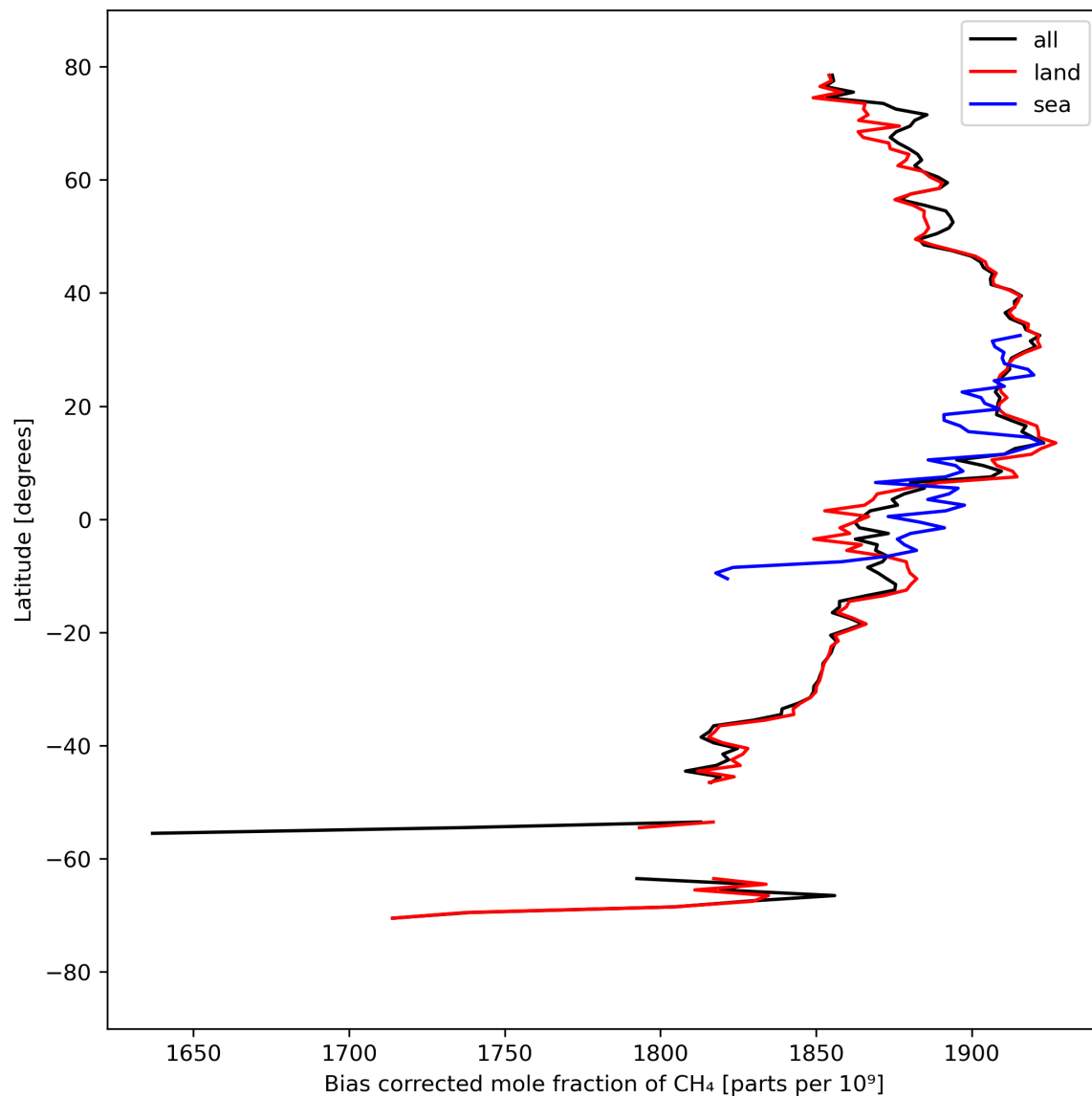
Figure 14: Zonal average of “Bias corrected mole fraction of CH 4 ” for 2023-09-12 to 2023-09-14.
