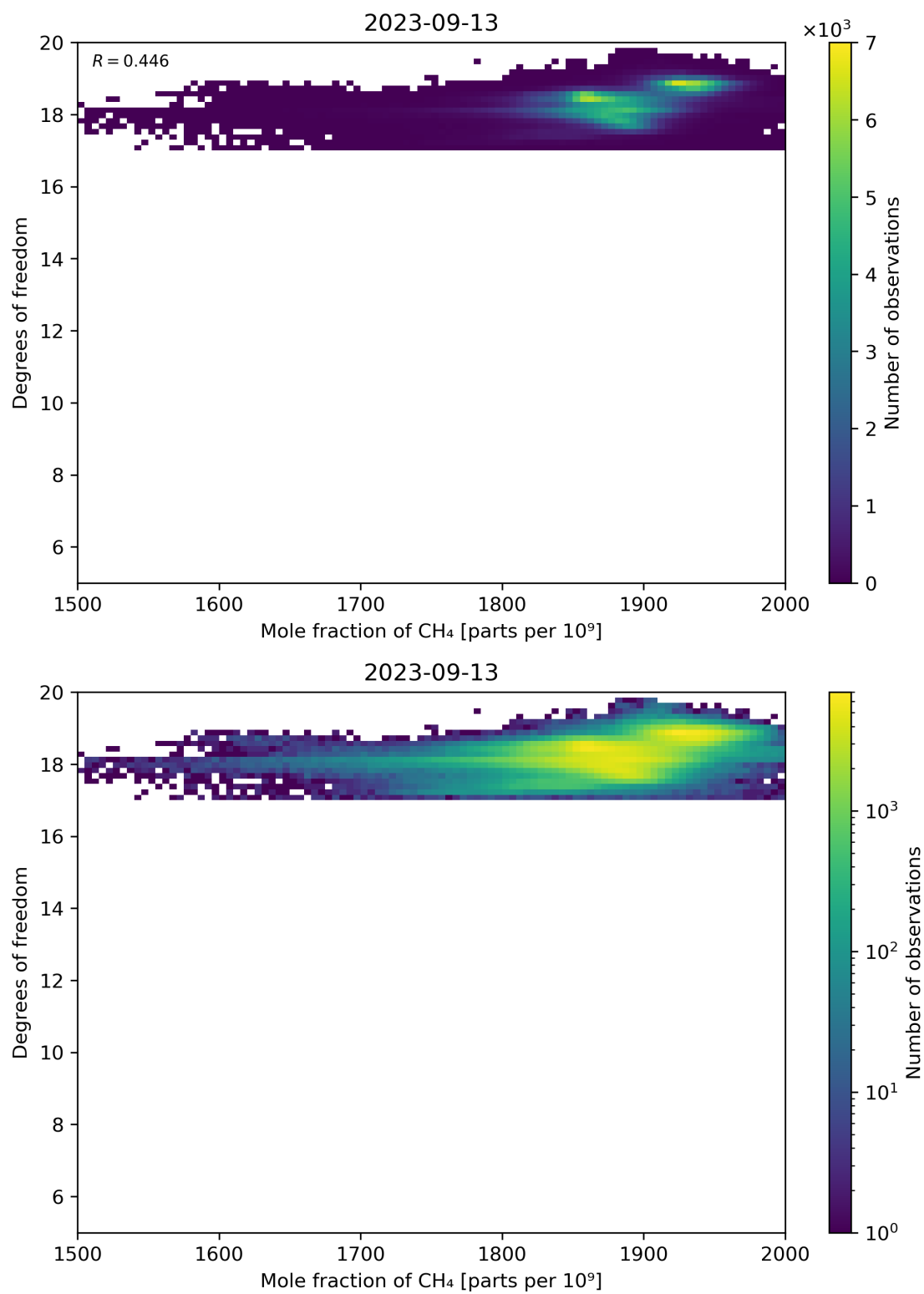
Figure 72: Scatter density plot of “Mole fraction of CH 4 ” against “Degrees of freedom” for 2023-09-12 to 2023-09-14.
