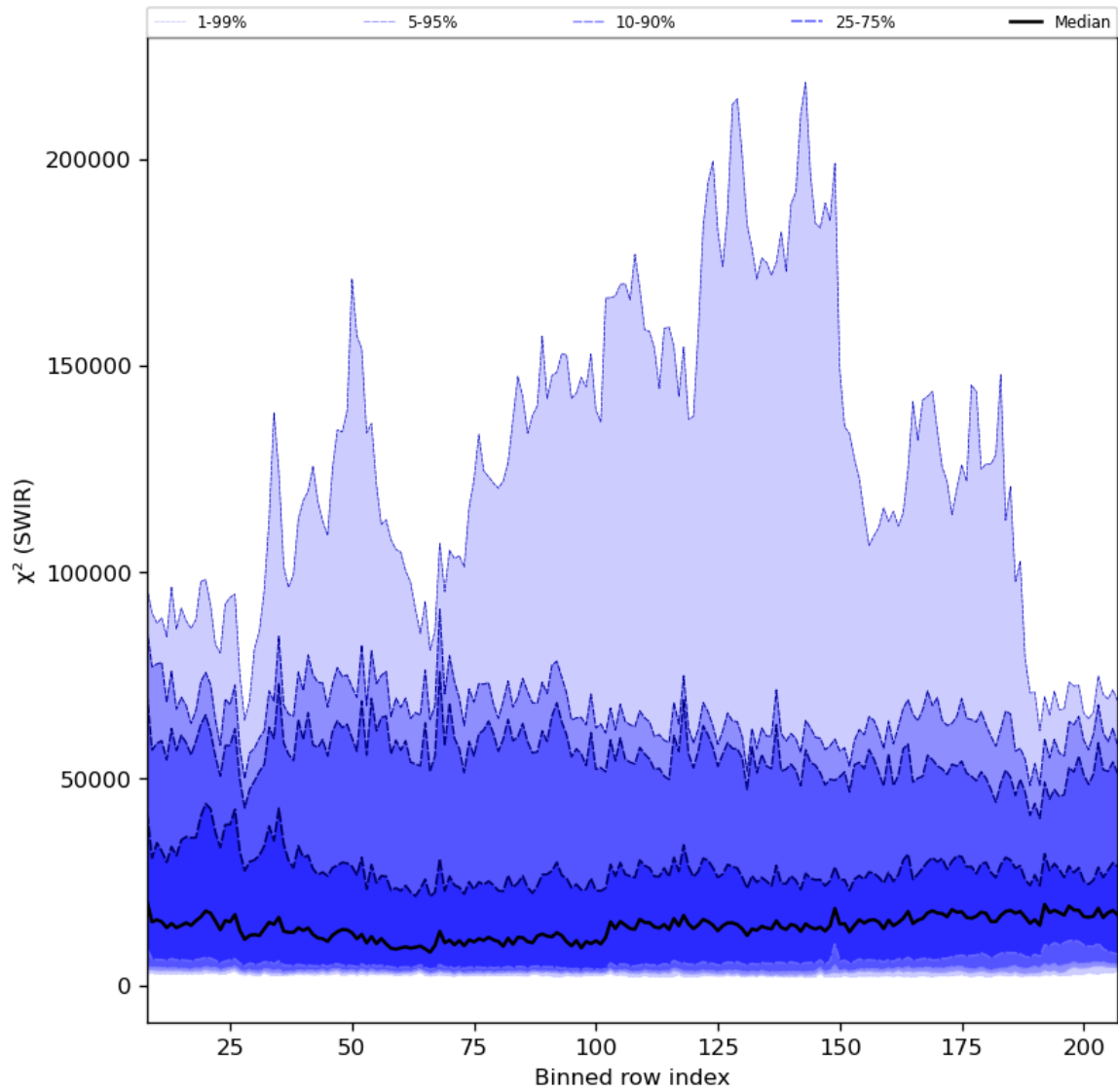
Figure 39: Along track statistics of “ \chi^2 (SWIR)” for 2023-09-12 to 2023-09-14
