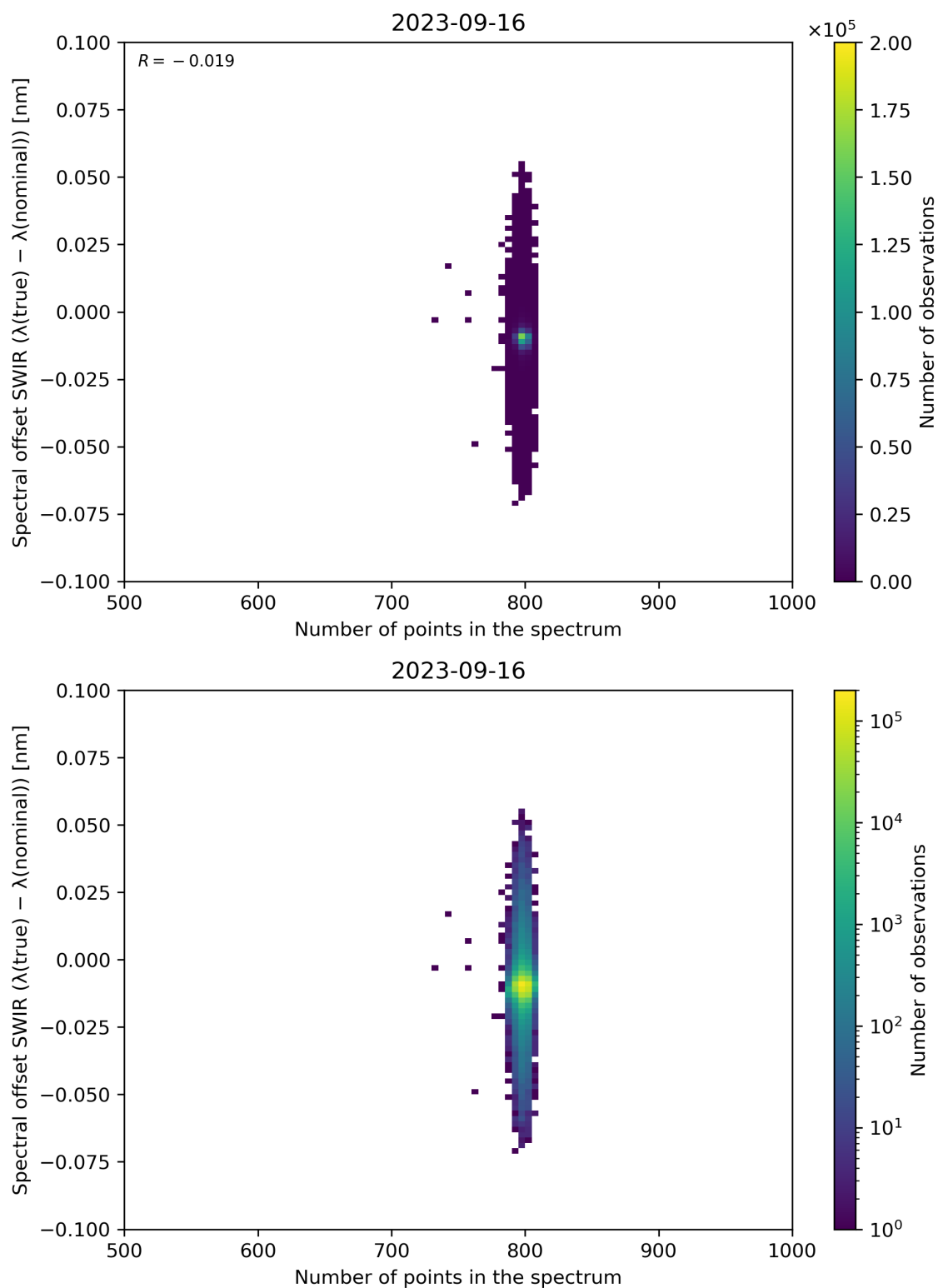
Figure 93: Scatter density plot of “Number of points in the spectrum” against “Spectral offset SWIR ( \lambda(\text{true}) - \lambda(\text{nominal}) )” for 2023-09-15 to 2023-09-17.
