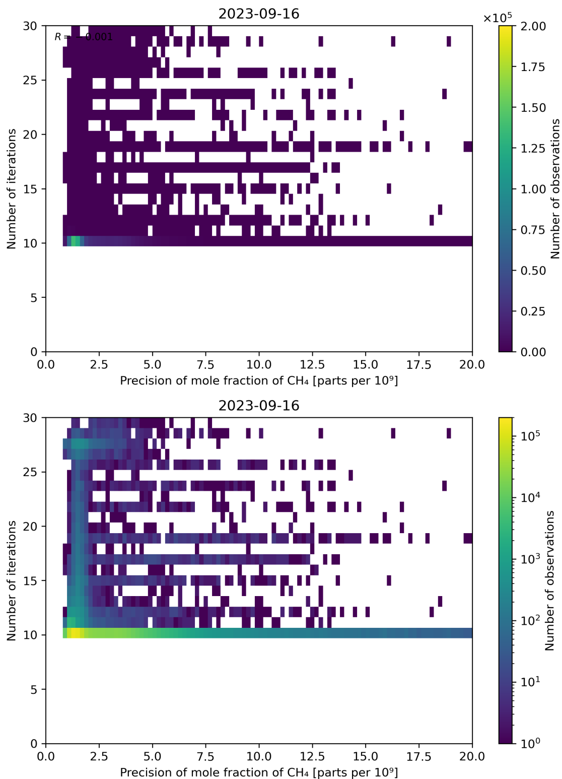
Figure 83: Scatter density plot of “Precision of mole fraction of CH 4 ” against “Number of iterations” for 2023-09-15 to 2023-09-17.
