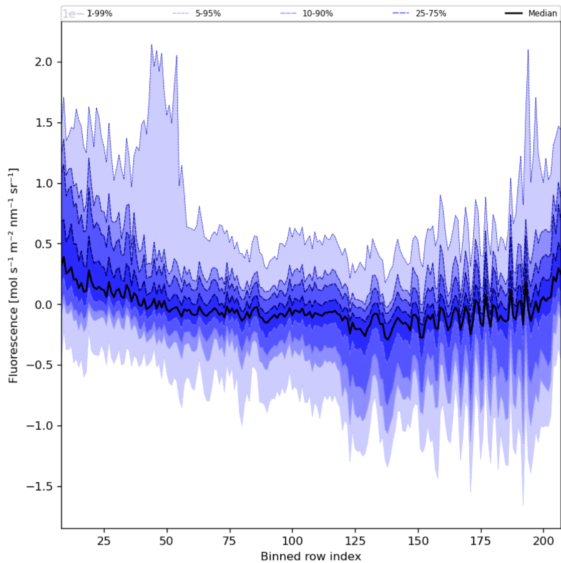
Figure 43: Along track statistics of “Fluorescence” for 2023-09-15 to 2023-09-17
