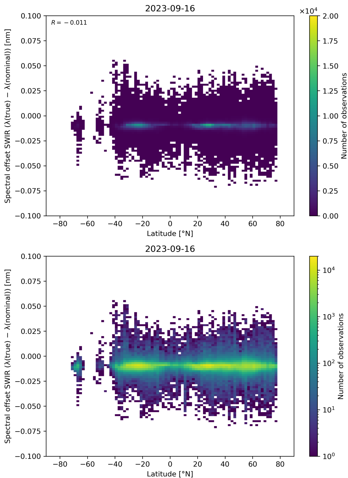
Figure 62: Scatter density plot of “Latitude” against “Spectral offset SWIR ( \lambda(\text{true}) - \lambda(\text{nominal}) )” for 2023-09-15 to 2023-09-17.
