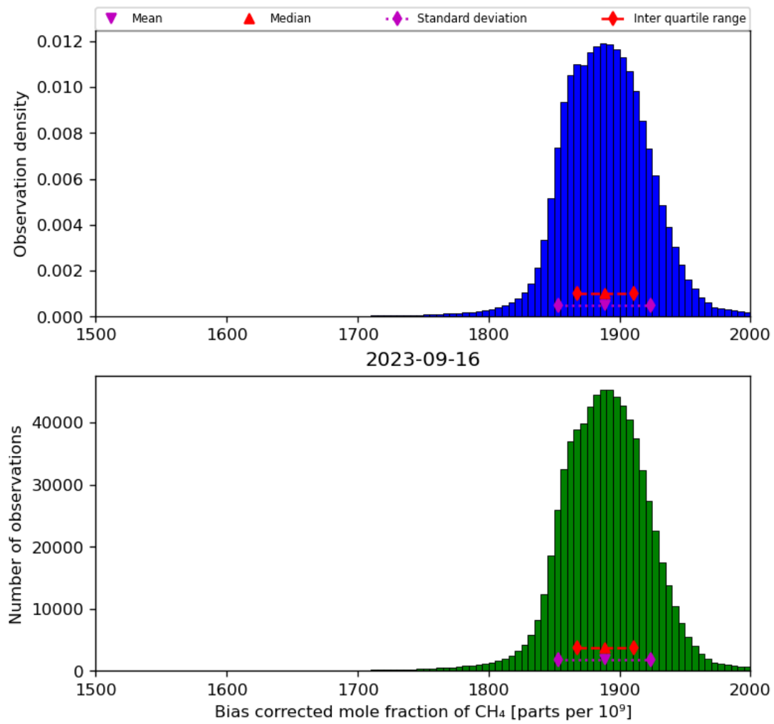
Figure 25: Histogram of “Bias corrected mole fraction of CH 4 ” for 2023-09-15 to 2023-09-17
