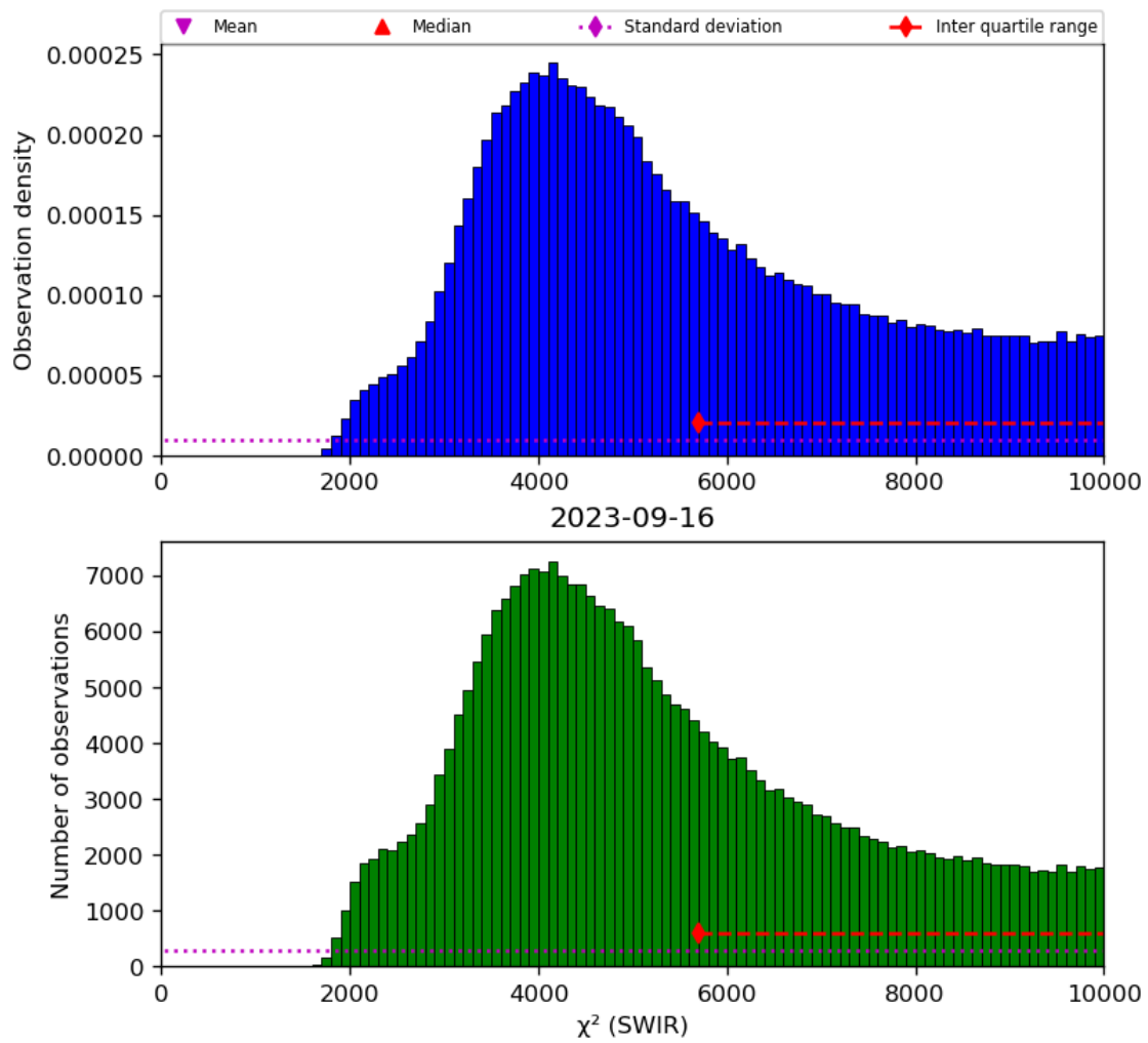
Figure 28: Histogram of “ \chi^2 (SWIR)” for 2023-09-15 to 2023-09-17
