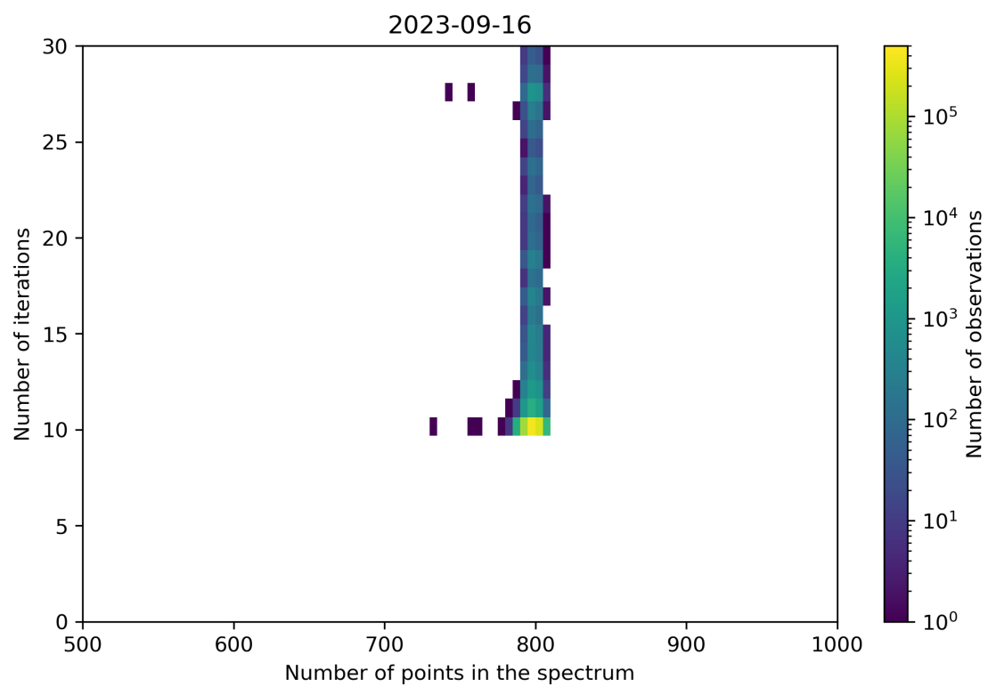
Figure 92: Scatter density plot of “Number of points in the spectrum” against “Number of iterations” for 2023-09-15 to 2023-09-17.
