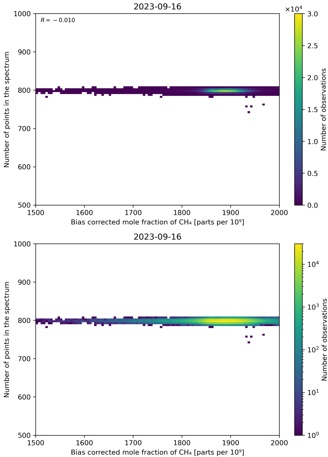
Figure 68: Scatter density plot of “Bias corrected mole fraction of CH 4 ” against “Number of points in the spectrum” for 2023-09-15 to 2023-09-17.
