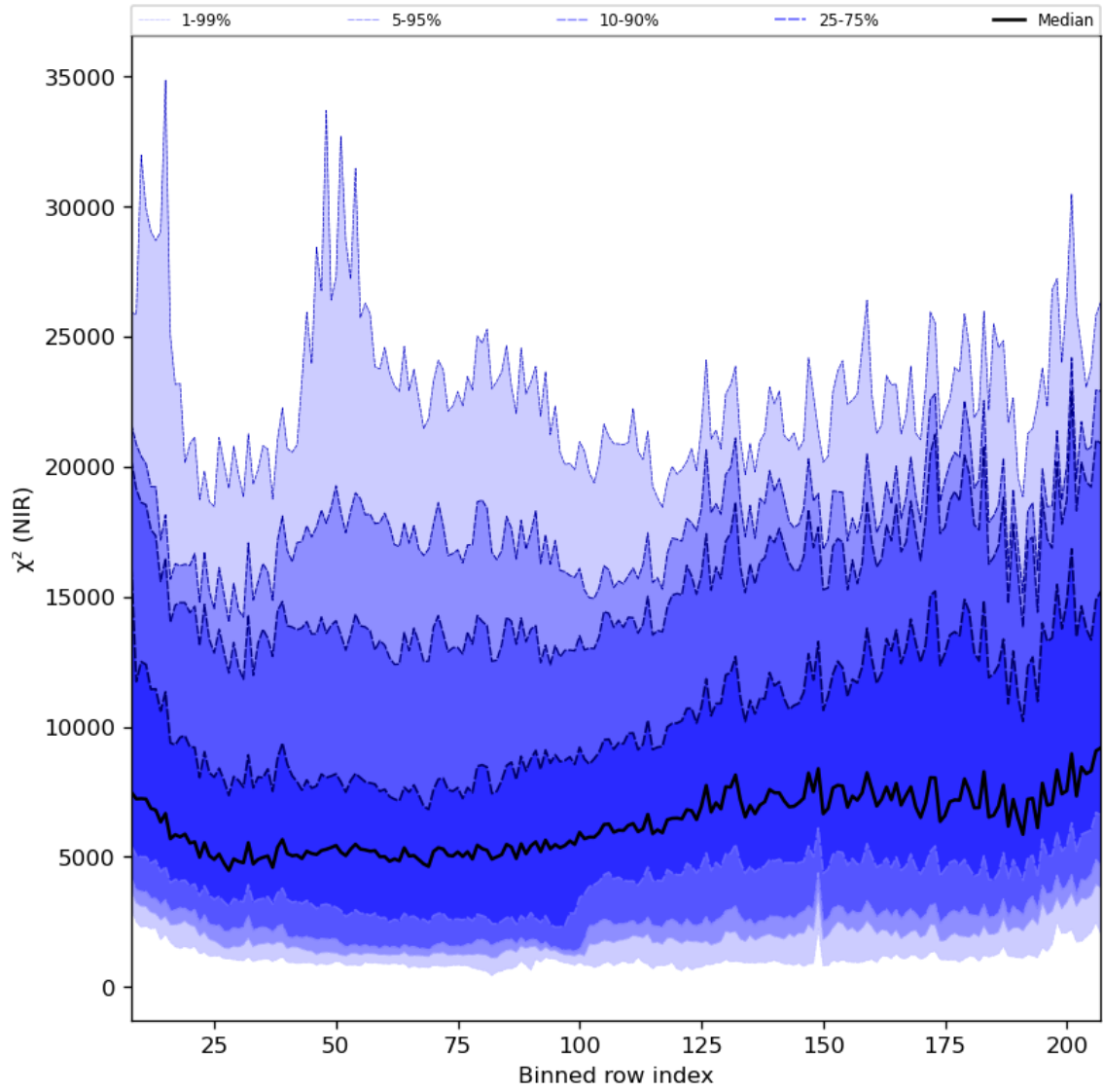
Figure 40: Along track statistics of “ \chi^2 (NIR)” for 2023-09-15 to 2023-09-17
