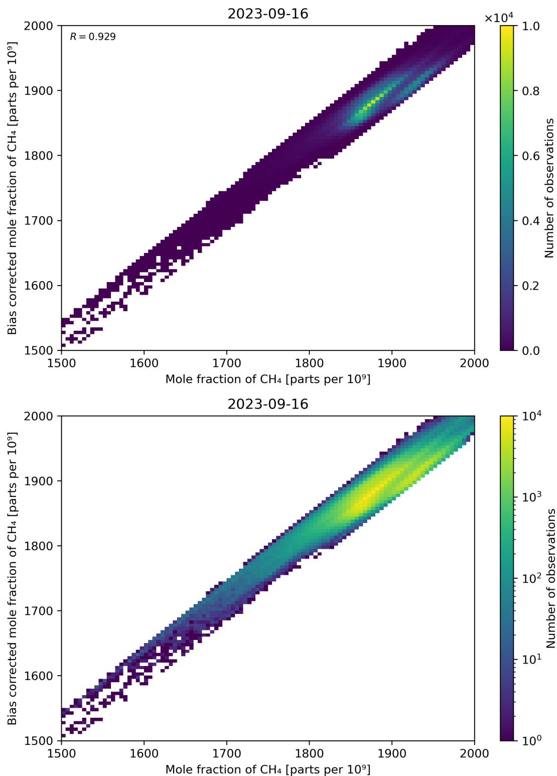
Figure 74: Scatter density plot of “Mole fraction of CH 4 ” against “Bias corrected mole fraction of CH 4 ” for 2023-09-15 to 2023-09-17.
