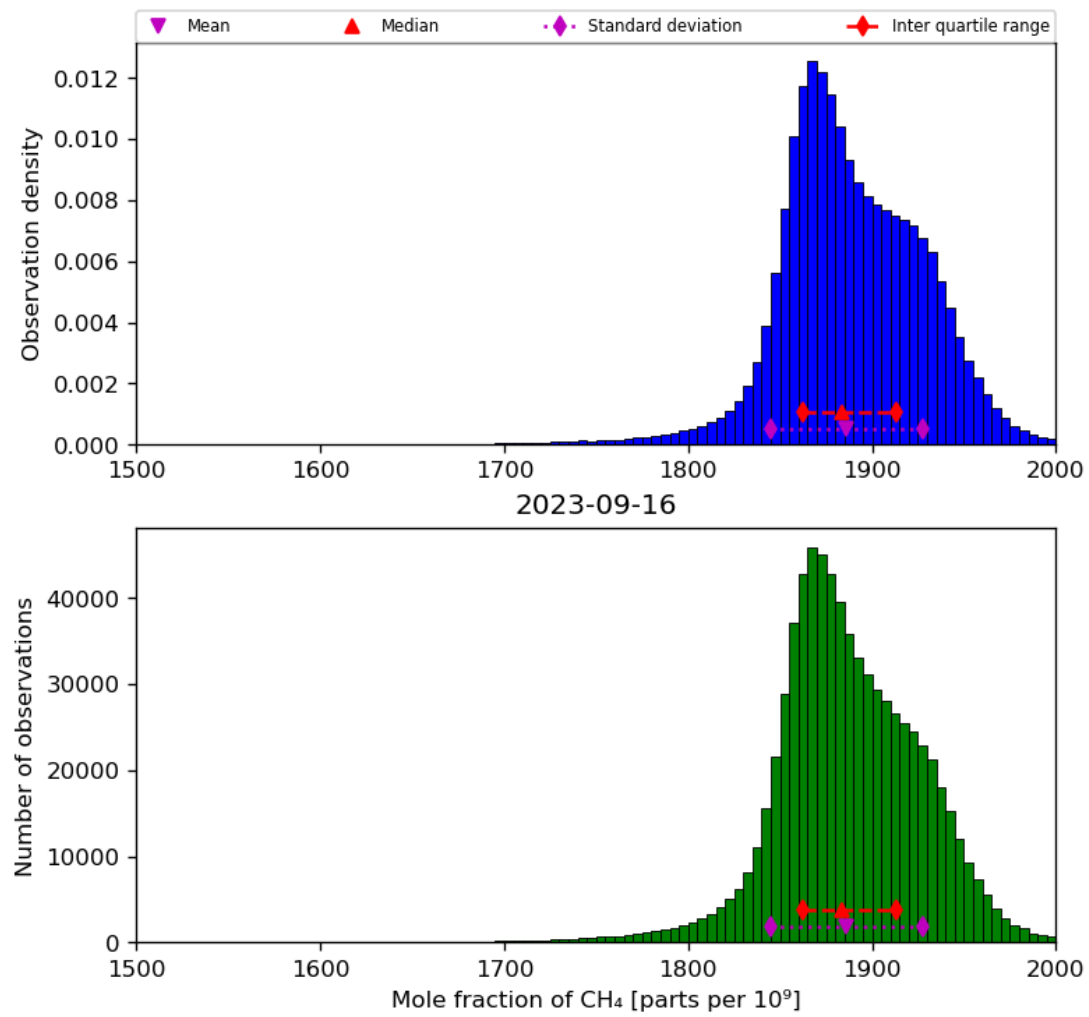
Figure 23: Histogram of “Mole fraction of CH 4 ” for 2023-09-15 to 2023-09-17
