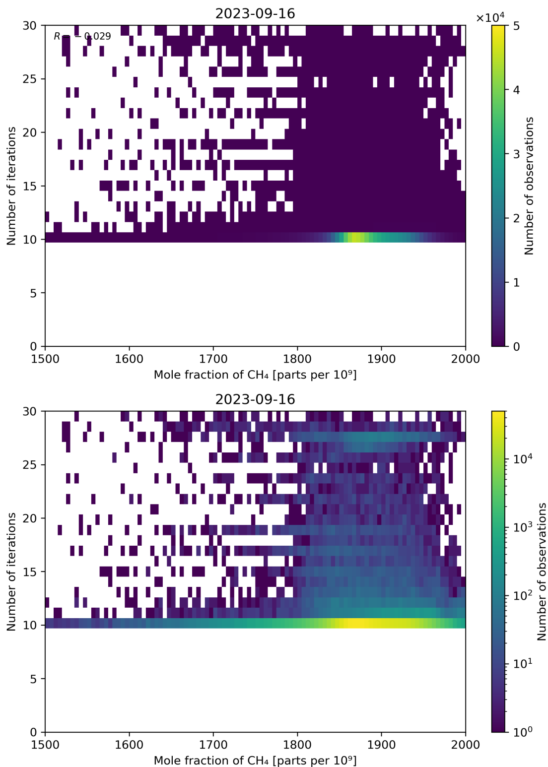
Figure 76: Scatter density plot of “Mole fraction of CH 4 ” against “Number of iterations” for 2023-09-15 to 2023-09-17.
