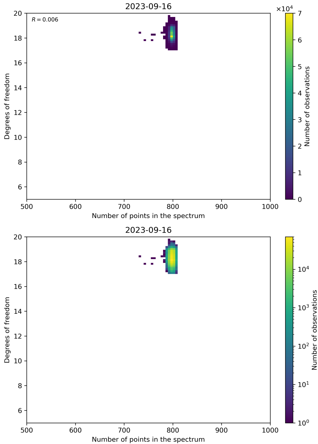
Figure 90: Scatter density plot of “Number of points in the spectrum” against “Degrees of freedom” for 2023-09-15 to 2023-09-17.
