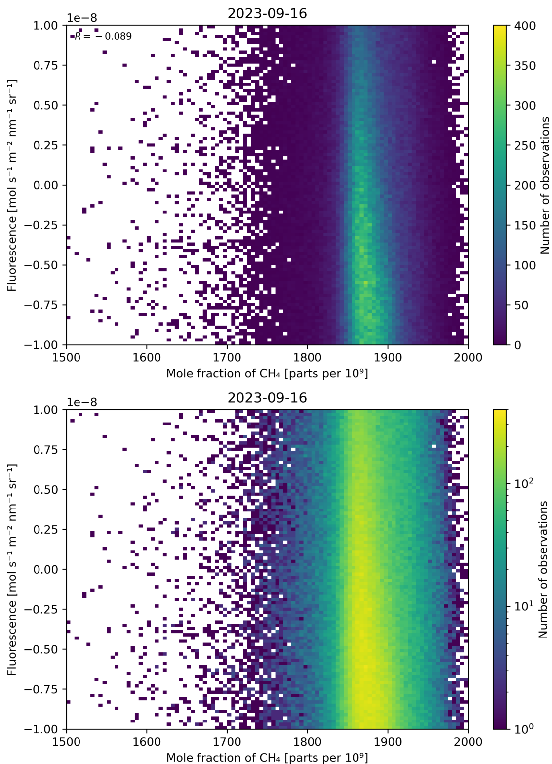
Figure 73: Scatter density plot of “Mole fraction of \text{CH}_4 ” against “Fluorescence” for 2023-09-15 to 2023-09-17.
