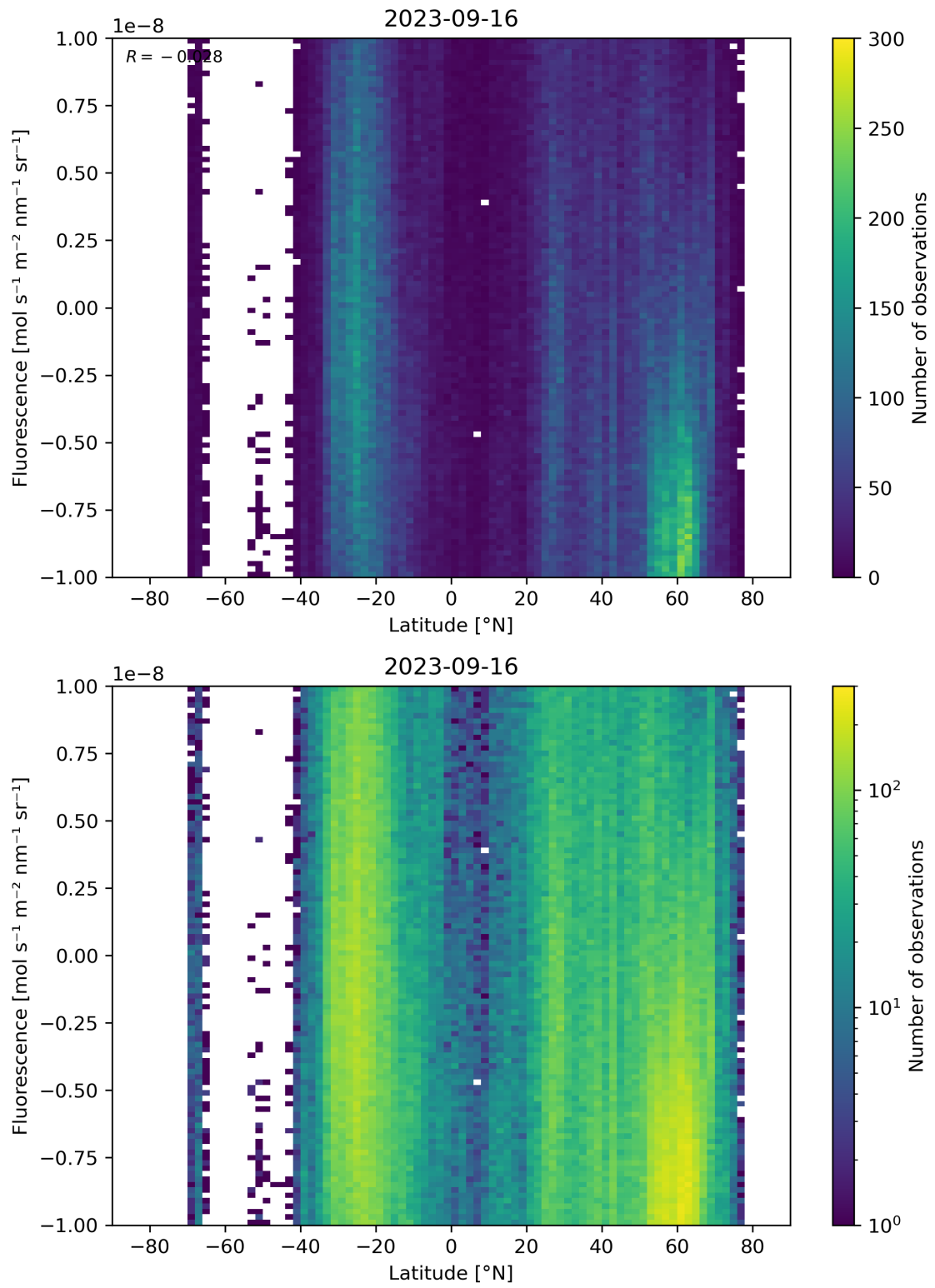
Figure 56: Scatter density plot of “Latitude” against “Fluorescence” for 2023-09-15 to 2023-09-17.
