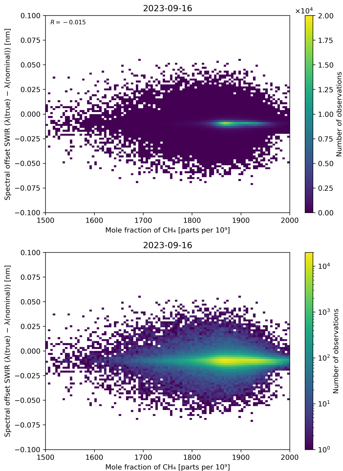
Figure 86: Scatter density plot of “Mole fraction of CH 4 ” against “Spectral offset SWIR ( \lambda(\text{true}) - \lambda(\text{nominal}) )” for 2023-09-15 to 2023-09-17.
