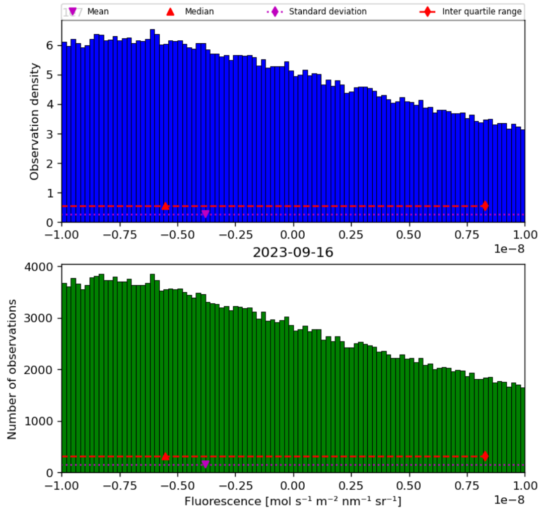
Figure 32: Histogram of “Fluorescence” for 2023-09-15 to 2023-09-17
