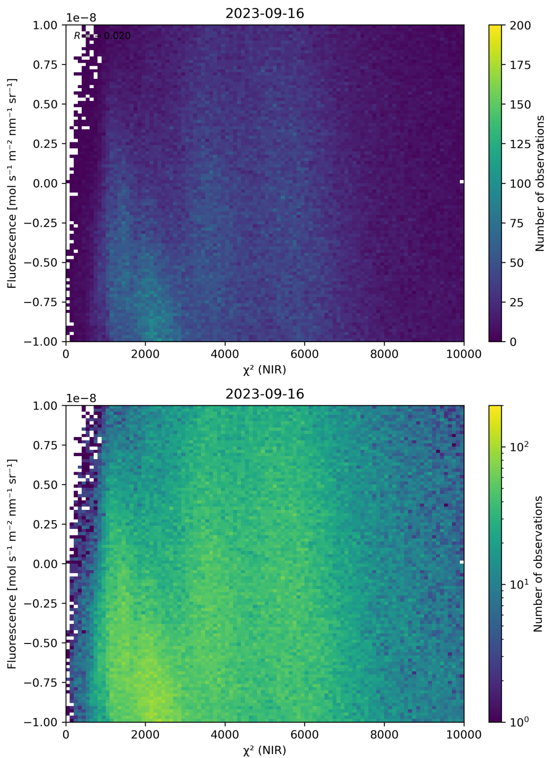
Figure 45: Scatter density plot of “ \chi^2 (NIR)” against “Fluorescence” for 2023-09-15 to 2023-09-17.
