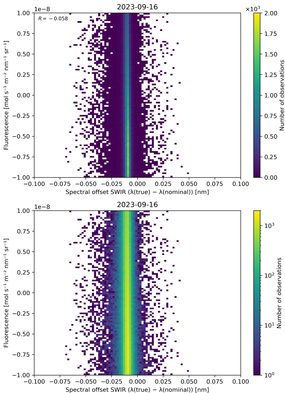
Figure 120: Scatter density plot of “Spectral offset SWIR ( \lambda(\text{true}) - \lambda(\text{nominal}) )” against “Fluorescence” for 2023-09-15 to 2023-09-17.
