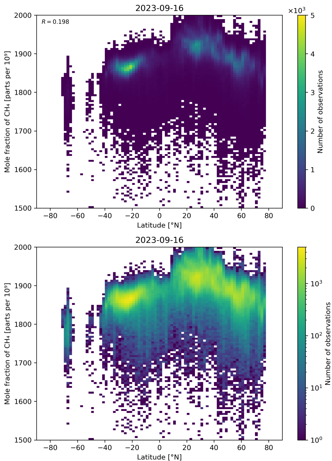
Figure 57: Scatter density plot of “Latitude” against “Mole fraction of \text{CH}_4 ” for 2023-09-15 to 2023-09-17.
