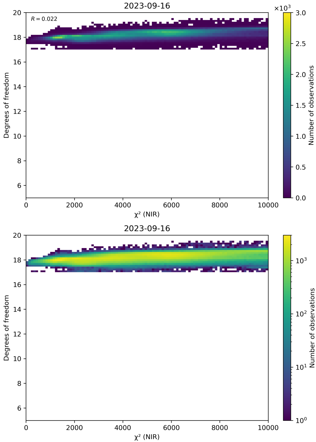
Figure 44: Scatter density plot of “ \chi^2 (NIR)” against “Degrees of freedom” for 2023-09-15 to 2023-09-17.
