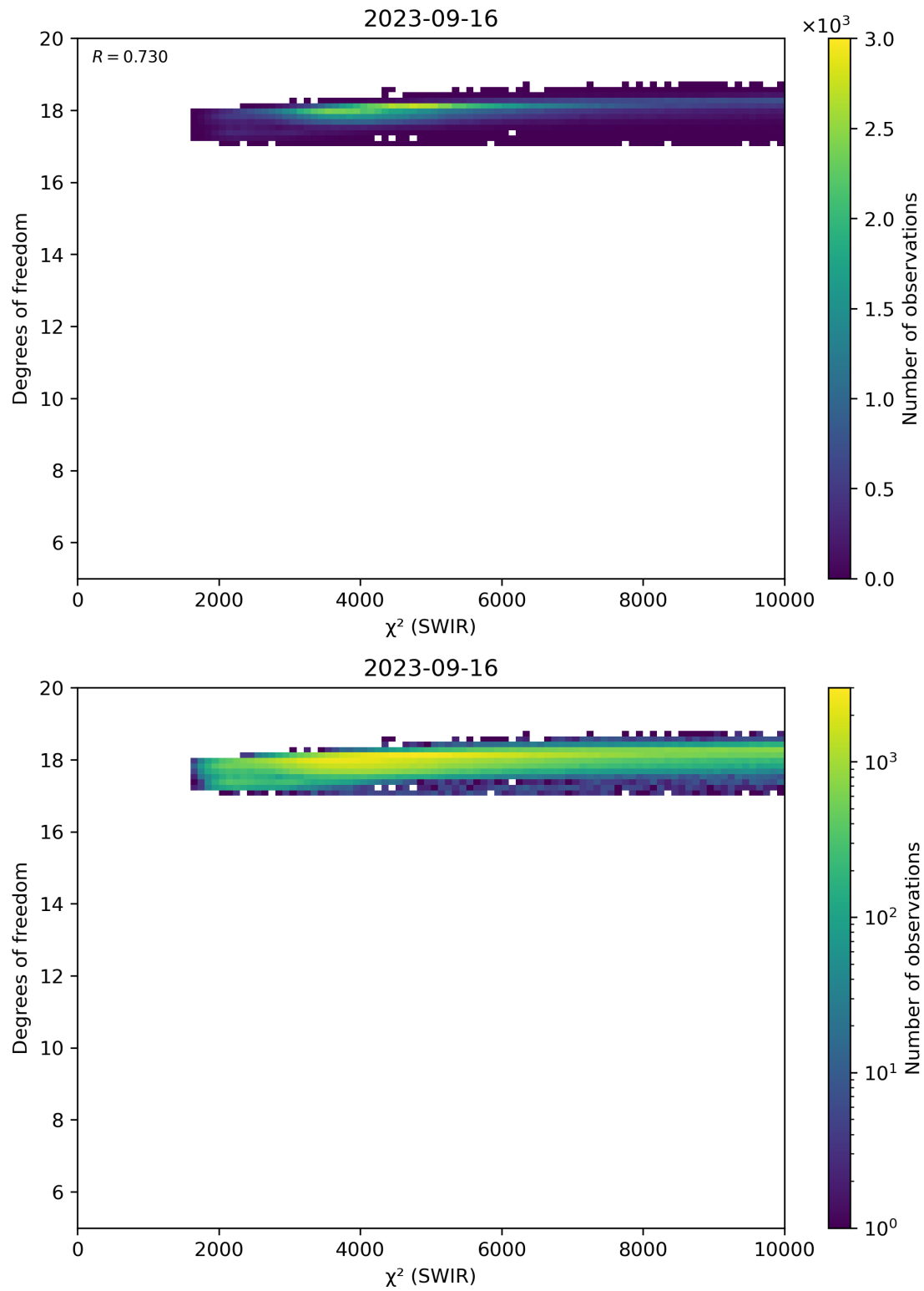
Figure 48: Scatter density plot of “ \chi^2 (SWIR)” against “Degrees of freedom” for 2023-09-15 to 2023-09-17.
