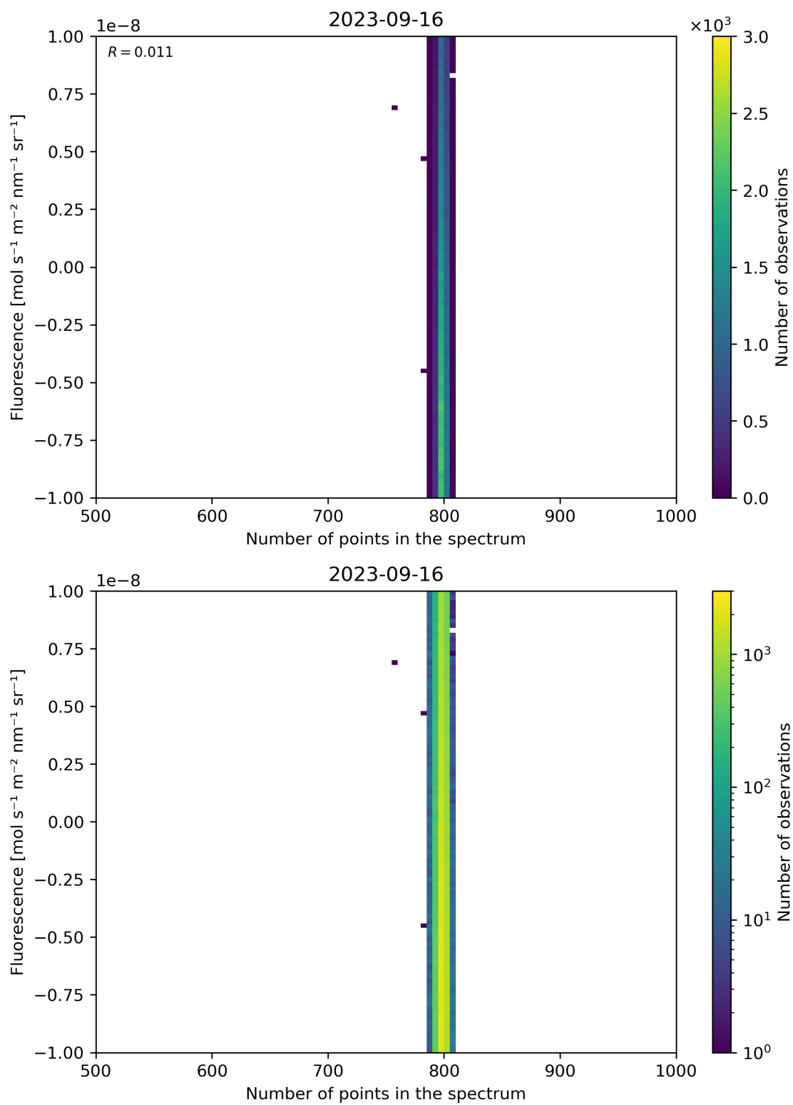
Figure 91: Scatter density plot of “Number of points in the spectrum” against “Fluorescence” for 2023-09-15 to 2023-09-17.
