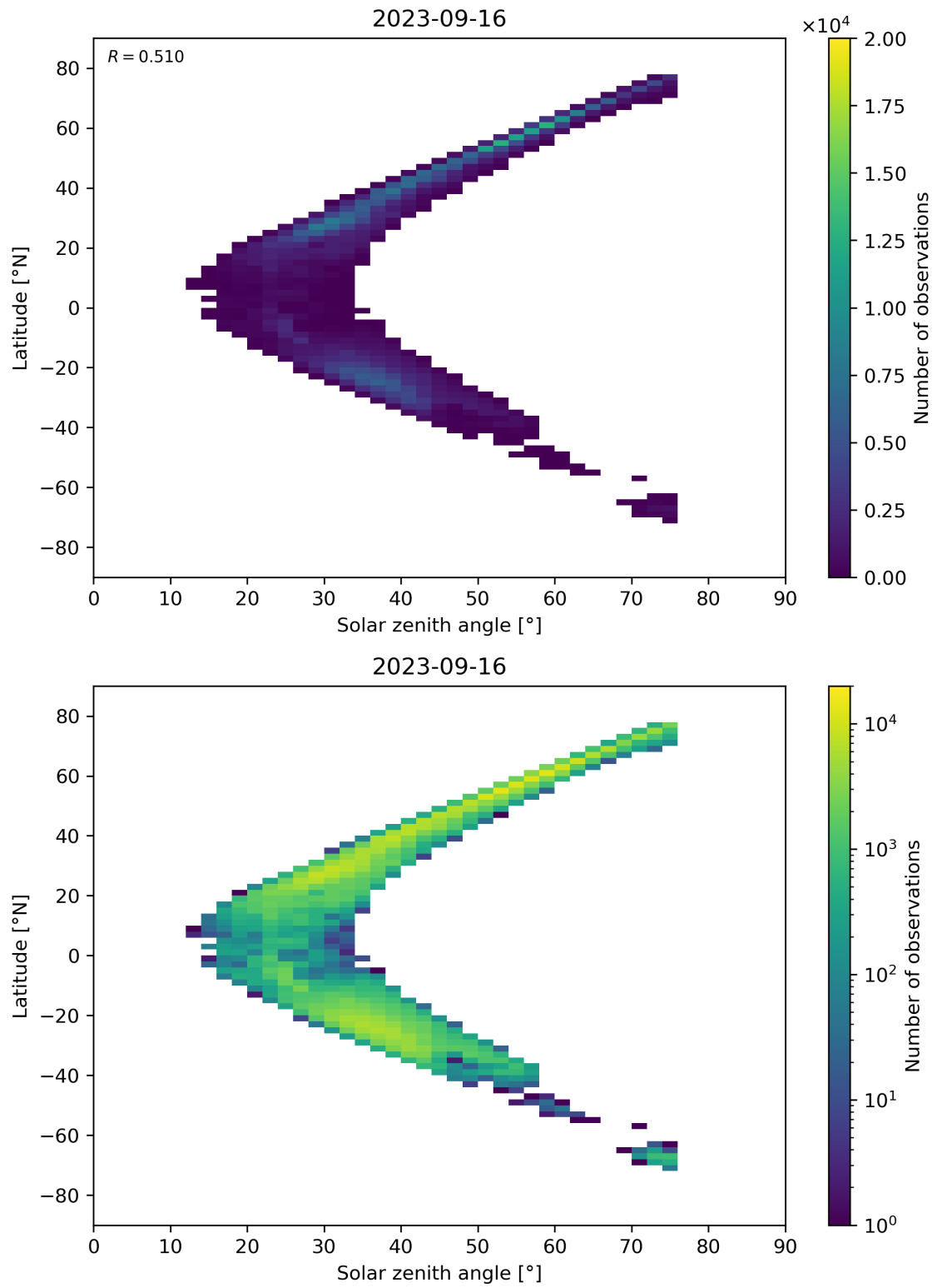
Figure 98: Scatter density plot of “Solar zenith angle” against “Latitude” for 2023-09-15 to 2023-09-17.
