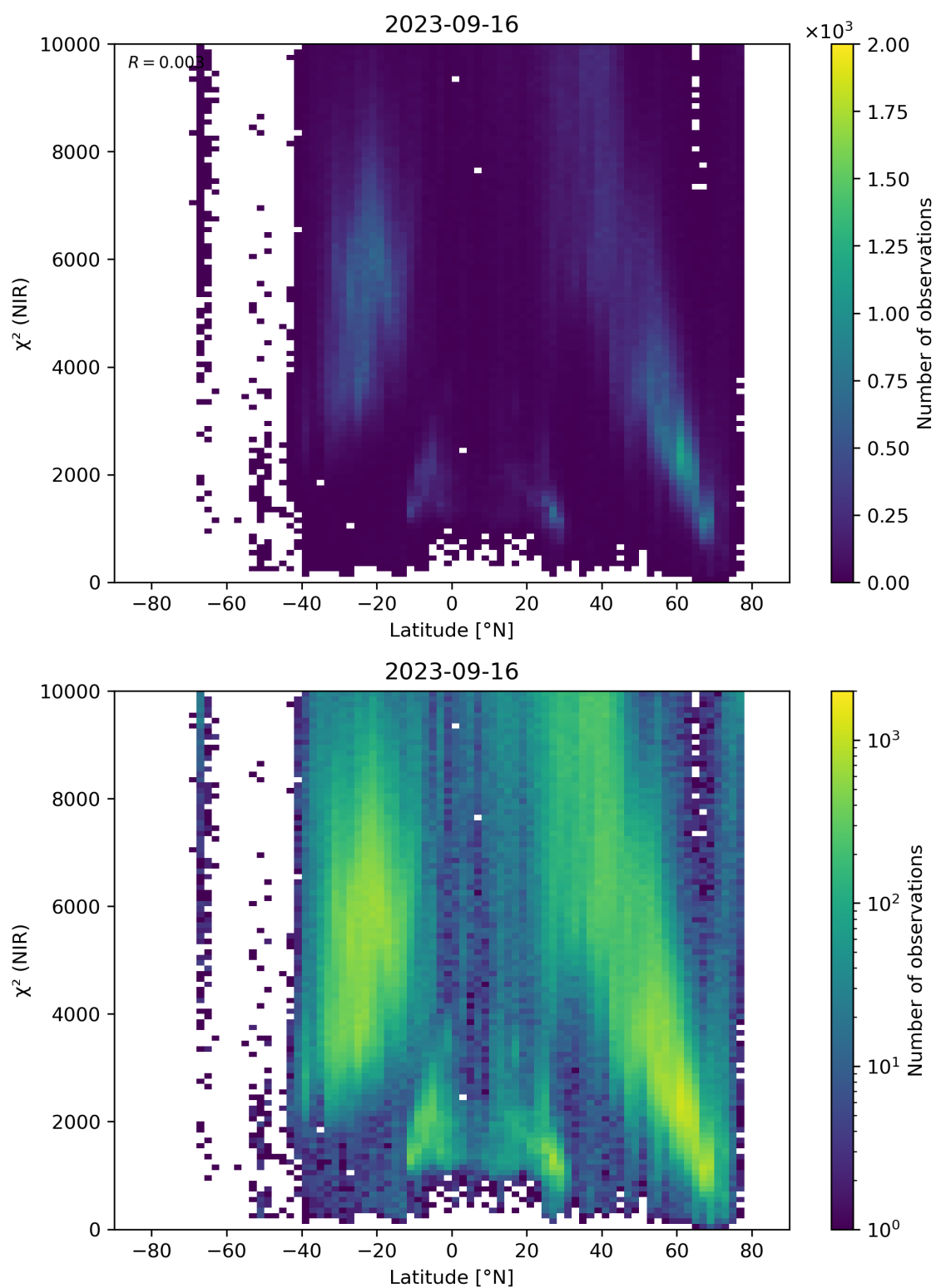
Figure 53: Scatter density plot of “Latitude” against “ \chi^2 (NIR)” for 2023-09-15 to 2023-09-17.
