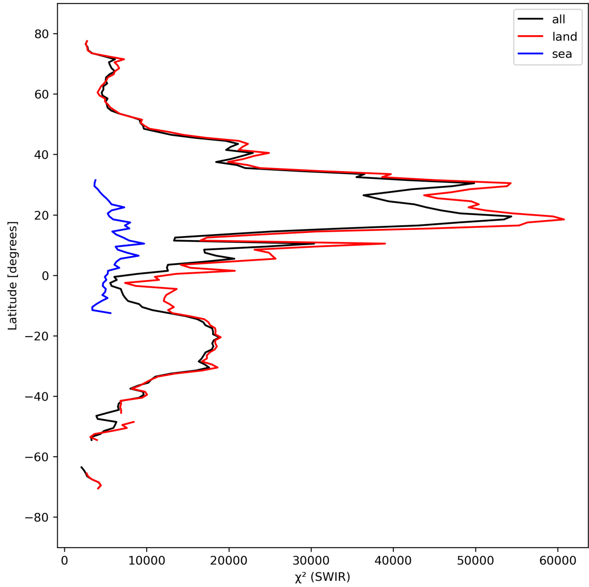
Figure 17: Zonal average of “ \chi^2 (SWIR)” for 2023-09-15 to 2023-09-17.
