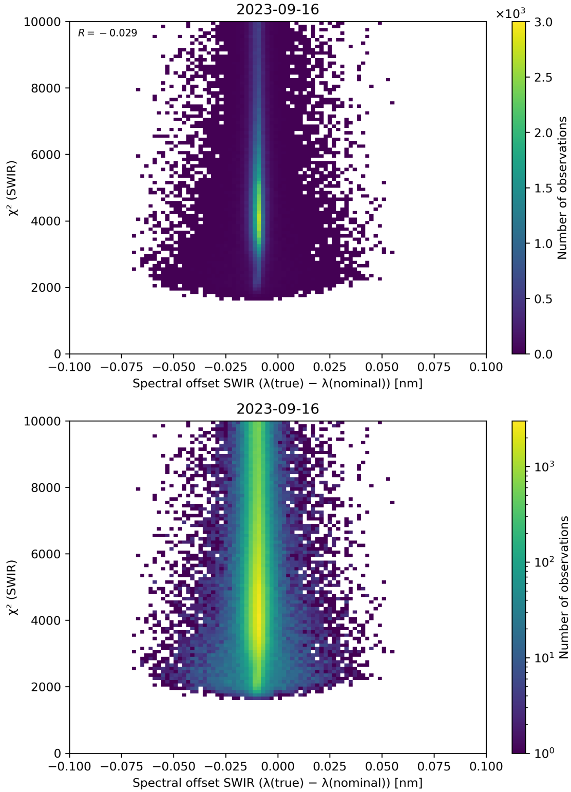
Figure 118: Scatter density plot of “Spectral offset SWIR ( \lambda(\text{true}) - \lambda(\text{nominal}) )” against “ \chi^2 (SWIR)” for 2023-09-15 to 2023-09-17.
