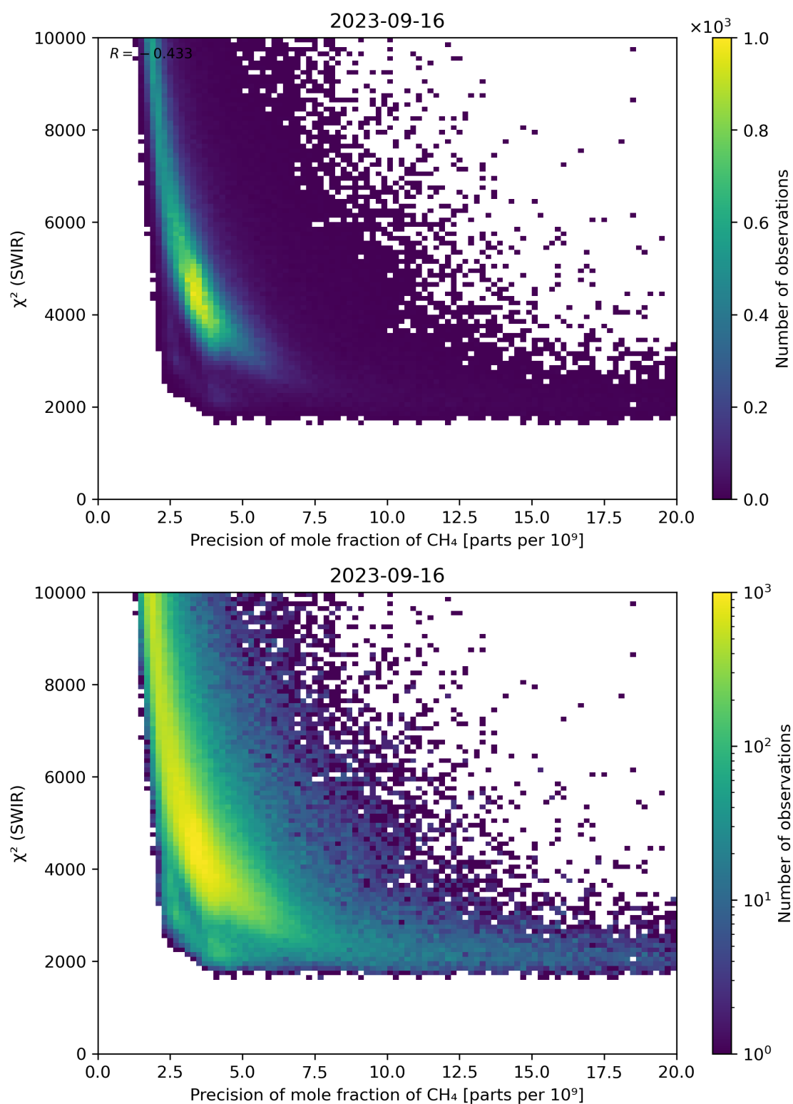
Figure 79: Scatter density plot of “Precision of mole fraction of \text{CH}_4 ” against “ \chi^2 (SWIR)” for 2023-09-15 to 2023-09-17.
