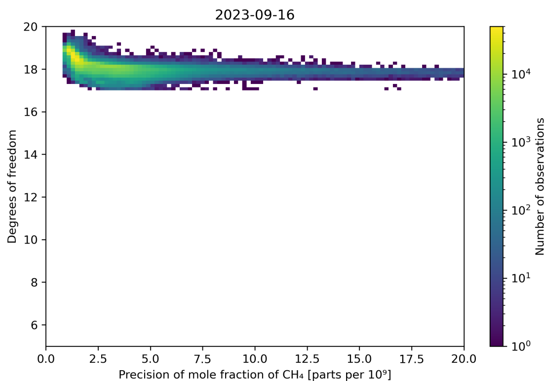
Figure 80: Scatter density plot of “Precision of mole fraction of CH 4 ” against “Degrees of freedom” for 2023-09-15 to 2023-09-17.
