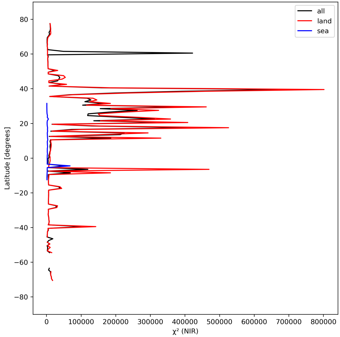
Figure 18: Zonal average of “ \chi^2 (NIR)” for 2023-09-15 to 2023-09-17.
