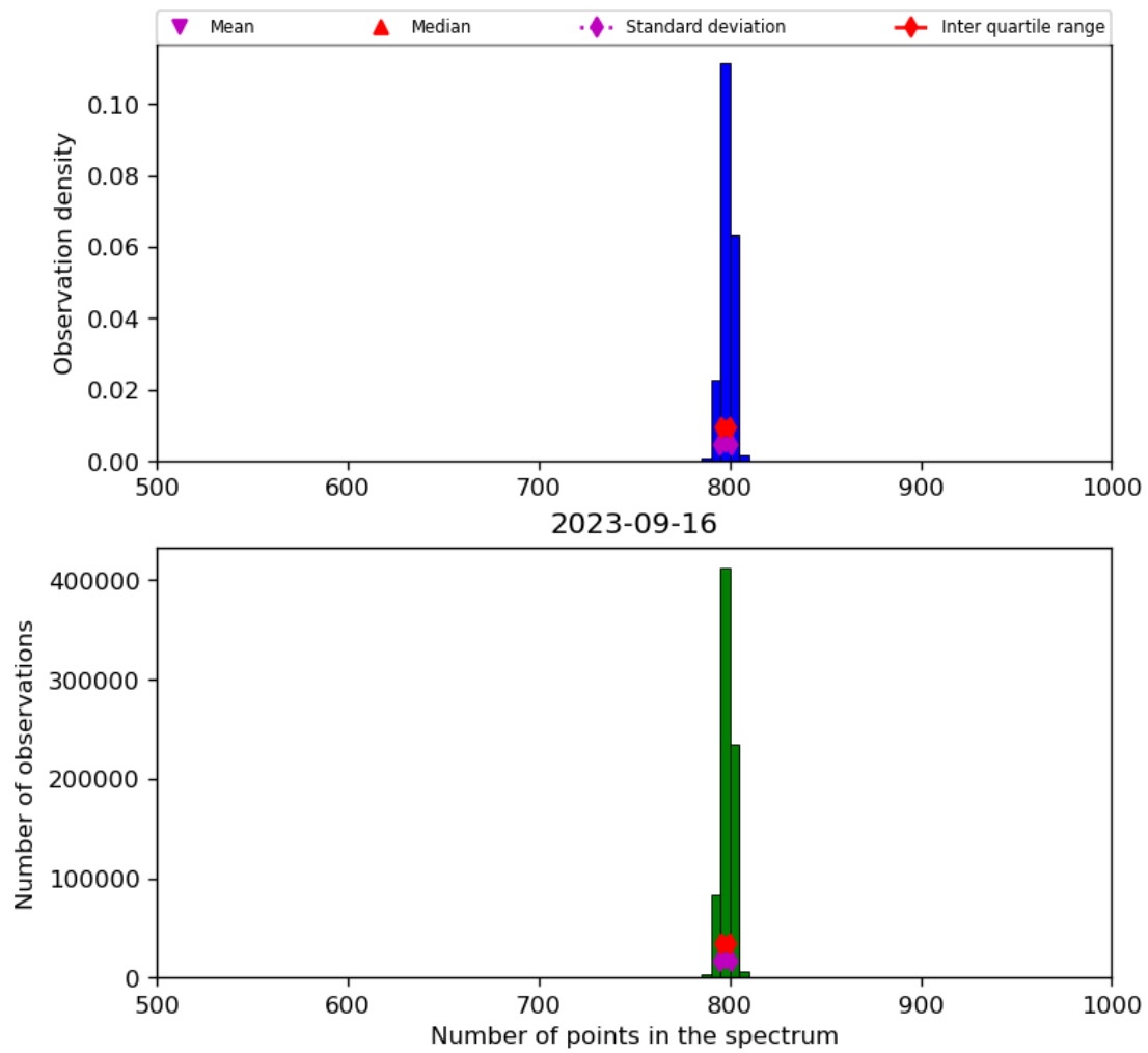
Figure 26: Histogram of “Number of points in the spectrum” for 2023-09-15 to 2023-09-17
