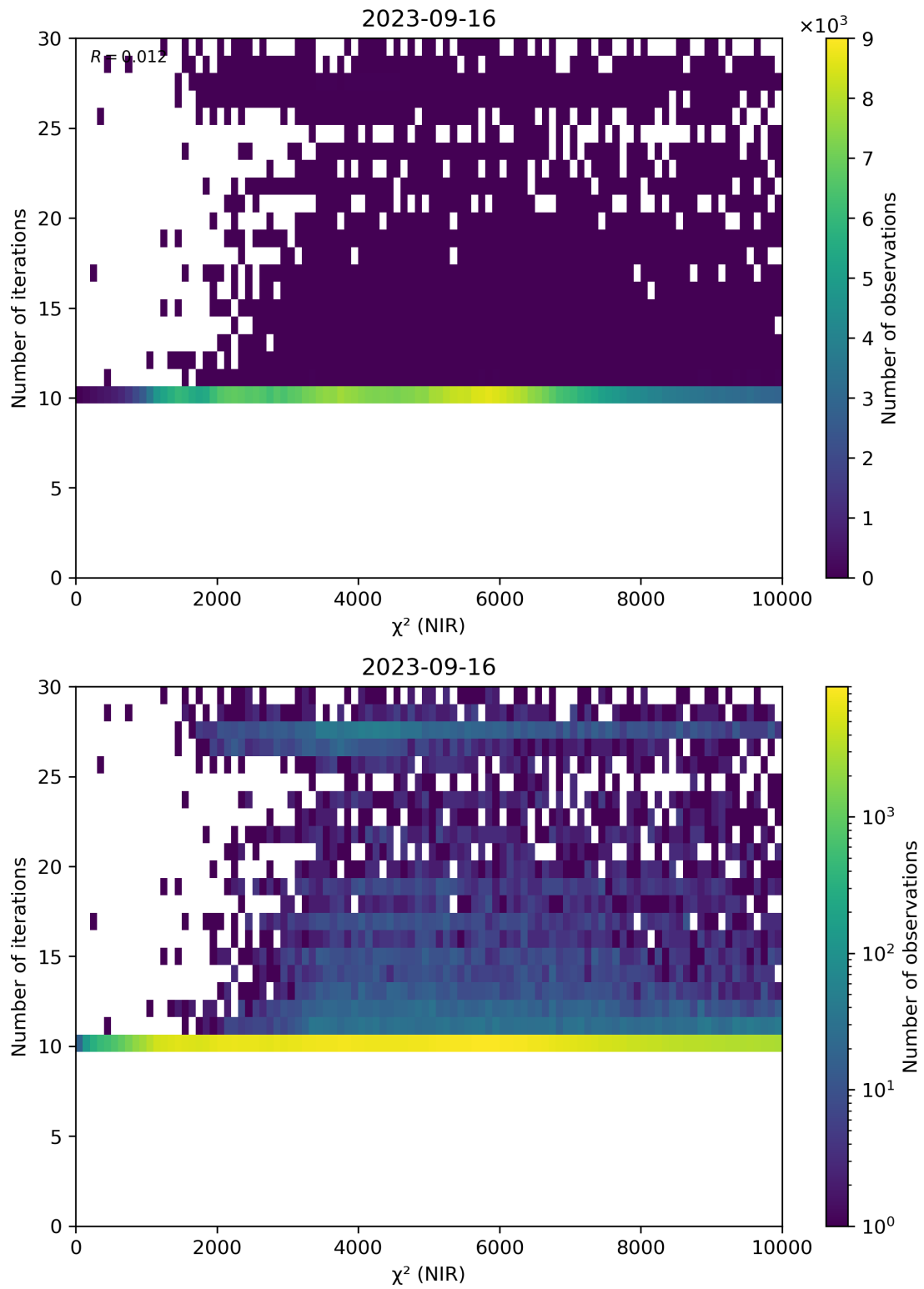
Figure 46: Scatter density plot of “ \chi^2 (NIR)” against “Number of iterations” for 2023-09-15 to 2023-09-17.
