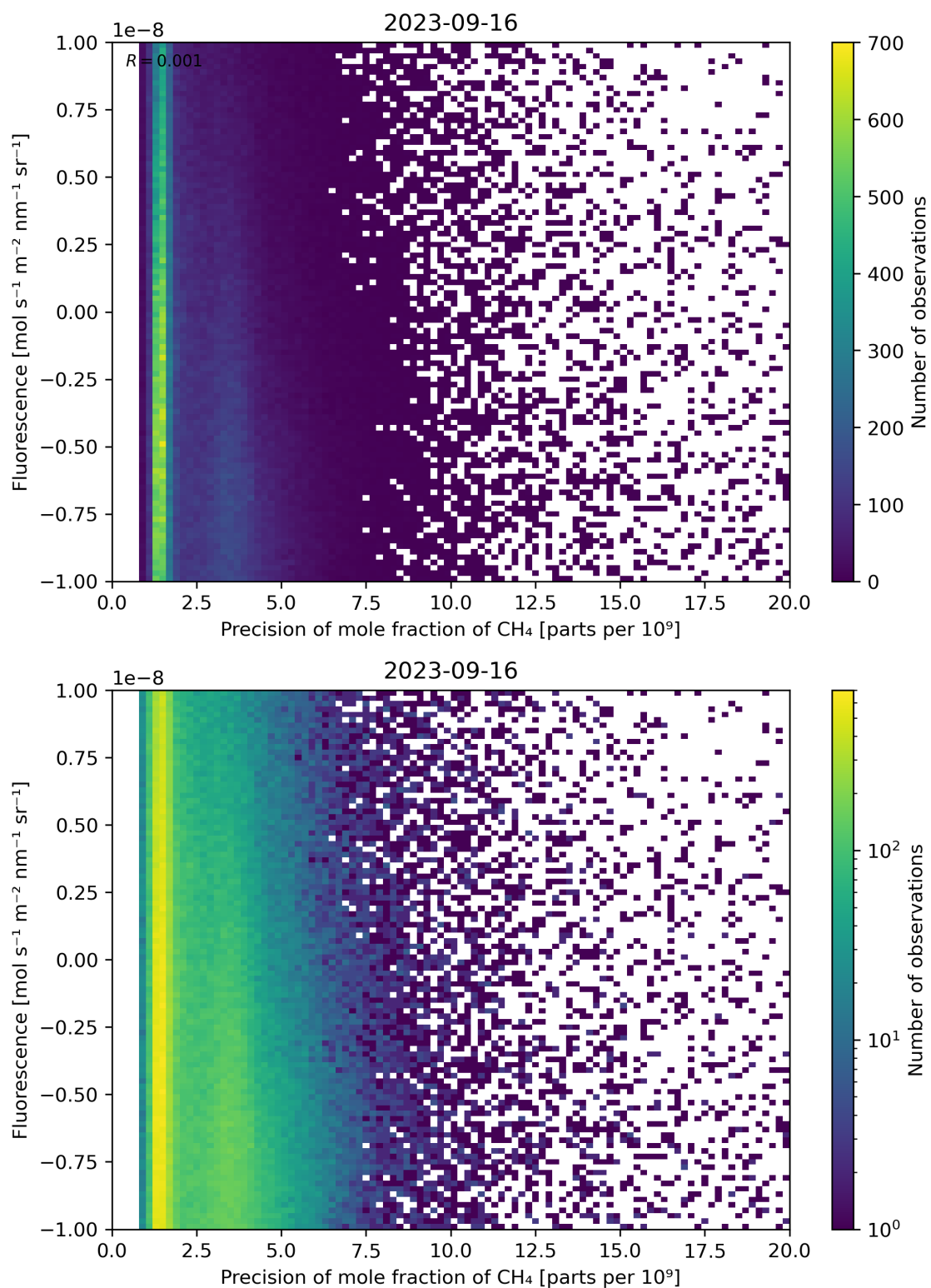
Figure 81: Scatter density plot of “Precision of mole fraction of \text{CH}_4 ” against “Fluorescence” for 2023-09-15 to 2023-09-17.
