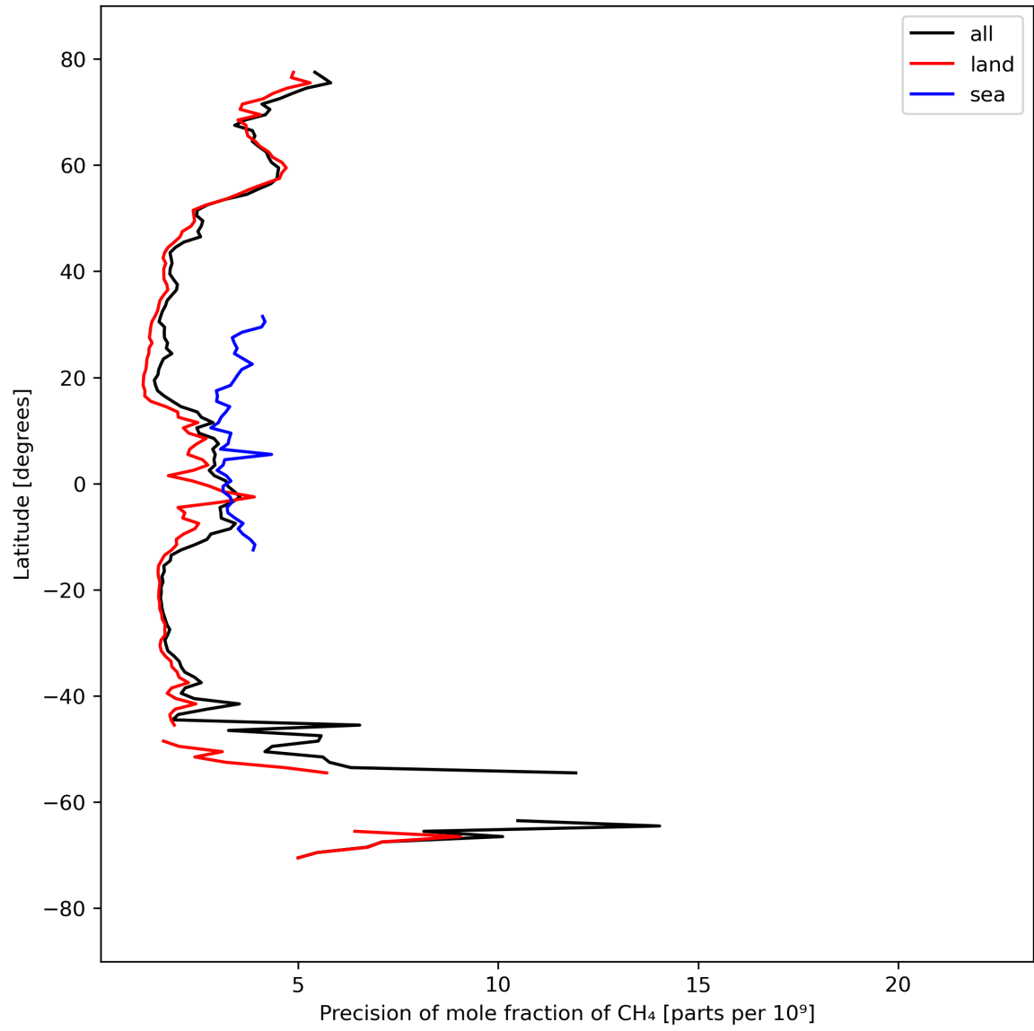
Figure 13: Zonal average of “Precision of mole fraction of CH 4 ” for 2023-09-15 to 2023-09-17.
