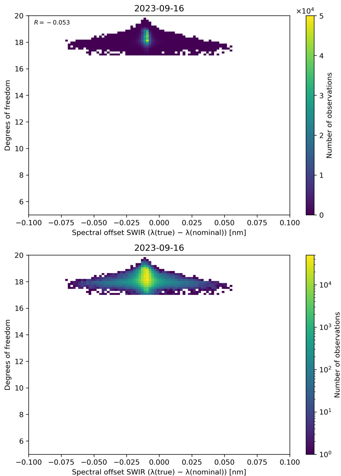
Figure 119: Scatter density plot of “Spectral offset SWIR ( \lambda(\text{true}) - \lambda(\text{nominal}) )” against “Degrees of freedom” for 2023-09-15 to 2023-09-17.
