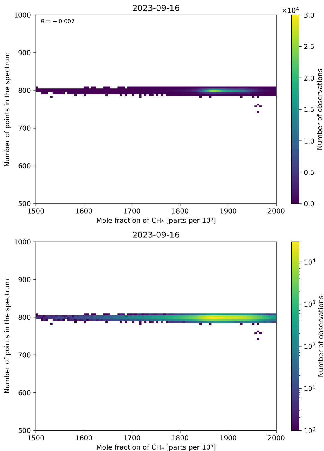
Figure 77: Scatter density plot of “Mole fraction of CH 4 ” against “Number of points in the spectrum” for 2023-09-15 to 2023-09-17.
