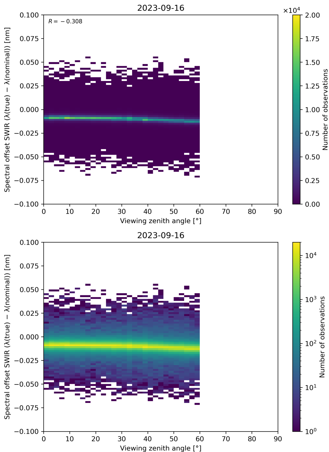
Figure 116: Scatter density plot of “Viewing zenith angle” against “Spectral offset SWIR ( \lambda(\text{true}) - \lambda(\text{nominal}) )” for 2023-09-15 to 2023-09-17.
