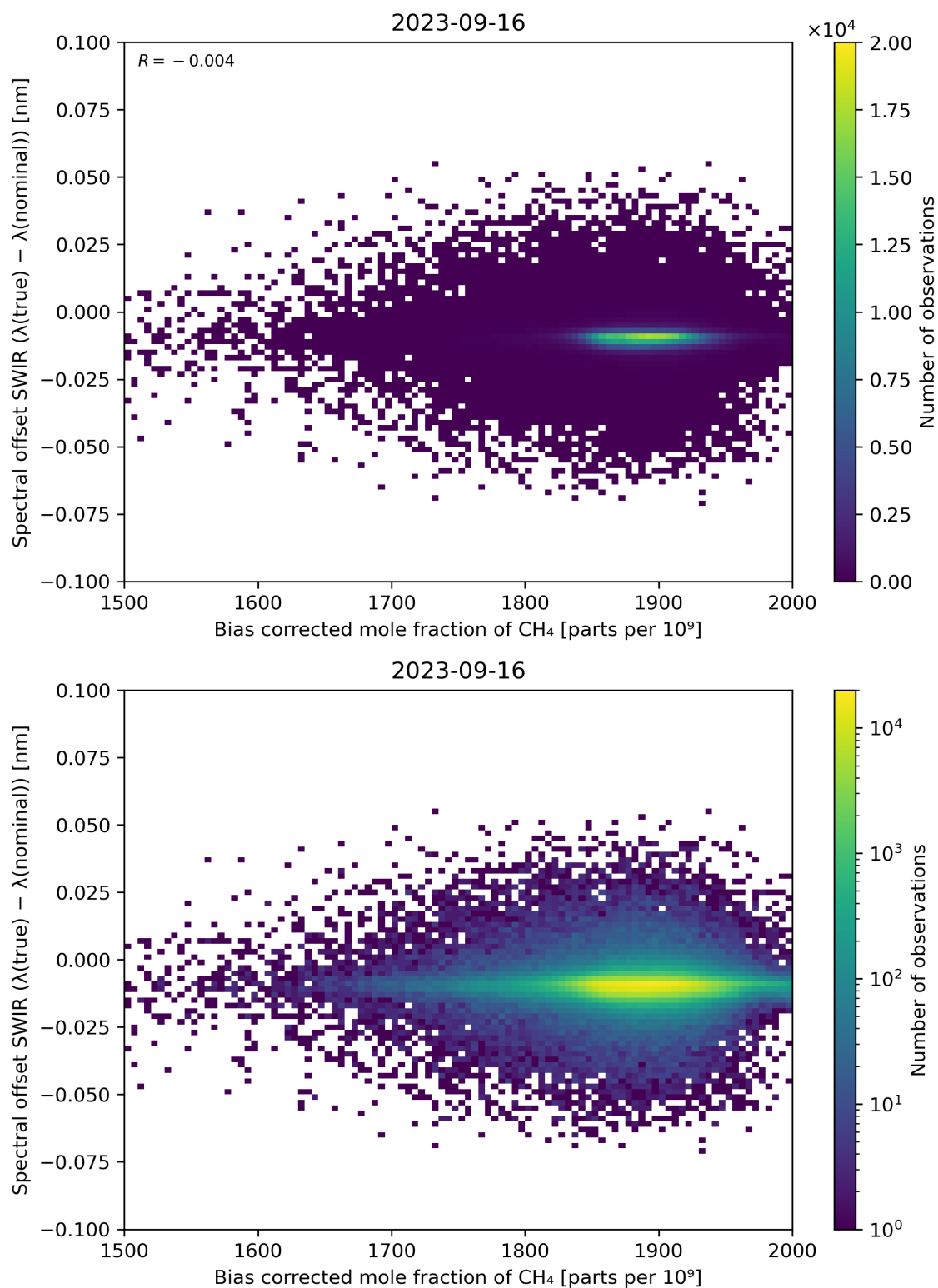
Figure 69: Scatter density plot of “Bias corrected mole fraction of \text{CH}_4 ” against “Spectral offset SWIR ( \lambda(\text{true}) - \lambda(\text{nominal}) )” for 2023-09-15 to 2023-09-17.
