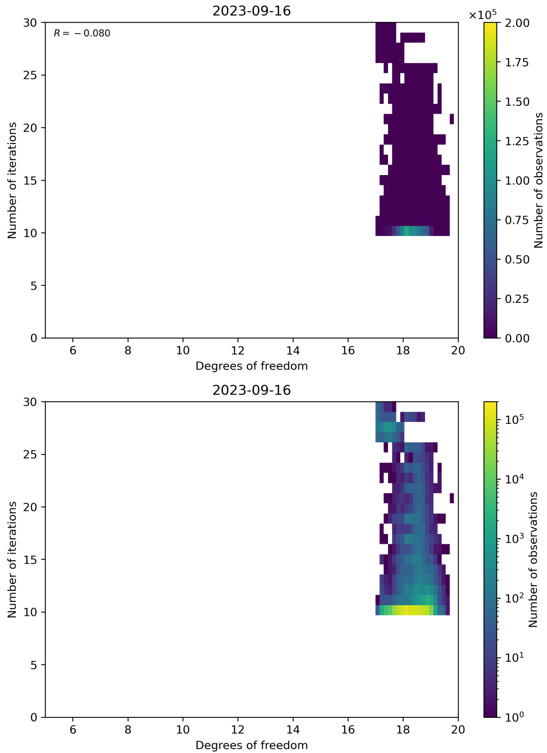
Figure 52: Scatter density plot of “Degrees of freedom” against “Number of iterations” for 2023-09-15 to 2023-09-17.
