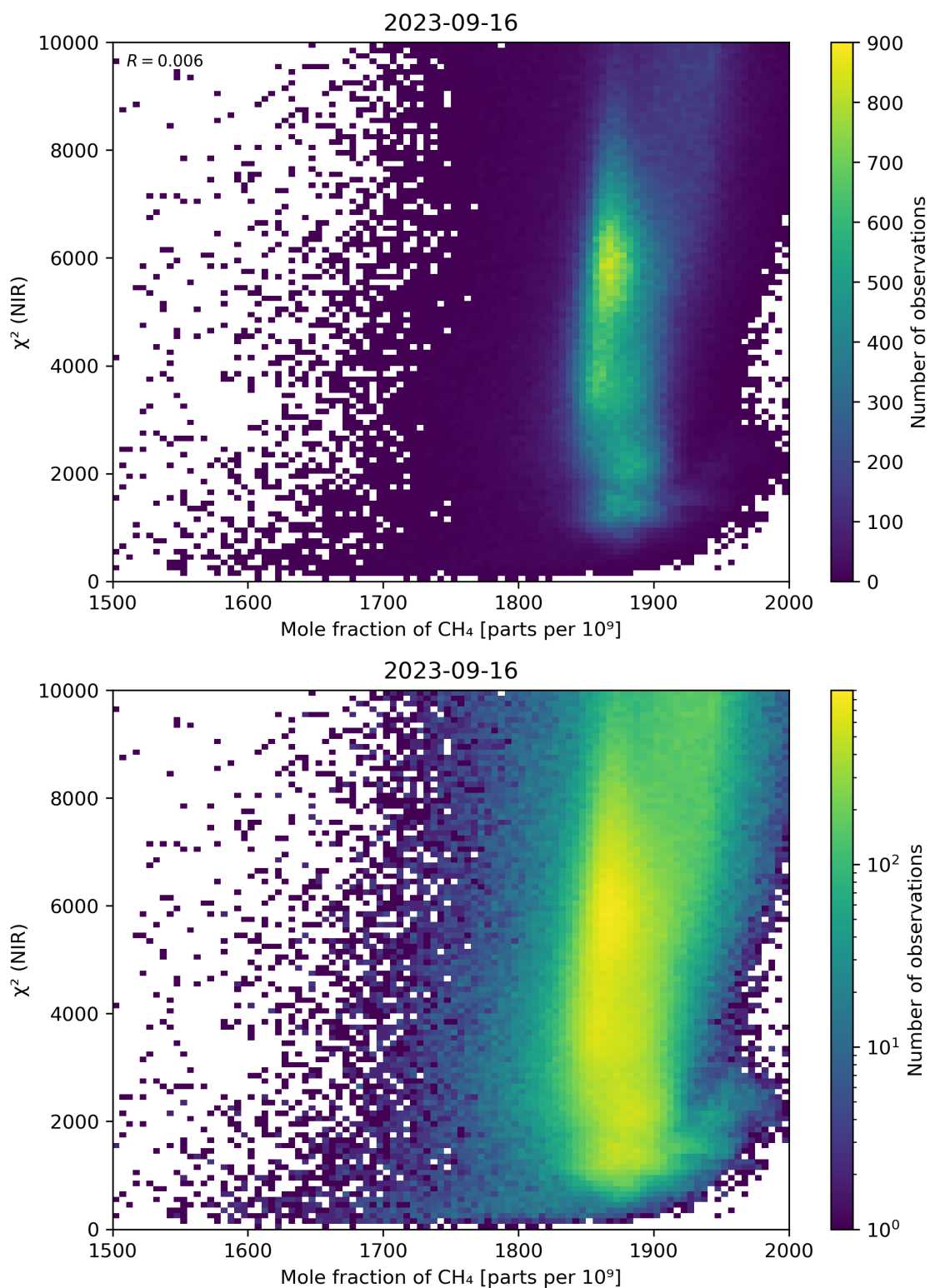
Figure 70: Scatter density plot of “Mole fraction of CH 4 ” against “ \chi^2 (NIR)” for 2023-09-15 to 2023-09-17.
