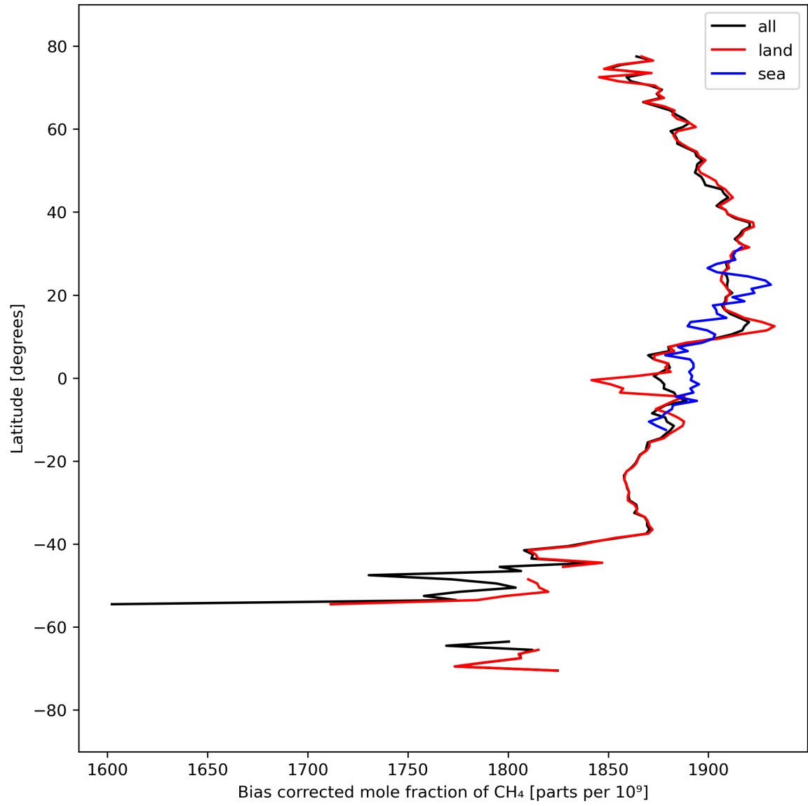
Figure 14: Zonal average of “Bias corrected mole fraction of CH 4 ” for 2023-09-15 to 2023-09-17.
