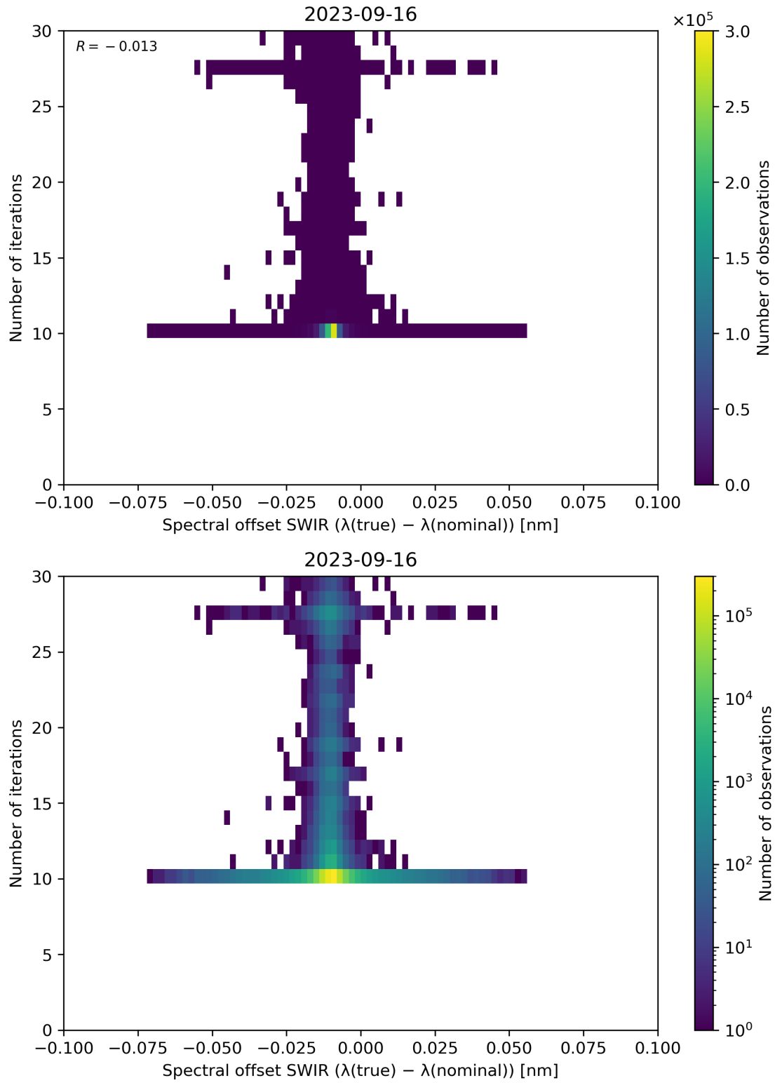
Figure 121: Scatter density plot of “Spectral offset SWIR ( \lambda(\text{true}) - \lambda(\text{nominal}) )” against “Number of iterations” for 2023-09-15 to 2023-09-17.
