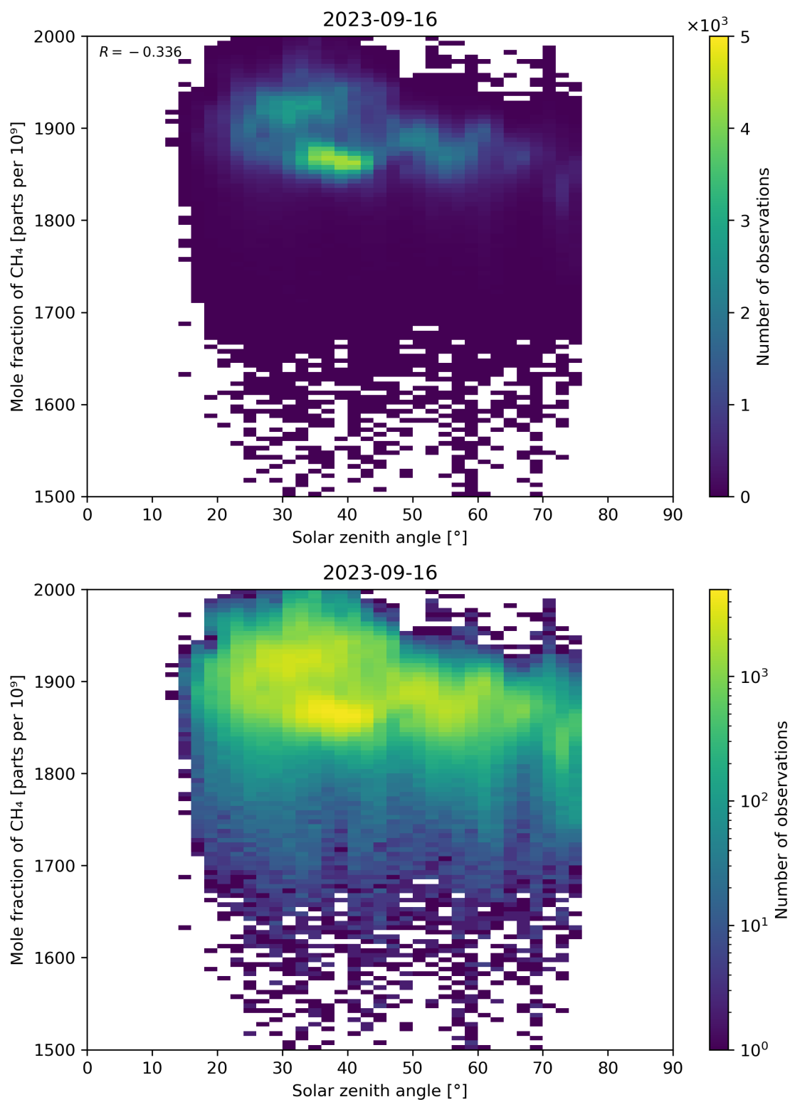
Figure 99: Scatter density plot of “Solar zenith angle” against “Mole fraction of CH 4 ” for 2023-09-15 to 2023-09-17.
