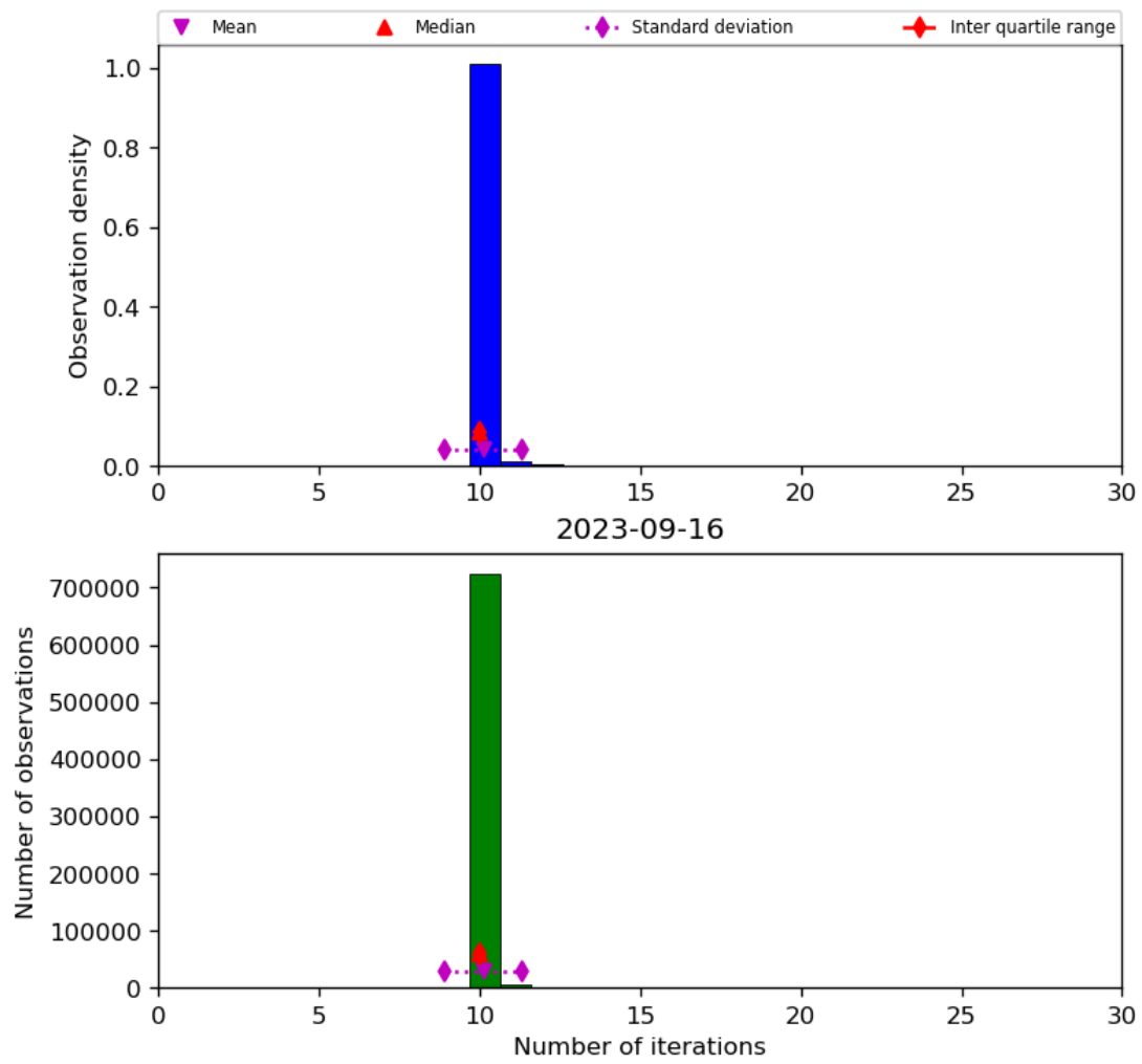
Figure 31: Histogram of “Number of iterations” for 2023-09-15 to 2023-09-17
