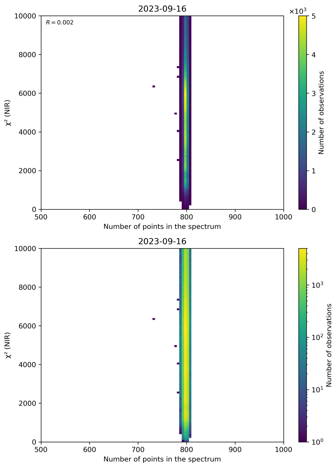
Figure 88: Scatter density plot of “Number of points in the spectrum” against “ \chi^2 (NIR)” for 2023-09-15 to 2023-09-17.
