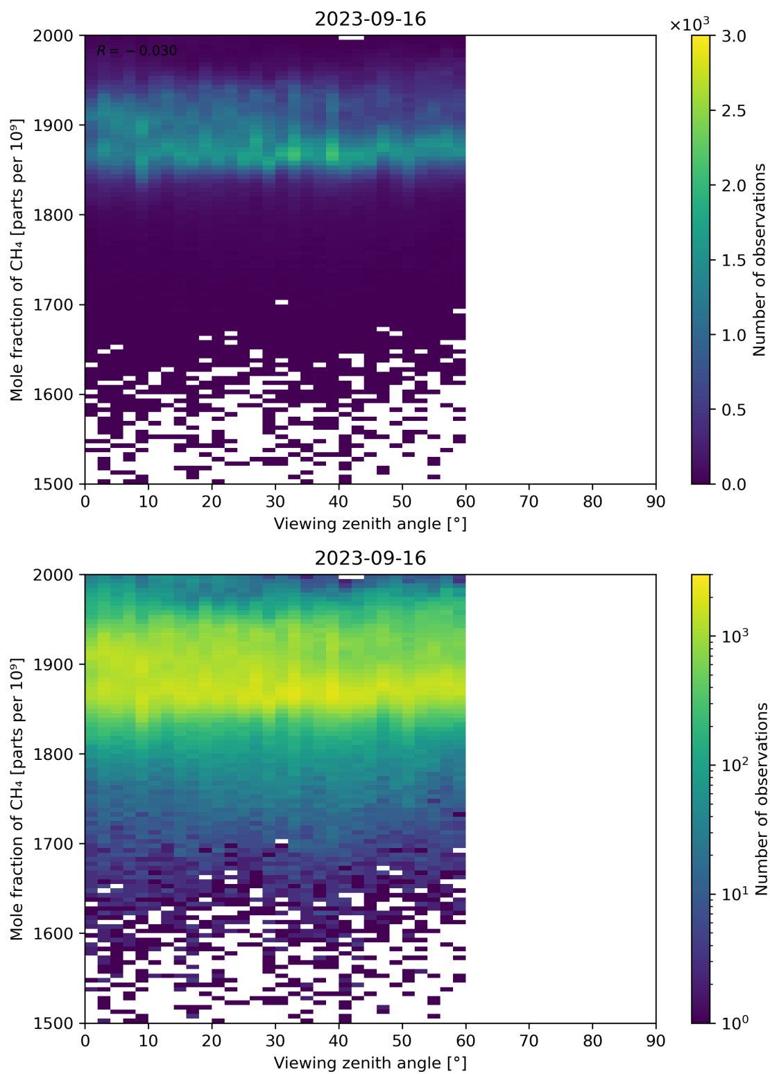
Figure 110: Scatter density plot of “Viewing zenith angle” against “Mole fraction of CH 4 ” for 2023-09-15 to 2023-09-17.
