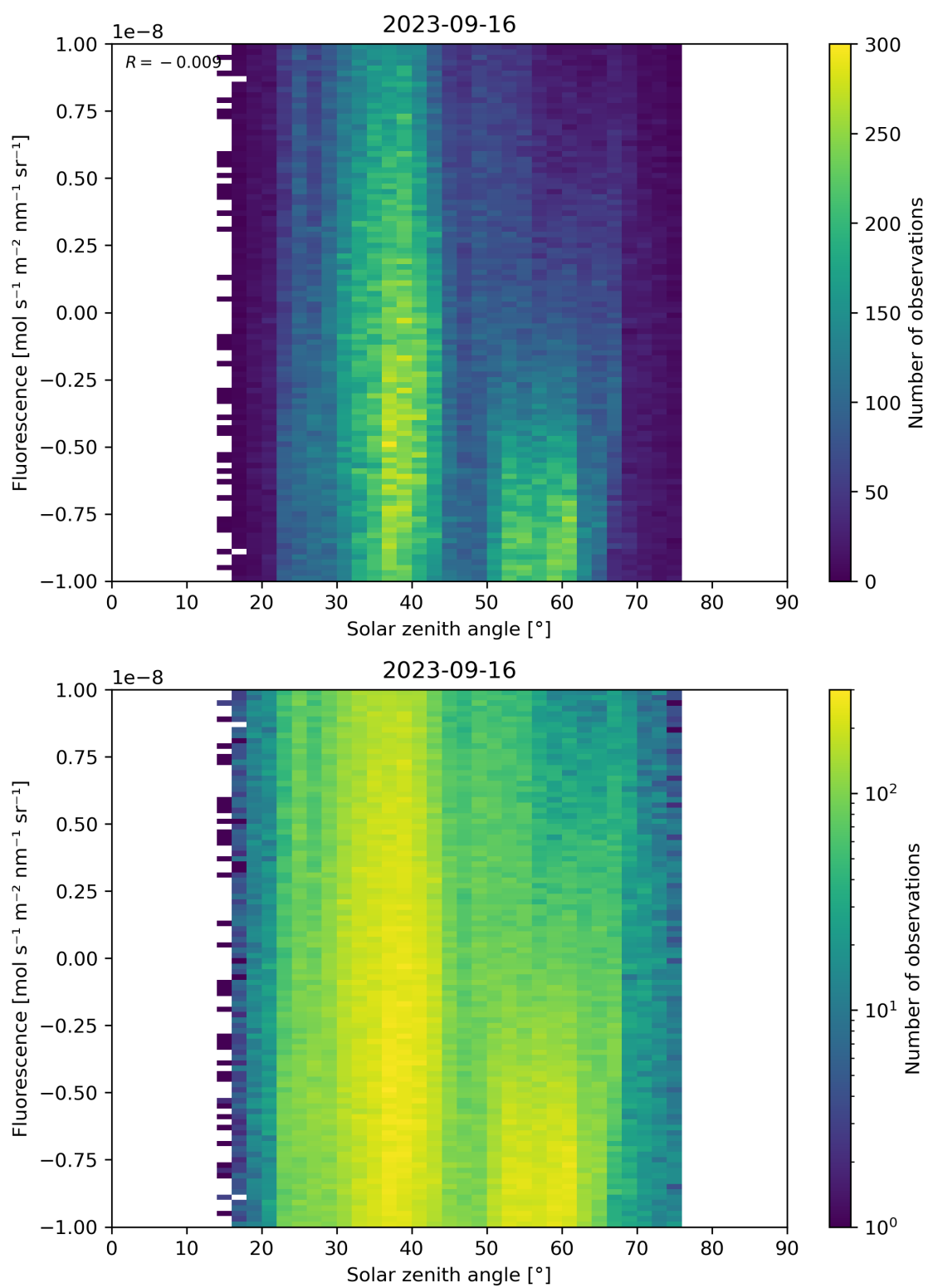
Figure 97: Scatter density plot of “Solar zenith angle” against “Fluorescence” for 2023-09-15 to 2023-09-17.
