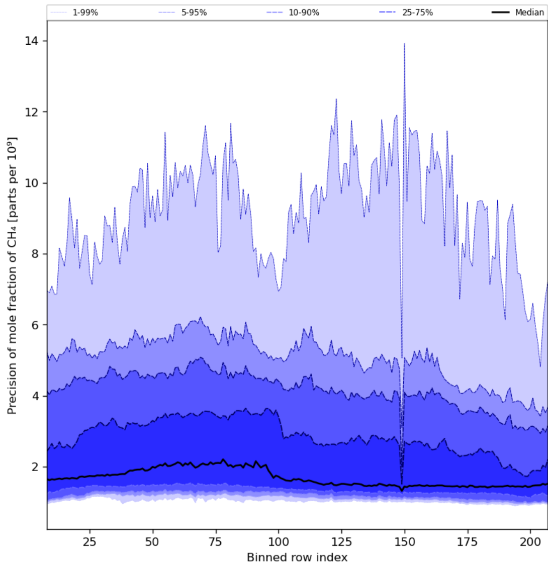
Figure 35: Along track statistics of “Precision of mole fraction of CH 4 ” for 2023-09-15 to 2023-09-17
