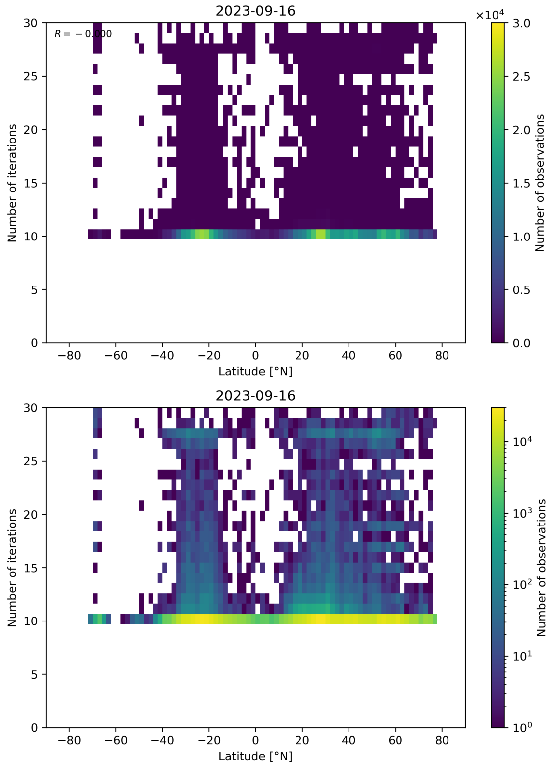
Figure 60: Scatter density plot of “Latitude” against “Number of iterations” for 2023-09-15 to 2023-09-17.
