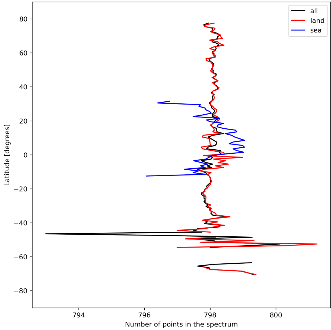
Figure 15: Zonal average of “Number of points in the spectrum” for 2023-09-15 to 2023-09-17.
