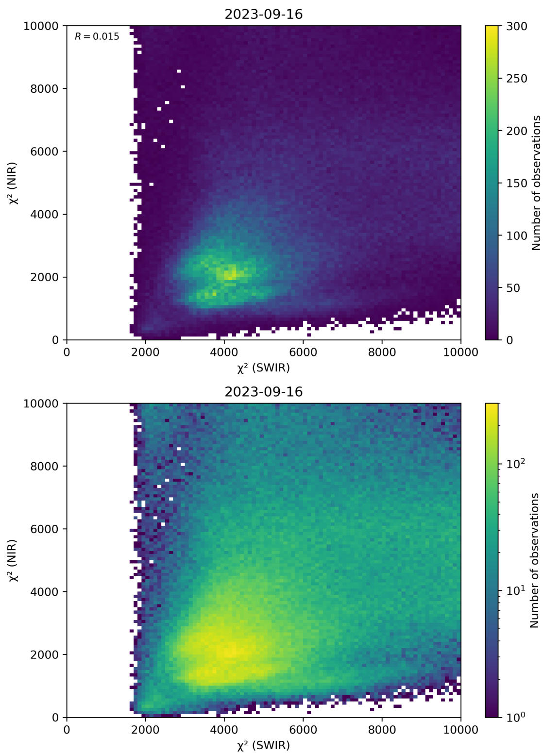
Figure 47: Scatter density plot of “ \chi^2 (SWIR)” against “ \chi^2 (NIR)” for 2023-09-15 to 2023-09-17.
