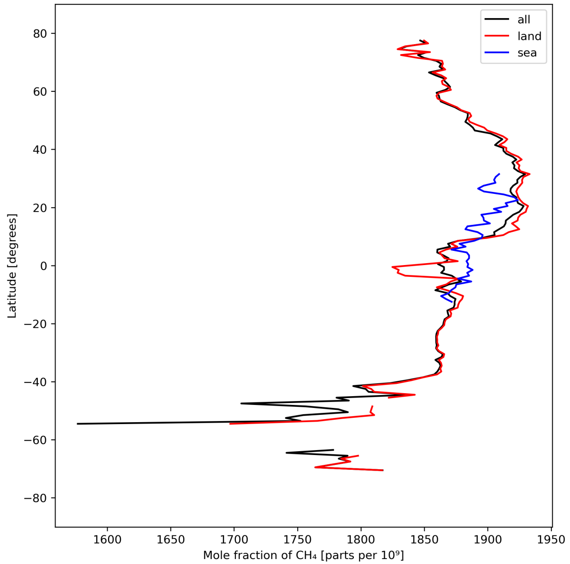
Figure 12: Zonal average of “Mole fraction of \text{CH}_4 ” for 2023-09-15 to 2023-09-17.
