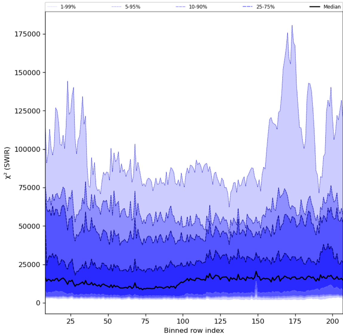
Figure 39: Along track statistics of “ \chi^2 (SWIR)” for 2023-09-15 to 2023-09-17
