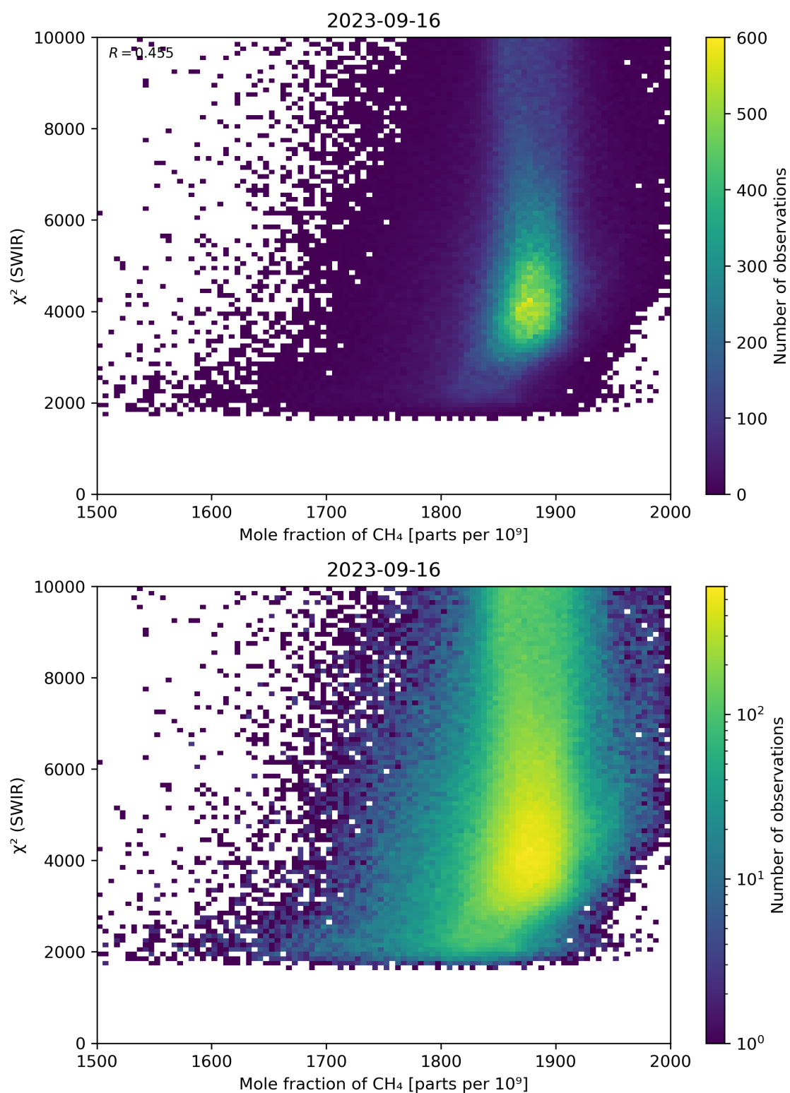
Figure 71: Scatter density plot of “Mole fraction of CH 4 ” against “ \chi^2 (SWIR)” for 2023-09-15 to 2023-09-17.
