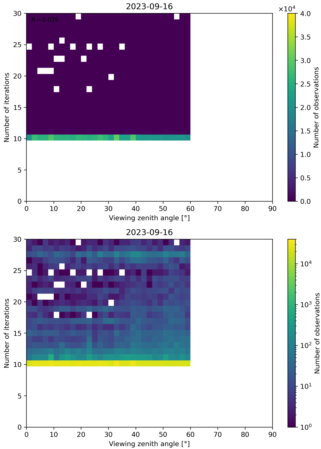
Figure 113: Scatter density plot of “Viewing zenith angle” against “Number of iterations” for 2023-09-15 to 2023-09-17.
