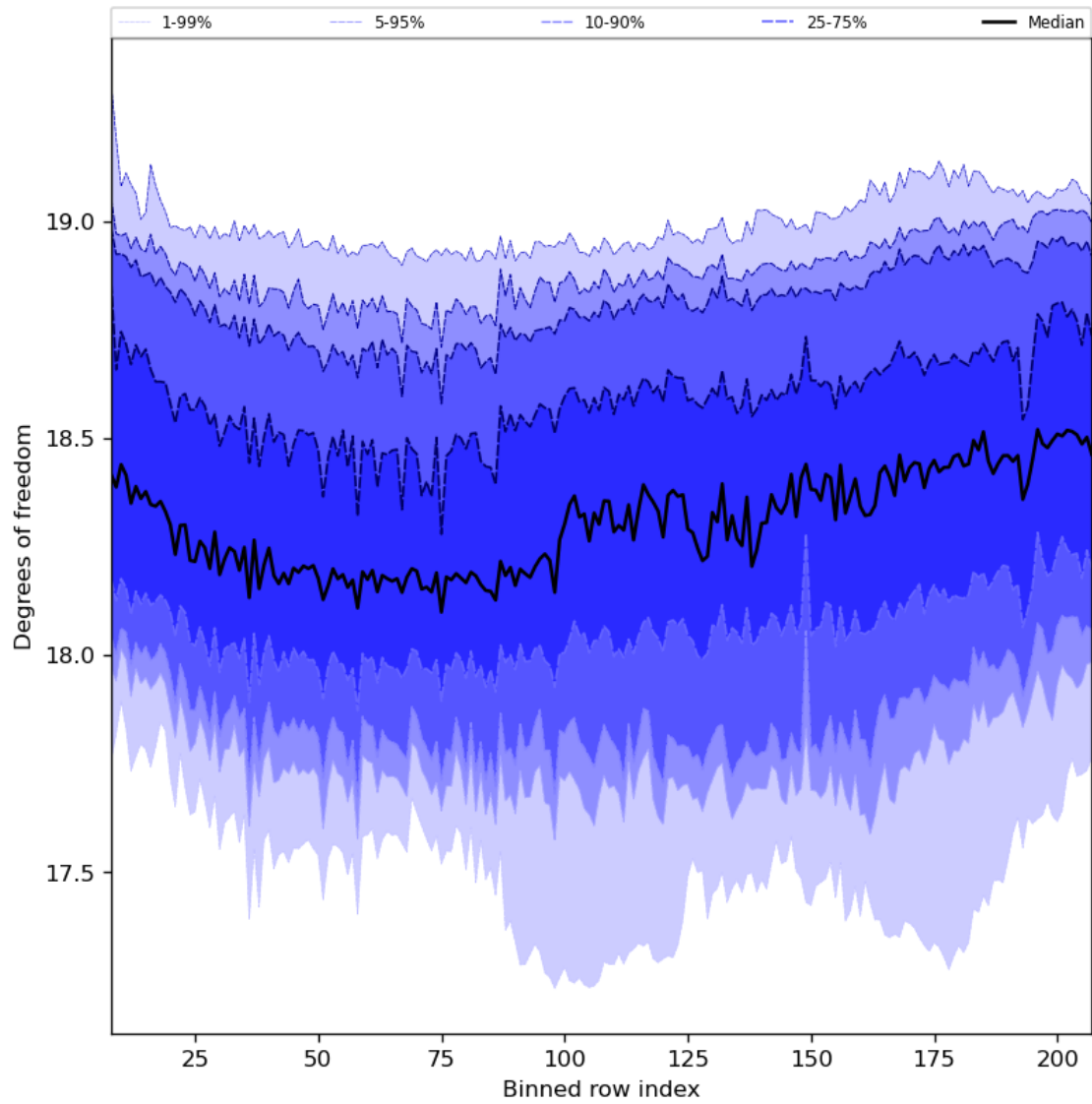
Figure 41: Along track statistics of “Degrees of freedom” for 2023-09-15 to 2023-09-17
