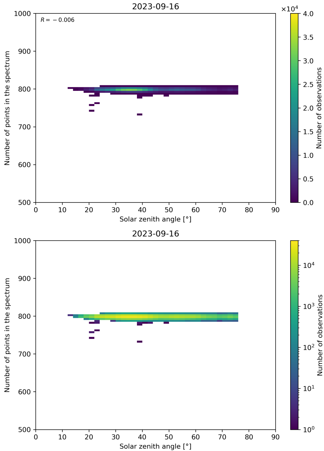
Figure 103: Scatter density plot of “Solar zenith angle” against “Number of points in the spectrum” for 2023-09-15 to 2023-09-17.
