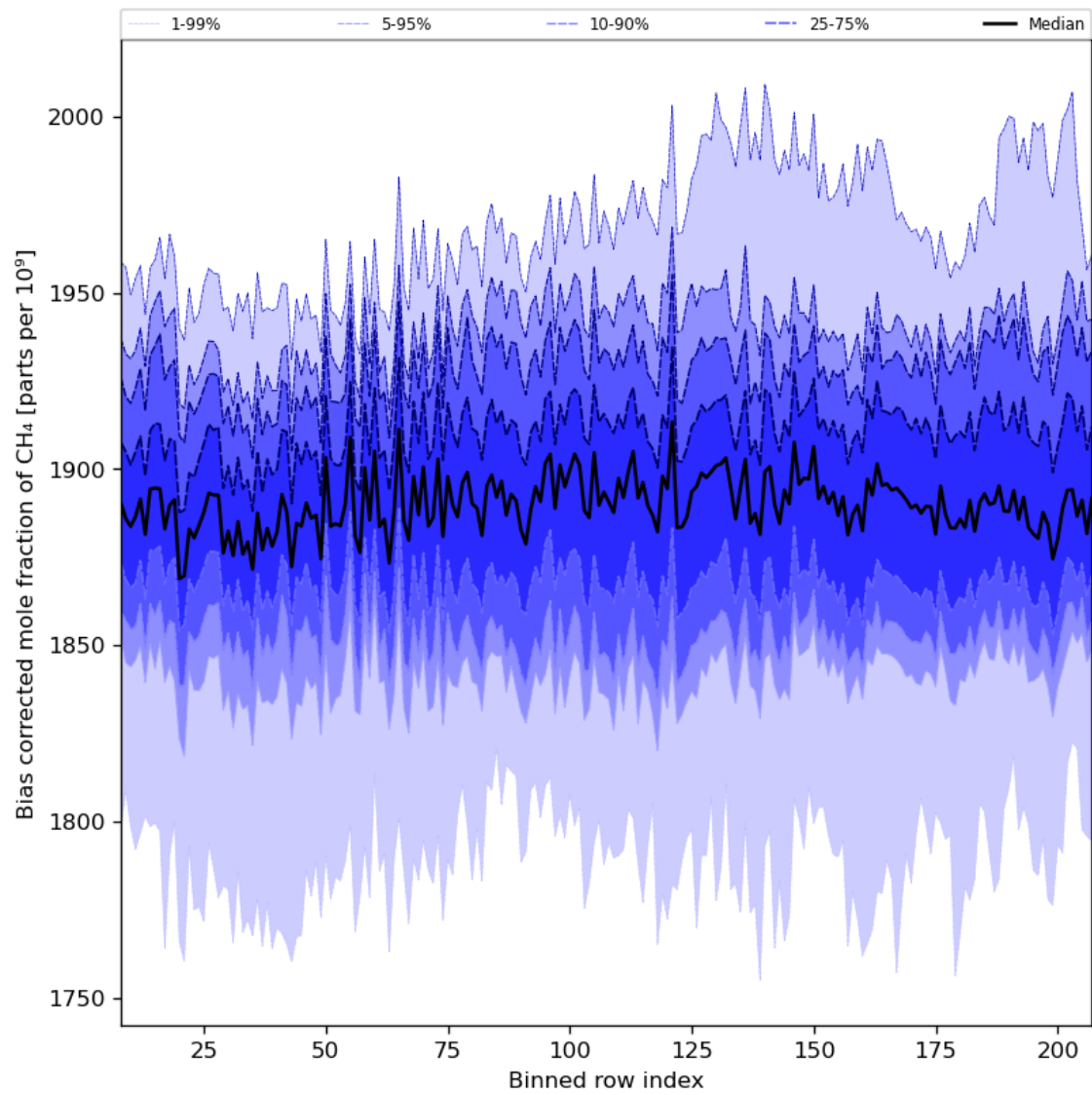
Figure 36: Along track statistics of “Bias corrected mole fraction of \text{CH}_4 ” for 2023-09-15 to 2023-09-17
