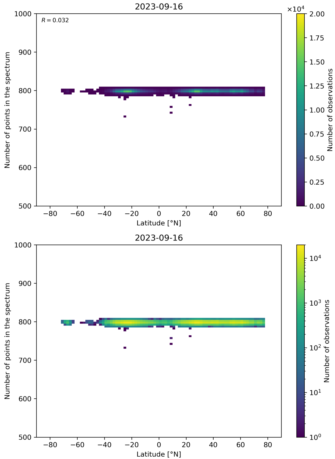
Figure 61: Scatter density plot of “Latitude” against “Number of points in the spectrum” for 2023-09-15 to 2023-09-17.
