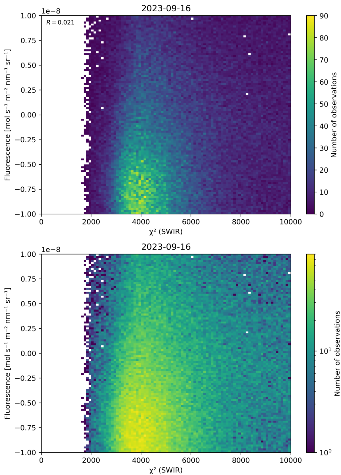
Figure 49: Scatter density plot of “ \chi^2 (SWIR)” against “Fluorescence” for 2023-09-15 to 2023-09-17.
