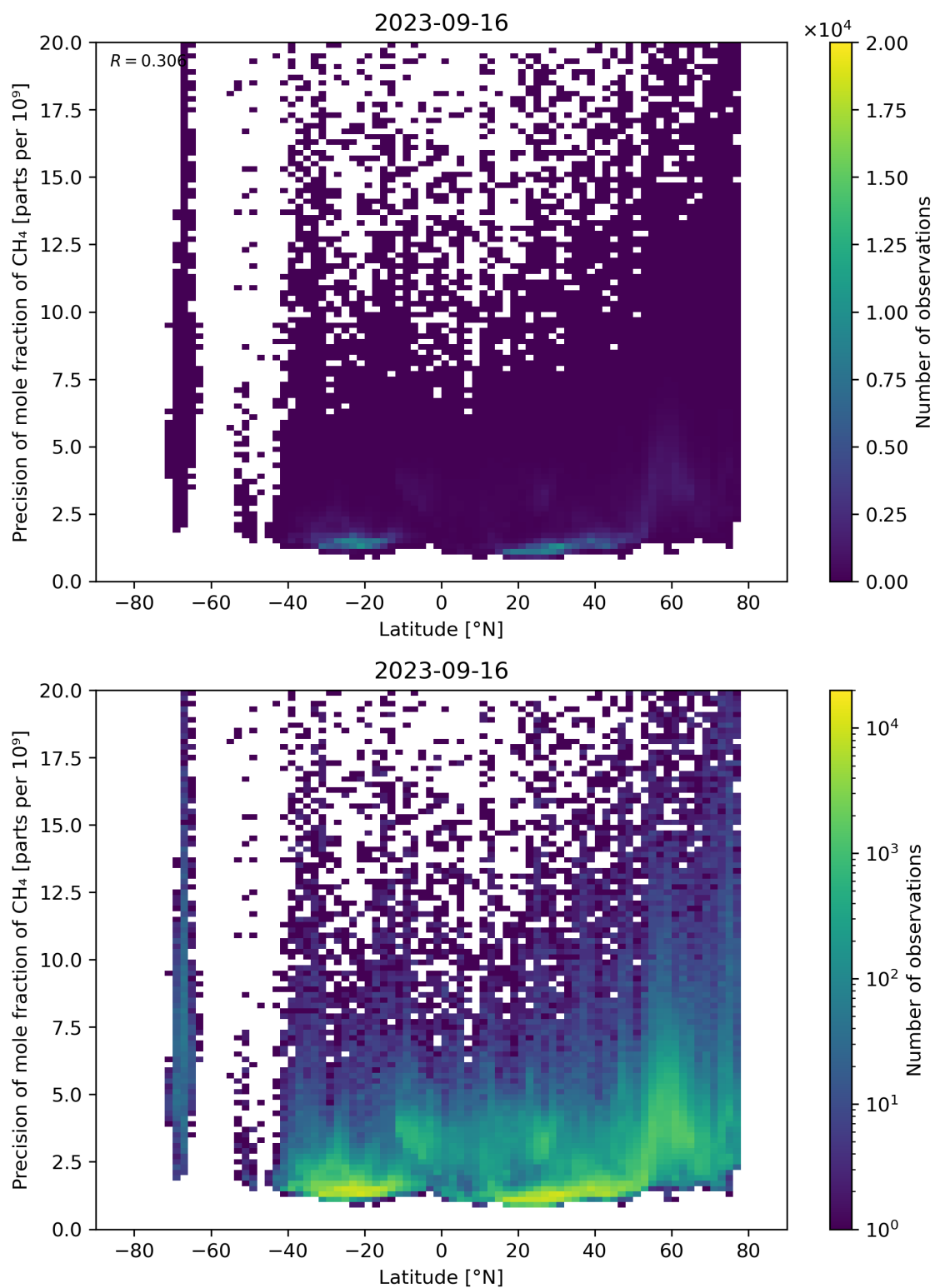
Figure 59: Scatter density plot of “Latitude” against “Precision of mole fraction of CH 4 ” for 2023-09-15 to 2023-09-17.
