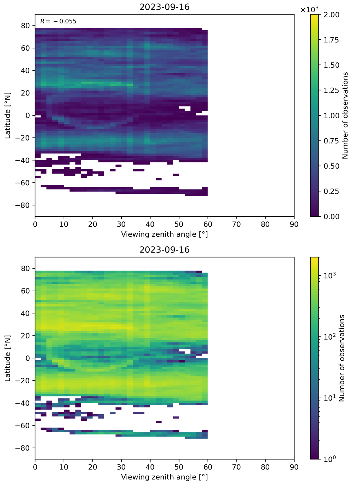
Figure 109: Scatter density plot of “Viewing zenith angle” against “Latitude” for 2023-09-15 to 2023-09-17.
