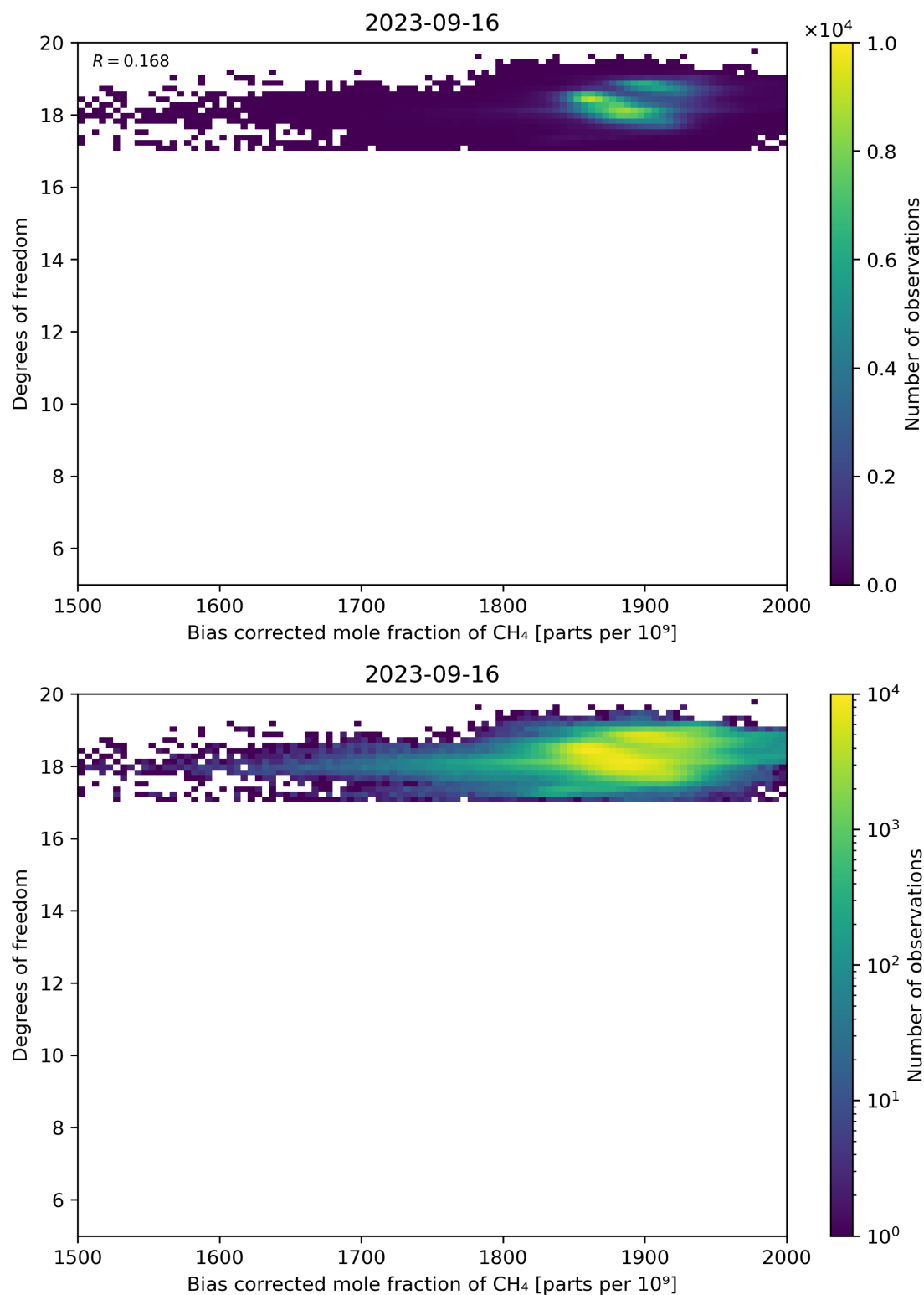
Figure 65: Scatter density plot of “Bias corrected mole fraction of CH 4 ” against “Degrees of freedom” for 2023-09-15 to 2023-09-17.
