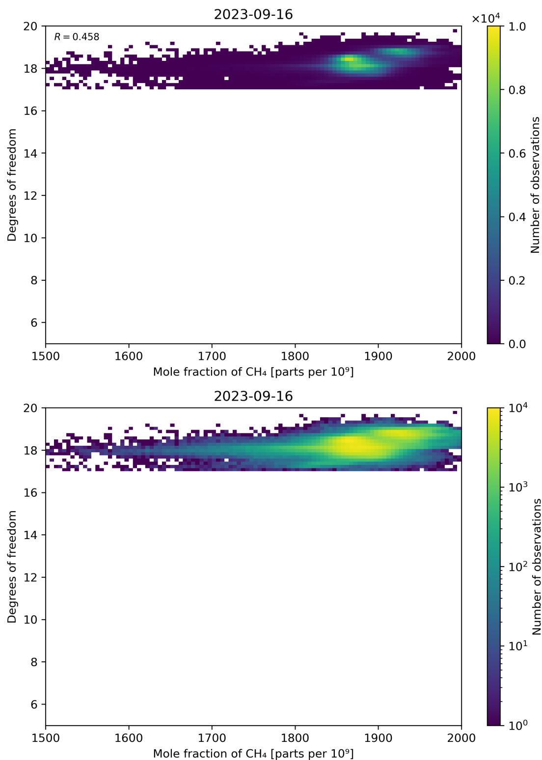
Figure 72: Scatter density plot of “Mole fraction of CH 4 ” against “Degrees of freedom” for 2023-09-15 to 2023-09-17.
