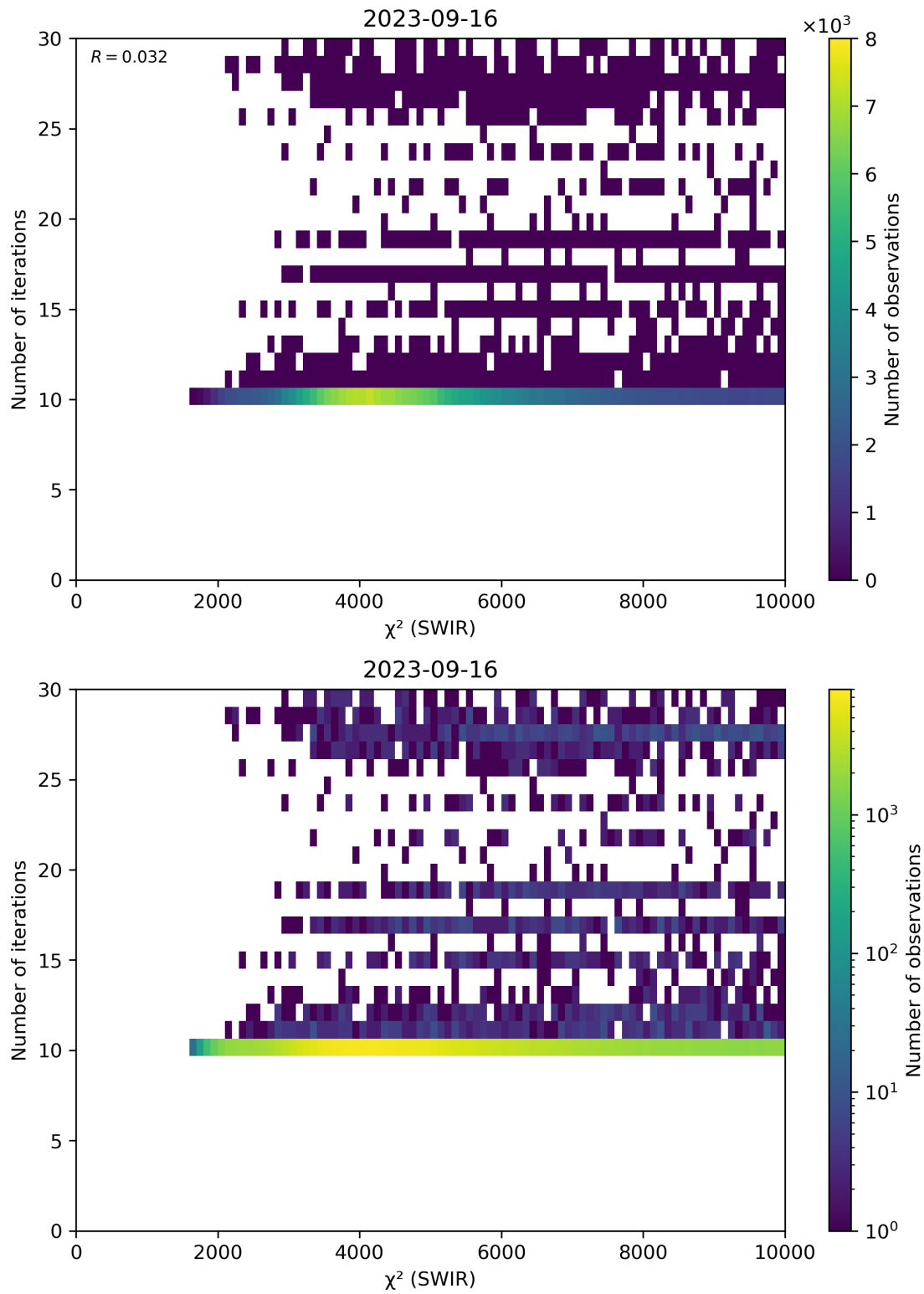
Figure 50: Scatter density plot of “ \chi^2 (SWIR)” against “Number of iterations” for 2023-09-15 to 2023-09-17.
