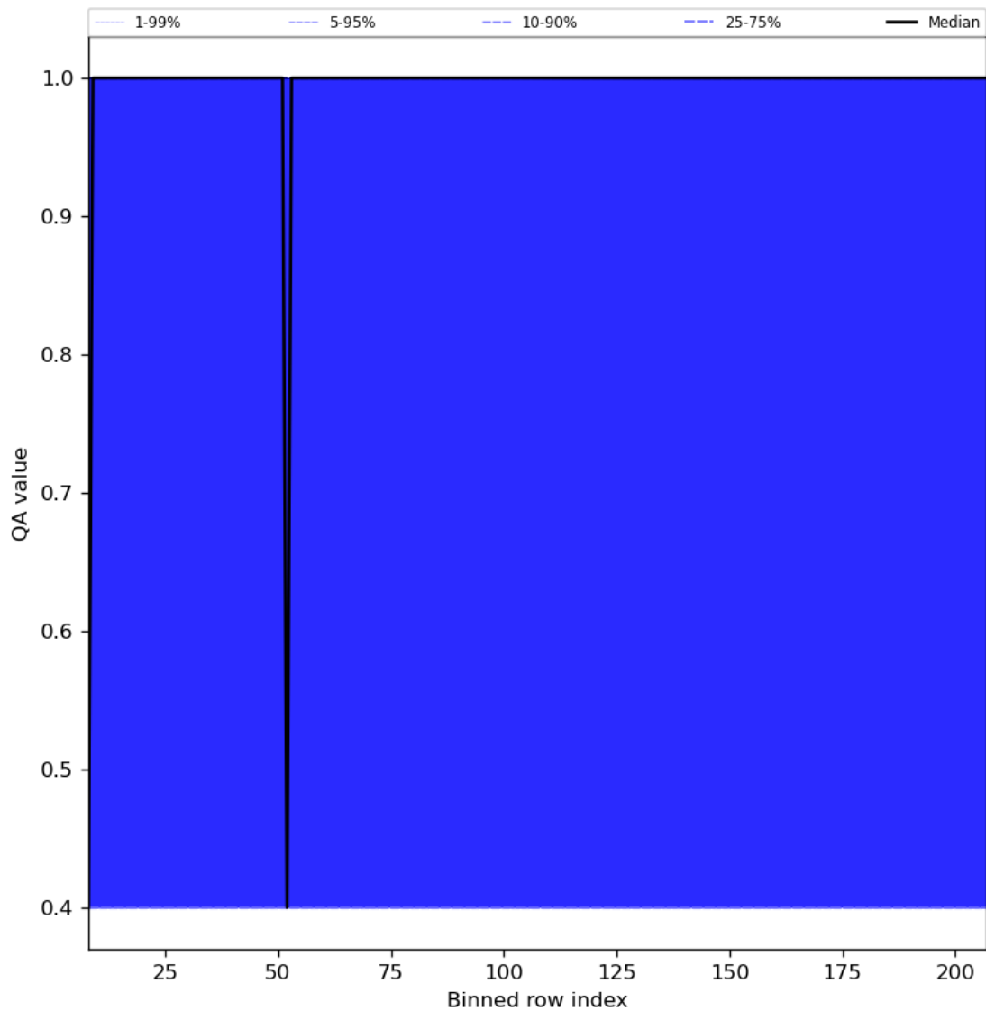
Figure 33: Along track statistics of “QA value” for 2023-09-15 to 2023-09-17
