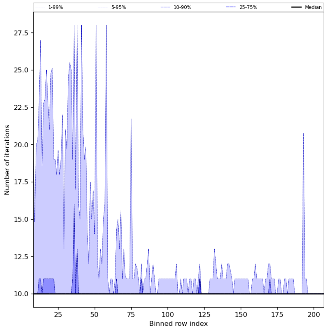
Figure 42: Along track statistics of “Number of iterations” for 2023-09-15 to 2023-09-17
