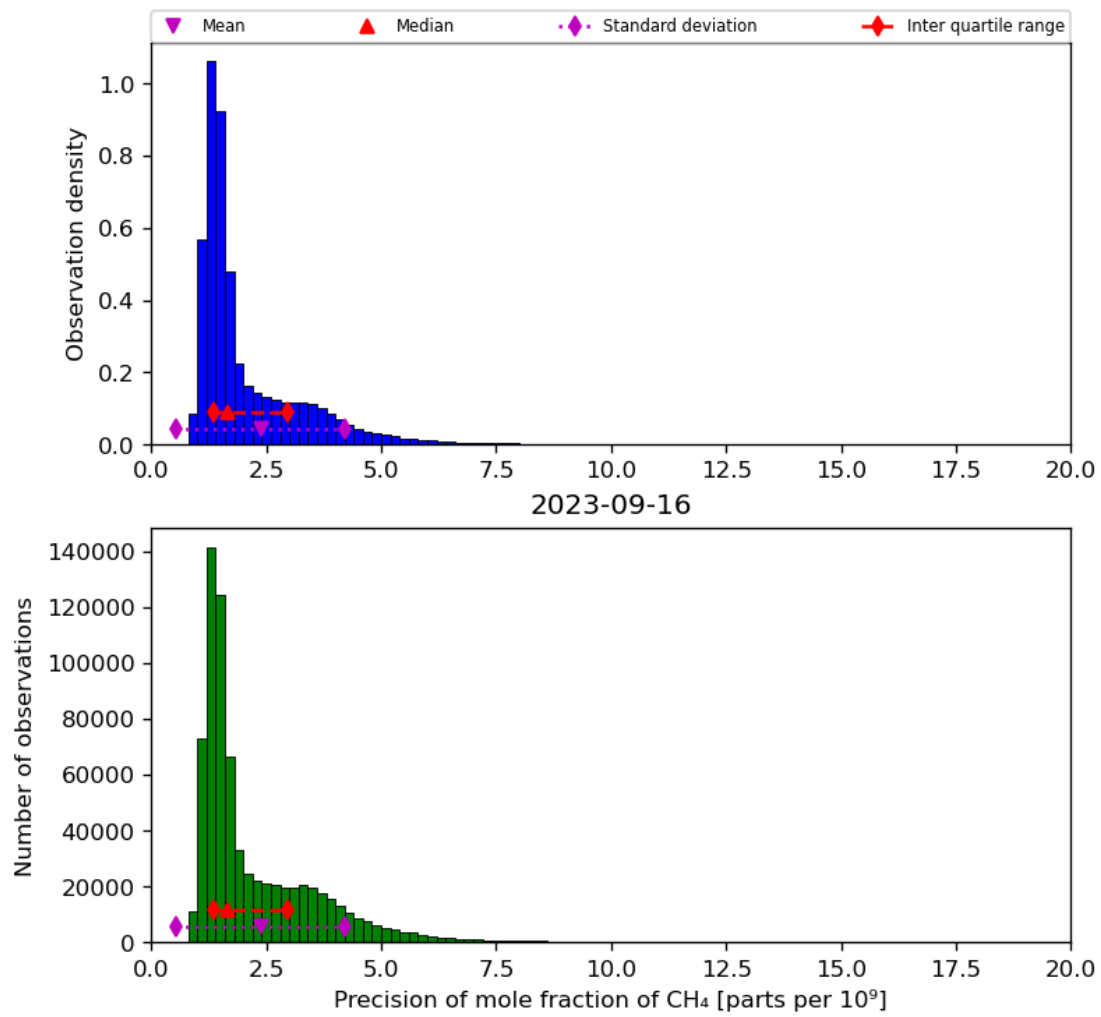
Figure 24: Histogram of “Precision of mole fraction of CH 4 ” for 2023-09-15 to 2023-09-17
