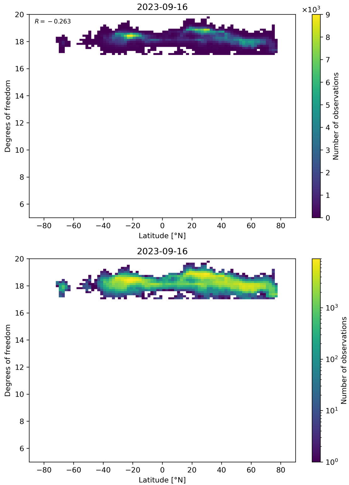
Figure 55: Scatter density plot of “Latitude” against “Degrees of freedom” for 2023-09-15 to 2023-09-17.
