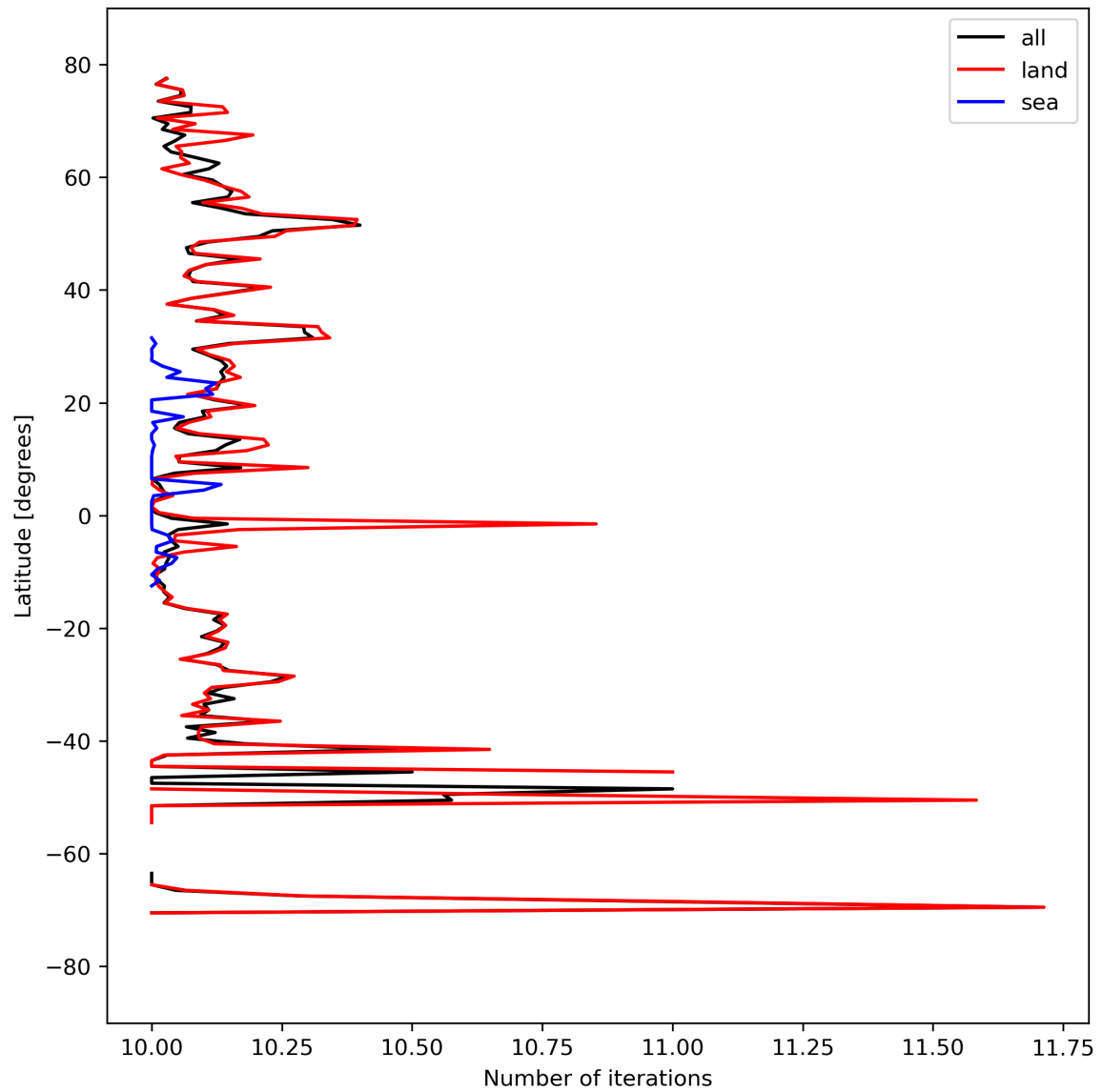
Figure 20: Zonal average of “Number of iterations” for 2023-09-15 to 2023-09-17.
