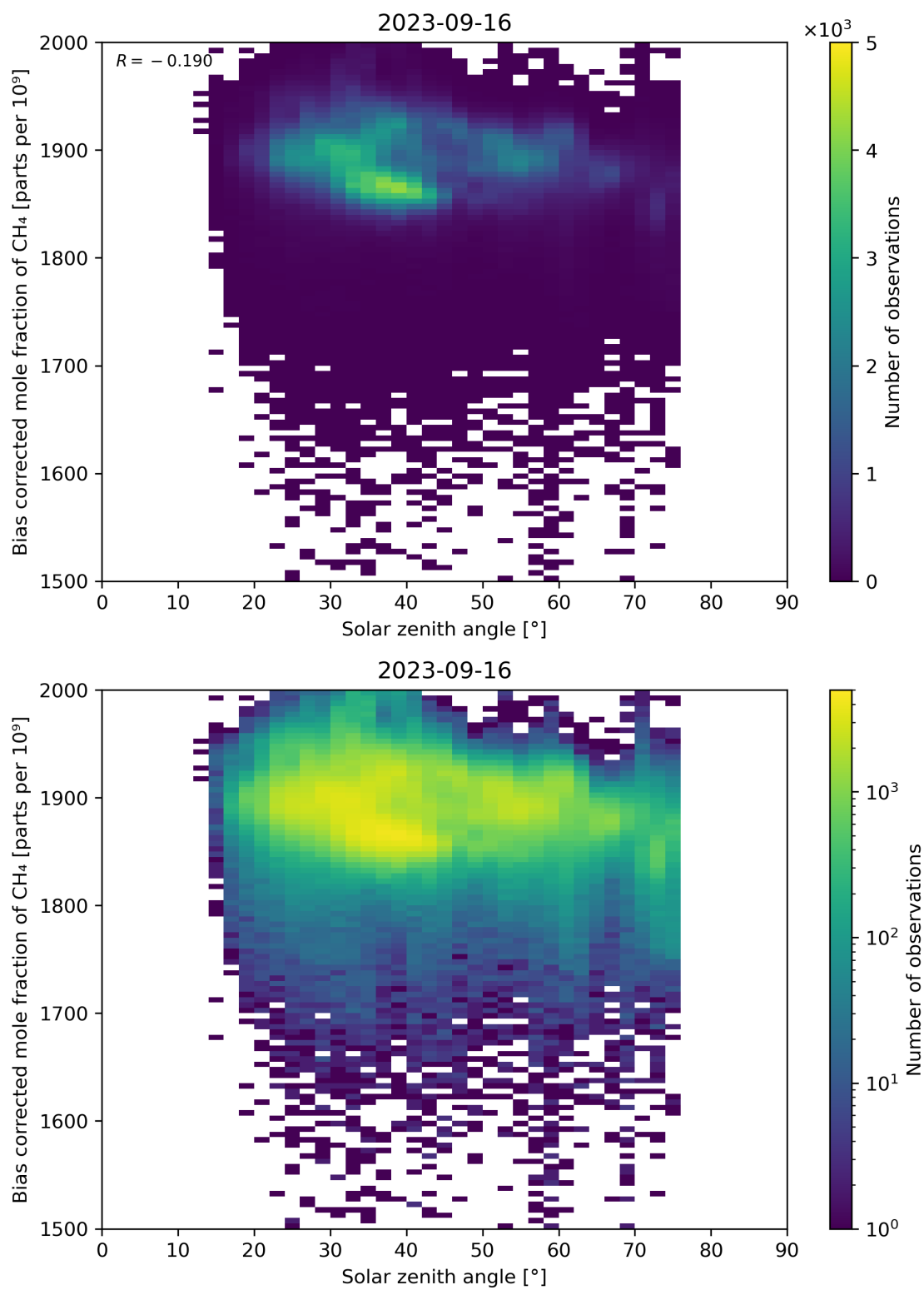
Figure 100: Scatter density plot of “Solar zenith angle” against “Bias corrected mole fraction of \text{CH}_4 ” for 2023-09-15 to 2023-09-17.
