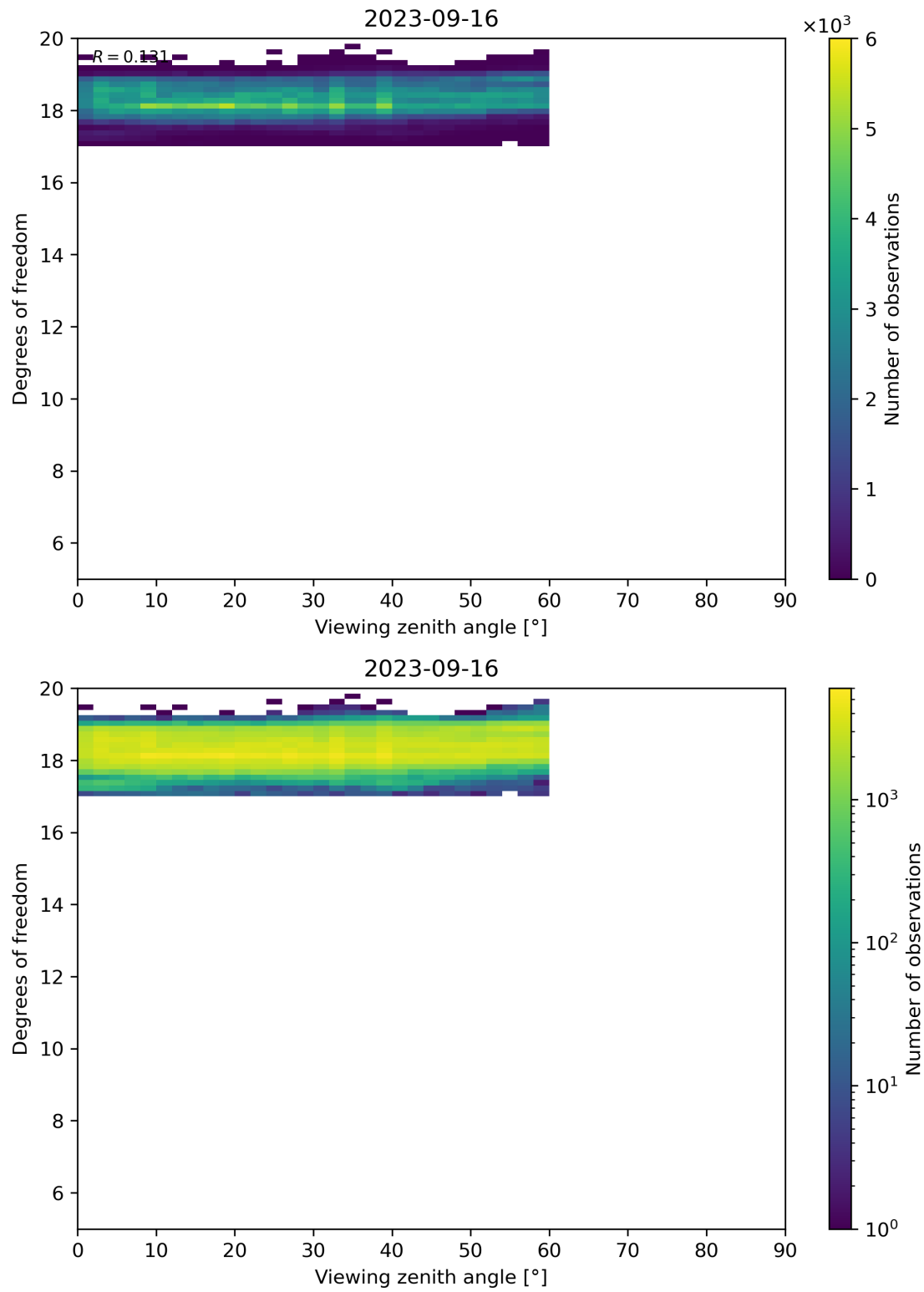
Figure 107: Scatter density plot of “Viewing zenith angle” against “Degrees of freedom” for 2023-09-15 to 2023-09-17.
