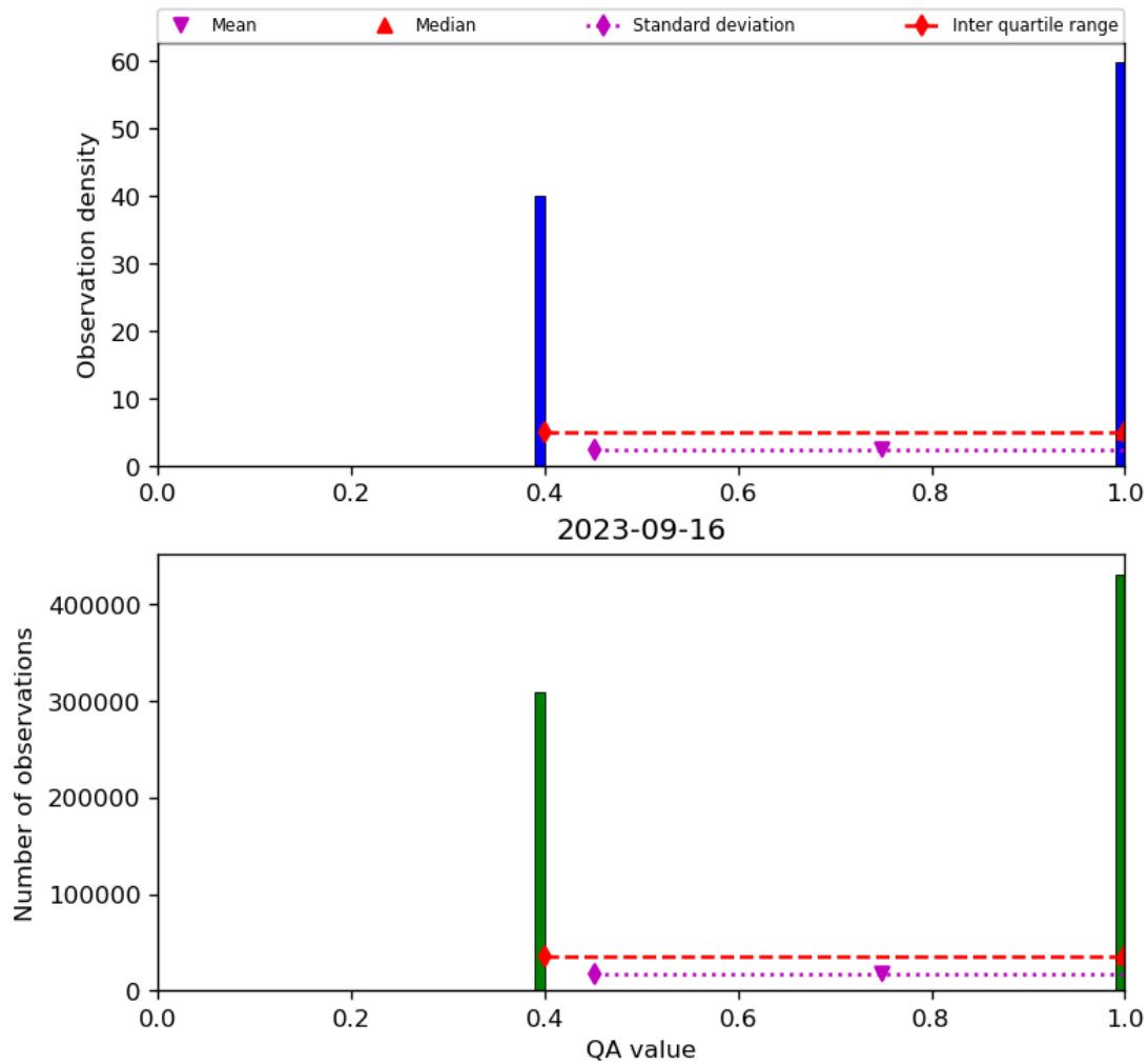
Figure 22: Histogram of “QA value” for 2023-09-15 to 2023-09-17
