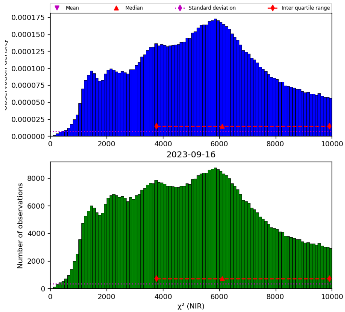
Figure 29: Histogram of “ \chi^2 (NIR)” for 2023-09-15 to 2023-09-17
