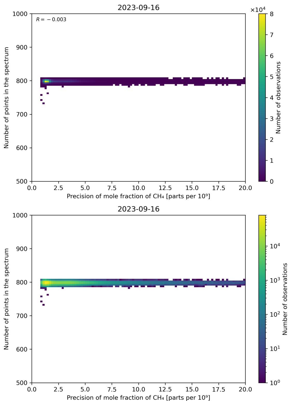
Figure 84: Scatter density plot of “Precision of mole fraction of CH 4 ” against “Number of points in the spectrum” for 2023-09-15 to 2023-09-17.
