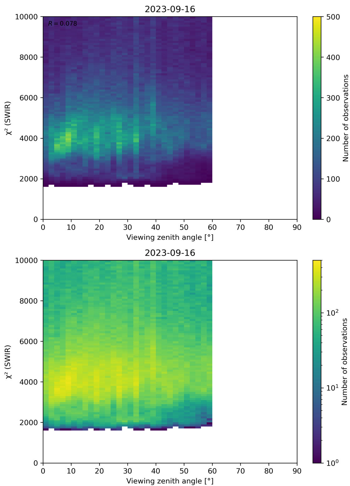
Figure 106: Scatter density plot of “Viewing zenith angle” against “ \chi^2 (SWIR)” for 2023-09-15 to 2023-09-17.
