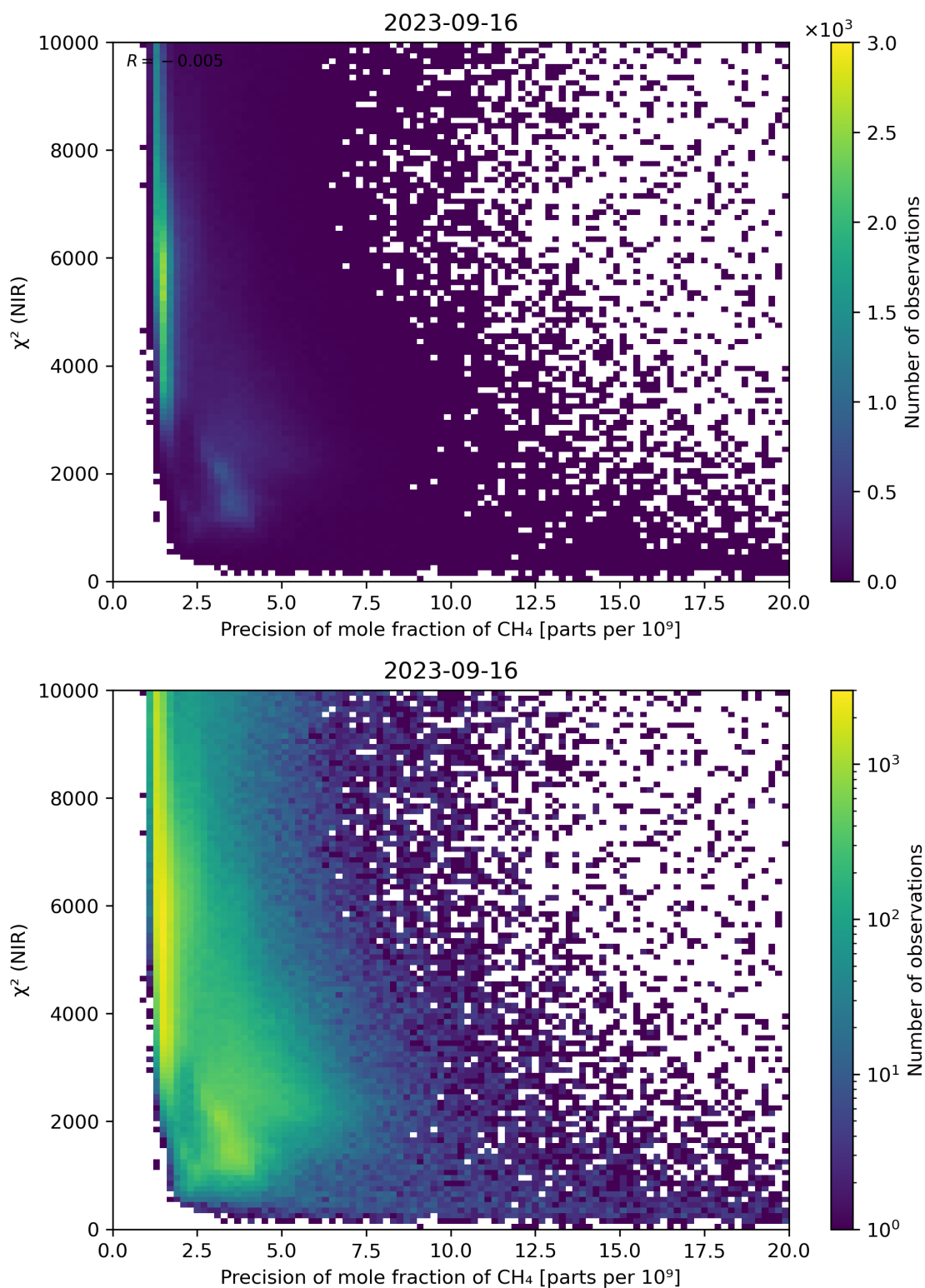
Figure 78: Scatter density plot of “Precision of mole fraction of CH 4 ” against “ \chi^2 (NIR)” for 2023-09-15 to 2023-09-17.
