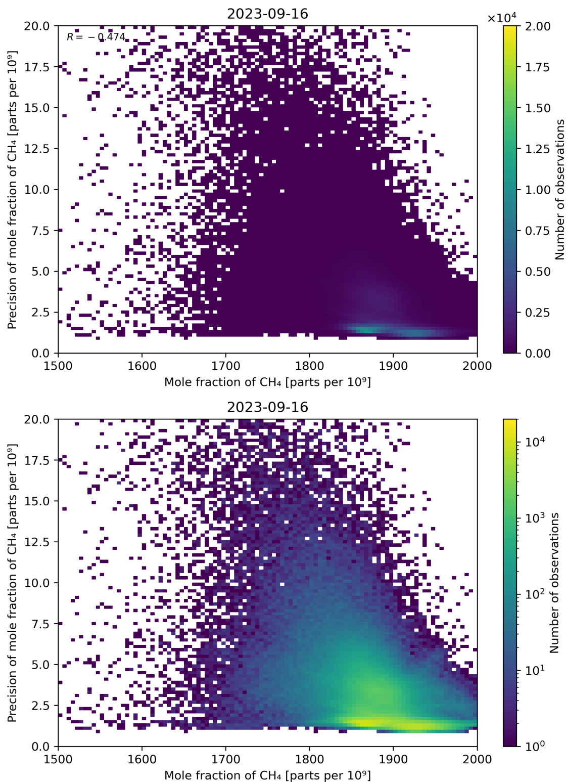
Figure 75: Scatter density plot of “Mole fraction of CH 4 ” against “Precision of mole fraction of CH 4 ” for 2023-09-15 to 2023-09-17.
