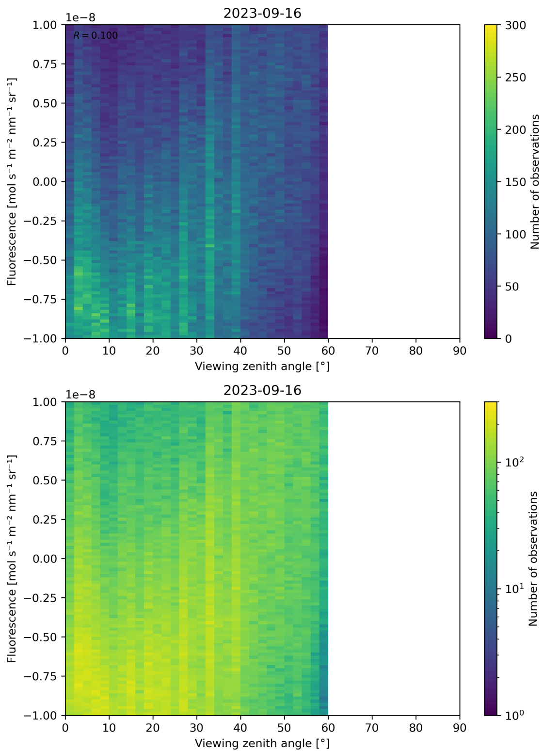
Figure 108: Scatter density plot of “Viewing zenith angle” against “Fluorescence” for 2023-09-15 to 2023-09-17.
