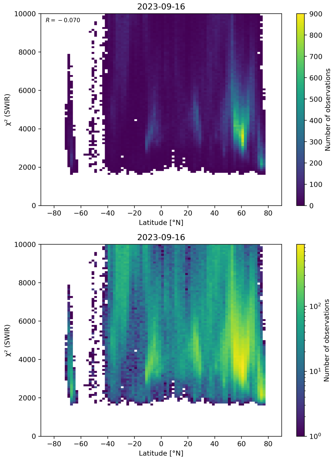
Figure 54: Scatter density plot of “Latitude” against “ \chi^2 (SWIR)” for 2023-09-15 to 2023-09-17.
