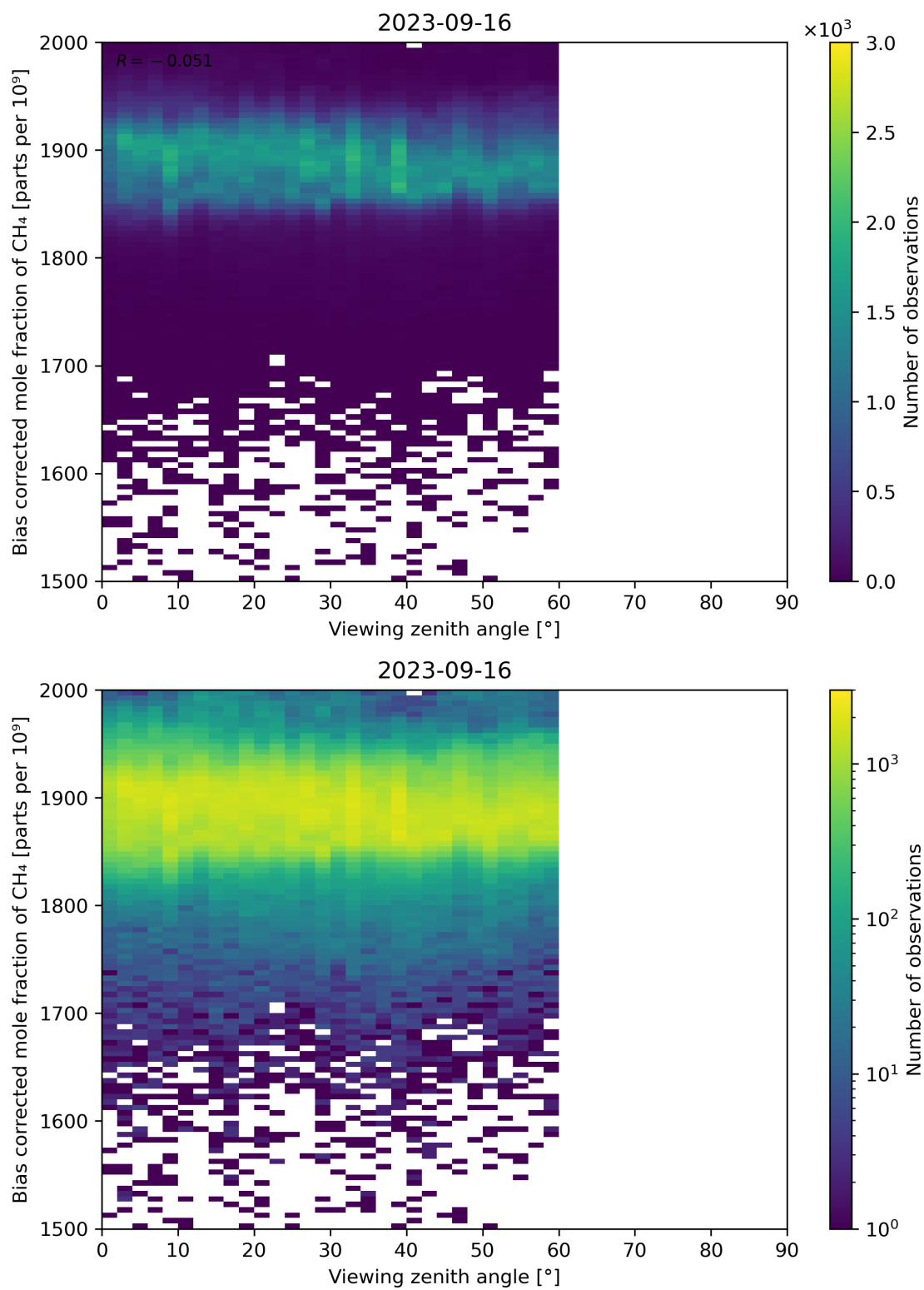
Figure 111: Scatter density plot of “Viewing zenith angle” against “Bias corrected mole fraction of CH 4 ” for 2023-09-15 to 2023-09-17.
