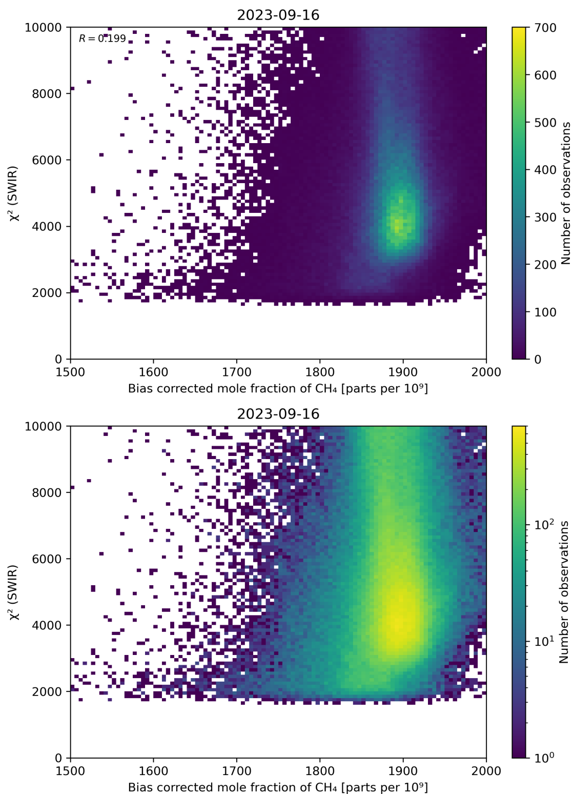
Figure 64: Scatter density plot of “Bias corrected mole fraction of CH 4 ” against “ \chi^2 (SWIR)” for 2023-09-15 to 2023-09-17.
