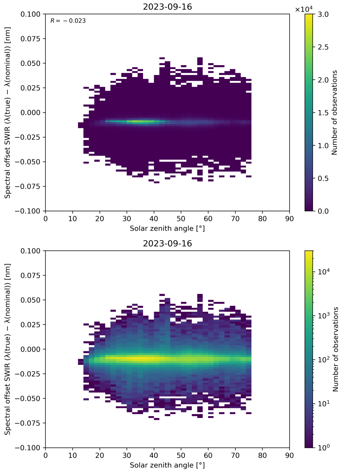
Figure 104: Scatter density plot of “Solar zenith angle” against “Spectral offset SWIR ( \lambda(\text{true}) - \lambda(\text{nominal}) )” for 2023-09-15 to 2023-09-17.
