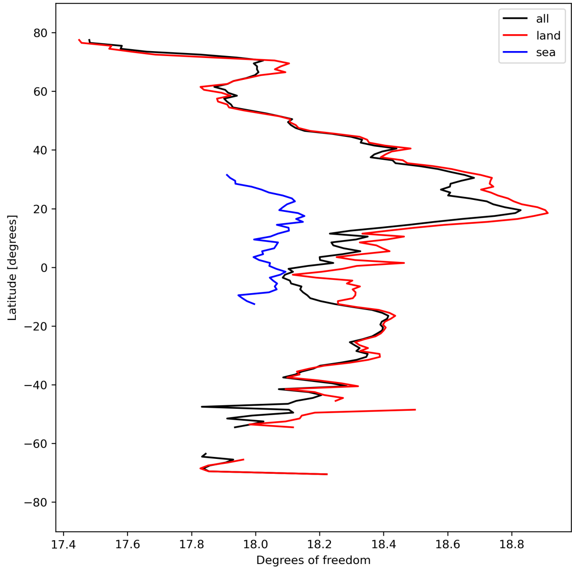
Figure 19: Zonal average of “Degrees of freedom” for 2023-09-15 to 2023-09-17.
