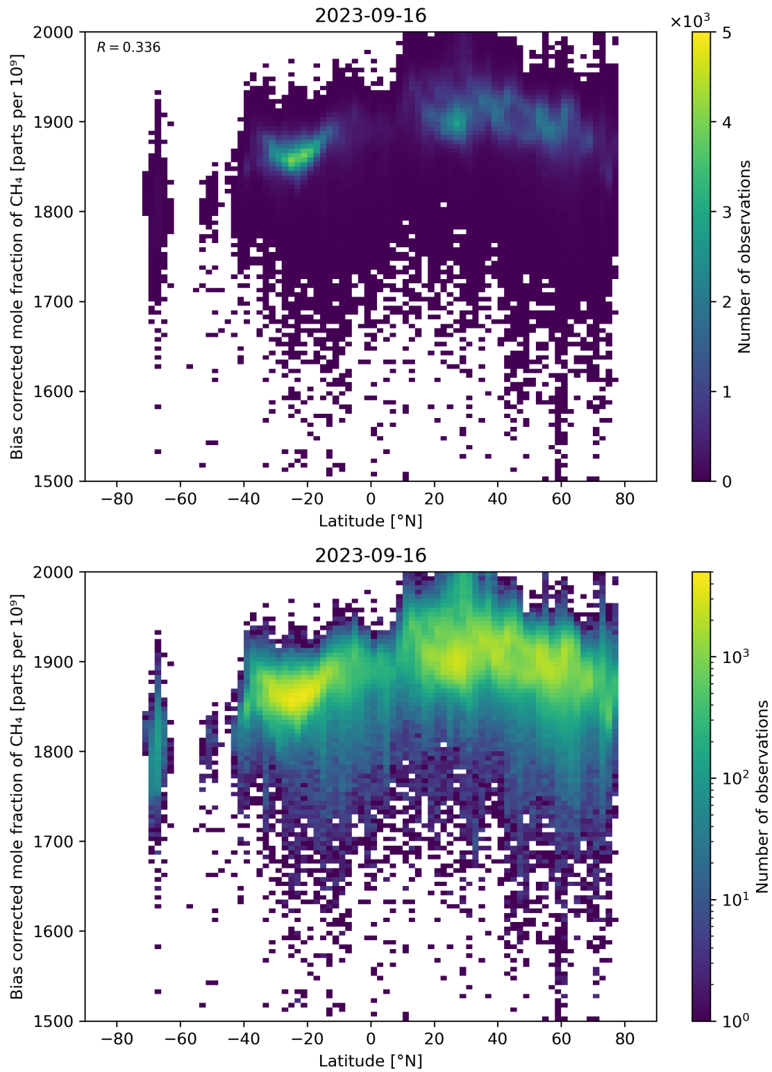
Figure 58: Scatter density plot of “Latitude” against “Bias corrected mole fraction of \text{CH}_4 ” for 2023-09-15 to 2023-09-17.
