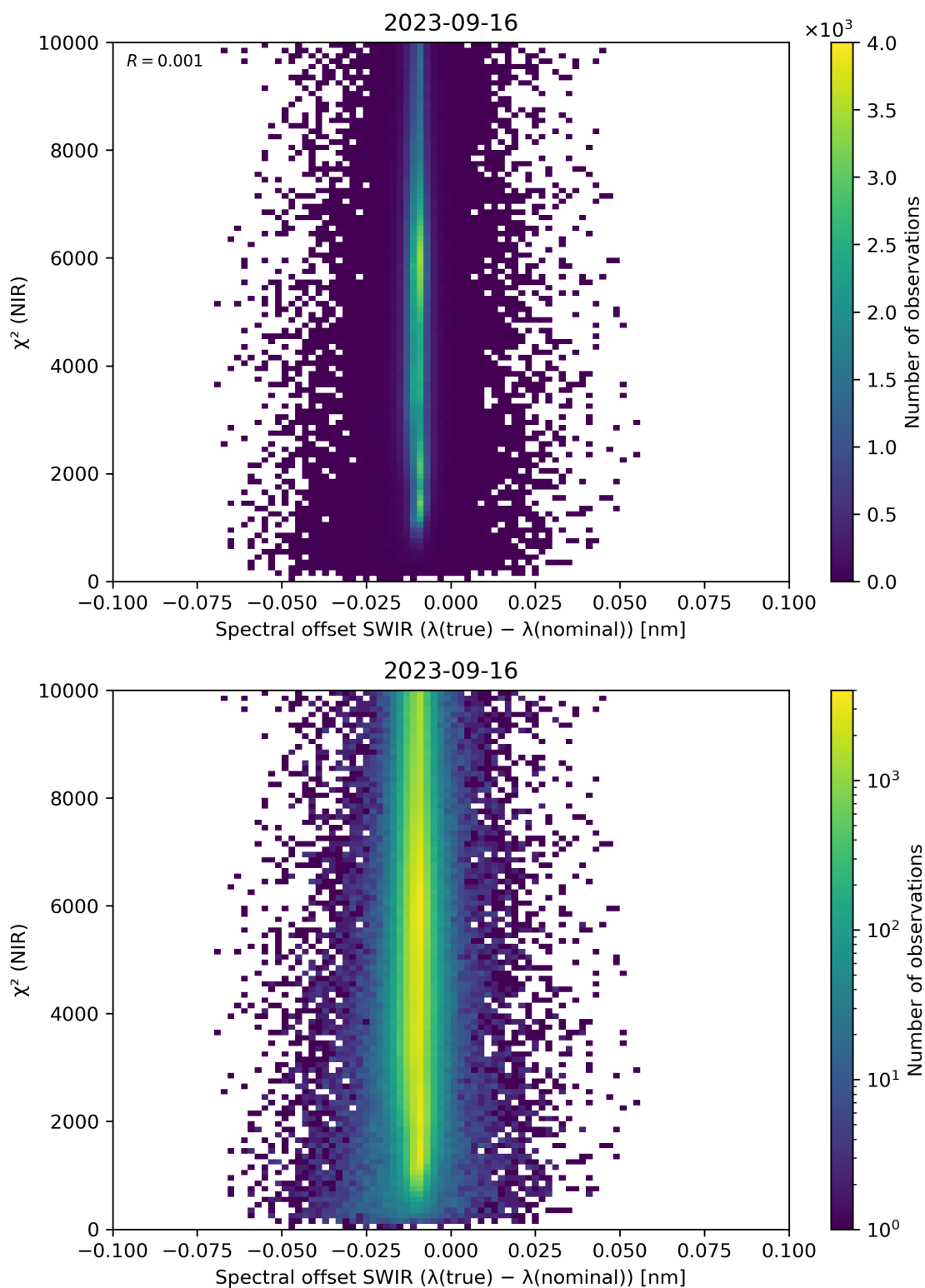
Figure 117: Scatter density plot of “Spectral offset SWIR ( \lambda(\text{true}) - \lambda(\text{nominal}) )” against “ \chi^2 (NIR)” for 2023-09-15 to 2023-09-17.
