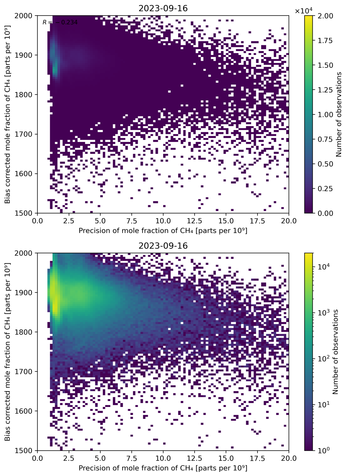
Figure 82: Scatter density plot of “Precision of mole fraction of CH 4 ” against “Bias corrected mole fraction of CH 4 ” for 2023-09-15 to 2023-09-17.
