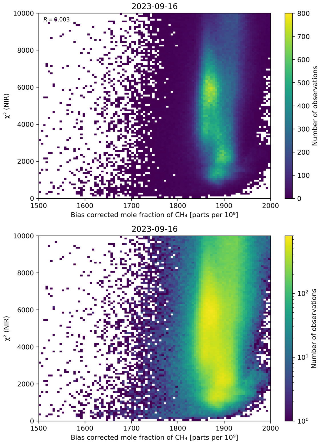
Figure 63: Scatter density plot of “Bias corrected mole fraction of CH 4 ” against “ \chi^2 (NIR)” for 2023-09-15 to 2023-09-17.
