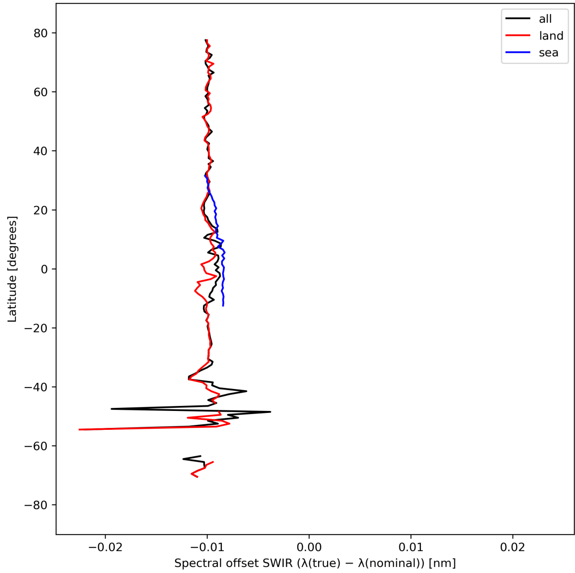
Figure 16: Zonal average of “Spectral offset SWIR ( \lambda(\text{true}) - \lambda(\text{nominal}) )” for 2023-09-15 to 2023-09-17.
