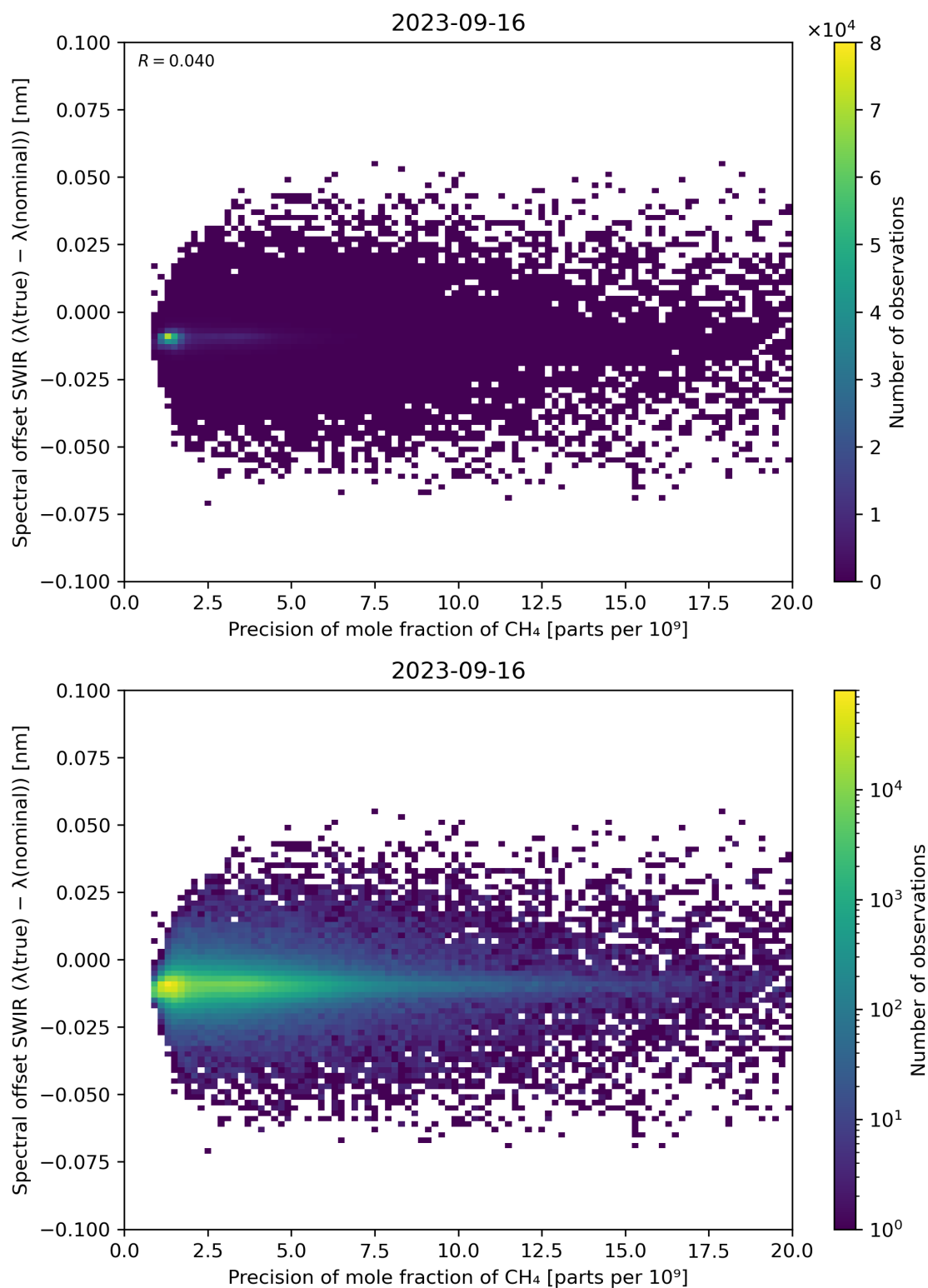
Figure 85: Scatter density plot of “Precision of mole fraction of \text{CH}_4 ” against “Spectral offset SWIR ( \lambda(\text{true}) - \lambda(\text{nominal}) )” for 2023-09-15 to 2023-09-17.
