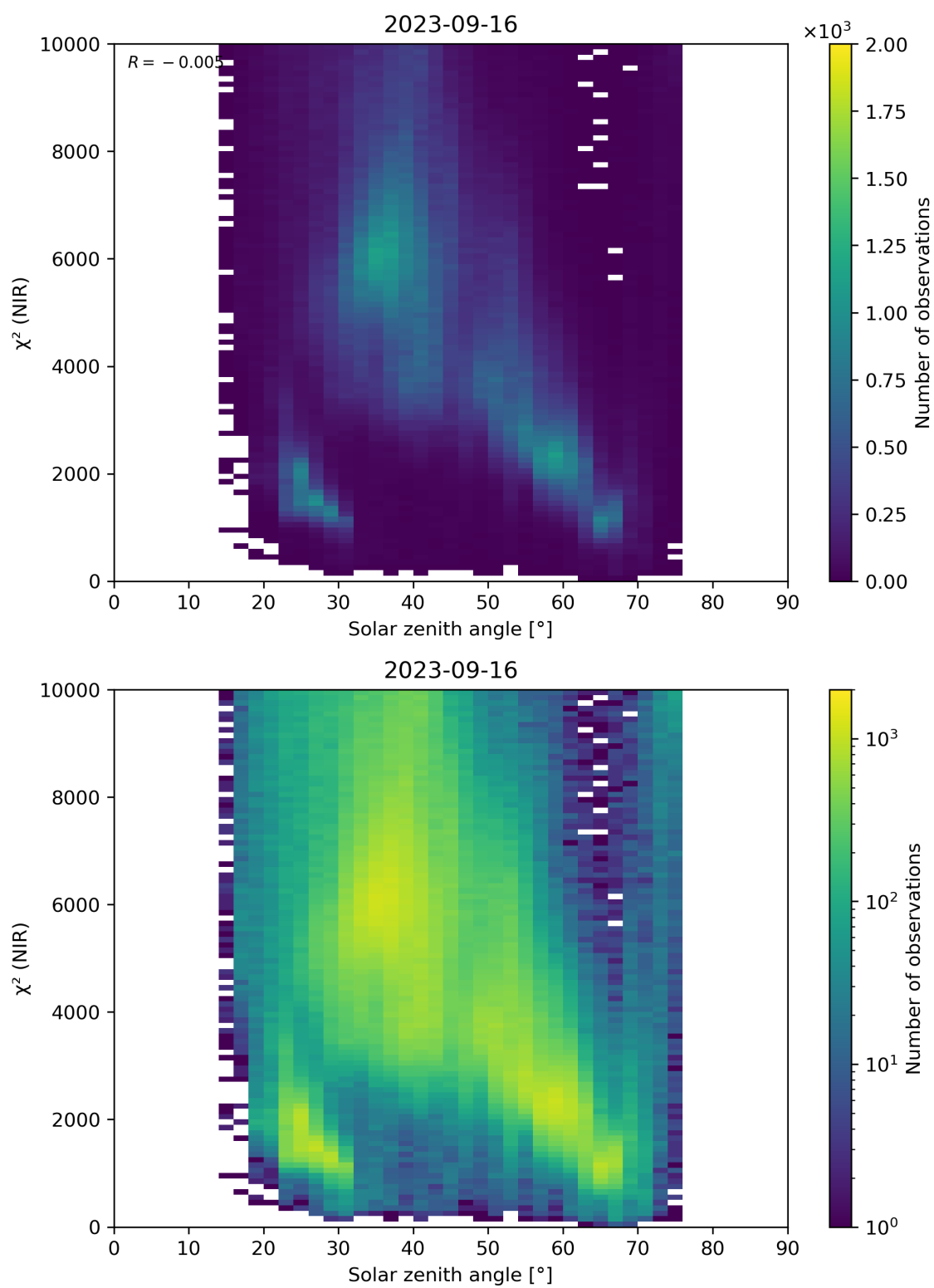
Figure 94: Scatter density plot of “Solar zenith angle” against “ \chi^2 (NIR)” for 2023-09-15 to 2023-09-17.
