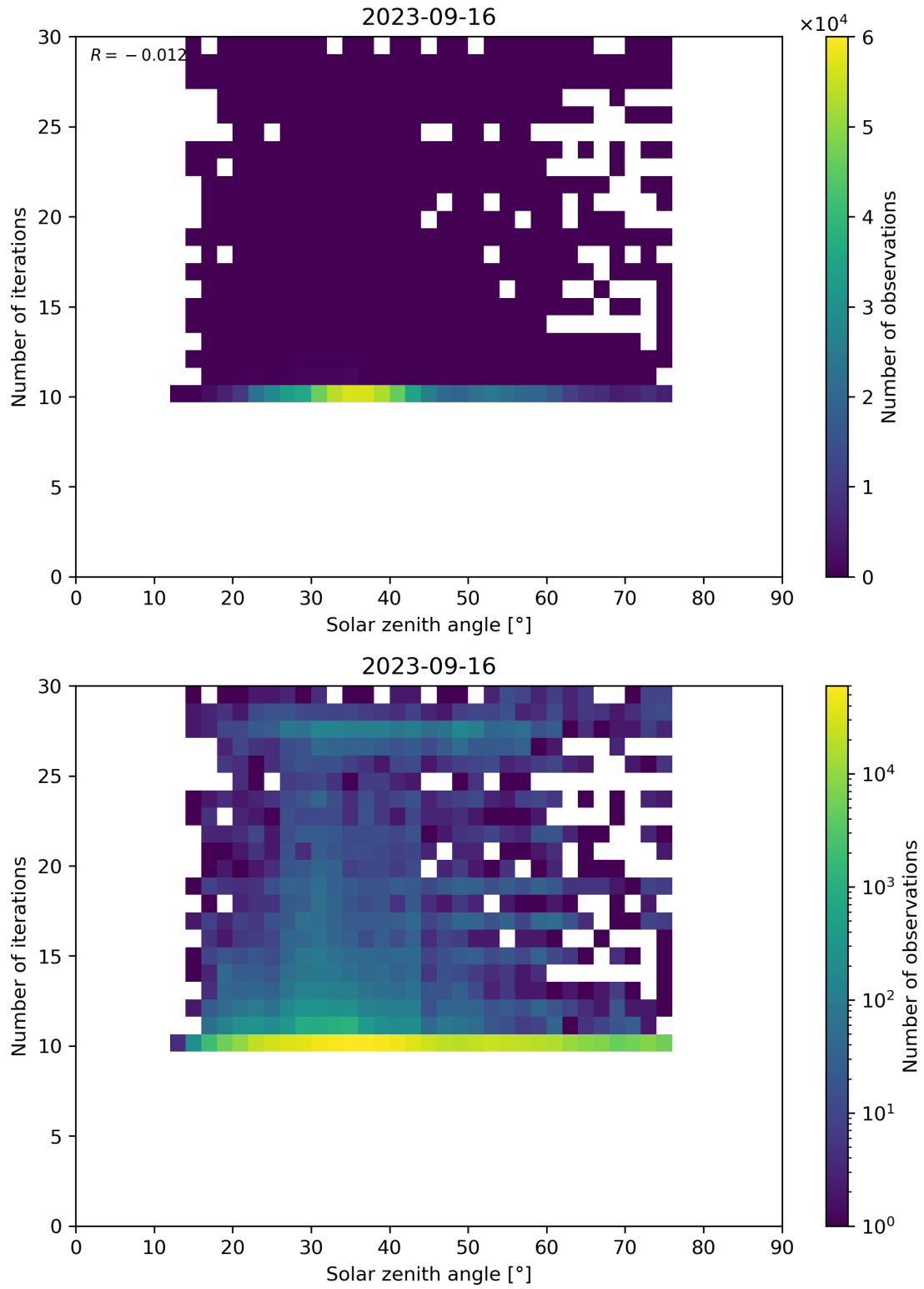
Figure 102: Scatter density plot of “Solar zenith angle” against “Number of iterations” for 2023-09-15 to 2023-09-17.
