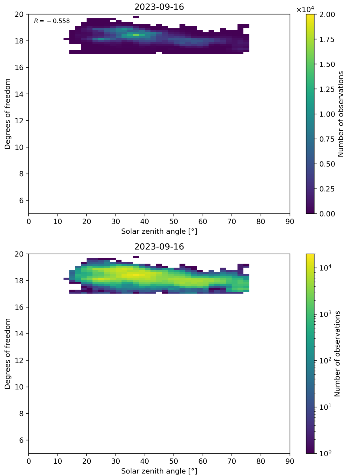
Figure 96: Scatter density plot of “Solar zenith angle” against “Degrees of freedom” for 2023-09-15 to 2023-09-17.
