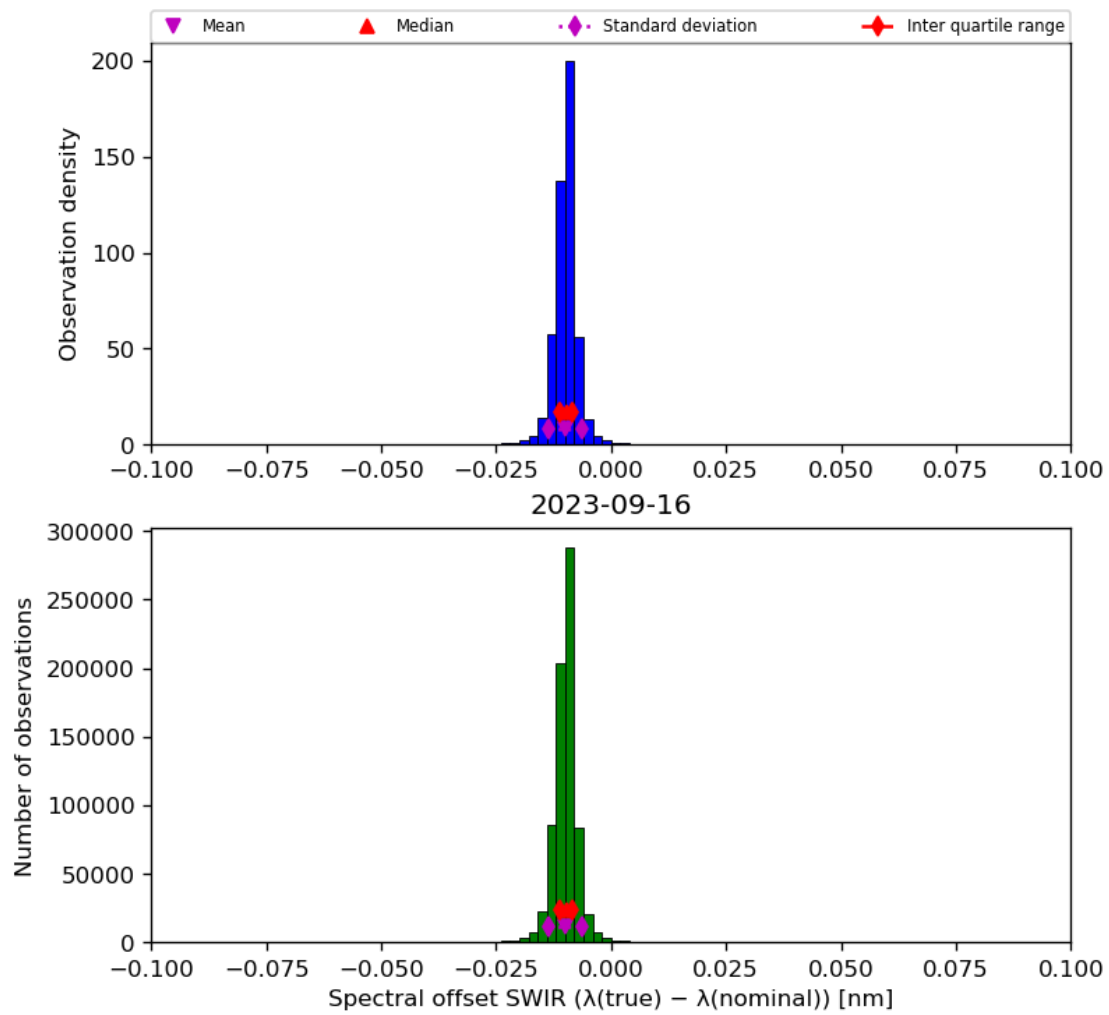
Figure 27: Histogram of “Spectral offset SWIR ( \lambda(\text{true}) - \lambda(\text{nominal}) )” for 2023-09-15 to 2023-09-17
