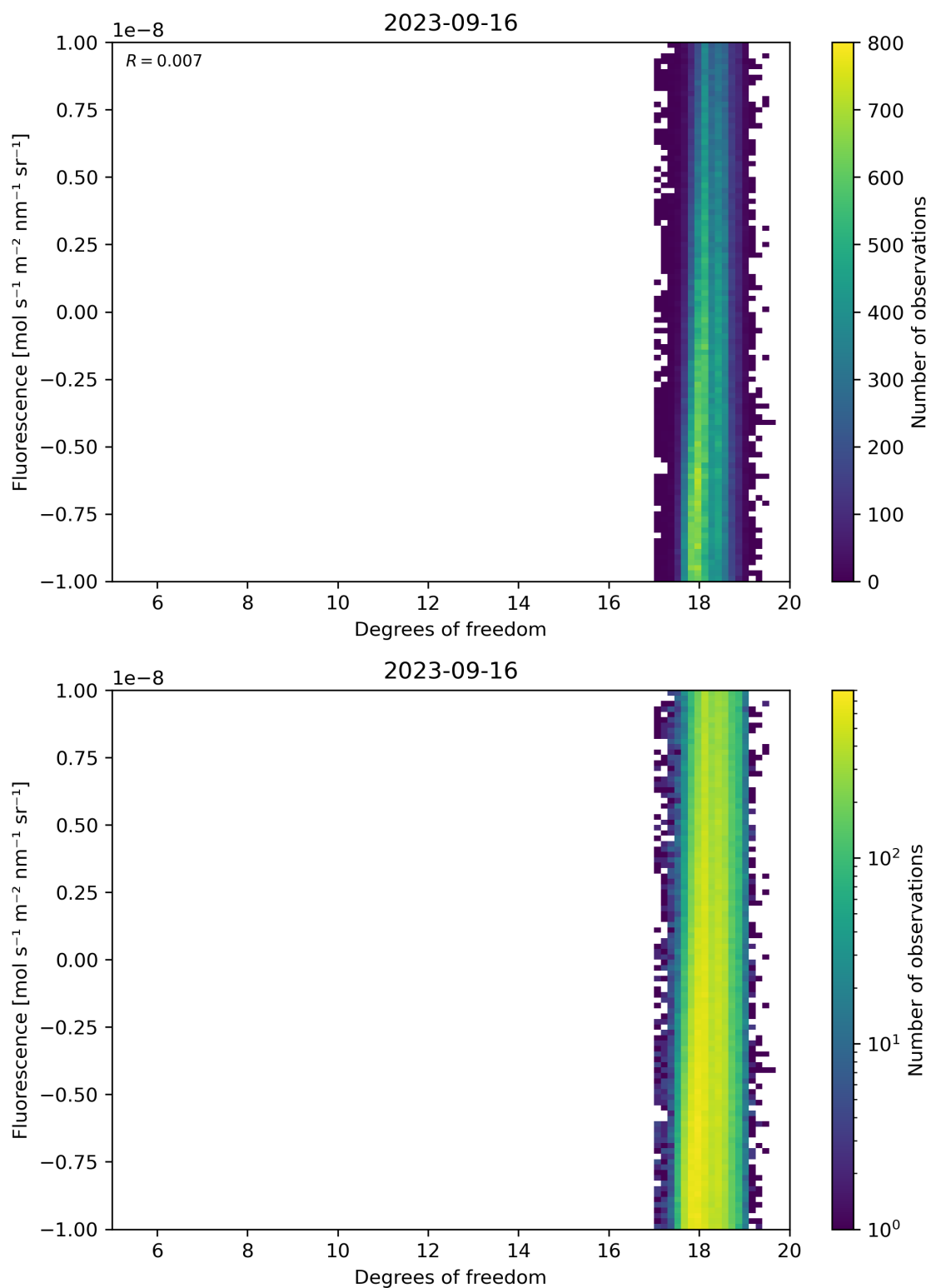
Figure 51: Scatter density plot of “Degrees of freedom” against “Fluorescence” for 2023-09-15 to 2023-09-17.
