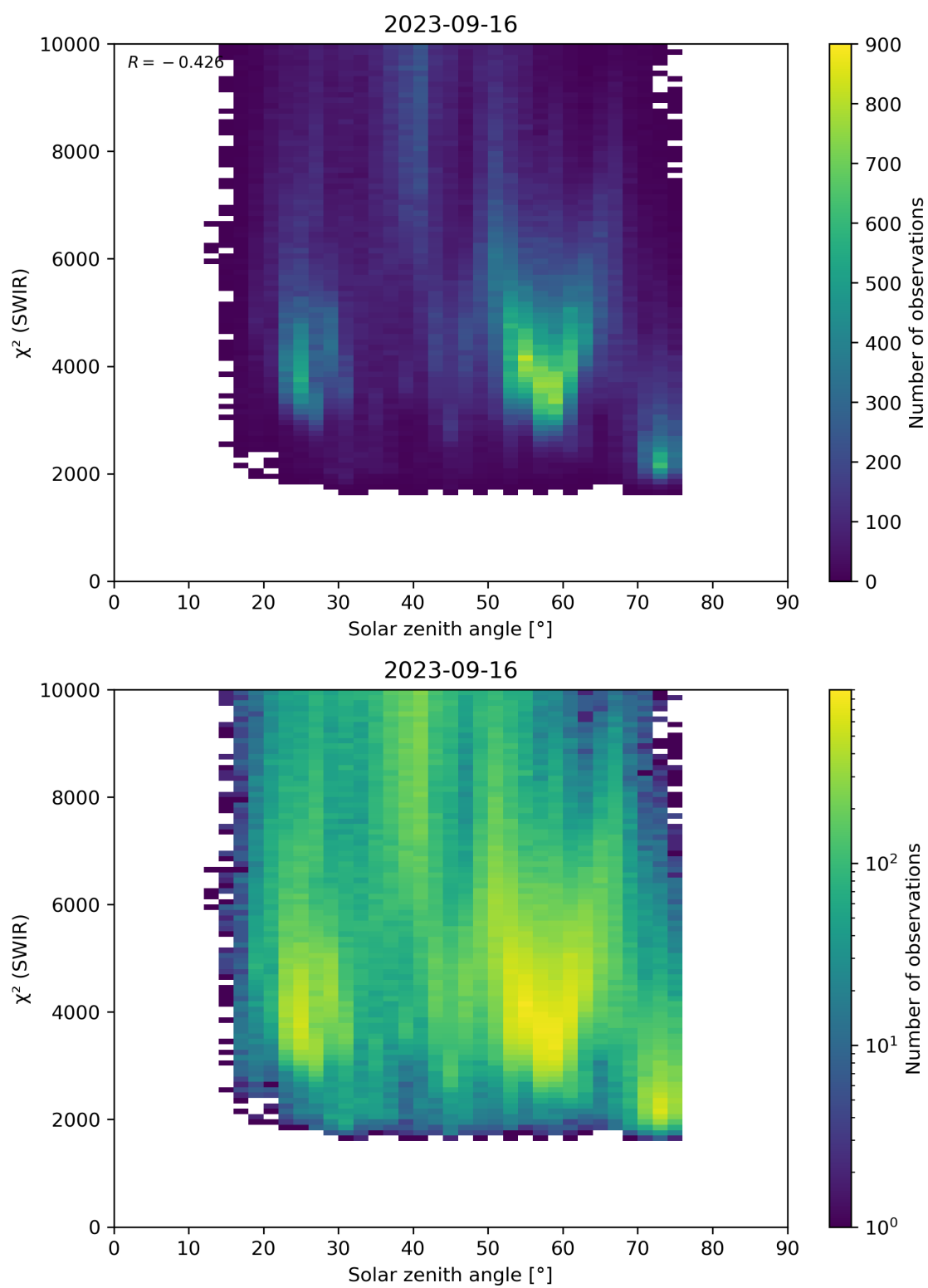
Figure 95: Scatter density plot of “Solar zenith angle” against “ \chi^2 (SWIR)” for 2023-09-15 to 2023-09-17.
