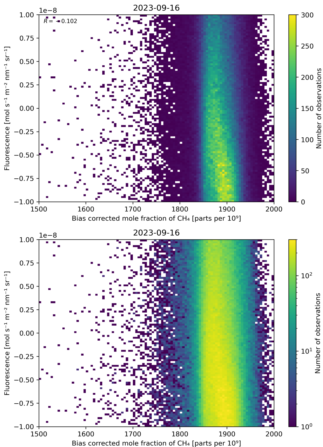
Figure 66: Scatter density plot of “Bias corrected mole fraction of \text{CH}_4 ” against “Fluorescence” for 2023-09-15 to 2023-09-17.
