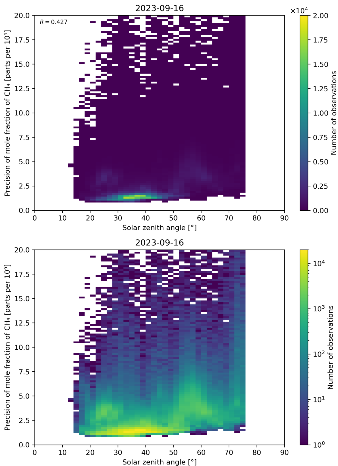
Figure 101: Scatter density plot of “Solar zenith angle” against “Precision of mole fraction of CH 4 ” for 2023-09-15 to 2023-09-17.
