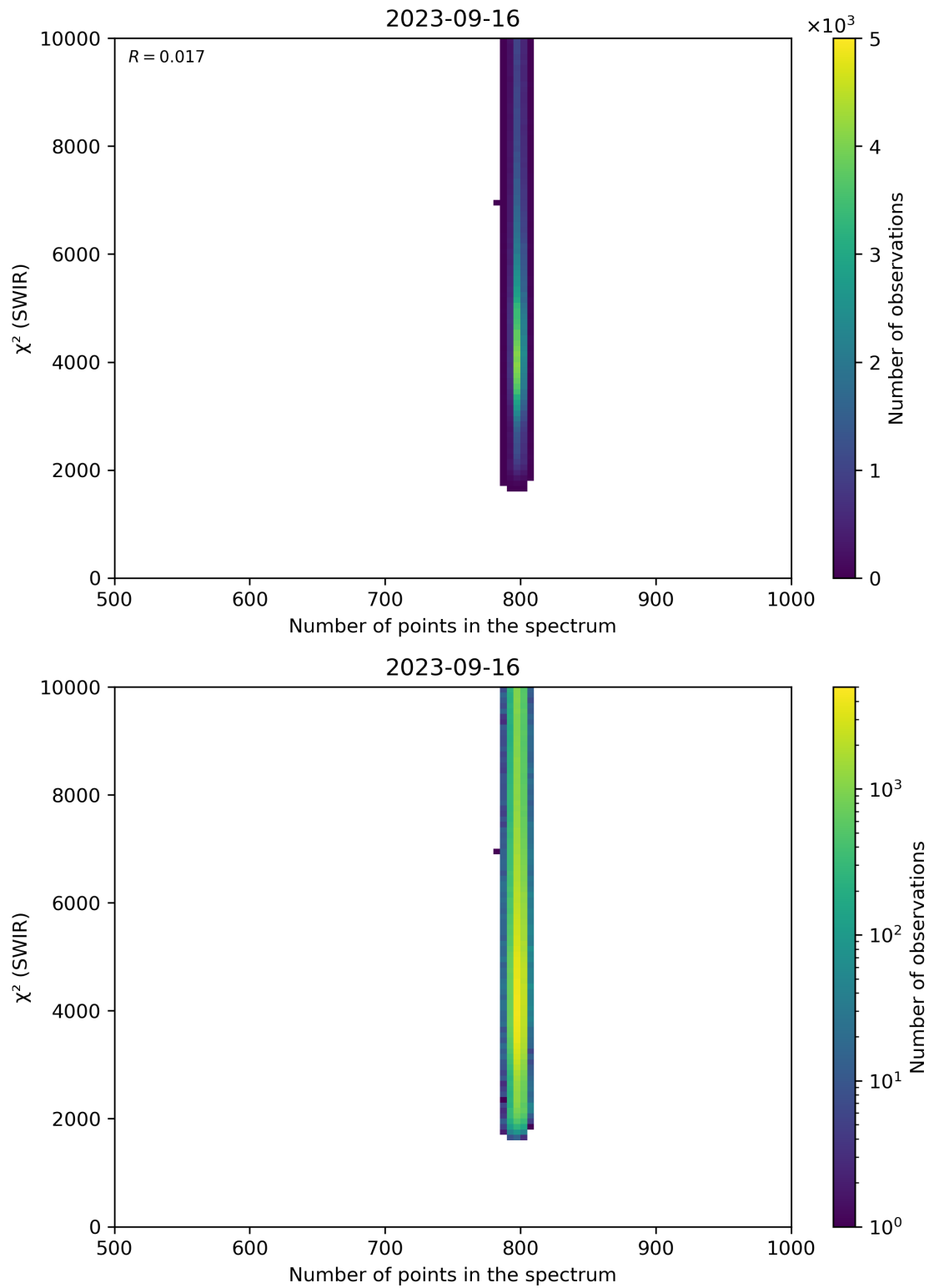
Figure 89: Scatter density plot of “Number of points in the spectrum” against “ \chi^2 (SWIR)” for 2023-09-15 to 2023-09-17.
