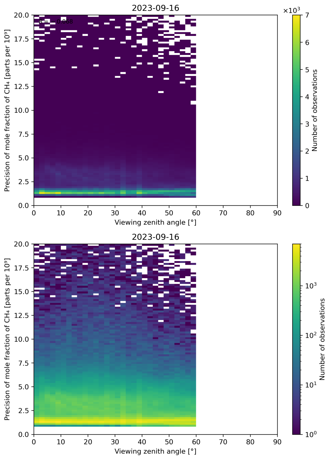
Figure 112: Scatter density plot of “Viewing zenith angle” against “Precision of mole fraction of CH 4 ” for 2023-09-15 to 2023-09-17.
