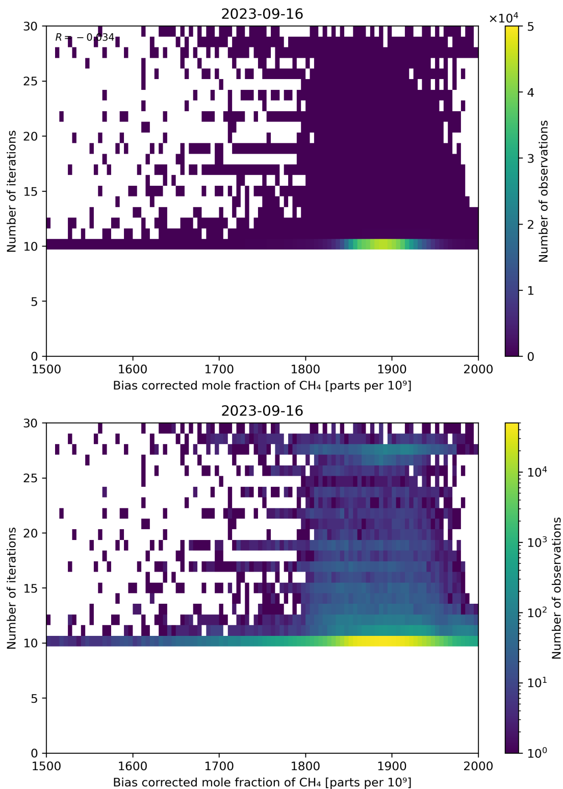
Figure 67: Scatter density plot of “Bias corrected mole fraction of CH 4 ” against “Number of iterations” for 2023-09-15 to 2023-09-17.
