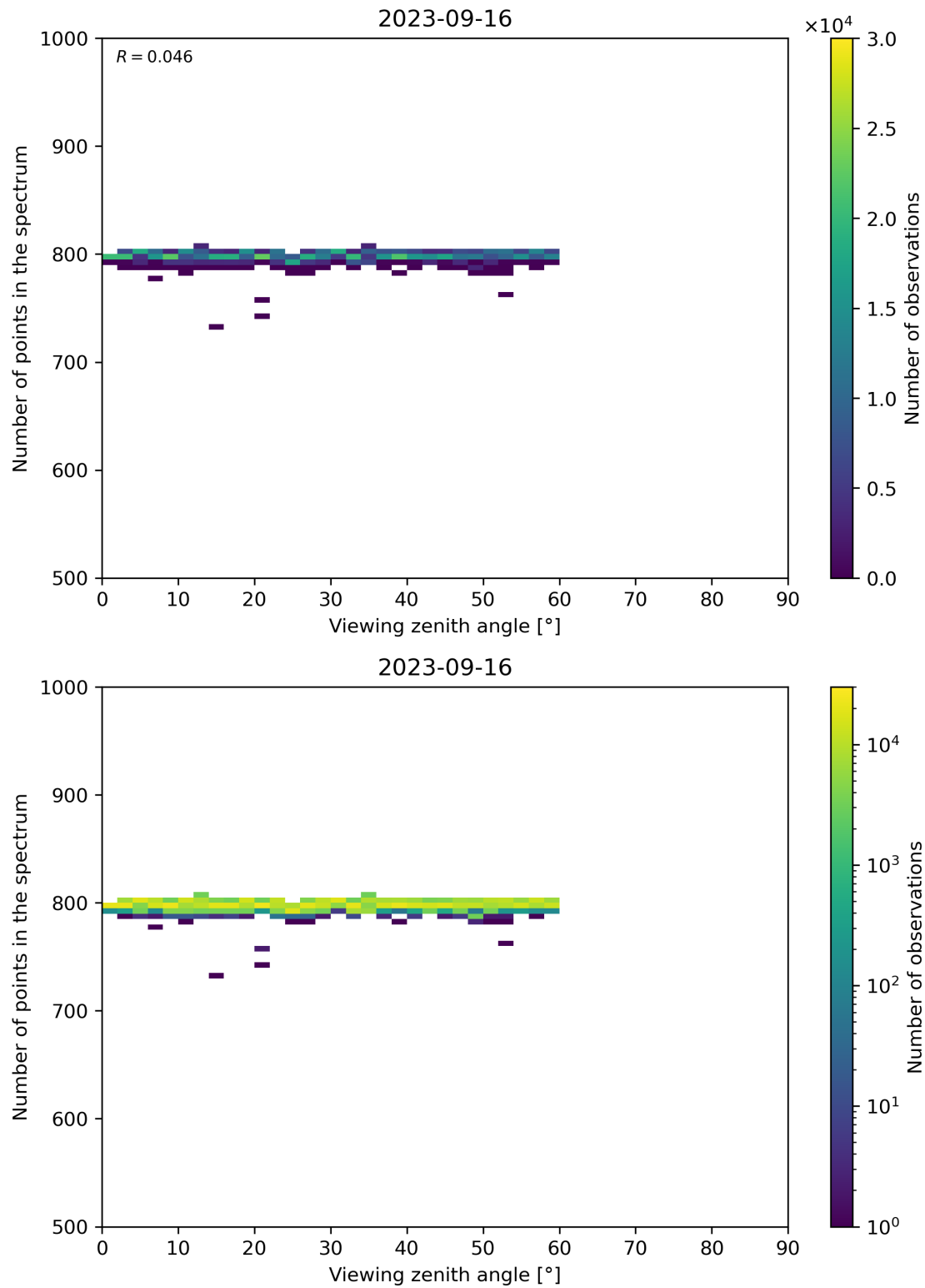
Figure 114: Scatter density plot of “Viewing zenith angle” against “Number of points in the spectrum” for 2023-09-15 to 2023-09-17.
