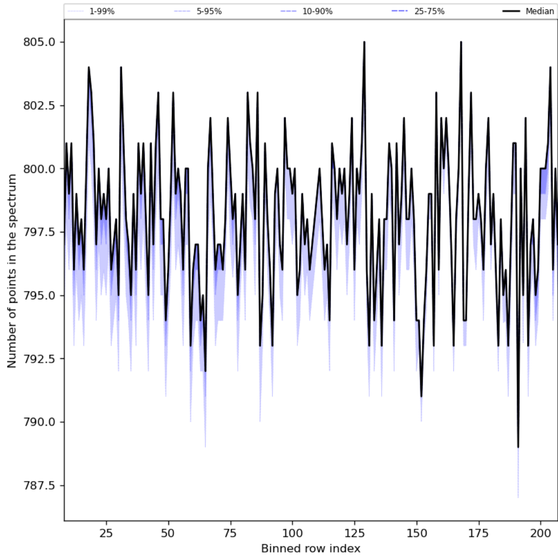
Figure 37: Along track statistics of “Number of points in the spectrum” for 2023-09-15 to 2023-09-17
