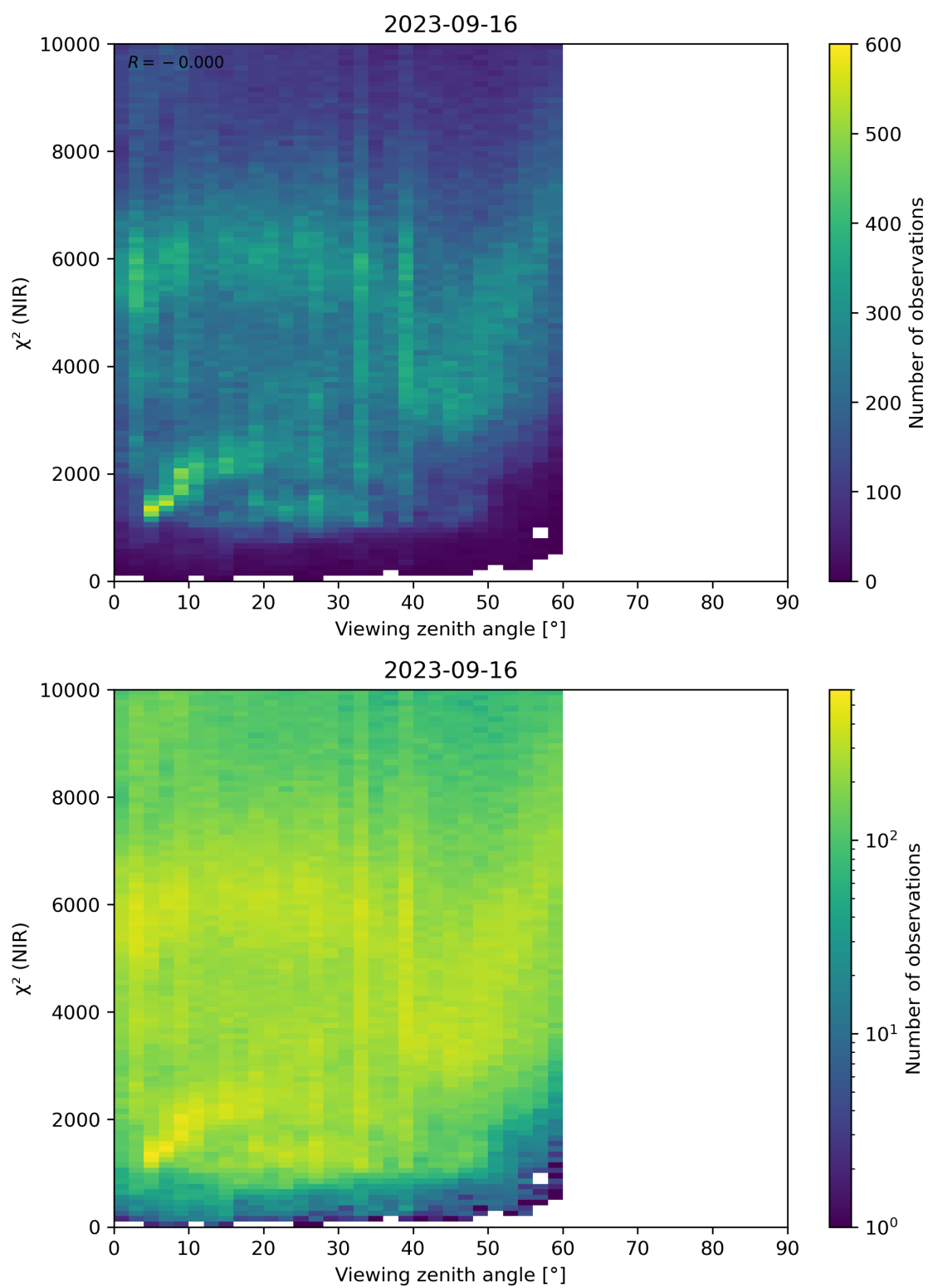
Figure 105: Scatter density plot of “Viewing zenith angle” against “ \chi^2 (NIR)” for 2023-09-15 to 2023-09-17.
