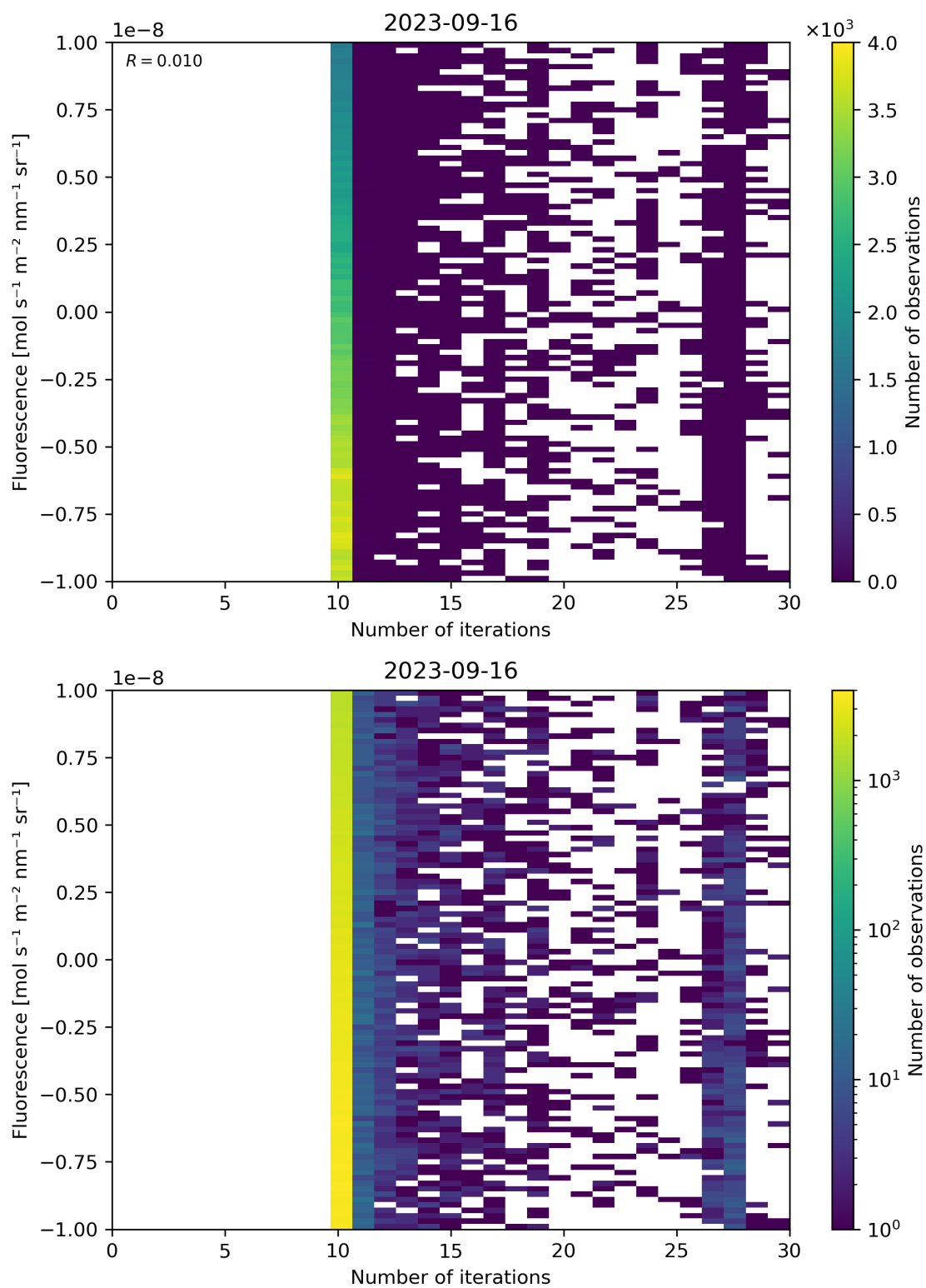
Figure 87: Scatter density plot of “Number of iterations” against “Fluorescence” for 2023-09-15 to 2023-09-17.
