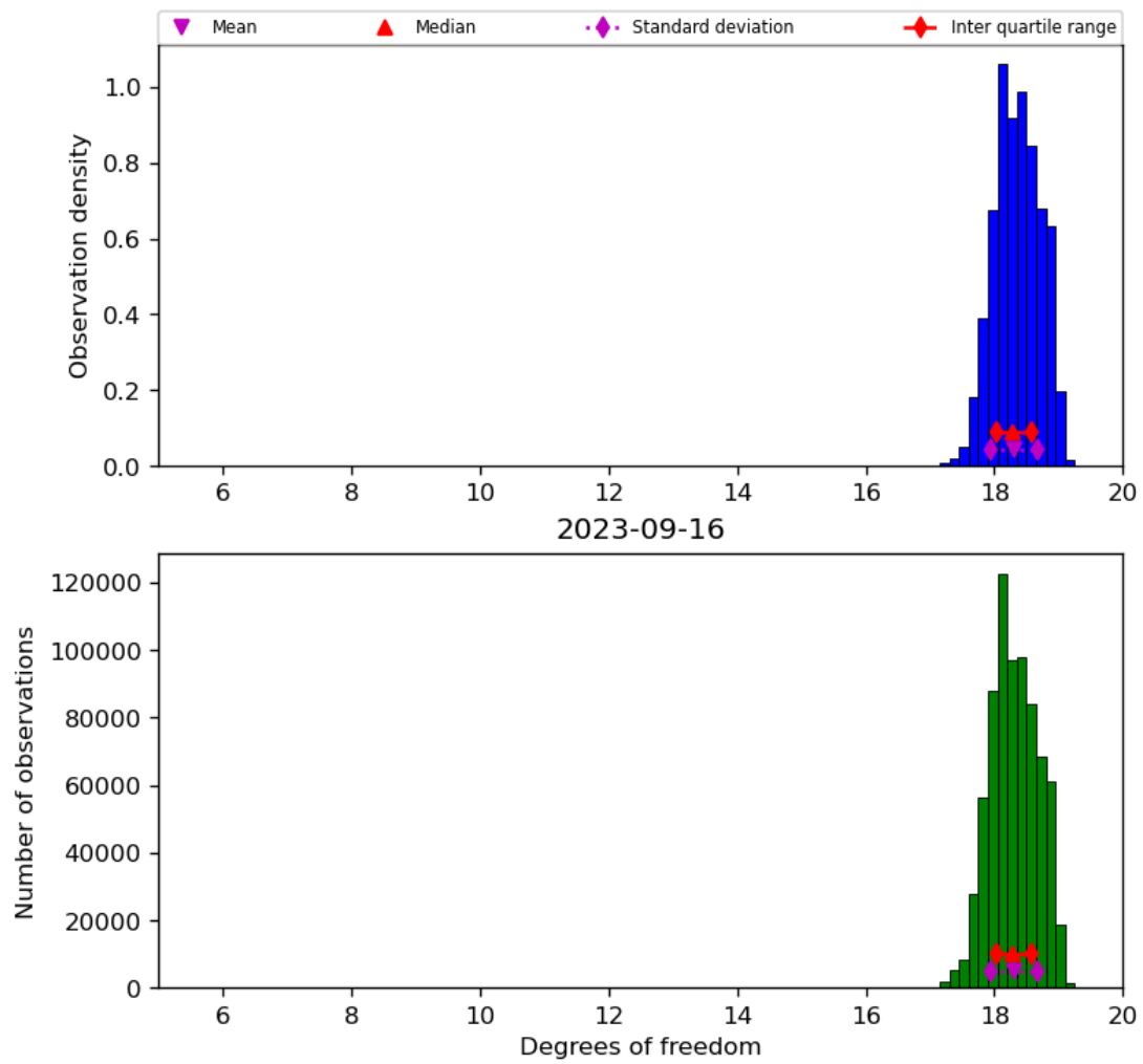
Figure 30: Histogram of “Degrees of freedom” for 2023-09-15 to 2023-09-17
