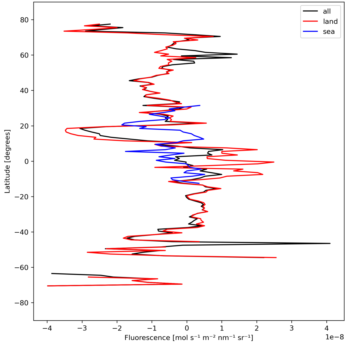
Figure 21: Zonal average of “Fluorescence” for 2023-09-15 to 2023-09-17.
