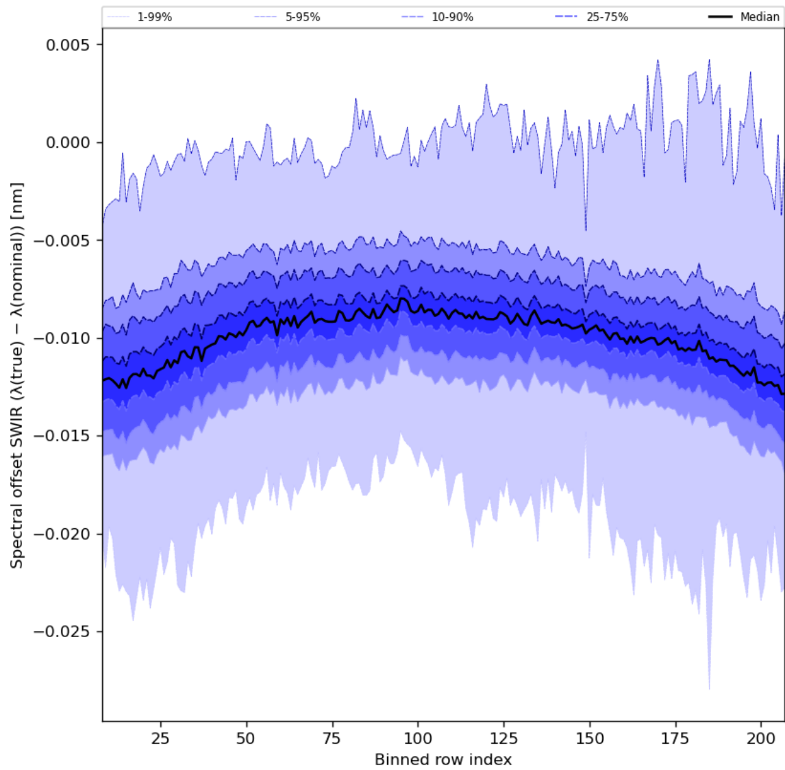
Figure 38: Along track statistics of “Spectral offset SWIR ( \lambda(\text{true}) - \lambda(\text{nominal}) )” for 2023-09-15 to 2023-09-17
