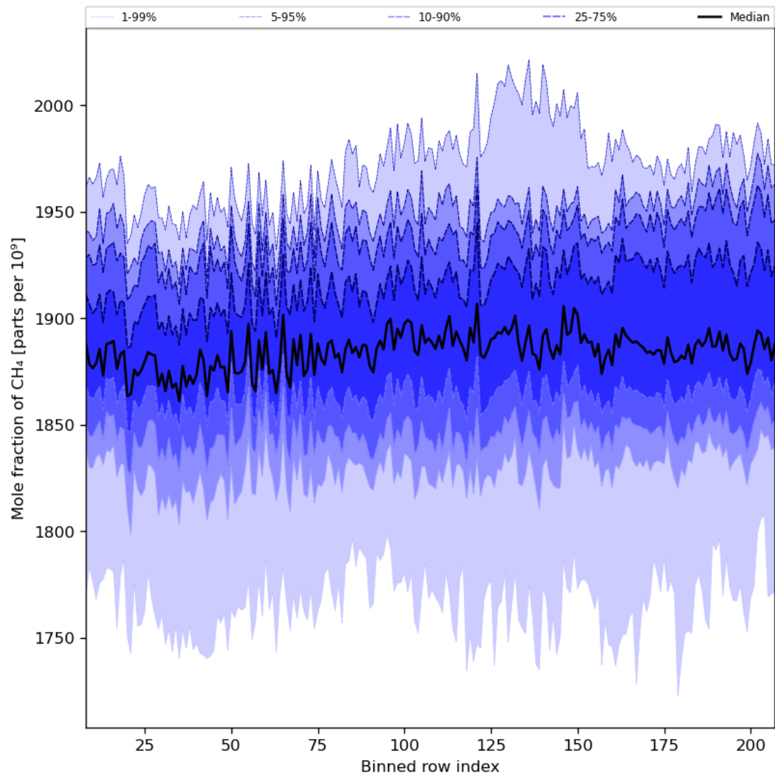
Figure 34: Along track statistics of “Mole fraction of CH 4 ” for 2023-09-15 to 2023-09-17
