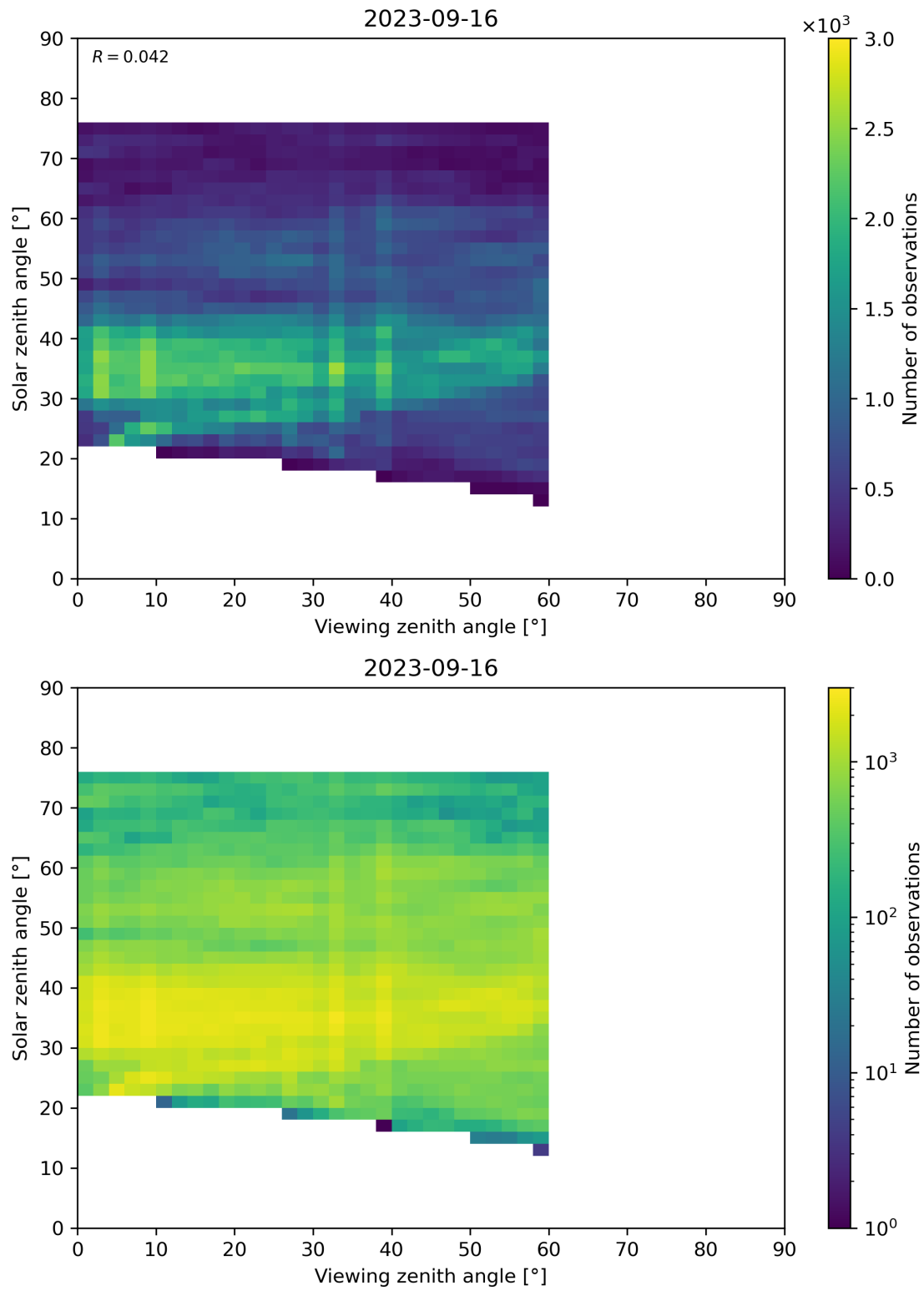
Figure 115: Scatter density plot of “Viewing zenith angle” against “Solar zenith angle” for 2023-09-15 to 2023-09-17.
