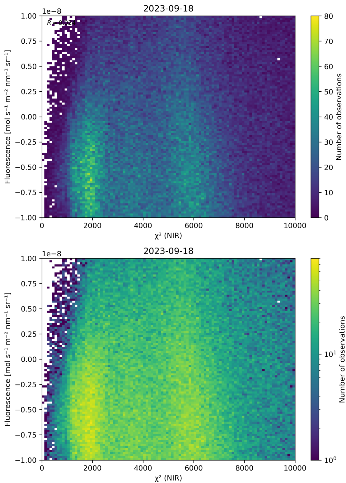
Figure 45: Scatter density plot of “ \chi^2 (NIR)” against “Fluorescence” for 2023-09-17 to 2023-09-19.
