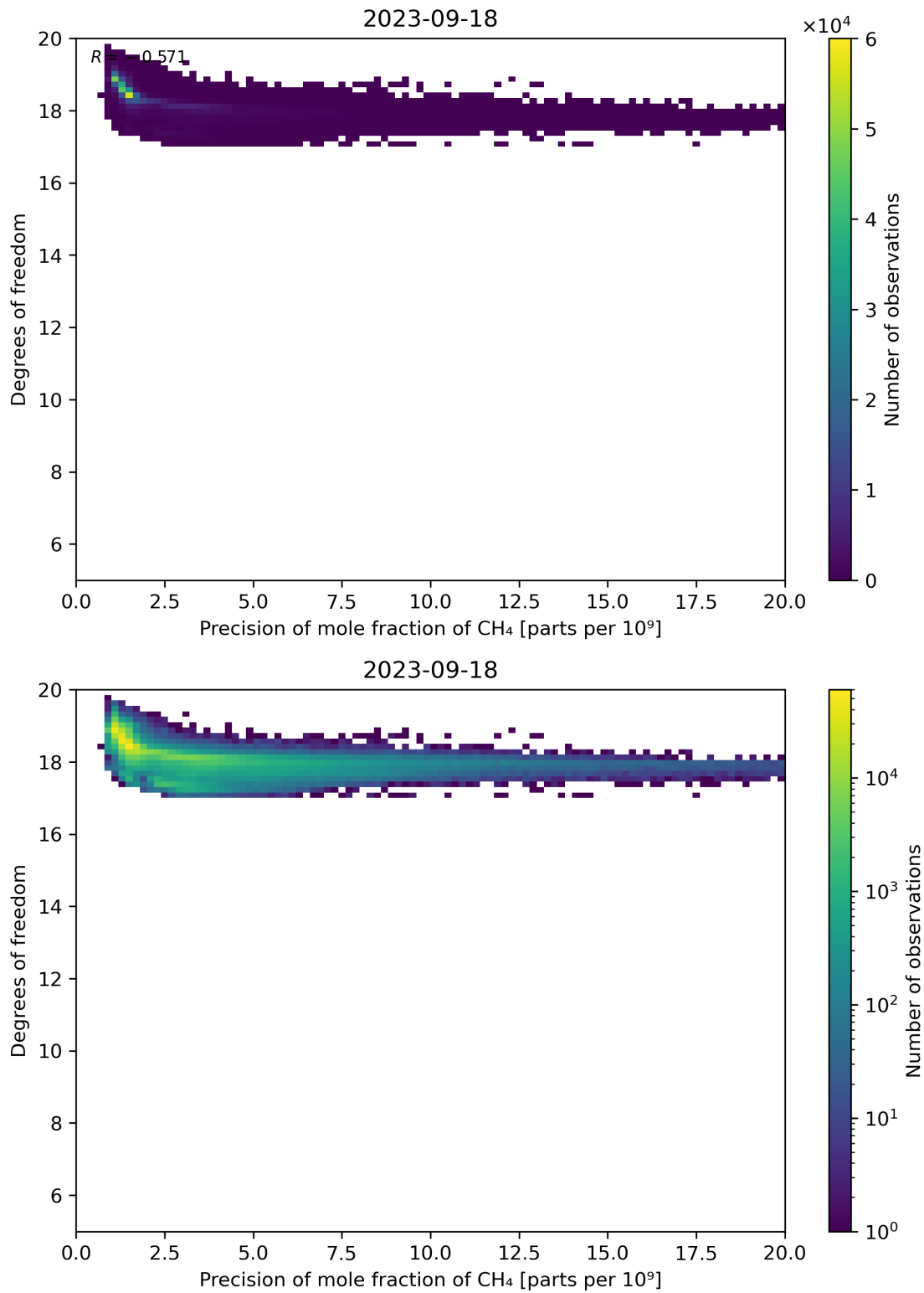
Figure 80: Scatter density plot of “Precision of mole fraction of CH 4 ” against “Degrees of freedom” for 2023-09-17 to 2023-09-19.
