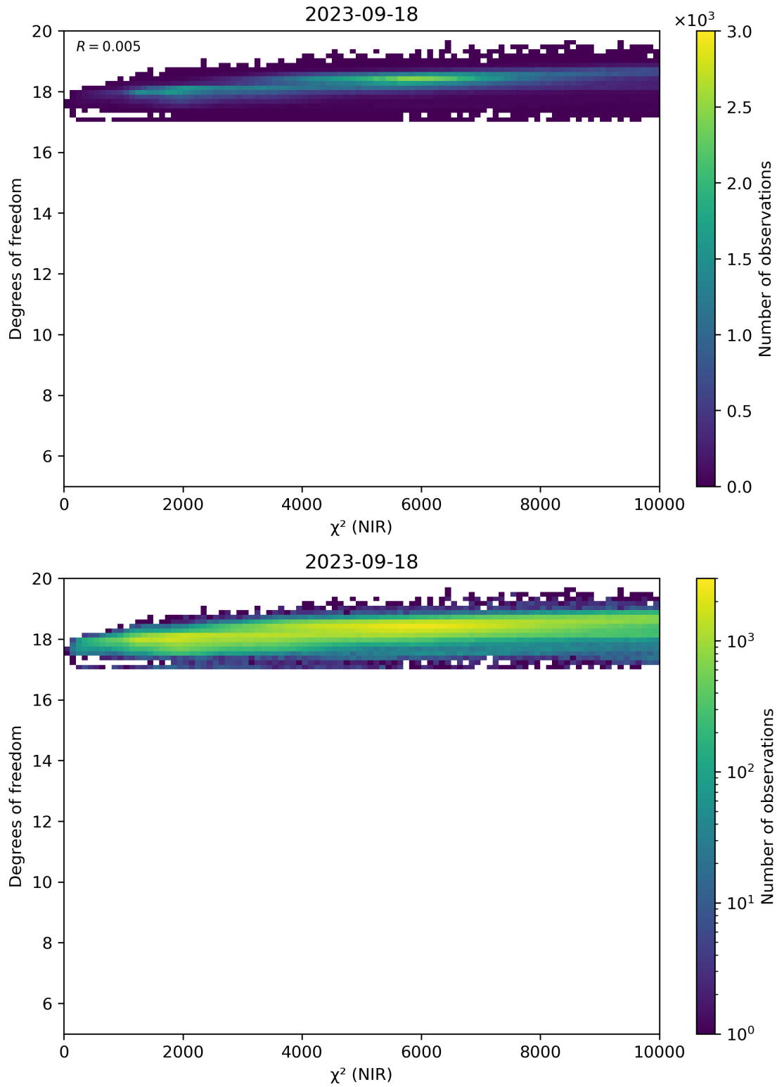
Figure 44: Scatter density plot of “ \chi^2 (NIR)” against “Degrees of freedom” for 2023-09-17 to 2023-09-19.
