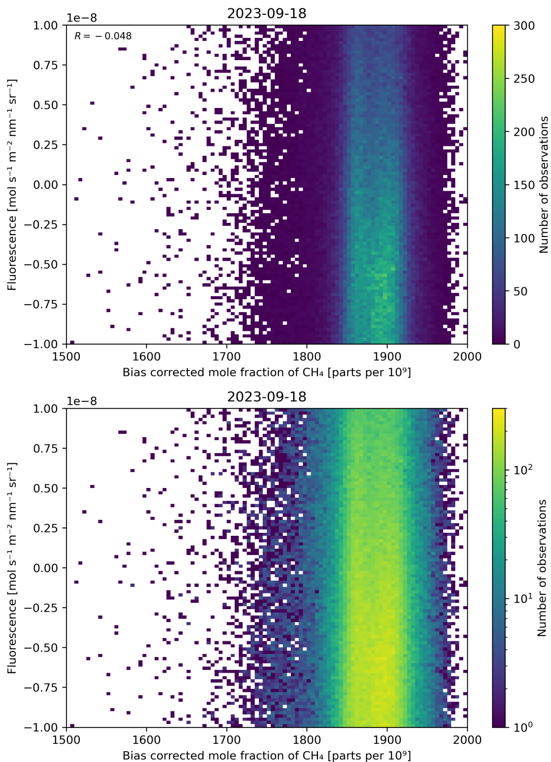
Figure 66: Scatter density plot of “Bias corrected mole fraction of \text{CH}_4 ” against “Fluorescence” for 2023-09-17 to 2023-09-19.
