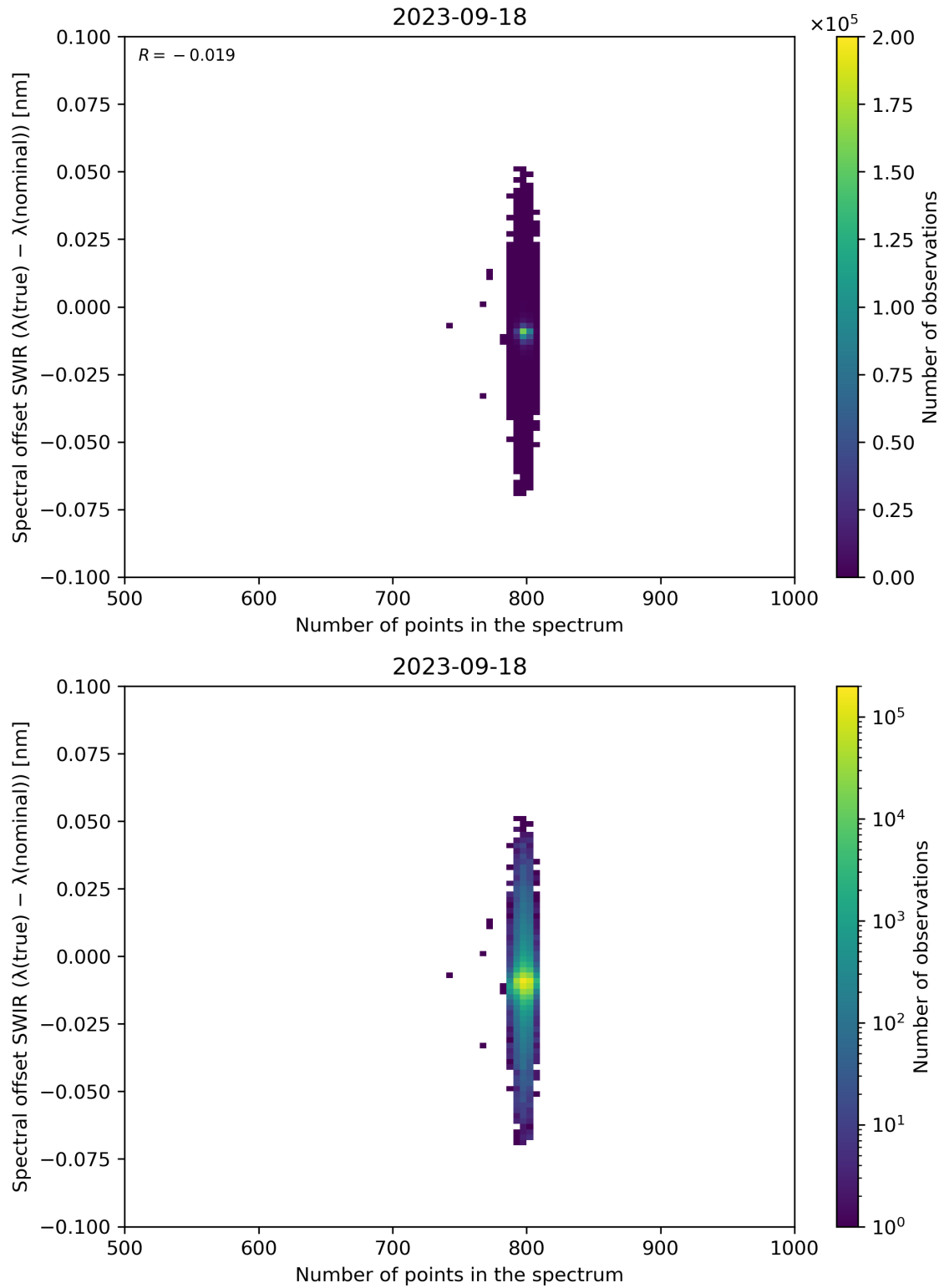
Figure 93: Scatter density plot of “Number of points in the spectrum” against “Spectral offset SWIR ( \lambda(\text{true}) - \lambda(\text{nominal}) )” for 2023-09-17 to 2023-09-19.
