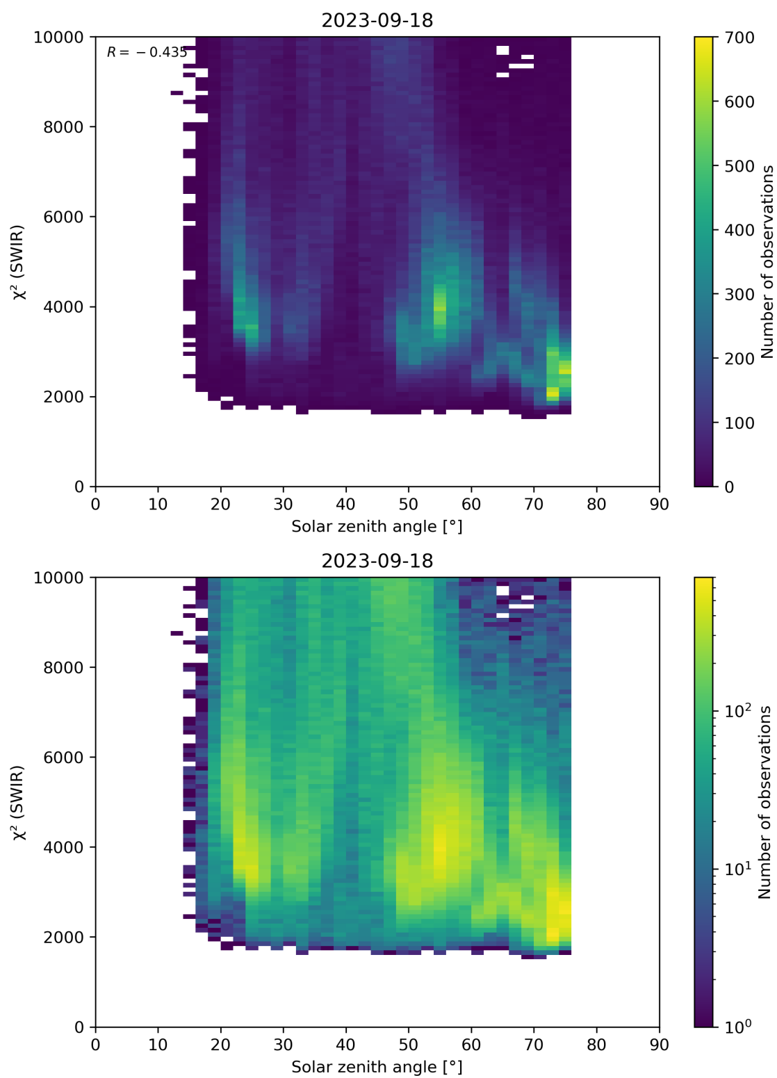
Figure 95: Scatter density plot of “Solar zenith angle” against “ \chi^2 (SWIR)” for 2023-09-17 to 2023-09-19.
