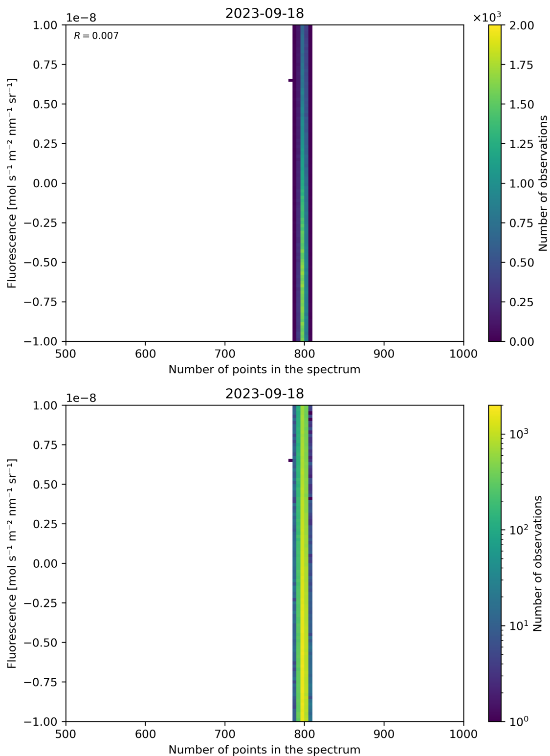
Figure 91: Scatter density plot of “Number of points in the spectrum” against “Fluorescence” for 2023-09-17 to 2023-09-19.
