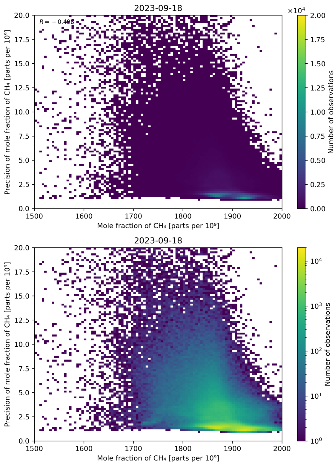
Figure 75: Scatter density plot of “Mole fraction of CH 4 ” against “Precision of mole fraction of CH 4 ” for 2023-09-17 to 2023-09-19.
