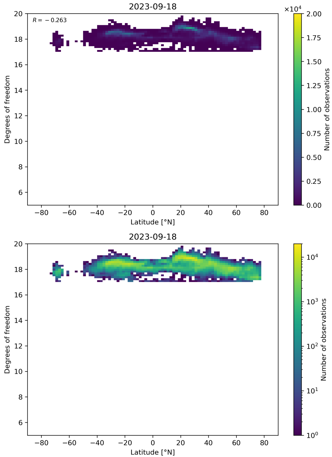
Figure 55: Scatter density plot of “Latitude” against “Degrees of freedom” for 2023-09-17 to 2023-09-19.
