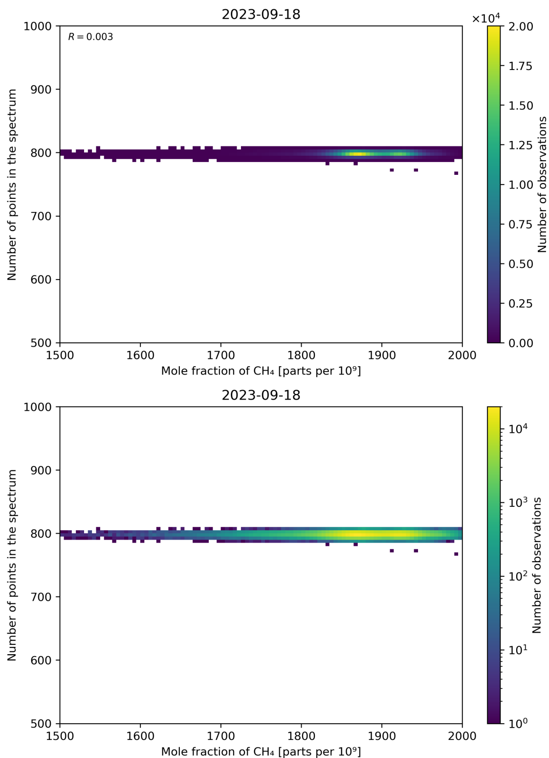
Figure 77: Scatter density plot of “Mole fraction of CH 4 ” against “Number of points in the spectrum” for 2023-09-17 to 2023-09-19.
