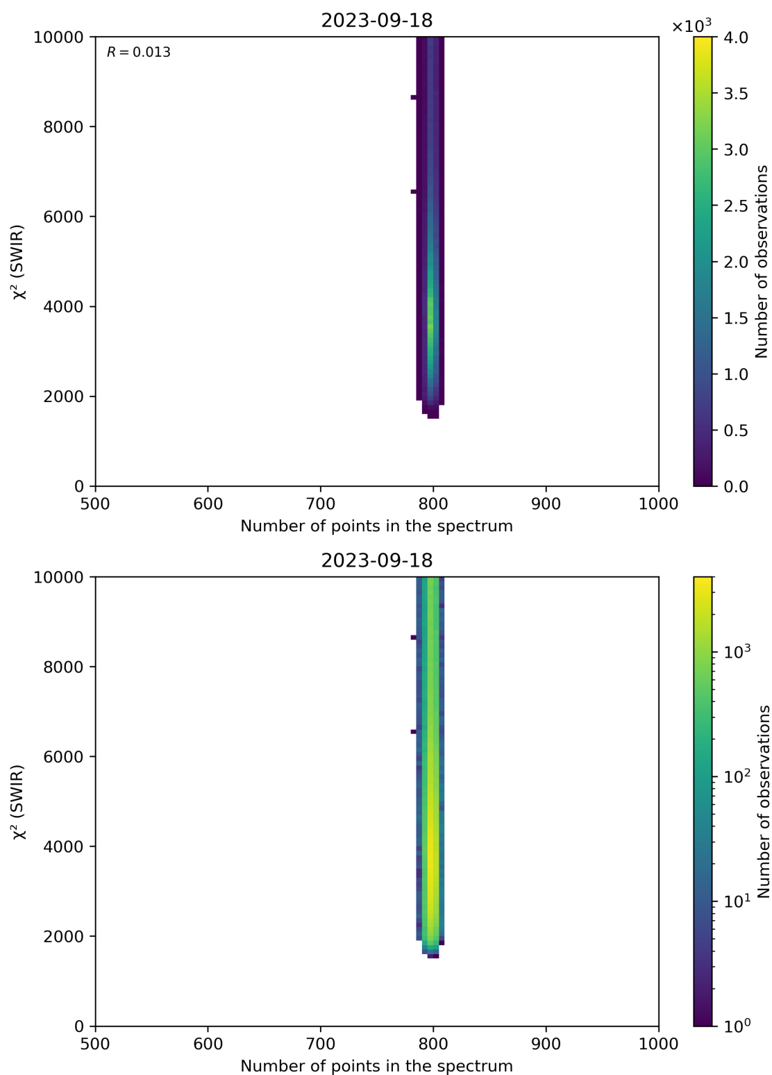
Figure 89: Scatter density plot of “Number of points in the spectrum” against “ \chi^2 (SWIR)” for 2023-09-17 to 2023-09-19.
