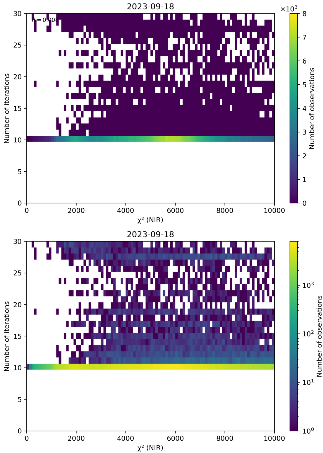
Figure 46: Scatter density plot of “ \chi^2 (NIR)” against “Number of iterations” for 2023-09-17 to 2023-09-19.
