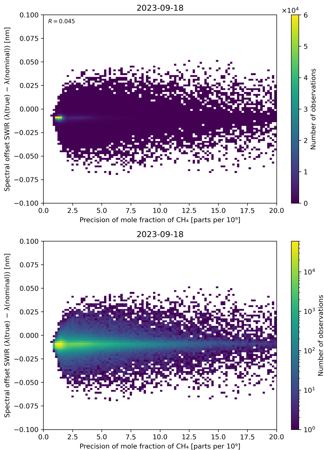
Figure 85: Scatter density plot of “Precision of mole fraction of CH 4 ” against “Spectral offset SWIR ( \lambda(\text{true}) - \lambda(\text{nominal}) )” for 2023-09-17 to 2023-09-19.
