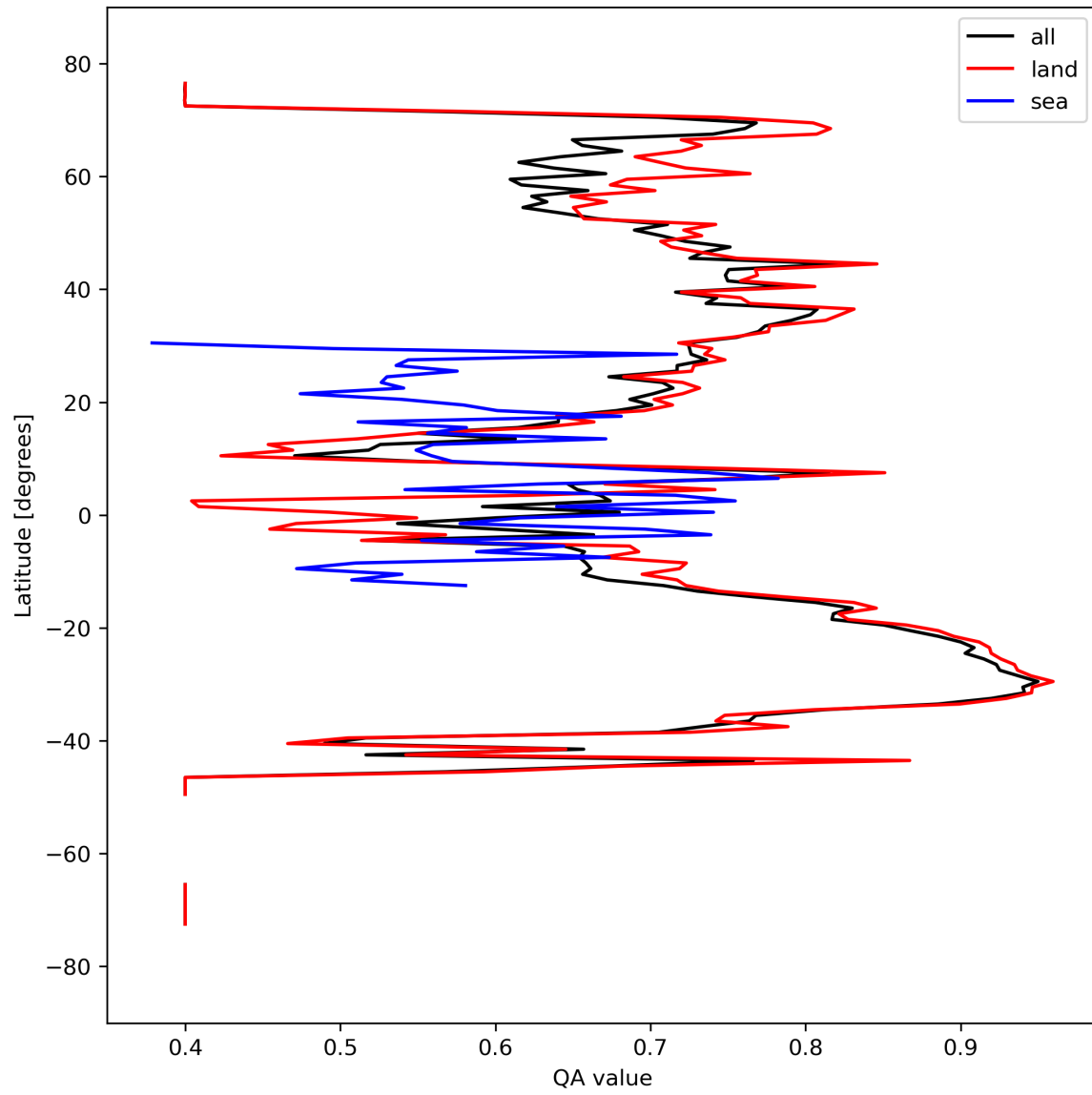
Figure 11: Zonal average of “QA value” for 2023-09-17 to 2023-09-19.
