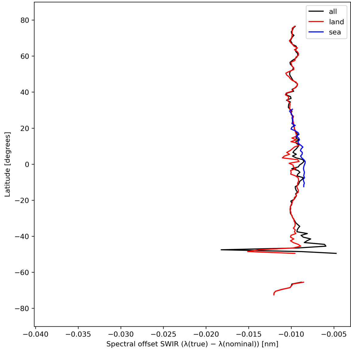
Figure 16: Zonal average of “Spectral offset SWIR ( \lambda(\text{true}) - \lambda(\text{nominal}) )” for 2023-09-17 to 2023-09-19.
