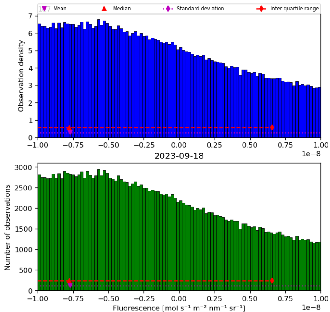
Figure 32: Histogram of “Fluorescence” for 2023-09-17 to 2023-09-19
