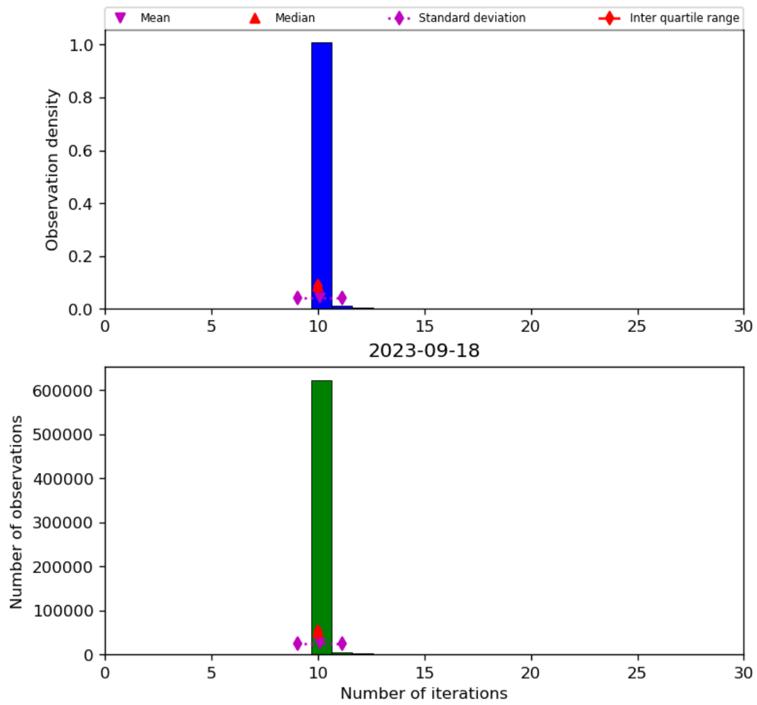
Figure 31: Histogram of “Number of iterations” for 2023-09-17 to 2023-09-19
