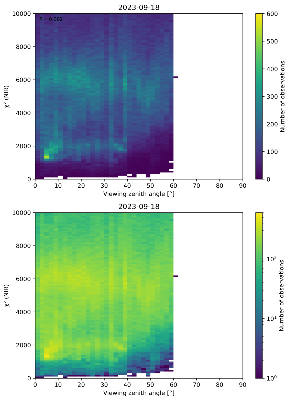
Figure 105: Scatter density plot of “Viewing zenith angle” against “ \chi^2 (NIR)” for 2023-09-17 to 2023-09-19.
