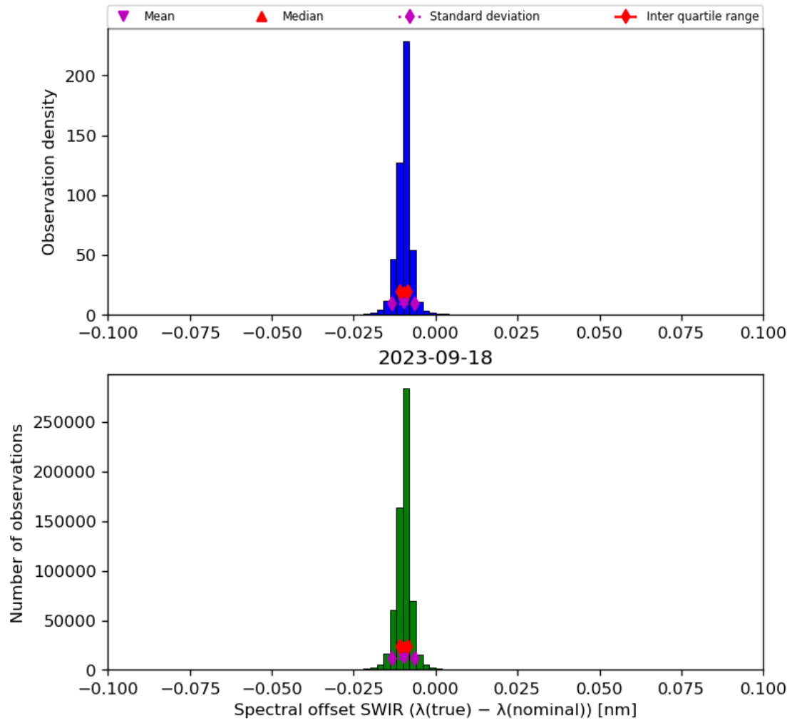
Figure 27: Histogram of “Spectral offset SWIR ( \lambda(\text{true}) - \lambda(\text{nominal}) )” for 2023-09-17 to 2023-09-19
