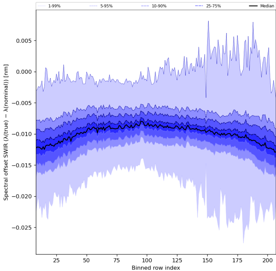
Figure 38: Along track statistics of “Spectral offset SWIR ( \lambda(\text{true}) - \lambda(\text{nominal}) )” for 2023-09-17 to 2023-09-19
