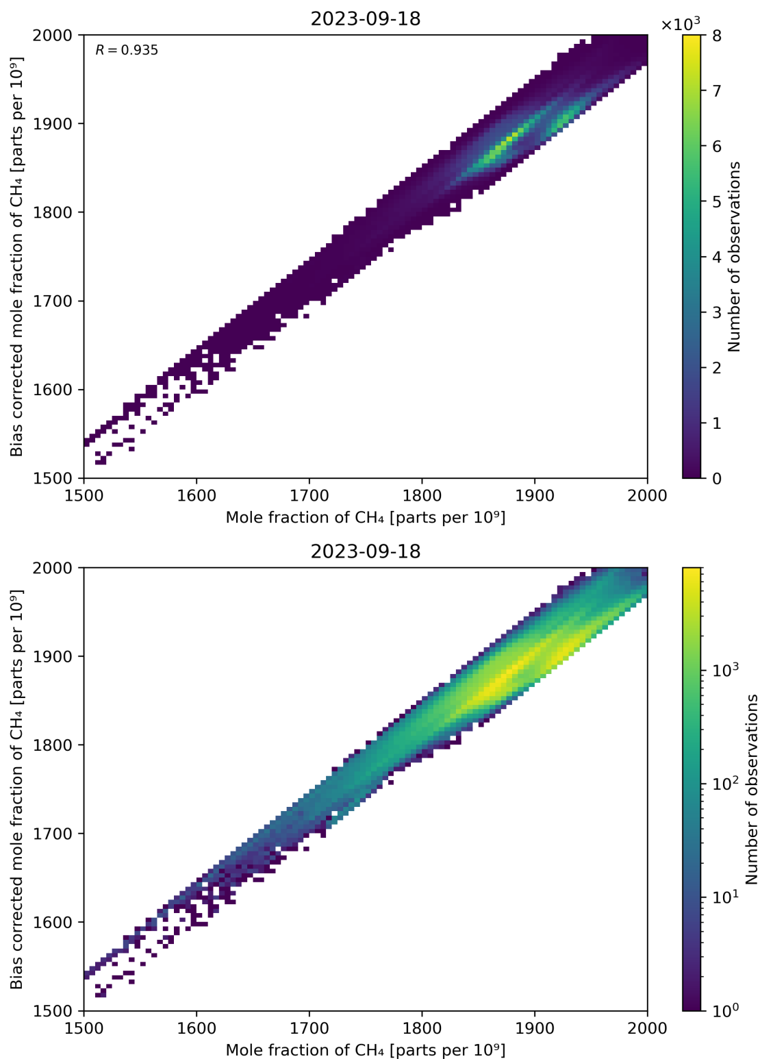
Figure 74: Scatter density plot of “Mole fraction of CH 4 ” against “Bias corrected mole fraction of CH 4 ” for 2023-09-17 to 2023-09-19.
