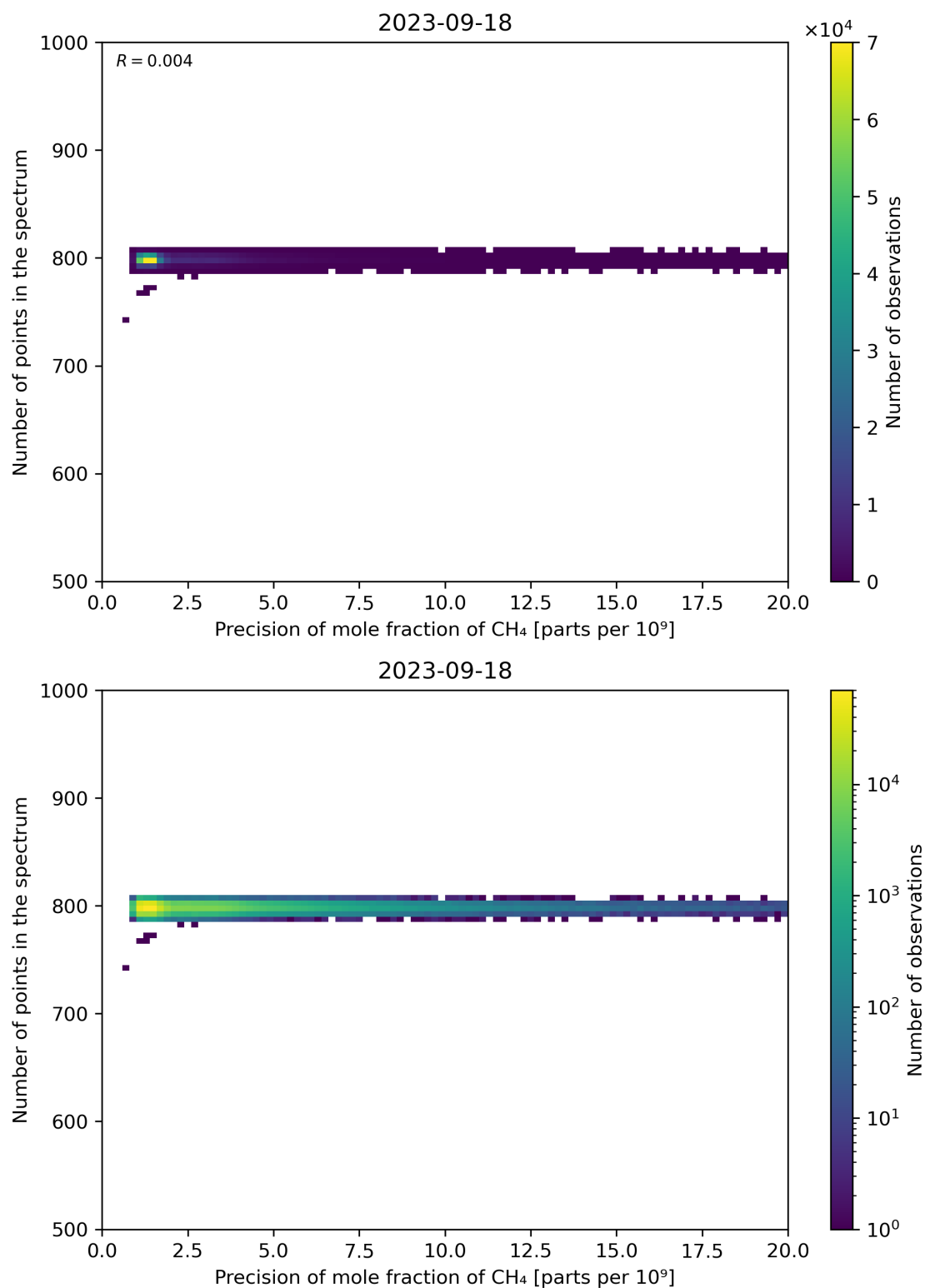
Figure 84: Scatter density plot of “Precision of mole fraction of CH 4 ” against “Number of points in the spectrum” for 2023-09-17 to 2023-09-19.
