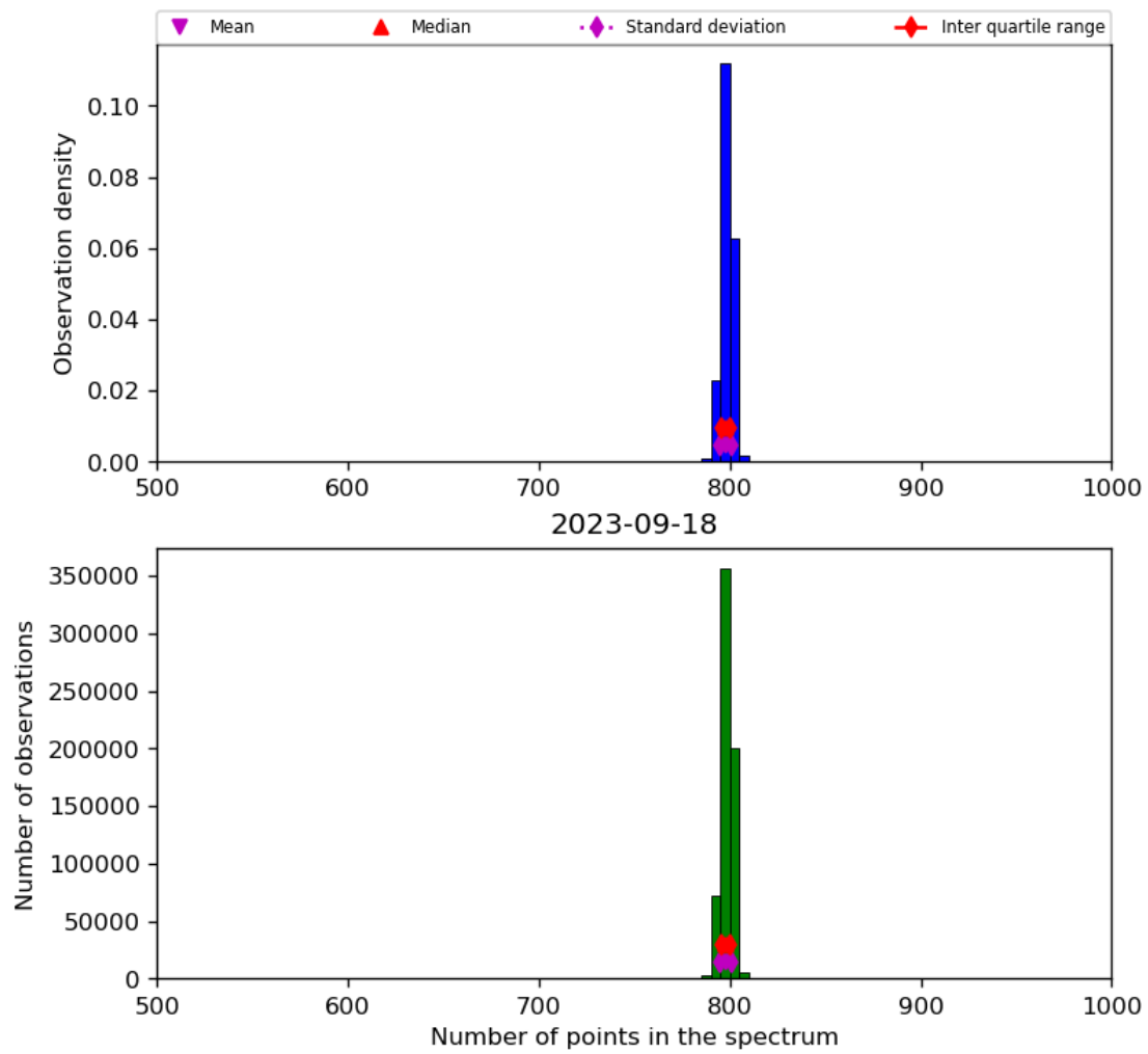
Figure 26: Histogram of “Number of points in the spectrum” for 2023-09-17 to 2023-09-19
