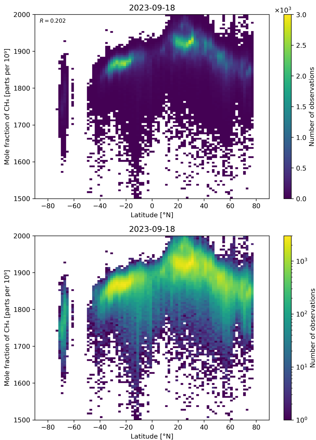
Figure 57: Scatter density plot of “Latitude” against “Mole fraction of \text{CH}_4 ” for 2023-09-17 to 2023-09-19.
