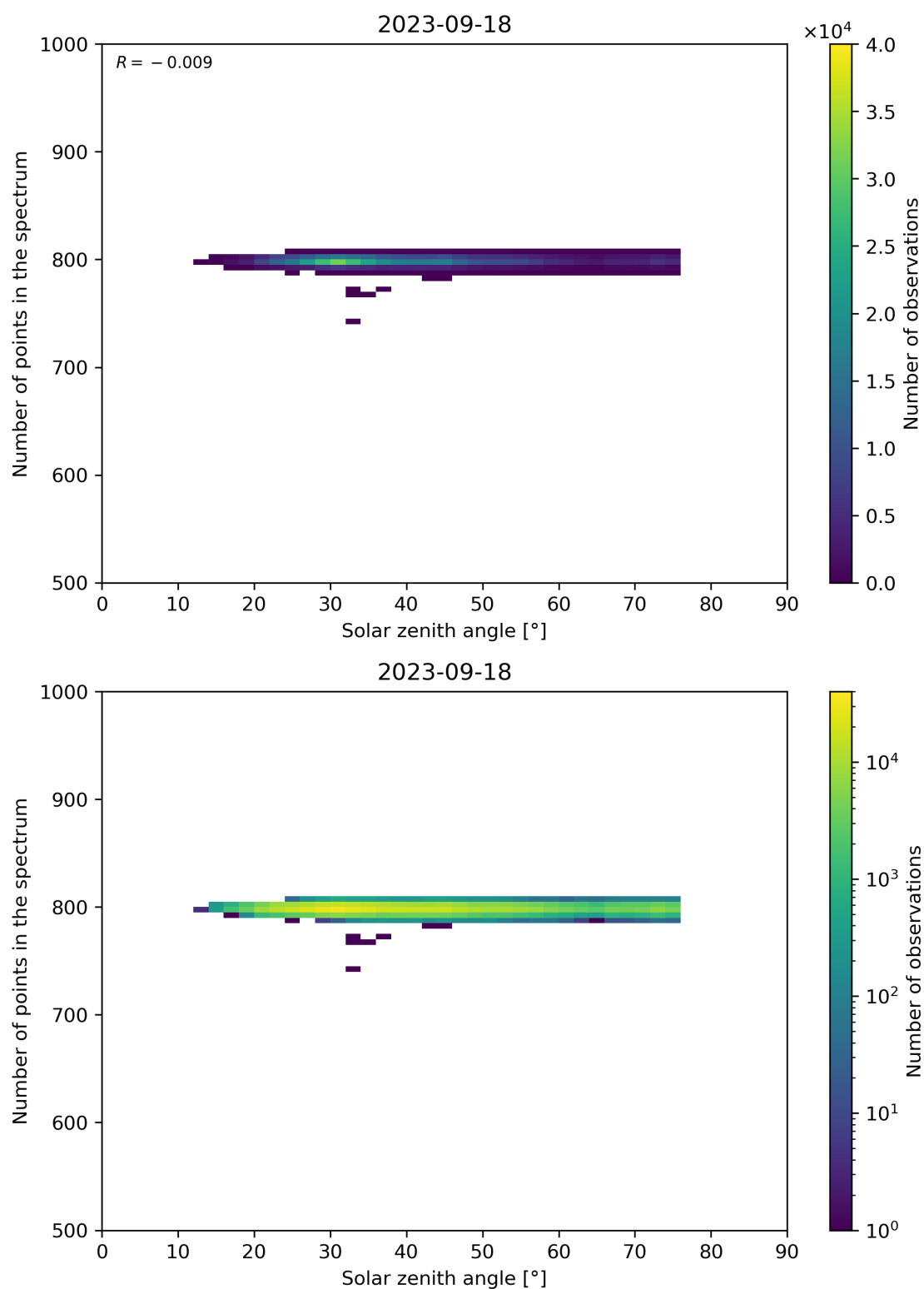
Figure 103: Scatter density plot of “Solar zenith angle” against “Number of points in the spectrum” for 2023-09-17 to 2023-09-19.
