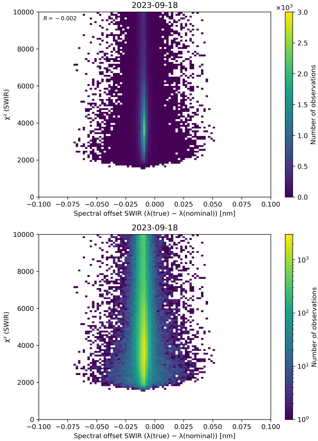
Figure 118: Scatter density plot of “Spectral offset SWIR ( \lambda(\text{true}) - \lambda(\text{nominal}) )” against “ \chi^2 (SWIR)” for 2023-09-17 to 2023-09-19.
