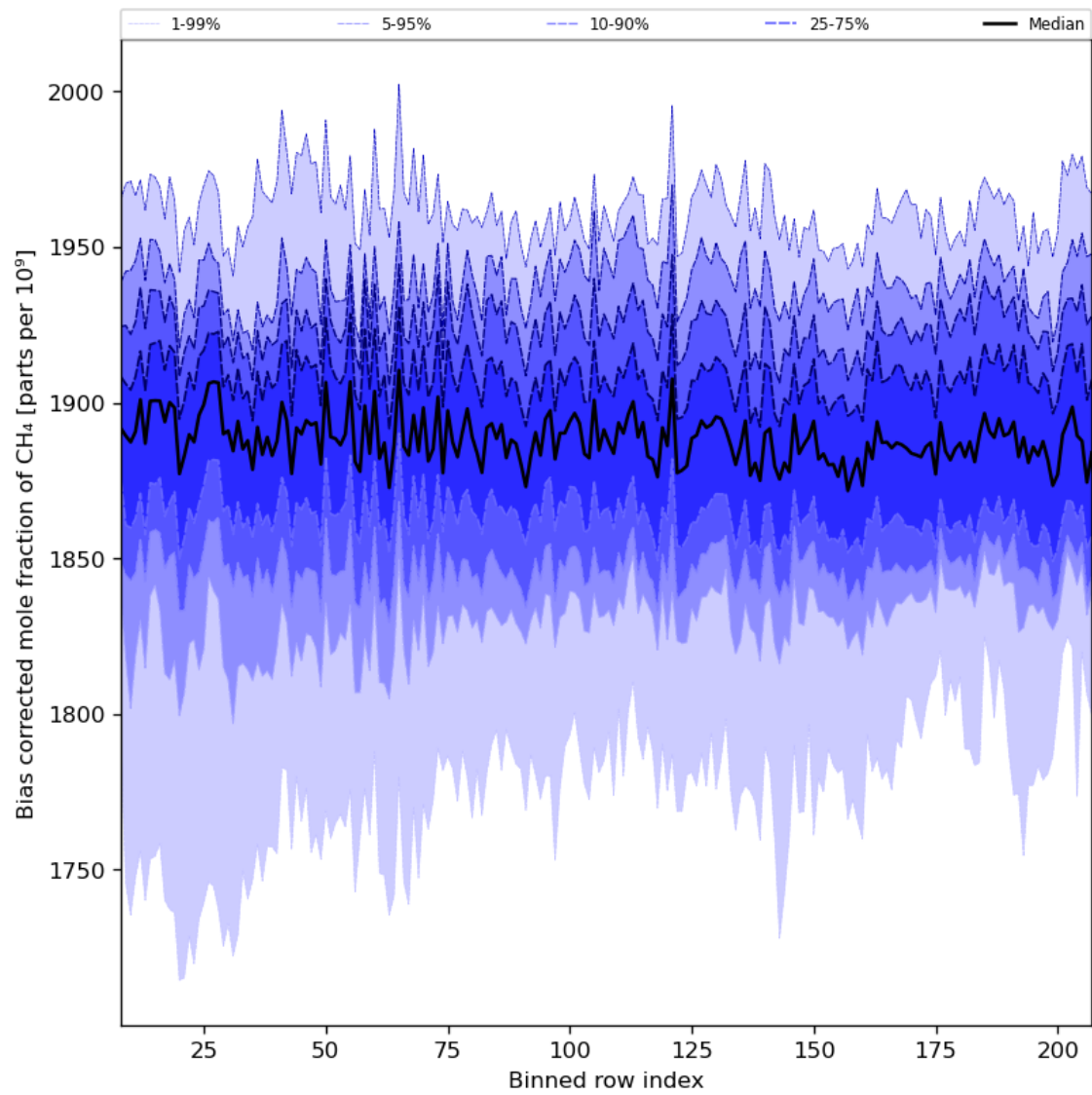
Figure 36: Along track statistics of “Bias corrected mole fraction of CH 4 ” for 2023-09-17 to 2023-09-19
