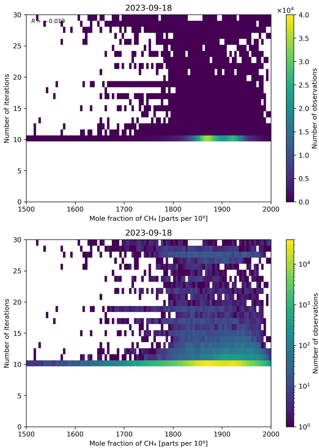
Figure 76: Scatter density plot of “Mole fraction of CH 4 ” against “Number of iterations” for 2023-09-17 to 2023-09-19.
