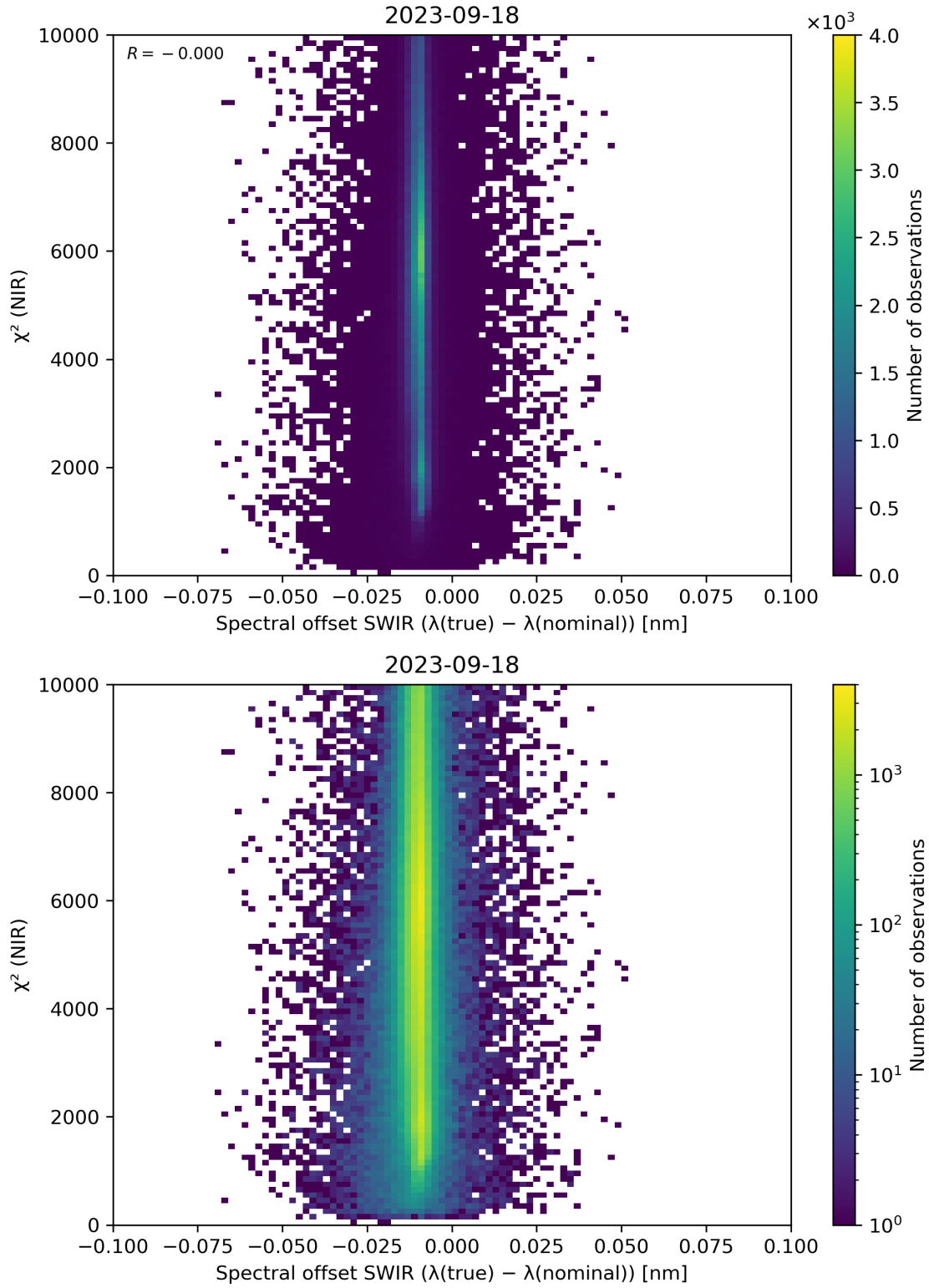
Figure 117: Scatter density plot of “Spectral offset SWIR ( \lambda(\text{true}) - \lambda(\text{nominal}) )” against “ \chi^2 (NIR)” for 2023-09-17 to 2023-09-19.
