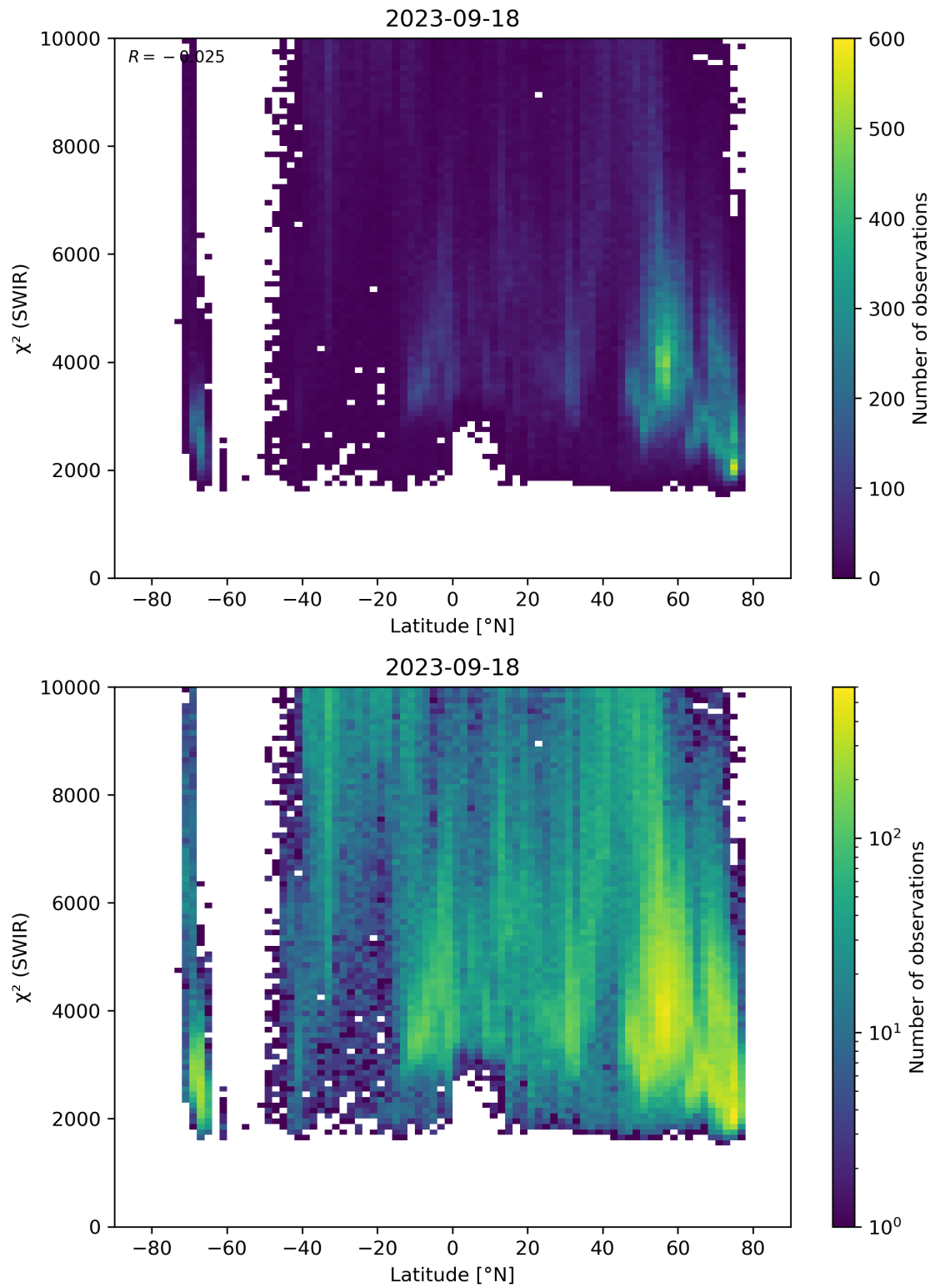
Figure 54: Scatter density plot of “Latitude” against “ \chi^2 (SWIR)” for 2023-09-17 to 2023-09-19.
