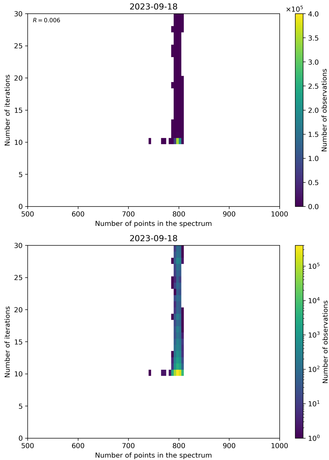
Figure 92: Scatter density plot of “Number of points in the spectrum” against “Number of iterations” for 2023-09-17 to 2023-09-19.
