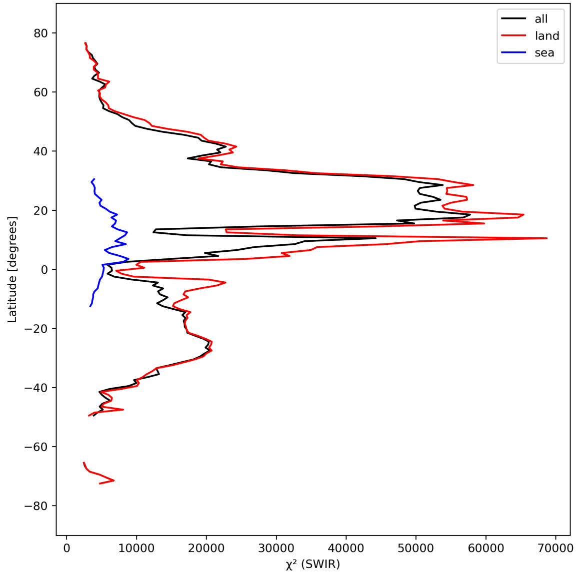
Figure 17: Zonal average of “ \chi^2 (SWIR)” for 2023-09-17 to 2023-09-19.
