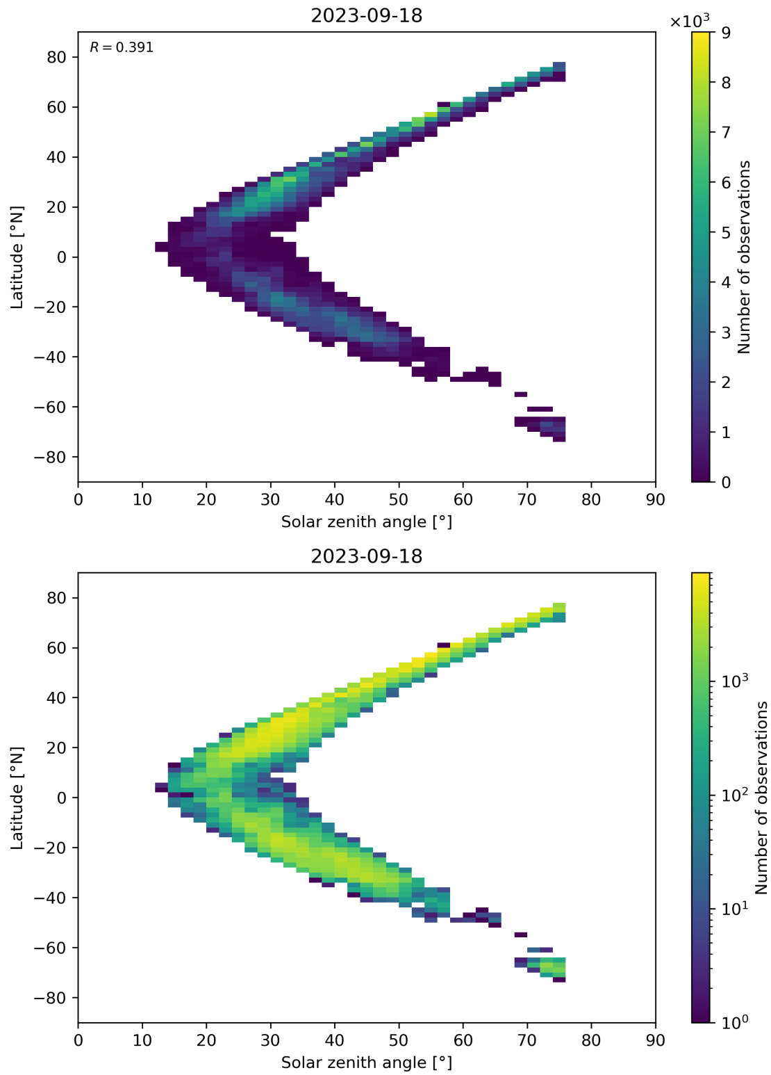
Figure 98: Scatter density plot of “Solar zenith angle” against “Latitude” for 2023-09-17 to 2023-09-19.
