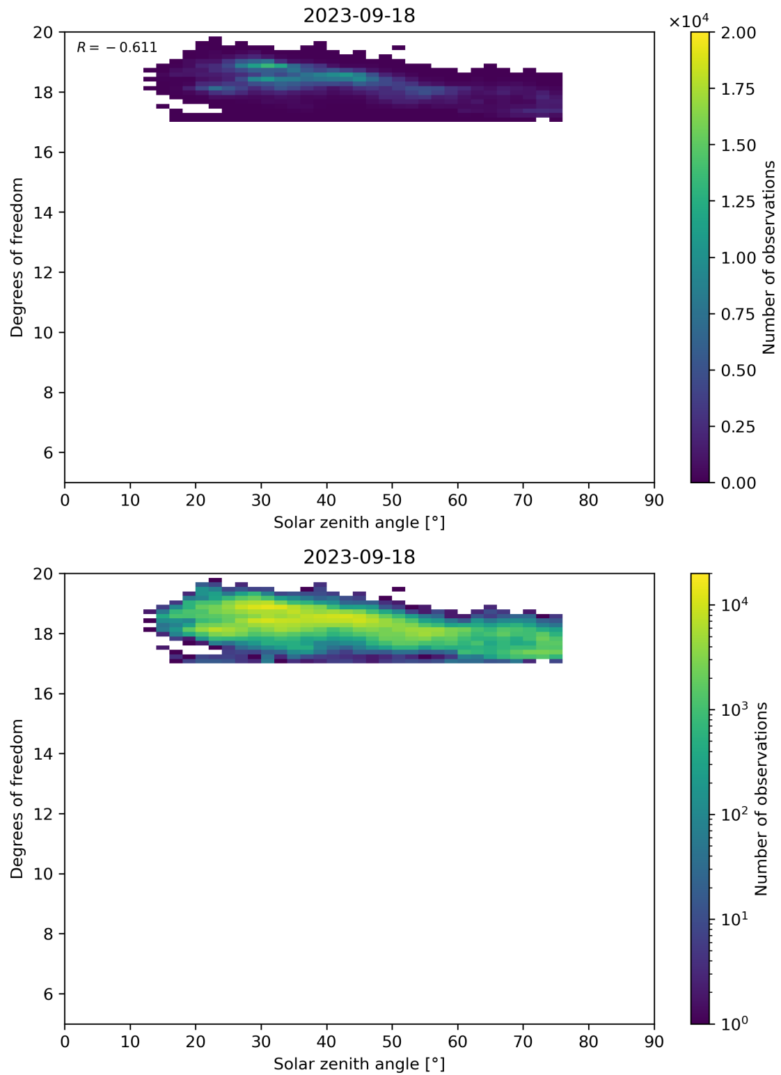
Figure 96: Scatter density plot of “Solar zenith angle” against “Degrees of freedom” for 2023-09-17 to 2023-09-19.
