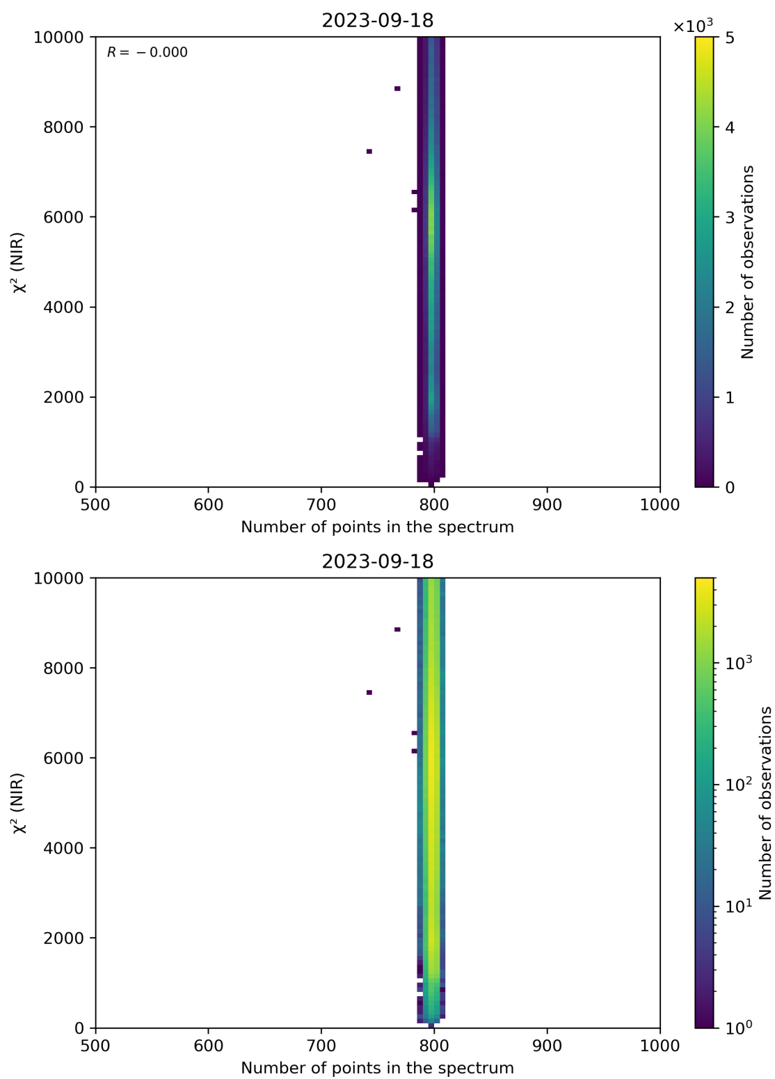
Figure 88: Scatter density plot of “Number of points in the spectrum” against “ \chi^2 (NIR)” for 2023-09-17 to 2023-09-19.
