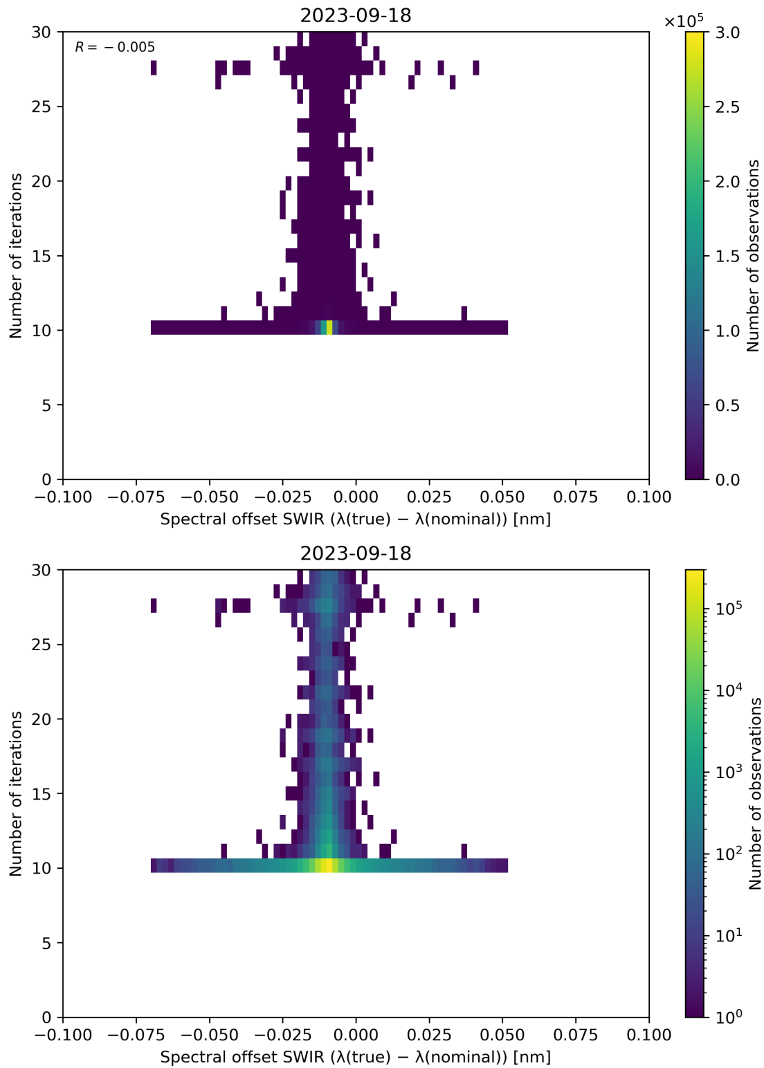
Figure 121: Scatter density plot of “Spectral offset SWIR ( \lambda(\text{true}) - \lambda(\text{nominal}) )” against “Number of iterations” for 2023-09-17 to 2023-09-19.
