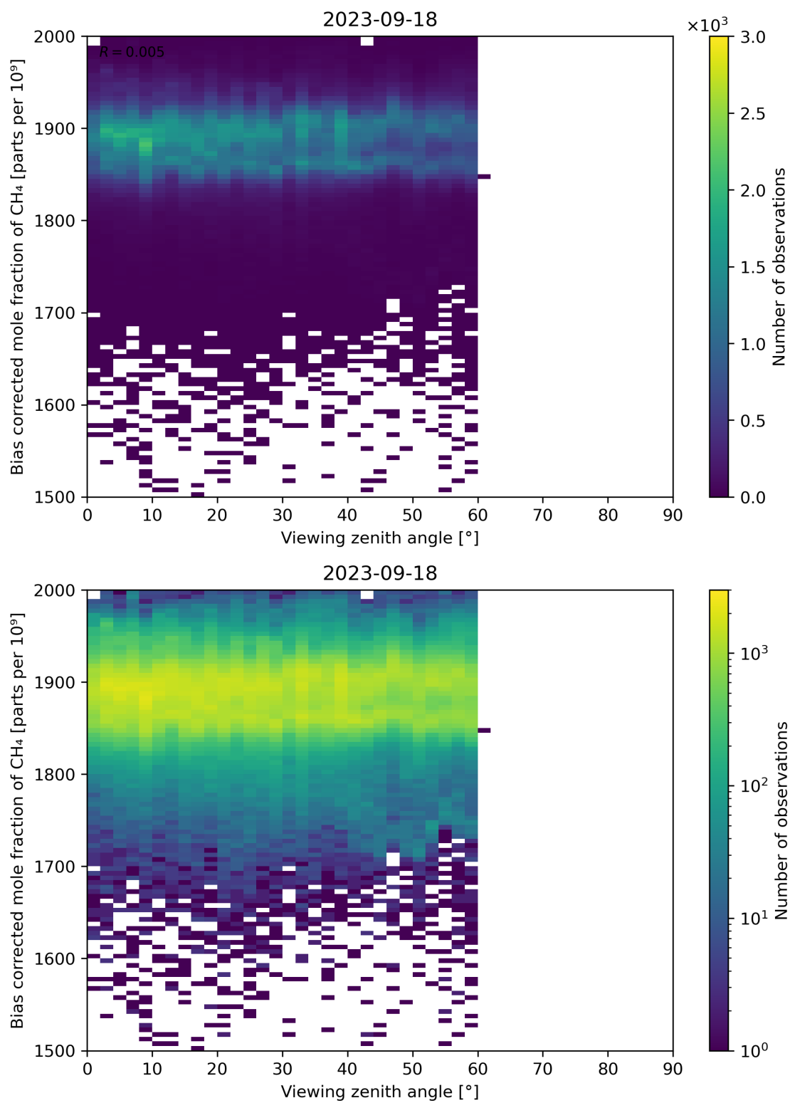
Figure 111: Scatter density plot of “Viewing zenith angle” against “Bias corrected mole fraction of CH 4 ” for 2023-09-17 to 2023-09-19.
