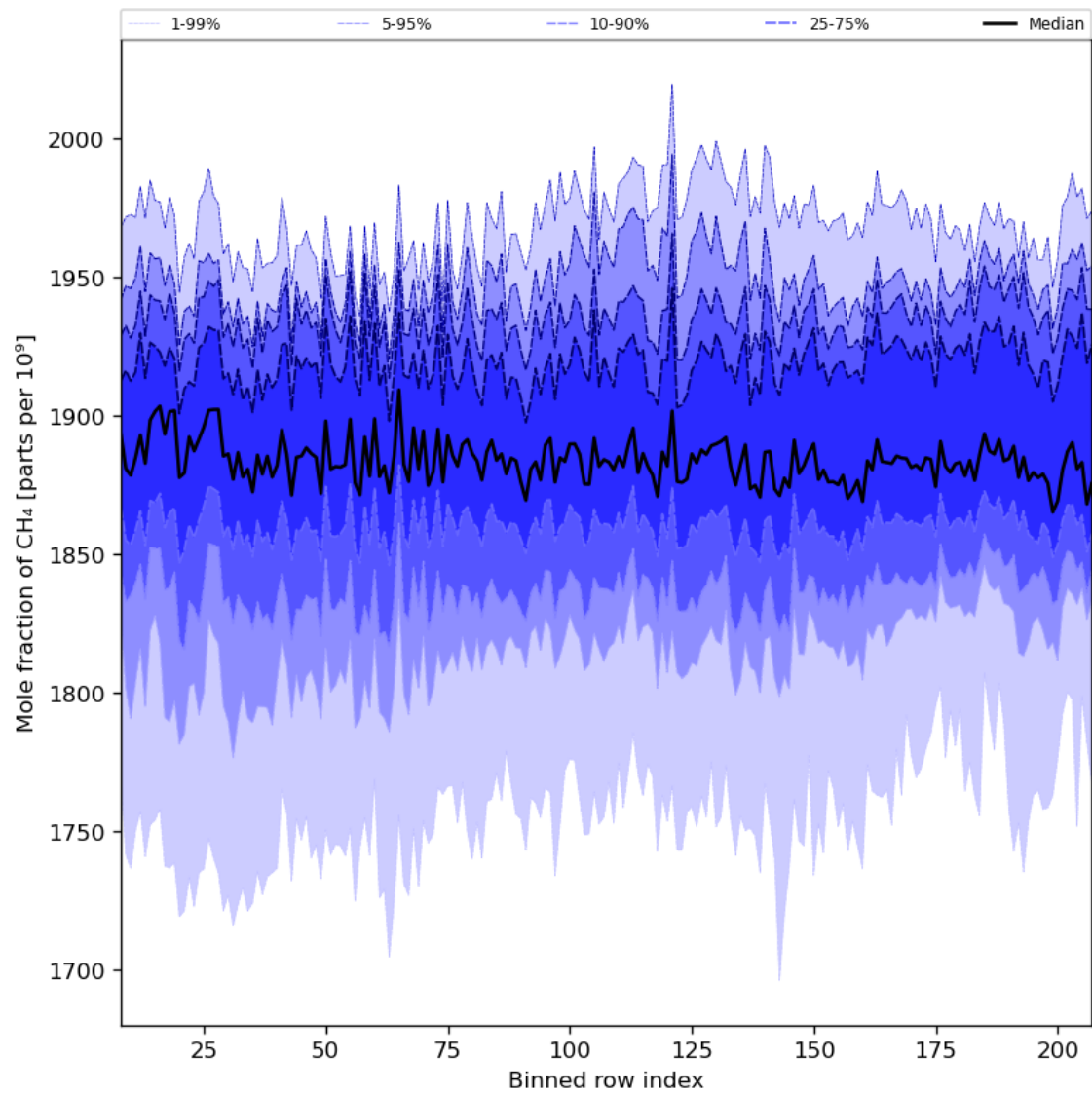
Figure 34: Along track statistics of “Mole fraction of CH 4 ” for 2023-09-17 to 2023-09-19
