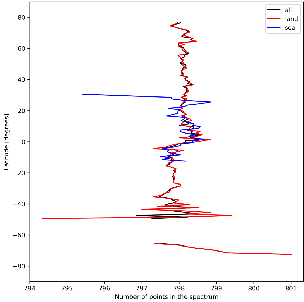
Figure 15: Zonal average of “Number of points in the spectrum” for 2023-09-17 to 2023-09-19.
