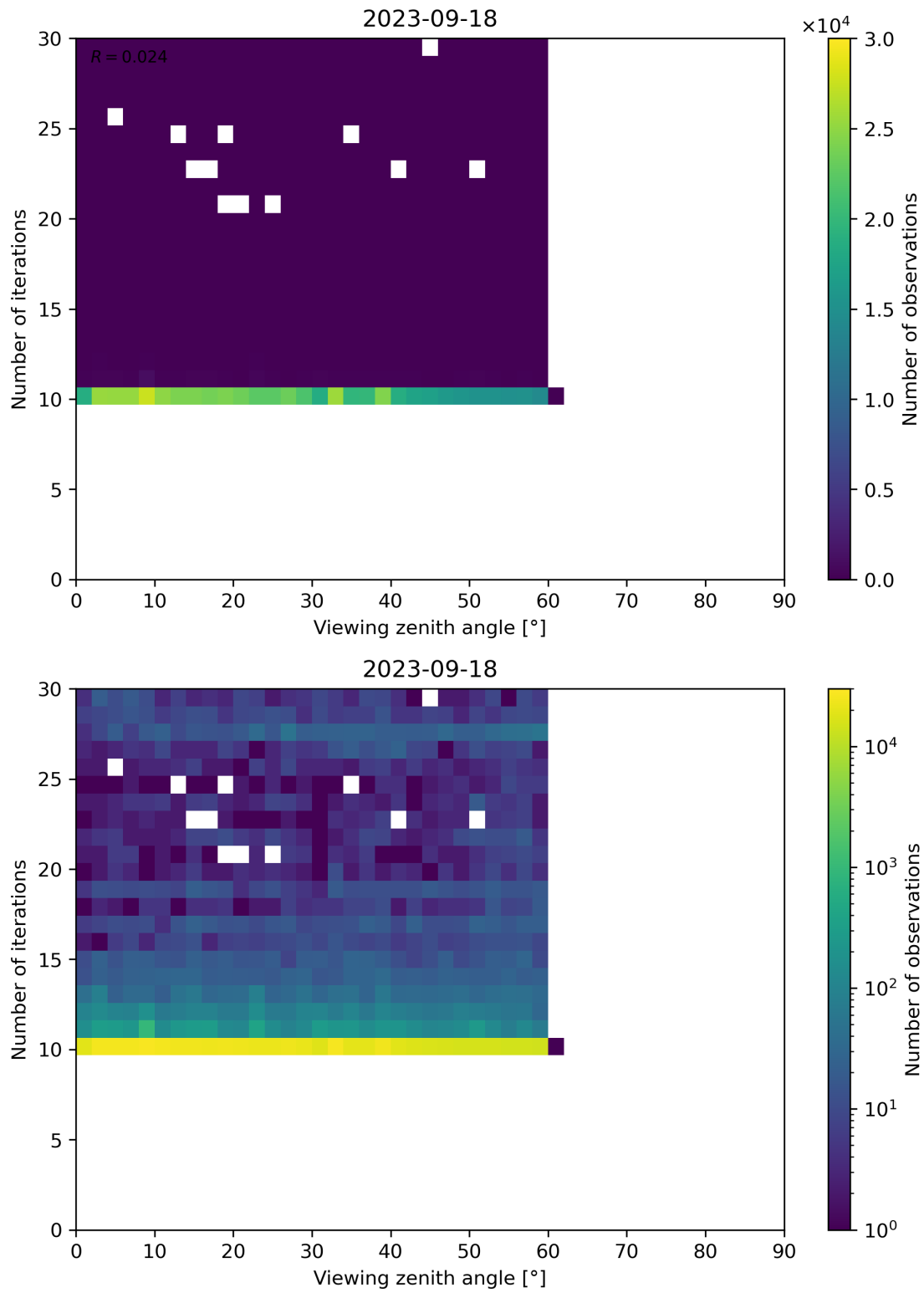
Figure 113: Scatter density plot of “Viewing zenith angle” against “Number of iterations” for 2023-09-17 to 2023-09-19.
