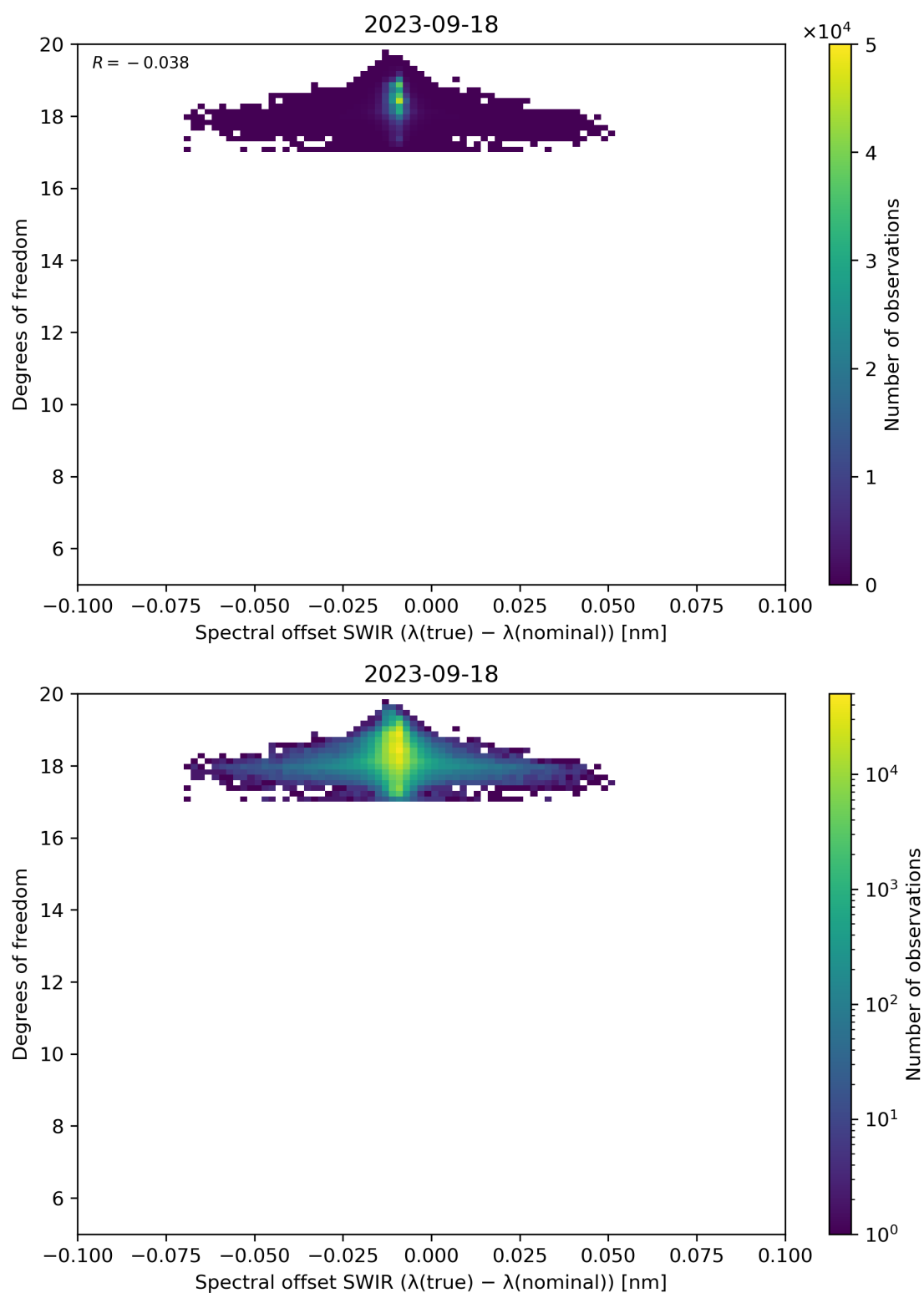
Figure 119: Scatter density plot of “Spectral offset SWIR ( \lambda(\text{true}) - \lambda(\text{nominal}) )” against “Degrees of freedom” for 2023-09-17 to 2023-09-19.
