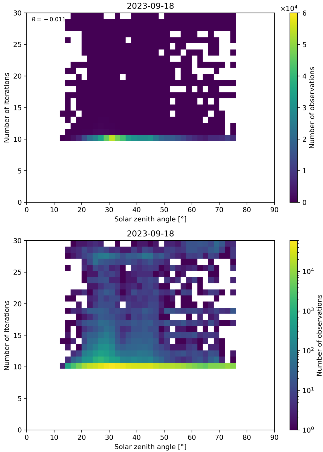
Figure 102: Scatter density plot of “Solar zenith angle” against “Number of iterations” for 2023-09-17 to 2023-09-19.
