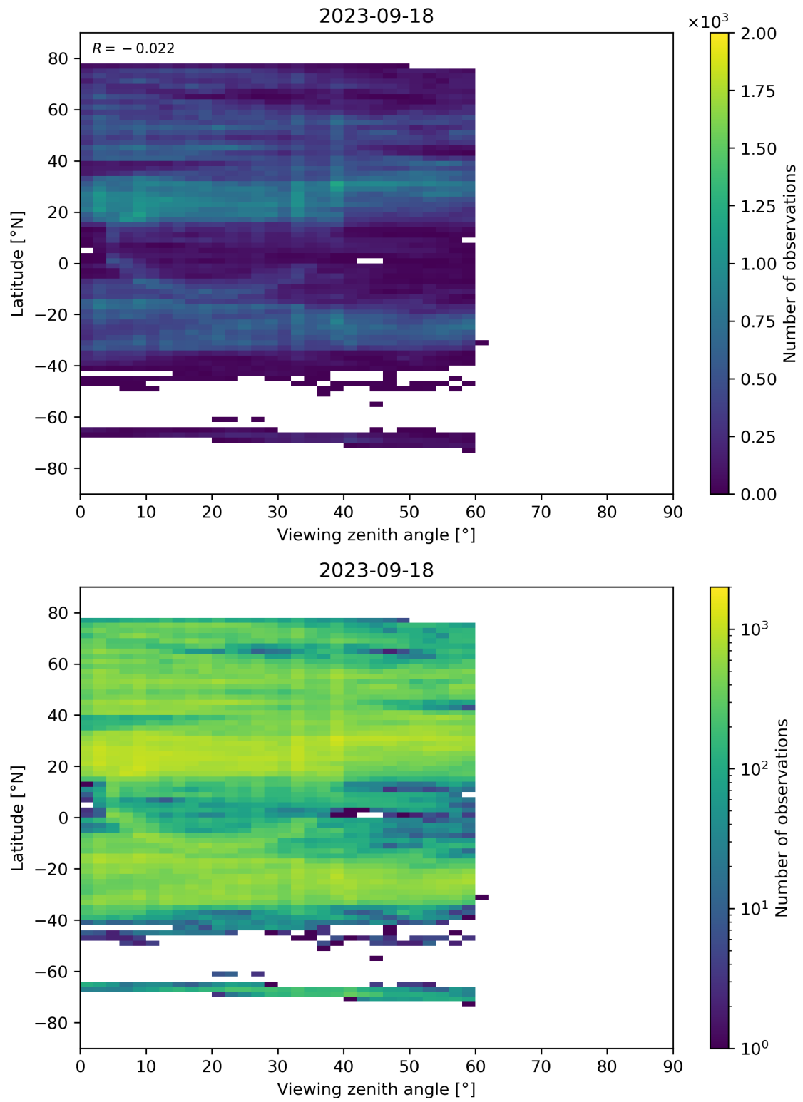
Figure 109: Scatter density plot of “Viewing zenith angle” against “Latitude” for 2023-09-17 to 2023-09-19.
