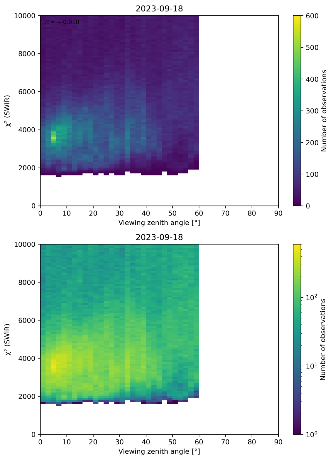
Figure 106: Scatter density plot of “Viewing zenith angle” against “ \chi^2 (SWIR)” for 2023-09-17 to 2023-09-19.
