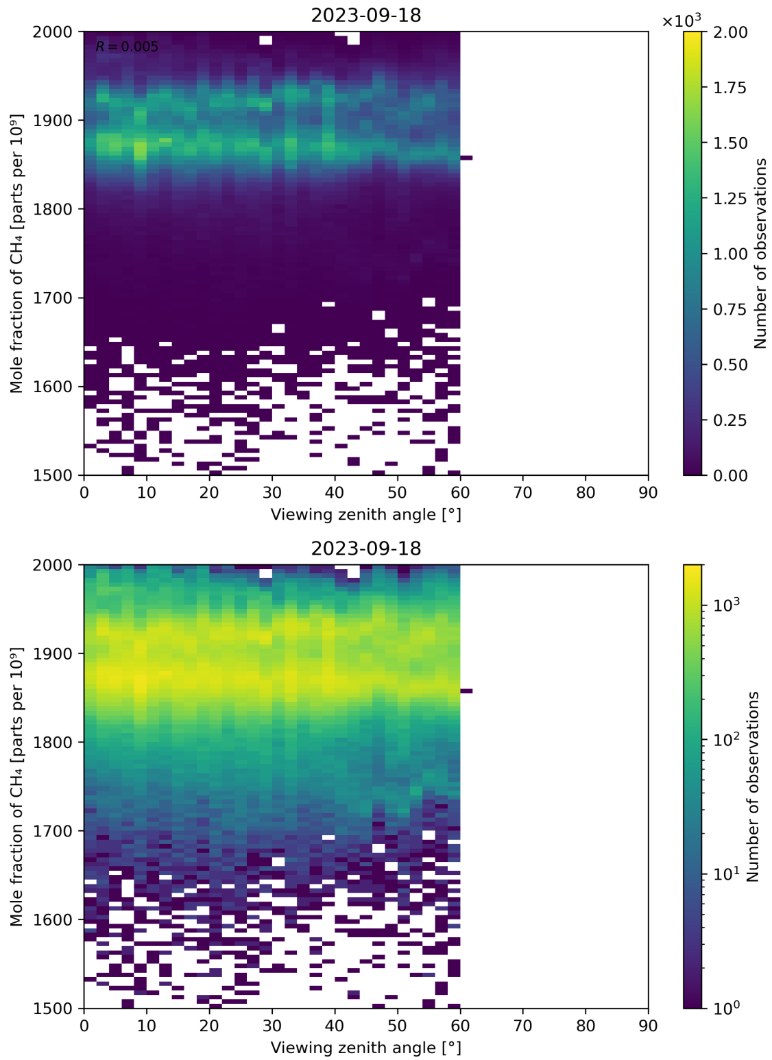
Figure 110: Scatter density plot of “Viewing zenith angle” against “Mole fraction of CH 4 ” for 2023-09-17 to 2023-09-19.
