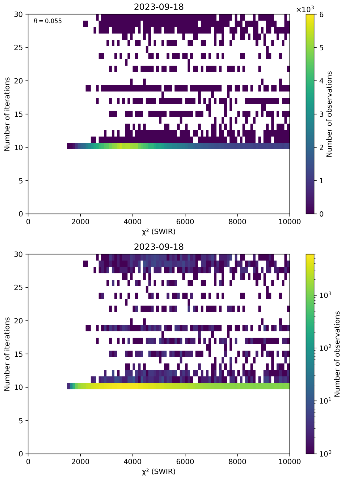
Figure 50: Scatter density plot of “ \chi^2 (SWIR)” against “Number of iterations” for 2023-09-17 to 2023-09-19.
