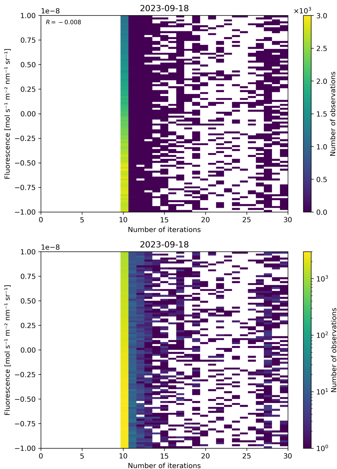
Figure 87: Scatter density plot of “Number of iterations” against “Fluorescence” for 2023-09-17 to 2023-09-19.
