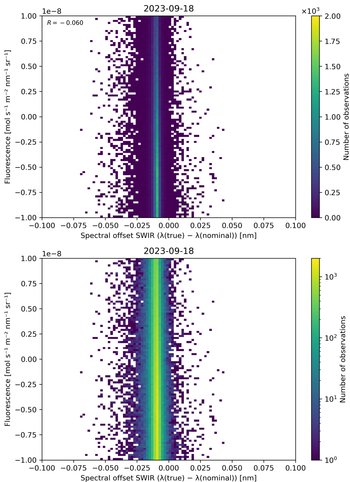
Figure 120: Scatter density plot of “Spectral offset SWIR ( \lambda(\text{true}) - \lambda(\text{nominal}) )” against “Fluorescence” for 2023-09-17 to 2023-09-19.
