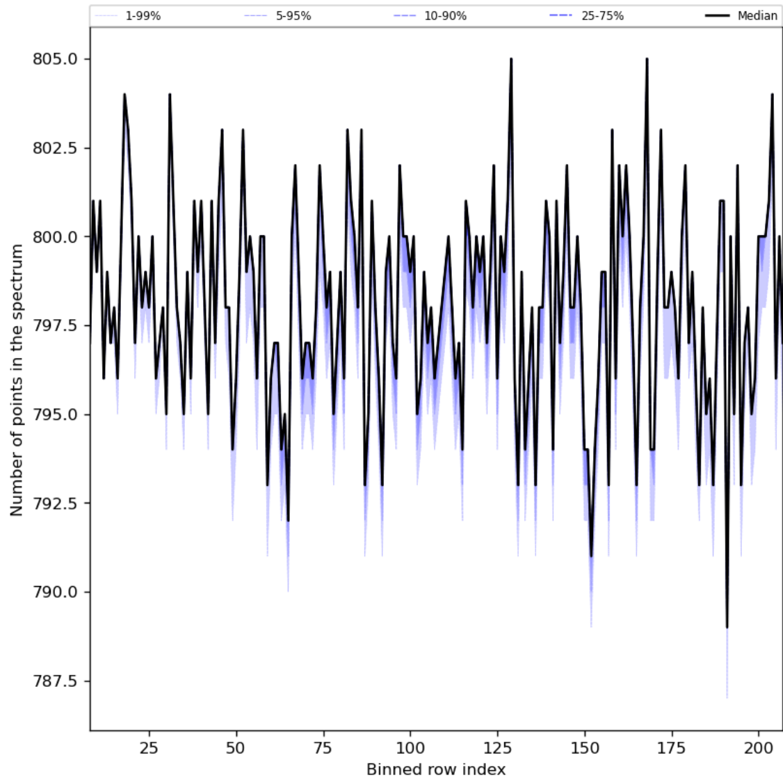
Figure 37: Along track statistics of “Number of points in the spectrum” for 2023-09-17 to 2023-09-19
