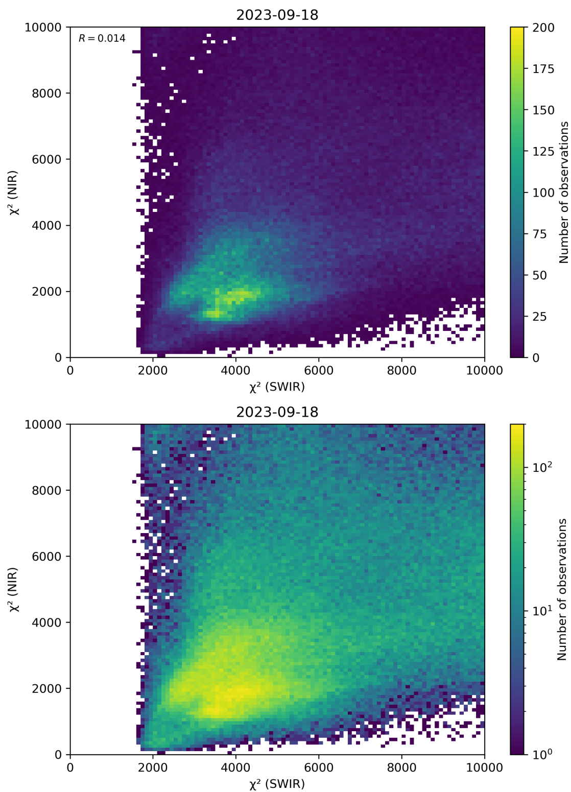
Figure 47: Scatter density plot of “ \chi^2 (SWIR)” against “ \chi^2 (NIR)” for 2023-09-17 to 2023-09-19.
