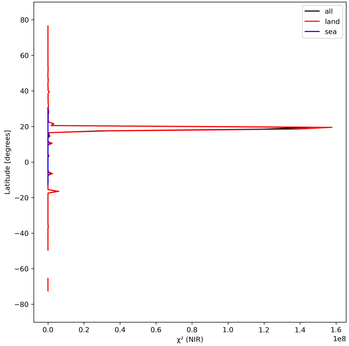
Figure 18: Zonal average of “ \chi^2 (NIR)” for 2023-09-17 to 2023-09-19.
