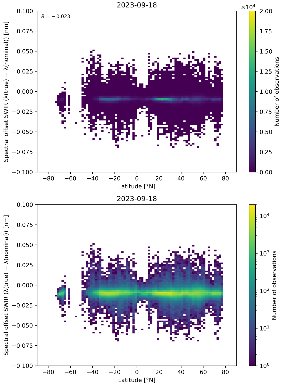
Figure 62: Scatter density plot of “Latitude” against “Spectral offset SWIR ( \lambda(\text{true}) - \lambda(\text{nominal}) )” for 2023-09-17 to 2023-09-19.
