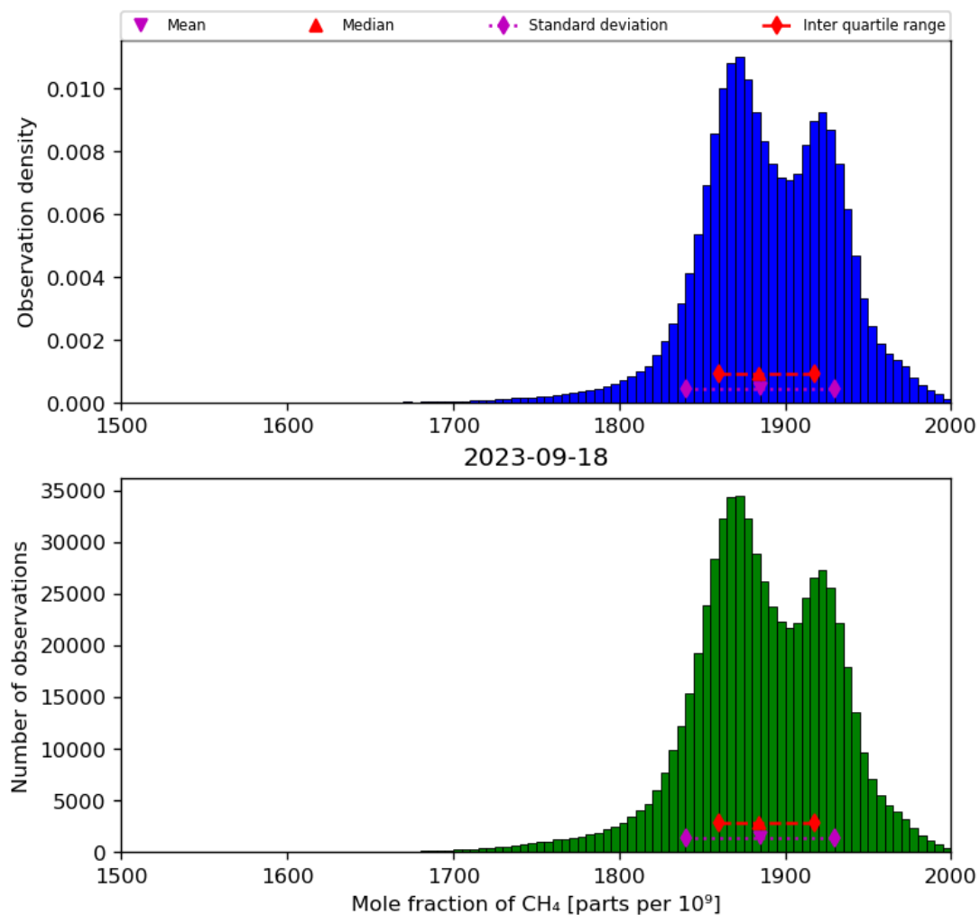
Figure 23: Histogram of “Mole fraction of CH 4 ” for 2023-09-17 to 2023-09-19
