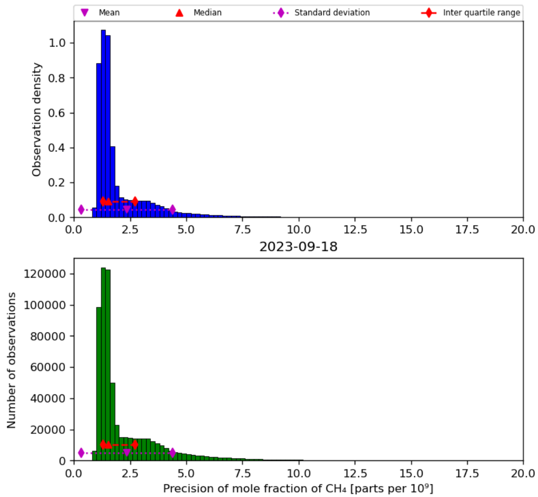
Figure 24: Histogram of “Precision of mole fraction of CH 4 ” for 2023-09-17 to 2023-09-19
