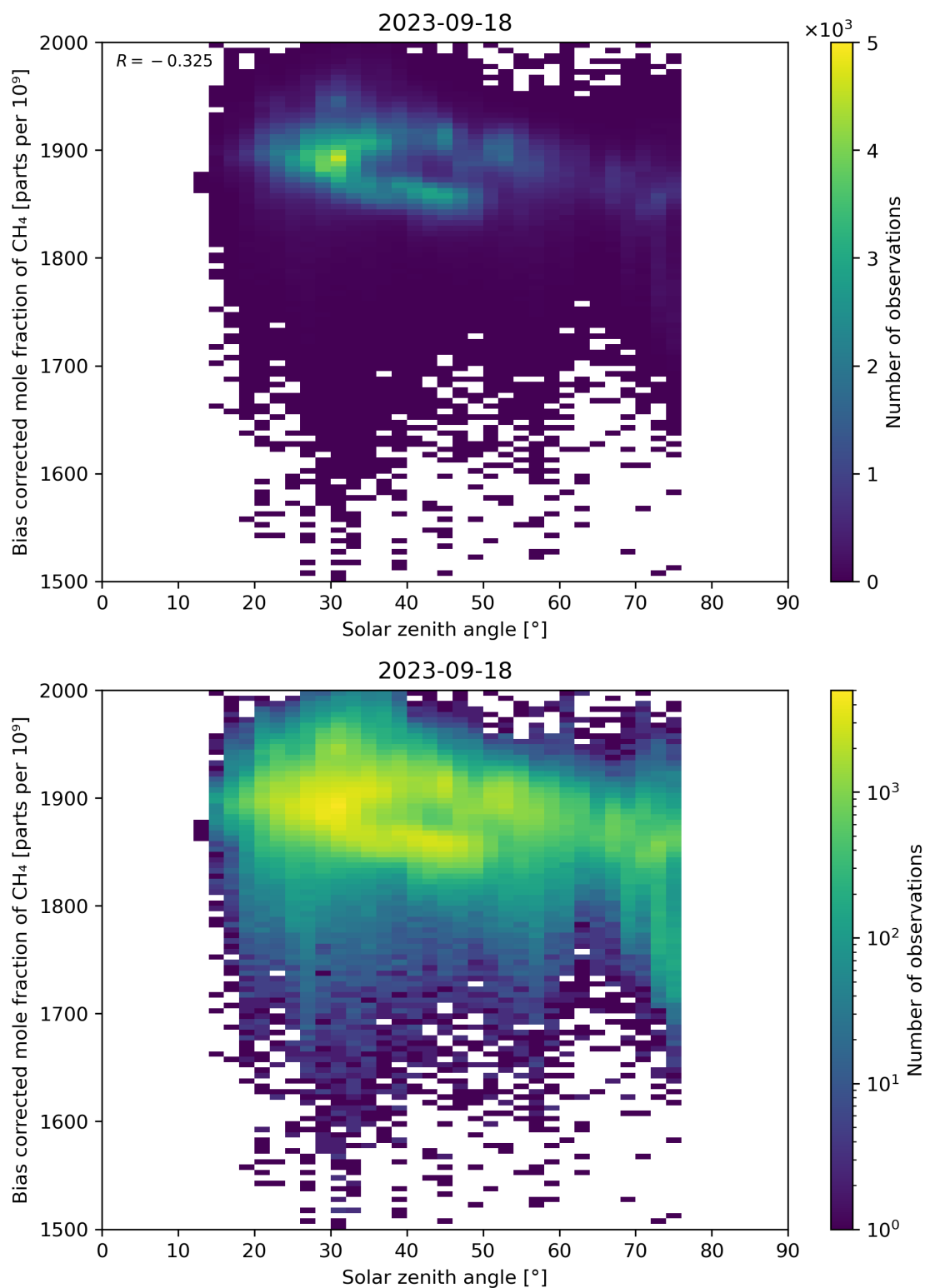
Figure 100: Scatter density plot of “Solar zenith angle” against “Bias corrected mole fraction of CH 4 ” for 2023-09-17 to 2023-09-19.
