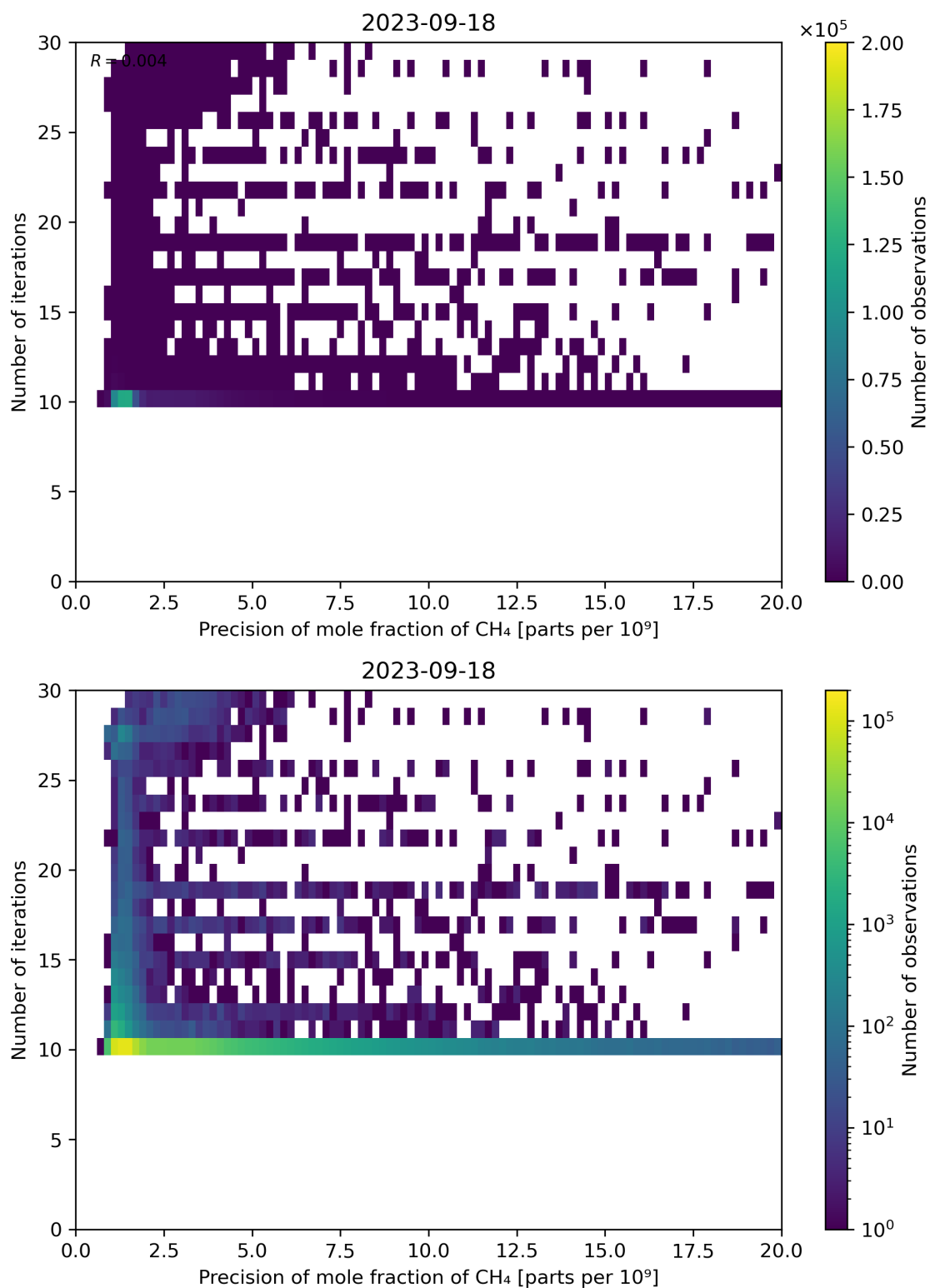
Figure 83: Scatter density plot of “Precision of mole fraction of CH 4 ” against “Number of iterations” for 2023-09-17 to 2023-09-19.
