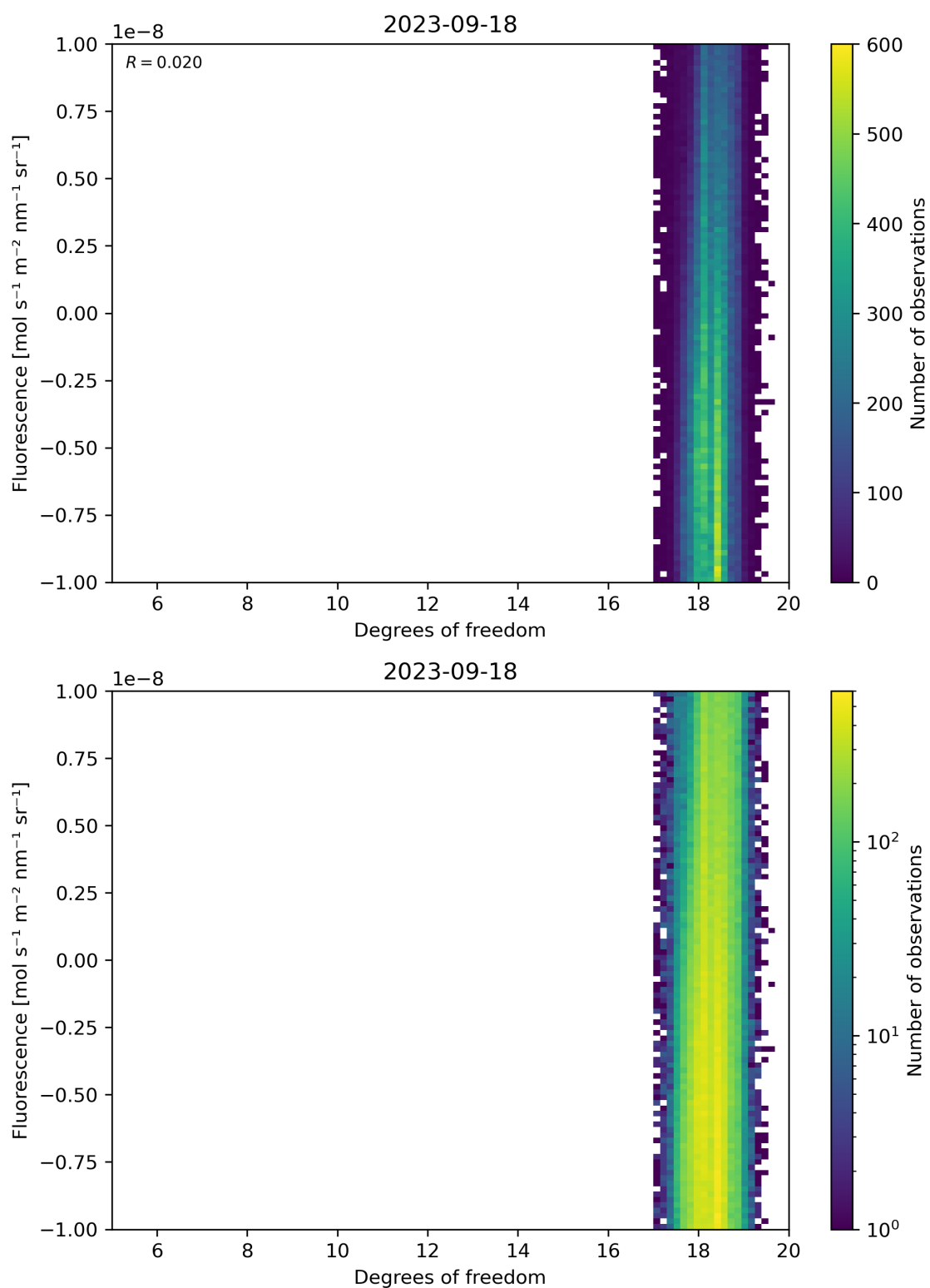
Figure 51: Scatter density plot of “Degrees of freedom” against “Fluorescence” for 2023-09-17 to 2023-09-19.
