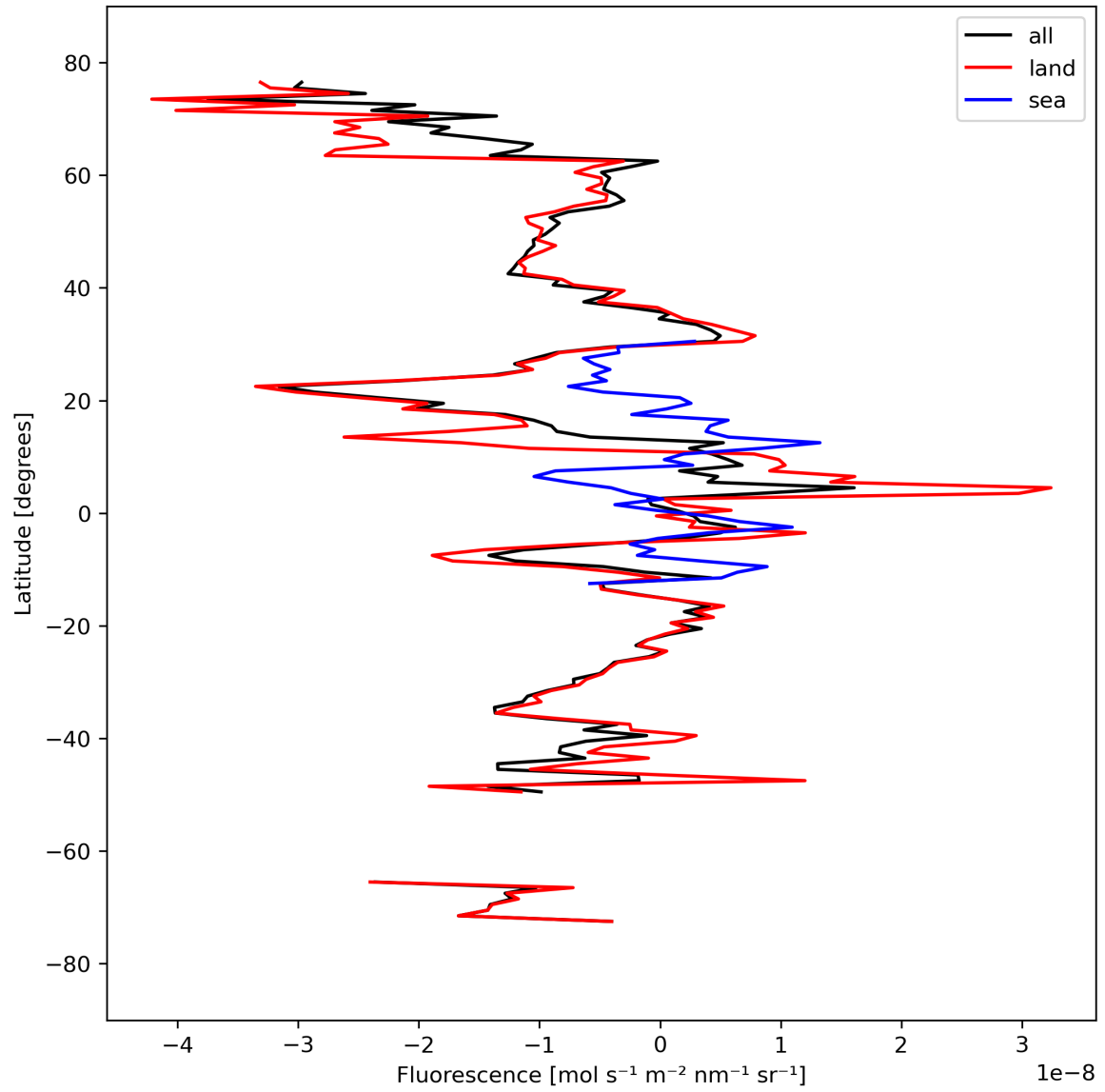
Figure 21: Zonal average of “Fluorescence” for 2023-09-17 to 2023-09-19.
