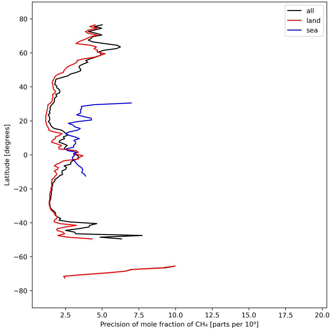
Figure 13: Zonal average of “Precision of mole fraction of \text{CH}_4 ” for 2023-09-17 to 2023-09-19.
