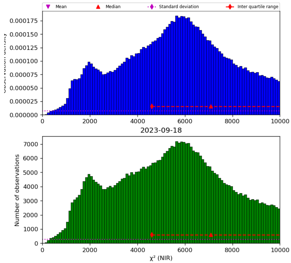
Figure 29: Histogram of “ \chi^2 (NIR)” for 2023-09-17 to 2023-09-19
