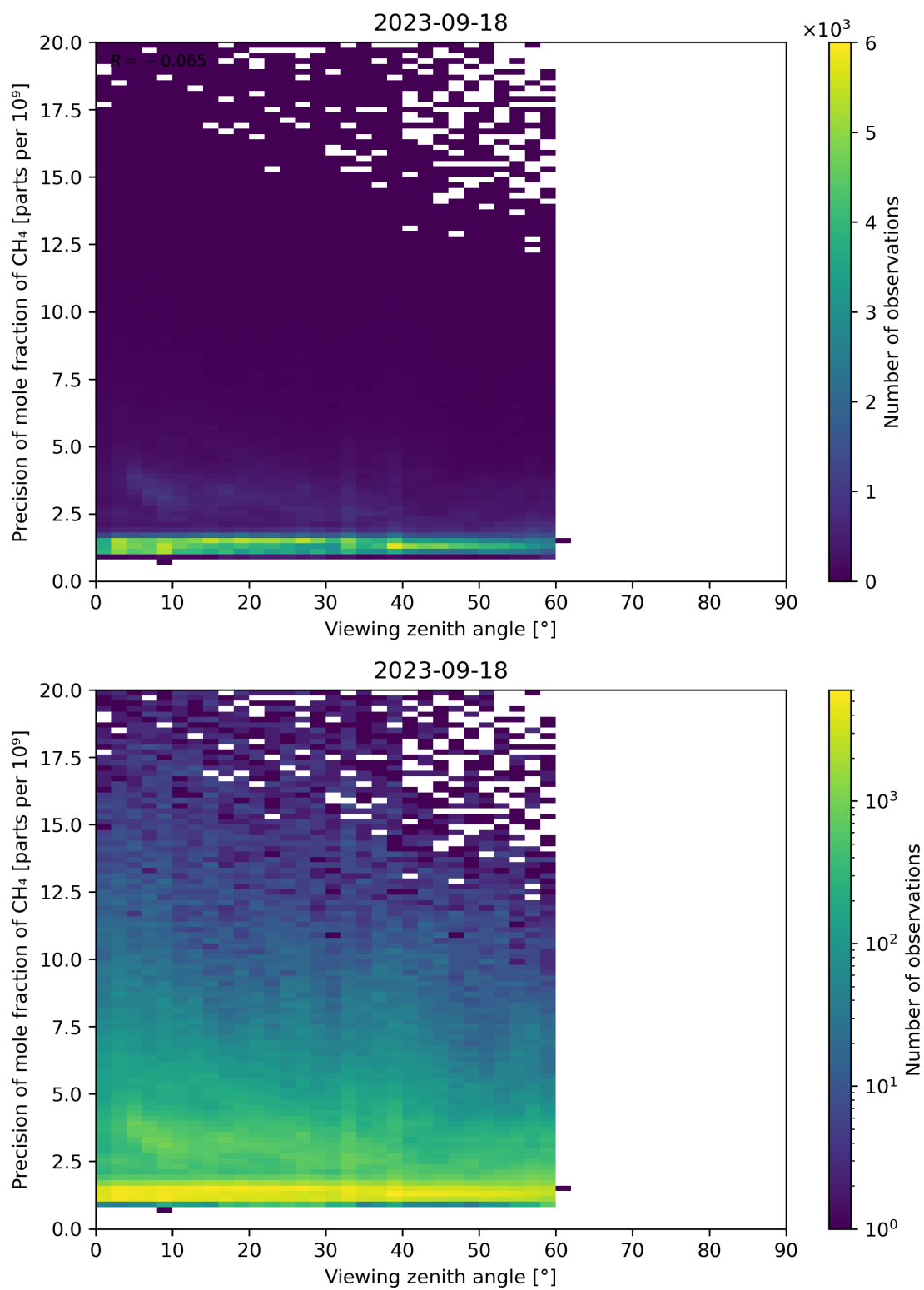
Figure 112: Scatter density plot of “Viewing zenith angle” against “Precision of mole fraction of CH 4 ” for 2023-09-17 to 2023-09-19.
