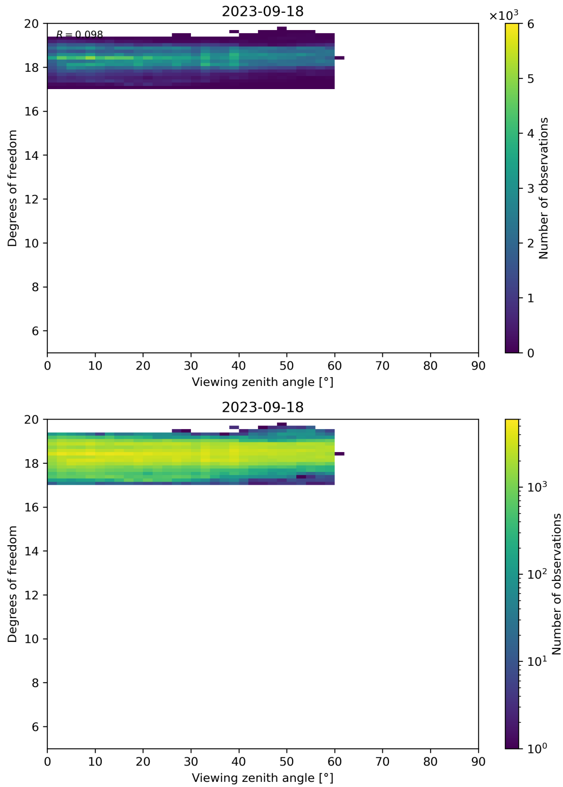
Figure 107: Scatter density plot of “Viewing zenith angle” against “Degrees of freedom” for 2023-09-17 to 2023-09-19.
