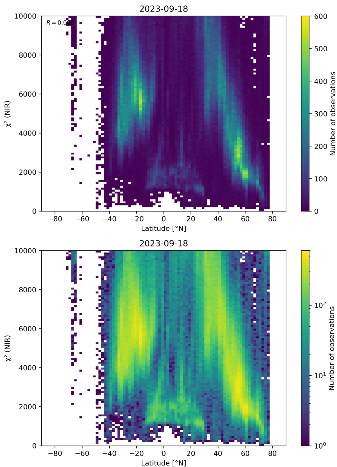
Figure 53: Scatter density plot of “Latitude” against “ \chi^2 (NIR)” for 2023-09-17 to 2023-09-19.
