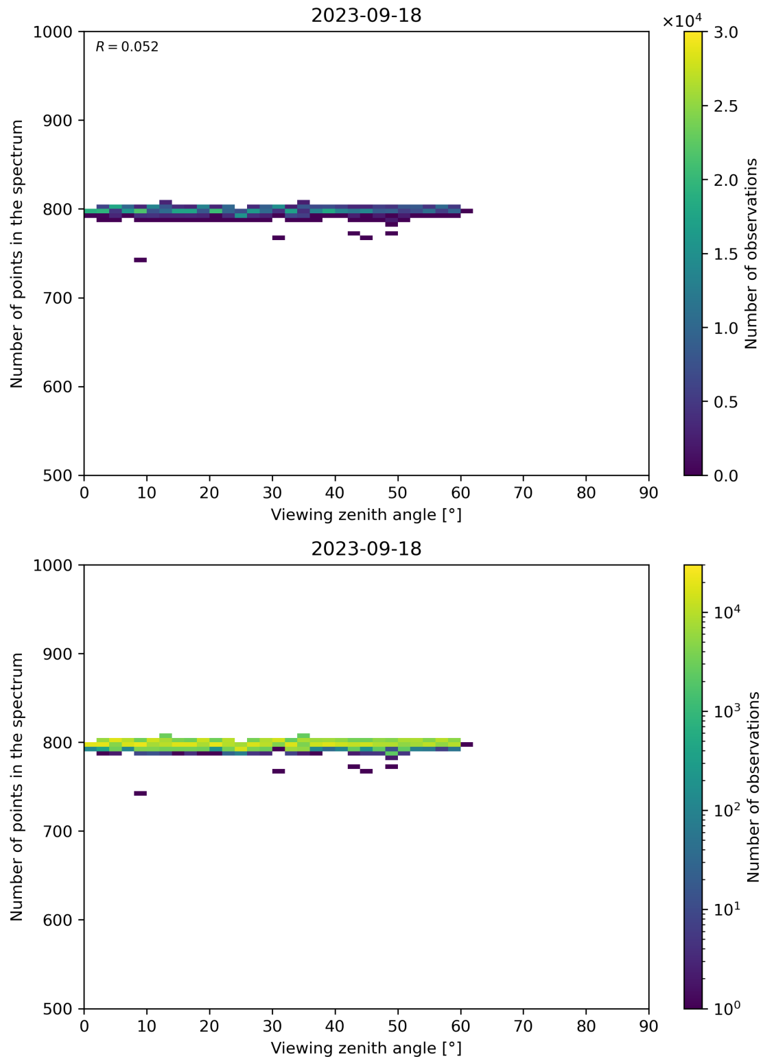
Figure 114: Scatter density plot of “Viewing zenith angle” against “Number of points in the spectrum” for 2023-09-17 to 2023-09-19.
