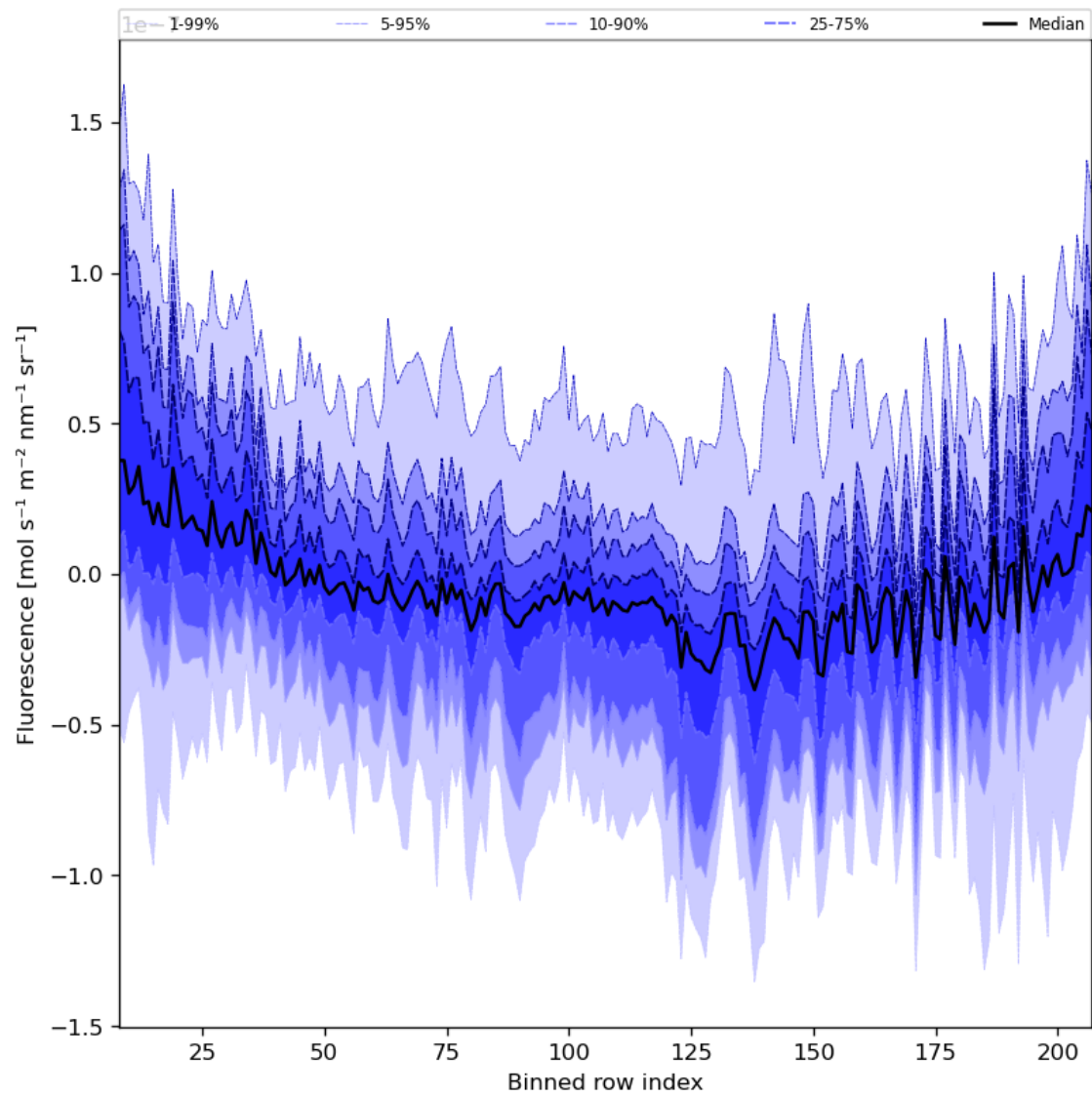
Figure 43: Along track statistics of “Fluorescence” for 2023-09-17 to 2023-09-19
