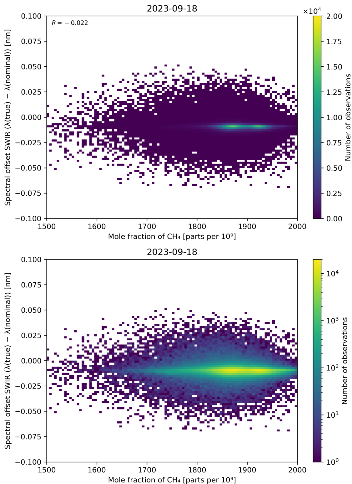
Figure 86: Scatter density plot of “Mole fraction of CH 4 ” against “Spectral offset SWIR ( \lambda(\text{true}) - \lambda(\text{nominal}) )” for 2023-09-17 to 2023-09-19.
