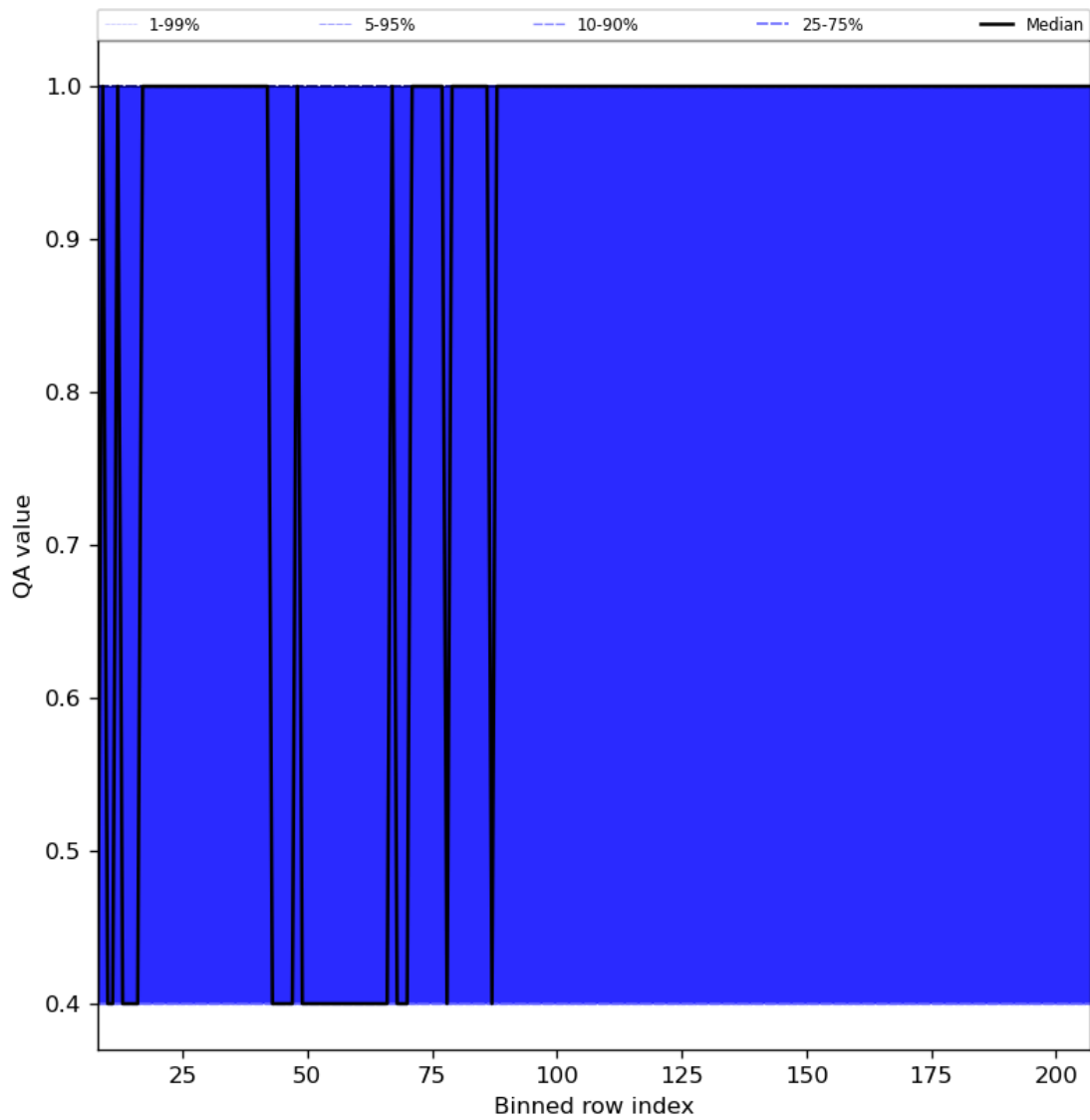
Figure 33: Along track statistics of “QA value” for 2023-09-17 to 2023-09-19
