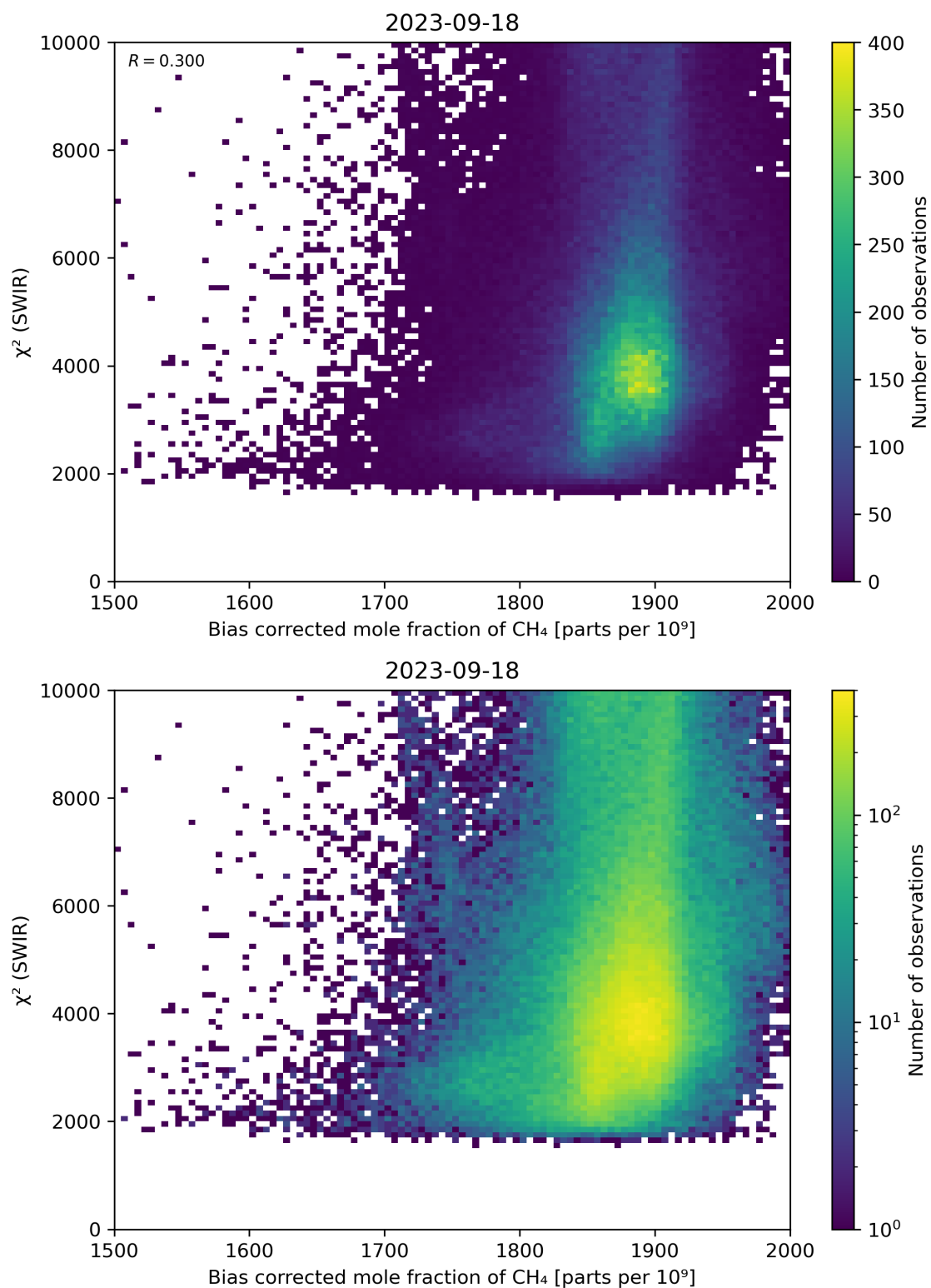
Figure 64: Scatter density plot of “Bias corrected mole fraction of CH 4 ” against “ \chi^2 (SWIR)” for 2023-09-17 to 2023-09-19.
