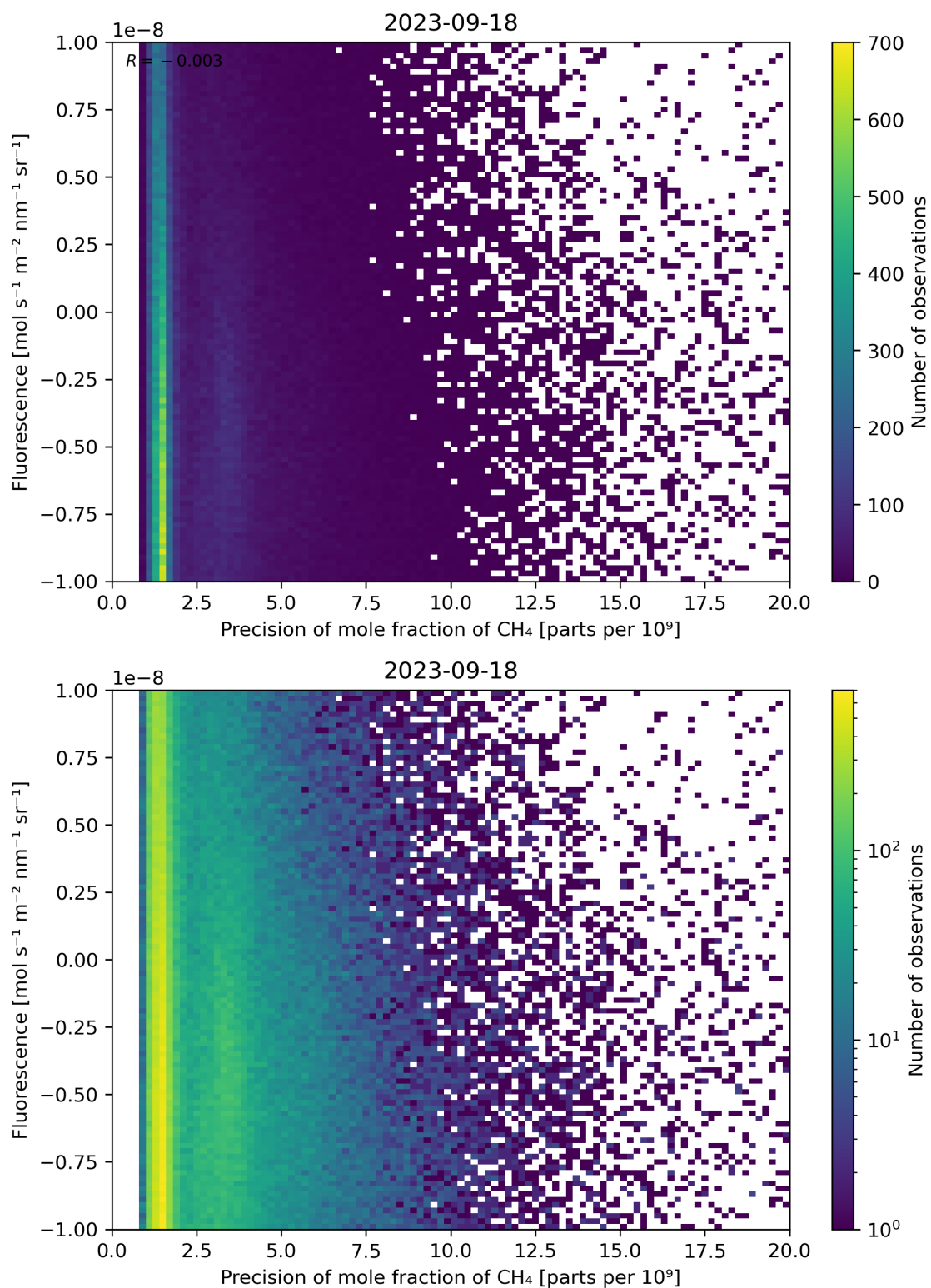
Figure 81: Scatter density plot of “Precision of mole fraction of \text{CH}_4 ” against “Fluorescence” for 2023-09-17 to 2023-09-19.
