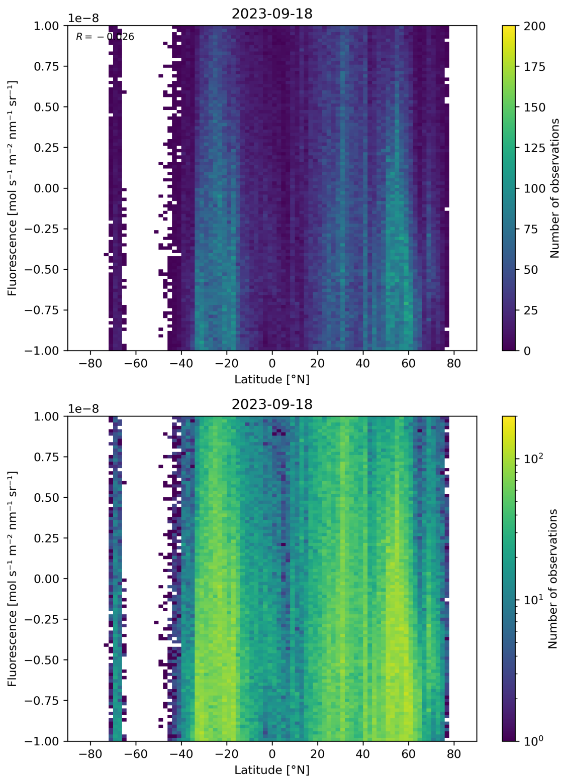
Figure 56: Scatter density plot of “Latitude” against “Fluorescence” for 2023-09-17 to 2023-09-19.
