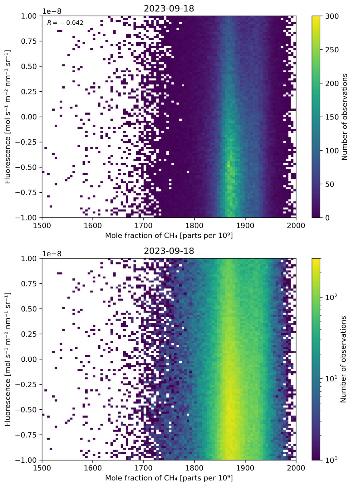
Figure 73: Scatter density plot of “Mole fraction of \text{CH}_4 ” against “Fluorescence” for 2023-09-17 to 2023-09-19.
