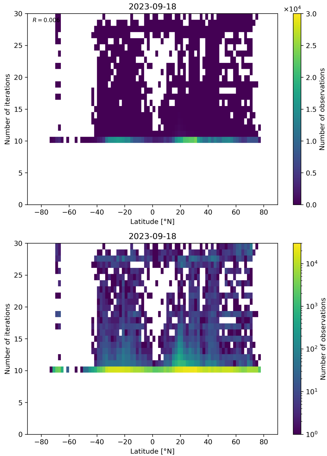
Figure 60: Scatter density plot of “Latitude” against “Number of iterations” for 2023-09-17 to 2023-09-19.
