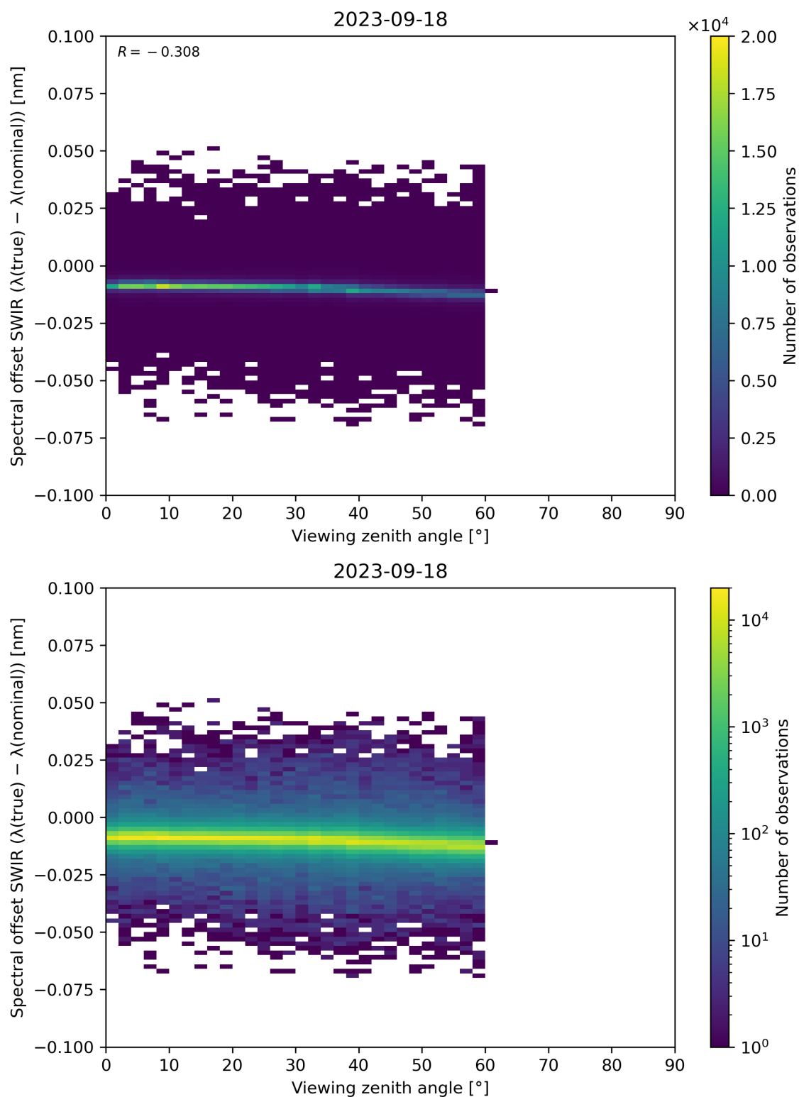
Figure 116: Scatter density plot of “Viewing zenith angle” against “Spectral offset SWIR ( \lambda(\text{true}) - \lambda(\text{nominal}) )” for 2023-09-17 to 2023-09-19.
