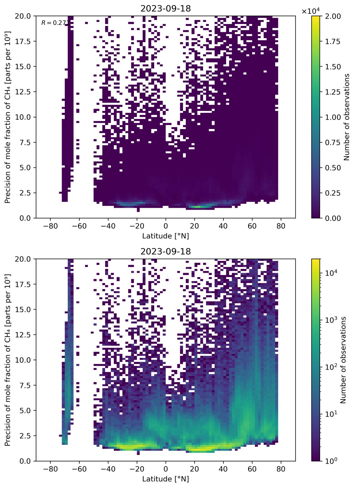
Figure 59: Scatter density plot of “Latitude” against “Precision of mole fraction of CH 4 ” for 2023-09-17 to 2023-09-19.
