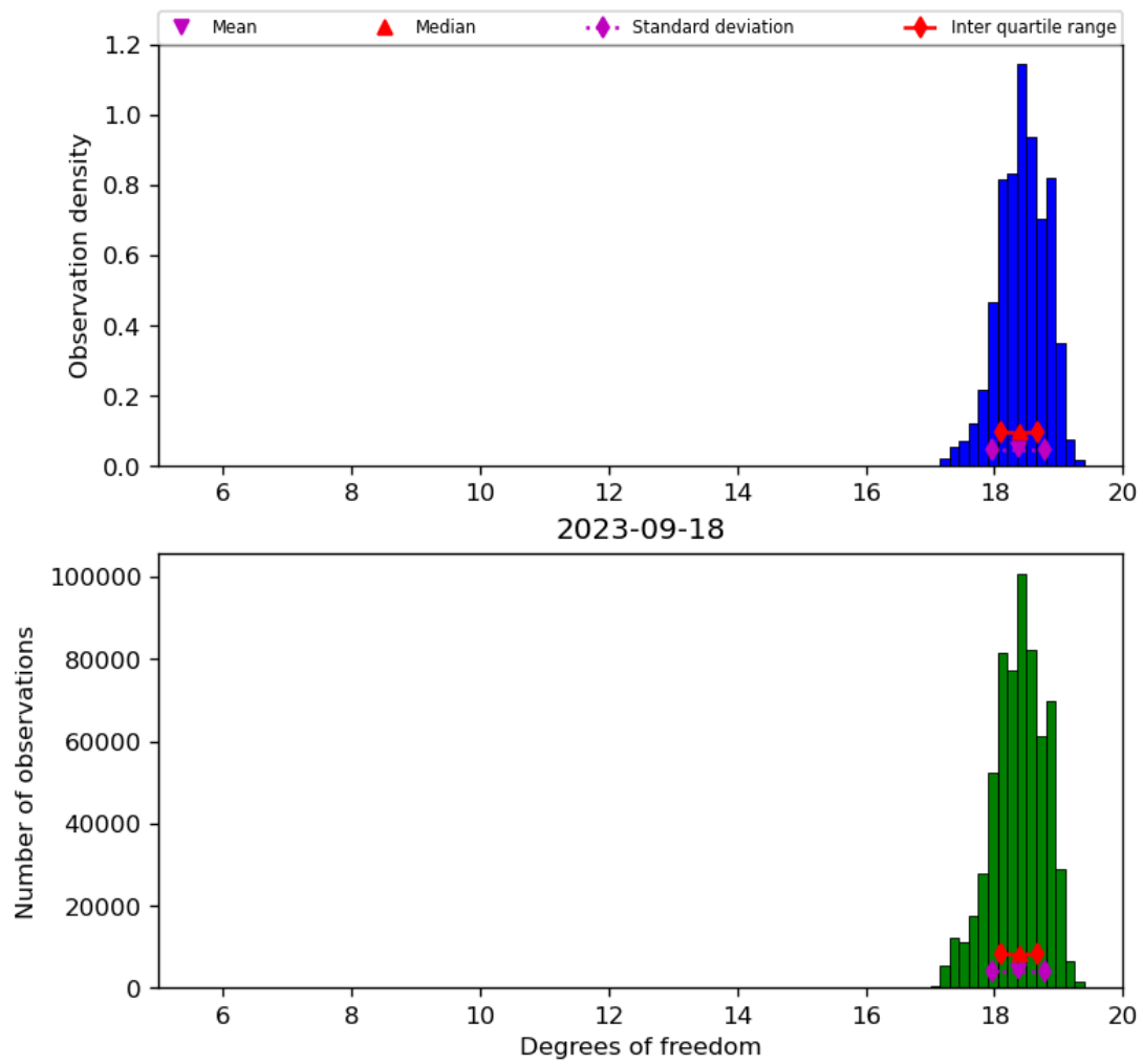
Figure 30: Histogram of “Degrees of freedom” for 2023-09-17 to 2023-09-19
