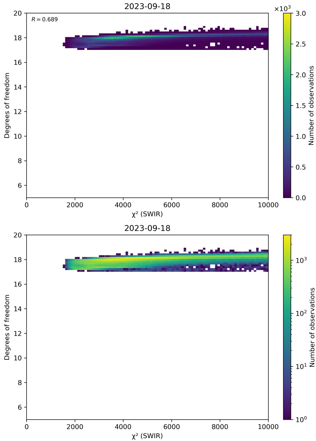
Figure 48: Scatter density plot of “ \chi^2 (SWIR)” against “Degrees of freedom” for 2023-09-17 to 2023-09-19.
