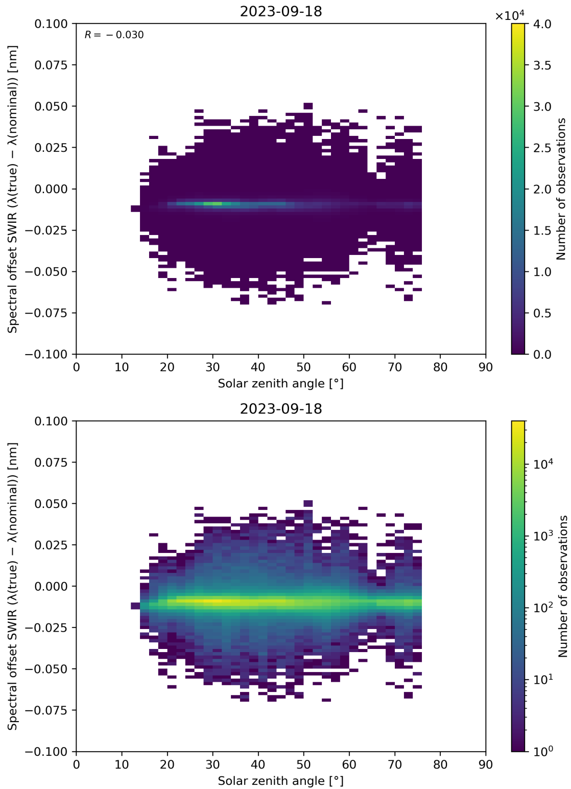
Figure 104: Scatter density plot of “Solar zenith angle” against “Spectral offset SWIR ( \lambda(\text{true}) - \lambda(\text{nominal}) )” for 2023-09-17 to 2023-09-19.
