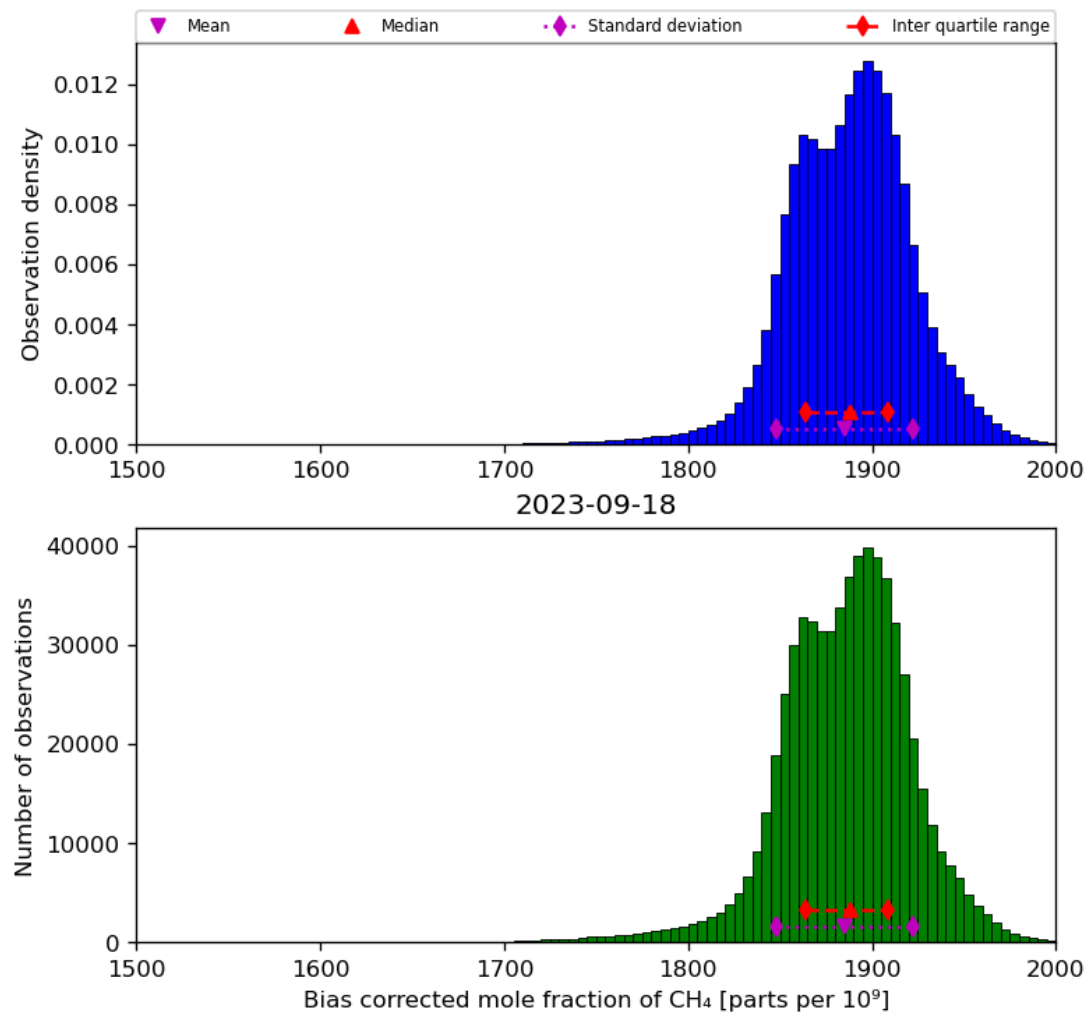
Figure 25: Histogram of “Bias corrected mole fraction of CH 4 ” for 2023-09-17 to 2023-09-19
