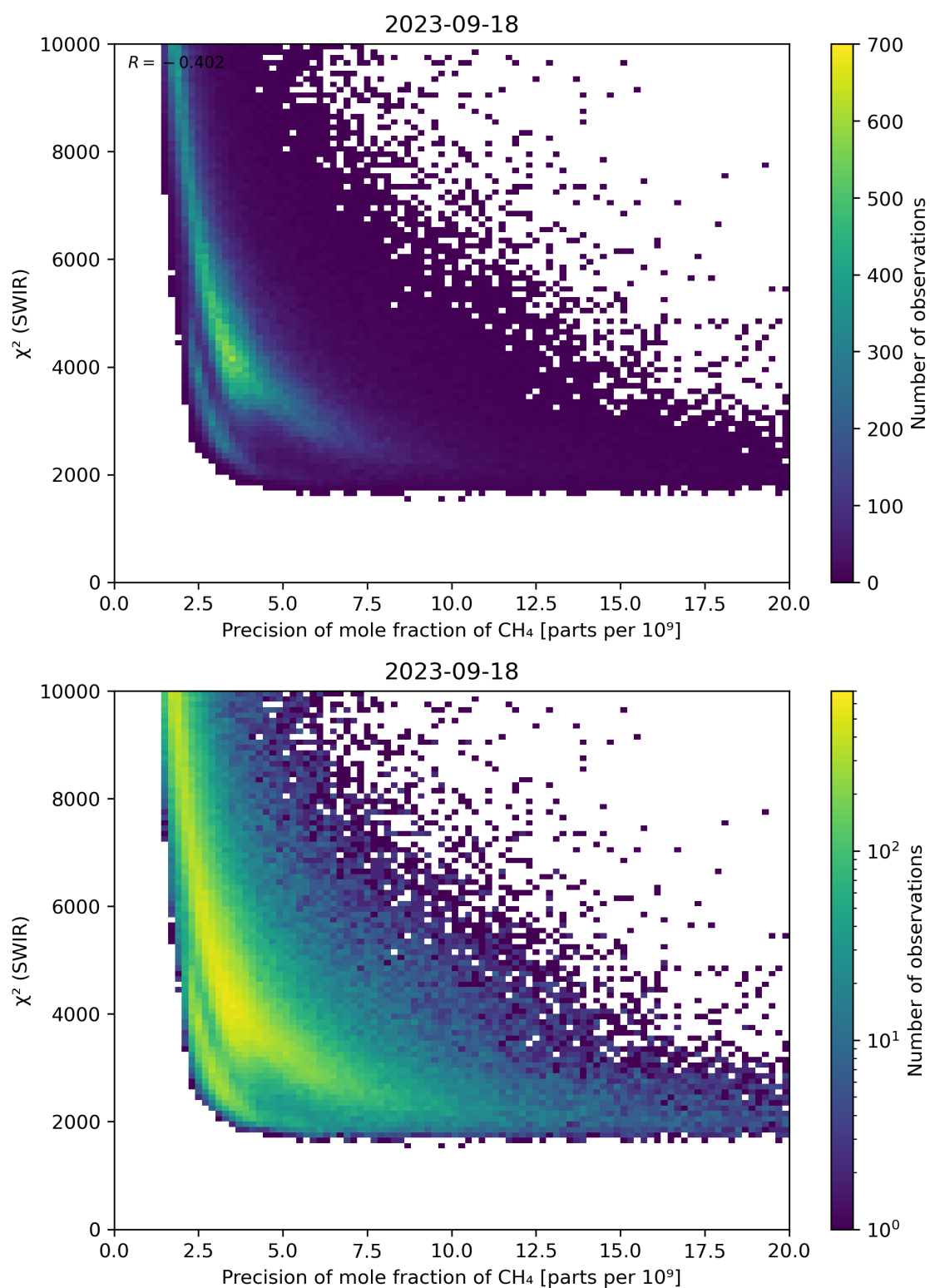
Figure 79: Scatter density plot of “Precision of mole fraction of \text{CH}_4 ” against “ \chi^2 (SWIR)” for 2023-09-17 to 2023-09-19.
