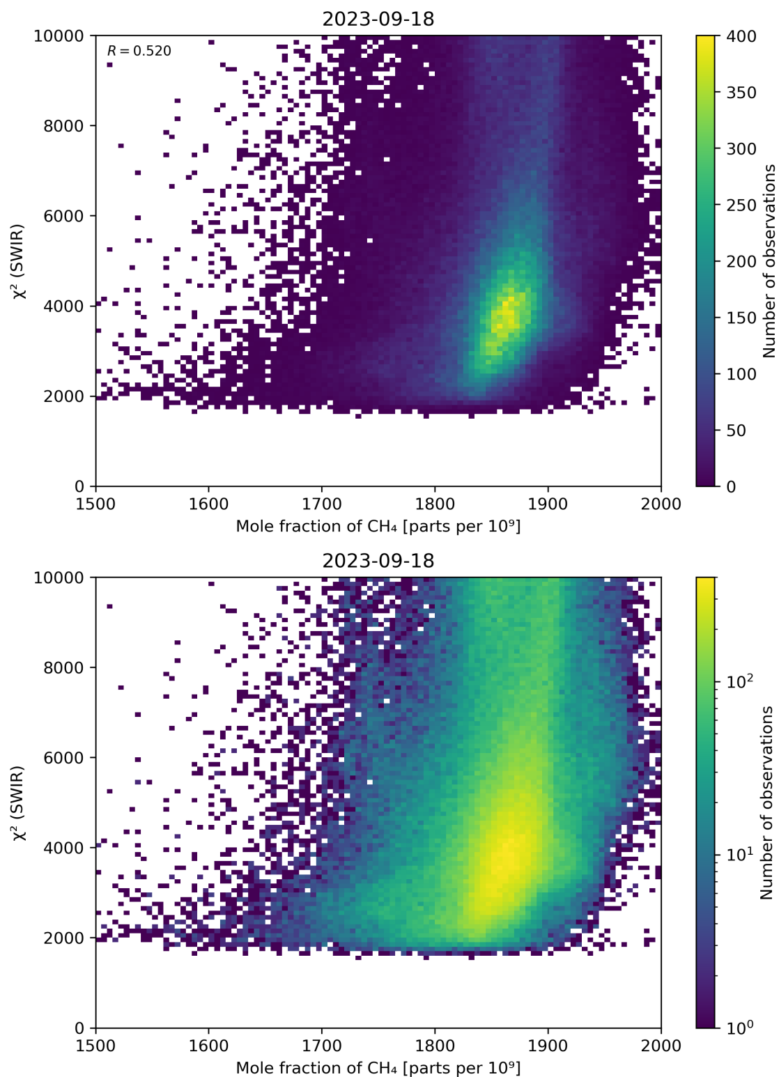
Figure 71: Scatter density plot of “Mole fraction of \text{CH}_4 ” against “ \chi^2 (SWIR)” for 2023-09-17 to 2023-09-19.
