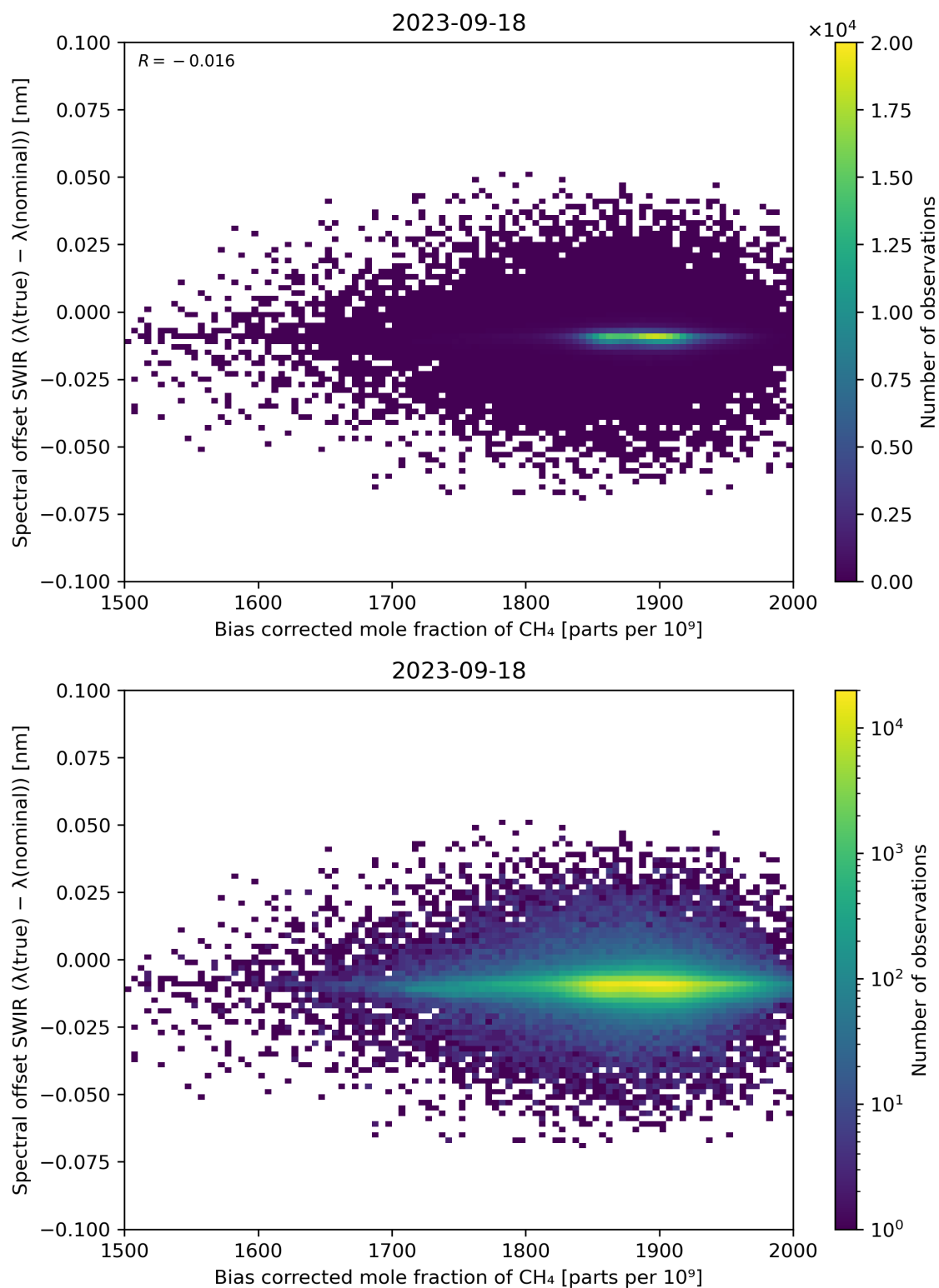
Figure 69: Scatter density plot of “Bias corrected mole fraction of \text{CH}_4 ” against “Spectral offset SWIR ( \lambda(\text{true}) - \lambda(\text{nominal}) )” for 2023-09-17 to 2023-09-19.
