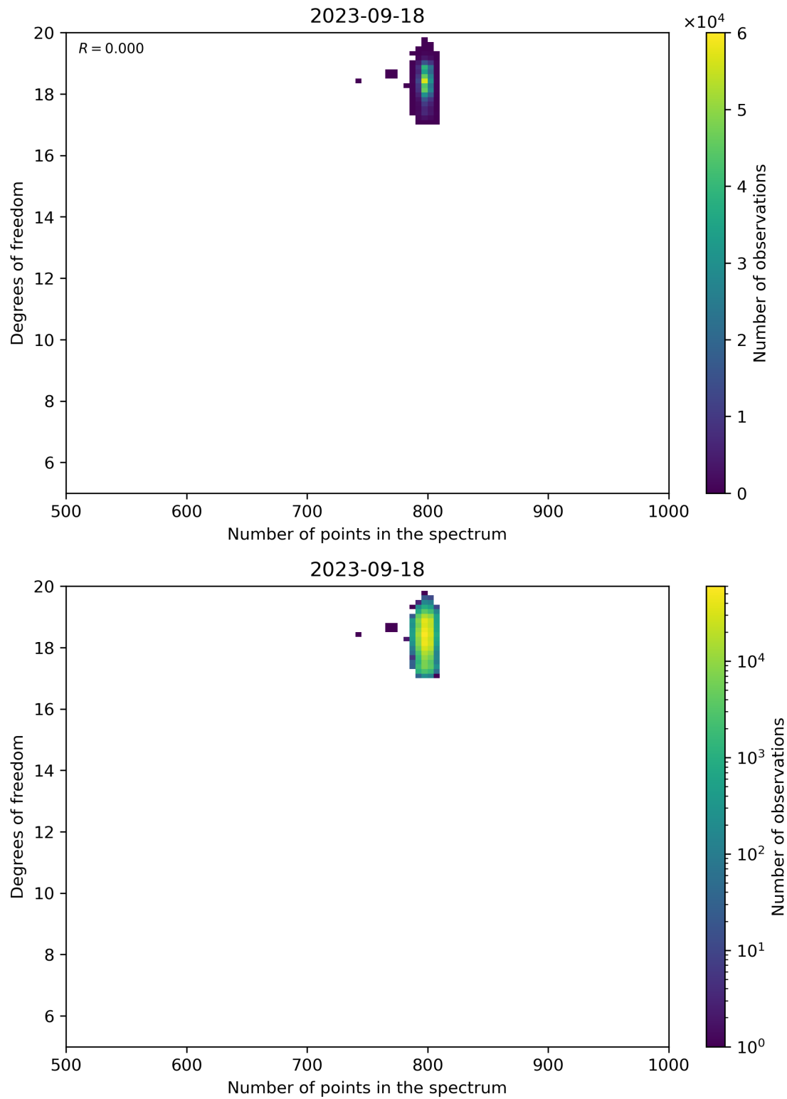
Figure 90: Scatter density plot of “Number of points in the spectrum” against “Degrees of freedom” for 2023-09-17 to 2023-09-19.
