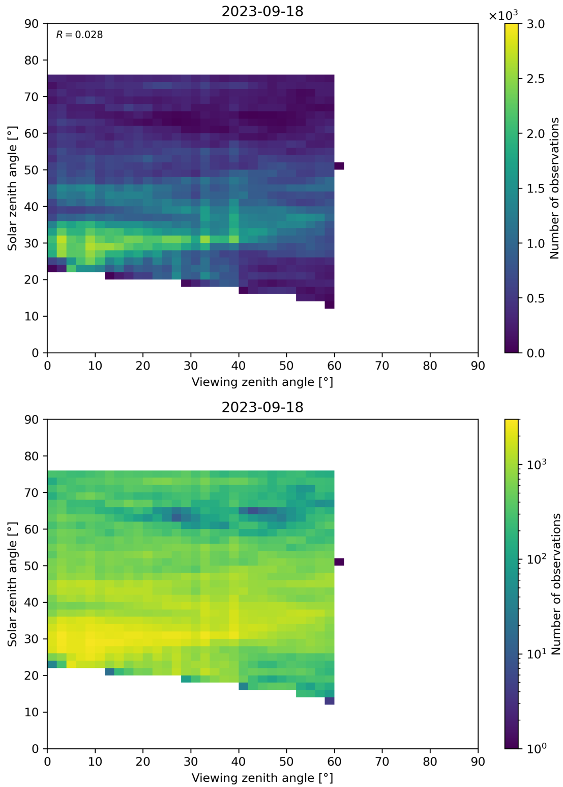
Figure 115: Scatter density plot of “Viewing zenith angle” against “Solar zenith angle” for 2023-09-17 to 2023-09-19.
