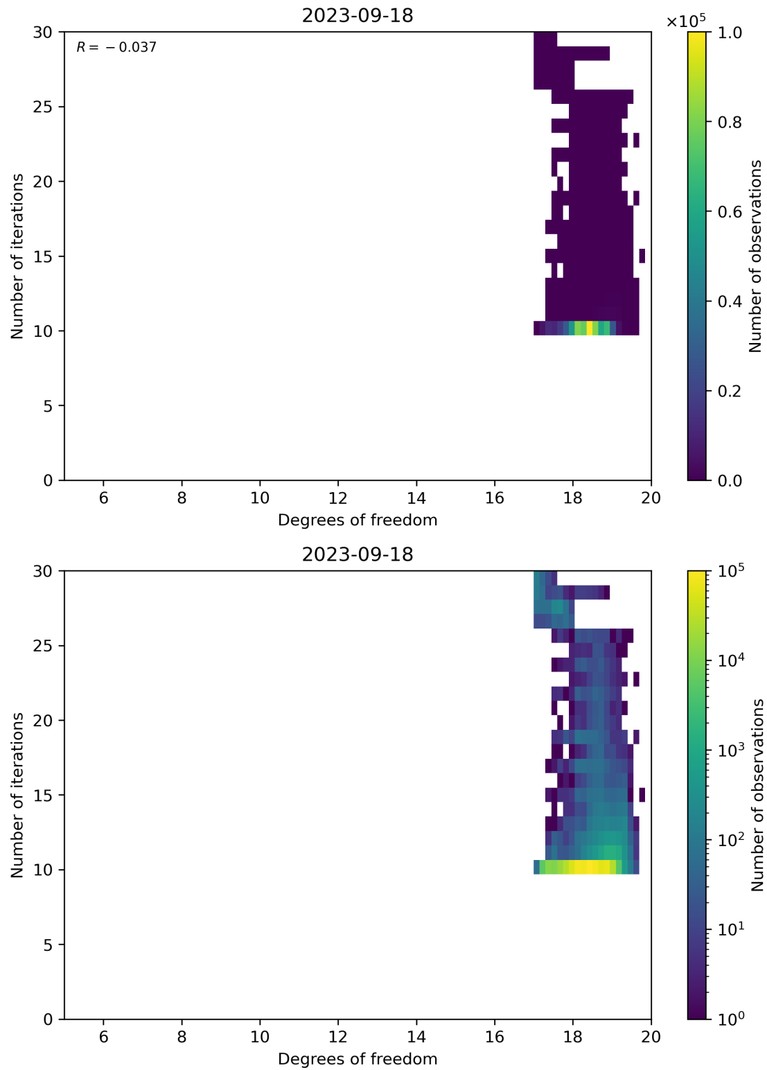
Figure 52: Scatter density plot of “Degrees of freedom” against “Number of iterations” for 2023-09-17 to 2023-09-19.
