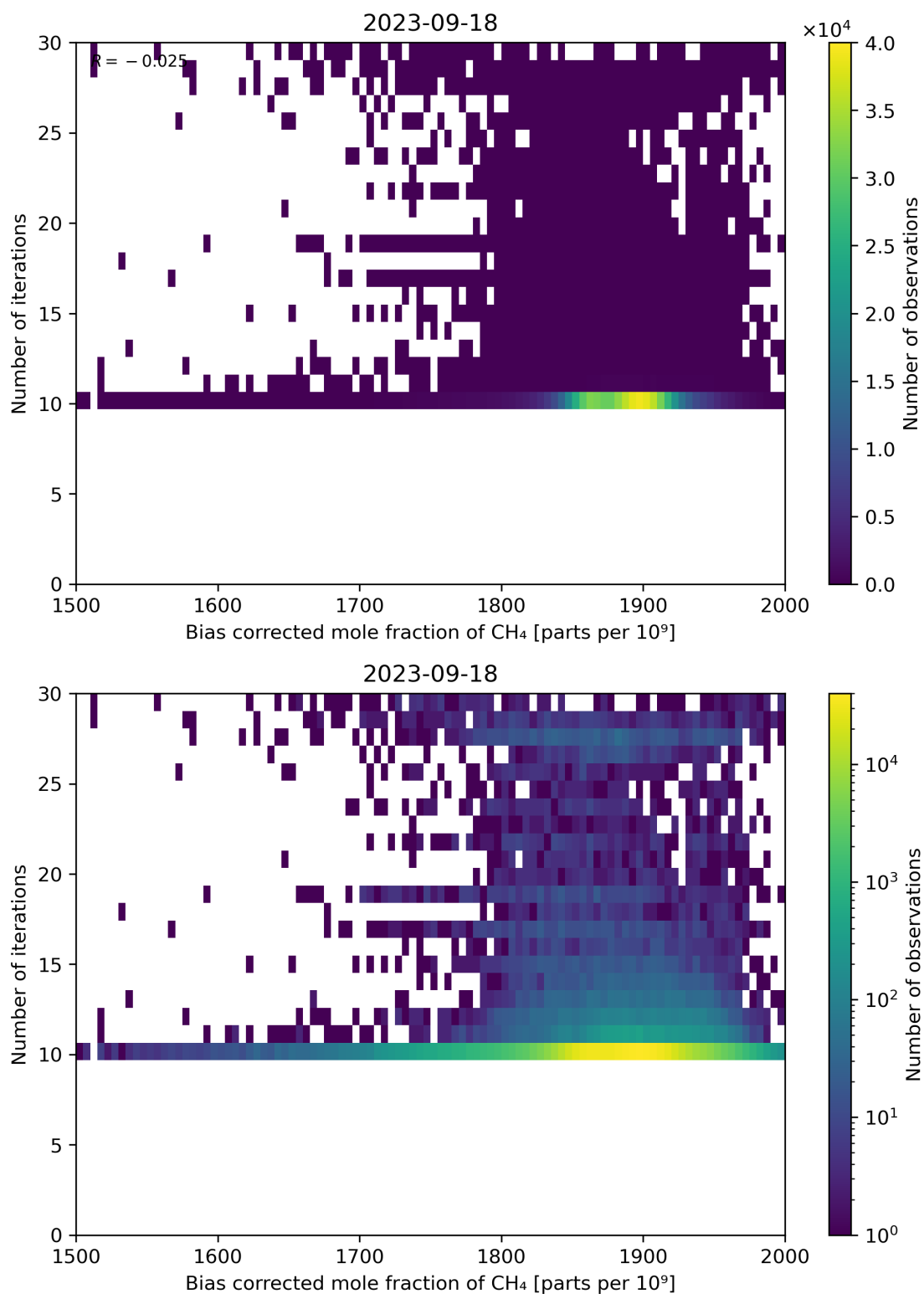
Figure 67: Scatter density plot of “Bias corrected mole fraction of CH 4 ” against “Number of iterations” for 2023-09-17 to 2023-09-19.
