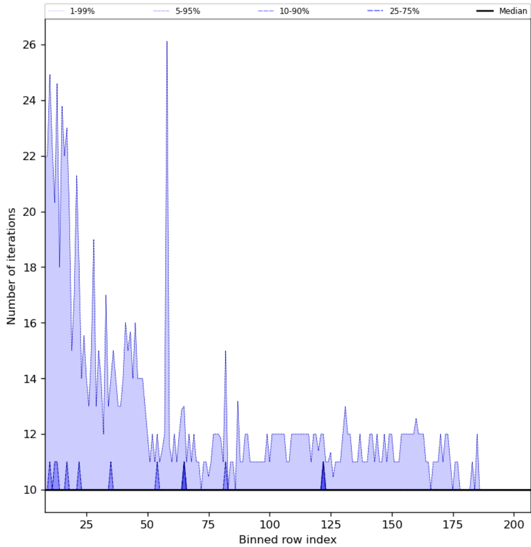
Figure 42: Along track statistics of “Number of iterations” for 2023-09-17 to 2023-09-19
