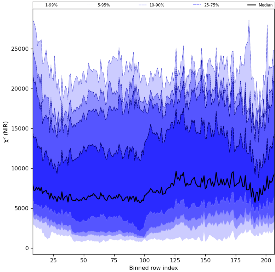
Figure 40: Along track statistics of “ \chi^2 (NIR)” for 2023-09-17 to 2023-09-19
