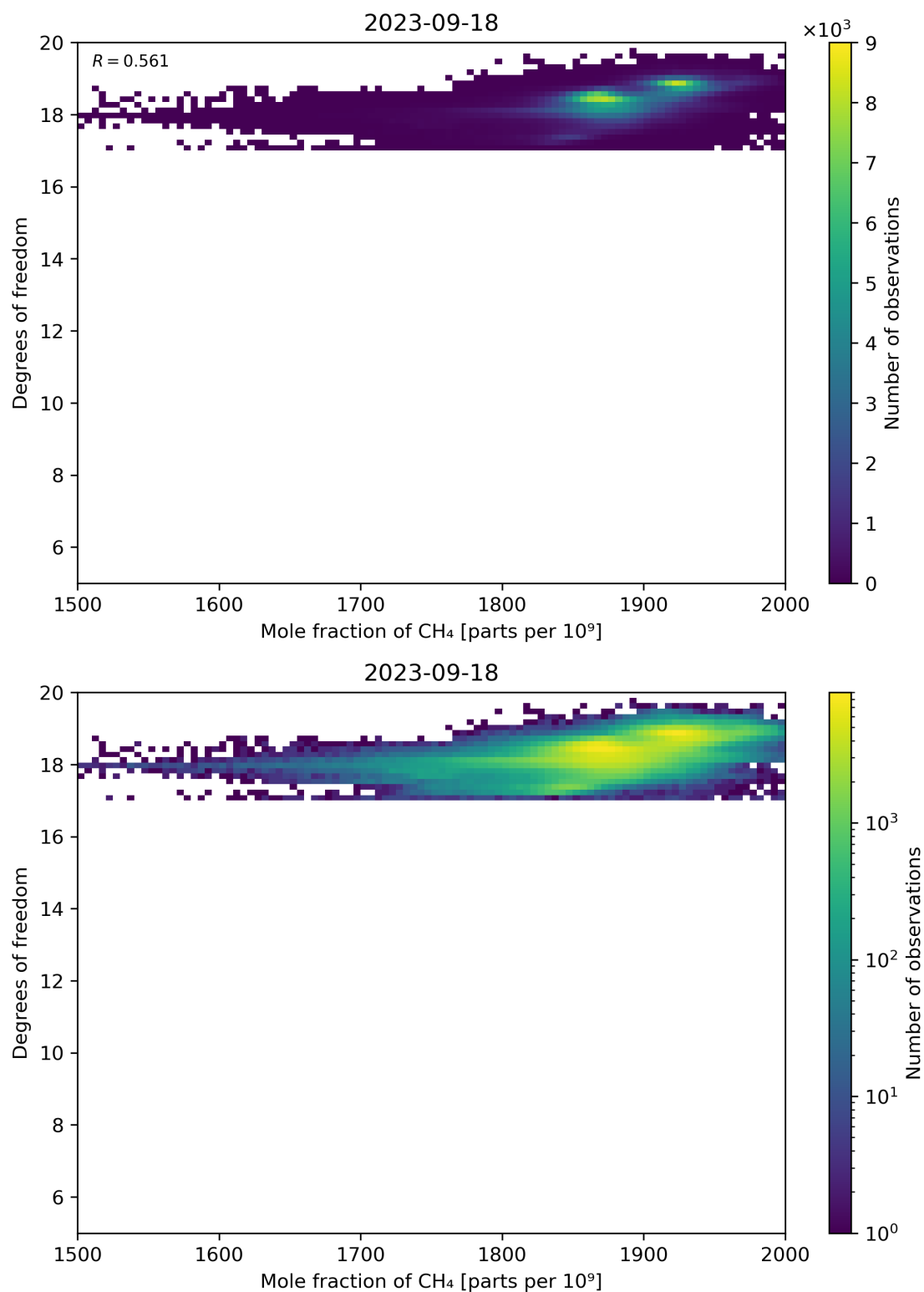
Figure 72: Scatter density plot of “Mole fraction of CH 4 ” against “Degrees of freedom” for 2023-09-17 to 2023-09-19.
