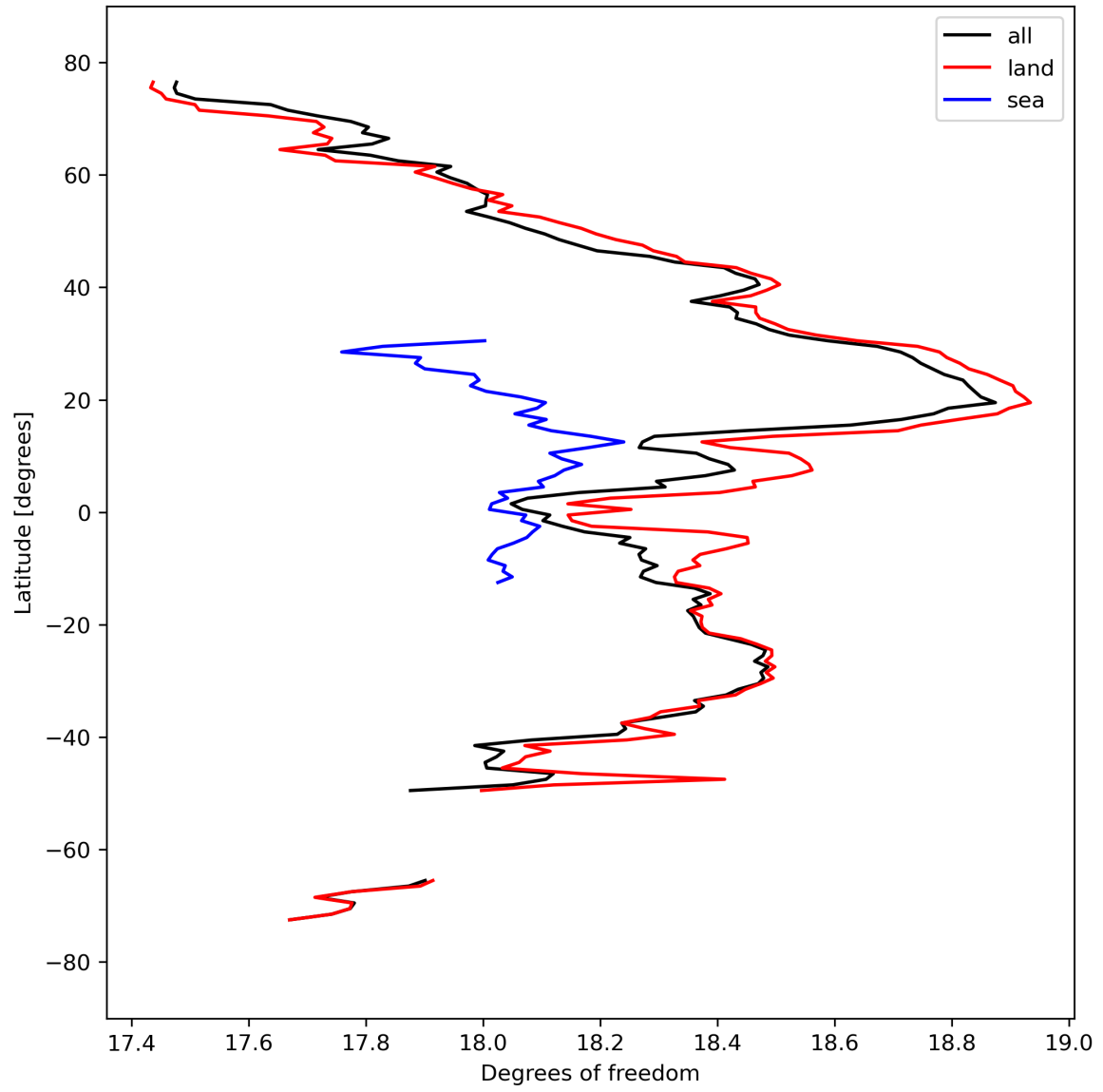
Figure 19: Zonal average of “Degrees of freedom” for 2023-09-17 to 2023-09-19.
