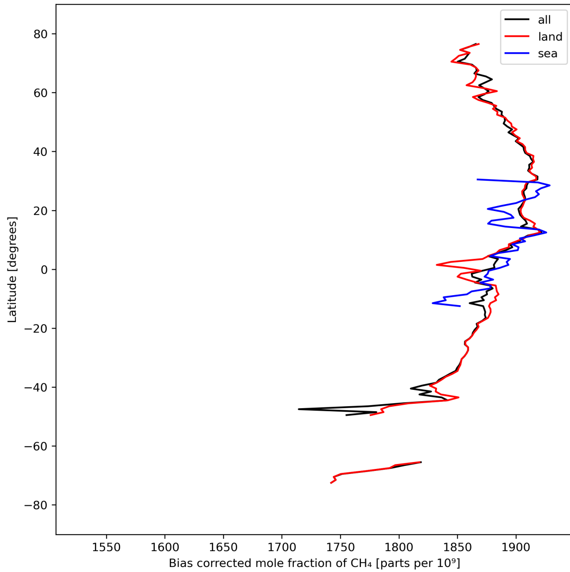
Figure 14: Zonal average of “Bias corrected mole fraction of CH 4 ” for 2023-09-17 to 2023-09-19.
