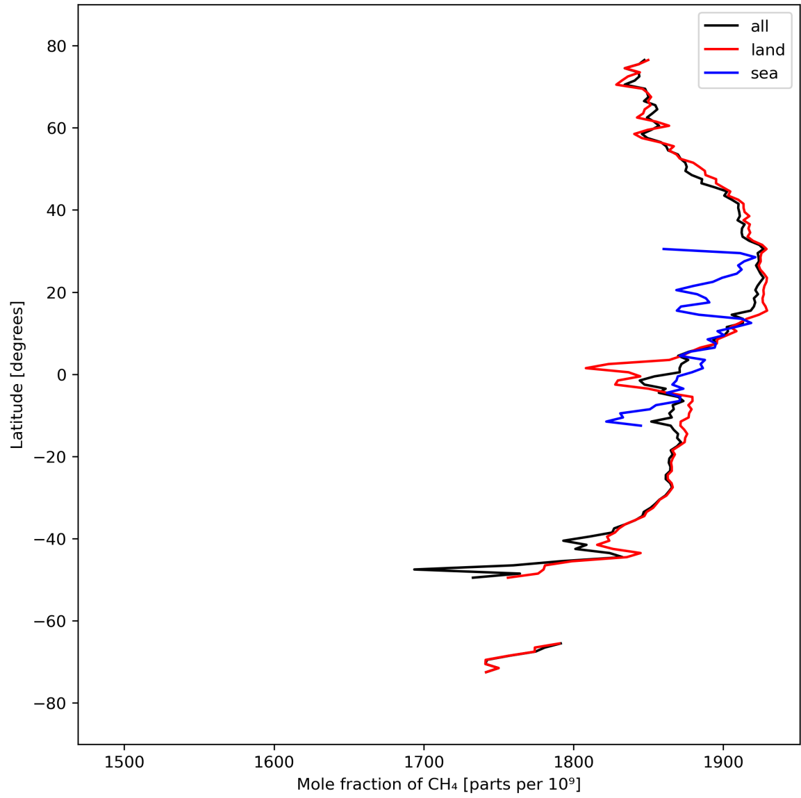
Figure 12: Zonal average of “Mole fraction of \text{CH}_4 ” for 2023-09-17 to 2023-09-19.
