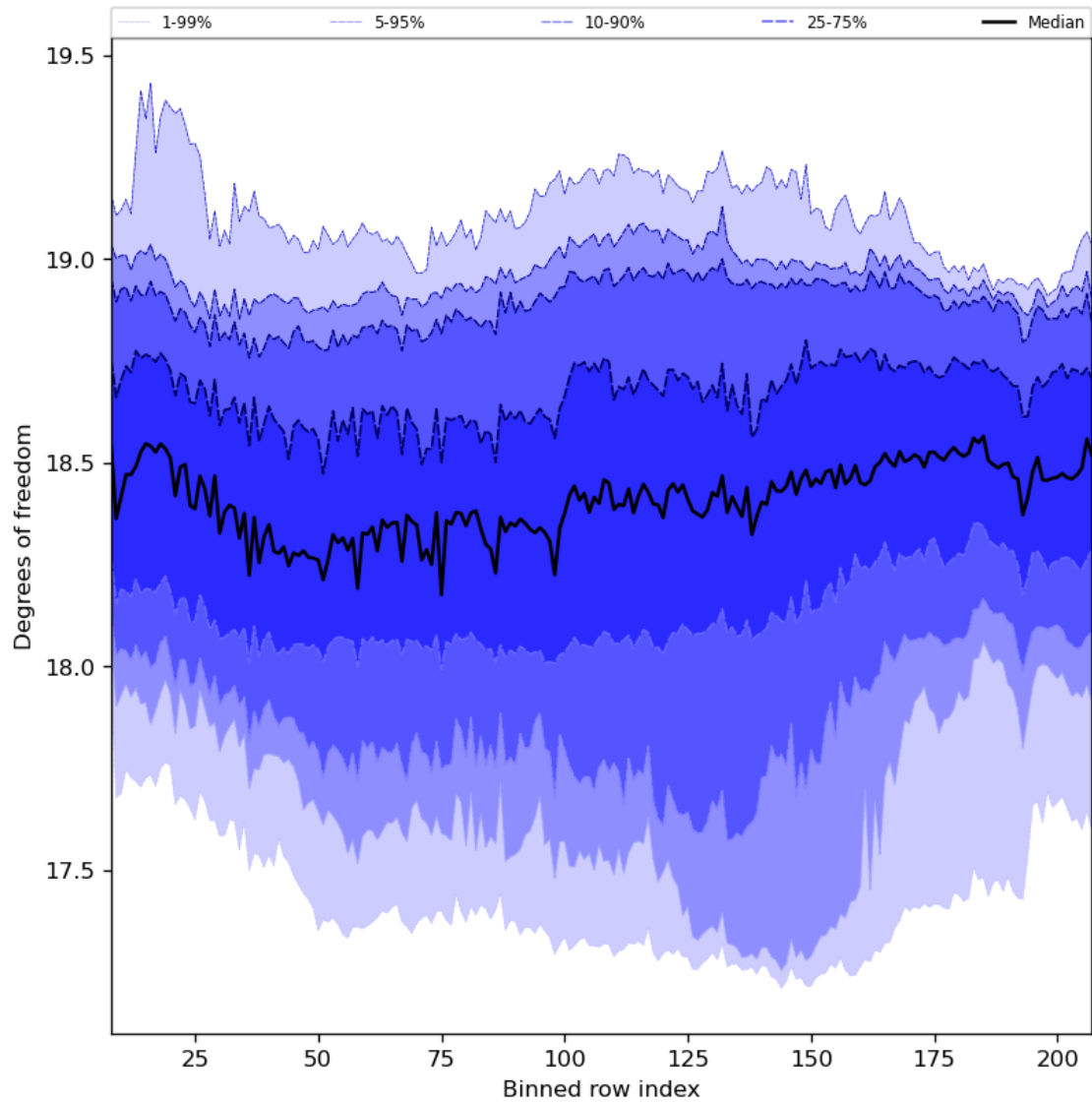
Figure 41: Along track statistics of “Degrees of freedom” for 2023-09-17 to 2023-09-19
