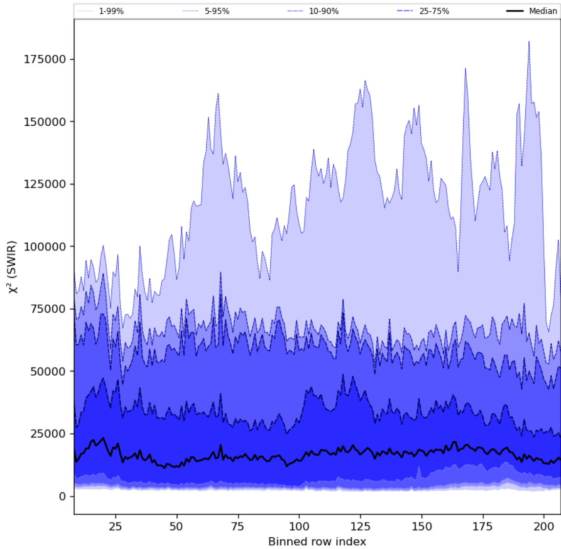
Figure 39: Along track statistics of “ \chi^2 (SWIR)” for 2023-09-17 to 2023-09-19
