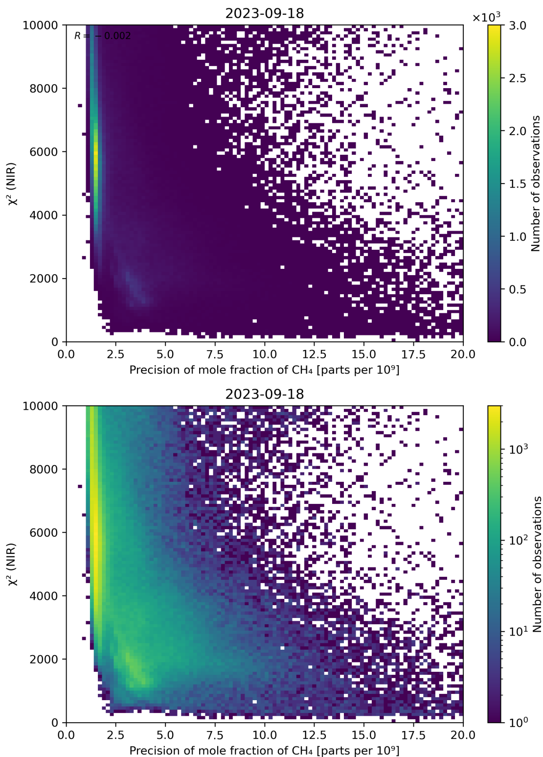
Figure 78: Scatter density plot of “Precision of mole fraction of CH 4 ” against “ \chi^2 (NIR)” for 2023-09-17 to 2023-09-19.
