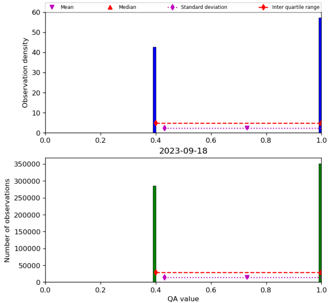
Figure 22: Histogram of “QA value” for 2023-09-17 to 2023-09-19
