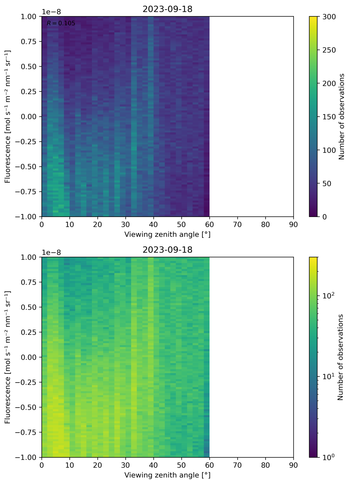
Figure 108: Scatter density plot of “Viewing zenith angle” against “Fluorescence” for 2023-09-17 to 2023-09-19.
