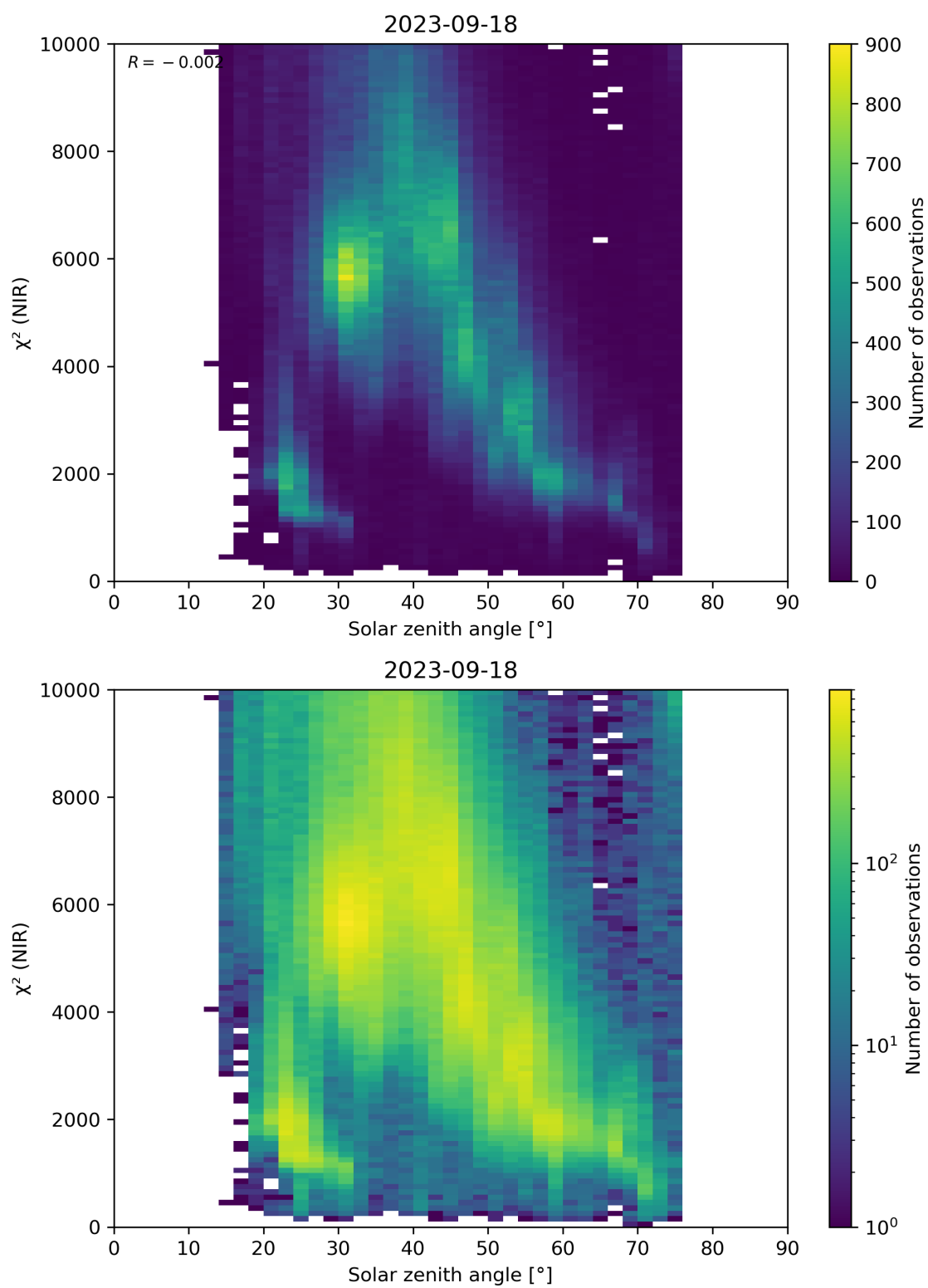
Figure 94: Scatter density plot of “Solar zenith angle” against “ \chi^2 (NIR)” for 2023-09-17 to 2023-09-19.
