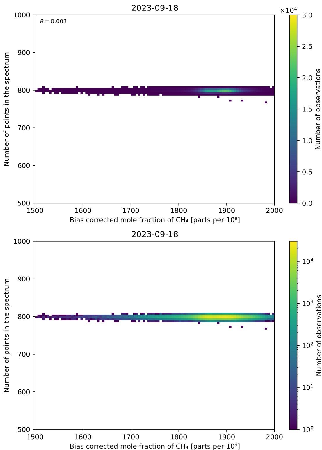
Figure 68: Scatter density plot of “Bias corrected mole fraction of CH 4 ” against “Number of points in the spectrum” for 2023-09-17 to 2023-09-19.
