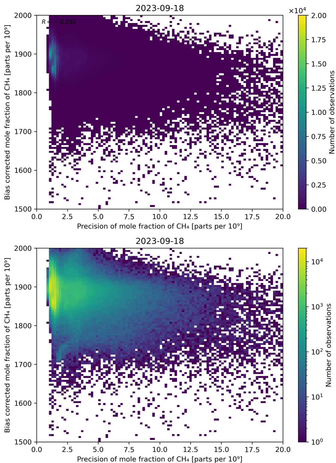
Figure 82: Scatter density plot of “Precision of mole fraction of CH 4 ” against “Bias corrected mole fraction of CH 4 ” for 2023-09-17 to 2023-09-19.
