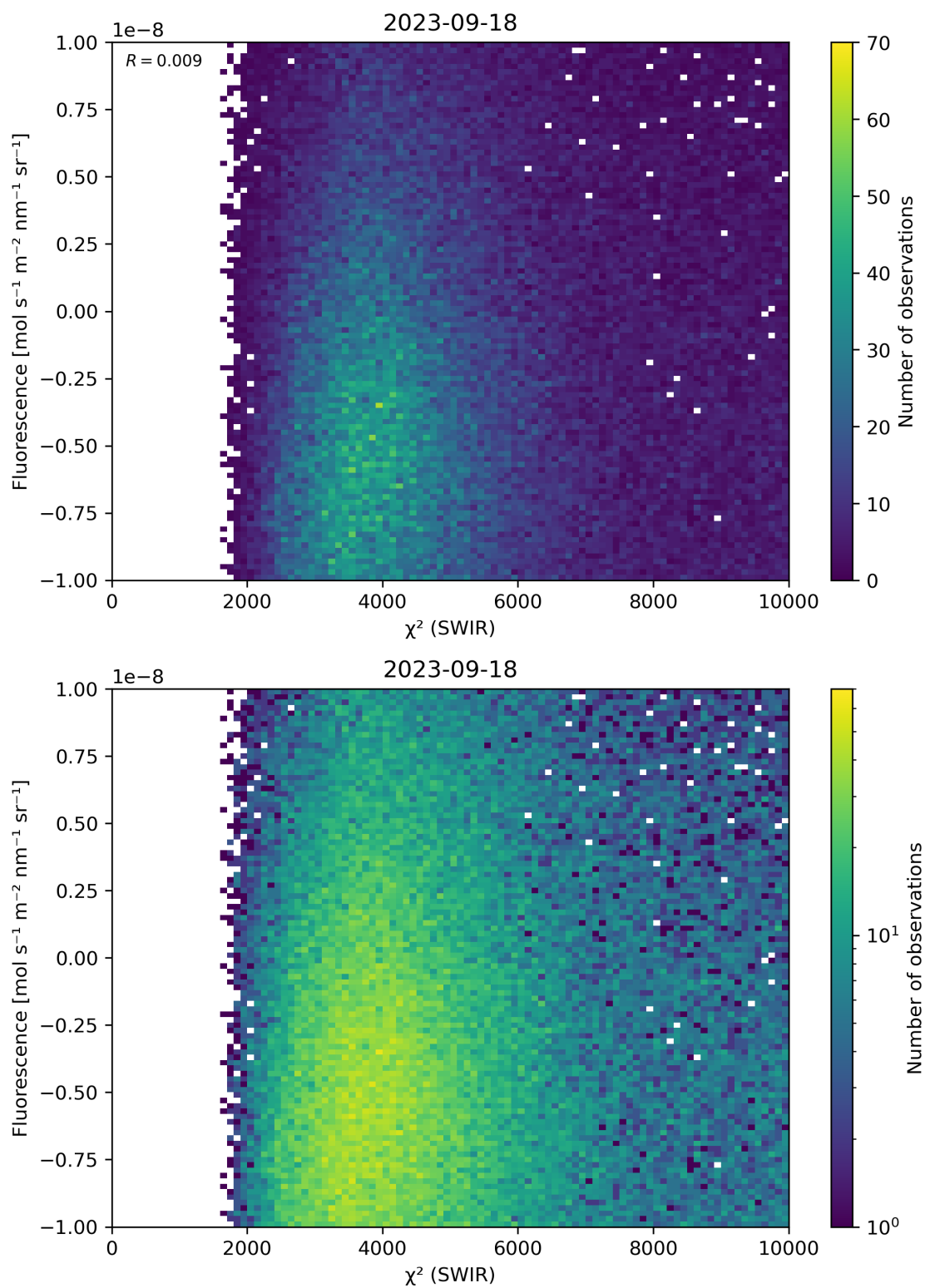
Figure 49: Scatter density plot of “ \chi^2 (SWIR)” against “Fluorescence” for 2023-09-17 to 2023-09-19.
