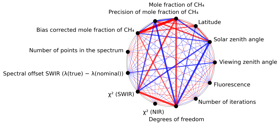
Figure 1: Map of correlation graph for 2023-09-17 to 2023-09-19.
