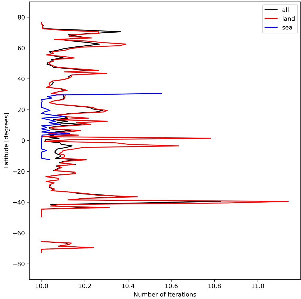
Figure 20: Zonal average of “Number of iterations” for 2023-09-17 to 2023-09-19.
