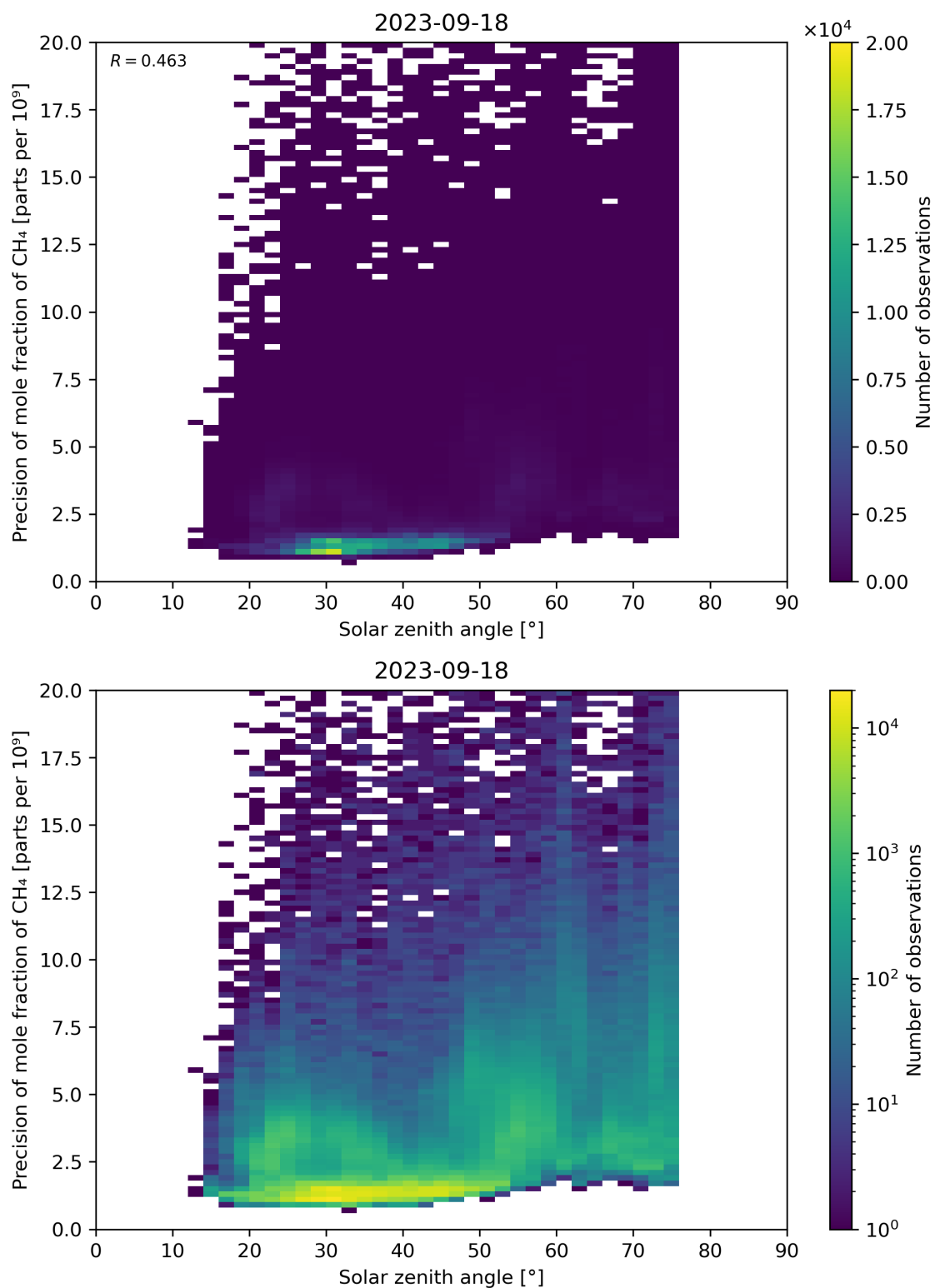
Figure 101: Scatter density plot of “Solar zenith angle” against “Precision of mole fraction of CH 4 ” for 2023-09-17 to 2023-09-19.
