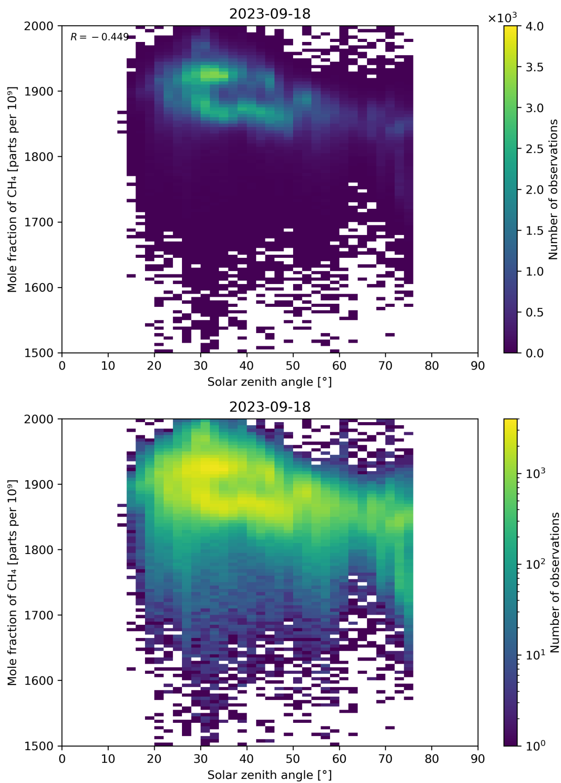
Figure 99: Scatter density plot of “Solar zenith angle” against “Mole fraction of \text{CH}_4 ” for 2023-09-17 to 2023-09-19.
