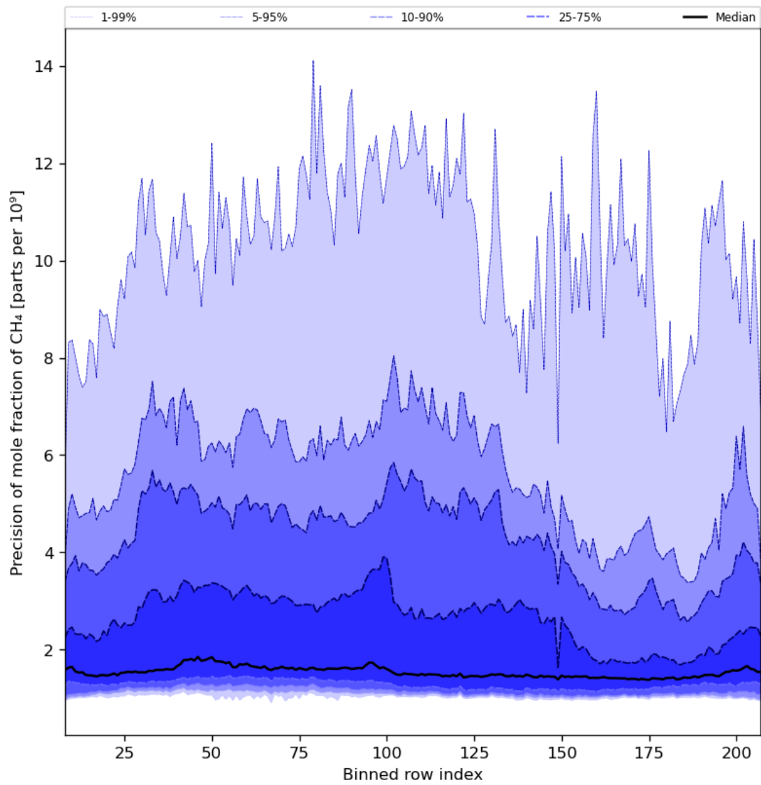
Figure 35: Along track statistics of “Precision of mole fraction of CH 4 ” for 2023-09-17 to 2023-09-19
