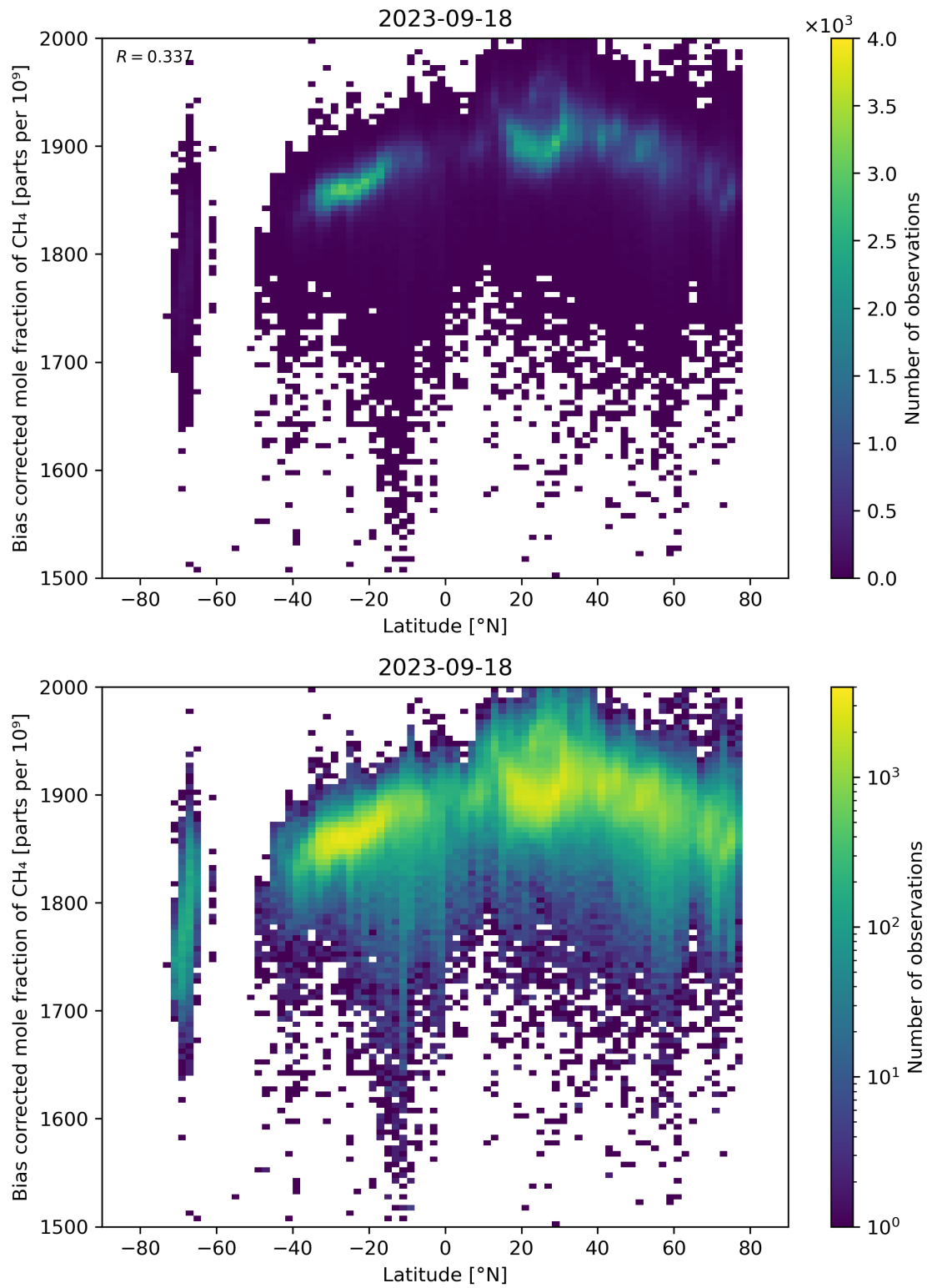
Figure 58: Scatter density plot of “Latitude” against “Bias corrected mole fraction of CH 4 ” for 2023-09-17 to 2023-09-19.
