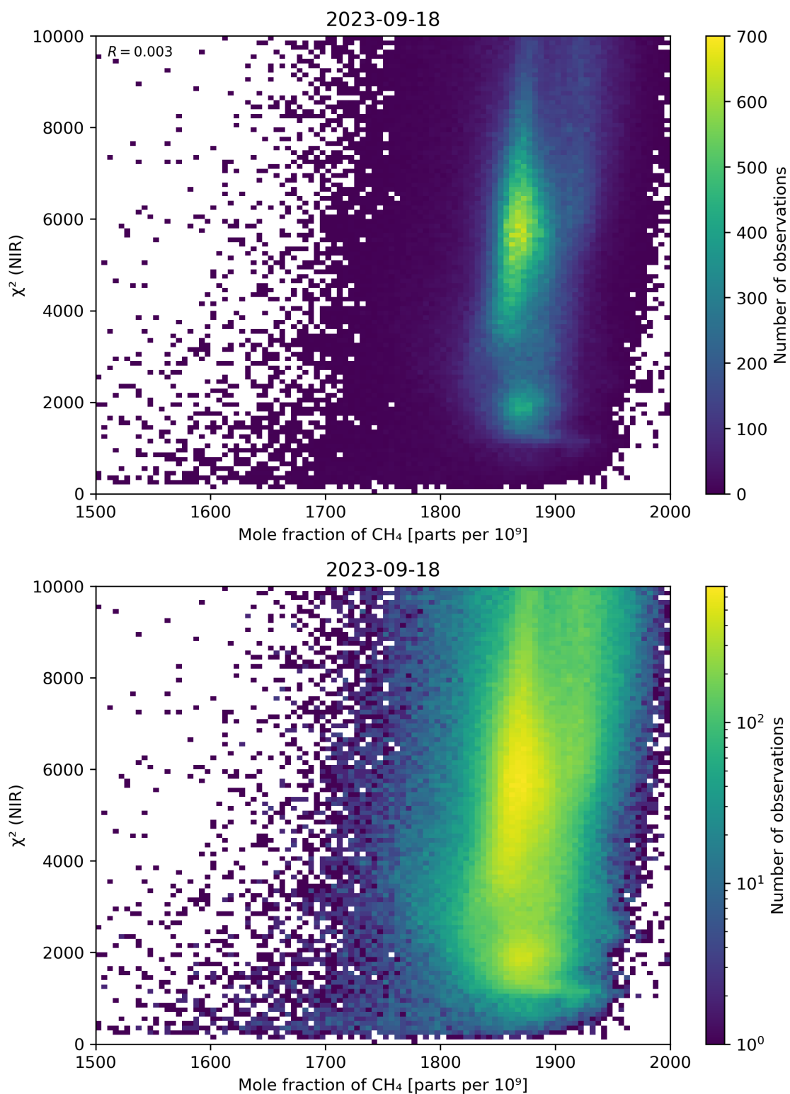
Figure 70: Scatter density plot of “Mole fraction of CH 4 ” against “ \chi^2 (NIR)” for 2023-09-17 to 2023-09-19.
