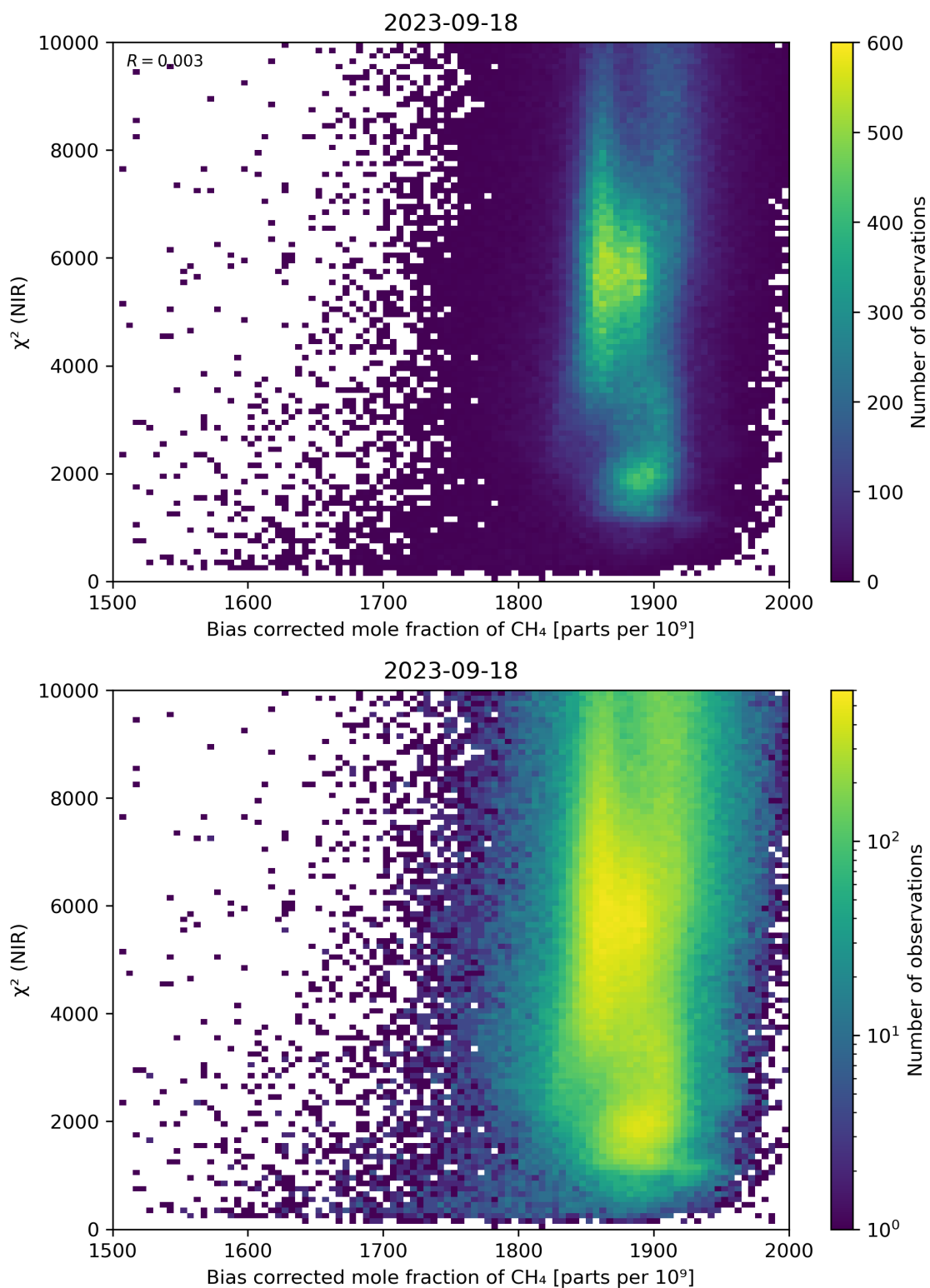
Figure 63: Scatter density plot of “Bias corrected mole fraction of CH 4 ” against “ \chi^2 (NIR)” for 2023-09-17 to 2023-09-19.
