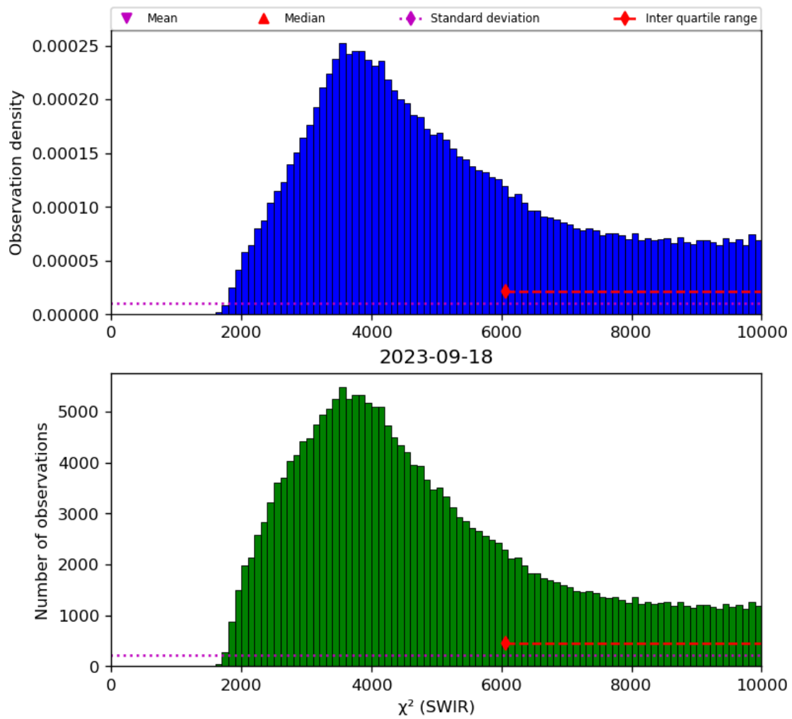
Figure 28: Histogram of “ \chi^2 (SWIR)” for 2023-09-17 to 2023-09-19
