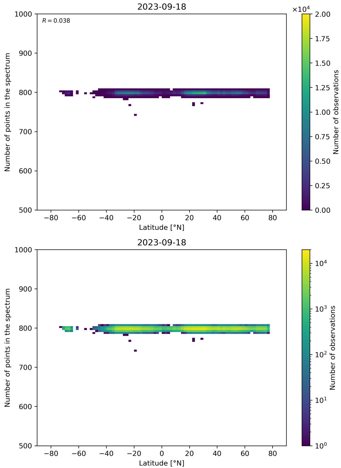
Figure 61: Scatter density plot of “Latitude” against “Number of points in the spectrum” for 2023-09-17 to 2023-09-19.
