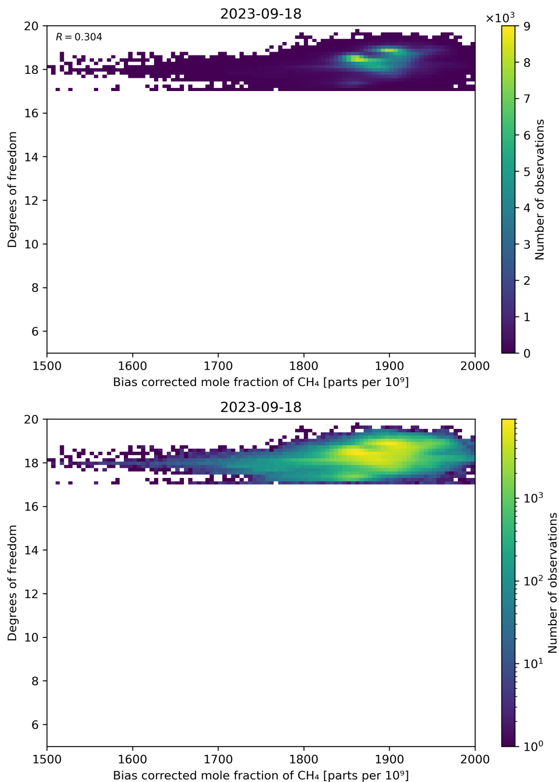
Figure 65: Scatter density plot of “Bias corrected mole fraction of CH 4 ” against “Degrees of freedom” for 2023-09-17 to 2023-09-19.
