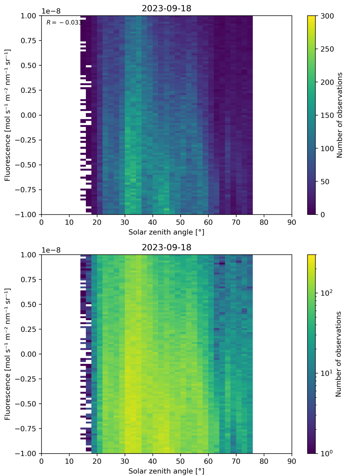
Figure 97: Scatter density plot of “Solar zenith angle” against “Fluorescence” for 2023-09-17 to 2023-09-19.
