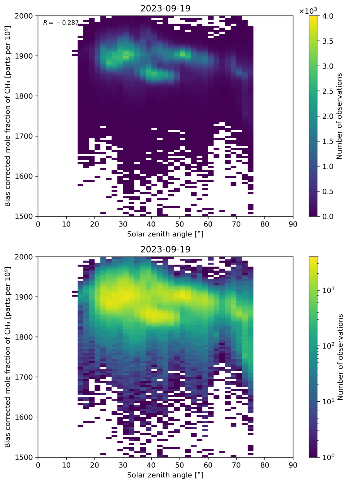
Figure 100: Scatter density plot of “Solar zenith angle” against “Bias corrected mole fraction of \text{CH}_4 ” for 2023-09-18 to 2023-09-20.
