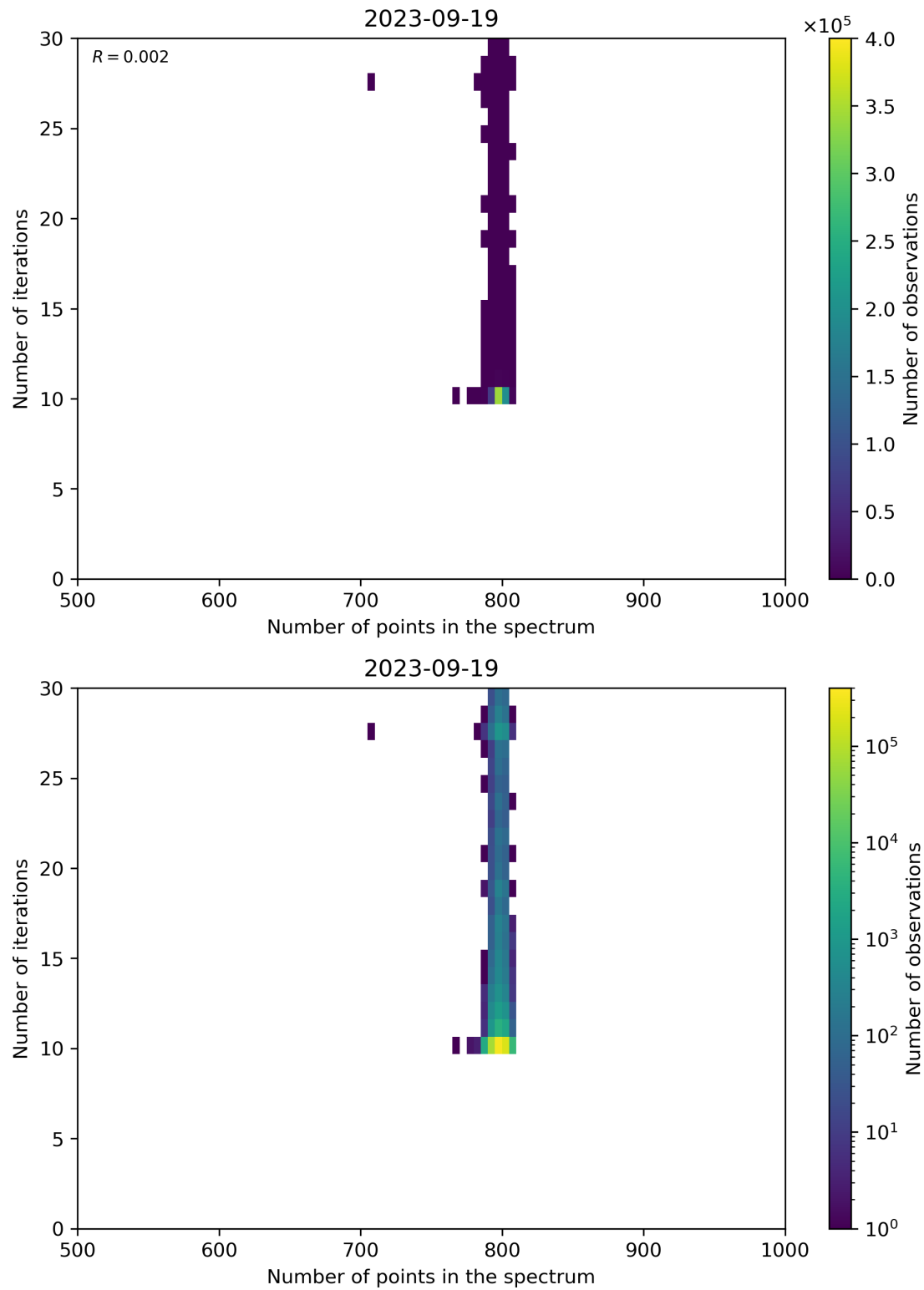
Figure 92: Scatter density plot of “Number of points in the spectrum” against “Number of iterations” for 2023-09-18 to 2023-09-20.
