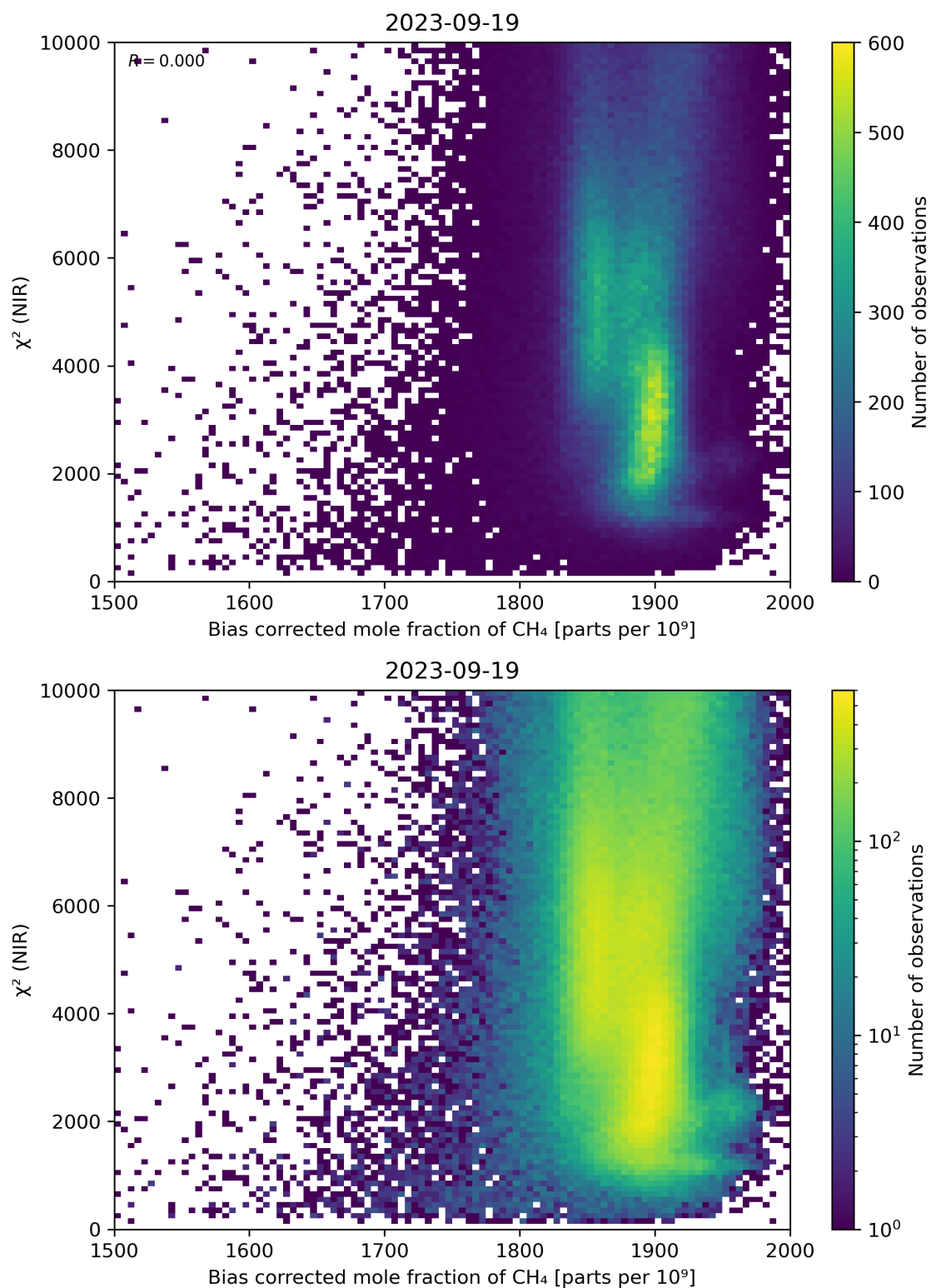
Figure 63: Scatter density plot of “Bias corrected mole fraction of CH 4 ” against “ \chi^2 (NIR)” for 2023-09-18 to 2023-09-20.
