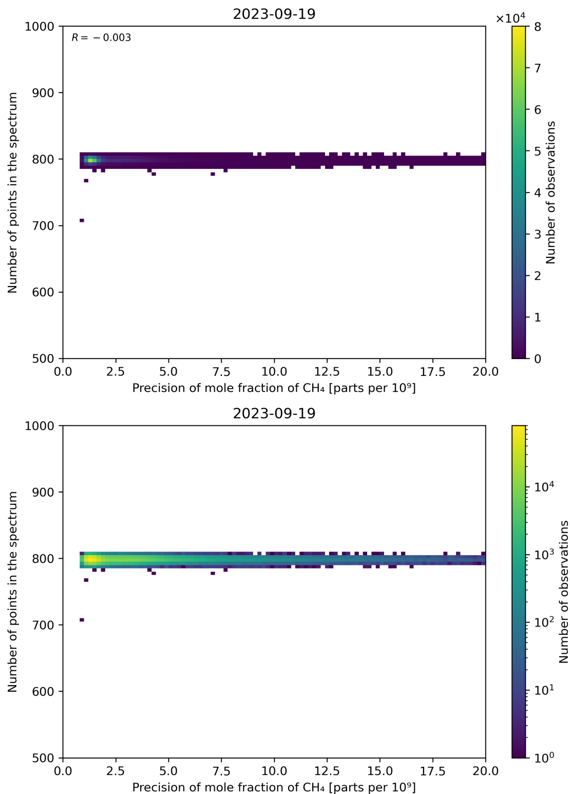
Figure 84: Scatter density plot of “Precision of mole fraction of CH 4 ” against “Number of points in the spectrum” for 2023-09-18 to 2023-09-20.
