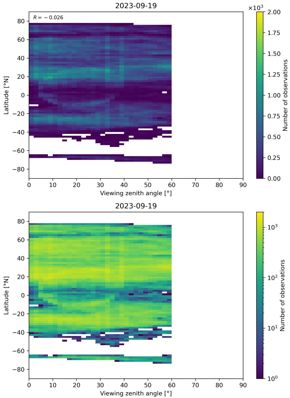
Figure 109: Scatter density plot of “Viewing zenith angle” against “Latitude” for 2023-09-18 to 2023-09-20.
