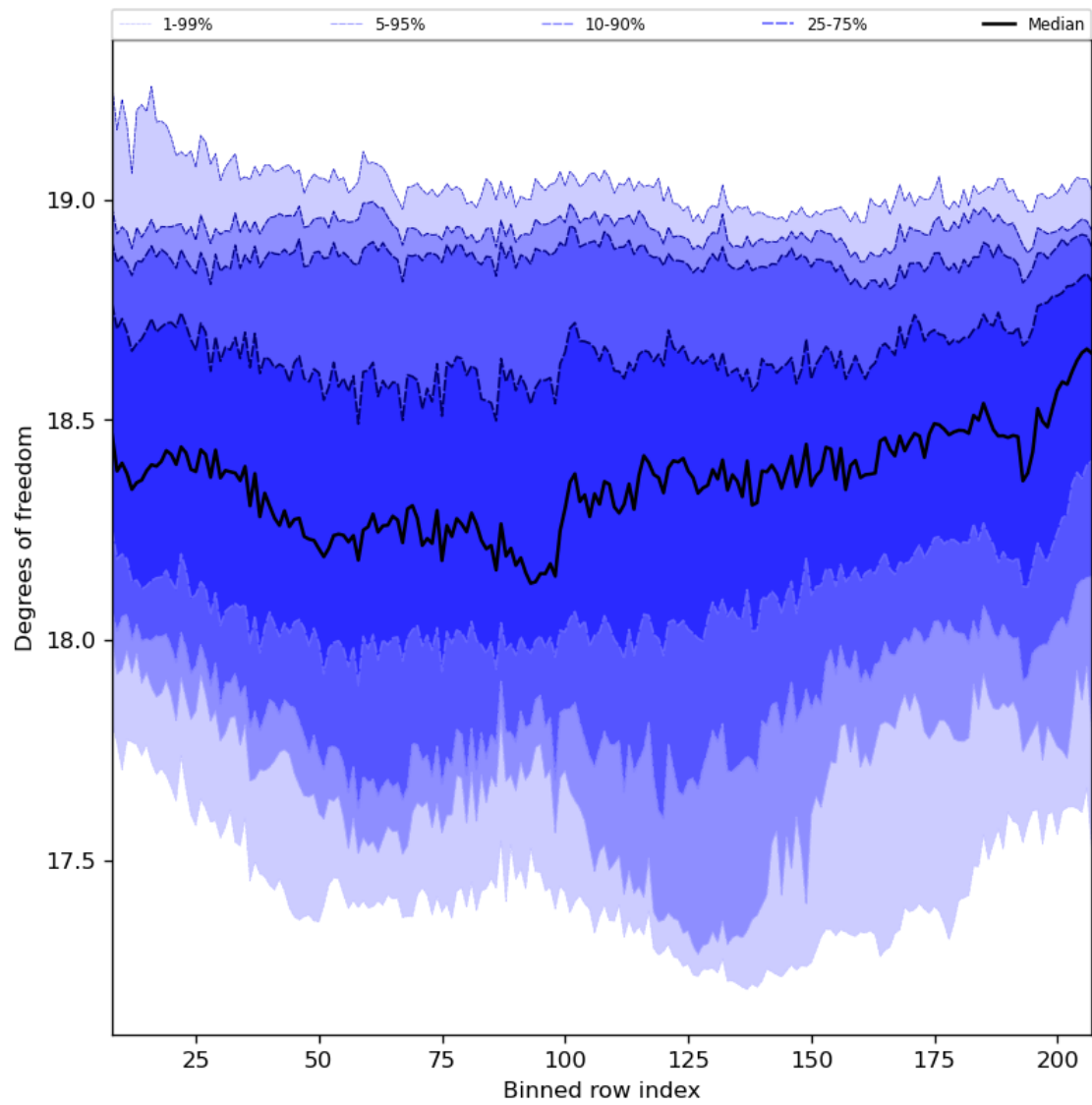
Figure 41: Along track statistics of “Degrees of freedom” for 2023-09-18 to 2023-09-20
