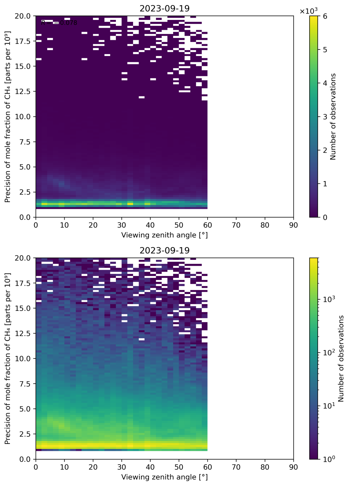
Figure 112: Scatter density plot of “Viewing zenith angle” against “Precision of mole fraction of \text{CH}_4 ” for 2023-09-18 to 2023-09-20.
