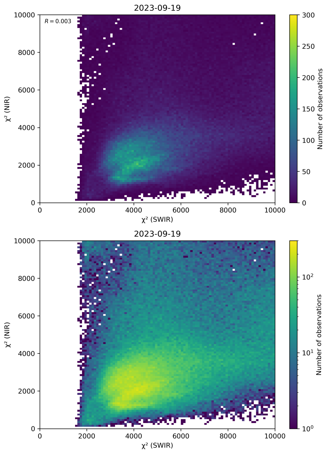
Figure 47: Scatter density plot of “ \chi^2 (SWIR)” against “ \chi^2 (NIR)” for 2023-09-18 to 2023-09-20.
