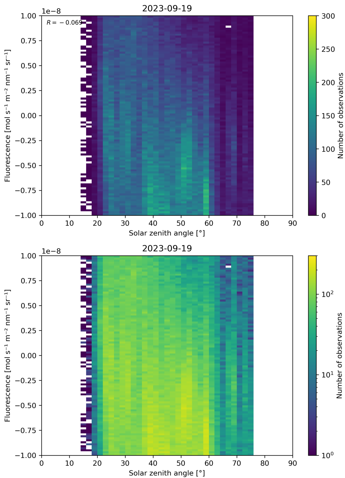
Figure 97: Scatter density plot of “Solar zenith angle” against “Fluorescence” for 2023-09-18 to 2023-09-20.
