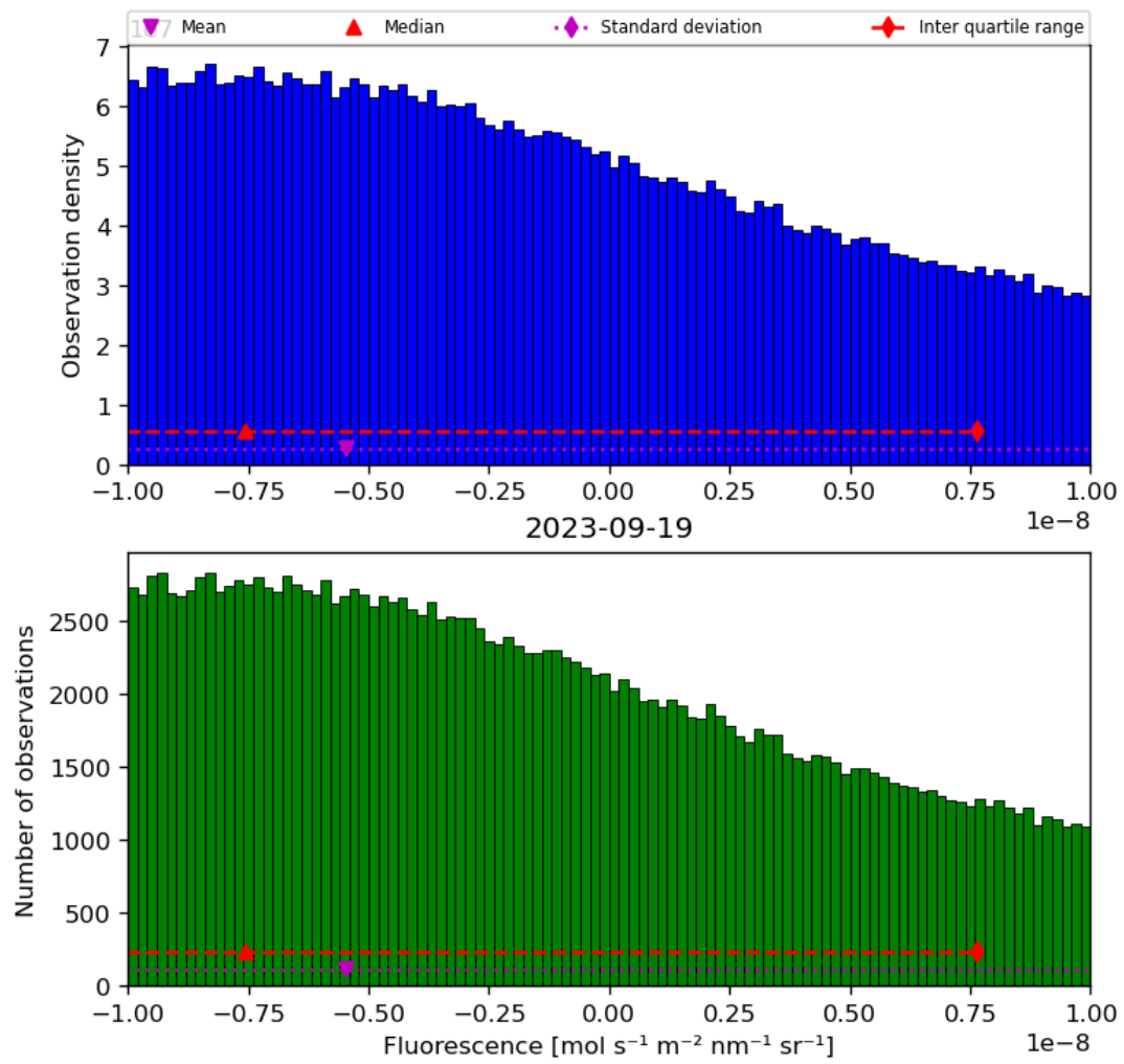
Figure 32: Histogram of “Fluorescence” for 2023-09-18 to 2023-09-20
