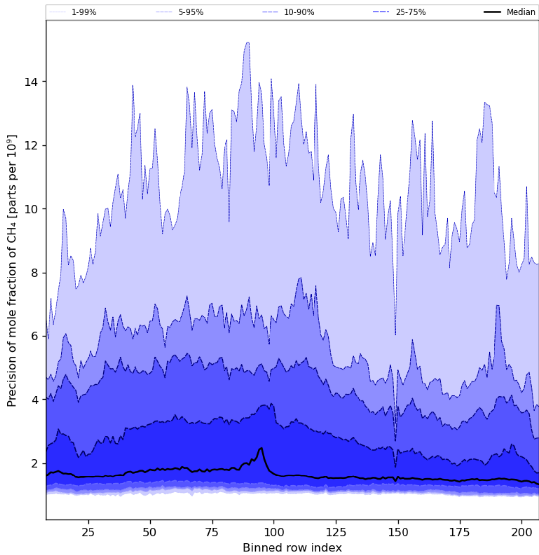
Figure 35: Along track statistics of “Precision of mole fraction of CH 4 ” for 2023-09-18 to 2023-09-20
