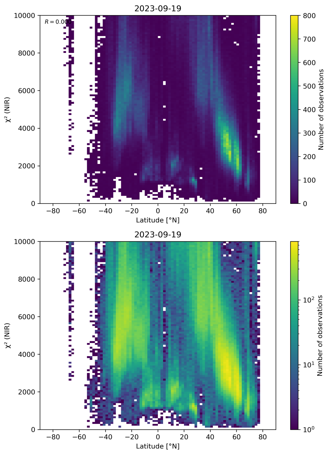
Figure 53: Scatter density plot of “Latitude” against “ \chi^2 (NIR)” for 2023-09-18 to 2023-09-20.
