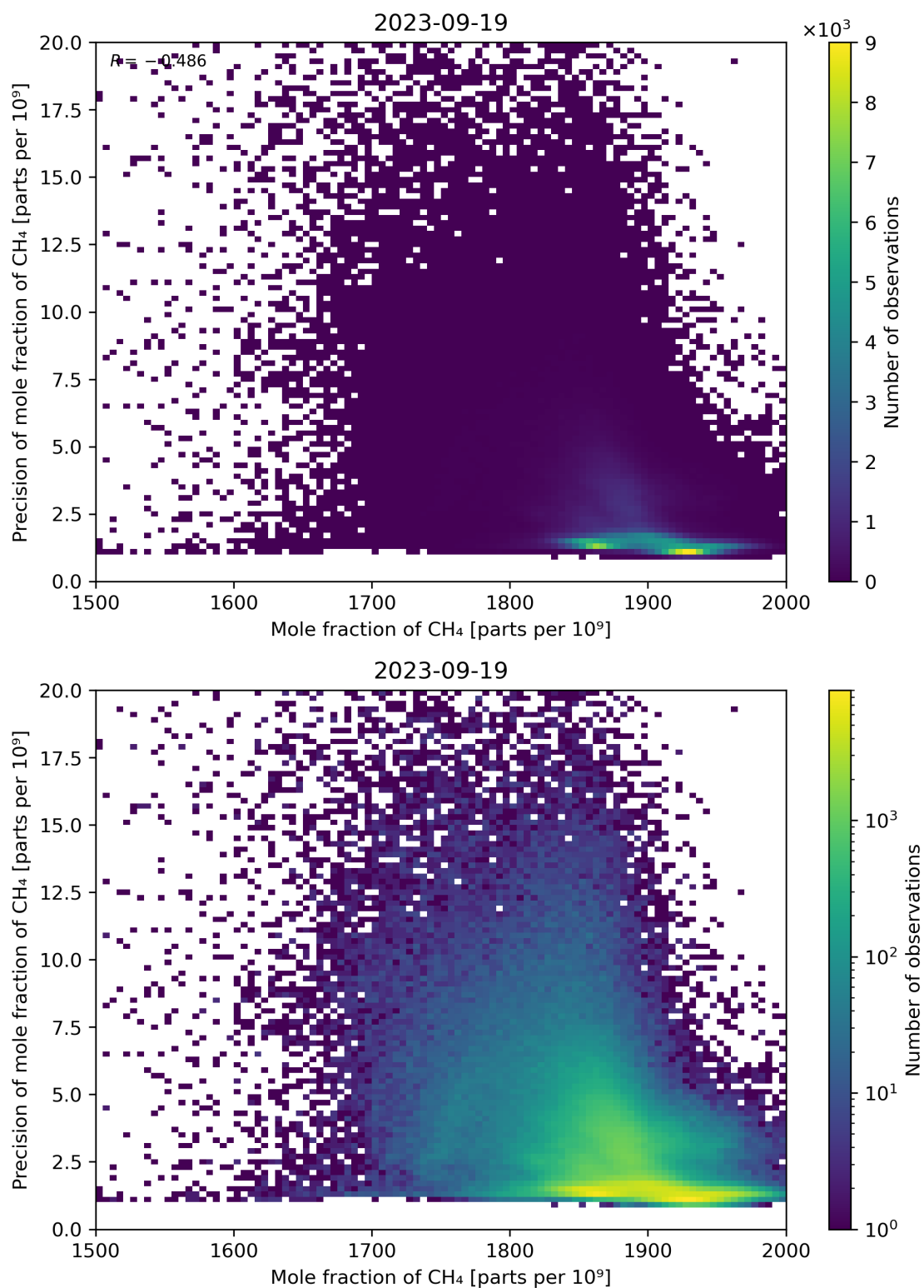
Figure 75: Scatter density plot of “Mole fraction of CH 4 ” against “Precision of mole fraction of CH 4 ” for 2023-09-18 to 2023-09-20.
