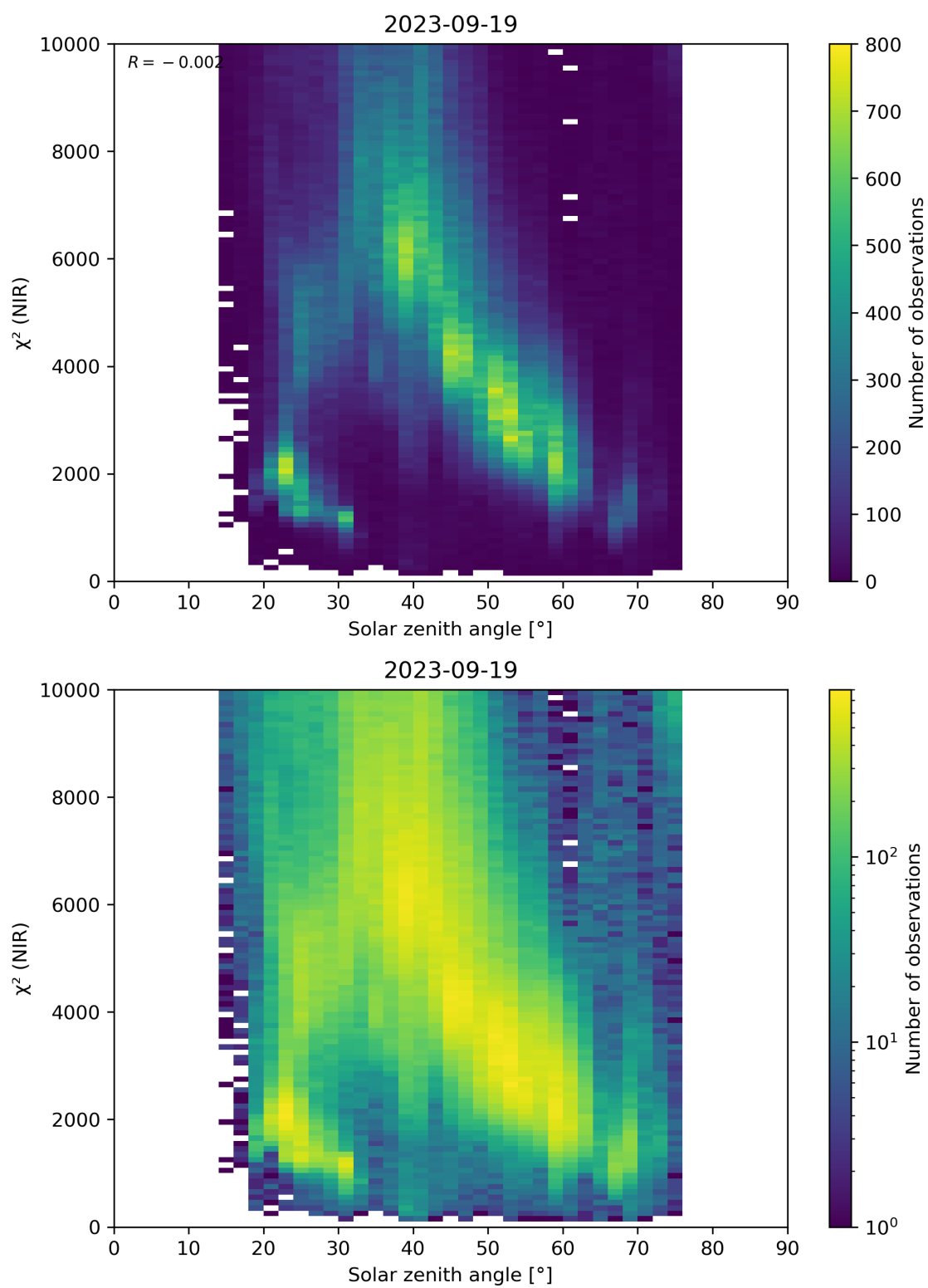
Figure 94: Scatter density plot of “Solar zenith angle” against “ \chi^2 (NIR)” for 2023-09-18 to 2023-09-20.
