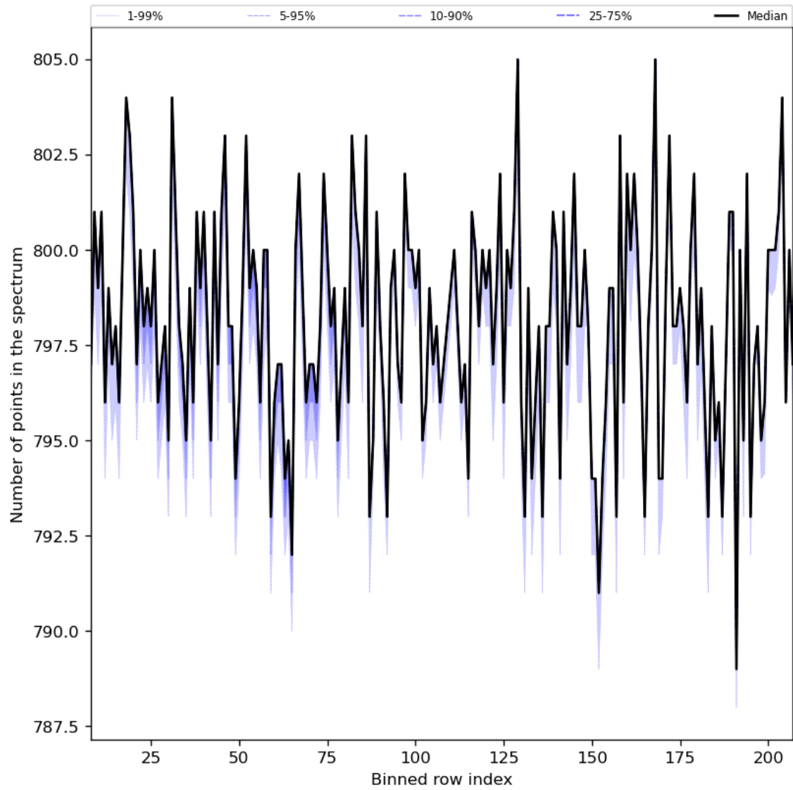
Figure 37: Along track statistics of “Number of points in the spectrum” for 2023-09-18 to 2023-09-20
