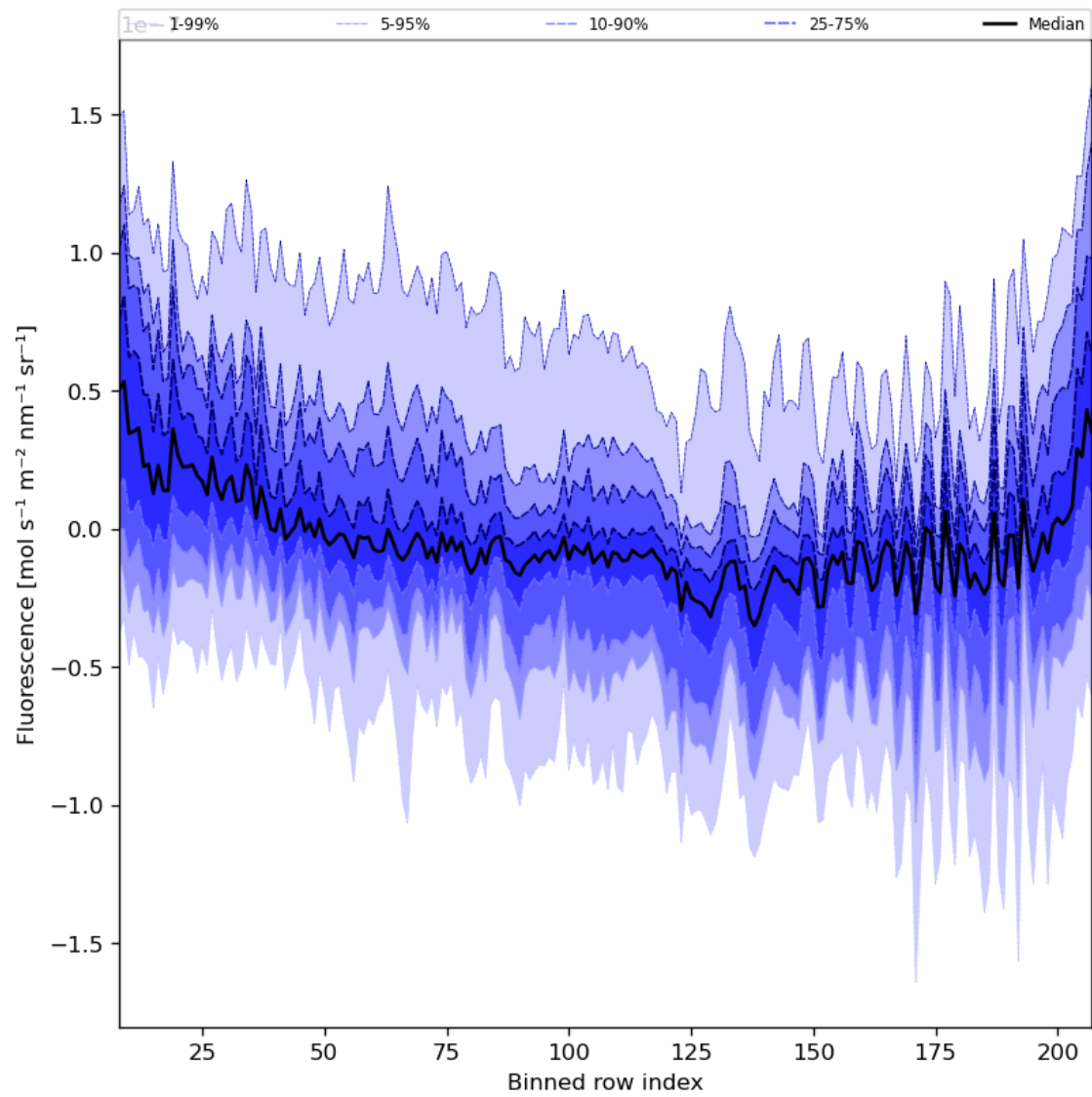
Figure 43: Along track statistics of “Fluorescence” for 2023-09-18 to 2023-09-20
