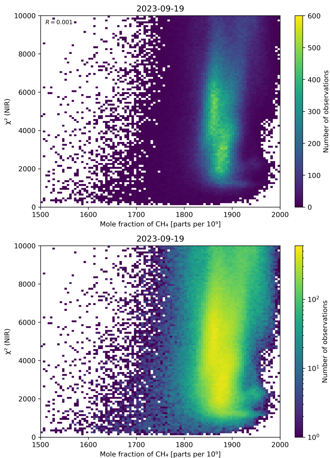
Figure 70: Scatter density plot of “Mole fraction of \text{CH}_4 ” against “ \chi^2 (NIR)” for 2023-09-18 to 2023-09-20.
