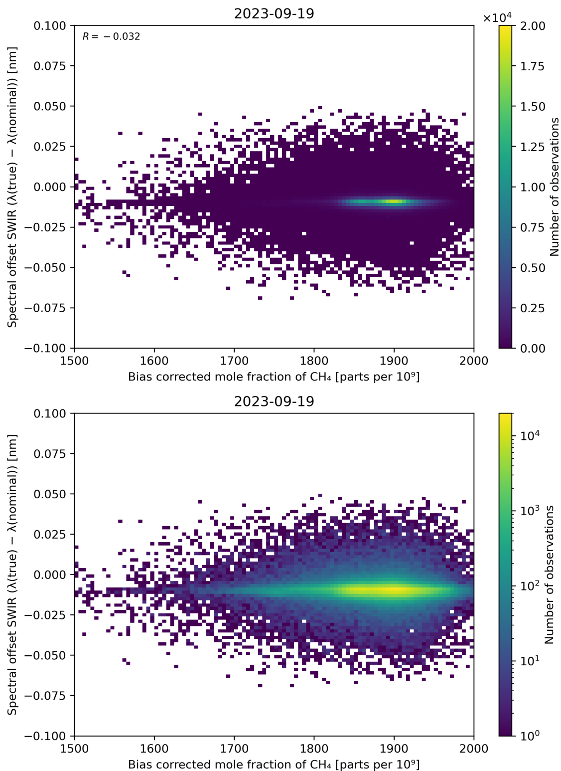
Figure 69: Scatter density plot of “Bias corrected mole fraction of \text{CH}_4 ” against “Spectral offset SWIR ( \lambda(\text{true}) - \lambda(\text{nominal}) )” for 2023-09-18 to 2023-09-20.
