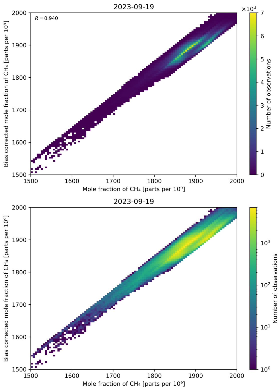
Figure 74: Scatter density plot of “Mole fraction of CH 4 ” against “Bias corrected mole fraction of CH 4 ” for 2023-09-18 to 2023-09-20.
