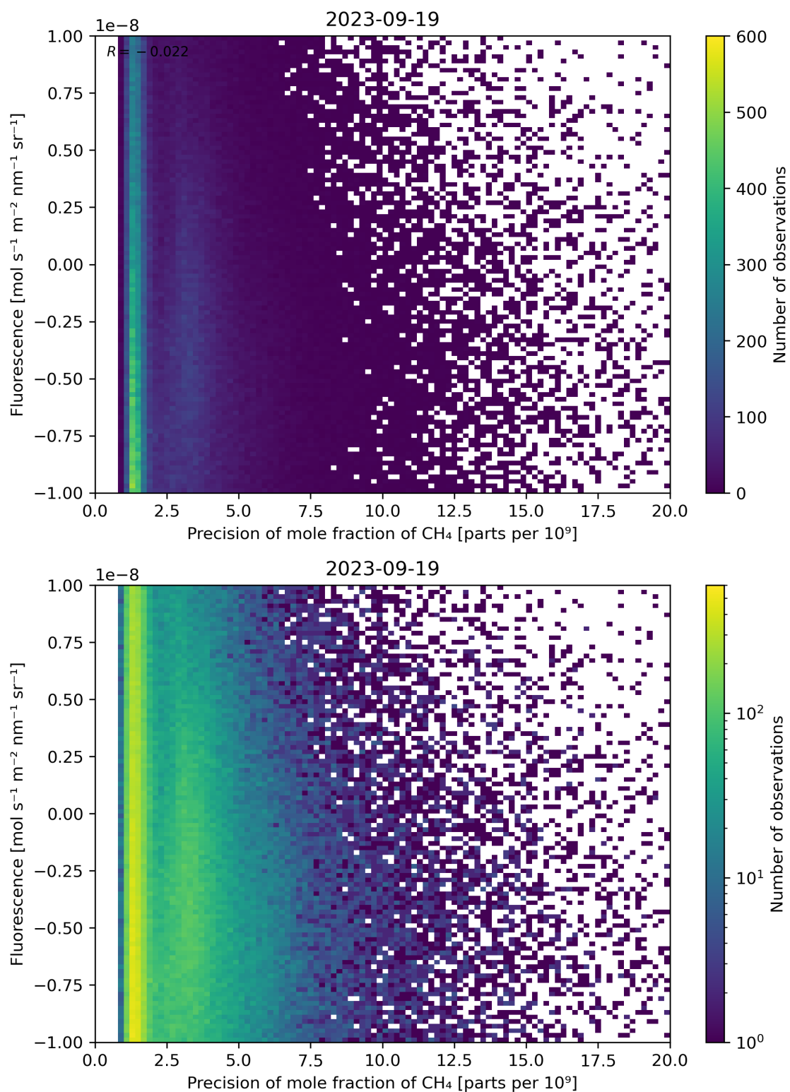
Figure 81: Scatter density plot of “Precision of mole fraction of CH 4 ” against “Fluorescence” for 2023-09-18 to 2023-09-20.
