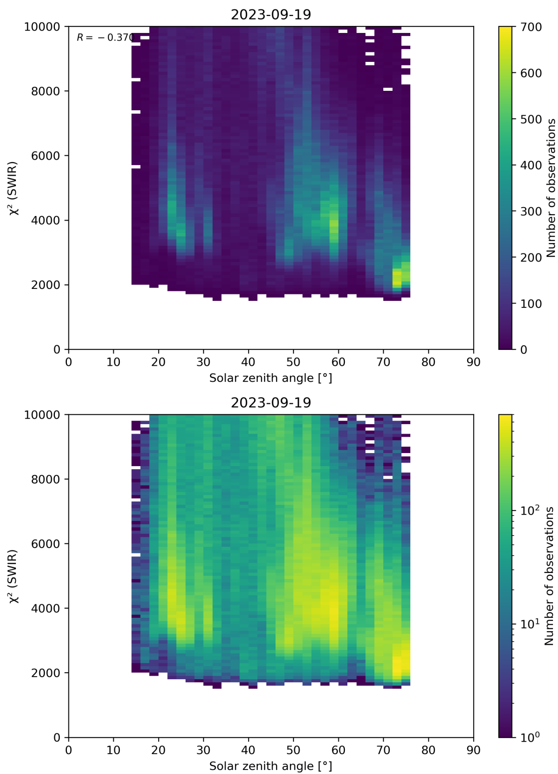
Figure 95: Scatter density plot of “Solar zenith angle” against “ \chi^2 (SWIR)” for 2023-09-18 to 2023-09-20.
