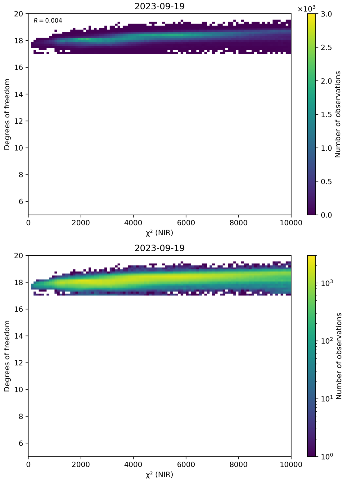
Figure 44: Scatter density plot of “ \chi^2 (NIR)” against “Degrees of freedom” for 2023-09-18 to 2023-09-20.
