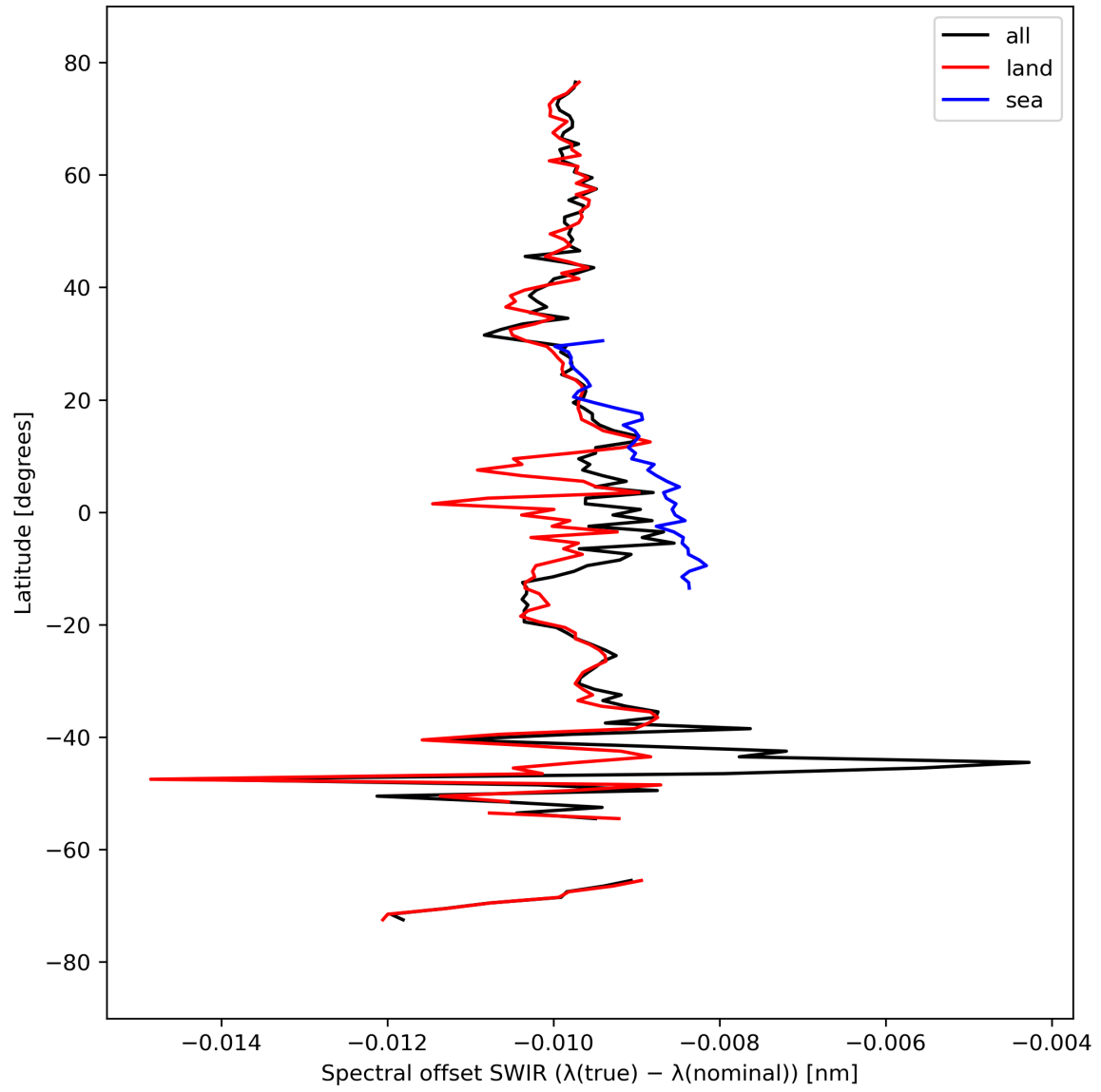
Figure 16: Zonal average of “Spectral offset SWIR ( \lambda(\text{true}) - \lambda(\text{nominal}) )” for 2023-09-18 to 2023-09-20.
