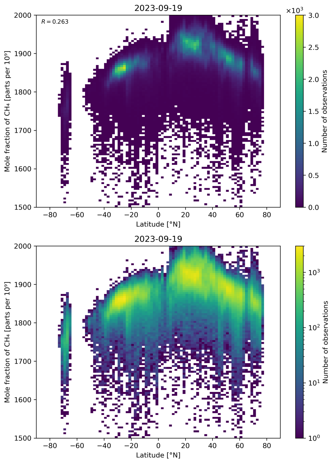
Figure 57: Scatter density plot of “Latitude” against “Mole fraction of \text{CH}_4 ” for 2023-09-18 to 2023-09-20.
