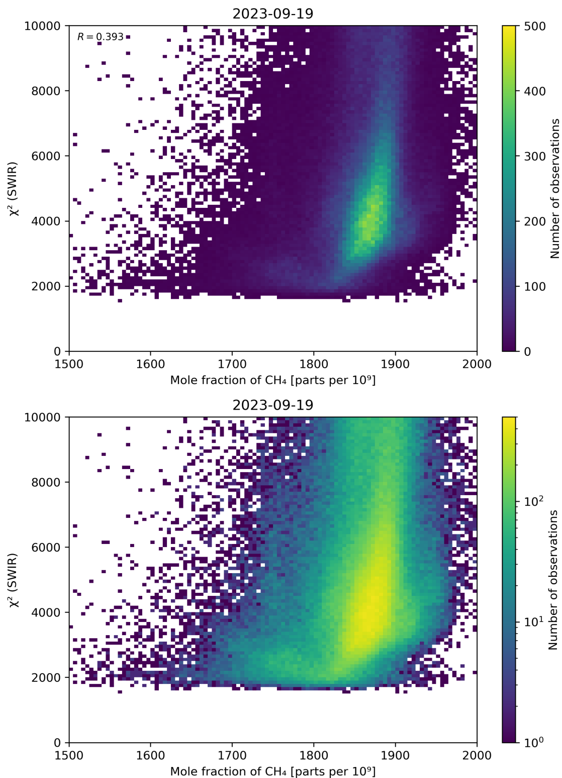
Figure 71: Scatter density plot of “Mole fraction of \text{CH}_4 ” against “ \chi^2 (SWIR)” for 2023-09-18 to 2023-09-20.
