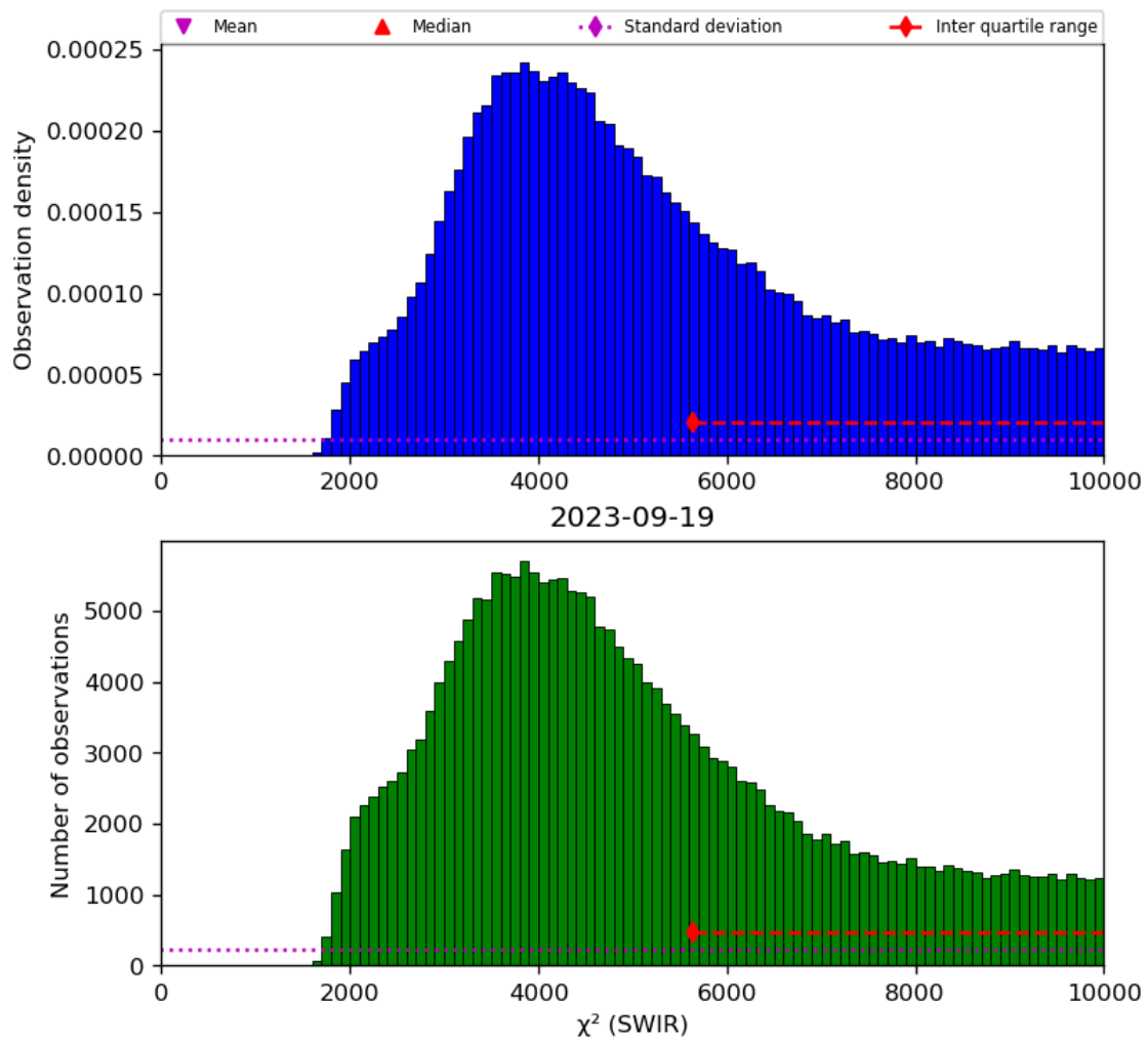
Figure 28: Histogram of " \chi^2 (SWIR)" for 2023-09-18 to 2023-09-20
