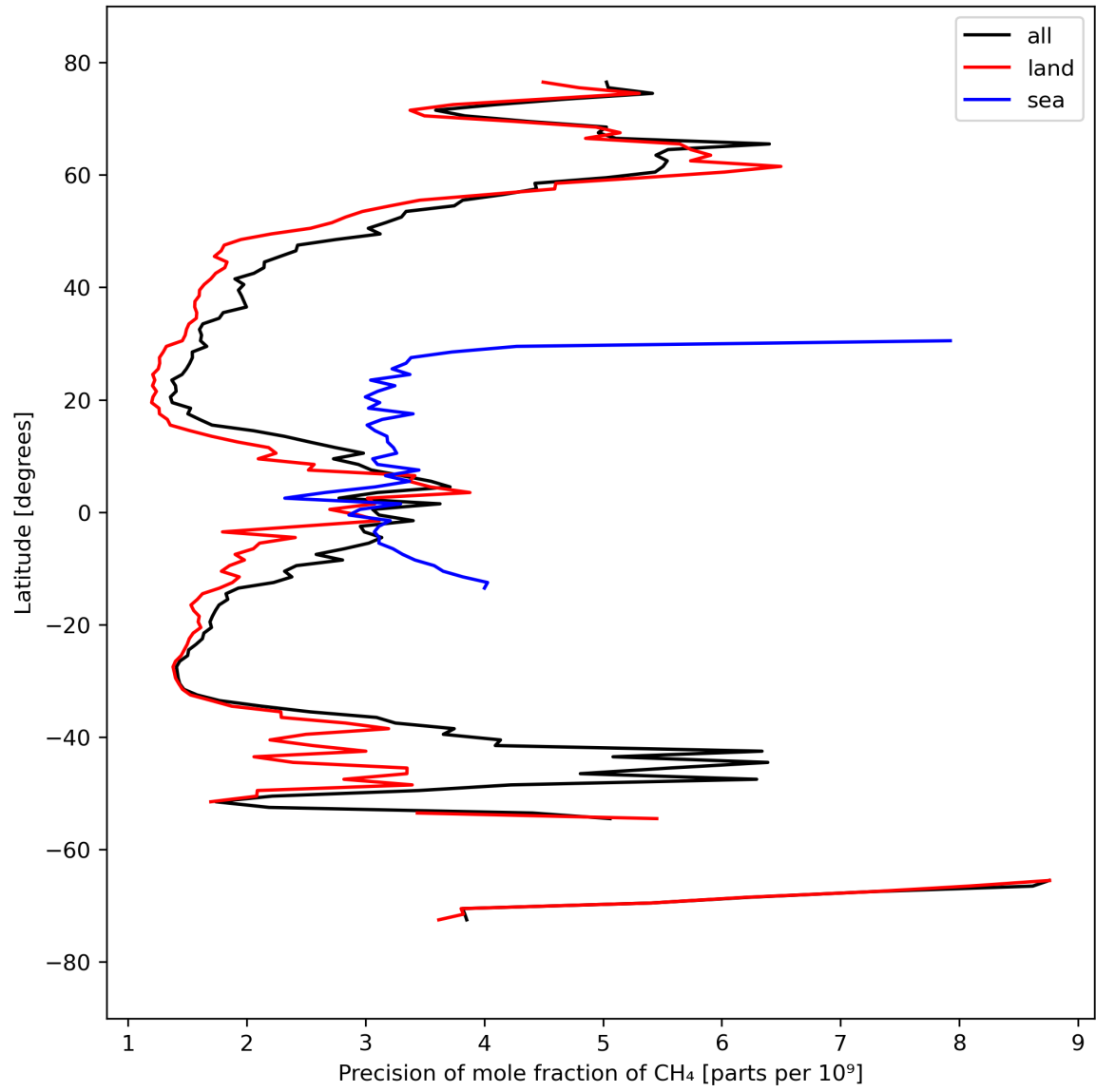
Figure 13: Zonal average of “Precision of mole fraction of CH 4 ” for 2023-09-18 to 2023-09-20.
