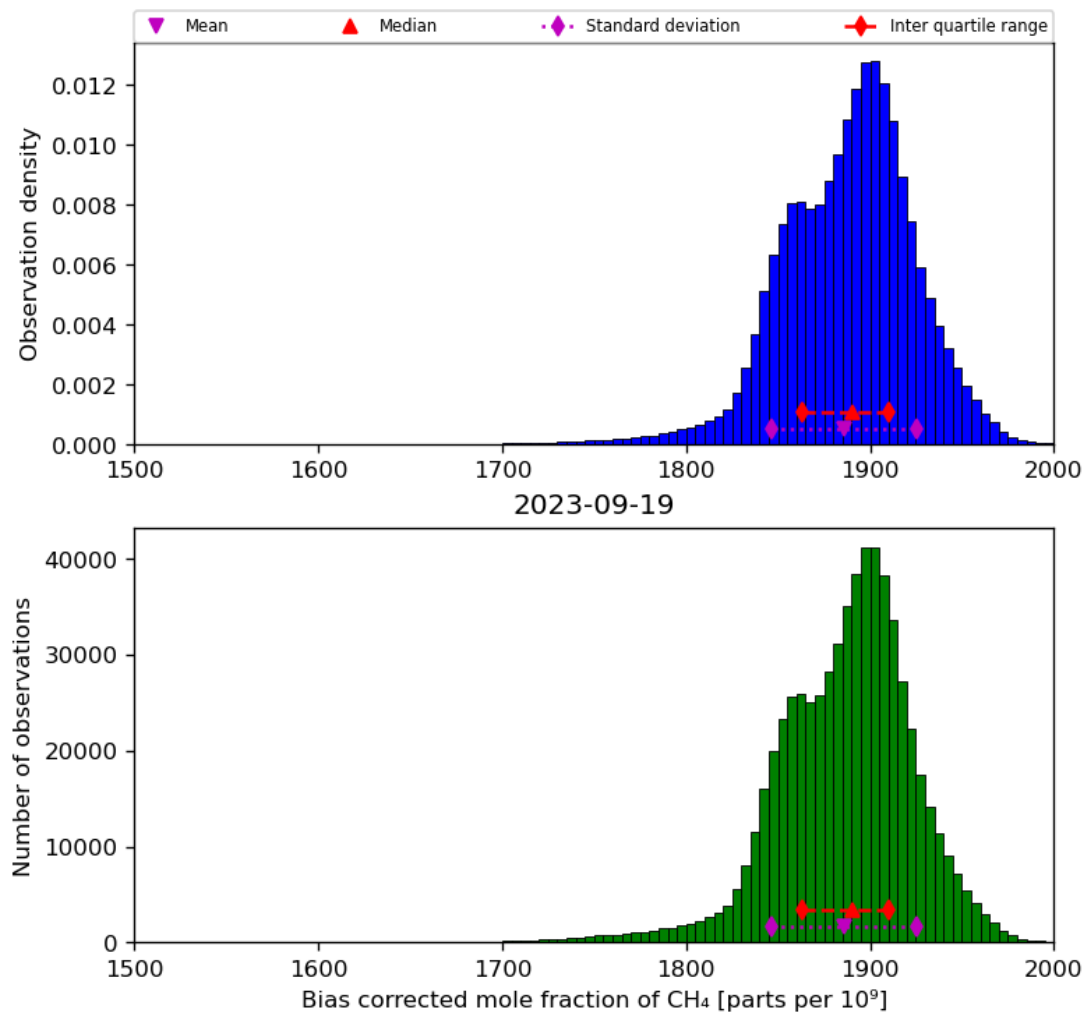
Figure 25: Histogram of “Bias corrected mole fraction of CH 4 ” for 2023-09-18 to 2023-09-20
