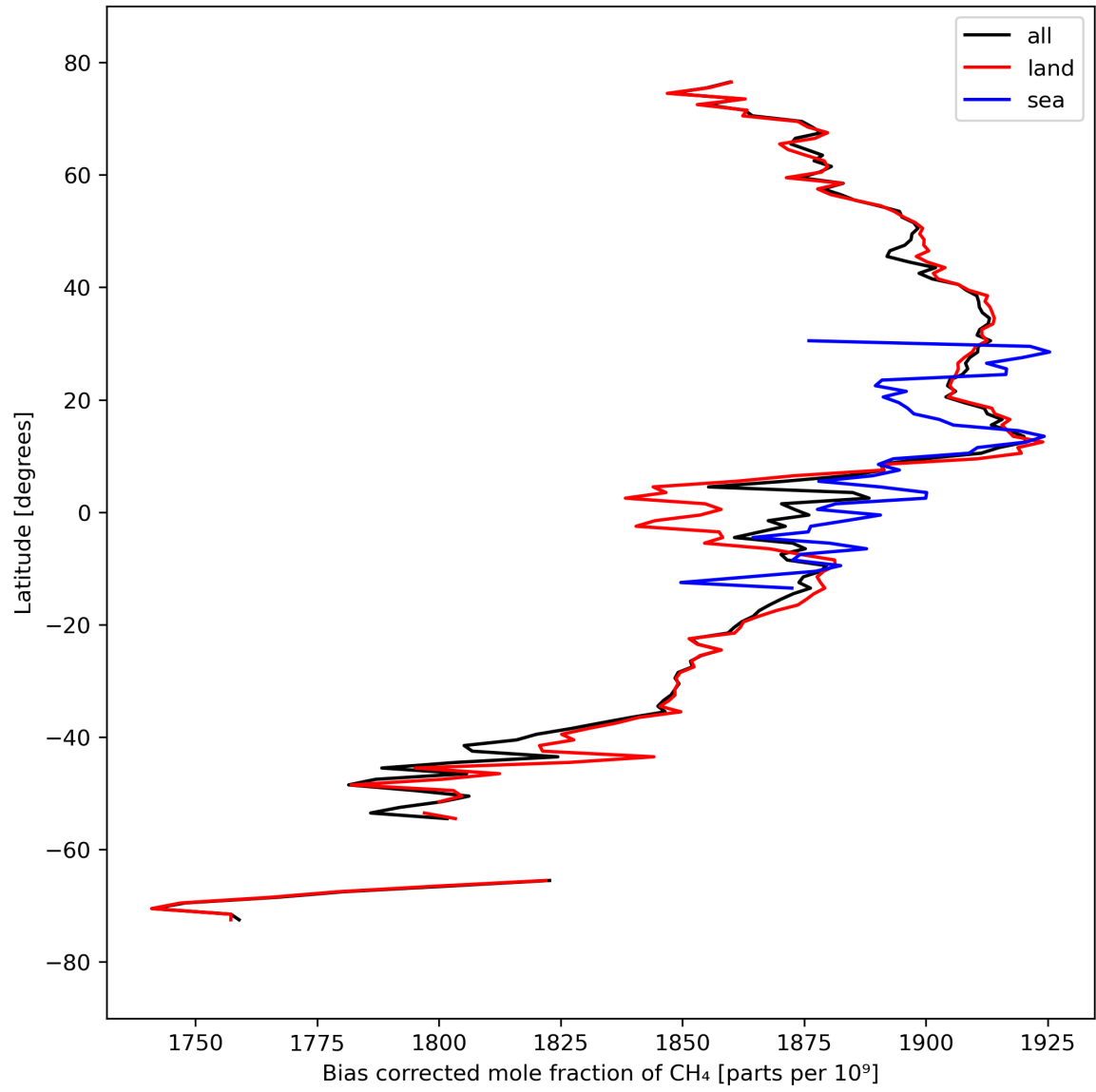
Figure 14: Zonal average of “Bias corrected mole fraction of CH 4 ” for 2023-09-18 to 2023-09-20.
