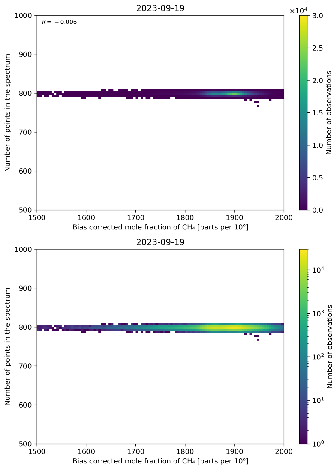
Figure 68: Scatter density plot of “Bias corrected mole fraction of CH 4 ” against “Number of points in the spectrum” for 2023-09-18 to 2023-09-20.
