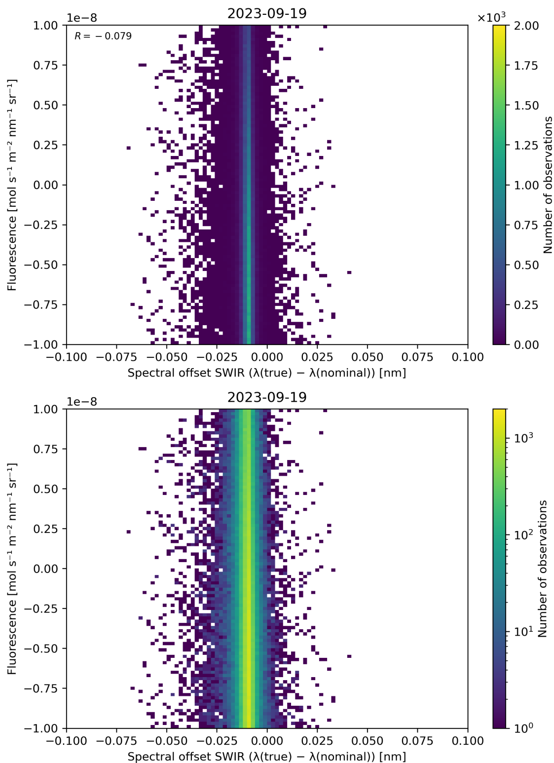
Figure 120: Scatter density plot of “Spectral offset SWIR ( \lambda(\text{true}) - \lambda(\text{nominal}) )” against “Fluorescence” for 2023-09-18 to 2023-09-20.
