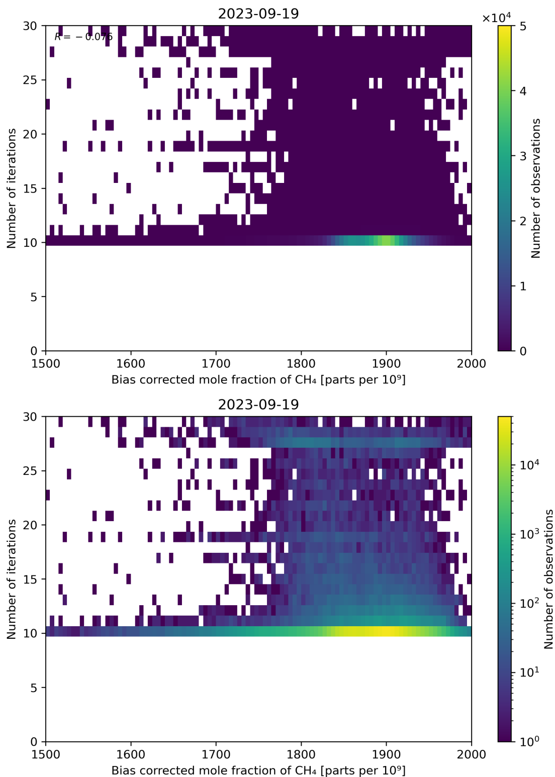
Figure 67: Scatter density plot of “Bias corrected mole fraction of CH 4 ” against “Number of iterations” for 2023-09-18 to 2023-09-20.
