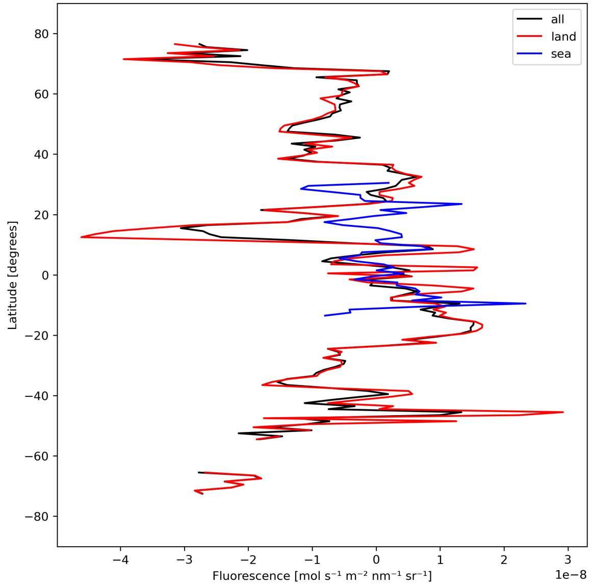
Figure 21: Zonal average of “Fluorescence” for 2023-09-18 to 2023-09-20.
