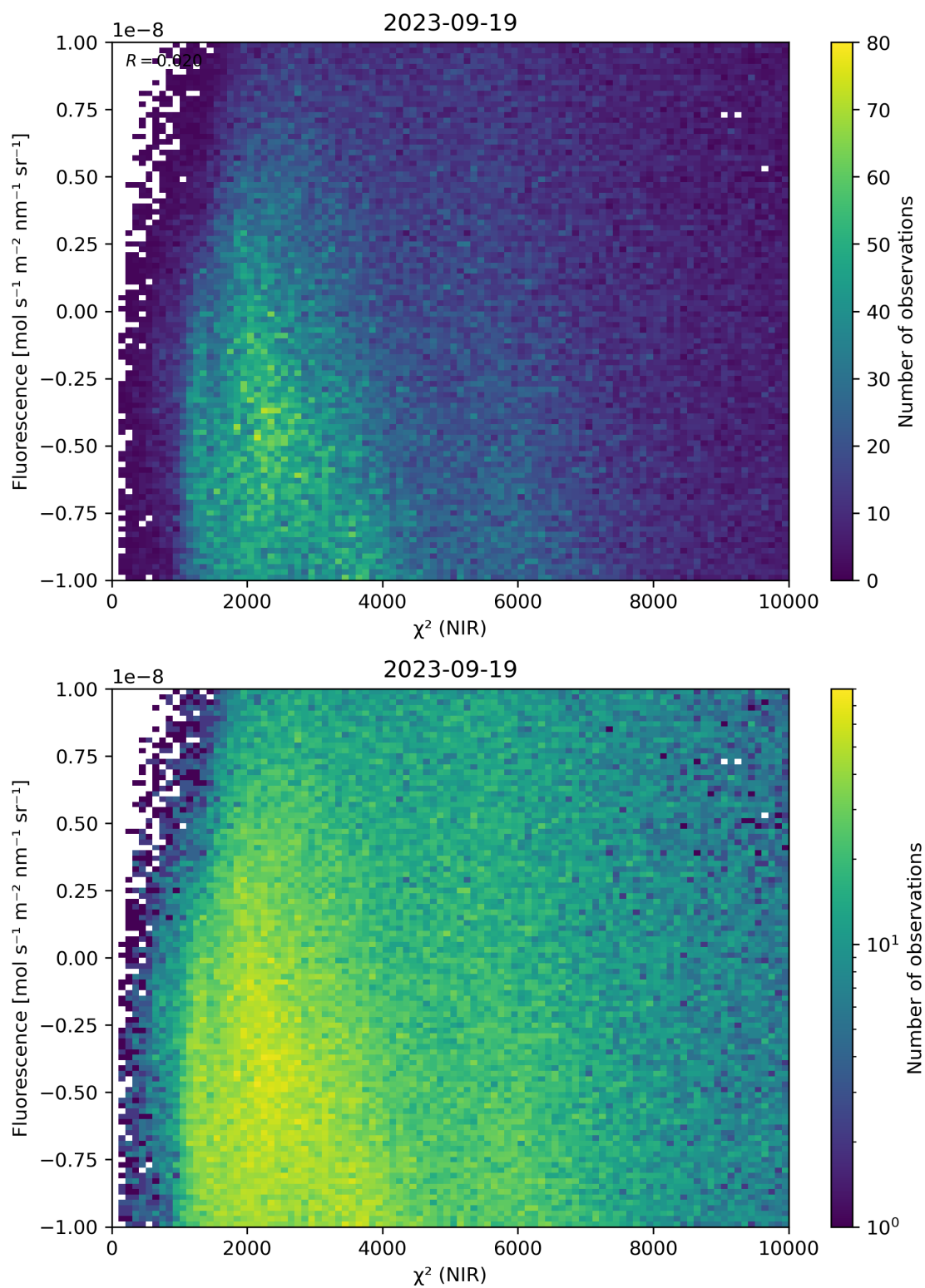
Figure 45: Scatter density plot of “ \chi^2 (NIR)” against “Fluorescence” for 2023-09-18 to 2023-09-20.
