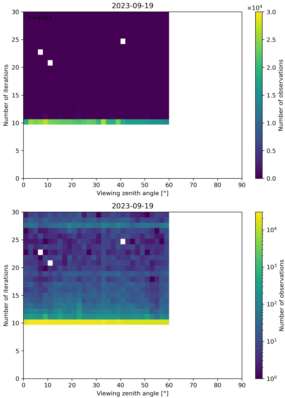
Figure 113: Scatter density plot of “Viewing zenith angle” against “Number of iterations” for 2023-09-18 to 2023-09-20.
