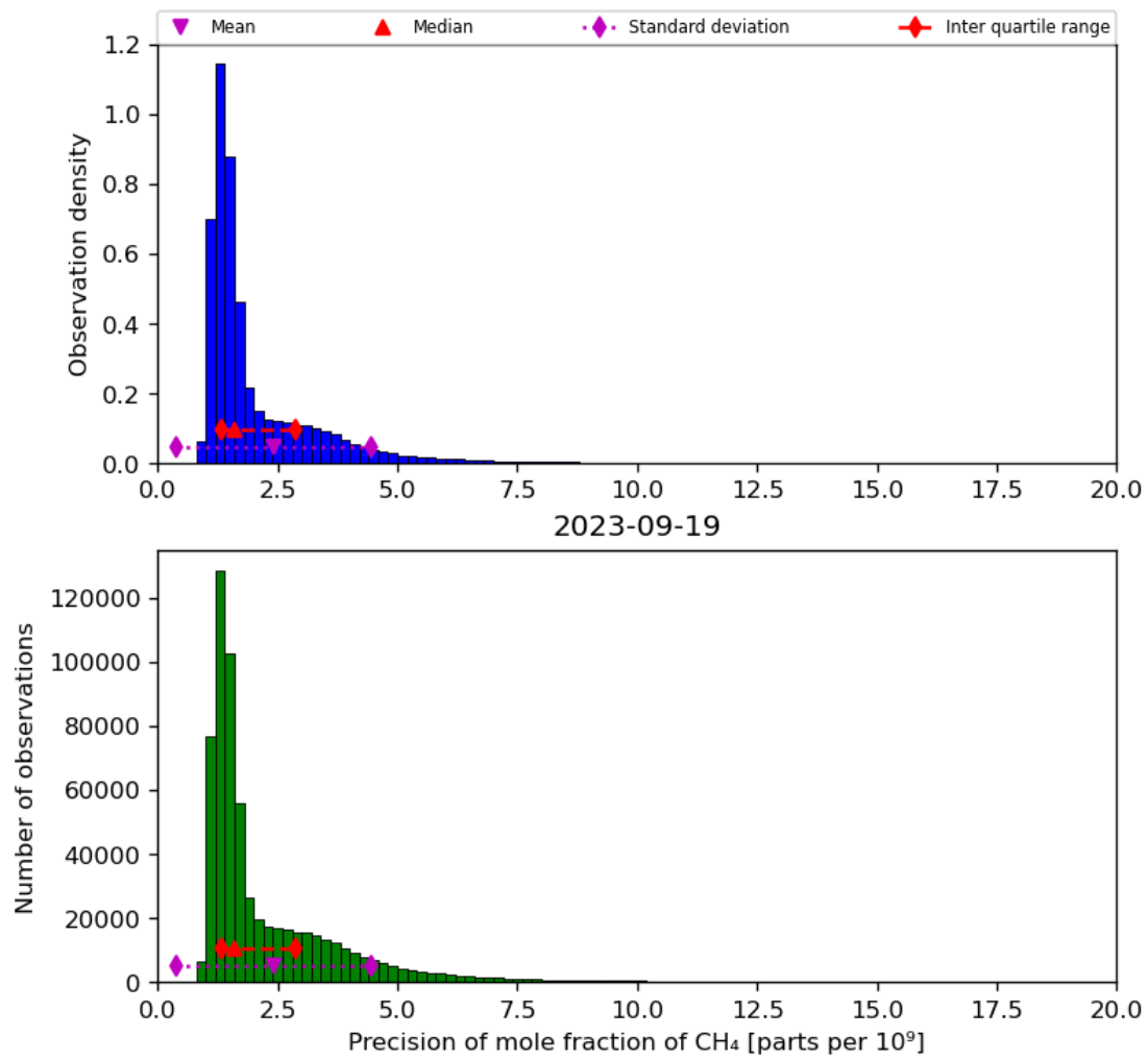
Figure 24: Histogram of “Precision of mole fraction of CH 4 ” for 2023-09-18 to 2023-09-20
