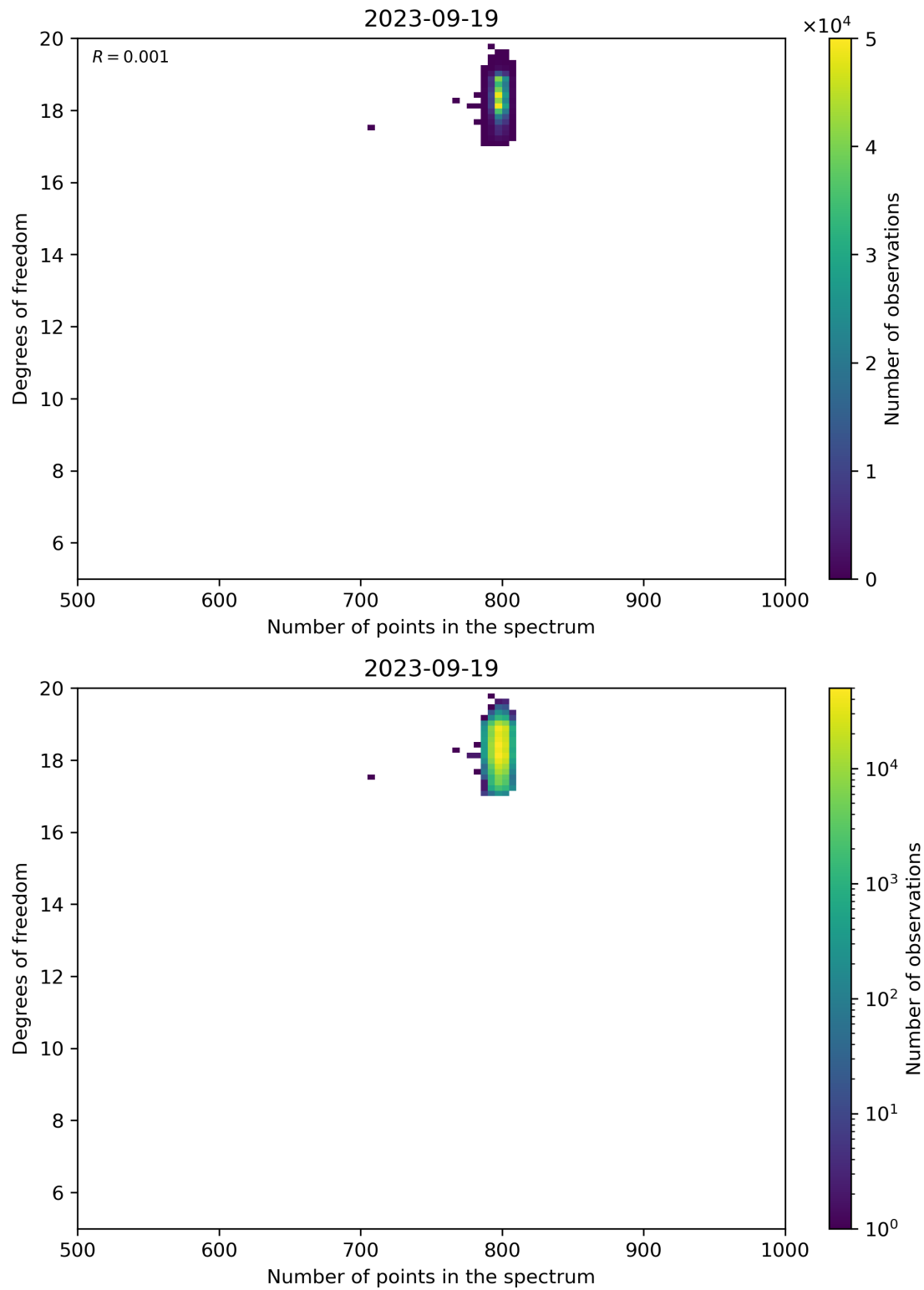
Figure 90: Scatter density plot of “Number of points in the spectrum” against “Degrees of freedom” for 2023-09-18 to 2023-09-20.
