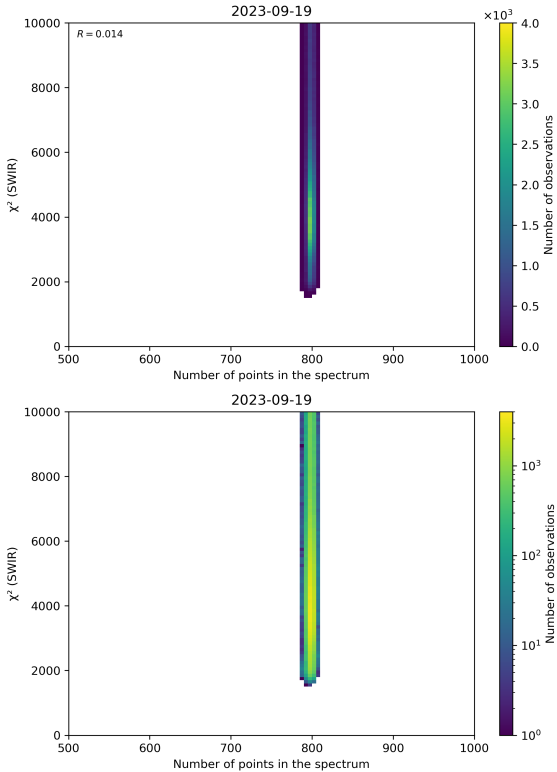
Figure 89: Scatter density plot of “Number of points in the spectrum” against “ \chi^2 (SWIR)” for 2023-09-18 to 2023-09-20.
