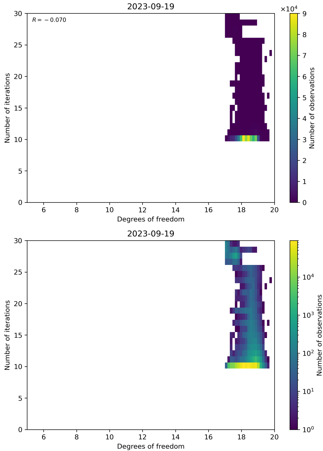
Figure 52: Scatter density plot of “Degrees of freedom” against “Number of iterations” for 2023-09-18 to 2023-09-20.
