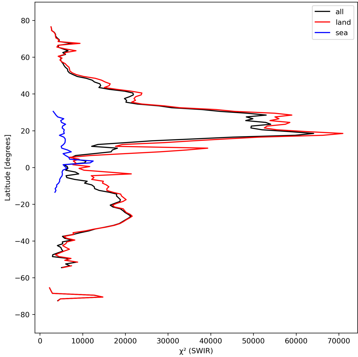
Figure 17: Zonal average of “ \chi^2 (SWIR)” for 2023-09-18 to 2023-09-20.
