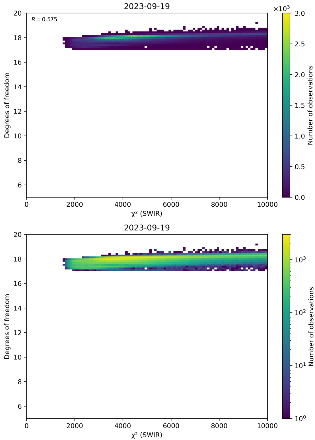
Figure 48: Scatter density plot of “ \chi^2 (SWIR)” against “Degrees of freedom” for 2023-09-18 to 2023-09-20.
