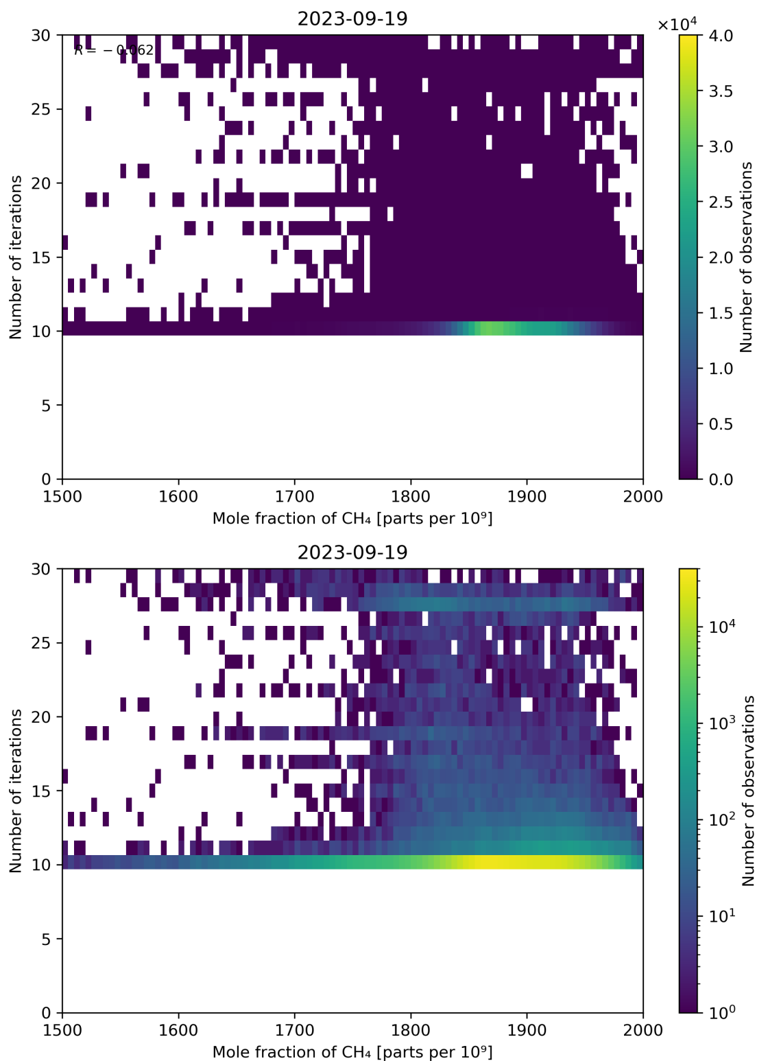
Figure 76: Scatter density plot of “Mole fraction of CH 4 ” against “Number of iterations” for 2023-09-18 to 2023-09-20.
