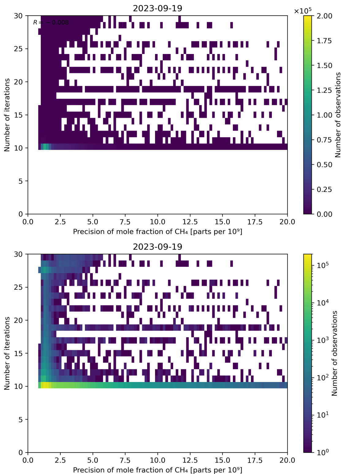
Figure 83: Scatter density plot of “Precision of mole fraction of CH 4 ” against “Number of iterations” for 2023-09-18 to 2023-09-20.
