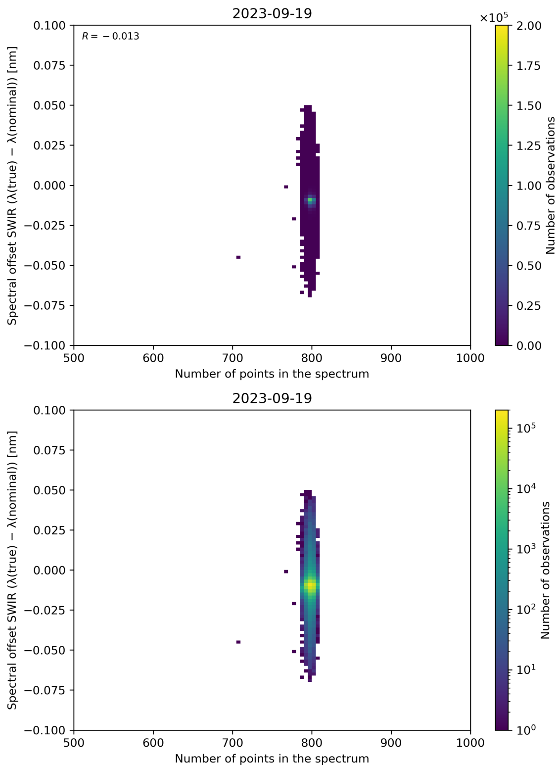
Figure 93: Scatter density plot of “Number of points in the spectrum” against “Spectral offset SWIR ( \lambda(\text{true}) - \lambda(\text{nominal}) )” for 2023-09-18 to 2023-09-20.
