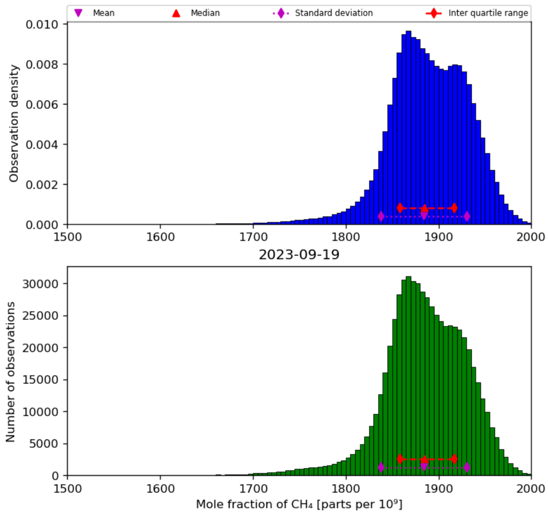
Figure 23: Histogram of “Mole fraction of CH 4 ” for 2023-09-18 to 2023-09-20
