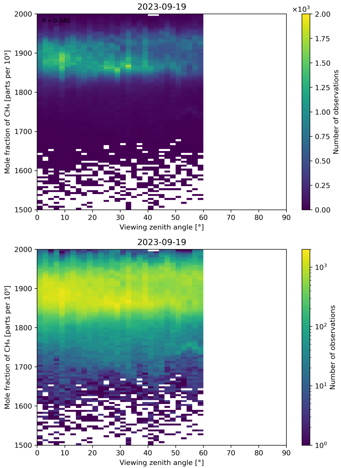
Figure 110: Scatter density plot of “Viewing zenith angle” against “Mole fraction of CH 4 ” for 2023-09-18 to 2023-09-20.
