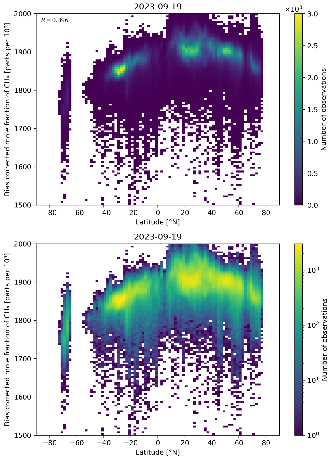
Figure 58: Scatter density plot of “Latitude” against “Bias corrected mole fraction of \text{CH}_4 ” for 2023-09-18 to 2023-09-20.
