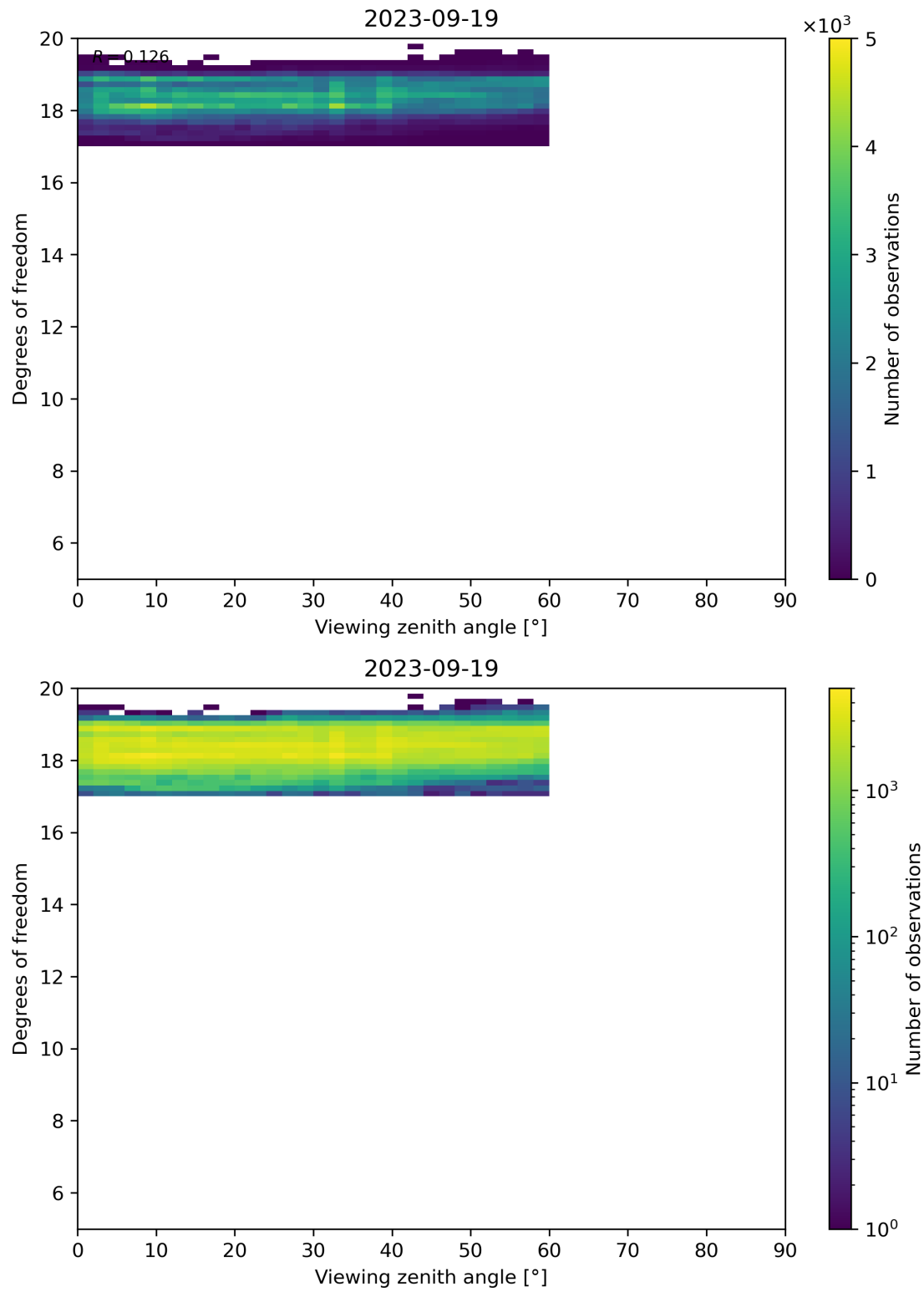
Figure 107: Scatter density plot of “Viewing zenith angle” against “Degrees of freedom” for 2023-09-18 to 2023-09-20.
