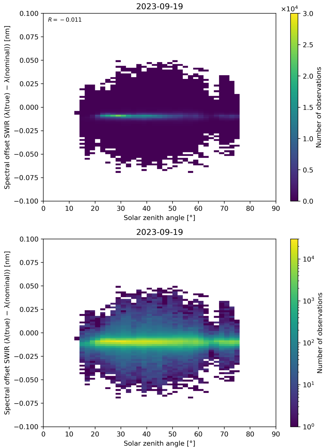
Figure 104: Scatter density plot of “Solar zenith angle” against “Spectral offset SWIR ( \lambda(\text{true}) - \lambda(\text{nominal}) )” for 2023-09-18 to 2023-09-20.
