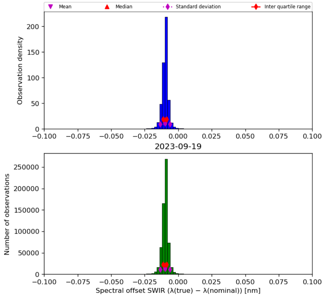
Figure 27: Histogram of “Spectral offset SWIR ( \lambda(\text{true}) - \lambda(\text{nominal}) )” for 2023-09-18 to 2023-09-20
