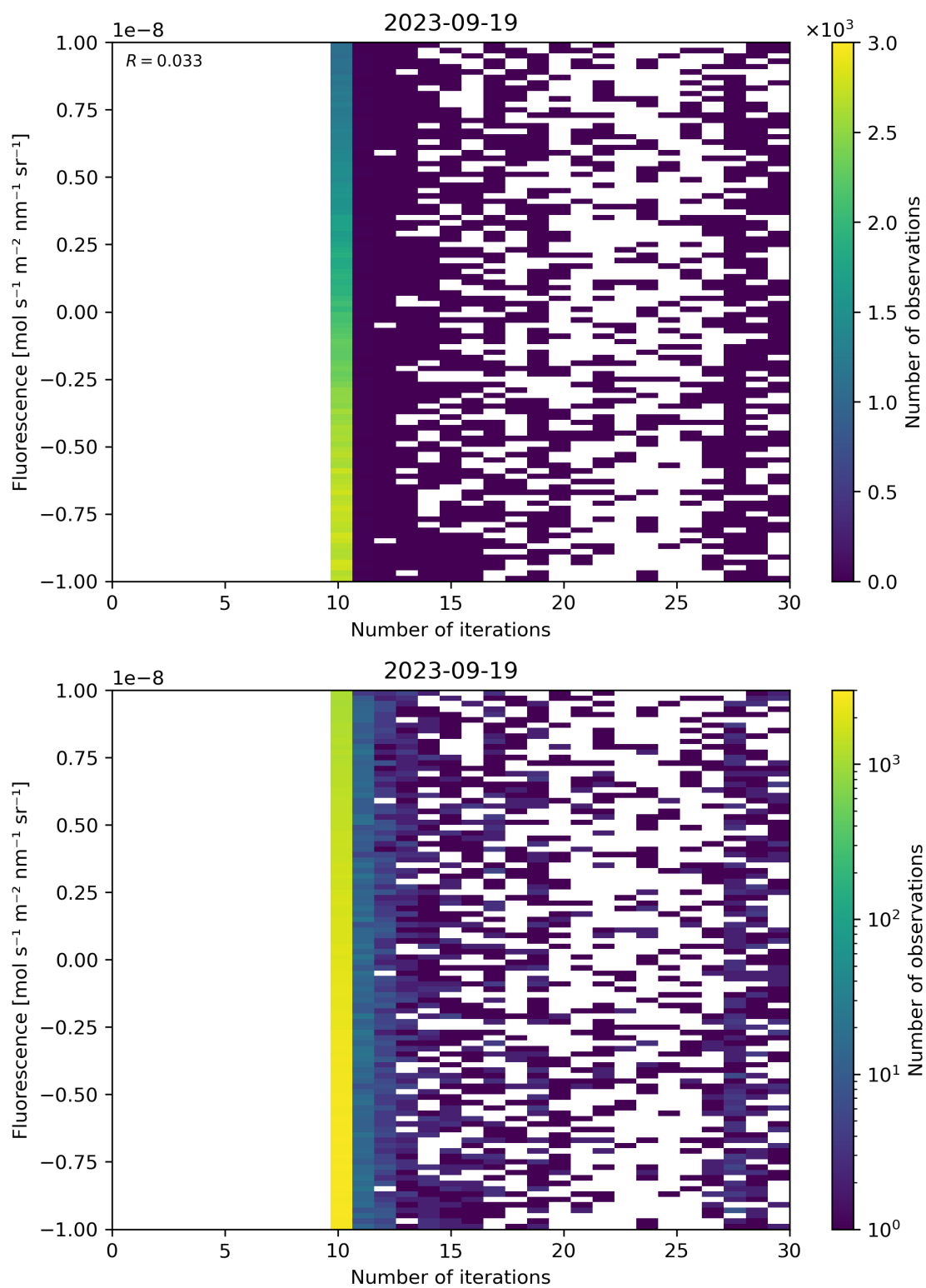
Figure 87: Scatter density plot of “Number of iterations” against “Fluorescence” for 2023-09-18 to 2023-09-20.
