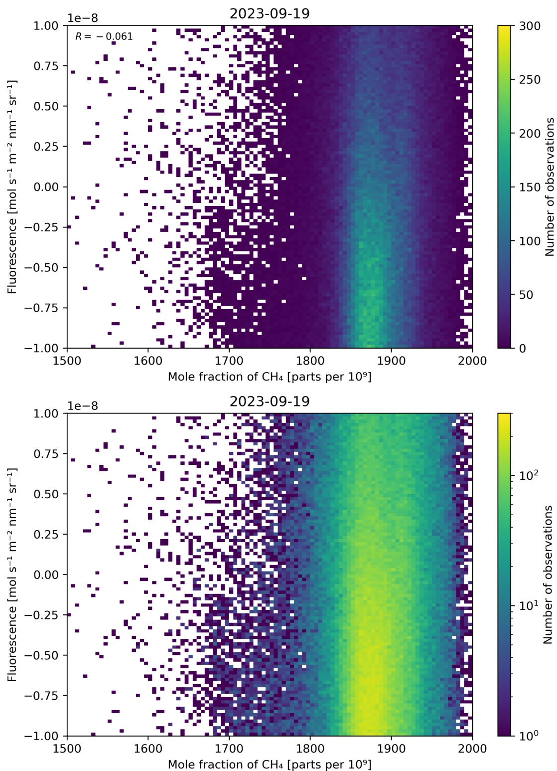
Figure 73: Scatter density plot of “Mole fraction of \text{CH}_4 ” against “Fluorescence” for 2023-09-18 to 2023-09-20.
