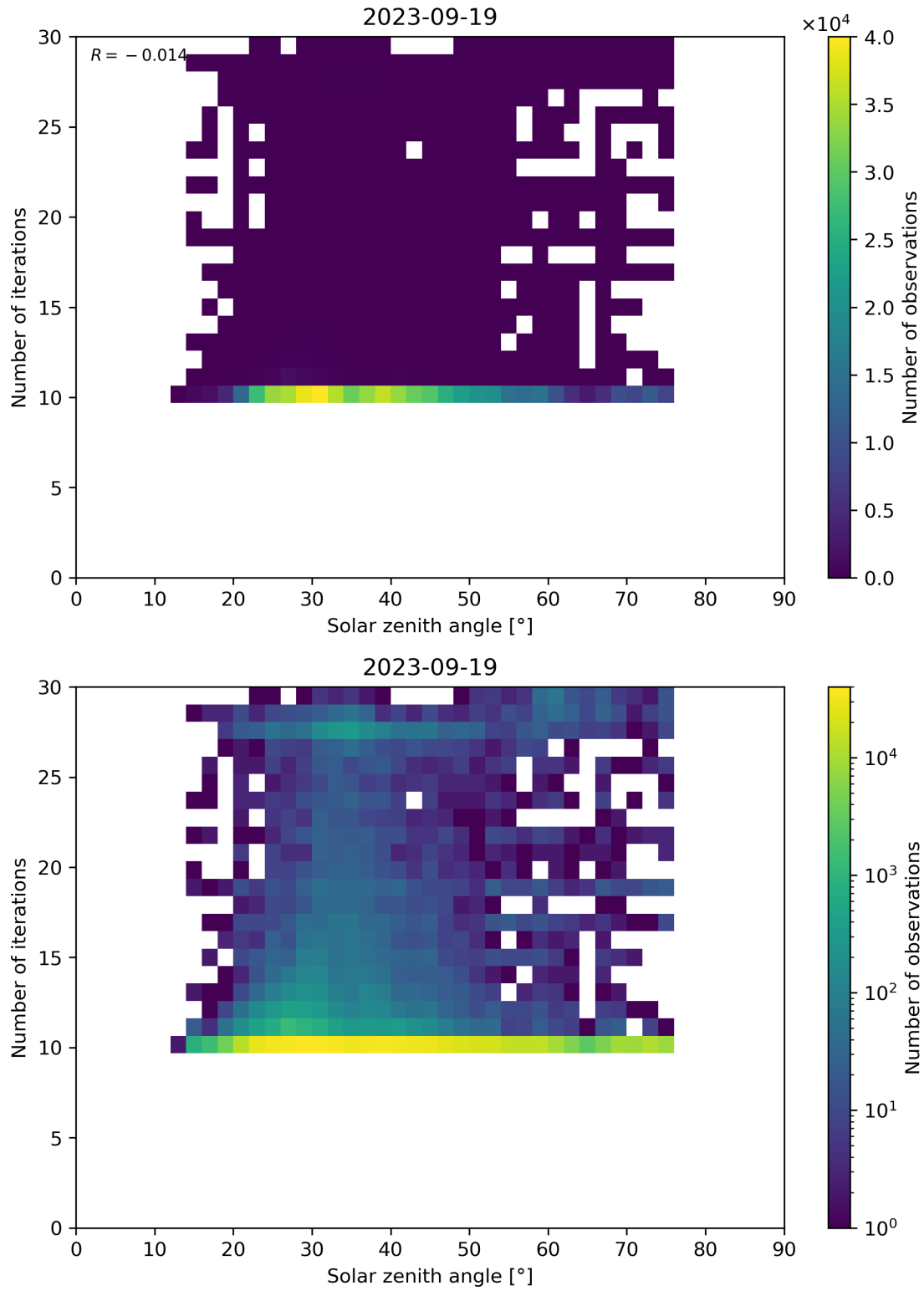
Figure 102: Scatter density plot of “Solar zenith angle” against “Number of iterations” for 2023-09-18 to 2023-09-20.
