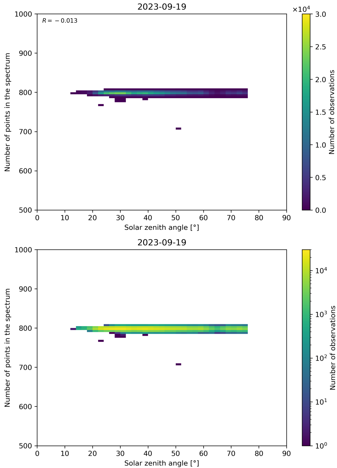
Figure 103: Scatter density plot of “Solar zenith angle” against “Number of points in the spectrum” for 2023-09-18 to 2023-09-20.
