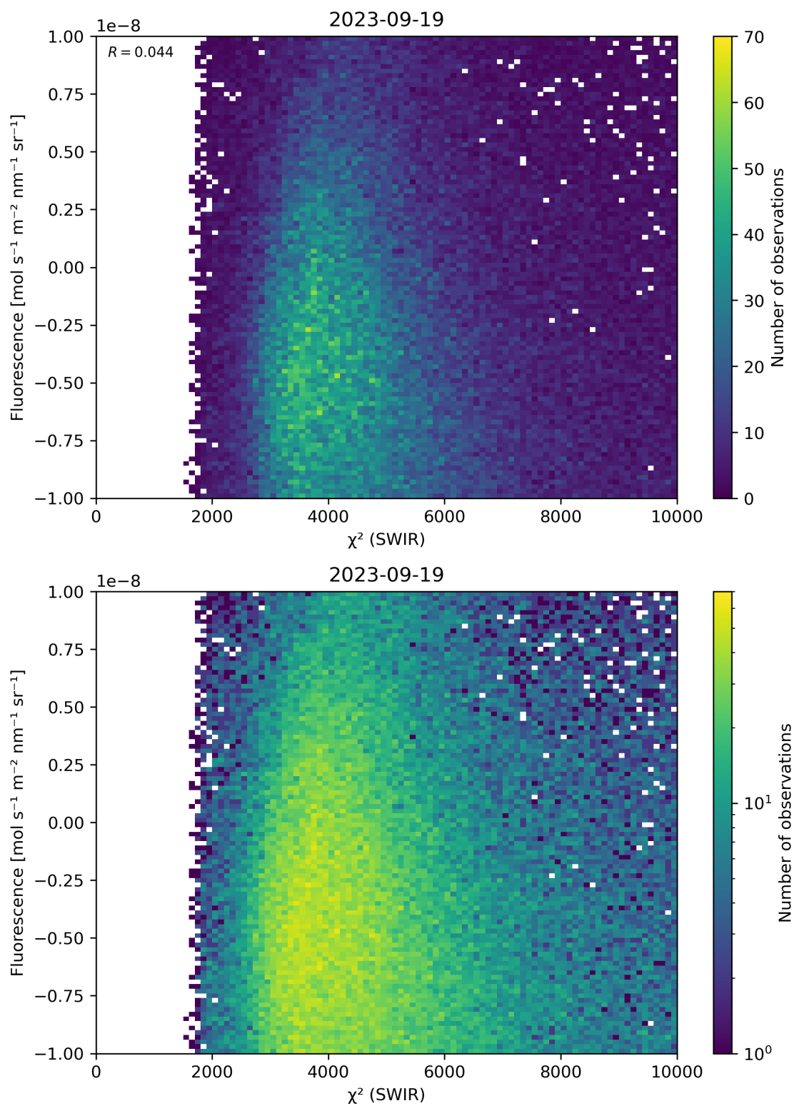
Figure 49: Scatter density plot of “ \chi^2 (SWIR)” against “Fluorescence” for 2023-09-18 to 2023-09-20.
