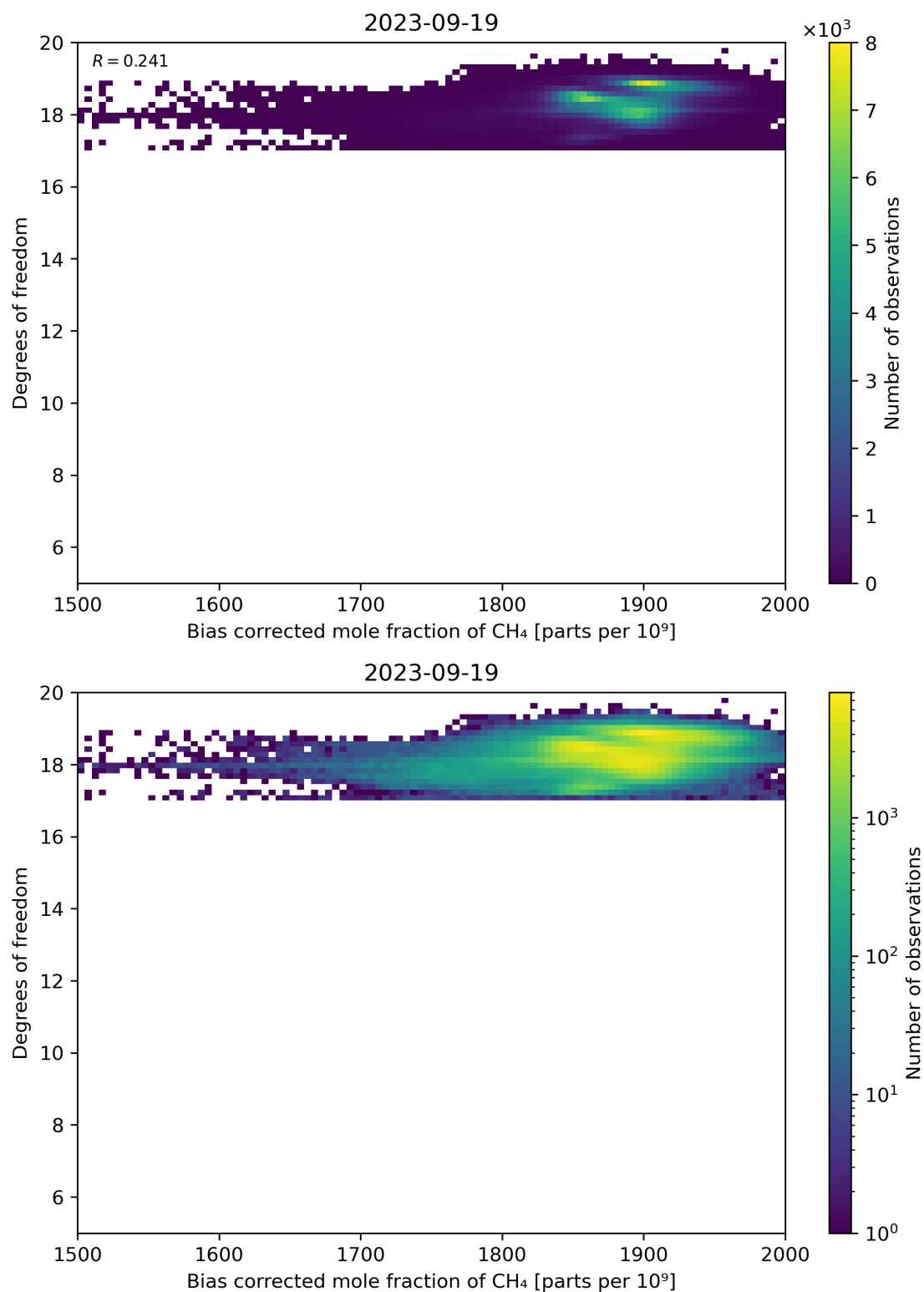
Figure 65: Scatter density plot of “Bias corrected mole fraction of CH 4 ” against “Degrees of freedom” for 2023-09-18 to 2023-09-20.
