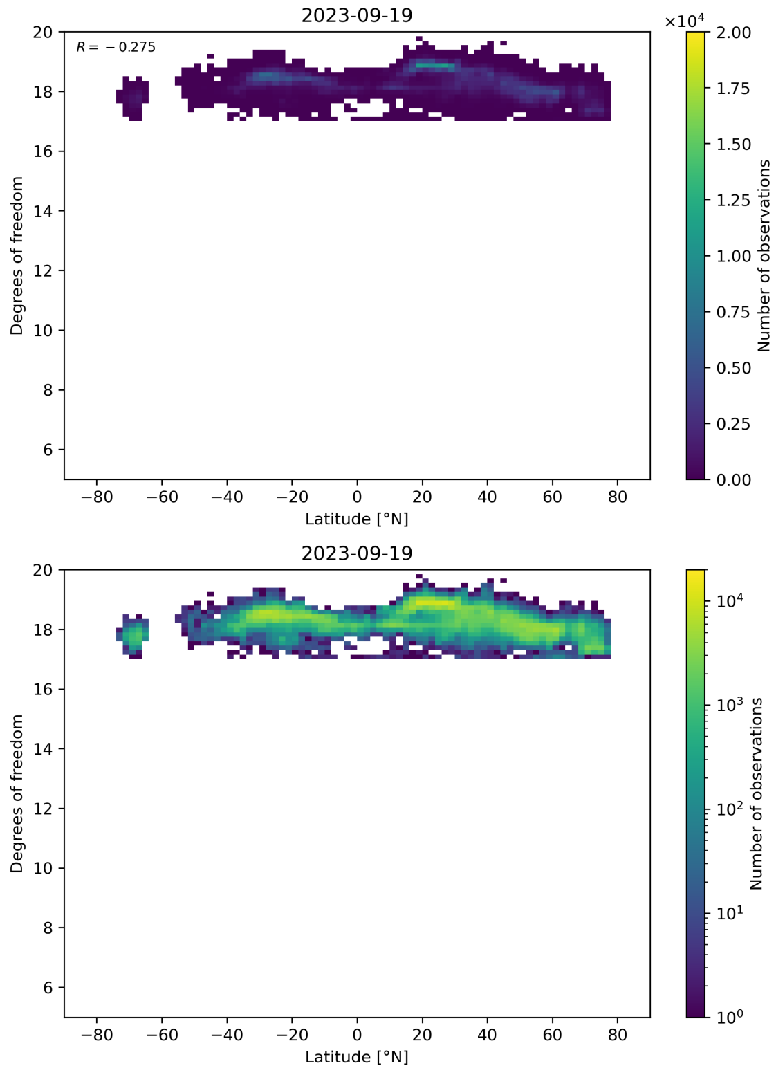
Figure 55: Scatter density plot of “Latitude” against “Degrees of freedom” for 2023-09-18 to 2023-09-20.
