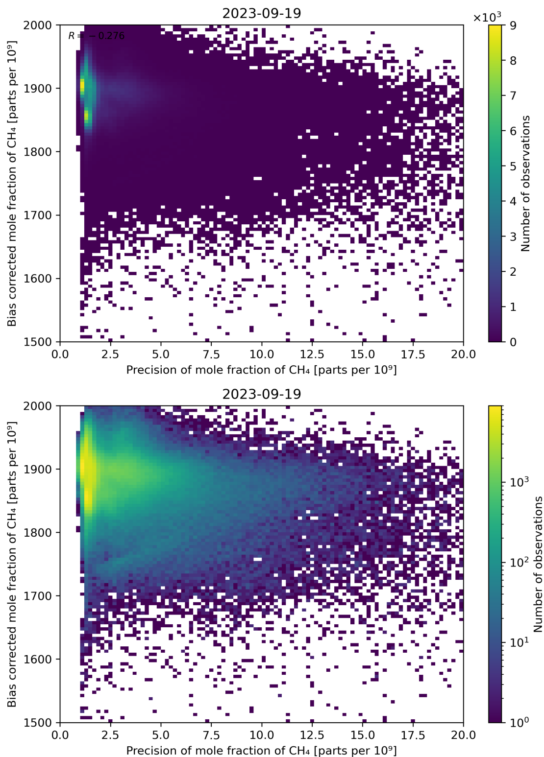
Figure 82: Scatter density plot of “Precision of mole fraction of CH 4 ” against “Bias corrected mole fraction of CH 4 ” for 2023-09-18 to 2023-09-20.
