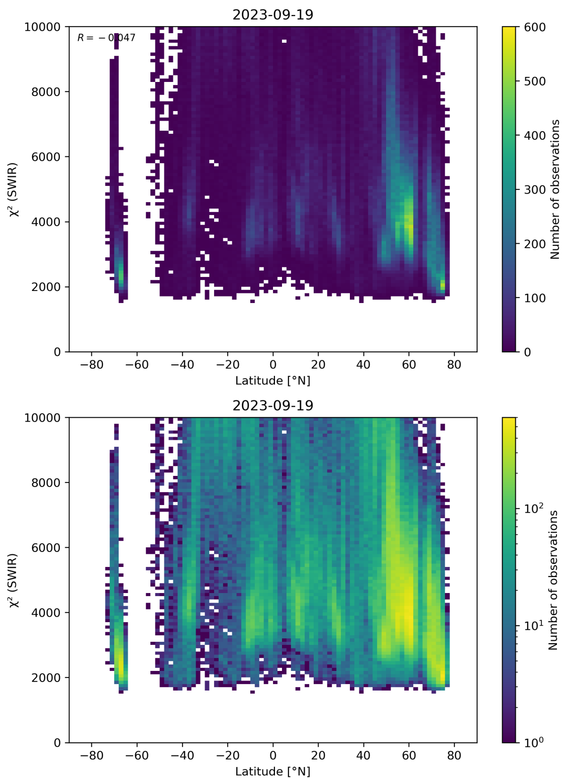
Figure 54: Scatter density plot of “Latitude” against “ \chi^2 (SWIR)” for 2023-09-18 to 2023-09-20.
