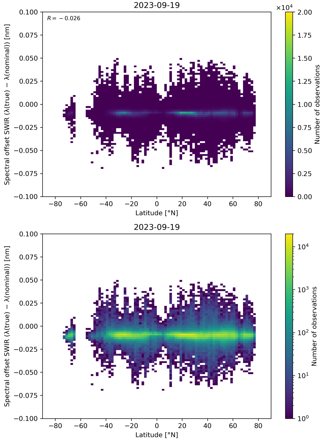
Figure 62: Scatter density plot of “Latitude” against “Spectral offset SWIR ( \lambda(\text{true}) - \lambda(\text{nominal}) )” for 2023-09-18 to 2023-09-20.
