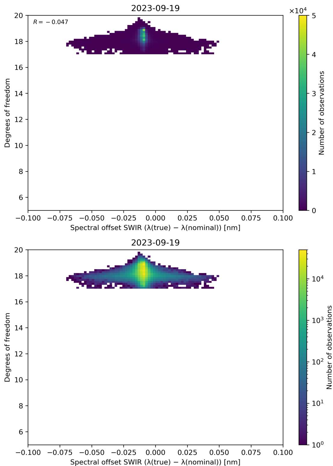
Figure 119: Scatter density plot of “Spectral offset SWIR ( \lambda(\text{true}) - \lambda(\text{nominal}) )” against “Degrees of freedom” for 2023-09-18 to 2023-09-20.
