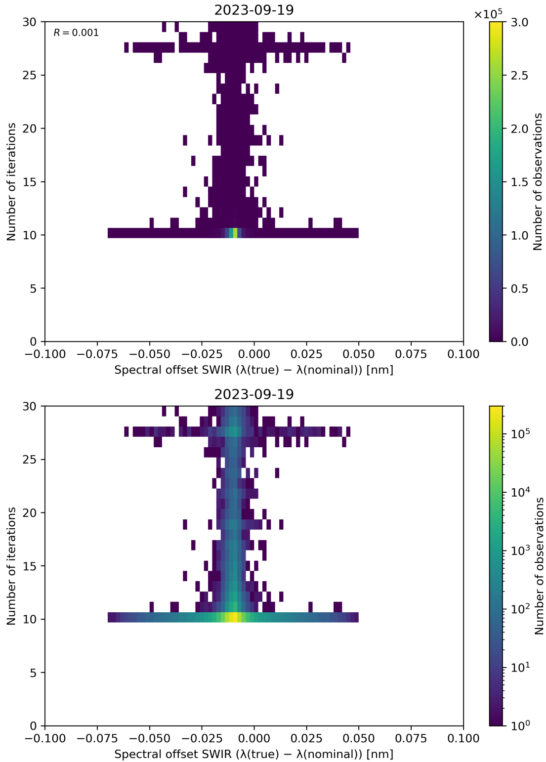
Figure 121: Scatter density plot of “Spectral offset SWIR ( \lambda(\text{true}) - \lambda(\text{nominal}) )” against “Number of iterations” for 2023-09-18 to 2023-09-20.
