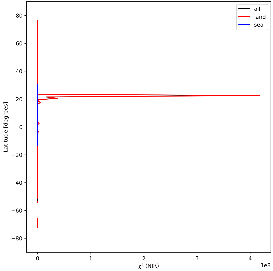
Figure 18: Zonal average of “ \chi^2 (NIR)” for 2023-09-18 to 2023-09-20.
