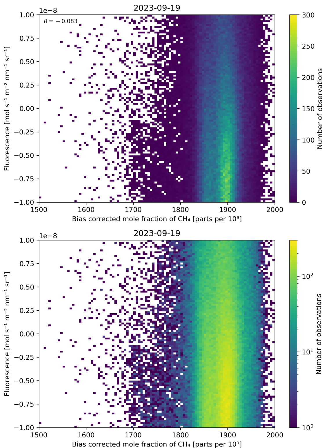
Figure 66: Scatter density plot of “Bias corrected mole fraction of \text{CH}_4 ” against “Fluorescence” for 2023-09-18 to 2023-09-20.
