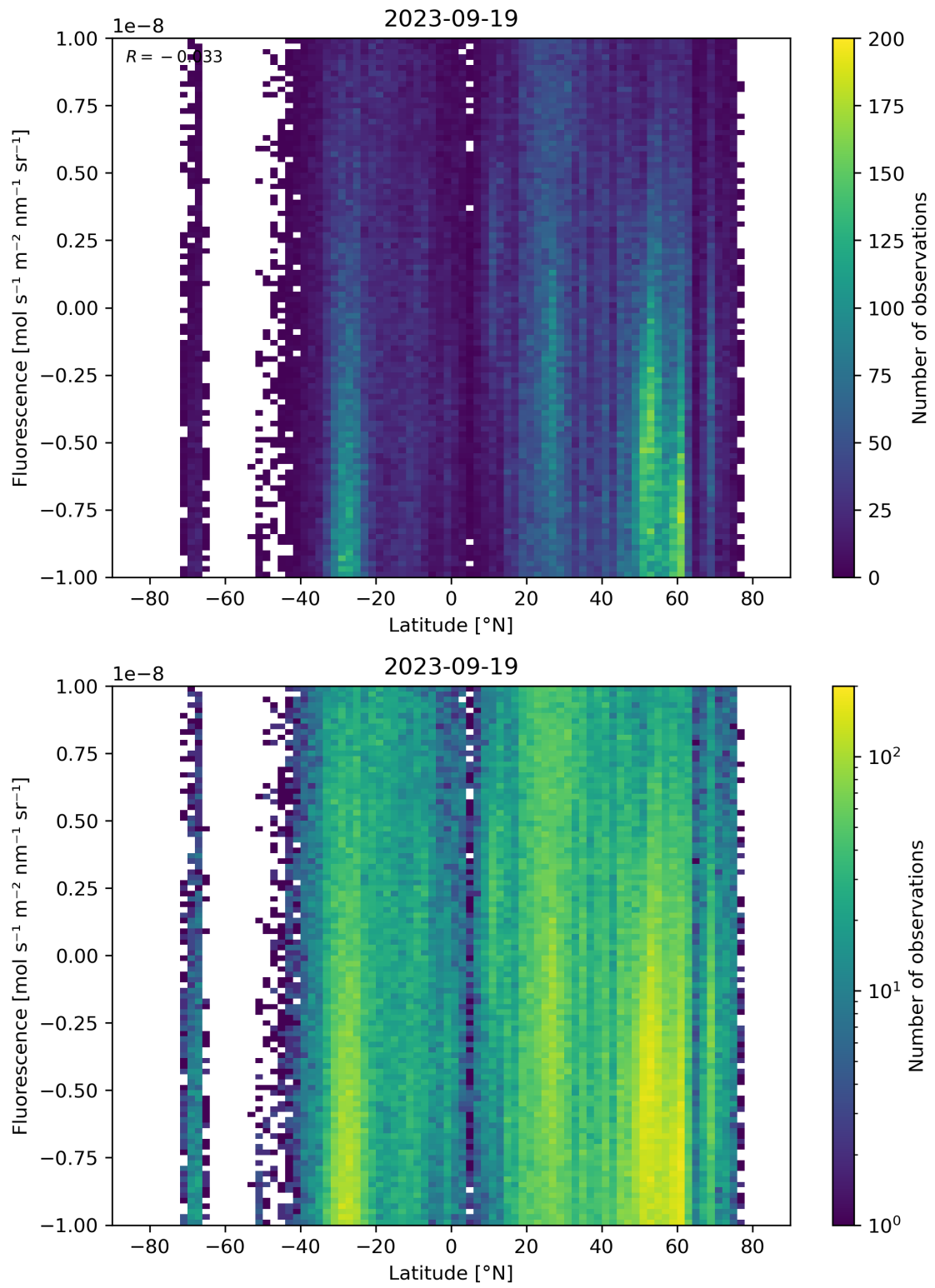
Figure 56: Scatter density plot of “Latitude” against “Fluorescence” for 2023-09-18 to 2023-09-20.
