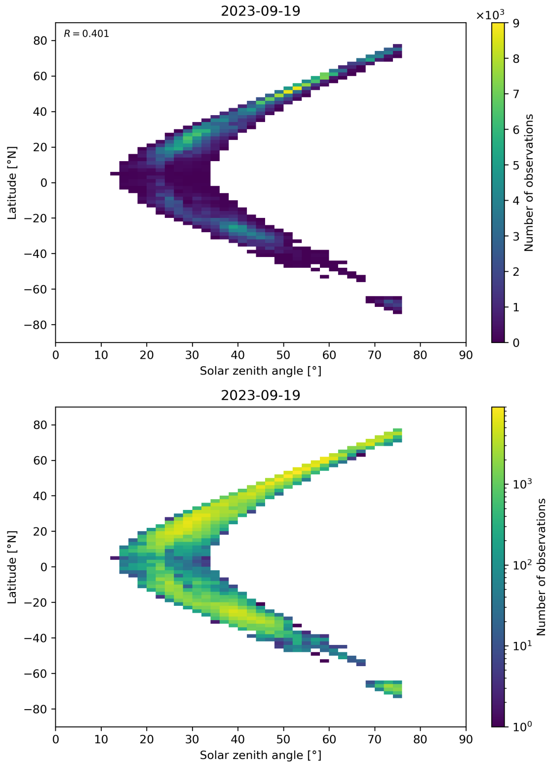
Figure 98: Scatter density plot of “Solar zenith angle” against “Latitude” for 2023-09-18 to 2023-09-20.
