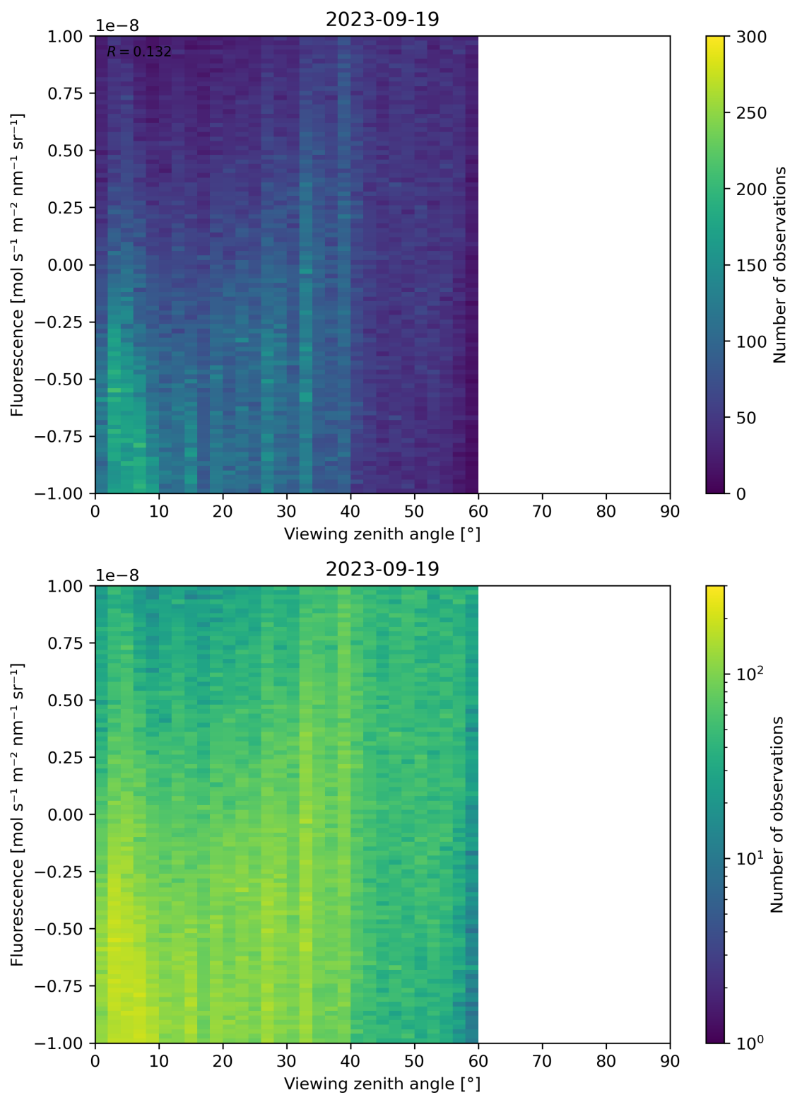
Figure 108: Scatter density plot of “Viewing zenith angle” against “Fluorescence” for 2023-09-18 to 2023-09-20.
