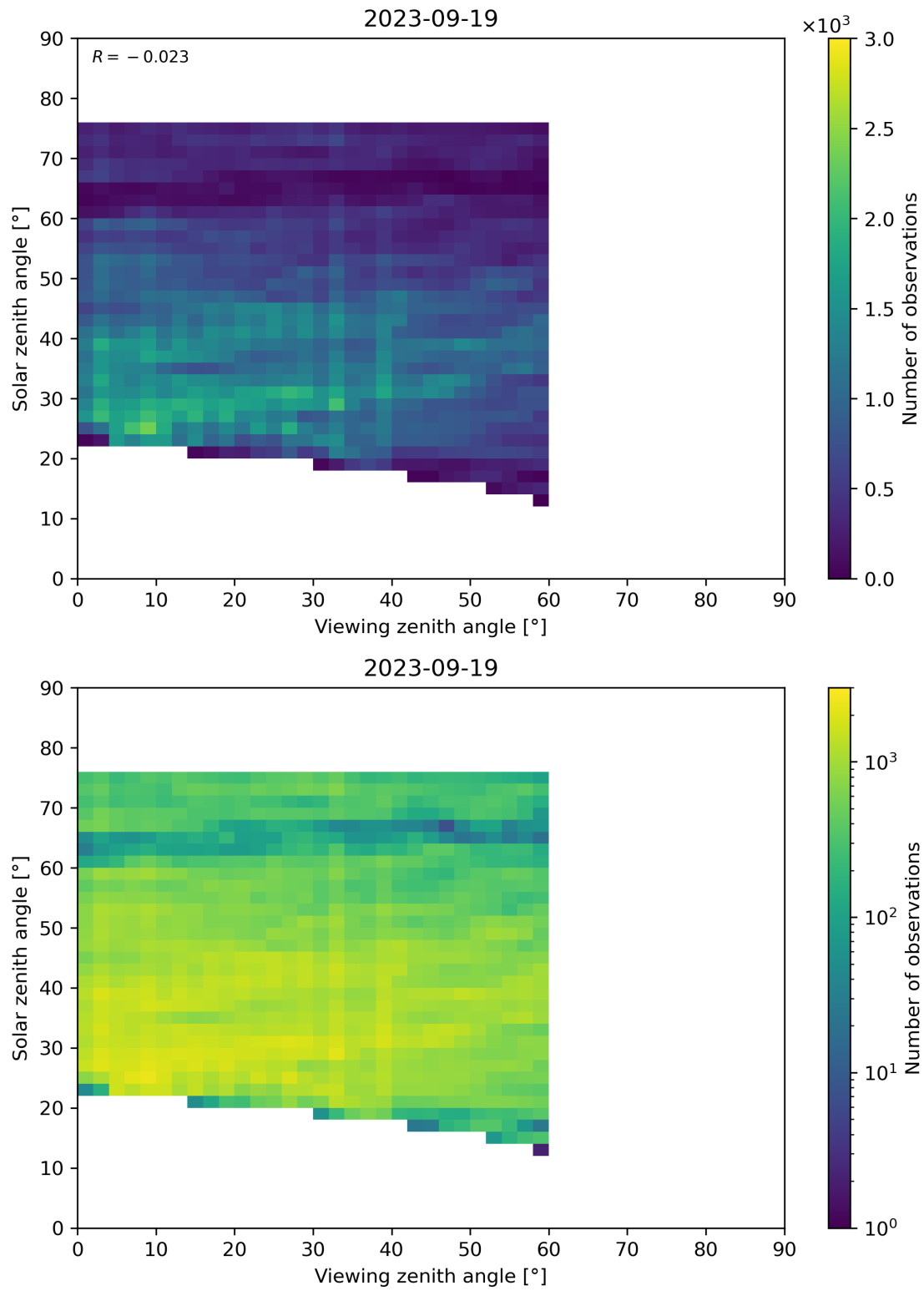
Figure 115: Scatter density plot of “Viewing zenith angle” against “Solar zenith angle” for 2023-09-18 to 2023-09-20.
