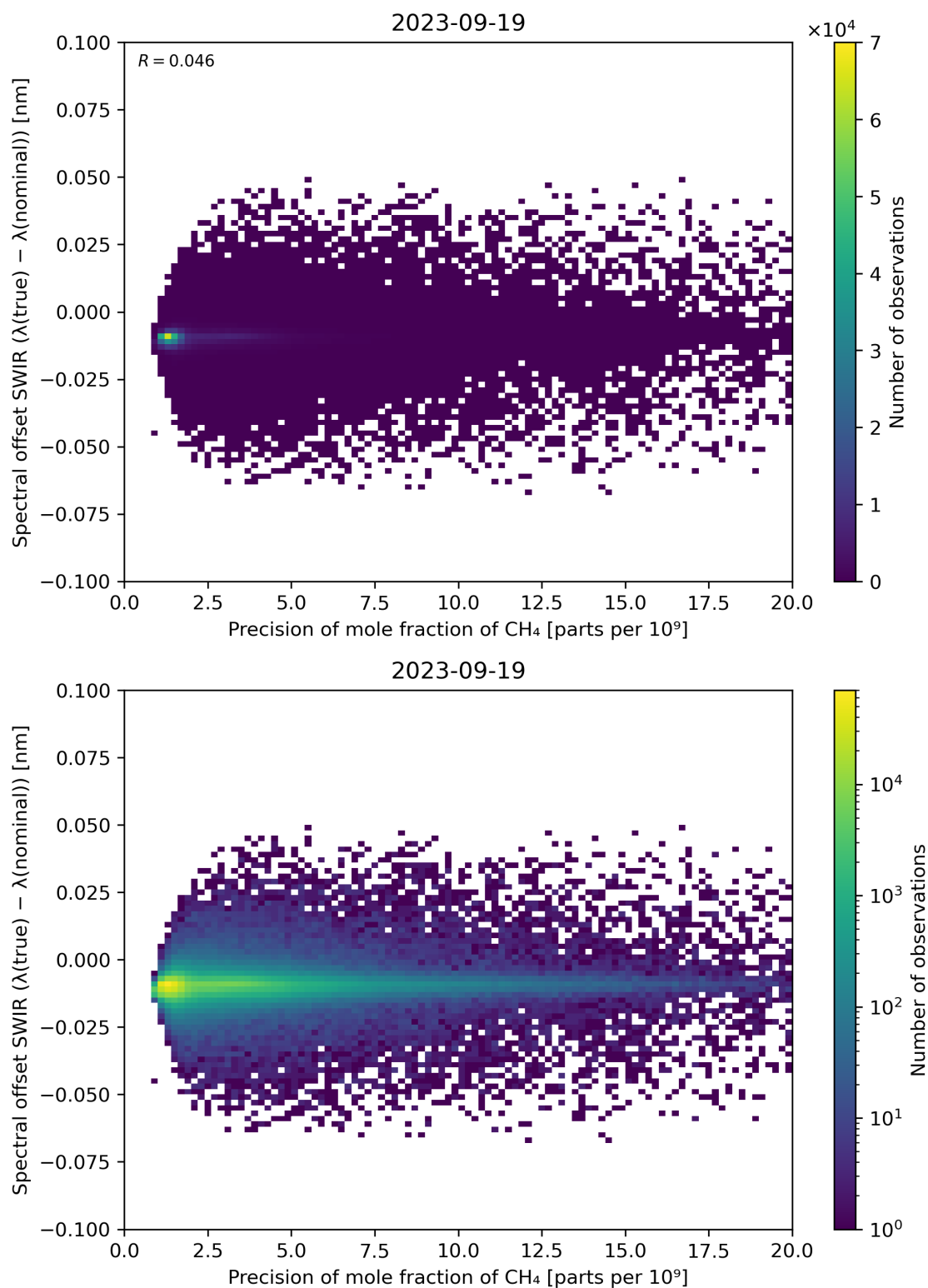
Figure 85: Scatter density plot of “Precision of mole fraction of CH 4 ” against “Spectral offset SWIR ( \lambda(\text{true}) - \lambda(\text{nominal}) )” for 2023-09-18 to 2023-09-20.
