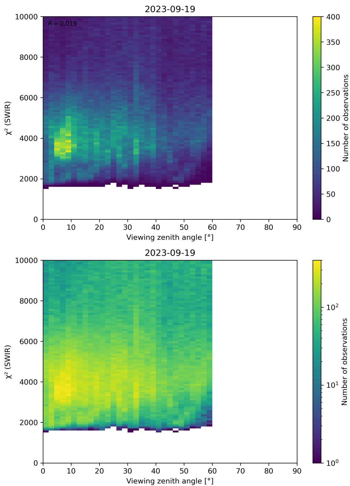
Figure 106: Scatter density plot of “Viewing zenith angle” against “ \chi^2 (SWIR)” for 2023-09-18 to 2023-09-20.
