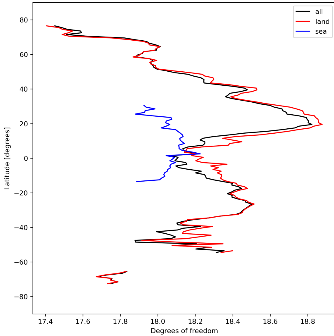
Figure 19: Zonal average of “Degrees of freedom” for 2023-09-18 to 2023-09-20.
