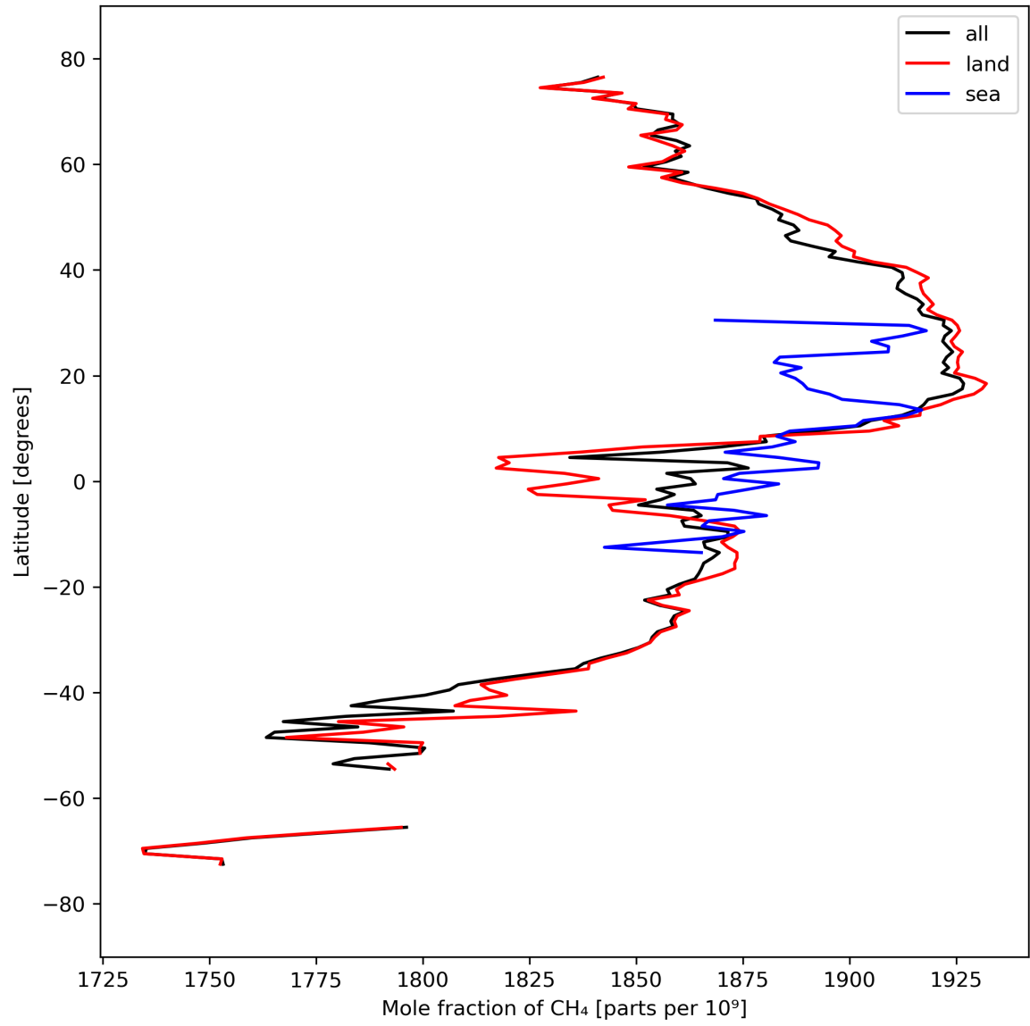
Figure 12: Zonal average of “Mole fraction of \text{CH}_4 ” for 2023-09-18 to 2023-09-20.
