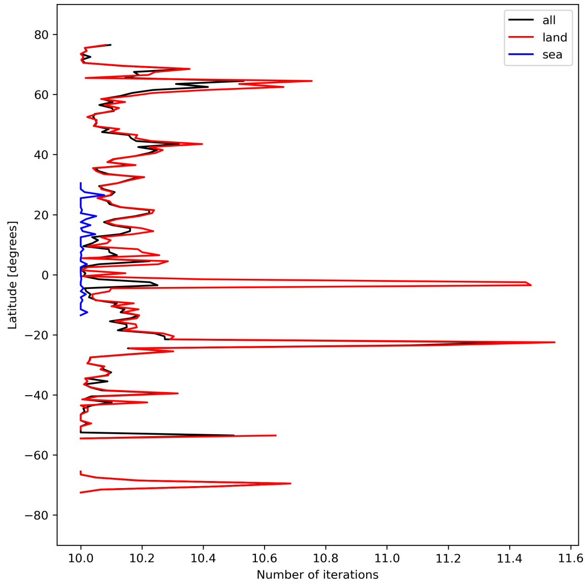
Figure 20: Zonal average of “Number of iterations” for 2023-09-18 to 2023-09-20.
