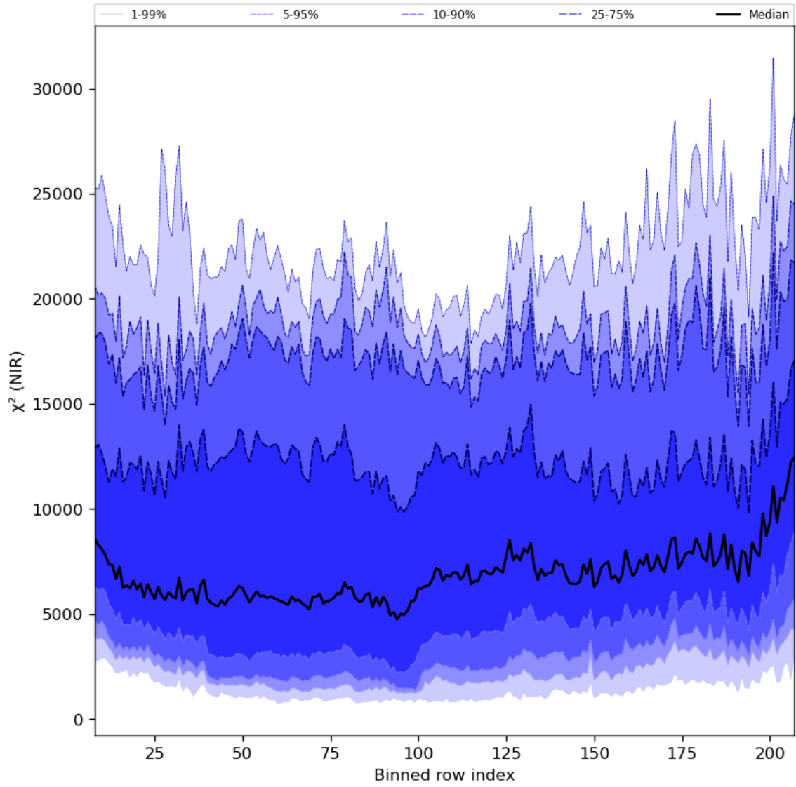
Figure 40: Along track statistics of “ \chi^2 (NIR)” for 2023-09-18 to 2023-09-20
