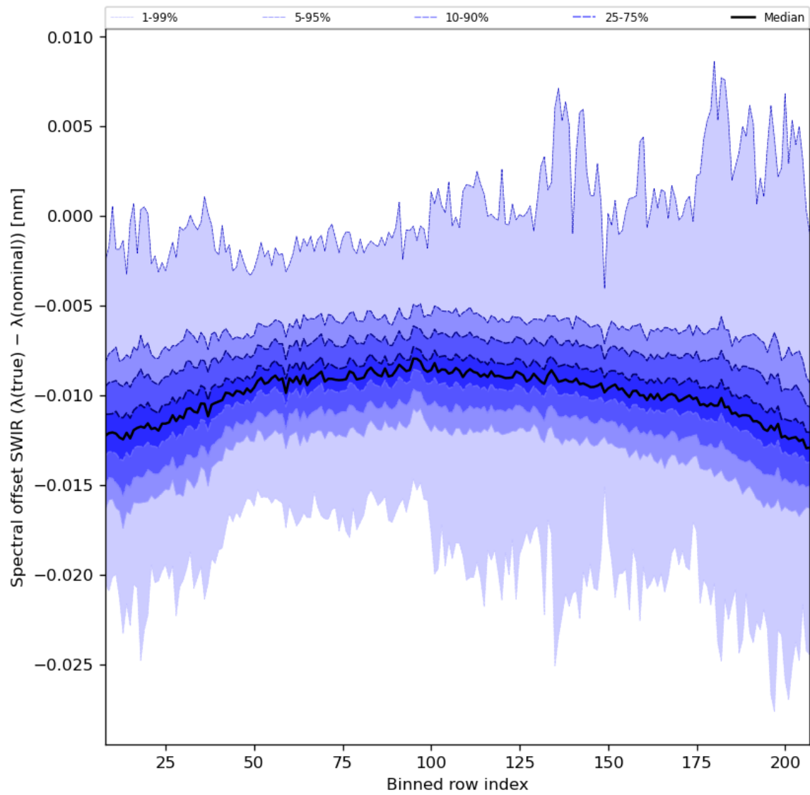
Figure 38: Along track statistics of “Spectral offset SWIR ( \lambda(\text{true}) - \lambda(\text{nominal}) )” for 2023-09-18 to 2023-09-20
