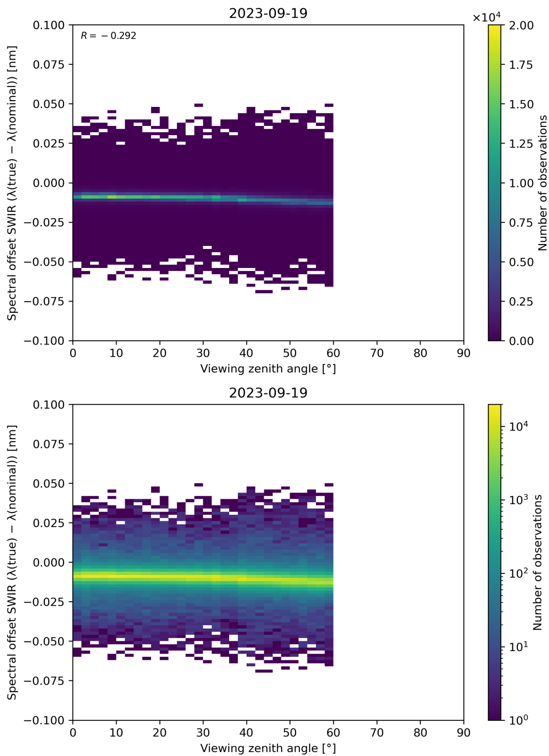
Figure 116: Scatter density plot of “Viewing zenith angle” against “Spectral offset SWIR ( \lambda(\text{true}) - \lambda(\text{nominal}) )” for 2023-09-18 to 2023-09-20.
