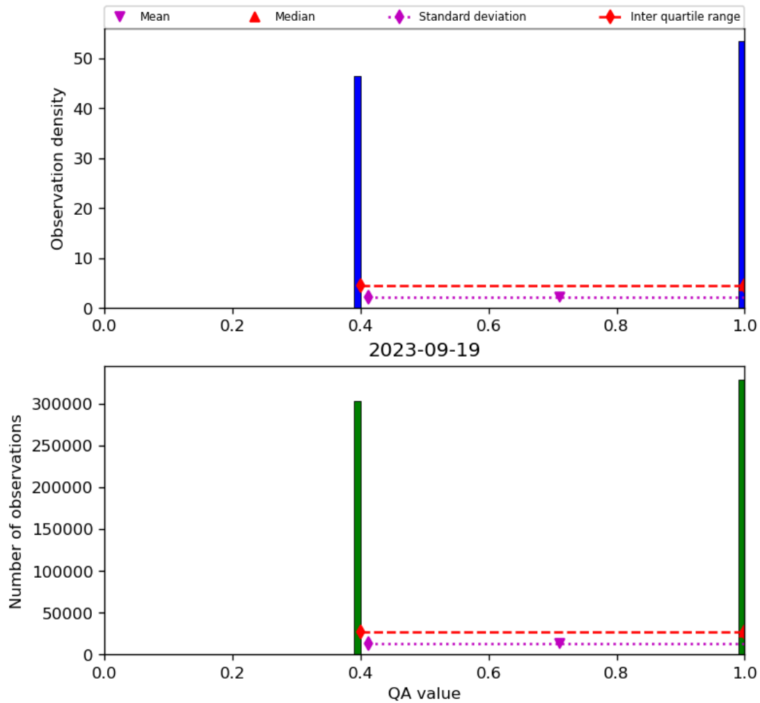
Figure 22: Histogram of “QA value” for 2023-09-18 to 2023-09-20
