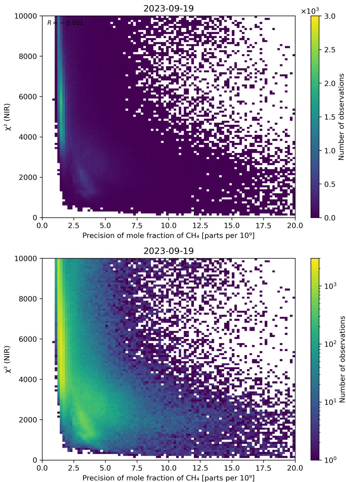
Figure 78: Scatter density plot of “Precision of mole fraction of CH 4 ” against “ \chi^2 (NIR)” for 2023-09-18 to 2023-09-20.
