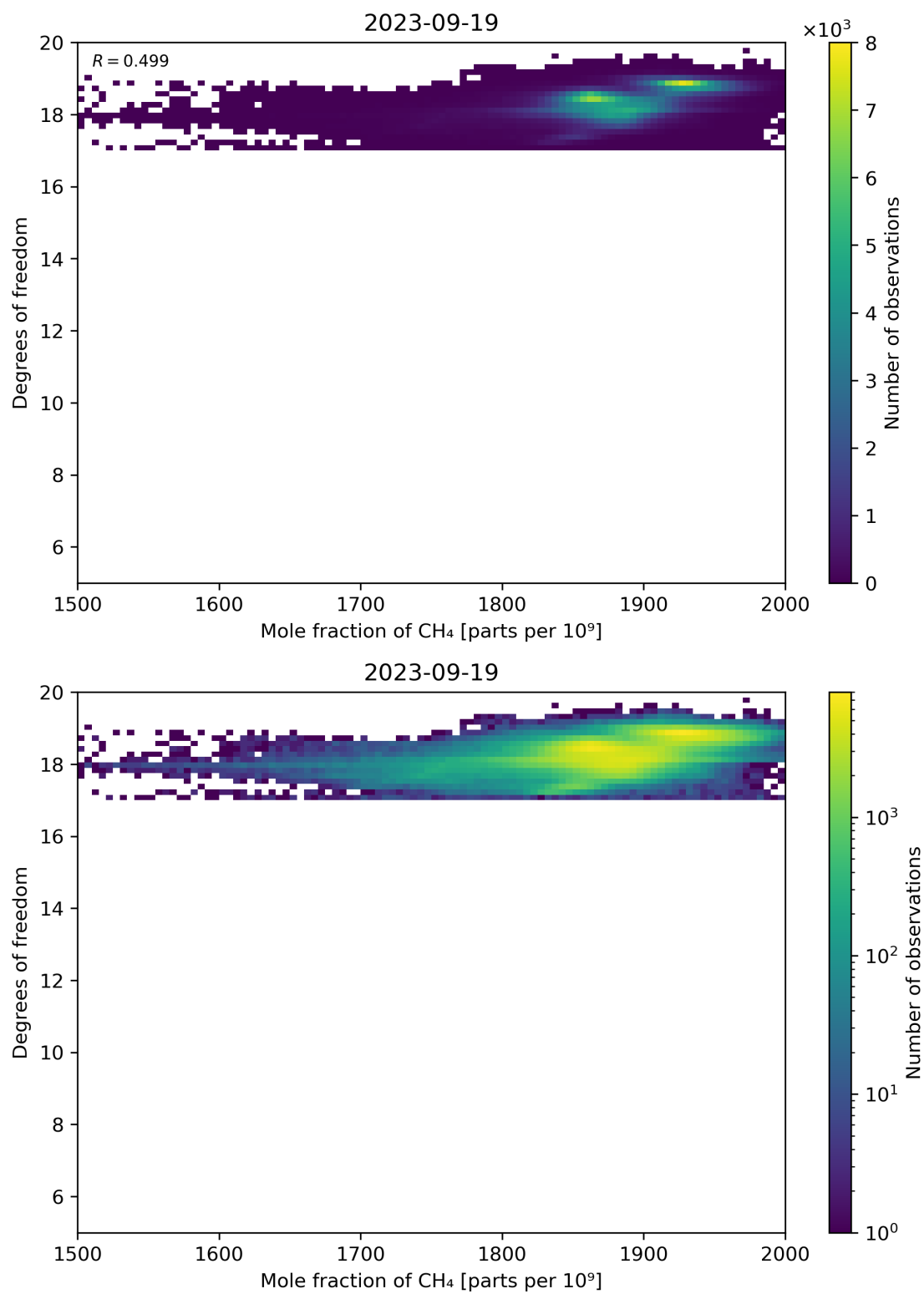
Figure 72: Scatter density plot of “Mole fraction of CH 4 ” against “Degrees of freedom” for 2023-09-18 to 2023-09-20.
