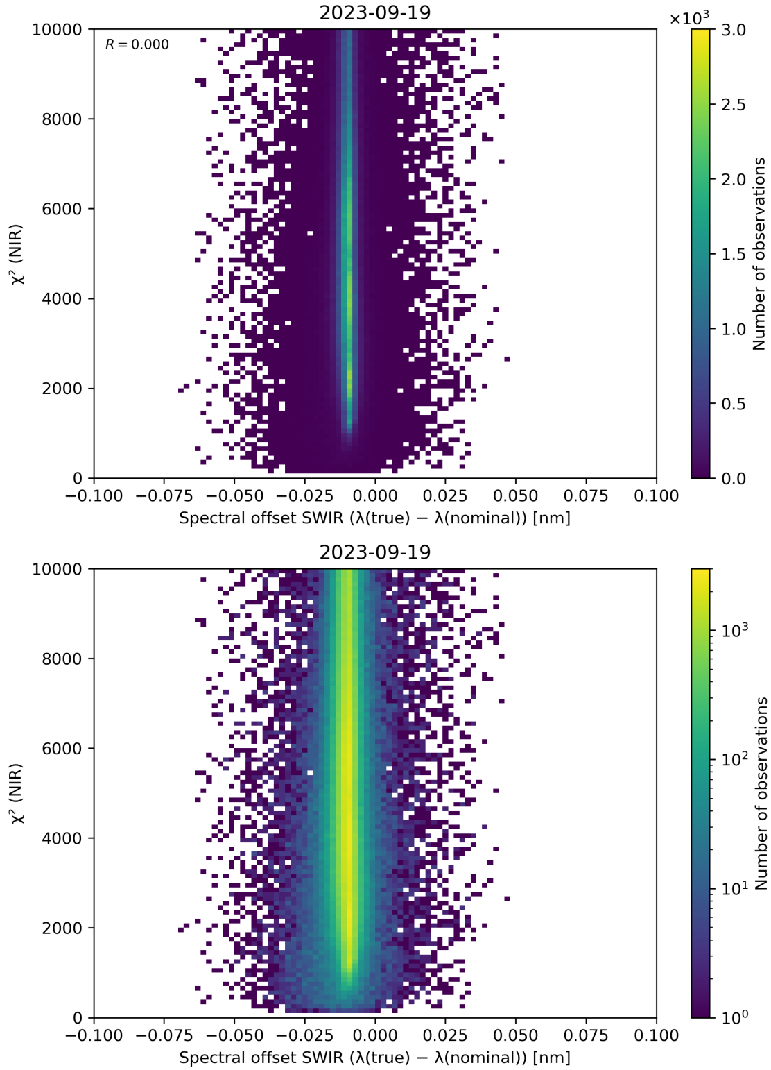
Figure 117: Scatter density plot of “Spectral offset SWIR ( \lambda(\text{true}) - \lambda(\text{nominal}) )” against “ \chi^2 (NIR)” for 2023-09-18 to 2023-09-20.
