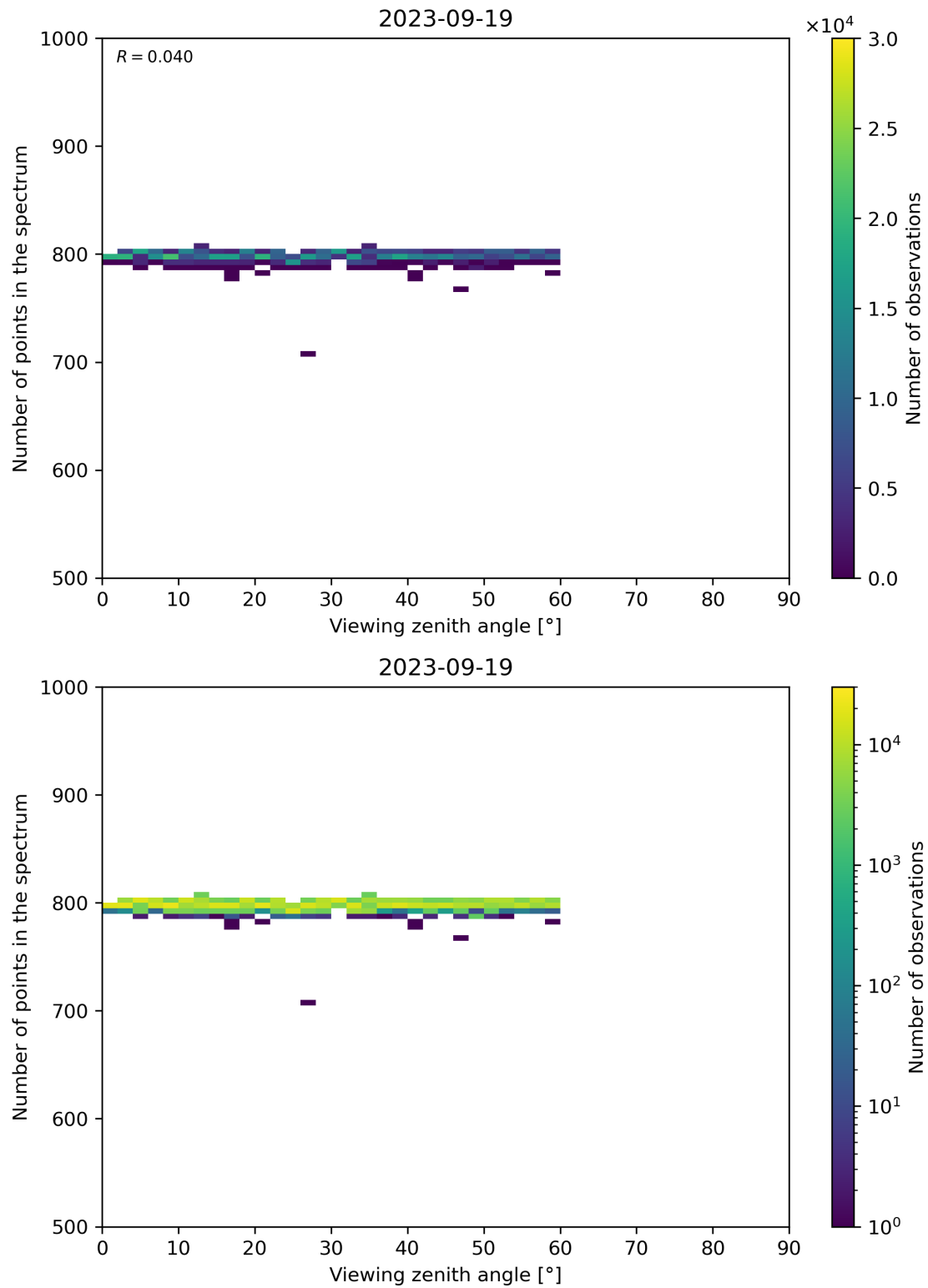
Figure 114: Scatter density plot of “Viewing zenith angle” against “Number of points in the spectrum” for 2023-09-18 to 2023-09-20.
