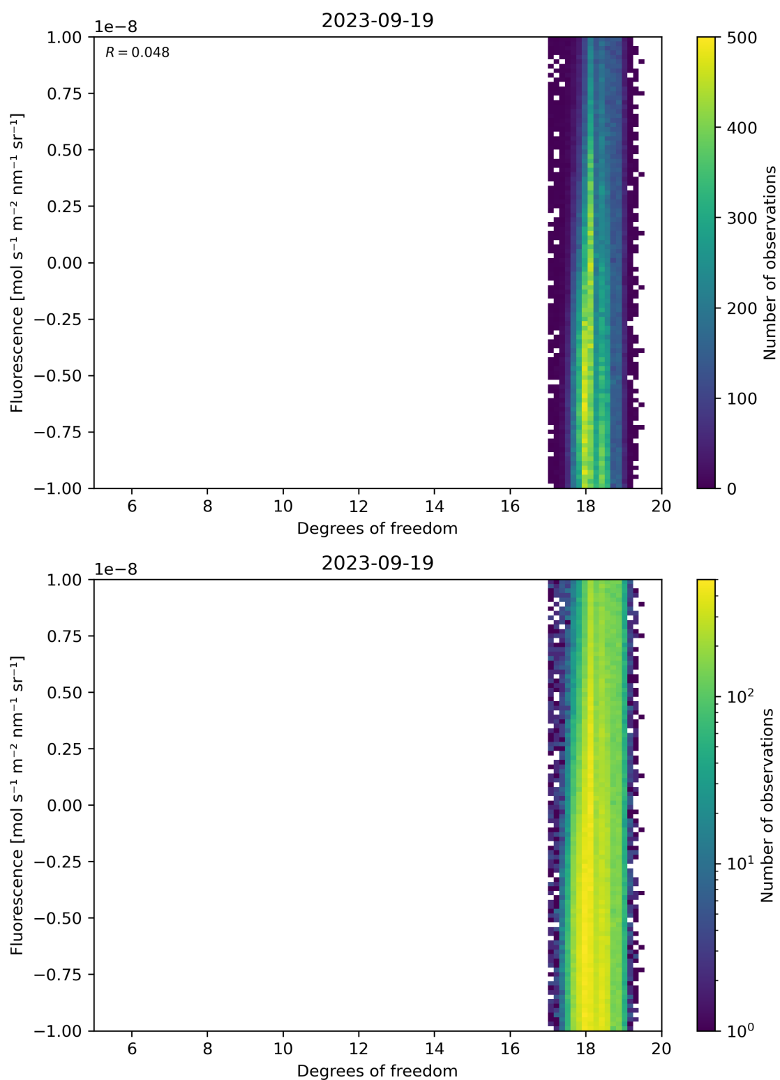
Figure 51: Scatter density plot of “Degrees of freedom” against “Fluorescence” for 2023-09-18 to 2023-09-20.
