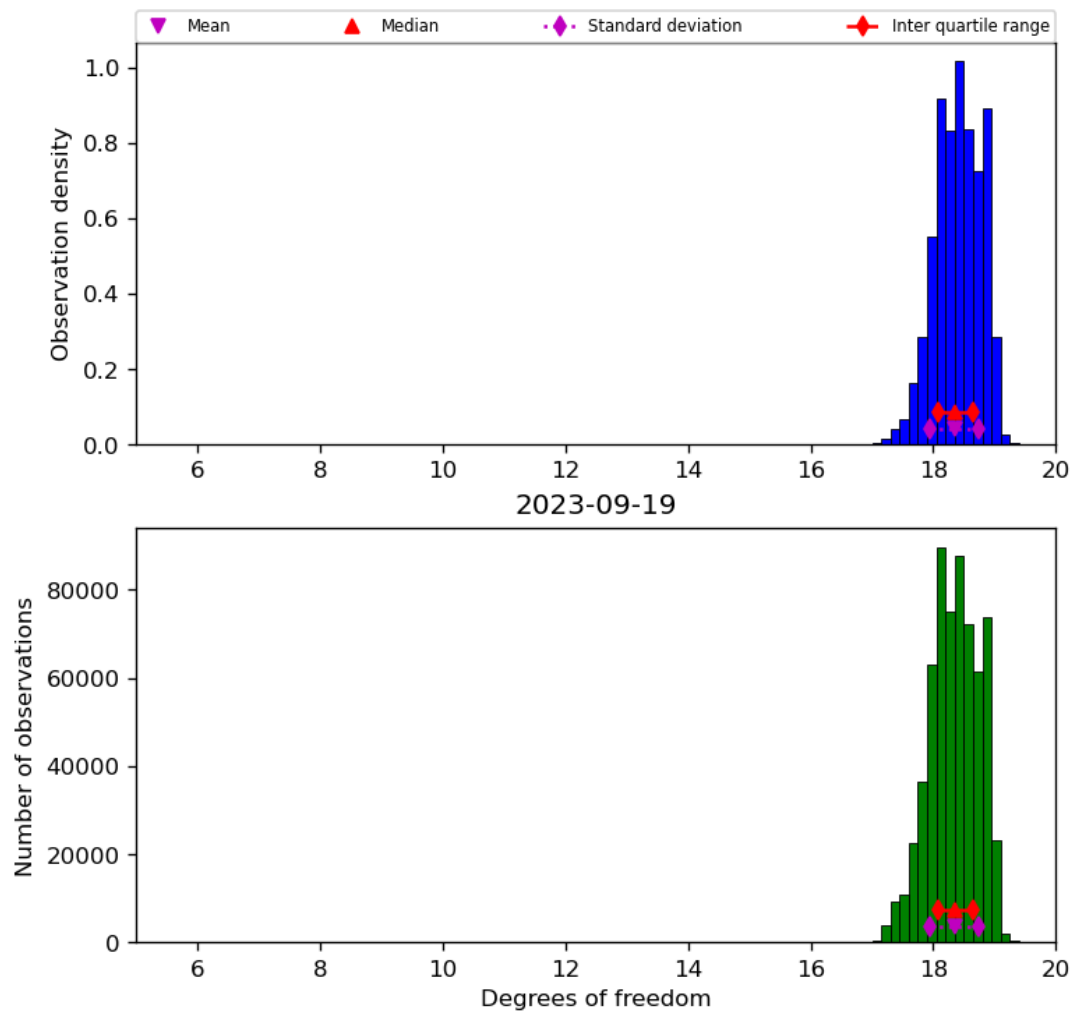
Figure 30: Histogram of “Degrees of freedom” for 2023-09-18 to 2023-09-20
