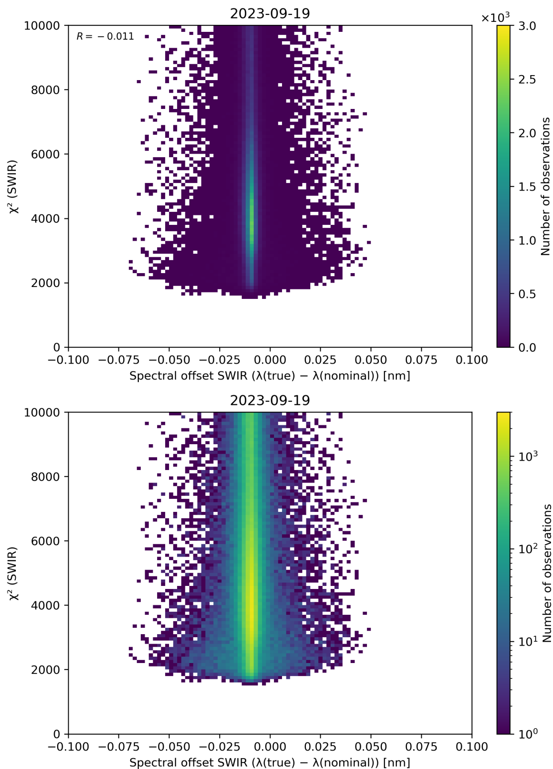
Figure 118: Scatter density plot of “Spectral offset SWIR ( \lambda(\text{true}) - \lambda(\text{nominal}) )” against “ \chi^2 (SWIR)” for 2023-09-18 to 2023-09-20.
