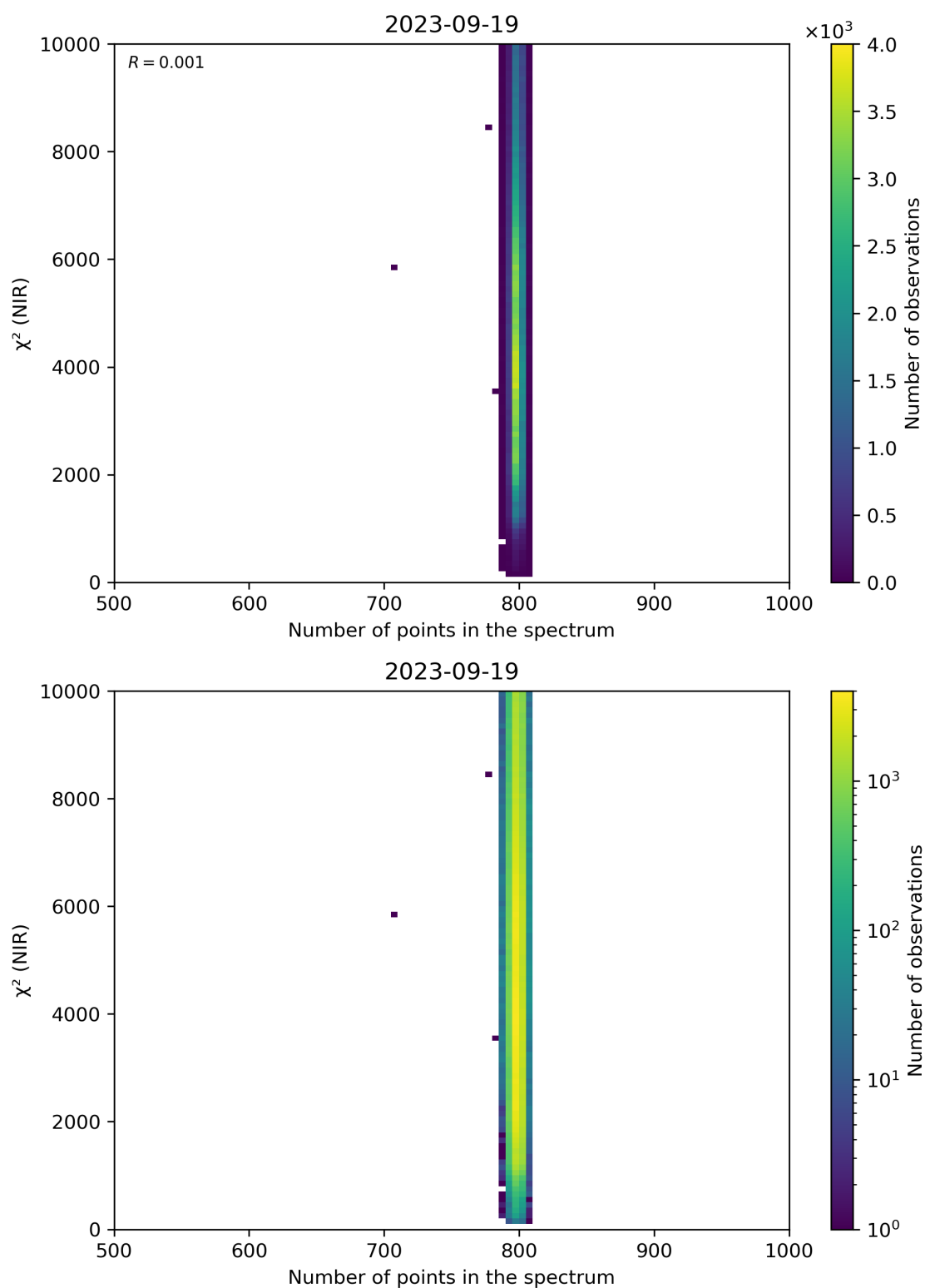
Figure 88: Scatter density plot of “Number of points in the spectrum” against “ \chi^2 (NIR)” for 2023-09-18 to 2023-09-20.
