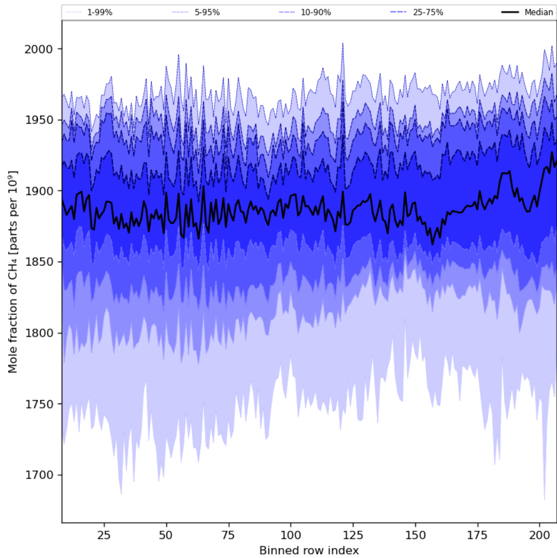
Figure 34: Along track statistics of “Mole fraction of CH 4 ” for 2023-09-18 to 2023-09-20
