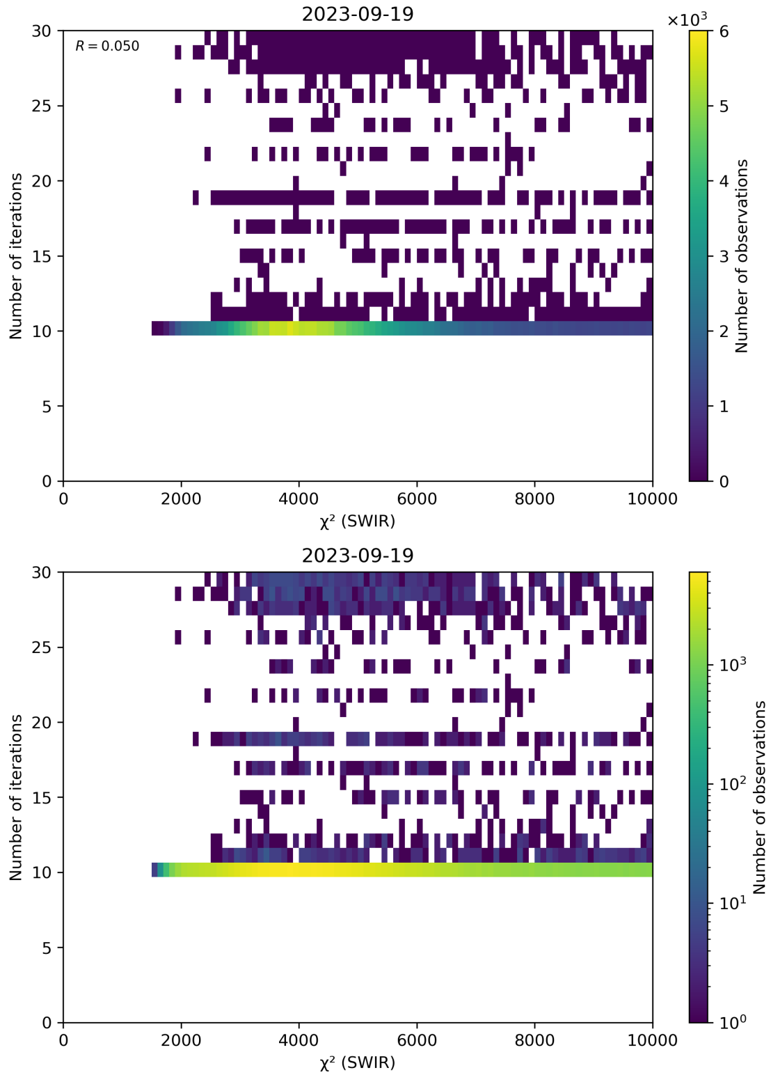
Figure 50: Scatter density plot of “ \chi^2 (SWIR)” against “Number of iterations” for 2023-09-18 to 2023-09-20.
