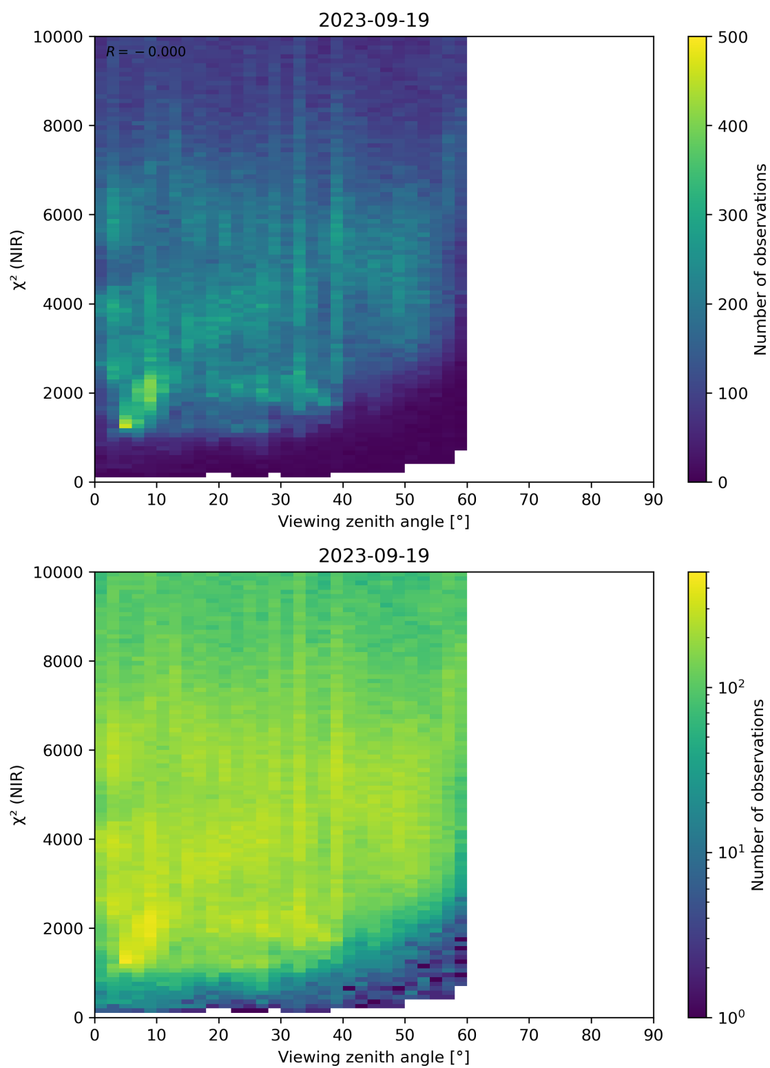
Figure 105: Scatter density plot of “Viewing zenith angle” against “ \chi^2 (NIR)” for 2023-09-18 to 2023-09-20.
