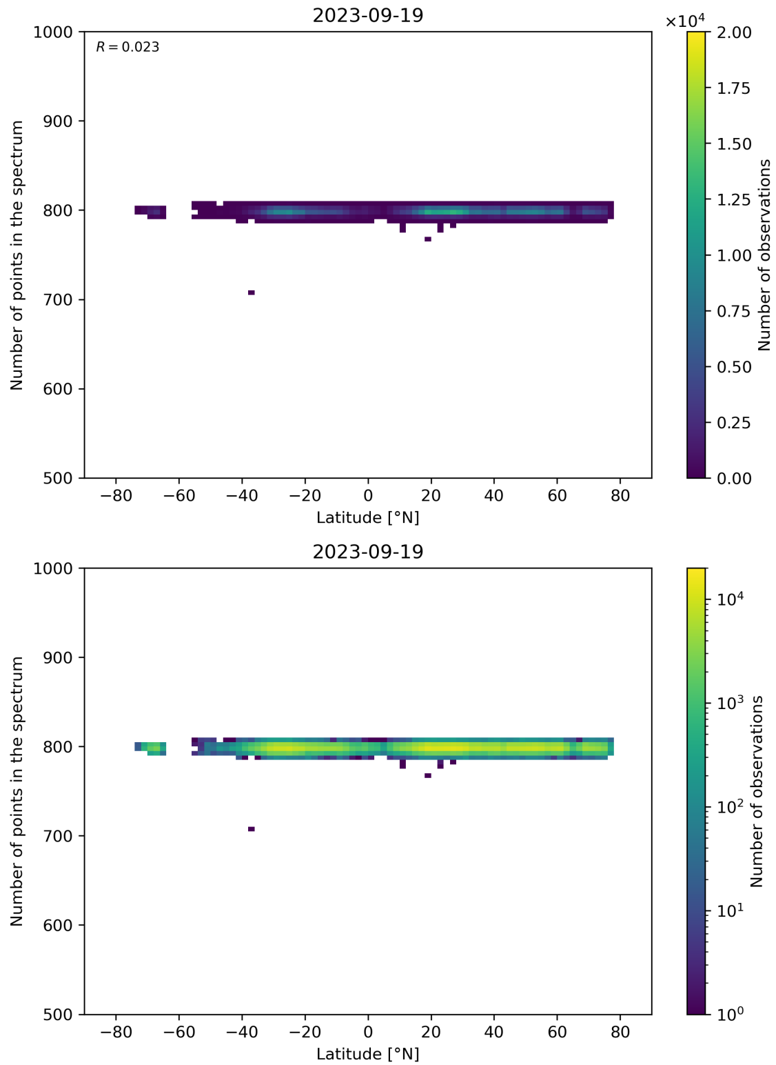
Figure 61: Scatter density plot of “Latitude” against “Number of points in the spectrum” for 2023-09-18 to 2023-09-20.
