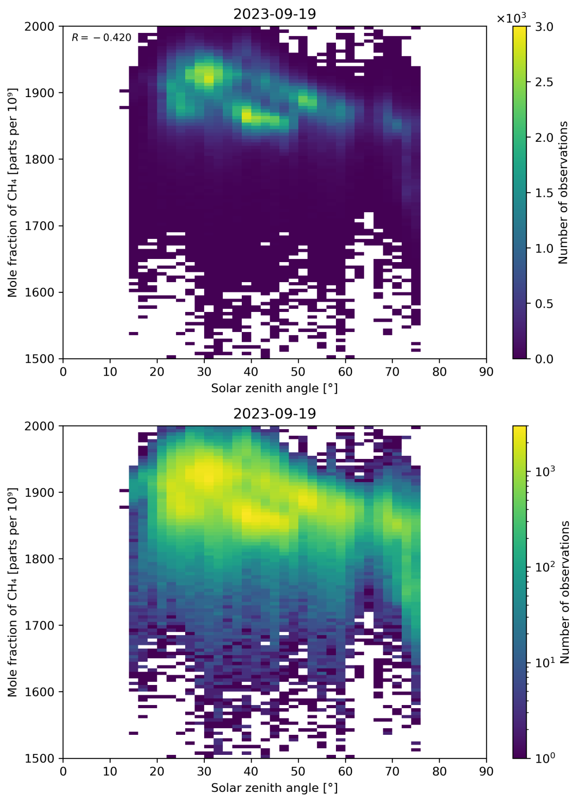
Figure 99: Scatter density plot of “Solar zenith angle” against “Mole fraction of \text{CH}_4 ” for 2023-09-18 to 2023-09-20.
