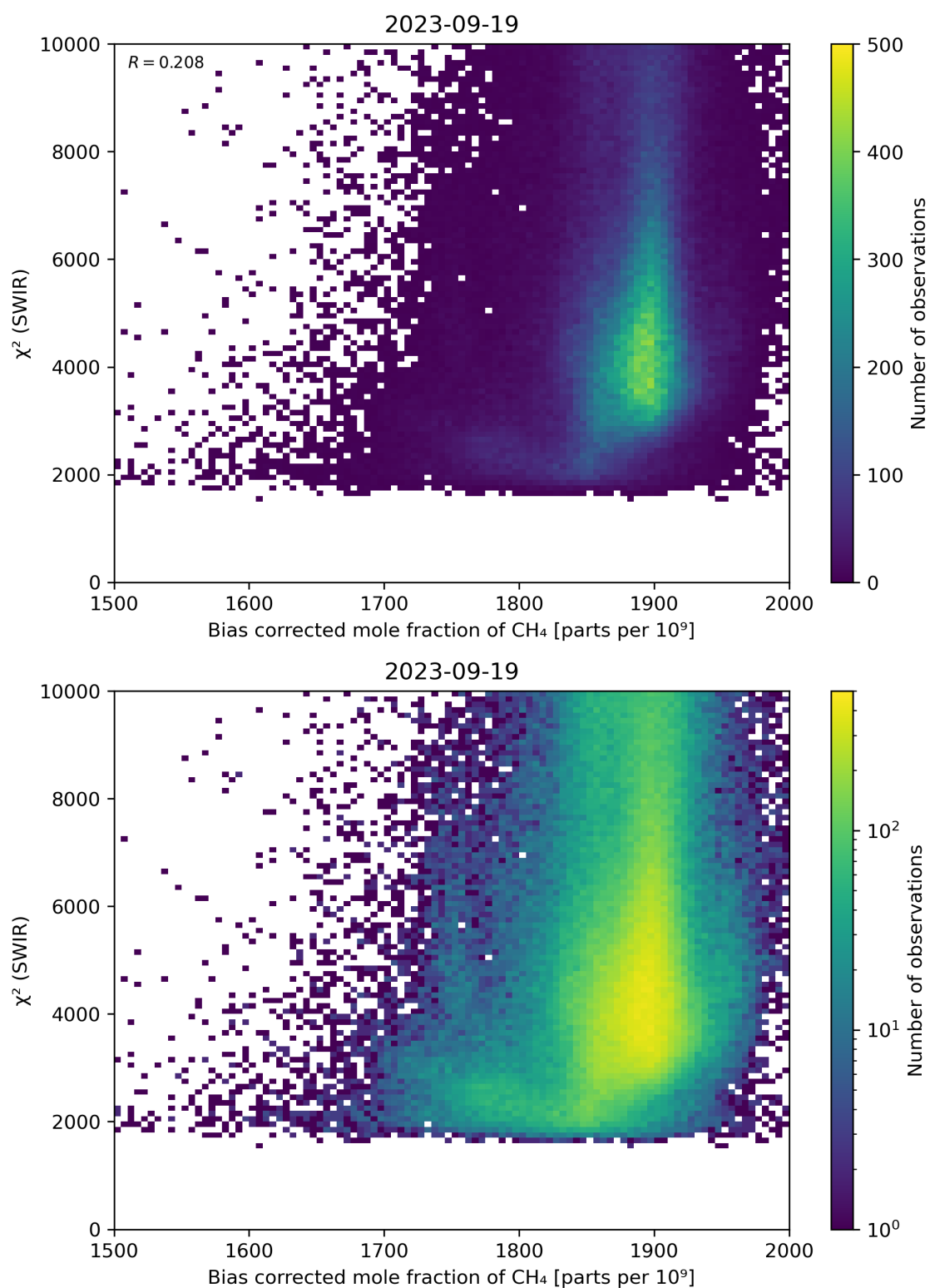
Figure 64: Scatter density plot of “Bias corrected mole fraction of \text{CH}_4 ” against “ \chi^2 (SWIR)” for 2023-09-18 to 2023-09-20.
