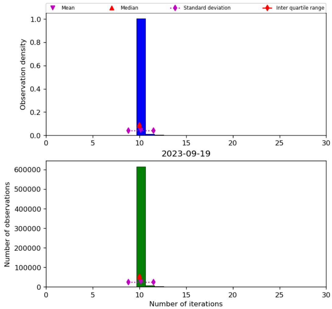
Figure 31: Histogram of “Number of iterations” for 2023-09-18 to 2023-09-20
