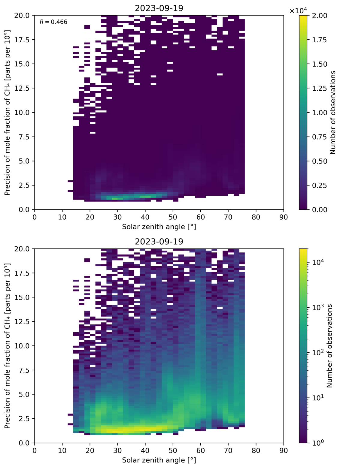
Figure 101: Scatter density plot of “Solar zenith angle” against “Precision of mole fraction of CH 4 ” for 2023-09-18 to 2023-09-20.
