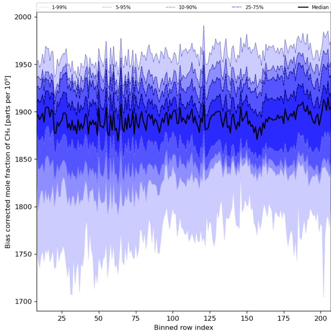
Figure 36: Along track statistics of “Bias corrected mole fraction of CH 4 ” for 2023-09-18 to 2023-09-20
