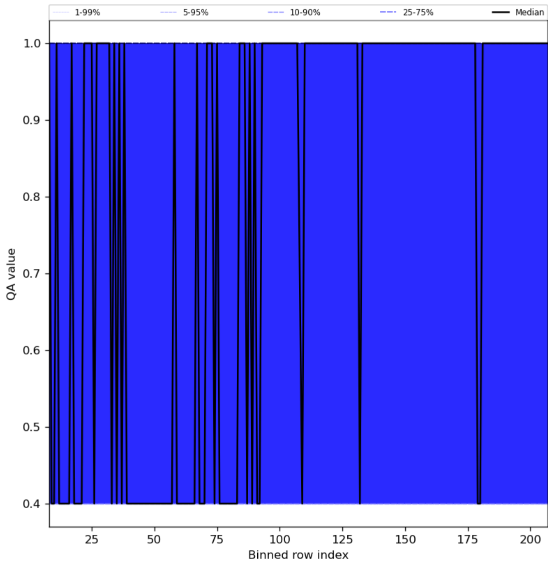
Figure 33: Along track statistics of “QA value” for 2023-09-18 to 2023-09-20
