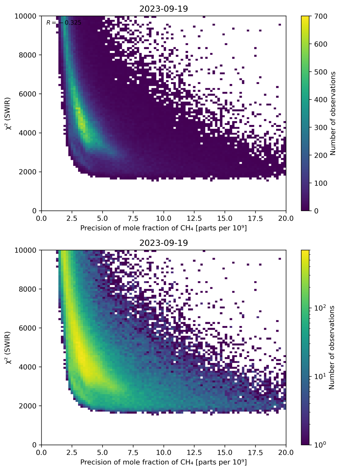
Figure 79: Scatter density plot of “Precision of mole fraction of CH 4 ” against “ \chi^2 (SWIR)” for 2023-09-18 to 2023-09-20.
