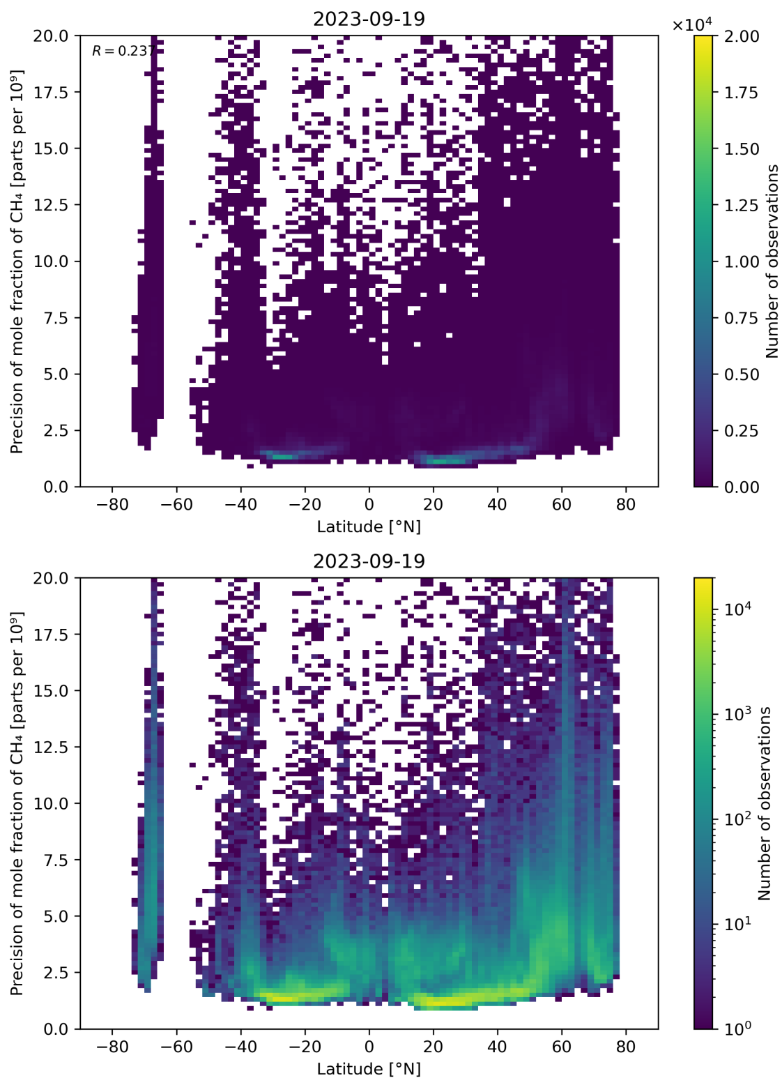
Figure 59: Scatter density plot of “Latitude” against “Precision of mole fraction of CH 4 ” for 2023-09-18 to 2023-09-20.
