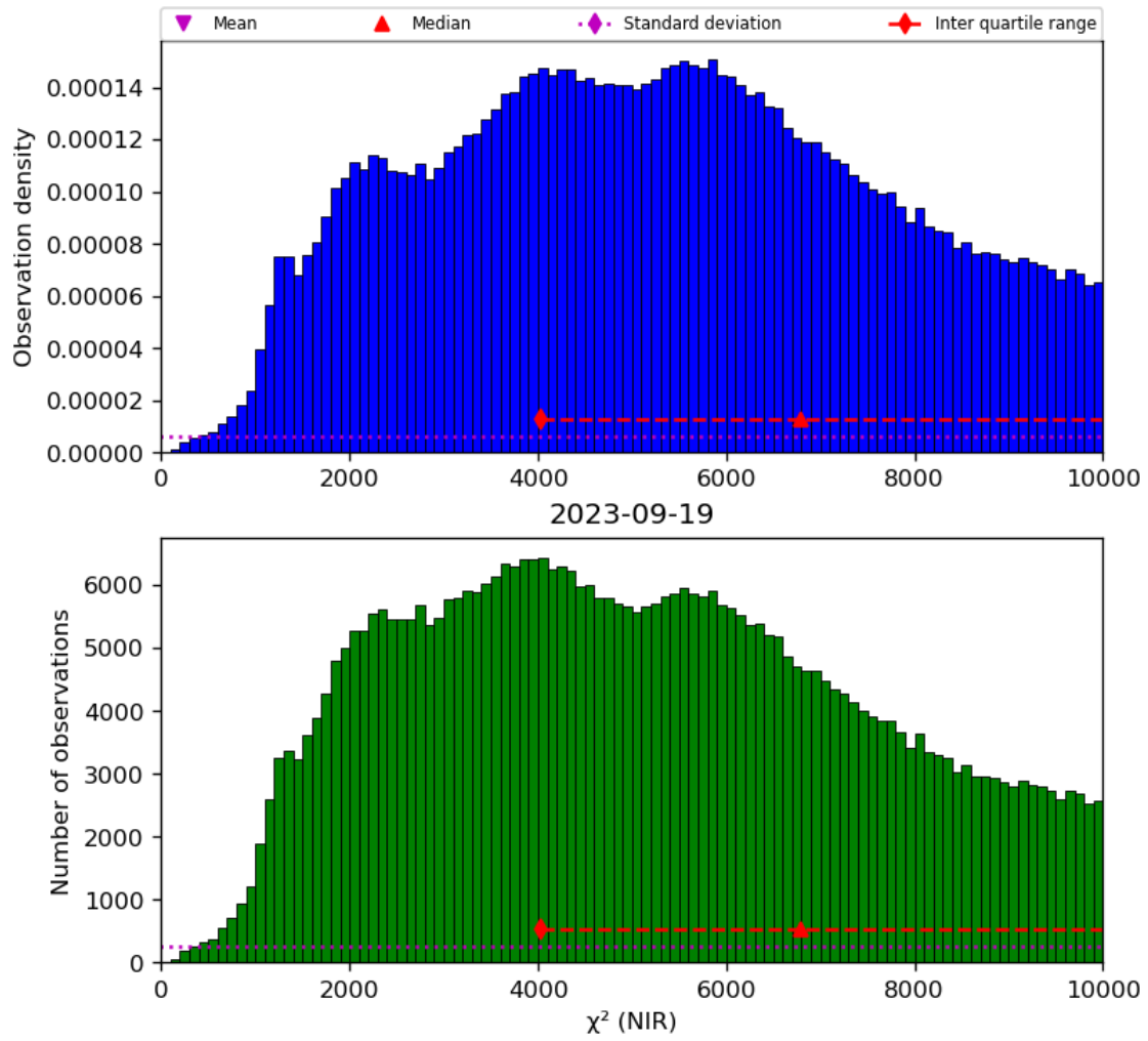
Figure 29: Histogram of “ \chi^2 (NIR)” for 2023-09-18 to 2023-09-20
