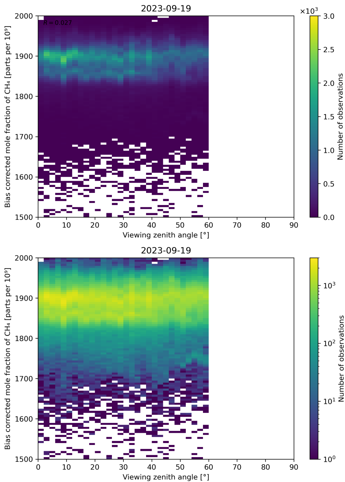
Figure 111: Scatter density plot of “Viewing zenith angle” against “Bias corrected mole fraction of \text{CH}_4 ” for 2023-09-18 to 2023-09-20.
