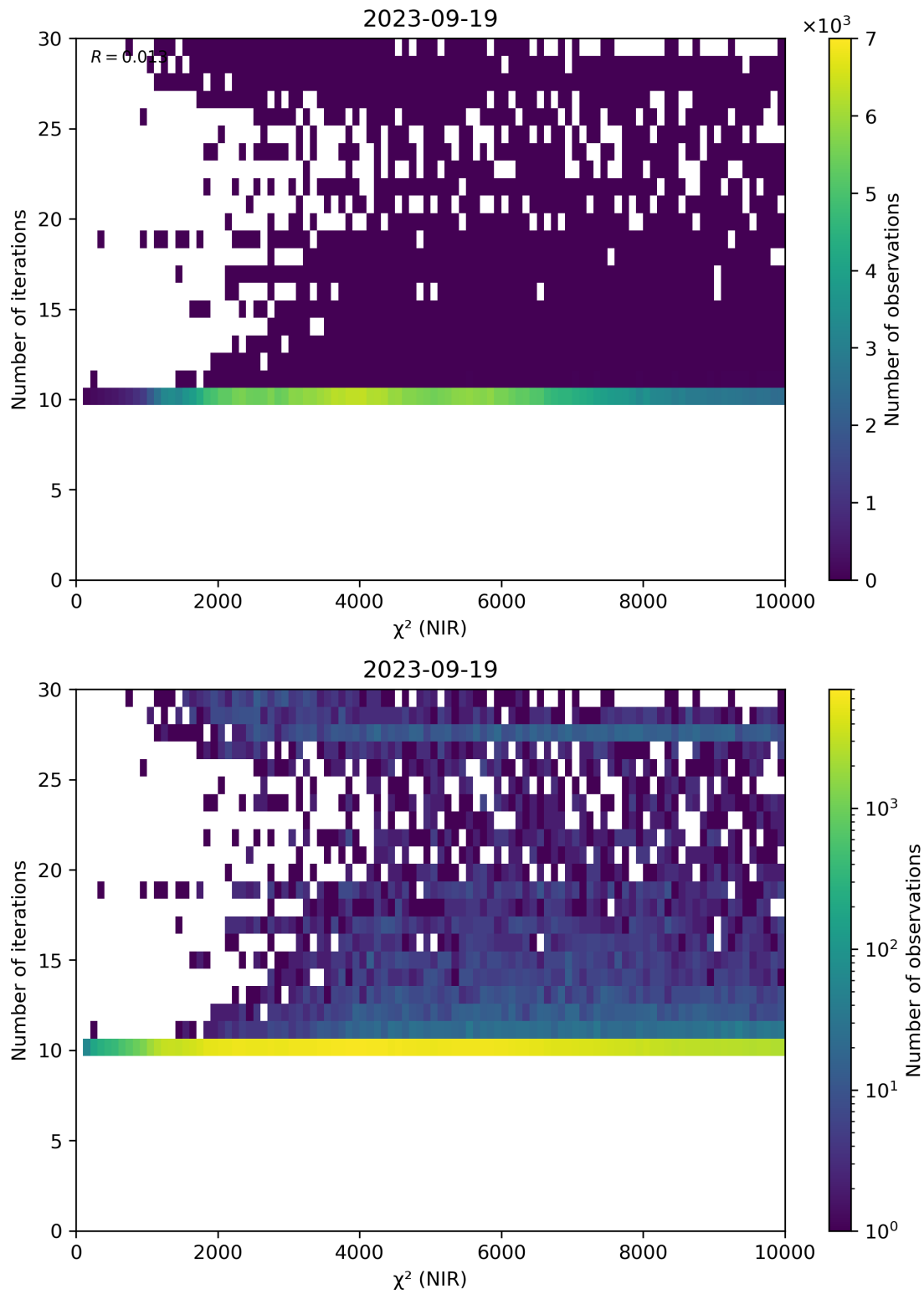
Figure 46: Scatter density plot of “ \chi^2 (NIR)” against “Number of iterations” for 2023-09-18 to 2023-09-20.
