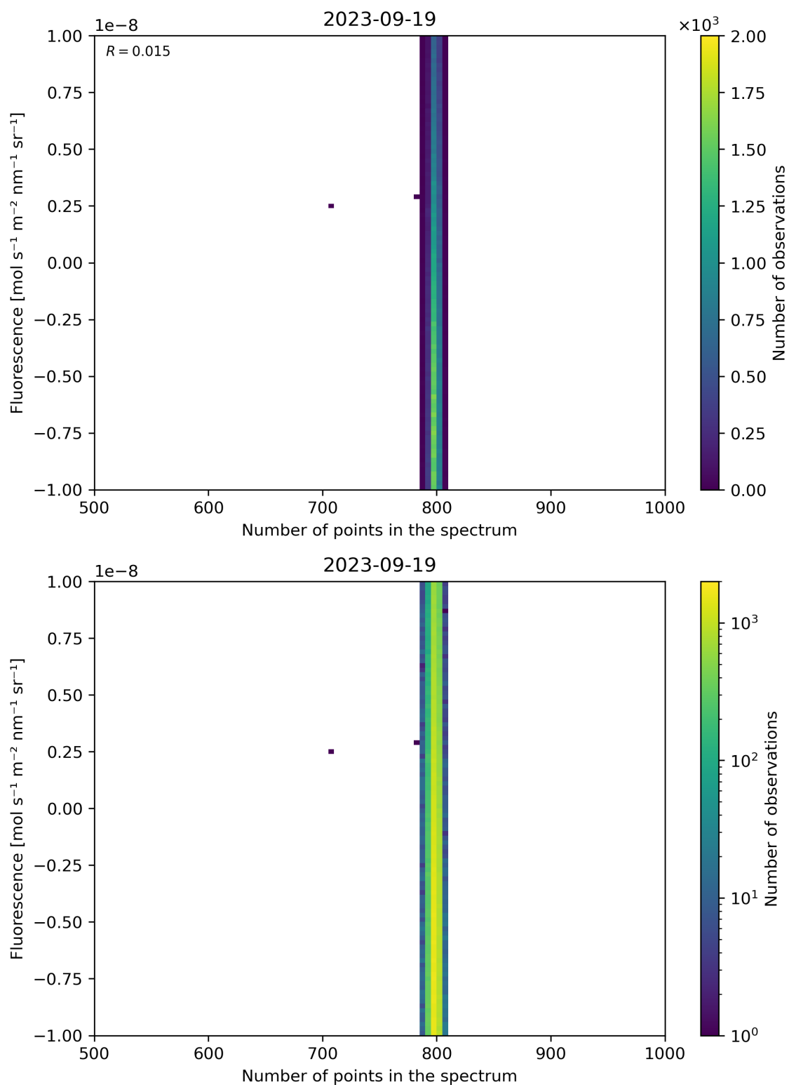
Figure 91: Scatter density plot of “Number of points in the spectrum” against “Fluorescence” for 2023-09-18 to 2023-09-20.
