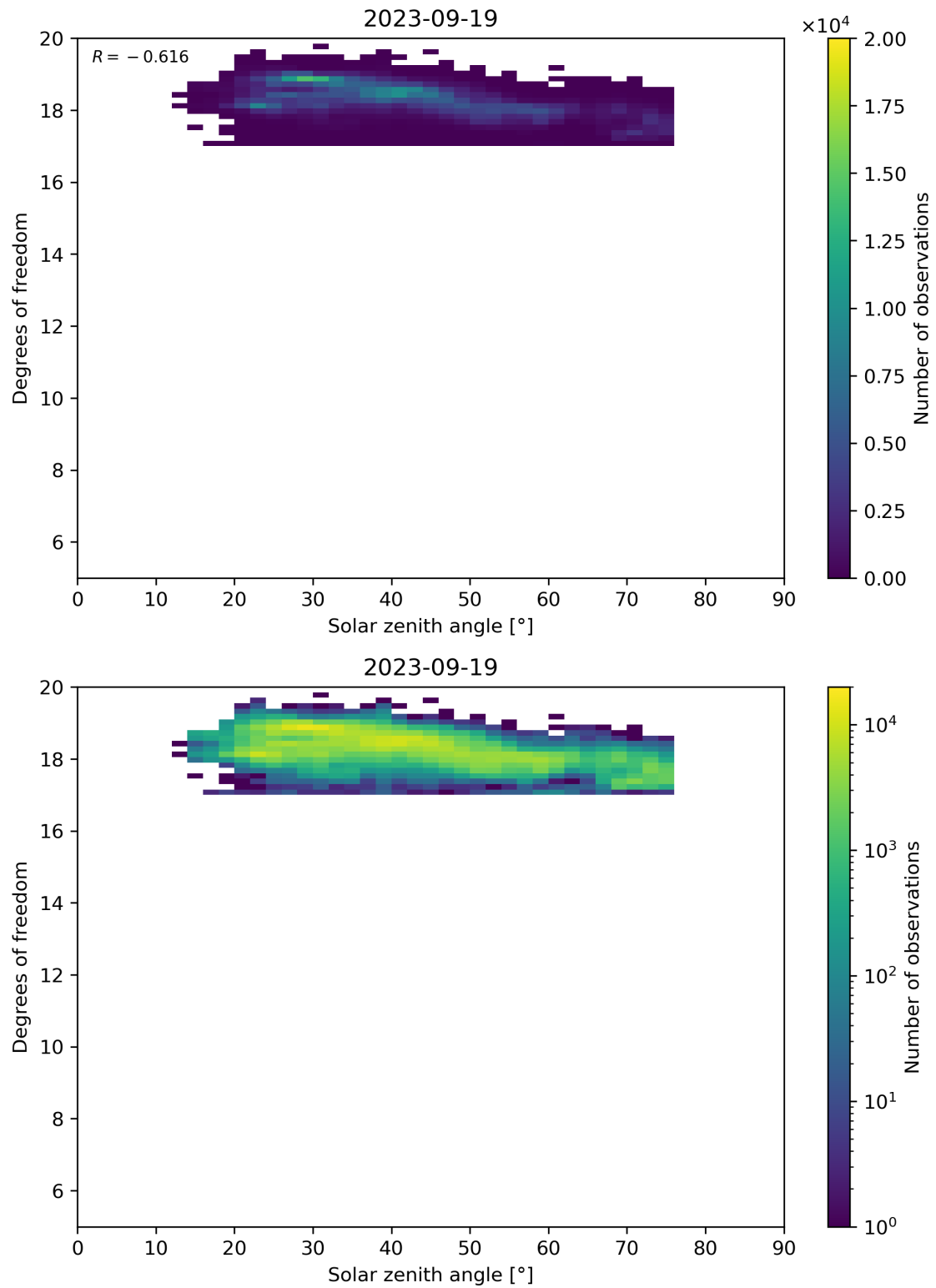
Figure 96: Scatter density plot of “Solar zenith angle” against “Degrees of freedom” for 2023-09-18 to 2023-09-20.
