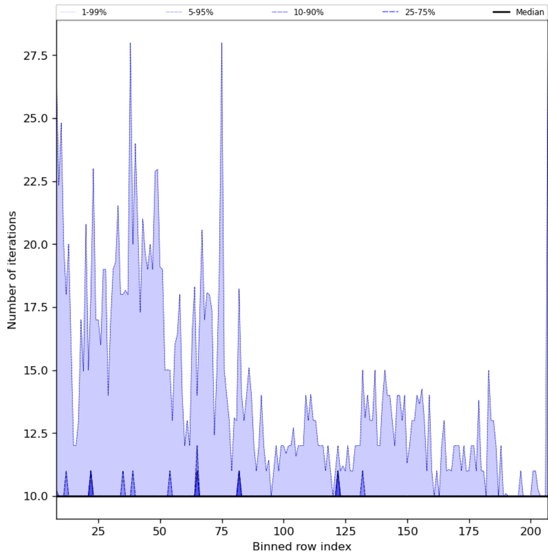
Figure 42: Along track statistics of “Number of iterations” for 2023-09-18 to 2023-09-20
