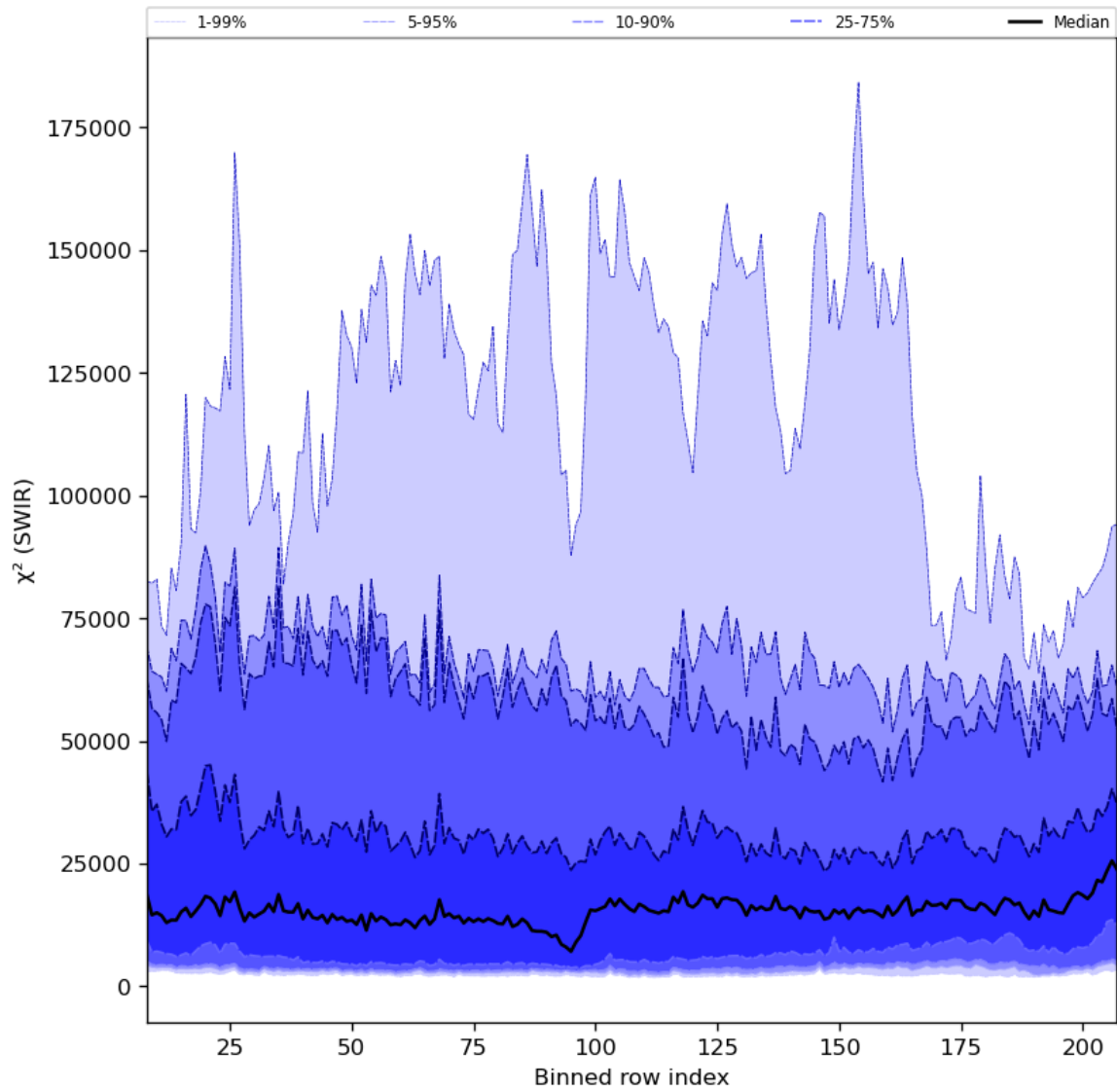
Figure 39: Along track statistics of “ \chi^2 (SWIR)” for 2023-09-18 to 2023-09-20
