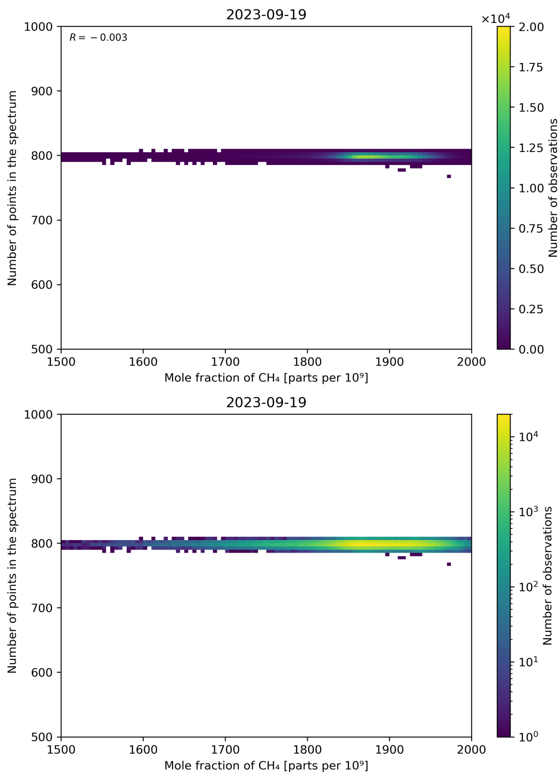
Figure 77: Scatter density plot of “Mole fraction of CH 4 ” against “Number of points in the spectrum” for 2023-09-18 to 2023-09-20.
