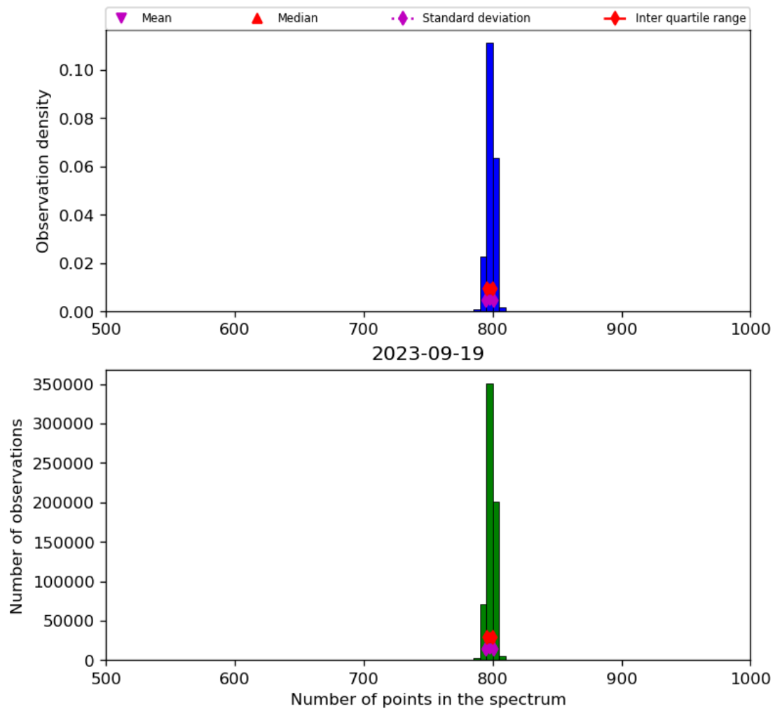
Figure 26: Histogram of “Number of points in the spectrum” for 2023-09-18 to 2023-09-20
