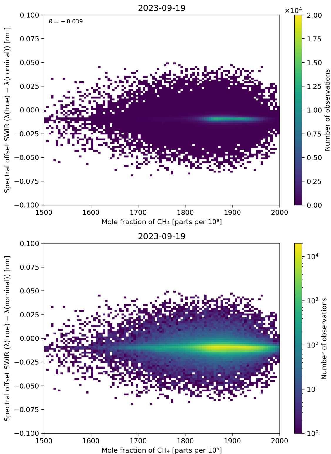
Figure 86: Scatter density plot of “Mole fraction of CH 4 ” against “Spectral offset SWIR ( \lambda(\text{true}) - \lambda(\text{nominal}) )” for 2023-09-18 to 2023-09-20.
