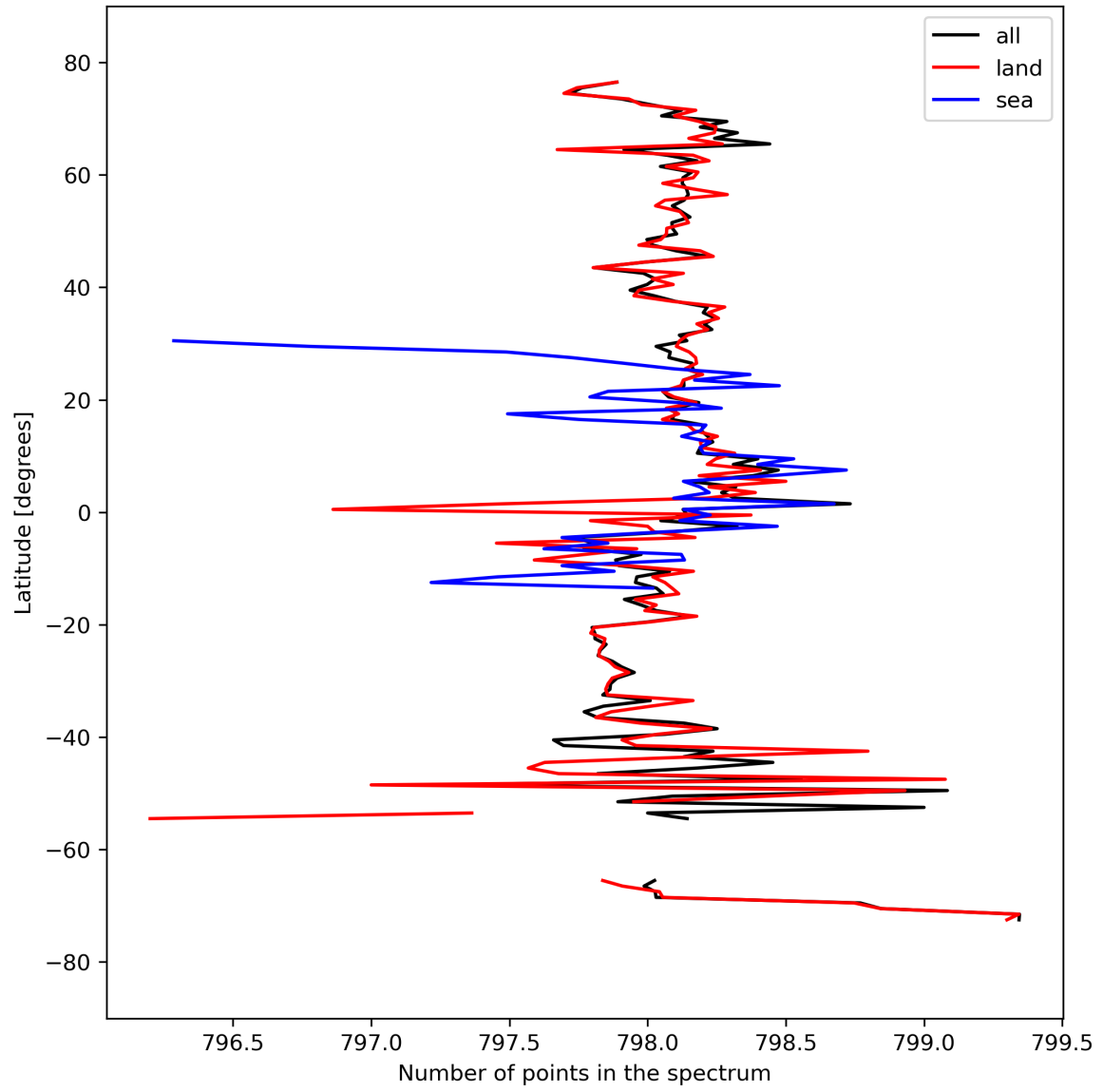
Figure 15: Zonal average of “Number of points in the spectrum” for 2023-09-18 to 2023-09-20.
