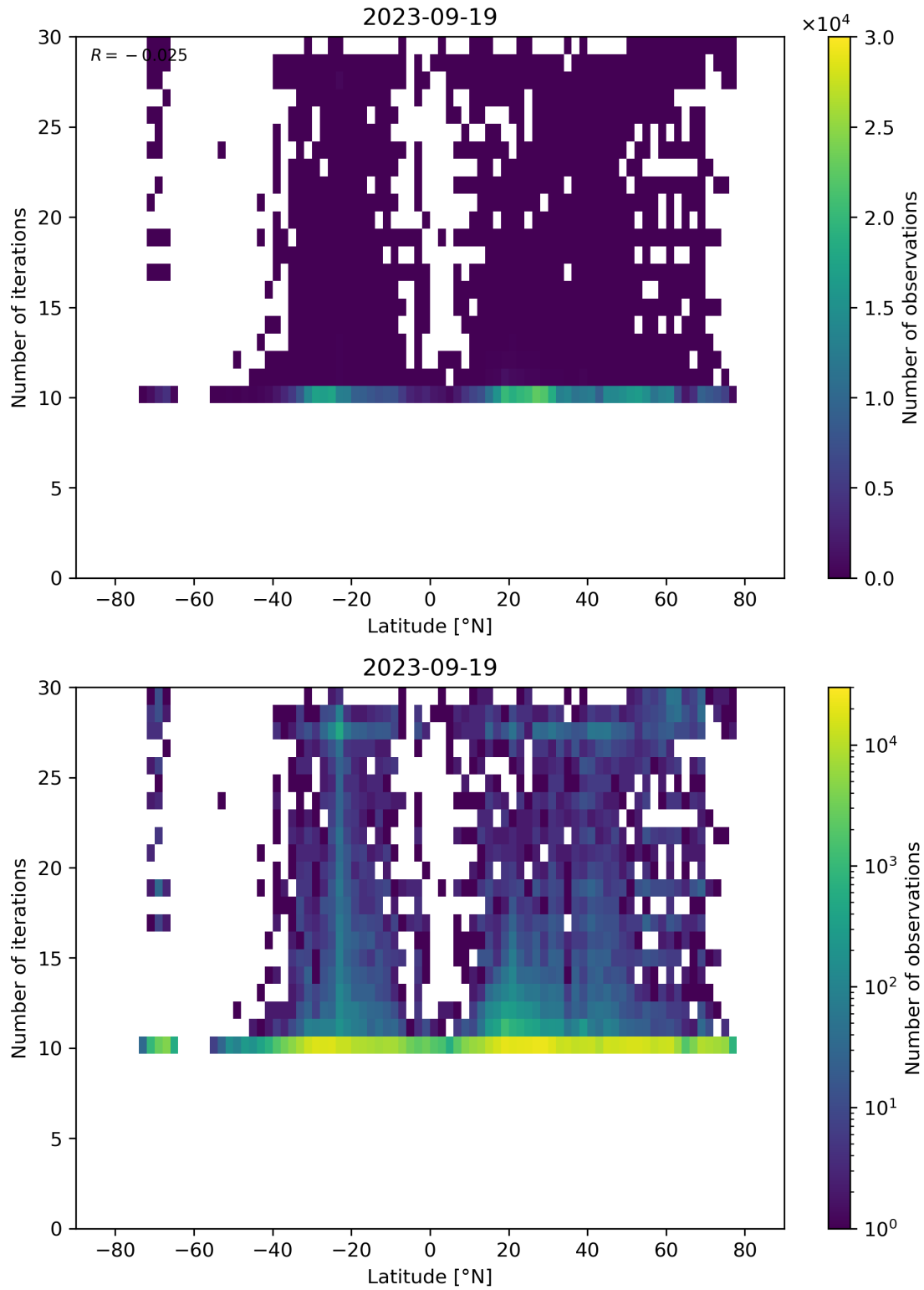
Figure 60: Scatter density plot of “Latitude” against “Number of iterations” for 2023-09-18 to 2023-09-20.
