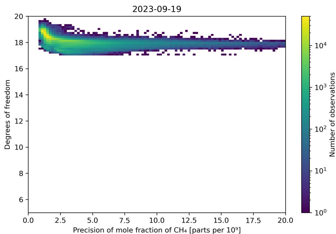
Figure 80: Scatter density plot of “Precision of mole fraction of CH 4 ” against “Degrees of freedom” for 2023-09-18 to 2023-09-20.
