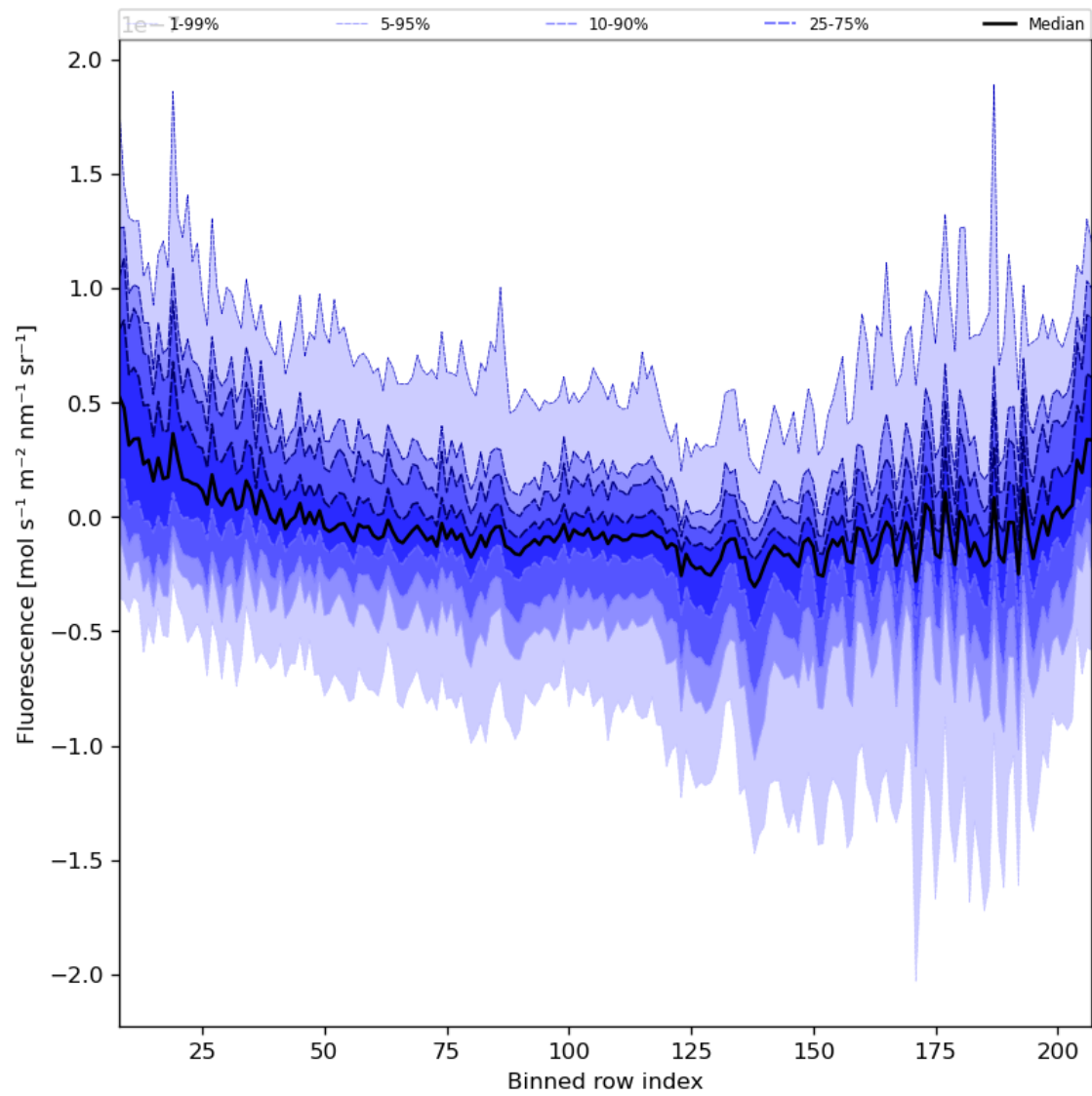
Figure 43: Along track statistics of “Fluorescence” for 2023-09-20 to 2023-09-21
