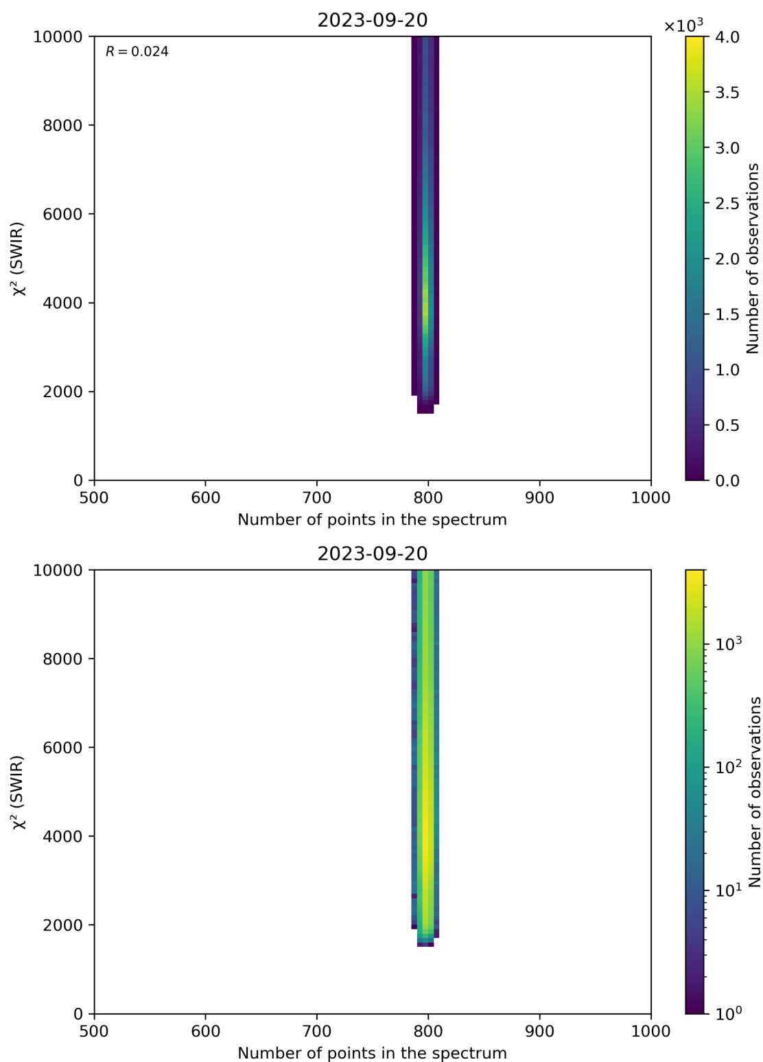
Figure 89: Scatter density plot of “Number of points in the spectrum” against “ \chi^2 (SWIR)” for 2023-09-20 to 2023-09-21.
