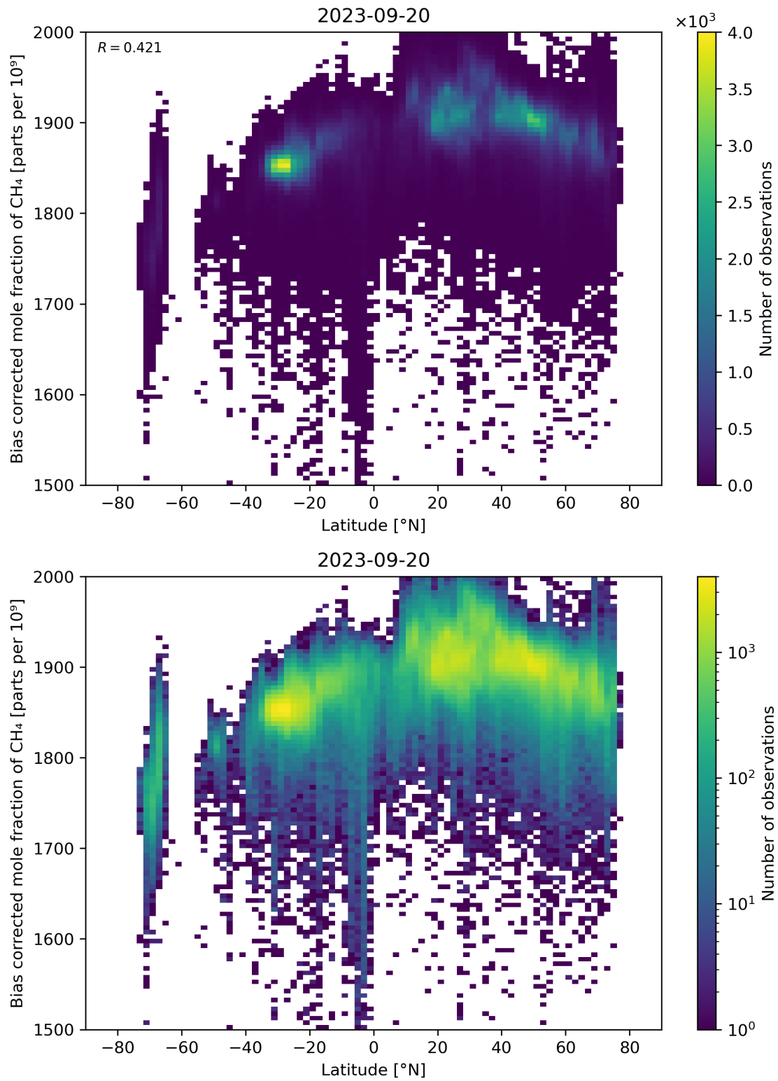
Figure 58: Scatter density plot of “Latitude” against “Bias corrected mole fraction of CH 4 ” for 2023-09-20 to 2023-09-21.
