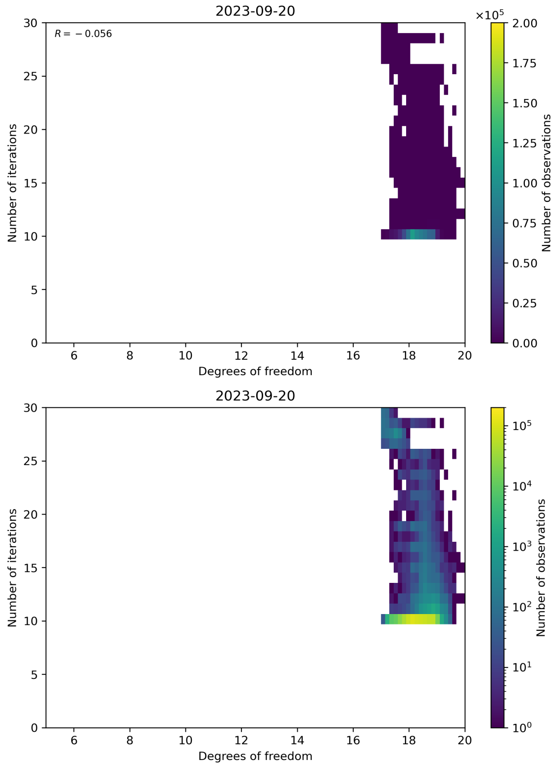
Figure 52: Scatter density plot of “Degrees of freedom” against “Number of iterations” for 2023-09-20 to 2023-09-21.
