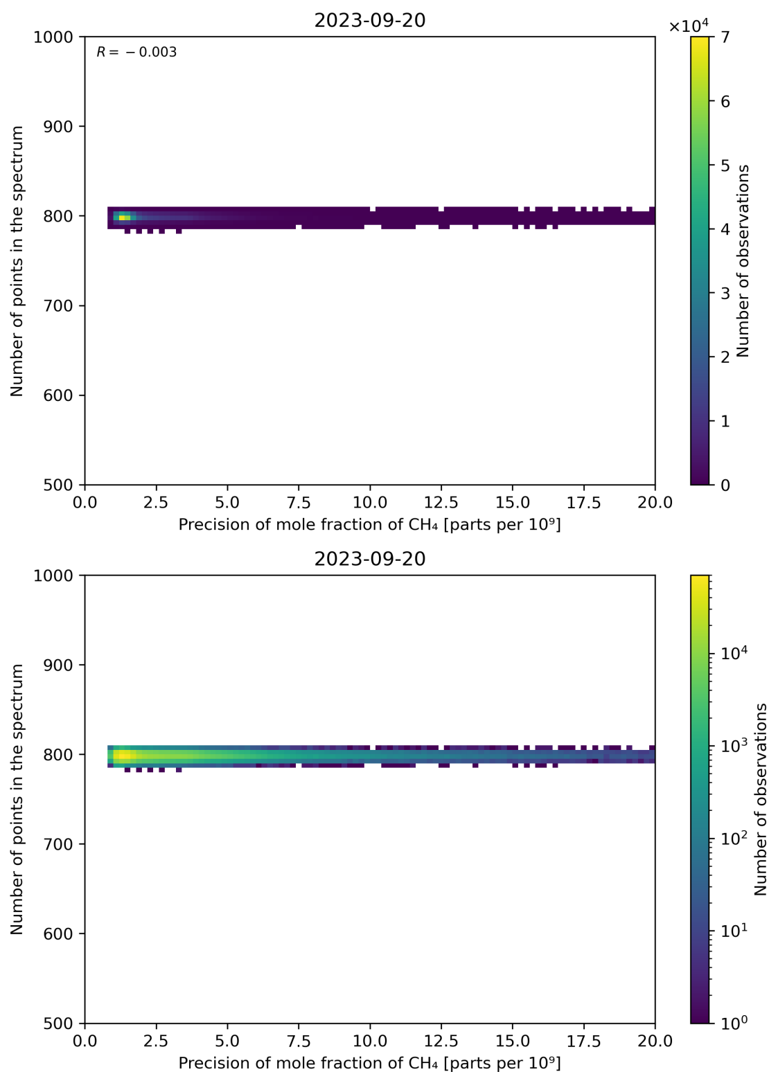
Figure 84: Scatter density plot of “Precision of mole fraction of \text{CH}_4 ” against “Number of points in the spectrum” for 2023-09-20 to 2023-09-21.
