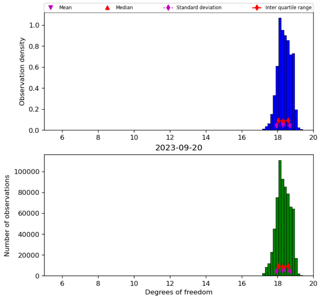
Figure 30: Histogram of “Degrees of freedom” for 2023-09-20 to 2023-09-21
