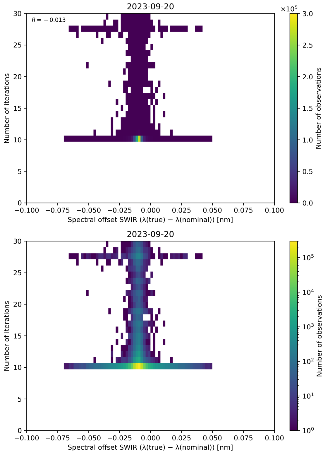
Figure 121: Scatter density plot of “Spectral offset SWIR ( \lambda(\text{true}) - \lambda(\text{nominal}) )” against “Number of iterations” for 2023-09-20 to 2023-09-21.
