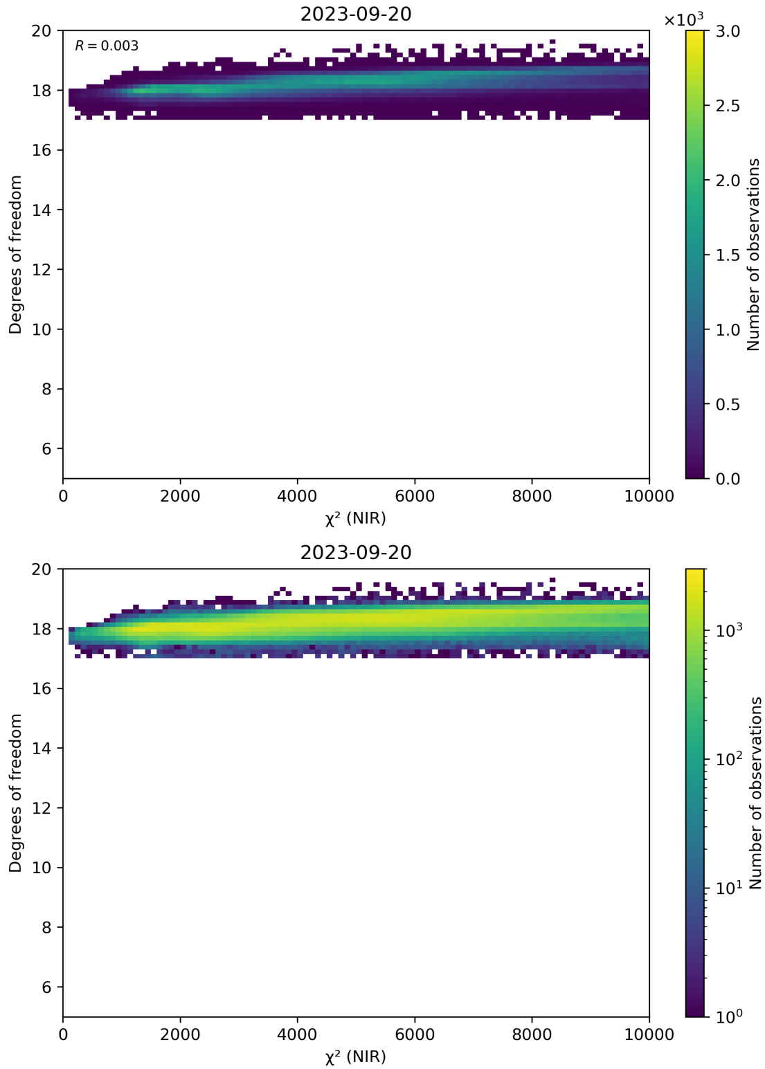
Figure 44: Scatter density plot of “ \chi^2 (NIR)” against “Degrees of freedom” for 2023-09-20 to 2023-09-21.
