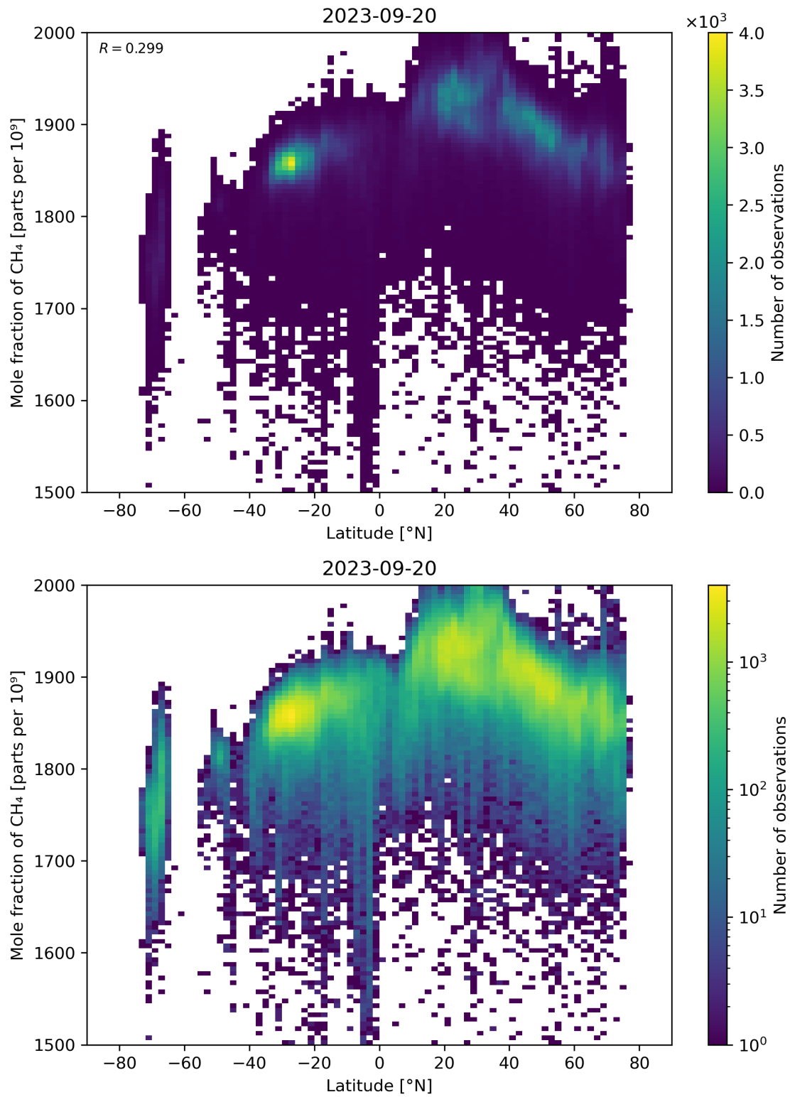
Figure 57: Scatter density plot of “Latitude” against “Mole fraction of CH 4 ” for 2023-09-20 to 2023-09-21.
