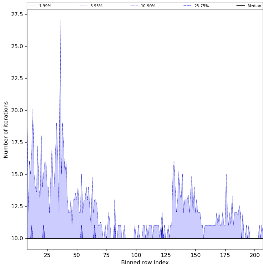
Figure 42: Along track statistics of “Number of iterations” for 2023-09-20 to 2023-09-21
