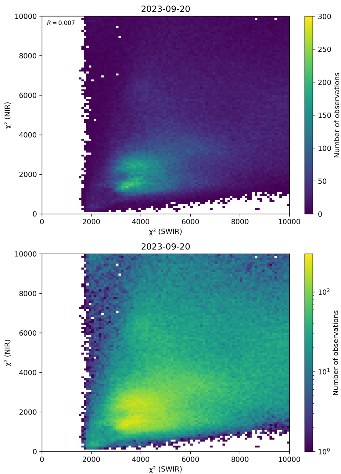
Figure 47: Scatter density plot of “ \chi^2 (SWIR)” against “ \chi^2 (NIR)” for 2023-09-20 to 2023-09-21.
