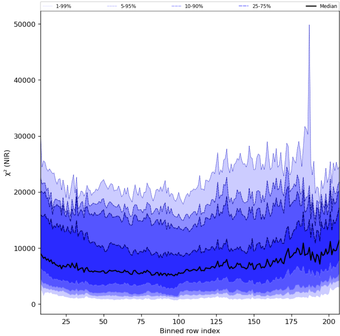
Figure 40: Along track statistics of “ \chi^2 (NIR)” for 2023-09-20 to 2023-09-21
