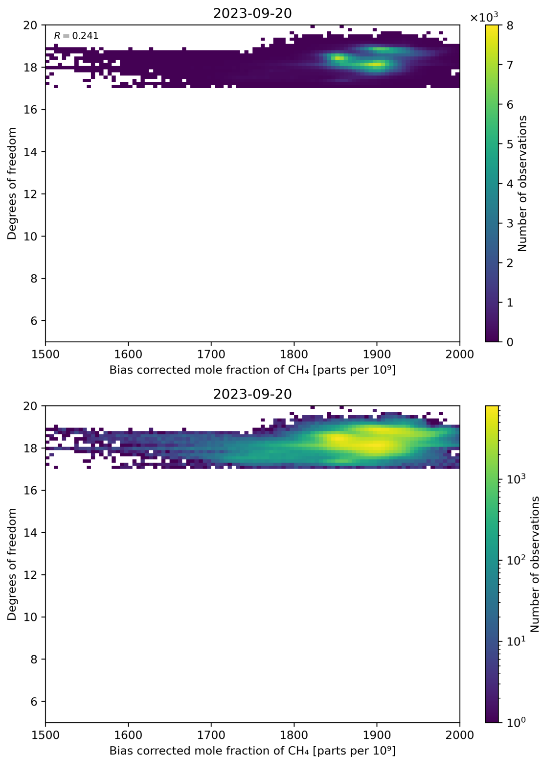
Figure 65: Scatter density plot of “Bias corrected mole fraction of CH 4 ” against “Degrees of freedom” for 2023-09-20 to 2023-09-21.
