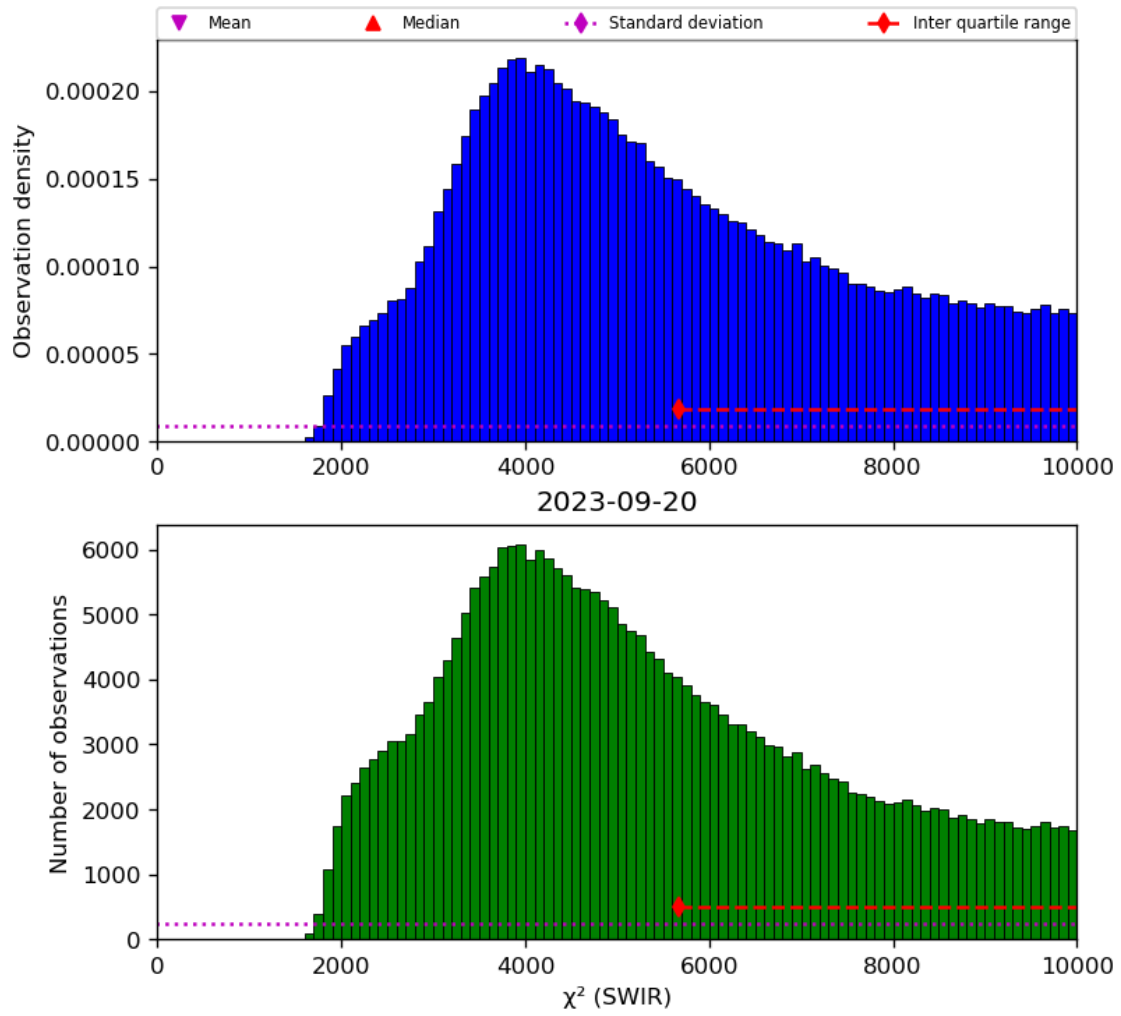
Figure 28: Histogram of " \chi^2 (SWIR)" for 2023-09-20 to 2023-09-21
