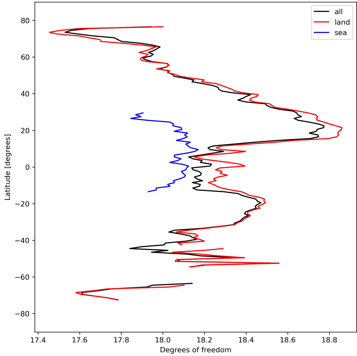
Figure 19: Zonal average of “Degrees of freedom” for 2023-09-20 to 2023-09-21.
