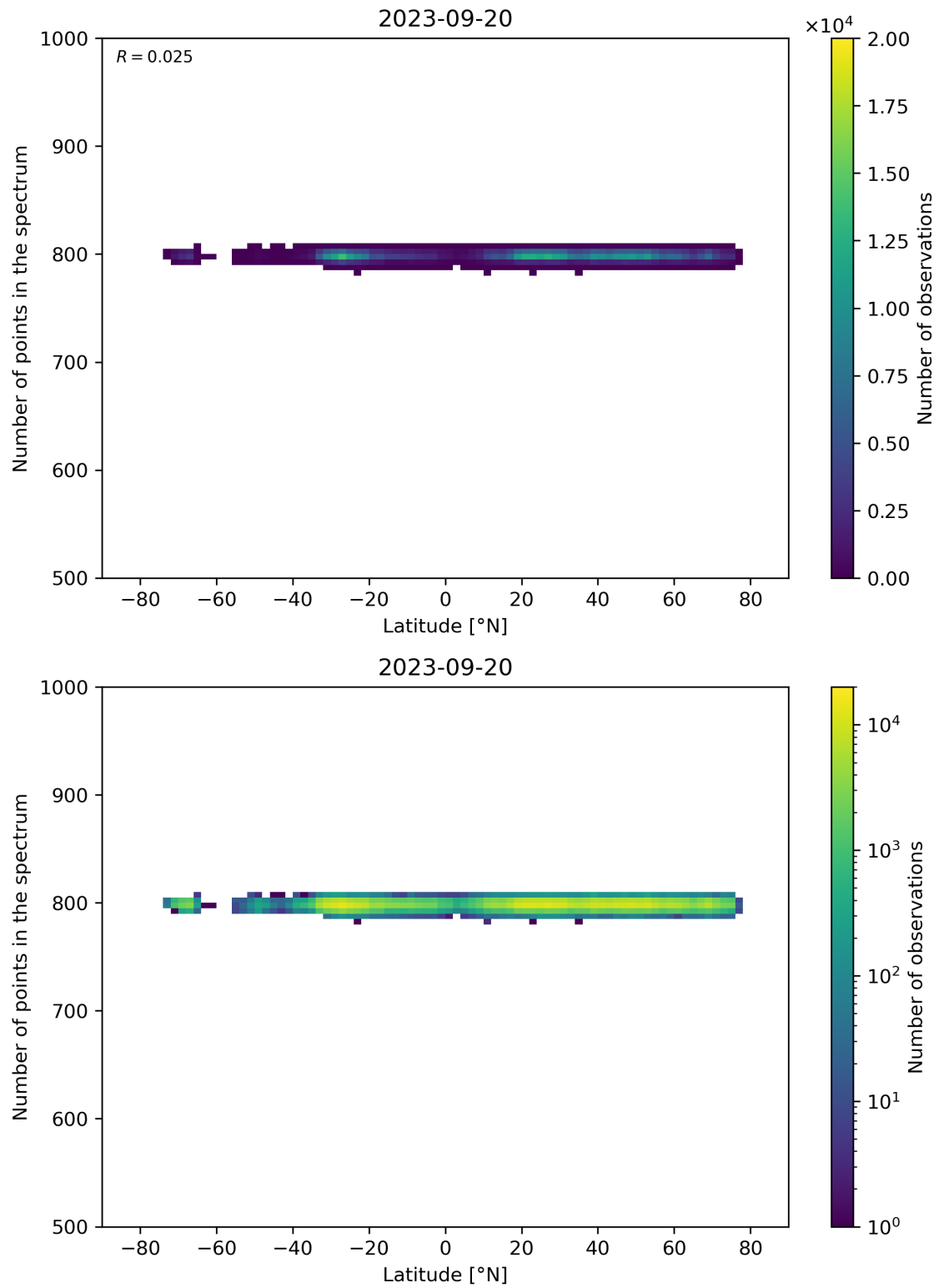
Figure 61: Scatter density plot of “Latitude” against “Number of points in the spectrum” for 2023-09-20 to 2023-09-21.
