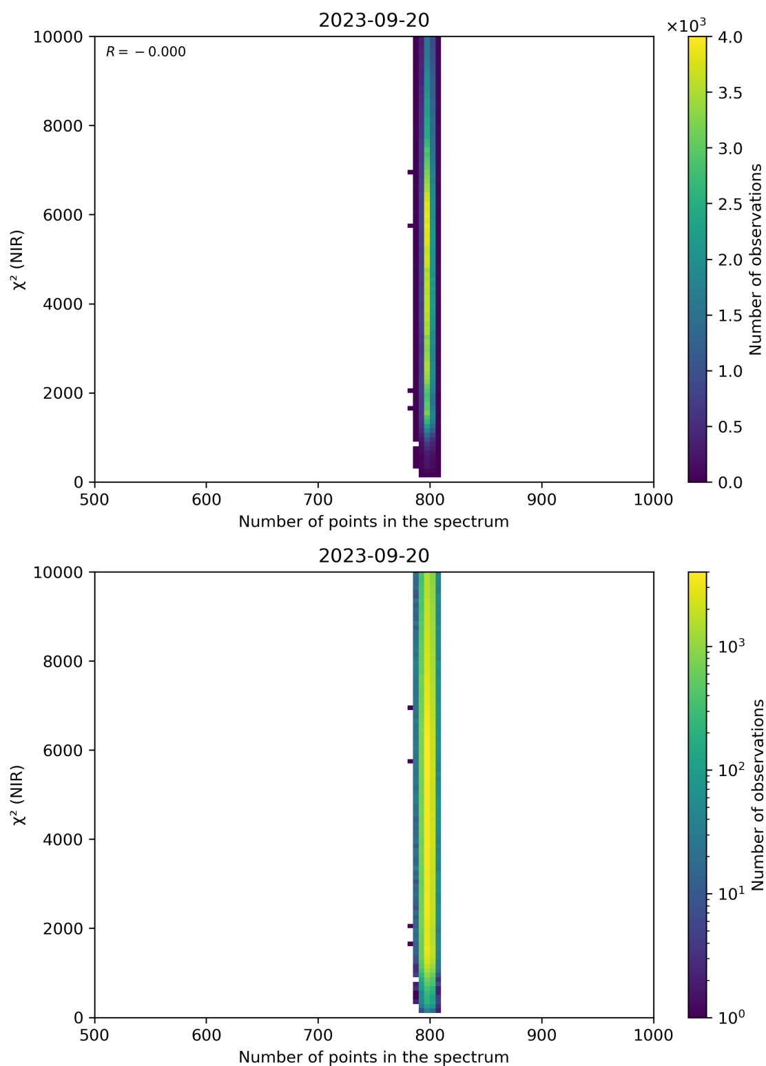
Figure 88: Scatter density plot of “Number of points in the spectrum” against “ \chi^2 (NIR)” for 2023-09-20 to 2023-09-21.
