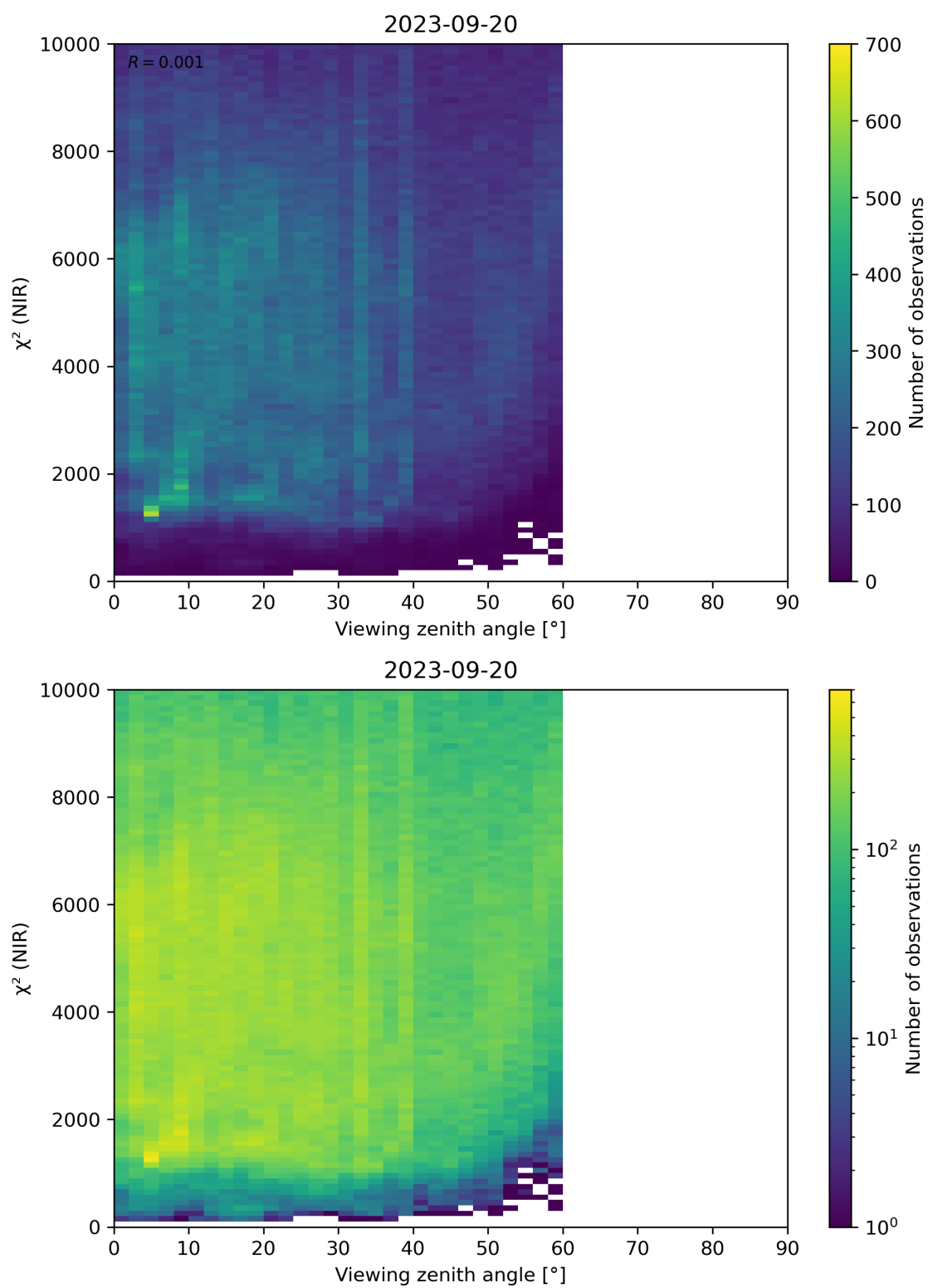
Figure 105: Scatter density plot of “Viewing zenith angle” against “ \chi^2 (NIR)” for 2023-09-20 to 2023-09-21.
