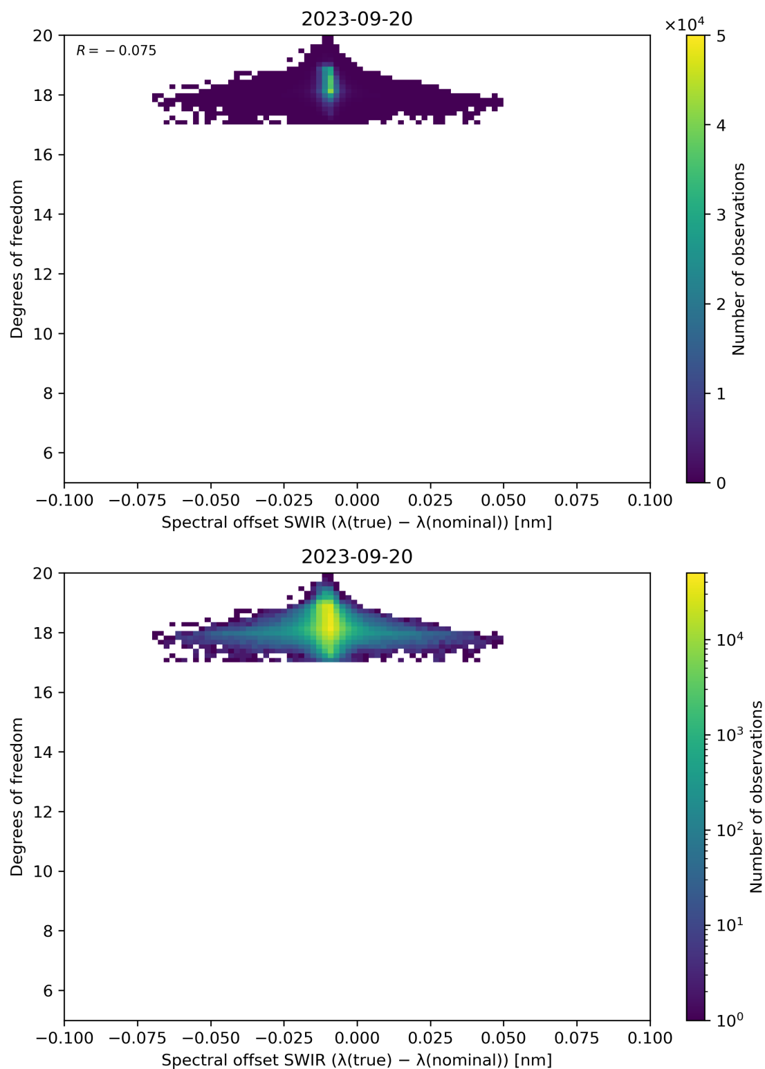
Figure 119: Scatter density plot of “Spectral offset SWIR ( \lambda(\text{true}) - \lambda(\text{nominal}) )” against “Degrees of freedom” for 2023-09-20 to 2023-09-21.
