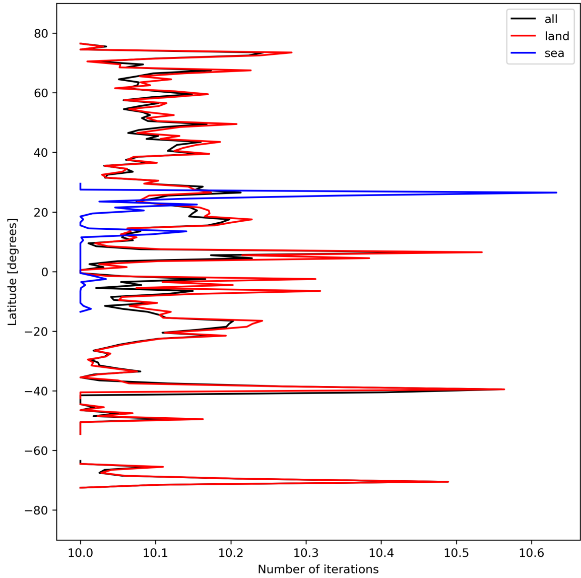
Figure 20: Zonal average of “Number of iterations” for 2023-09-20 to 2023-09-21.
