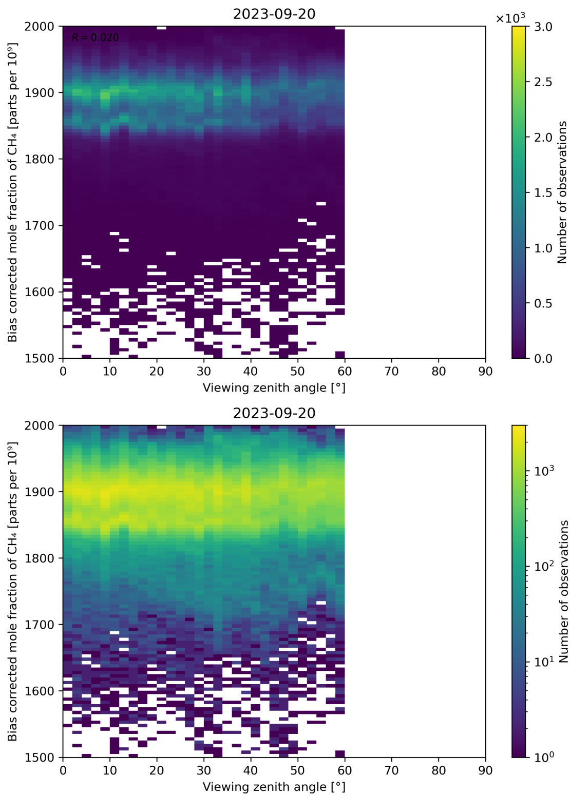
Figure 111: Scatter density plot of “Viewing zenith angle” against “Bias corrected mole fraction of CH 4 ” for 2023-09-20 to 2023-09-21.
