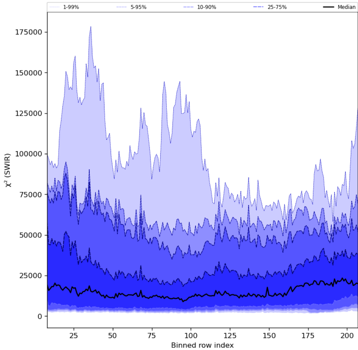
Figure 39: Along track statistics of “ \chi^2 (SWIR)” for 2023-09-20 to 2023-09-21
