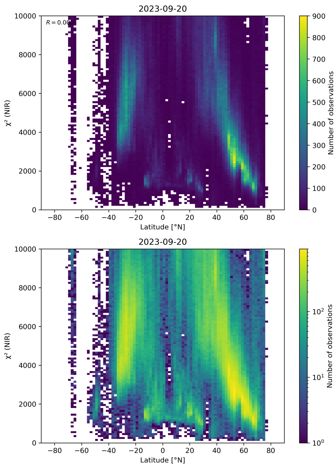
Figure 53: Scatter density plot of “Latitude” against “ \chi^2 (NIR)” for 2023-09-20 to 2023-09-21.
