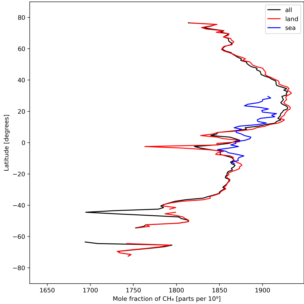
Figure 12: Zonal average of “Mole fraction of CH 4 ” for 2023-09-20 to 2023-09-21.
