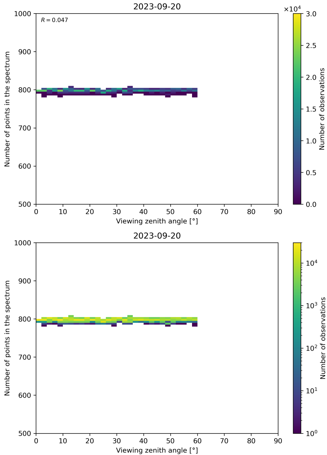
Figure 114: Scatter density plot of “Viewing zenith angle” against “Number of points in the spectrum” for 2023-09-20 to 2023-09-21.
