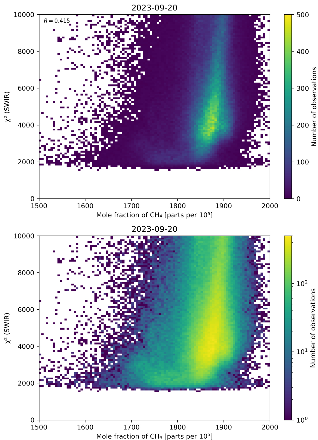
Figure 71: Scatter density plot of “Mole fraction of \text{CH}_4 ” against “ \chi^2 (SWIR)” for 2023-09-20 to 2023-09-21.
