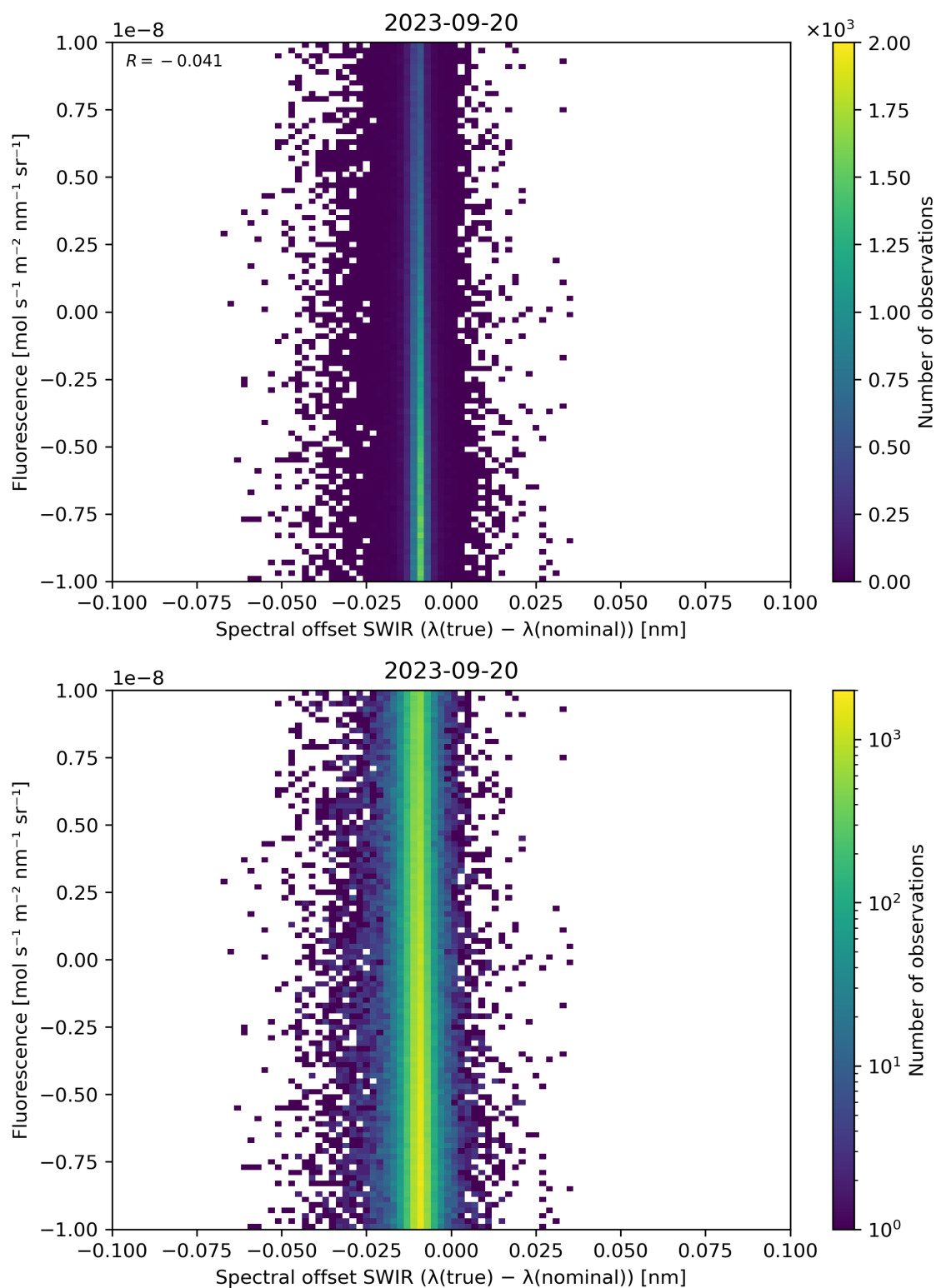
Figure 120: Scatter density plot of “Spectral offset SWIR ( \lambda(\text{true}) - \lambda(\text{nominal}) )” against “Fluorescence” for 2023-09-20 to 2023-09-21.
