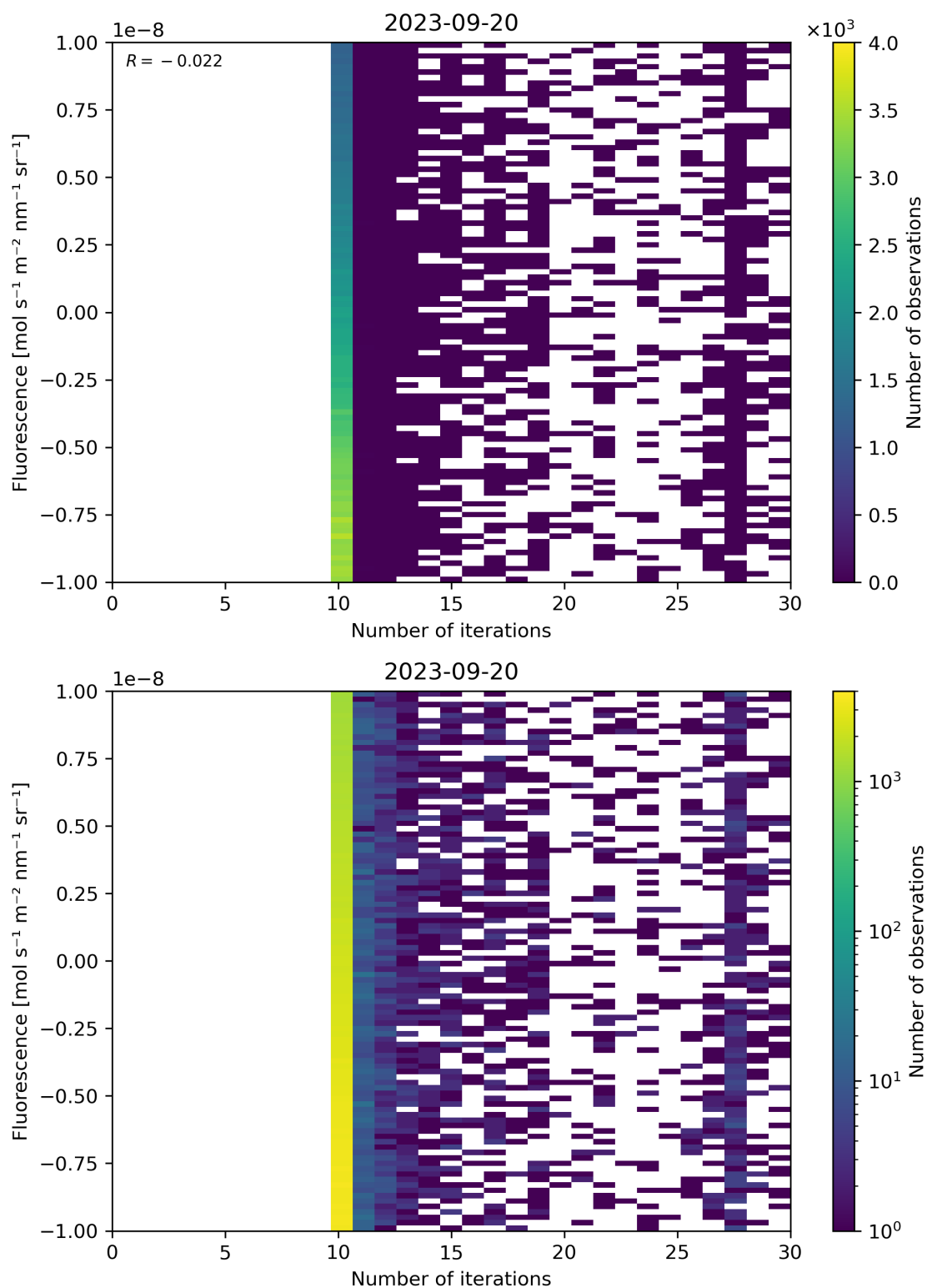
Figure 87: Scatter density plot of “Number of iterations” against “Fluorescence” for 2023-09-20 to 2023-09-21.
