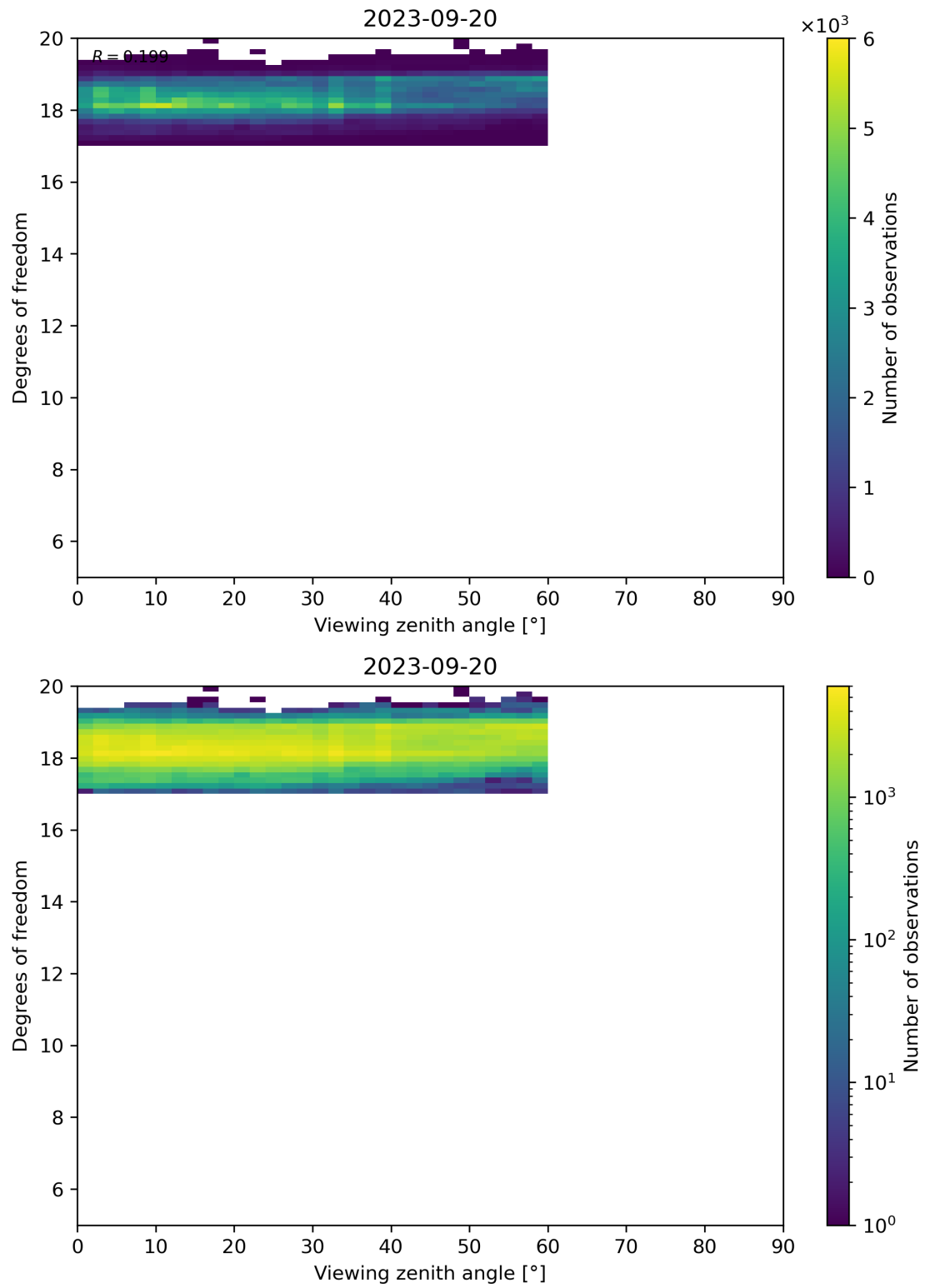
Figure 107: Scatter density plot of “Viewing zenith angle” against “Degrees of freedom” for 2023-09-20 to 2023-09-21.
