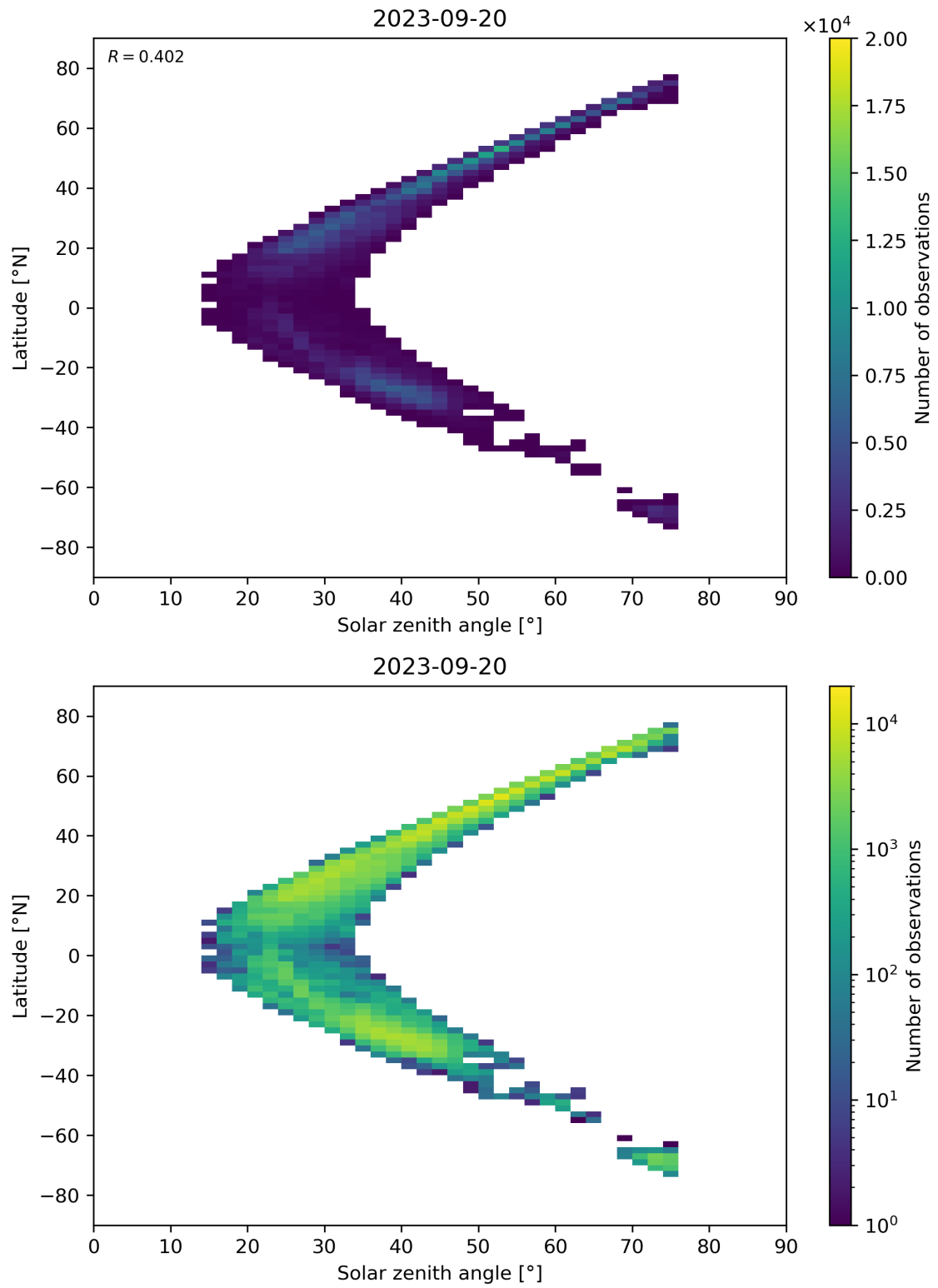
Figure 98: Scatter density plot of “Solar zenith angle” against “Latitude” for 2023-09-20 to 2023-09-21.
