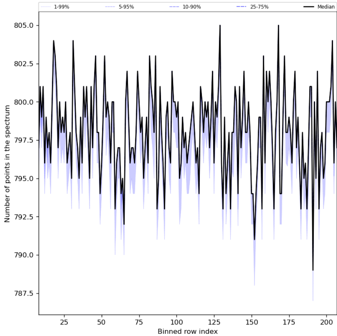
Figure 37: Along track statistics of “Number of points in the spectrum” for 2023-09-20 to 2023-09-21
