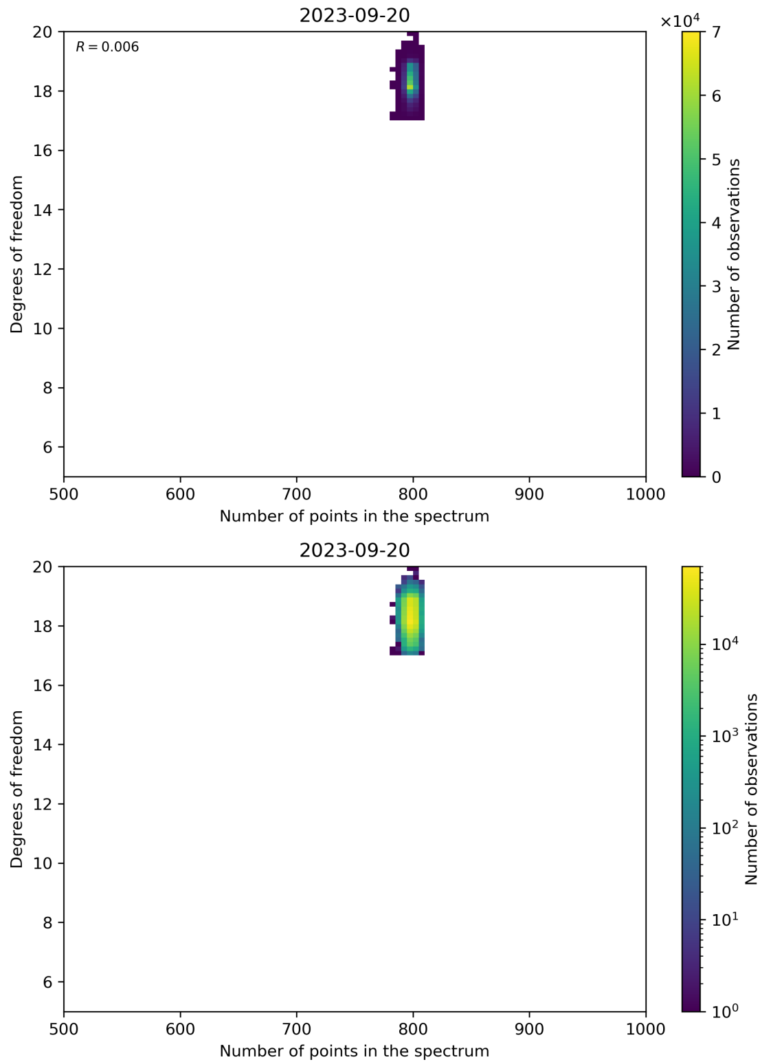
Figure 90: Scatter density plot of “Number of points in the spectrum” against “Degrees of freedom” for 2023-09-20 to 2023-09-21.
