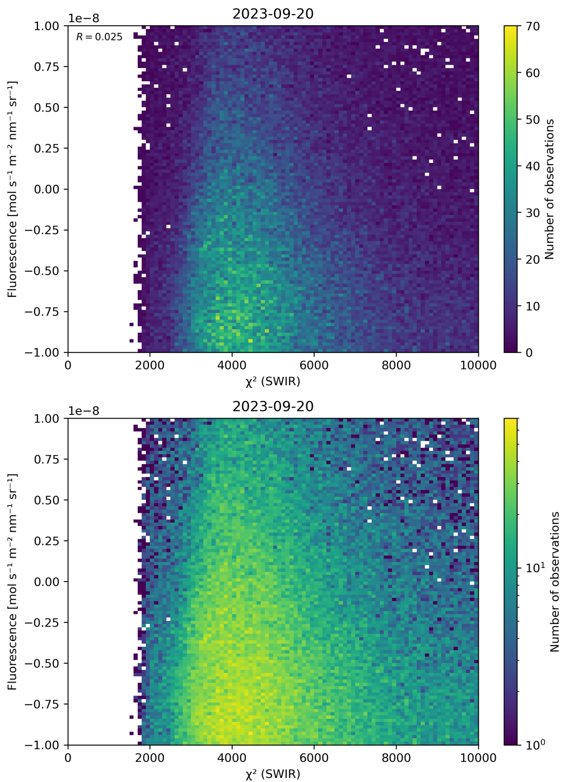
Figure 49: Scatter density plot of “ \chi^2 (SWIR)” against “Fluorescence” for 2023-09-20 to 2023-09-21.
