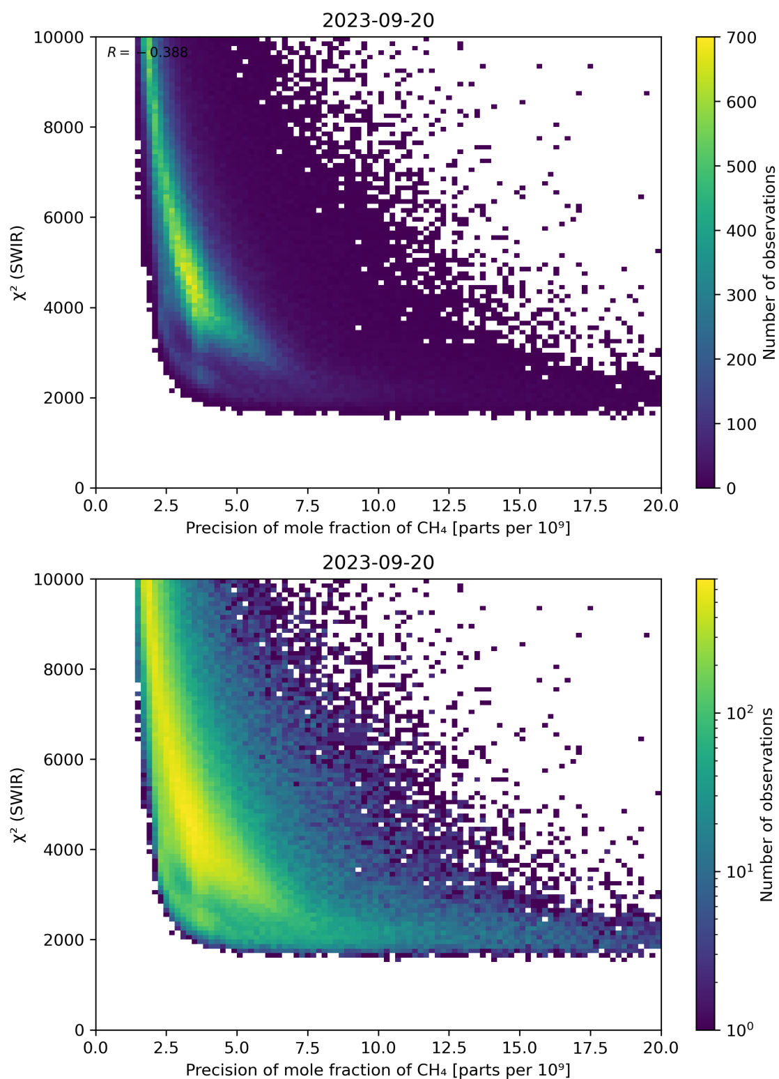
Figure 79: Scatter density plot of “Precision of mole fraction of CH 4 ” against “ \chi^2 (SWIR)” for 2023-09-20 to 2023-09-21.
