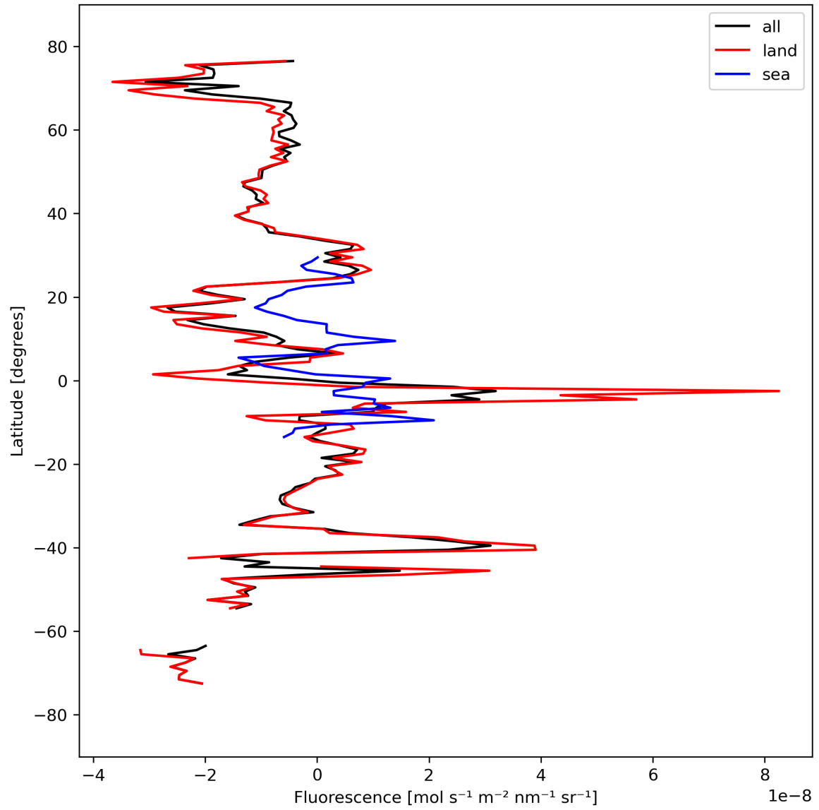
Figure 21: Zonal average of “Fluorescence” for 2023-09-20 to 2023-09-21.
