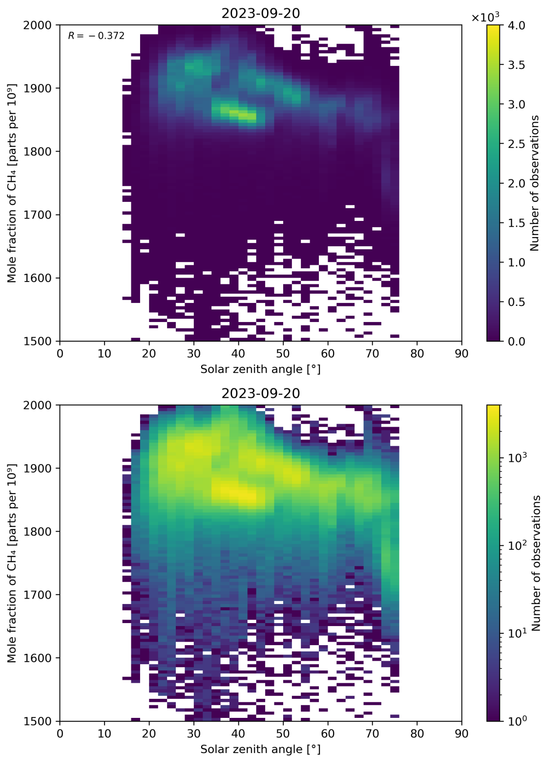
Figure 99: Scatter density plot of “Solar zenith angle” against “Mole fraction of CH 4 ” for 2023-09-20 to 2023-09-21.
