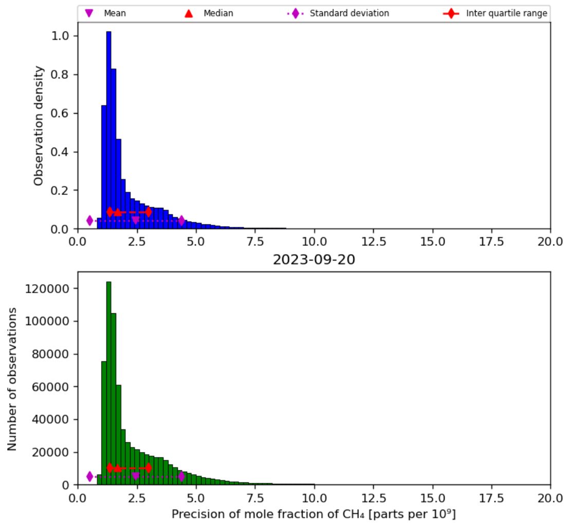
Figure 24: Histogram of “Precision of mole fraction of CH 4 ” for 2023-09-20 to 2023-09-21
