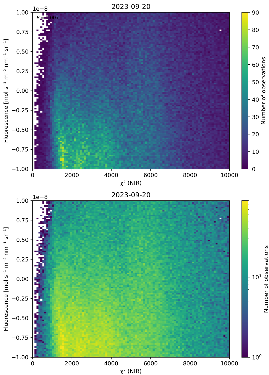
Figure 45: Scatter density plot of “ \chi^2 (NIR)” against “Fluorescence” for 2023-09-20 to 2023-09-21.
