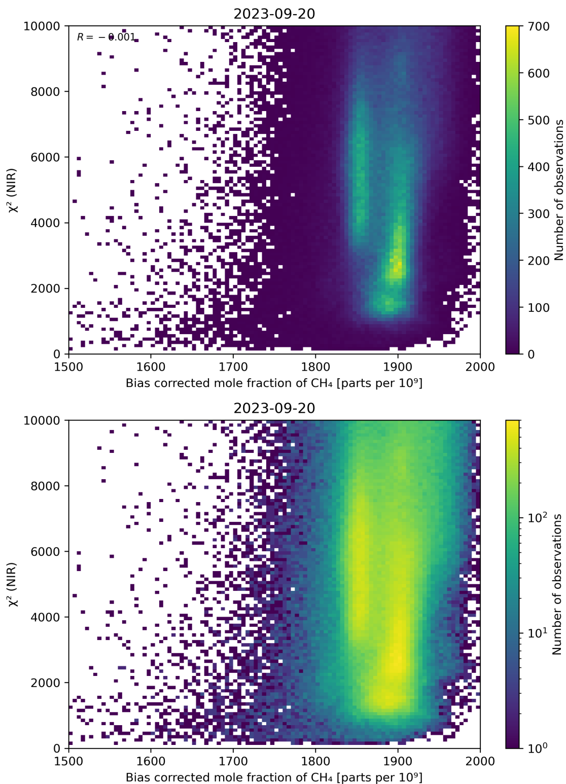
Figure 63: Scatter density plot of “Bias corrected mole fraction of CH 4 ” against “ \chi^2 (NIR)” for 2023-09-20 to 2023-09-21.
