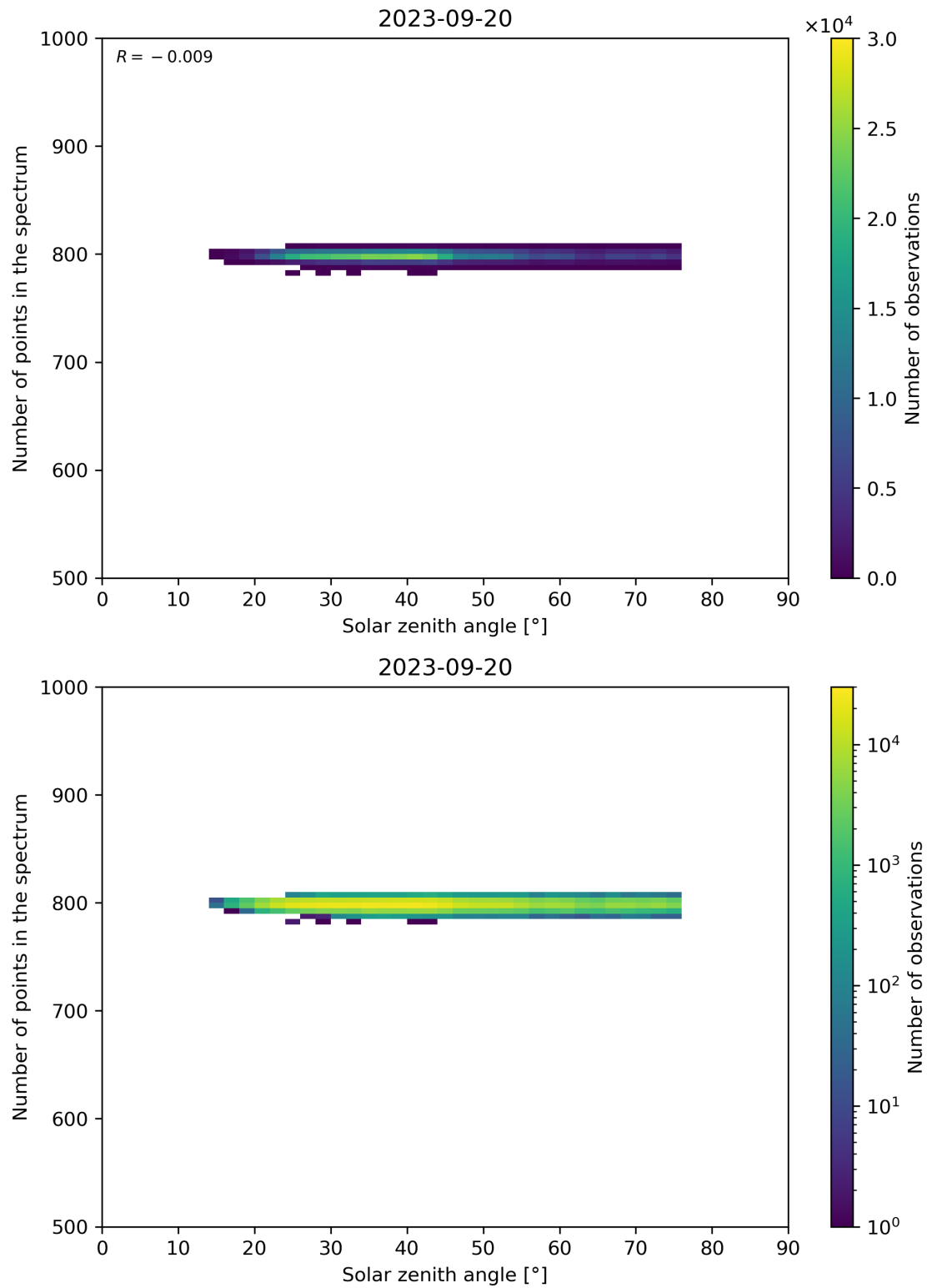
Figure 103: Scatter density plot of “Solar zenith angle” against “Number of points in the spectrum” for 2023-09-20 to 2023-09-21.
