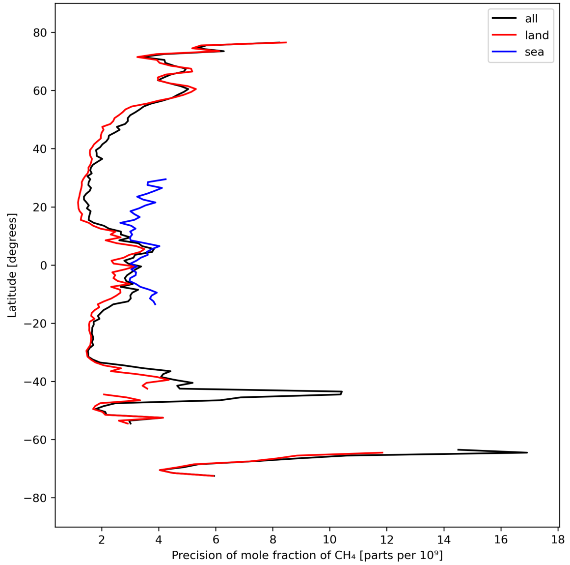
Figure 13: Zonal average of “Precision of mole fraction of \text{CH}_4 ” for 2023-09-20 to 2023-09-21.
