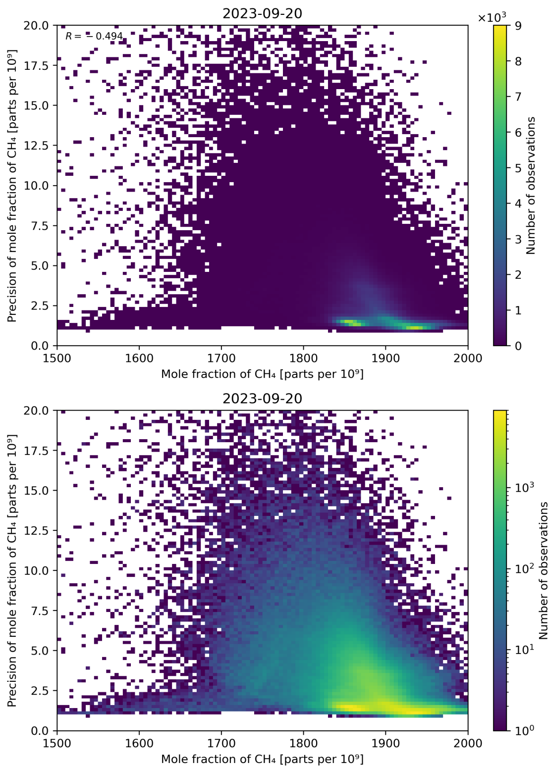
Figure 75: Scatter density plot of “Mole fraction of CH 4 ” against “Precision of mole fraction of CH 4 ” for 2023-09-20 to 2023-09-21.
