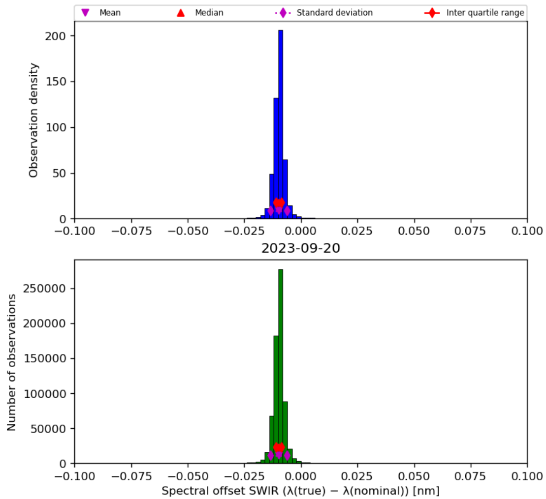
Figure 27: Histogram of “Spectral offset SWIR ( \lambda(\text{true}) - \lambda(\text{nominal}) )” for 2023-09-20 to 2023-09-21
