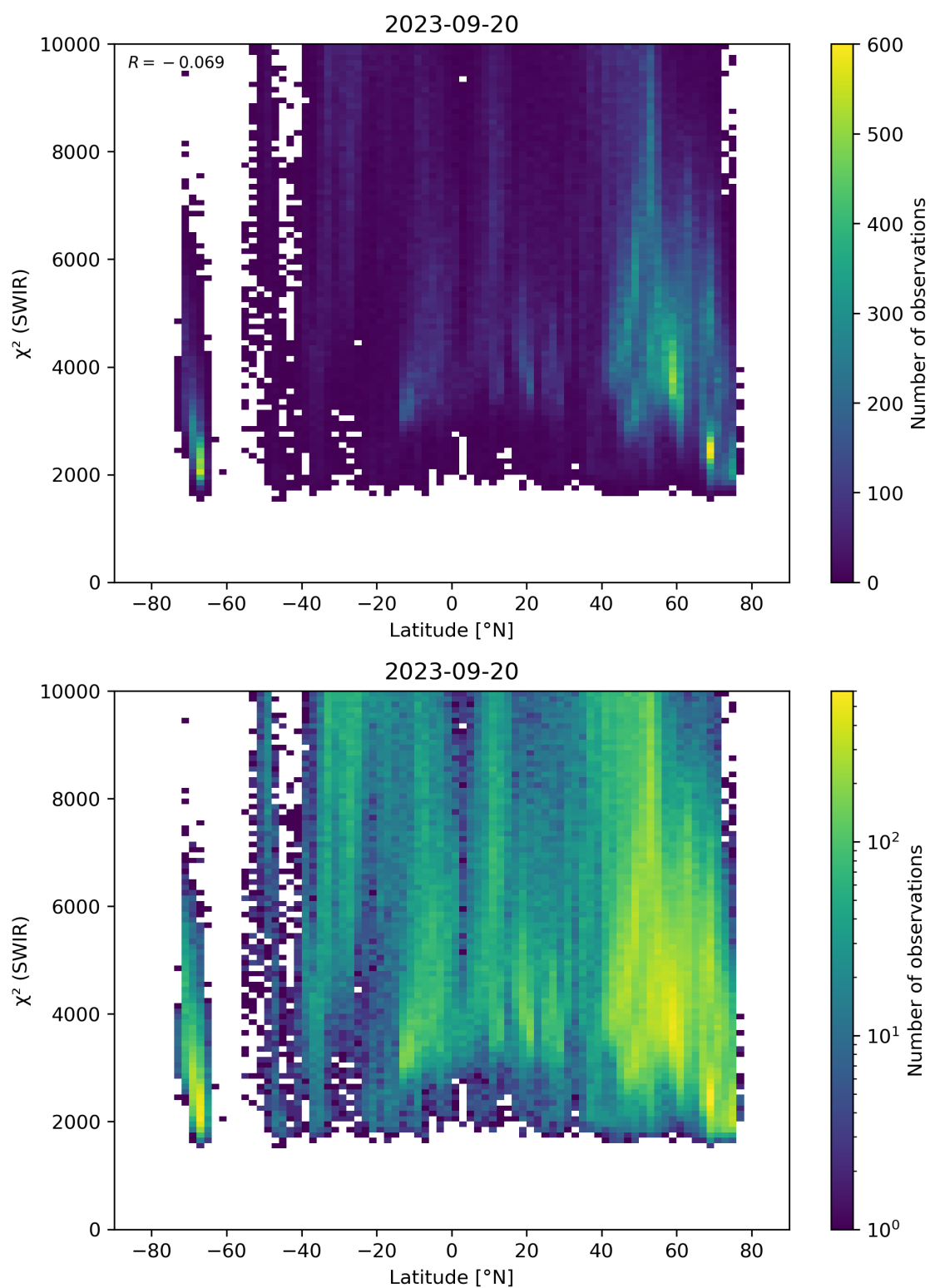
Figure 54: Scatter density plot of “Latitude” against “ \chi^2 (SWIR)” for 2023-09-20 to 2023-09-21.
