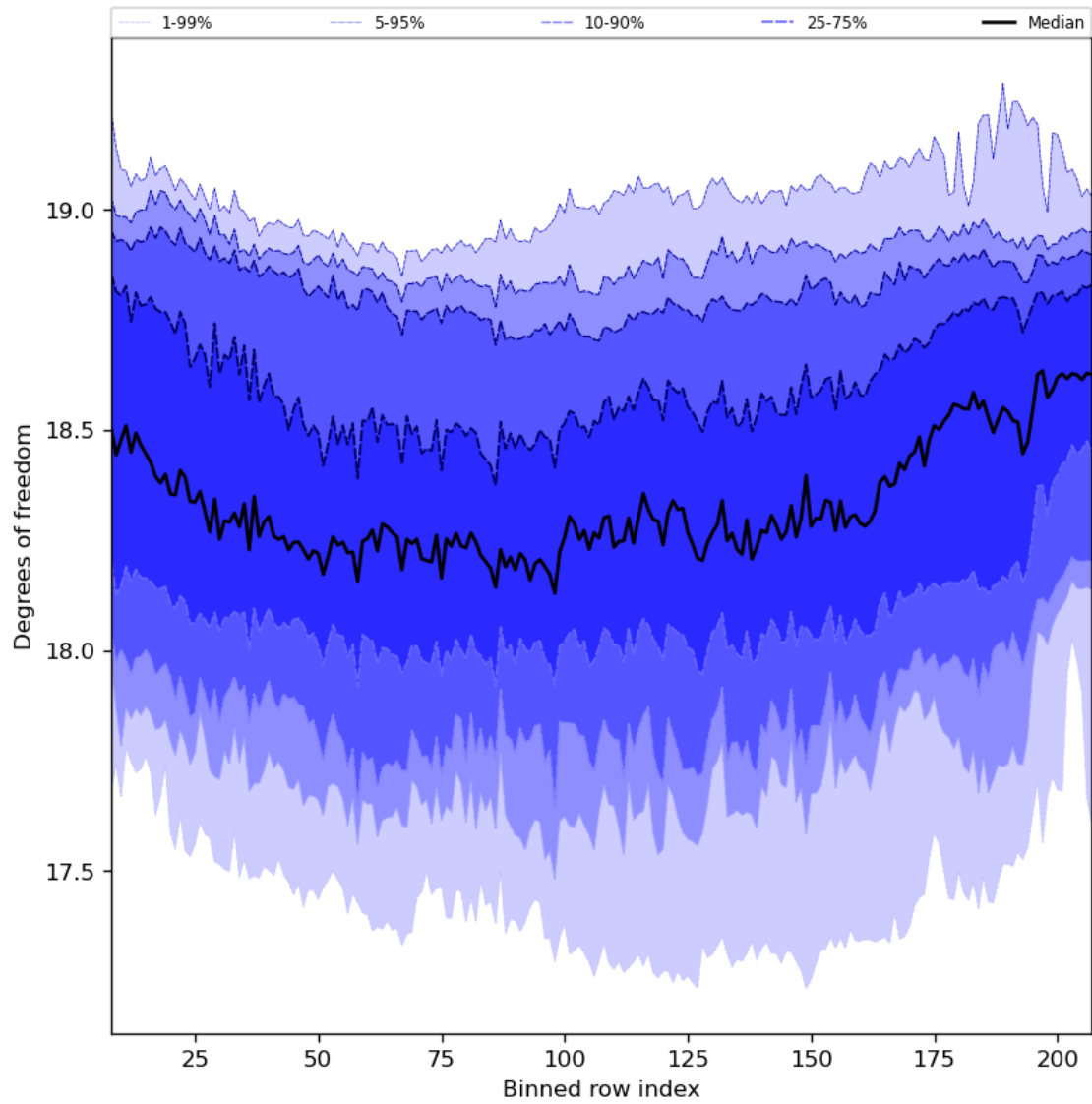
Figure 41: Along track statistics of “Degrees of freedom” for 2023-09-20 to 2023-09-21
