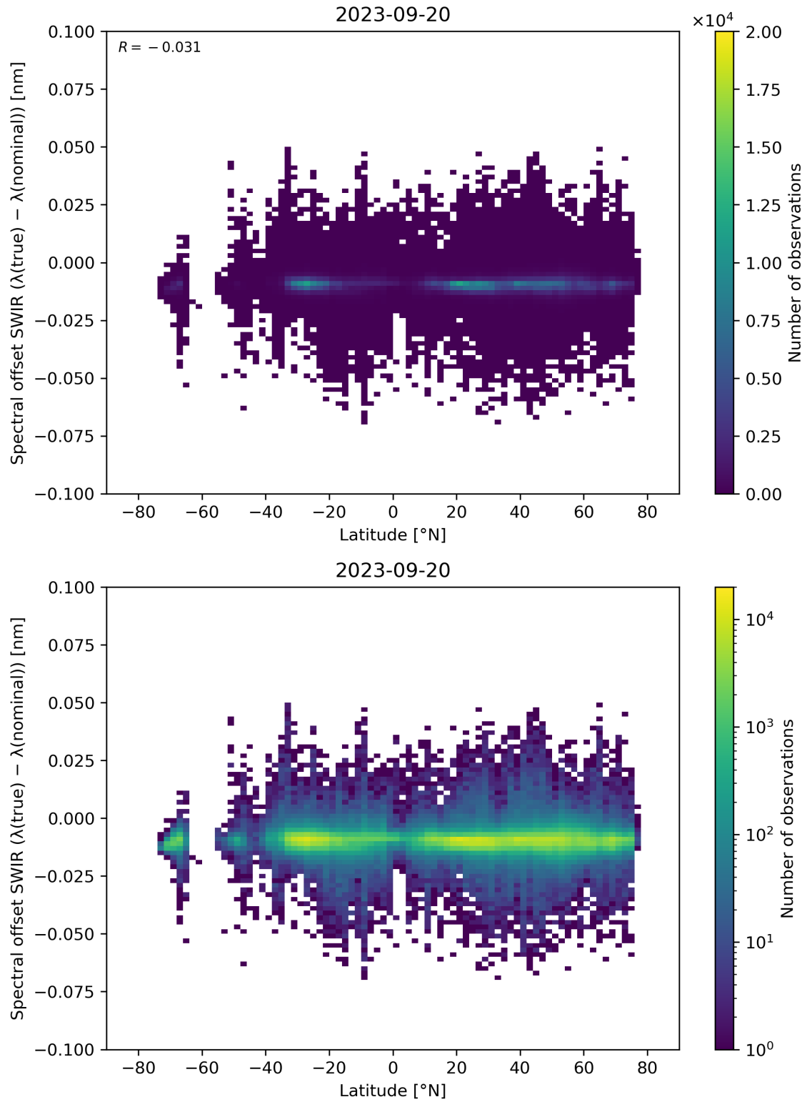
Figure 62: Scatter density plot of “Latitude” against “Spectral offset SWIR ( \lambda(\text{true}) - \lambda(\text{nominal}) )” for 2023-09-20 to 2023-09-21.
