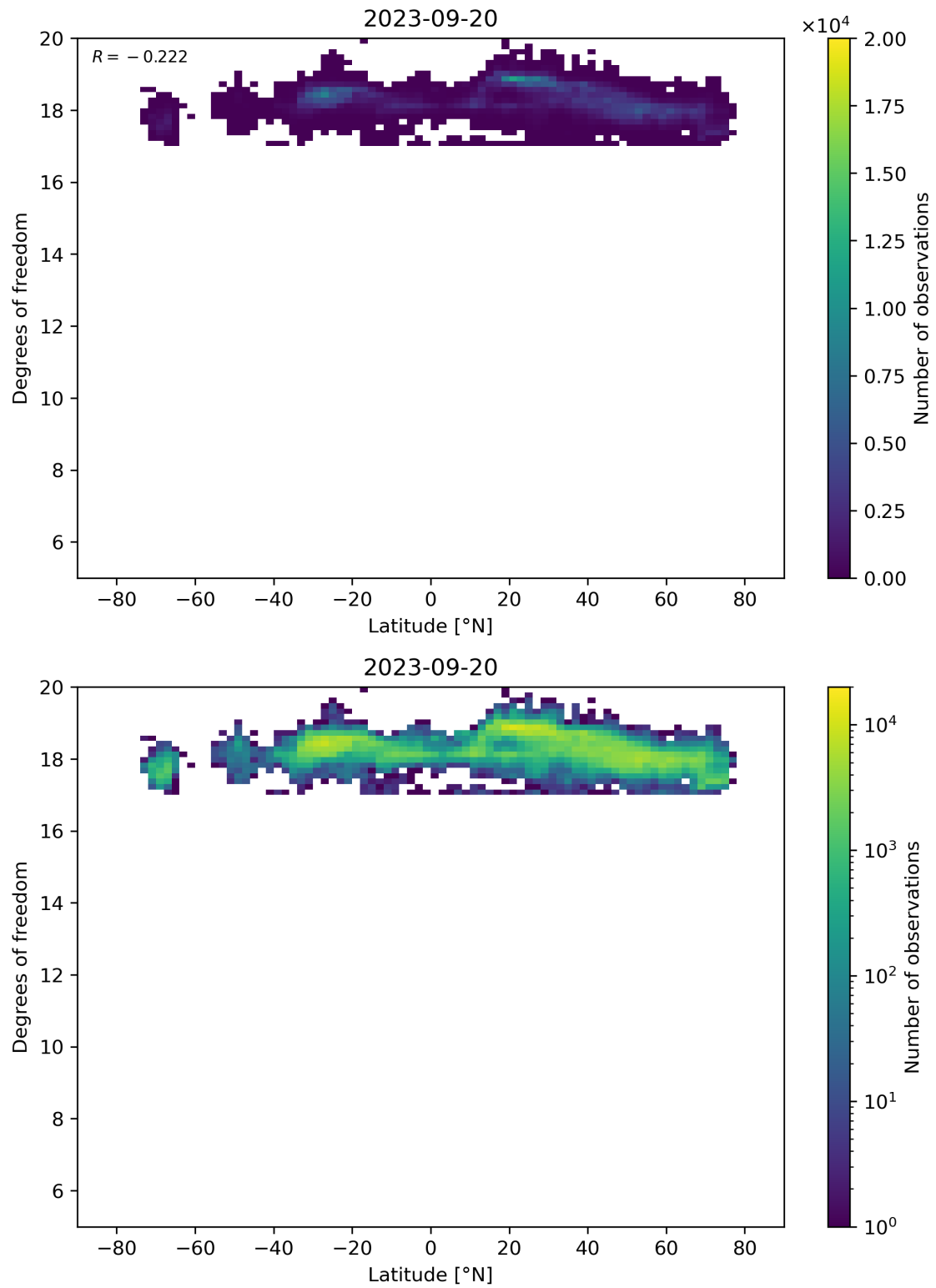
Figure 55: Scatter density plot of “Latitude” against “Degrees of freedom” for 2023-09-20 to 2023-09-21.
