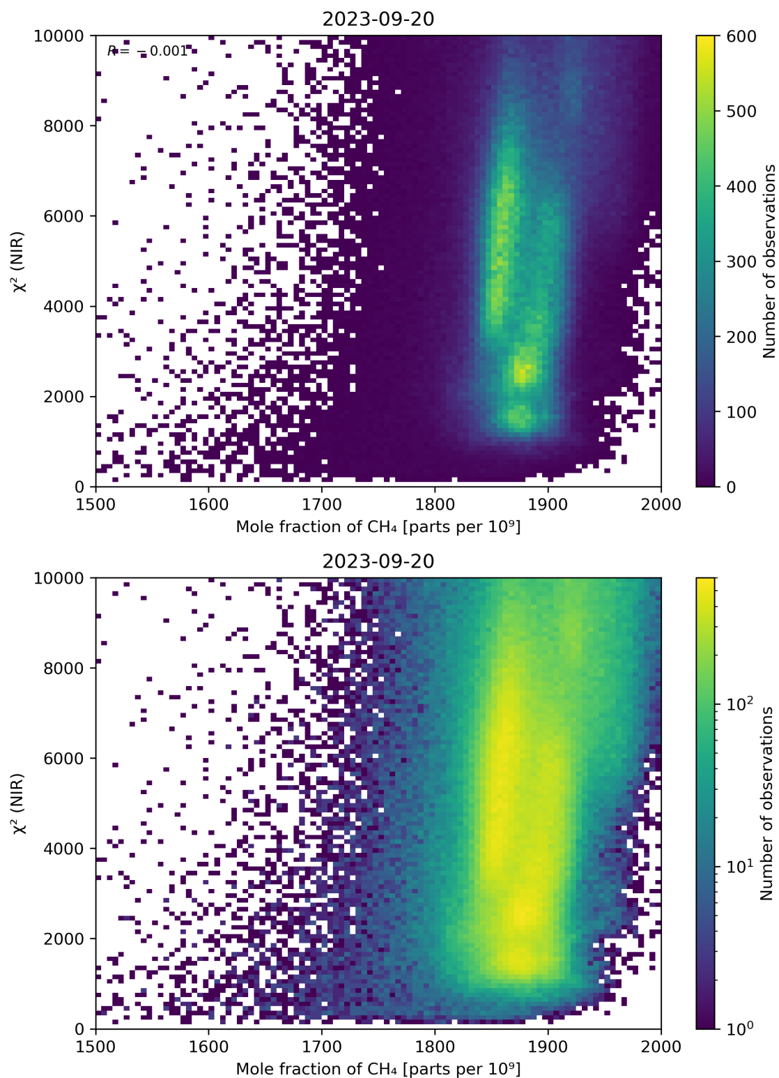
Figure 70: Scatter density plot of “Mole fraction of \text{CH}_4 ” against “ \chi^2 (NIR)” for 2023-09-20 to 2023-09-21.
