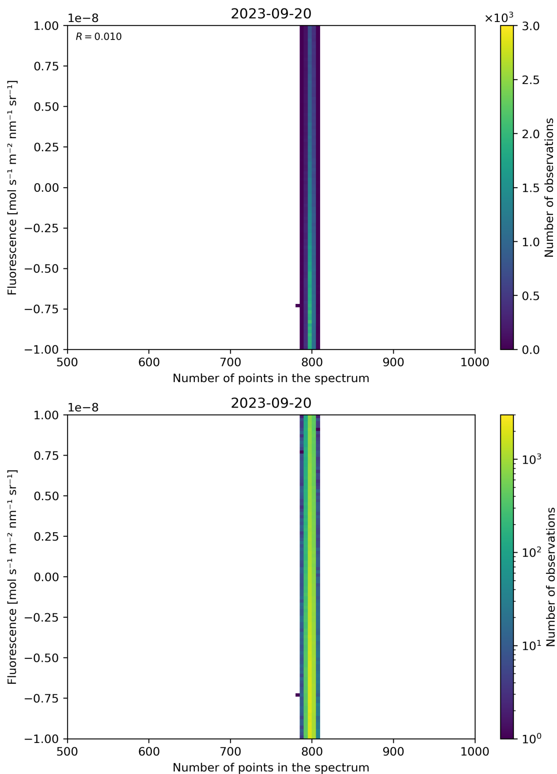
Figure 91: Scatter density plot of “Number of points in the spectrum” against “Fluorescence” for 2023-09-20 to 2023-09-21.
