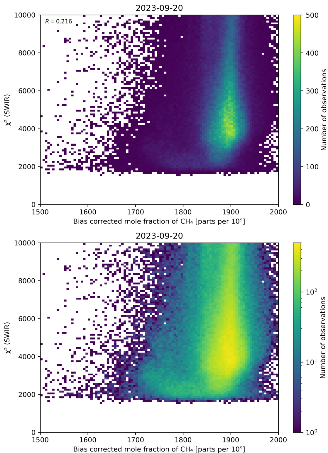
Figure 64: Scatter density plot of “Bias corrected mole fraction of \text{CH}_4 ” against “ \chi^2 (SWIR)” for 2023-09-20 to 2023-09-21.
