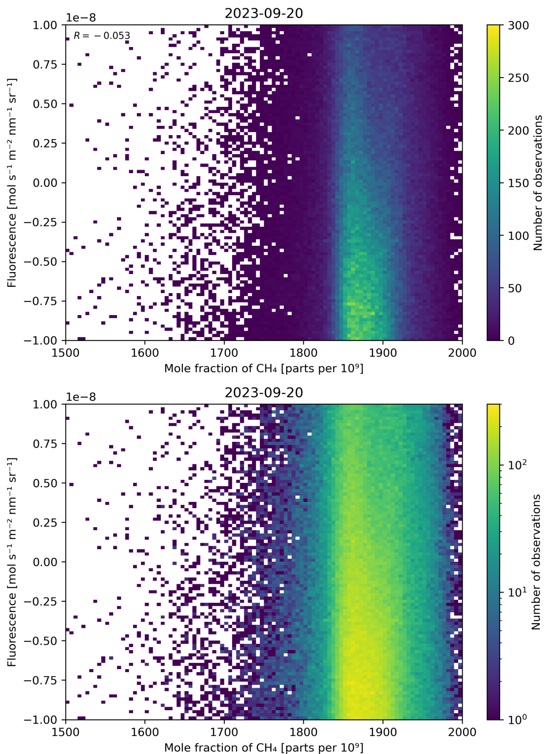
Figure 73: Scatter density plot of “Mole fraction of \text{CH}_4 ” against “Fluorescence” for 2023-09-20 to 2023-09-21.
