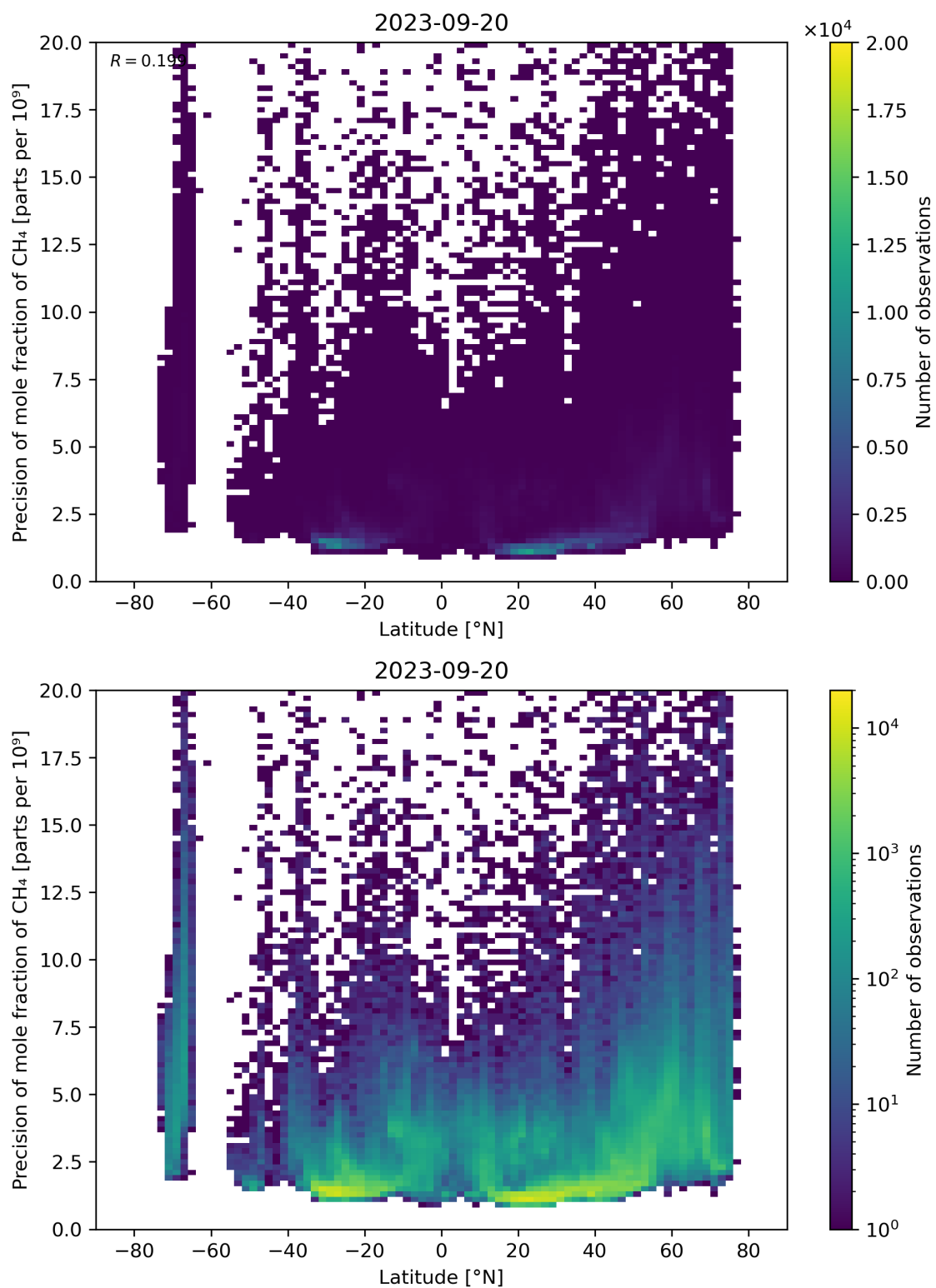
Figure 59: Scatter density plot of “Latitude” against “Precision of mole fraction of CH 4 ” for 2023-09-20 to 2023-09-21.
