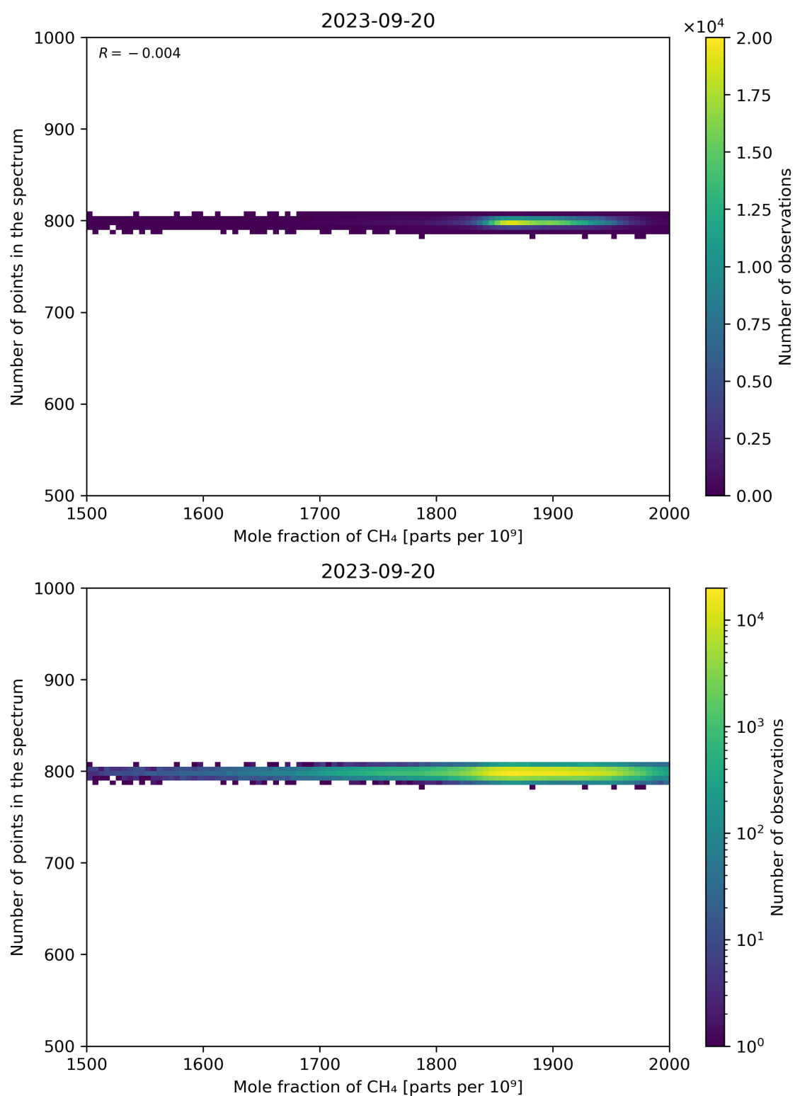
Figure 77: Scatter density plot of “Mole fraction of CH 4 ” against “Number of points in the spectrum” for 2023-09-20 to 2023-09-21.
