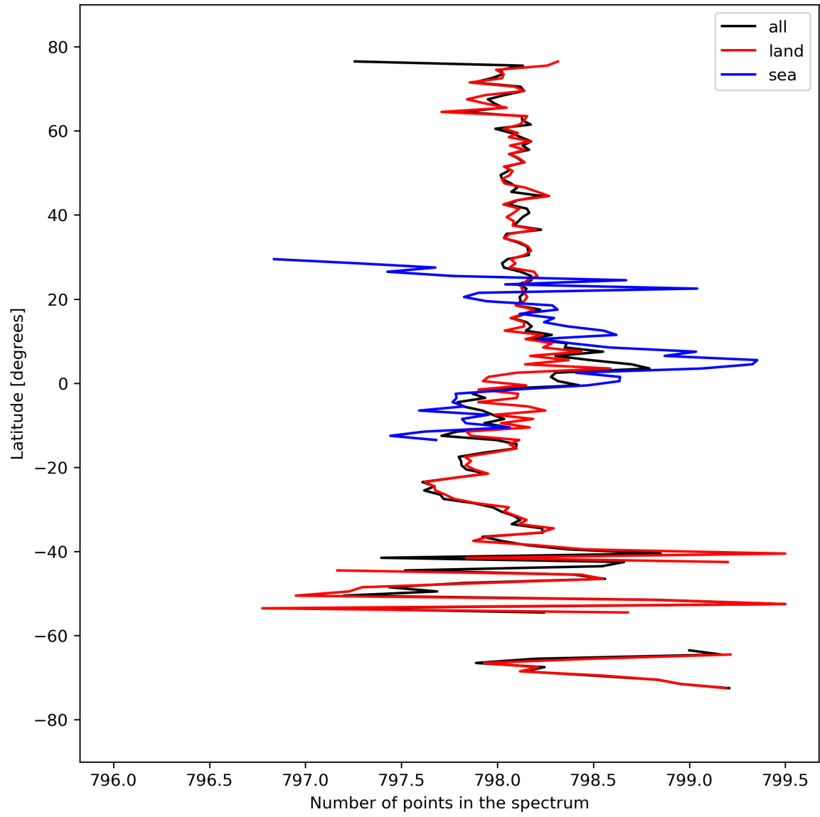
Figure 15: Zonal average of “Number of points in the spectrum” for 2023-09-20 to 2023-09-21.
