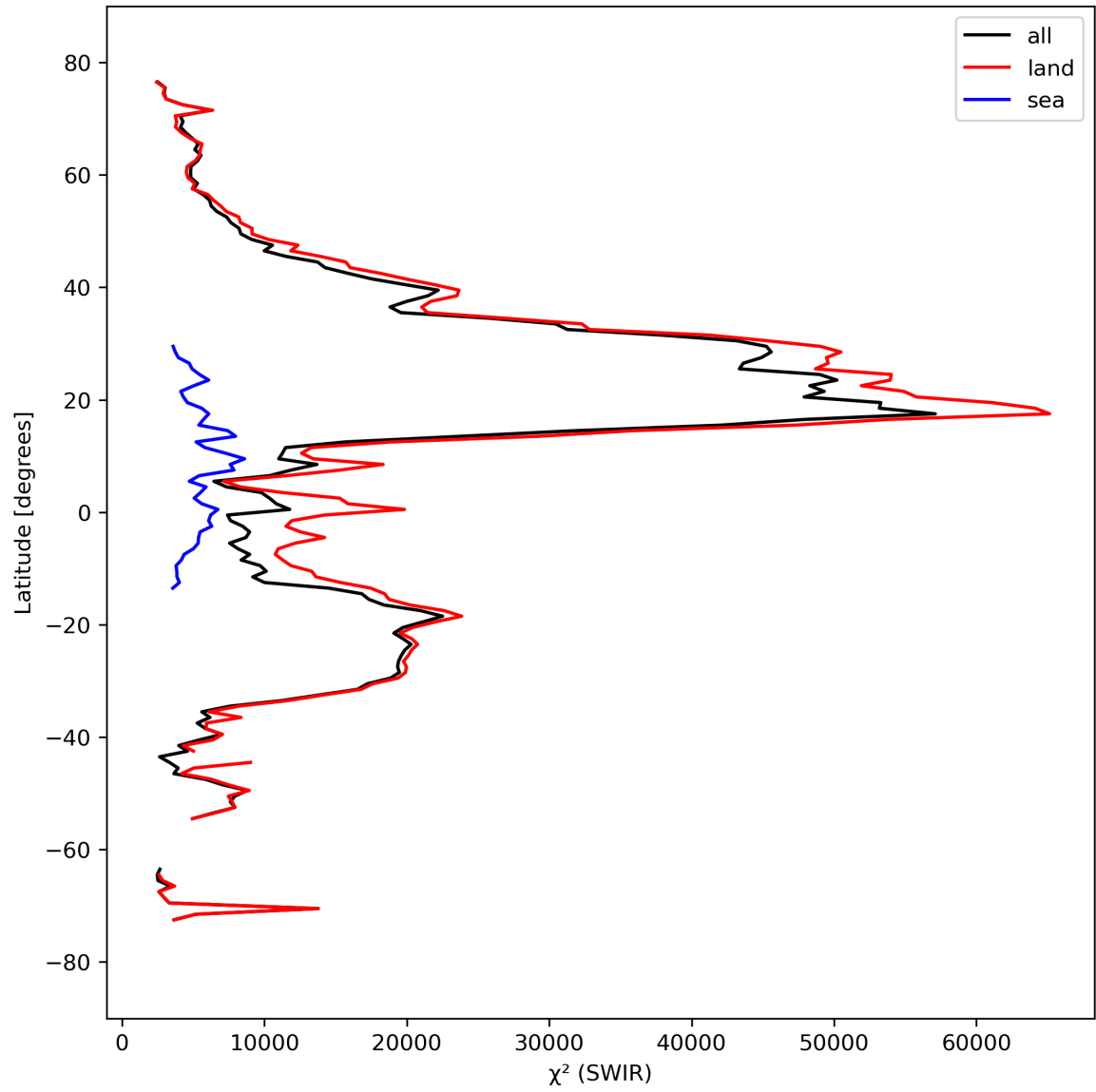
Figure 17: Zonal average of “ \chi^2 (SWIR)” for 2023-09-20 to 2023-09-21.
