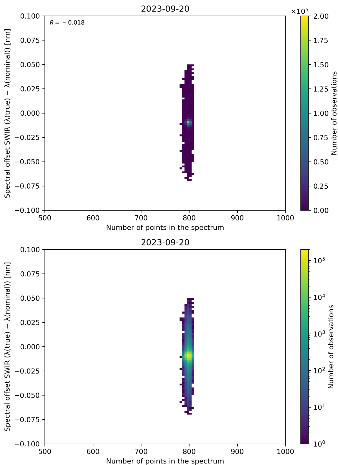
Figure 93: Scatter density plot of “Number of points in the spectrum” against “Spectral offset SWIR ( \lambda(\text{true}) - \lambda(\text{nominal}) )” for 2023-09-20 to 2023-09-21.
