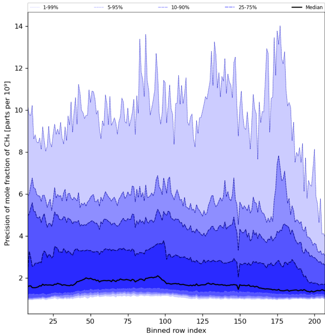
Figure 35: Along track statistics of "Precision of mole fraction of CH 4 " for 2023-09-20 to 2023-09-21
