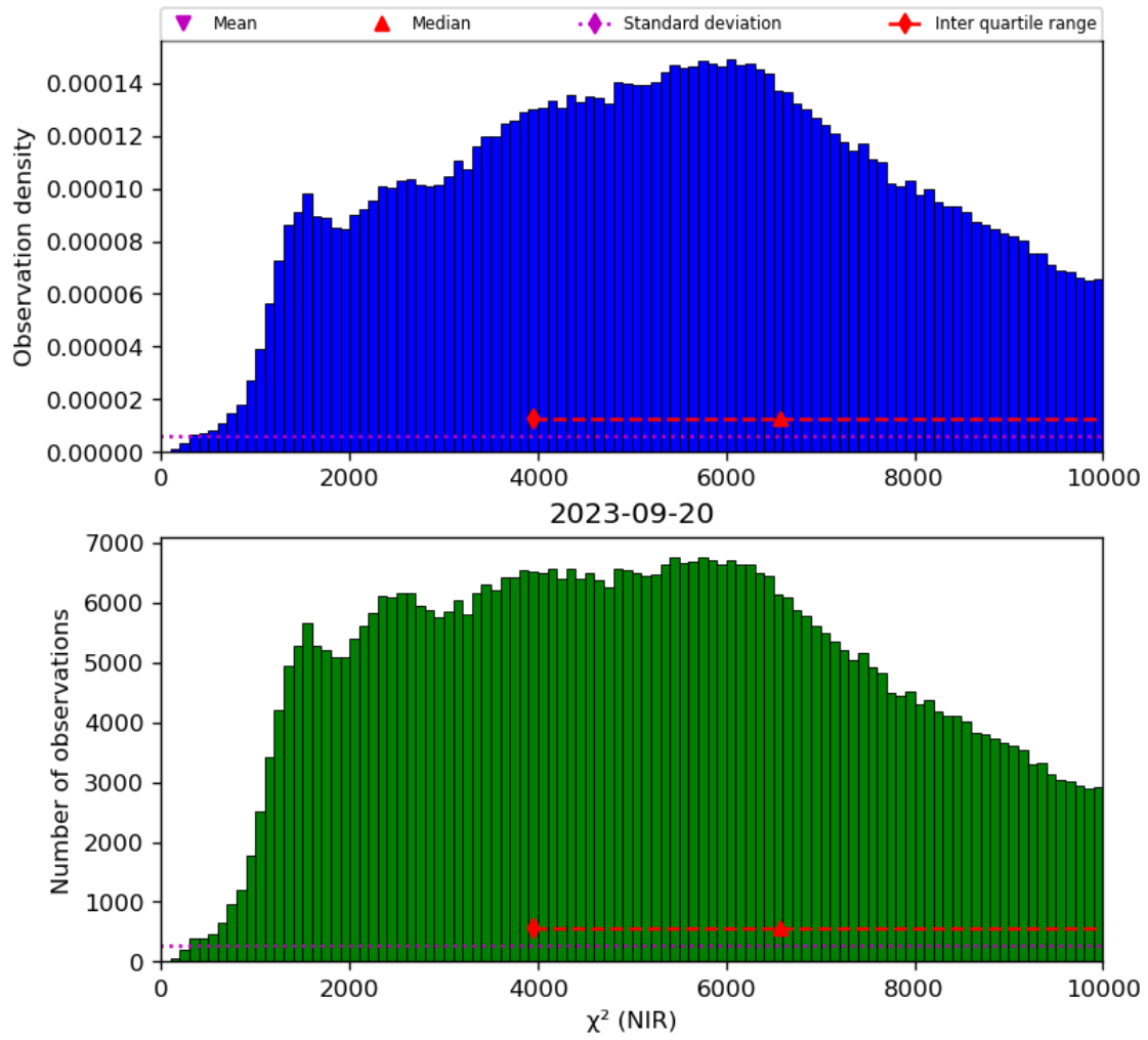
Figure 29: Histogram of “ \chi^2 (NIR)” for 2023-09-20 to 2023-09-21
