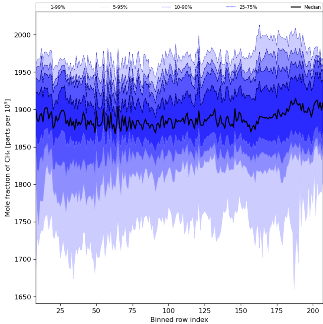
Figure 34: Along track statistics of “Mole fraction of CH 4 ” for 2023-09-20 to 2023-09-21
