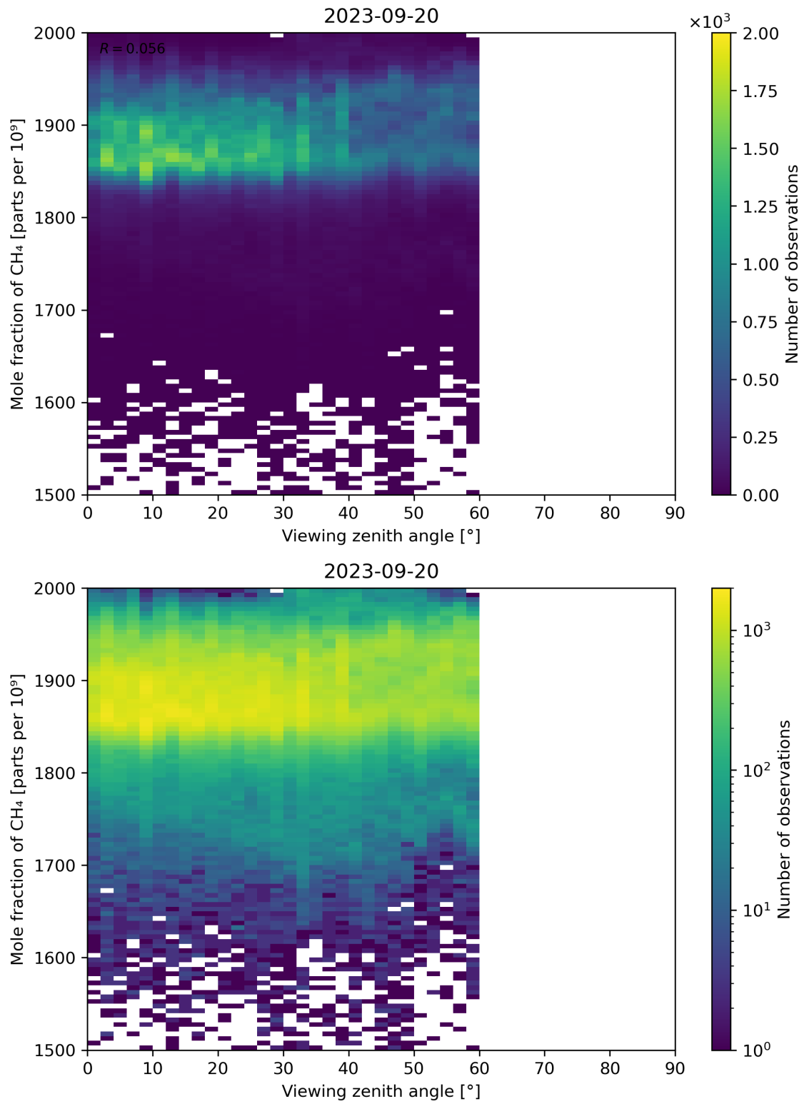
Figure 110: Scatter density plot of “Viewing zenith angle” against “Mole fraction of CH 4 ” for 2023-09-20 to 2023-09-21.
