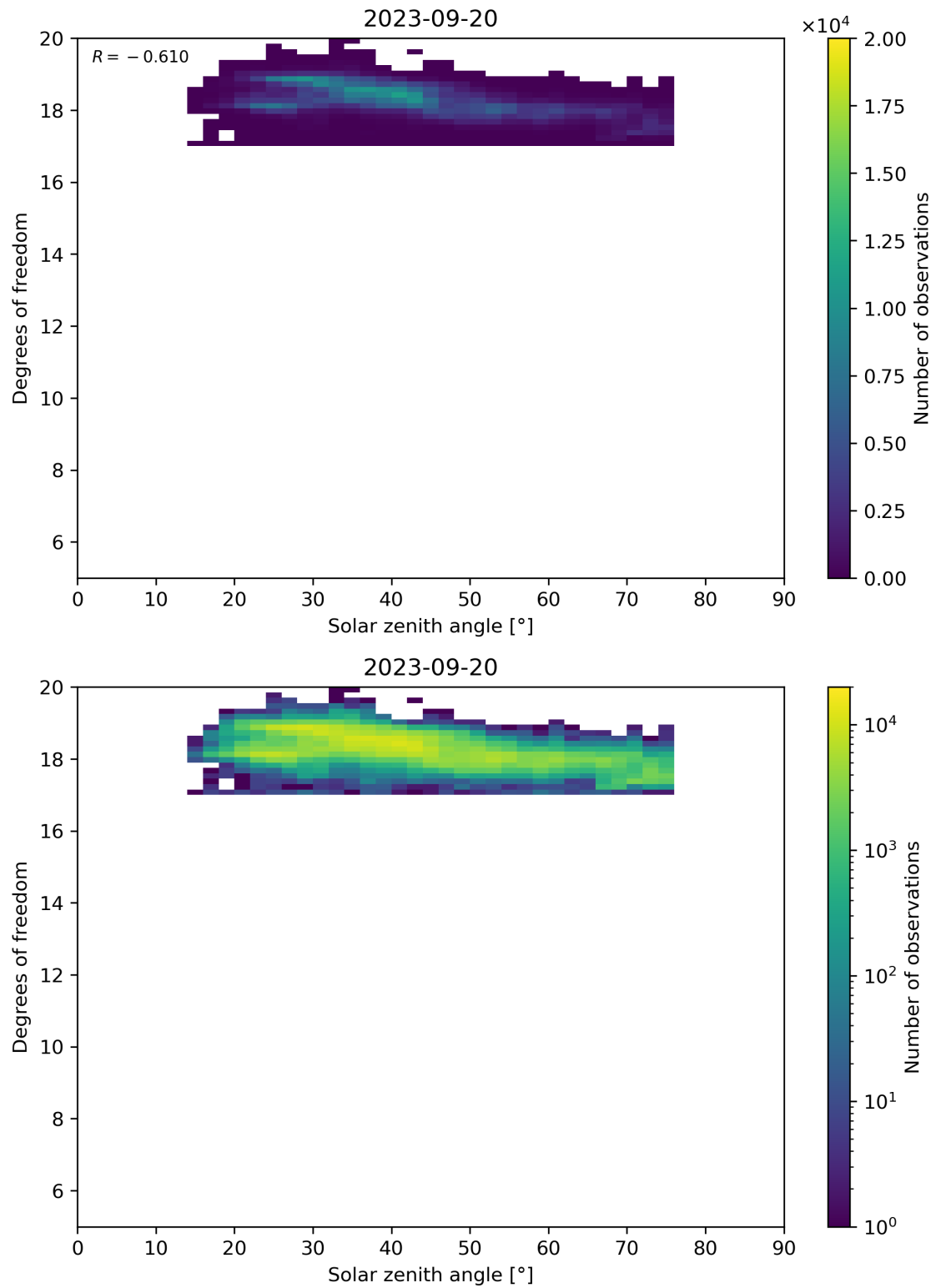
Figure 96: Scatter density plot of “Solar zenith angle” against “Degrees of freedom” for 2023-09-20 to 2023-09-21.
