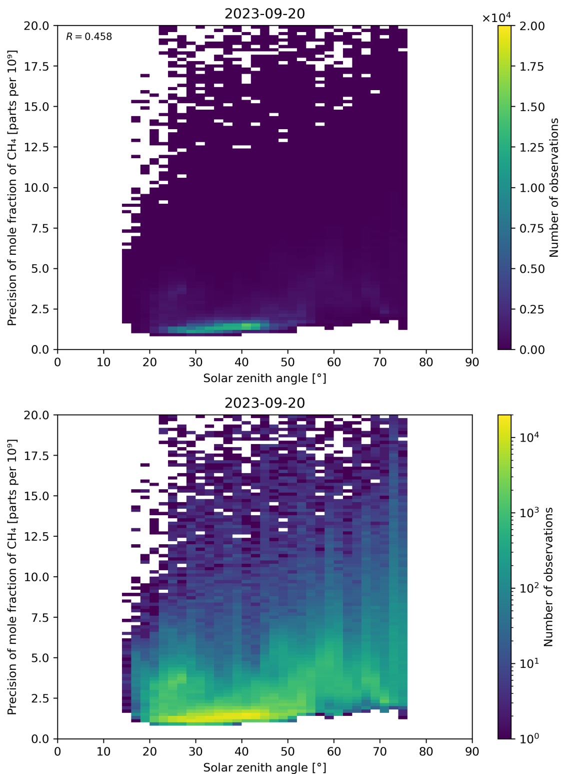
Figure 101: Scatter density plot of “Solar zenith angle” against “Precision of mole fraction of CH 4 ” for 2023-09-20 to 2023-09-21.
