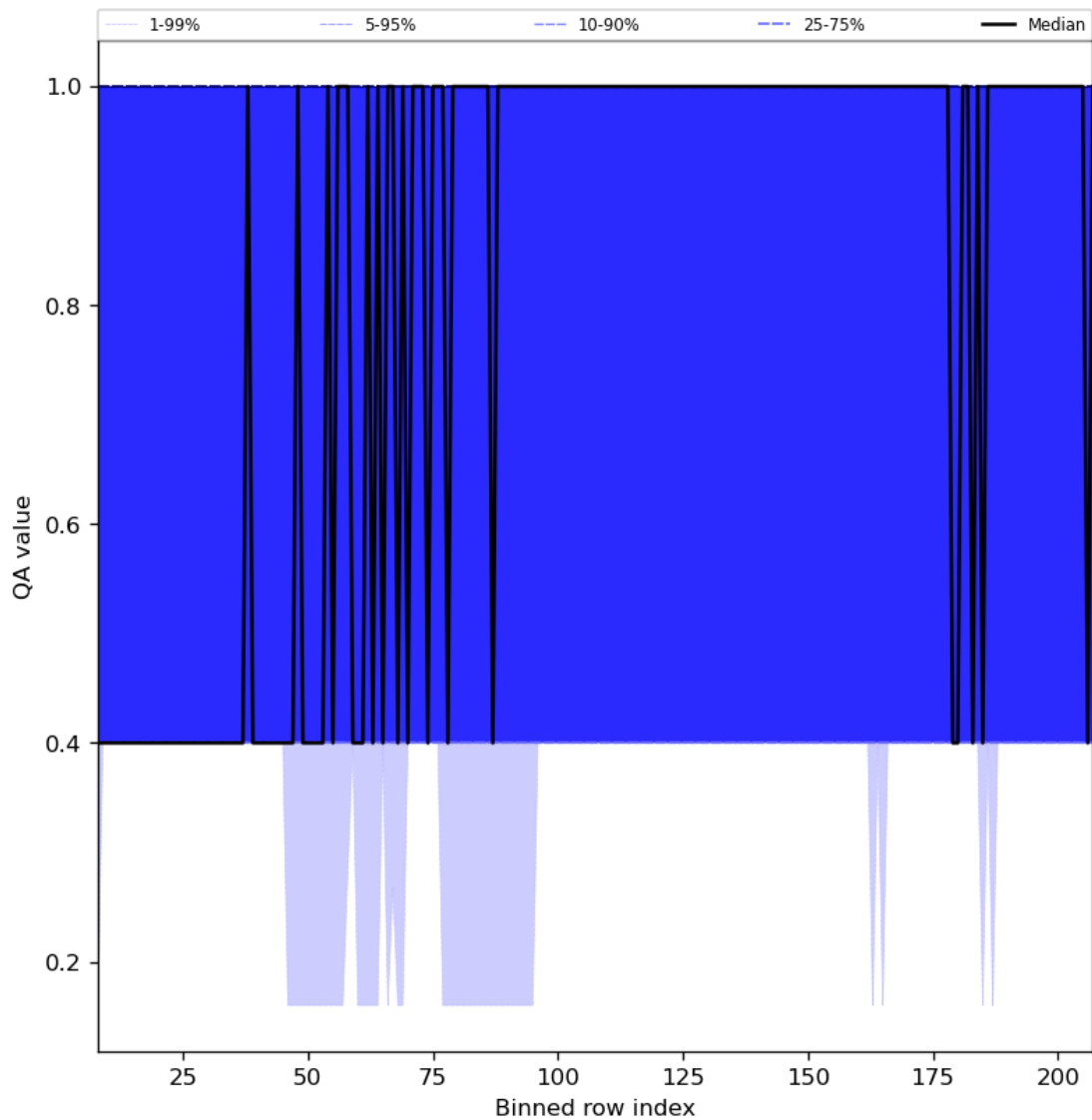
Figure 33: Along track statistics of “QA value” for 2023-09-20 to 2023-09-21
