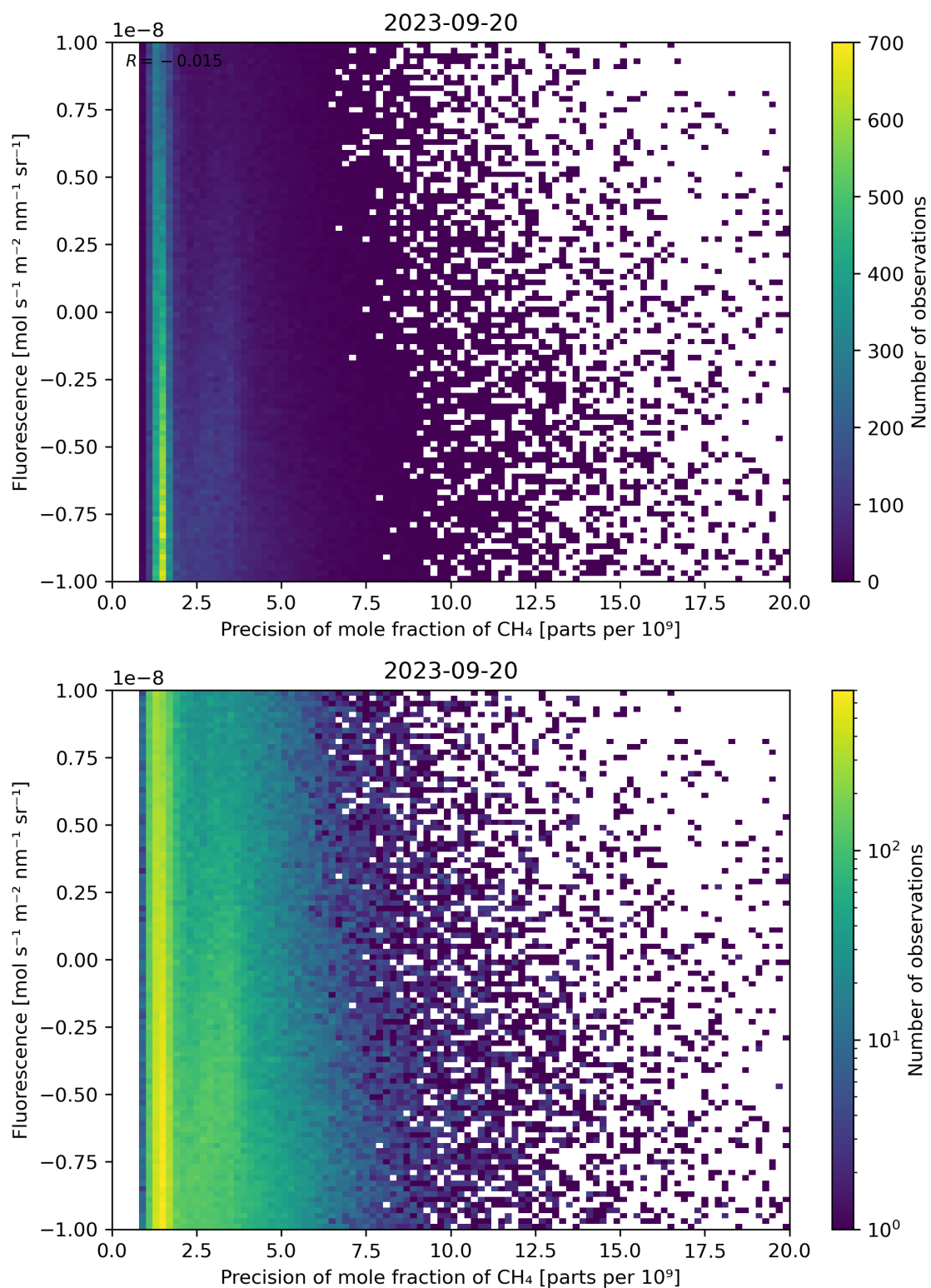
Figure 81: Scatter density plot of “Precision of mole fraction of CH 4 ” against “Fluorescence” for 2023-09-20 to 2023-09-21.
