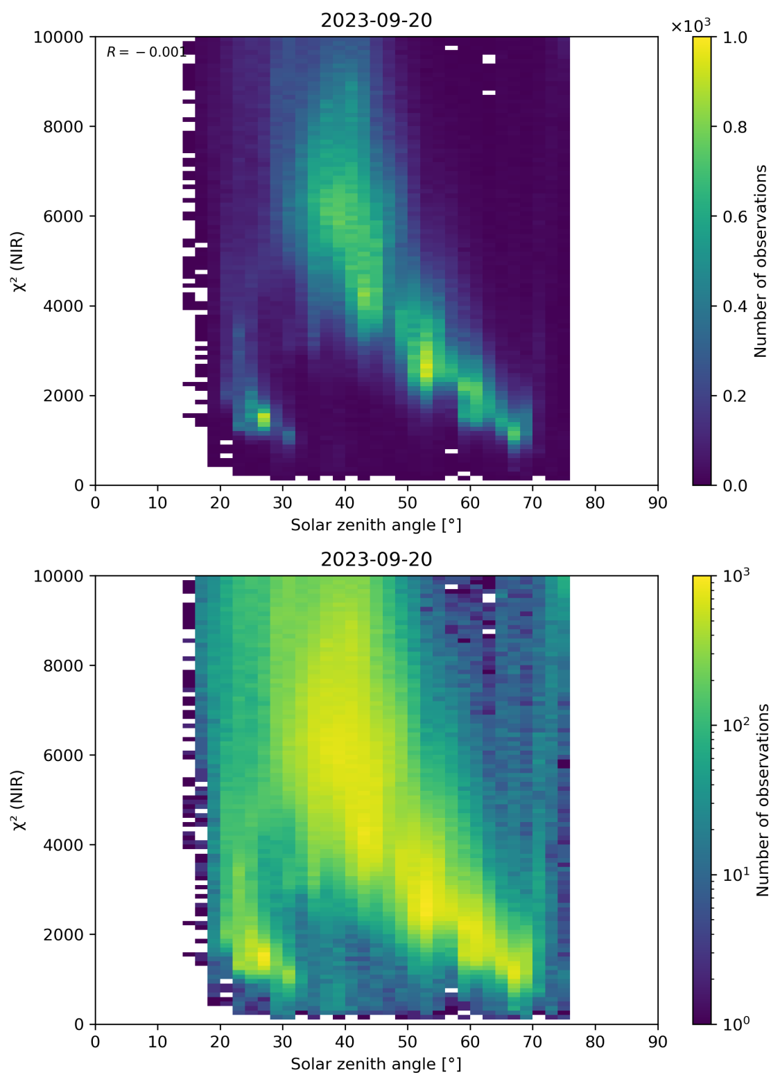
Figure 94: Scatter density plot of “Solar zenith angle” against “ \chi^2 (NIR)” for 2023-09-20 to 2023-09-21.
