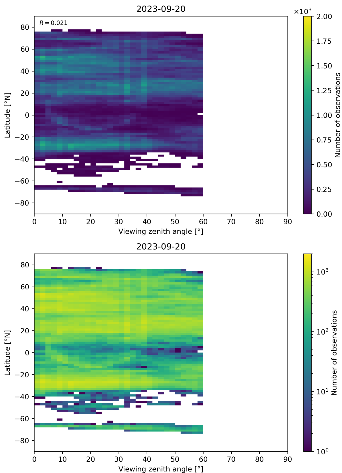
Figure 109: Scatter density plot of “Viewing zenith angle” against “Latitude” for 2023-09-20 to 2023-09-21.
