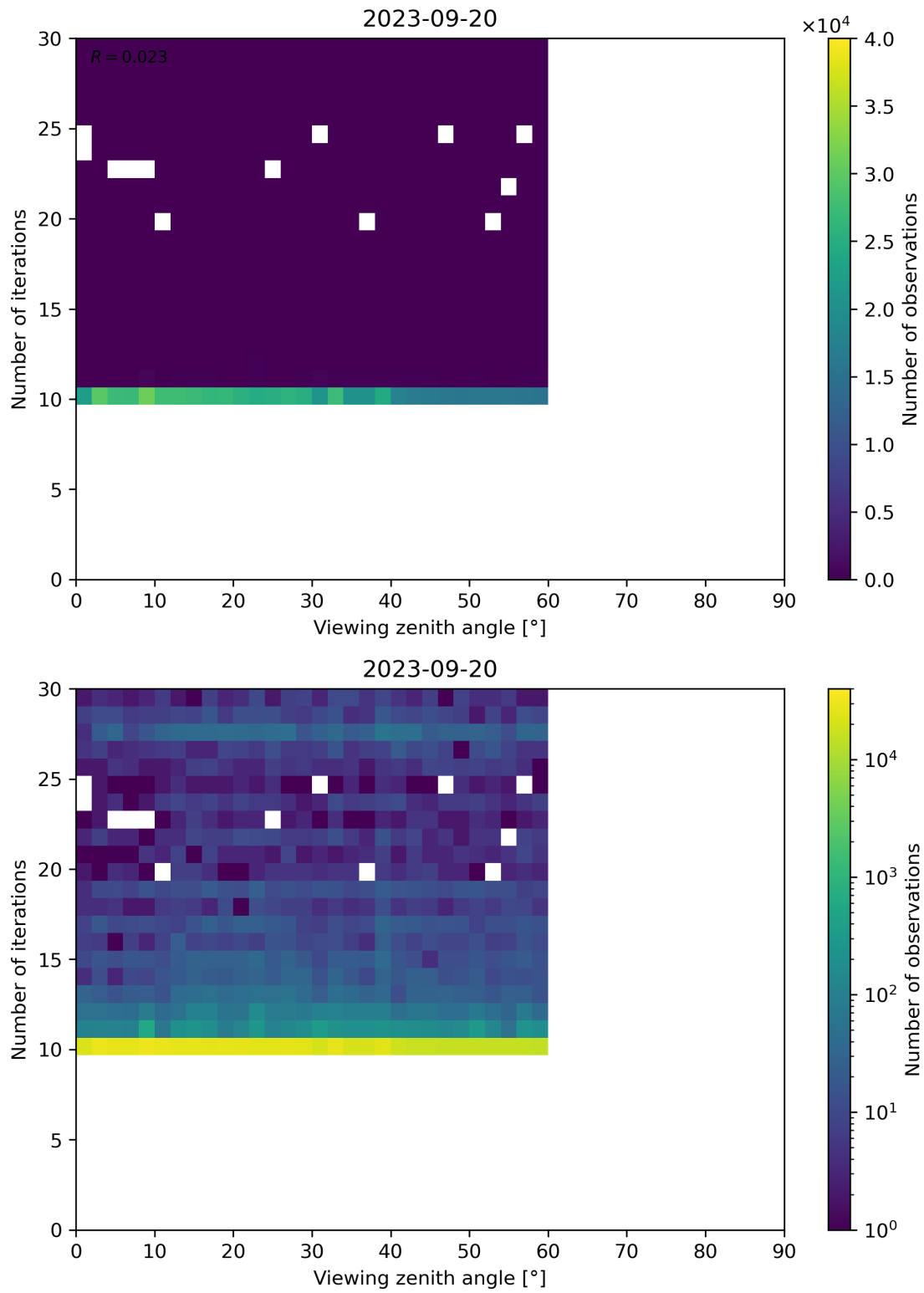
Figure 113: Scatter density plot of “Viewing zenith angle” against “Number of iterations” for 2023-09-20 to 2023-09-21.
