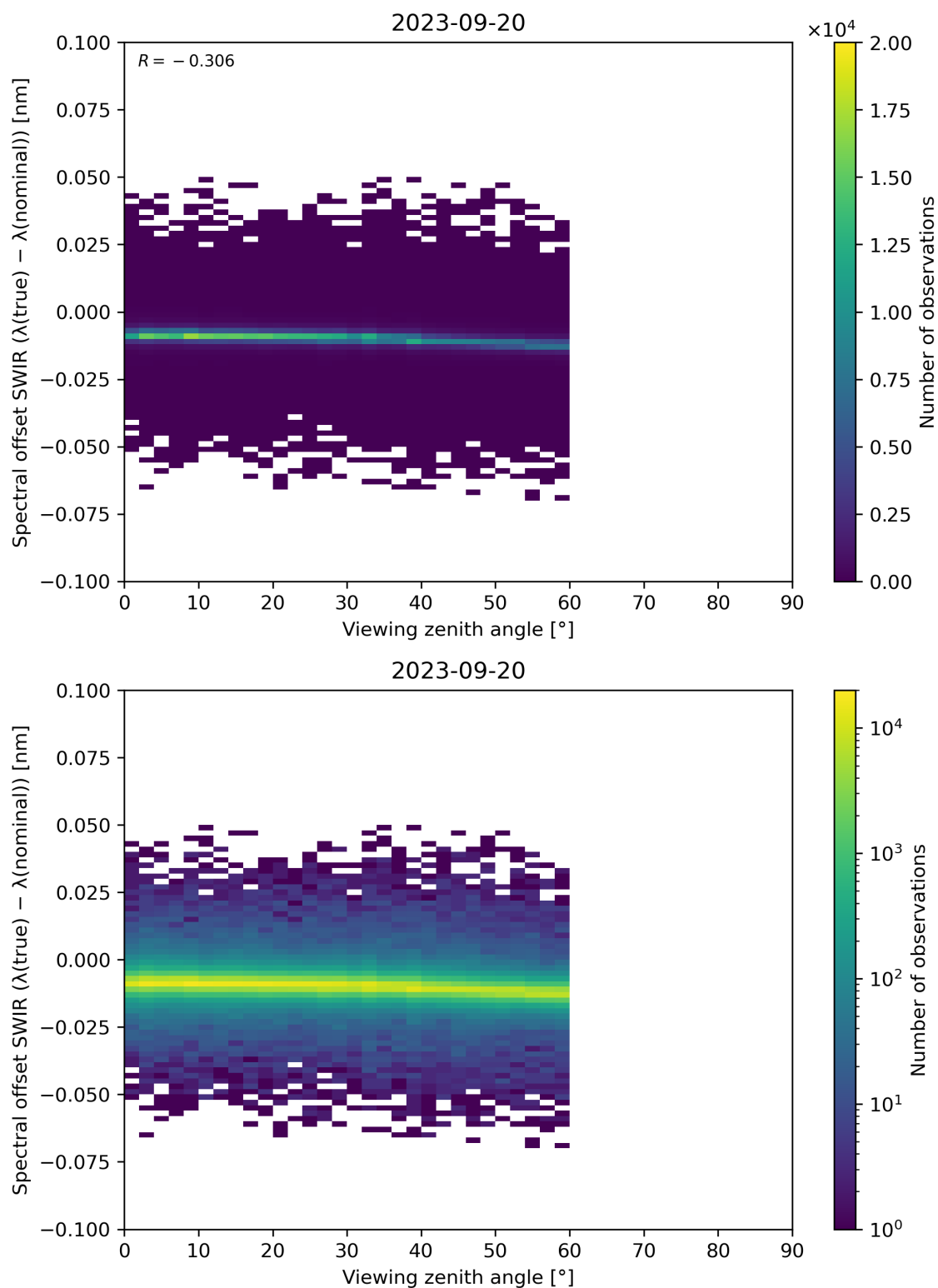
Figure 116: Scatter density plot of “Viewing zenith angle” against “Spectral offset SWIR ( \lambda(\text{true}) - \lambda(\text{nominal}) )” for 2023-09-20 to 2023-09-21.
