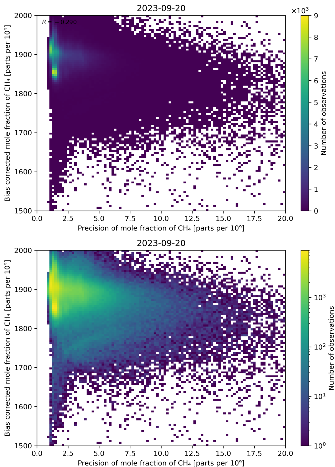
Figure 82: Scatter density plot of “Precision of mole fraction of CH 4 ” against “Bias corrected mole fraction of CH 4 ” for 2023-09-20 to 2023-09-21.
