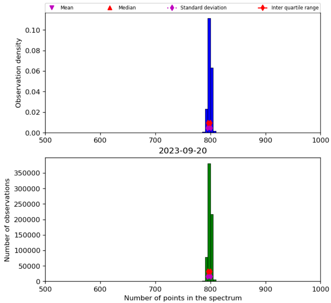
Figure 26: Histogram of “Number of points in the spectrum” for 2023-09-20 to 2023-09-21
