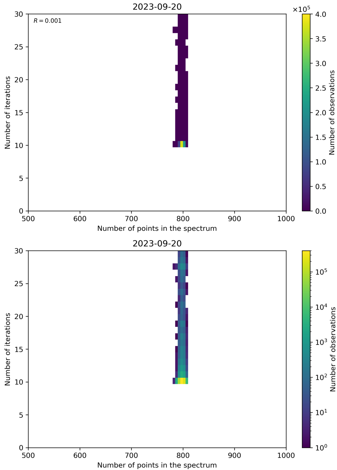
Figure 92: Scatter density plot of “Number of points in the spectrum” against “Number of iterations” for 2023-09-20 to 2023-09-21.
