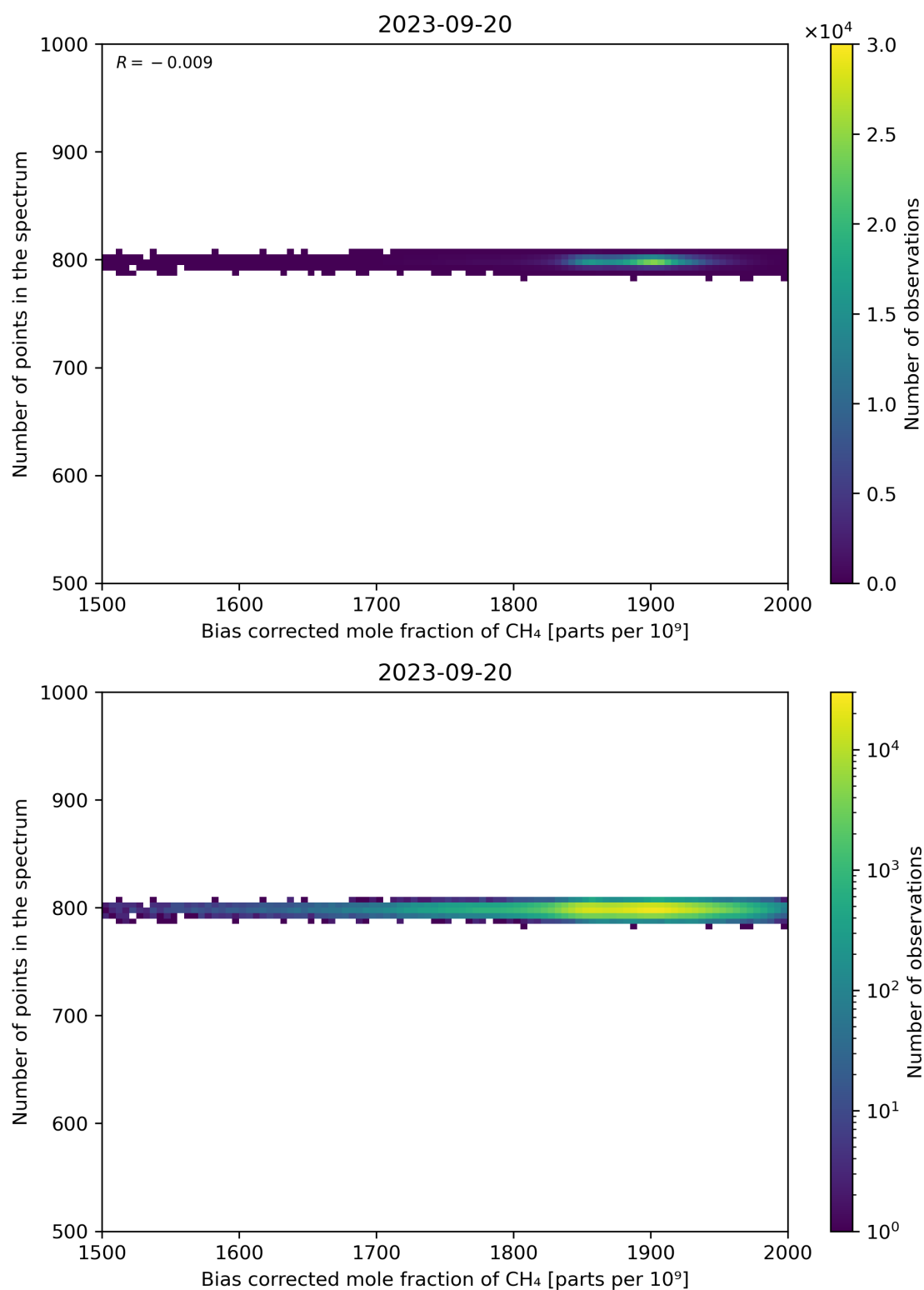
Figure 68: Scatter density plot of “Bias corrected mole fraction of CH 4 ” against “Number of points in the spectrum” for 2023-09-20 to 2023-09-21.
