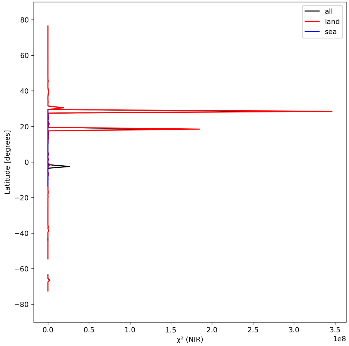
Figure 18: Zonal average of “ \chi^2 (NIR)” for 2023-09-20 to 2023-09-21.
