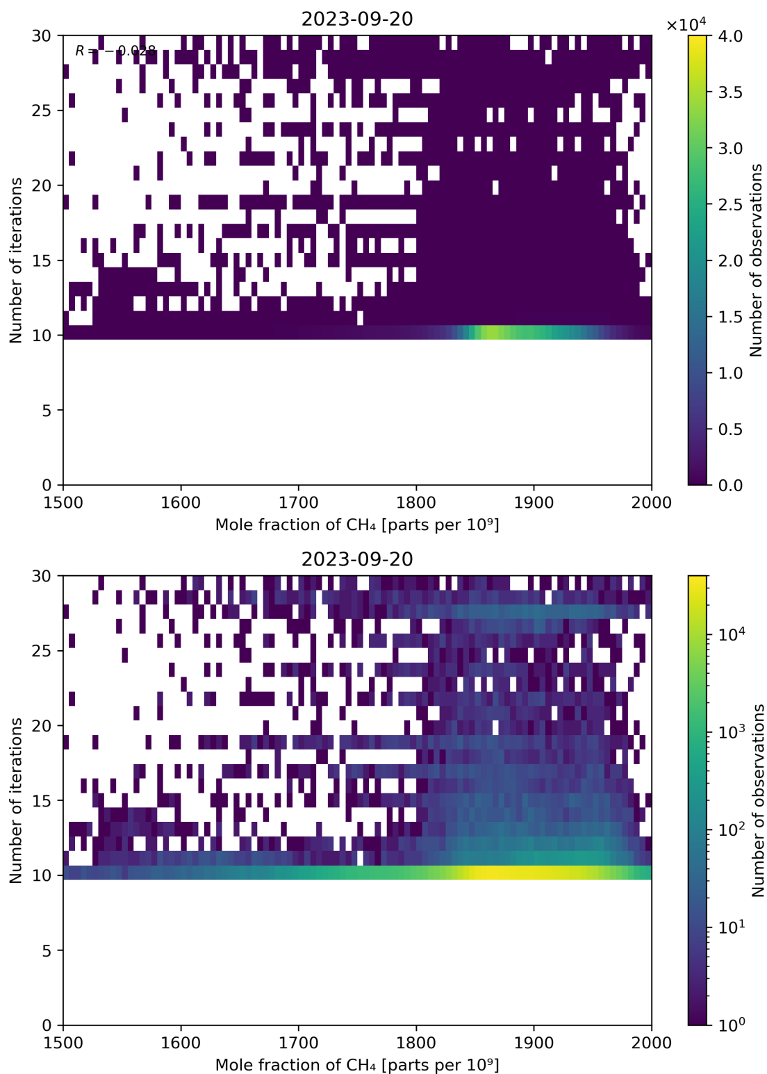
Figure 76: Scatter density plot of “Mole fraction of CH 4 ” against “Number of iterations” for 2023-09-20 to 2023-09-21.
