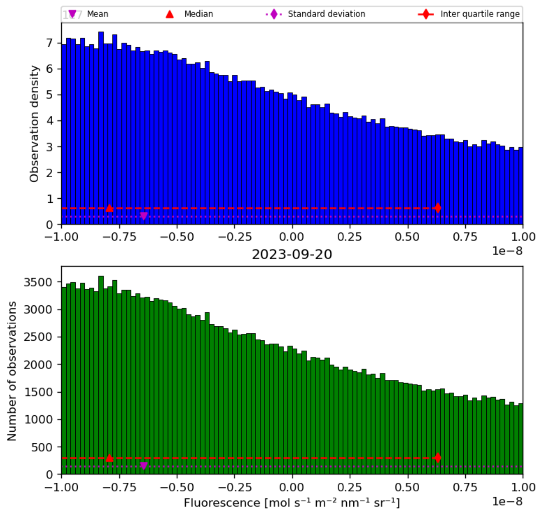
Figure 32: Histogram of “Fluorescence” for 2023-09-20 to 2023-09-21
