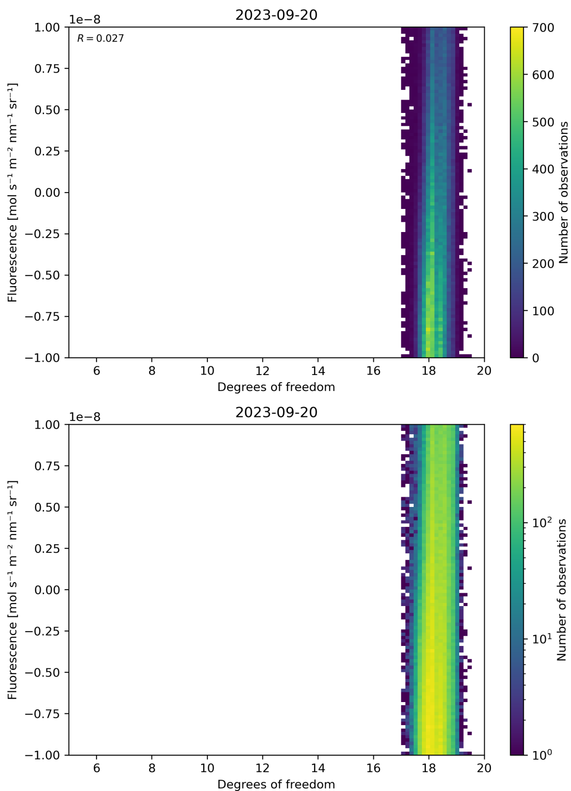
Figure 51: Scatter density plot of “Degrees of freedom” against “Fluorescence” for 2023-09-20 to 2023-09-21.
