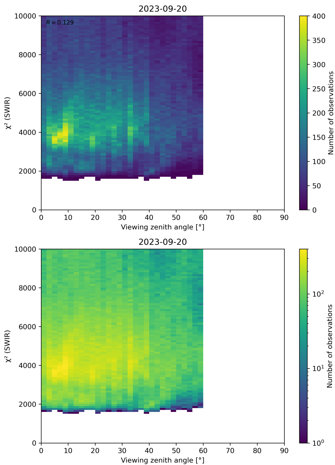
Figure 106: Scatter density plot of “Viewing zenith angle” against “ \chi^2 (SWIR)” for 2023-09-20 to 2023-09-21.
