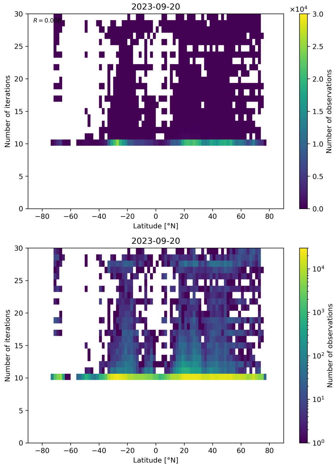
Figure 60: Scatter density plot of “Latitude” against “Number of iterations” for 2023-09-20 to 2023-09-21.
