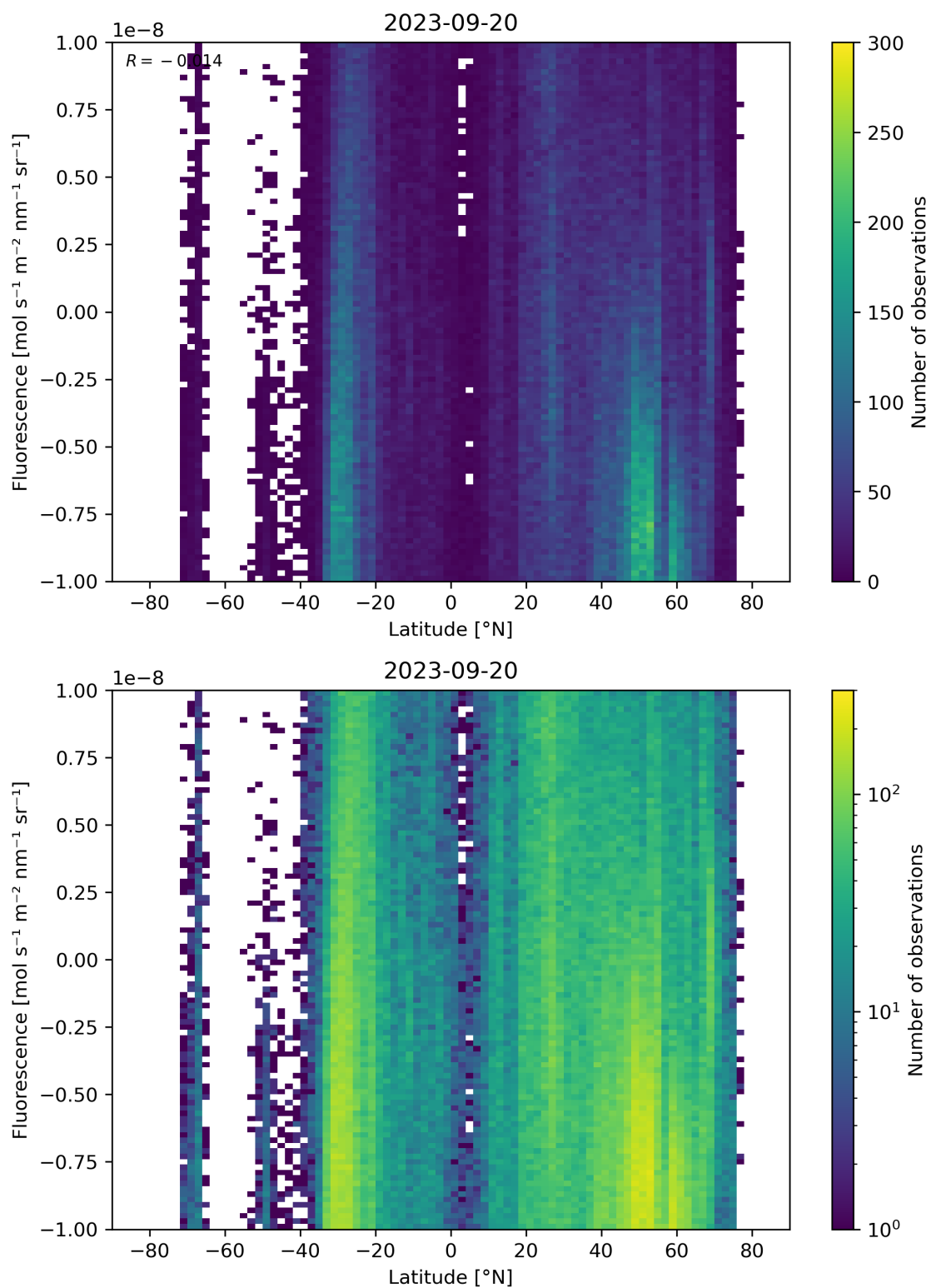
Figure 56: Scatter density plot of “Latitude” against “Fluorescence” for 2023-09-20 to 2023-09-21.
