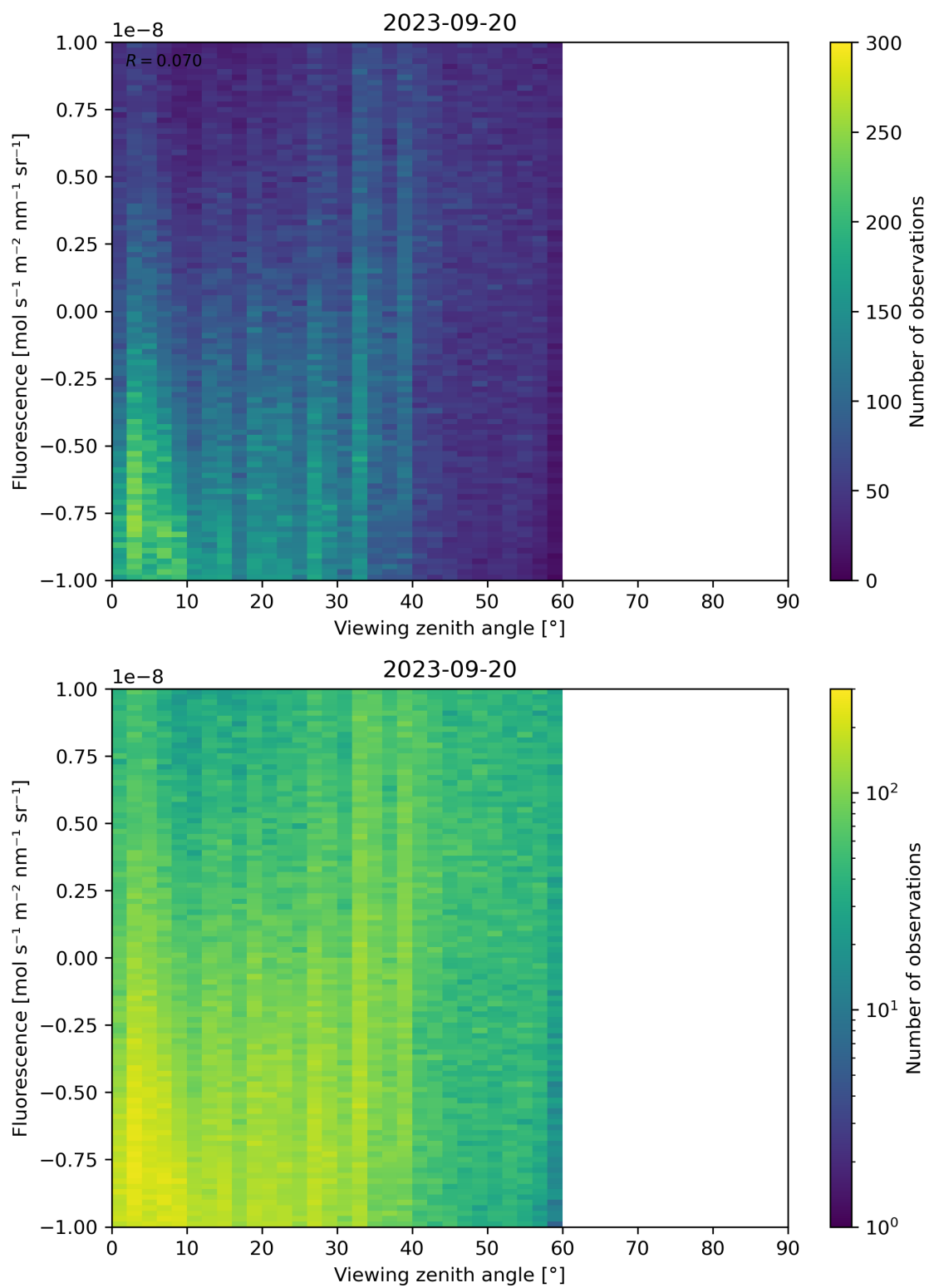
Figure 108: Scatter density plot of “Viewing zenith angle” against “Fluorescence” for 2023-09-20 to 2023-09-21.
