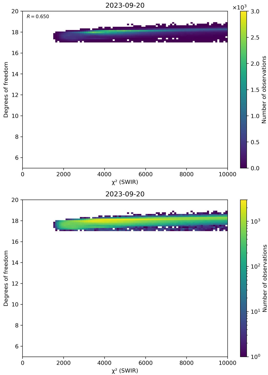
Figure 48: Scatter density plot of “ \chi^2 (SWIR)” against “Degrees of freedom” for 2023-09-20 to 2023-09-21.
