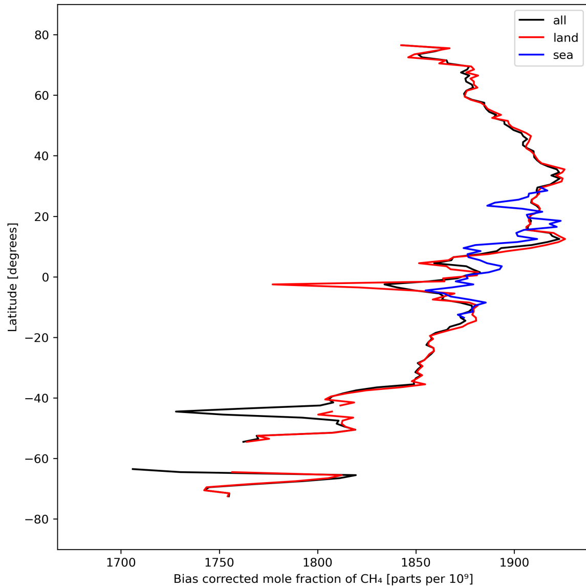
Figure 14: Zonal average of “Bias corrected mole fraction of CH 4 ” for 2023-09-20 to 2023-09-21.
