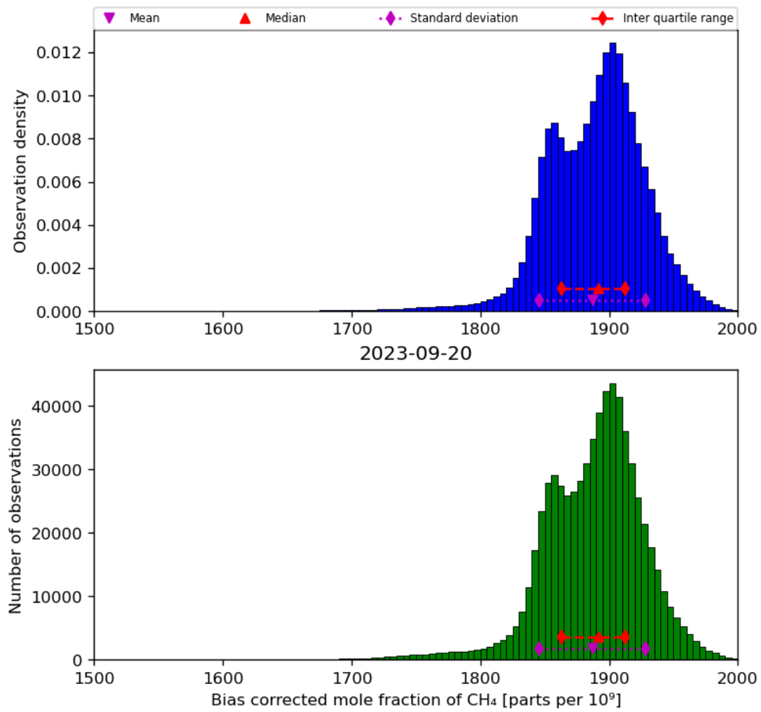
Figure 25: Histogram of “Bias corrected mole fraction of CH 4 ” for 2023-09-20 to 2023-09-21
