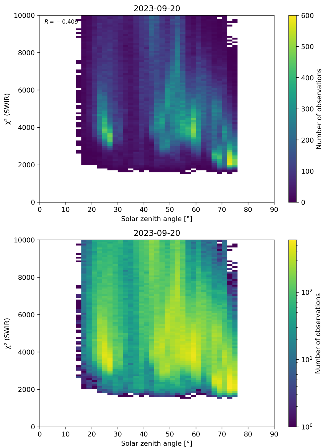
Figure 95: Scatter density plot of “Solar zenith angle” against “ \chi^2 (SWIR)” for 2023-09-20 to 2023-09-21.
