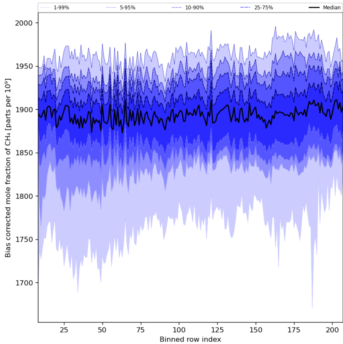
Figure 36: Along track statistics of “Bias corrected mole fraction of CH 4 ” for 2023-09-20 to 2023-09-21
