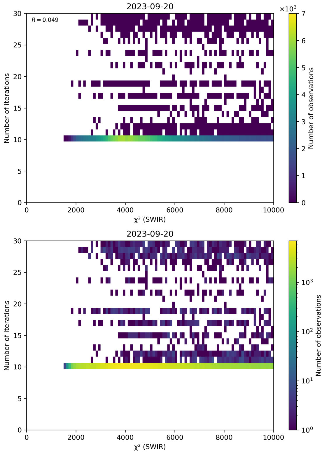
Figure 50: Scatter density plot of “ \chi^2 (SWIR)” against “Number of iterations” for 2023-09-20 to 2023-09-21.
