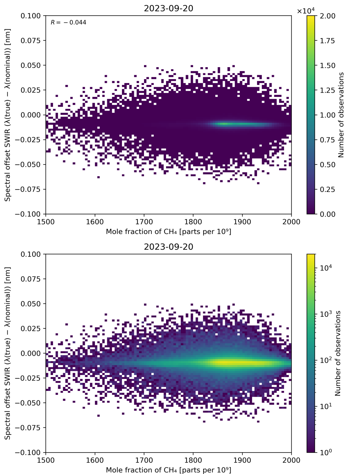
Figure 86: Scatter density plot of “Mole fraction of CH 4 ” against “Spectral offset SWIR ( \lambda(\text{true}) - \lambda(\text{nominal}) )” for 2023-09-20 to 2023-09-21.
