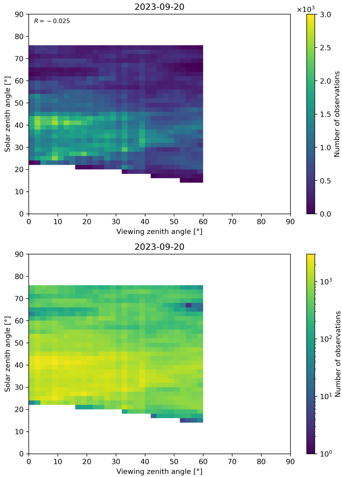
Figure 115: Scatter density plot of “Viewing zenith angle” against “Solar zenith angle” for 2023-09-20 to 2023-09-21.
