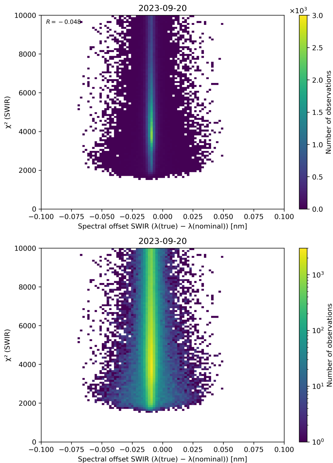
Figure 118: Scatter density plot of “Spectral offset SWIR ( \lambda(\text{true}) - \lambda(\text{nominal}) )” against “ \chi^2 (SWIR)” for 2023-09-20 to 2023-09-21.
