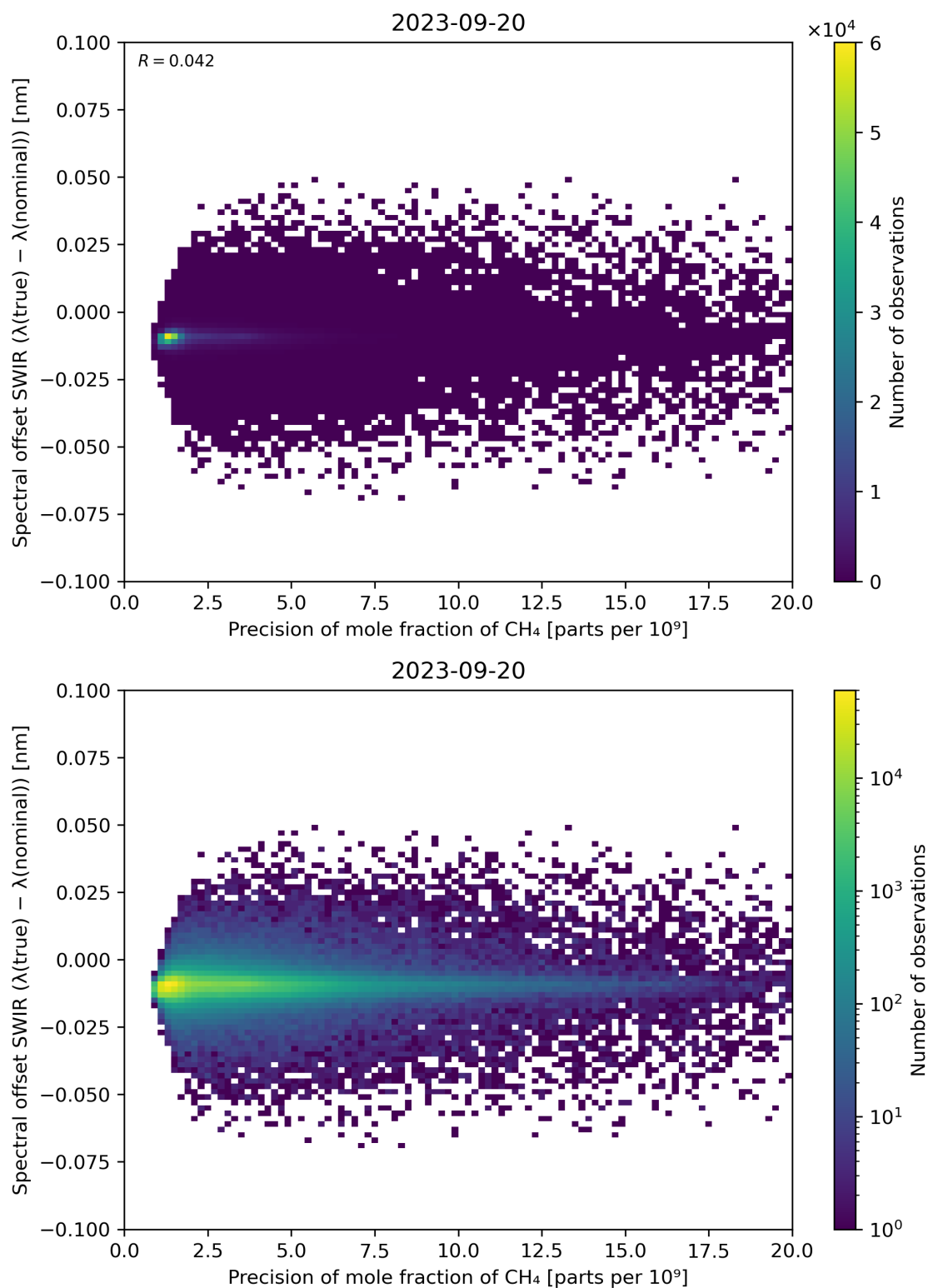
Figure 85: Scatter density plot of “Precision of mole fraction of CH 4 ” against “Spectral offset SWIR ( \lambda(\text{true}) - \lambda(\text{nominal}) )” for 2023-09-20 to 2023-09-21.
