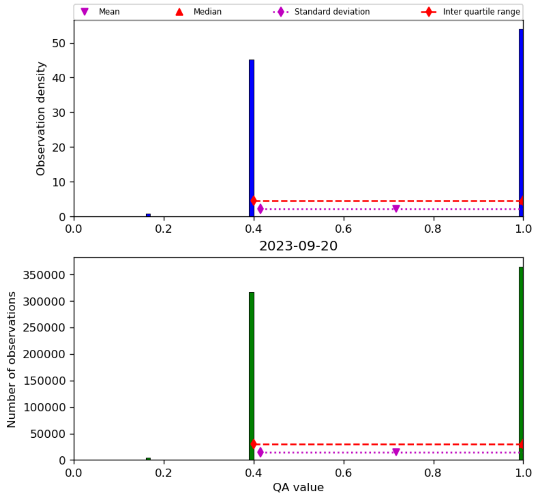
Figure 22: Histogram of “QA value” for 2023-09-20 to 2023-09-21
