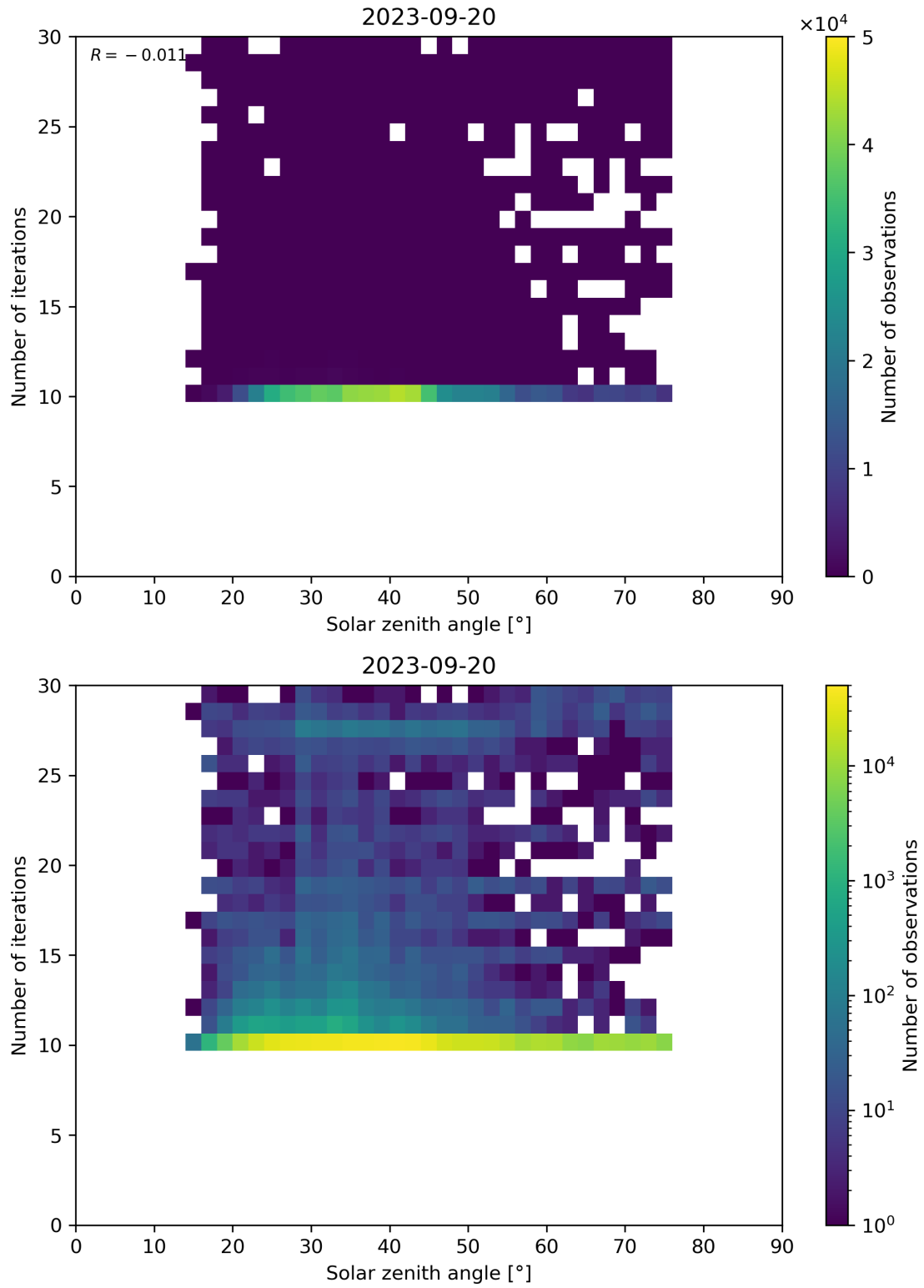
Figure 102: Scatter density plot of “Solar zenith angle” against “Number of iterations” for 2023-09-20 to 2023-09-21.
