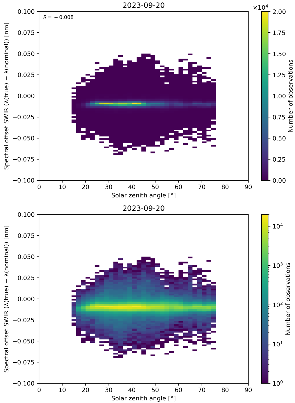
Figure 104: Scatter density plot of “Solar zenith angle” against “Spectral offset SWIR ( \lambda(\text{true}) - \lambda(\text{nominal}) )” for 2023-09-20 to 2023-09-21.
