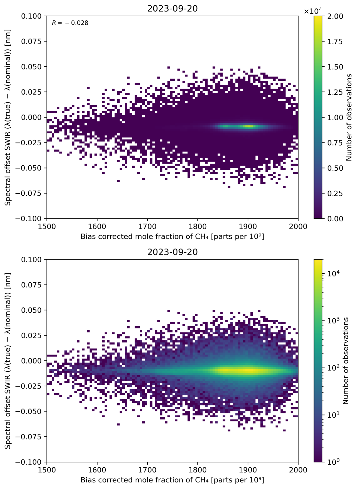
Figure 69: Scatter density plot of “Bias corrected mole fraction of \text{CH}_4 ” against “Spectral offset SWIR ( \lambda(\text{true}) - \lambda(\text{nominal}) )” for 2023-09-20 to 2023-09-21.
