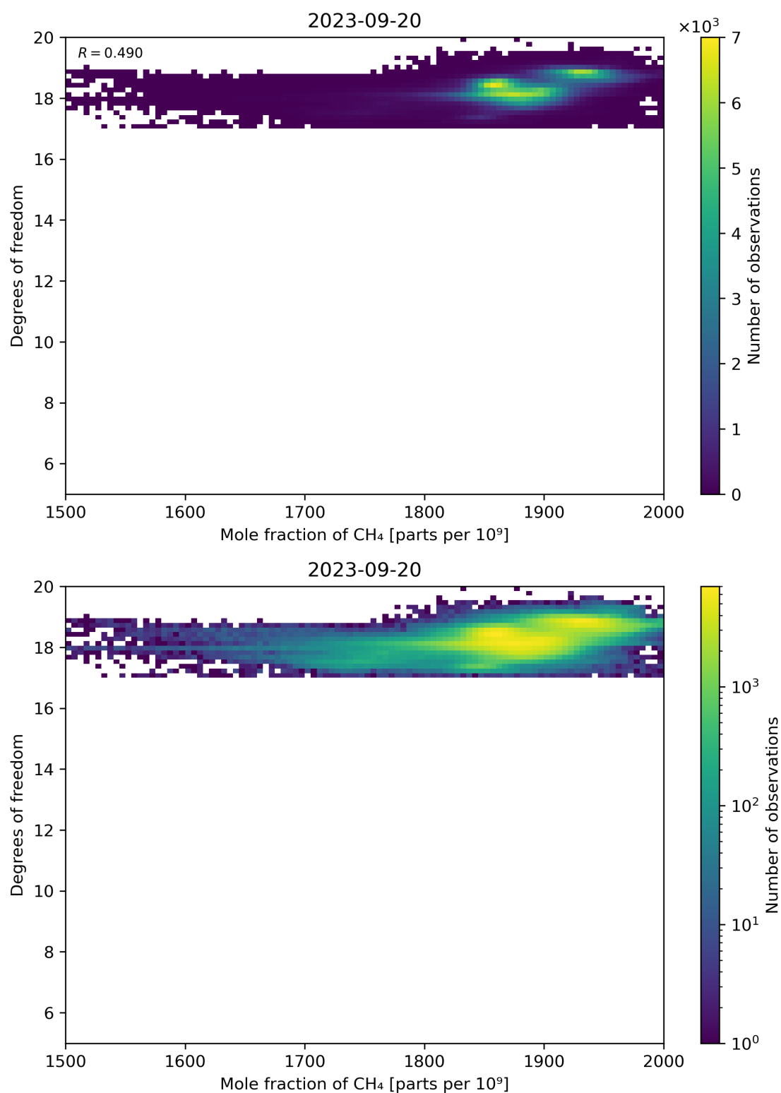
Figure 72: Scatter density plot of “Mole fraction of CH 4 ” against “Degrees of freedom” for 2023-09-20 to 2023-09-21.
