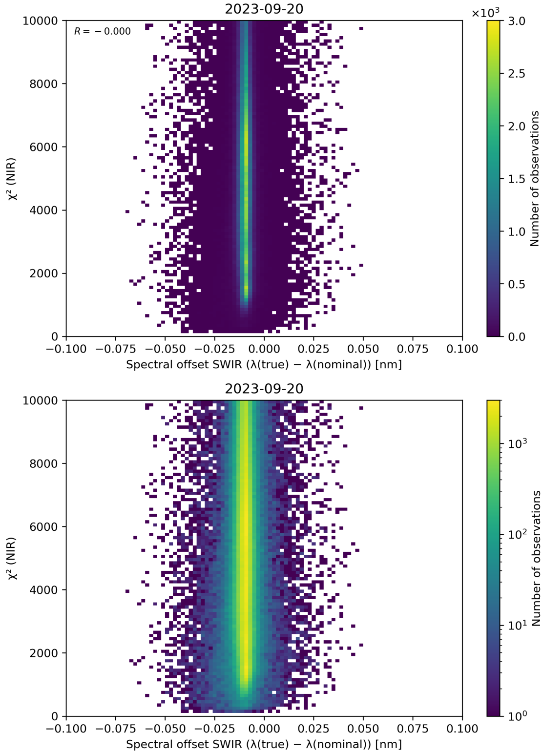
Figure 117: Scatter density plot of “Spectral offset SWIR ( \lambda(\text{true}) - \lambda(\text{nominal}) )” against “ \chi^2 (NIR)” for 2023-09-20 to 2023-09-21.
