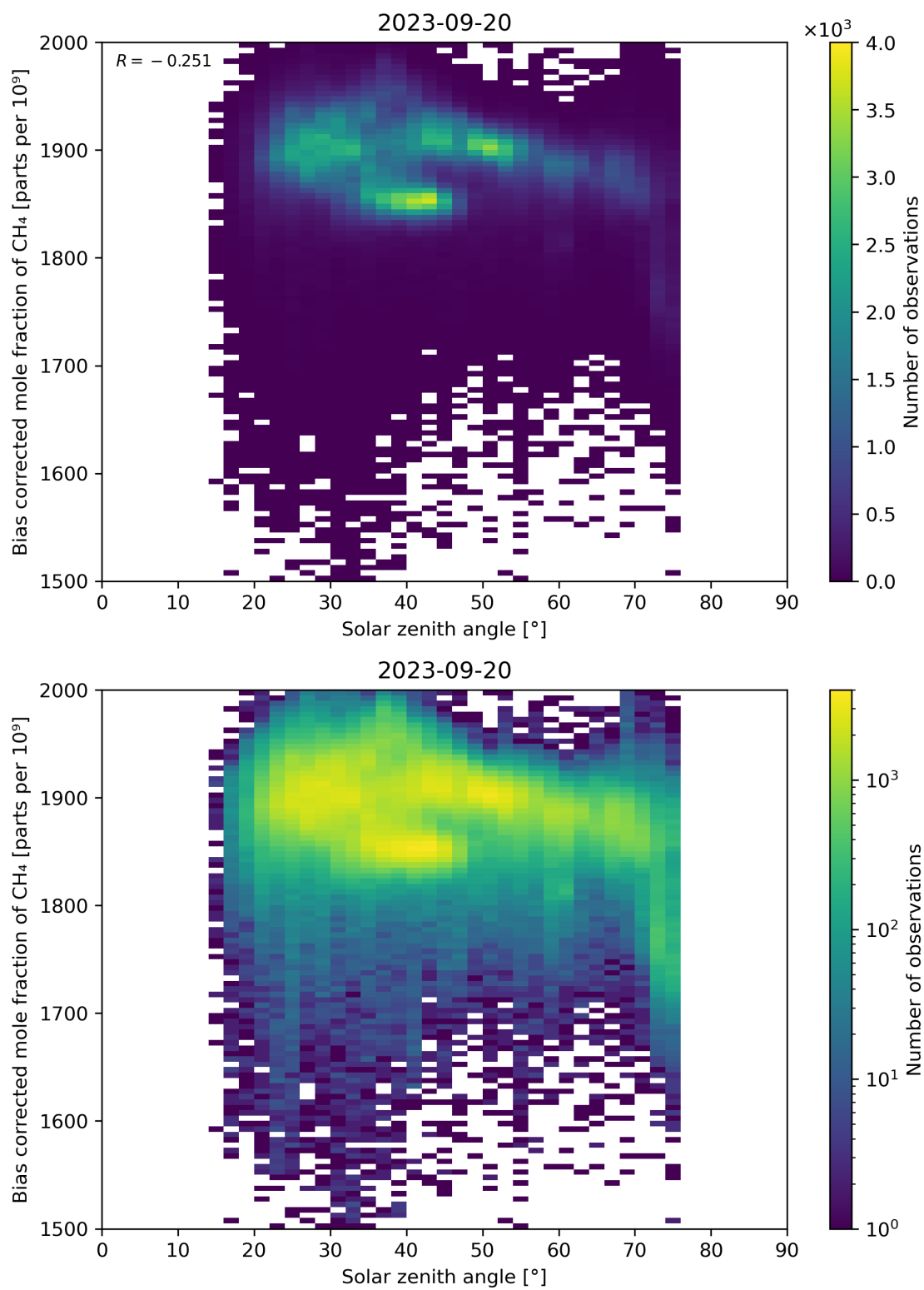
Figure 100: Scatter density plot of “Solar zenith angle” against “Bias corrected mole fraction of CH 4 ” for 2023-09-20 to 2023-09-21.
