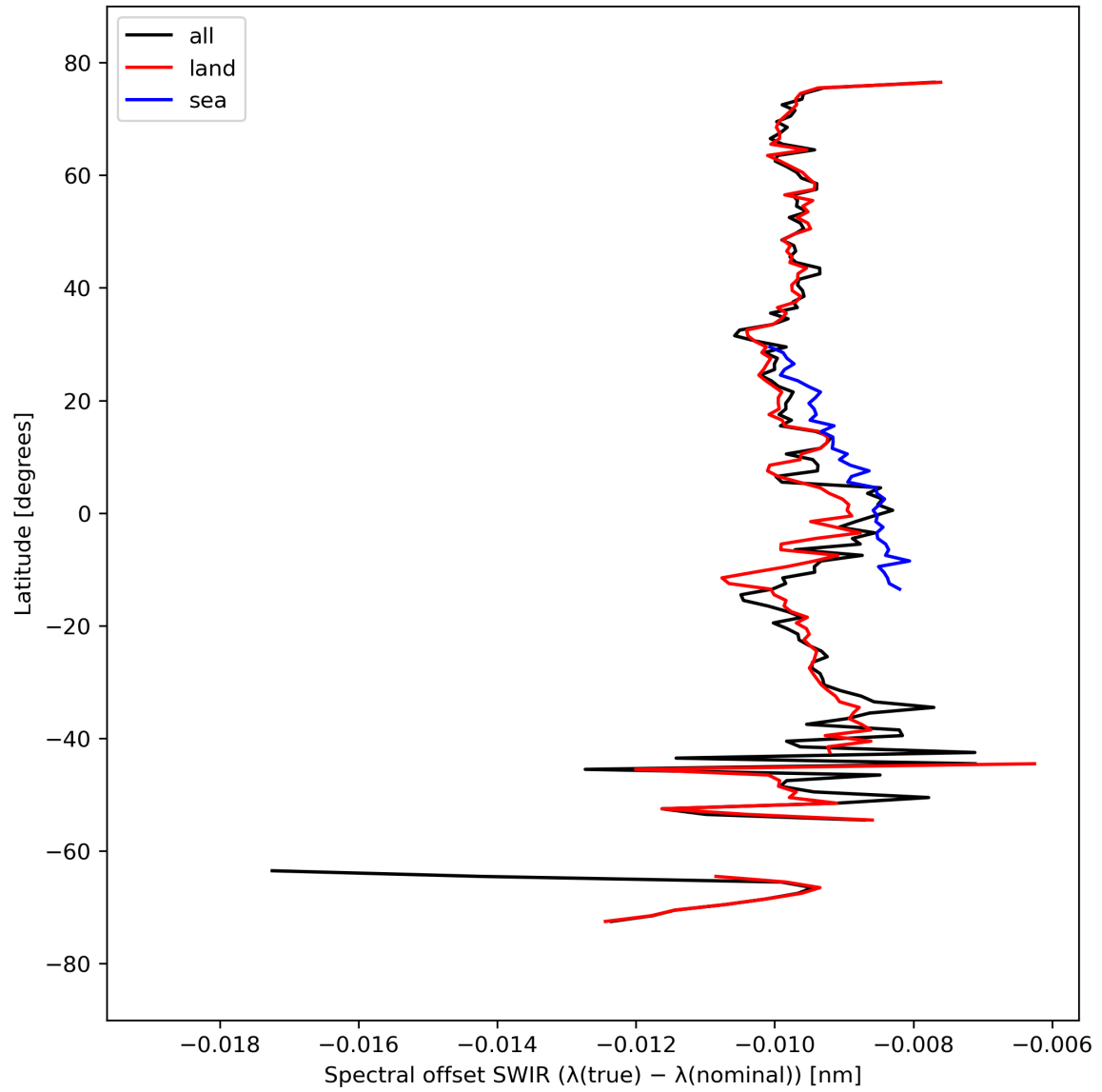
Figure 16: Zonal average of “Spectral offset SWIR ( \lambda(\text{true}) - \lambda(\text{nominal}) )” for 2023-09-20 to 2023-09-21.
