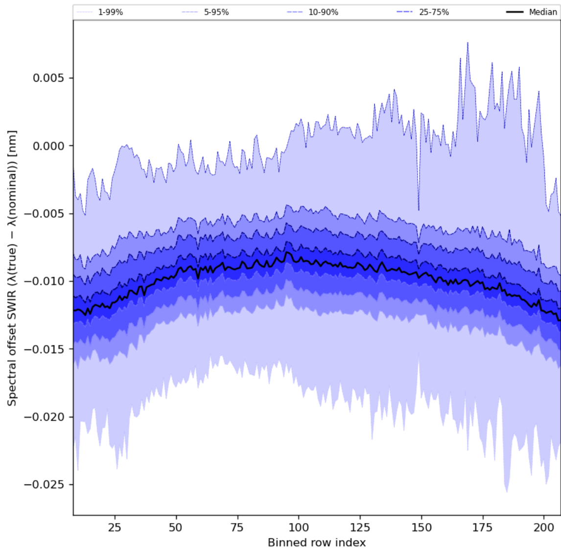
Figure 38: Along track statistics of “Spectral offset SWIR ( \lambda(\text{true}) - \lambda(\text{nominal}) )” for 2023-09-20 to 2023-09-21
