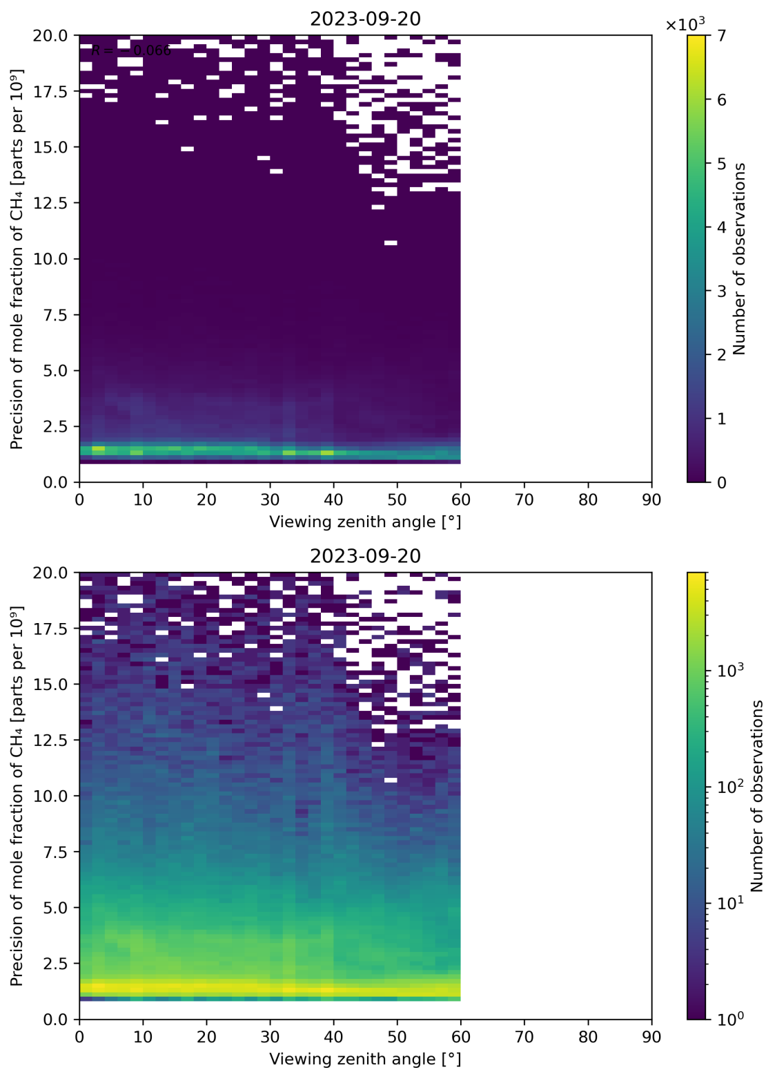
Figure 112: Scatter density plot of “Viewing zenith angle” against “Precision of mole fraction of CH 4 ” for 2023-09-20 to 2023-09-21.
