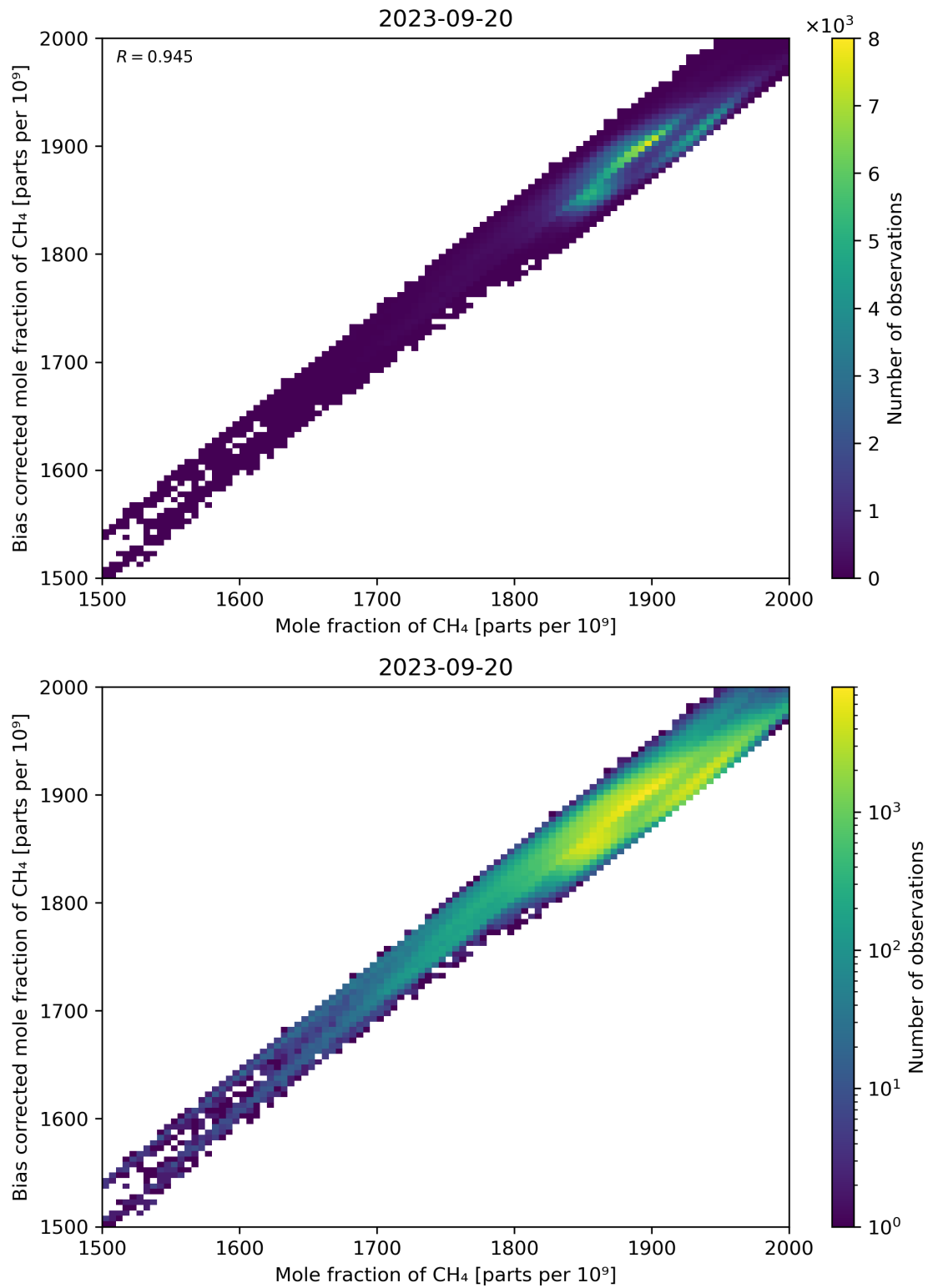
Figure 74: Scatter density plot of “Mole fraction of CH 4 ” against “Bias corrected mole fraction of CH 4 ” for 2023-09-20 to 2023-09-21.
