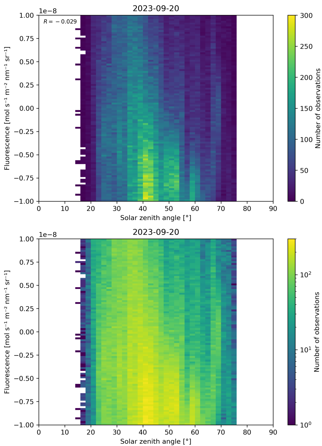
Figure 97: Scatter density plot of “Solar zenith angle” against “Fluorescence” for 2023-09-20 to 2023-09-21.
