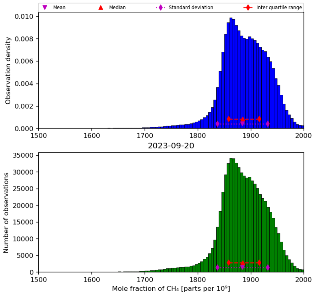
Figure 23: Histogram of “Mole fraction of CH 4 ” for 2023-09-20 to 2023-09-21
