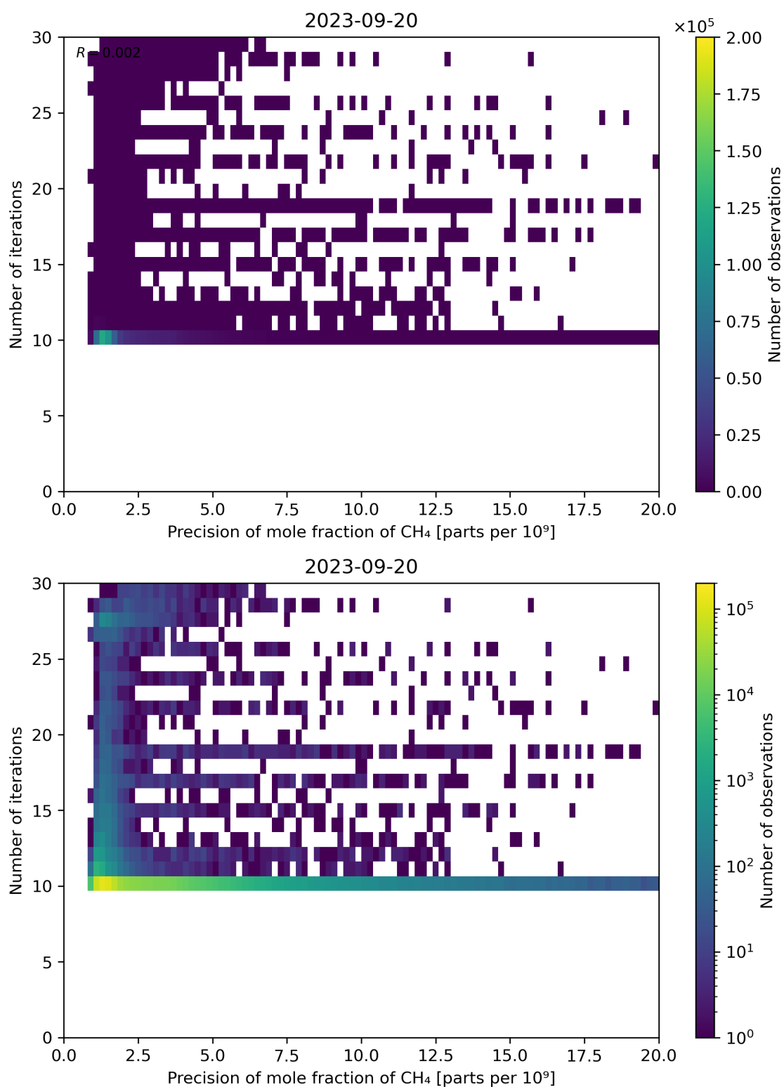
Figure 83: Scatter density plot of “Precision of mole fraction of CH 4 ” against “Number of iterations” for 2023-09-20 to 2023-09-21.
