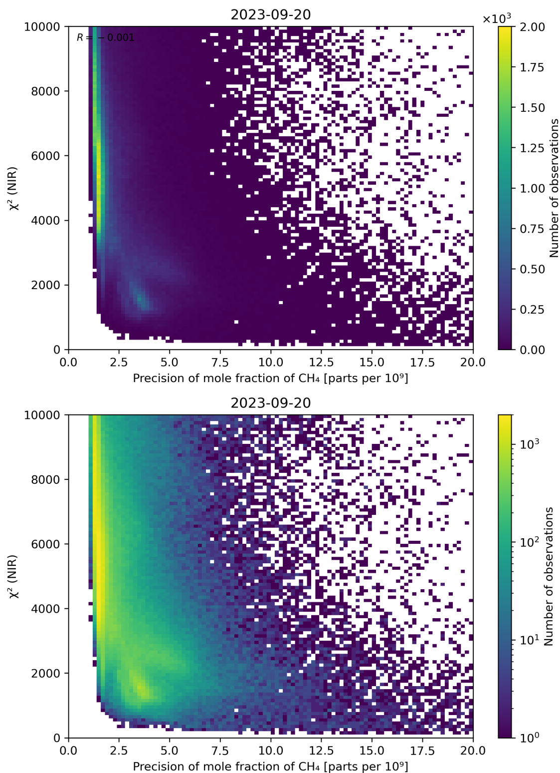
Figure 78: Scatter density plot of “Precision of mole fraction of \text{CH}_4 ” against “ \chi^2 (NIR)” for 2023-09-20 to 2023-09-21.
