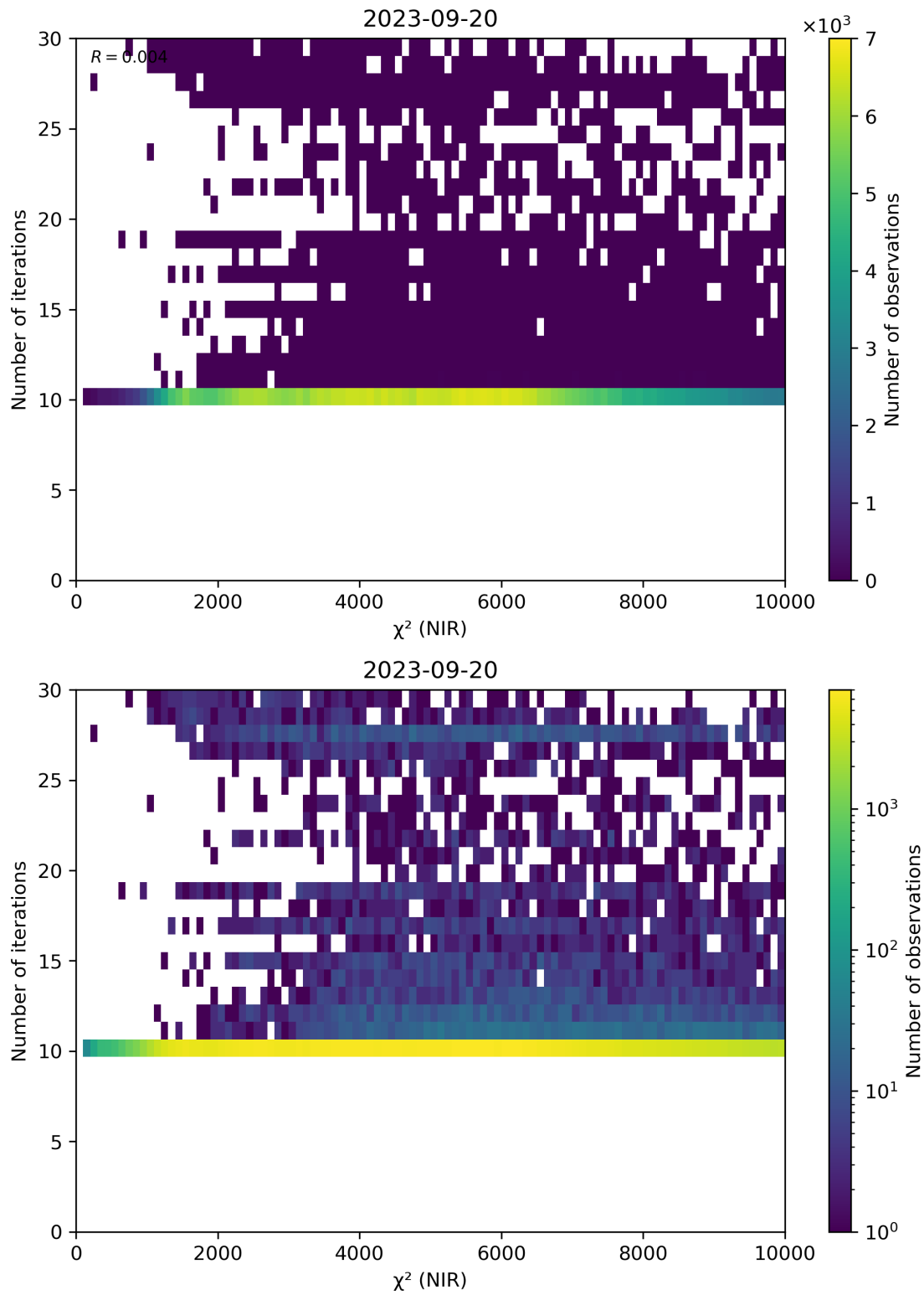
Figure 46: Scatter density plot of “ \chi^2 (NIR)” against “Number of iterations” for 2023-09-20 to 2023-09-21.
