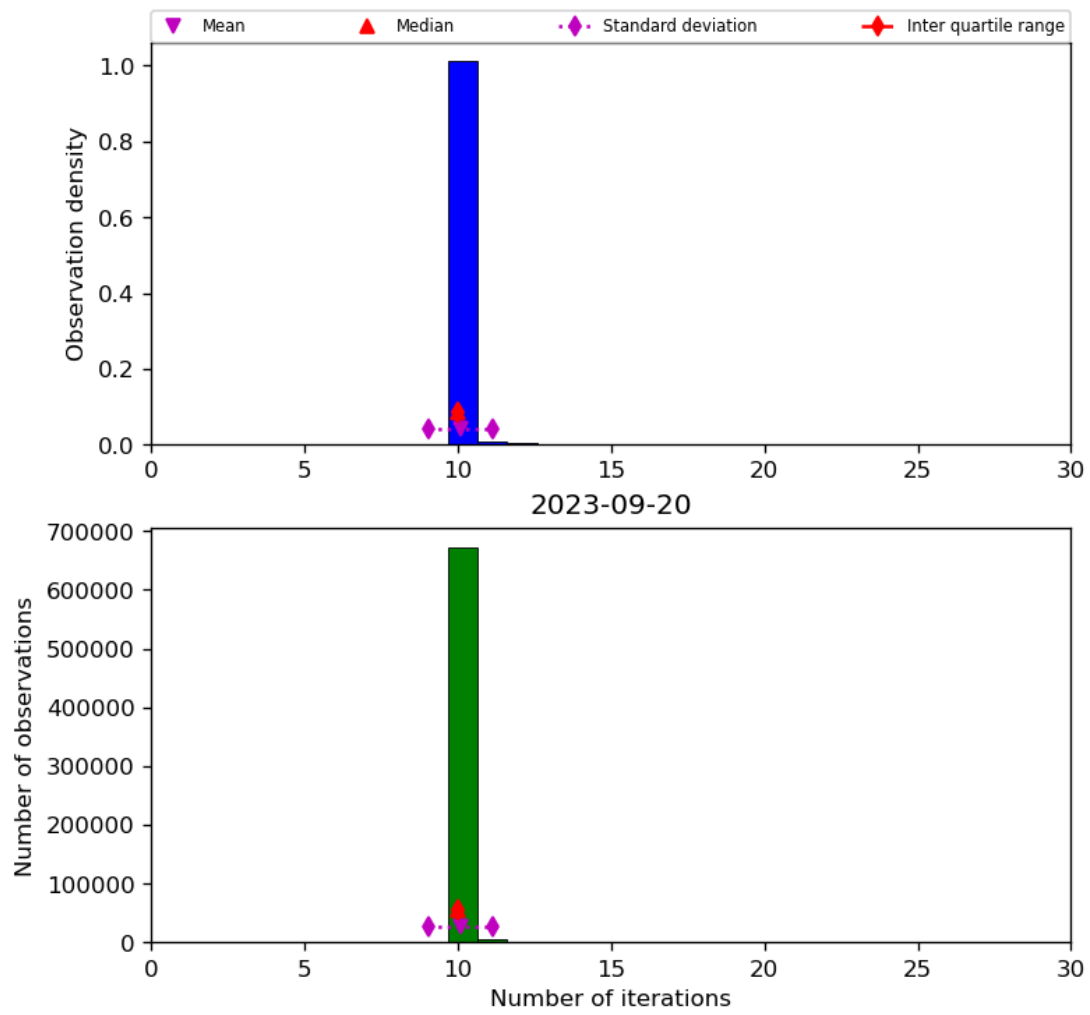
Figure 31: Histogram of “Number of iterations” for 2023-09-20 to 2023-09-21
