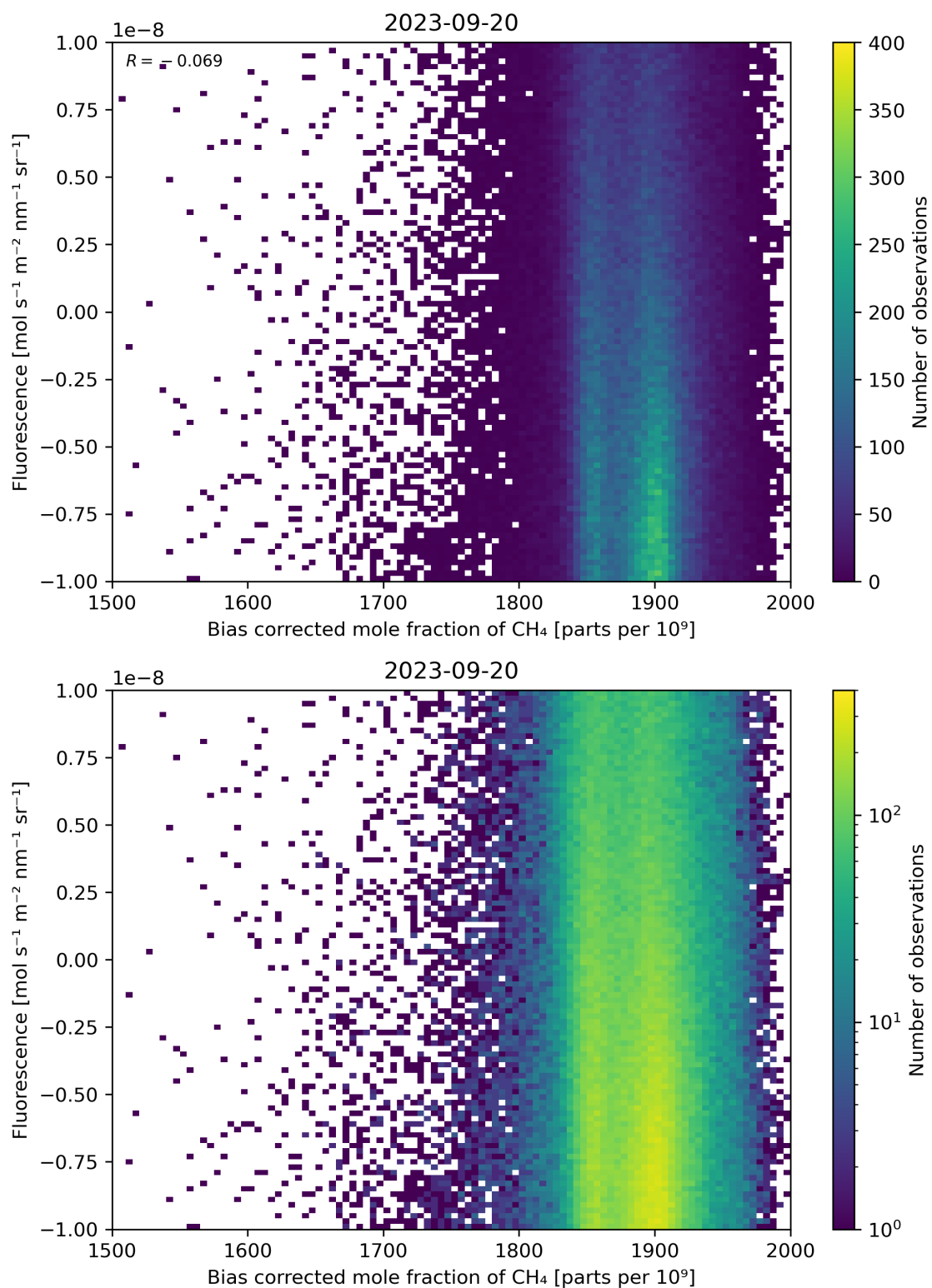
Figure 66: Scatter density plot of “Bias corrected mole fraction of \text{CH}_4 ” against “Fluorescence” for 2023-09-20 to 2023-09-21.
