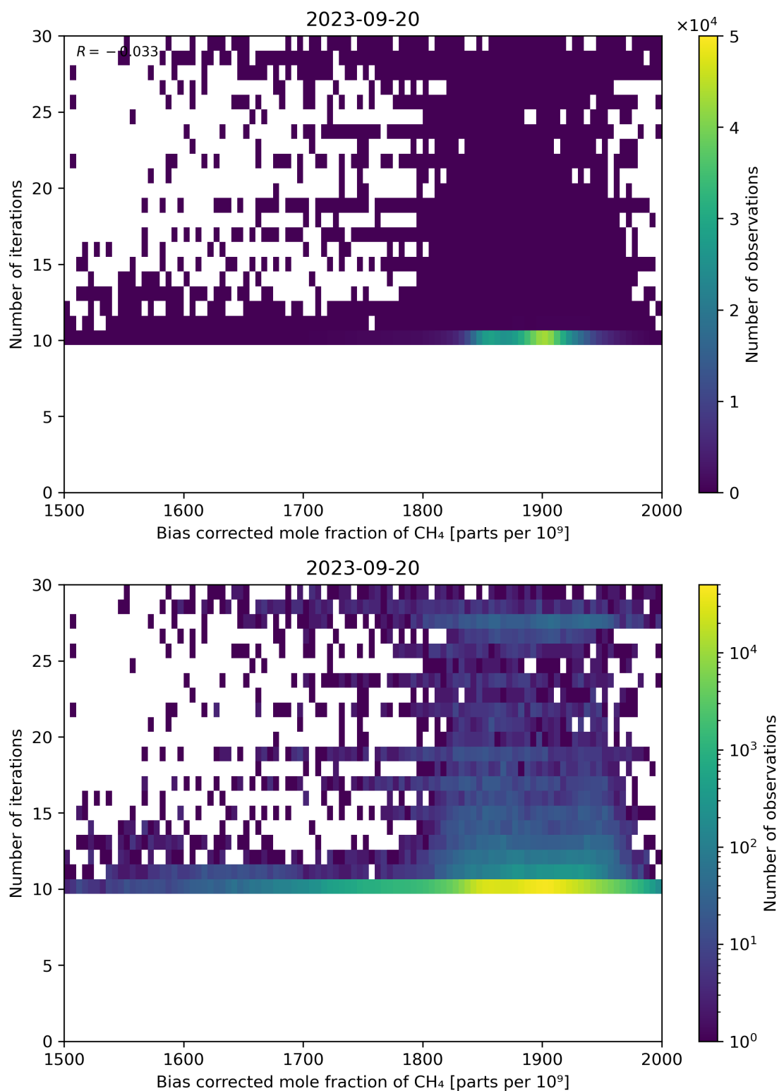
Figure 67: Scatter density plot of “Bias corrected mole fraction of CH 4 ” against “Number of iterations” for 2023-09-20 to 2023-09-21.
