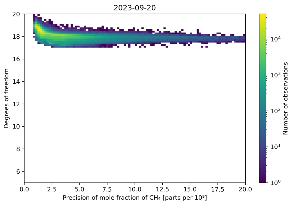
Figure 80: Scatter density plot of “Precision of mole fraction of CH 4 ” against “Degrees of freedom” for 2023-09-20 to 2023-09-21.
