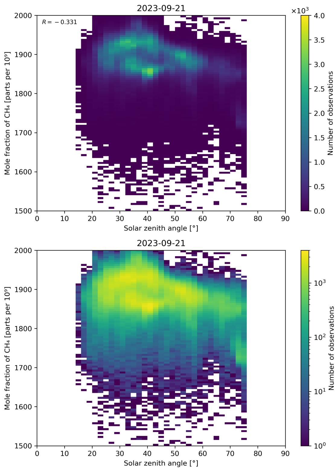
Figure 99: Scatter density plot of “Solar zenith angle” against “Mole fraction of CH 4 ” for 2023-09-20 to 2023-09-22.
