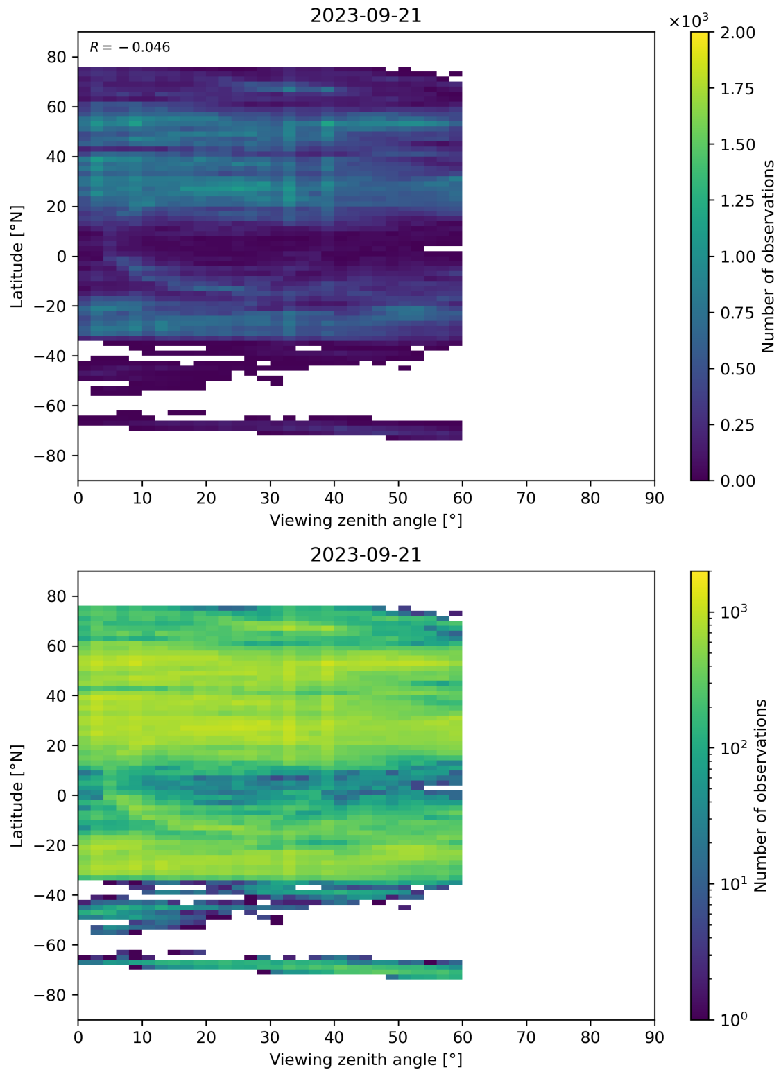
Figure 109: Scatter density plot of “Viewing zenith angle” against “Latitude” for 2023-09-20 to 2023-09-22.
