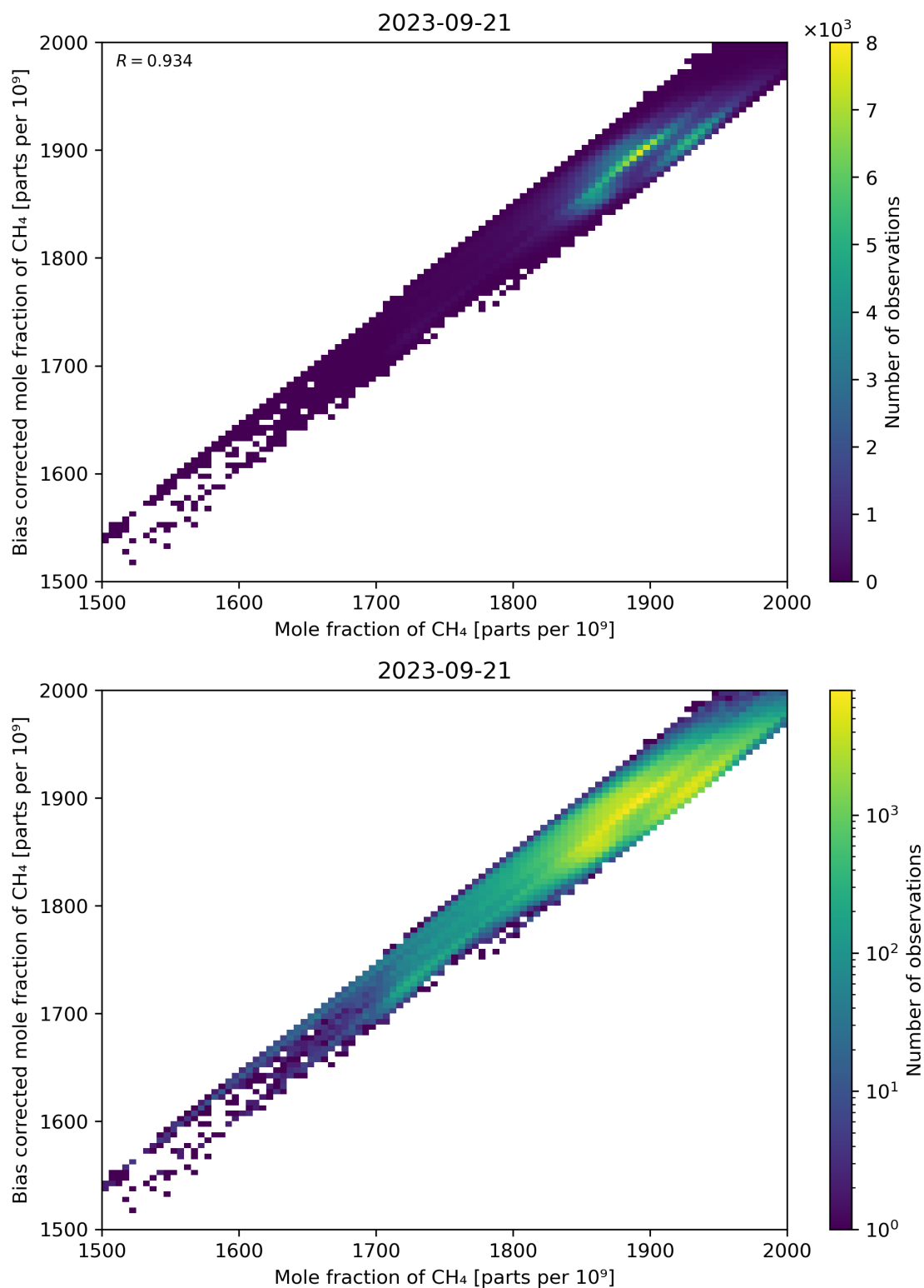
Figure 74: Scatter density plot of “Mole fraction of CH 4 ” against “Bias corrected mole fraction of CH 4 ” for 2023-09-20 to 2023-09-22.
