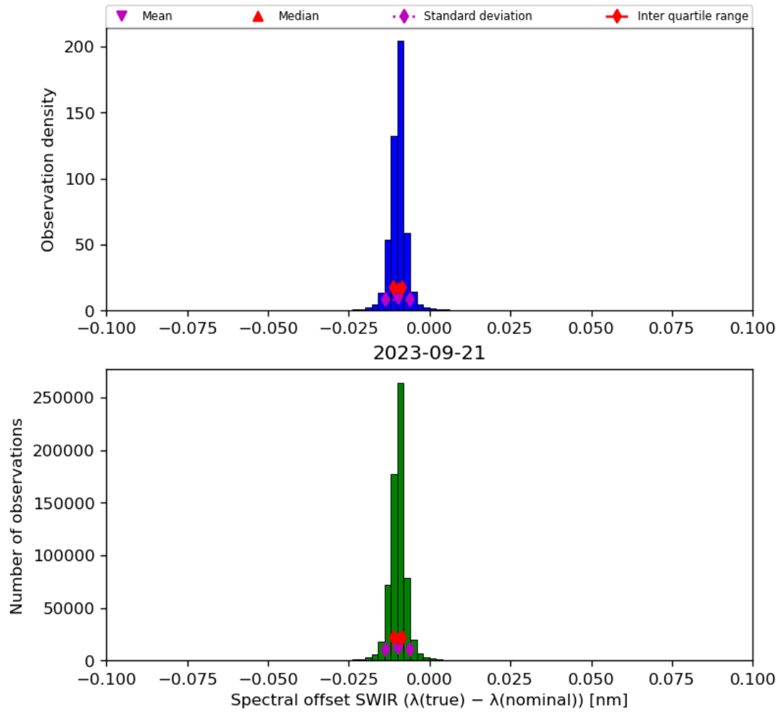
Figure 27: Histogram of “Spectral offset SWIR ( \lambda(\text{true}) - \lambda(\text{nominal}) )” for 2023-09-20 to 2023-09-22
