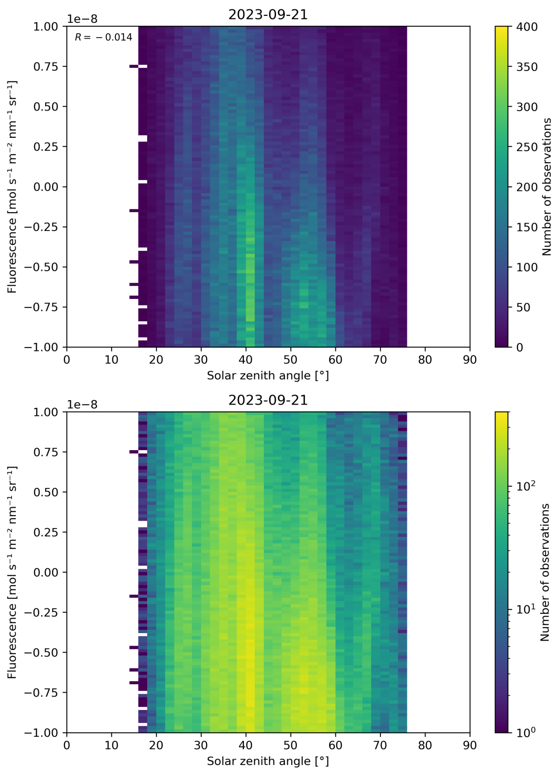
Figure 97: Scatter density plot of “Solar zenith angle” against “Fluorescence” for 2023-09-20 to 2023-09-22.
