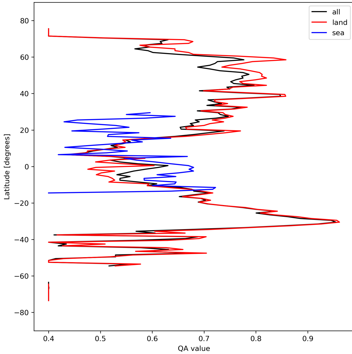
Figure 11: Zonal average of “QA value” for 2023-09-20 to 2023-09-22.
