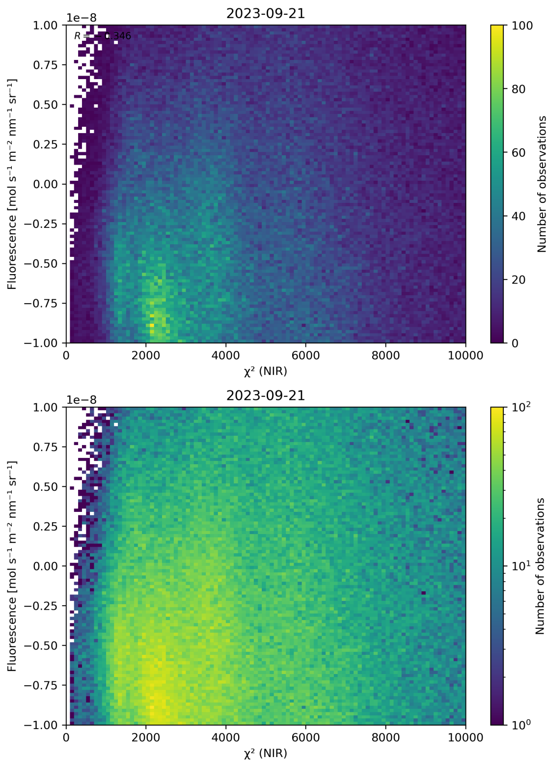
Figure 45: Scatter density plot of “ \chi^2 (NIR)” against “Fluorescence” for 2023-09-20 to 2023-09-22.
