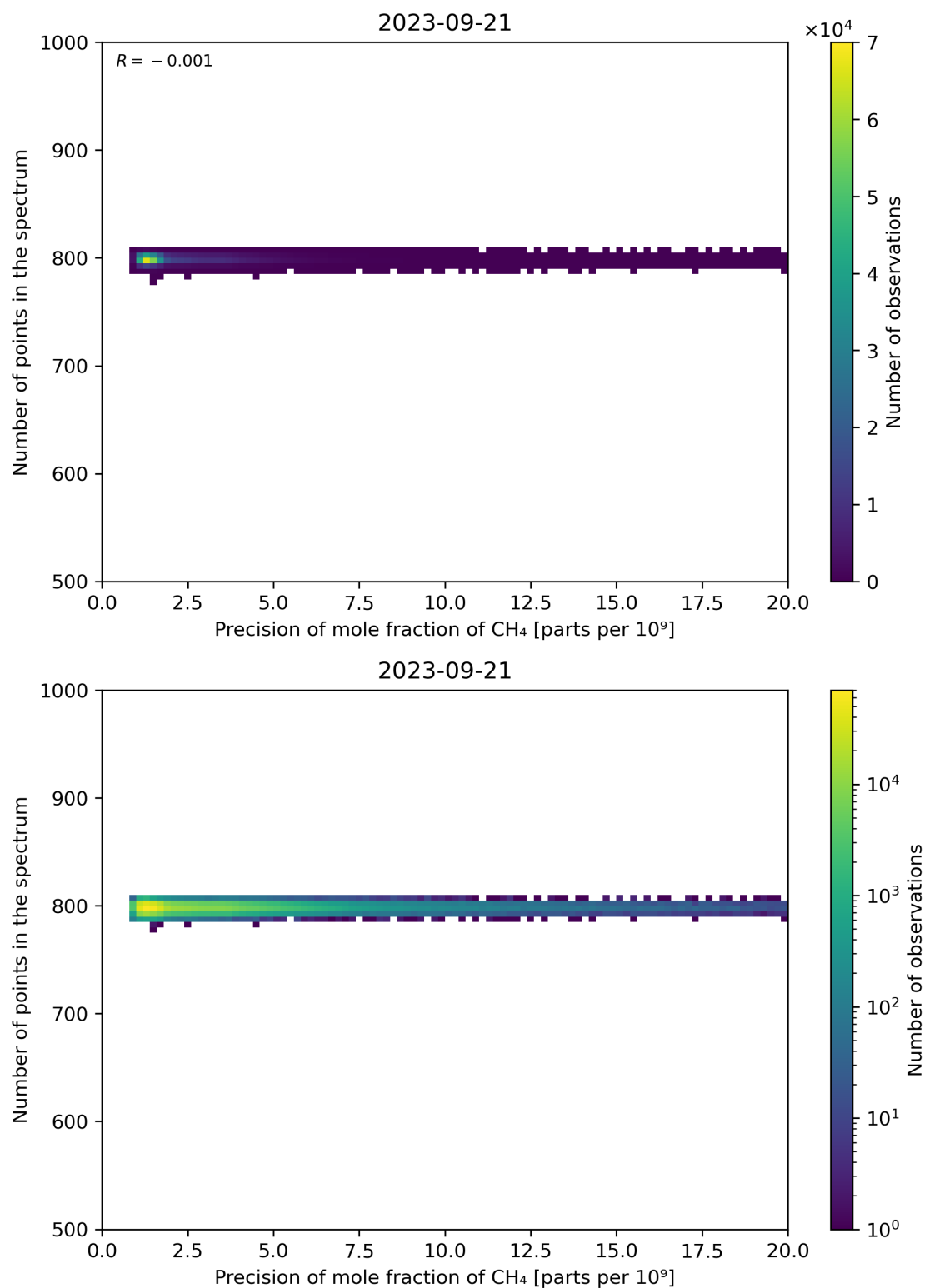
Figure 84: Scatter density plot of “Precision of mole fraction of CH 4 ” against “Number of points in the spectrum” for 2023-09-20 to 2023-09-22.
