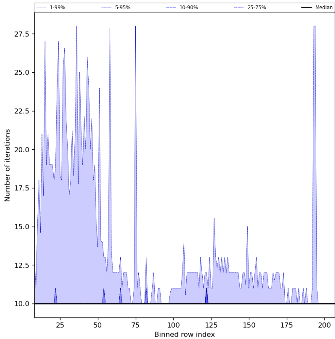
Figure 42: Along track statistics of “Number of iterations” for 2023-09-20 to 2023-09-22
