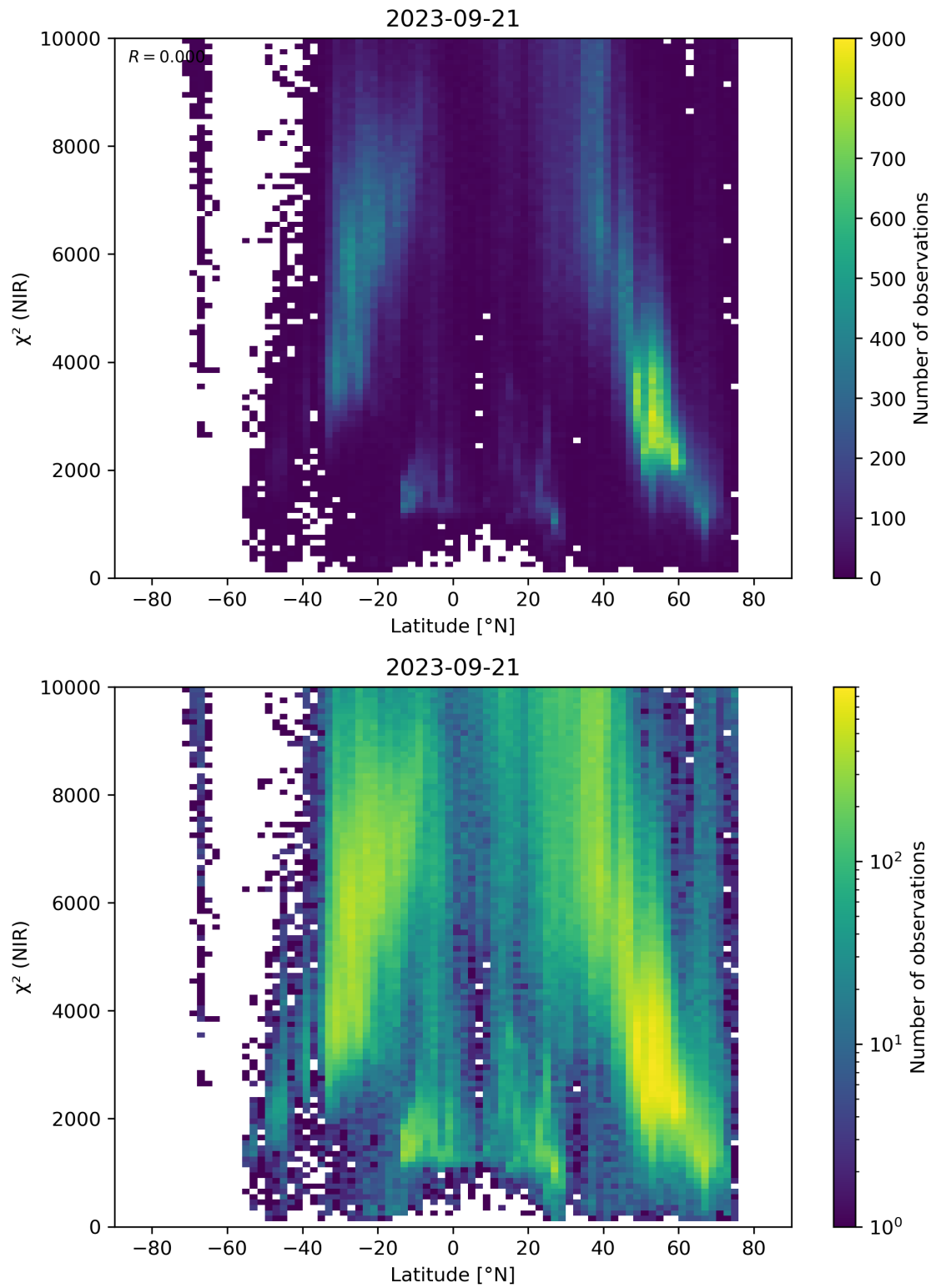
Figure 53: Scatter density plot of “Latitude” against “ \chi^2 (NIR)” for 2023-09-20 to 2023-09-22.
