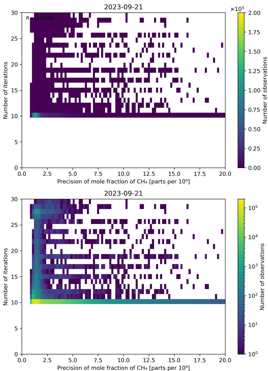
Figure 83: Scatter density plot of “Precision of mole fraction of CH 4 ” against “Number of iterations” for 2023-09-20 to 2023-09-22.
