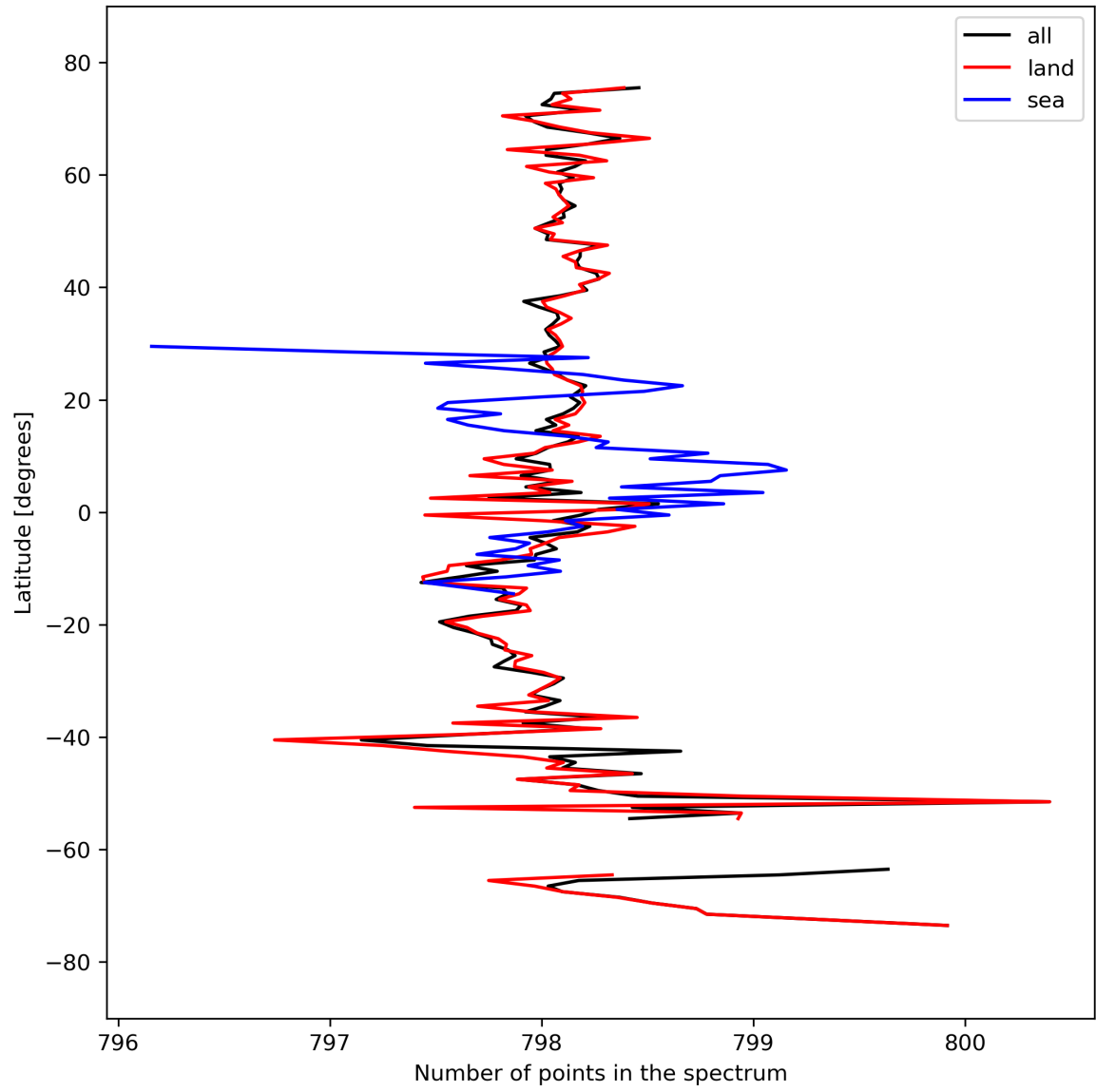
Figure 15: Zonal average of “Number of points in the spectrum” for 2023-09-20 to 2023-09-22.
