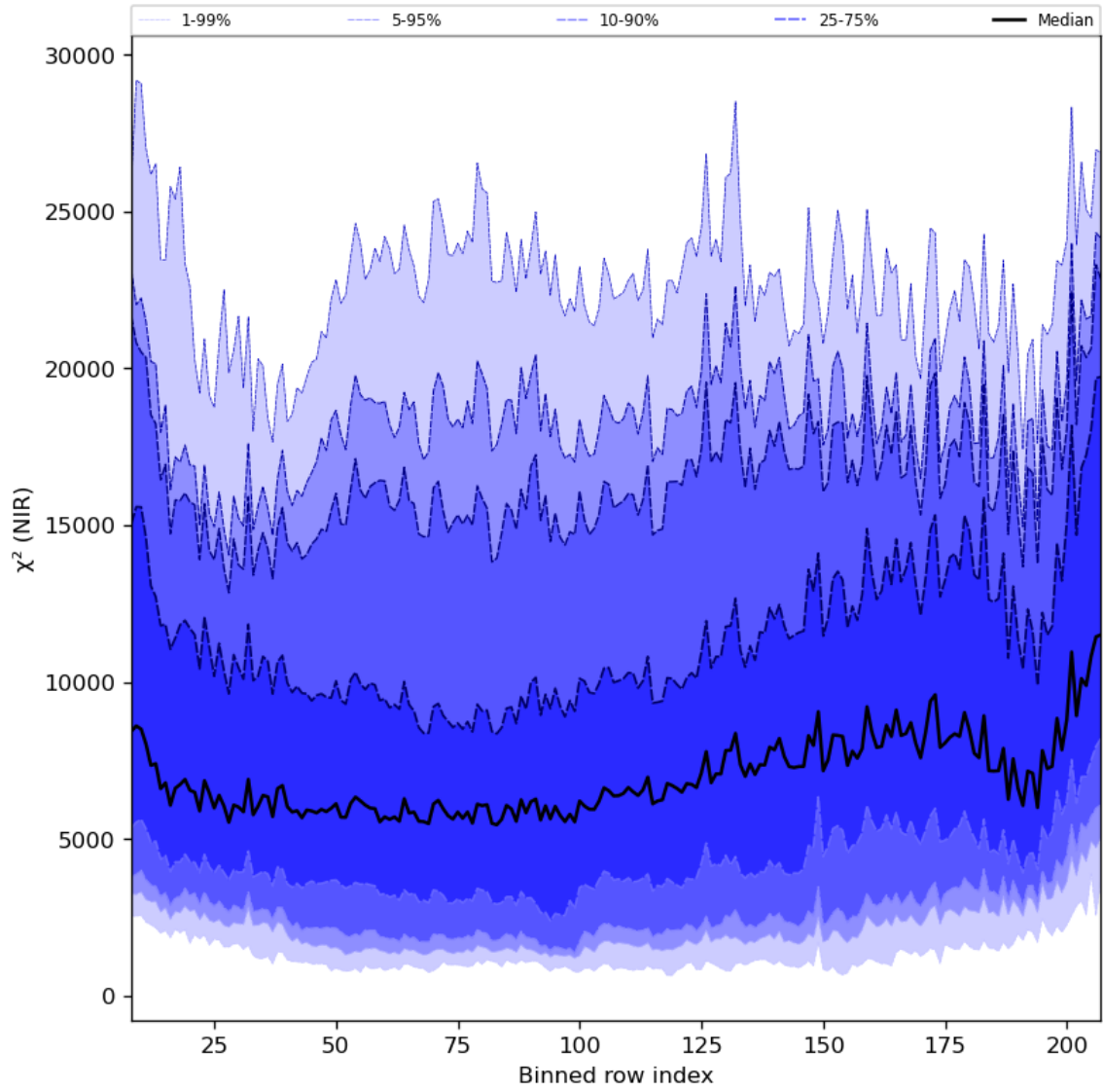
Figure 40: Along track statistics of “ \chi^2 (NIR)” for 2023-09-20 to 2023-09-22
