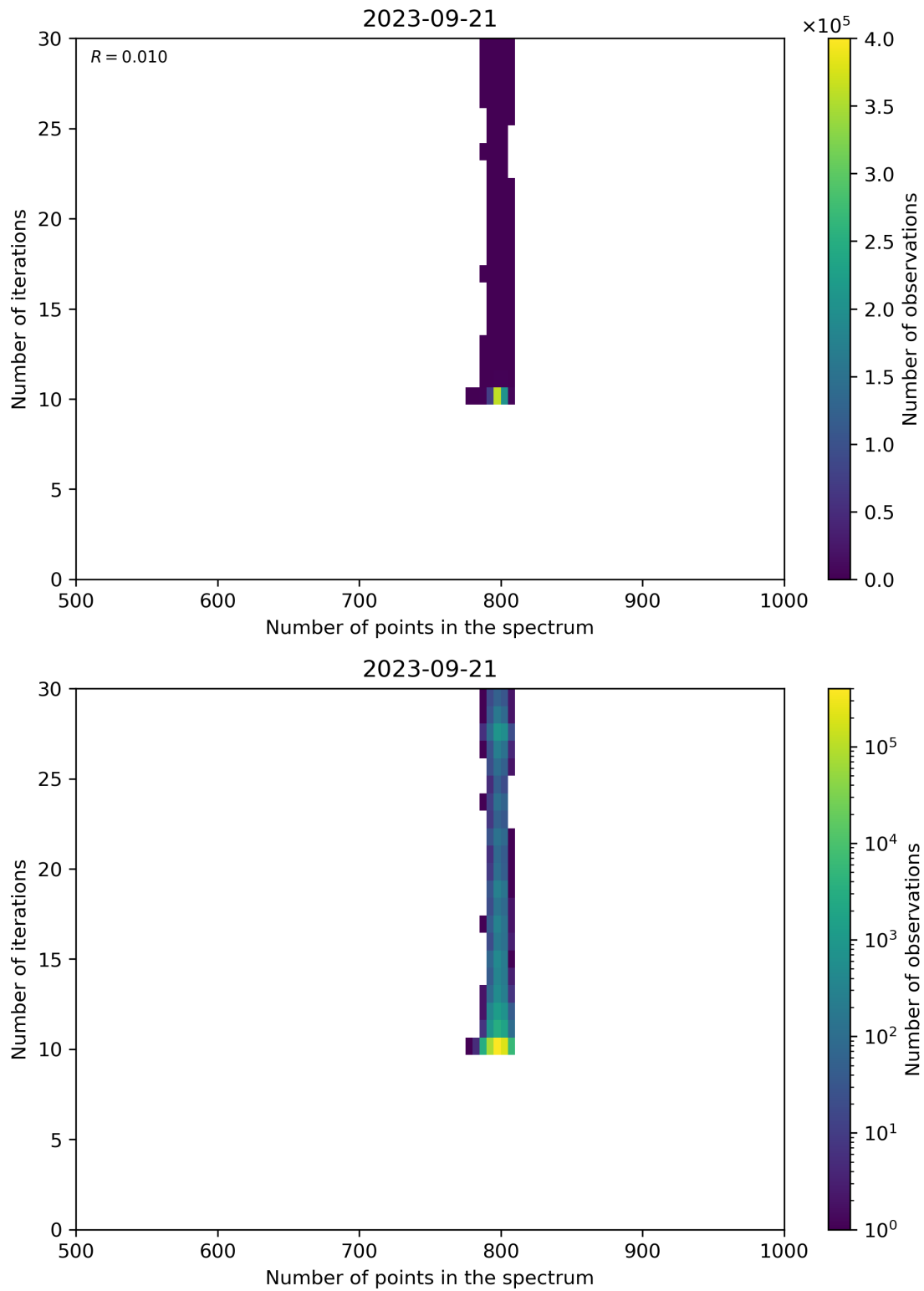
Figure 92: Scatter density plot of “Number of points in the spectrum” against “Number of iterations” for 2023-09-20 to 2023-09-22.
