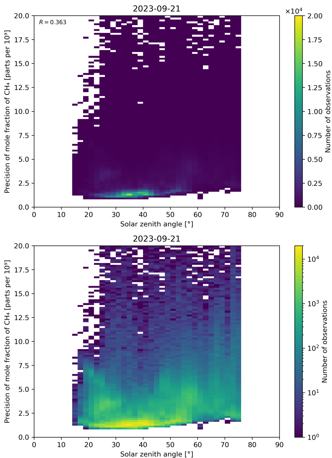
Figure 101: Scatter density plot of “Solar zenith angle” against “Precision of mole fraction of \text{CH}_4 ” for 2023-09-20 to 2023-09-22.
