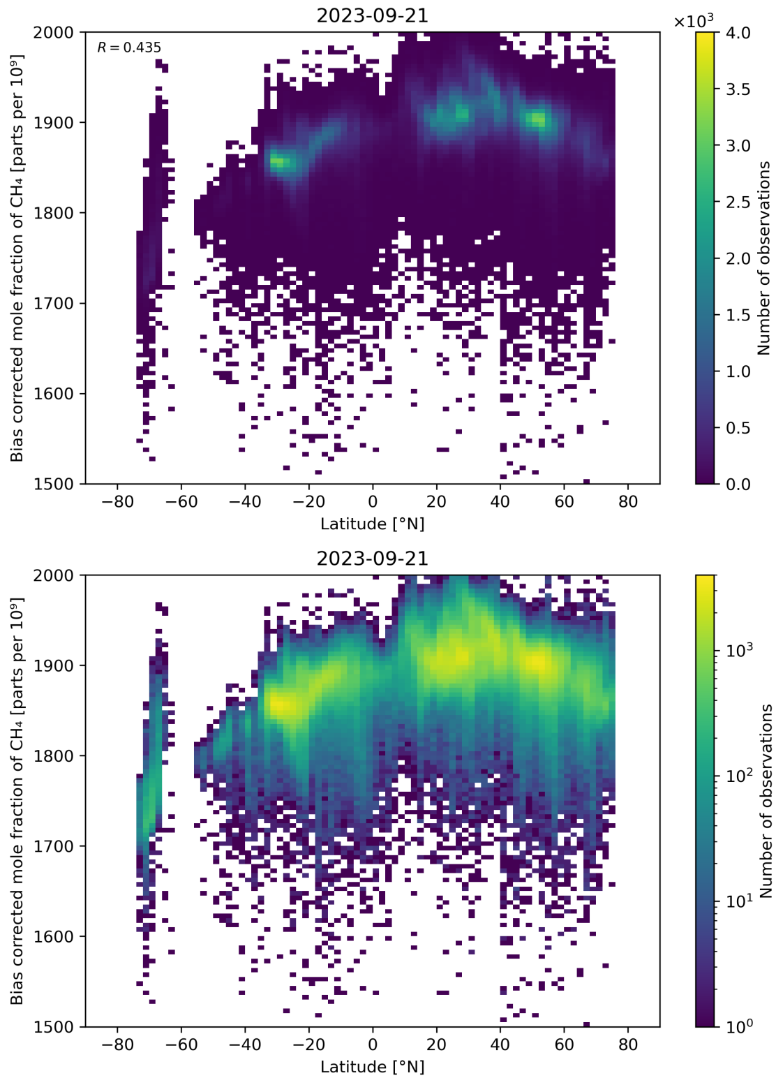
Figure 58: Scatter density plot of “Latitude” against “Bias corrected mole fraction of CH 4 ” for 2023-09-20 to 2023-09-22.
