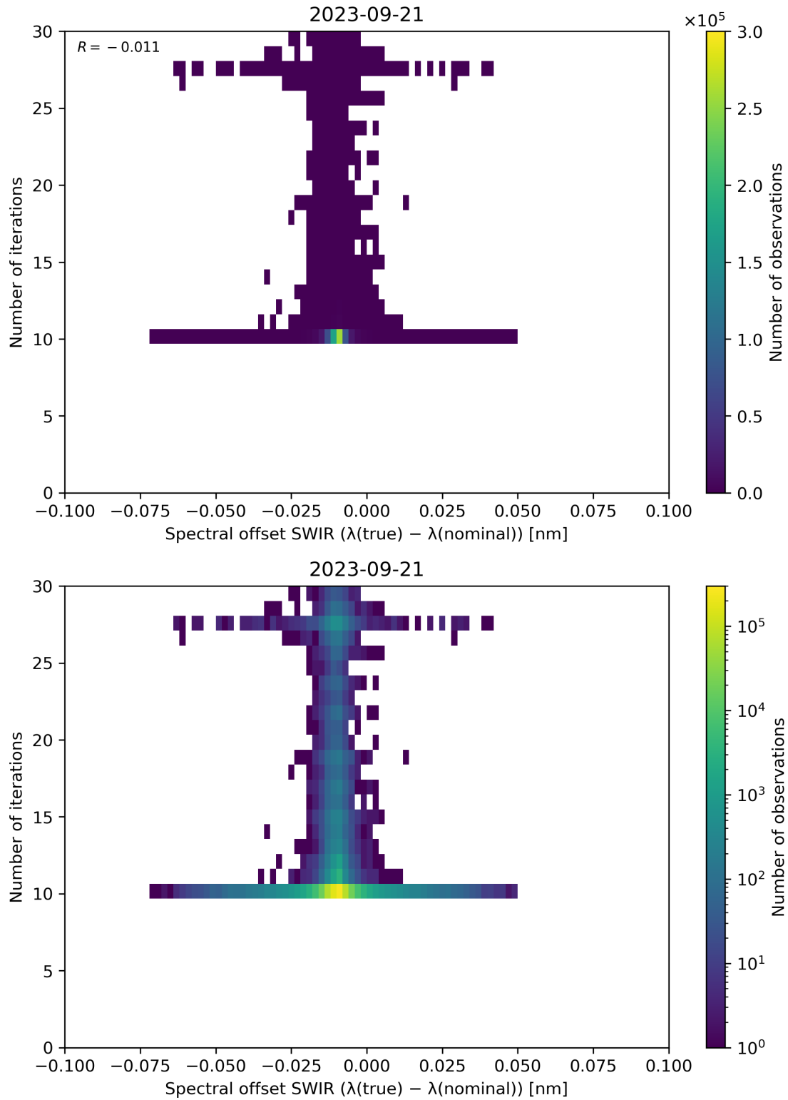
Figure 121: Scatter density plot of “Spectral offset SWIR ( \lambda(\text{true}) - \lambda(\text{nominal}) )” against “Number of iterations” for 2023-09-20 to 2023-09-22.
