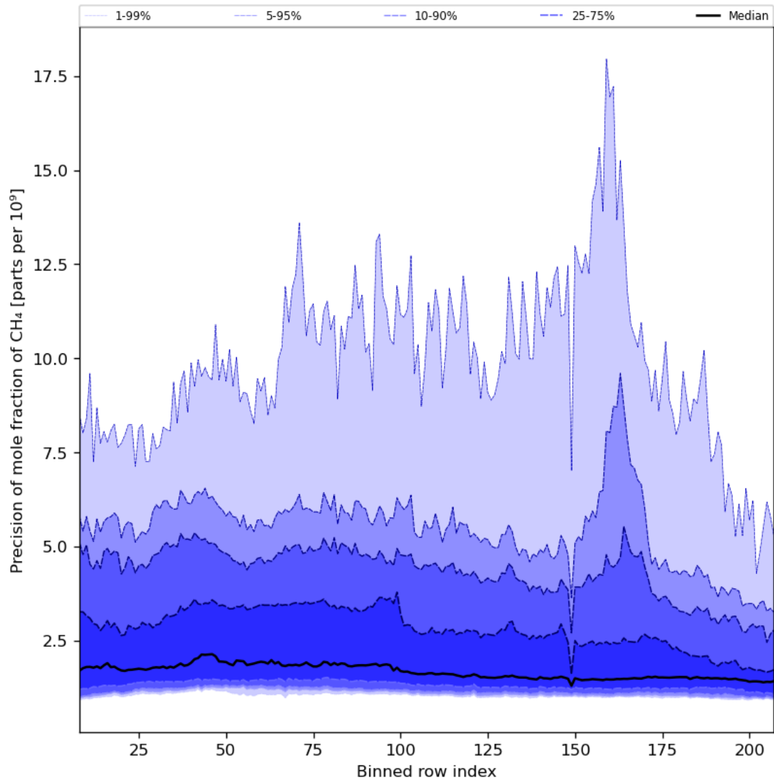
Figure 35: Along track statistics of “Precision of mole fraction of CH 4 ” for 2023-09-20 to 2023-09-22
