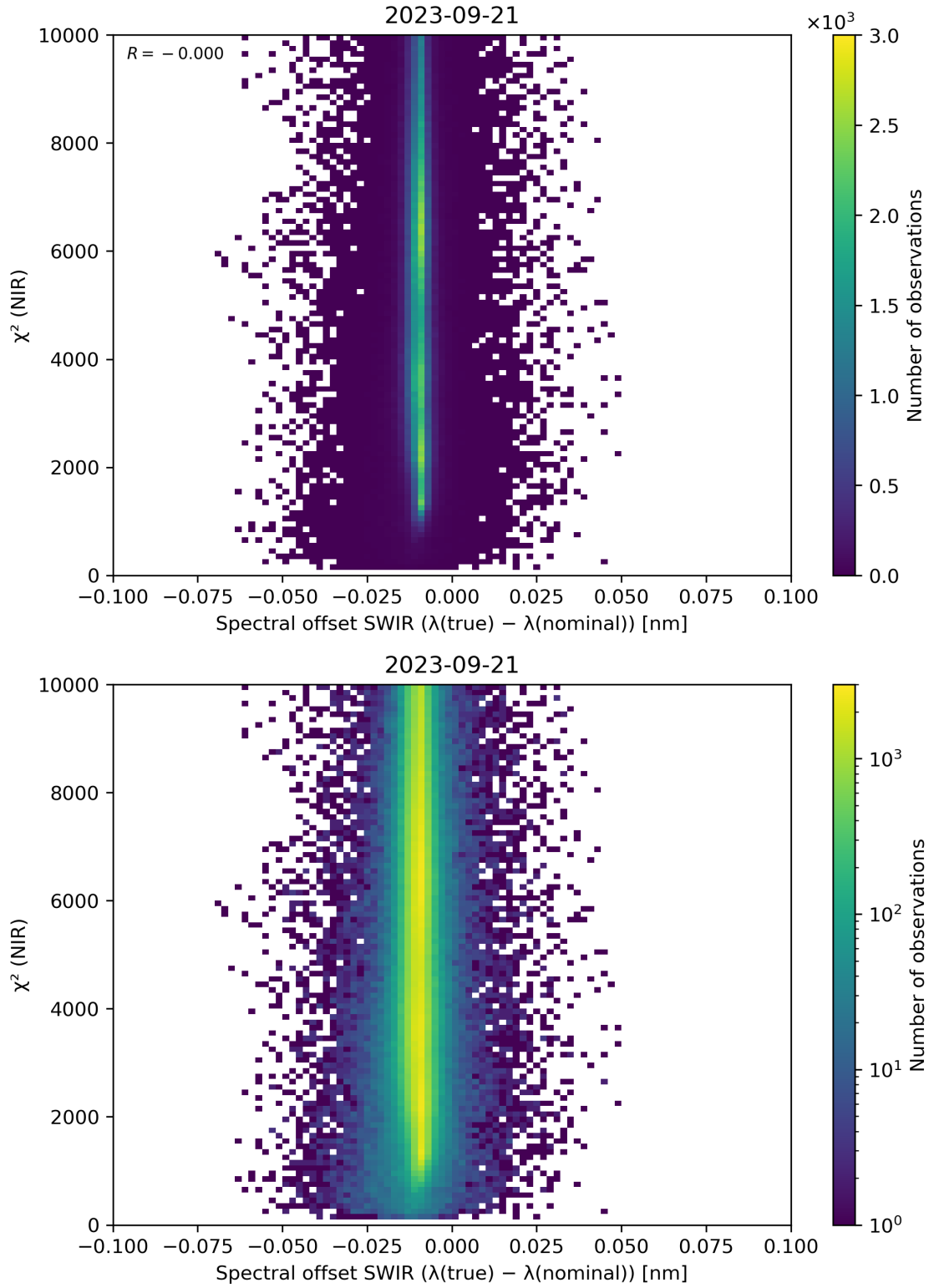
Figure 117: Scatter density plot of “Spectral offset SWIR ( \lambda(\text{true}) - \lambda(\text{nominal}) )” against “ \chi^2 (NIR)” for 2023-09-20 to 2023-09-22.
