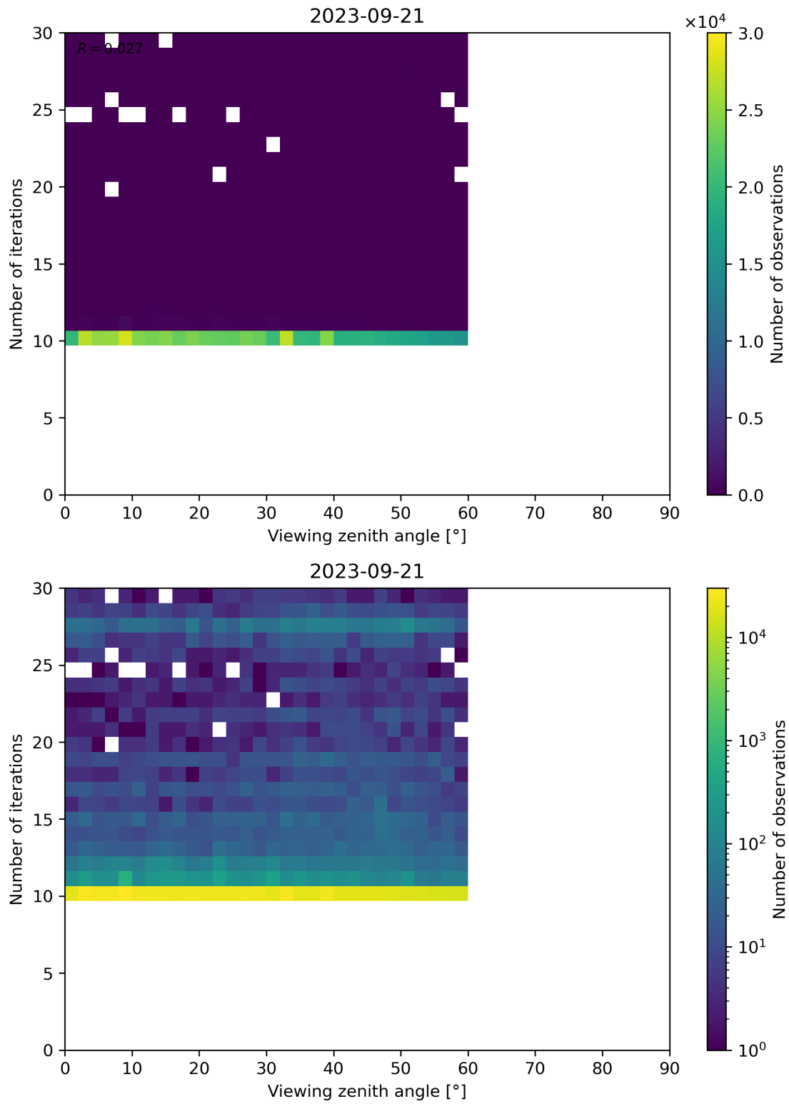
Figure 113: Scatter density plot of “Viewing zenith angle” against “Number of iterations” for 2023-09-20 to 2023-09-22.
