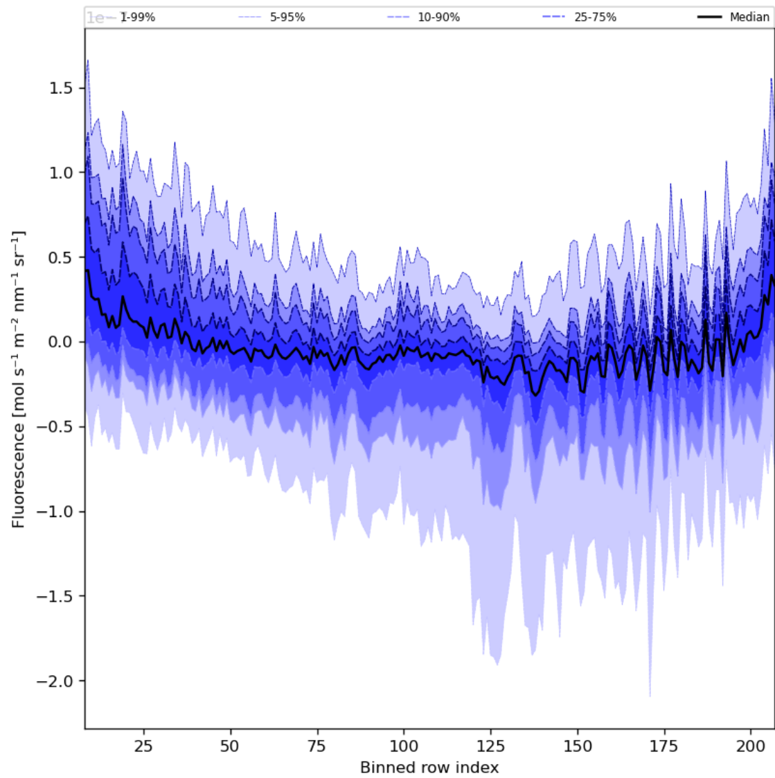
Figure 43: Along track statistics of “Fluorescence” for 2023-09-20 to 2023-09-22
