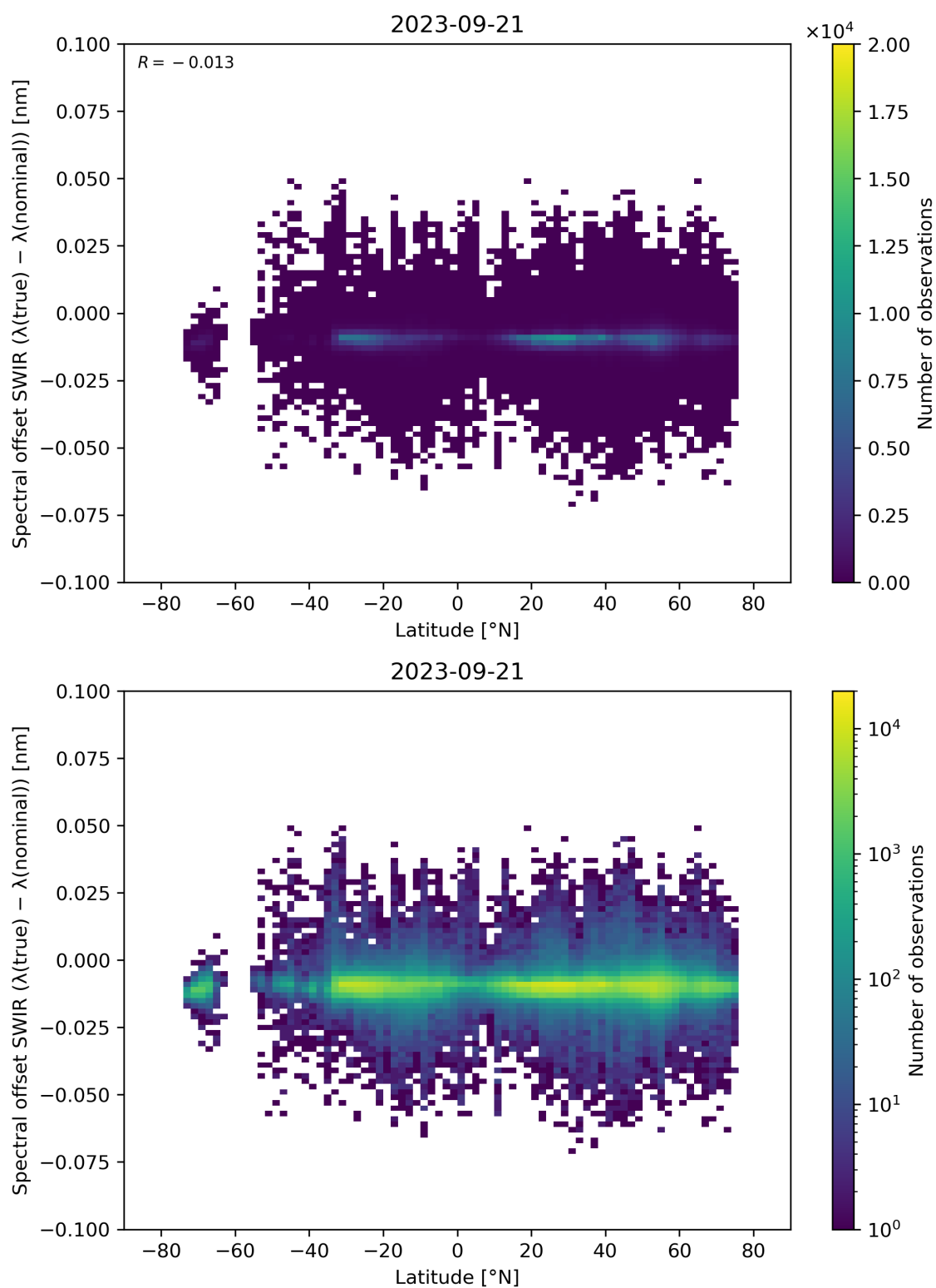
Figure 62: Scatter density plot of “Latitude” against “Spectral offset SWIR ( \lambda(\text{true}) - \lambda(\text{nominal}) )” for 2023-09-20 to 2023-09-22.
