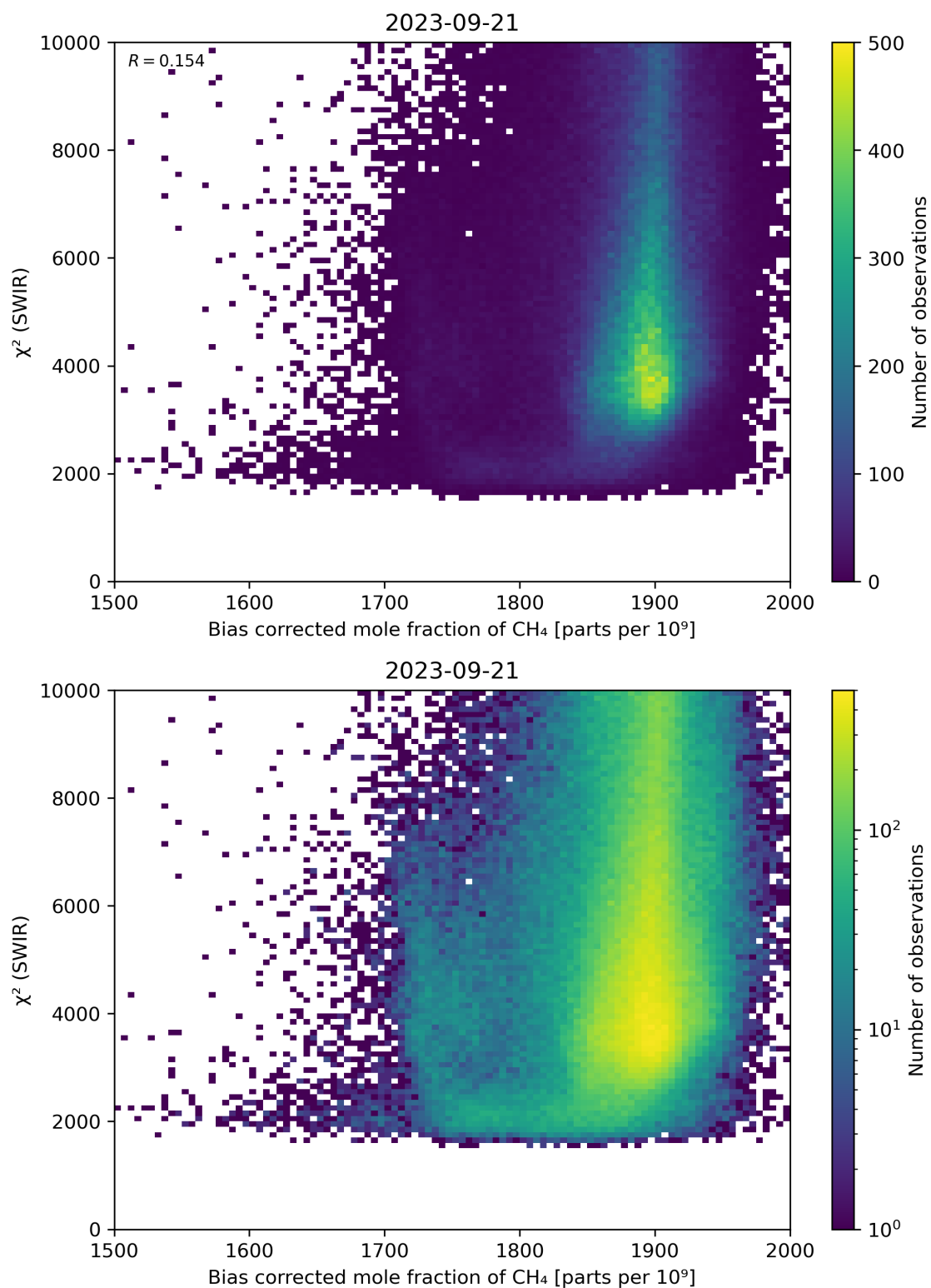
Figure 64: Scatter density plot of “Bias corrected mole fraction of CH 4 ” against “ \chi^2 (SWIR)” for 2023-09-20 to 2023-09-22.
