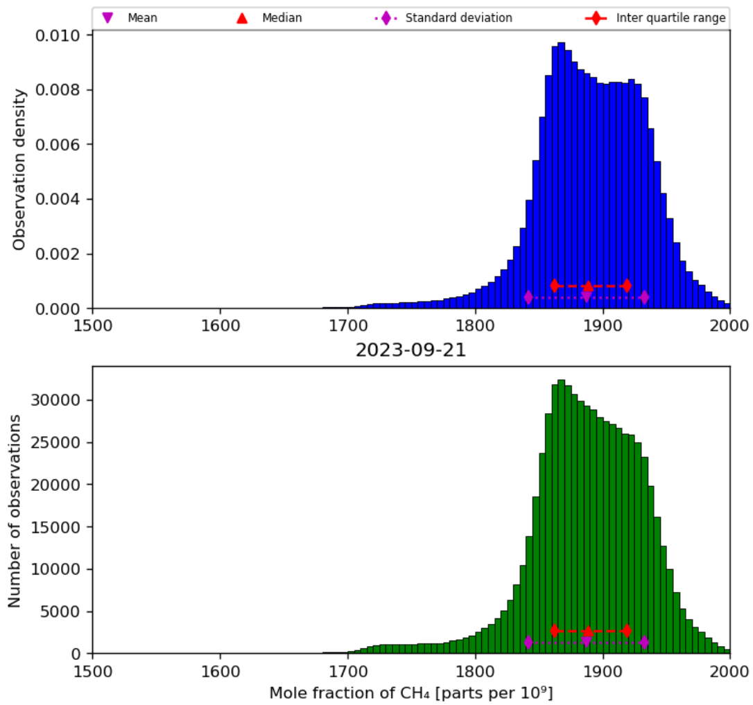
Figure 23: Histogram of “Mole fraction of CH 4 ” for 2023-09-20 to 2023-09-22
