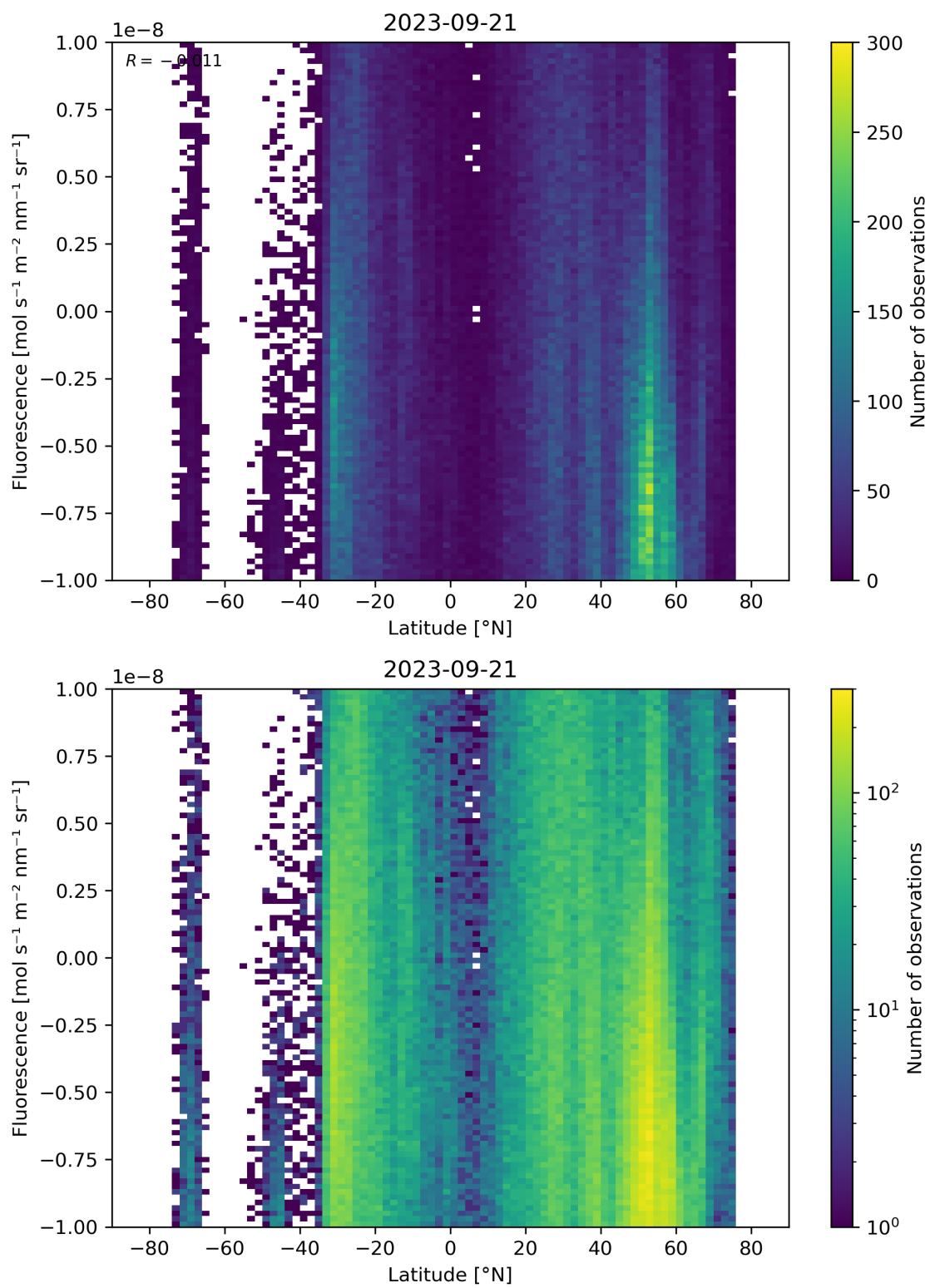
Figure 56: Scatter density plot of “Latitude” against “Fluorescence” for 2023-09-20 to 2023-09-22.
