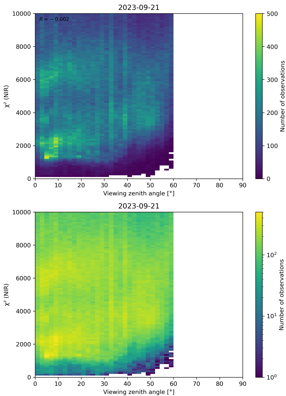
Figure 105: Scatter density plot of “Viewing zenith angle” against “ \chi^2 (NIR)” for 2023-09-20 to 2023-09-22.
