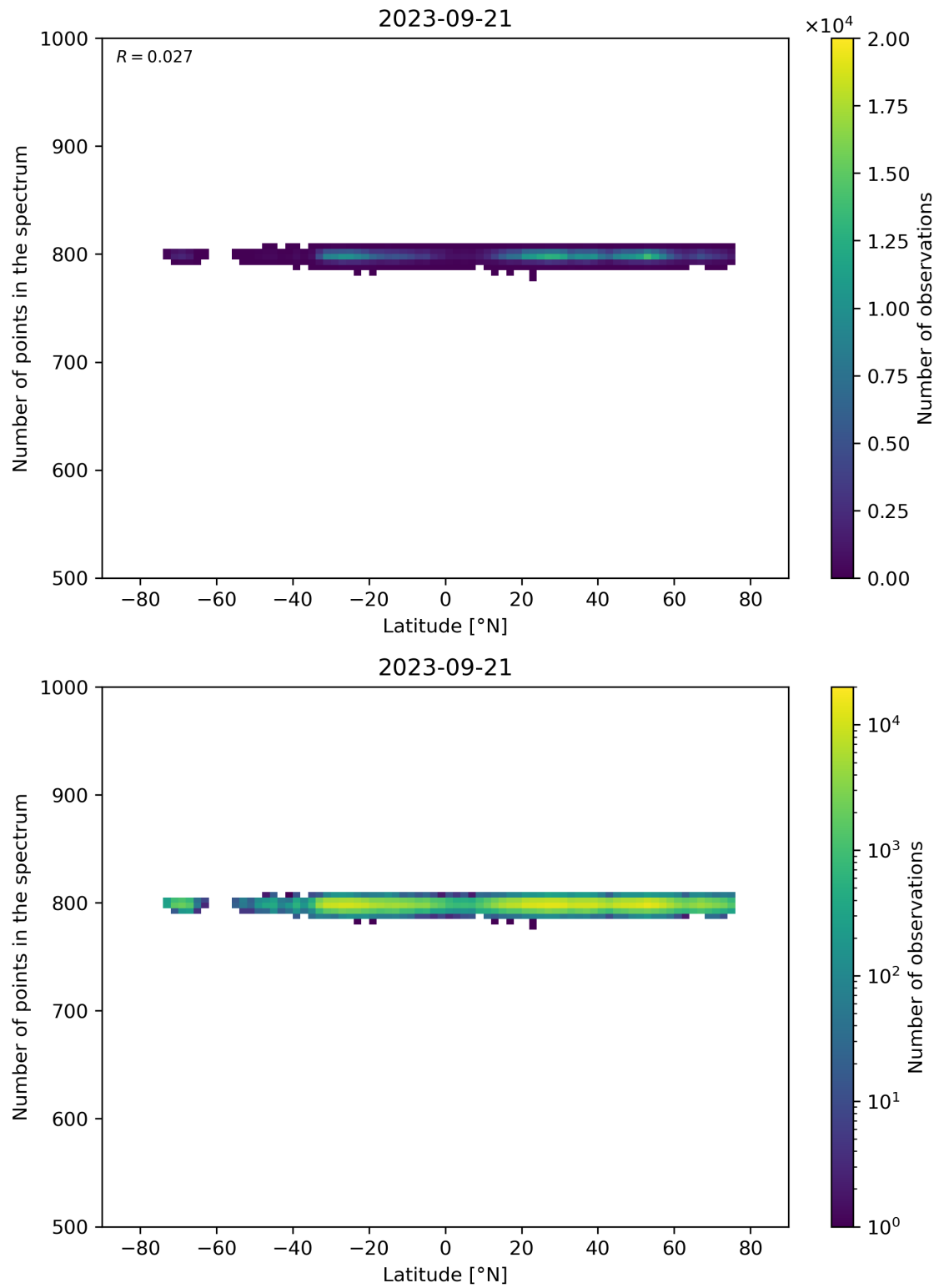
Figure 61: Scatter density plot of “Latitude” against “Number of points in the spectrum” for 2023-09-20 to 2023-09-22.
