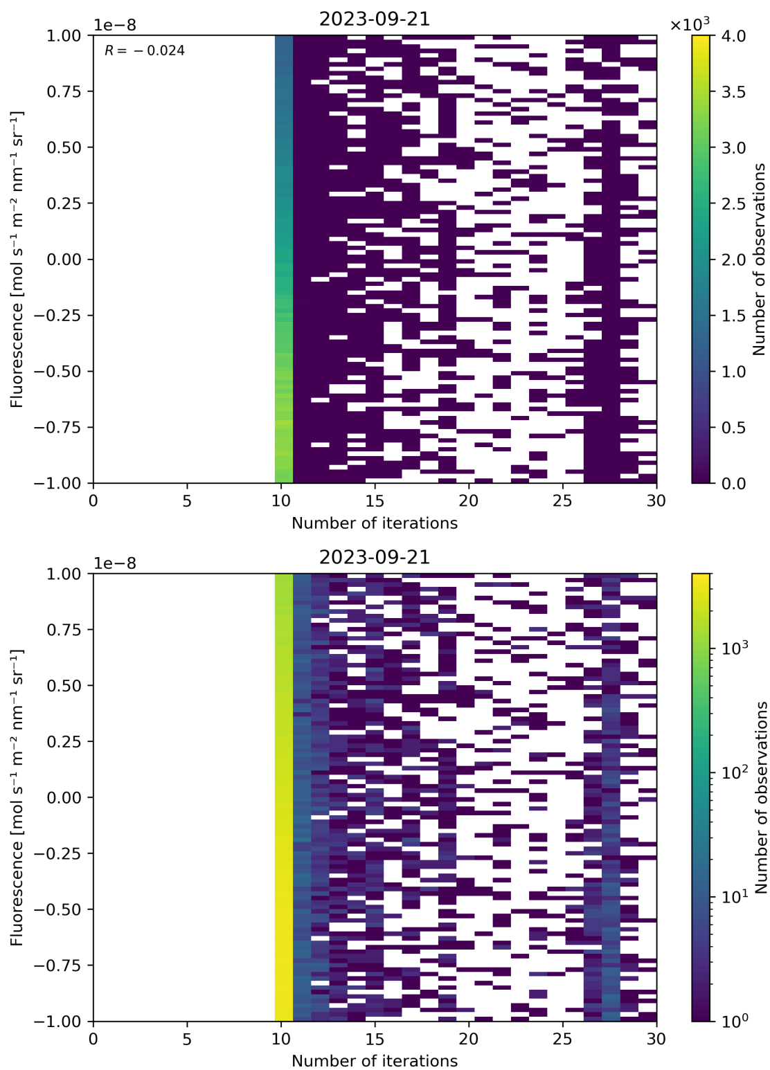
Figure 87: Scatter density plot of “Number of iterations” against “Fluorescence” for 2023-09-20 to 2023-09-22.
