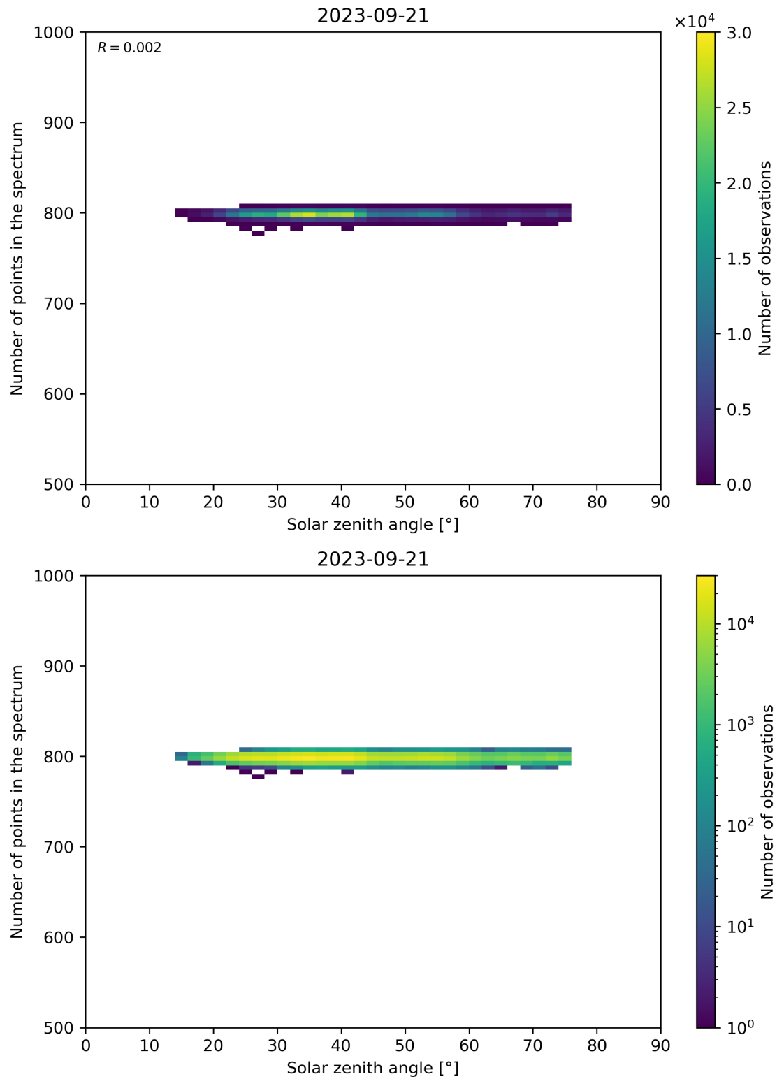
Figure 103: Scatter density plot of “Solar zenith angle” against “Number of points in the spectrum” for 2023-09-20 to 2023-09-22.
