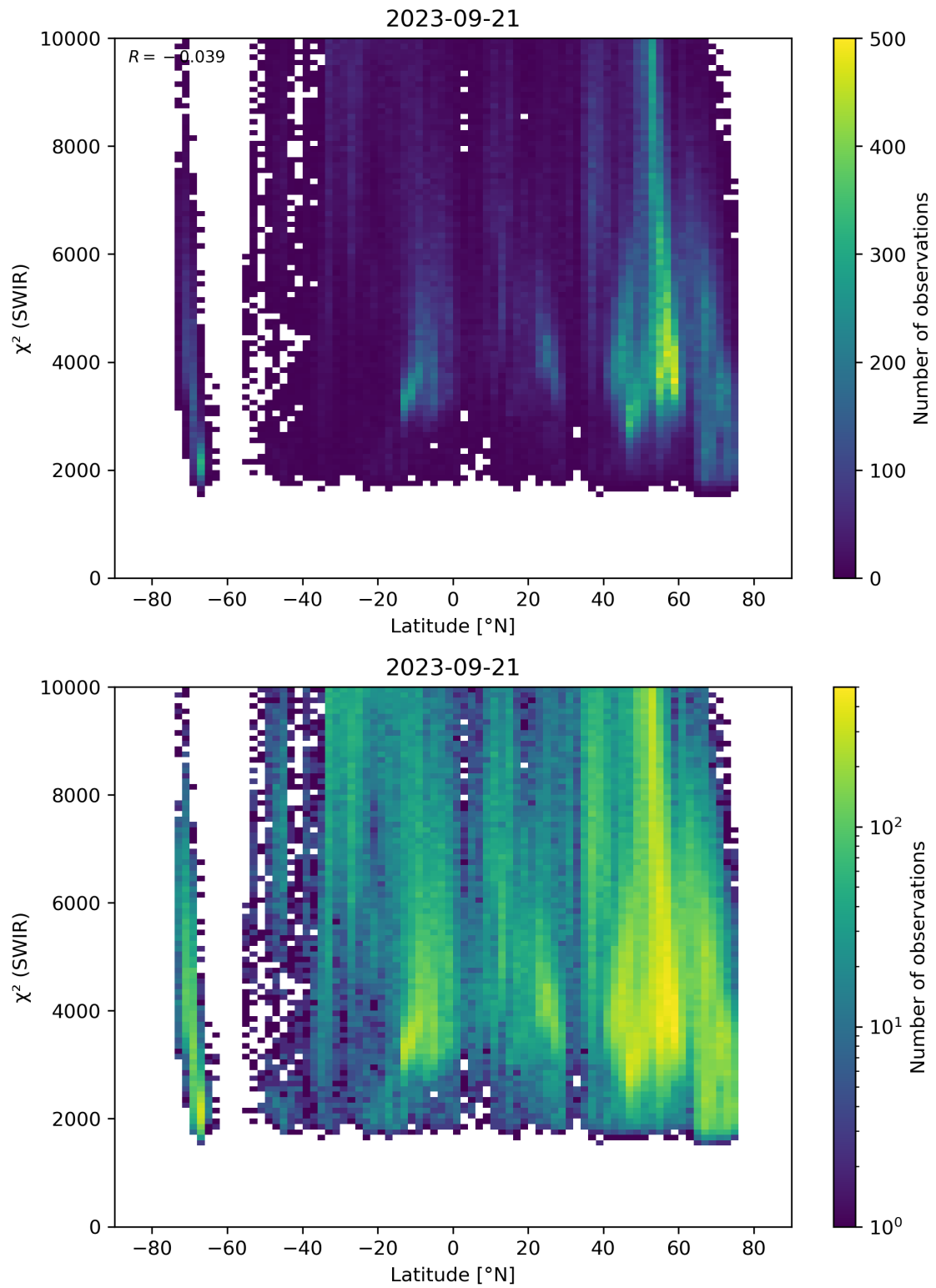
Figure 54: Scatter density plot of “Latitude” against “ \chi^2 (SWIR)” for 2023-09-20 to 2023-09-22.
