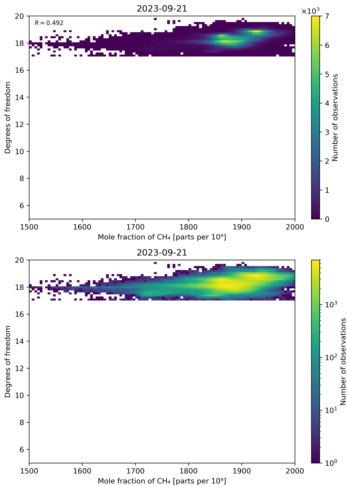
Figure 72: Scatter density plot of “Mole fraction of CH 4 ” against “Degrees of freedom” for 2023-09-20 to 2023-09-22.
