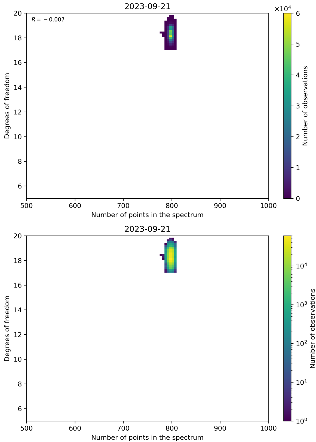
Figure 90: Scatter density plot of “Number of points in the spectrum” against “Degrees of freedom” for 2023-09-20 to 2023-09-22.
