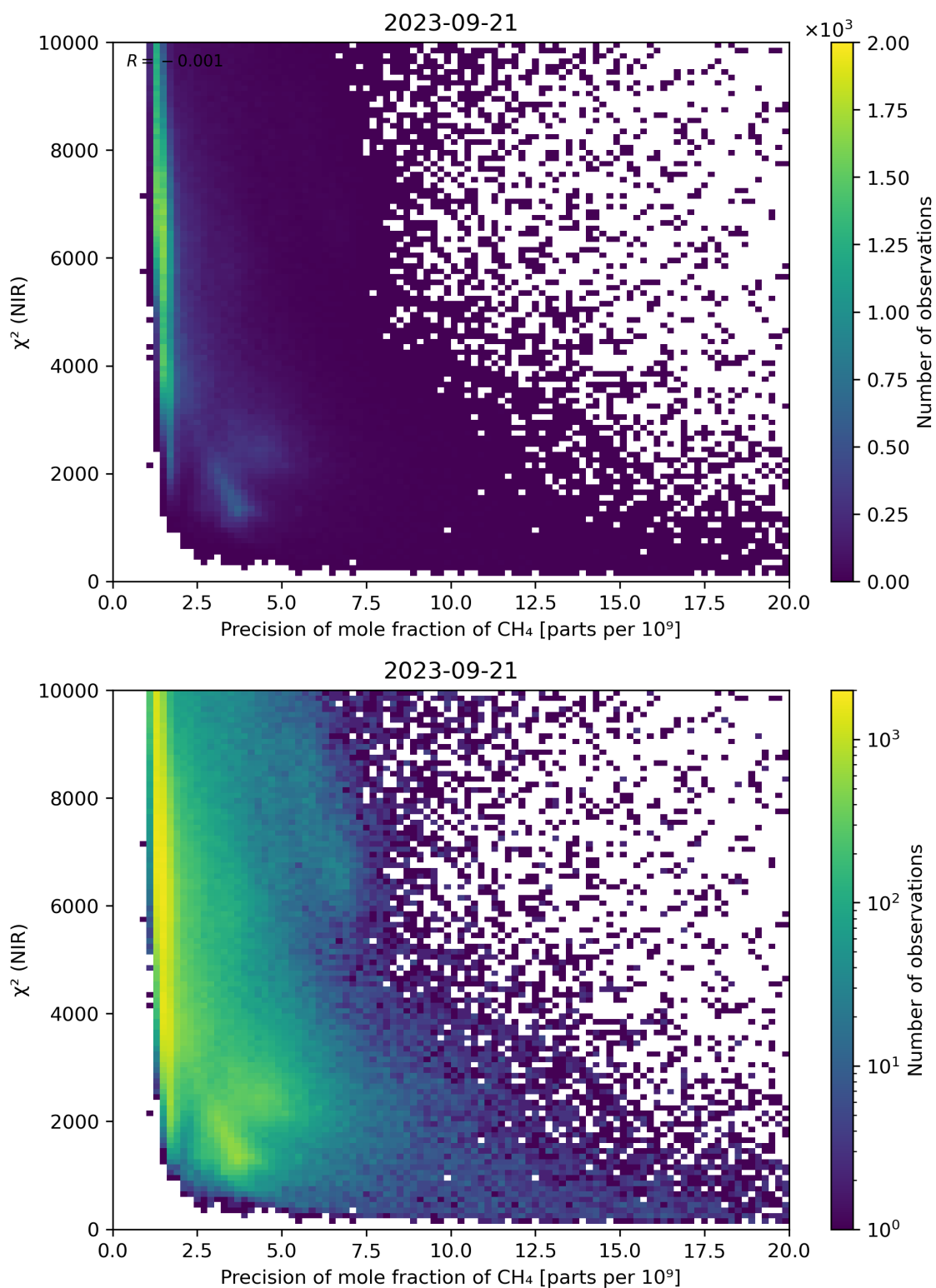
Figure 78: Scatter density plot of “Precision of mole fraction of CH 4 ” against “ \chi^2 (NIR)” for 2023-09-20 to 2023-09-22.
