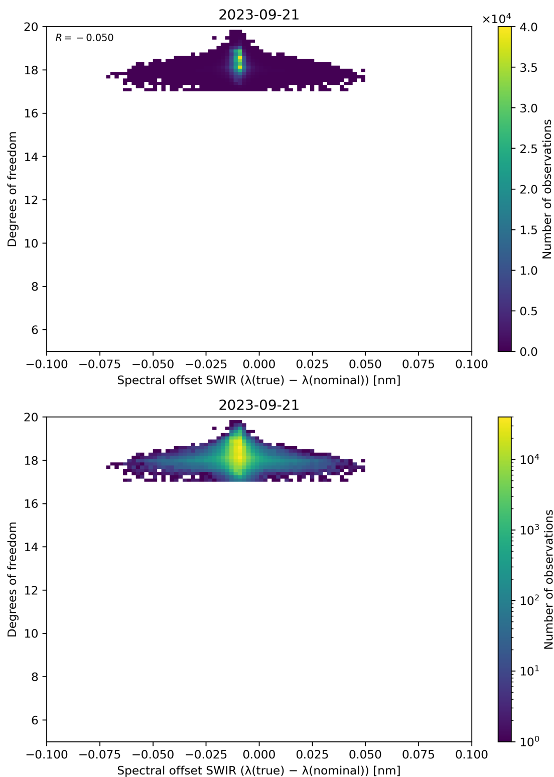
Figure 119: Scatter density plot of “Spectral offset SWIR ( \lambda(\text{true}) - \lambda(\text{nominal}) )” against “Degrees of freedom” for 2023-09-20 to 2023-09-22.
