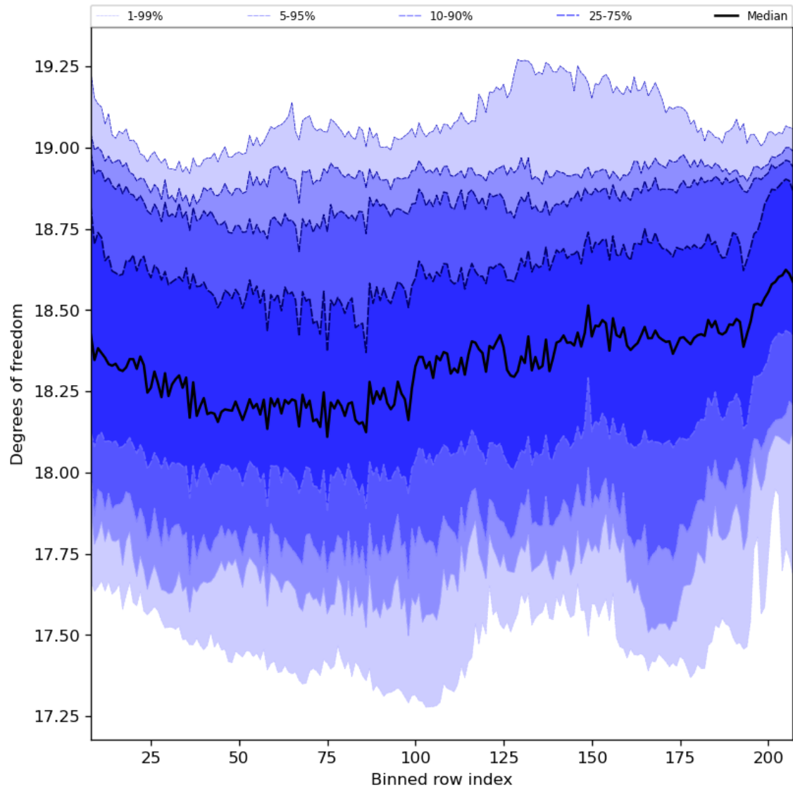
Figure 41: Along track statistics of “Degrees of freedom” for 2023-09-20 to 2023-09-22
