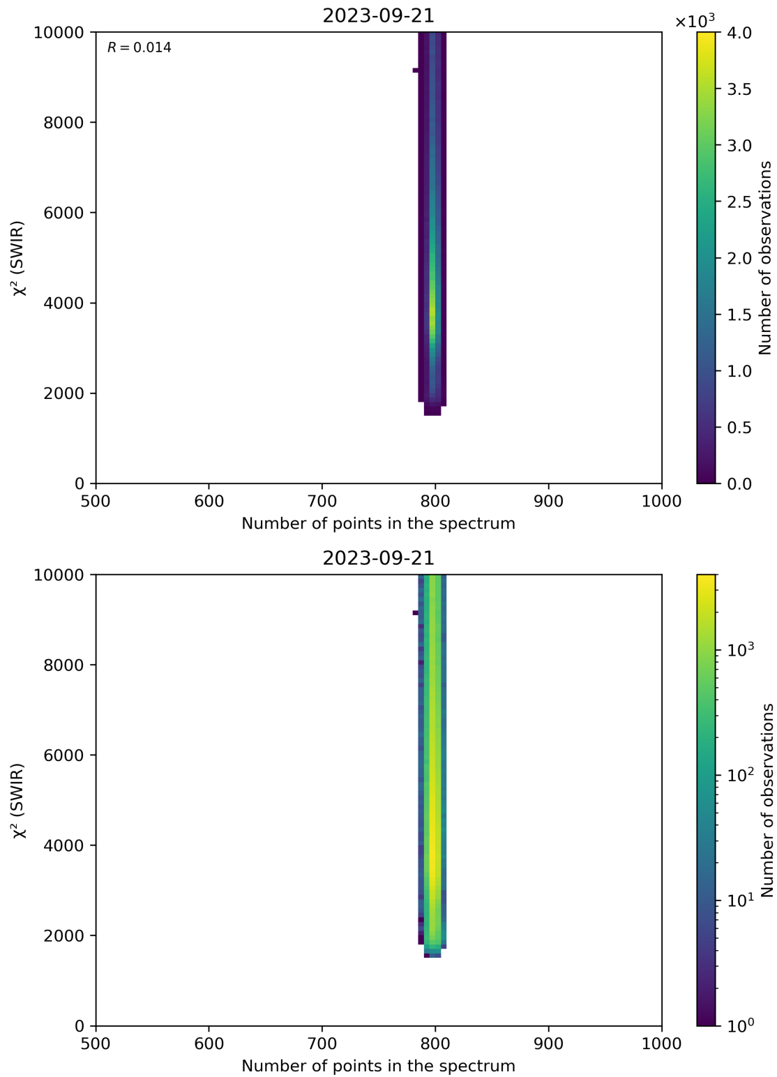
Figure 89: Scatter density plot of “Number of points in the spectrum” against “ \chi^2 (SWIR)” for 2023-09-20 to 2023-09-22.
