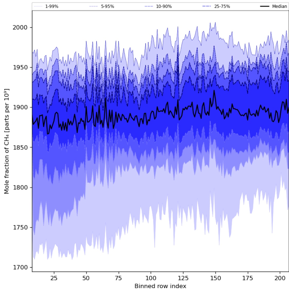
Figure 34: Along track statistics of “Mole fraction of CH 4 ” for 2023-09-20 to 2023-09-22
