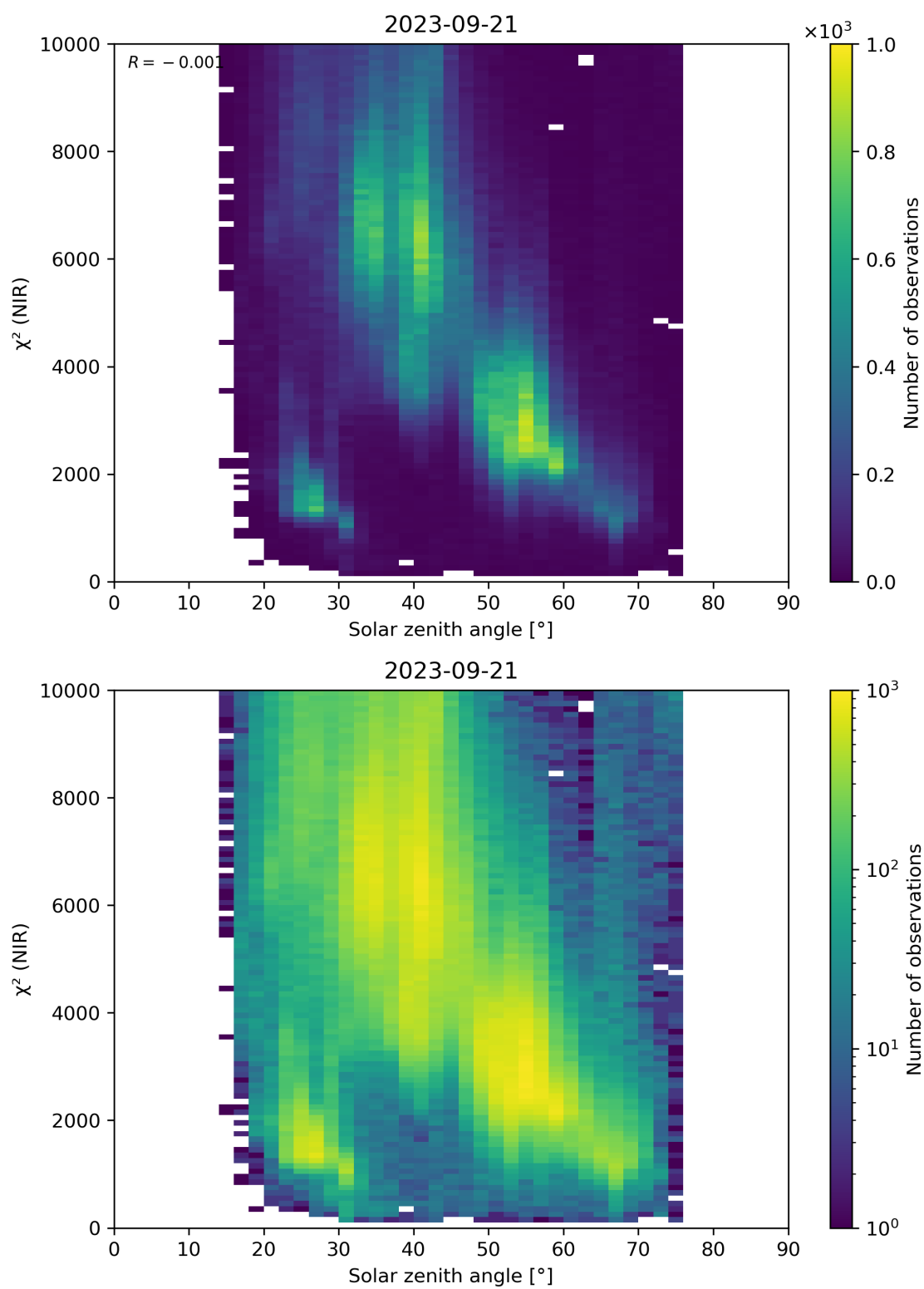
Figure 94: Scatter density plot of “Solar zenith angle” against “ \chi^2 (NIR)” for 2023-09-20 to 2023-09-22.
