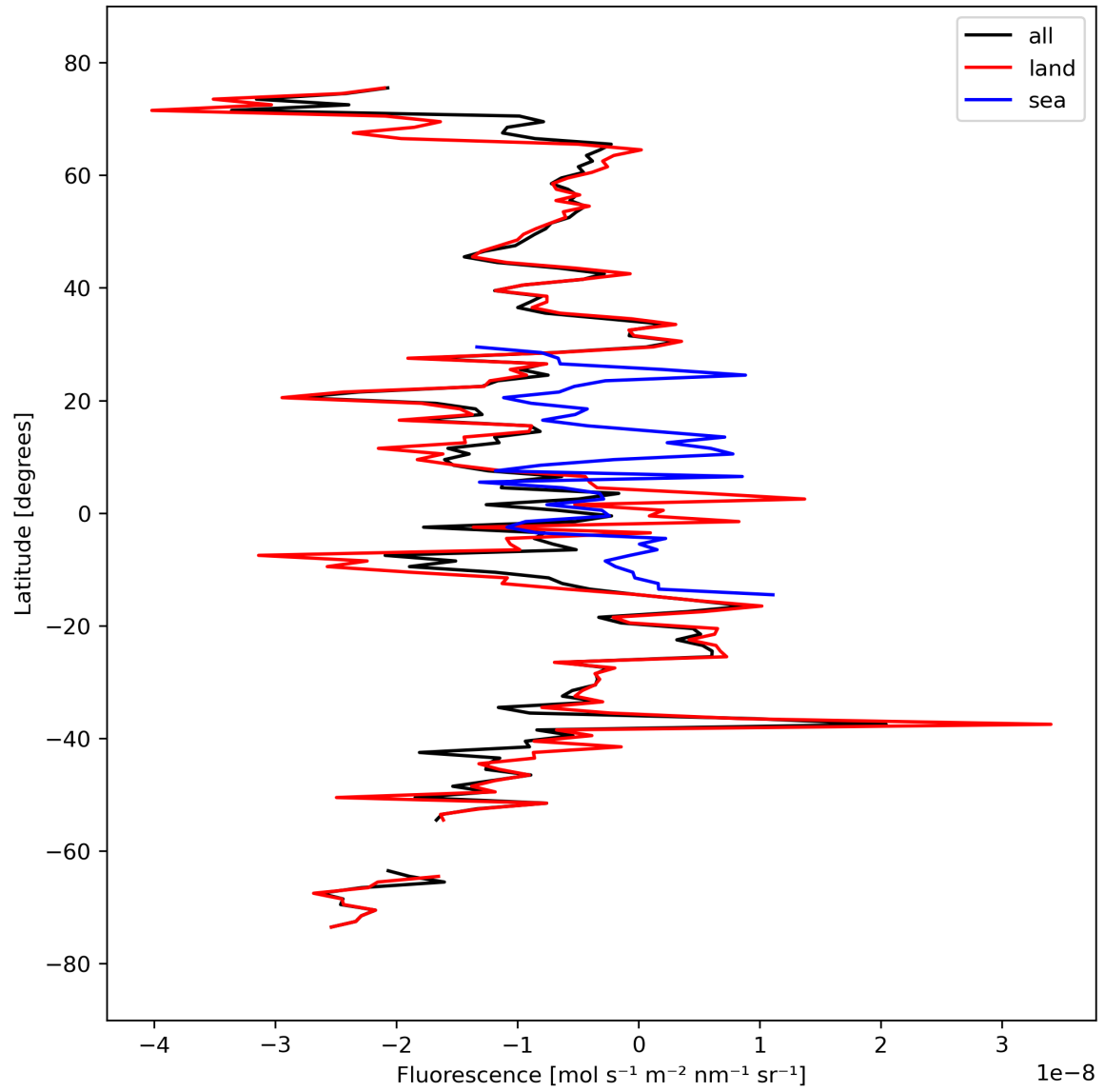
Figure 21: Zonal average of “Fluorescence” for 2023-09-20 to 2023-09-22.
