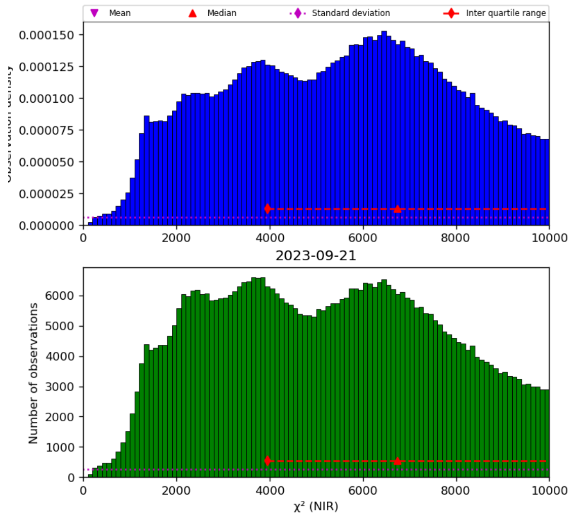
Figure 29: Histogram of " \chi^2 (NIR)" for 2023-09-20 to 2023-09-22
