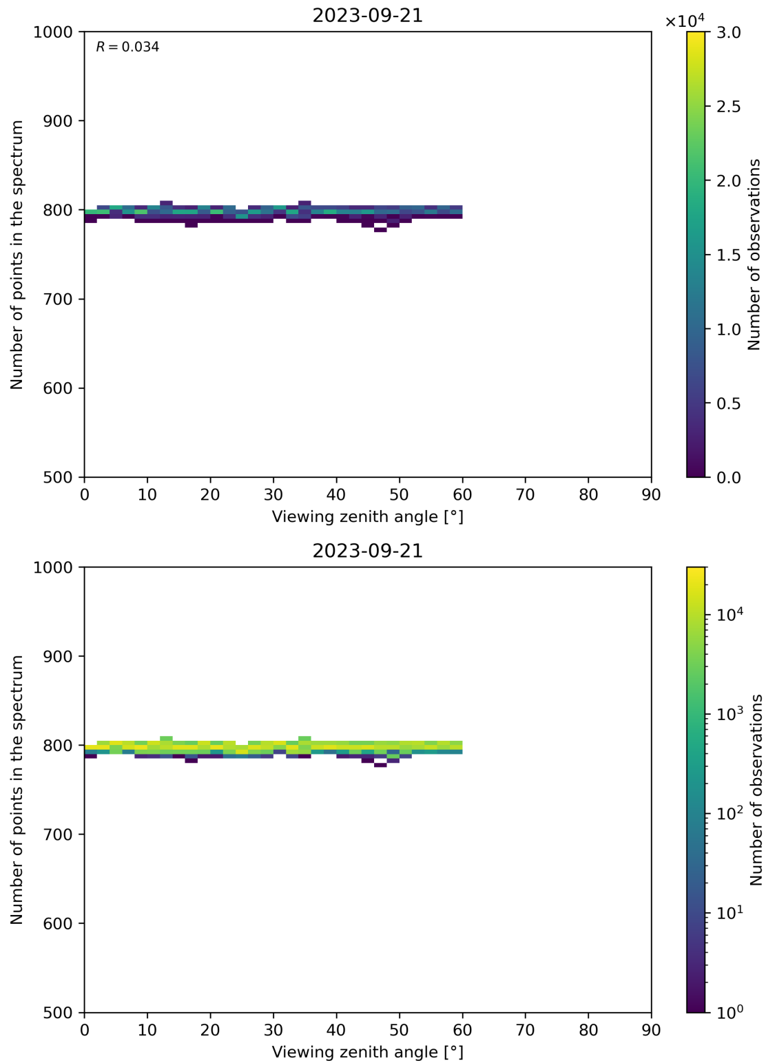
Figure 114: Scatter density plot of “Viewing zenith angle” against “Number of points in the spectrum” for 2023-09-20 to 2023-09-22.
