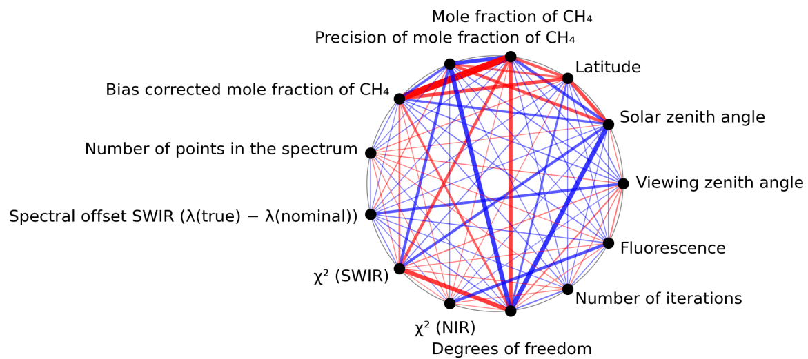
Figure 1: Map of correlation graph for 2023-09-20 to 2023-09-22.
