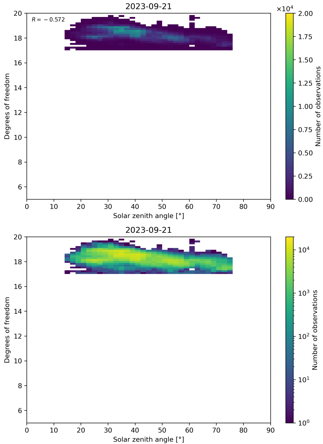
Figure 96: Scatter density plot of “Solar zenith angle” against “Degrees of freedom” for 2023-09-20 to 2023-09-22.
