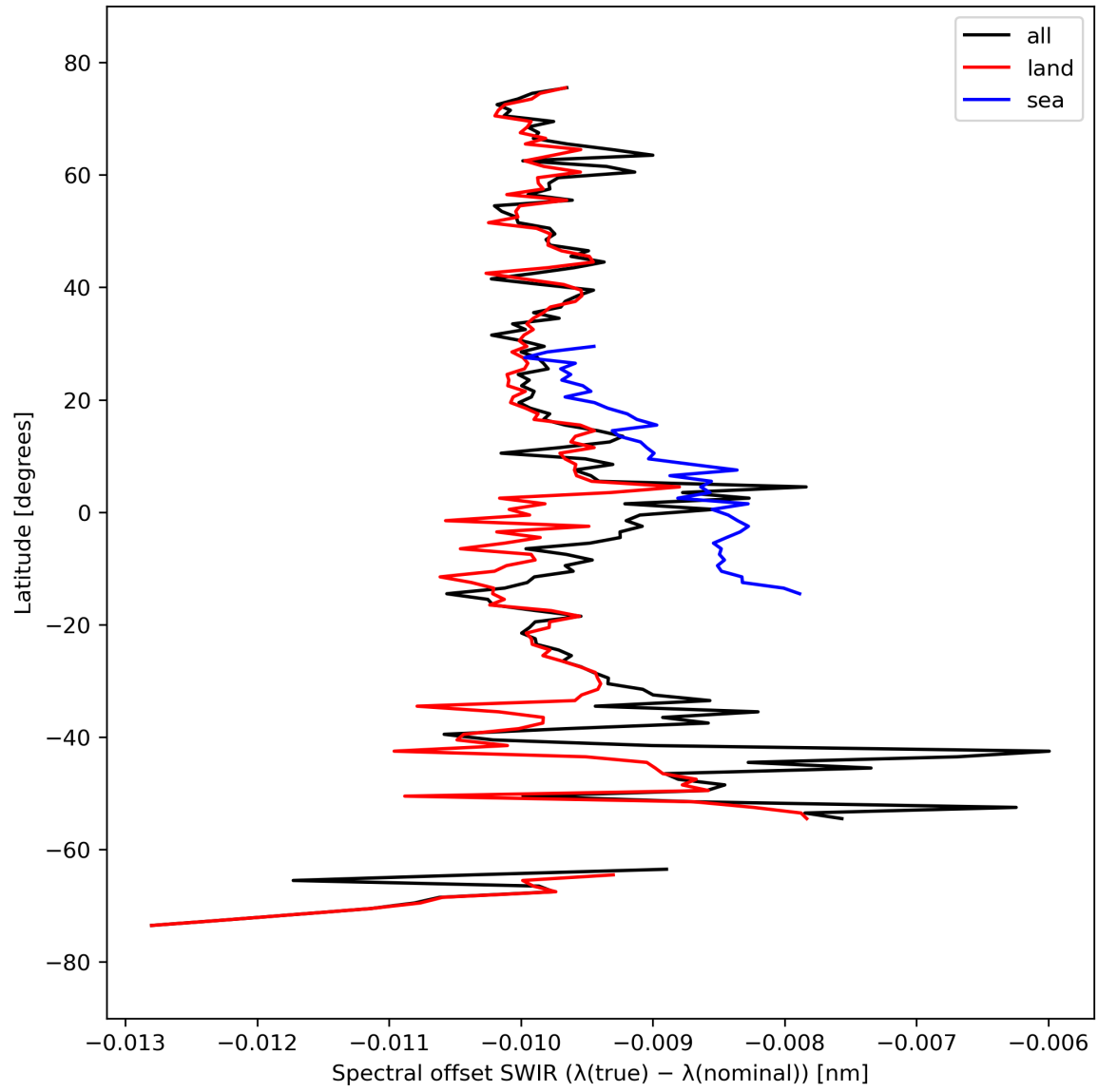
Figure 16: Zonal average of “Spectral offset SWIR ( \lambda(\text{true}) - \lambda(\text{nominal}) )” for 2023-09-20 to 2023-09-22.
