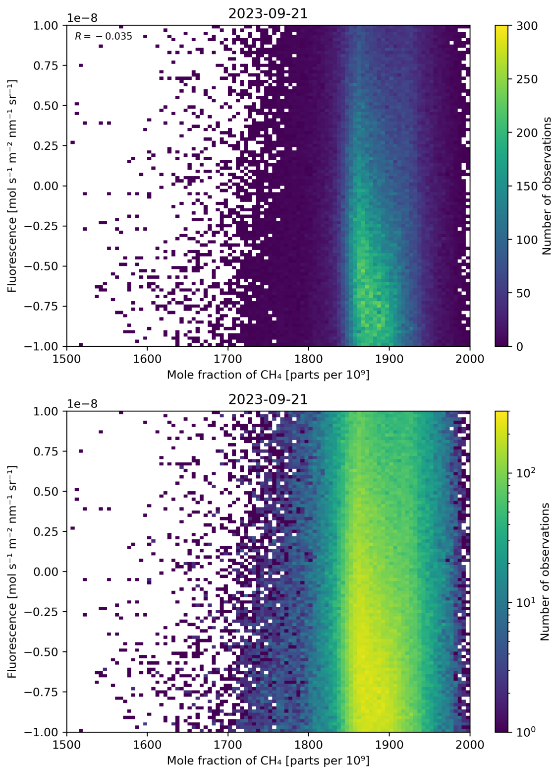
Figure 73: Scatter density plot of “Mole fraction of \text{CH}_4 ” against “Fluorescence” for 2023-09-20 to 2023-09-22.
