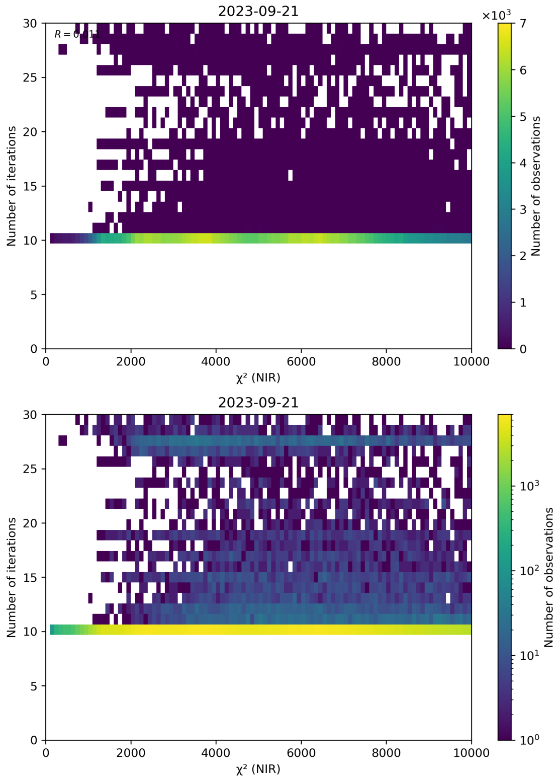
Figure 46: Scatter density plot of “ \chi^2 (NIR)” against “Number of iterations” for 2023-09-20 to 2023-09-22.
