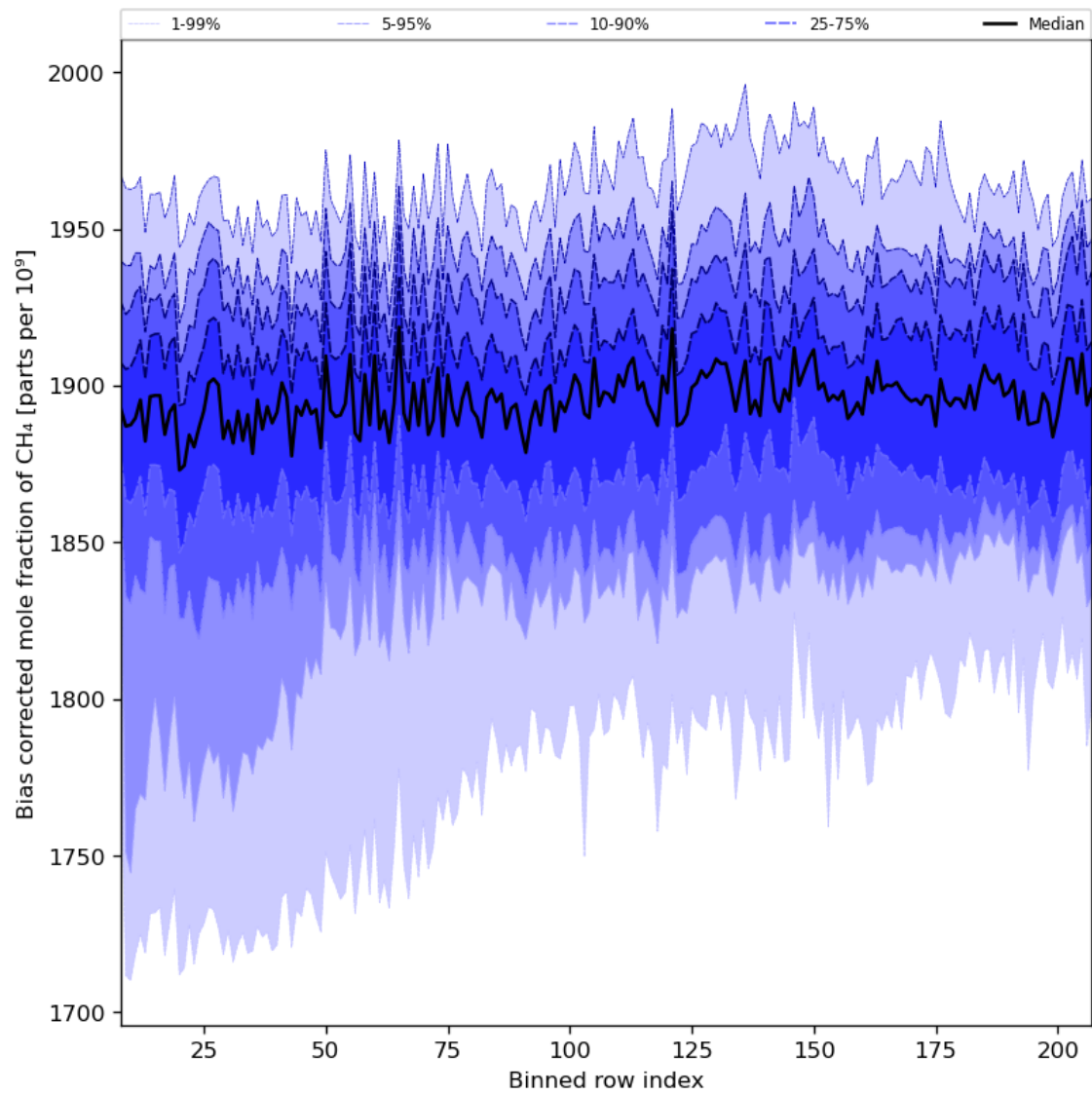
Figure 36: Along track statistics of “Bias corrected mole fraction of CH 4 ” for 2023-09-20 to 2023-09-22
