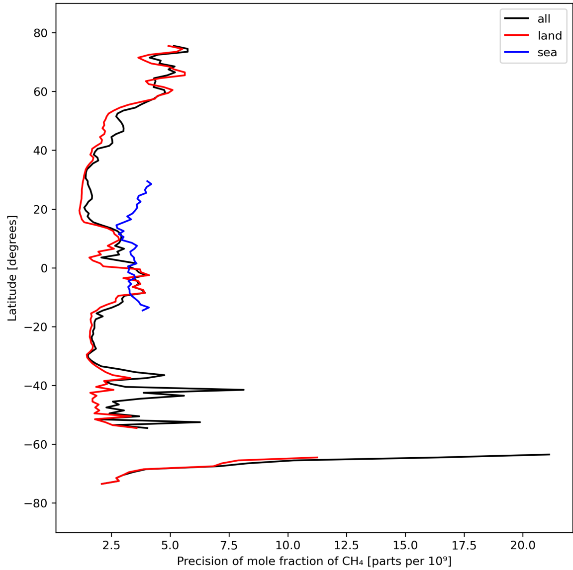
Figure 13: Zonal average of “Precision of mole fraction of CH 4 ” for 2023-09-20 to 2023-09-22.
