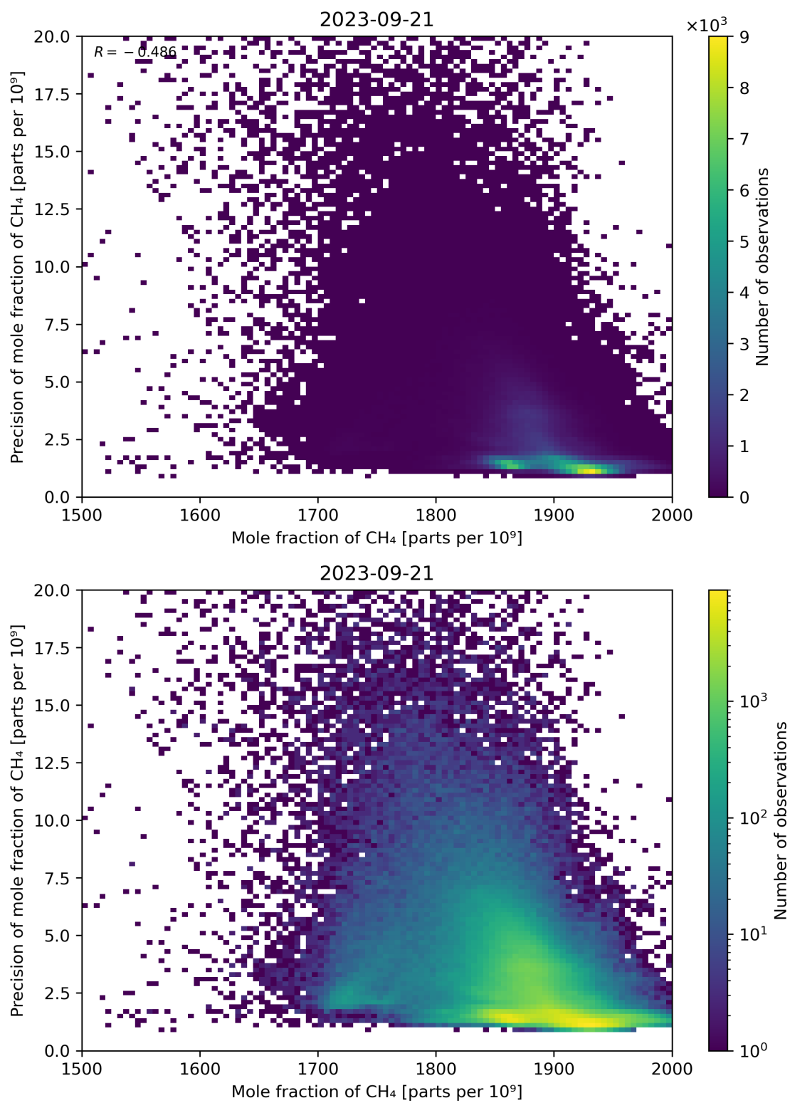
Figure 75: Scatter density plot of “Mole fraction of CH 4 ” against “Precision of mole fraction of CH 4 ” for 2023-09-20 to 2023-09-22.
