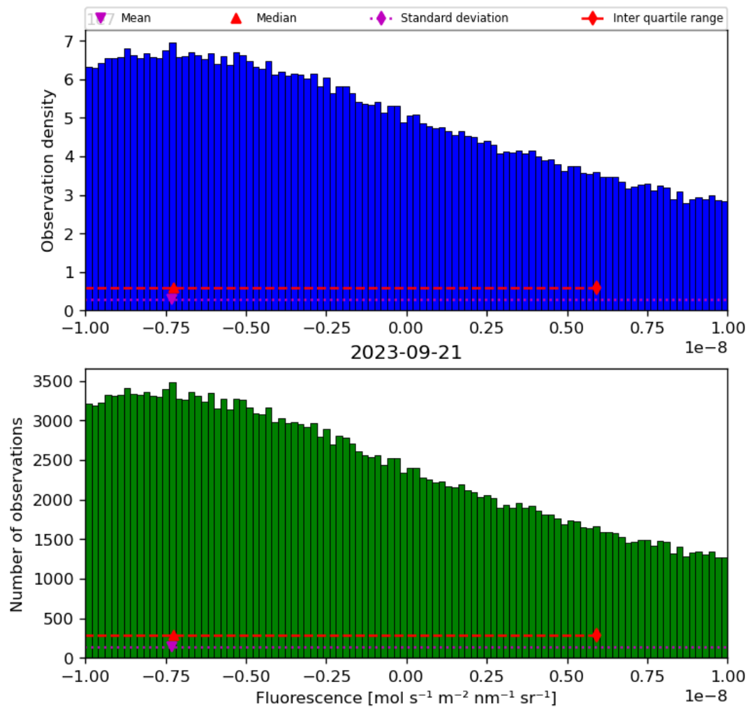
Figure 32: Histogram of “Fluorescence” for 2023-09-20 to 2023-09-22
