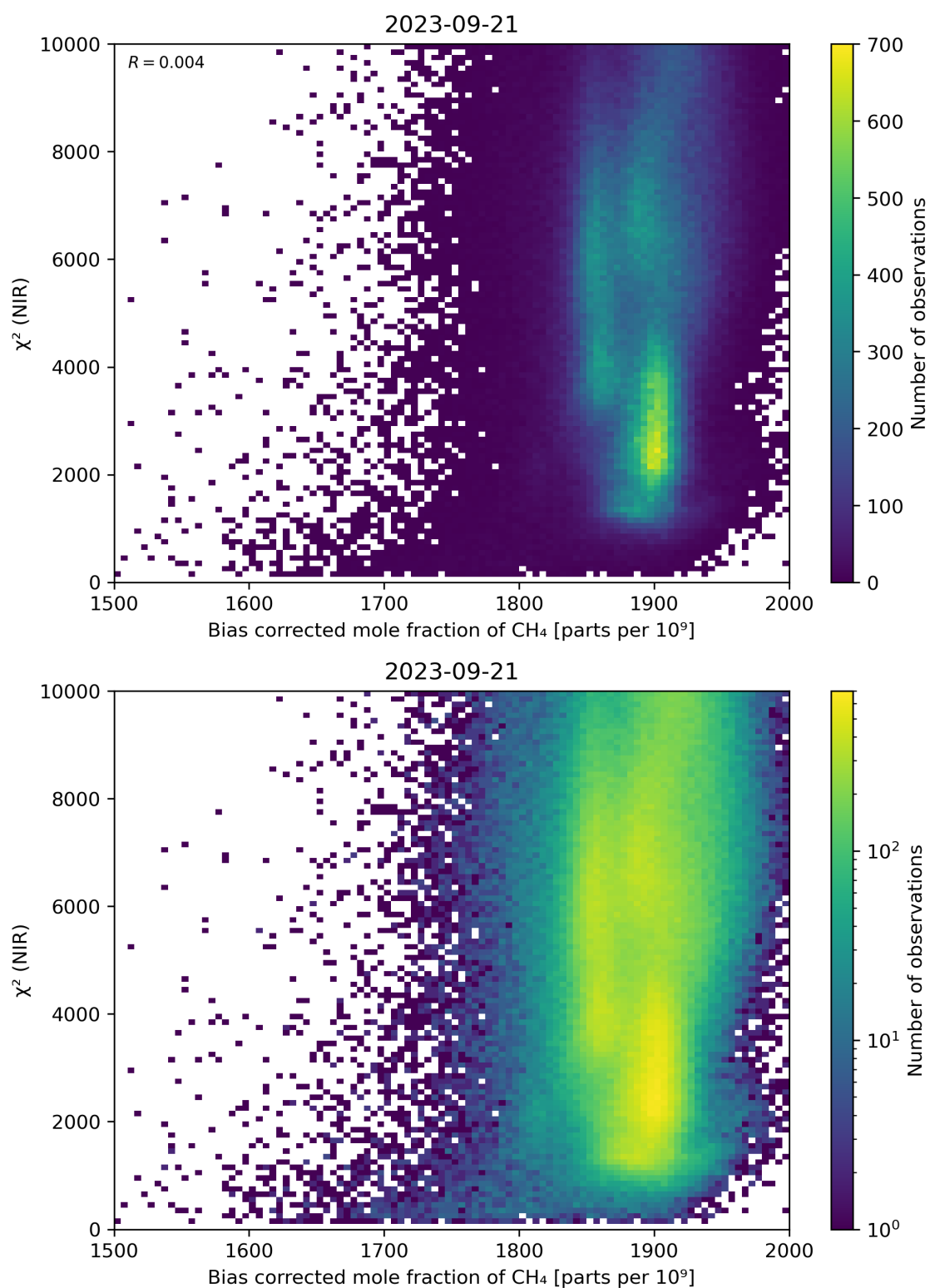
Figure 63: Scatter density plot of “Bias corrected mole fraction of \text{CH}_4 ” against “ \chi^2 (NIR)” for 2023-09-20 to 2023-09-22.
