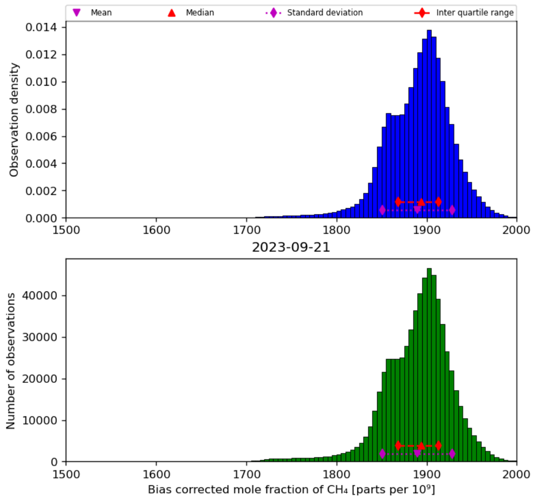
Figure 25: Histogram of “Bias corrected mole fraction of CH 4 ” for 2023-09-20 to 2023-09-22
