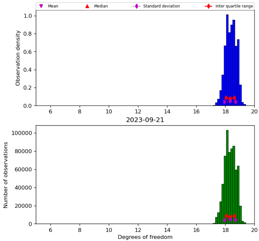
Figure 30: Histogram of “Degrees of freedom” for 2023-09-20 to 2023-09-22
