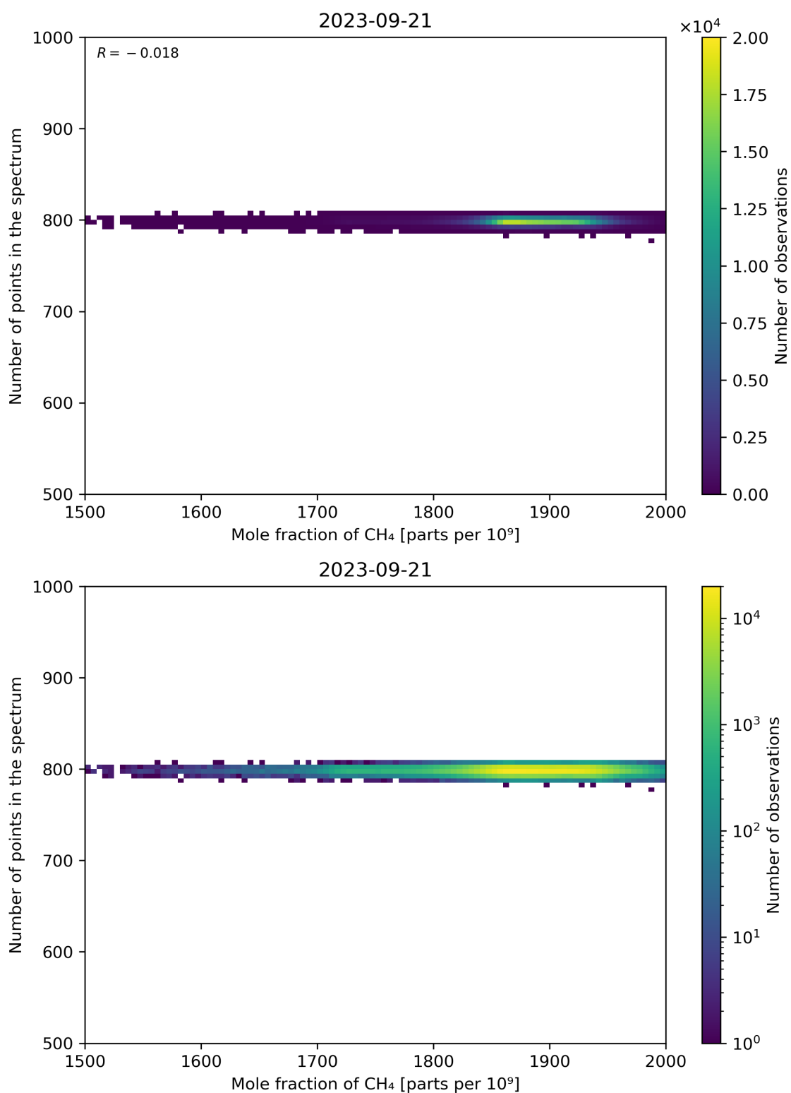
Figure 77: Scatter density plot of “Mole fraction of CH 4 ” against “Number of points in the spectrum” for 2023-09-20 to 2023-09-22.
