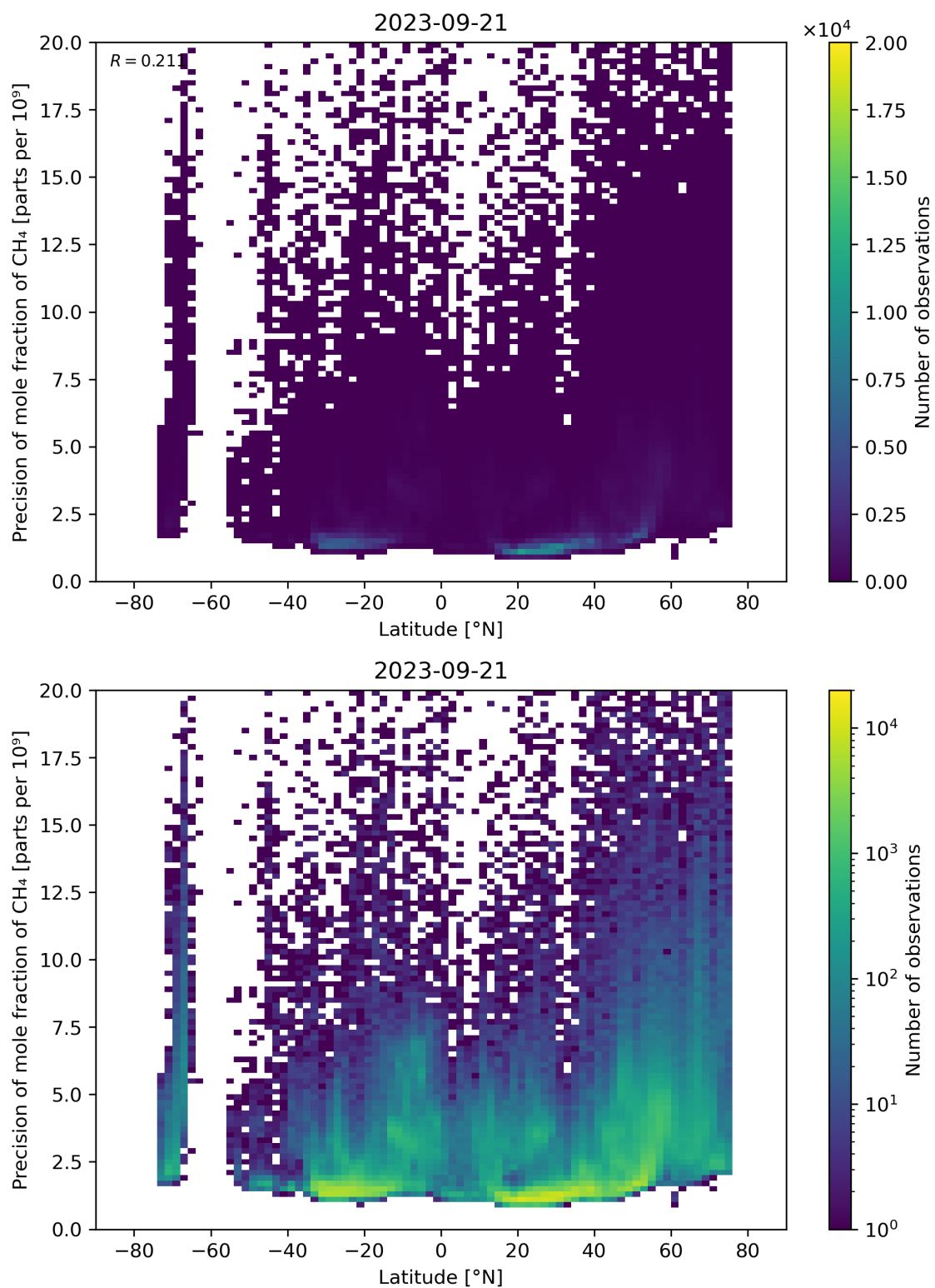
Figure 59: Scatter density plot of “Latitude” against “Precision of mole fraction of \text{CH}_4 ” for 2023-09-20 to 2023-09-22.
