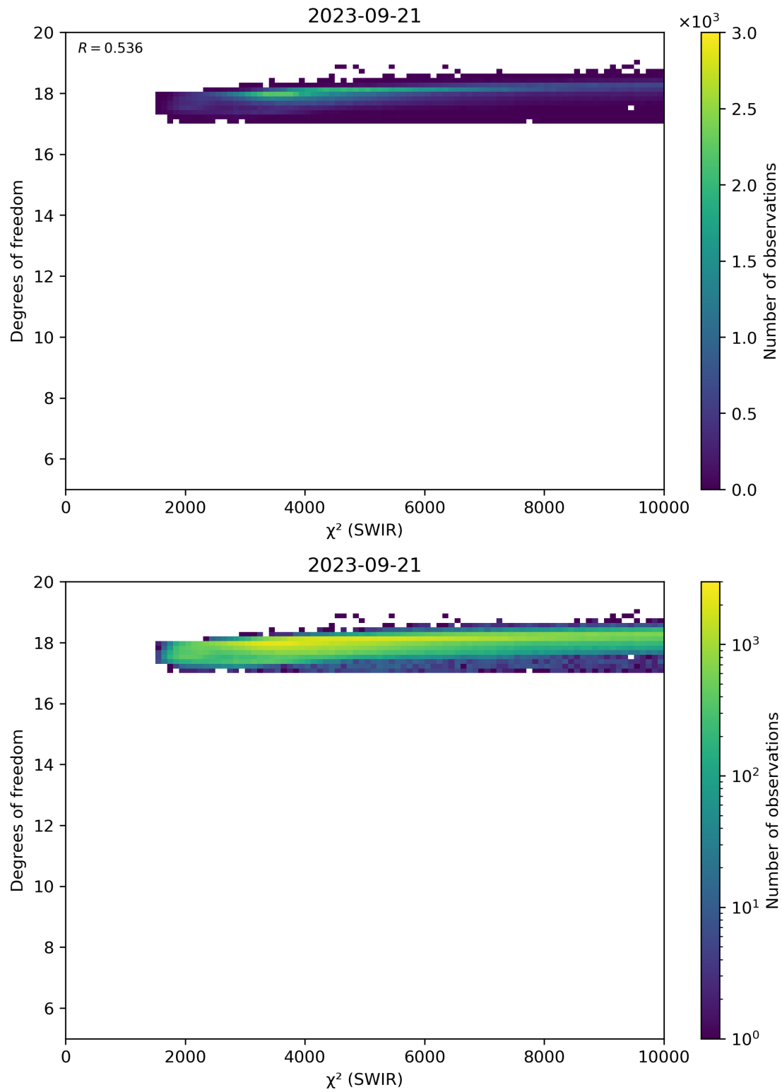
Figure 48: Scatter density plot of “ \chi^2 (SWIR)” against “Degrees of freedom” for 2023-09-20 to 2023-09-22.
