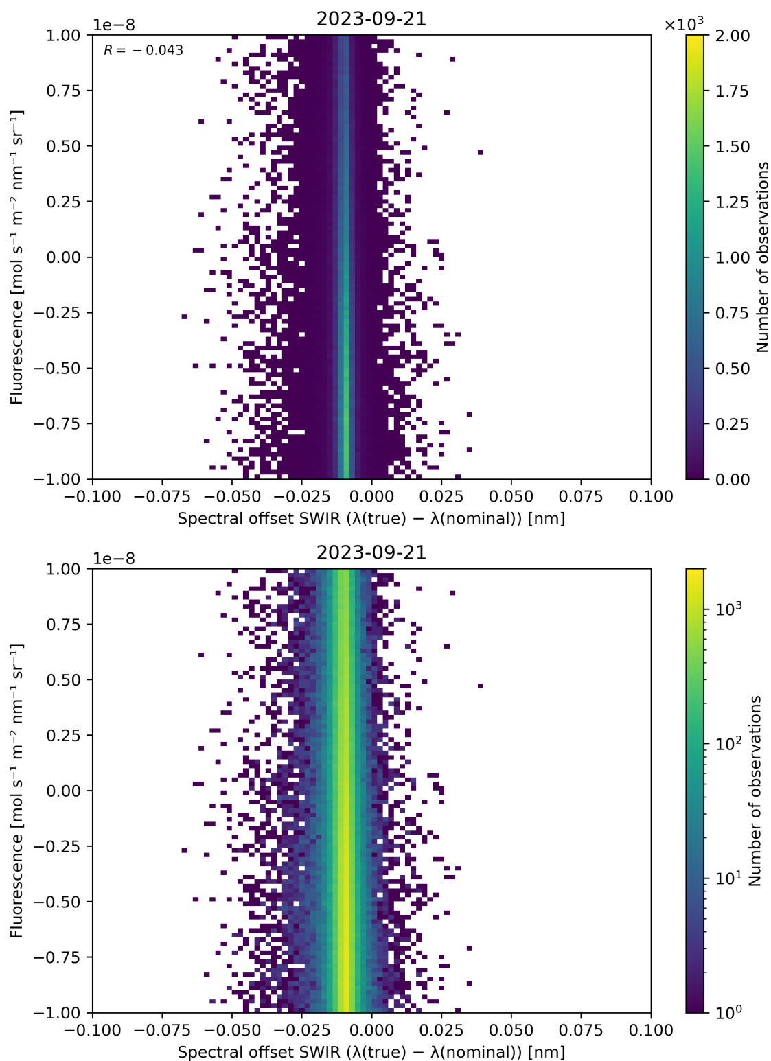
Figure 120: Scatter density plot of “Spectral offset SWIR ( \lambda(\text{true}) - \lambda(\text{nominal}) )” against “Fluorescence” for 2023-09-20 to 2023-09-22.
