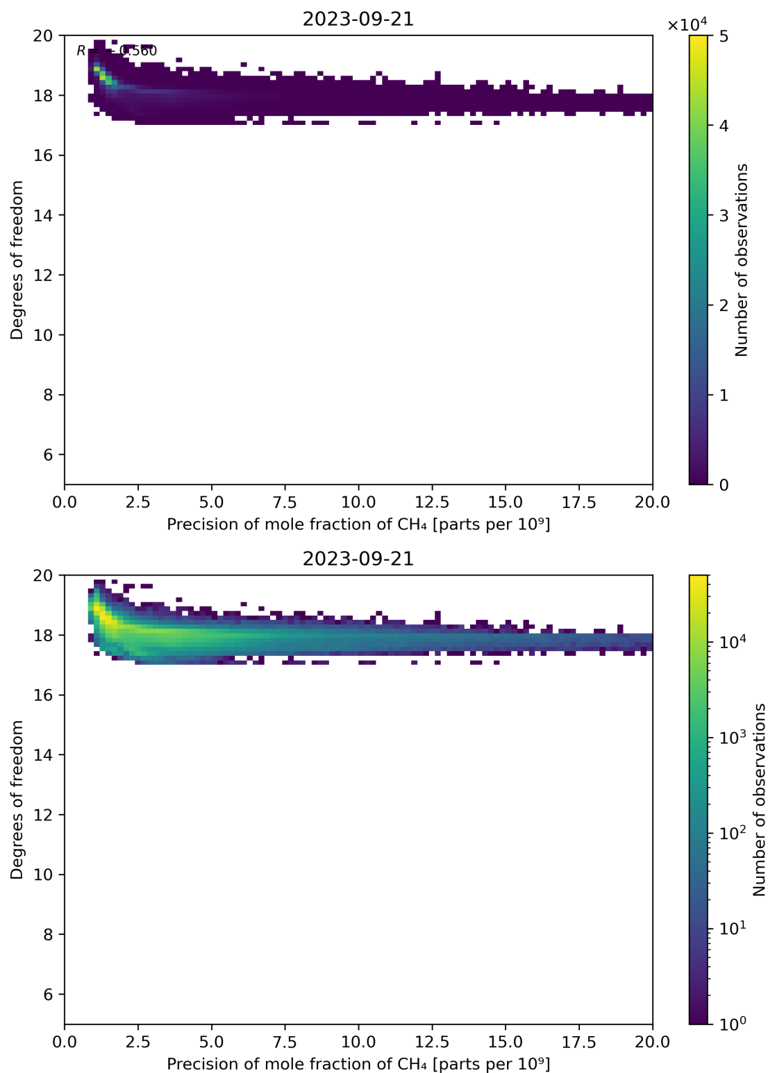
Figure 80: Scatter density plot of “Precision of mole fraction of CH 4 ” against “Degrees of freedom” for 2023-09-20 to 2023-09-22.
