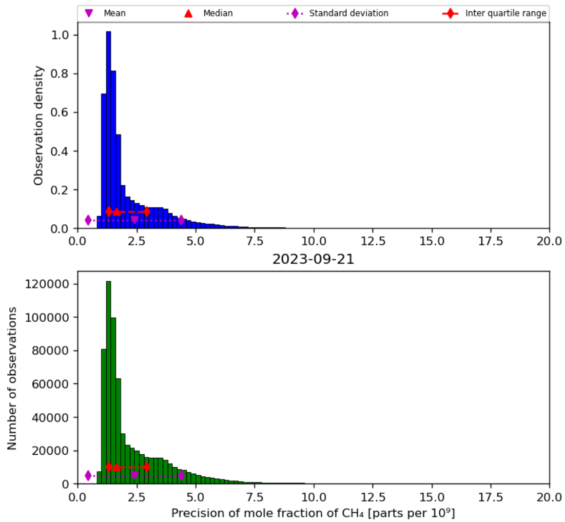
Figure 24: Histogram of “Precision of mole fraction of CH 4 ” for 2023-09-20 to 2023-09-22
