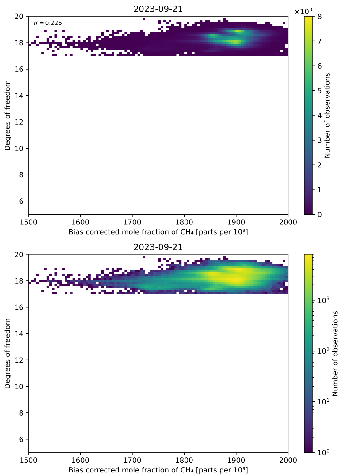
Figure 65: Scatter density plot of “Bias corrected mole fraction of CH 4 ” against “Degrees of freedom” for 2023-09-20 to 2023-09-22.
