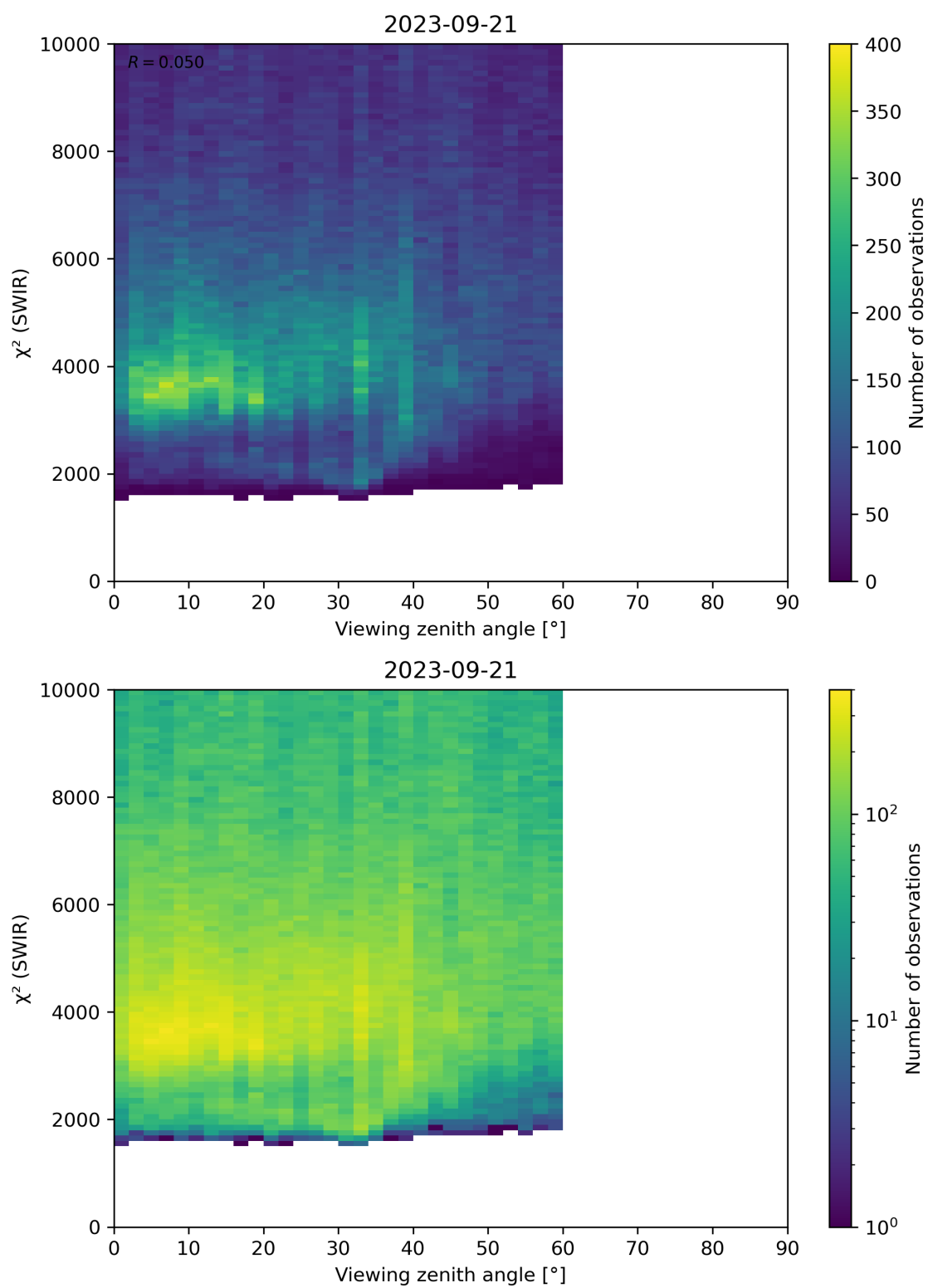
Figure 106: Scatter density plot of “Viewing zenith angle” against “ \chi^2 (SWIR)” for 2023-09-20 to 2023-09-22.
