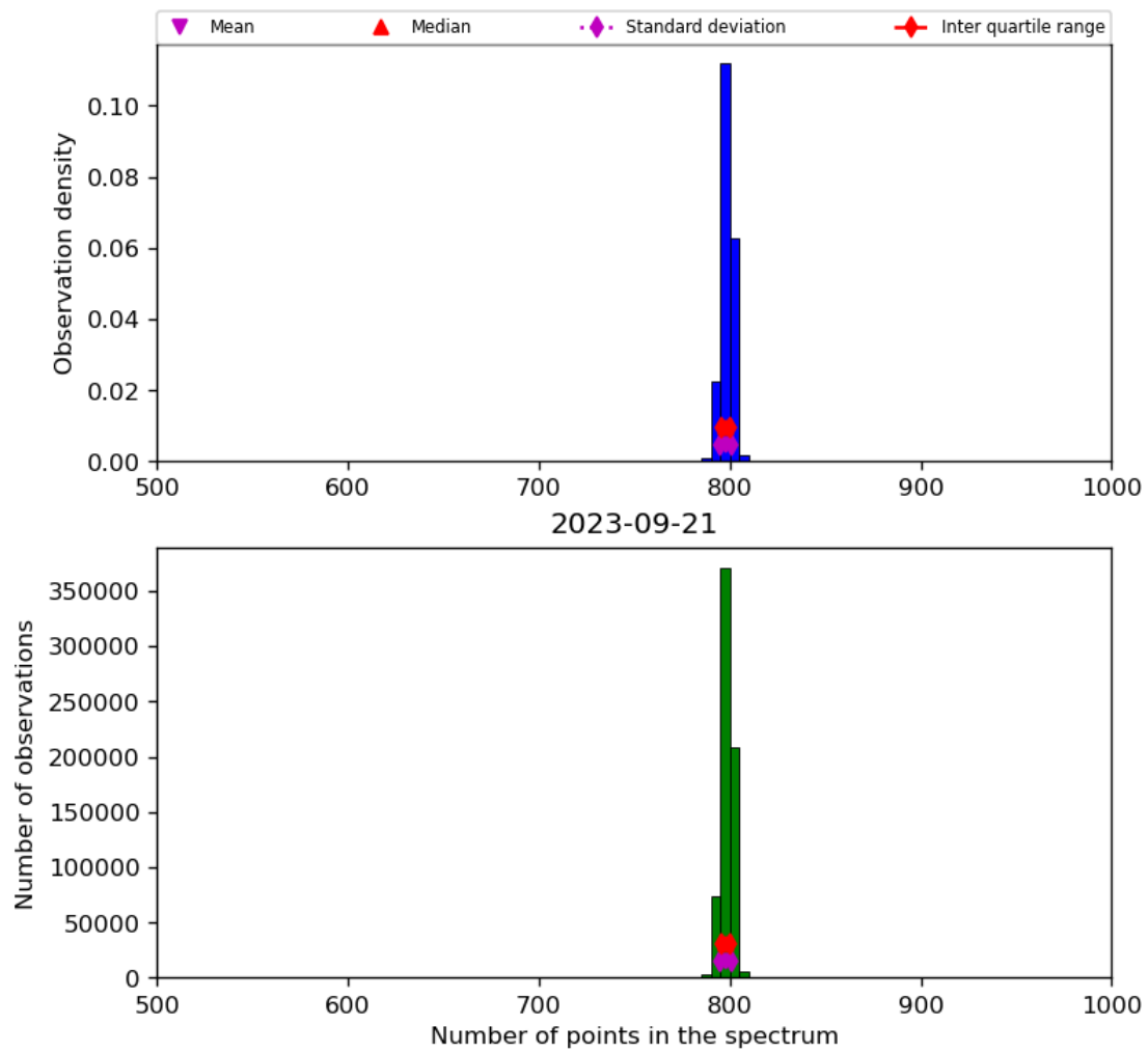
Figure 26: Histogram of “Number of points in the spectrum” for 2023-09-20 to 2023-09-22
