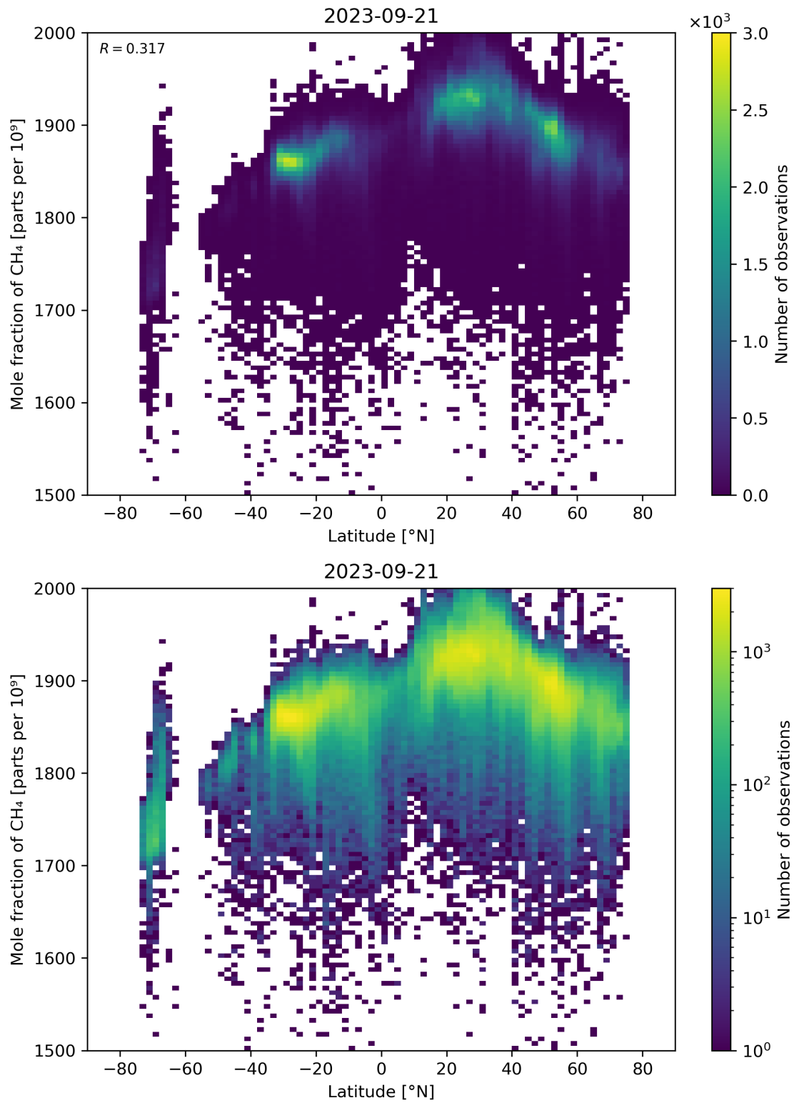
Figure 57: Scatter density plot of “Latitude” against “Mole fraction of CH 4 ” for 2023-09-20 to 2023-09-22.
