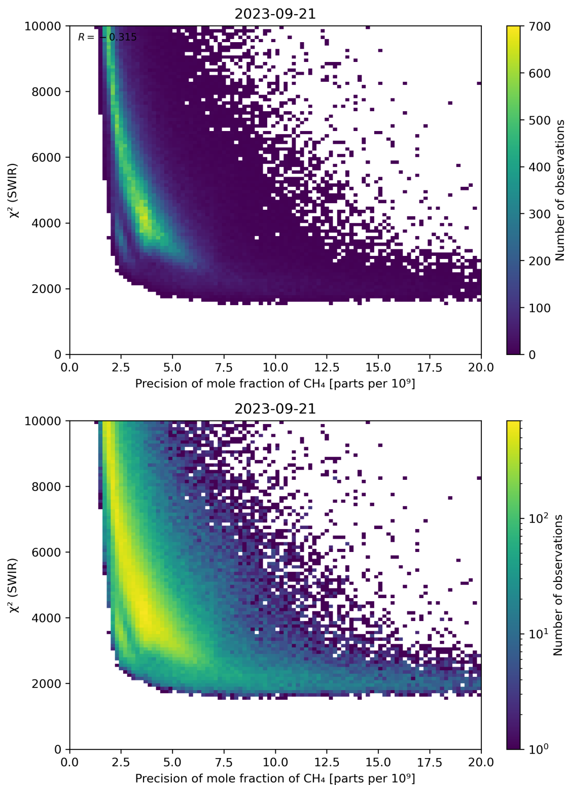
Figure 79: Scatter density plot of “Precision of mole fraction of CH 4 ” against “ \chi^2 (SWIR)” for 2023-09-20 to 2023-09-22.
