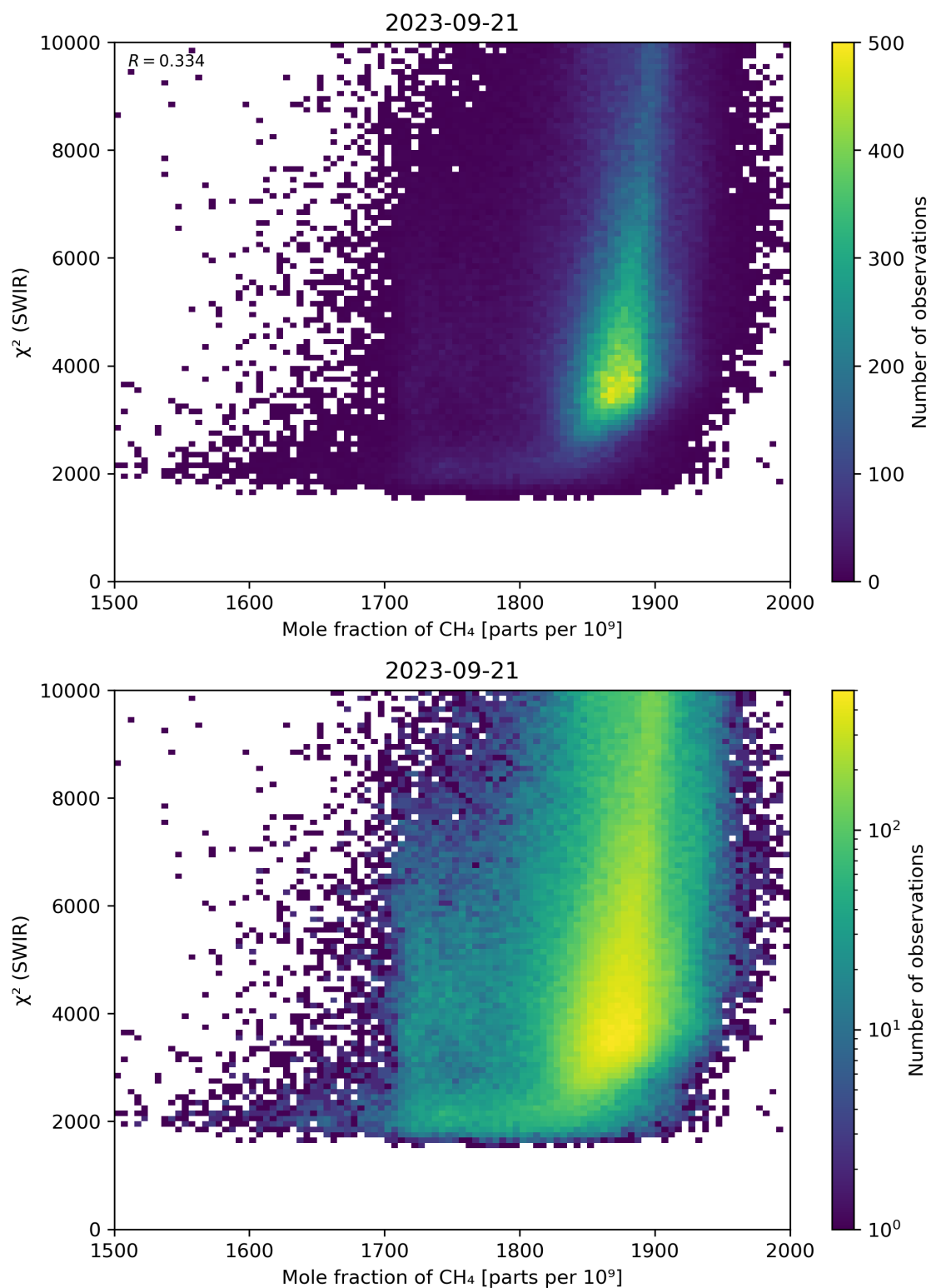
Figure 71: Scatter density plot of “Mole fraction of \text{CH}_4 ” against “ \chi^2 (SWIR)” for 2023-09-20 to 2023-09-22.
