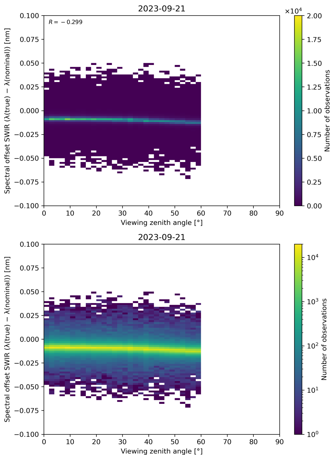
Figure 116: Scatter density plot of “Viewing zenith angle” against “Spectral offset SWIR ( \lambda(\text{true}) - \lambda(\text{nominal}) )” for 2023-09-20 to 2023-09-22.
