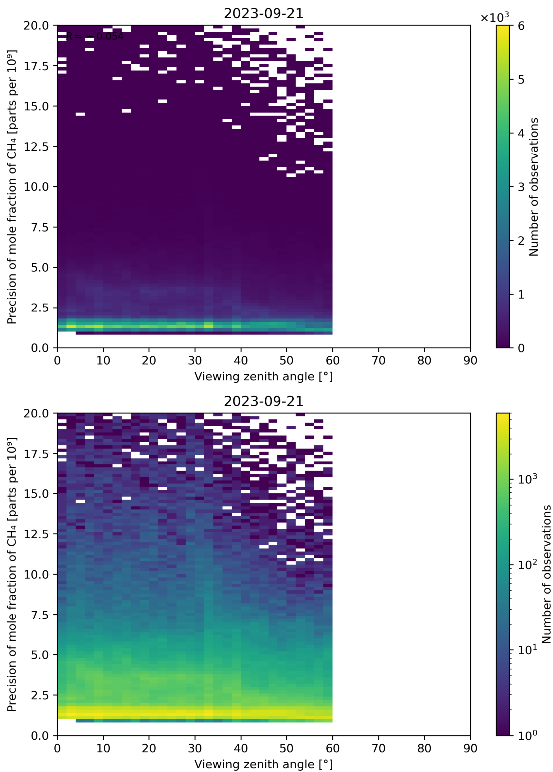
Figure 112: Scatter density plot of “Viewing zenith angle” against “Precision of mole fraction of \text{CH}_4 ” for 2023-09-20 to 2023-09-22.
