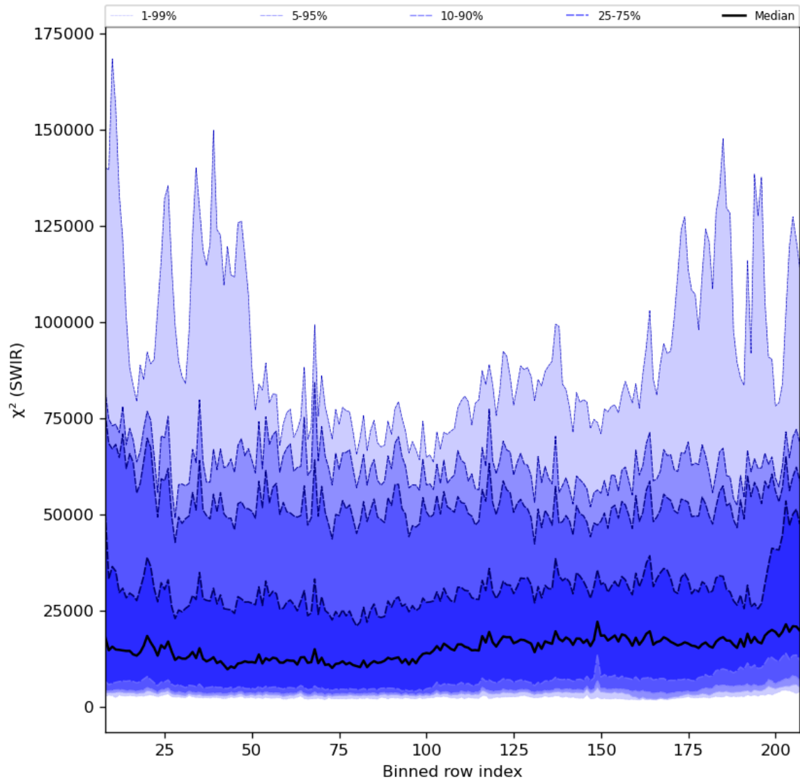
Figure 39: Along track statistics of “ \chi^2 (SWIR)” for 2023-09-20 to 2023-09-22
