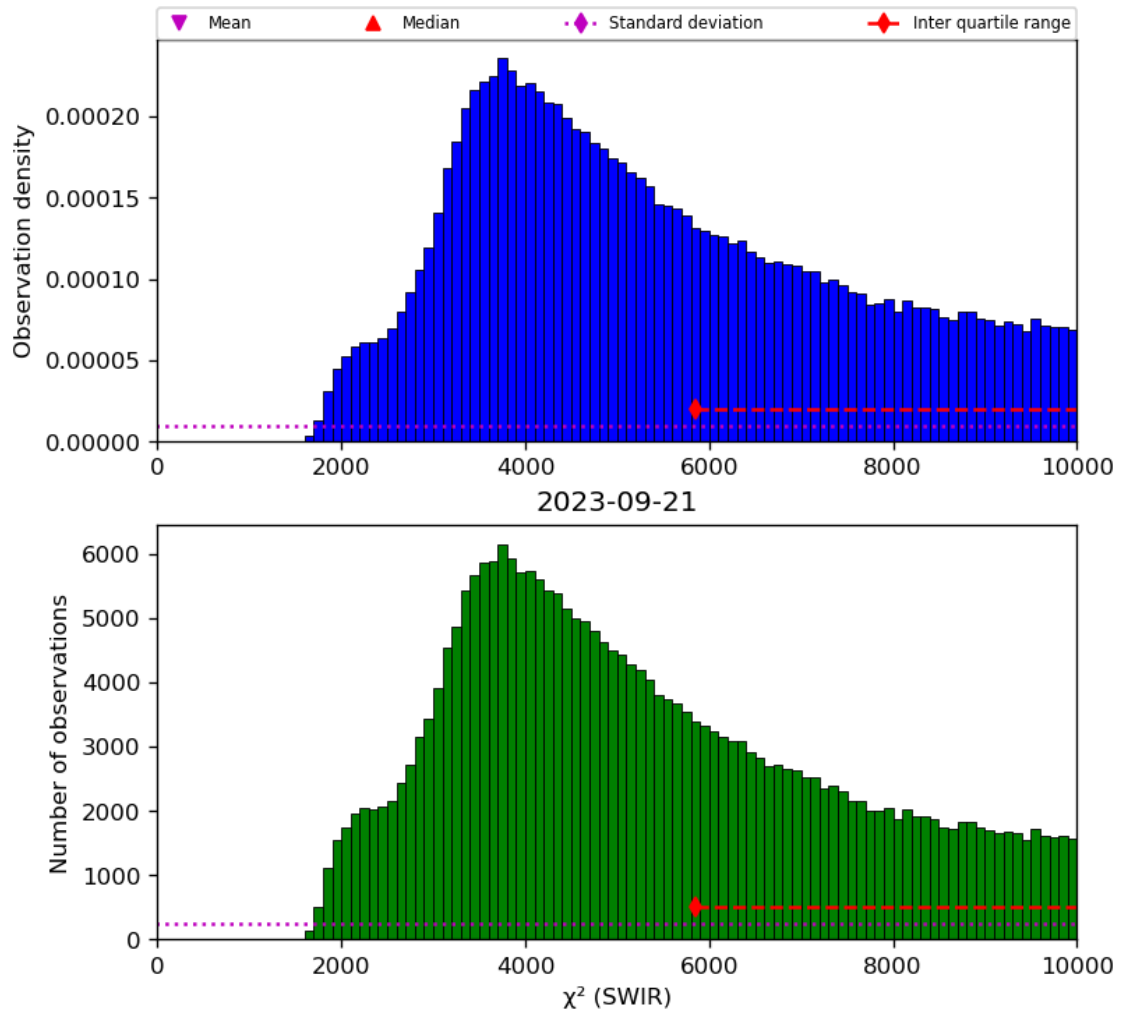
Figure 28: Histogram of “ \chi^2 (SWIR)” for 2023-09-20 to 2023-09-22
