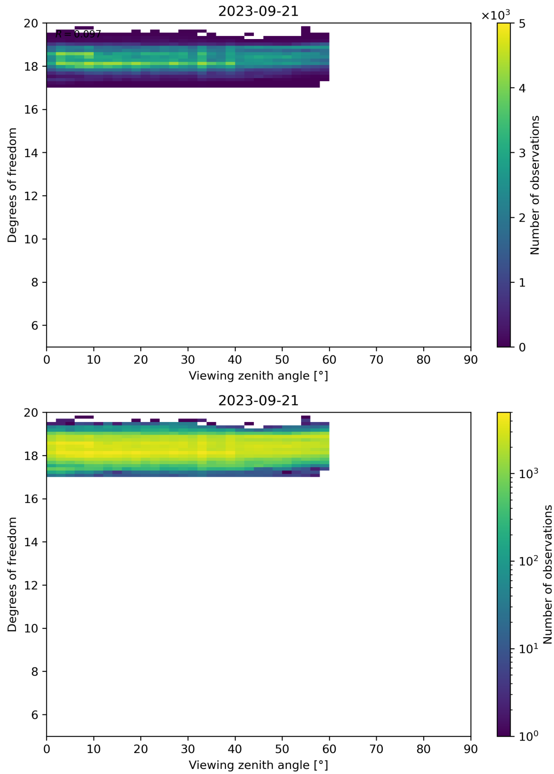
Figure 107: Scatter density plot of “Viewing zenith angle” against “Degrees of freedom” for 2023-09-20 to 2023-09-22.
