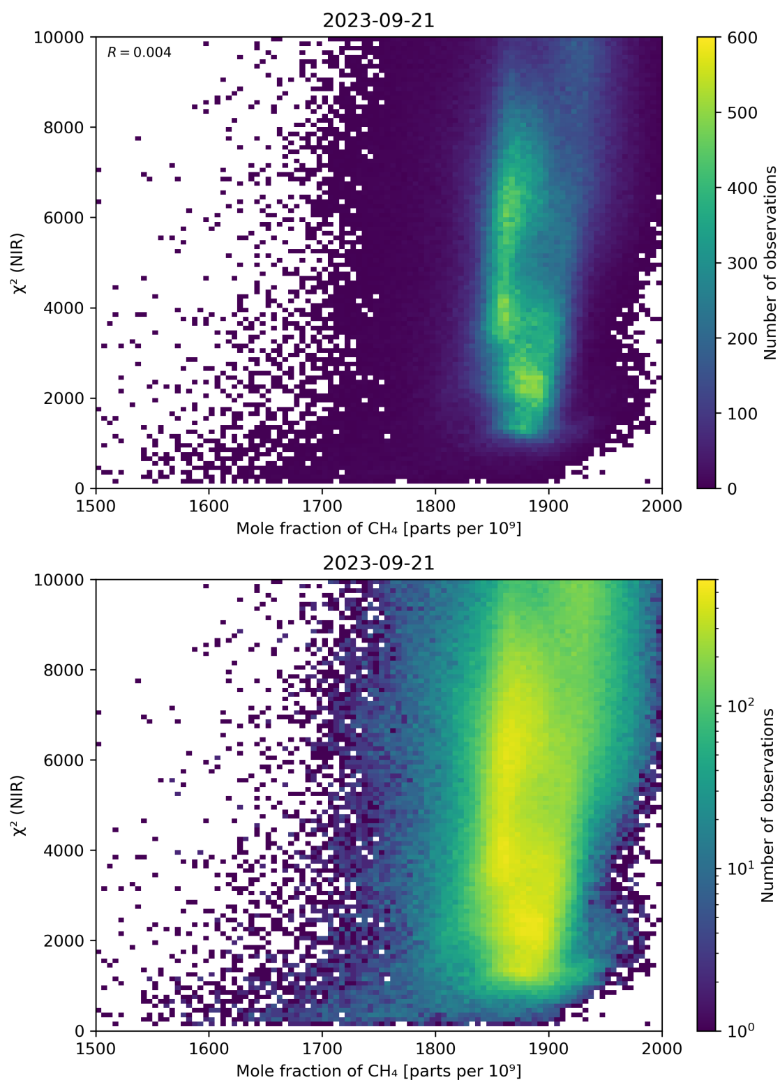
Figure 70: Scatter density plot of “Mole fraction of \text{CH}_4 ” against “ \chi^2 (NIR)” for 2023-09-20 to 2023-09-22.
