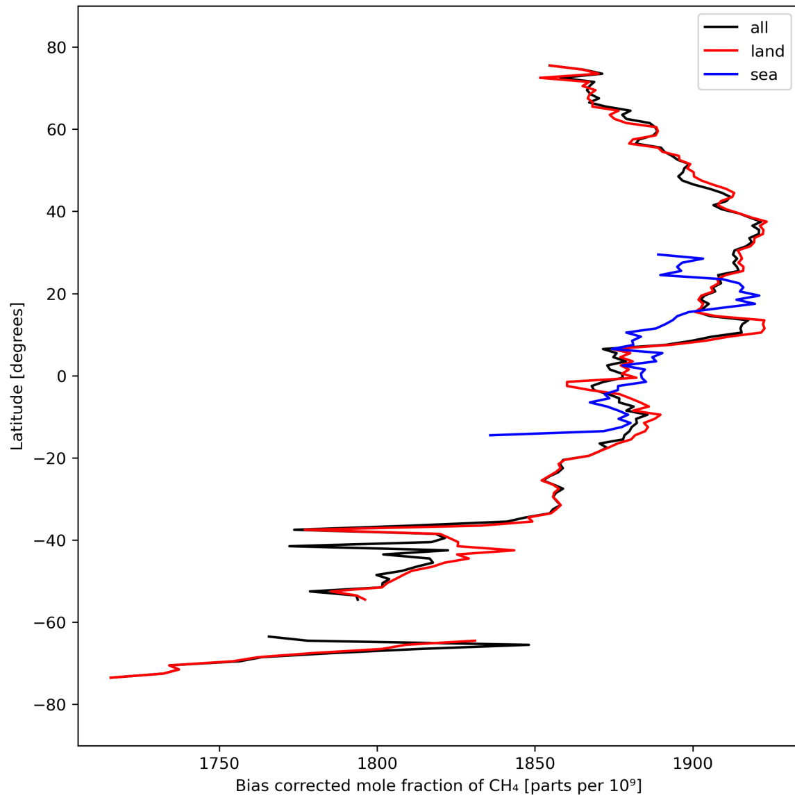
Figure 14: Zonal average of “Bias corrected mole fraction of CH 4 ” for 2023-09-20 to 2023-09-22.
