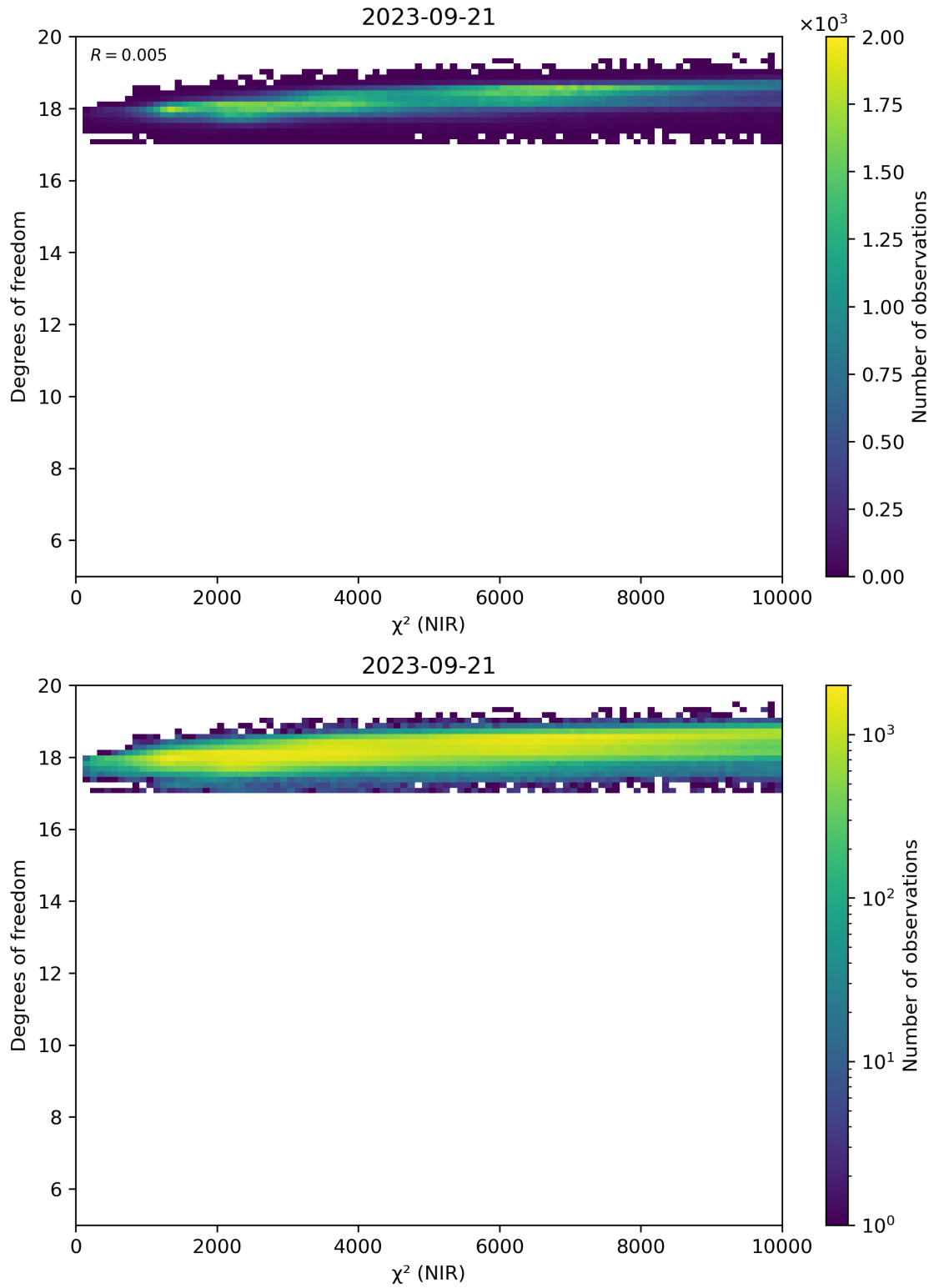
Figure 44: Scatter density plot of “ \chi^2 (NIR)” against “Degrees of freedom” for 2023-09-20 to 2023-09-22.
