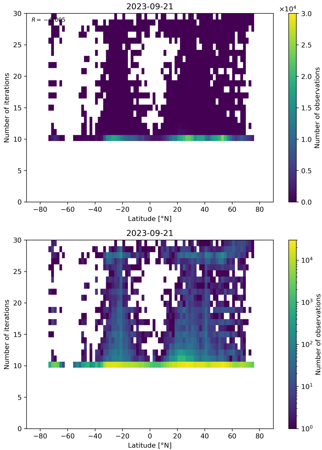
Figure 60: Scatter density plot of “Latitude” against “Number of iterations” for 2023-09-20 to 2023-09-22.
