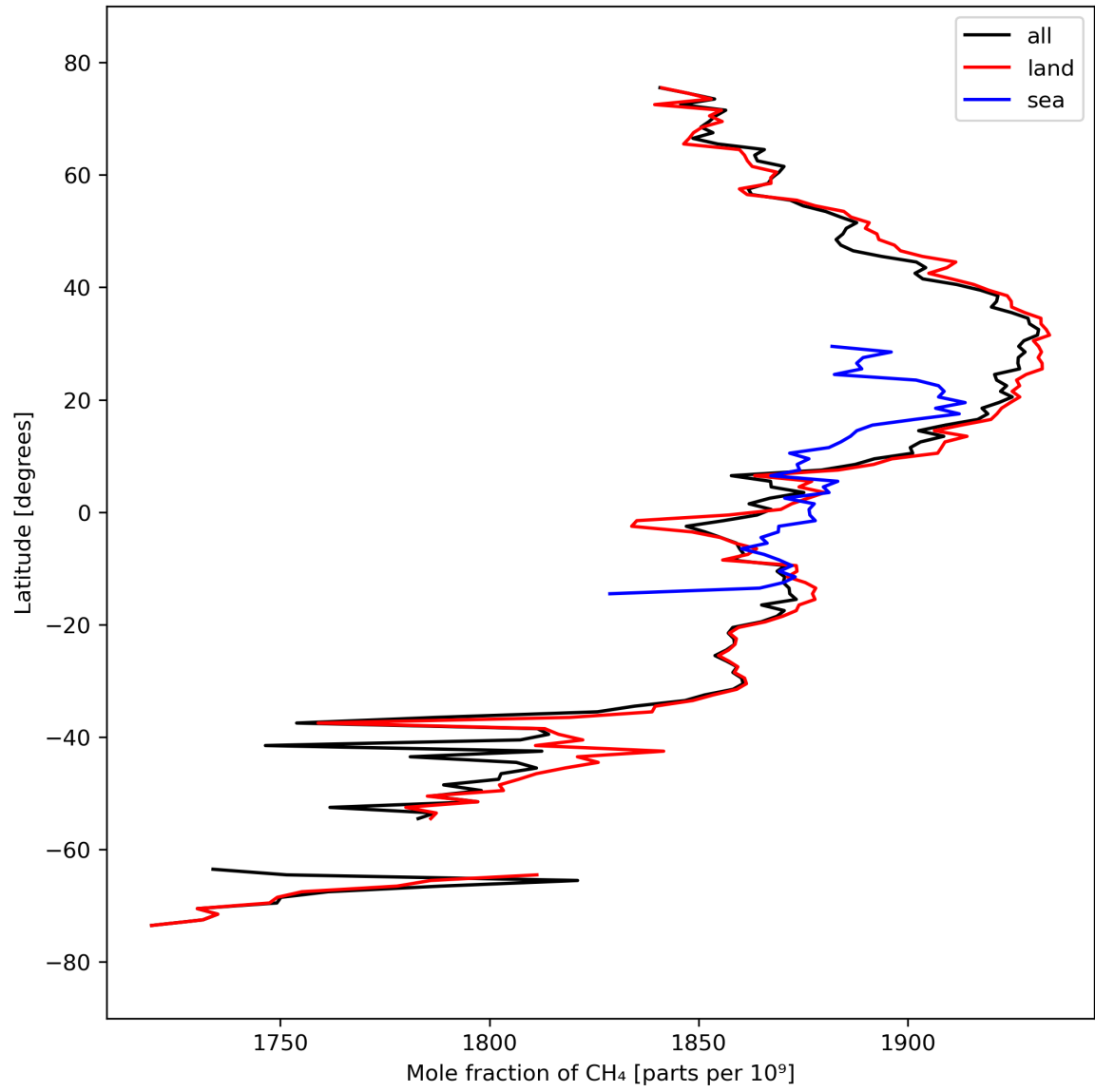
Figure 12: Zonal average of “Mole fraction of CH 4 ” for 2023-09-20 to 2023-09-22.
