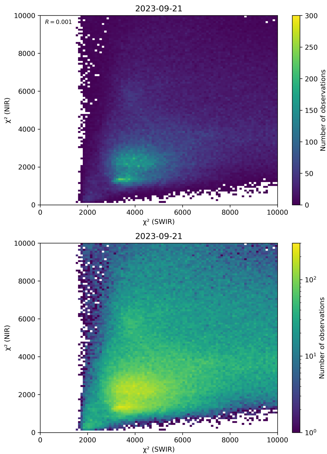
Figure 47: Scatter density plot of “ \chi^2 (SWIR)” against “ \chi^2 (NIR)” for 2023-09-20 to 2023-09-22.
