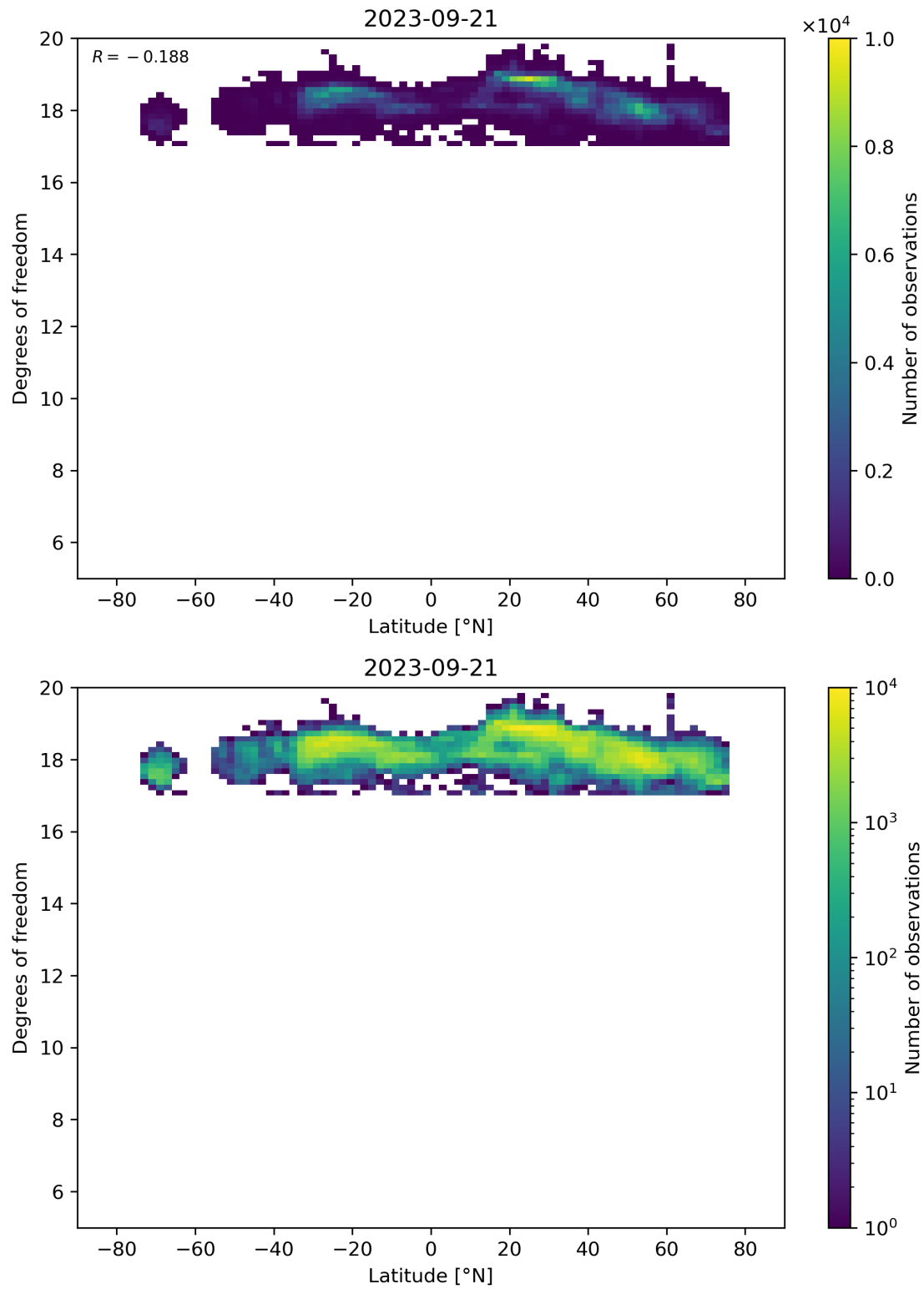
Figure 55: Scatter density plot of “Latitude” against “Degrees of freedom” for 2023-09-20 to 2023-09-22.
