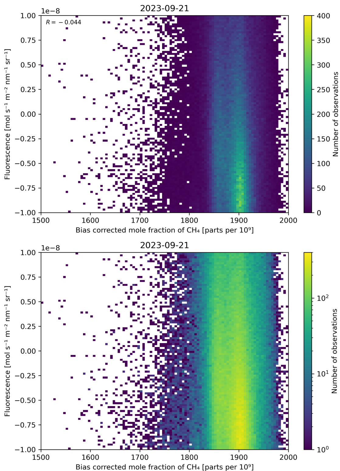
Figure 66: Scatter density plot of “Bias corrected mole fraction of \text{CH}_4 ” against “Fluorescence” for 2023-09-20 to 2023-09-22.
