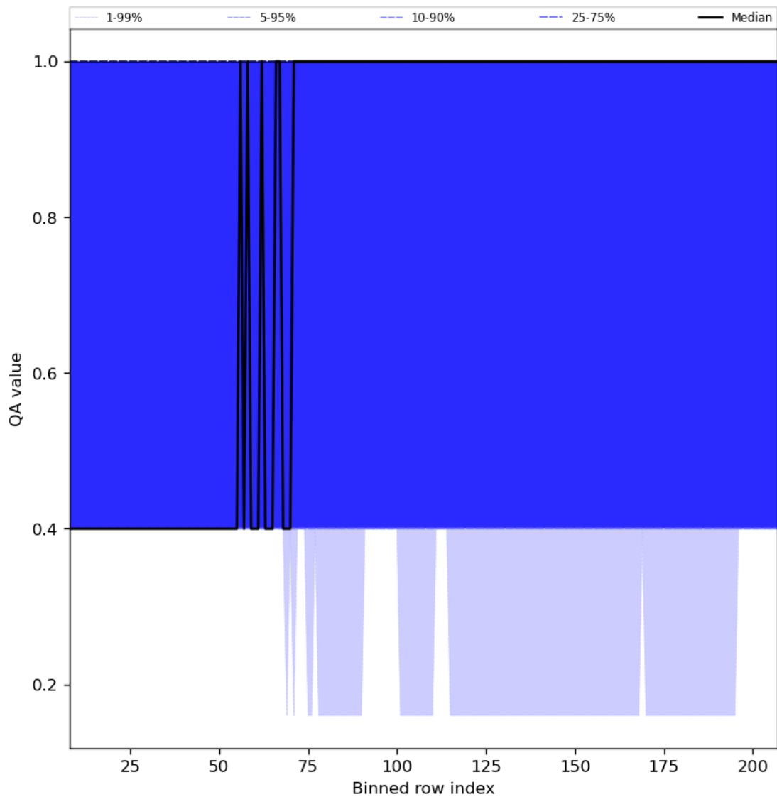
Figure 33: Along track statistics of “QA value” for 2023-09-20 to 2023-09-22
