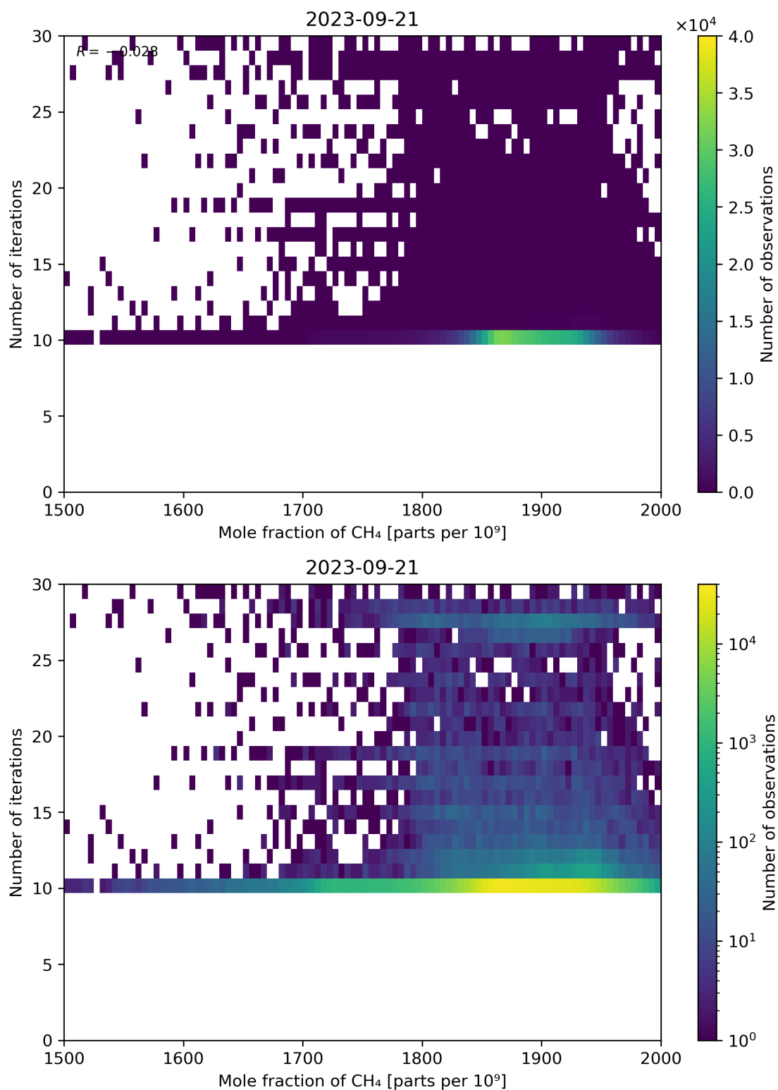
Figure 76: Scatter density plot of “Mole fraction of CH 4 ” against “Number of iterations” for 2023-09-20 to 2023-09-22.
