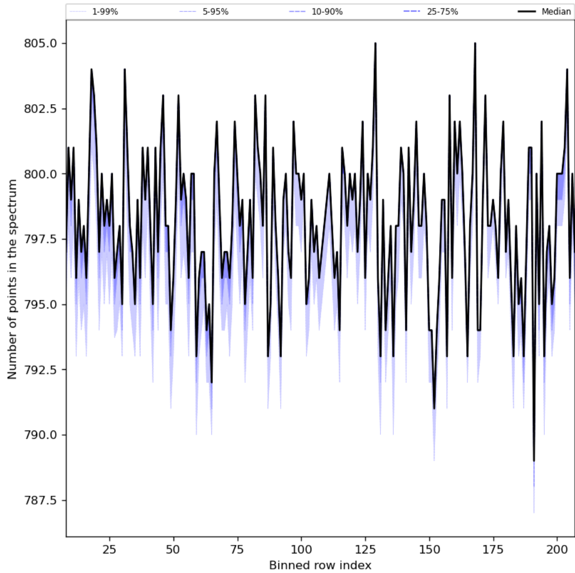
Figure 37: Along track statistics of “Number of points in the spectrum” for 2023-09-20 to 2023-09-22
