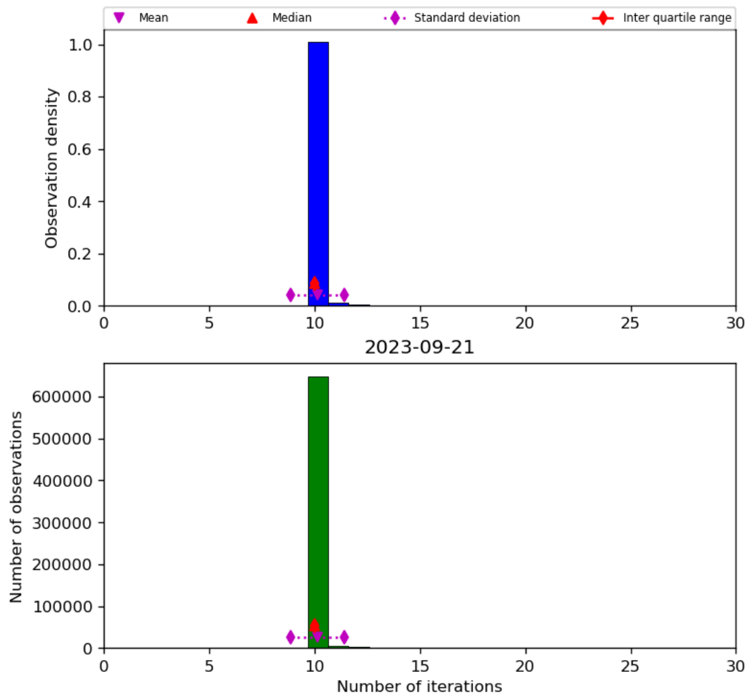
Figure 31: Histogram of “Number of iterations” for 2023-09-20 to 2023-09-22
