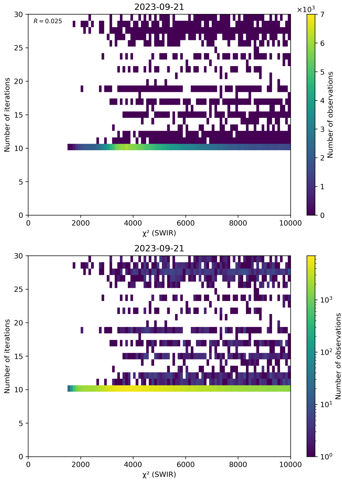
Figure 50: Scatter density plot of “ \chi^2 (SWIR)” against “Number of iterations” for 2023-09-20 to 2023-09-22.
