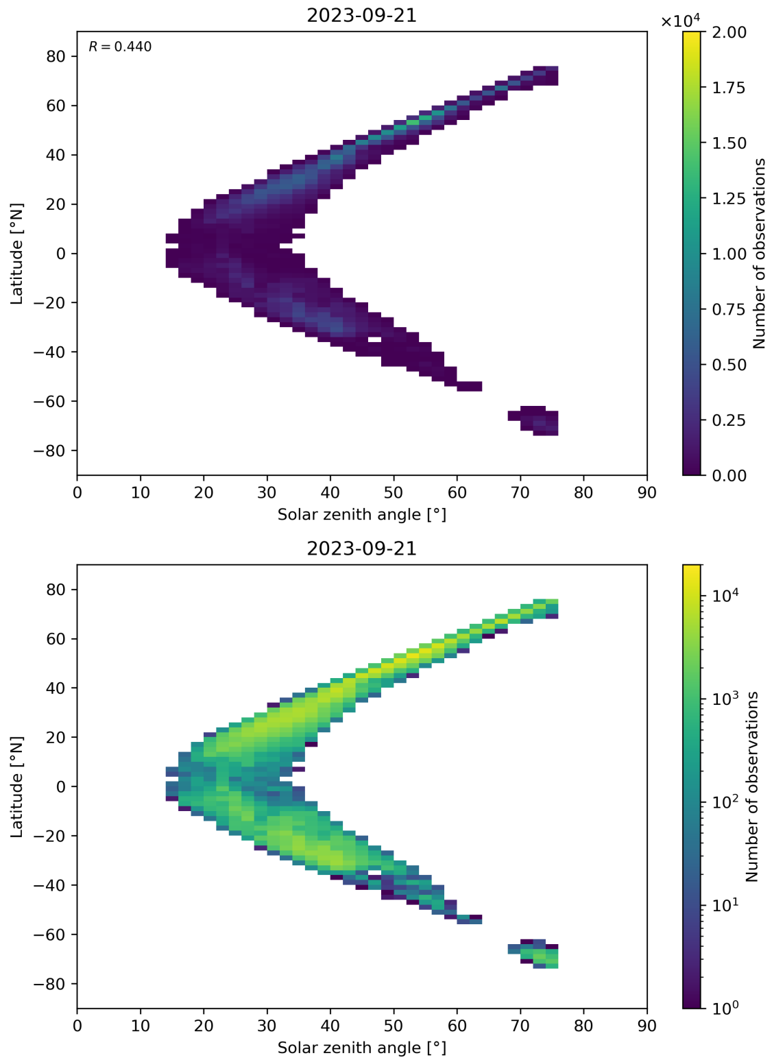
Figure 98: Scatter density plot of “Solar zenith angle” against “Latitude” for 2023-09-20 to 2023-09-22.
