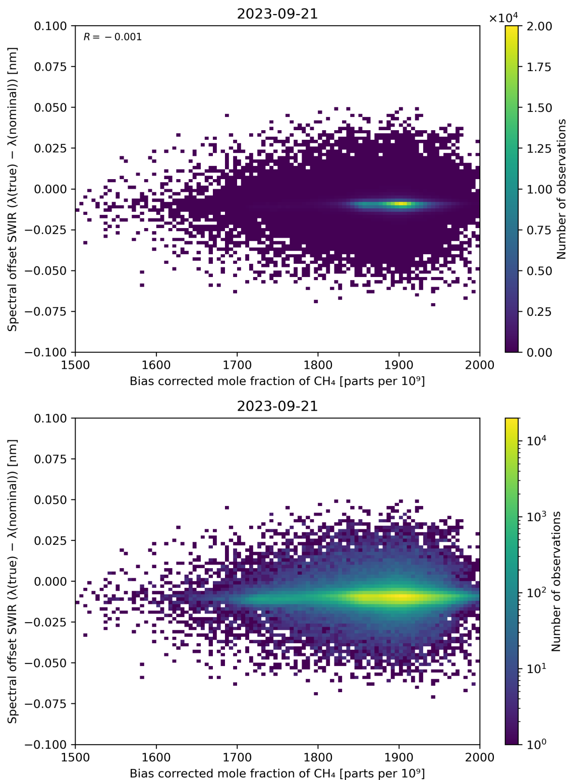
Figure 69: Scatter density plot of “Bias corrected mole fraction of \text{CH}_4 ” against “Spectral offset SWIR ( \lambda(\text{true}) - \lambda(\text{nominal}) )” for 2023-09-20 to 2023-09-22.
