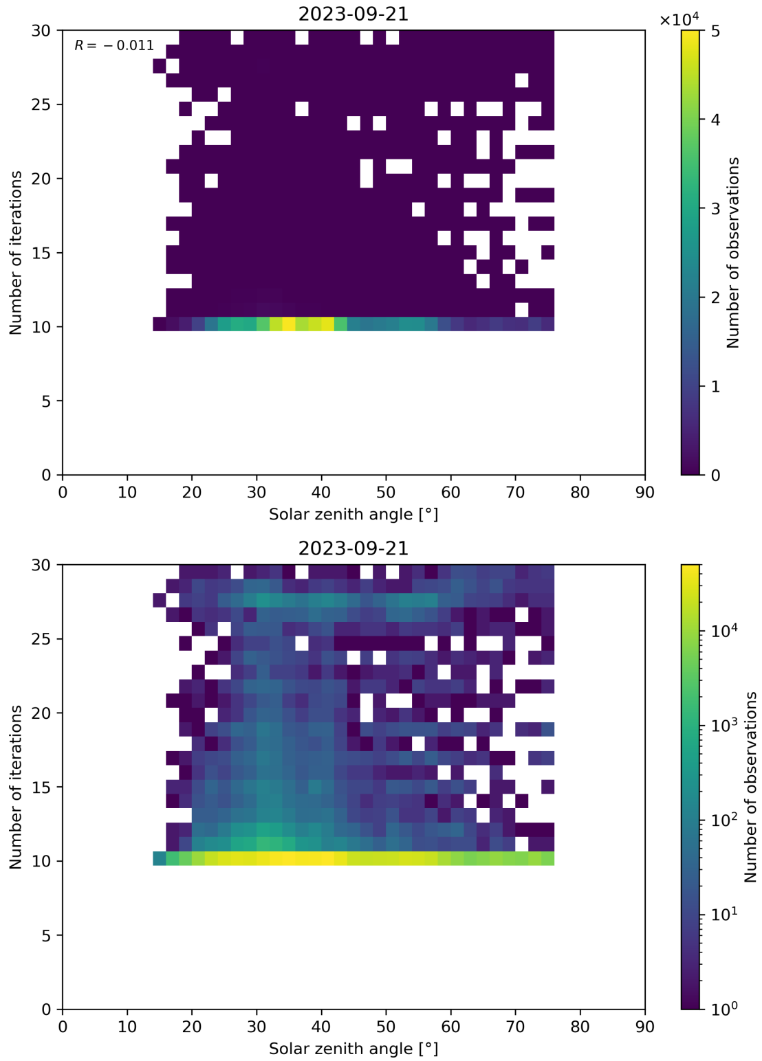
Figure 102: Scatter density plot of “Solar zenith angle” against “Number of iterations” for 2023-09-20 to 2023-09-22.
