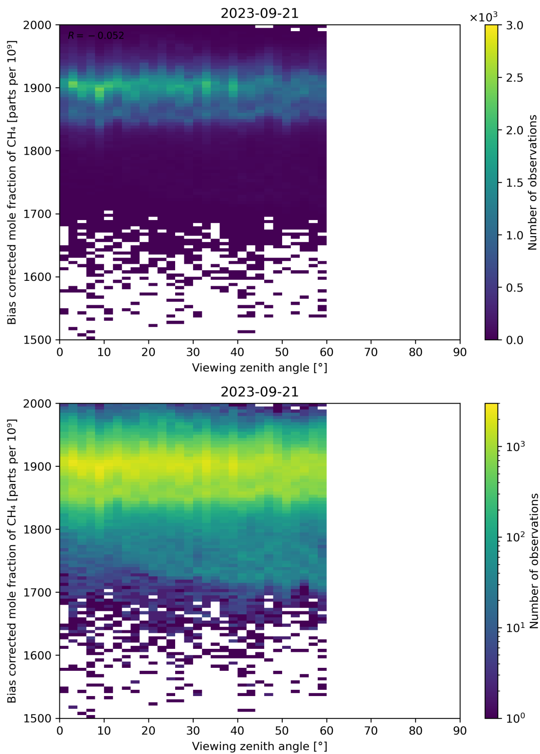
Figure 111: Scatter density plot of “Viewing zenith angle” against “Bias corrected mole fraction of CH 4 ” for 2023-09-20 to 2023-09-22.
