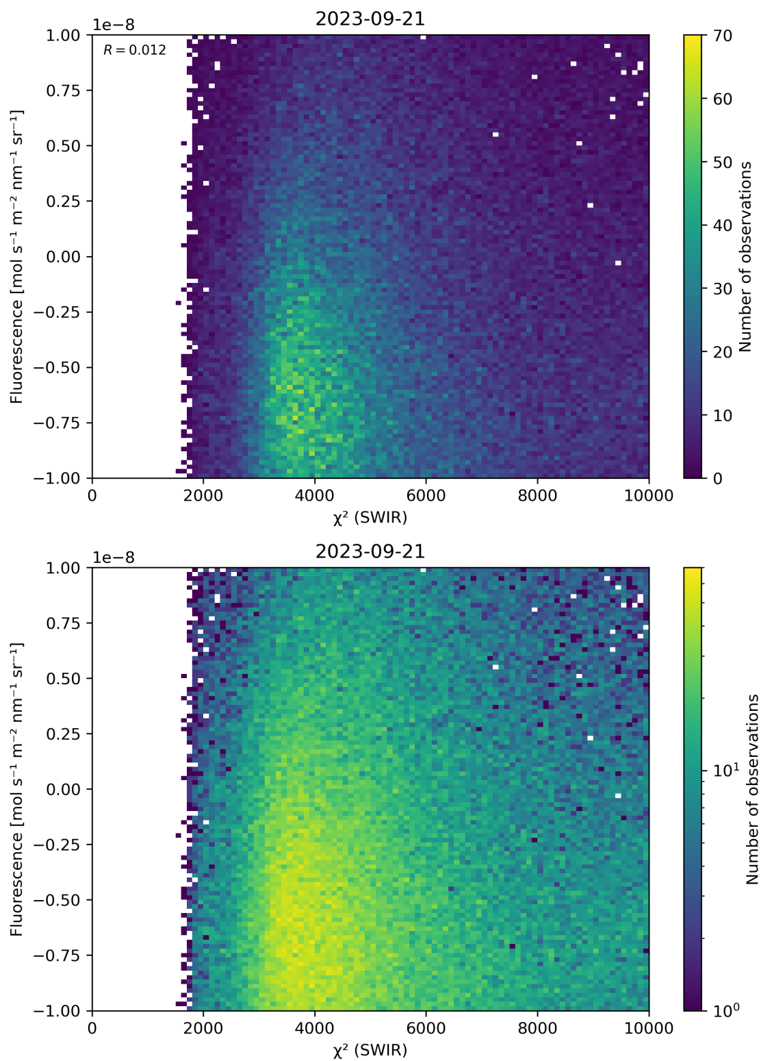
Figure 49: Scatter density plot of “ \chi^2 (SWIR)” against “Fluorescence” for 2023-09-20 to 2023-09-22.
