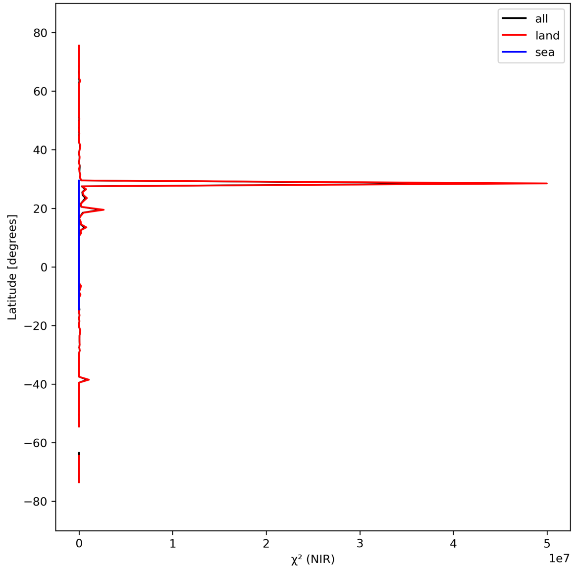
Figure 18: Zonal average of “ \chi^2 (NIR)” for 2023-09-20 to 2023-09-22.
