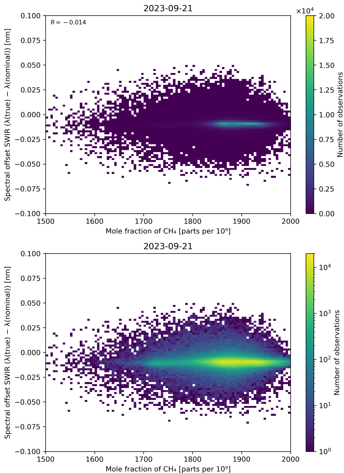
Figure 86: Scatter density plot of “Mole fraction of CH 4 ” against “Spectral offset SWIR ( \lambda(\text{true}) - \lambda(\text{nominal}) )” for 2023-09-20 to 2023-09-22.
