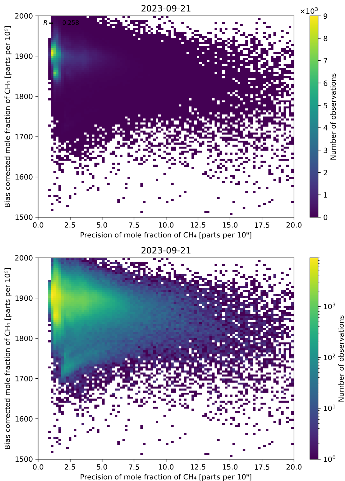
Figure 82: Scatter density plot of “Precision of mole fraction of CH 4 ” against “Bias corrected mole fraction of CH 4 ” for 2023-09-20 to 2023-09-22.
