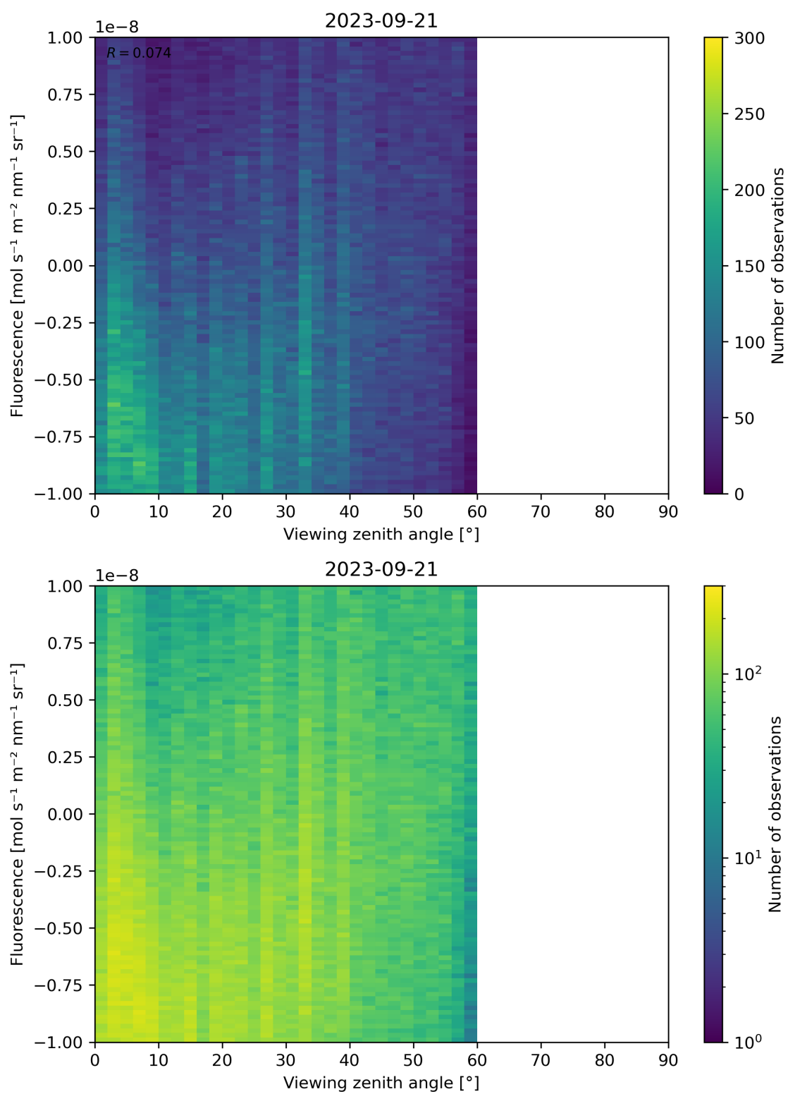
Figure 108: Scatter density plot of “Viewing zenith angle” against “Fluorescence” for 2023-09-20 to 2023-09-22.
