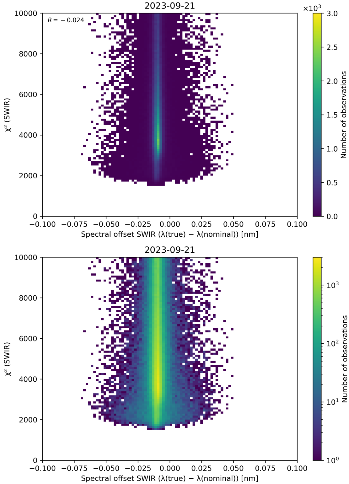
Figure 118: Scatter density plot of “Spectral offset SWIR ( \lambda(\text{true}) - \lambda(\text{nominal}) )” against “ \chi^2 (SWIR)” for 2023-09-20 to 2023-09-22.
