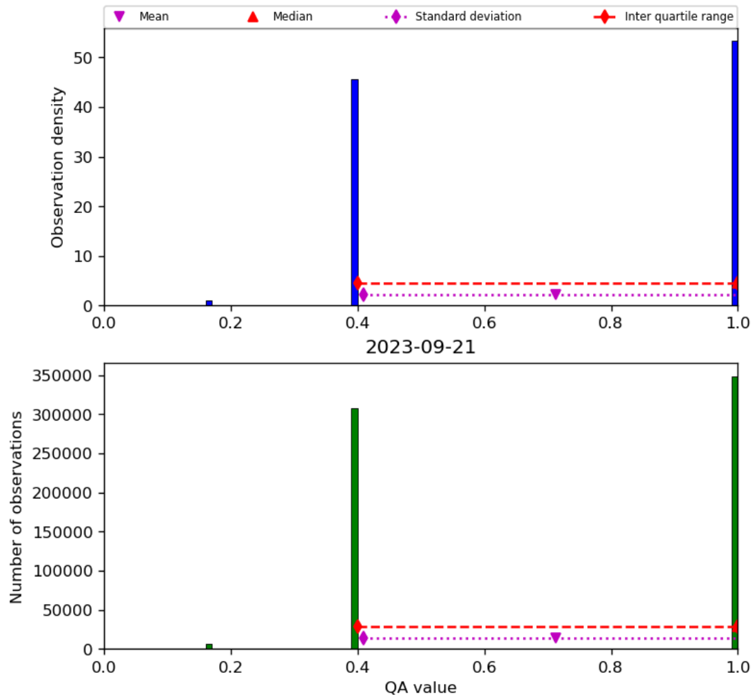
Figure 22: Histogram of “QA value” for 2023-09-20 to 2023-09-22
