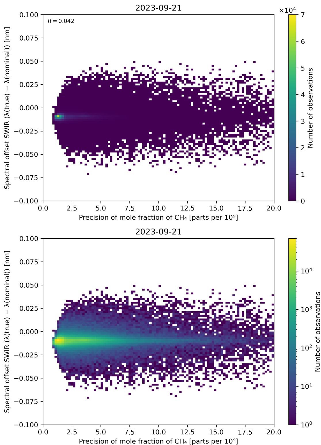
Figure 85: Scatter density plot of “Precision of mole fraction of CH 4 ” against “Spectral offset SWIR ( \lambda(\text{true}) - \lambda(\text{nominal}) )” for 2023-09-20 to 2023-09-22.
