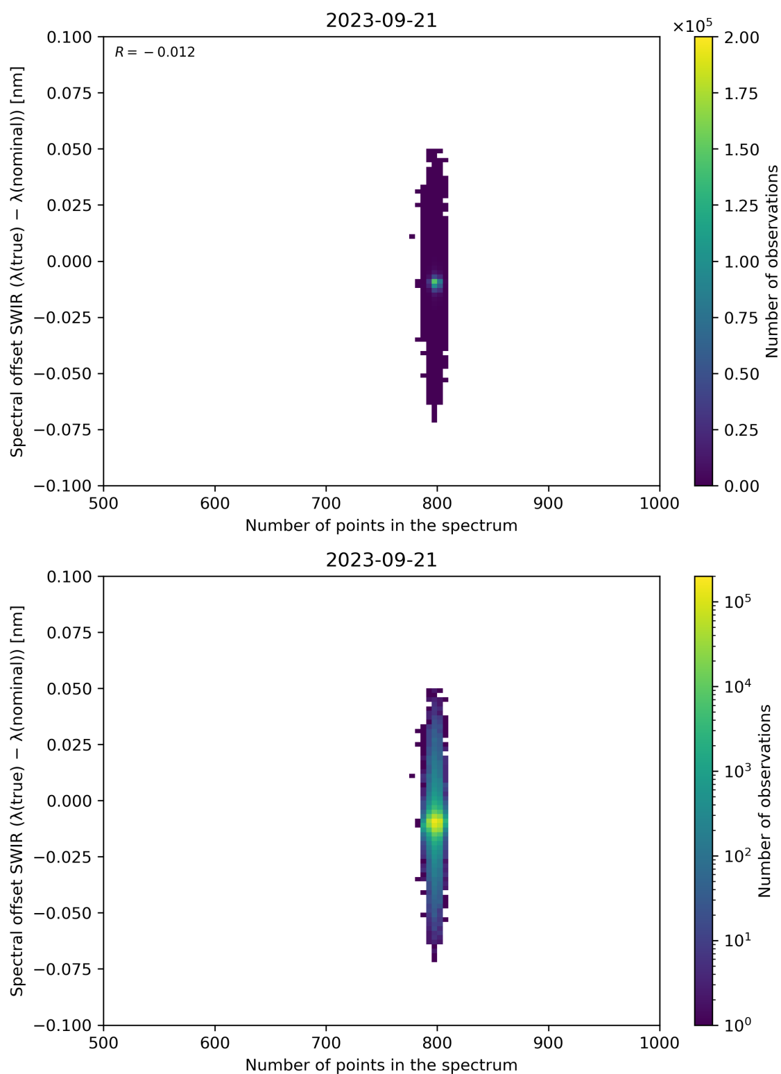
Figure 93: Scatter density plot of “Number of points in the spectrum” against “Spectral offset SWIR ( \lambda(\text{true}) - \lambda(\text{nominal}) )” for 2023-09-20 to 2023-09-22.
