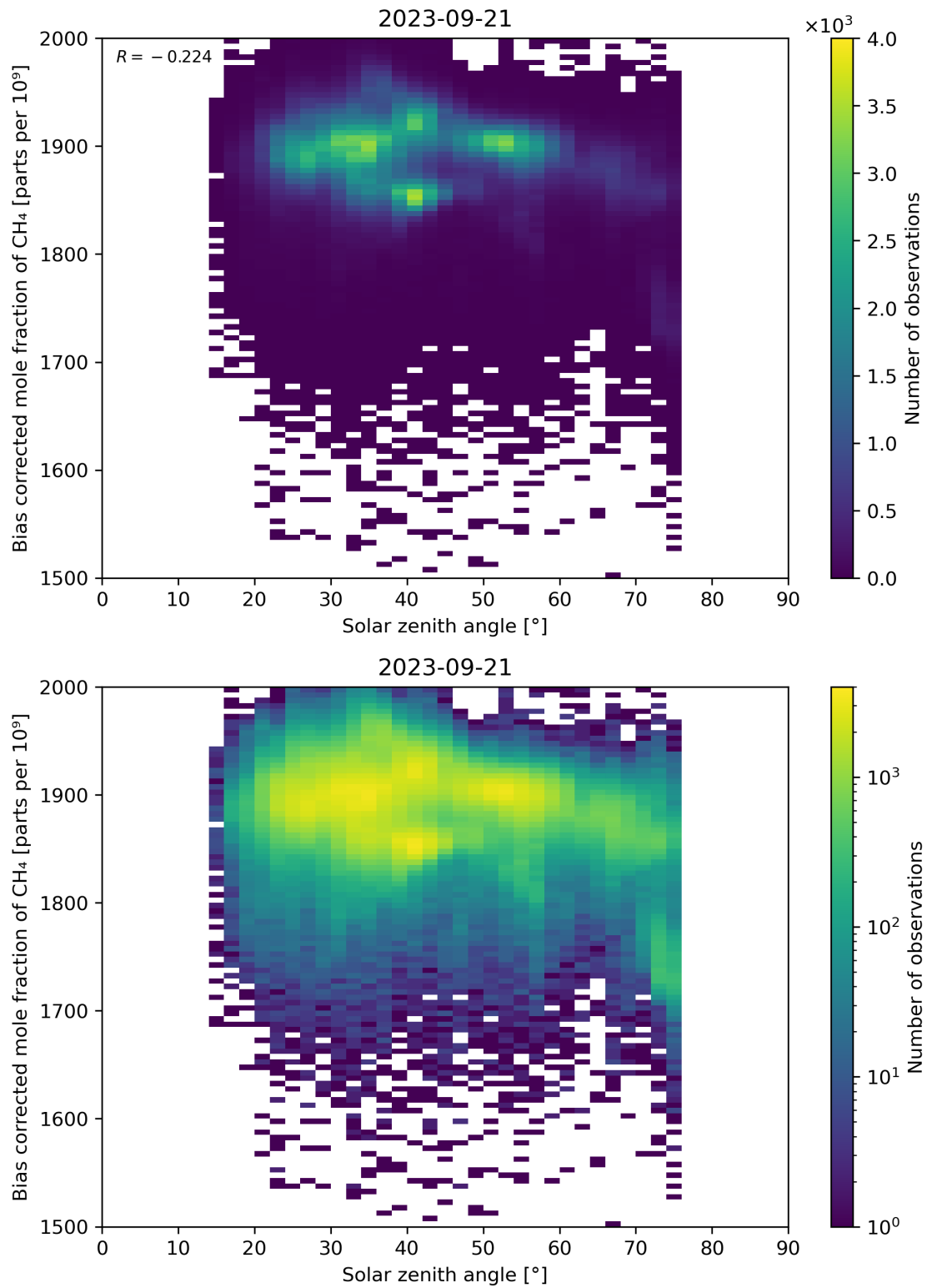
Figure 100: Scatter density plot of “Solar zenith angle” against “Bias corrected mole fraction of CH 4 ” for 2023-09-20 to 2023-09-22.
