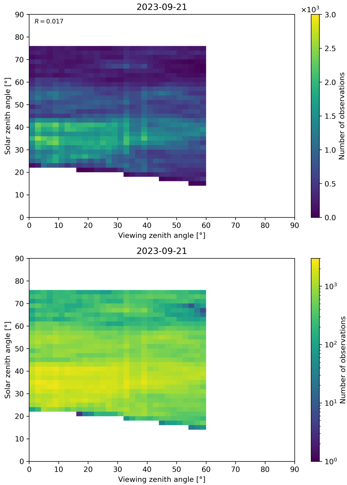
Figure 115: Scatter density plot of “Viewing zenith angle” against “Solar zenith angle” for 2023-09-20 to 2023-09-22.
