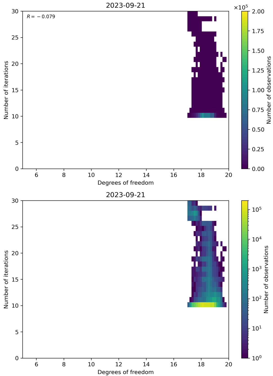
Figure 52: Scatter density plot of “Degrees of freedom” against “Number of iterations” for 2023-09-20 to 2023-09-22.
