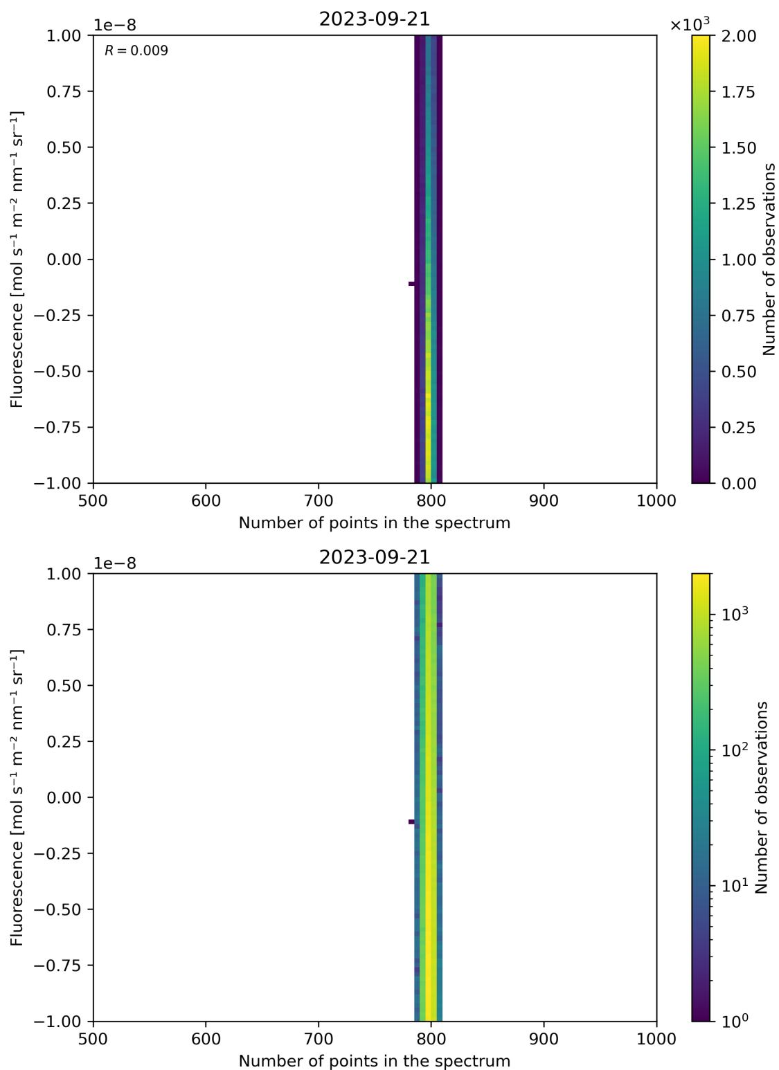
Figure 91: Scatter density plot of “Number of points in the spectrum” against “Fluorescence” for 2023-09-20 to 2023-09-22.
