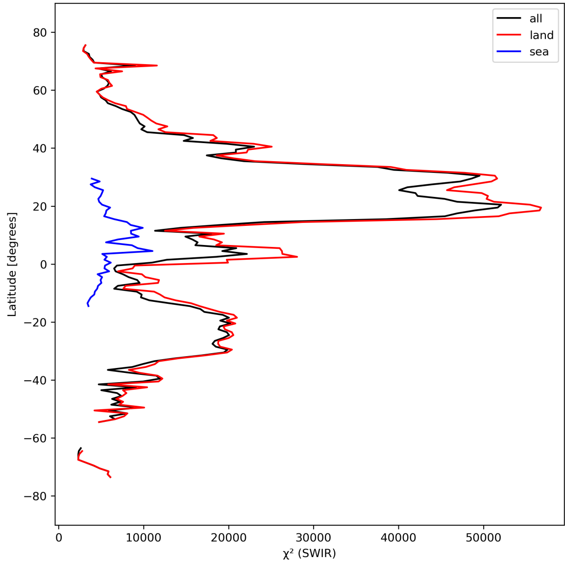
Figure 17: Zonal average of “ \chi^2 (SWIR)” for 2023-09-20 to 2023-09-22.
