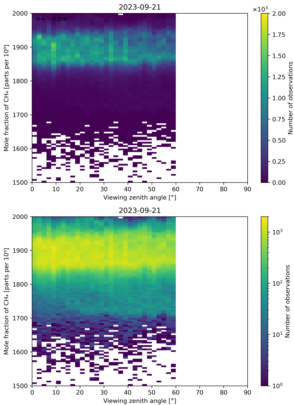
Figure 110: Scatter density plot of “Viewing zenith angle” against “Mole fraction of CH 4 ” for 2023-09-20 to 2023-09-22.
