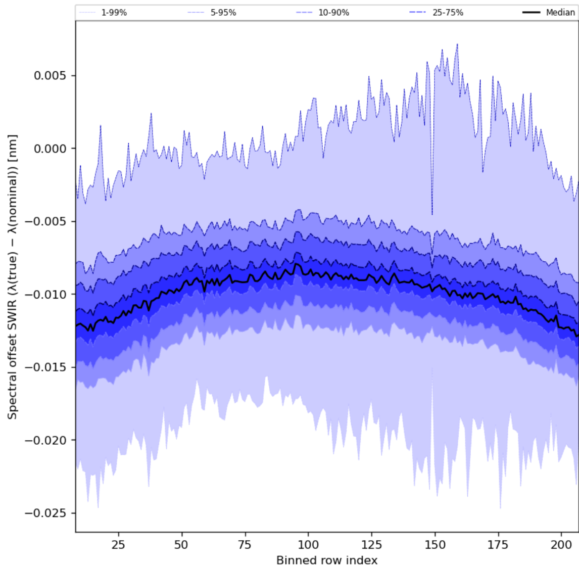
Figure 38: Along track statistics of “Spectral offset SWIR ( \lambda(\text{true}) - \lambda(\text{nominal}) )” for 2023-09-20 to 2023-09-22
