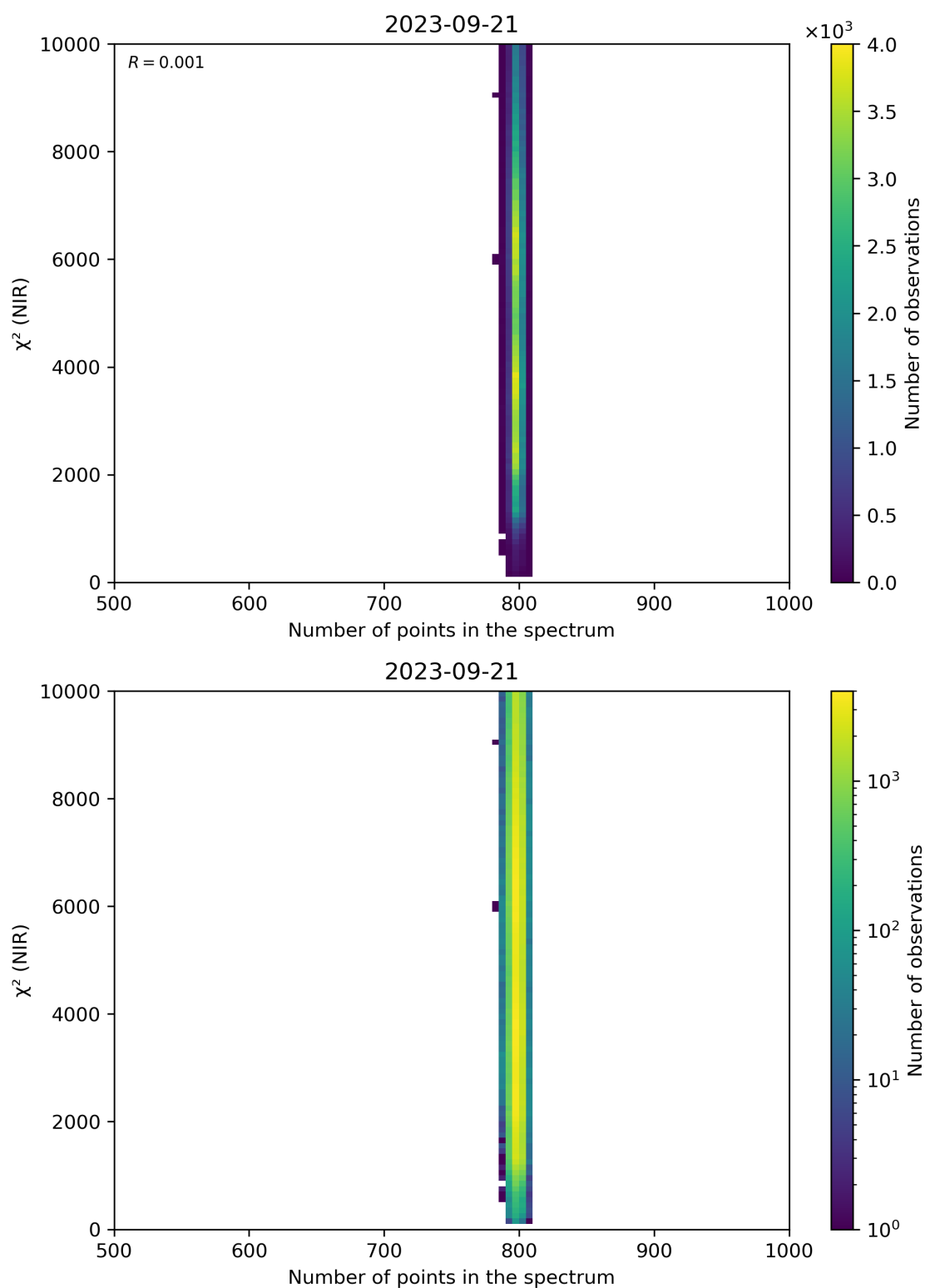
Figure 88: Scatter density plot of “Number of points in the spectrum” against “ \chi^2 (NIR)” for 2023-09-20 to 2023-09-22.
