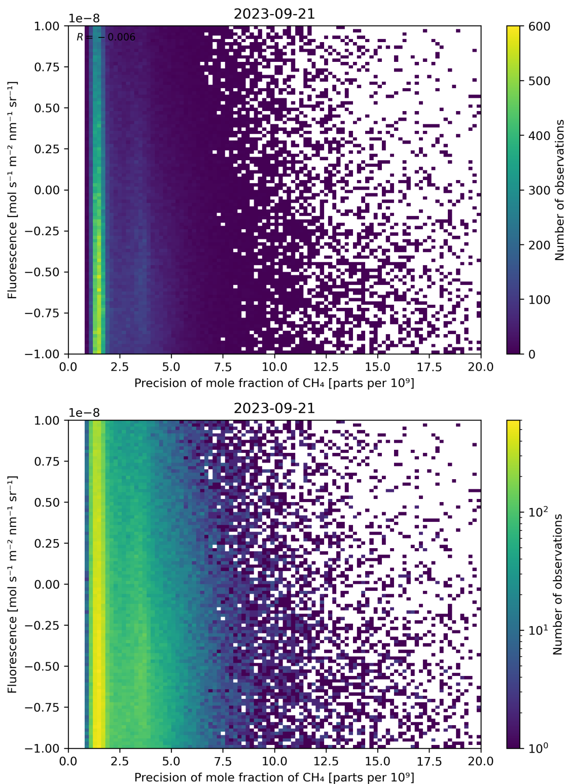
Figure 81: Scatter density plot of “Precision of mole fraction of \text{CH}_4 ” against “Fluorescence” for 2023-09-20 to 2023-09-22.
