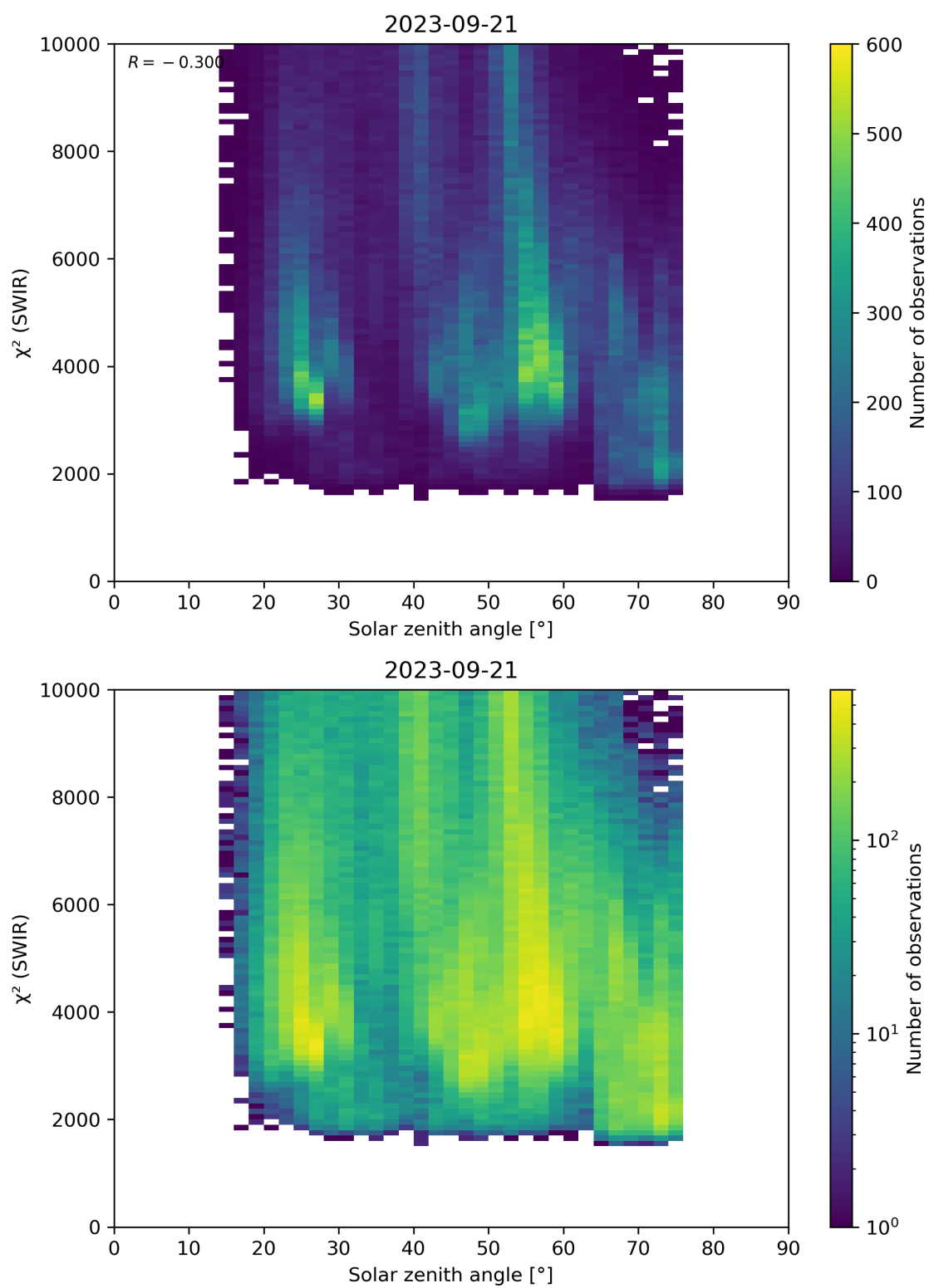
Figure 95: Scatter density plot of “Solar zenith angle” against “ \chi^2 (SWIR)” for 2023-09-20 to 2023-09-22.
