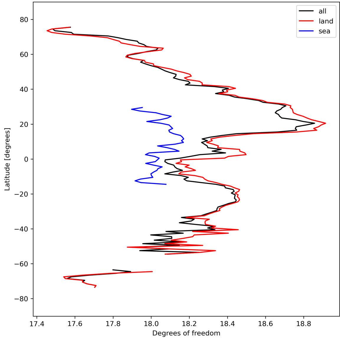
Figure 19: Zonal average of “Degrees of freedom” for 2023-09-20 to 2023-09-22.
