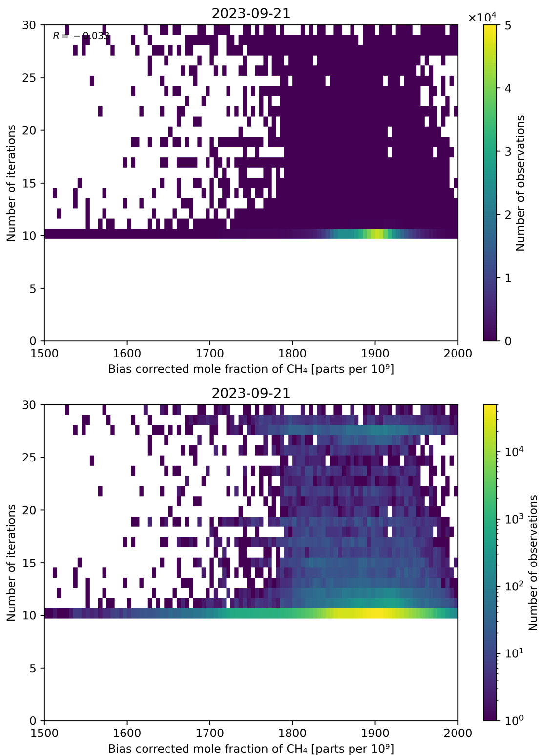
Figure 67: Scatter density plot of “Bias corrected mole fraction of CH 4 ” against “Number of iterations” for 2023-09-20 to 2023-09-22.
