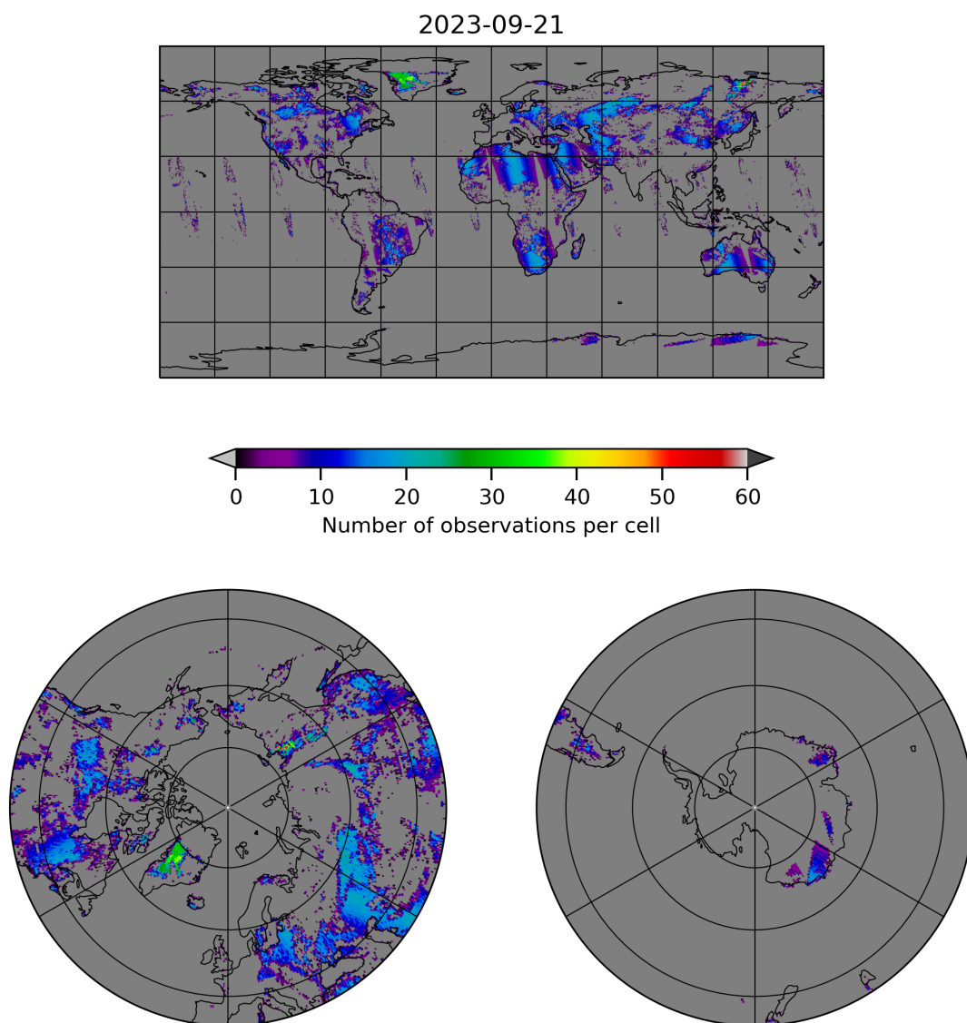
Figure 10: Map of the number of observations for 2023-09-20 to 2023-09-22
