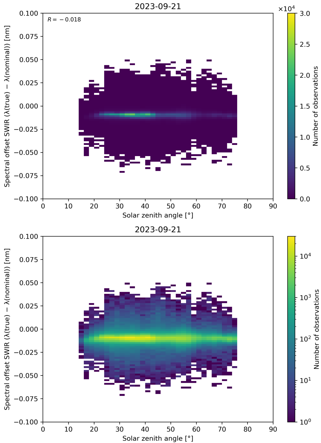
Figure 104: Scatter density plot of “Solar zenith angle” against “Spectral offset SWIR ( \lambda(\text{true}) - \lambda(\text{nominal}) )” for 2023-09-20 to 2023-09-22.
