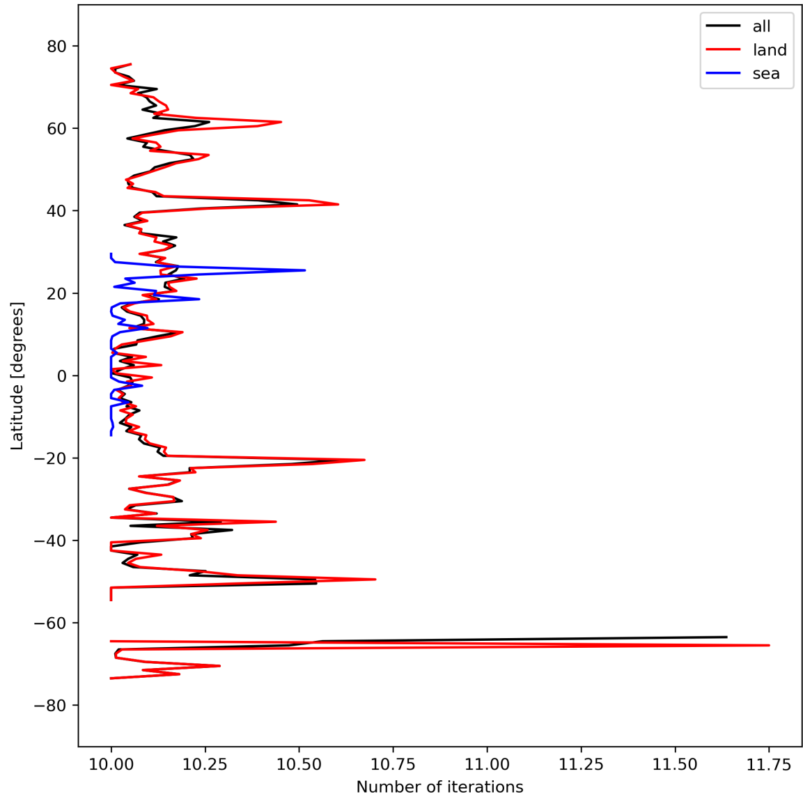
Figure 20: Zonal average of “Number of iterations” for 2023-09-20 to 2023-09-22.
