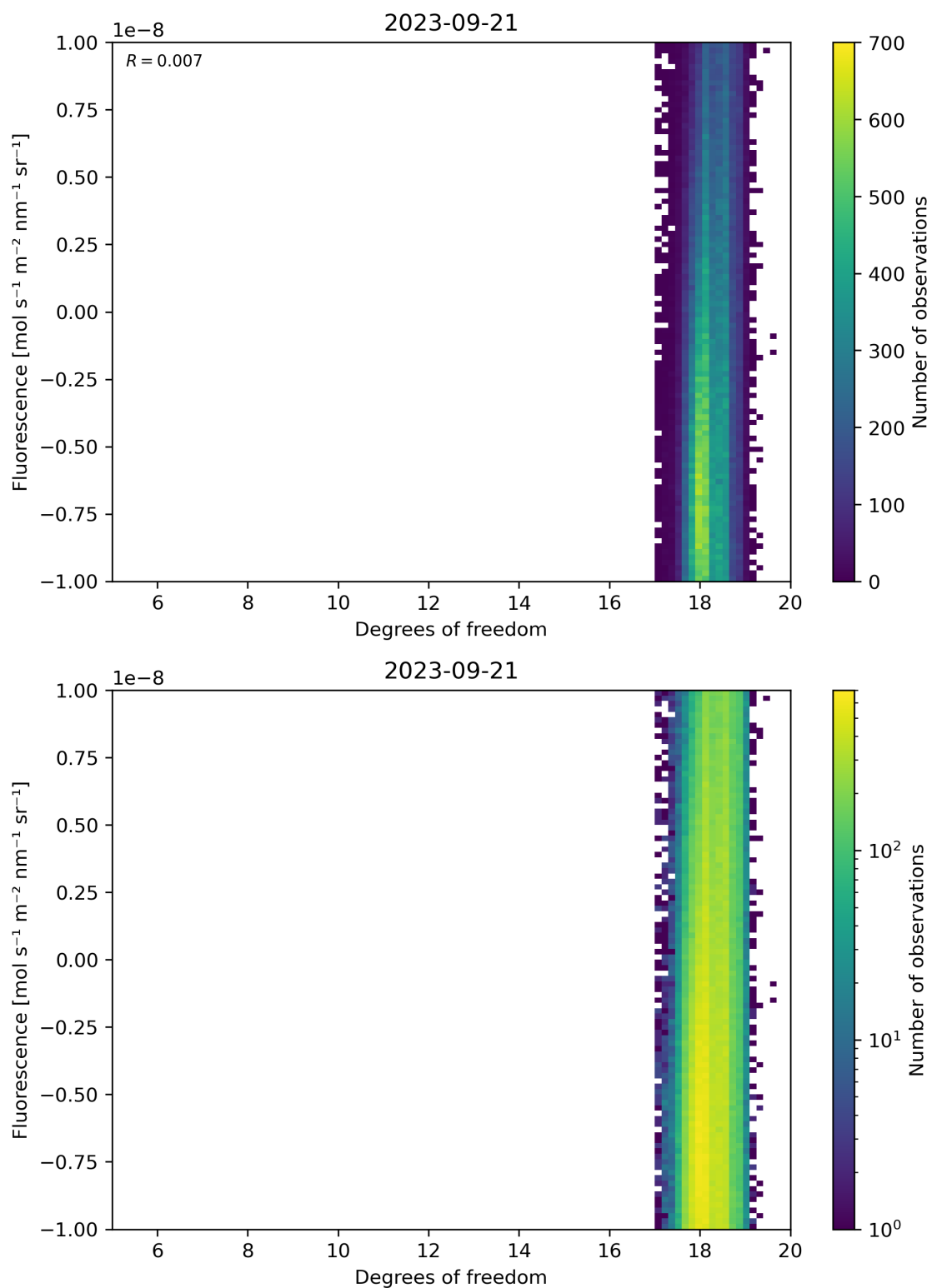
Figure 51: Scatter density plot of “Degrees of freedom” against “Fluorescence” for 2023-09-20 to 2023-09-22.
