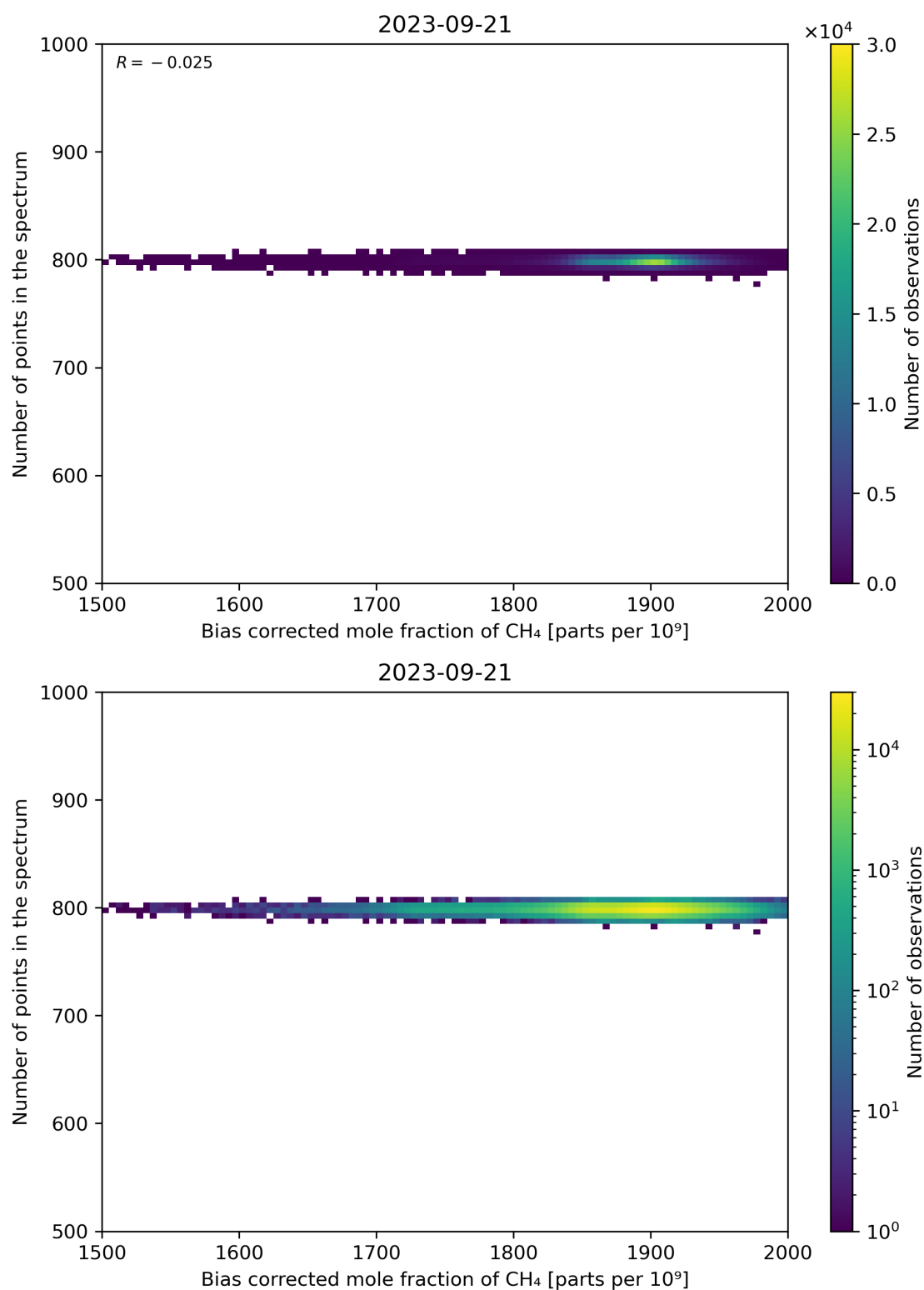
Figure 68: Scatter density plot of “Bias corrected mole fraction of CH 4 ” against “Number of points in the spectrum” for 2023-09-20 to 2023-09-22.
