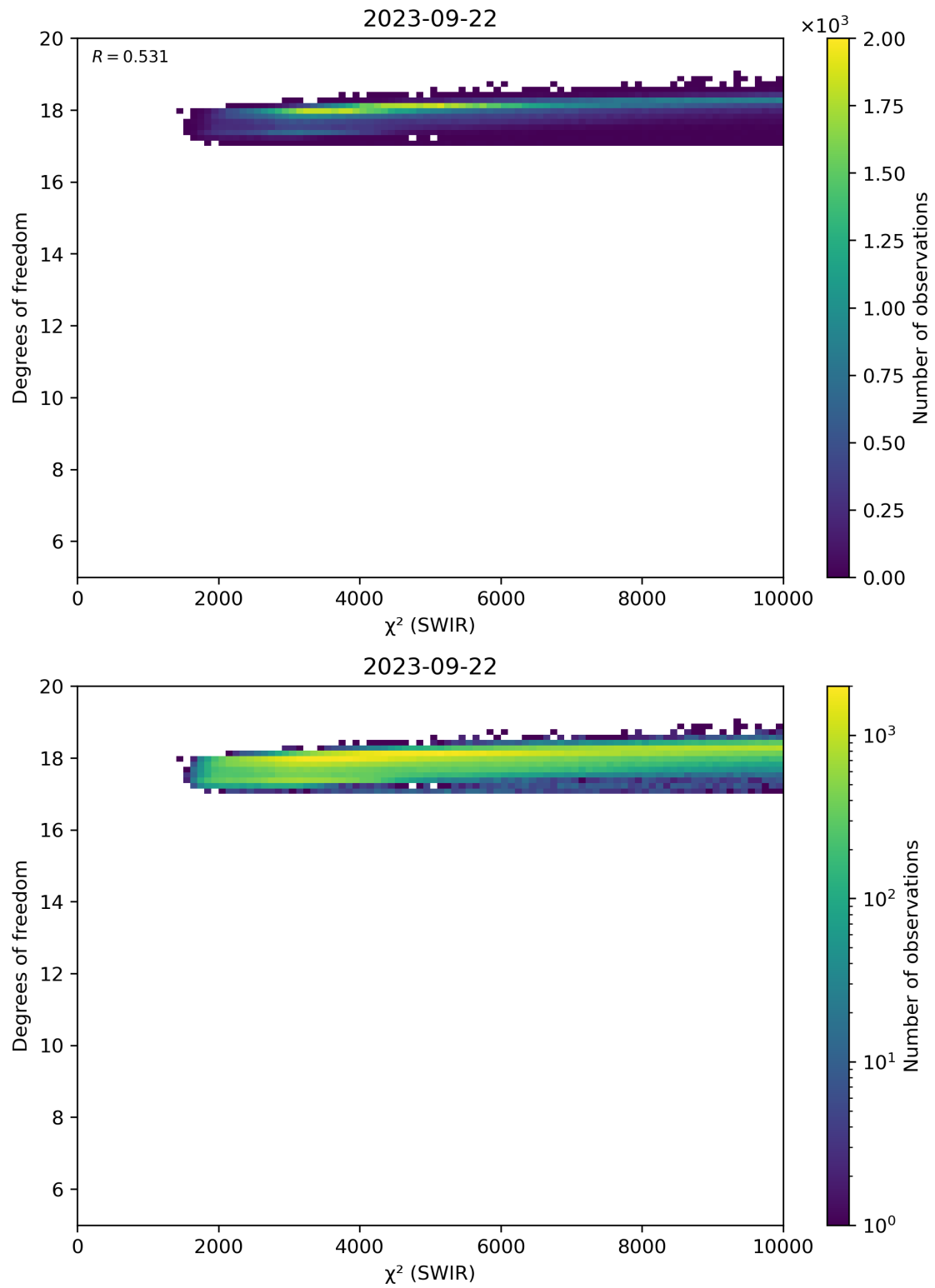
Figure 48: Scatter density plot of “ \chi^2 (SWIR)” against “Degrees of freedom” for 2023-09-21 to 2023-09-23.
