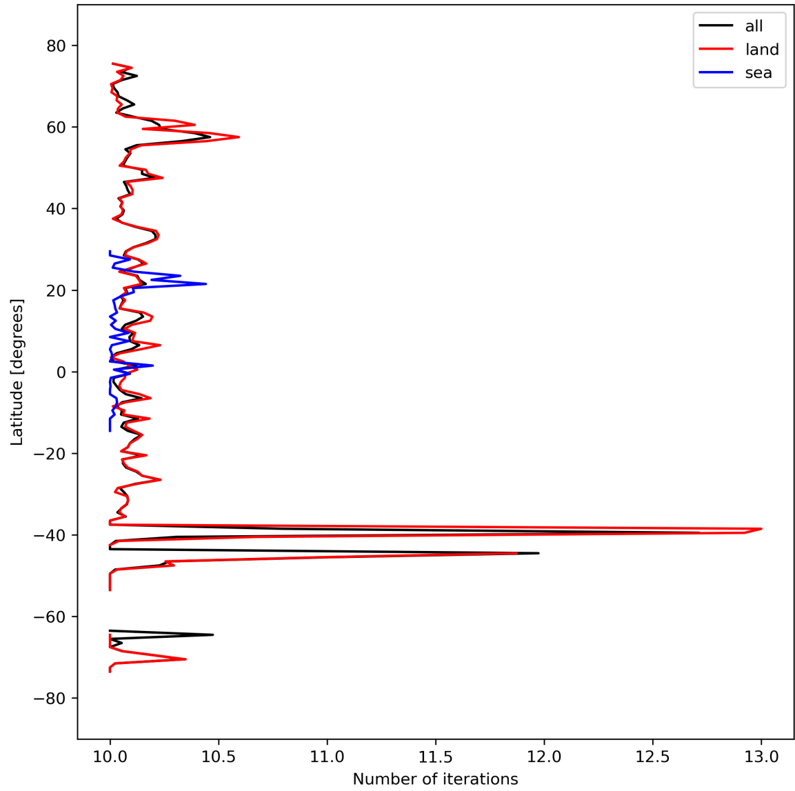
Figure 20: Zonal average of “Number of iterations” for 2023-09-21 to 2023-09-23.
