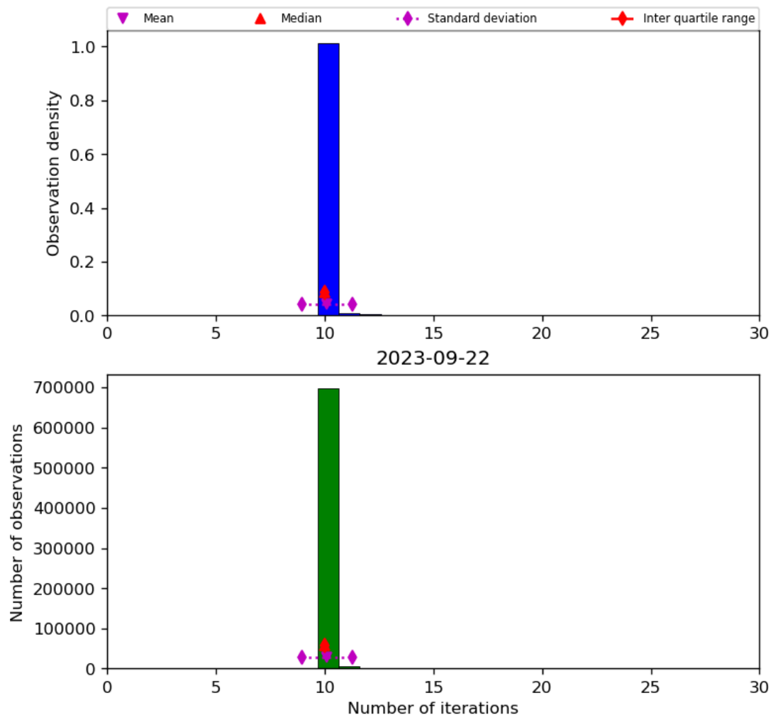
Figure 31: Histogram of “Number of iterations” for 2023-09-21 to 2023-09-23
