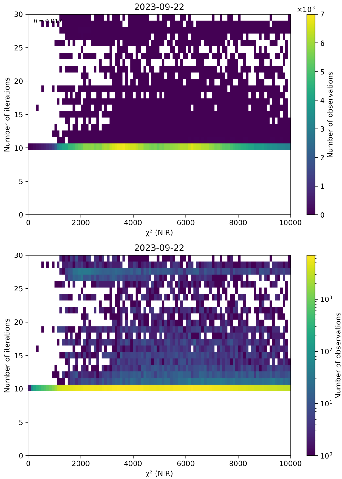
Figure 46: Scatter density plot of “ \chi^2 (NIR)” against “Number of iterations” for 2023-09-21 to 2023-09-23.
