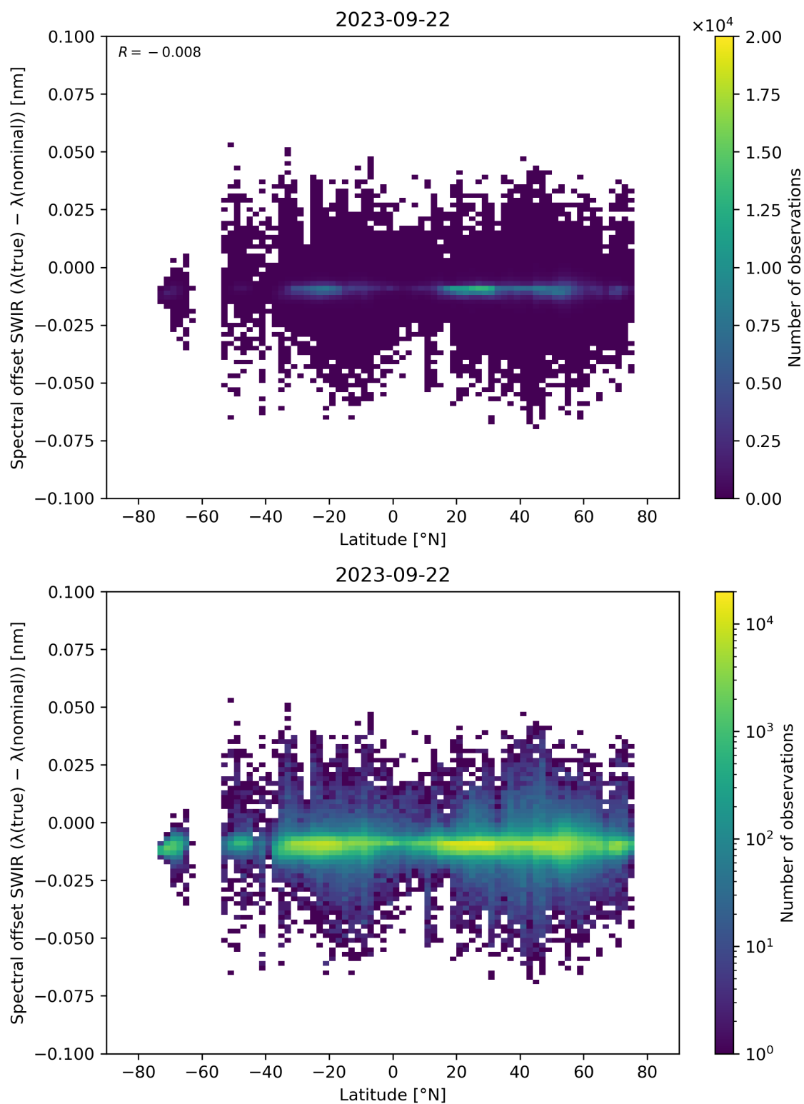
Figure 62: Scatter density plot of “Latitude” against “Spectral offset SWIR ( \lambda(\text{true}) - \lambda(\text{nominal}) )” for 2023-09-21 to 2023-09-23.
