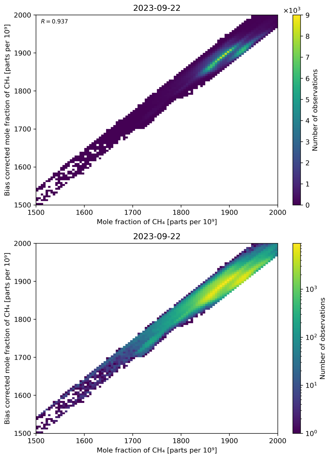
Figure 74: Scatter density plot of “Mole fraction of CH 4 ” against “Bias corrected mole fraction of CH 4 ” for 2023-09-21 to 2023-09-23.
