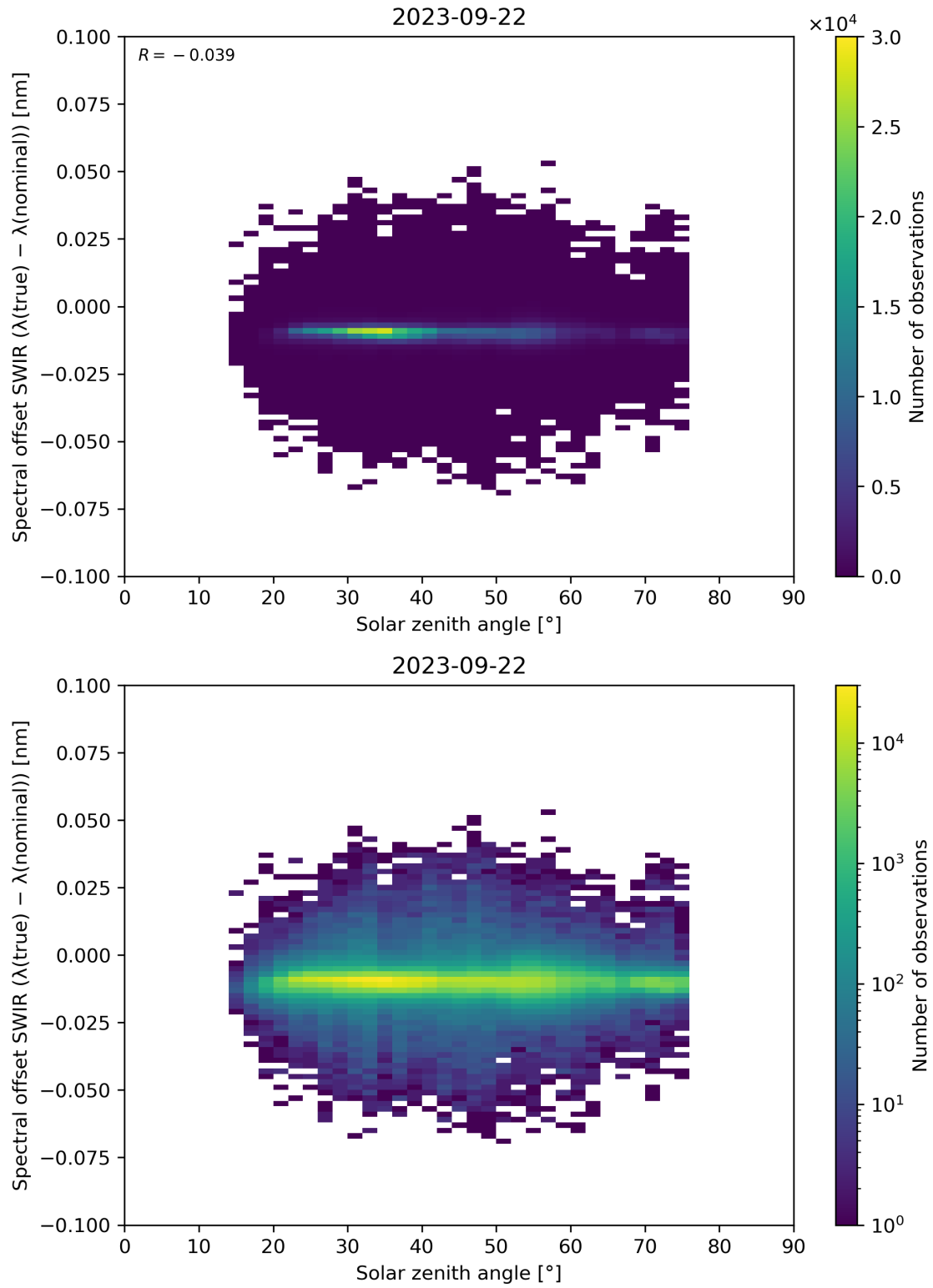
Figure 104: Scatter density plot of “Solar zenith angle” against “Spectral offset SWIR ( \lambda(\text{true}) - \lambda(\text{nominal}) )” for 2023-09-21 to 2023-09-23.
