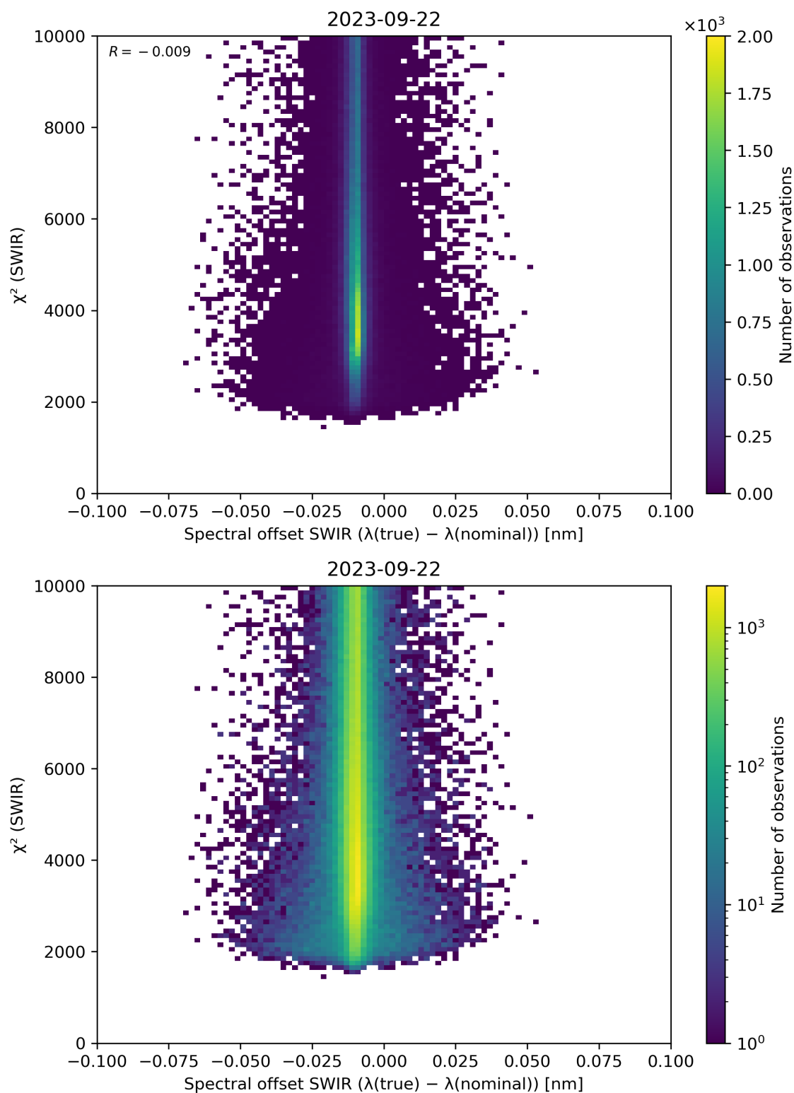
Figure 118: Scatter density plot of “Spectral offset SWIR ( \lambda(\text{true}) - \lambda(\text{nominal}) )” against “ \chi^2 (SWIR)” for 2023-09-21 to 2023-09-23.
