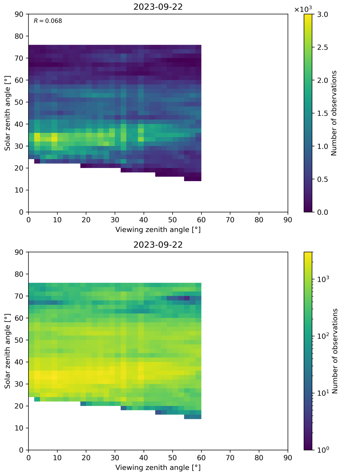
Figure 115: Scatter density plot of “Viewing zenith angle” against “Solar zenith angle” for 2023-09-21 to 2023-09-23.
