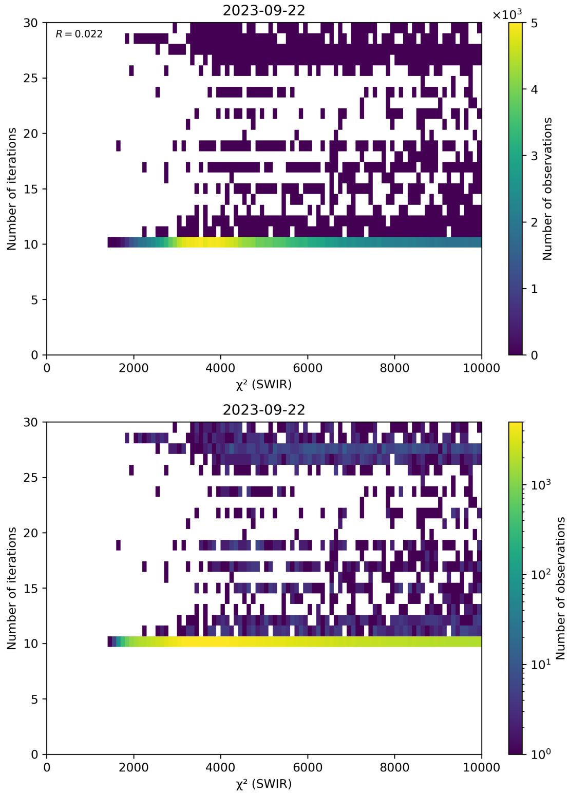
Figure 50: Scatter density plot of “ \chi^2 (SWIR)” against “Number of iterations” for 2023-09-21 to 2023-09-23.
