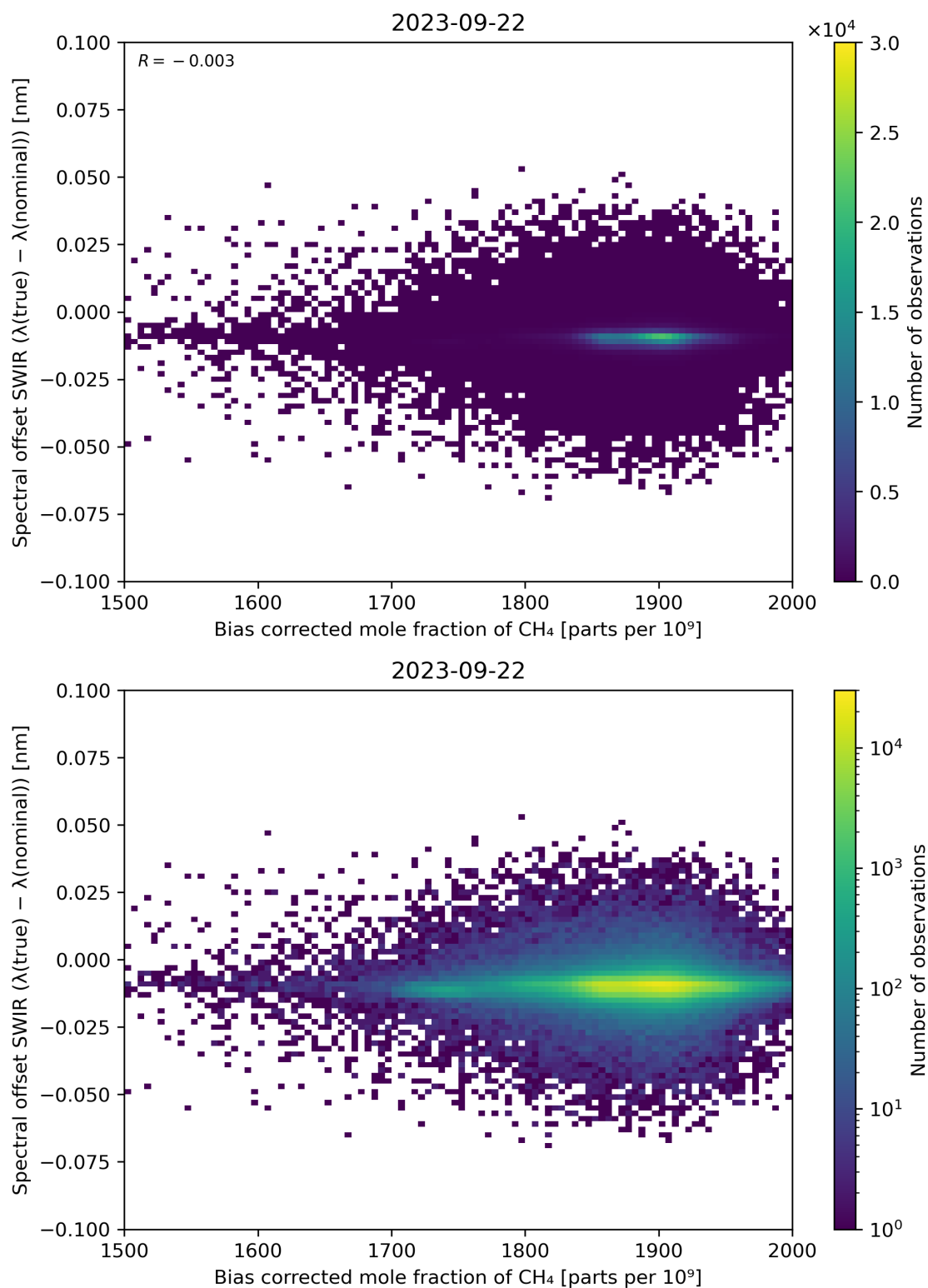
Figure 69: Scatter density plot of “Bias corrected mole fraction of \text{CH}_4 ” against “Spectral offset SWIR ( \lambda(\text{true}) - \lambda(\text{nominal}) )” for 2023-09-21 to 2023-09-23.
