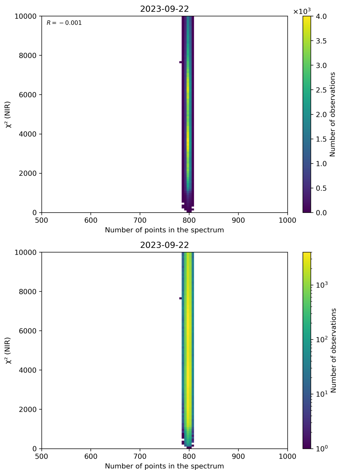
Figure 88: Scatter density plot of “Number of points in the spectrum” against “ \chi^2 (NIR)” for 2023-09-21 to 2023-09-23.
