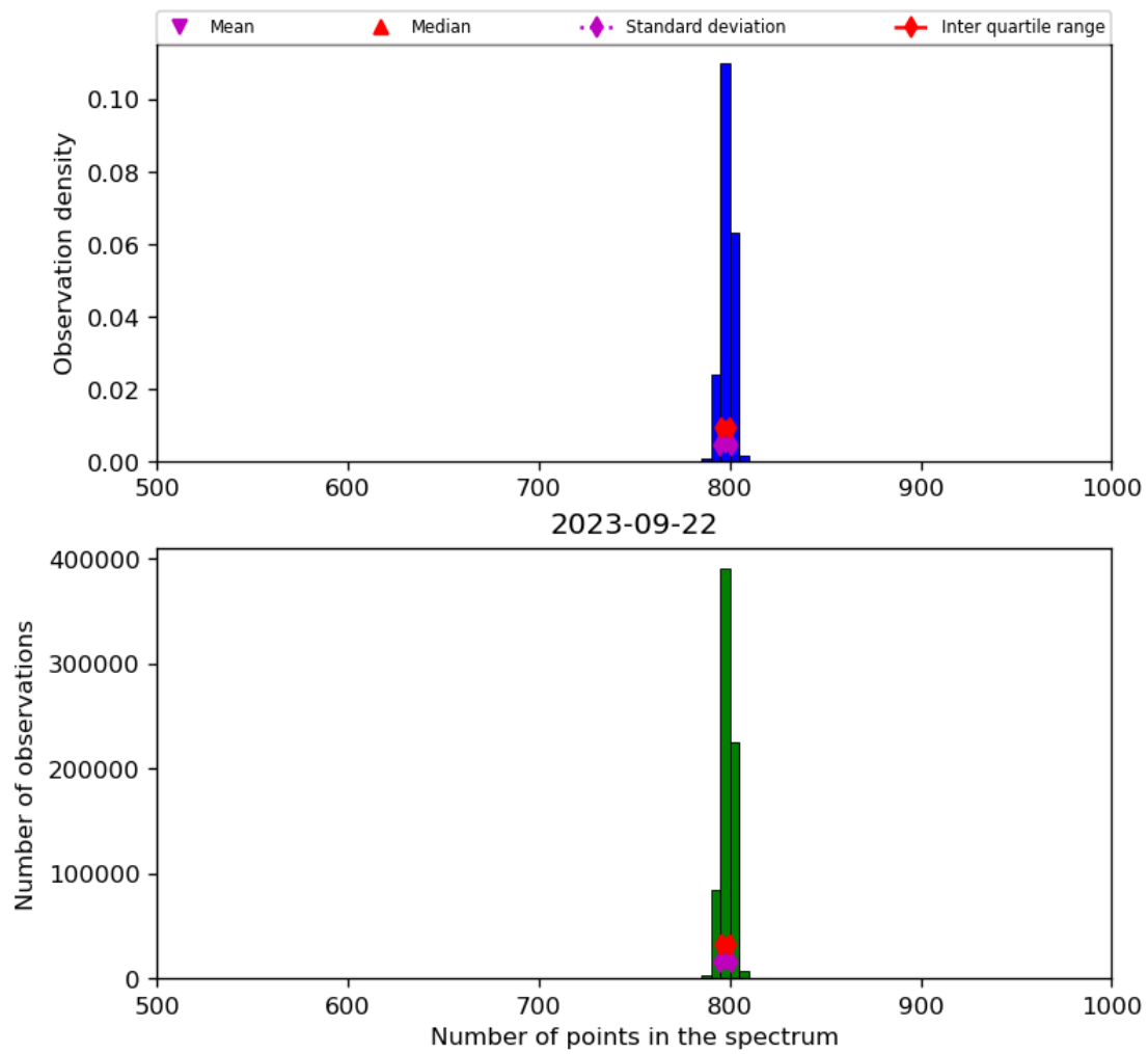
Figure 26: Histogram of “Number of points in the spectrum” for 2023-09-21 to 2023-09-23
