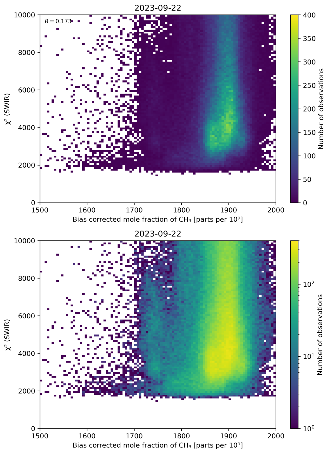
Figure 64: Scatter density plot of “Bias corrected mole fraction of \text{CH}_4 ” against “ \chi^2 (SWIR)” for 2023-09-21 to 2023-09-23.
