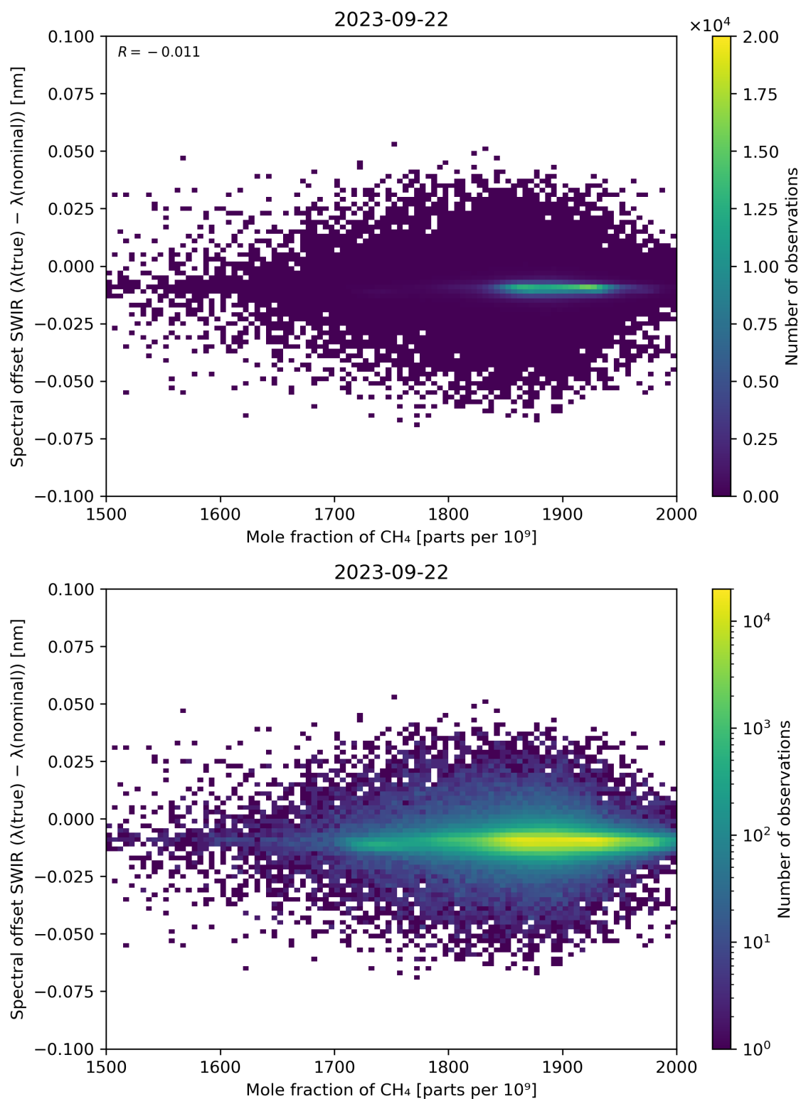
Figure 86: Scatter density plot of “Mole fraction of CH 4 ” against “Spectral offset SWIR ( \lambda(\text{true}) - \lambda(\text{nominal}) )” for 2023-09-21 to 2023-09-23.
