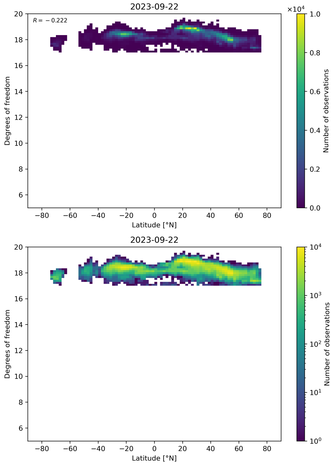
Figure 55: Scatter density plot of “Latitude” against “Degrees of freedom” for 2023-09-21 to 2023-09-23.
