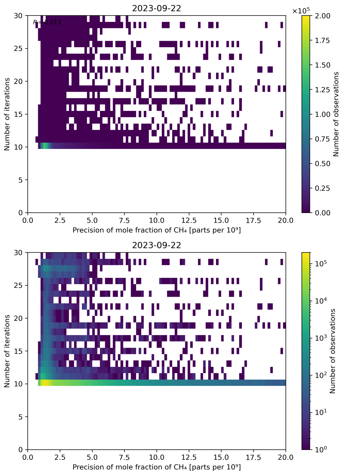
Figure 83: Scatter density plot of “Precision of mole fraction of CH 4 ” against “Number of iterations” for 2023-09-21 to 2023-09-23.
