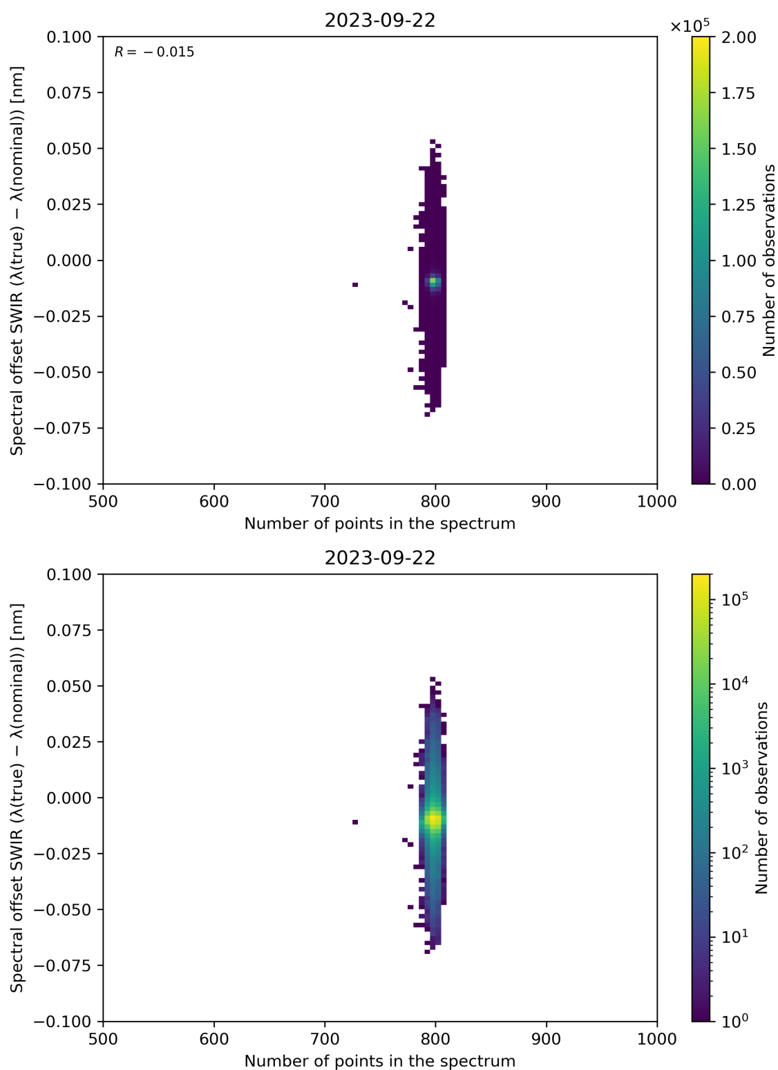
Figure 93: Scatter density plot of “Number of points in the spectrum” against “Spectral offset SWIR ( \lambda(\text{true}) - \lambda(\text{nominal}) )” for 2023-09-21 to 2023-09-23.
