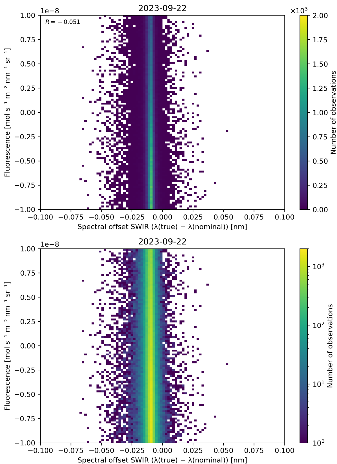
Figure 120: Scatter density plot of “Spectral offset SWIR ( \lambda(\text{true}) - \lambda(\text{nominal}) )” against “Fluorescence” for 2023-09-21 to 2023-09-23.
