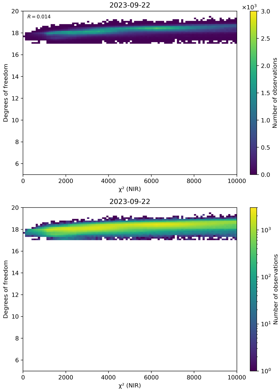
Figure 44: Scatter density plot of “ \chi^2 (NIR)” against “Degrees of freedom” for 2023-09-21 to 2023-09-23.
