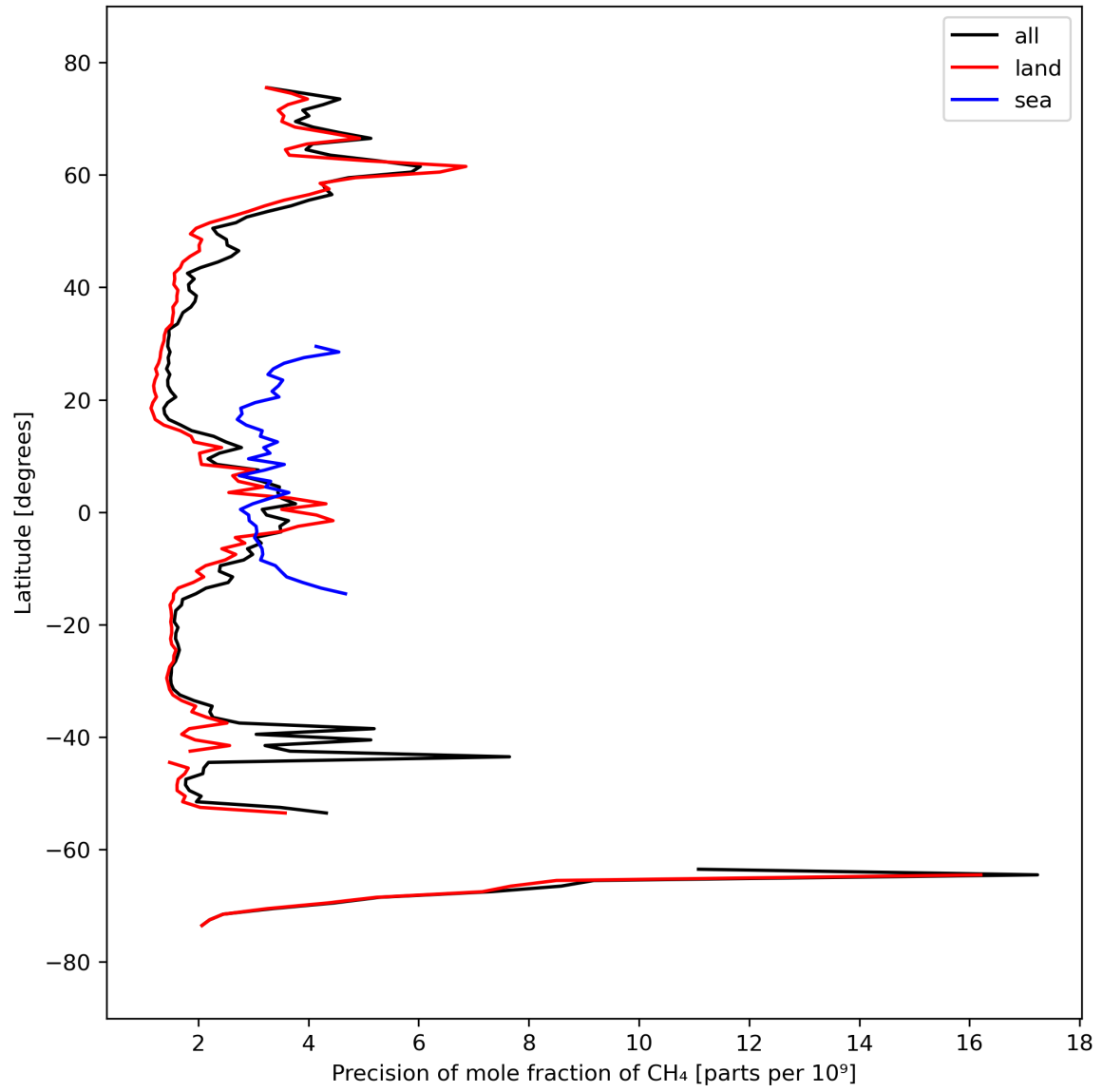
Figure 13: Zonal average of “Precision of mole fraction of CH 4 ” for 2023-09-21 to 2023-09-23.
