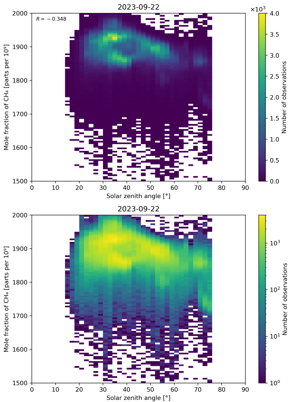
Figure 99: Scatter density plot of “Solar zenith angle” against “Mole fraction of \text{CH}_4 ” for 2023-09-21 to 2023-09-23.
