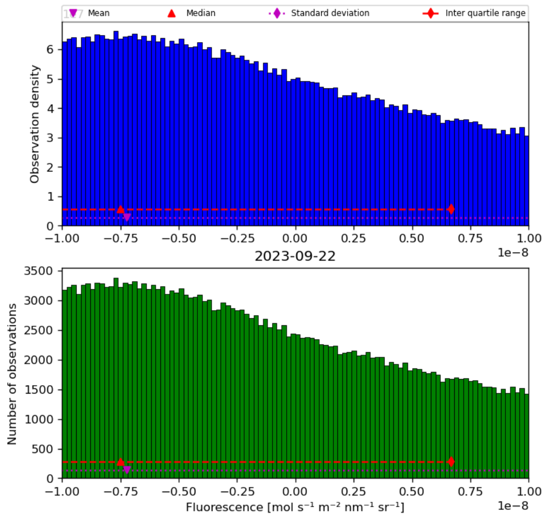
Figure 32: Histogram of “Fluorescence” for 2023-09-21 to 2023-09-23
