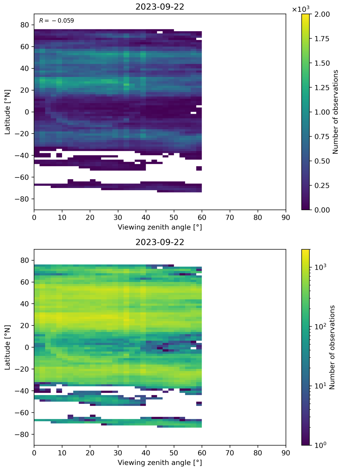
Figure 109: Scatter density plot of “Viewing zenith angle” against “Latitude” for 2023-09-21 to 2023-09-23.
