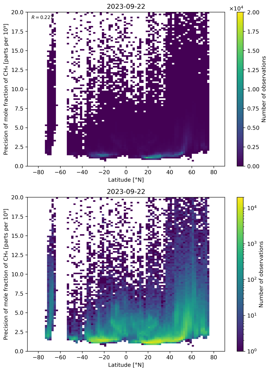
Figure 59: Scatter density plot of “Latitude” against “Precision of mole fraction of \text{CH}_4 ” for 2023-09-21 to 2023-09-23.
