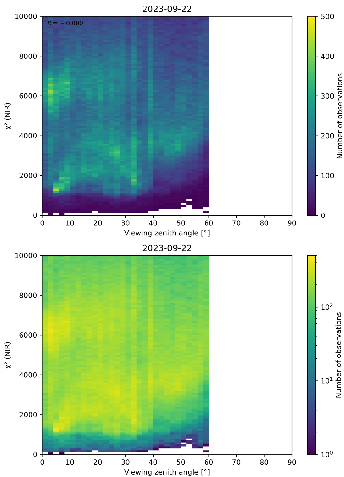
Figure 105: Scatter density plot of “Viewing zenith angle” against “ \chi^2 (NIR)” for 2023-09-21 to 2023-09-23.
