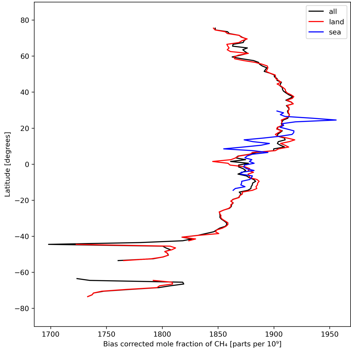
Figure 14: Zonal average of “Bias corrected mole fraction of CH 4 ” for 2023-09-21 to 2023-09-23.
