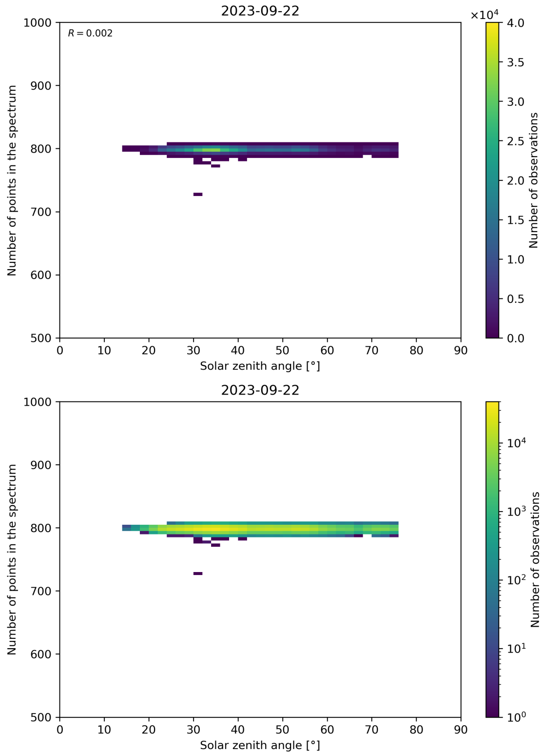
Figure 103: Scatter density plot of “Solar zenith angle” against “Number of points in the spectrum” for 2023-09-21 to 2023-09-23.
