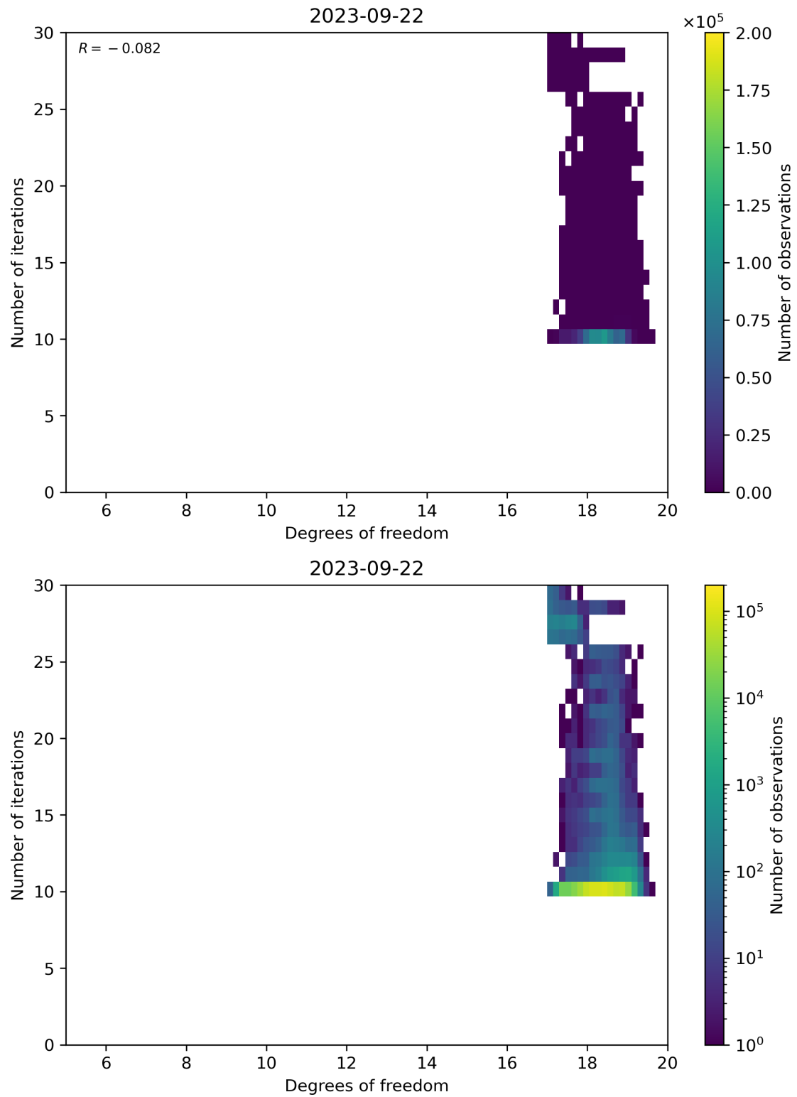
Figure 52: Scatter density plot of “Degrees of freedom” against “Number of iterations” for 2023-09-21 to 2023-09-23.
