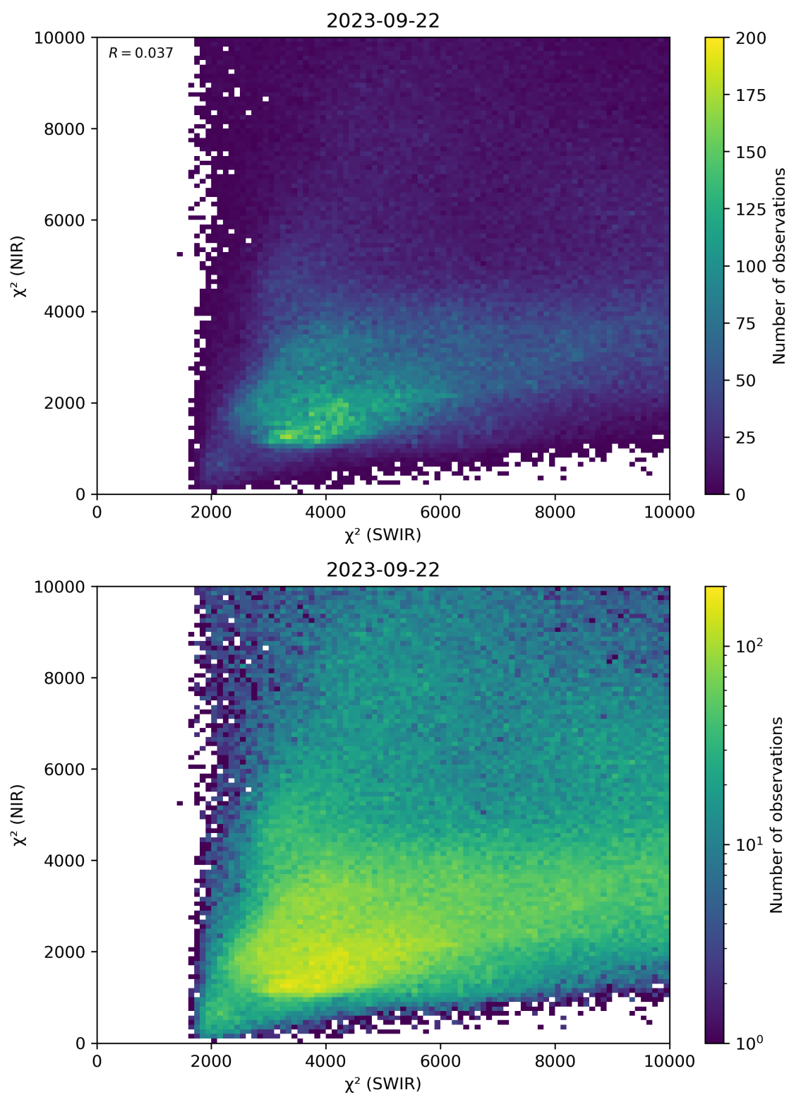
Figure 47: Scatter density plot of “ \chi^2 (SWIR)” against “ \chi^2 (NIR)” for 2023-09-21 to 2023-09-23.
