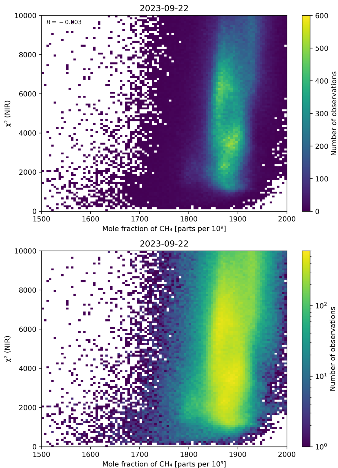
Figure 70: Scatter density plot of “Mole fraction of CH 4 ” against “ \chi^2 (NIR)” for 2023-09-21 to 2023-09-23.
