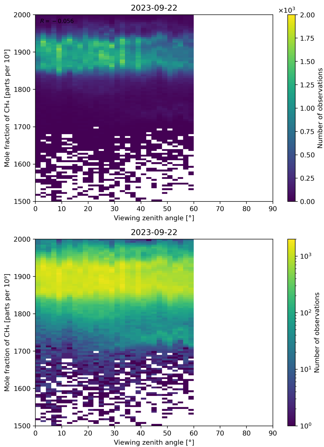
Figure 110: Scatter density plot of “Viewing zenith angle” against “Mole fraction of CH 4 ” for 2023-09-21 to 2023-09-23.
