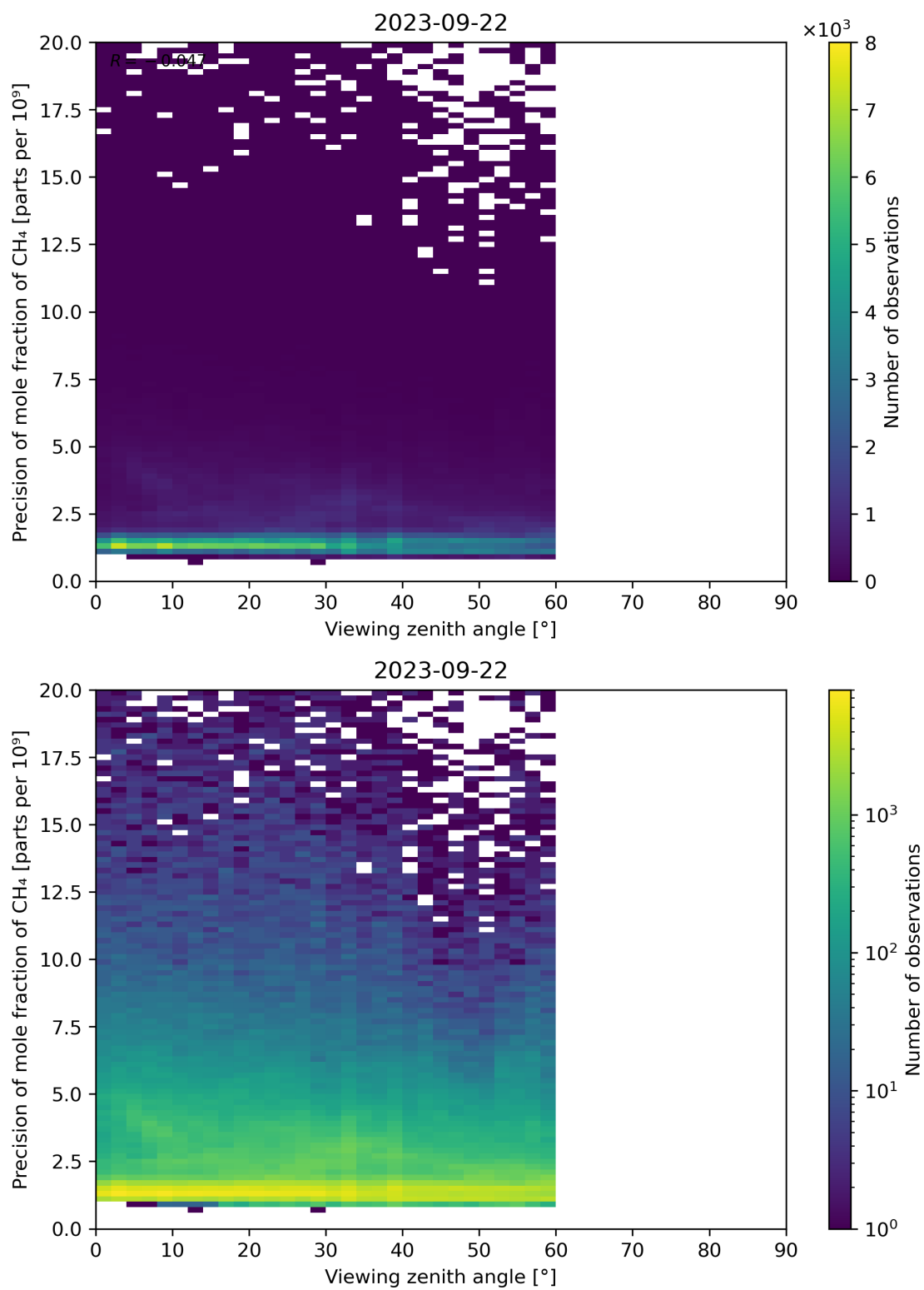
Figure 112: Scatter density plot of “Viewing zenith angle” against “Precision of mole fraction of CH 4 ” for 2023-09-21 to 2023-09-23.
