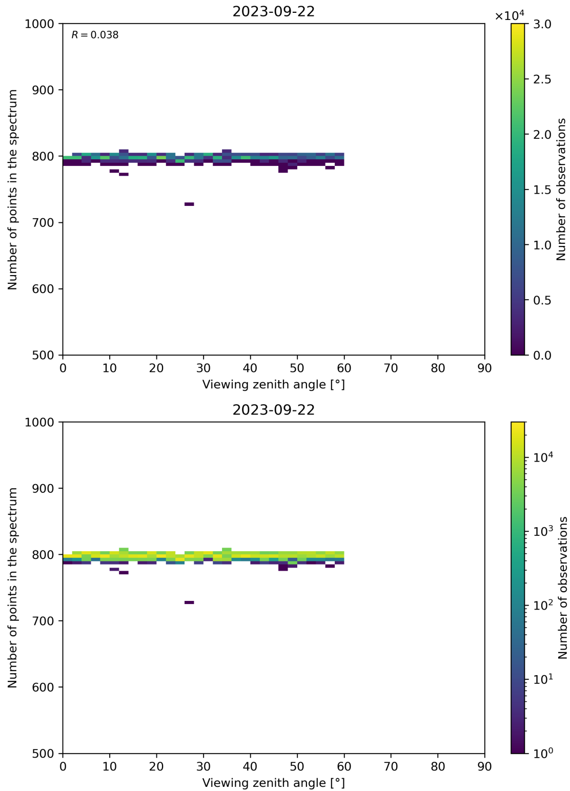
Figure 114: Scatter density plot of “Viewing zenith angle” against “Number of points in the spectrum” for 2023-09-21 to 2023-09-23.
