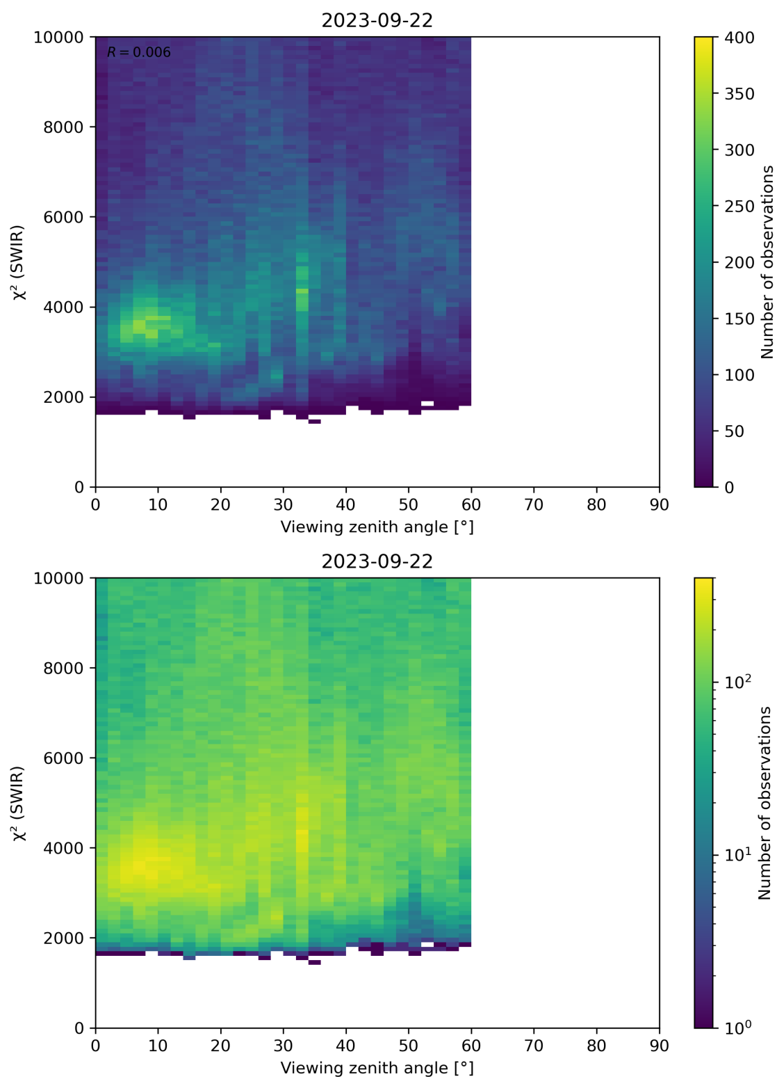
Figure 106: Scatter density plot of “Viewing zenith angle” against “ \chi^2 (SWIR)” for 2023-09-21 to 2023-09-23.
