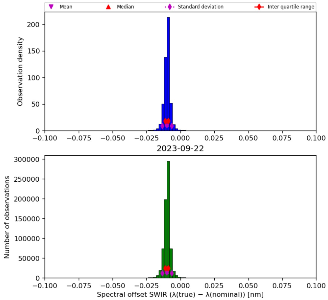
Figure 27: Histogram of “Spectral offset SWIR ( \lambda(\text{true}) - \lambda(\text{nominal}) )” for 2023-09-21 to 2023-09-23
