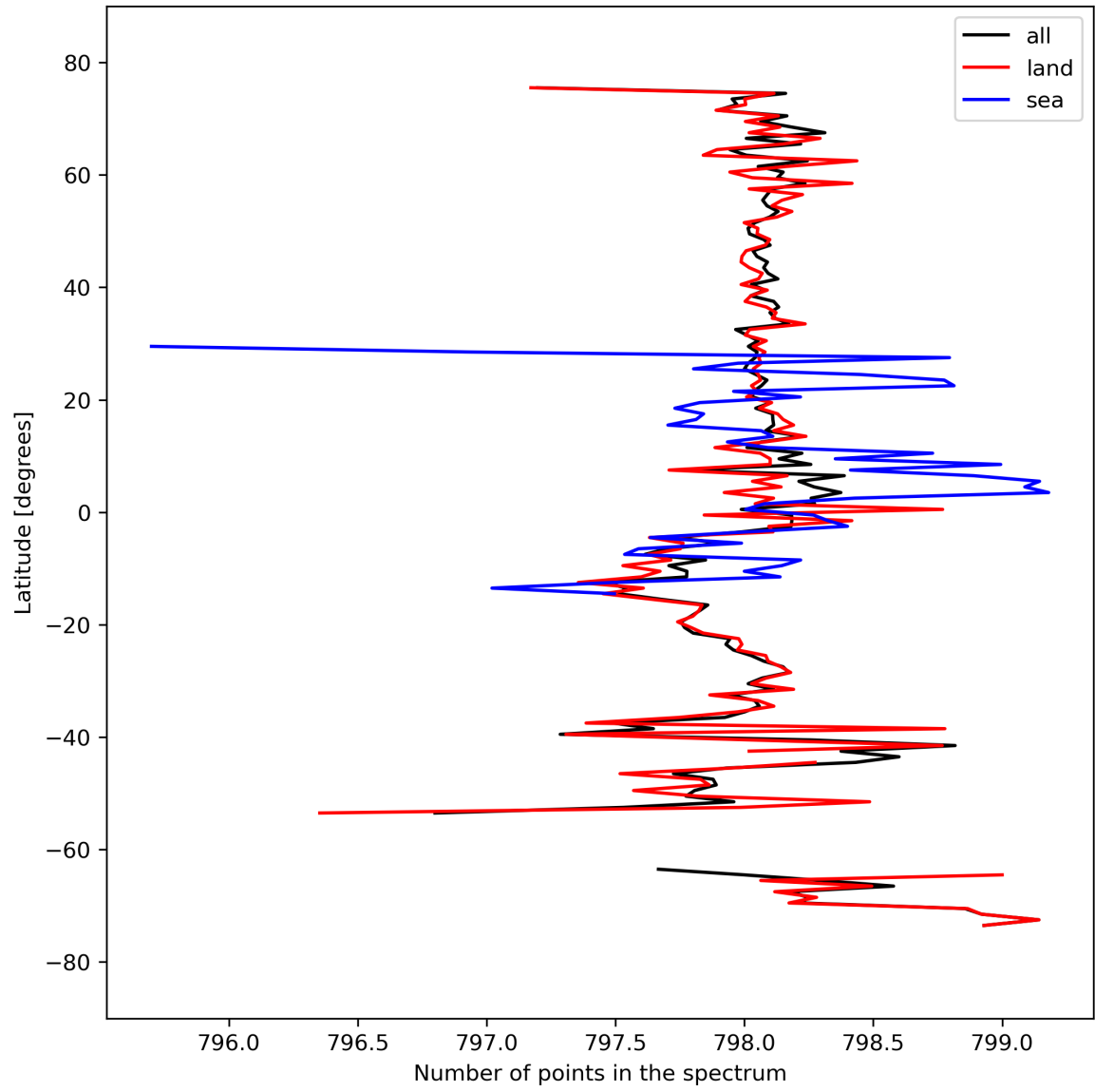
Figure 15: Zonal average of “Number of points in the spectrum” for 2023-09-21 to 2023-09-23.
