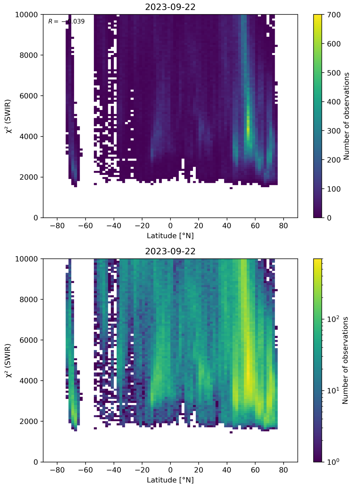
Figure 54: Scatter density plot of “Latitude” against “ \chi^2 (SWIR)” for 2023-09-21 to 2023-09-23.
