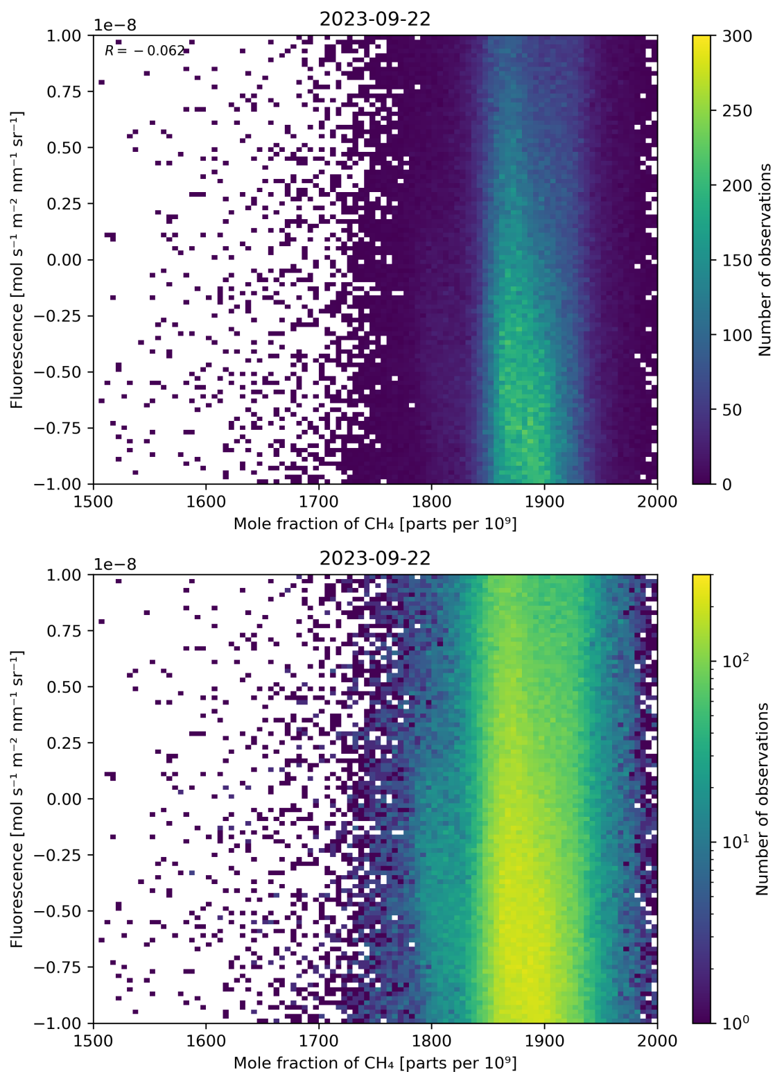
Figure 73: Scatter density plot of “Mole fraction of \text{CH}_4 ” against “Fluorescence” for 2023-09-21 to 2023-09-23.
