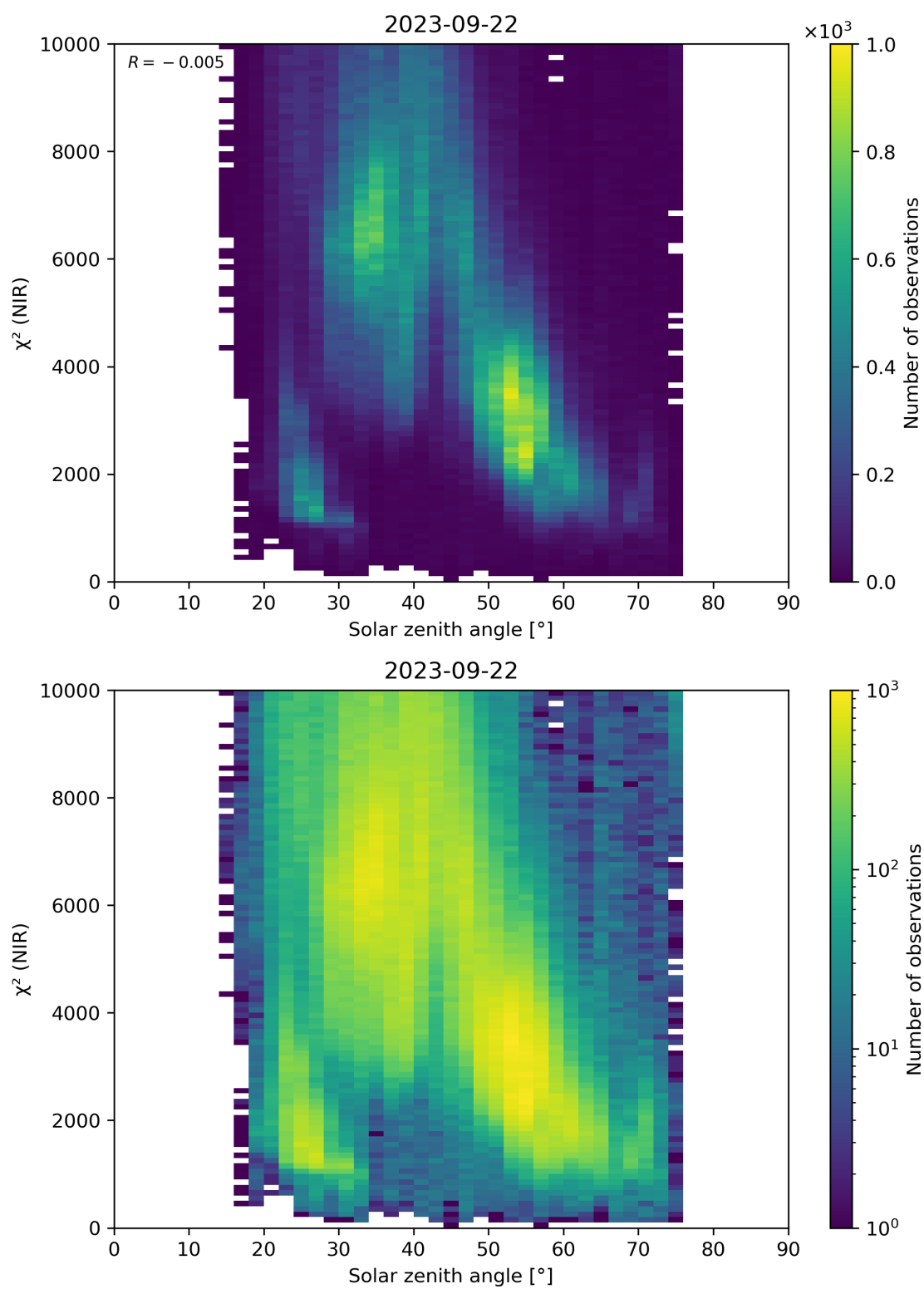
Figure 94: Scatter density plot of “Solar zenith angle” against “ \chi^2 (NIR)” for 2023-09-21 to 2023-09-23.
