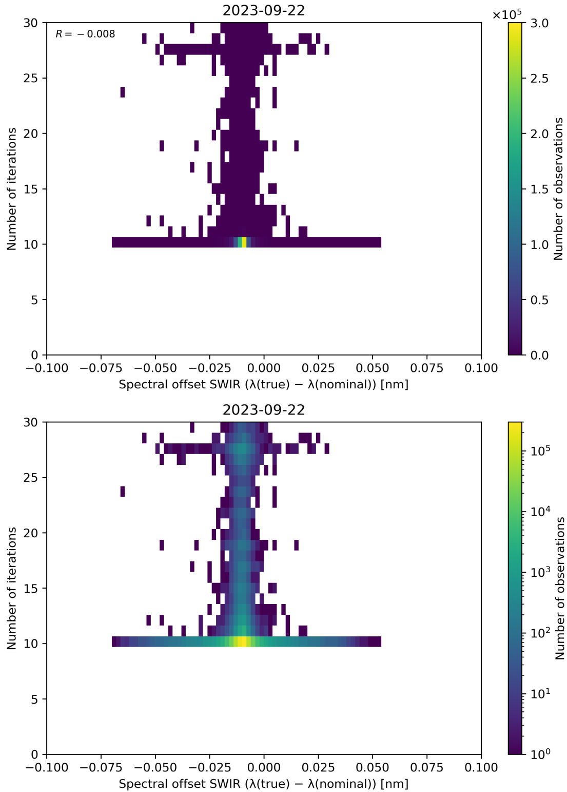
Figure 121: Scatter density plot of “Spectral offset SWIR ( \lambda(\text{true}) - \lambda(\text{nominal}) )” against “Number of iterations” for 2023-09-21 to 2023-09-23.
