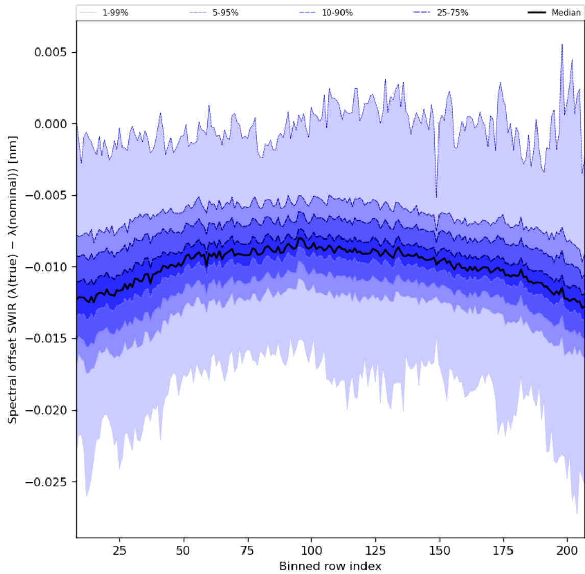
Figure 38: Along track statistics of “Spectral offset SWIR ( \lambda(\text{true}) - \lambda(\text{nominal}) )” for 2023-09-21 to 2023-09-23
