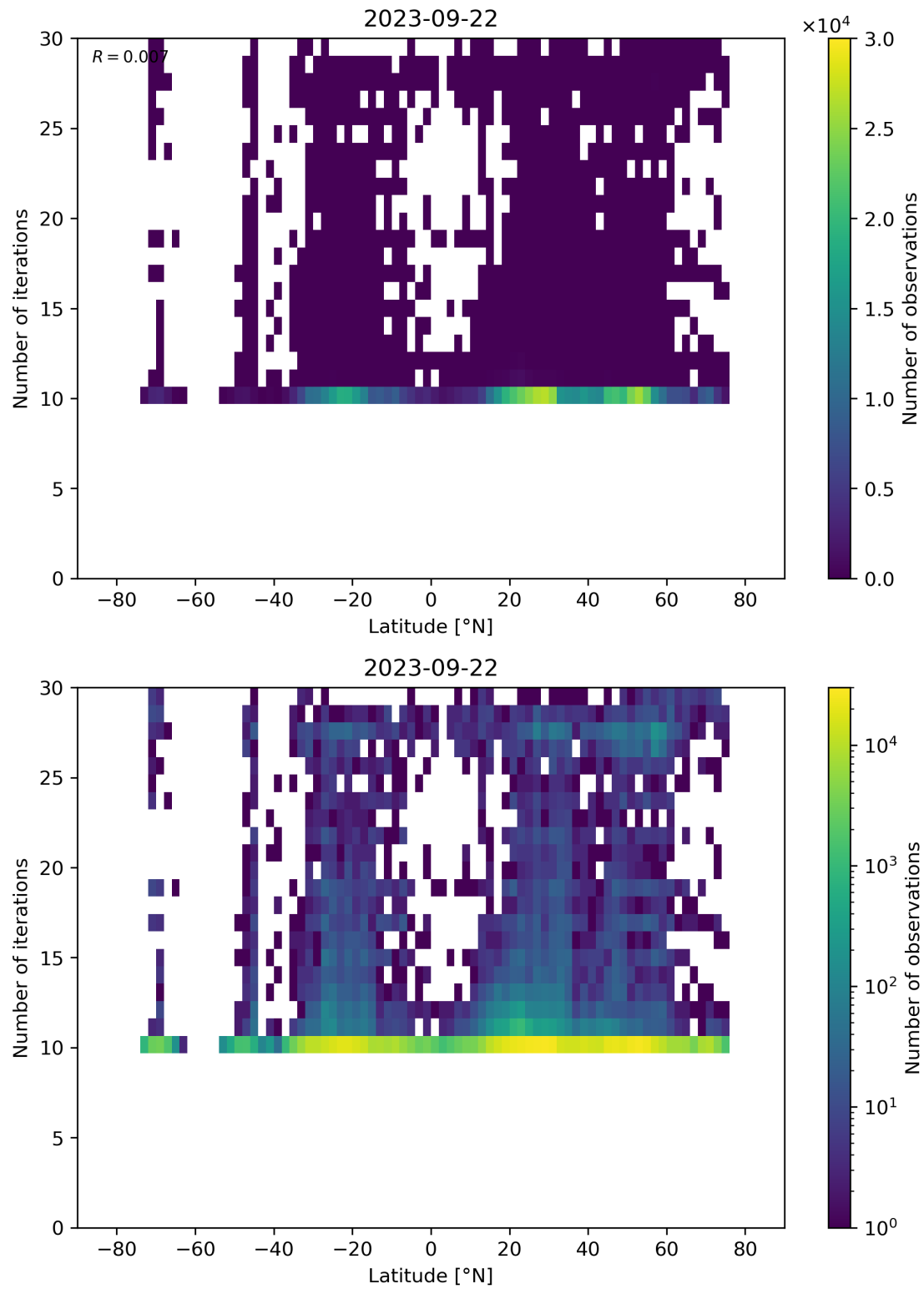
Figure 60: Scatter density plot of “Latitude” against “Number of iterations” for 2023-09-21 to 2023-09-23.
