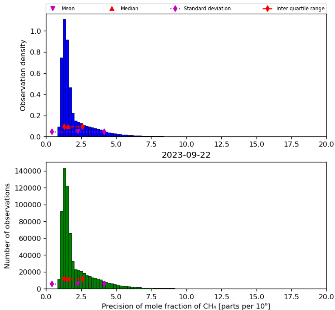
Figure 24: Histogram of “Precision of mole fraction of CH 4 ” for 2023-09-21 to 2023-09-23
