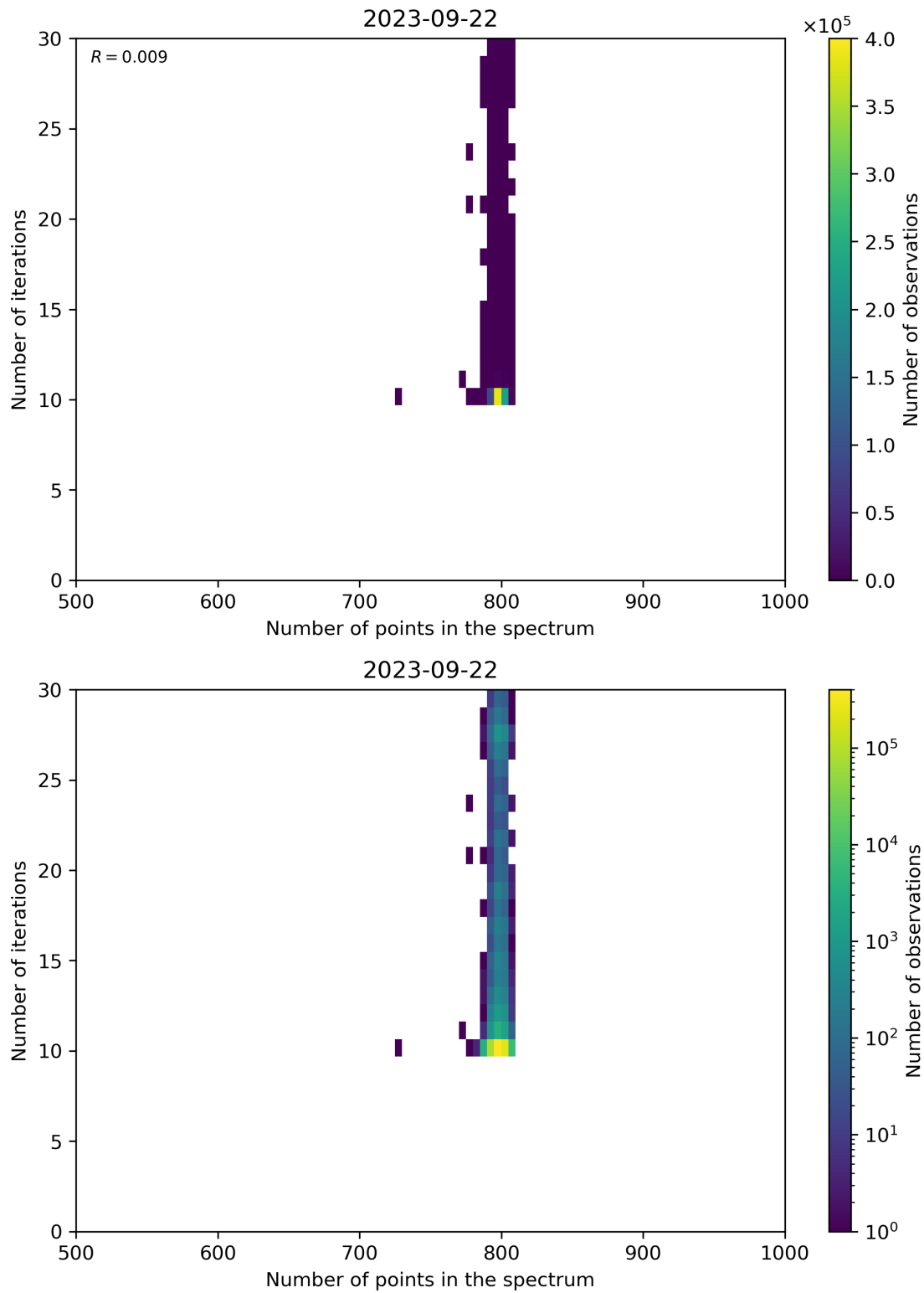
Figure 92: Scatter density plot of “Number of points in the spectrum” against “Number of iterations” for 2023-09-21 to 2023-09-23.
