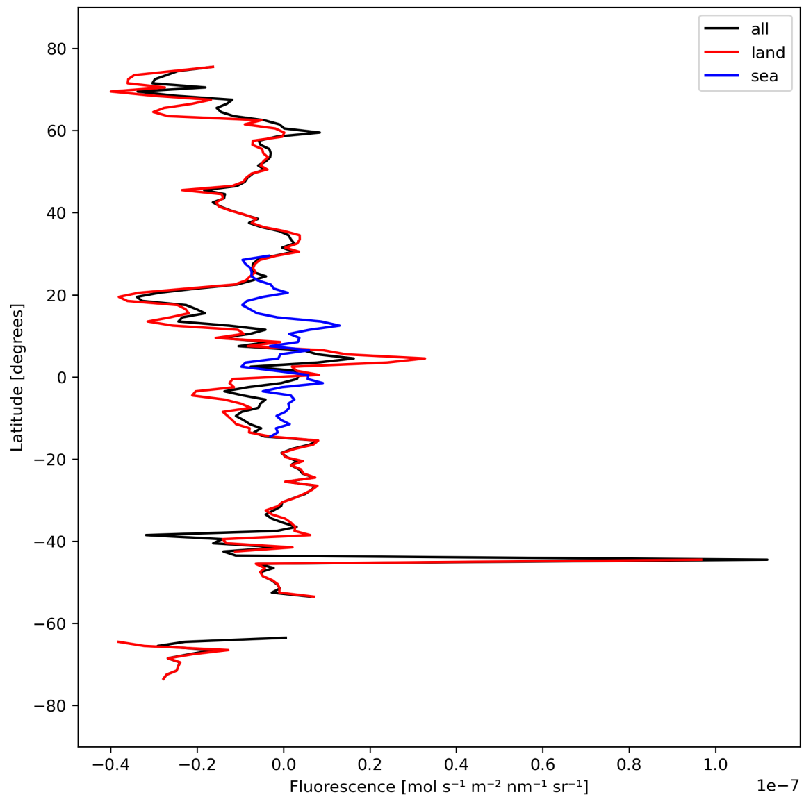
Figure 21: Zonal average of “Fluorescence” for 2023-09-21 to 2023-09-23.
