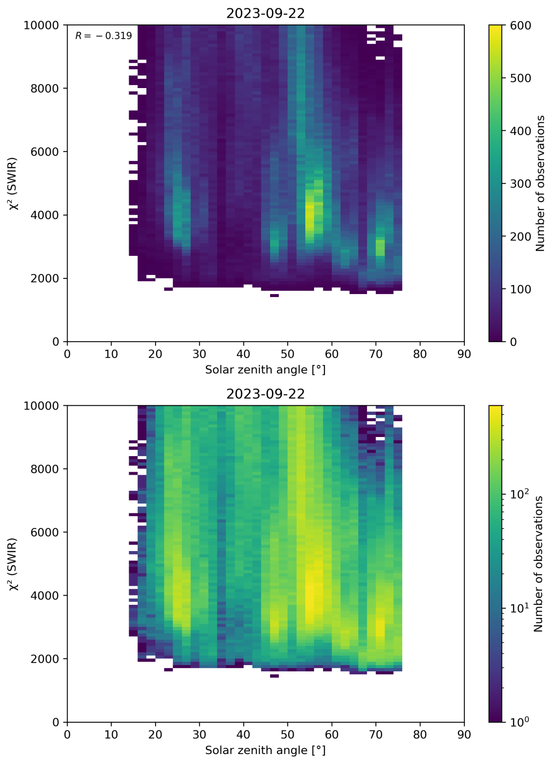
Figure 95: Scatter density plot of “Solar zenith angle” against “ \chi^2 (SWIR)” for 2023-09-21 to 2023-09-23.
