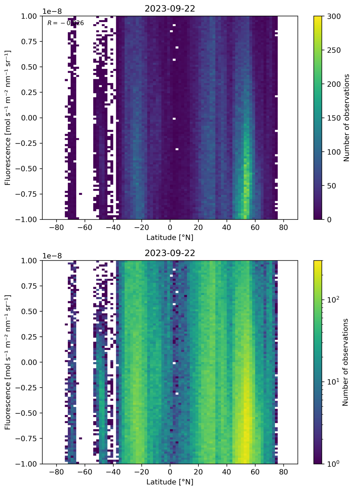
Figure 56: Scatter density plot of “Latitude” against “Fluorescence” for 2023-09-21 to 2023-09-23.
