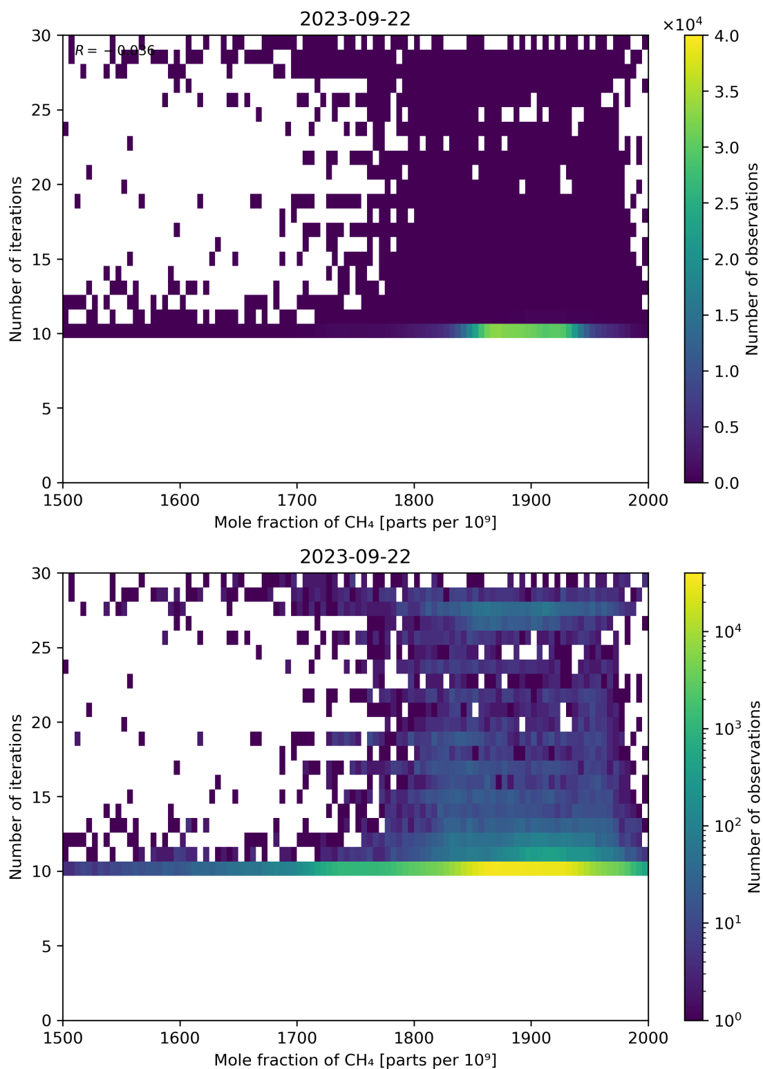
Figure 76: Scatter density plot of “Mole fraction of CH 4 ” against “Number of iterations” for 2023-09-21 to 2023-09-23.
