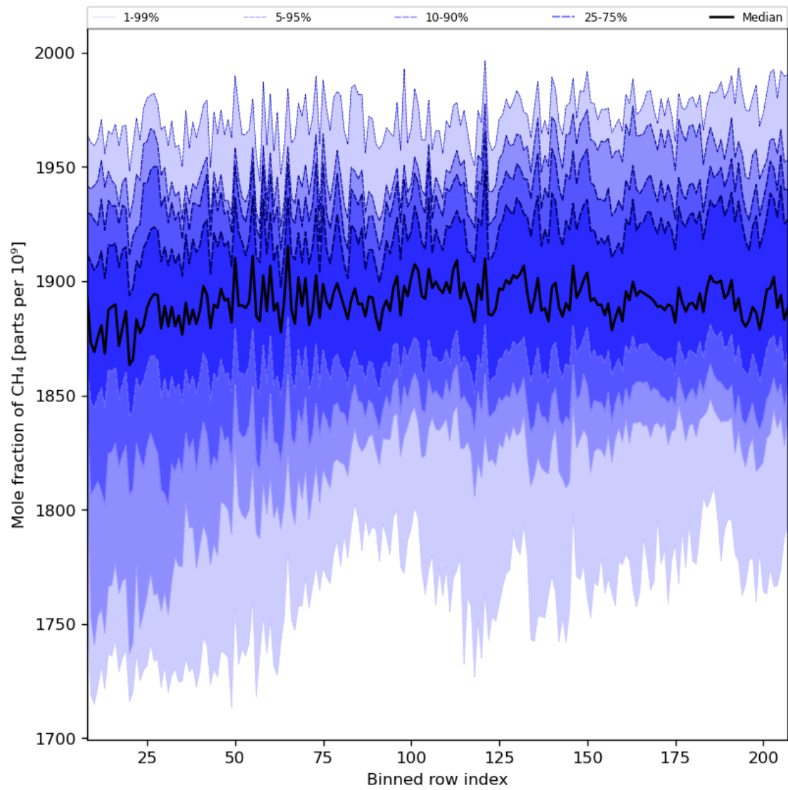
Figure 34: Along track statistics of “Mole fraction of CH 4 ” for 2023-09-21 to 2023-09-23
