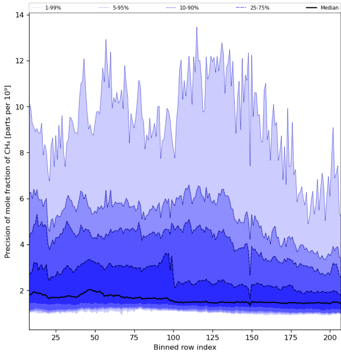
Figure 35: Along track statistics of “Precision of mole fraction of CH 4 ” for 2023-09-21 to 2023-09-23
