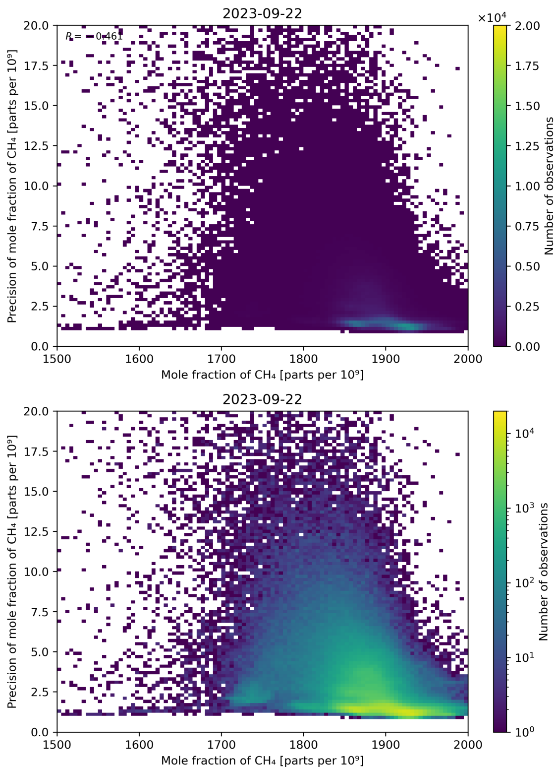
Figure 75: Scatter density plot of “Mole fraction of CH 4 ” against “Precision of mole fraction of CH 4 ” for 2023-09-21 to 2023-09-23.
