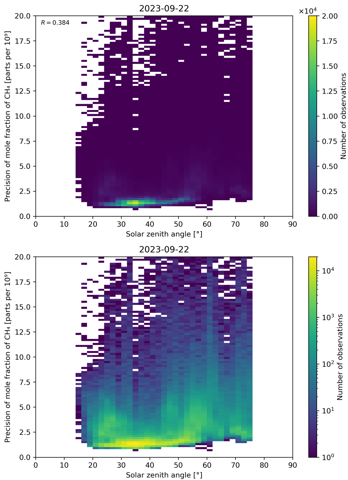
Figure 101: Scatter density plot of “Solar zenith angle” against “Precision of mole fraction of CH 4 ” for 2023-09-21 to 2023-09-23.
