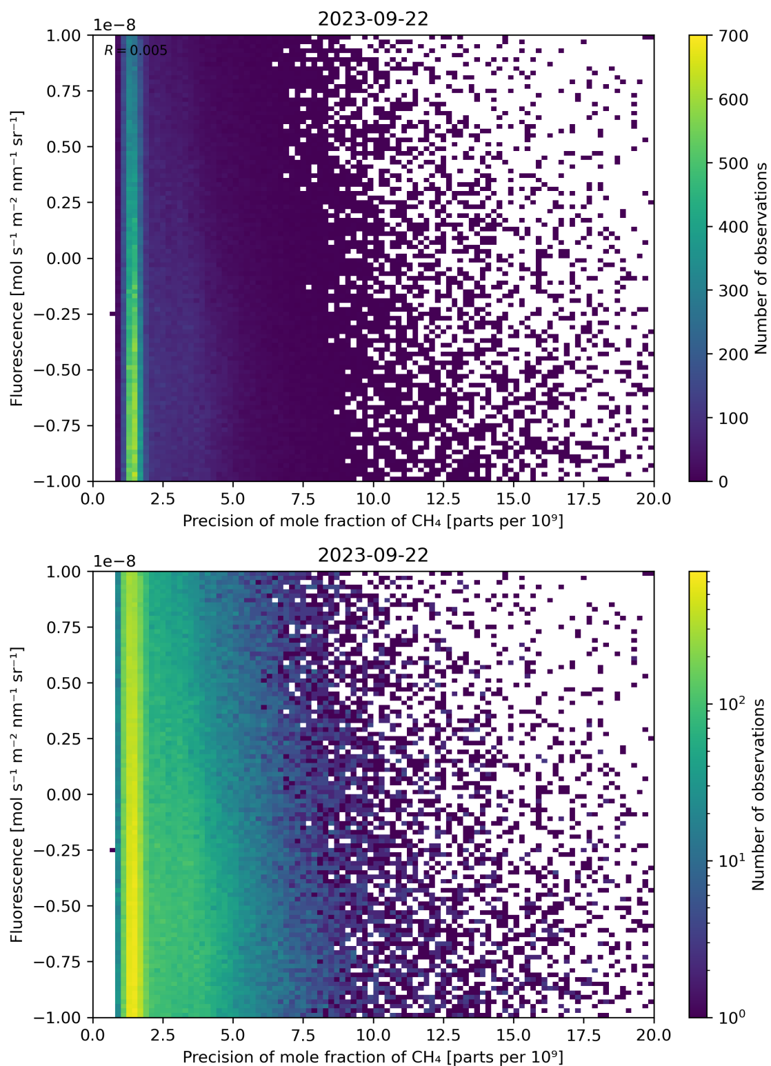
Figure 81: Scatter density plot of “Precision of mole fraction of \text{CH}_4 ” against “Fluorescence” for 2023-09-21 to 2023-09-23.
