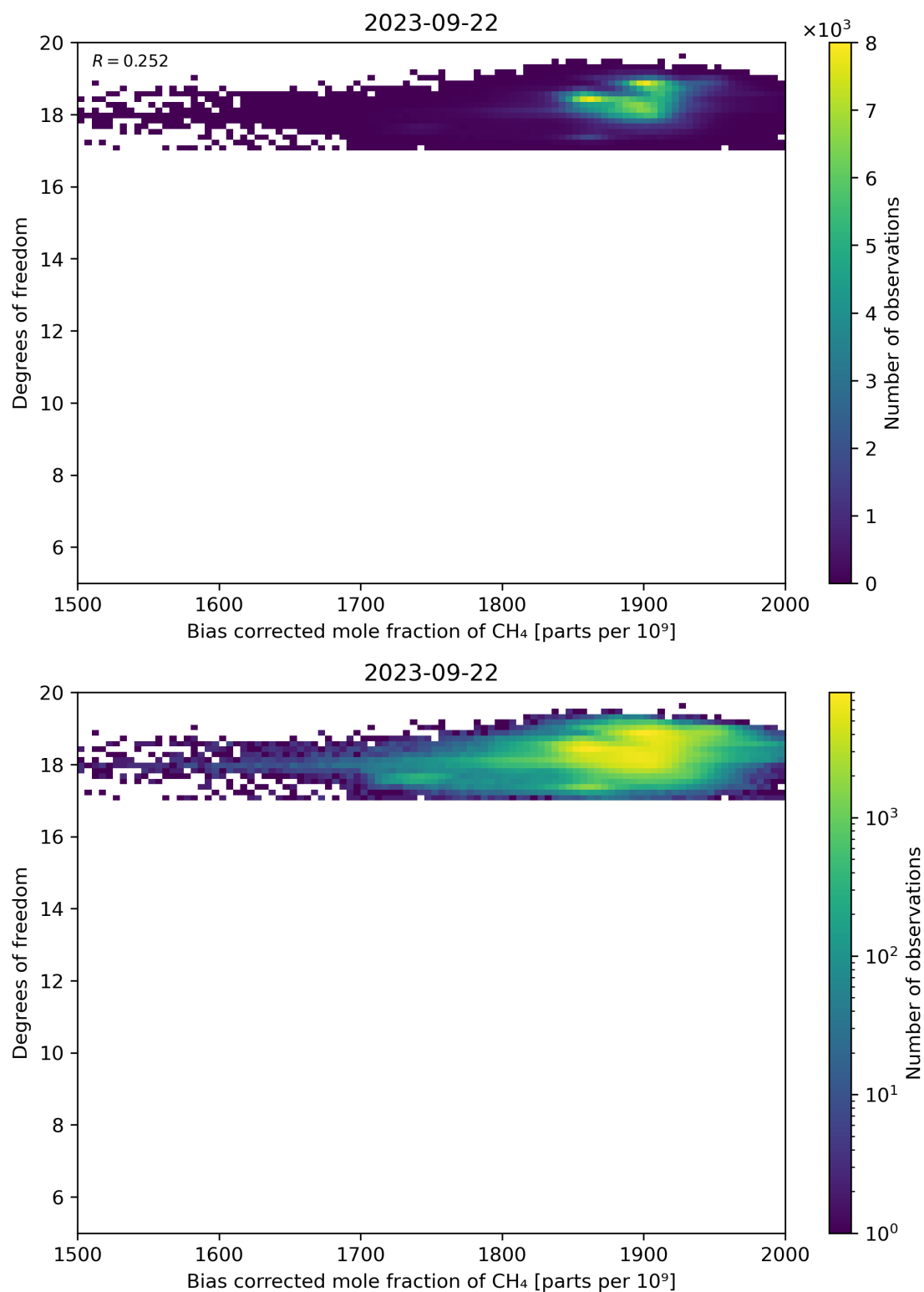
Figure 65: Scatter density plot of “Bias corrected mole fraction of CH 4 ” against “Degrees of freedom” for 2023-09-21 to 2023-09-23.
