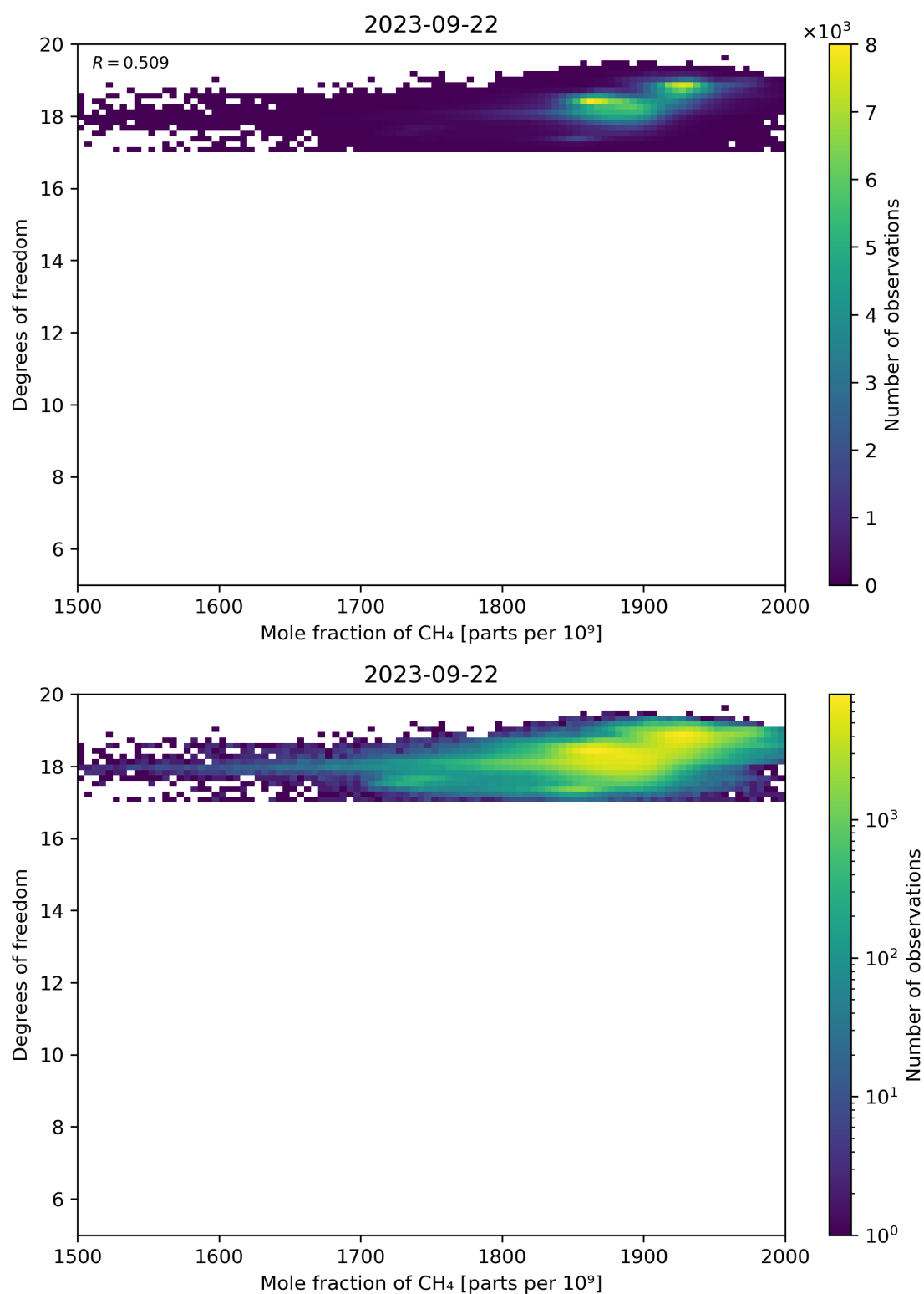
Figure 72: Scatter density plot of “Mole fraction of CH 4 ” against “Degrees of freedom” for 2023-09-21 to 2023-09-23.
