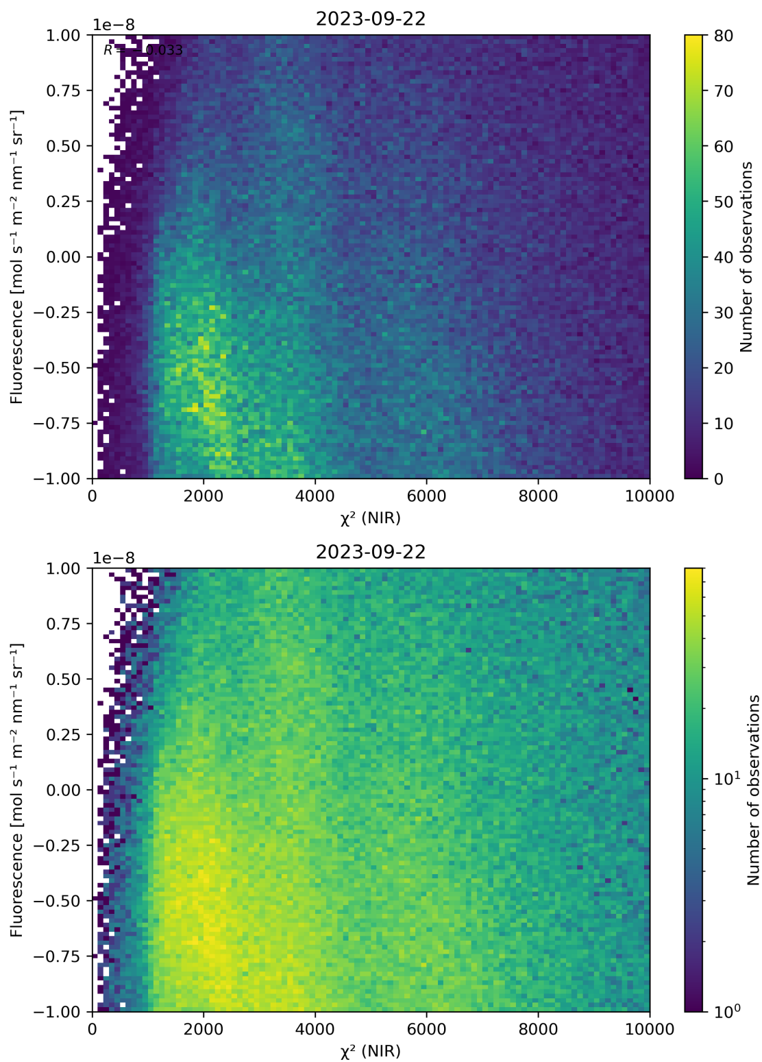
Figure 45: Scatter density plot of “ \chi^2 (NIR)” against “Fluorescence” for 2023-09-21 to 2023-09-23.
