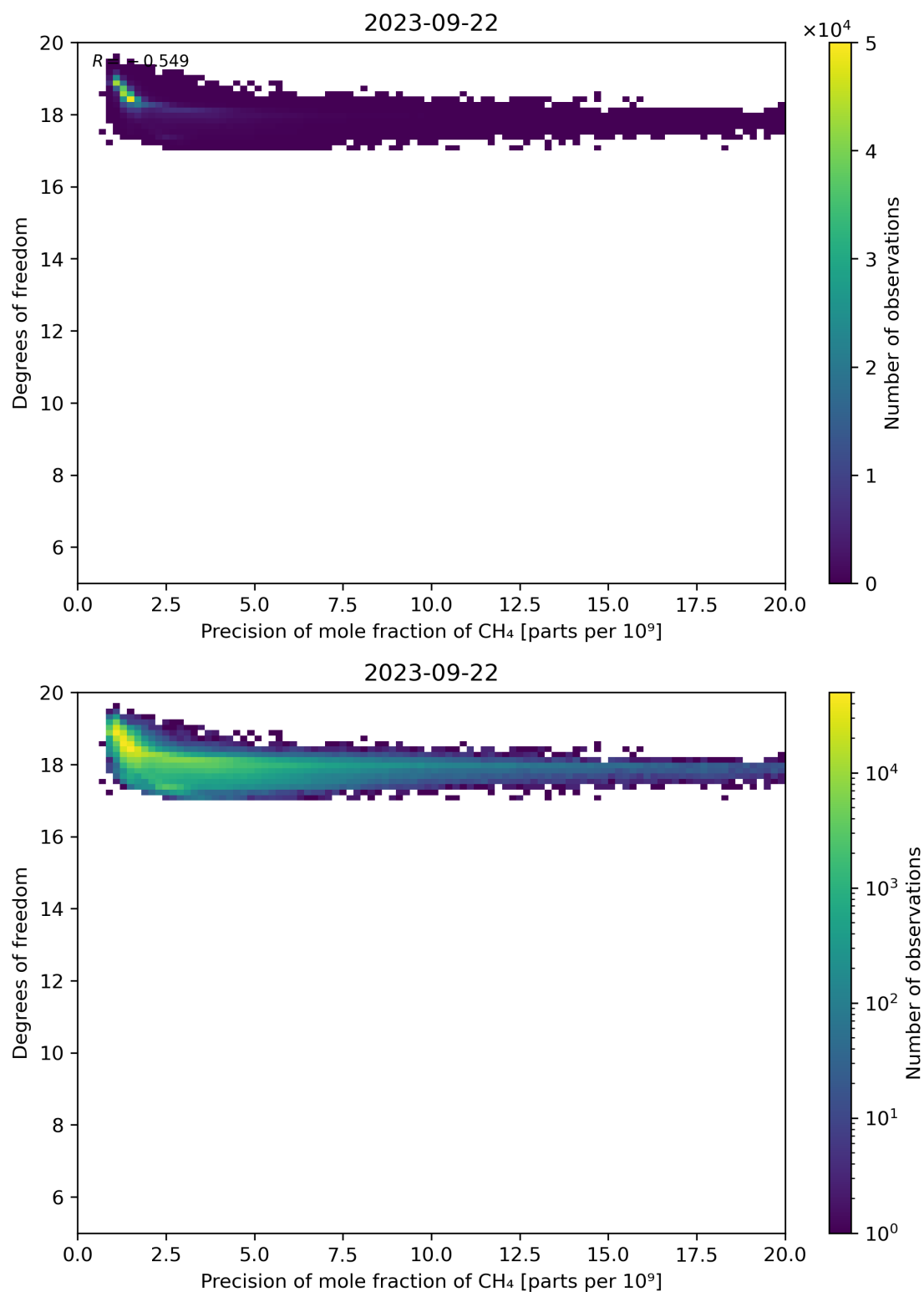
Figure 80: Scatter density plot of “Precision of mole fraction of CH 4 ” against “Degrees of freedom” for 2023-09-21 to 2023-09-23.
