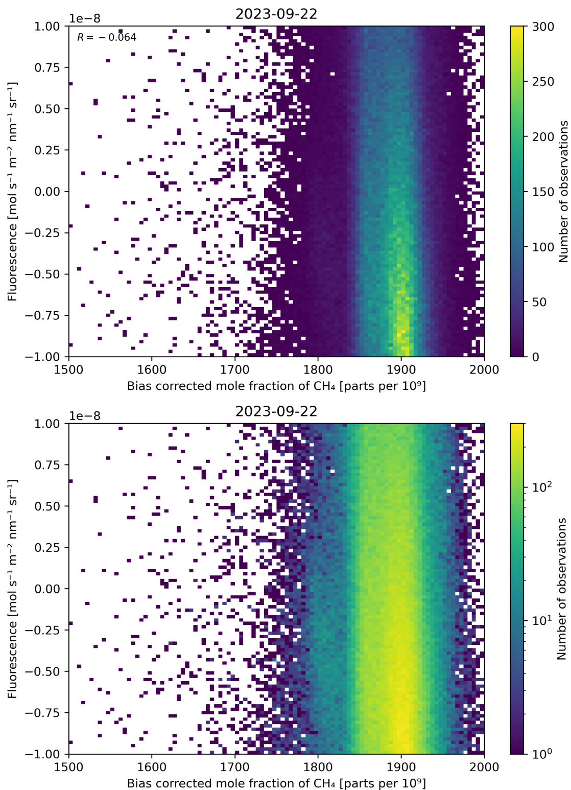
Figure 66: Scatter density plot of “Bias corrected mole fraction of \text{CH}_4 ” against “Fluorescence” for 2023-09-21 to 2023-09-23.
