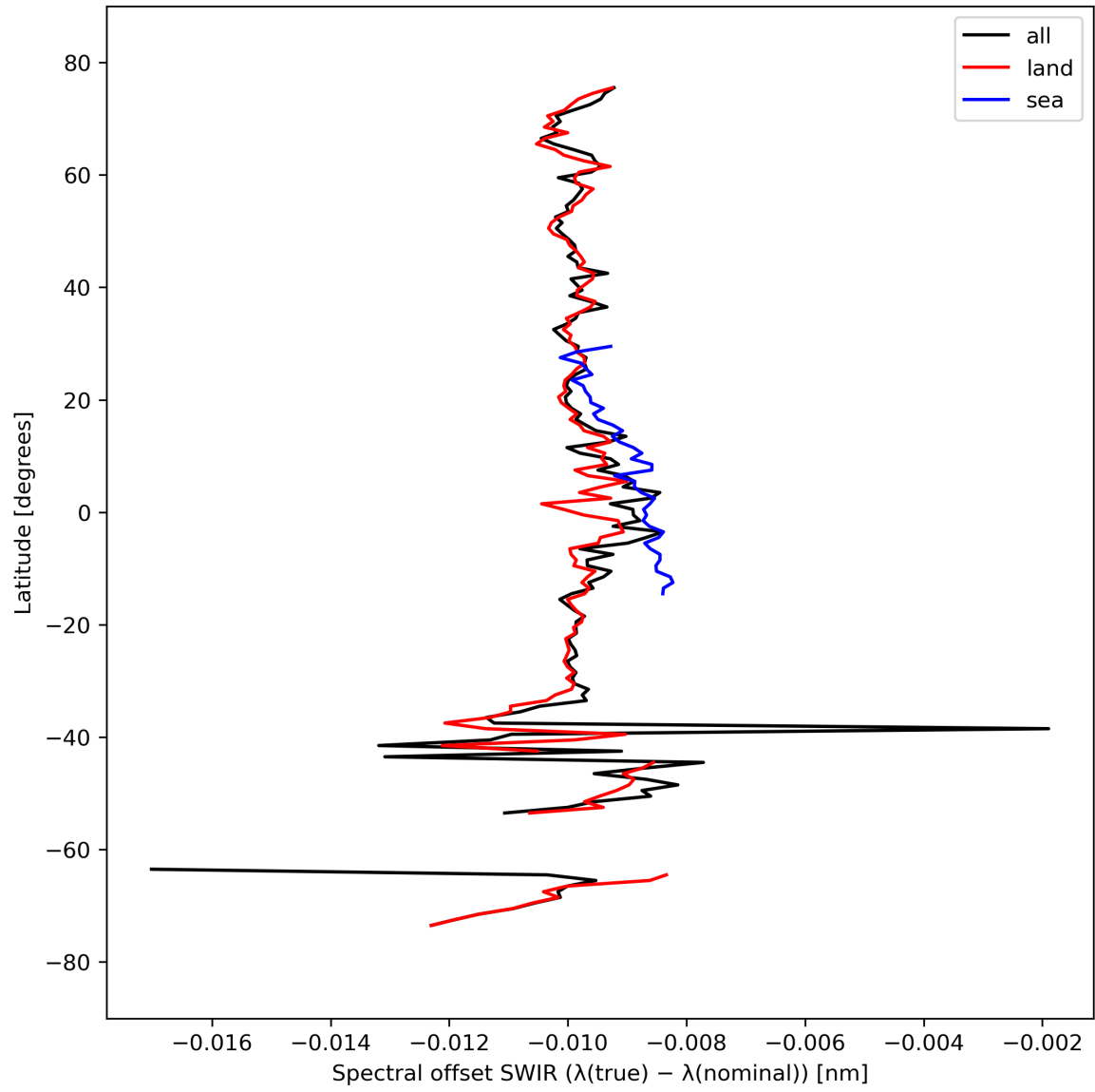
Figure 16: Zonal average of “Spectral offset SWIR ( \lambda(\text{true}) - \lambda(\text{nominal}) )” for 2023-09-21 to 2023-09-23.
