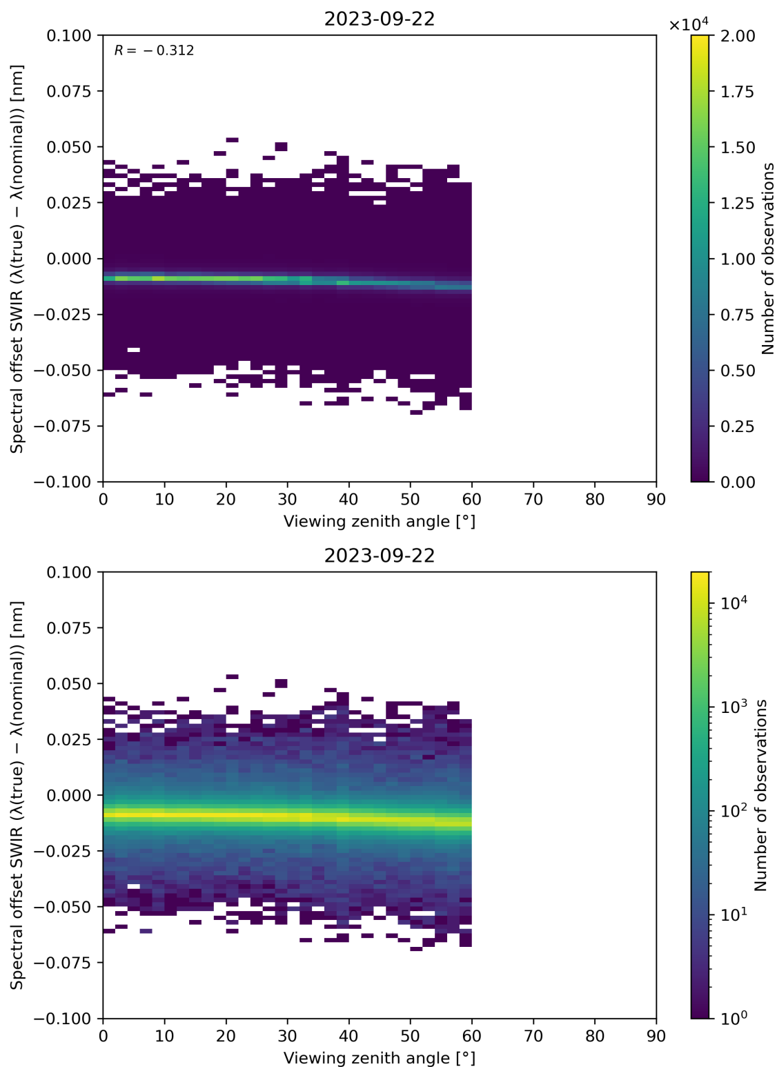
Figure 116: Scatter density plot of “Viewing zenith angle” against “Spectral offset SWIR ( \lambda(\text{true}) - \lambda(\text{nominal}) )” for 2023-09-21 to 2023-09-23.
