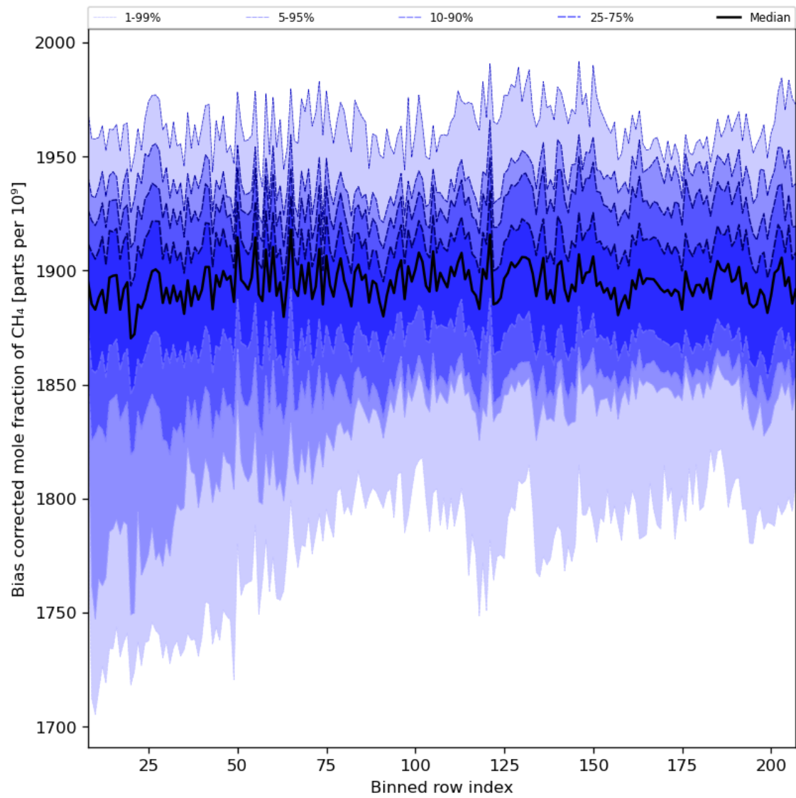
Figure 36: Along track statistics of “Bias corrected mole fraction of CH 4 ” for 2023-09-21 to 2023-09-23
