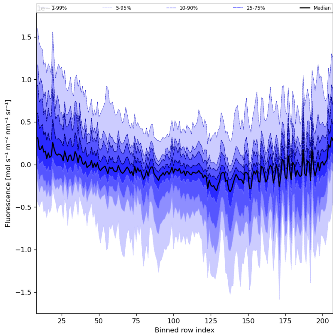
Figure 43: Along track statistics of "Fluorescence" for 2023-09-21 to 2023-09-23
