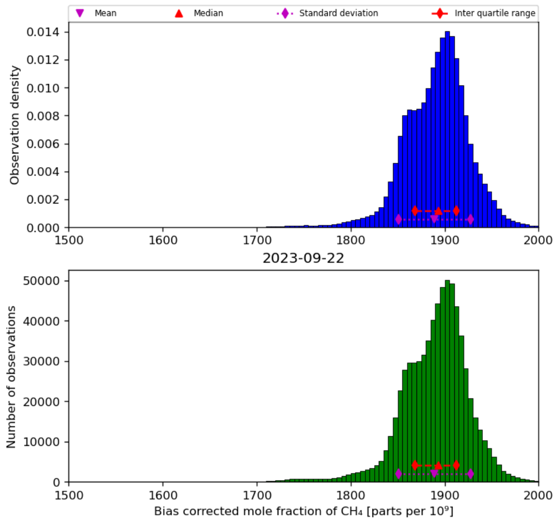
Figure 25: Histogram of “Bias corrected mole fraction of CH 4 ” for 2023-09-21 to 2023-09-23
