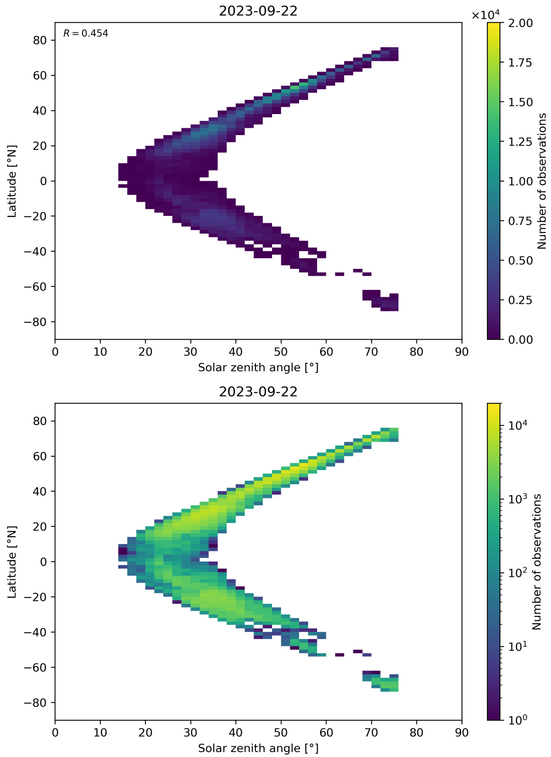
Figure 98: Scatter density plot of “Solar zenith angle” against “Latitude” for 2023-09-21 to 2023-09-23.
