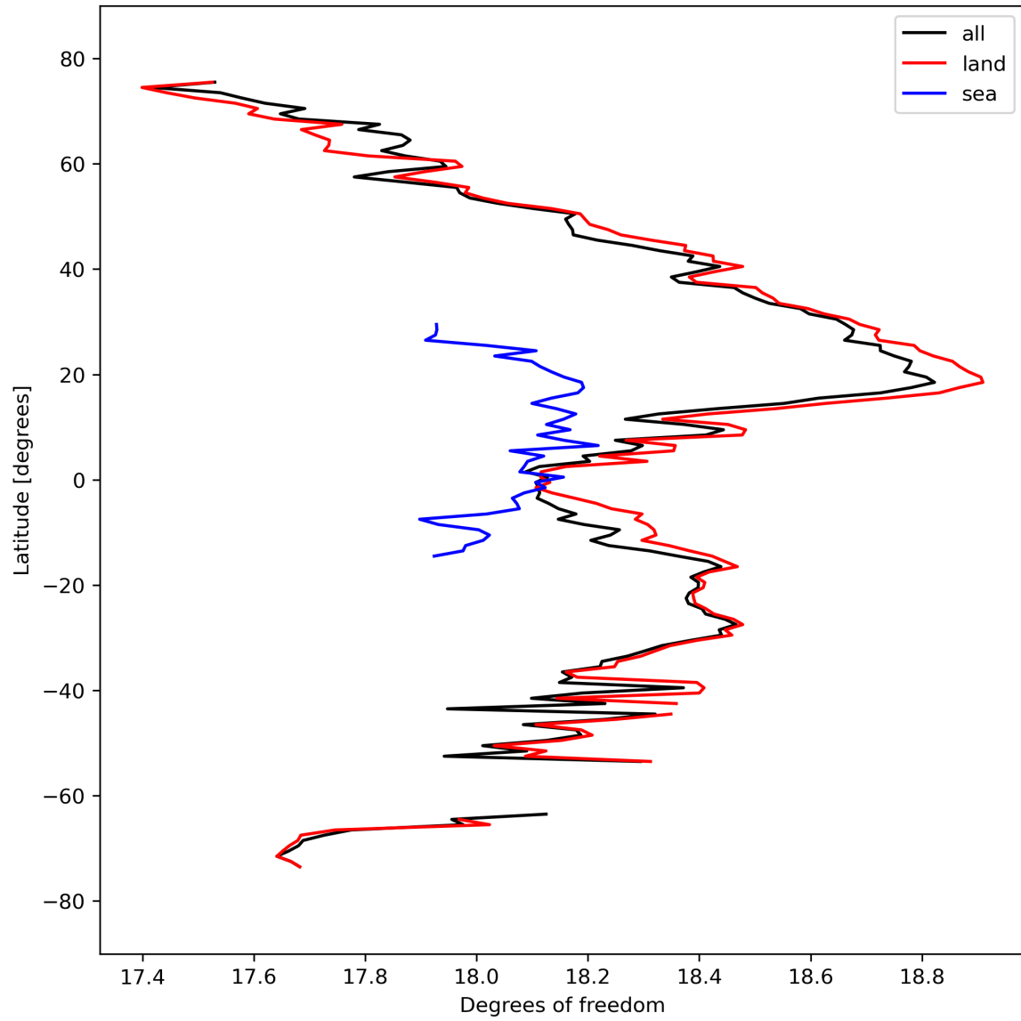
Figure 19: Zonal average of “Degrees of freedom” for 2023-09-21 to 2023-09-23.
