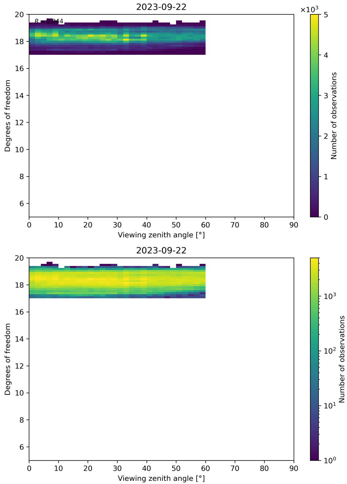
Figure 107: Scatter density plot of “Viewing zenith angle” against “Degrees of freedom” for 2023-09-21 to 2023-09-23.
