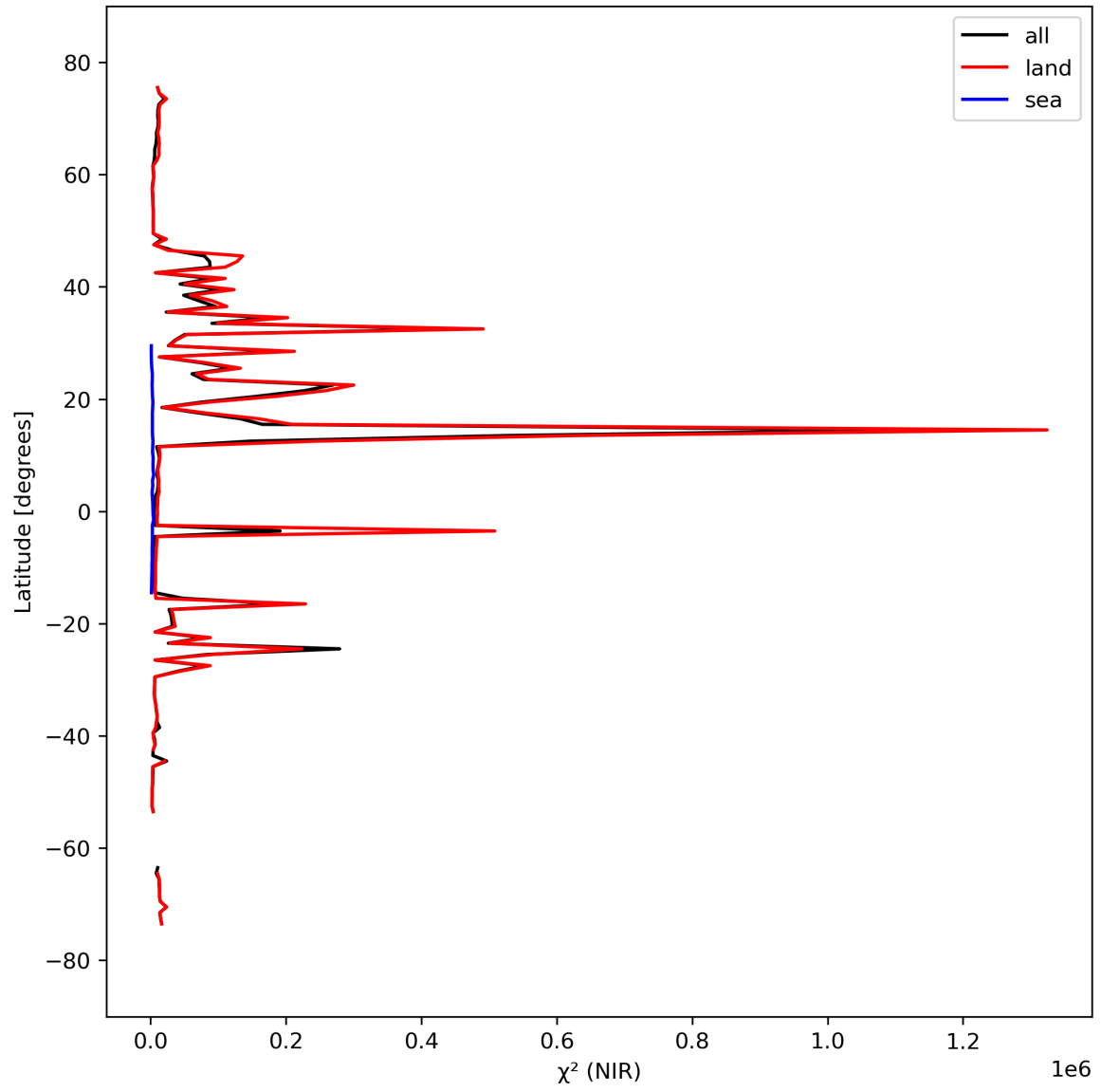
Figure 18: Zonal average of “ \chi^2 (NIR)” for 2023-09-21 to 2023-09-23.
