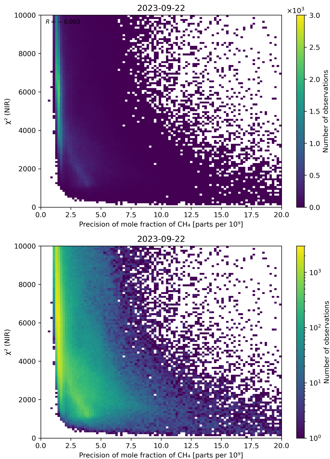
Figure 78: Scatter density plot of “Precision of mole fraction of CH 4 ” against “ \chi^2 (NIR)” for 2023-09-21 to 2023-09-23.
