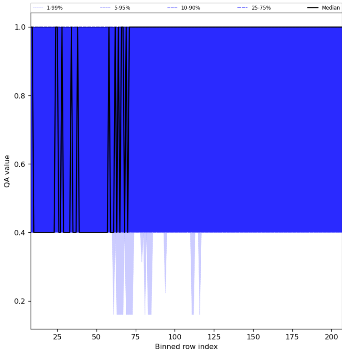
Figure 33: Along track statistics of “QA value” for 2023-09-21 to 2023-09-23
