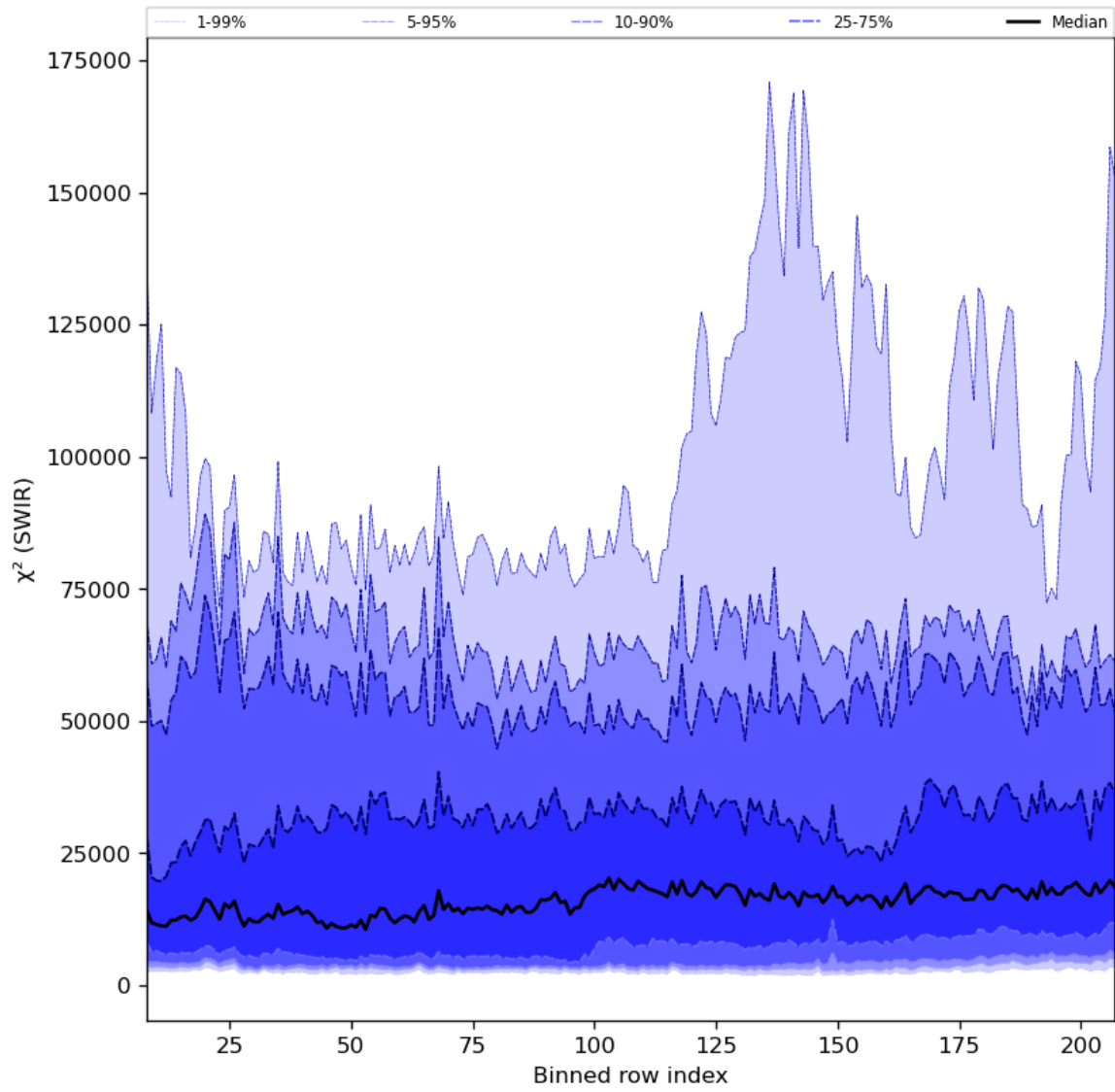
Figure 39: Along track statistics of " \chi^2 (SWIR)" for 2023-09-21 to 2023-09-23
