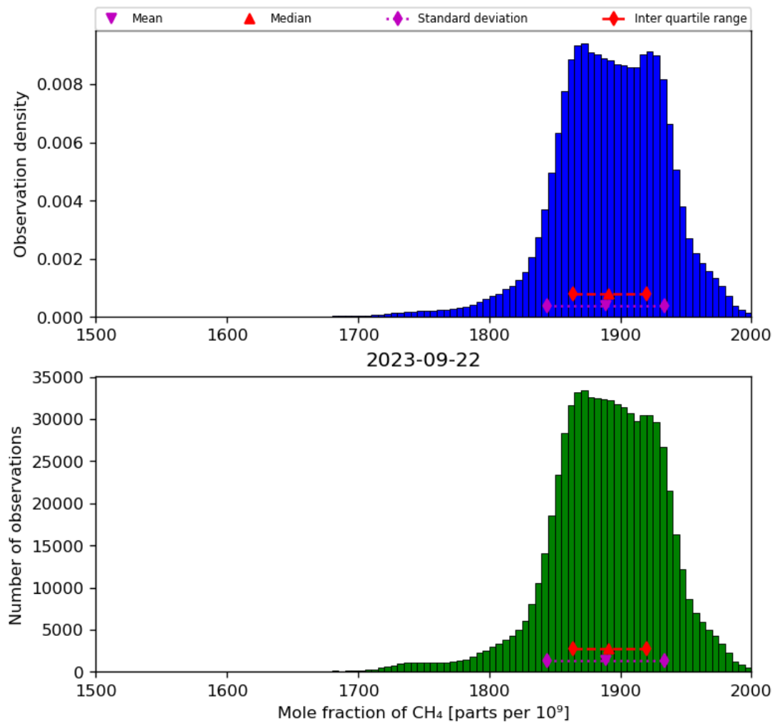
Figure 23: Histogram of “Mole fraction of CH 4 ” for 2023-09-21 to 2023-09-23
