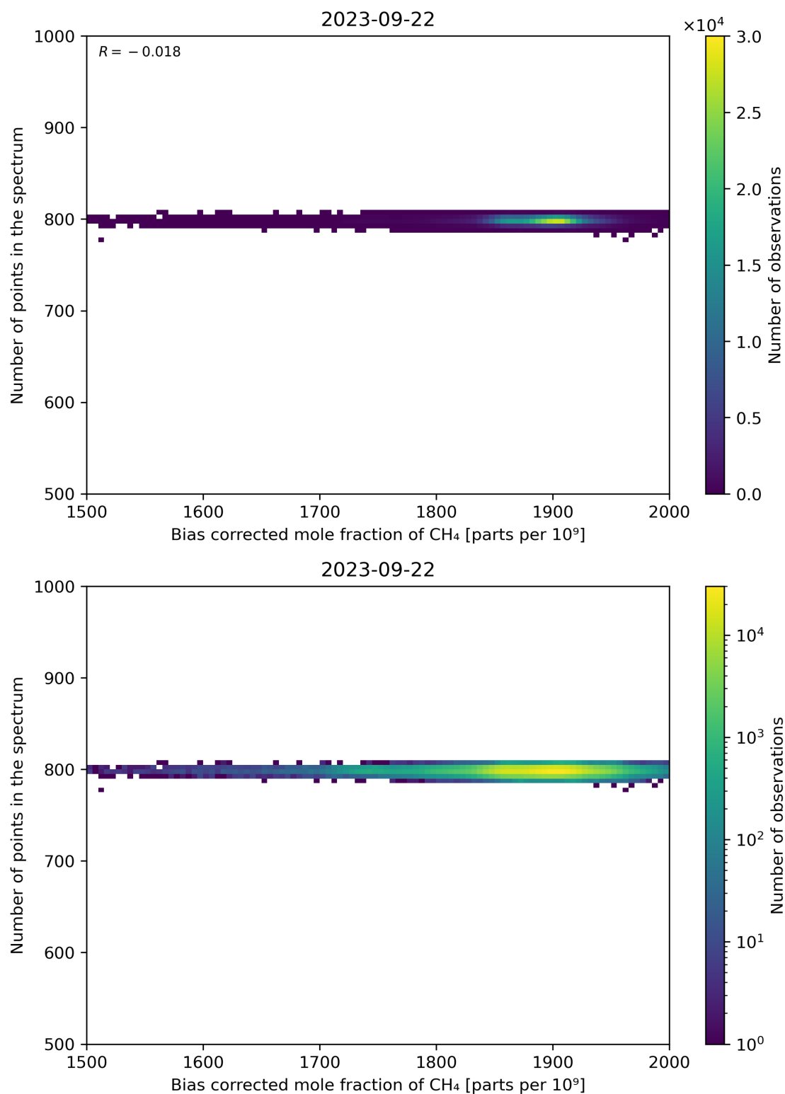
Figure 68: Scatter density plot of “Bias corrected mole fraction of CH 4 ” against “Number of points in the spectrum” for 2023-09-21 to 2023-09-23.
