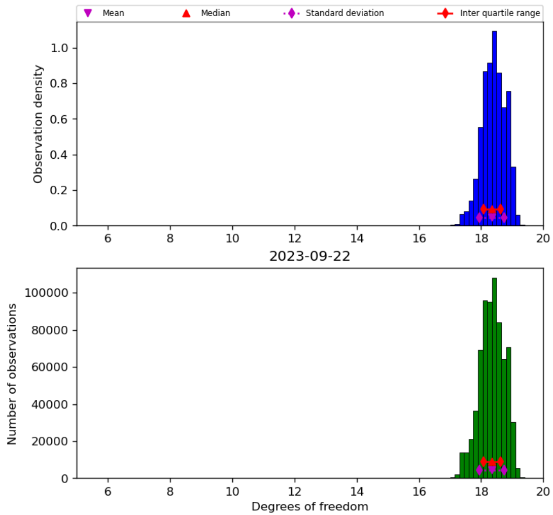
Figure 30: Histogram of “Degrees of freedom” for 2023-09-21 to 2023-09-23
