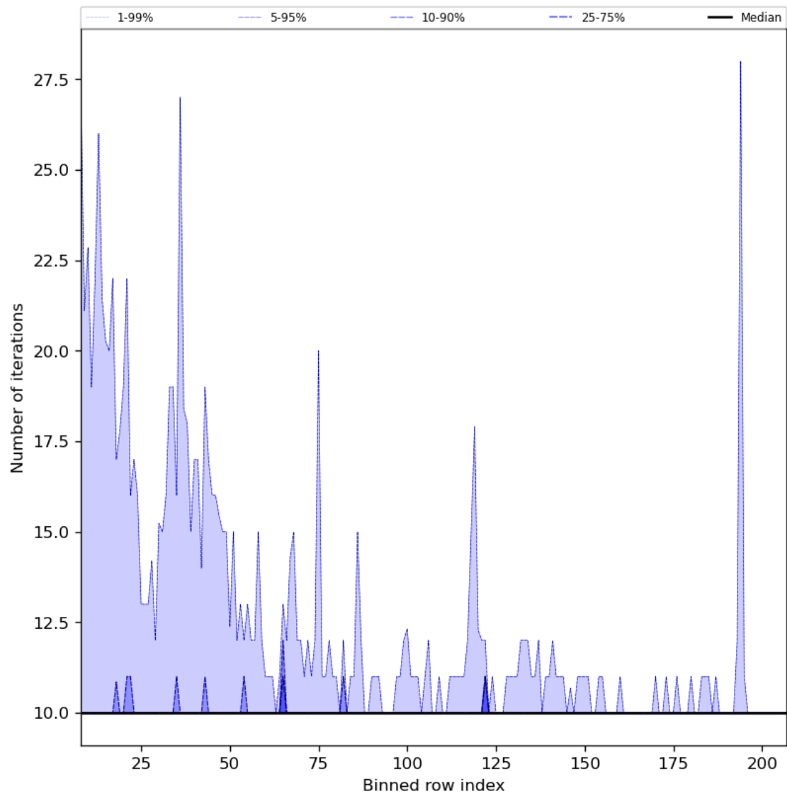
Figure 42: Along track statistics of “Number of iterations” for 2023-09-21 to 2023-09-23
