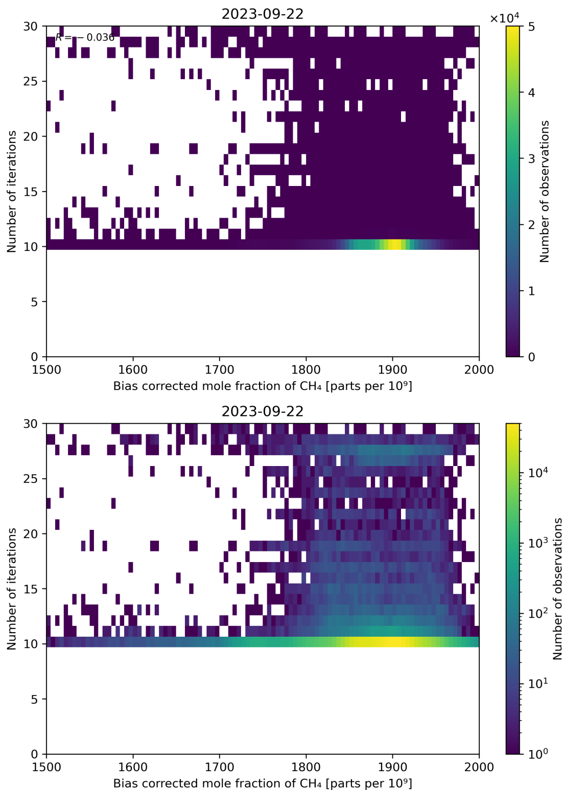
Figure 67: Scatter density plot of “Bias corrected mole fraction of CH 4 ” against “Number of iterations” for 2023-09-21 to 2023-09-23.
