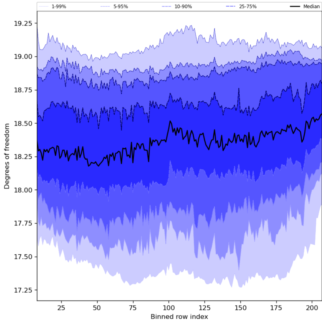
Figure 41: Along track statistics of “Degrees of freedom” for 2023-09-21 to 2023-09-23
