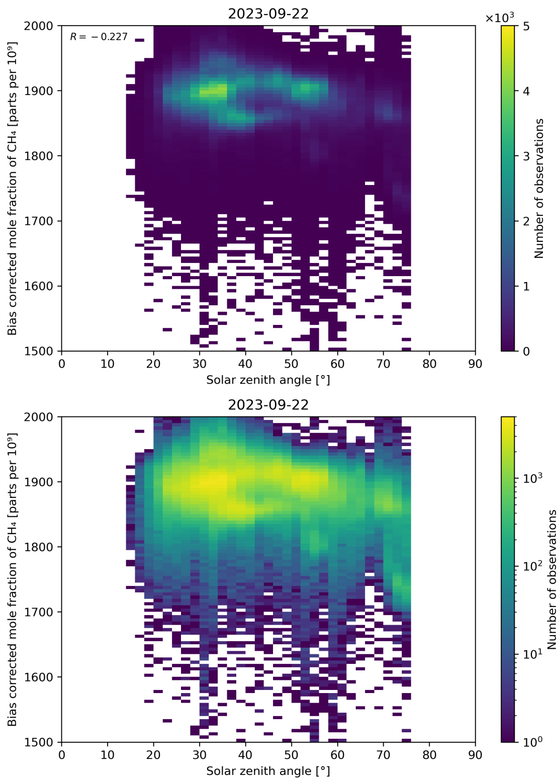
Figure 100: Scatter density plot of “Solar zenith angle” against “Bias corrected mole fraction of CH 4 ” for 2023-09-21 to 2023-09-23.
