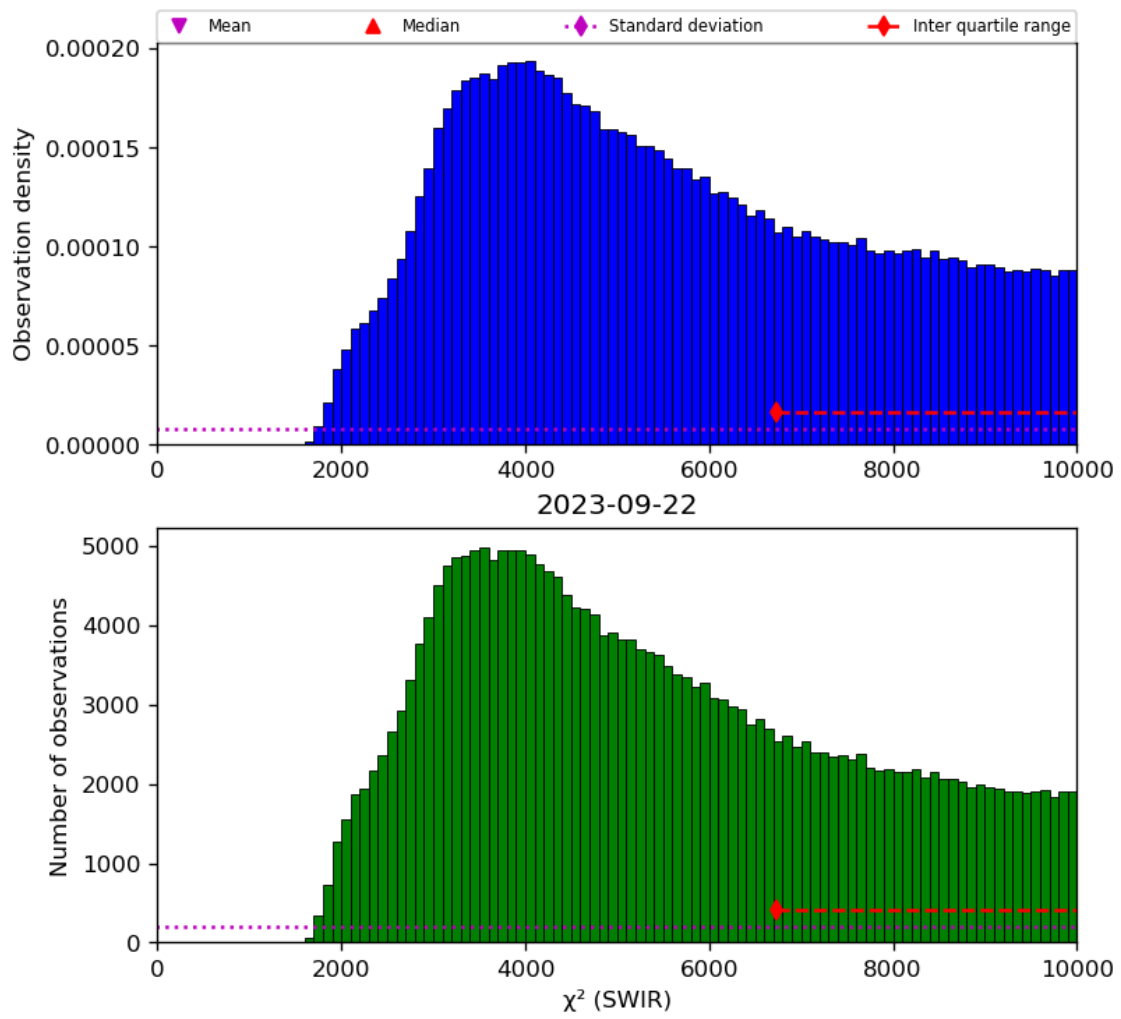
Figure 28: Histogram of “ \chi^2 (SWIR)” for 2023-09-21 to 2023-09-23
