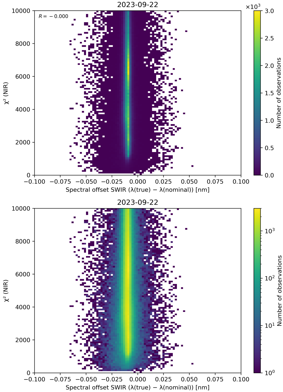
Figure 117: Scatter density plot of “Spectral offset SWIR ( \lambda(\text{true}) - \lambda(\text{nominal}) )” against “ \chi^2 (NIR)” for 2023-09-21 to 2023-09-23.
