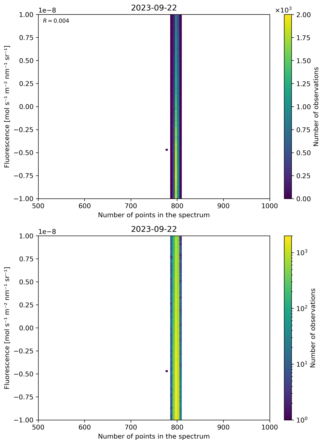
Figure 91: Scatter density plot of “Number of points in the spectrum” against “Fluorescence” for 2023-09-21 to 2023-09-23.
