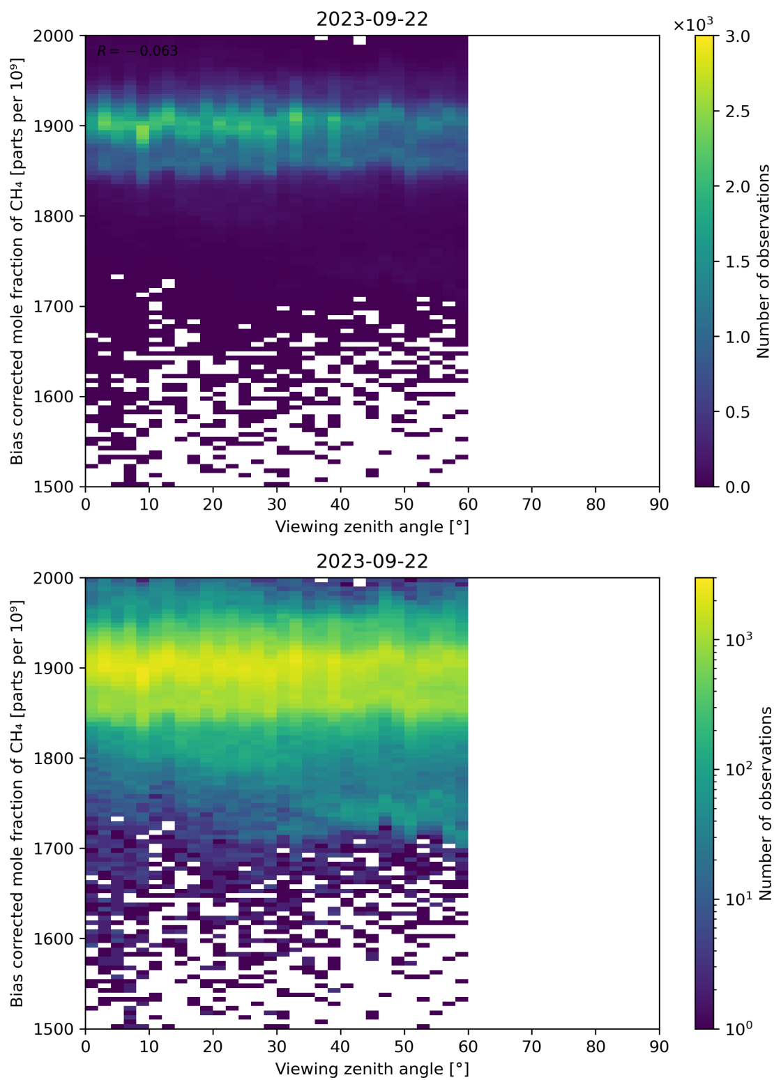
Figure 111: Scatter density plot of “Viewing zenith angle” against “Bias corrected mole fraction of CH 4 ” for 2023-09-21 to 2023-09-23.
