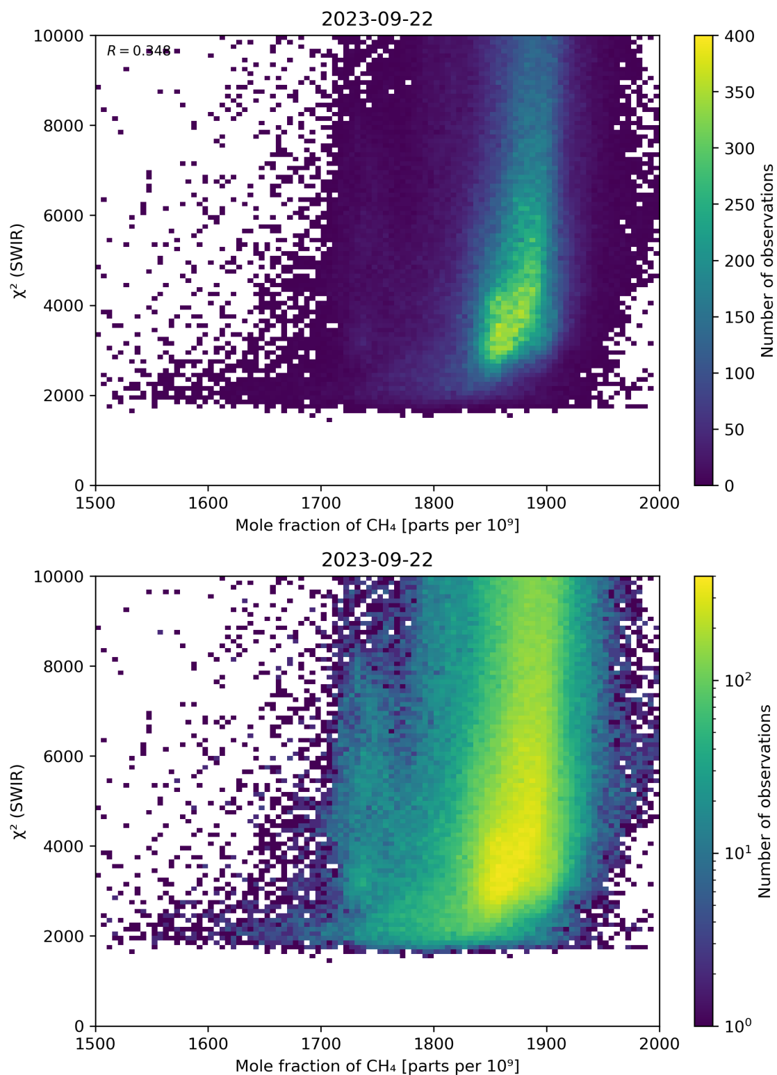
Figure 71: Scatter density plot of “Mole fraction of \text{CH}_4 ” against “ \chi^2 (SWIR)” for 2023-09-21 to 2023-09-23.
