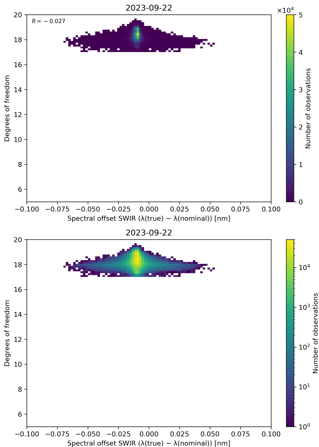
Figure 119: Scatter density plot of “Spectral offset SWIR ( \lambda(\text{true}) - \lambda(\text{nominal}) )” against “Degrees of freedom” for 2023-09-21 to 2023-09-23.
