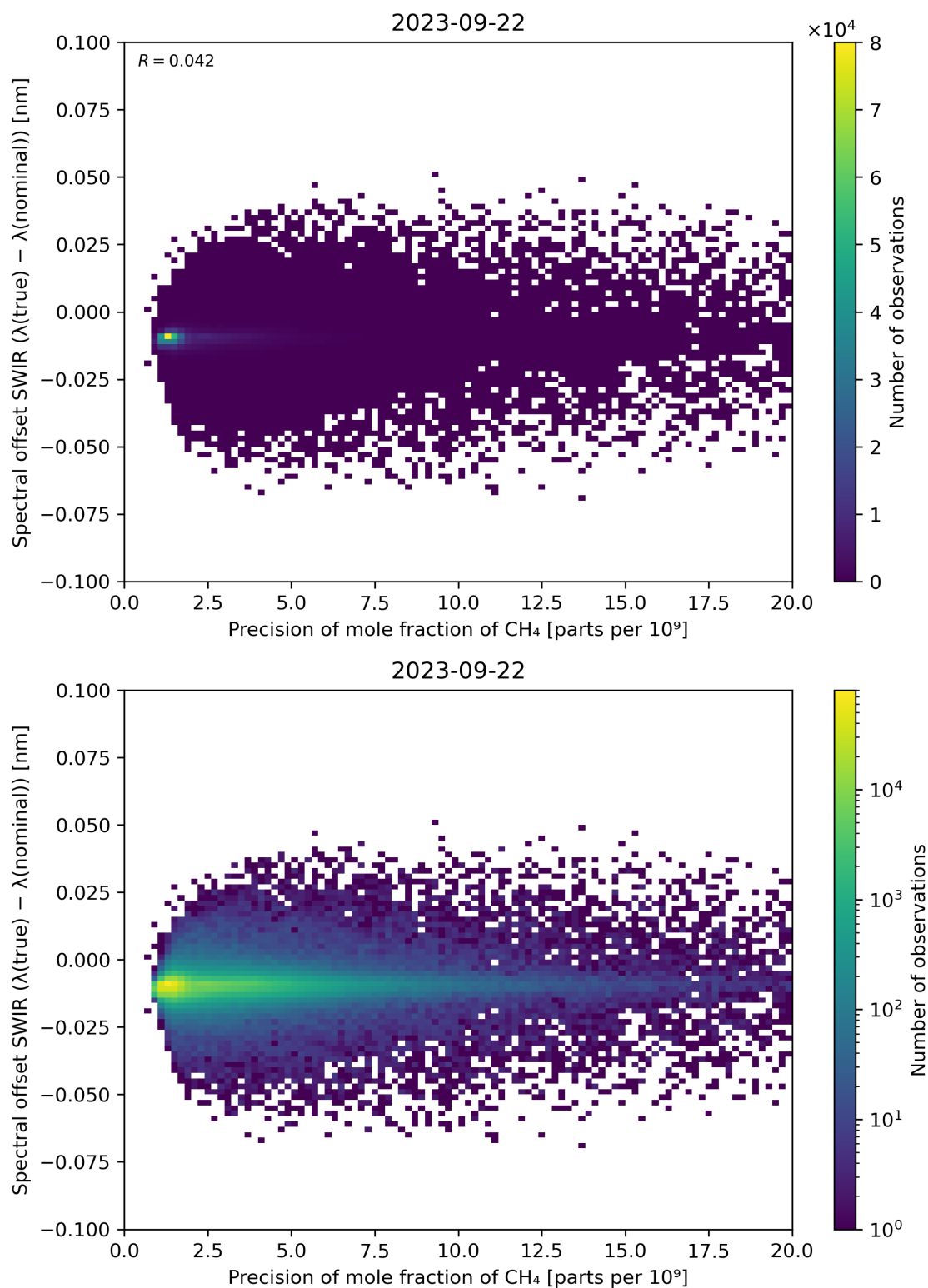
Figure 85: Scatter density plot of “Precision of mole fraction of \text{CH}_4 ” against “Spectral offset SWIR ( \lambda(\text{true}) - \lambda(\text{nominal}) )” for 2023-09-21 to 2023-09-23.
