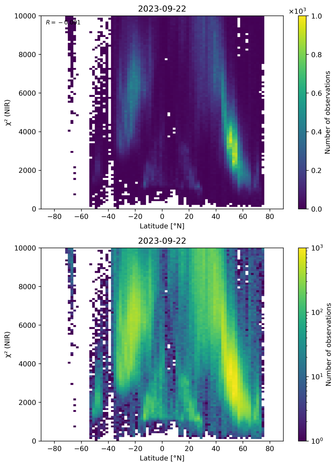
Figure 53: Scatter density plot of “Latitude” against “ \chi^2 (NIR)” for 2023-09-21 to 2023-09-23.
