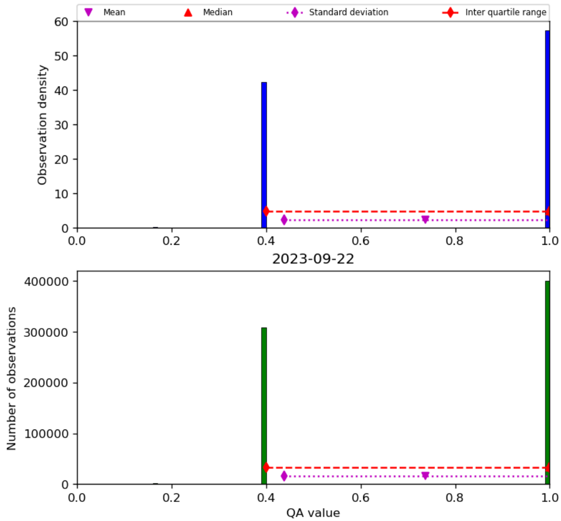
Figure 22: Histogram of “QA value” for 2023-09-21 to 2023-09-23
