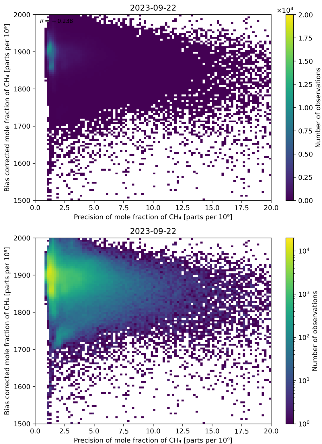
Figure 82: Scatter density plot of “Precision of mole fraction of CH 4 ” against “Bias corrected mole fraction of CH 4 ” for 2023-09-21 to 2023-09-23.
