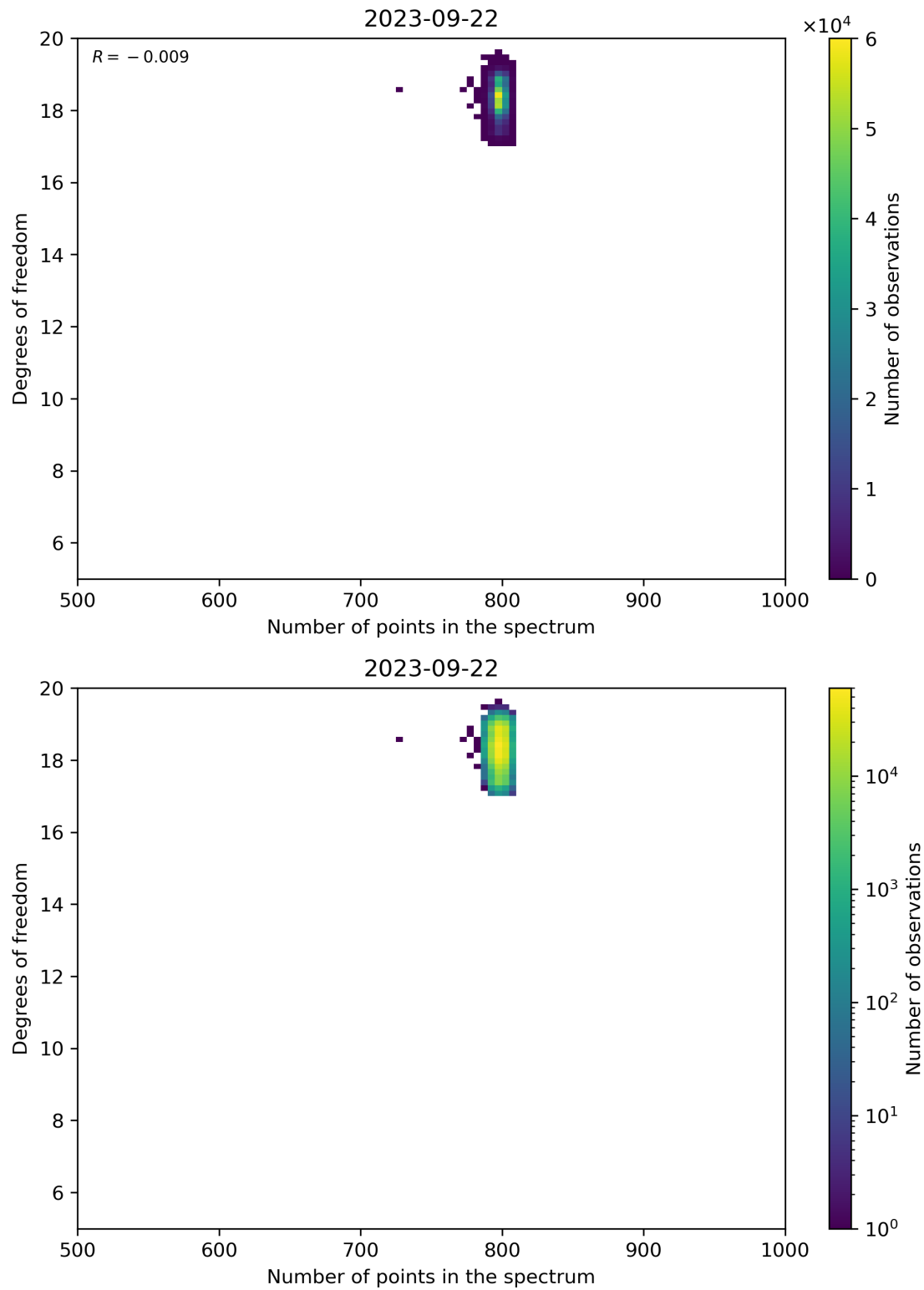
Figure 90: Scatter density plot of “Number of points in the spectrum” against “Degrees of freedom” for 2023-09-21 to 2023-09-23.
