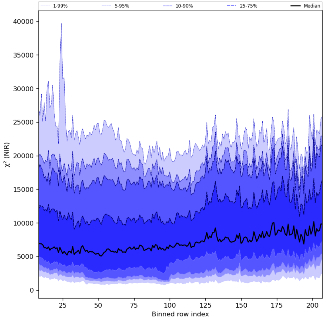
Figure 40: Along track statistics of " \chi^2 (NIR)" for 2023-09-21 to 2023-09-23
