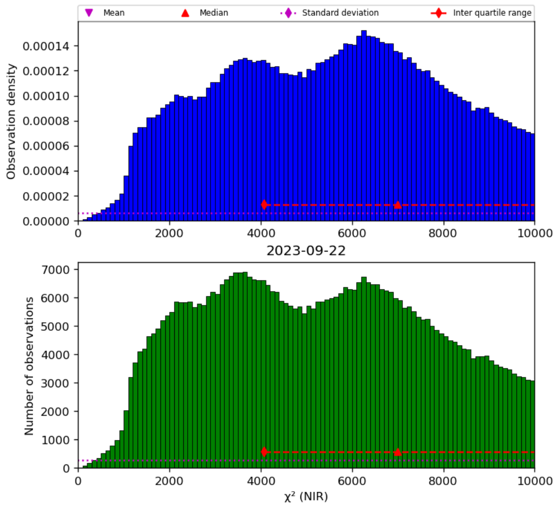
Figure 29: Histogram of " \chi^2 (NIR)" for 2023-09-21 to 2023-09-23
