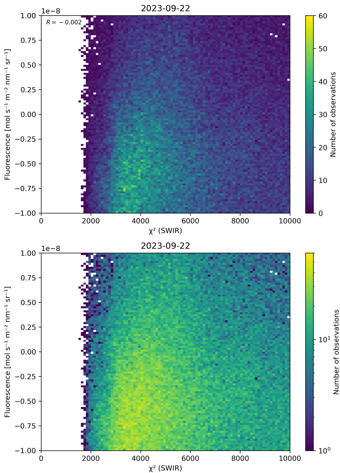
Figure 49: Scatter density plot of “ \chi^2 (SWIR)” against “Fluorescence” for 2023-09-21 to 2023-09-23.
