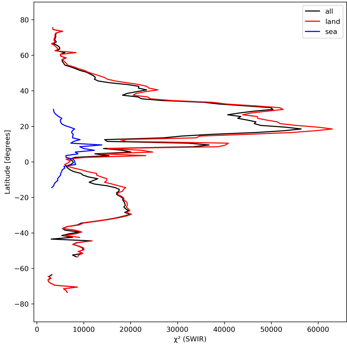
Figure 17: Zonal average of “ \chi^2 (SWIR)” for 2023-09-21 to 2023-09-23.
