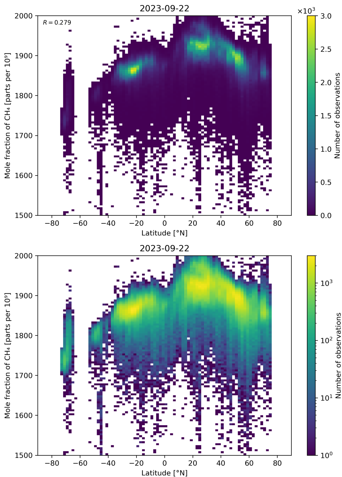
Figure 57: Scatter density plot of “Latitude” against “Mole fraction of CH 4 ” for 2023-09-21 to 2023-09-23.
