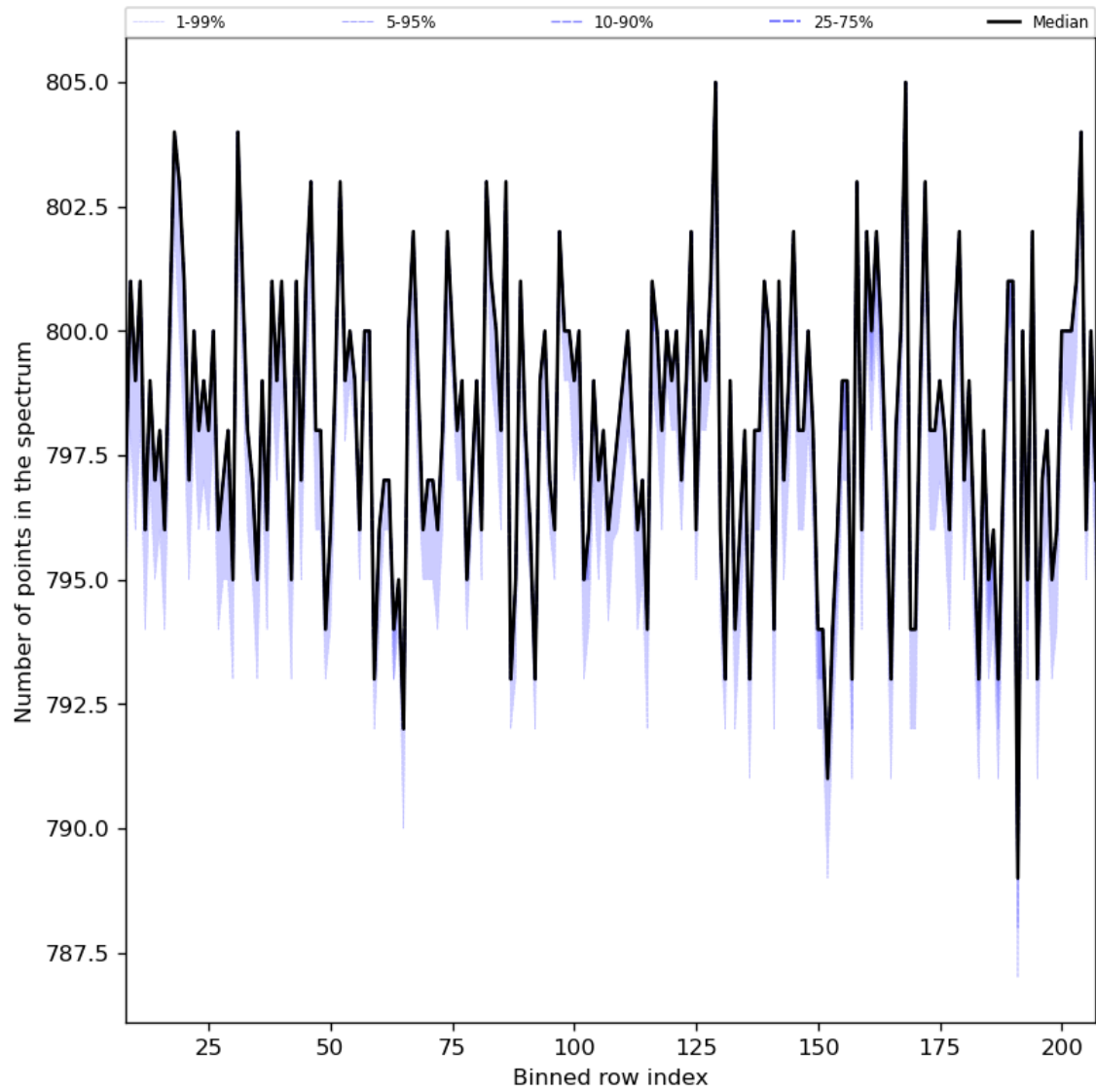
Figure 37: Along track statistics of “Number of points in the spectrum” for 2023-09-21 to 2023-09-23
