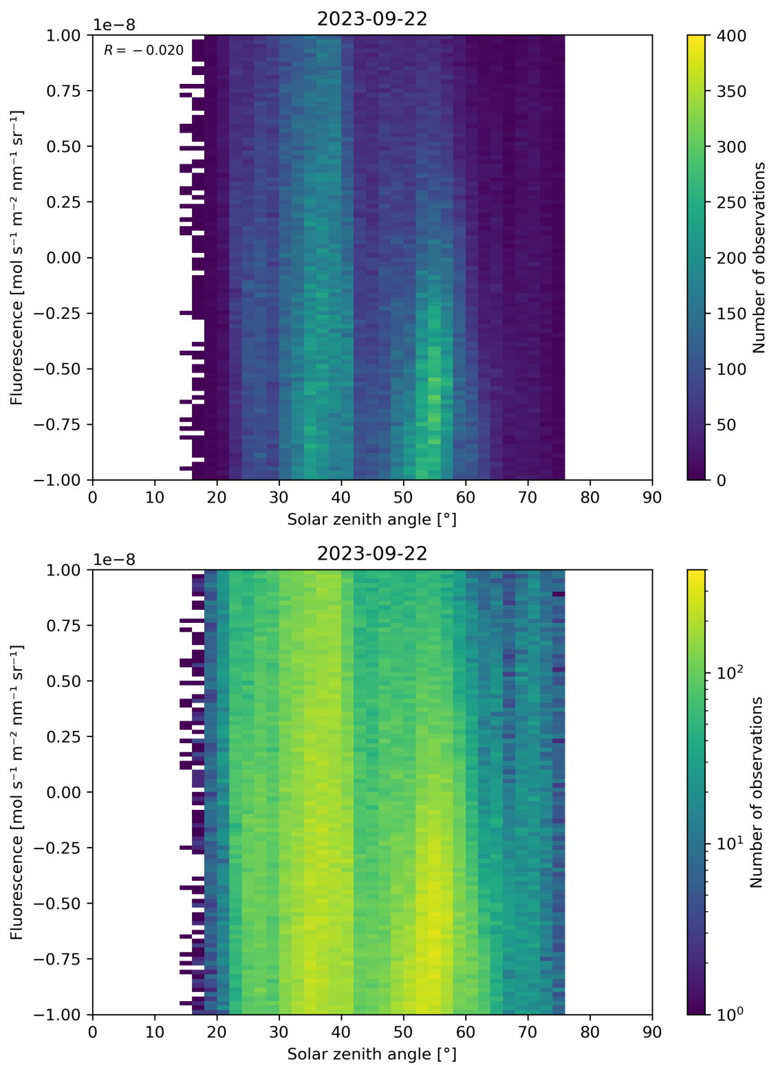
Figure 97: Scatter density plot of “Solar zenith angle” against “Fluorescence” for 2023-09-21 to 2023-09-23.
