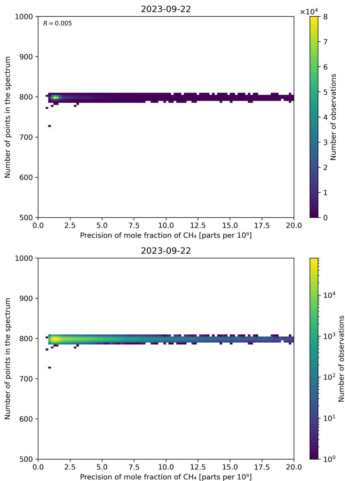
Figure 84: Scatter density plot of “Precision of mole fraction of CH 4 ” against “Number of points in the spectrum” for 2023-09-21 to 2023-09-23.
