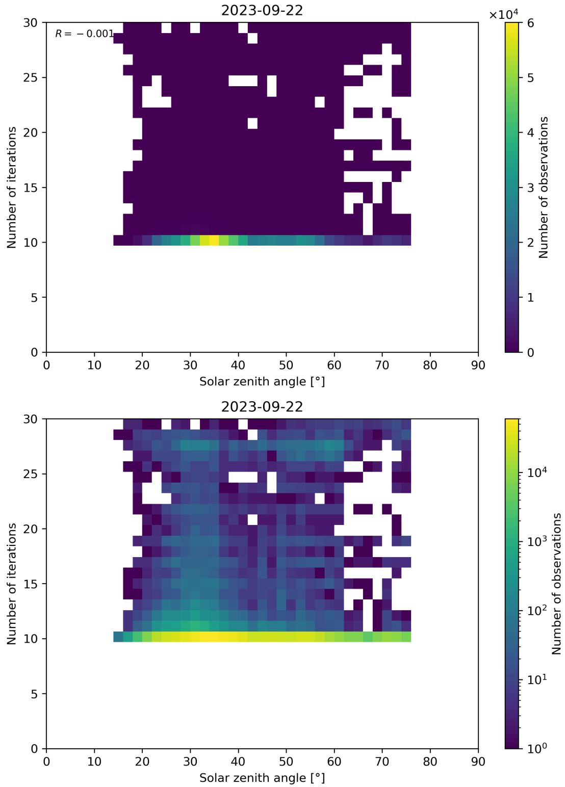
Figure 102: Scatter density plot of “Solar zenith angle” against “Number of iterations” for 2023-09-21 to 2023-09-23.
