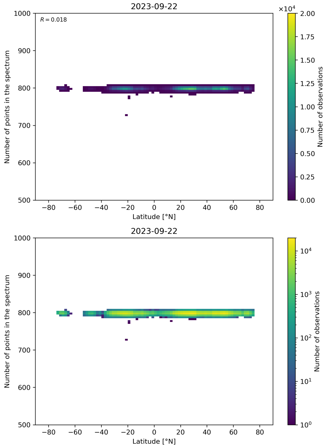
Figure 61: Scatter density plot of “Latitude” against “Number of points in the spectrum” for 2023-09-21 to 2023-09-23.
