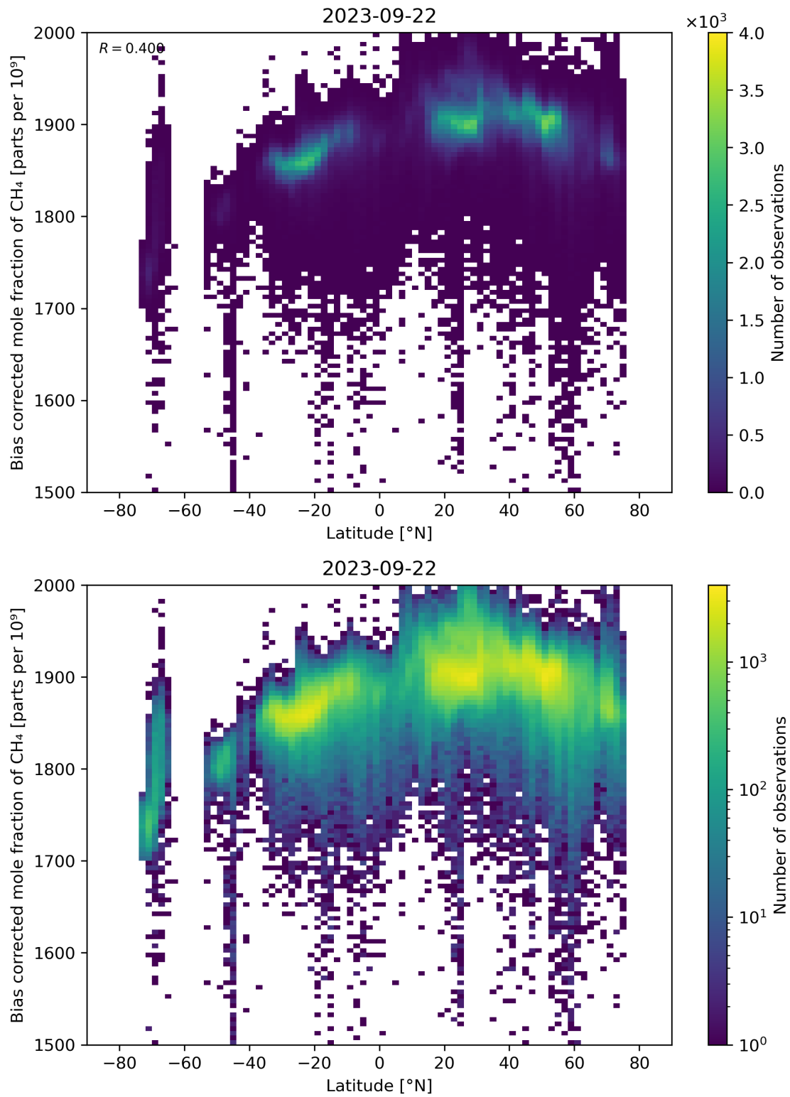
Figure 58: Scatter density plot of “Latitude” against “Bias corrected mole fraction of CH 4 ” for 2023-09-21 to 2023-09-23.
