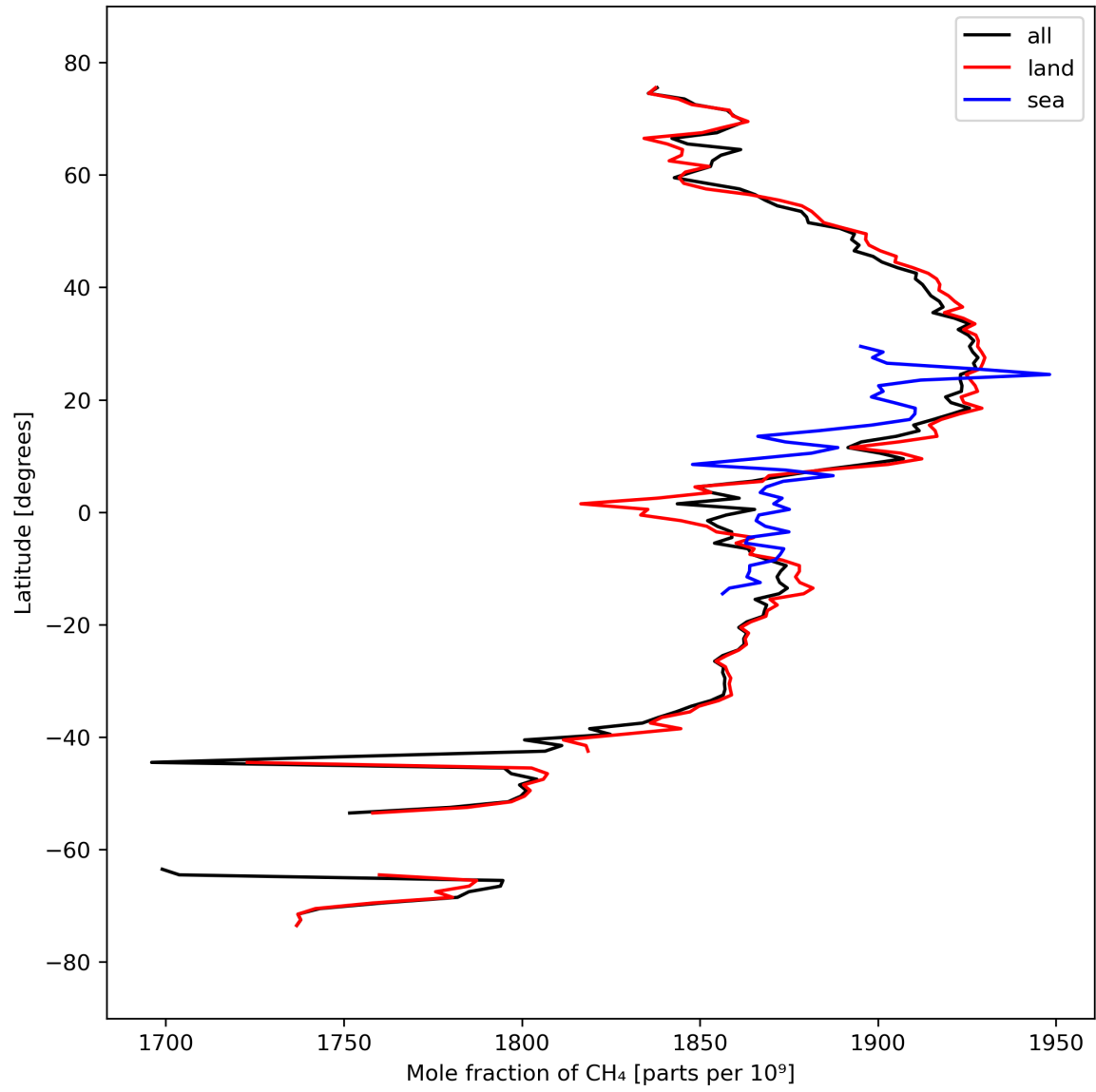
Figure 12: Zonal average of “Mole fraction of \text{CH}_4 ” for 2023-09-21 to 2023-09-23.
