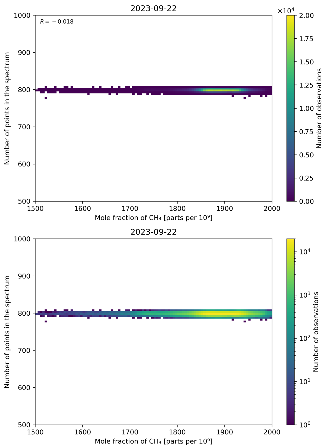
Figure 77: Scatter density plot of “Mole fraction of CH 4 ” against “Number of points in the spectrum” for 2023-09-21 to 2023-09-23.
