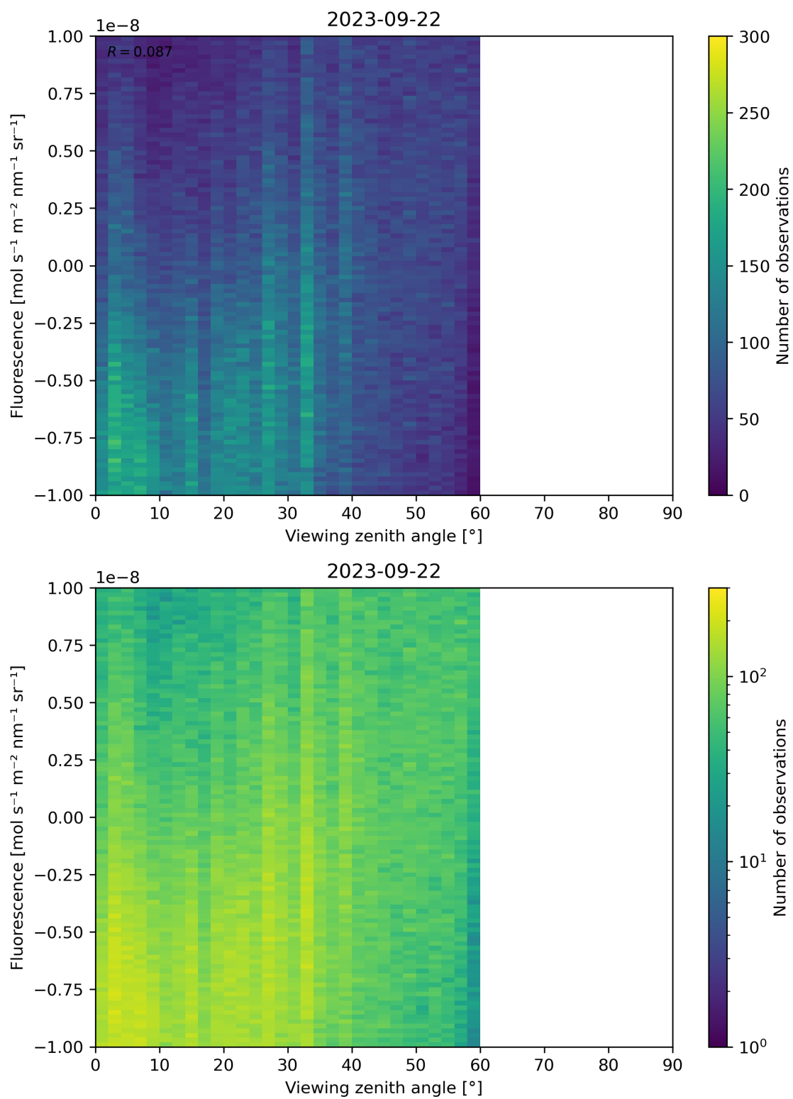
Figure 108: Scatter density plot of “Viewing zenith angle” against “Fluorescence” for 2023-09-21 to 2023-09-23.
