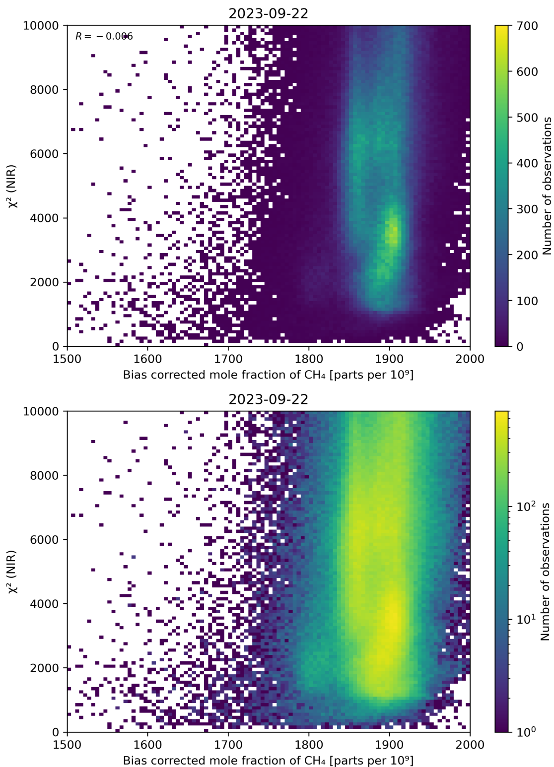
Figure 63: Scatter density plot of “Bias corrected mole fraction of CH 4 ” against “ \chi^2 (NIR)” for 2023-09-21 to 2023-09-23.
