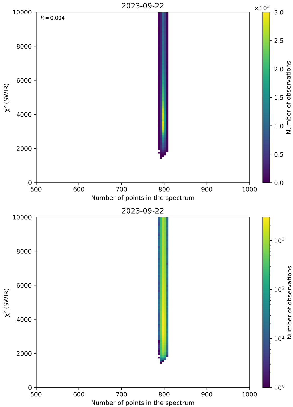
Figure 89: Scatter density plot of “Number of points in the spectrum” against “ \chi^2 (SWIR)” for 2023-09-21 to 2023-09-23.
