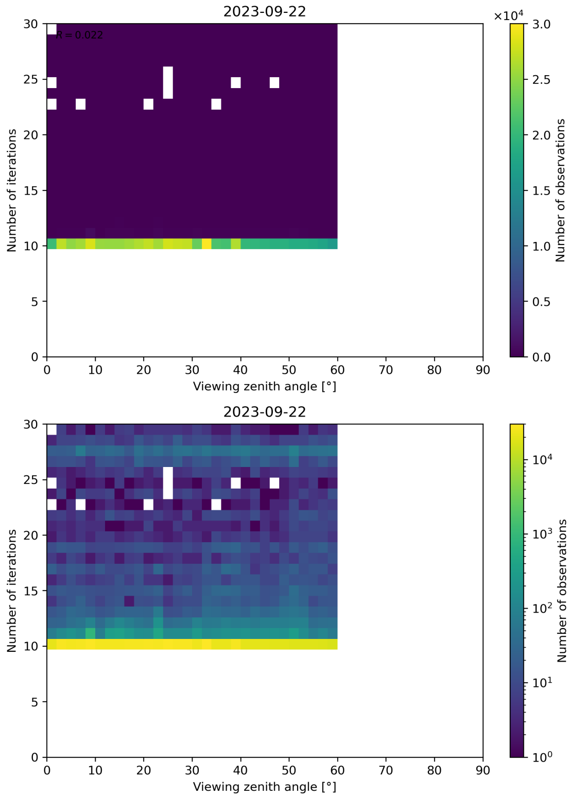
Figure 113: Scatter density plot of “Viewing zenith angle” against “Number of iterations” for 2023-09-21 to 2023-09-23.
