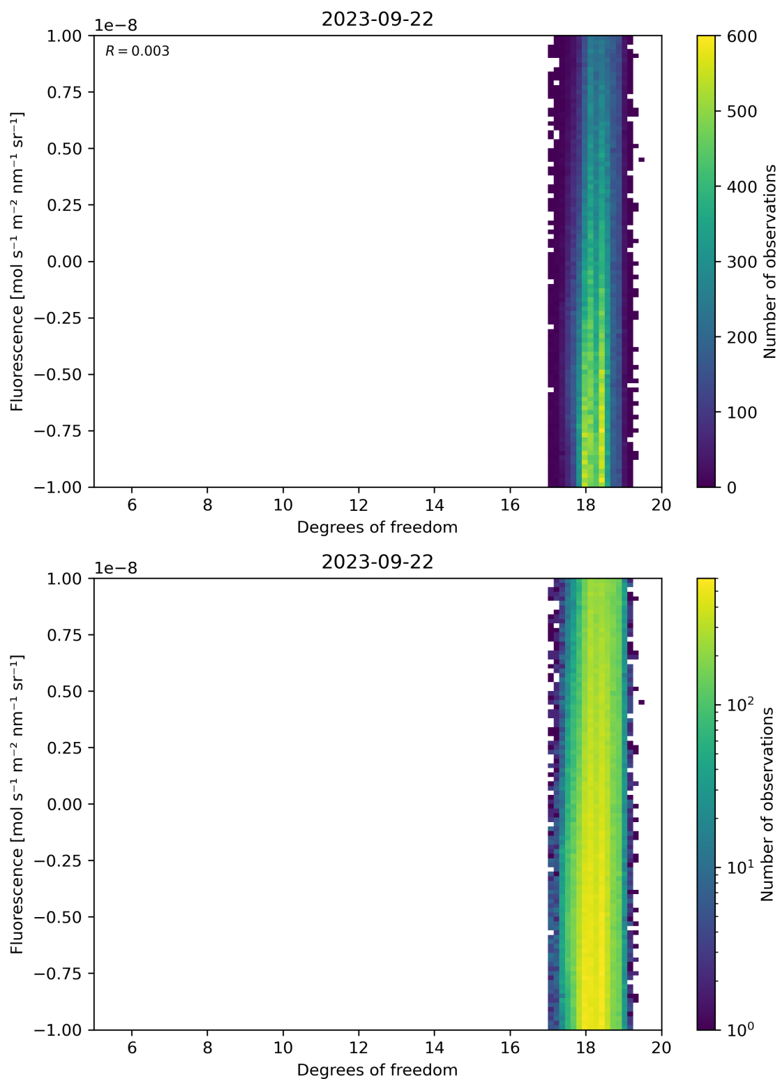
Figure 51: Scatter density plot of “Degrees of freedom” against “Fluorescence” for 2023-09-21 to 2023-09-23.
