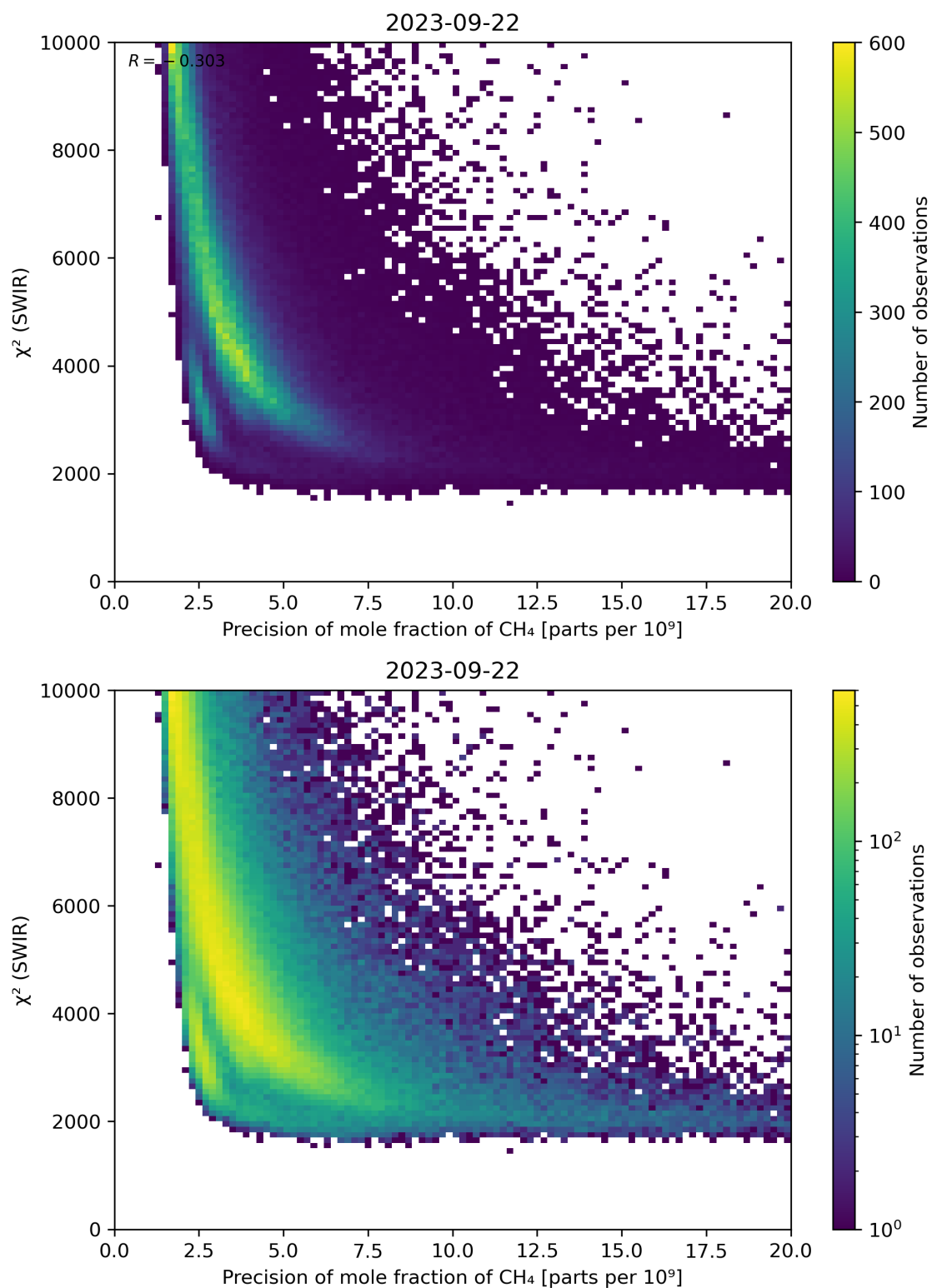
Figure 79: Scatter density plot of “Precision of mole fraction of CH 4 ” against “ \chi^2 (SWIR)” for 2023-09-21 to 2023-09-23.
