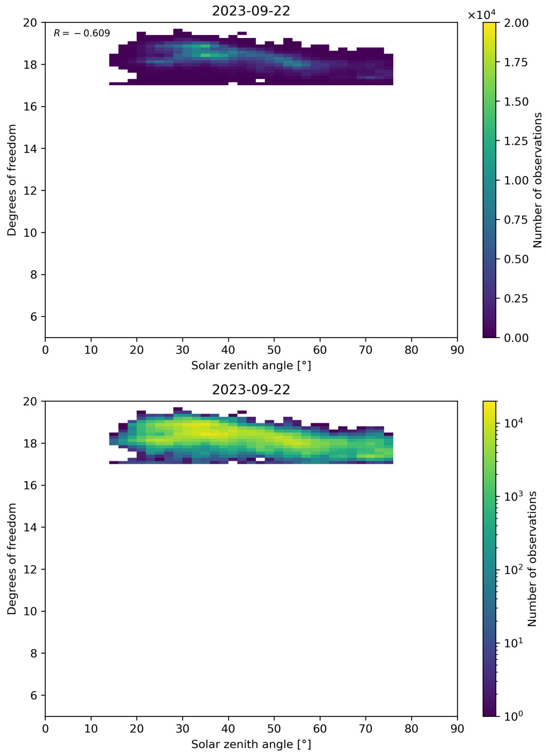
Figure 96: Scatter density plot of “Solar zenith angle” against “Degrees of freedom” for 2023-09-21 to 2023-09-23.
