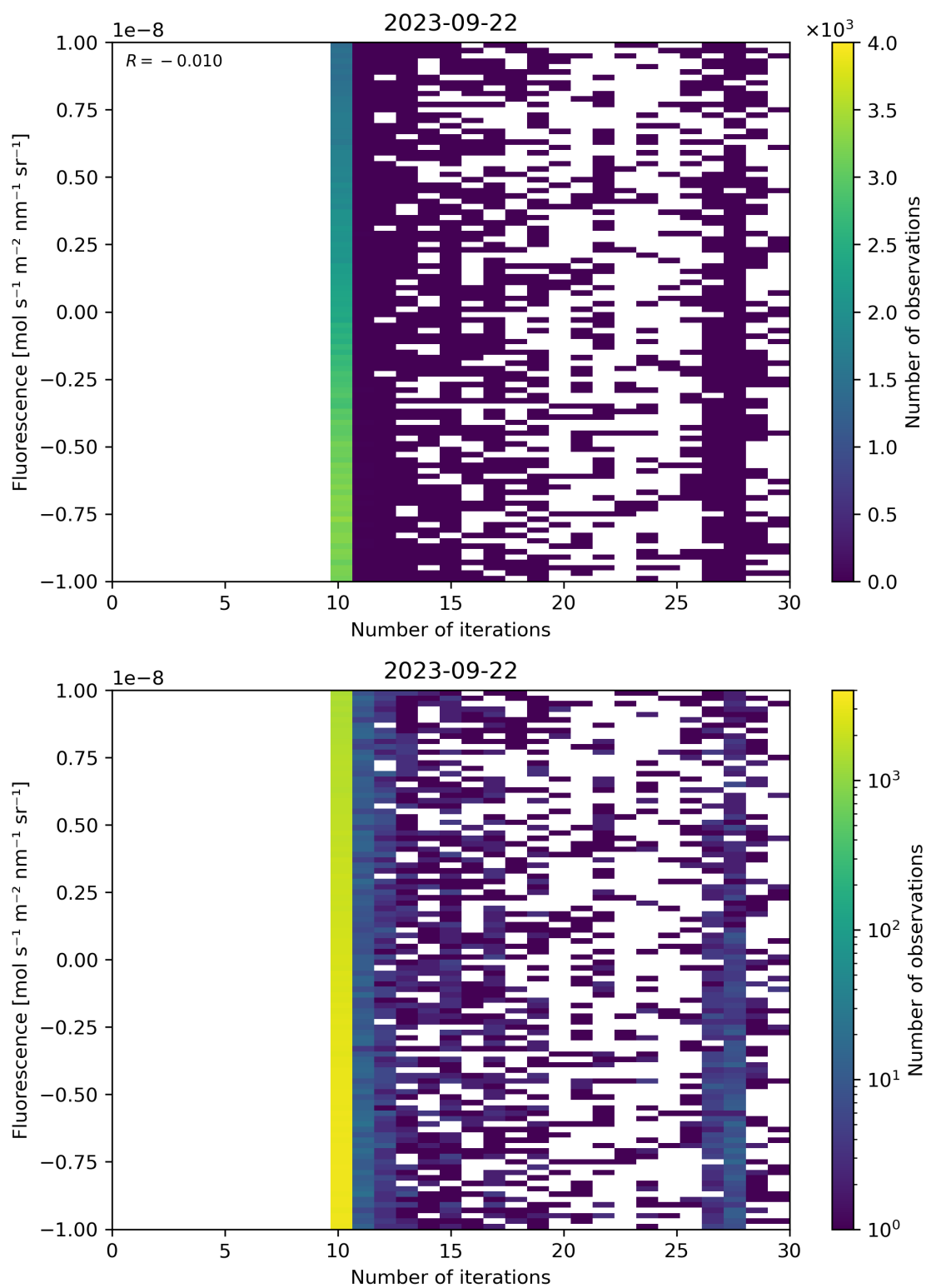
Figure 87: Scatter density plot of “Number of iterations” against “Fluorescence” for 2023-09-21 to 2023-09-23.
