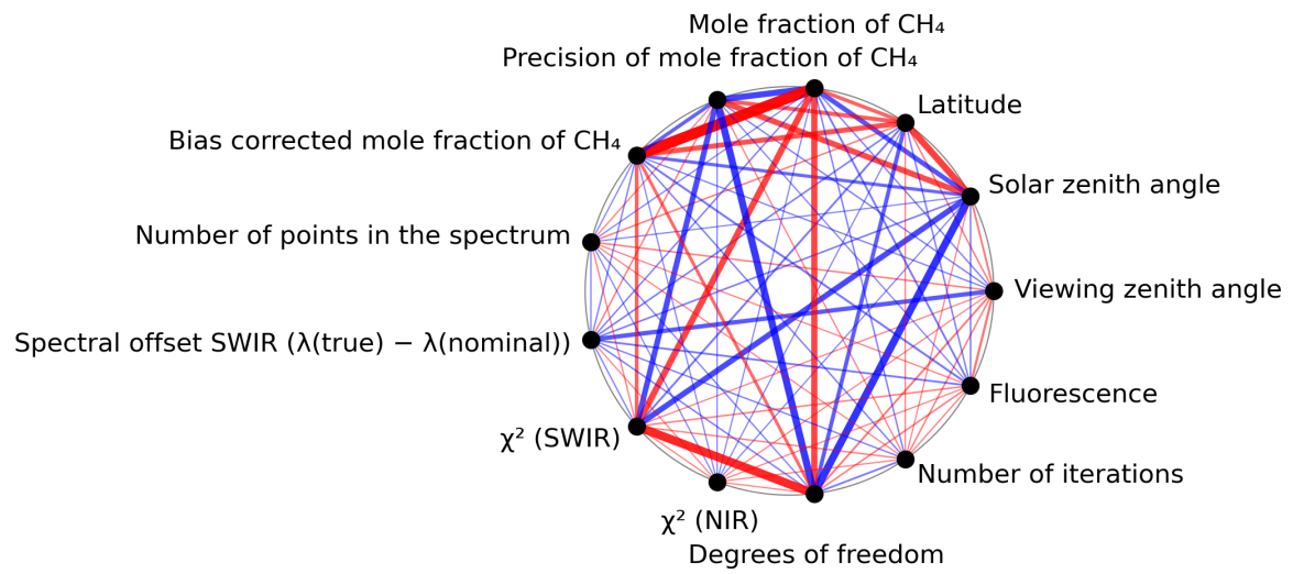
Figure 1: Map of correlation graph for 2023-09-22 to 2023-09-24.
