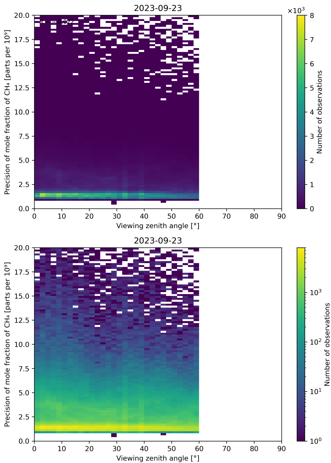
Figure 112: Scatter density plot of “Viewing zenith angle” against “Precision of mole fraction of CH 4 ” for 2023-09-22 to 2023-09-24.
