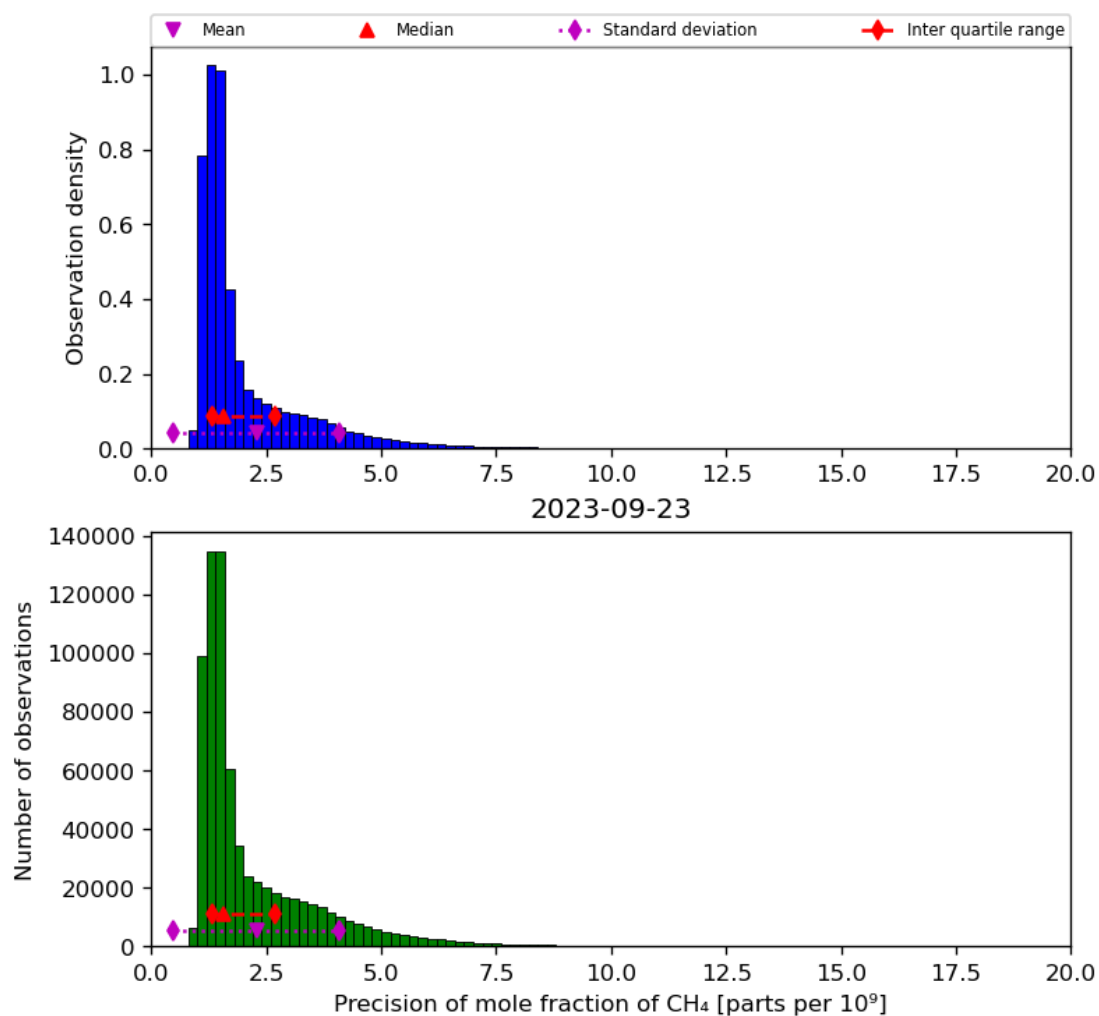
Figure 24: Histogram of “Precision of mole fraction of CH 4 ” for 2023-09-22 to 2023-09-24
