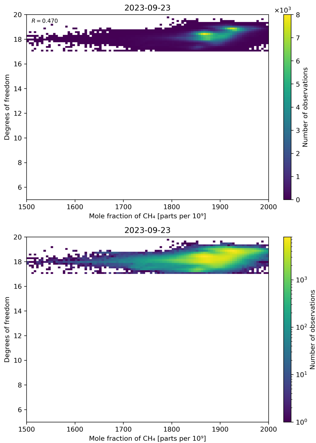
Figure 72: Scatter density plot of “Mole fraction of CH 4 ” against “Degrees of freedom” for 2023-09-22 to 2023-09-24.
