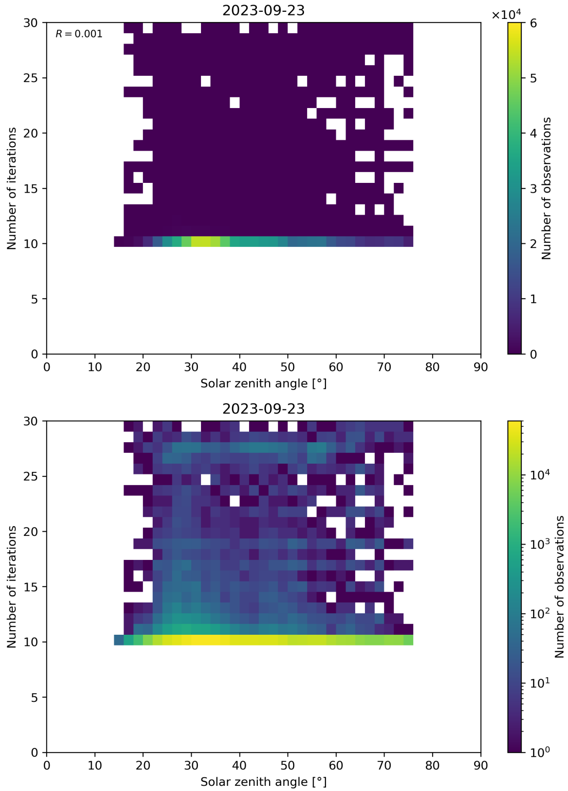
Figure 102: Scatter density plot of “Solar zenith angle” against “Number of iterations” for 2023-09-22 to 2023-09-24.
