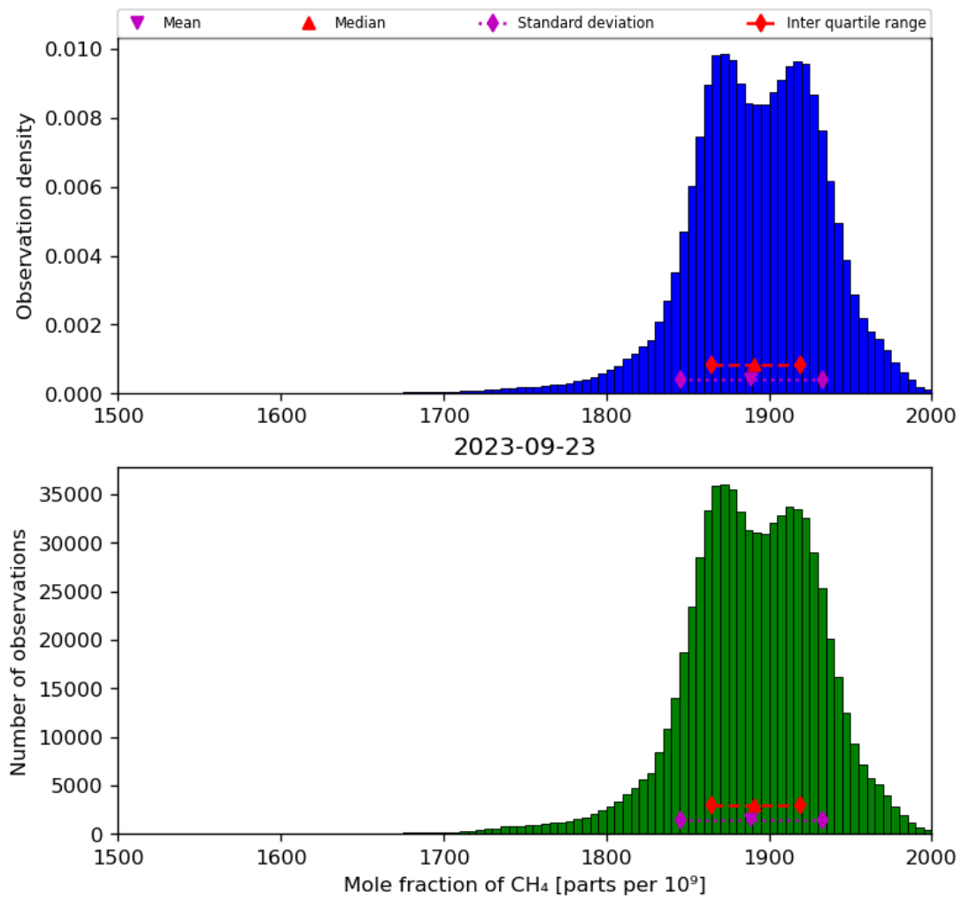
Figure 23: Histogram of “Mole fraction of CH 4 ” for 2023-09-22 to 2023-09-24
