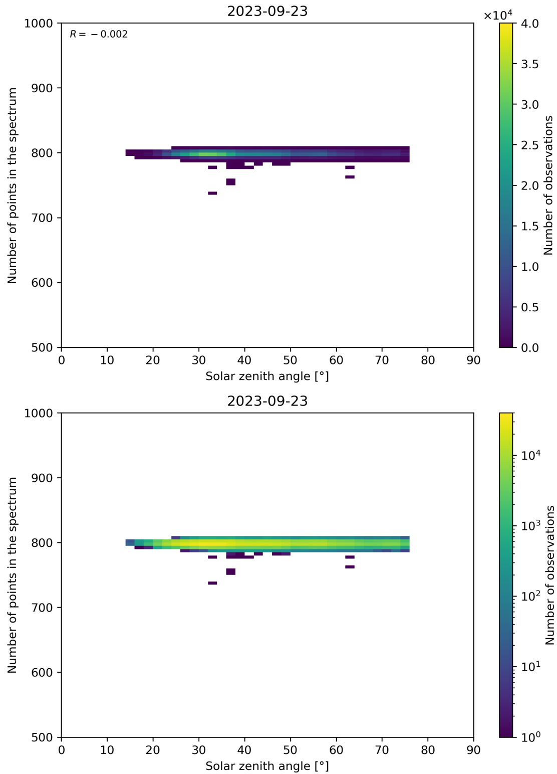
Figure 103: Scatter density plot of “Solar zenith angle” against “Number of points in the spectrum” for 2023-09-22 to 2023-09-24.
