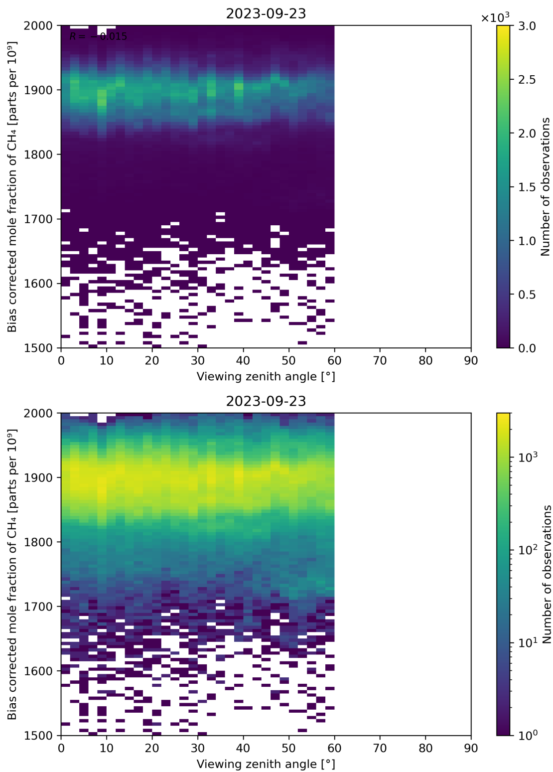
Figure 111: Scatter density plot of “Viewing zenith angle” against “Bias corrected mole fraction of CH 4 ” for 2023-09-22 to 2023-09-24.
