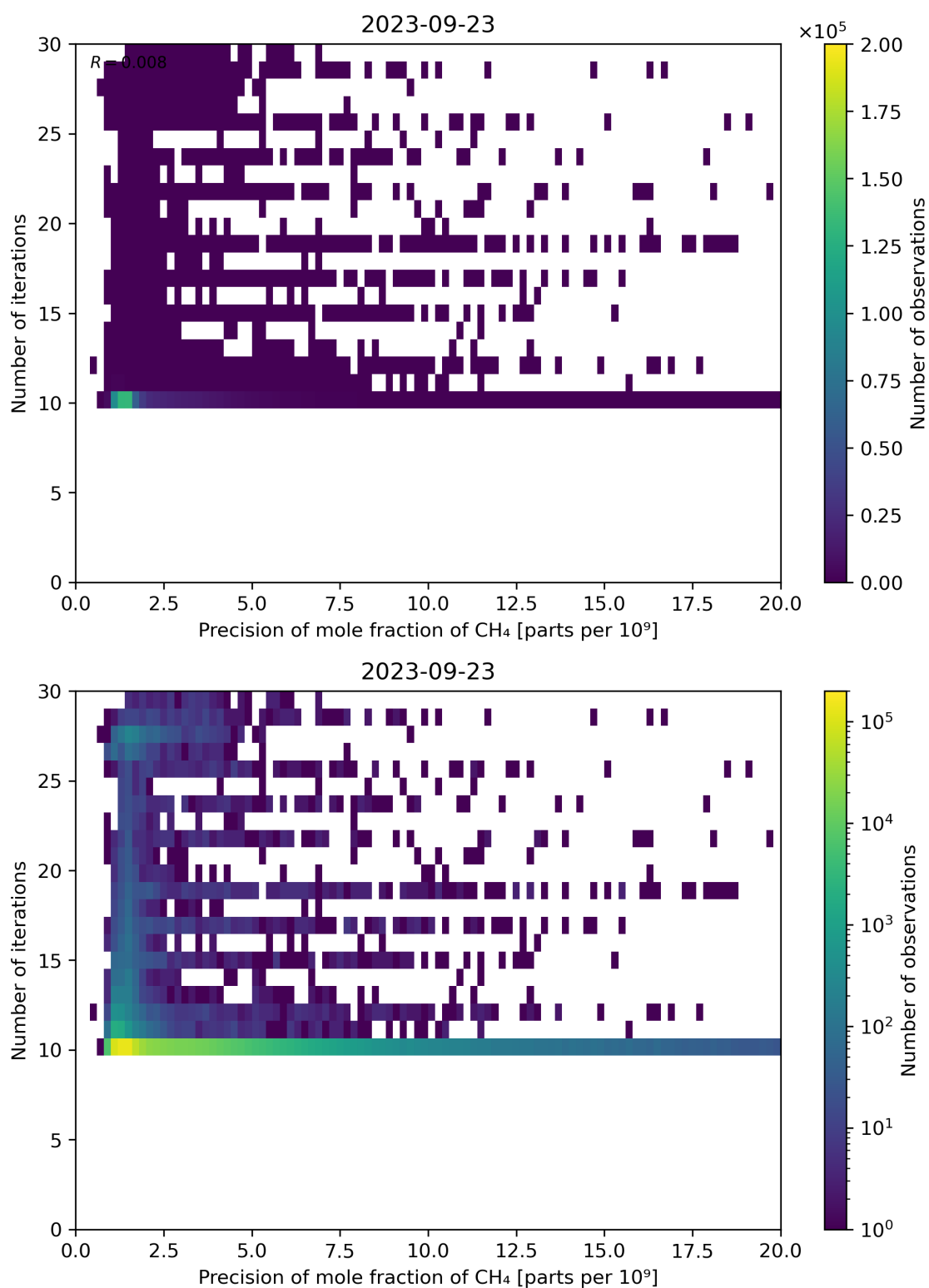
Figure 83: Scatter density plot of “Precision of mole fraction of CH 4 ” against “Number of iterations” for 2023-09-22 to 2023-09-24.
