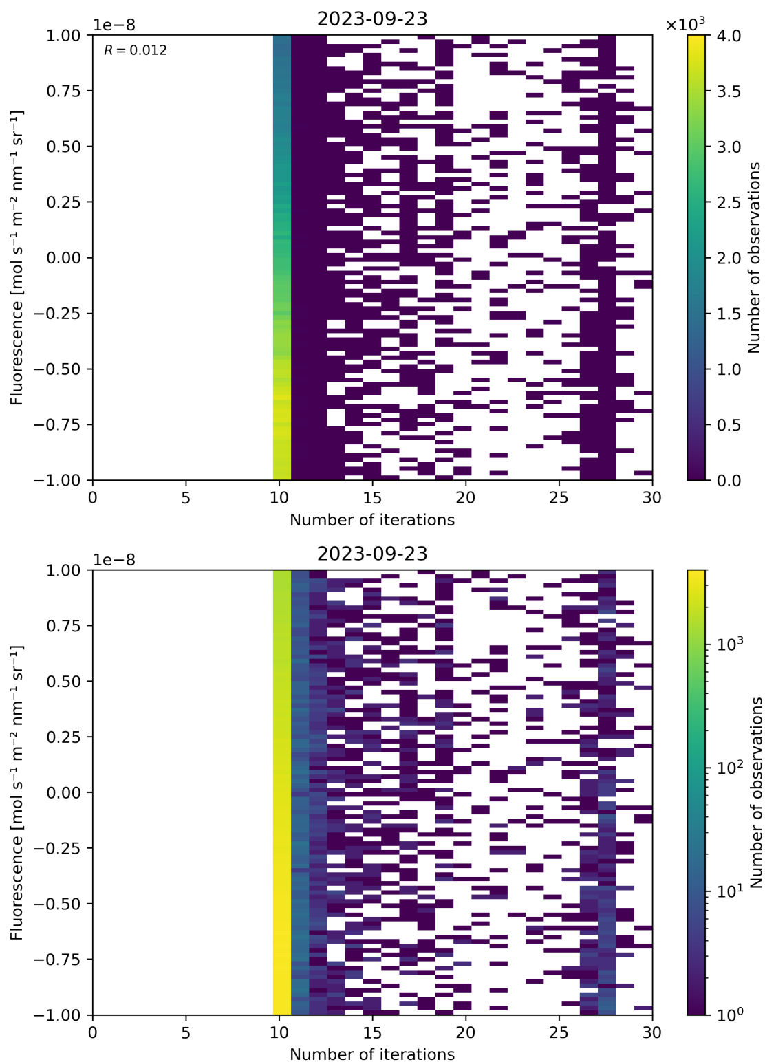
Figure 87: Scatter density plot of “Number of iterations” against “Fluorescence” for 2023-09-22 to 2023-09-24.
