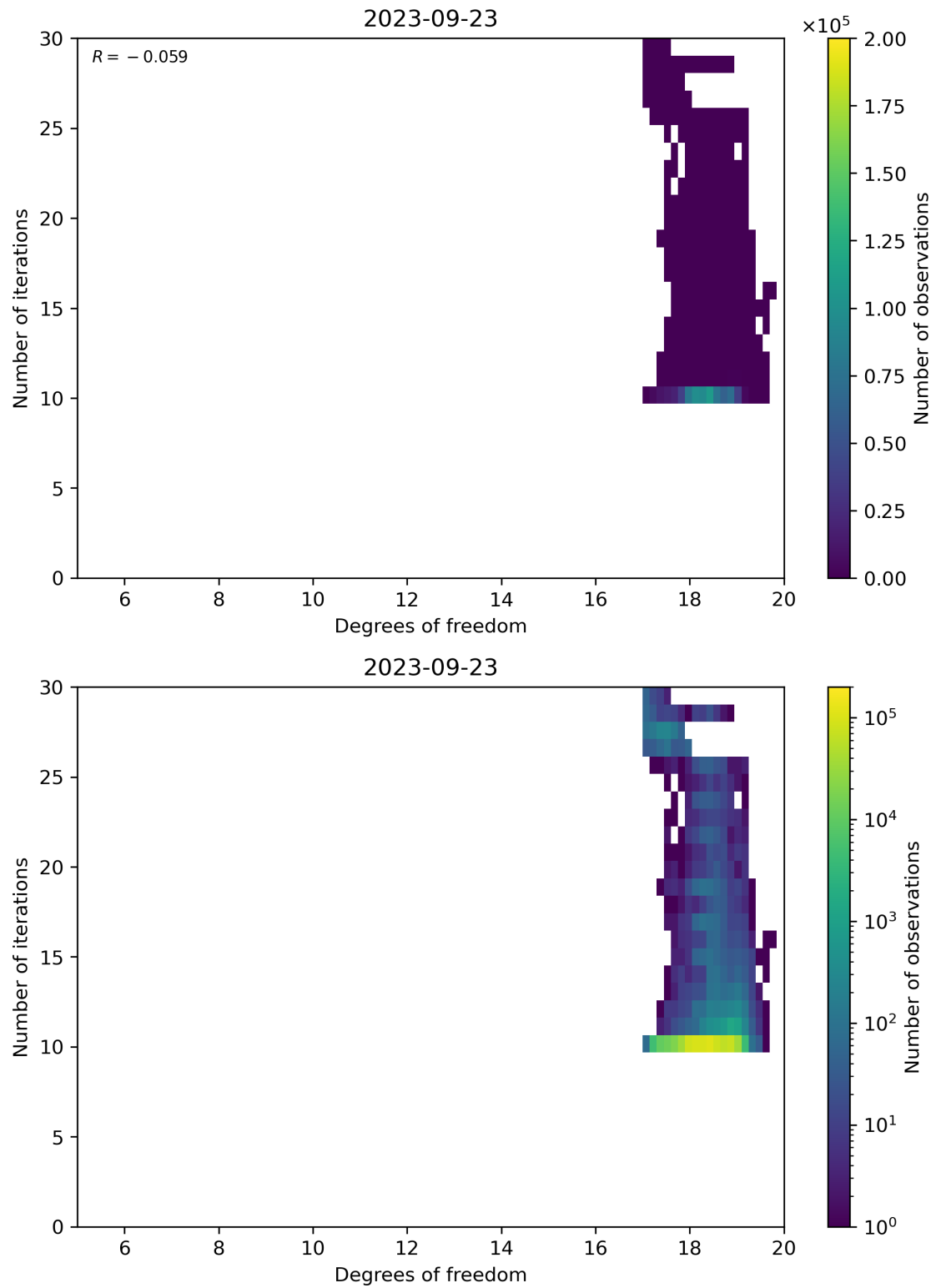
Figure 52: Scatter density plot of “Degrees of freedom” against “Number of iterations” for 2023-09-22 to 2023-09-24.
