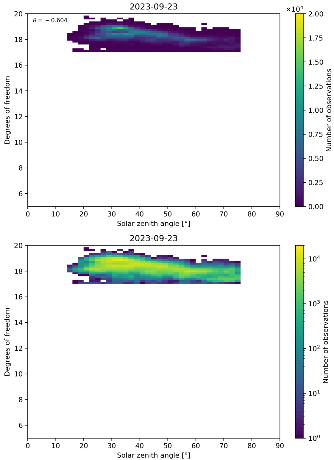
Figure 96: Scatter density plot of “Solar zenith angle” against “Degrees of freedom” for 2023-09-22 to 2023-09-24.
