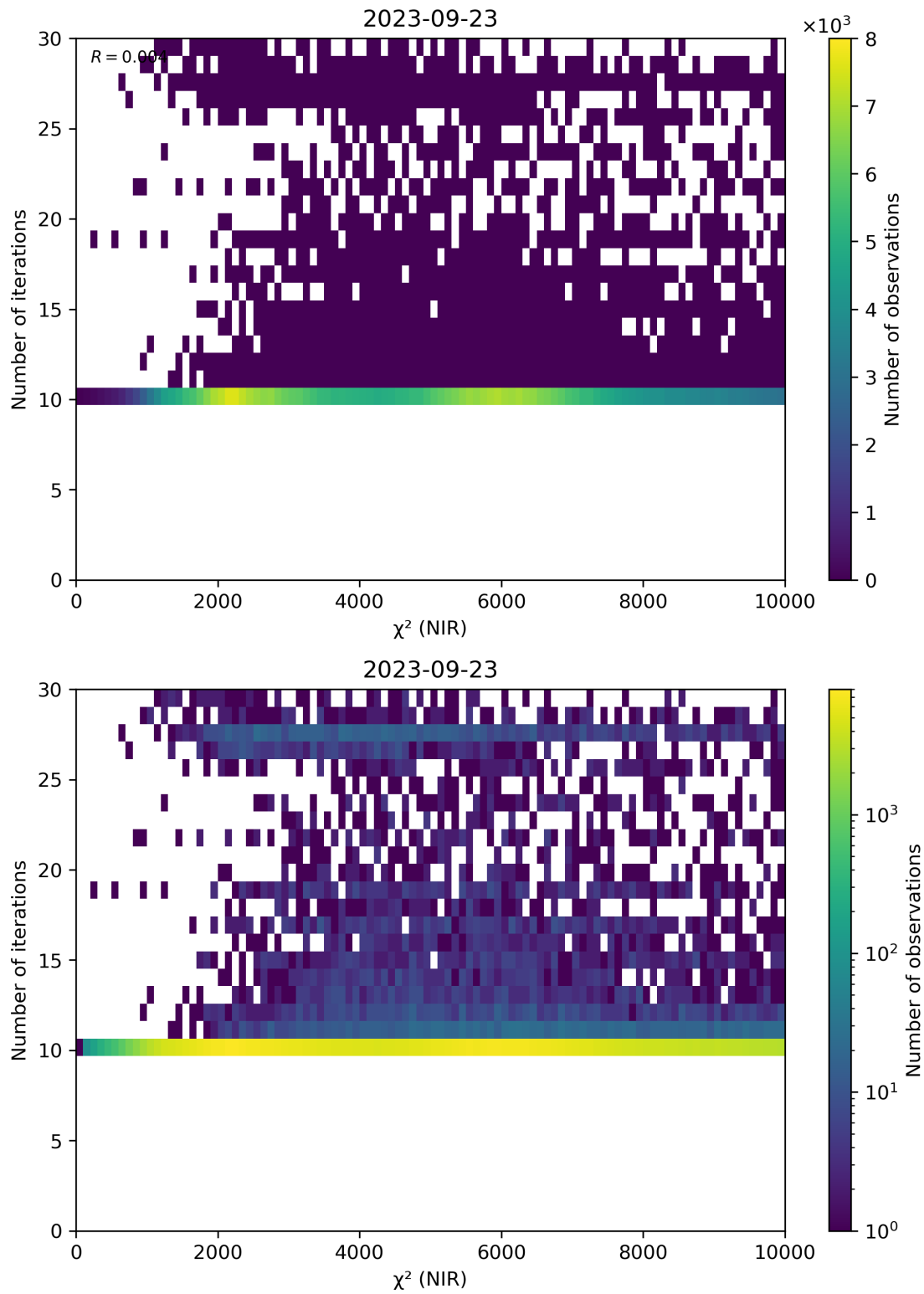
Figure 46: Scatter density plot of “ \chi^2 (NIR)” against “Number of iterations” for 2023-09-22 to 2023-09-24.
