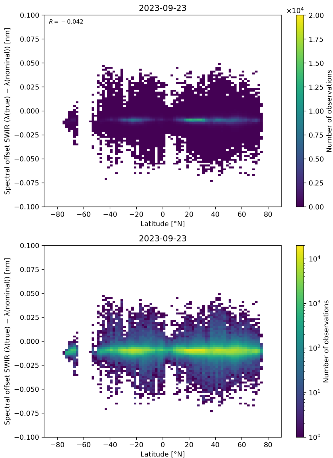
Figure 62: Scatter density plot of “Latitude” against “Spectral offset SWIR ( \lambda(\text{true}) - \lambda(\text{nominal}) )” for 2023-09-22 to 2023-09-24.
