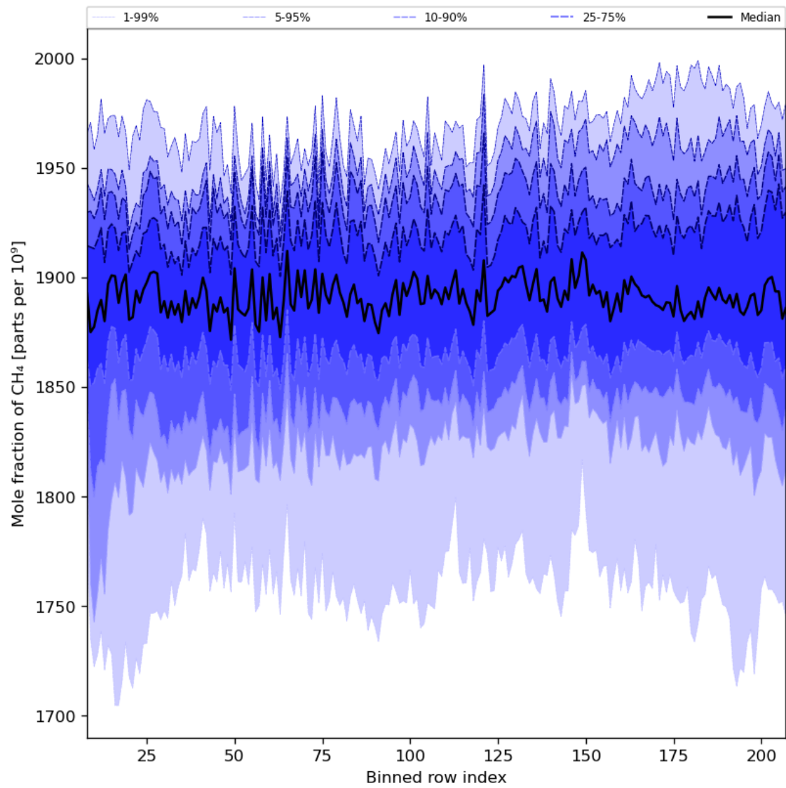
Figure 34: Along track statistics of “Mole fraction of CH 4 ” for 2023-09-22 to 2023-09-24
