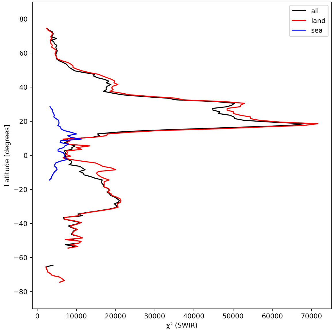
Figure 17: Zonal average of “ \chi^2 (SWIR)” for 2023-09-22 to 2023-09-24.
