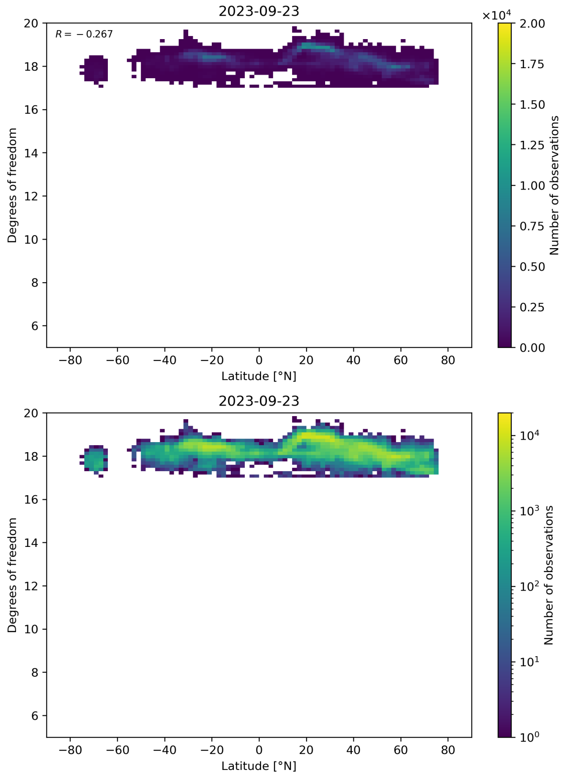
Figure 55: Scatter density plot of “Latitude” against “Degrees of freedom” for 2023-09-22 to 2023-09-24.
