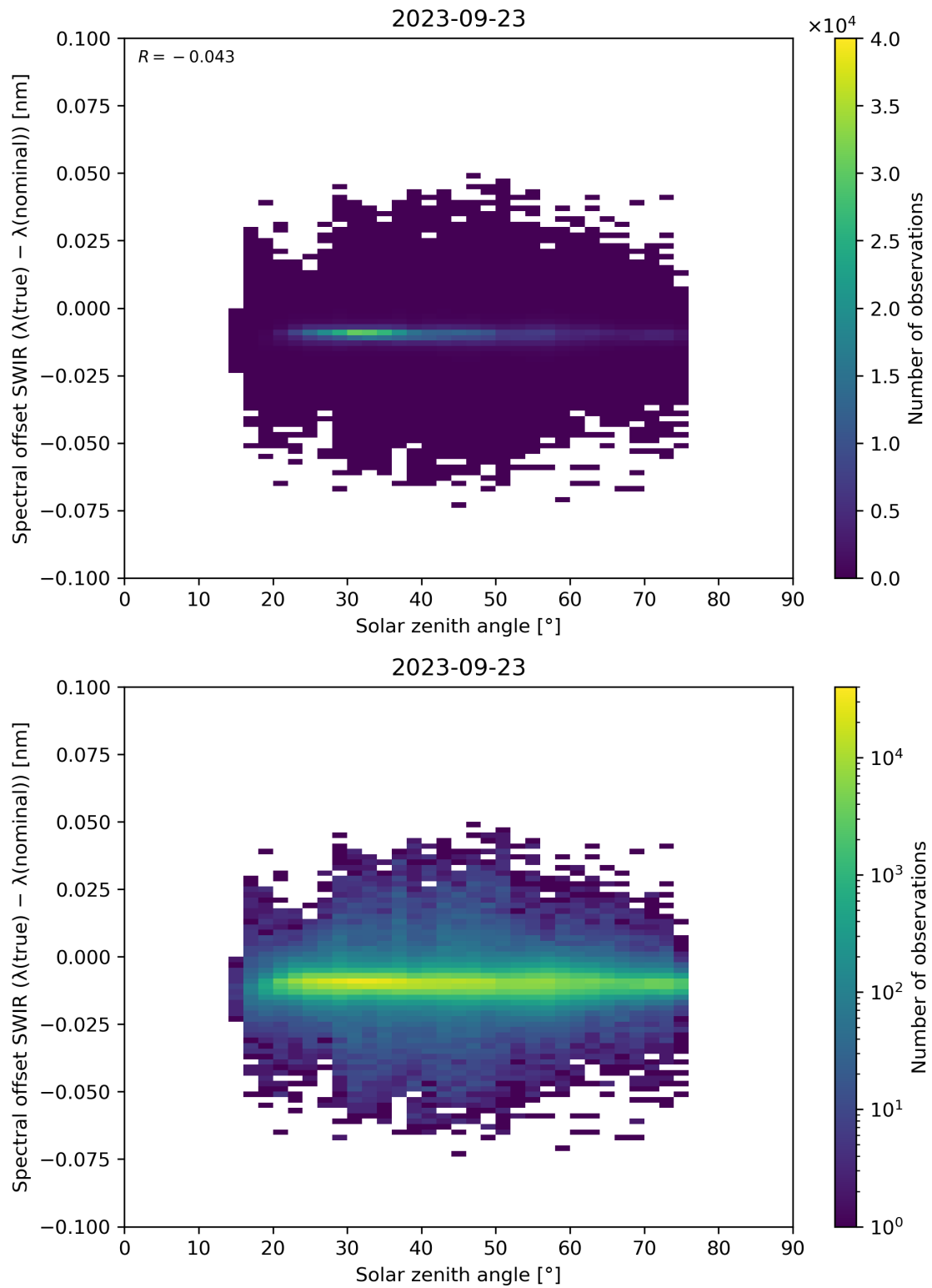
Figure 104: Scatter density plot of “Solar zenith angle” against “Spectral offset SWIR ( \lambda(\text{true}) - \lambda(\text{nominal}) )” for 2023-09-22 to 2023-09-24.
