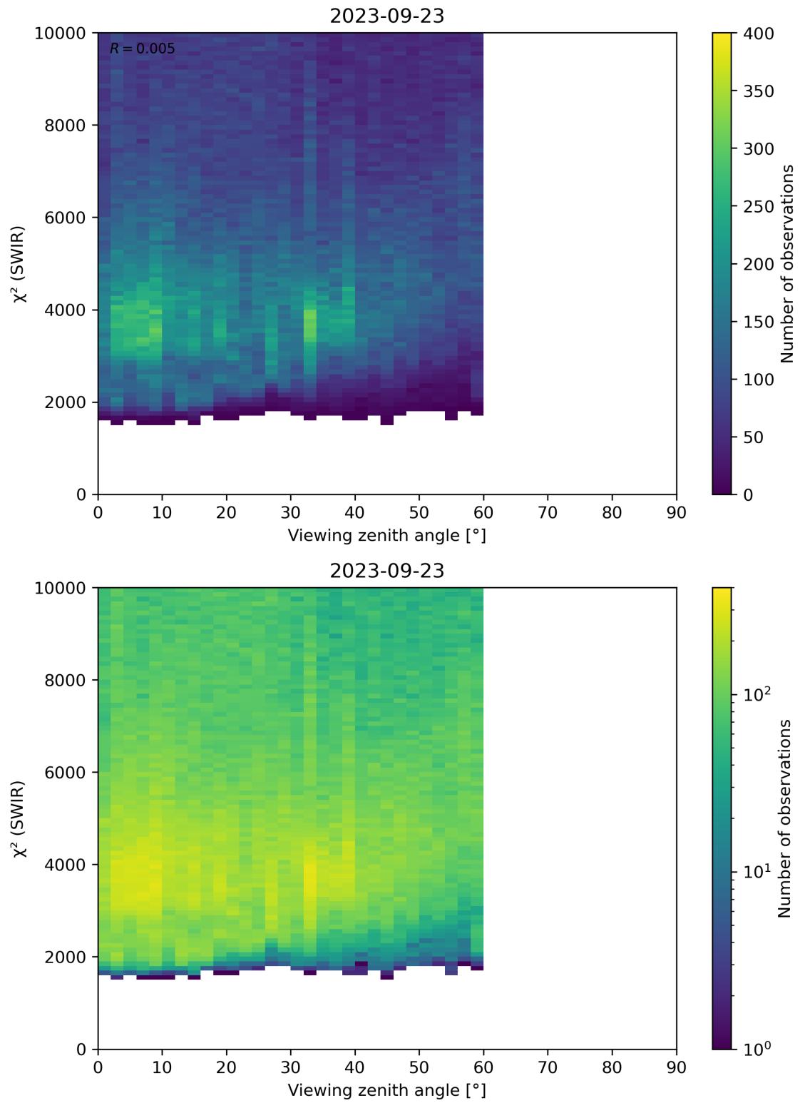
Figure 106: Scatter density plot of “Viewing zenith angle” against “ \chi^2 (SWIR)” for 2023-09-22 to 2023-09-24.
