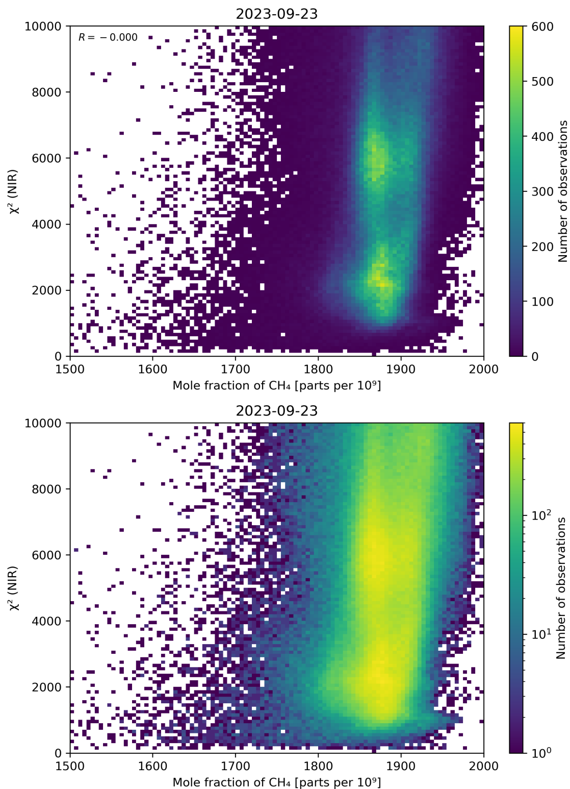
Figure 70: Scatter density plot of “Mole fraction of CH 4 ” against “ \chi^2 (NIR)” for 2023-09-22 to 2023-09-24.
