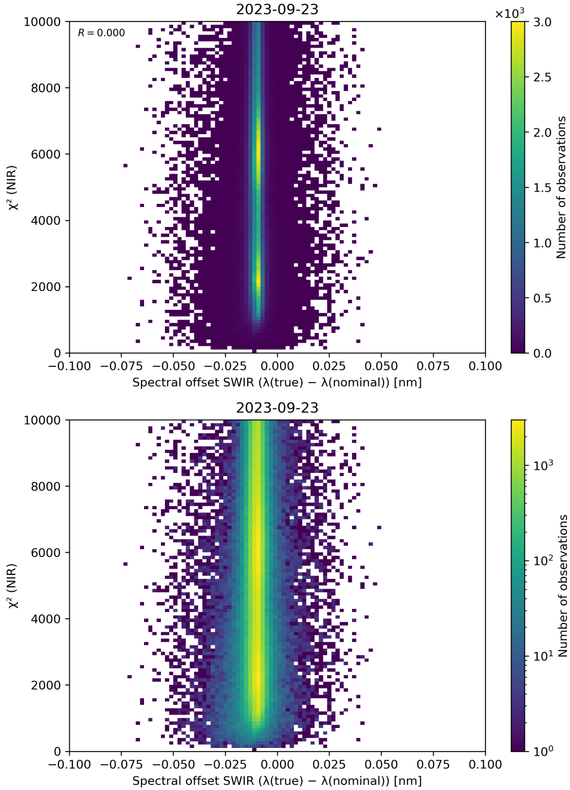
Figure 117: Scatter density plot of “Spectral offset SWIR ( \lambda(\text{true}) - \lambda(\text{nominal}) )” against “ \chi^2 (NIR)” for 2023-09-22 to 2023-09-24.
