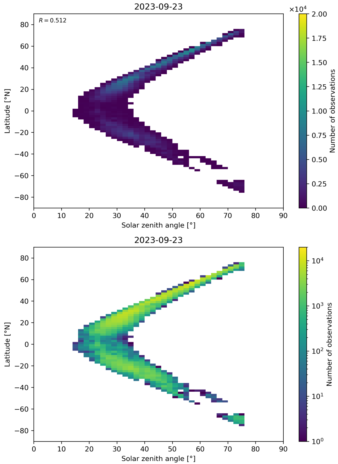
Figure 98: Scatter density plot of “Solar zenith angle” against “Latitude” for 2023-09-22 to 2023-09-24.
