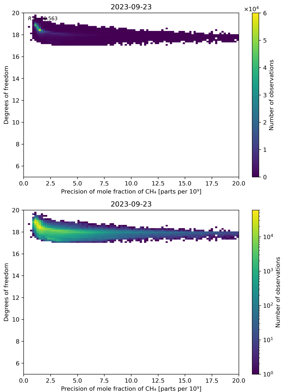
Figure 80: Scatter density plot of “Precision of mole fraction of CH 4 ” against “Degrees of freedom” for 2023-09-22 to 2023-09-24.
