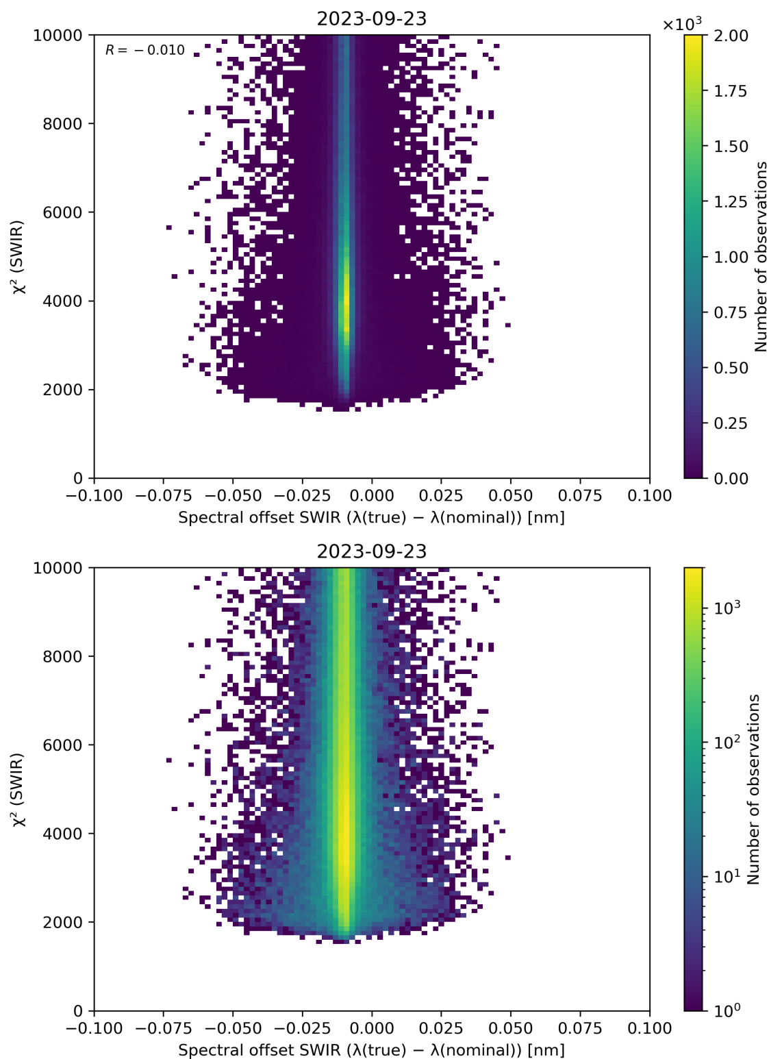
Figure 118: Scatter density plot of “Spectral offset SWIR ( \lambda(\text{true}) - \lambda(\text{nominal}) )” against “ \chi^2 (SWIR)” for 2023-09-22 to 2023-09-24.
