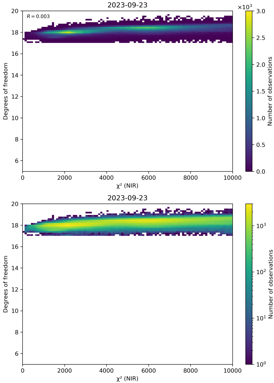
Figure 44: Scatter density plot of “ \chi^2 (NIR)” against “Degrees of freedom” for 2023-09-22 to 2023-09-24.
