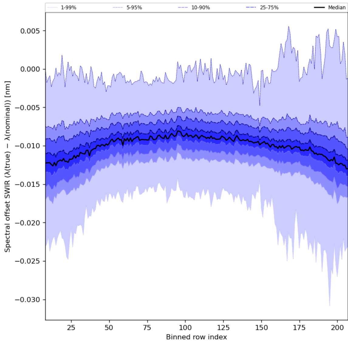
Figure 38: Along track statistics of “Spectral offset SWIR ( \lambda(\text{true}) - \lambda(\text{nominal}) )” for 2023-09-22 to 2023-09-24
