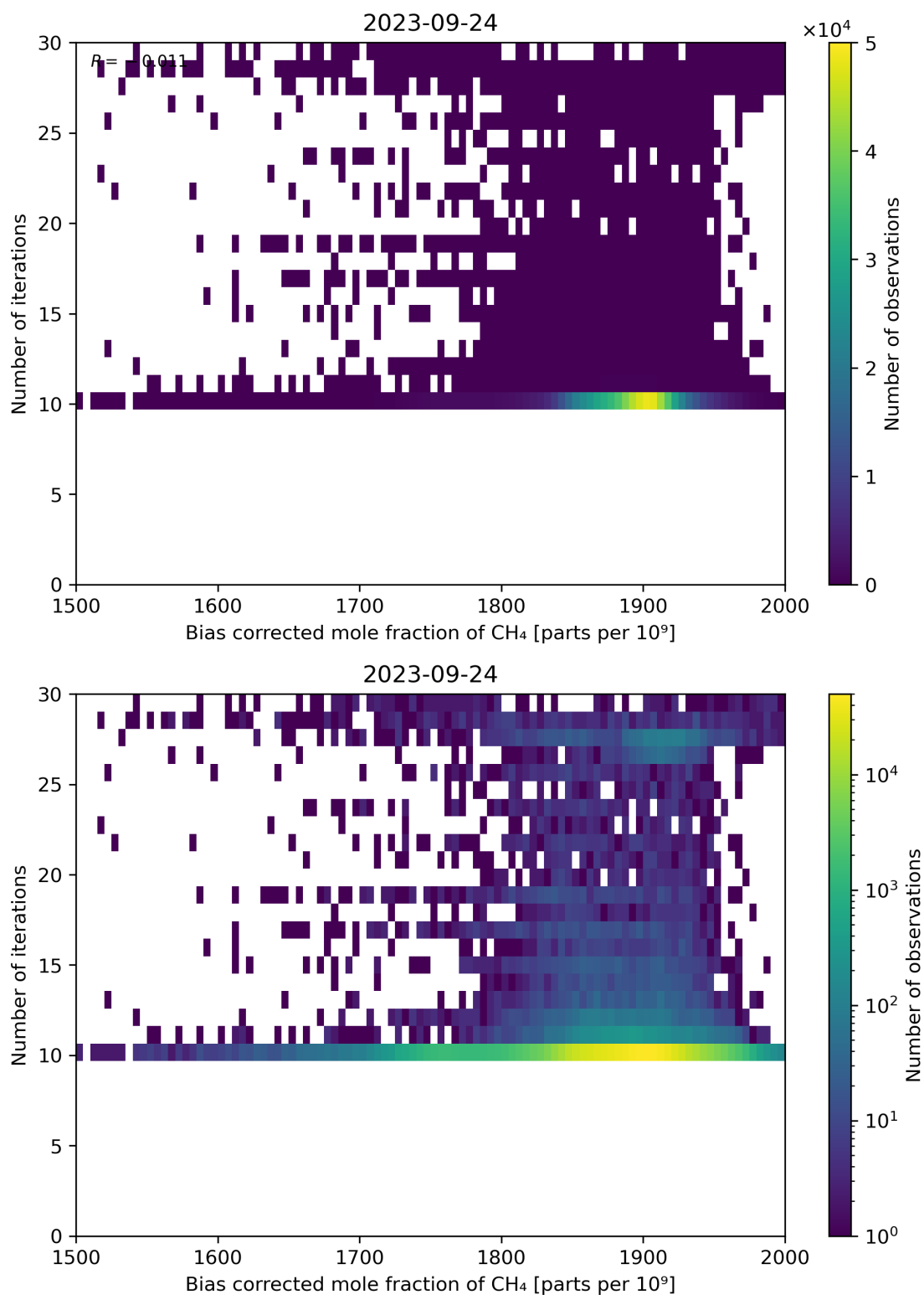
Figure 67: Scatter density plot of “Bias corrected mole fraction of \text{CH}_4 ” against “Number of iterations” for 2023-09-23 to 2023-09-25.
