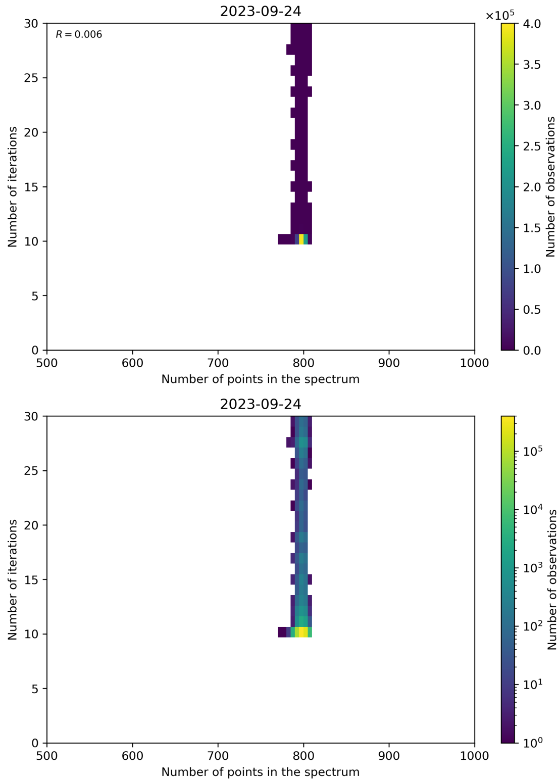
Figure 92: Scatter density plot of “Number of points in the spectrum” against “Number of iterations” for 2023-09-23 to 2023-09-25.
