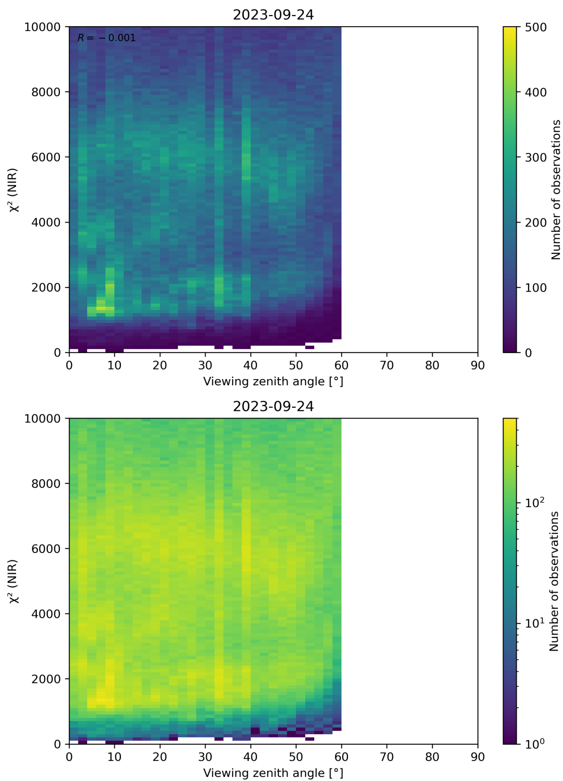
Figure 105: Scatter density plot of “Viewing zenith angle” against “ \chi^2 (NIR)” for 2023-09-23 to 2023-09-25.
