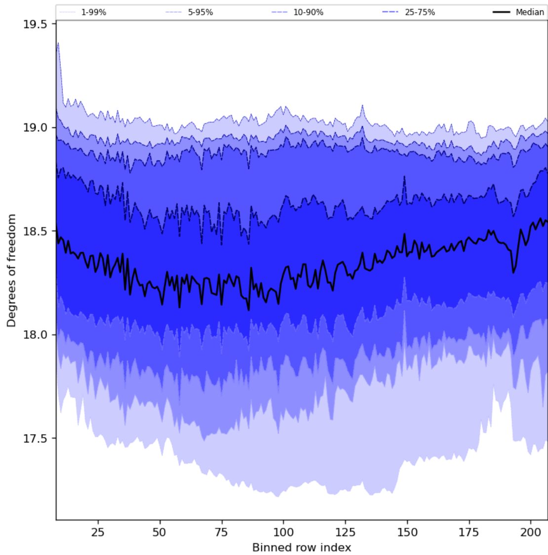
Figure 41: Along track statistics of “Degrees of freedom” for 2023-09-23 to 2023-09-25
