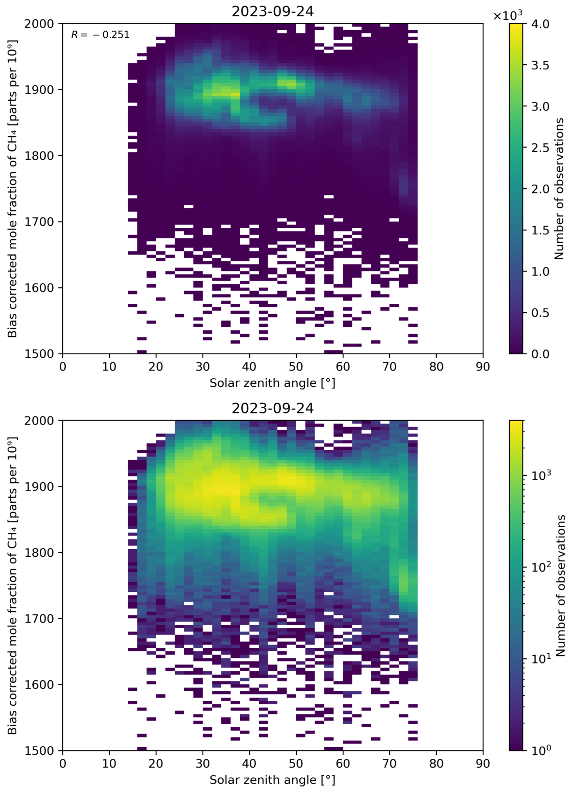
Figure 100: Scatter density plot of “Solar zenith angle” against “Bias corrected mole fraction of \text{CH}_4 ” for 2023-09-23 to 2023-09-25.
