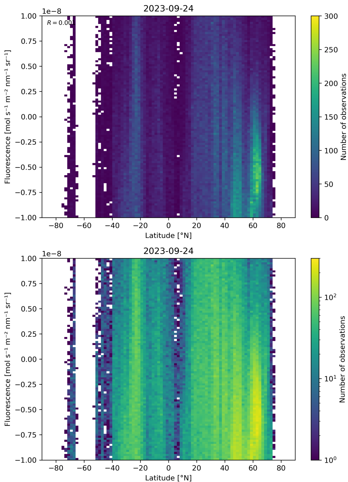
Figure 56: Scatter density plot of “Latitude” against “Fluorescence” for 2023-09-23 to 2023-09-25.
