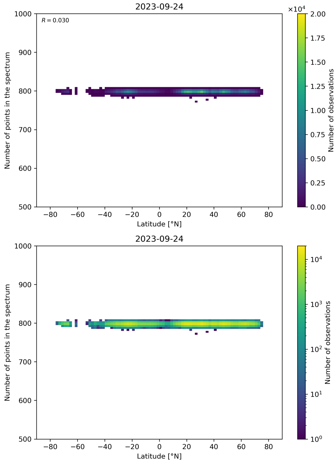
Figure 61: Scatter density plot of “Latitude” against “Number of points in the spectrum” for 2023-09-23 to 2023-09-25.
