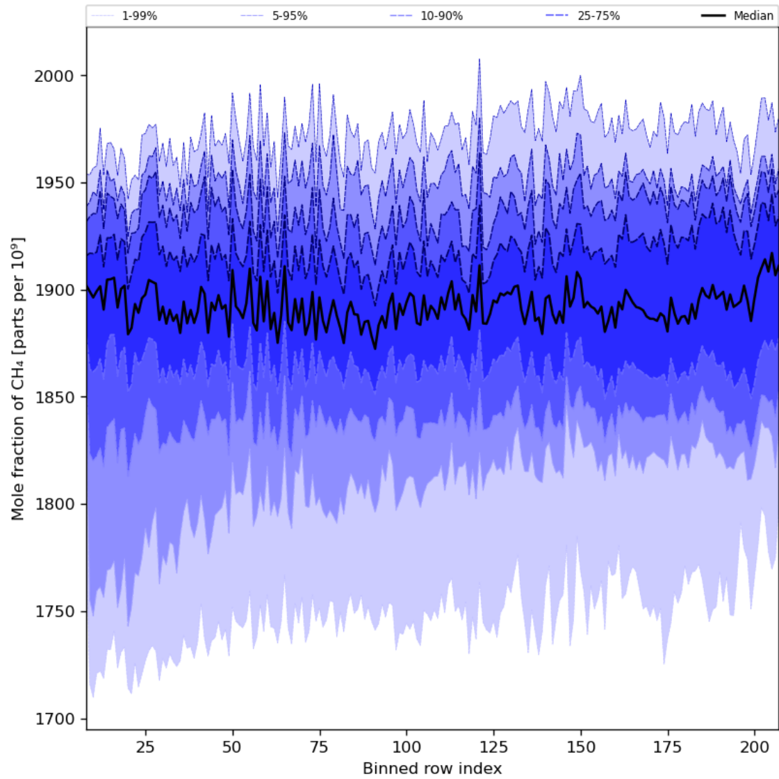
Figure 34: Along track statistics of “Mole fraction of CH 4 ” for 2023-09-23 to 2023-09-25
