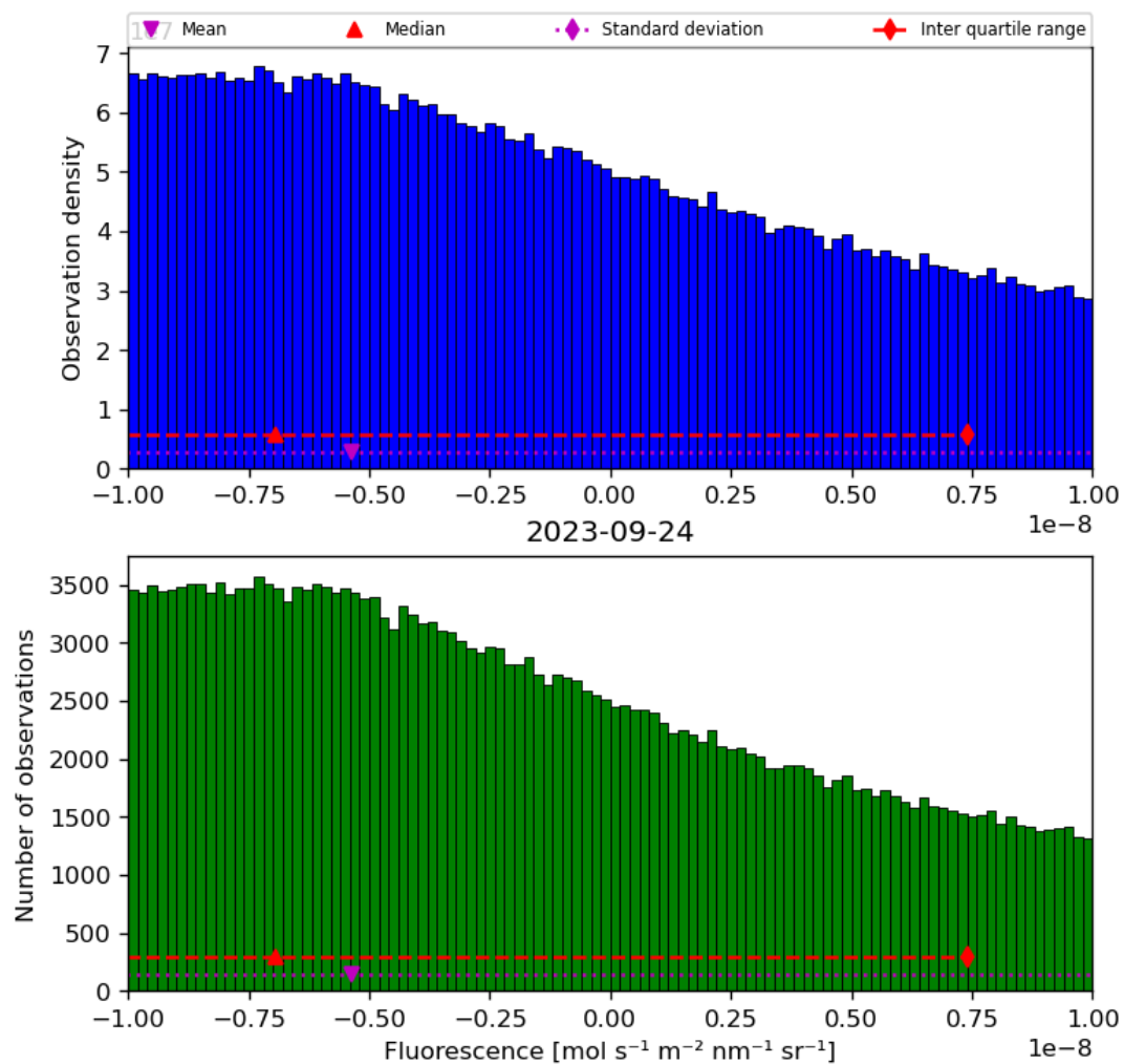
Figure 32: Histogram of “Fluorescence” for 2023-09-23 to 2023-09-25
