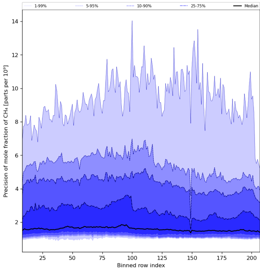
Figure 35: Along track statistics of “Precision of mole fraction of CH 4 ” for 2023-09-23 to 2023-09-25
