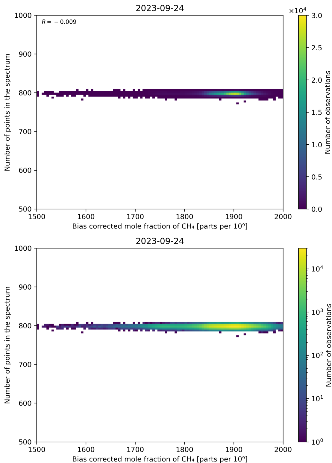
Figure 68: Scatter density plot of “Bias corrected mole fraction of CH 4 ” against “Number of points in the spectrum” for 2023-09-23 to 2023-09-25.
