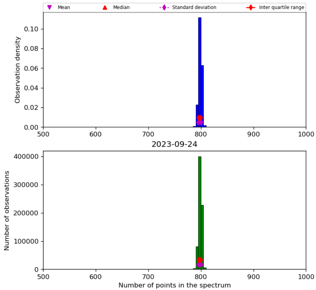
Figure 26: Histogram of “Number of points in the spectrum” for 2023-09-23 to 2023-09-25
