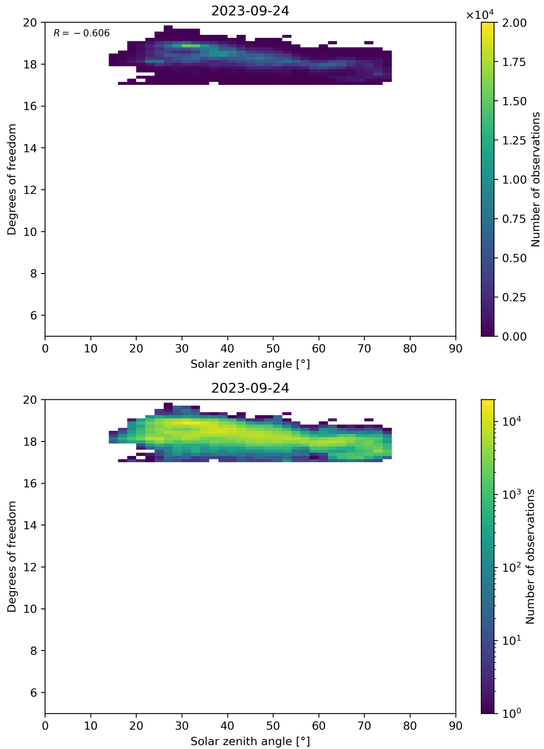
Figure 96: Scatter density plot of “Solar zenith angle” against “Degrees of freedom” for 2023-09-23 to 2023-09-25.
