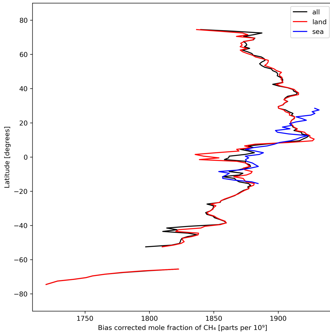
Figure 14: Zonal average of “Bias corrected mole fraction of \text{CH}_4 ” for 2023-09-23 to 2023-09-25.
