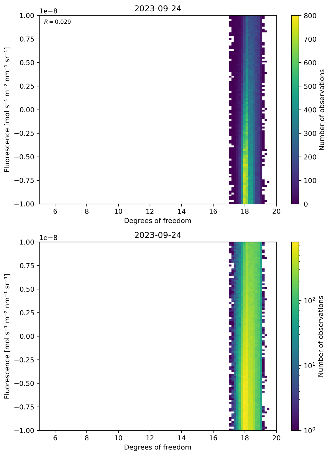
Figure 51: Scatter density plot of “Degrees of freedom” against “Fluorescence” for 2023-09-23 to 2023-09-25.
