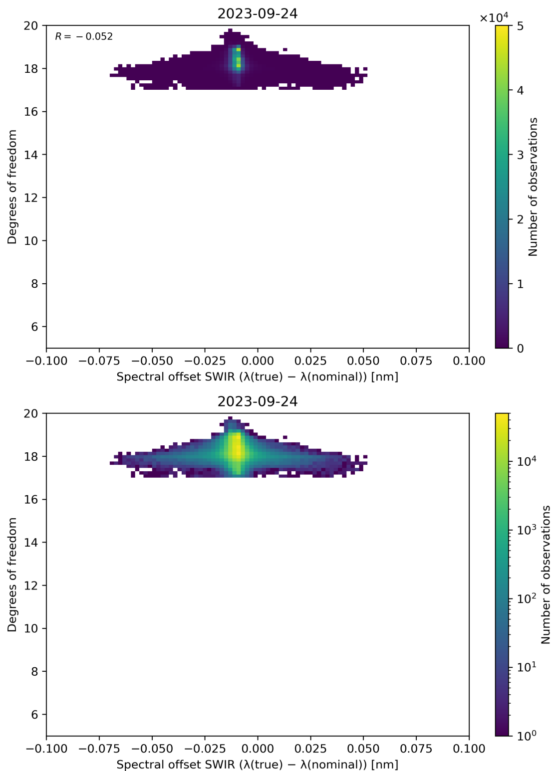
Figure 119: Scatter density plot of “Spectral offset SWIR ( \lambda(\text{true}) - \lambda(\text{nominal}) )” against “Degrees of freedom” for 2023-09-23 to 2023-09-25.
