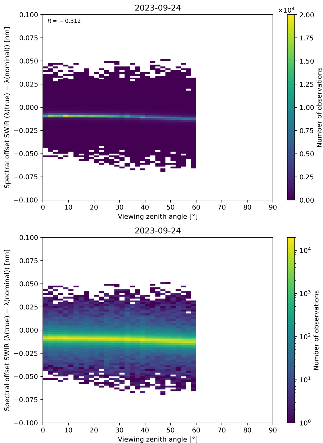
Figure 116: Scatter density plot of “Viewing zenith angle” against “Spectral offset SWIR ( \lambda(\text{true}) - \lambda(\text{nominal}) )” for 2023-09-23 to 2023-09-25.
