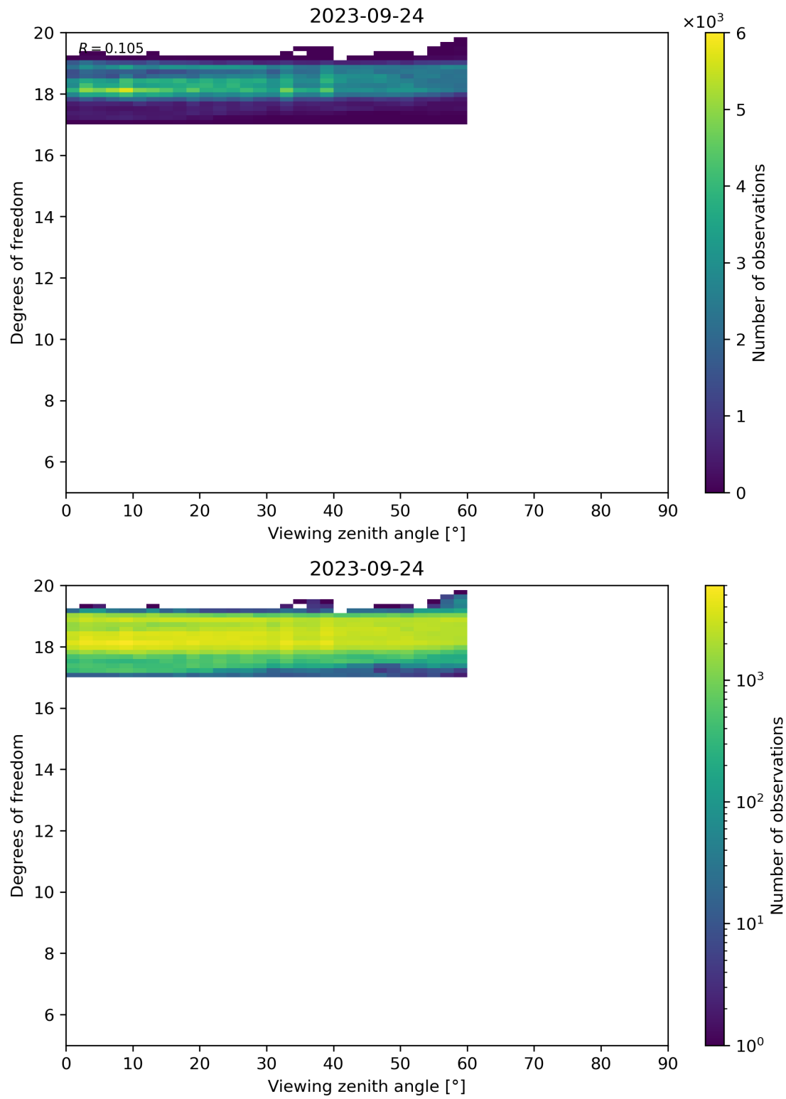
Figure 107: Scatter density plot of “Viewing zenith angle” against “Degrees of freedom” for 2023-09-23 to 2023-09-25.
