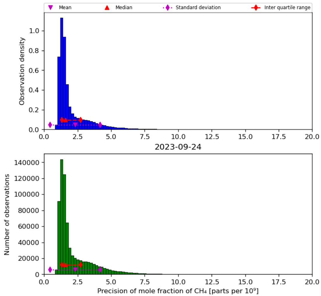
Figure 24: Histogram of “Precision of mole fraction of CH 4 ” for 2023-09-23 to 2023-09-25
