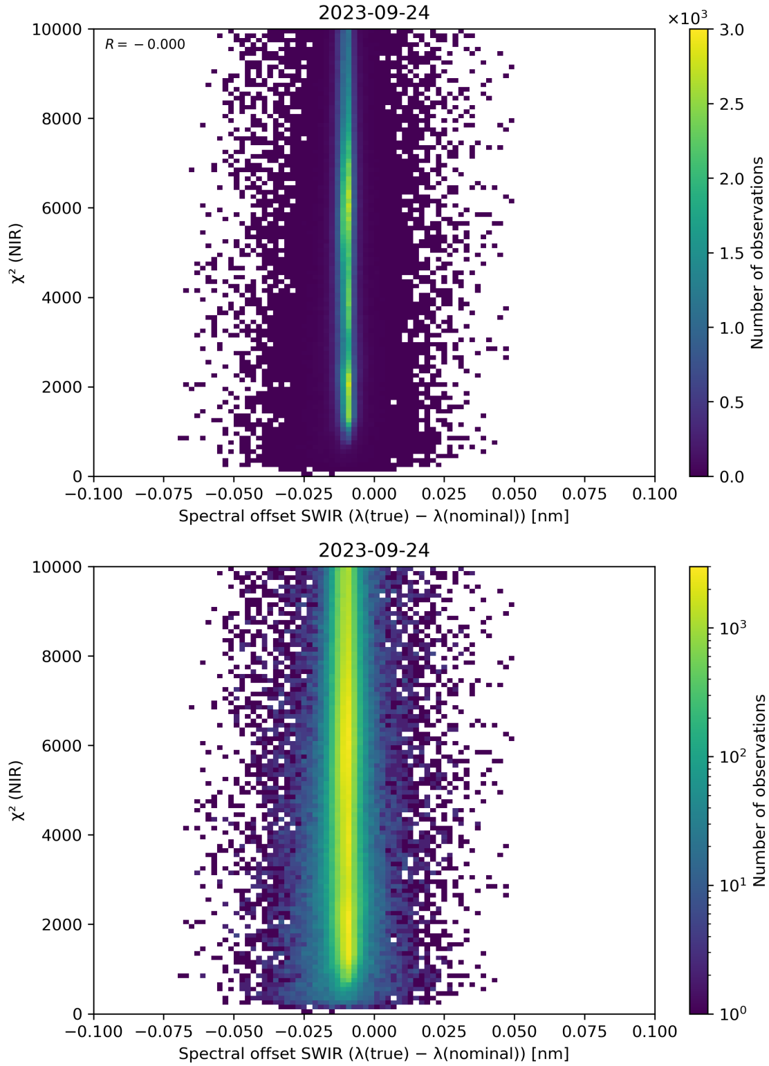
Figure 117: Scatter density plot of “Spectral offset SWIR ( \lambda(\text{true}) - \lambda(\text{nominal}) )” against “ \chi^2 (NIR)” for 2023-09-23 to 2023-09-25.
