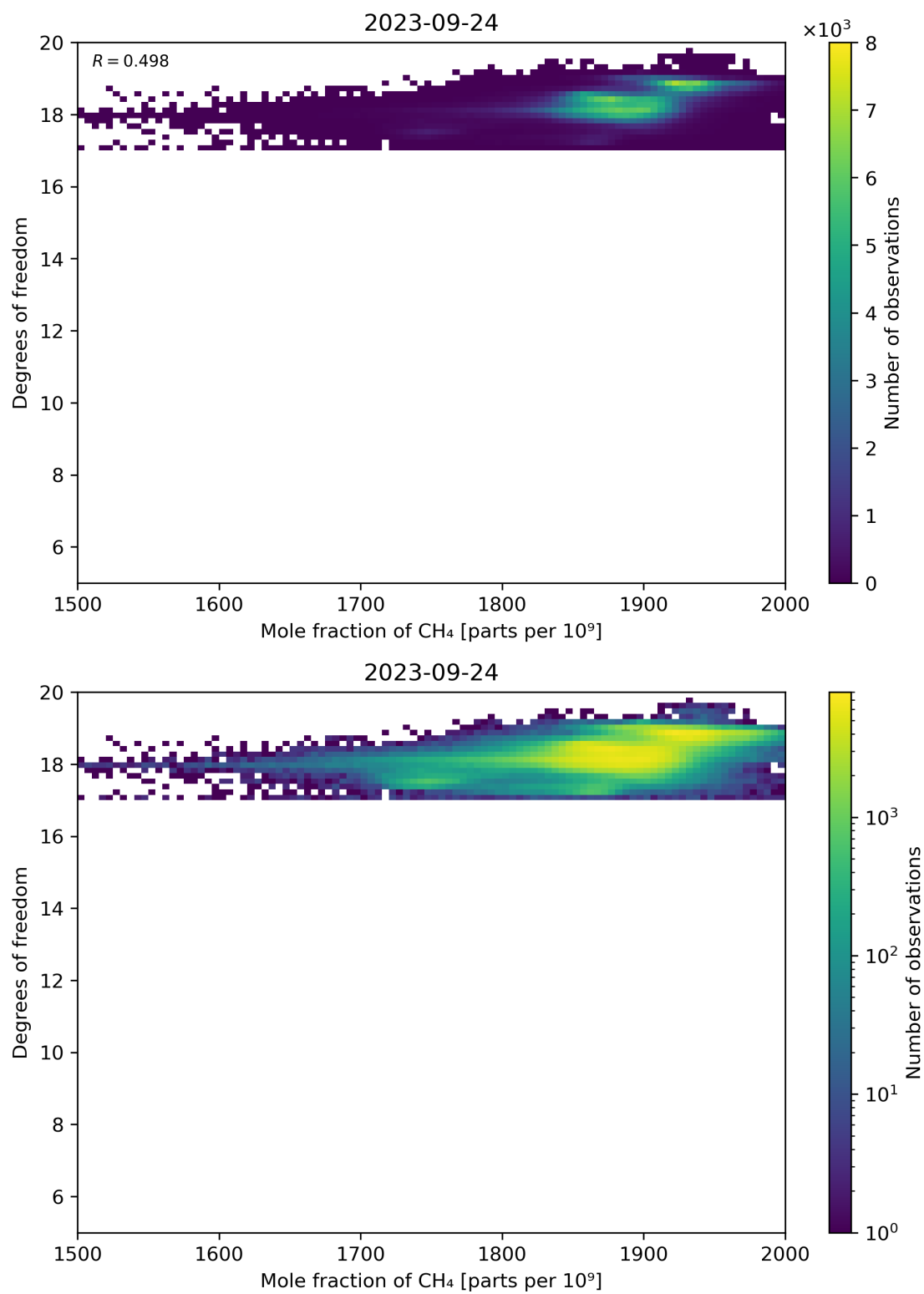
Figure 72: Scatter density plot of “Mole fraction of CH 4 ” against “Degrees of freedom” for 2023-09-23 to 2023-09-25.
