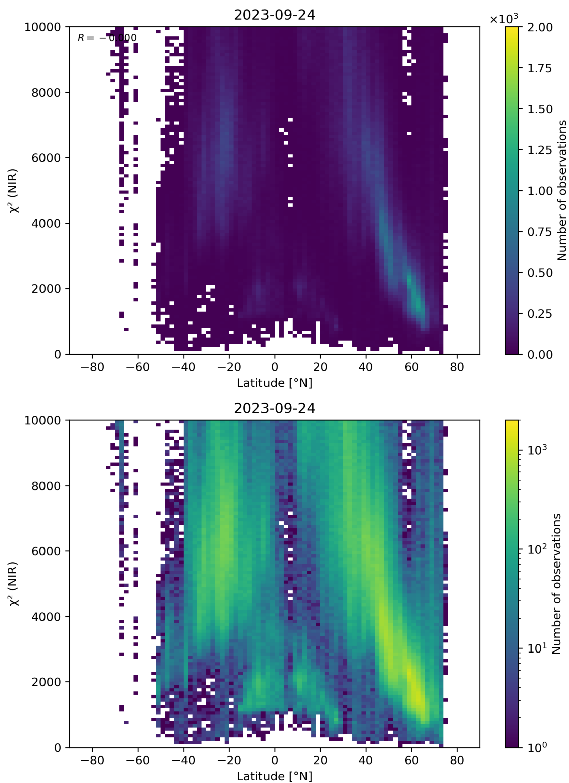
Figure 53: Scatter density plot of “Latitude” against “ \chi^2 (NIR)” for 2023-09-23 to 2023-09-25.
