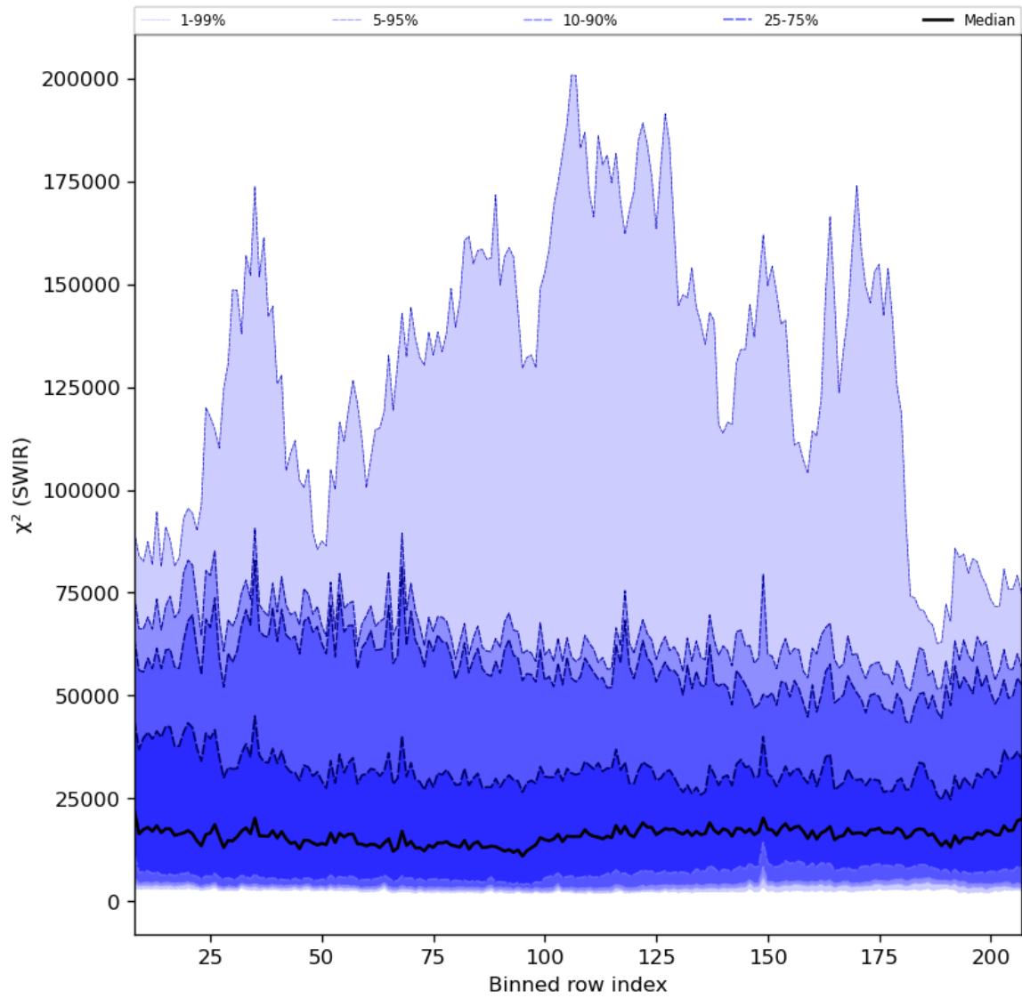
Figure 39: Along track statistics of " \chi^2 (SWIR)" for 2023-09-23 to 2023-09-25
