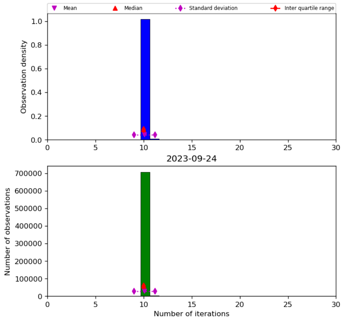
Figure 31: Histogram of “Number of iterations” for 2023-09-23 to 2023-09-25
