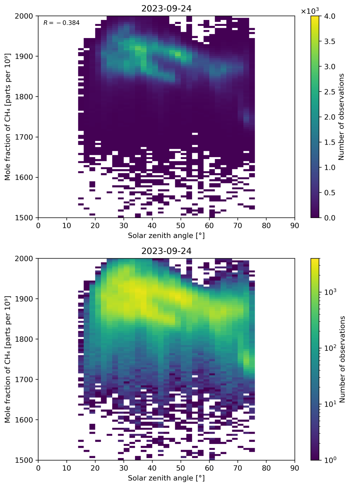
Figure 99: Scatter density plot of “Solar zenith angle” against “Mole fraction of CH 4 ” for 2023-09-23 to 2023-09-25.
