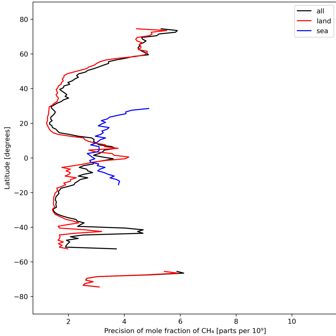
Figure 13: Zonal average of “Precision of mole fraction of CH 4 ” for 2023-09-23 to 2023-09-25.
