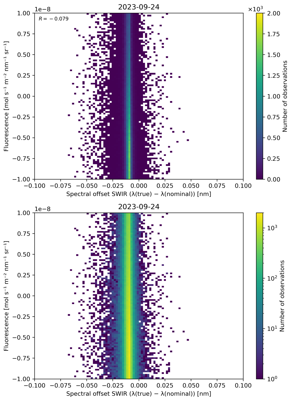
Figure 120: Scatter density plot of “Spectral offset SWIR ( \lambda(\text{true}) - \lambda(\text{nominal}) )” against “Fluorescence” for 2023-09-23 to 2023-09-25.
