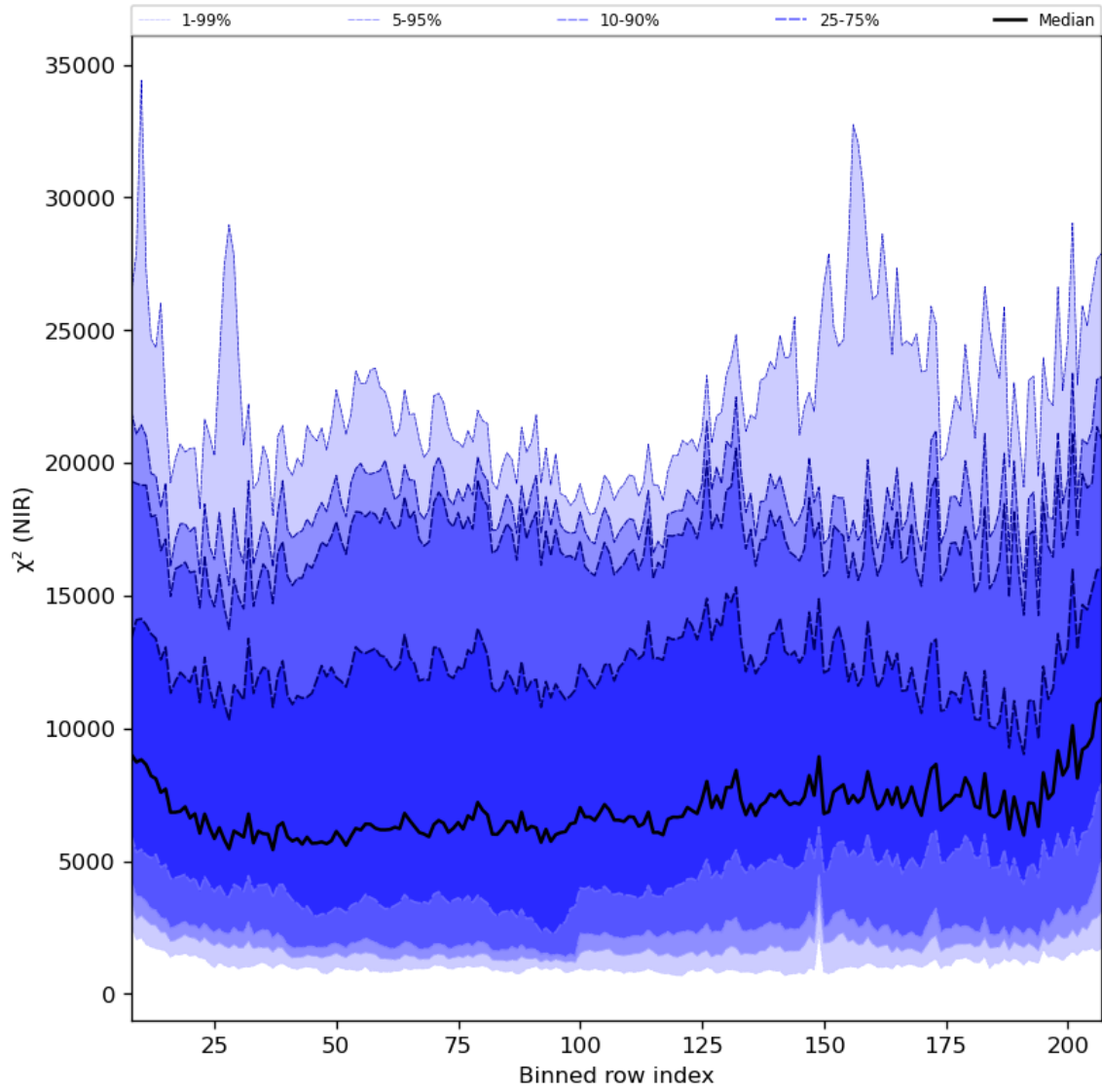
Figure 40: Along track statistics of “ \chi^2 (NIR)” for 2023-09-23 to 2023-09-25
