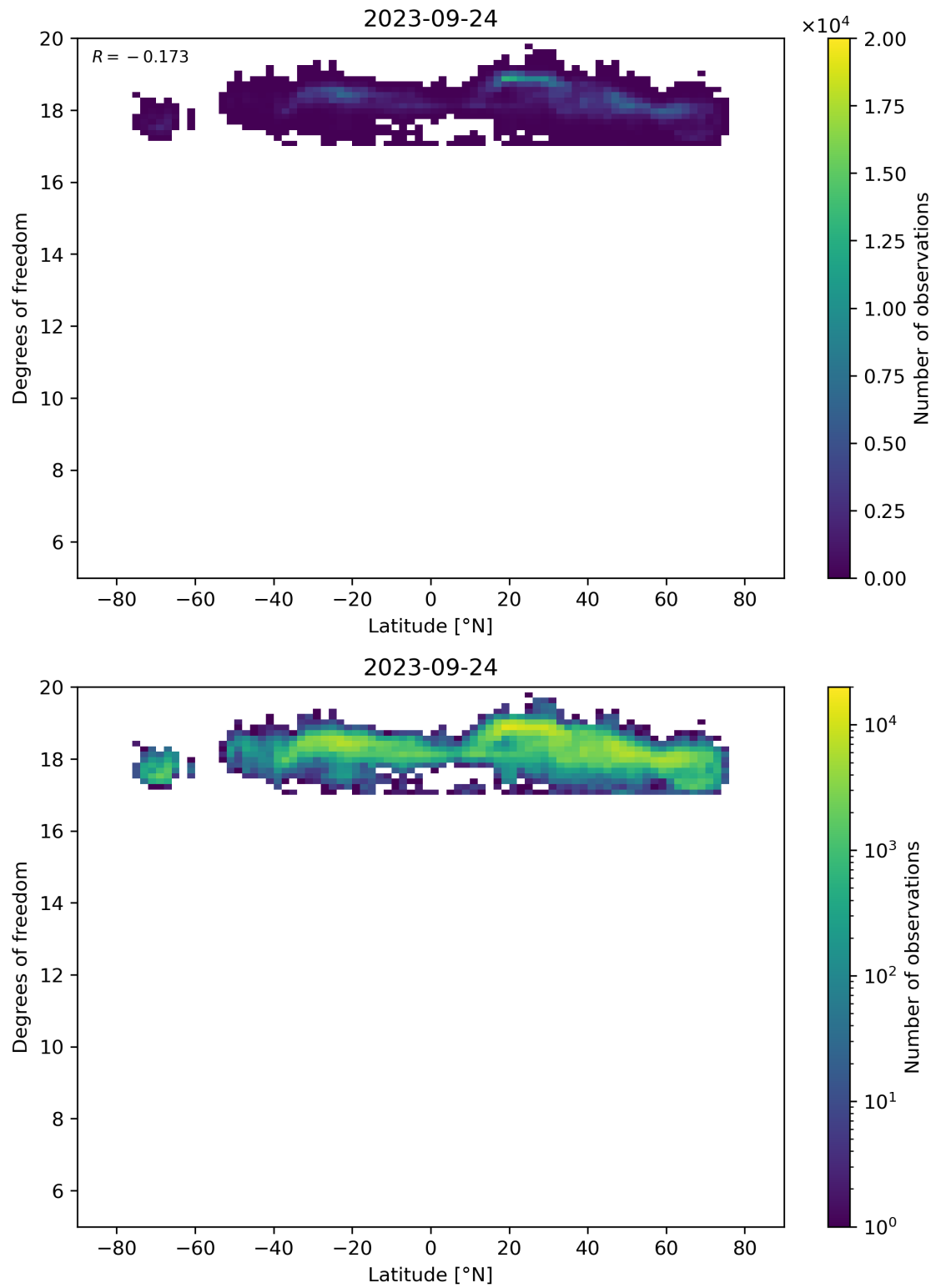
Figure 55: Scatter density plot of “Latitude” against “Degrees of freedom” for 2023-09-23 to 2023-09-25.
