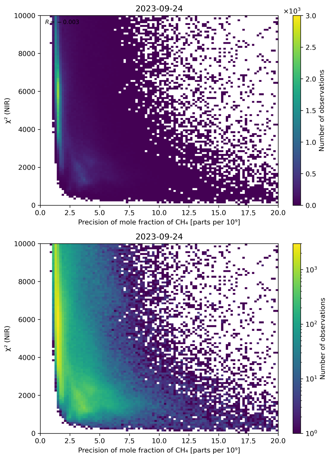
Figure 78: Scatter density plot of “Precision of mole fraction of CH 4 ” against “ \chi^2 (NIR)” for 2023-09-23 to 2023-09-25.
