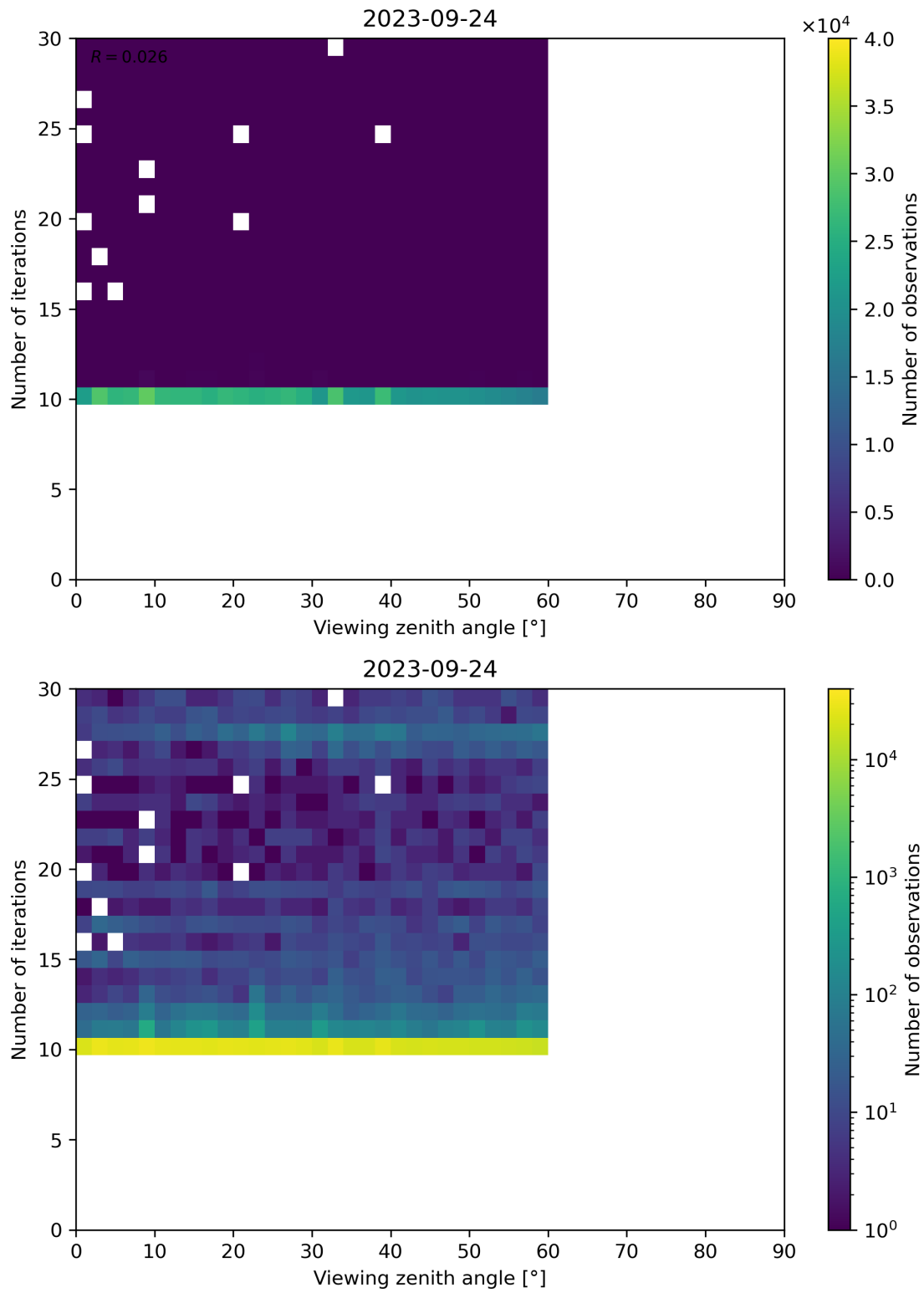
Figure 113: Scatter density plot of “Viewing zenith angle” against “Number of iterations” for 2023-09-23 to 2023-09-25.
