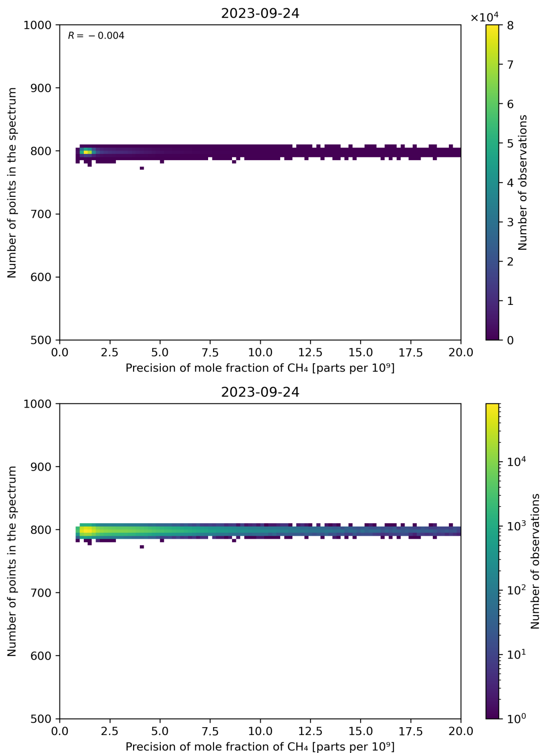
Figure 84: Scatter density plot of “Precision of mole fraction of CH 4 ” against “Number of points in the spectrum” for 2023-09-23 to 2023-09-25.
