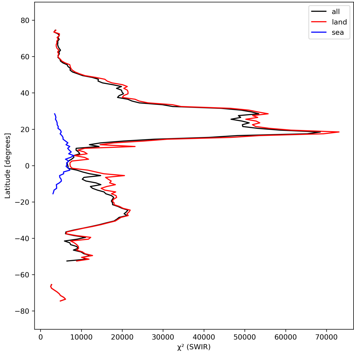
Figure 17: Zonal average of “ \chi^2 (SWIR)” for 2023-09-23 to 2023-09-25.
