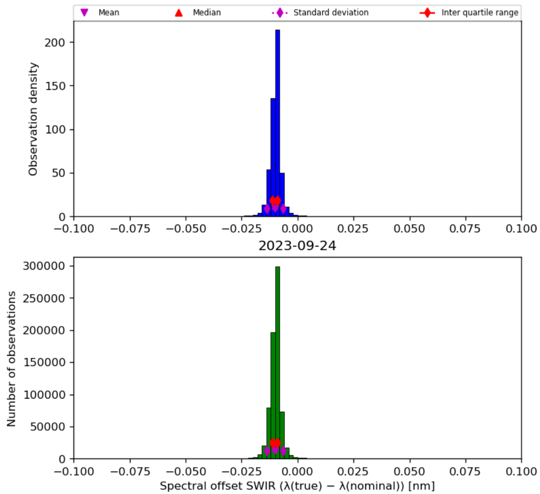
Figure 27: Histogram of “Spectral offset SWIR ( \lambda(\text{true}) - \lambda(\text{nominal}) )” for 2023-09-23 to 2023-09-25
