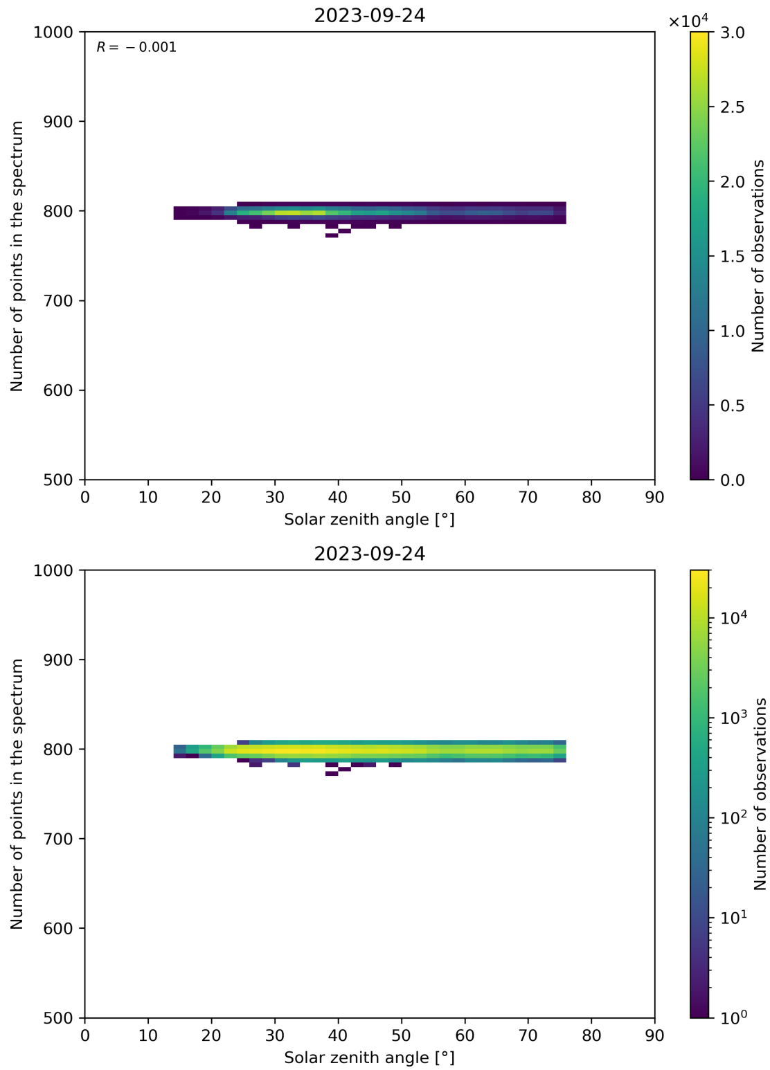
Figure 103: Scatter density plot of “Solar zenith angle” against “Number of points in the spectrum” for 2023-09-23 to 2023-09-25.
