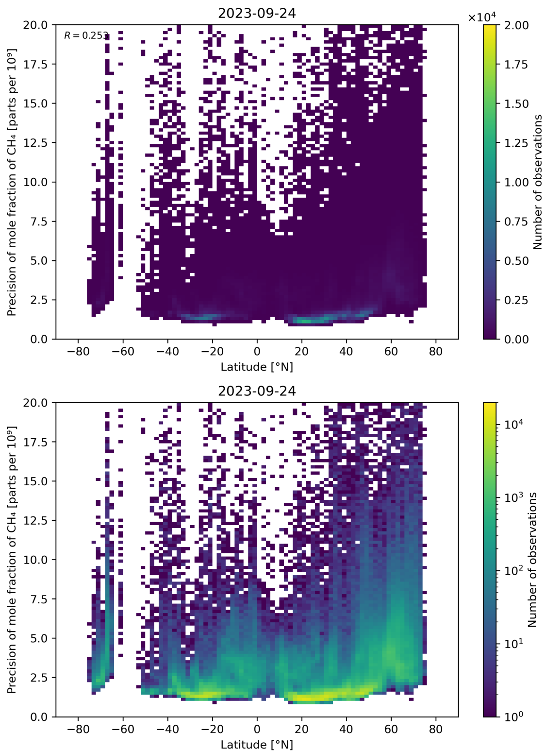
Figure 59: Scatter density plot of “Latitude” against “Precision of mole fraction of CH 4 ” for 2023-09-23 to 2023-09-25.
