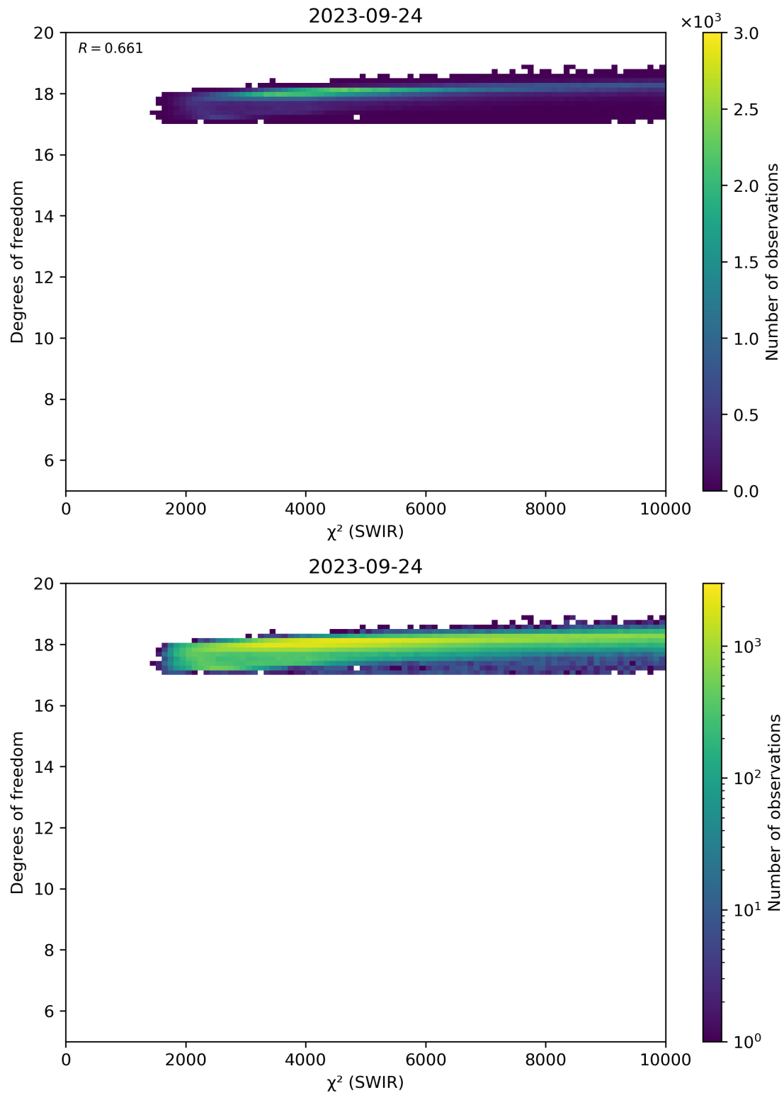
Figure 48: Scatter density plot of “ \chi^2 (SWIR)” against “Degrees of freedom” for 2023-09-23 to 2023-09-25.
