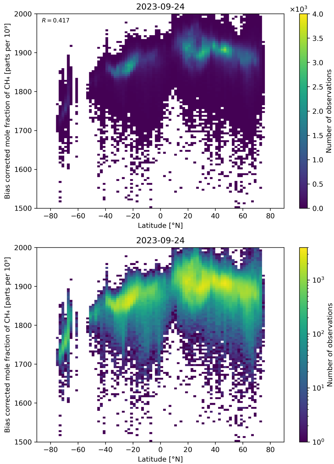
Figure 58: Scatter density plot of “Latitude” against “Bias corrected mole fraction of CH 4 ” for 2023-09-23 to 2023-09-25.
