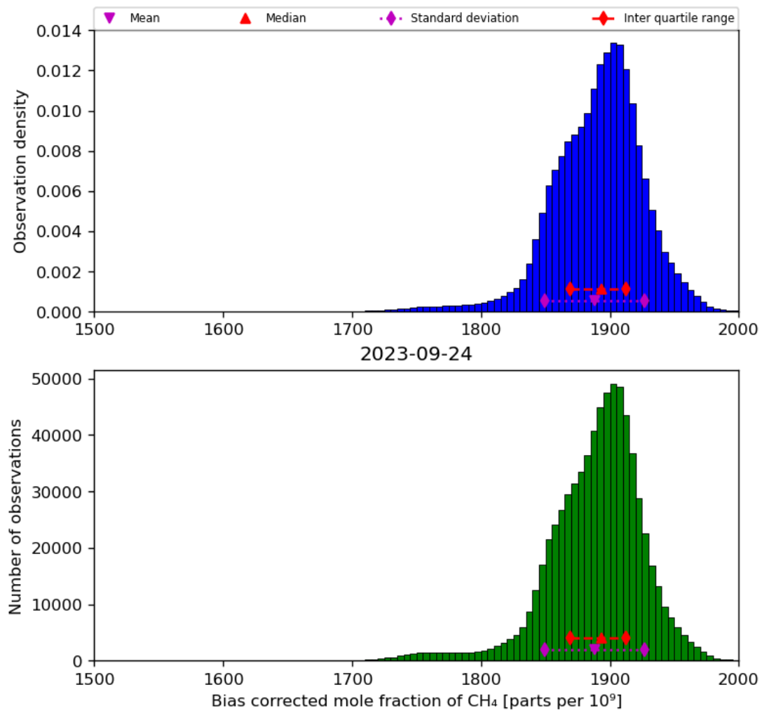
Figure 25: Histogram of “Bias corrected mole fraction of CH 4 ” for 2023-09-23 to 2023-09-25
