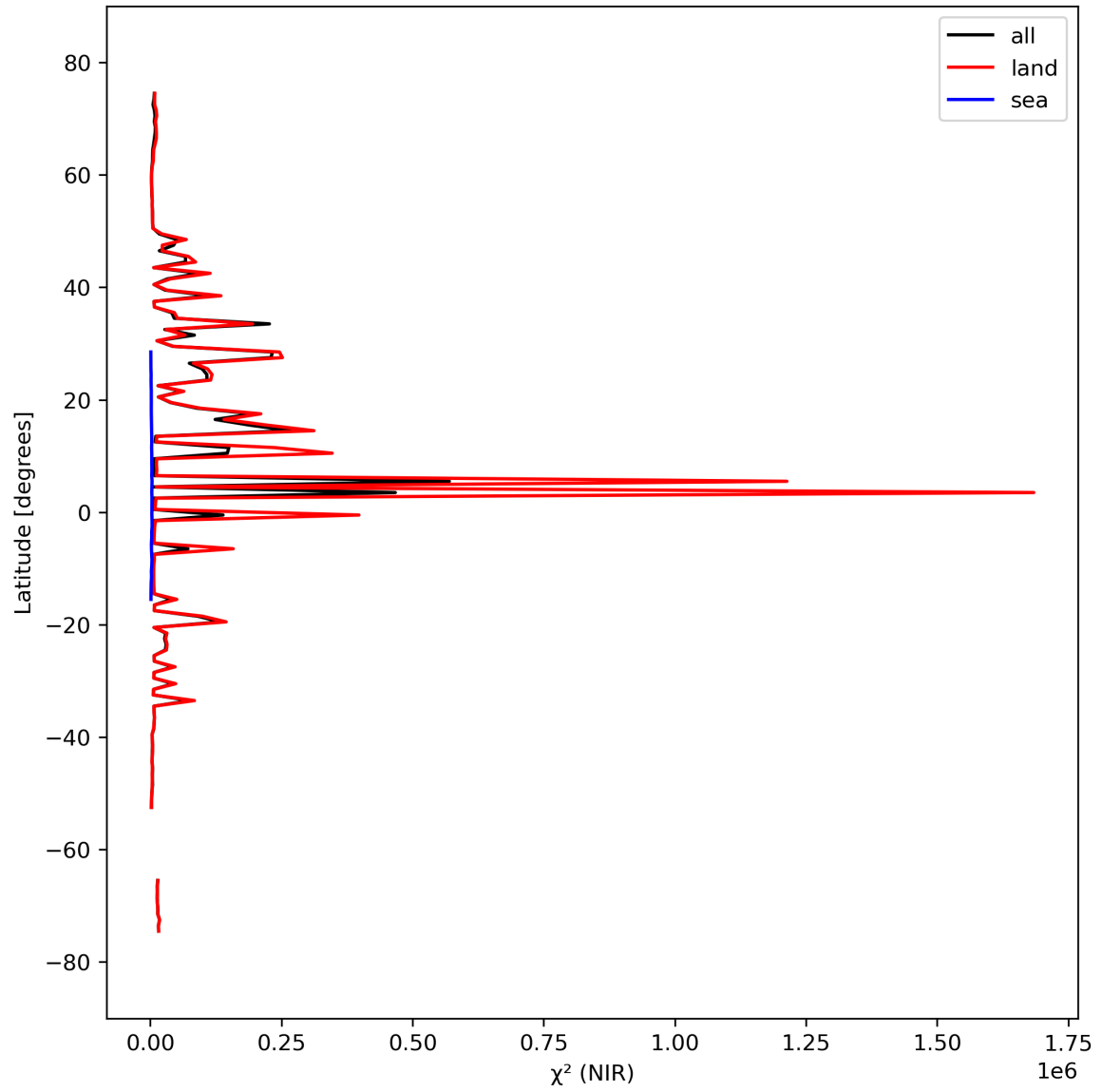
Figure 18: Zonal average of “ \chi^2 (NIR)” for 2023-09-23 to 2023-09-25.
