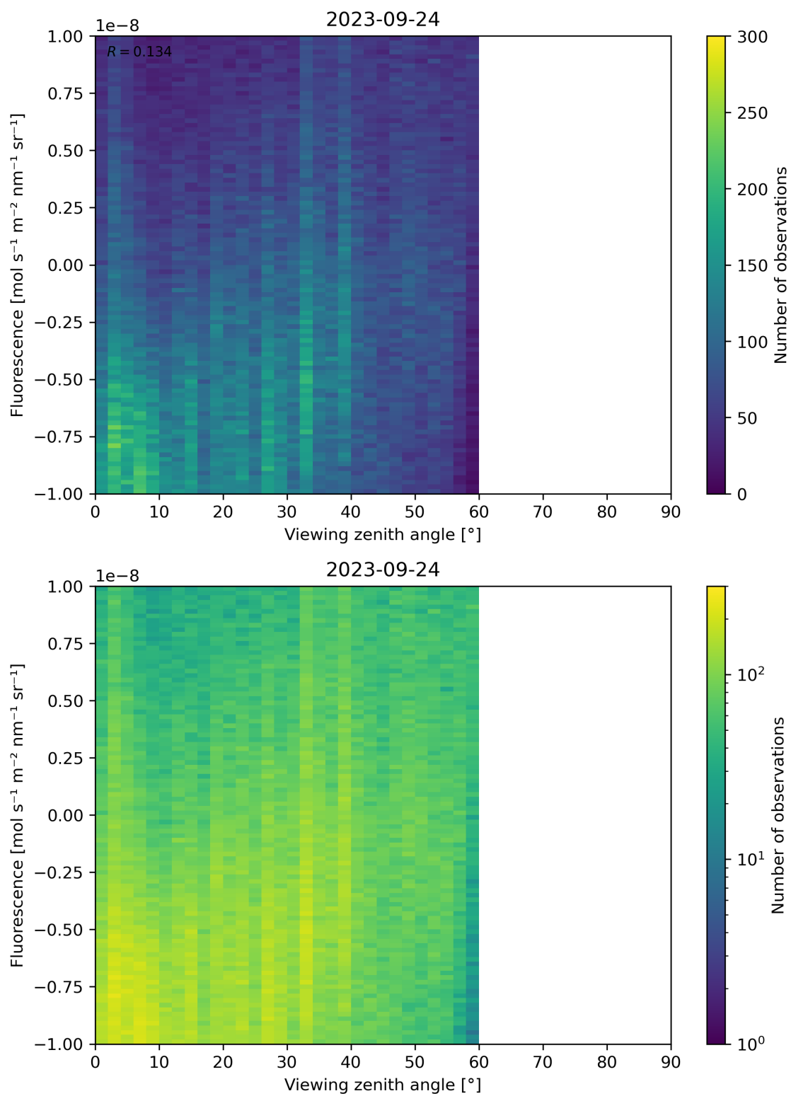
Figure 108: Scatter density plot of “Viewing zenith angle” against “Fluorescence” for 2023-09-23 to 2023-09-25.
