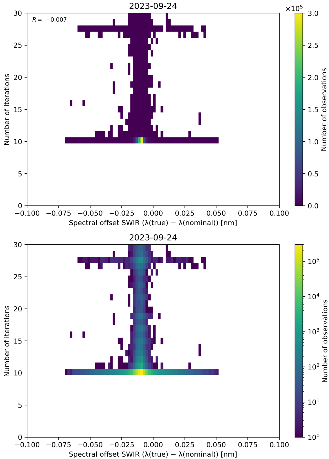
Figure 121: Scatter density plot of “Spectral offset SWIR ( \lambda(\text{true}) - \lambda(\text{nominal}) )” against “Number of iterations” for 2023-09-23 to 2023-09-25.
