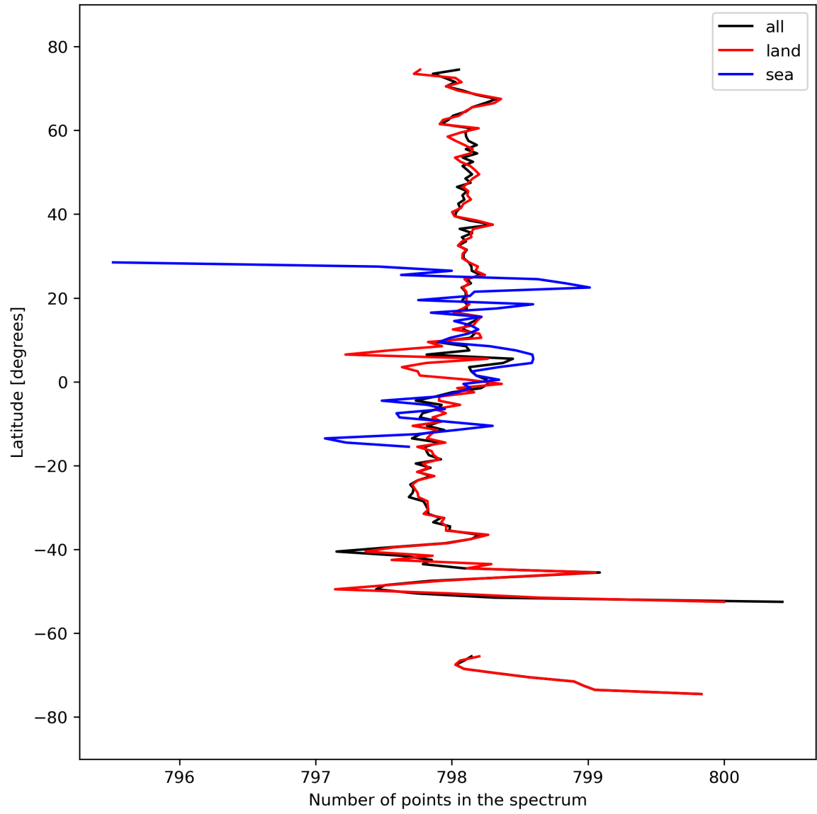
Figure 15: Zonal average of “Number of points in the spectrum” for 2023-09-23 to 2023-09-25.
