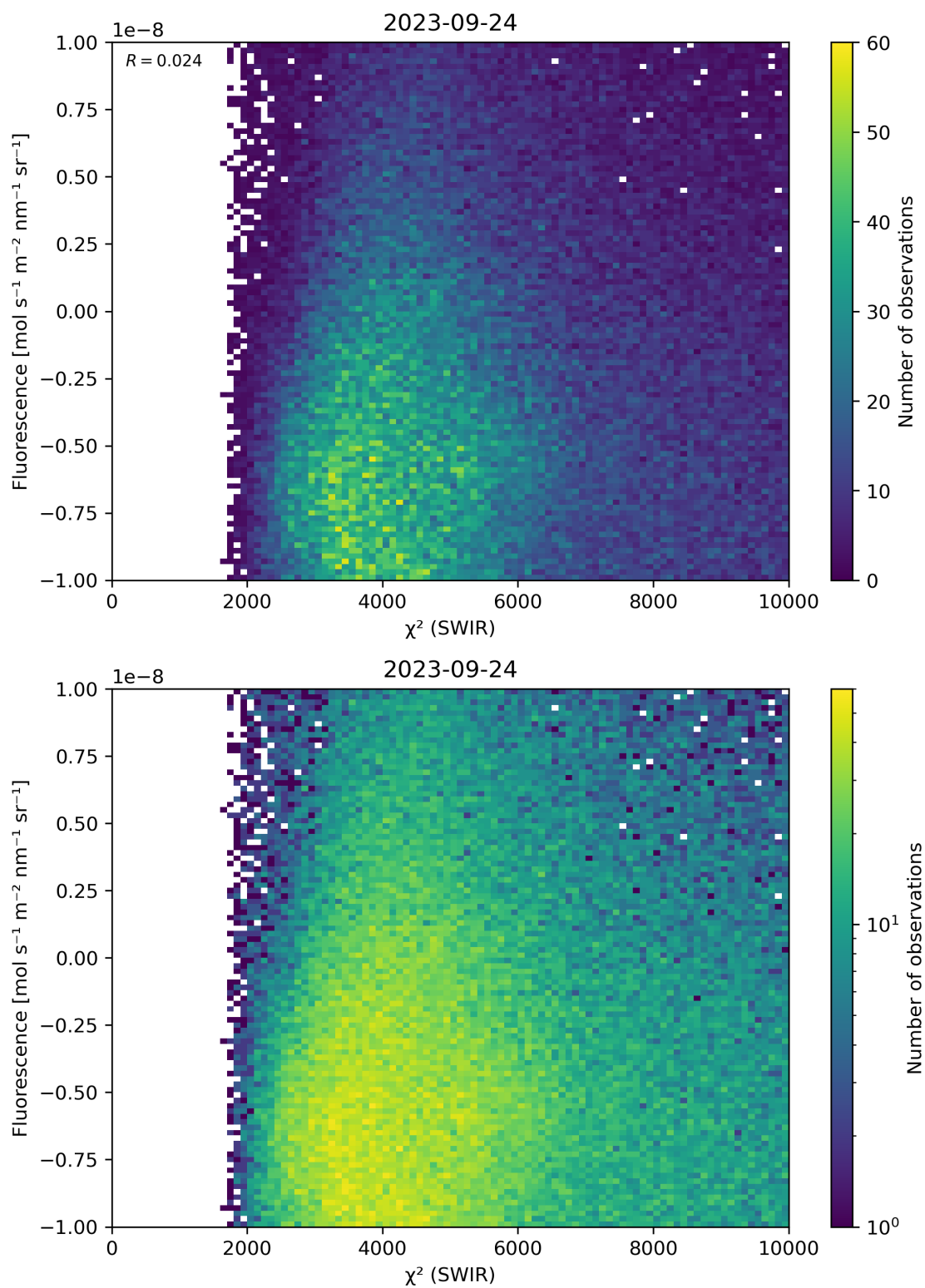
Figure 49: Scatter density plot of “ \chi^2 (SWIR)” against “Fluorescence” for 2023-09-23 to 2023-09-25.
