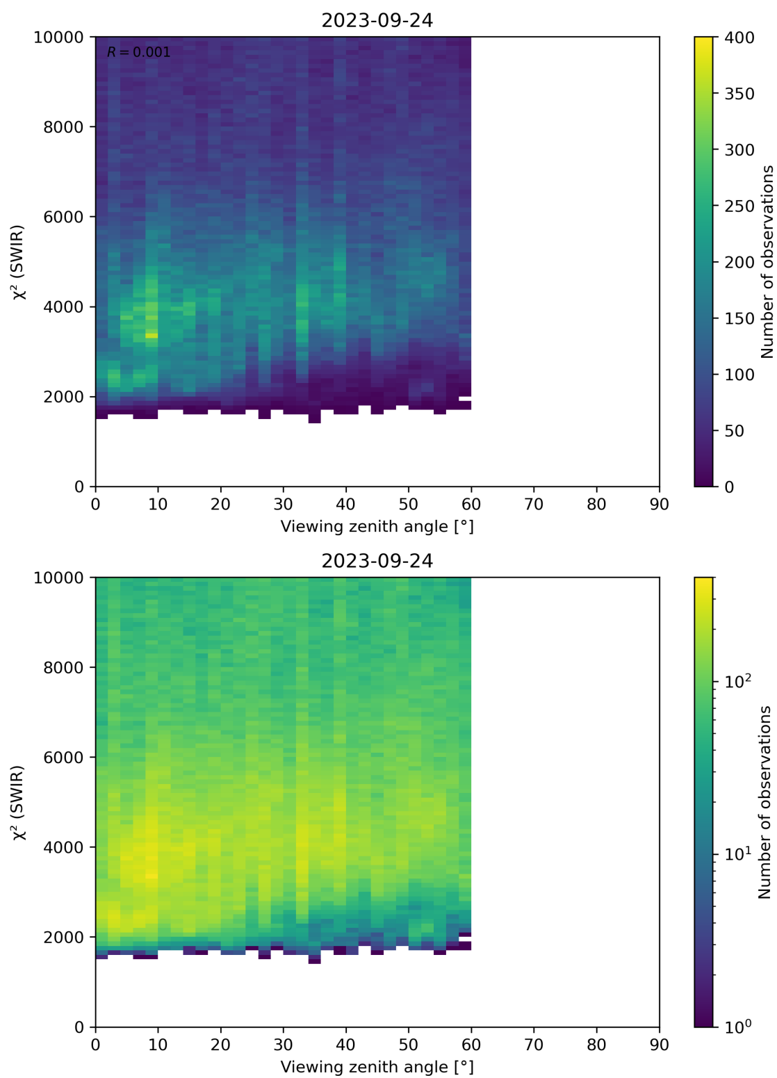
Figure 106: Scatter density plot of “Viewing zenith angle” against “ \chi^2 (SWIR)” for 2023-09-23 to 2023-09-25.
