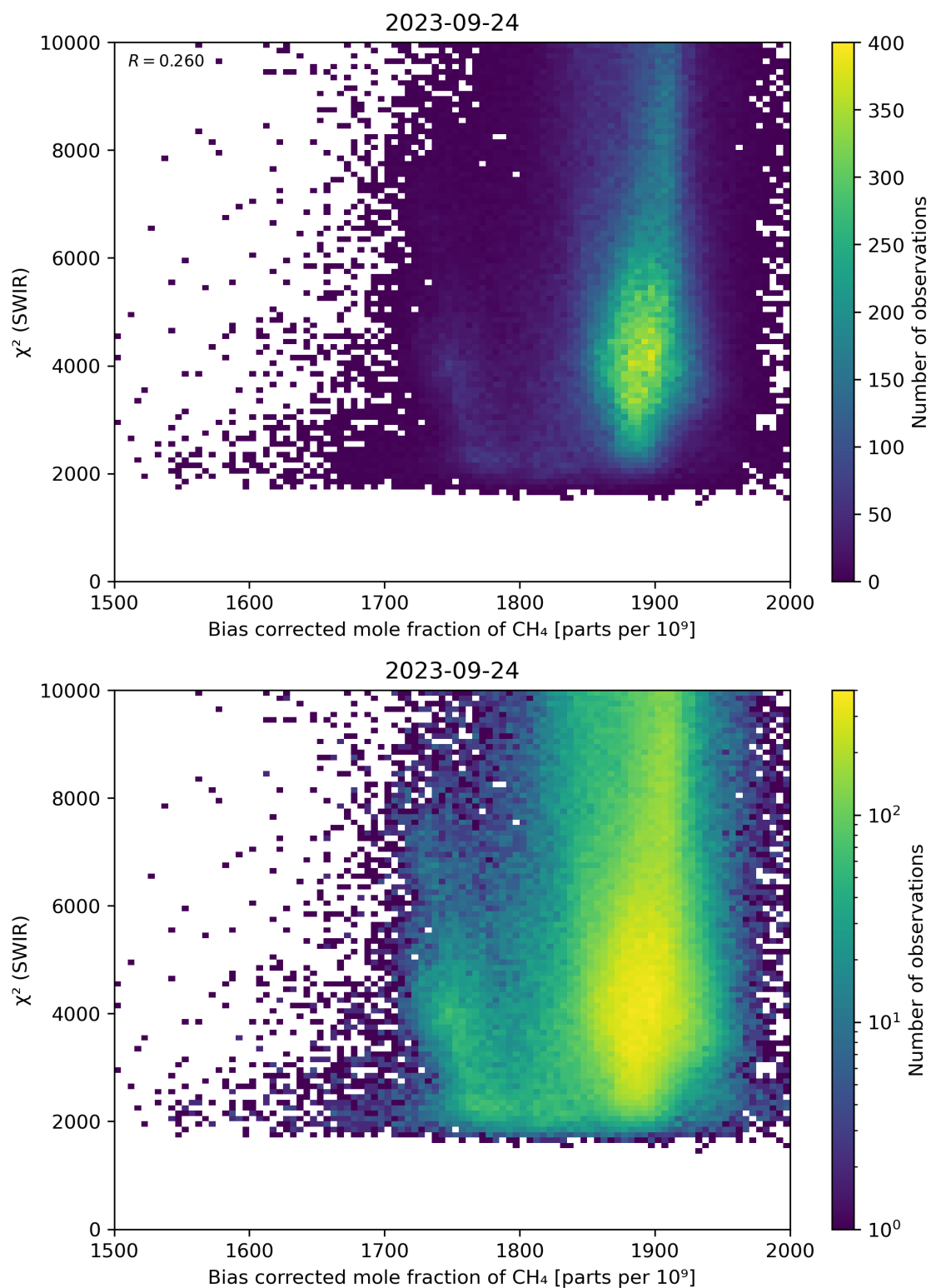
Figure 64: Scatter density plot of “Bias corrected mole fraction of CH 4 ” against “ \chi^2 (SWIR)” for 2023-09-23 to 2023-09-25.
