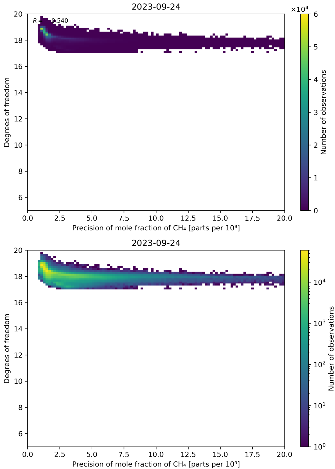
Figure 80: Scatter density plot of “Precision of mole fraction of CH 4 ” against “Degrees of freedom” for 2023-09-23 to 2023-09-25.
