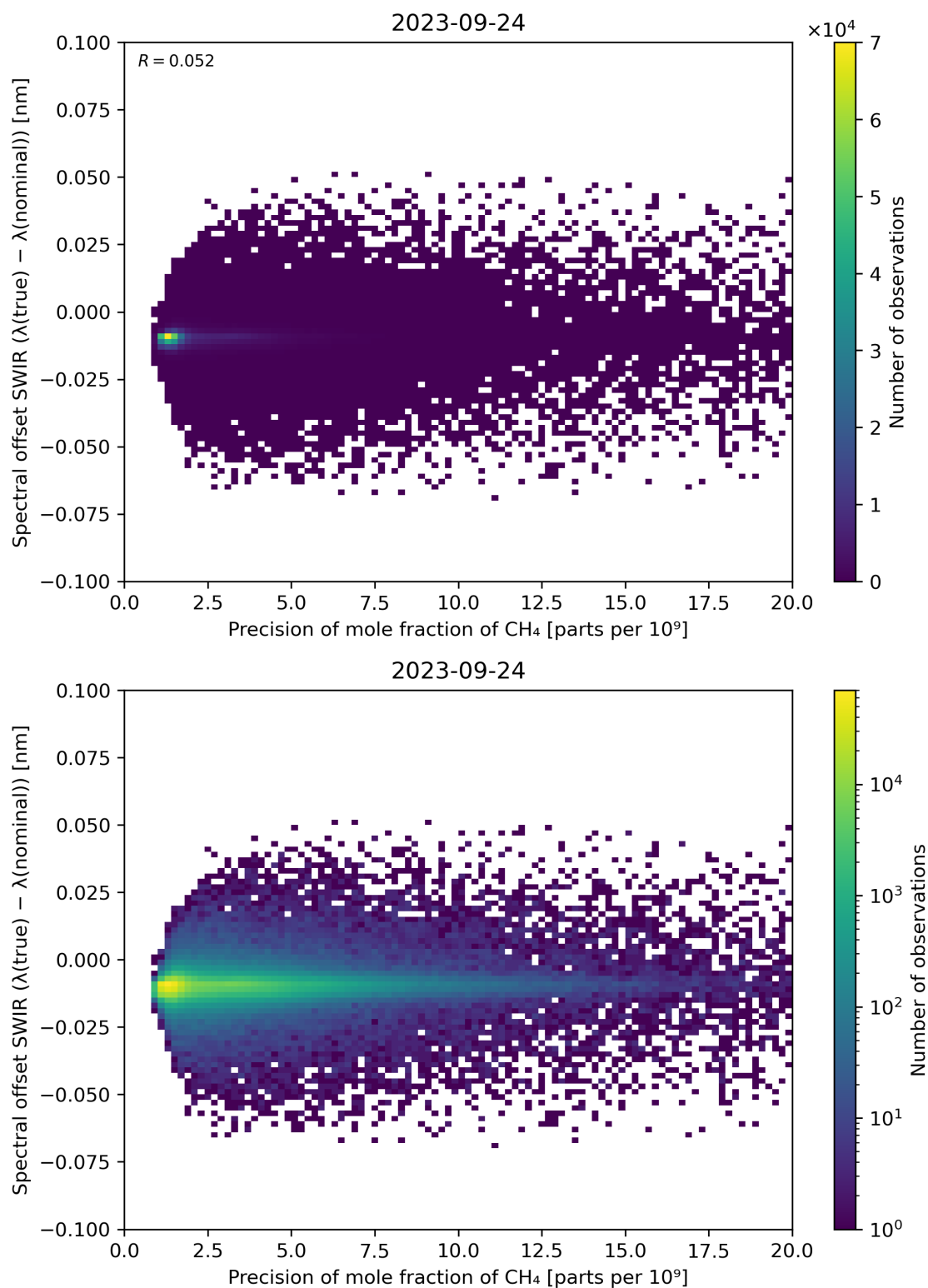
Figure 85: Scatter density plot of “Precision of mole fraction of CH 4 ” against “Spectral offset SWIR ( \lambda(\text{true}) - \lambda(\text{nominal}) )” for 2023-09-23 to 2023-09-25.
