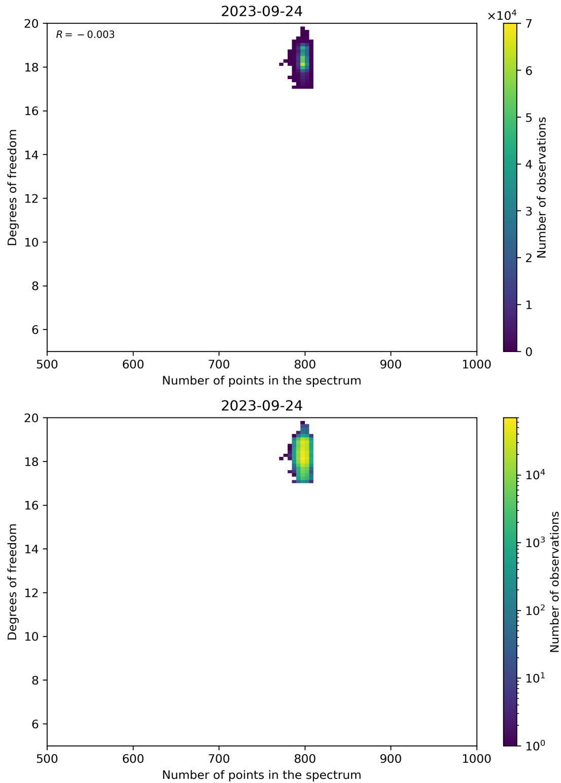
Figure 90: Scatter density plot of “Number of points in the spectrum” against “Degrees of freedom” for 2023-09-23 to 2023-09-25.
