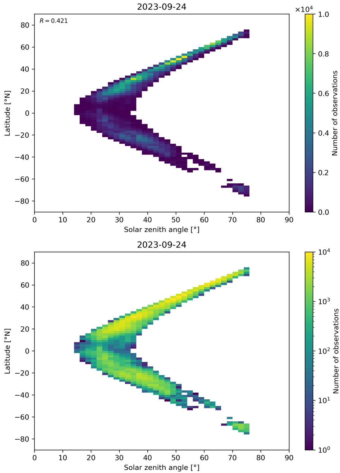
Figure 98: Scatter density plot of “Solar zenith angle” against “Latitude” for 2023-09-23 to 2023-09-25.
