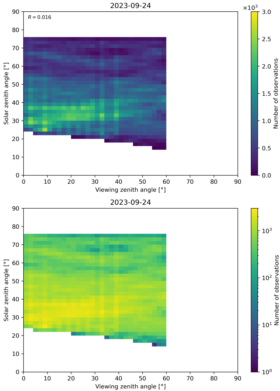
Figure 115: Scatter density plot of “Viewing zenith angle” against “Solar zenith angle” for 2023-09-23 to 2023-09-25.
