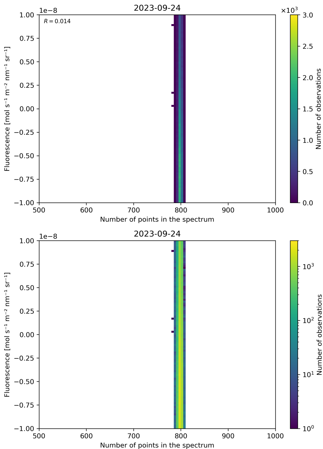
Figure 91: Scatter density plot of “Number of points in the spectrum” against “Fluorescence” for 2023-09-23 to 2023-09-25.
