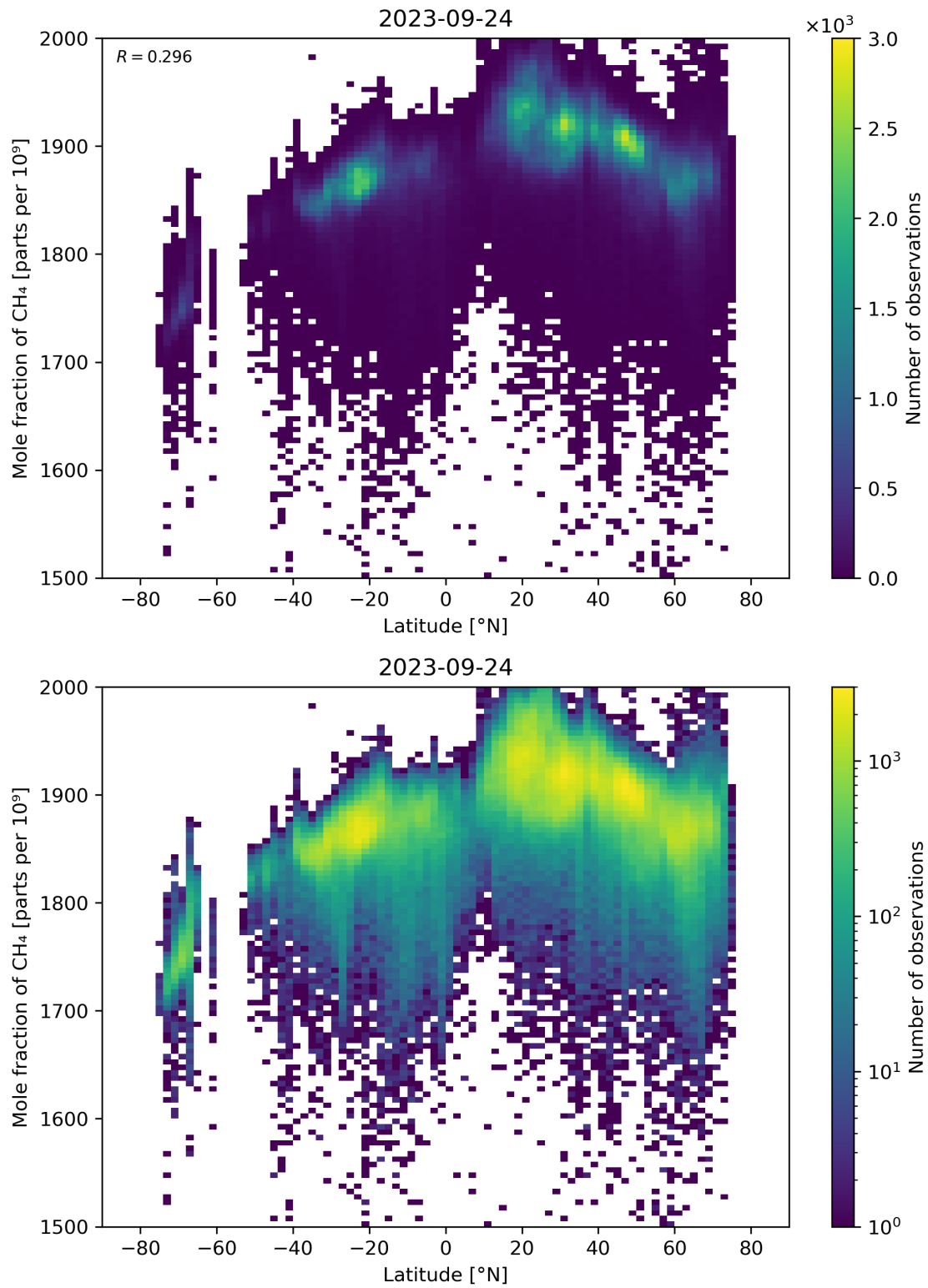
Figure 57: Scatter density plot of “Latitude” against “Mole fraction of \text{CH}_4 ” for 2023-09-23 to 2023-09-25.
