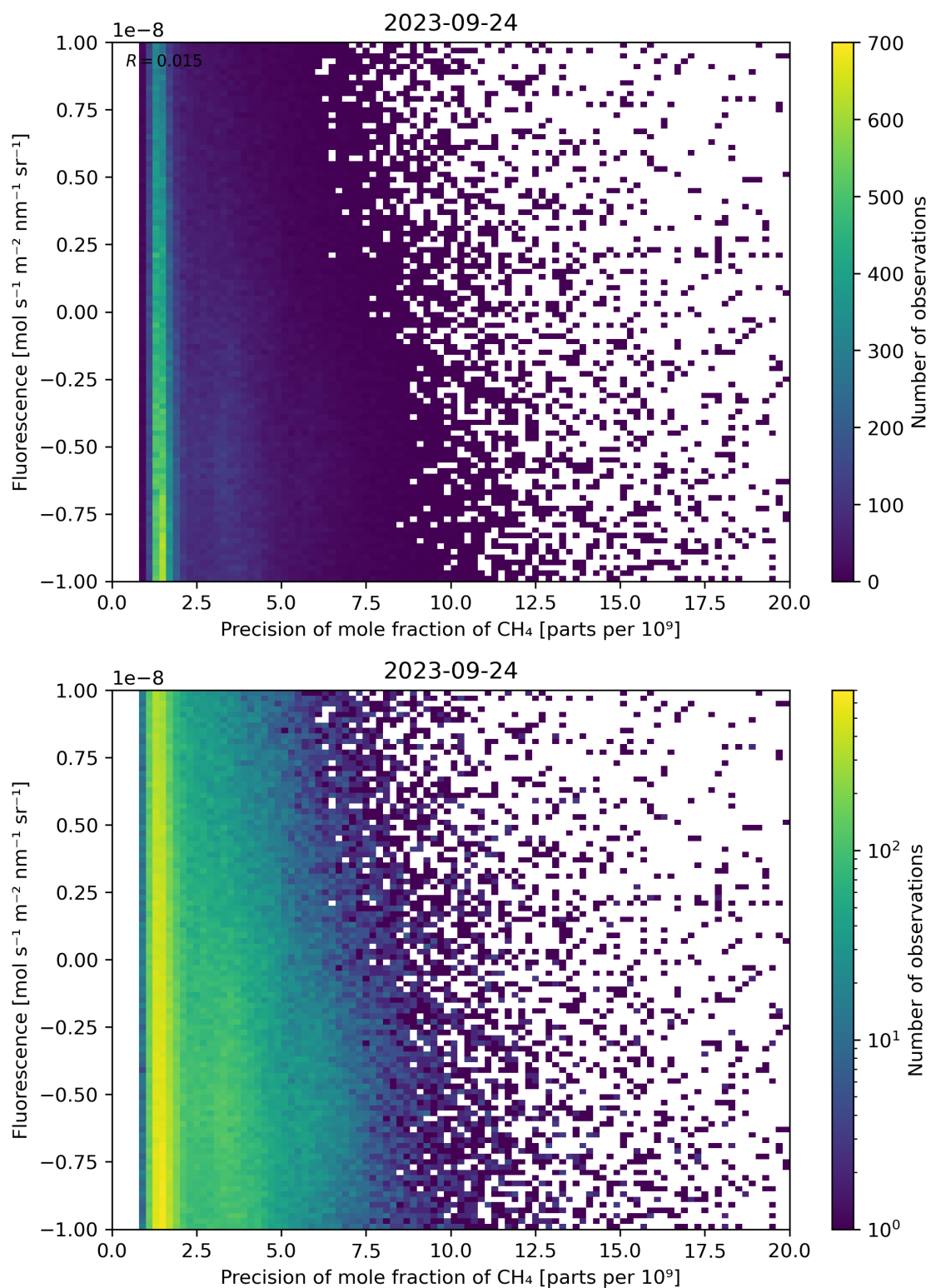
Figure 81: Scatter density plot of “Precision of mole fraction of \text{CH}_4 ” against “Fluorescence” for 2023-09-23 to 2023-09-25.
