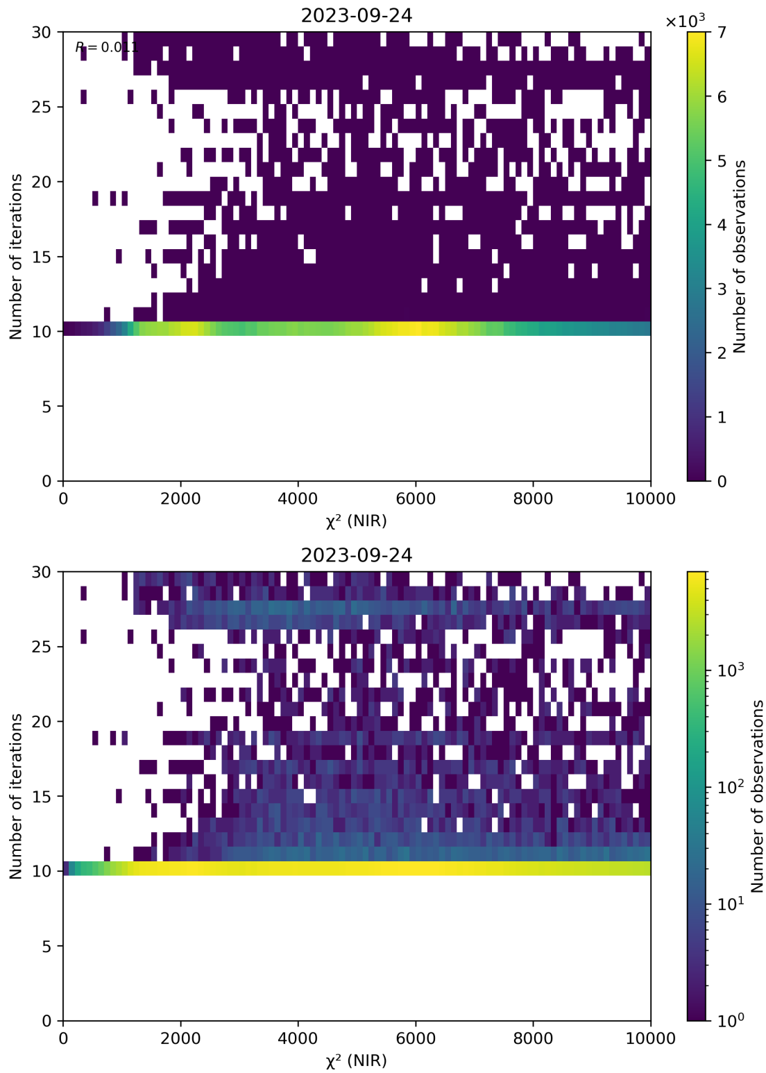
Figure 46: Scatter density plot of “ \chi^2 (NIR)” against “Number of iterations” for 2023-09-23 to 2023-09-25.
