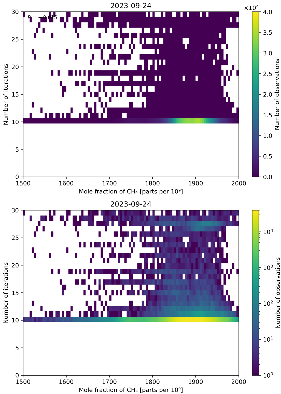
Figure 76: Scatter density plot of “Mole fraction of CH 4 ” against “Number of iterations” for 2023-09-23 to 2023-09-25.
