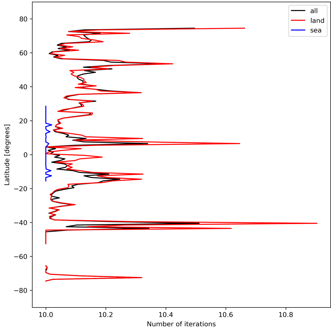
Figure 20: Zonal average of “Number of iterations” for 2023-09-23 to 2023-09-25.
