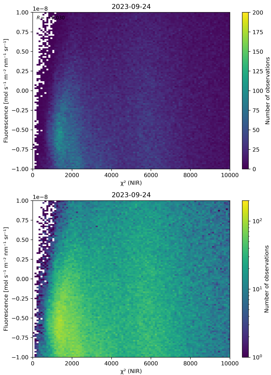
Figure 45: Scatter density plot of “ \chi^2 (NIR)” against “Fluorescence” for 2023-09-23 to 2023-09-25.
