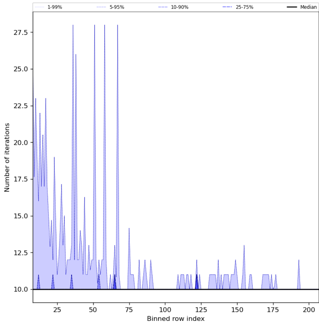
Figure 42: Along track statistics of “Number of iterations” for 2023-09-23 to 2023-09-25
