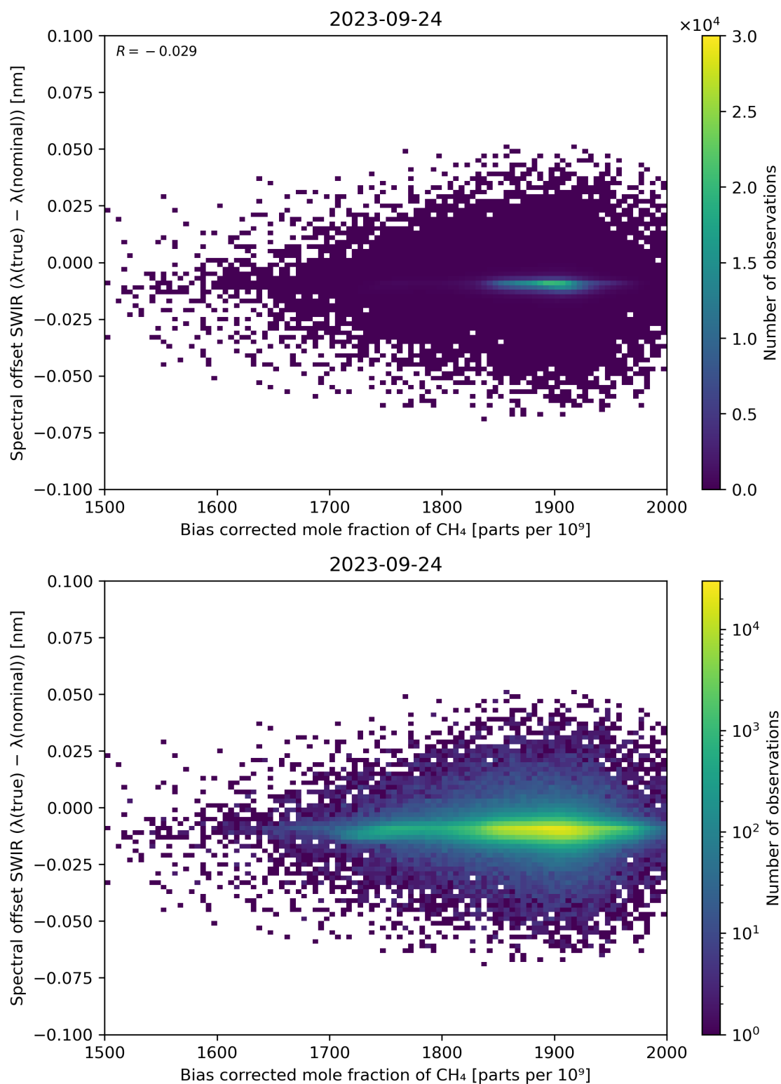
Figure 69: Scatter density plot of “Bias corrected mole fraction of \text{CH}_4 ” against “Spectral offset SWIR ( \lambda(\text{true}) - \lambda(\text{nominal}) )” for 2023-09-23 to 2023-09-25.
