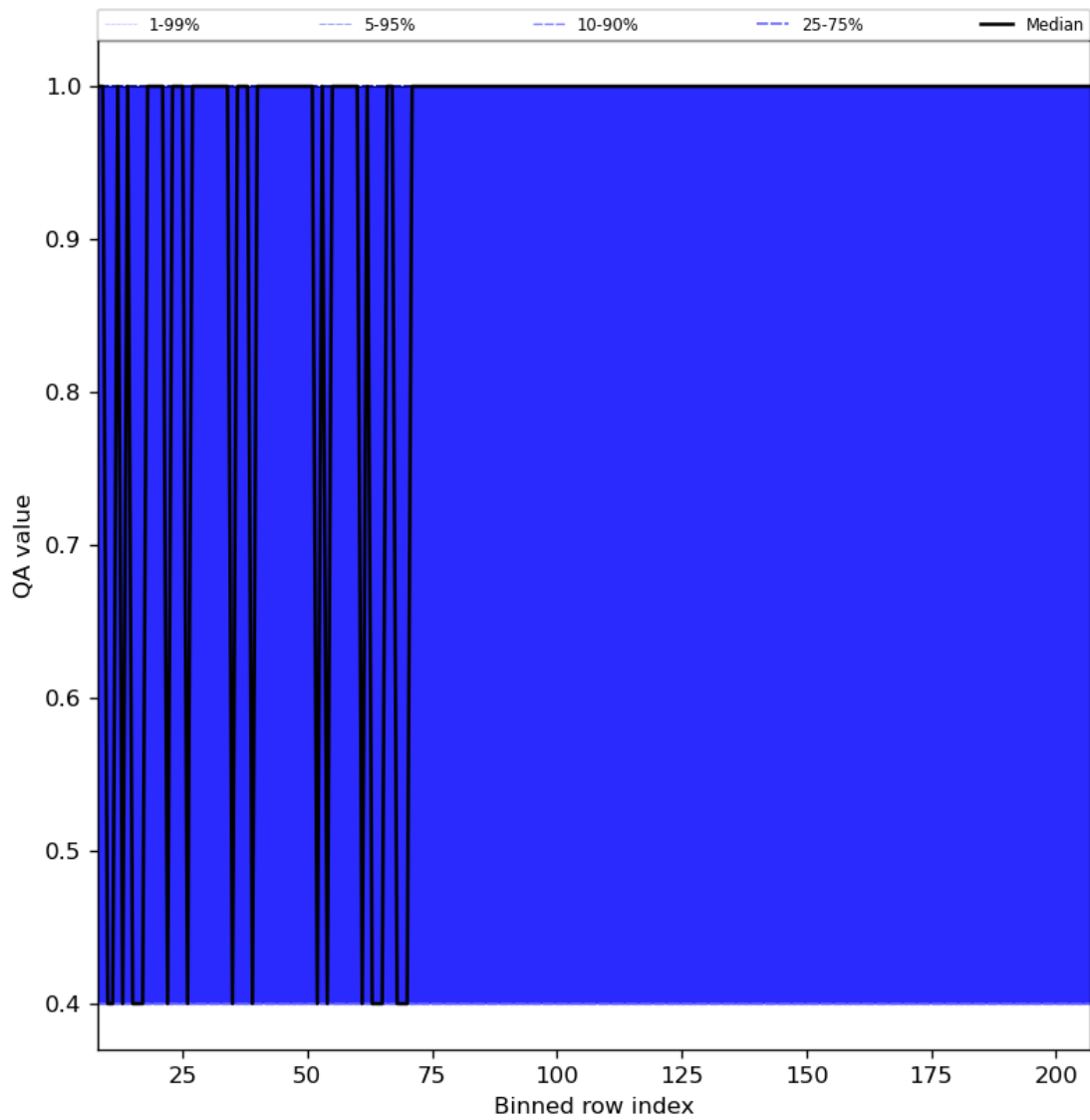
Figure 33: Along track statistics of “QA value” for 2023-09-23 to 2023-09-25
