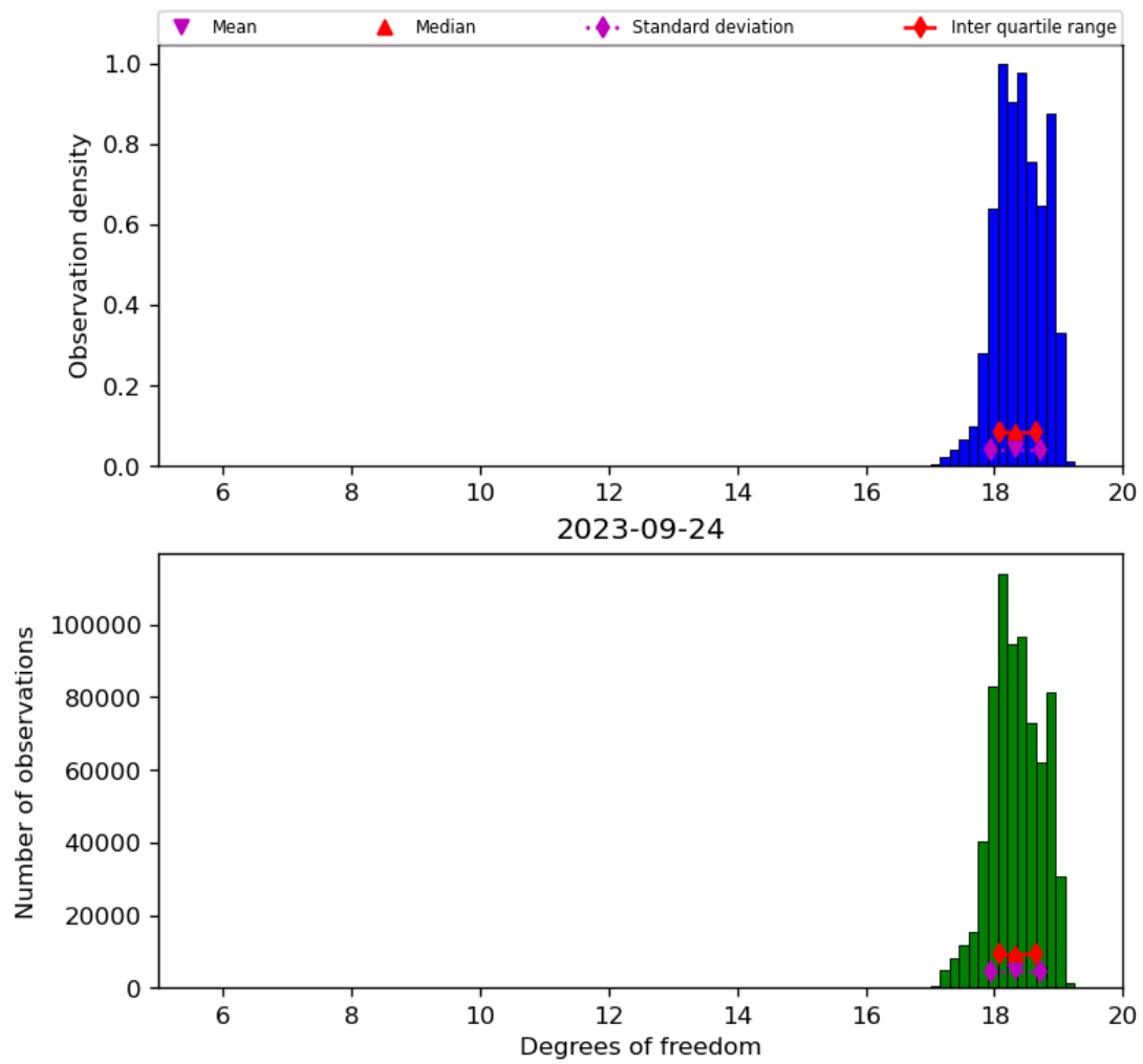
Figure 30: Histogram of “Degrees of freedom” for 2023-09-23 to 2023-09-25
