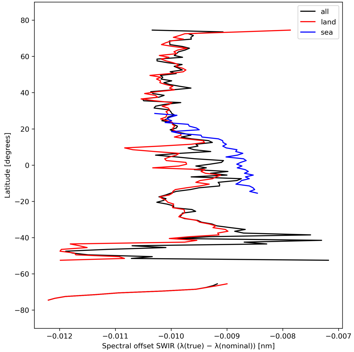
Figure 16: Zonal average of “Spectral offset SWIR ( \lambda(\text{true}) - \lambda(\text{nominal}) )” for 2023-09-23 to 2023-09-25.
