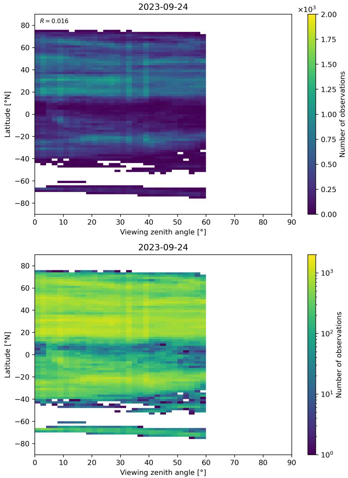
Figure 109: Scatter density plot of “Viewing zenith angle” against “Latitude” for 2023-09-23 to 2023-09-25.
