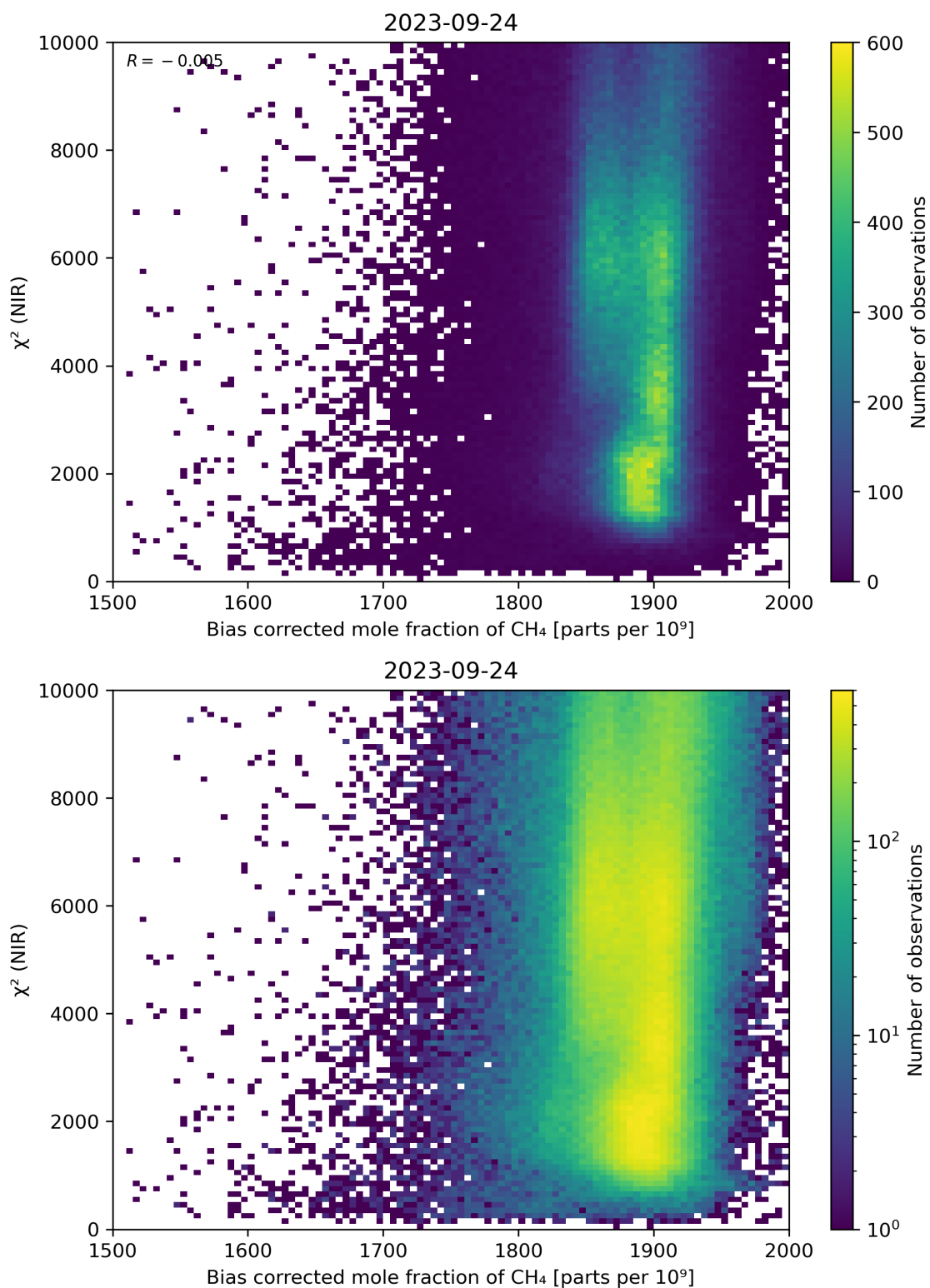
Figure 63: Scatter density plot of “Bias corrected mole fraction of CH 4 ” against “ \chi^2 (NIR)” for 2023-09-23 to 2023-09-25.
