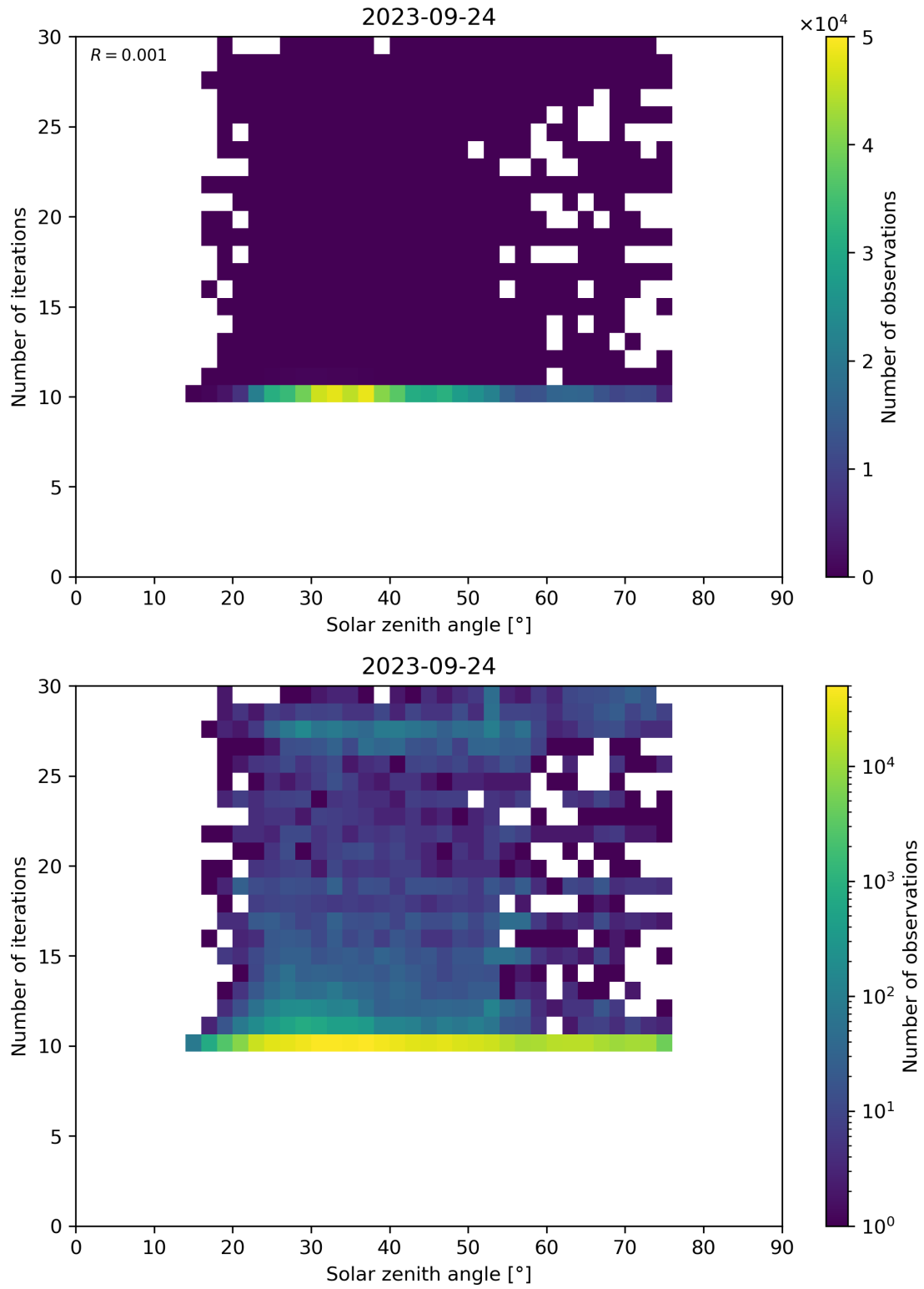
Figure 102: Scatter density plot of “Solar zenith angle” against “Number of iterations” for 2023-09-23 to 2023-09-25.
