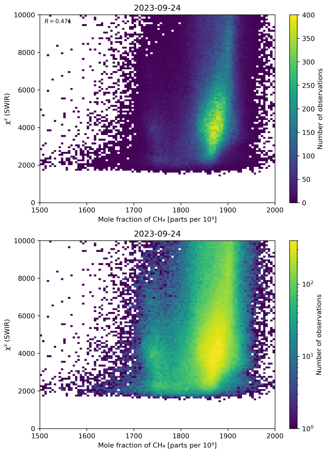
Figure 71: Scatter density plot of “Mole fraction of \text{CH}_4 ” against “ \chi^2 (SWIR)” for 2023-09-23 to 2023-09-25.
