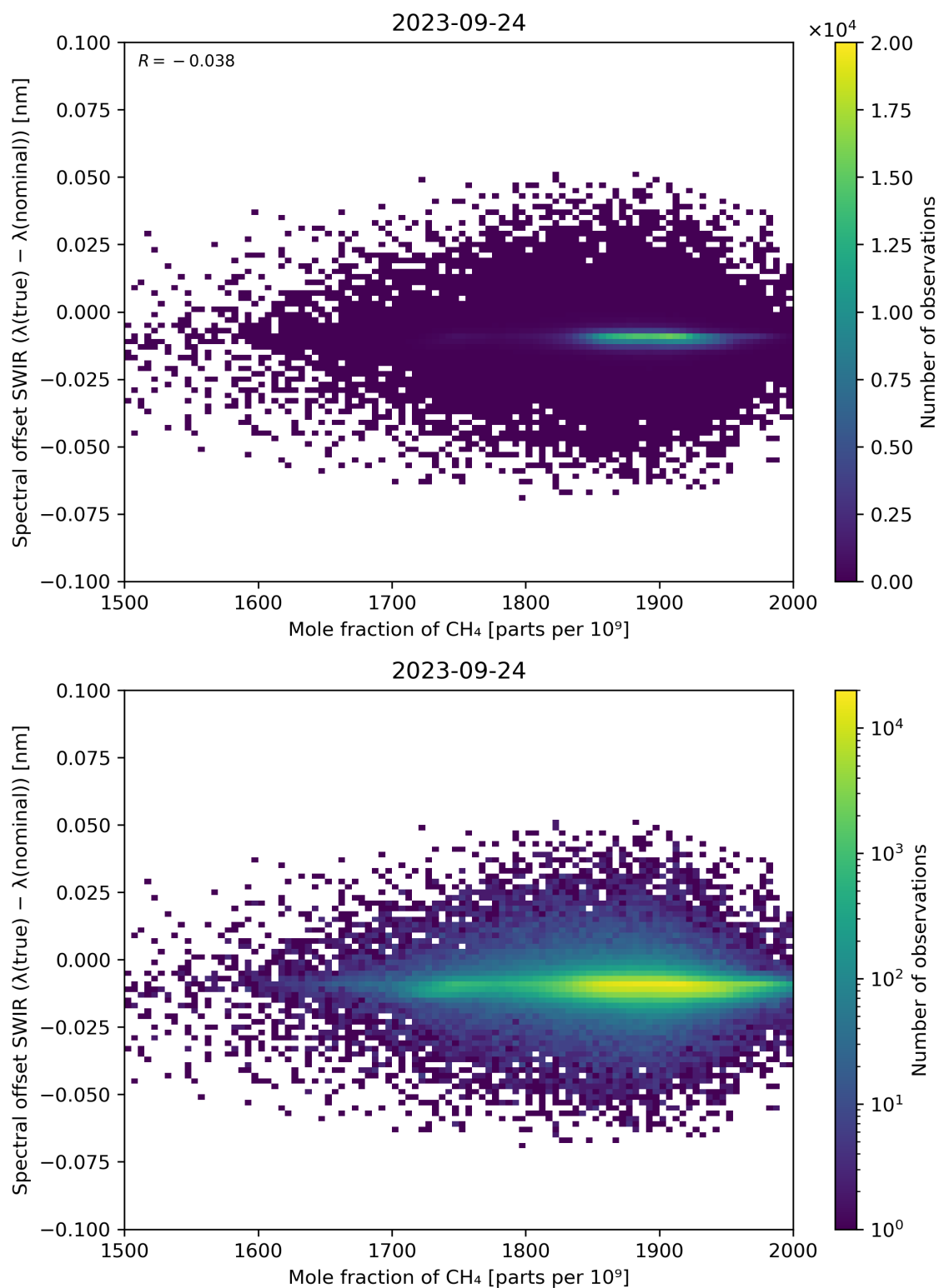
Figure 86: Scatter density plot of “Mole fraction of CH 4 ” against “Spectral offset SWIR ( \lambda(\text{true}) - \lambda(\text{nominal}) )” for 2023-09-23 to 2023-09-25.
