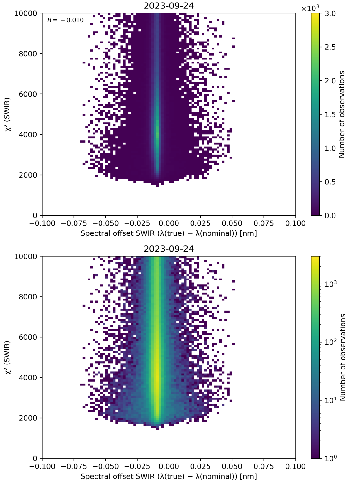
Figure 118: Scatter density plot of “Spectral offset SWIR ( \lambda(\text{true}) - \lambda(\text{nominal}) )” against “ \chi^2 (SWIR)” for 2023-09-23 to 2023-09-25.
