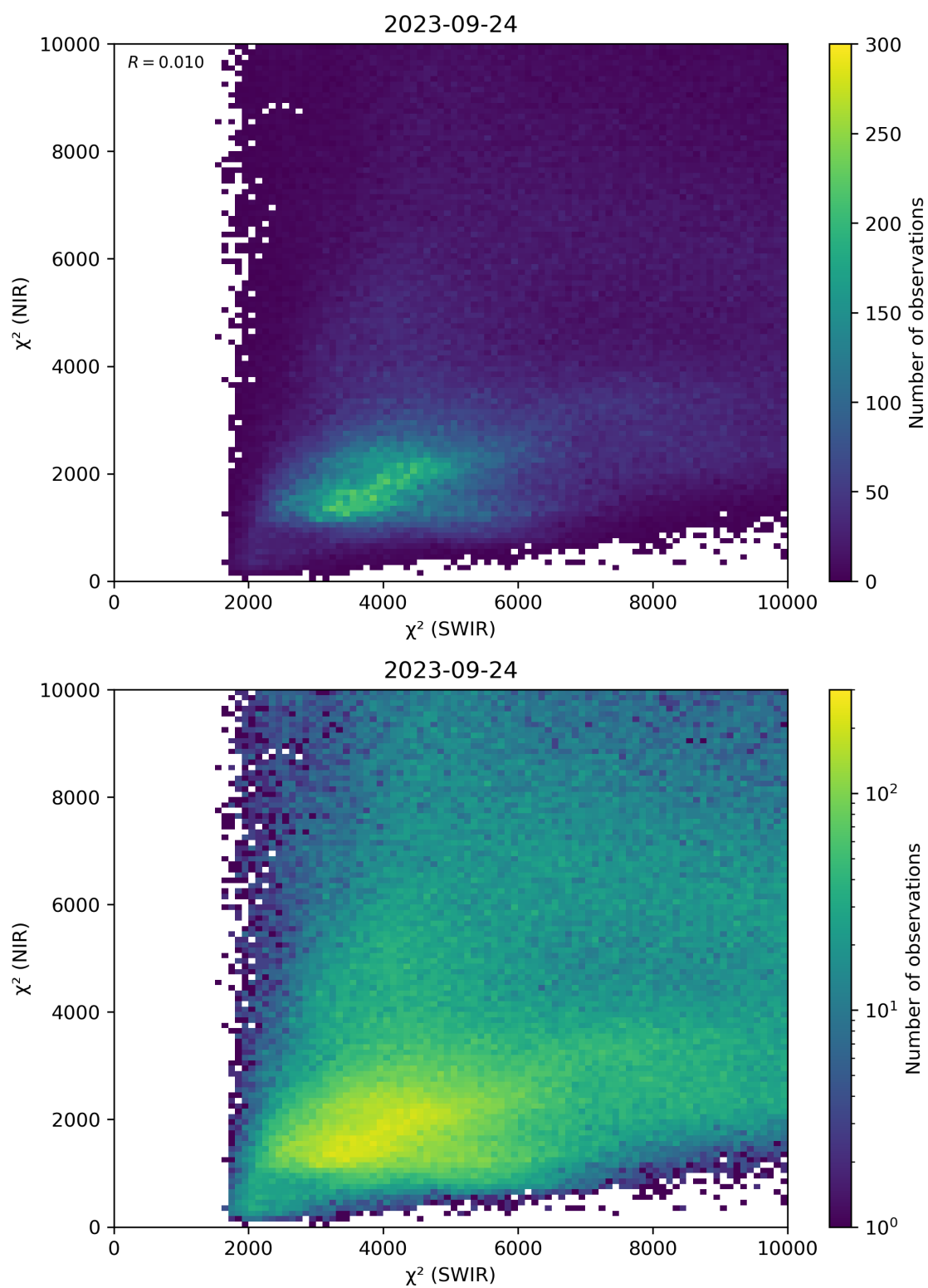
Figure 47: Scatter density plot of “ \chi^2 (SWIR)” against “ \chi^2 (NIR)” for 2023-09-23 to 2023-09-25.
