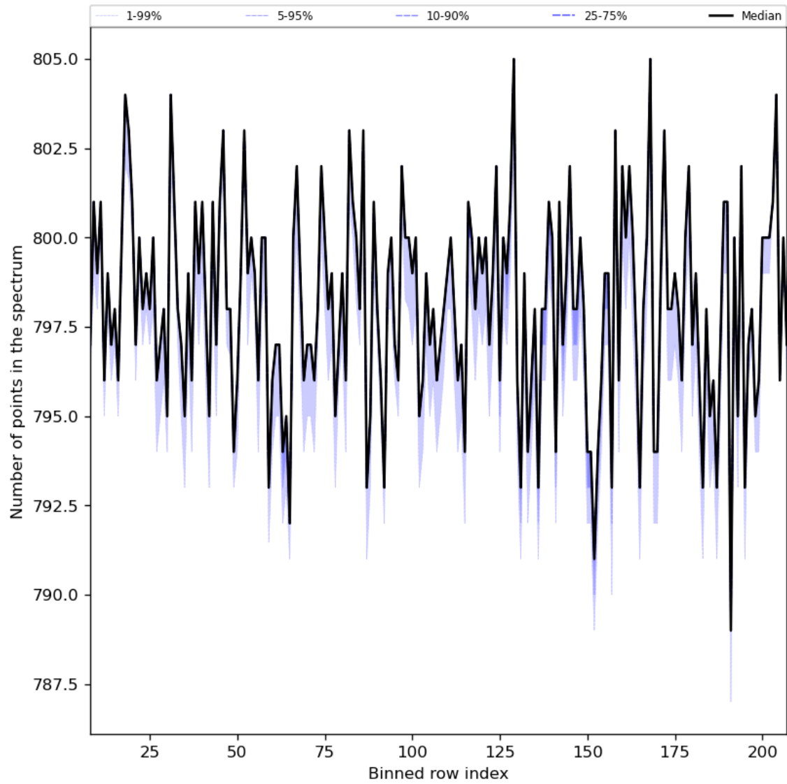
Figure 37: Along track statistics of “Number of points in the spectrum” for 2023-09-23 to 2023-09-25
