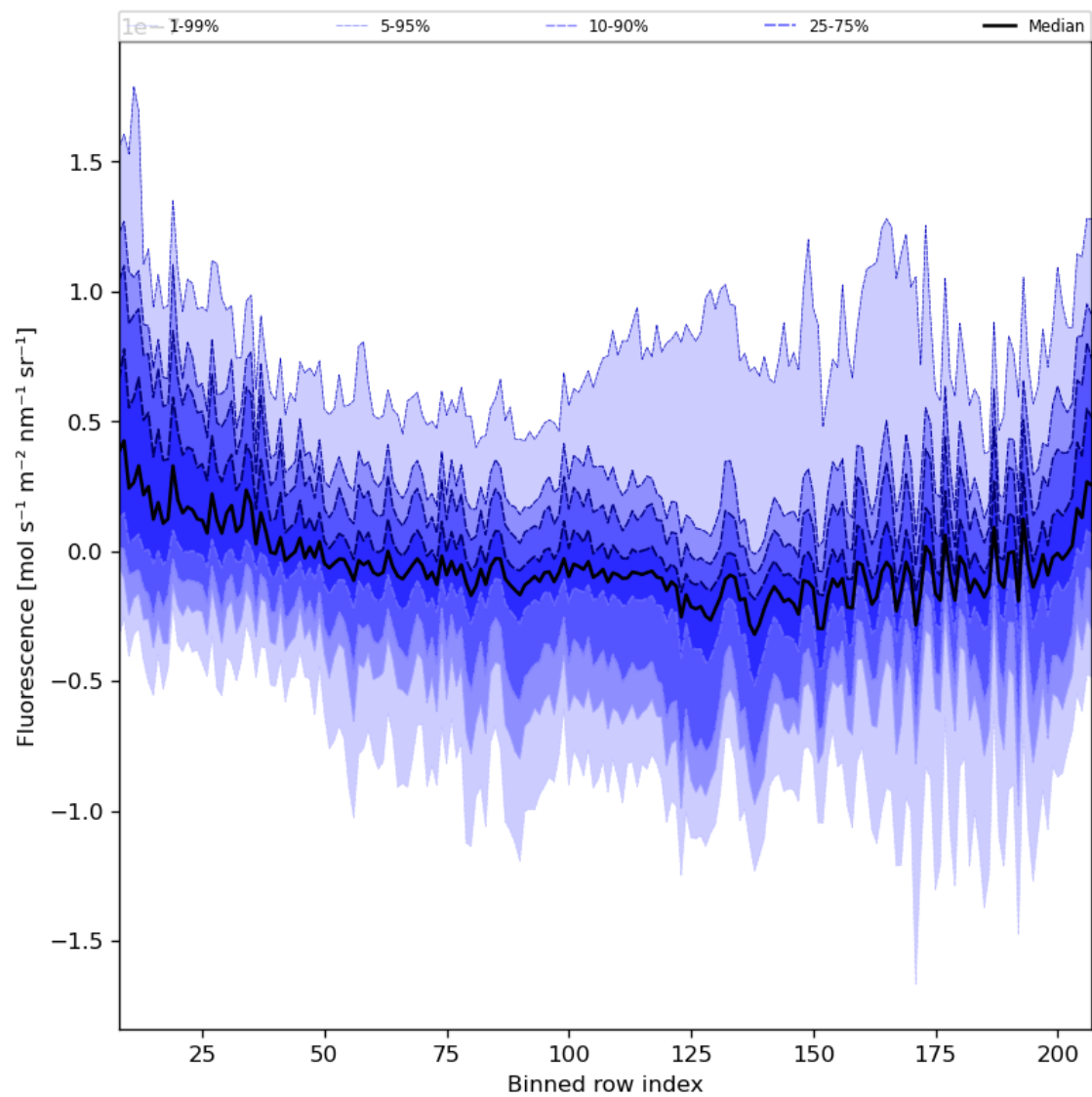
Figure 43: Along track statistics of “Fluorescence” for 2023-09-23 to 2023-09-25
