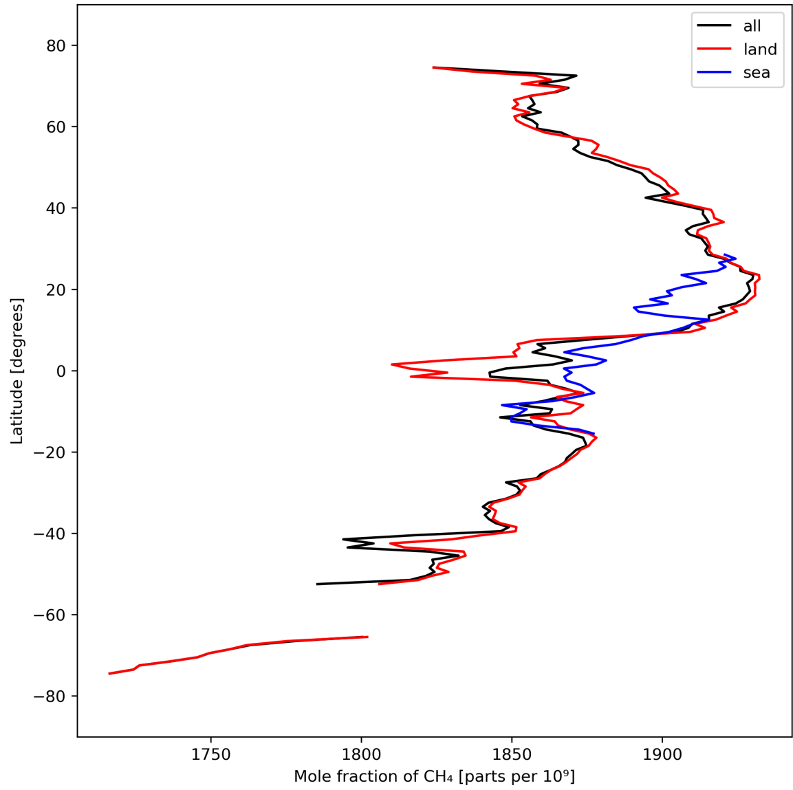
Figure 12: Zonal average of “Mole fraction of \text{CH}_4 ” for 2023-09-23 to 2023-09-25.
