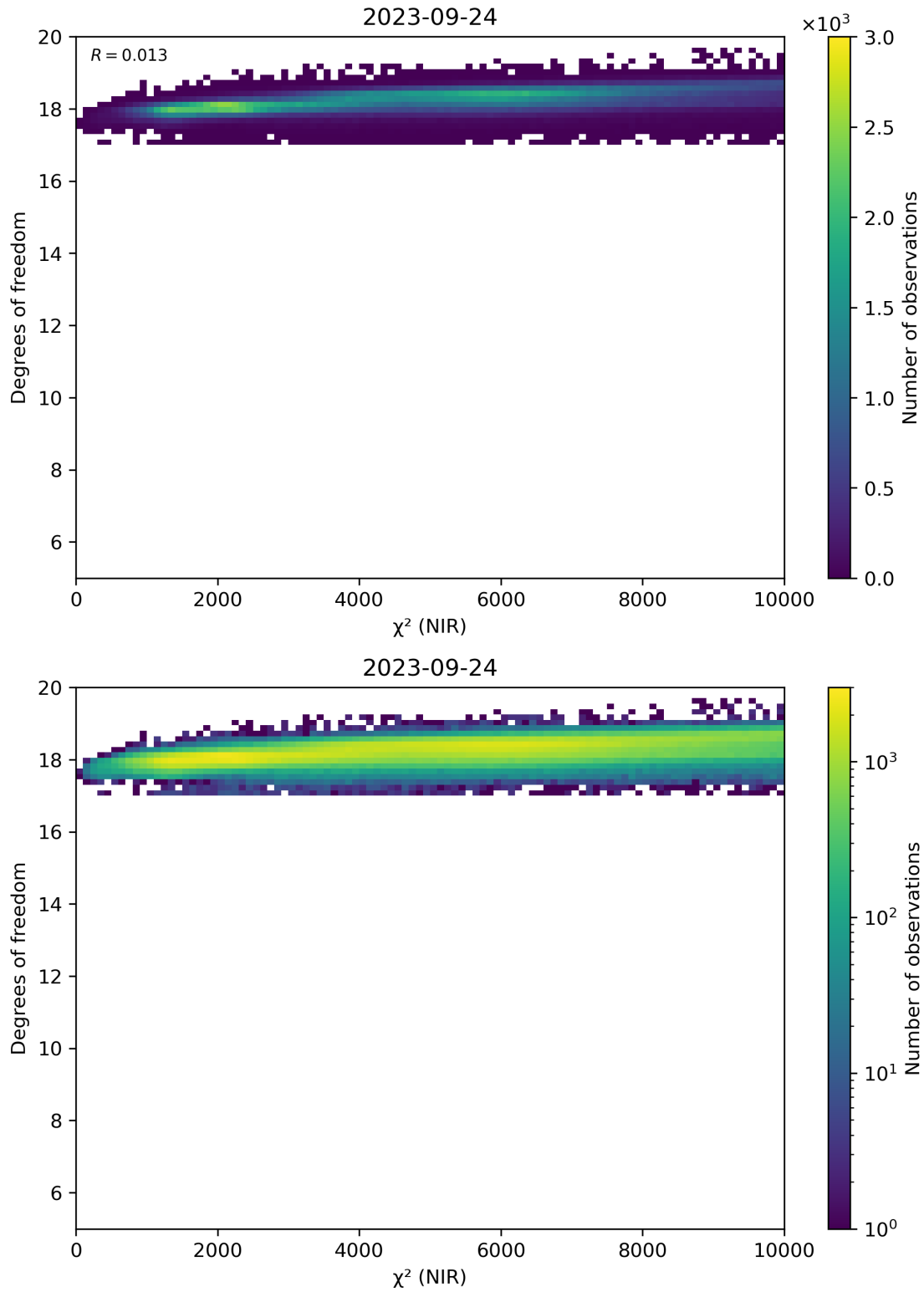
Figure 44: Scatter density plot of “ \chi^2 (NIR)” against “Degrees of freedom” for 2023-09-23 to 2023-09-25.
