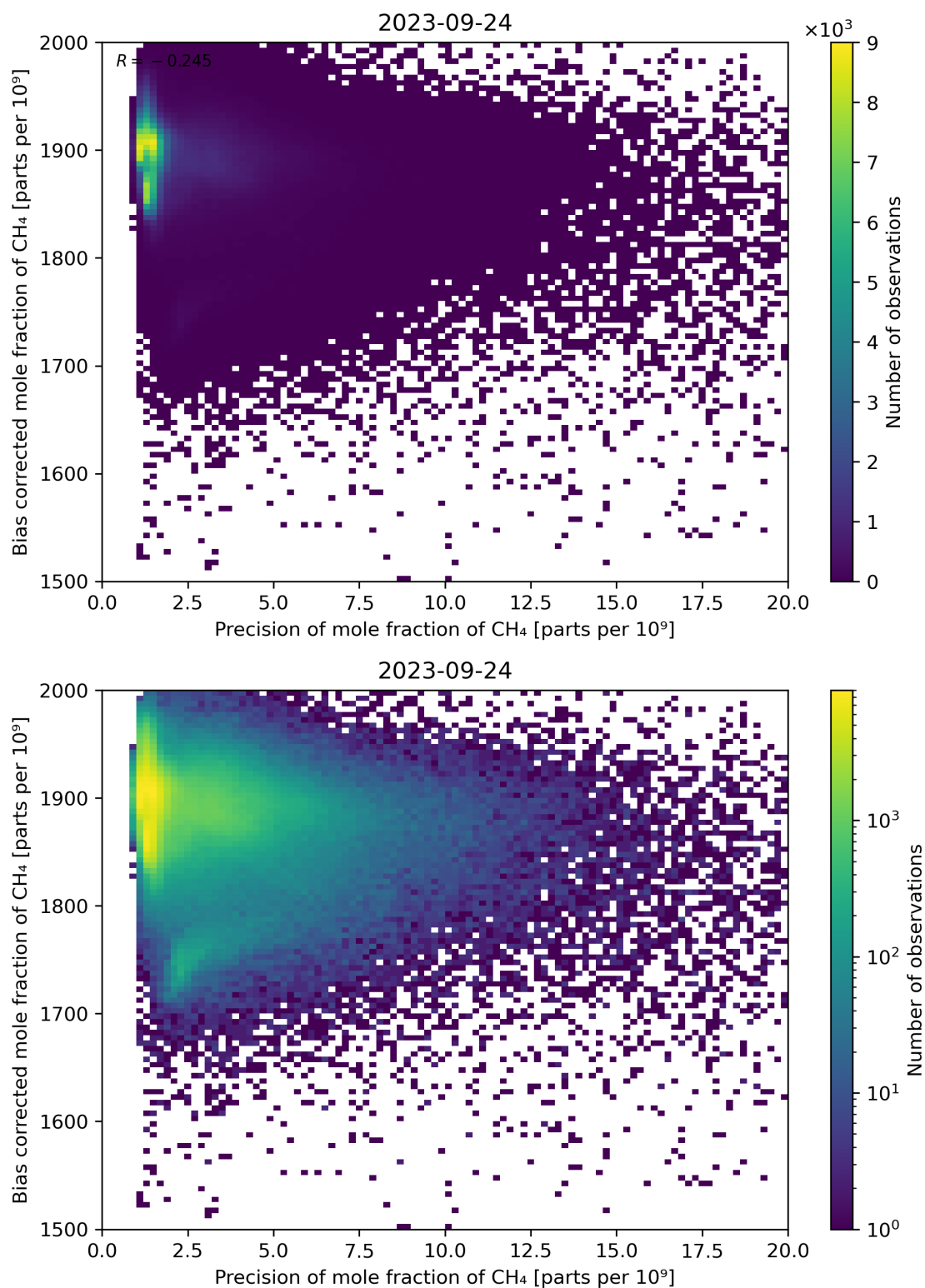
Figure 82: Scatter density plot of “Precision of mole fraction of CH 4 ” against “Bias corrected mole fraction of CH 4 ” for 2023-09-23 to 2023-09-25.
