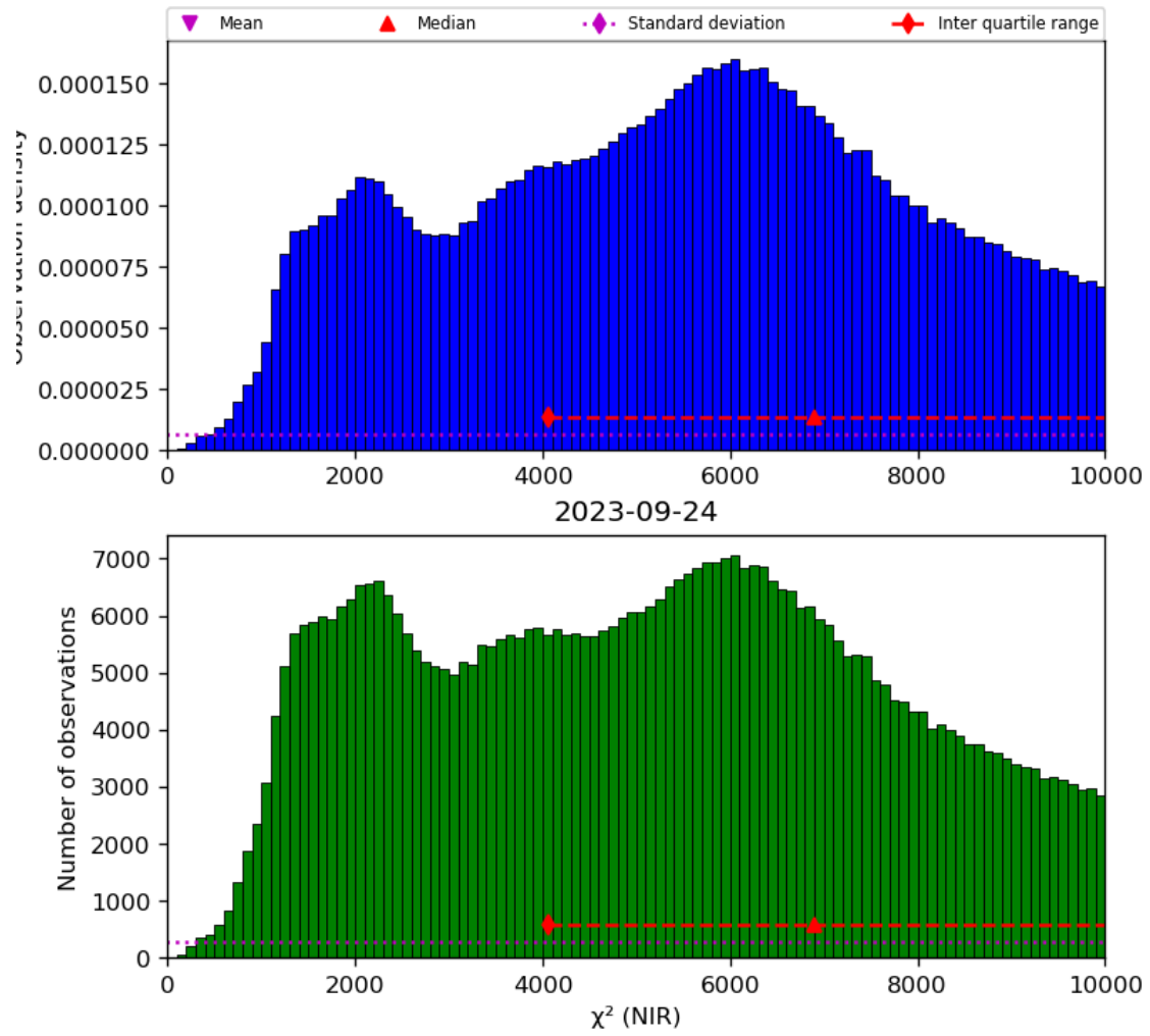
Figure 29: Histogram of “ \chi^2 (NIR)” for 2023-09-23 to 2023-09-25
