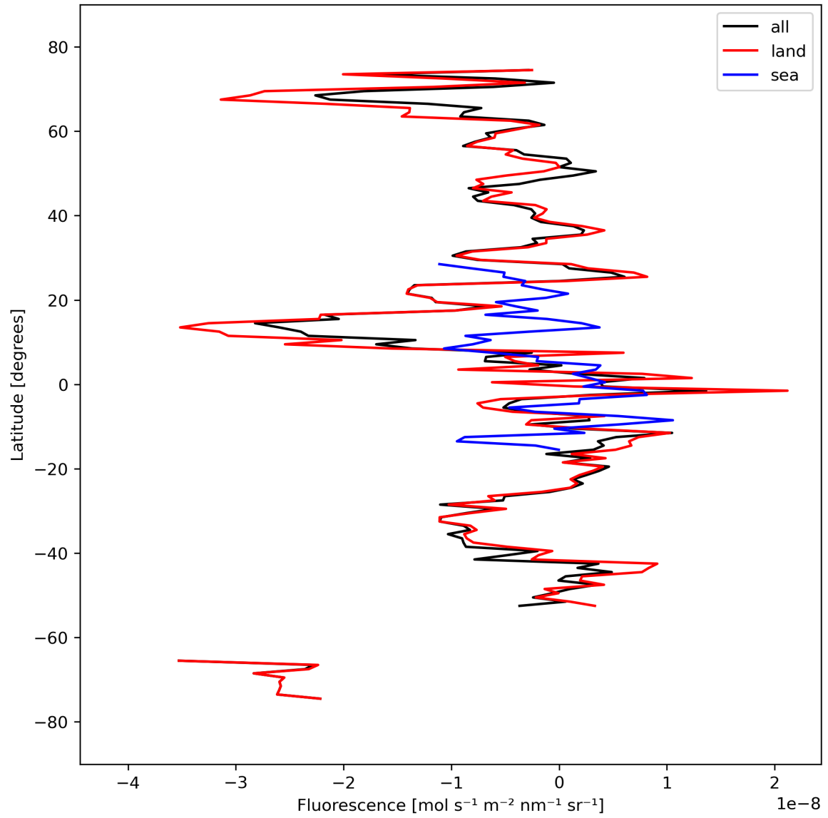
Figure 21: Zonal average of “Fluorescence” for 2023-09-23 to 2023-09-25.
