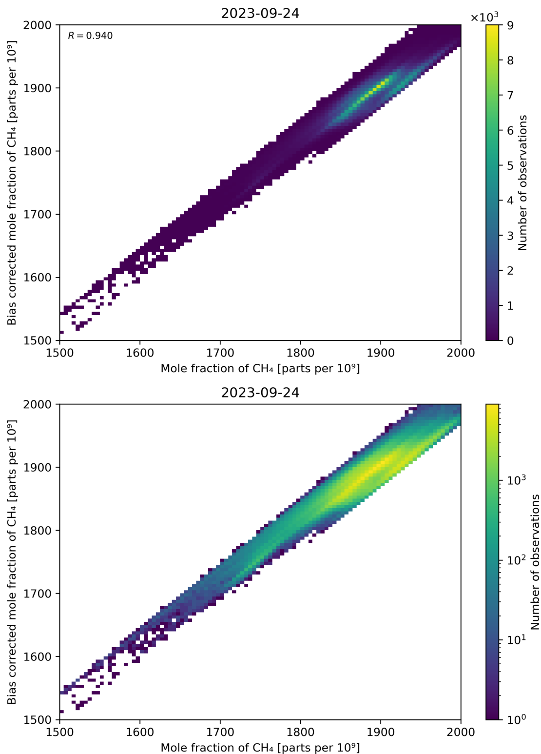
Figure 74: Scatter density plot of “Mole fraction of CH 4 ” against “Bias corrected mole fraction of CH 4 ” for 2023-09-23 to 2023-09-25.
