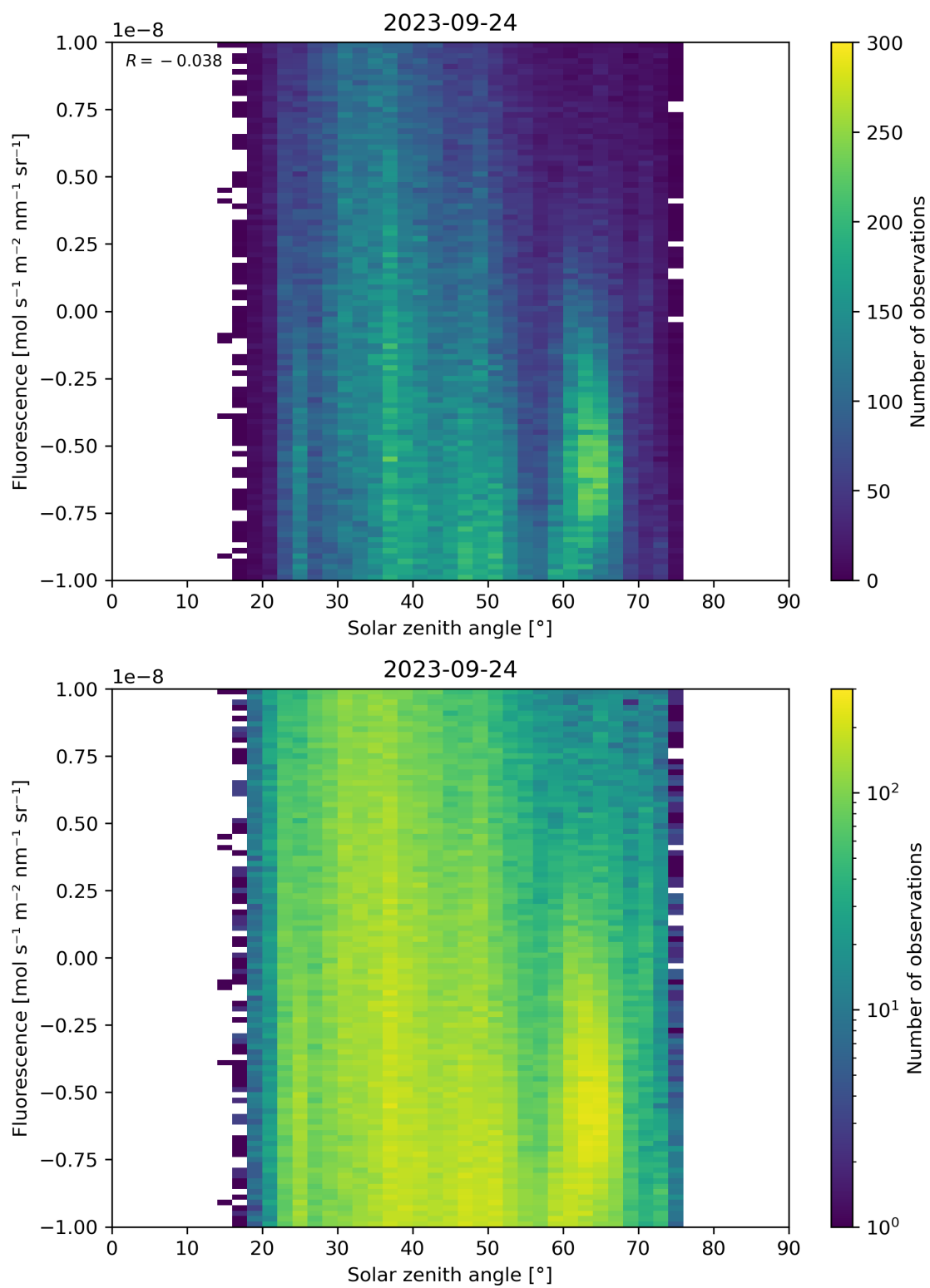
Figure 97: Scatter density plot of “Solar zenith angle” against “Fluorescence” for 2023-09-23 to 2023-09-25.
