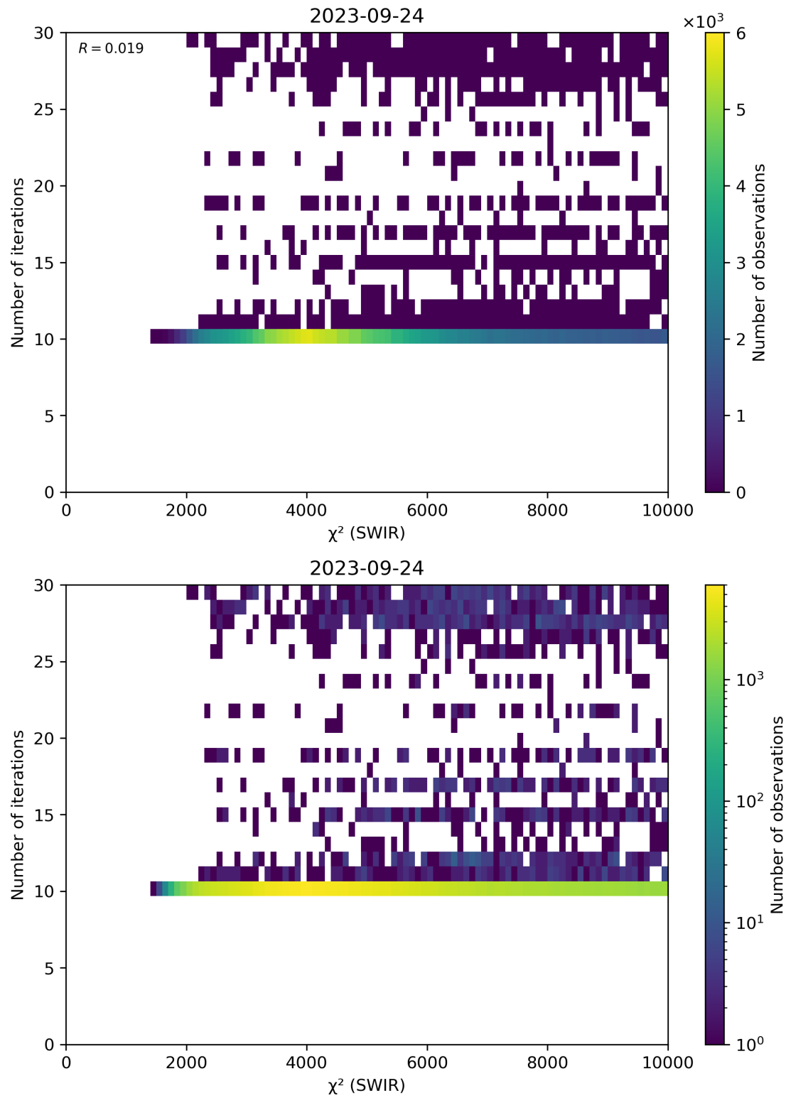
Figure 50: Scatter density plot of “ \chi^2 (SWIR)” against “Number of iterations” for 2023-09-23 to 2023-09-25.
