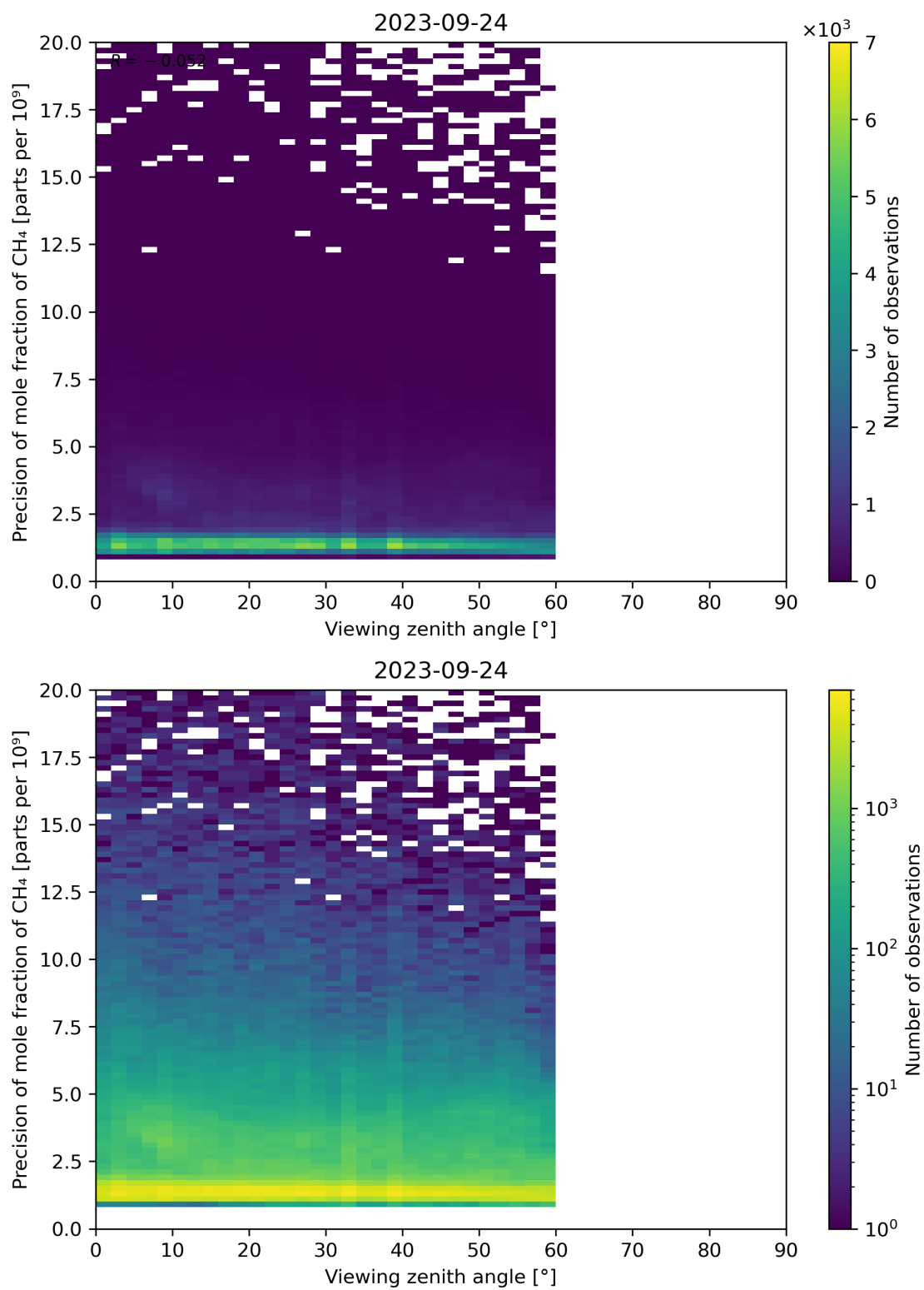
Figure 112: Scatter density plot of “Viewing zenith angle” against “Precision of mole fraction of CH 4 ” for 2023-09-23 to 2023-09-25.
