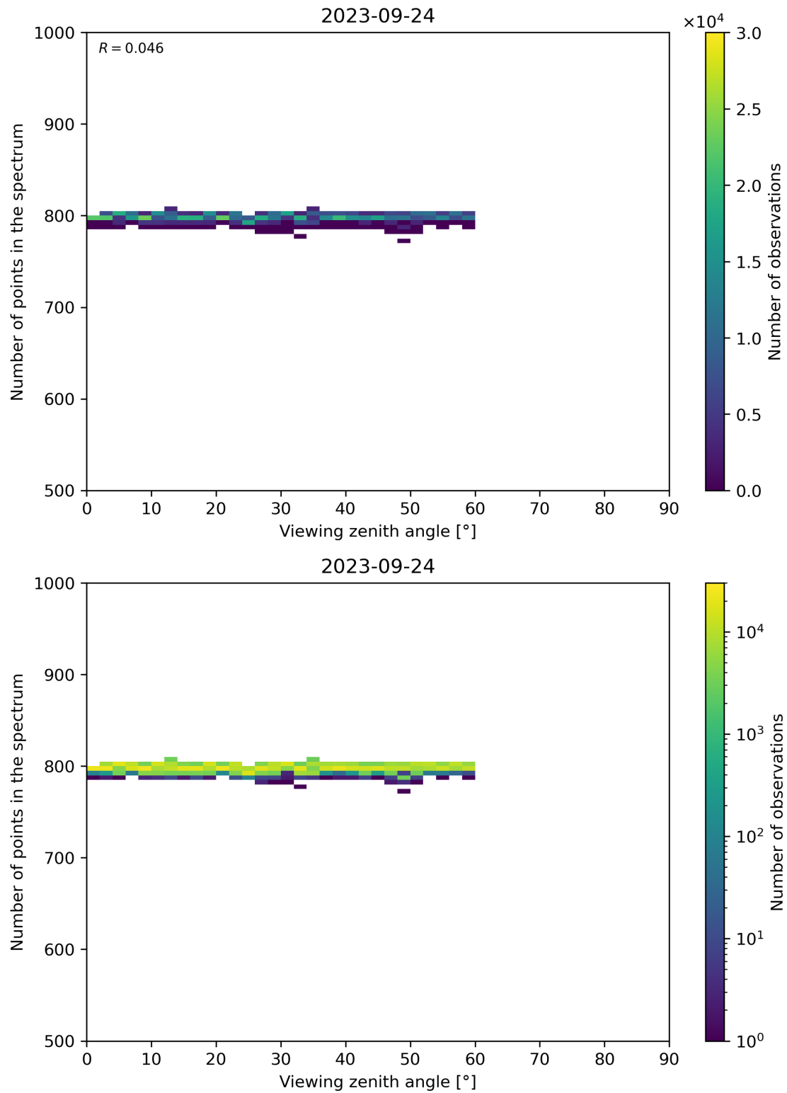
Figure 114: Scatter density plot of “Viewing zenith angle” against “Number of points in the spectrum” for 2023-09-23 to 2023-09-25.
