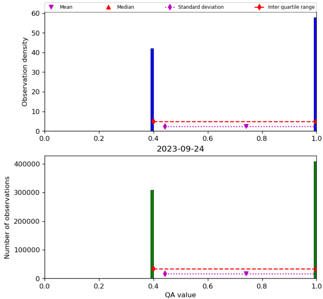
Figure 22: Histogram of “QA value” for 2023-09-23 to 2023-09-25
