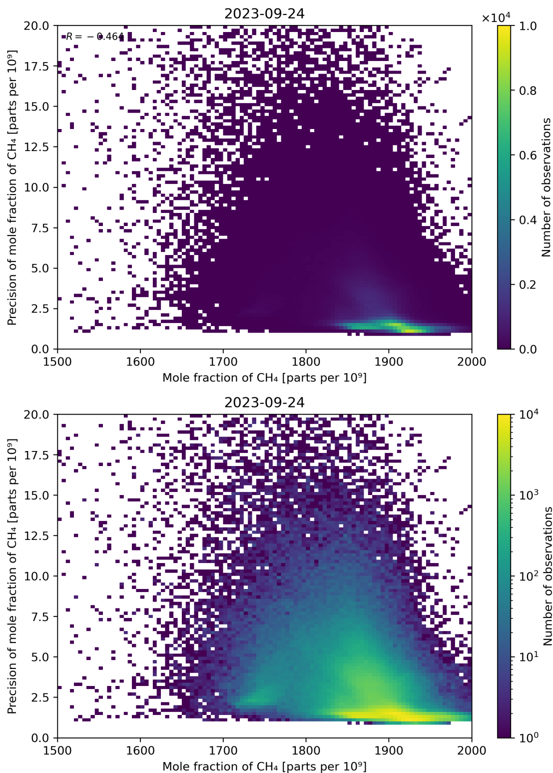
Figure 75: Scatter density plot of “Mole fraction of CH 4 ” against “Precision of mole fraction of CH 4 ” for 2023-09-23 to 2023-09-25.
