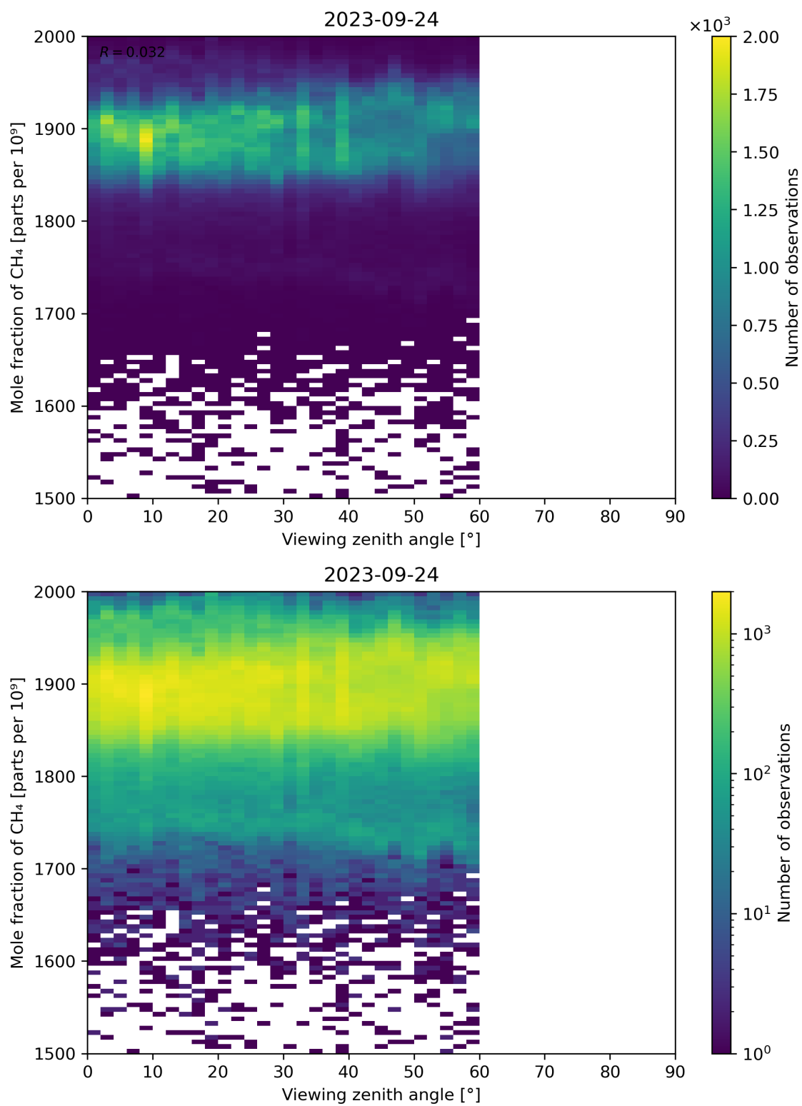
Figure 110: Scatter density plot of “Viewing zenith angle” against “Mole fraction of CH 4 ” for 2023-09-23 to 2023-09-25.
