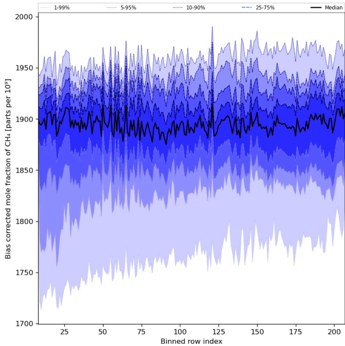
Figure 36: Along track statistics of “Bias corrected mole fraction of CH 4 ” for 2023-09-23 to 2023-09-25
