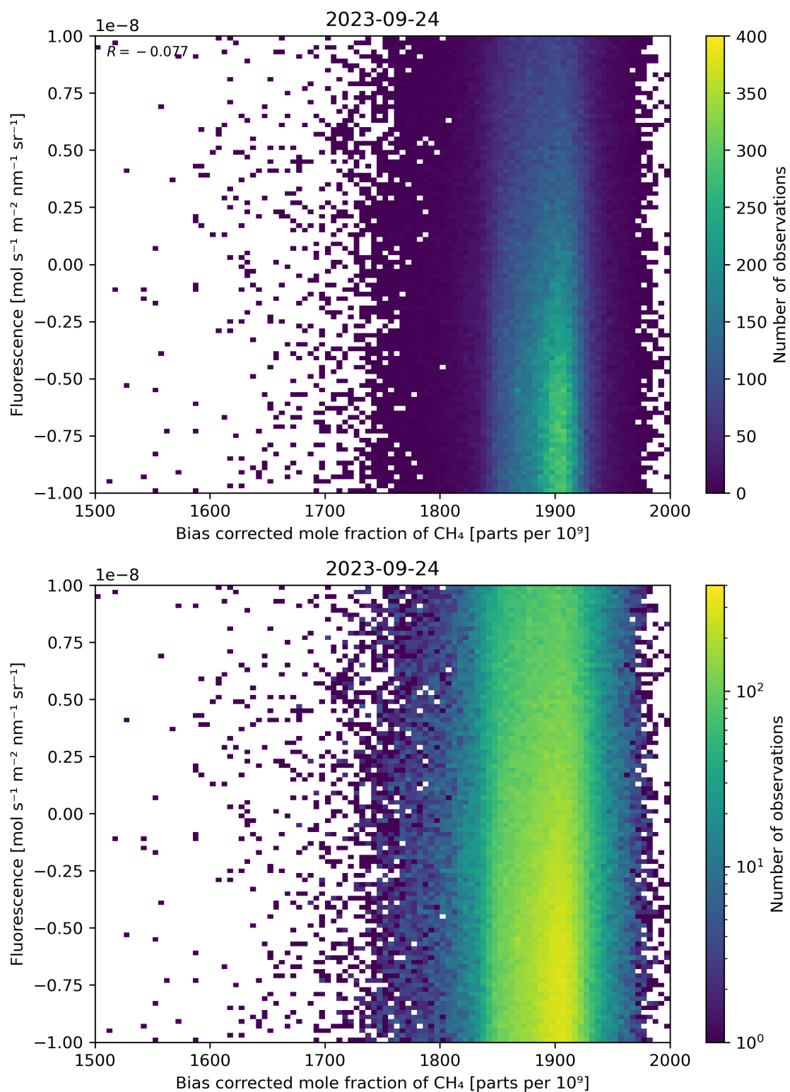
Figure 66: Scatter density plot of “Bias corrected mole fraction of \text{CH}_4 ” against “Fluorescence” for 2023-09-23 to 2023-09-25.
