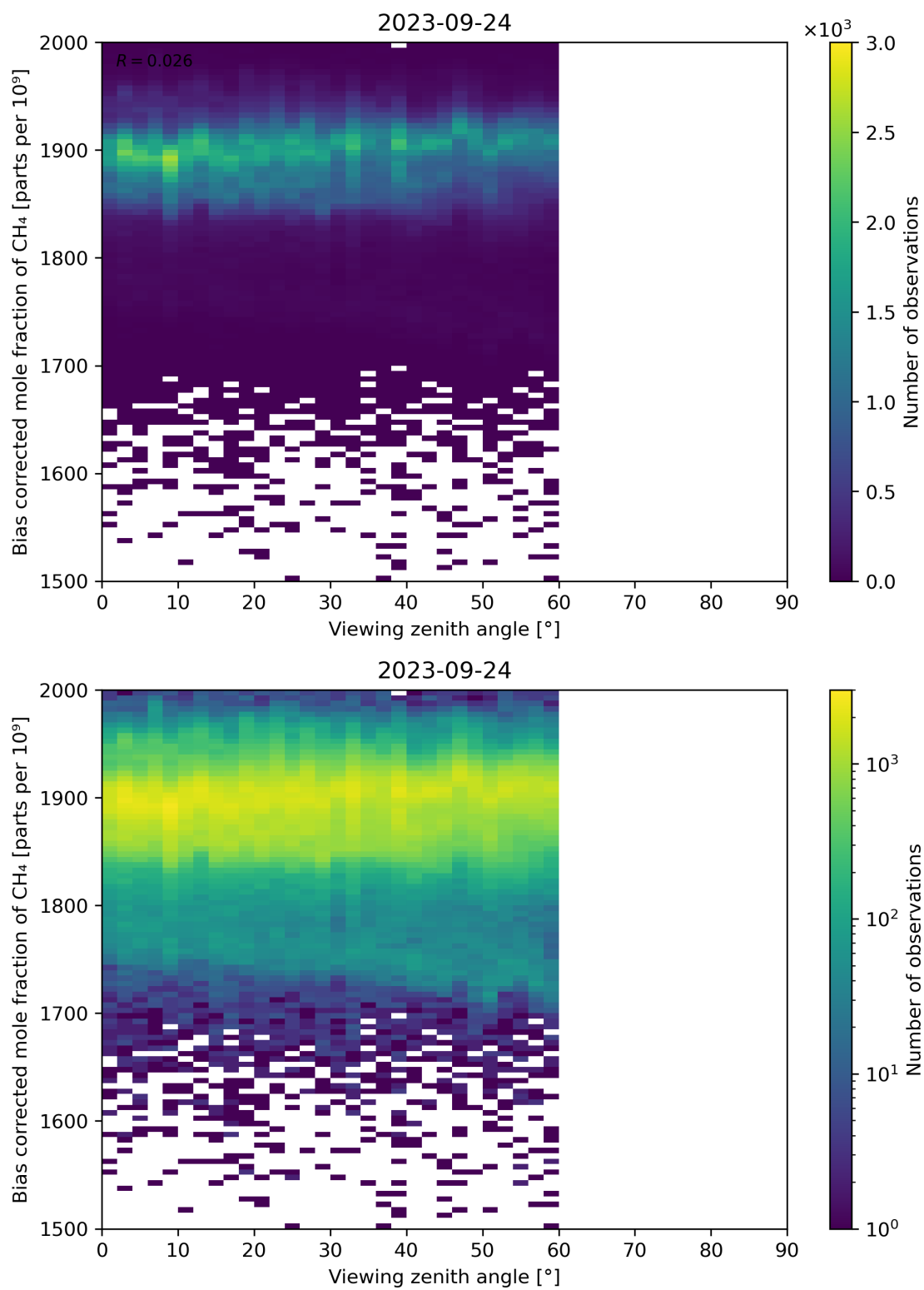
Figure 111: Scatter density plot of “Viewing zenith angle” against “Bias corrected mole fraction of CH 4 ” for 2023-09-23 to 2023-09-25.
