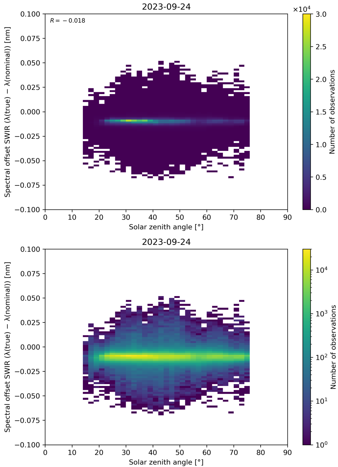
Figure 104: Scatter density plot of “Solar zenith angle” against “Spectral offset SWIR ( \lambda(\text{true}) - \lambda(\text{nominal}) )” for 2023-09-23 to 2023-09-25.
