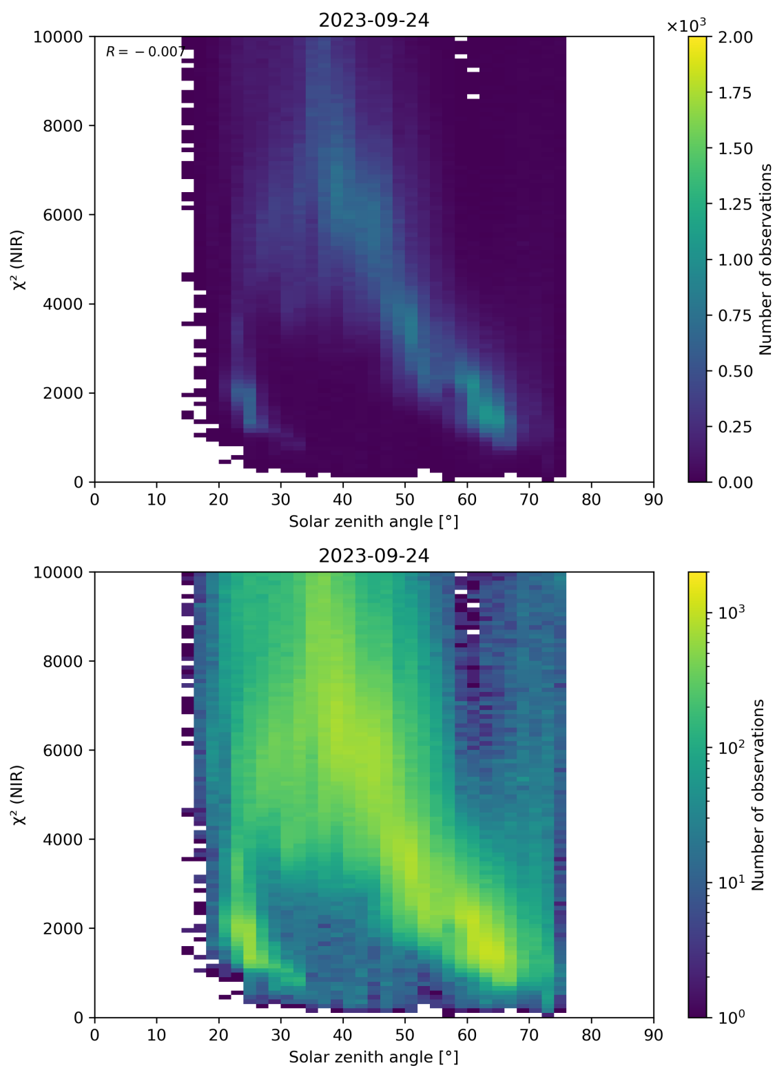
Figure 94: Scatter density plot of “Solar zenith angle” against “ \chi^2 (NIR)” for 2023-09-23 to 2023-09-25.
