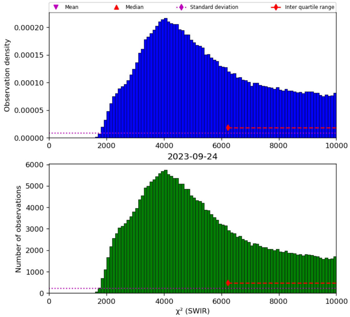
Figure 28: Histogram of " \chi^2 (SWIR)" for 2023-09-23 to 2023-09-25
