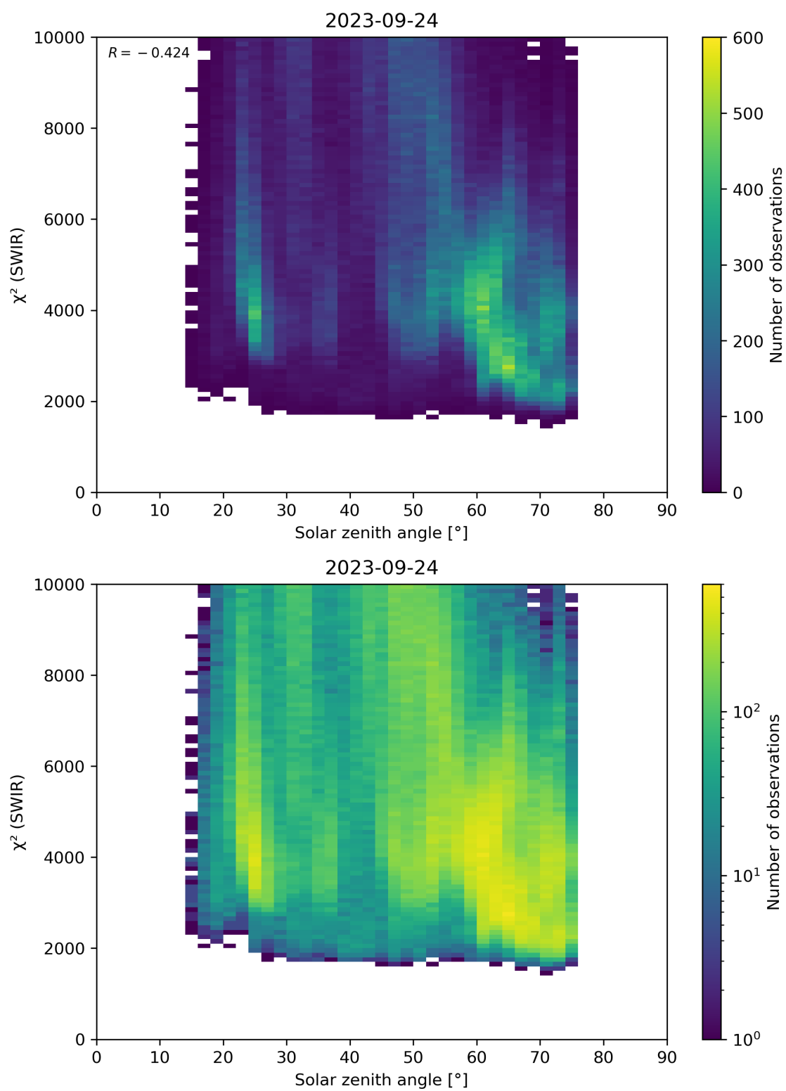
Figure 95: Scatter density plot of “Solar zenith angle” against “ \chi^2 (SWIR)” for 2023-09-23 to 2023-09-25.
