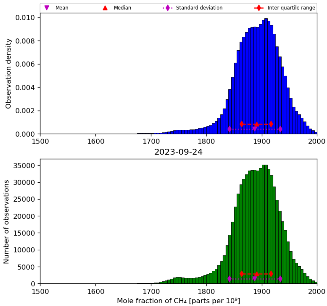
Figure 23: Histogram of “Mole fraction of CH 4 ” for 2023-09-23 to 2023-09-25
