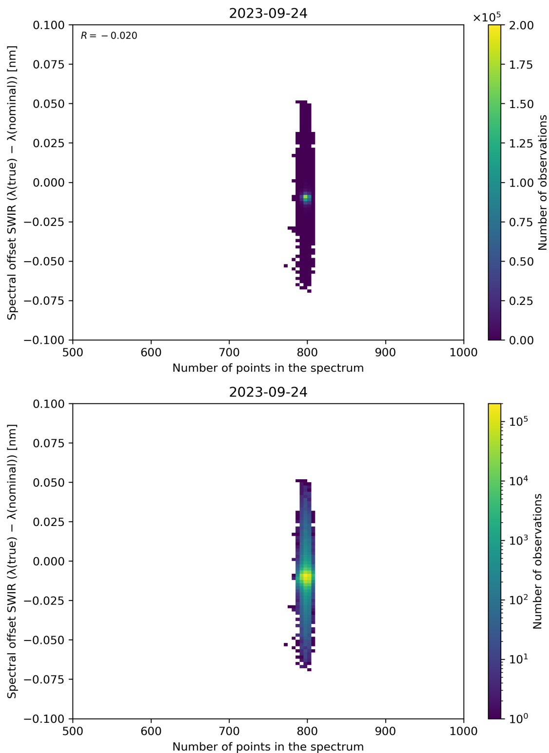
Figure 93: Scatter density plot of “Number of points in the spectrum” against “Spectral offset SWIR ( \lambda(\text{true}) - \lambda(\text{nominal}) )” for 2023-09-23 to 2023-09-25.
