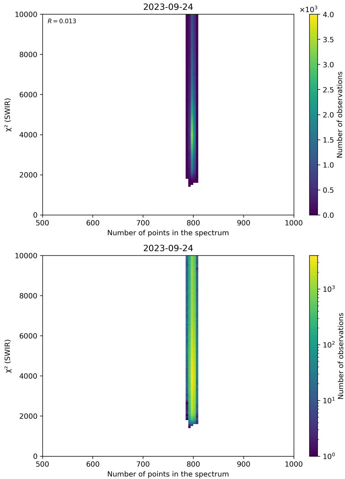
Figure 89: Scatter density plot of “Number of points in the spectrum” against “ \chi^2 (SWIR)” for 2023-09-23 to 2023-09-25.
