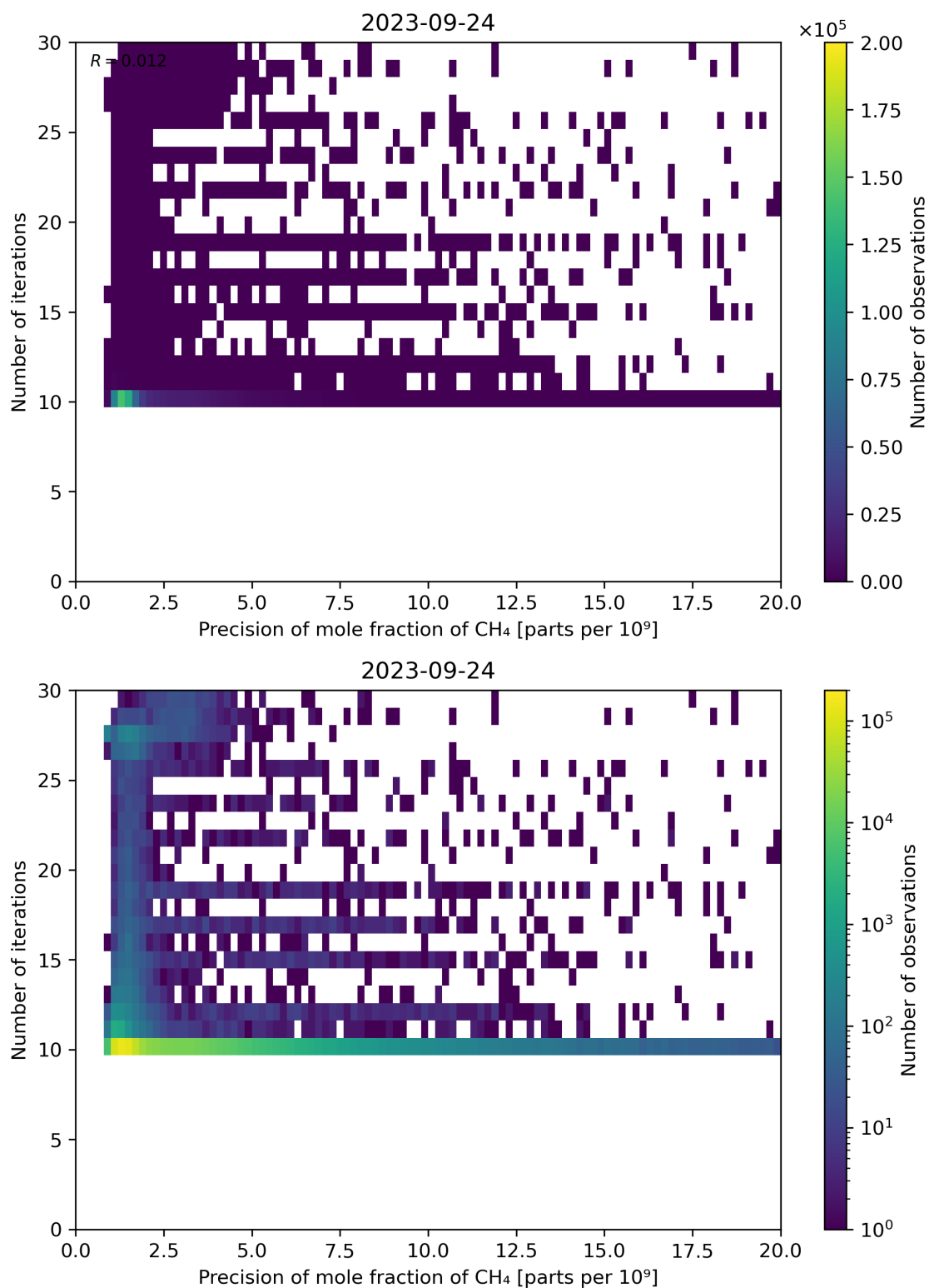
Figure 83: Scatter density plot of “Precision of mole fraction of CH 4 ” against “Number of iterations” for 2023-09-23 to 2023-09-25.
