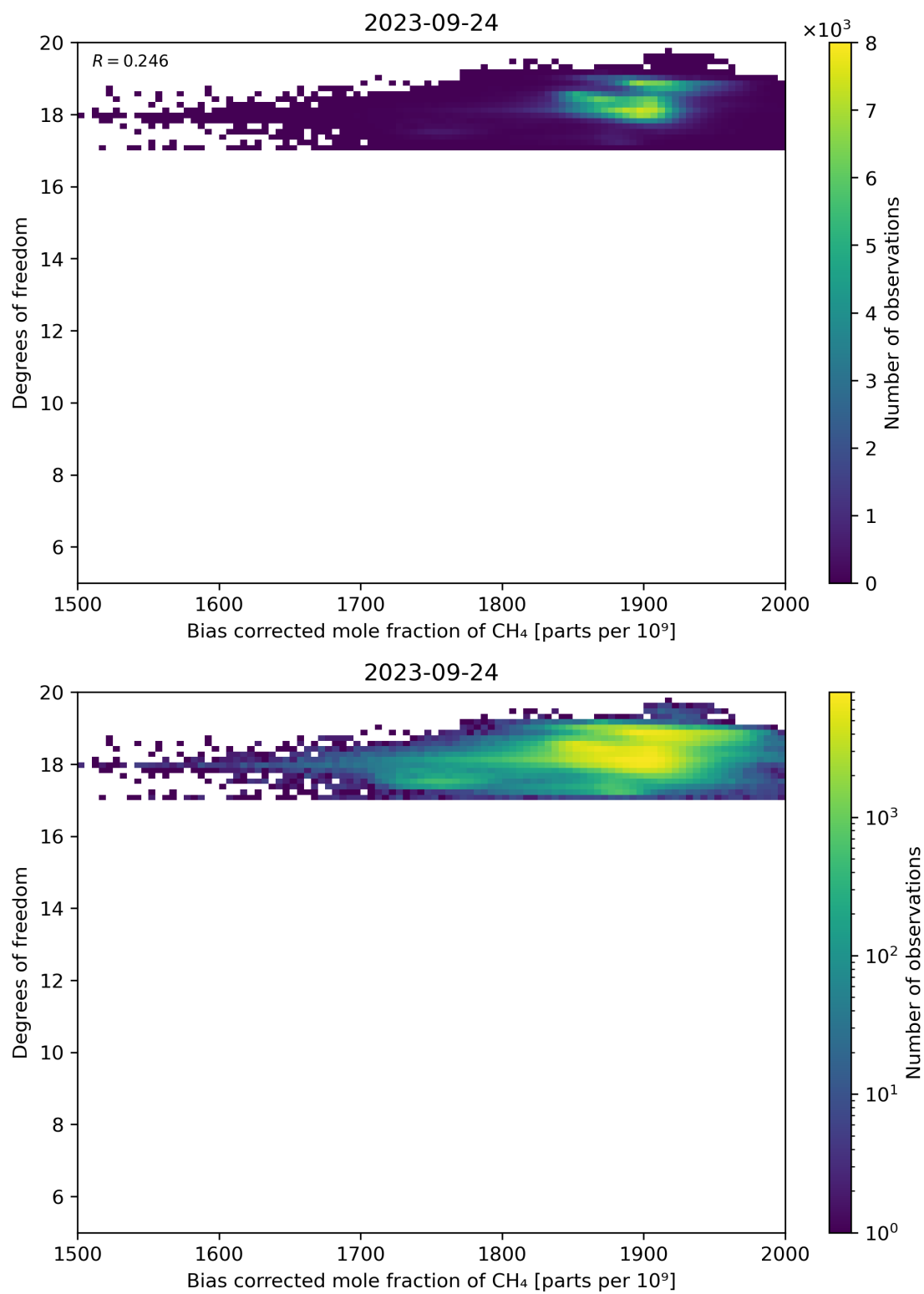
Figure 65: Scatter density plot of “Bias corrected mole fraction of CH 4 ” against “Degrees of freedom” for 2023-09-23 to 2023-09-25.
