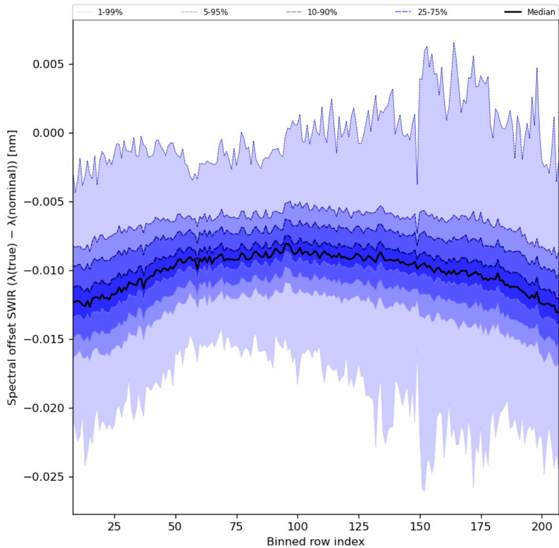
Figure 38: Along track statistics of “Spectral offset SWIR ( \lambda(\text{true}) - \lambda(\text{nominal}) )” for 2023-09-23 to 2023-09-25
