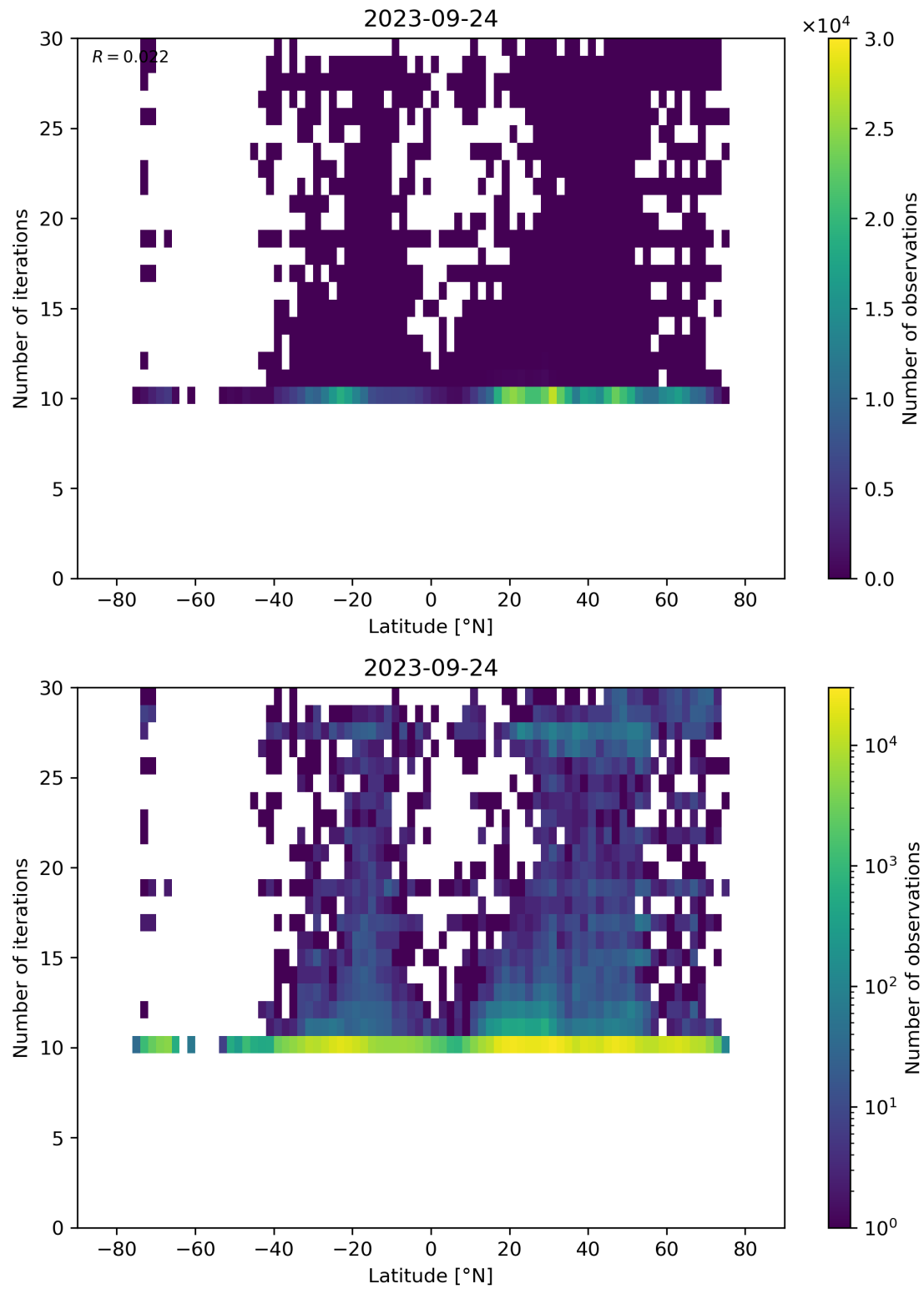
Figure 60: Scatter density plot of “Latitude” against “Number of iterations” for 2023-09-23 to 2023-09-25.
