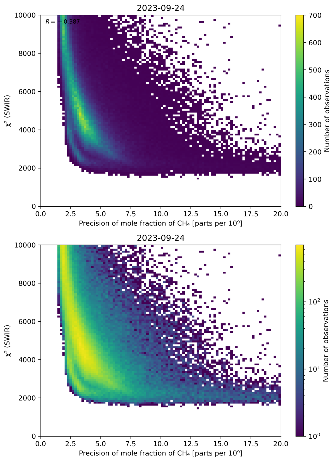
Figure 79: Scatter density plot of “Precision of mole fraction of CH 4 ” against “ \chi^2 (SWIR)” for 2023-09-23 to 2023-09-25.
