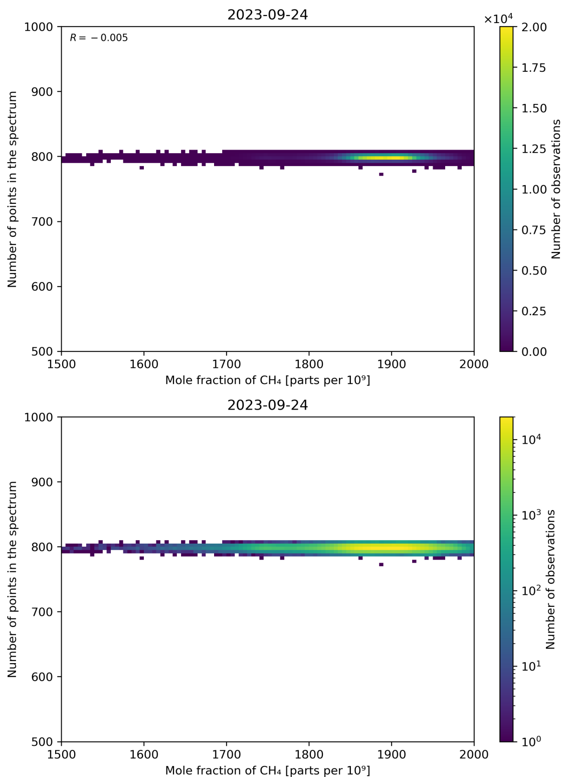
Figure 77: Scatter density plot of “Mole fraction of CH 4 ” against “Number of points in the spectrum” for 2023-09-23 to 2023-09-25.
