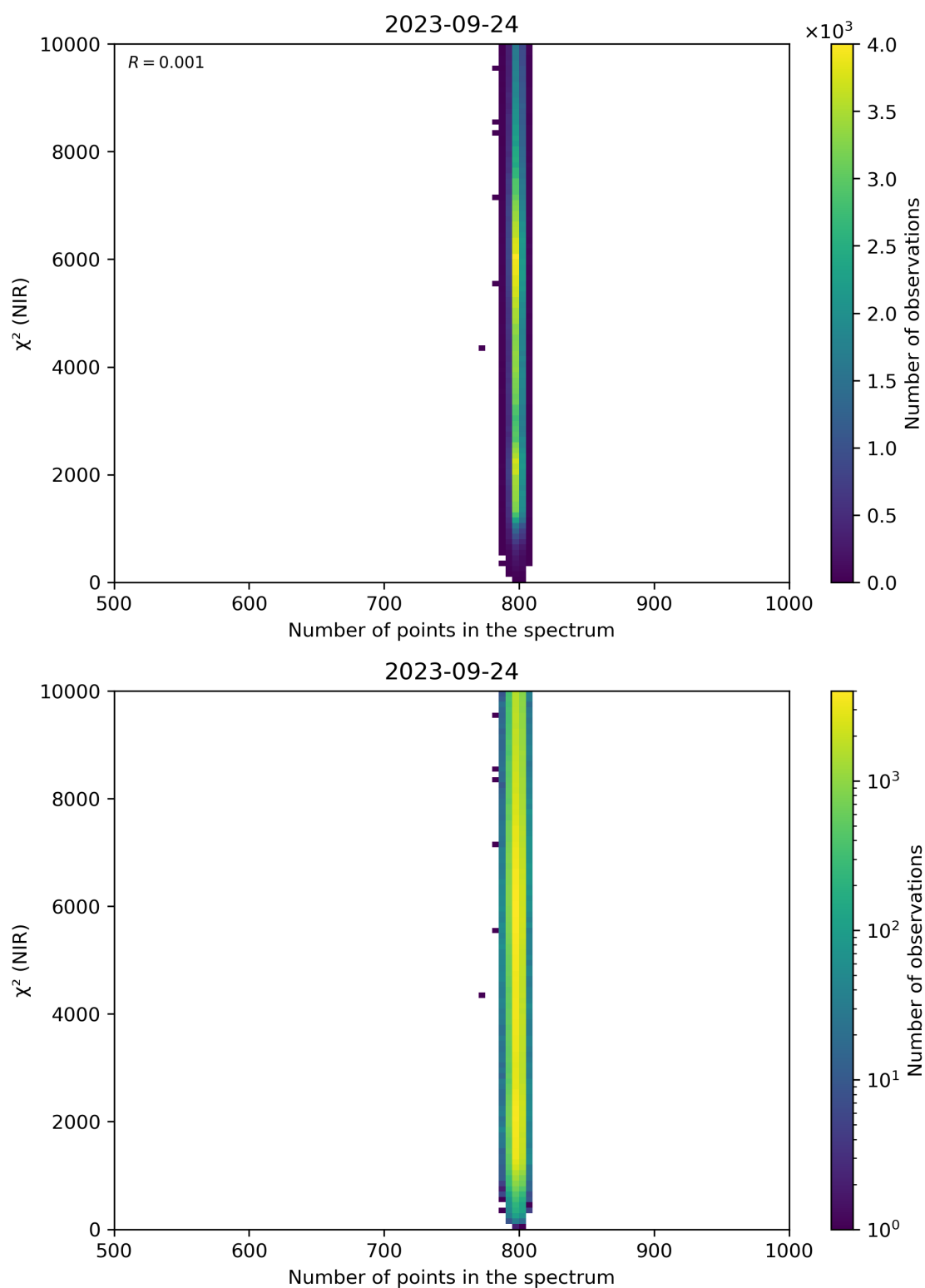
Figure 88: Scatter density plot of “Number of points in the spectrum” against “ \chi^2 (NIR)” for 2023-09-23 to 2023-09-25.
