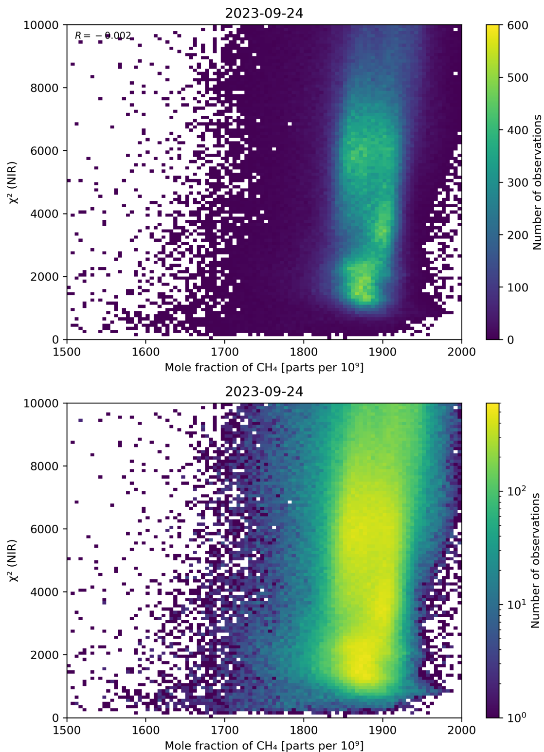
Figure 70: Scatter density plot of “Mole fraction of \text{CH}_4 ” against “ \chi^2 (NIR)” for 2023-09-23 to 2023-09-25.
