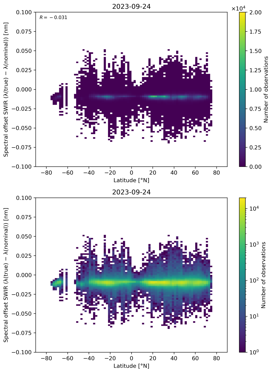
Figure 62: Scatter density plot of “Latitude” against “Spectral offset SWIR ( \lambda(\text{true}) - \lambda(\text{nominal}) )” for 2023-09-23 to 2023-09-25.
