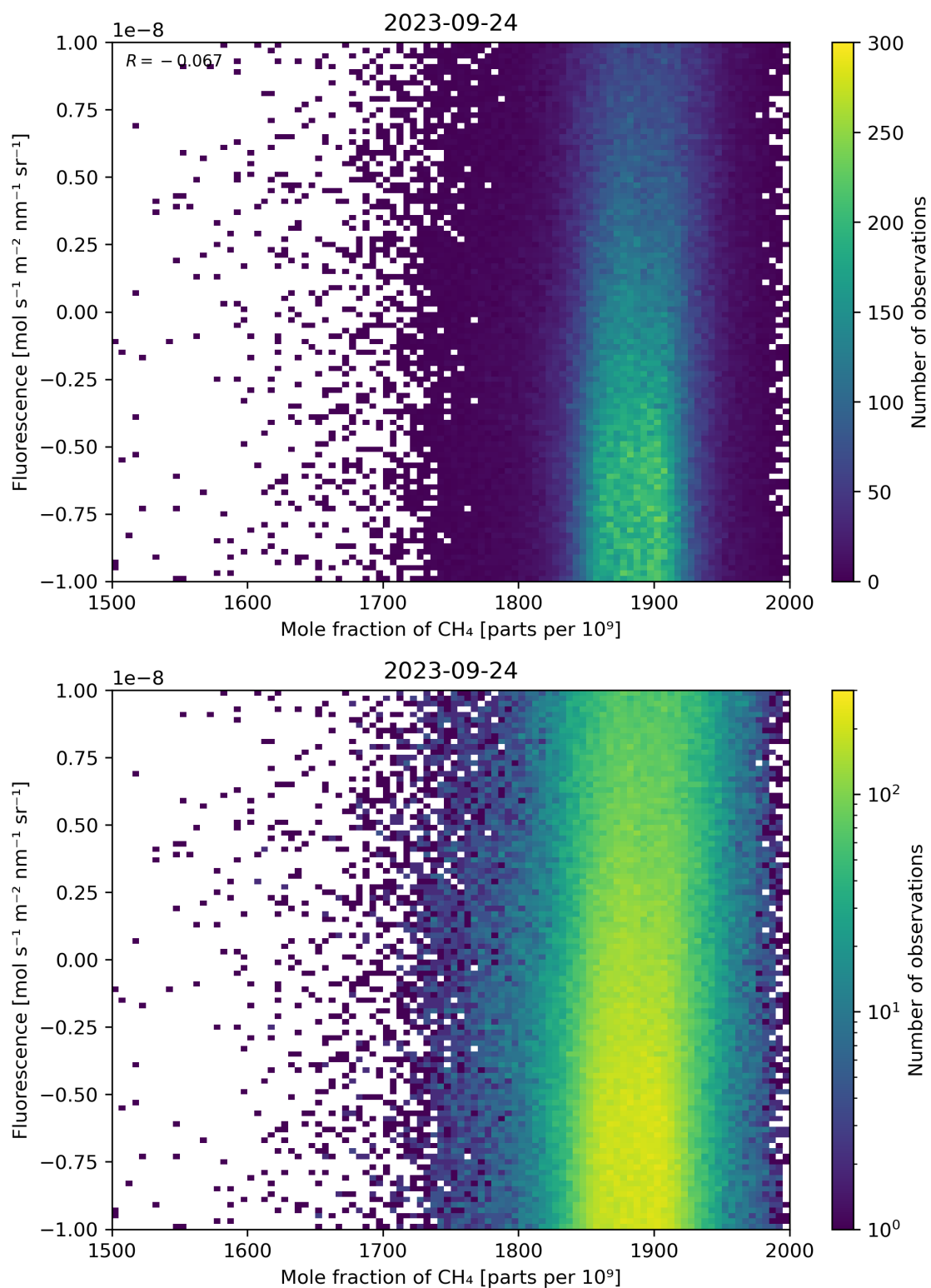
Figure 73: Scatter density plot of “Mole fraction of \text{CH}_4 ” against “Fluorescence” for 2023-09-23 to 2023-09-25.
