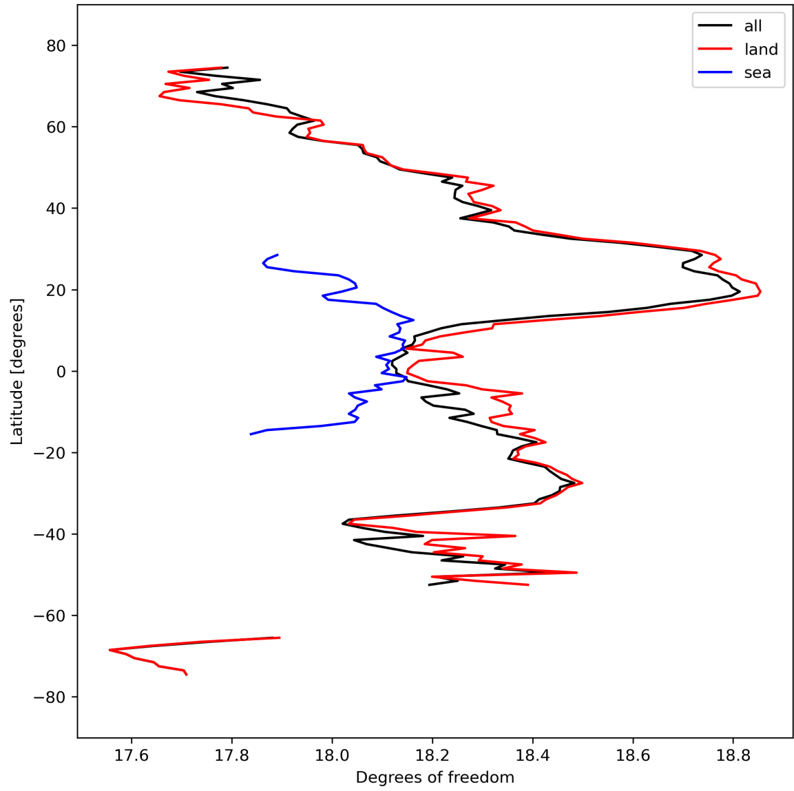
Figure 19: Zonal average of “Degrees of freedom” for 2023-09-23 to 2023-09-25.
