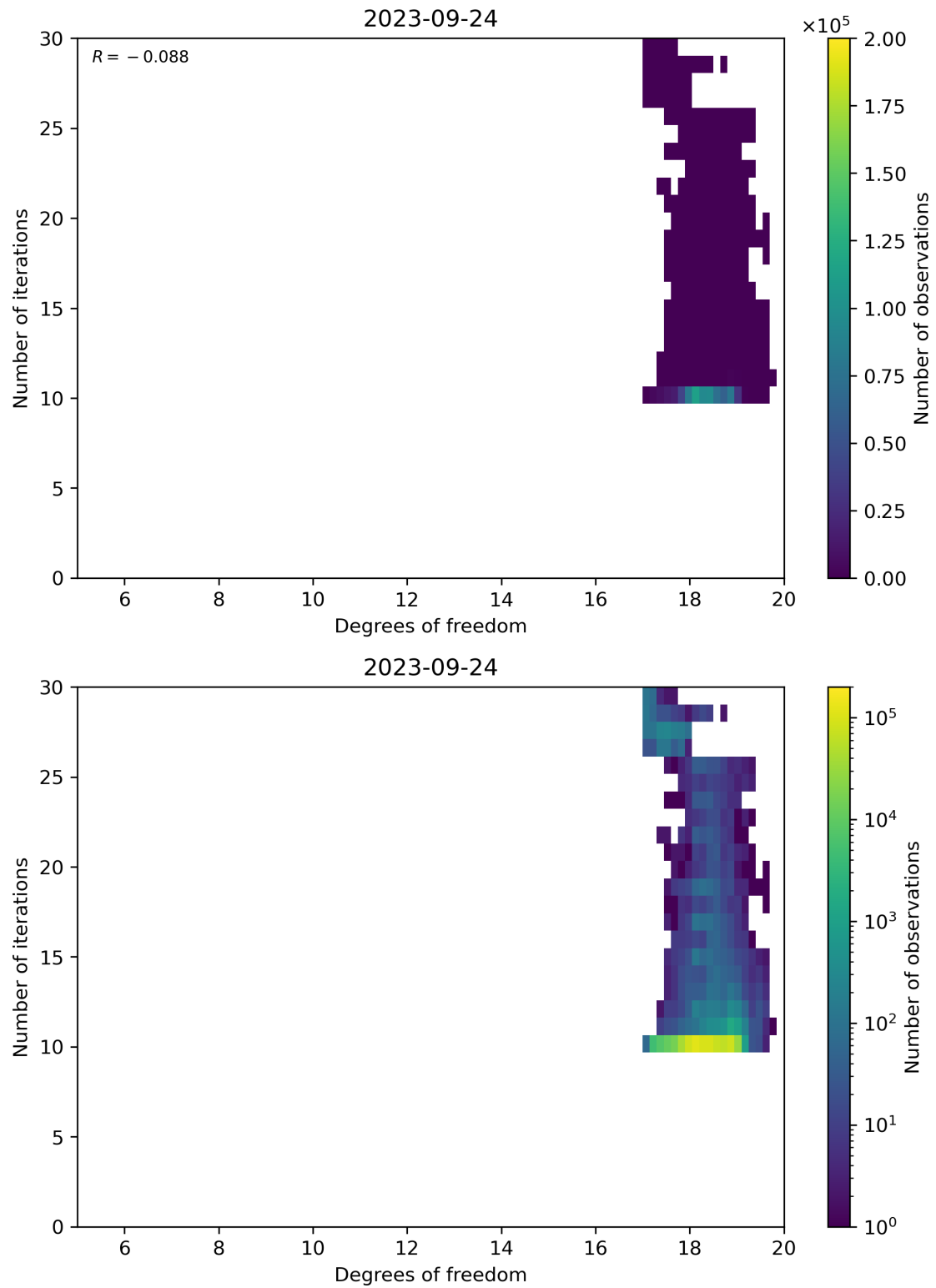
Figure 52: Scatter density plot of “Degrees of freedom” against “Number of iterations” for 2023-09-23 to 2023-09-25.
