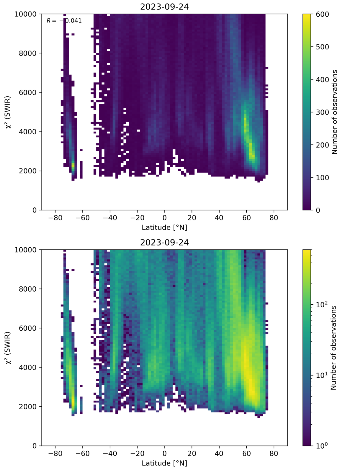
Figure 54: Scatter density plot of “Latitude” against “ \chi^2 (SWIR)” for 2023-09-23 to 2023-09-25.
