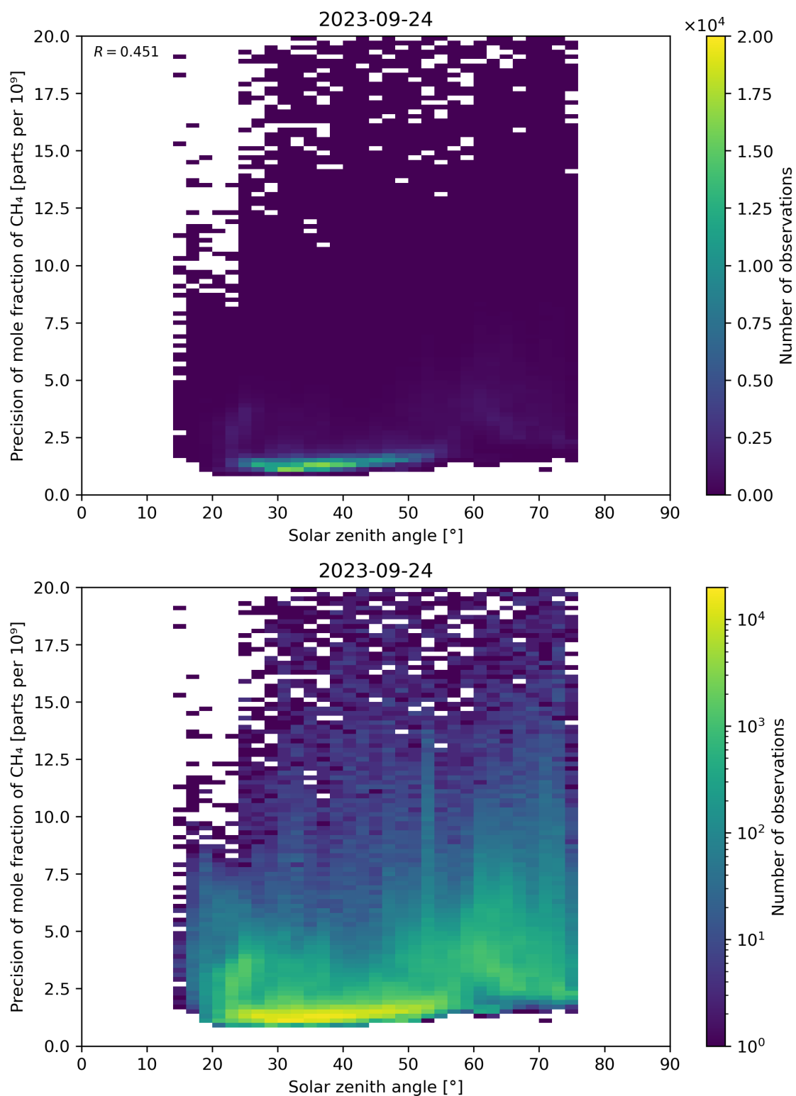
Figure 101: Scatter density plot of “Solar zenith angle” against “Precision of mole fraction of \text{CH}_4 ” for 2023-09-23 to 2023-09-25.
