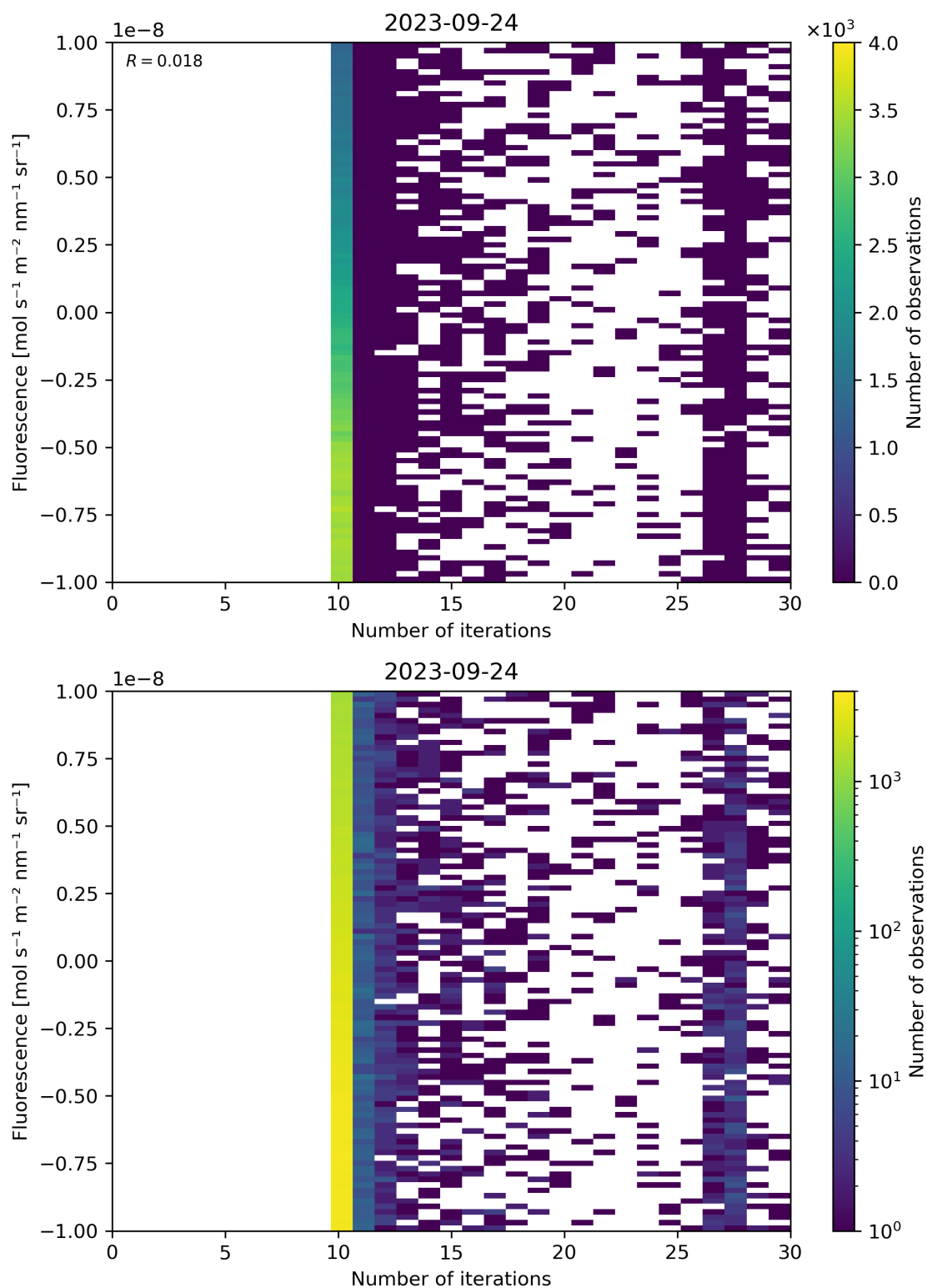
Figure 87: Scatter density plot of “Number of iterations” against “Fluorescence” for 2023-09-23 to 2023-09-25.
