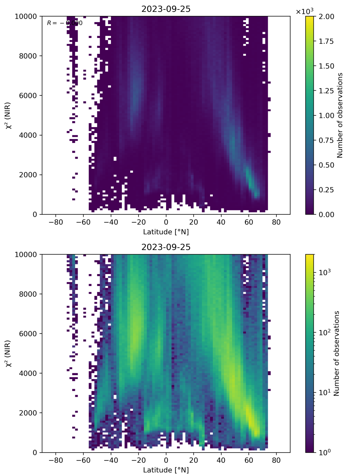
Figure 53: Scatter density plot of “Latitude” against “ \chi^2 (NIR)” for 2023-09-24 to 2023-09-26.
