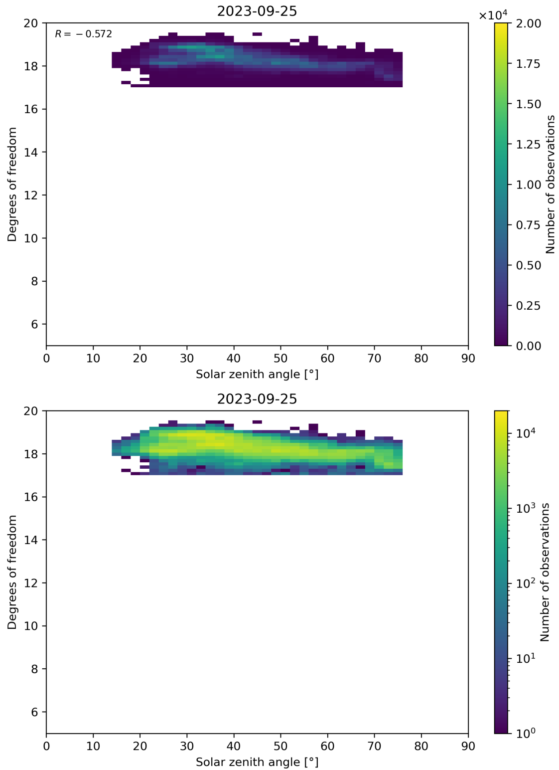
Figure 96: Scatter density plot of “Solar zenith angle” against “Degrees of freedom” for 2023-09-24 to 2023-09-26.
