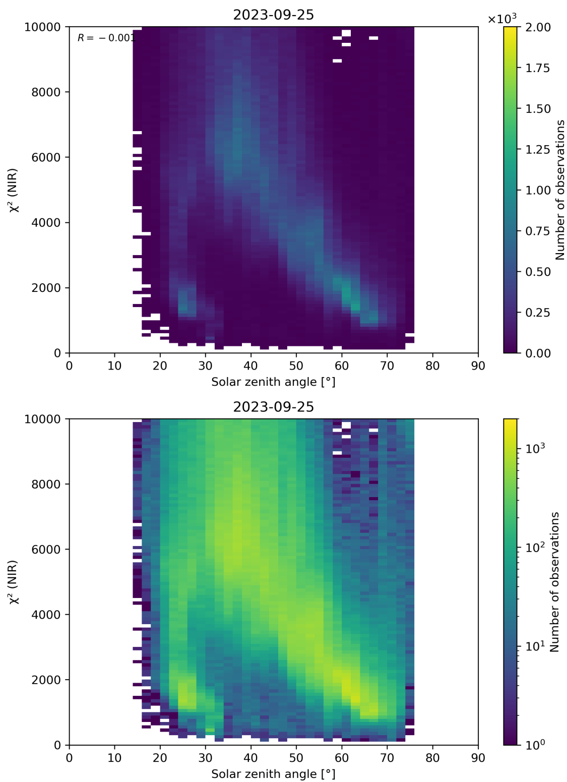
Figure 94: Scatter density plot of “Solar zenith angle” against “ \chi^2 (NIR)” for 2023-09-24 to 2023-09-26.
