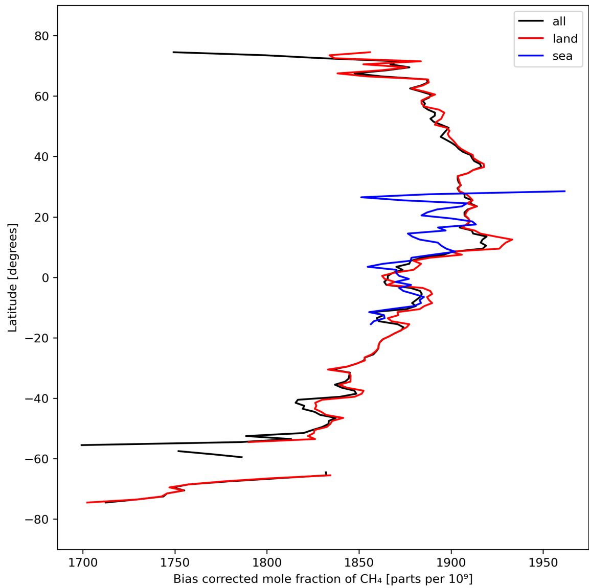
Figure 14: Zonal average of “Bias corrected mole fraction of CH 4 ” for 2023-09-24 to 2023-09-26.
