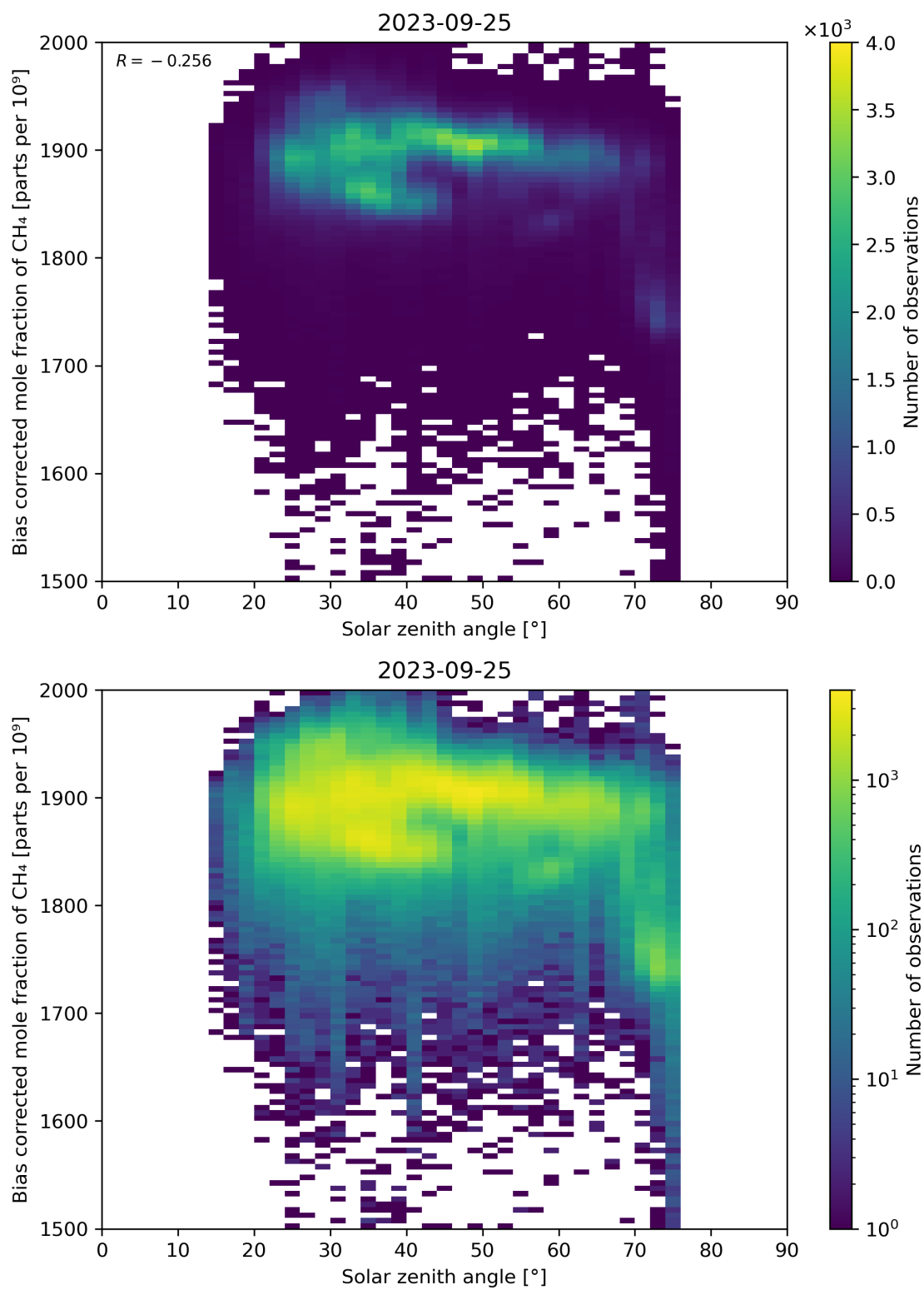
Figure 100: Scatter density plot of “Solar zenith angle” against “Bias corrected mole fraction of CH 4 ” for 2023-09-24 to 2023-09-26.
