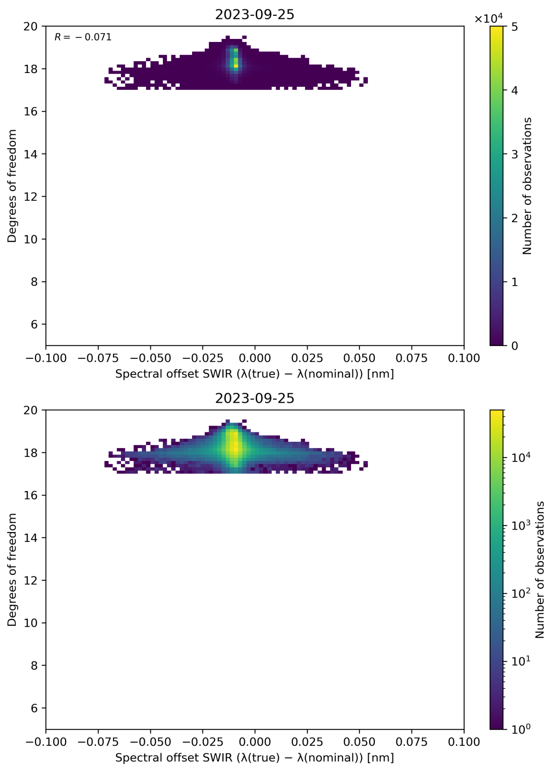
Figure 119: Scatter density plot of “Spectral offset SWIR ( \lambda(\text{true}) - \lambda(\text{nominal}) )” against “Degrees of freedom” for 2023-09-24 to 2023-09-26.
