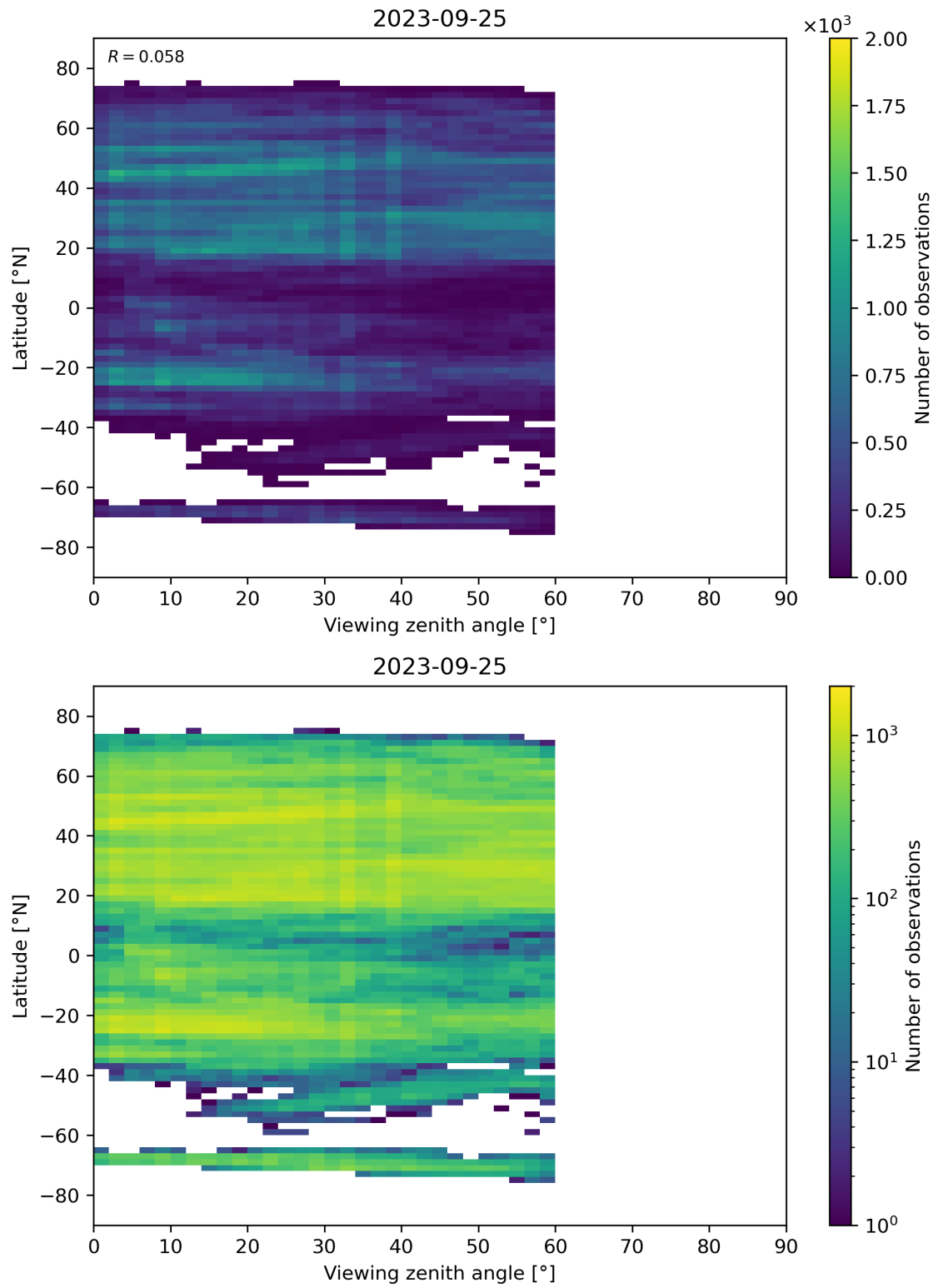
Figure 109: Scatter density plot of “Viewing zenith angle” against “Latitude” for 2023-09-24 to 2023-09-26.
