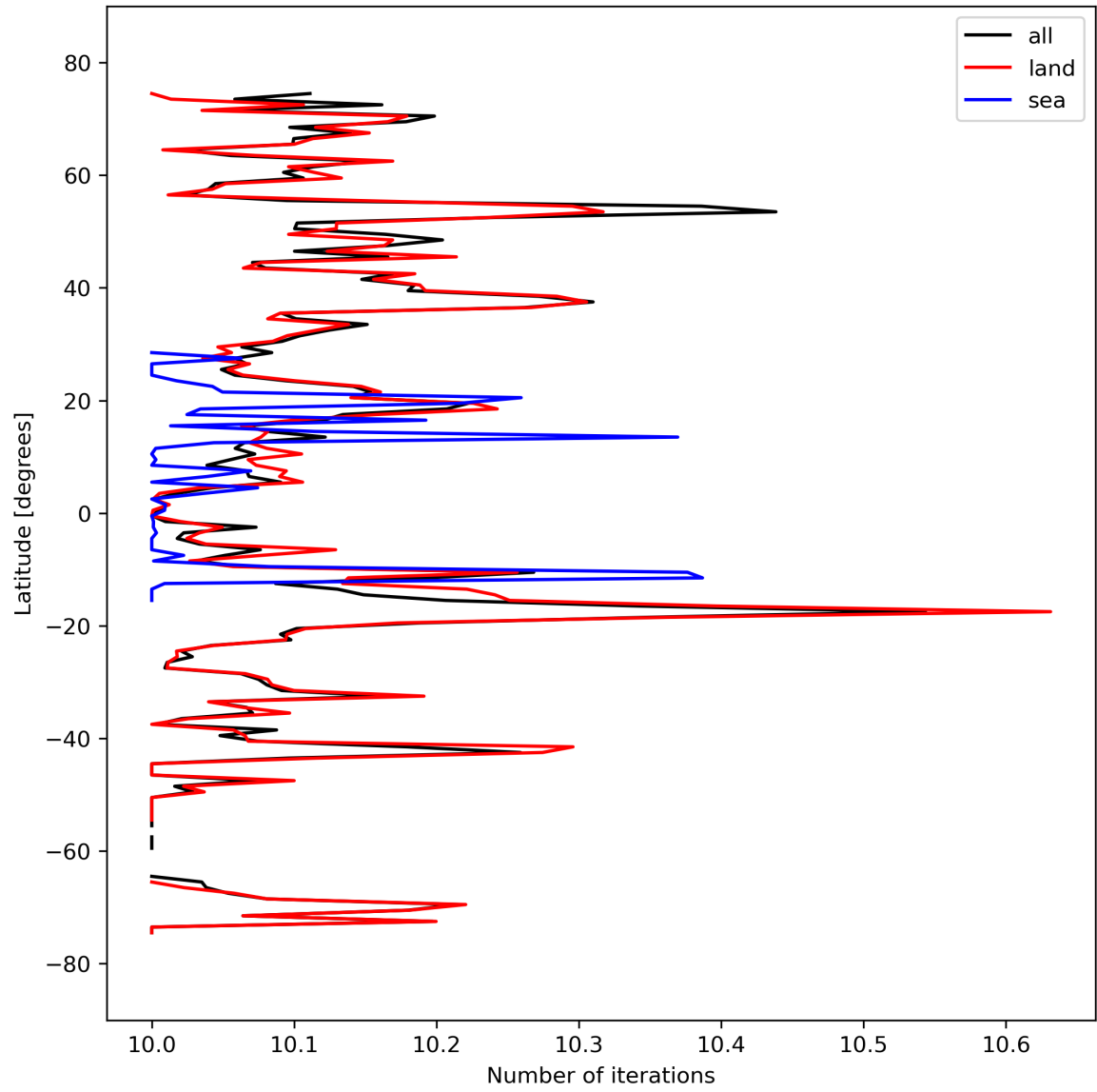
Figure 20: Zonal average of “Number of iterations” for 2023-09-24 to 2023-09-26.
