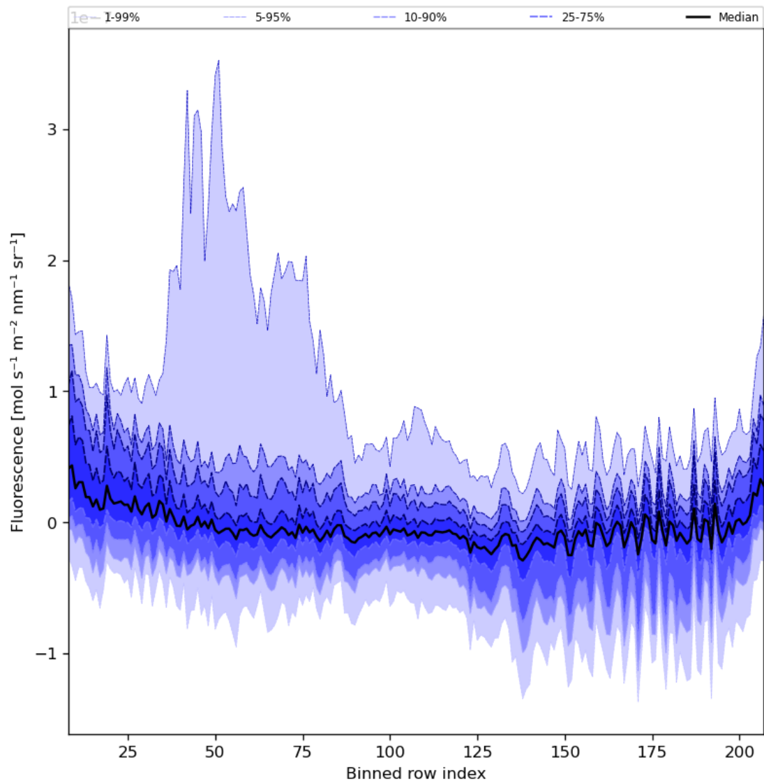
Figure 43: Along track statistics of “Fluorescence” for 2023-09-24 to 2023-09-26
