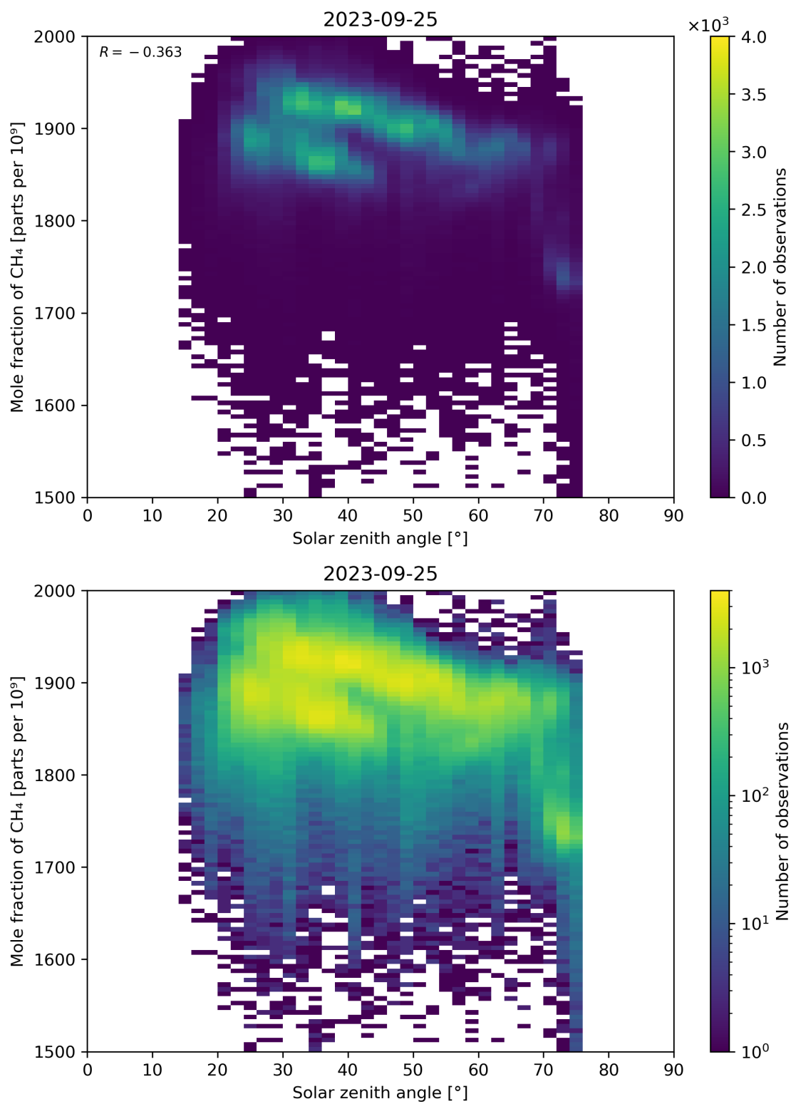
Figure 99: Scatter density plot of “Solar zenith angle” against “Mole fraction of CH 4 ” for 2023-09-24 to 2023-09-26.
