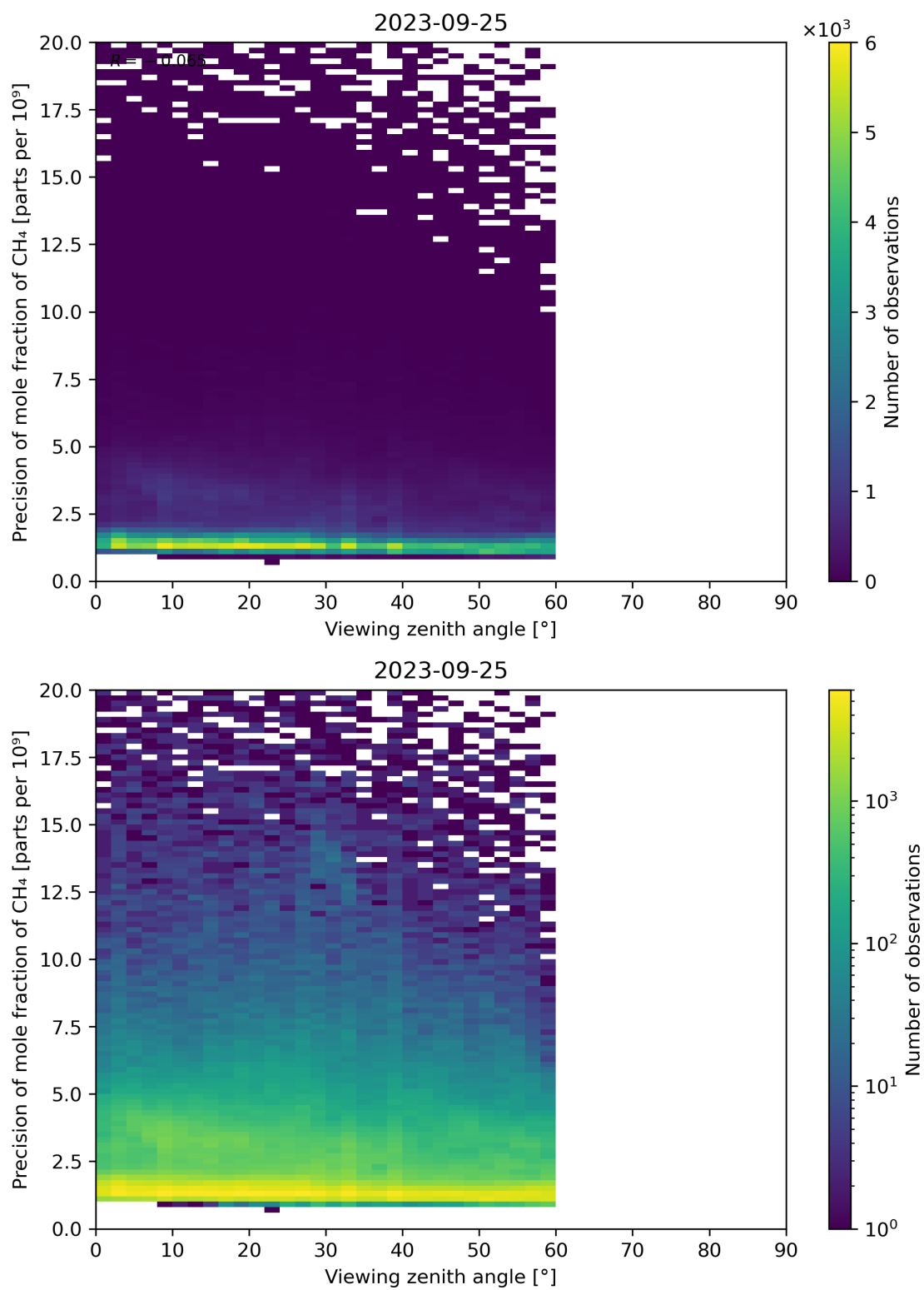
Figure 112: Scatter density plot of “Viewing zenith angle” against “Precision of mole fraction of CH 4 ” for 2023-09-24 to 2023-09-26.
