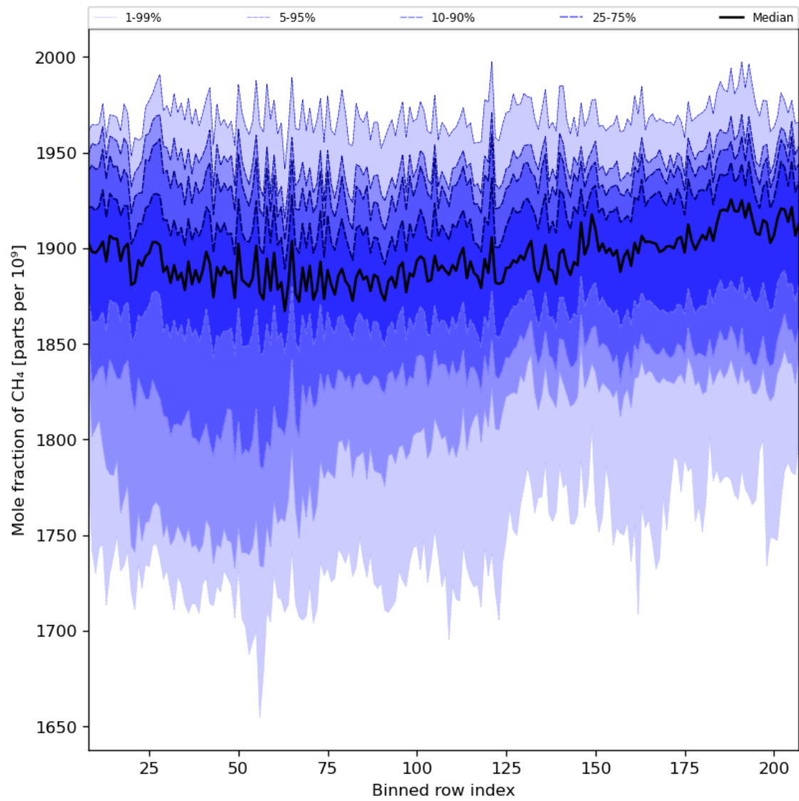
Figure 34: Along track statistics of “Mole fraction of CH 4 ” for 2023-09-24 to 2023-09-26
