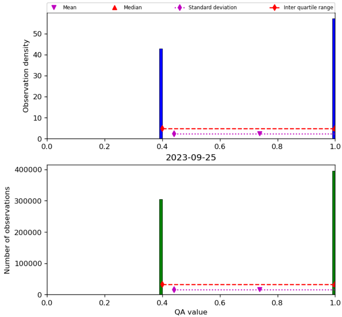
Figure 22: Histogram of “QA value” for 2023-09-24 to 2023-09-26
