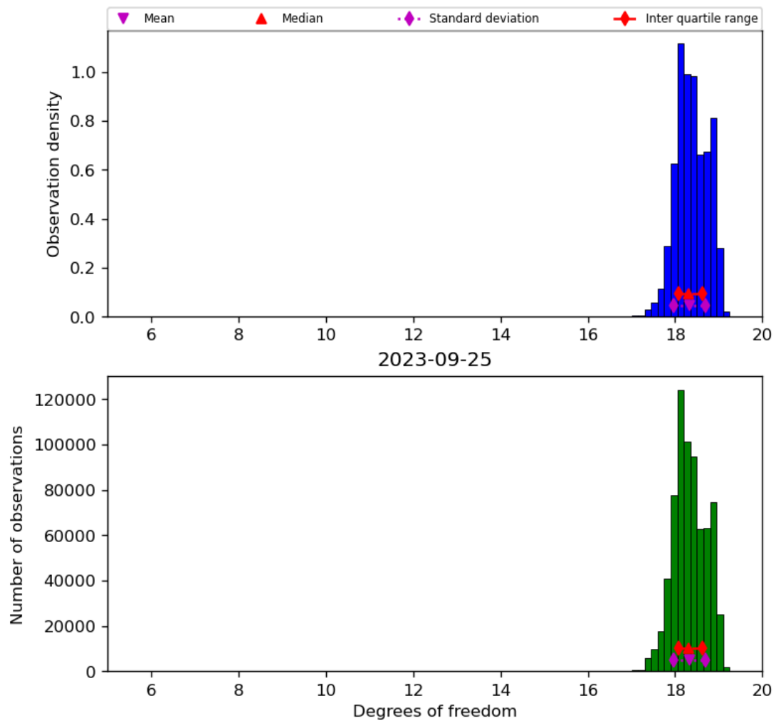
Figure 30: Histogram of “Degrees of freedom” for 2023-09-24 to 2023-09-26
