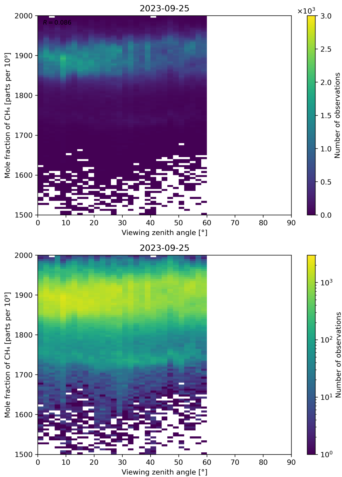
Figure 110: Scatter density plot of “Viewing zenith angle” against “Mole fraction of CH 4 ” for 2023-09-24 to 2023-09-26.
