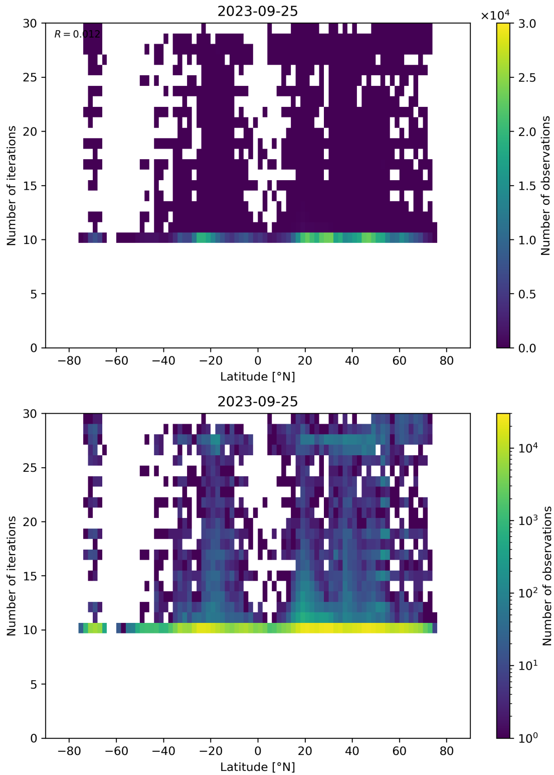
Figure 60: Scatter density plot of “Latitude” against “Number of iterations” for 2023-09-24 to 2023-09-26.
