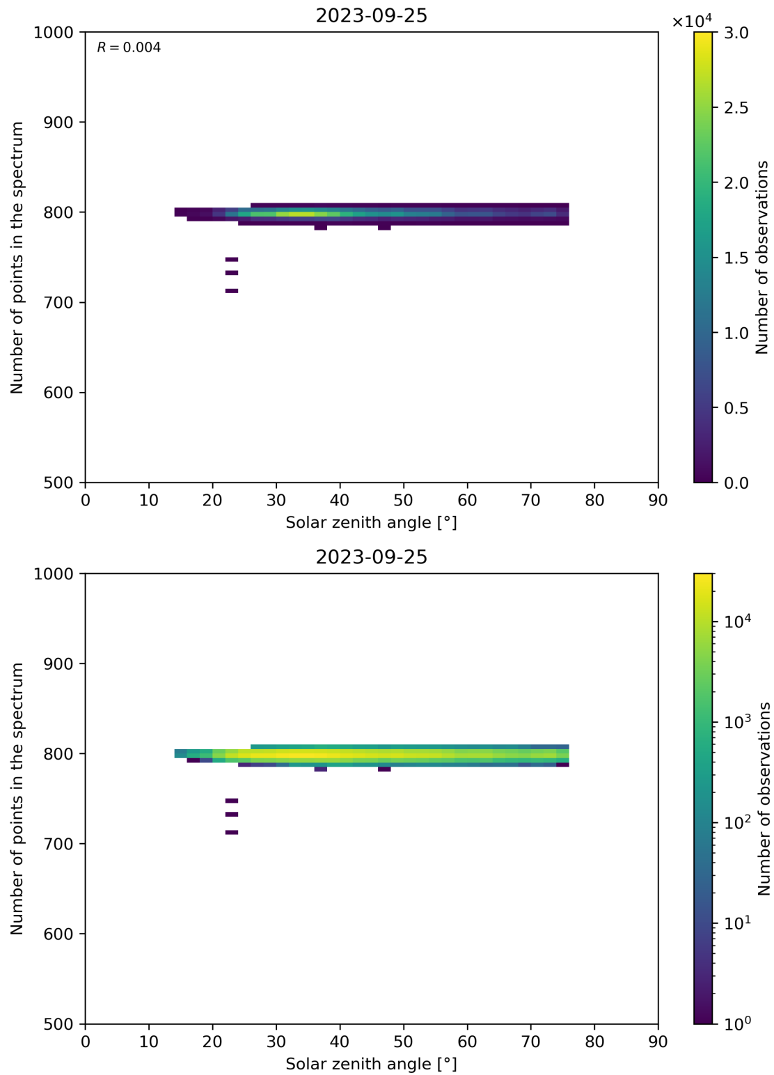
Figure 103: Scatter density plot of “Solar zenith angle” against “Number of points in the spectrum” for 2023-09-24 to 2023-09-26.
