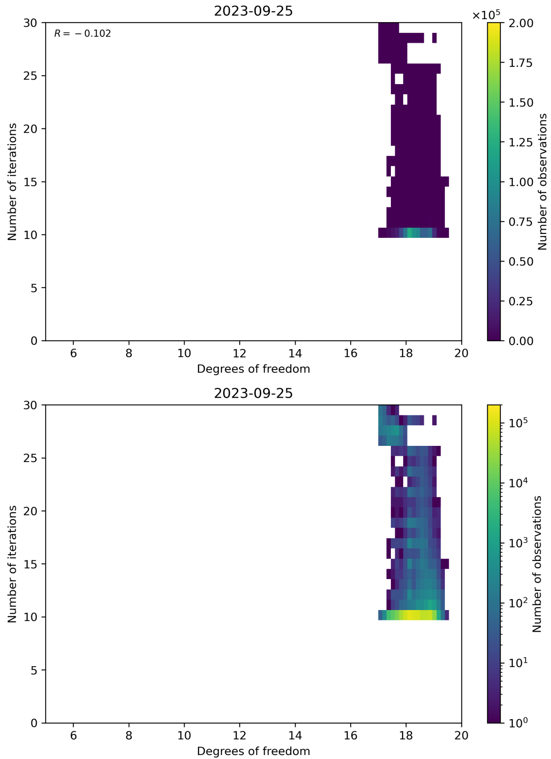
Figure 52: Scatter density plot of “Degrees of freedom” against “Number of iterations” for 2023-09-24 to 2023-09-26.
