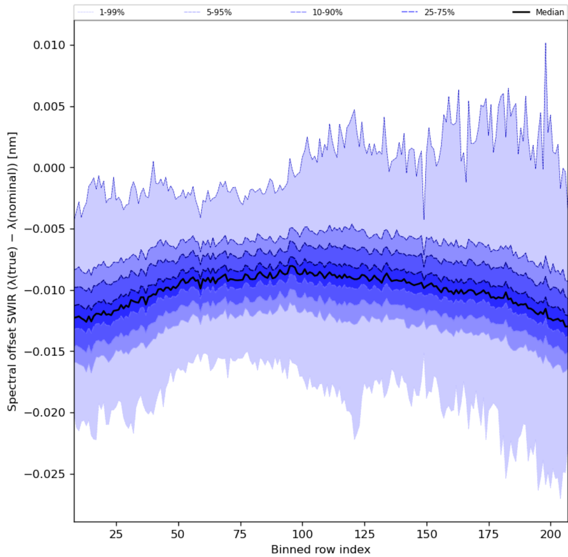
Figure 38: Along track statistics of “Spectral offset SWIR ( \lambda(\text{true}) - \lambda(\text{nominal}) )” for 2023-09-24 to 2023-09-26
