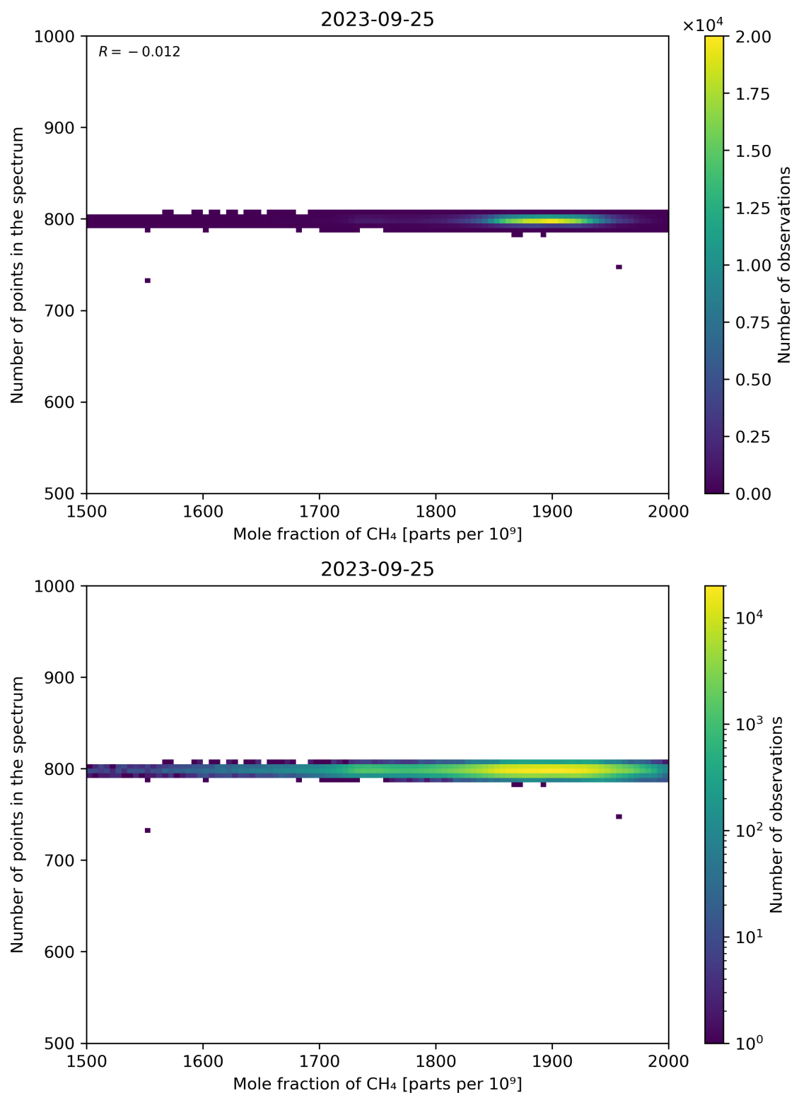
Figure 77: Scatter density plot of “Mole fraction of CH 4 ” against “Number of points in the spectrum” for 2023-09-24 to 2023-09-26.
