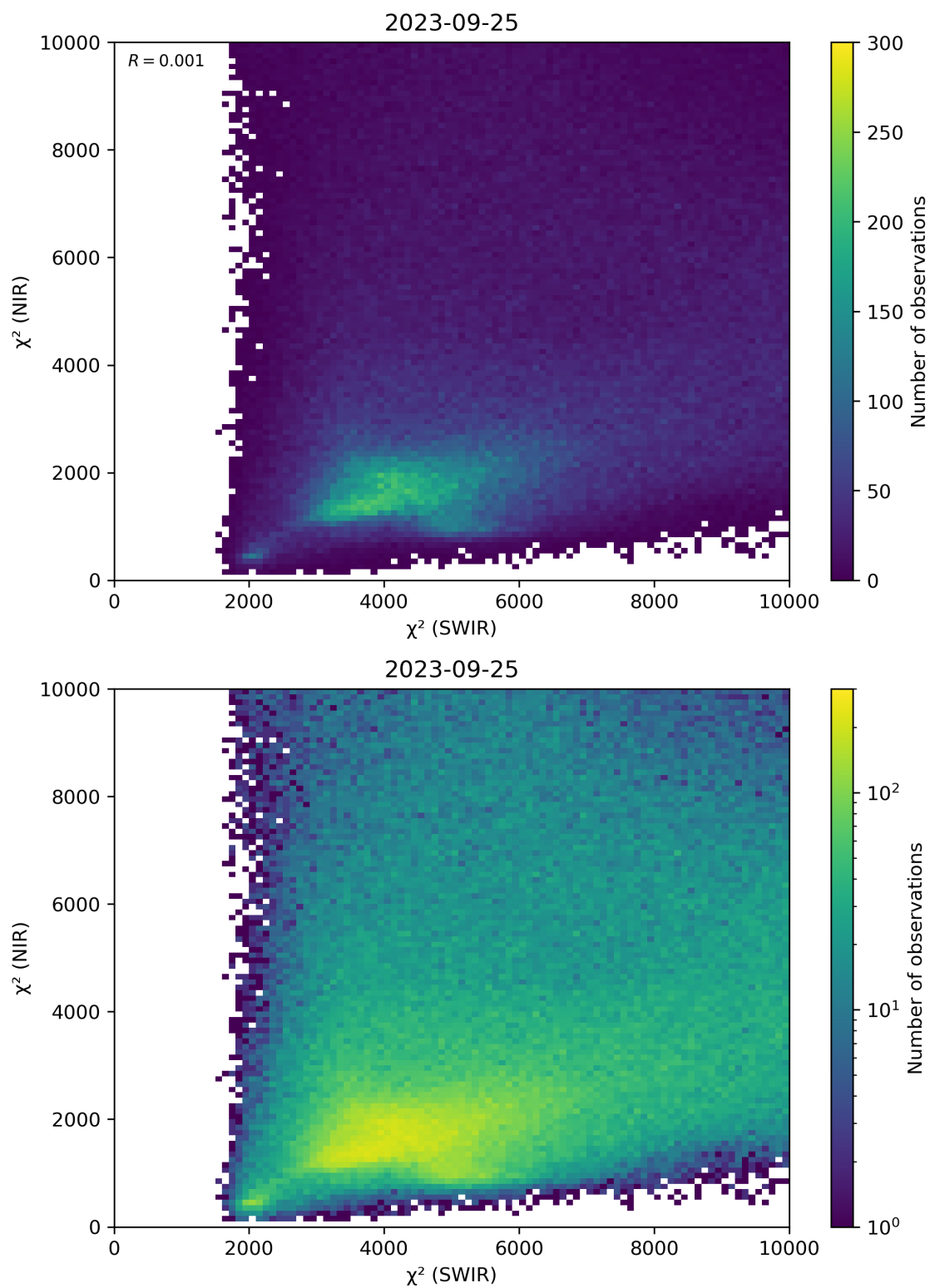
Figure 47: Scatter density plot of “ \chi^2 (SWIR)” against “ \chi^2 (NIR)” for 2023-09-24 to 2023-09-26.
