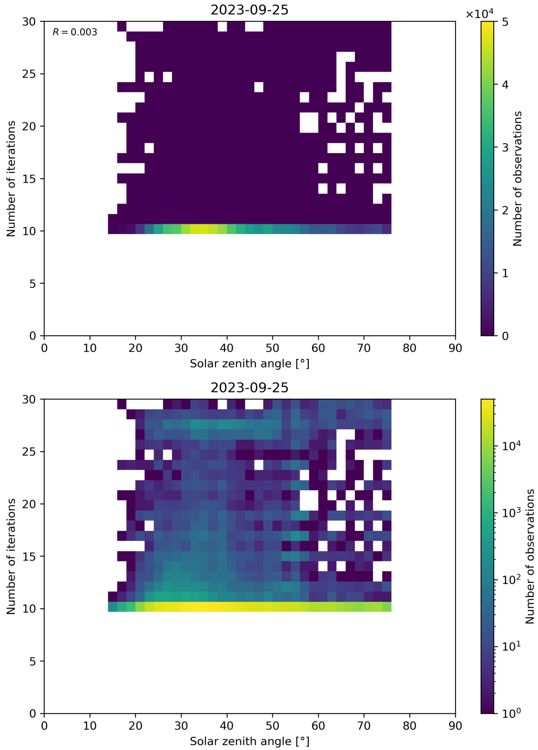
Figure 102: Scatter density plot of “Solar zenith angle” against “Number of iterations” for 2023-09-24 to 2023-09-26.
