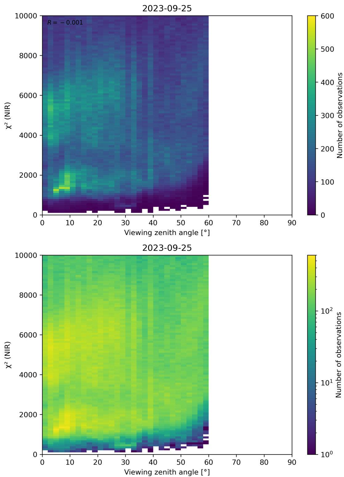
Figure 105: Scatter density plot of “Viewing zenith angle” against “ \chi^2 (NIR)” for 2023-09-24 to 2023-09-26.
