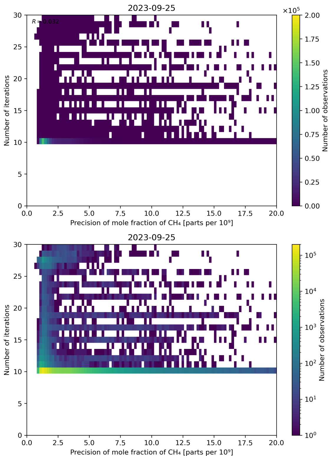
Figure 83: Scatter density plot of “Precision of mole fraction of CH 4 ” against “Number of iterations” for 2023-09-24 to 2023-09-26.
