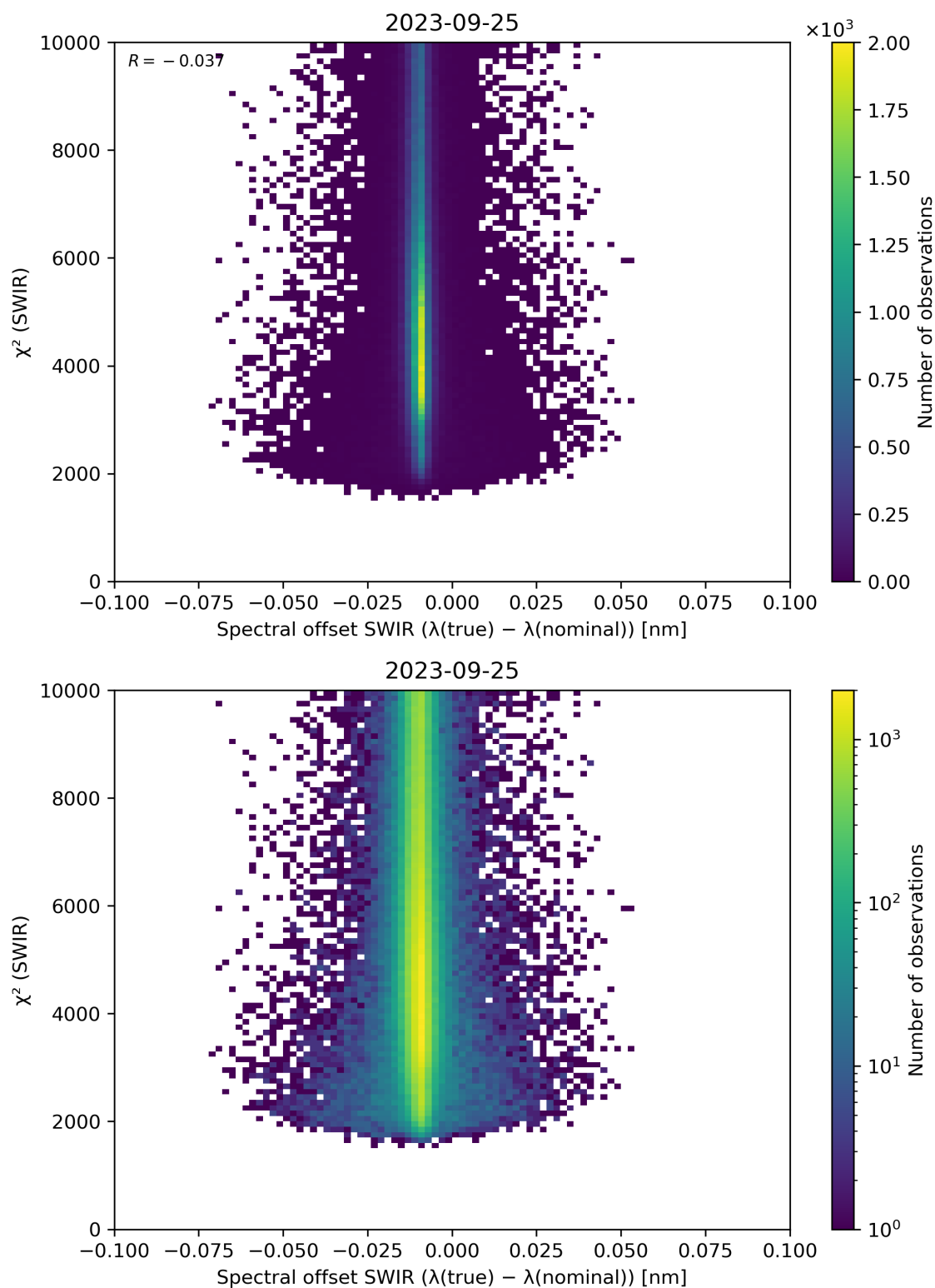
Figure 118: Scatter density plot of “Spectral offset SWIR ( \lambda(\text{true}) - \lambda(\text{nominal}) )” against “ \chi^2 (SWIR)” for 2023-09-24 to 2023-09-26.
