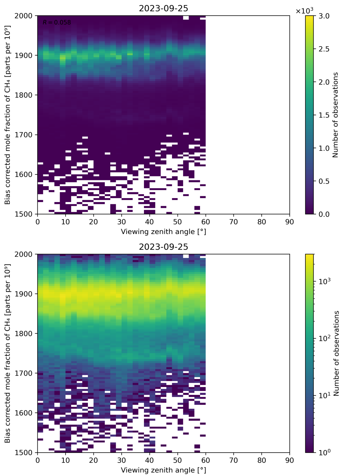
Figure 111: Scatter density plot of “Viewing zenith angle” against “Bias corrected mole fraction of CH 4 ” for 2023-09-24 to 2023-09-26.
