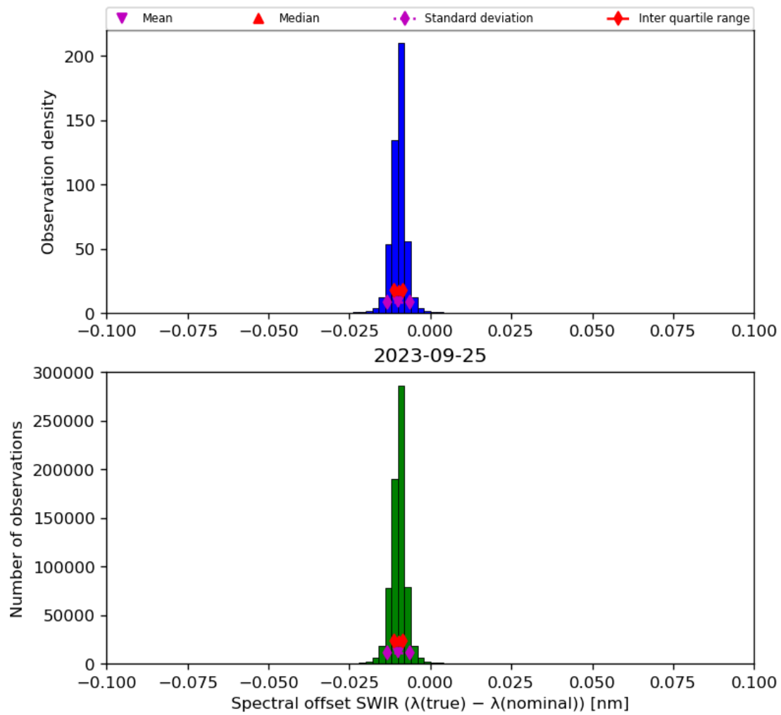
Figure 27: Histogram of “Spectral offset SWIR ( \lambda(\text{true}) - \lambda(\text{nominal}) )” for 2023-09-24 to 2023-09-26
