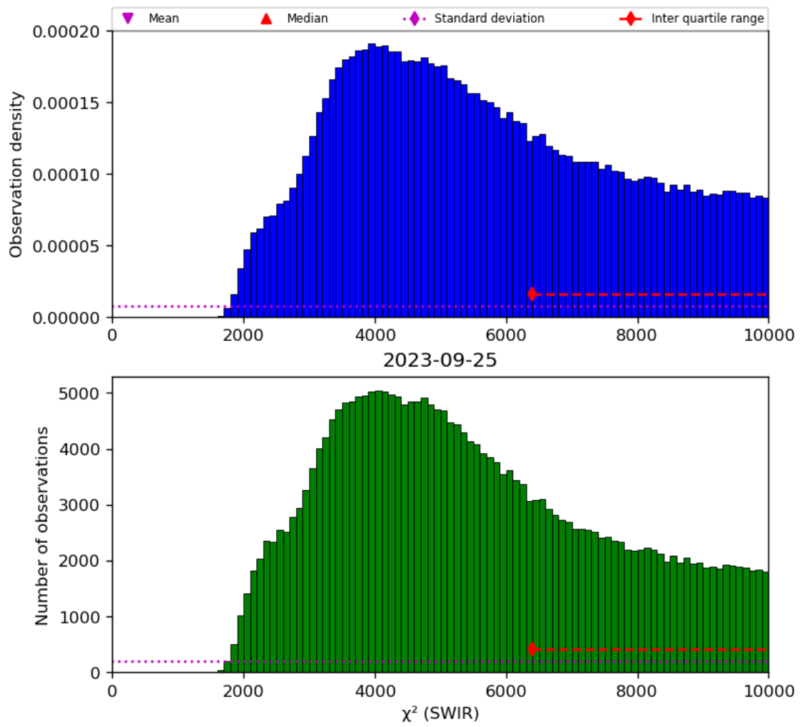
Figure 28: Histogram of “ \chi^2 (SWIR)” for 2023-09-24 to 2023-09-26
