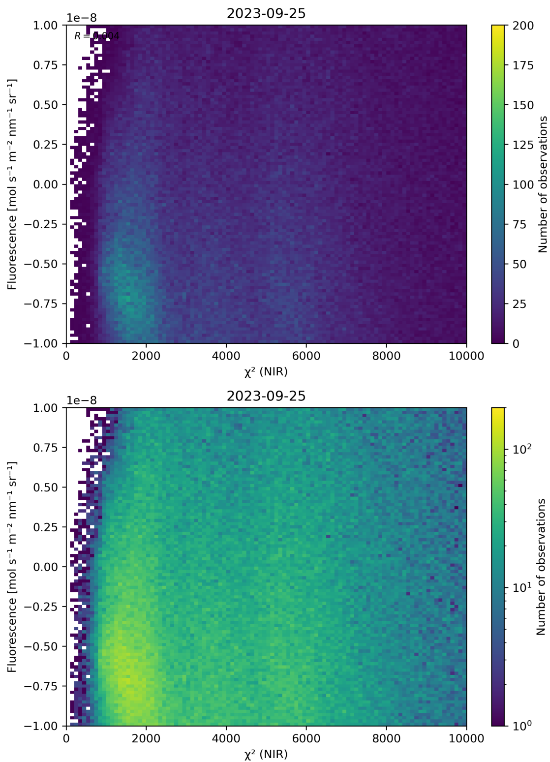
Figure 45: Scatter density plot of “ \chi^2 (NIR)” against “Fluorescence” for 2023-09-24 to 2023-09-26.
