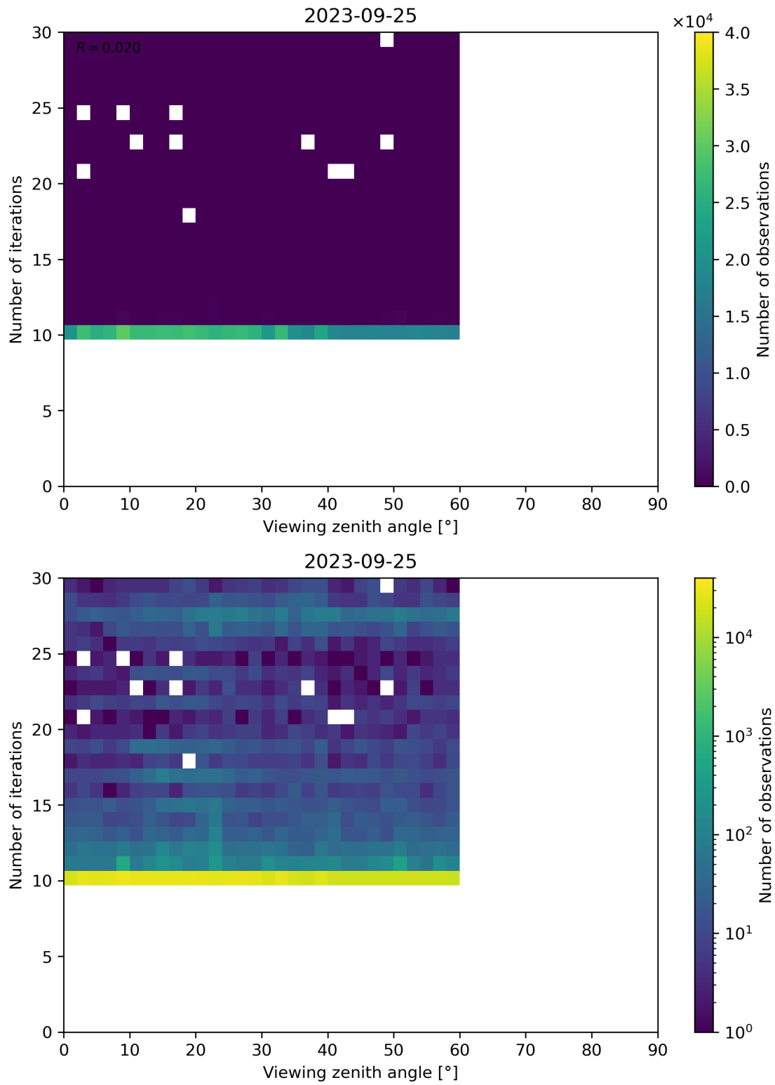
Figure 113: Scatter density plot of “Viewing zenith angle” against “Number of iterations” for 2023-09-24 to 2023-09-26.
