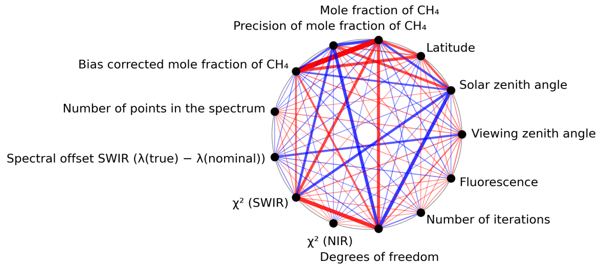
Figure 1: Map of correlation graph for 2023-09-24 to 2023-09-26.
