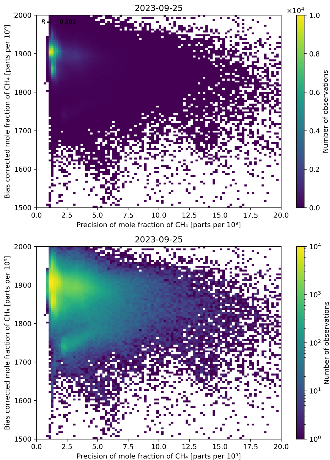
Figure 82: Scatter density plot of “Precision of mole fraction of CH 4 ” against “Bias corrected mole fraction of CH 4 ” for 2023-09-24 to 2023-09-26.
