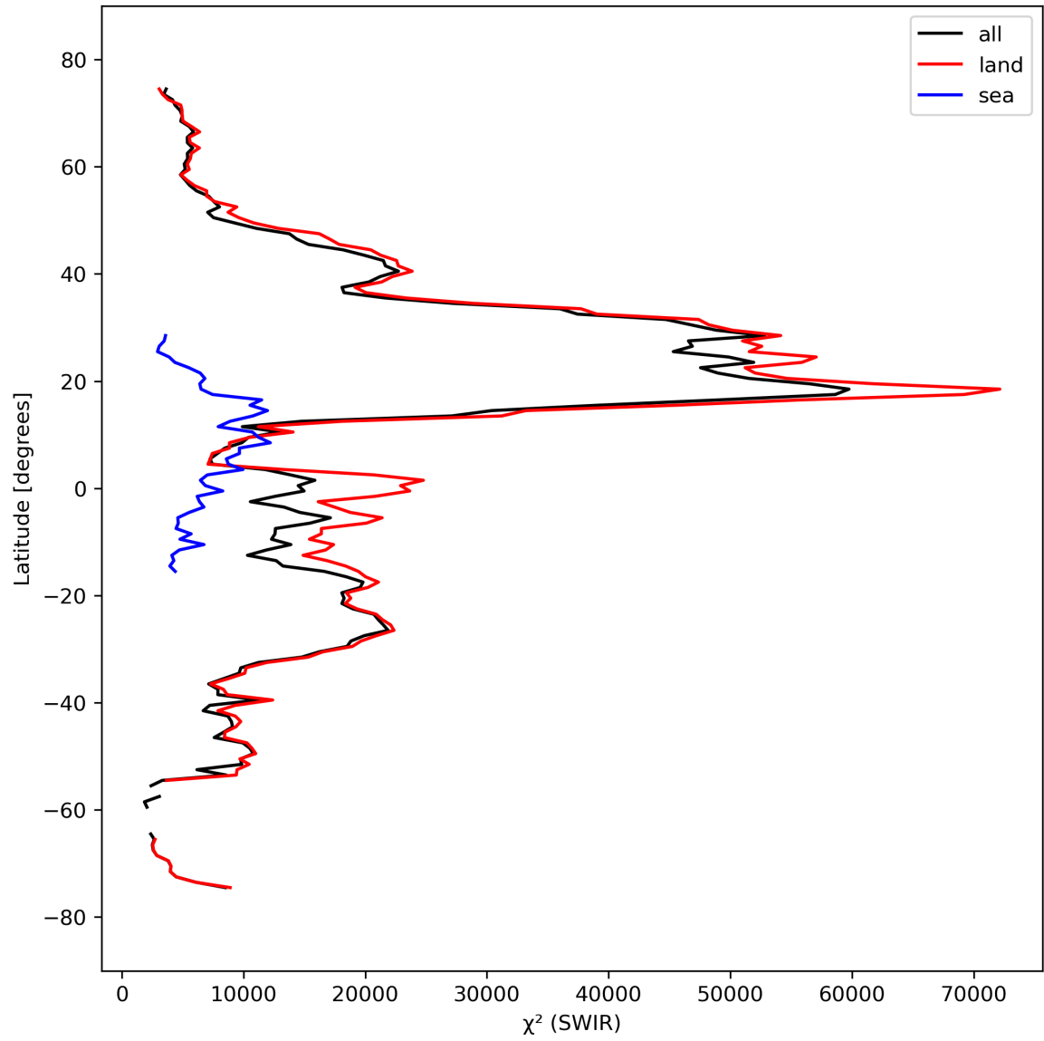
Figure 17: Zonal average of “ \chi^2 (SWIR)” for 2023-09-24 to 2023-09-26.
