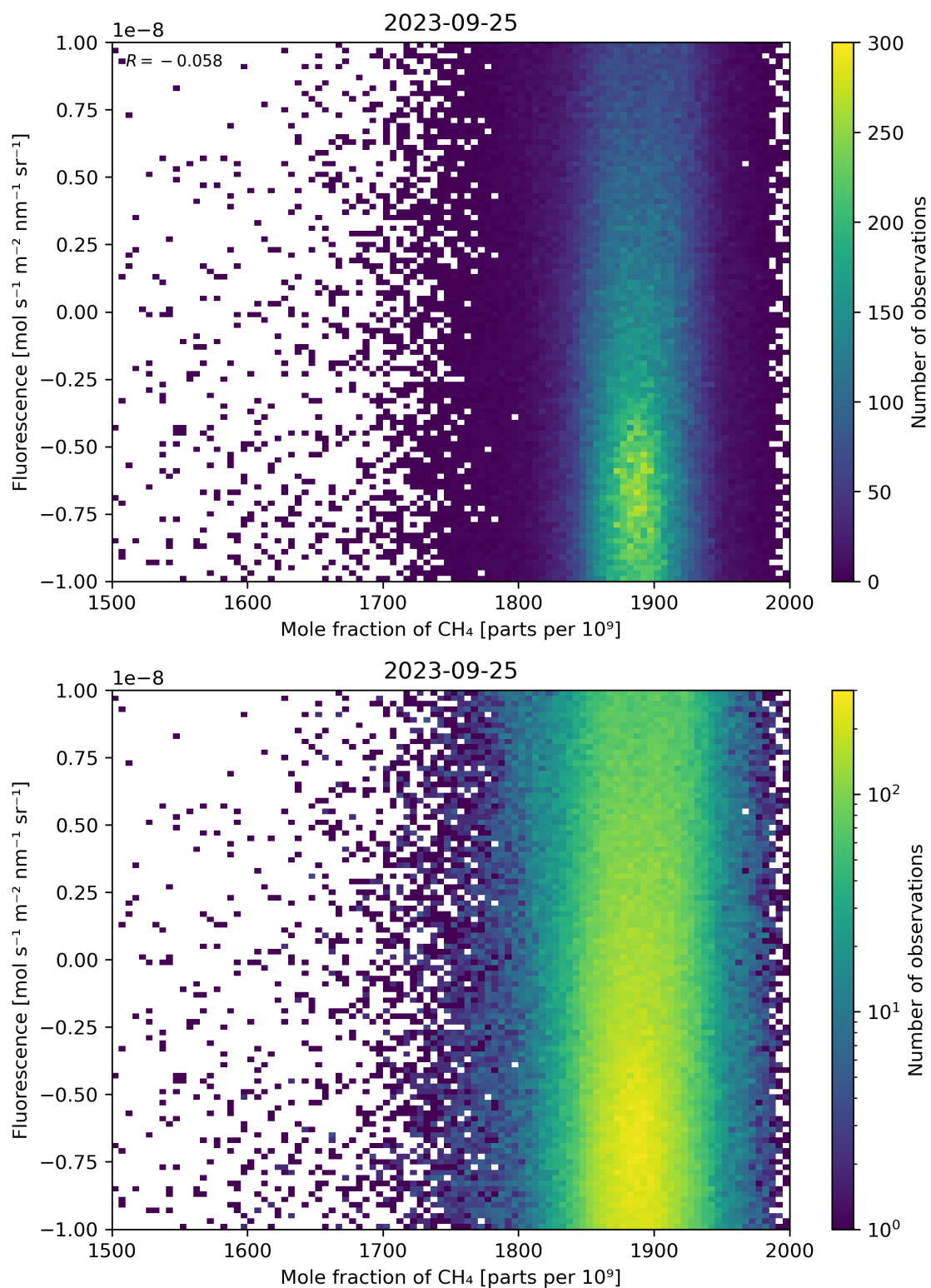
Figure 73: Scatter density plot of “Mole fraction of \text{CH}_4 ” against “Fluorescence” for 2023-09-24 to 2023-09-26.
