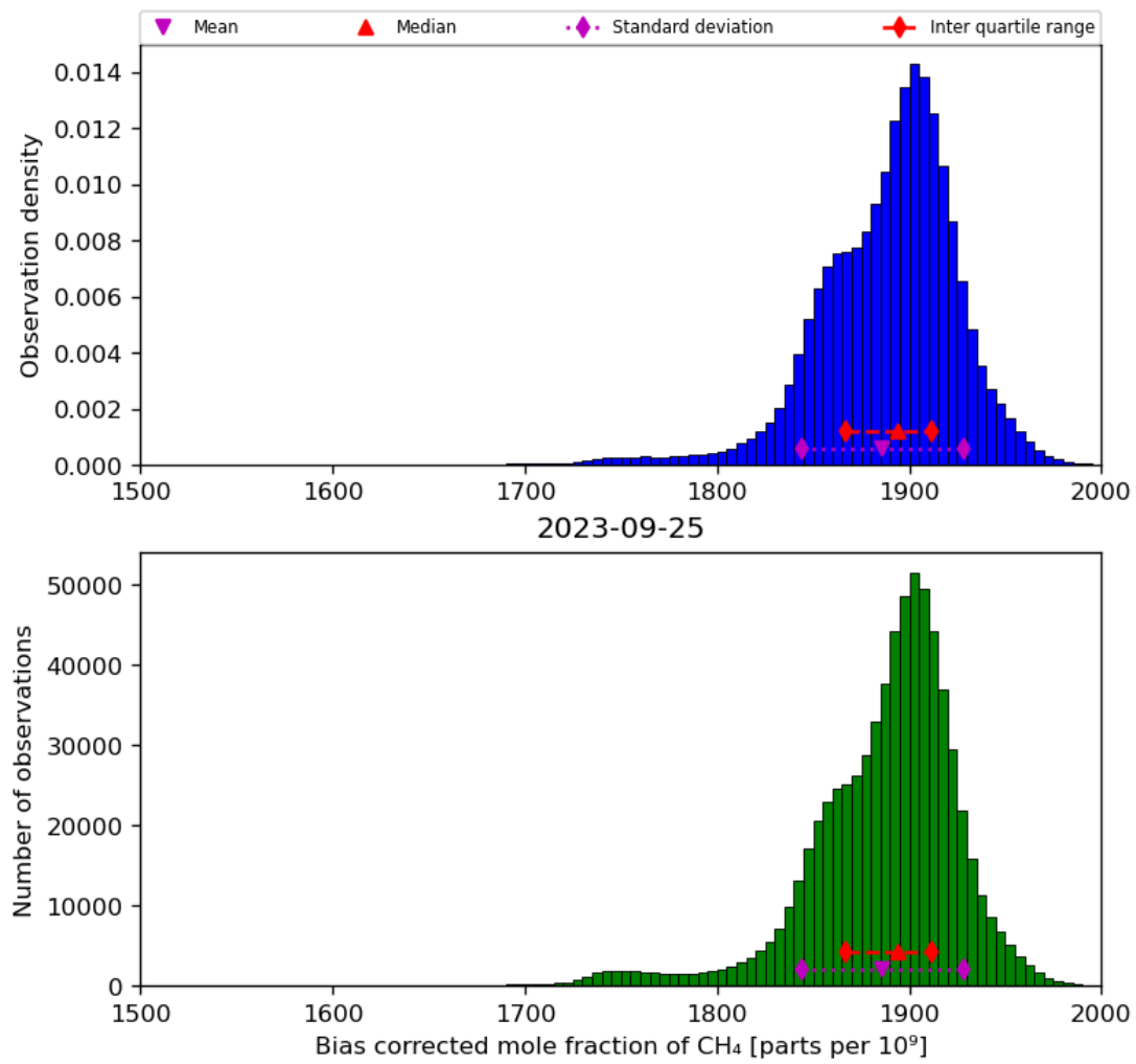
Figure 25: Histogram of “Bias corrected mole fraction of CH 4 ” for 2023-09-24 to 2023-09-26
