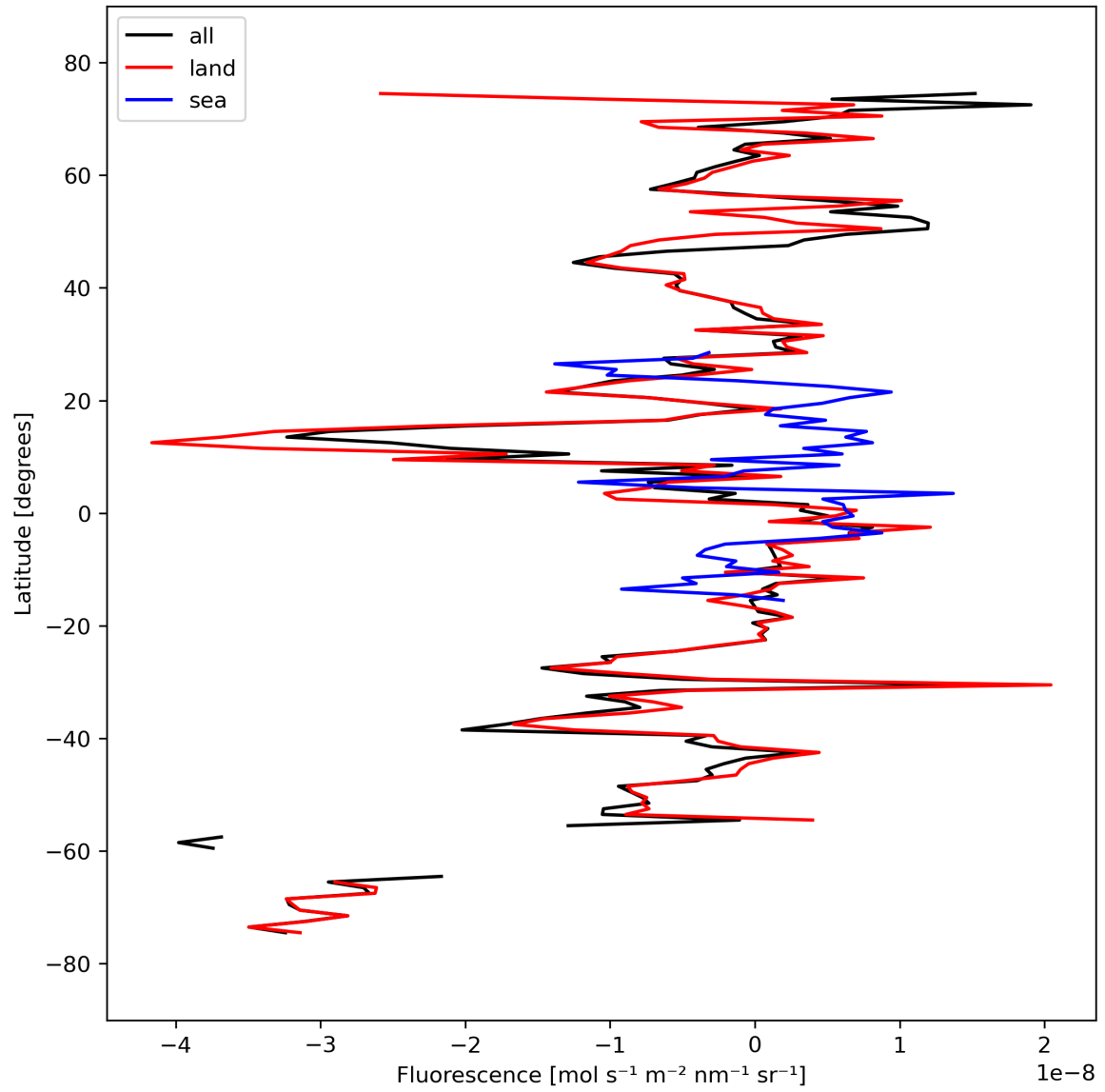
Figure 21: Zonal average of “Fluorescence” for 2023-09-24 to 2023-09-26.
