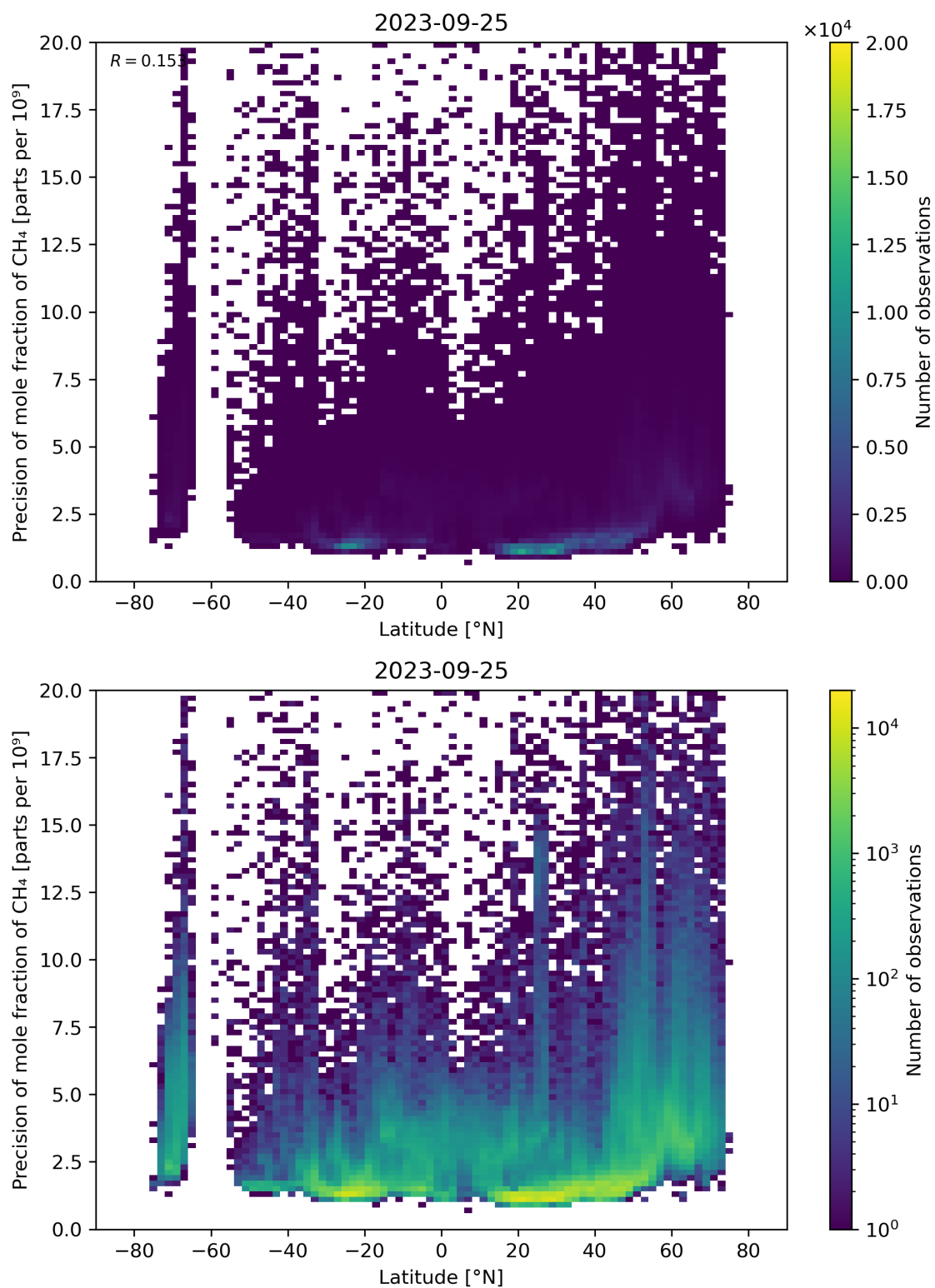
Figure 59: Scatter density plot of “Latitude” against “Precision of mole fraction of CH 4 ” for 2023-09-24 to 2023-09-26.
