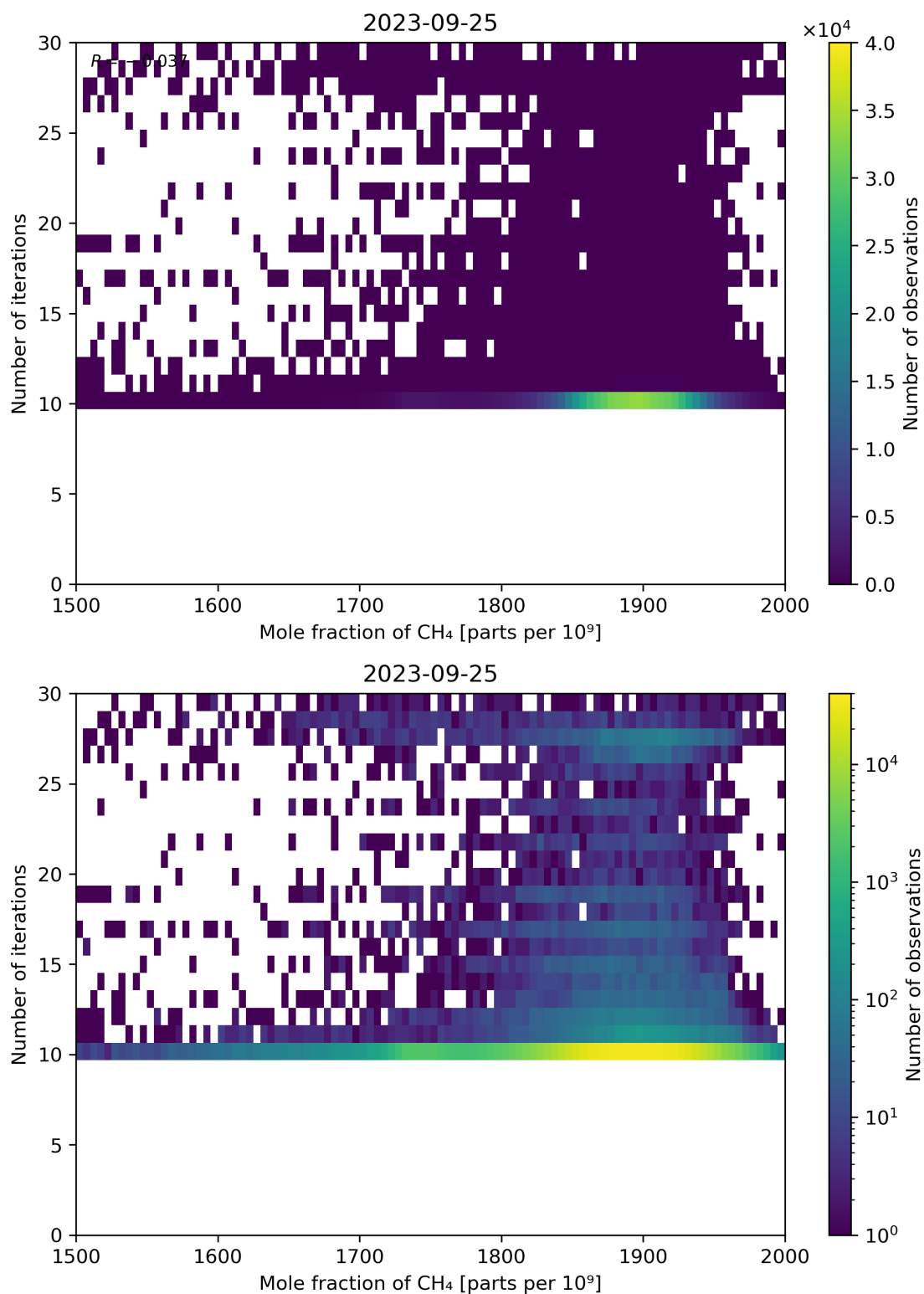
Figure 76: Scatter density plot of “Mole fraction of CH 4 ” against “Number of iterations” for 2023-09-24 to 2023-09-26.
