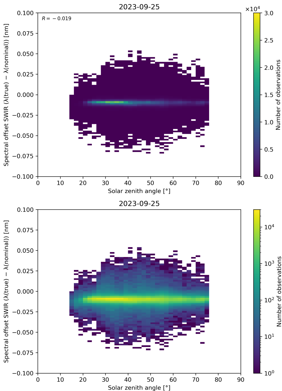
Figure 104: Scatter density plot of “Solar zenith angle” against “Spectral offset SWIR ( \lambda(\text{true}) - \lambda(\text{nominal}) )” for 2023-09-24 to 2023-09-26.
