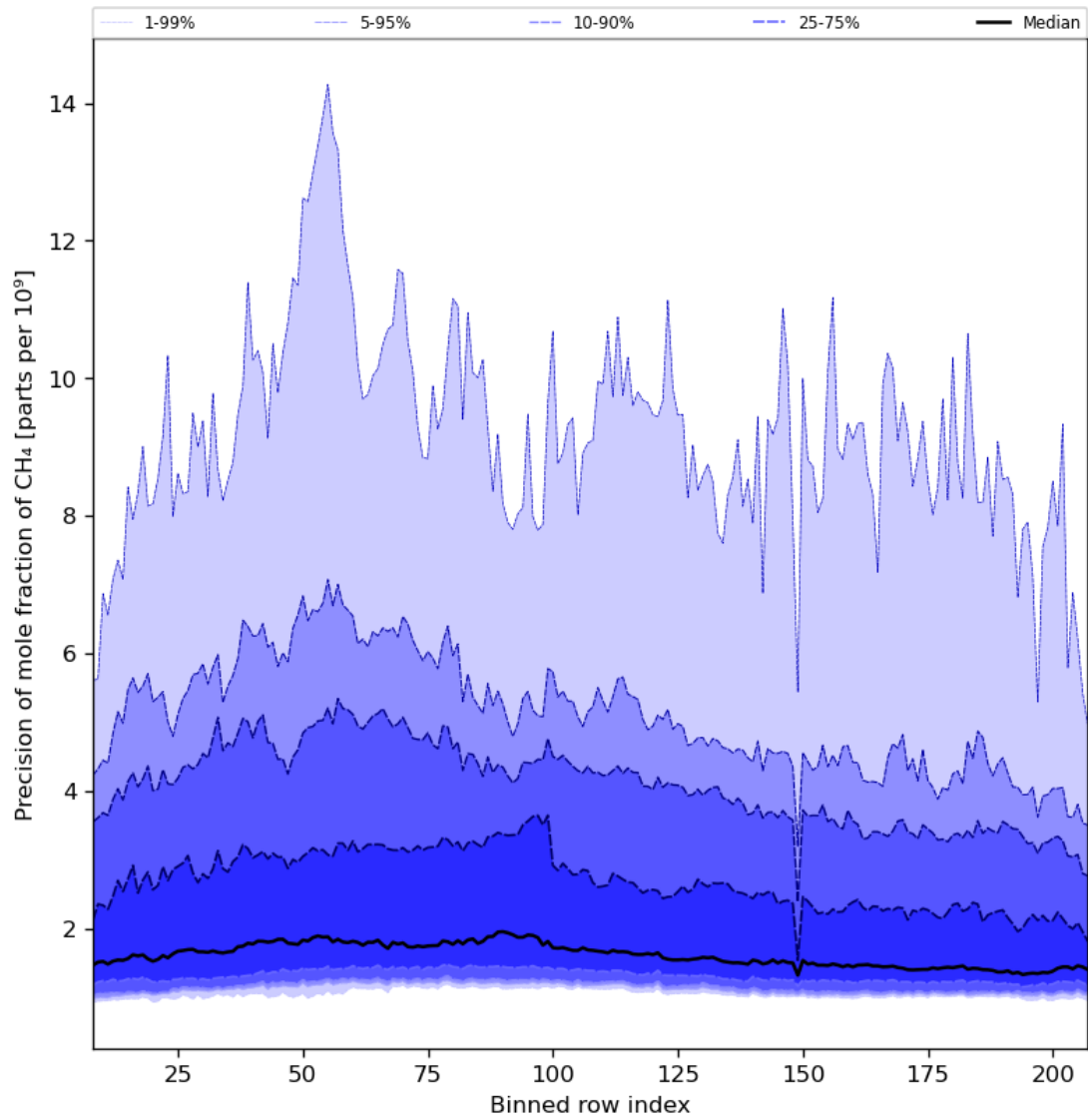
Figure 35: Along track statistics of “Precision of mole fraction of CH 4 ” for 2023-09-24 to 2023-09-26
