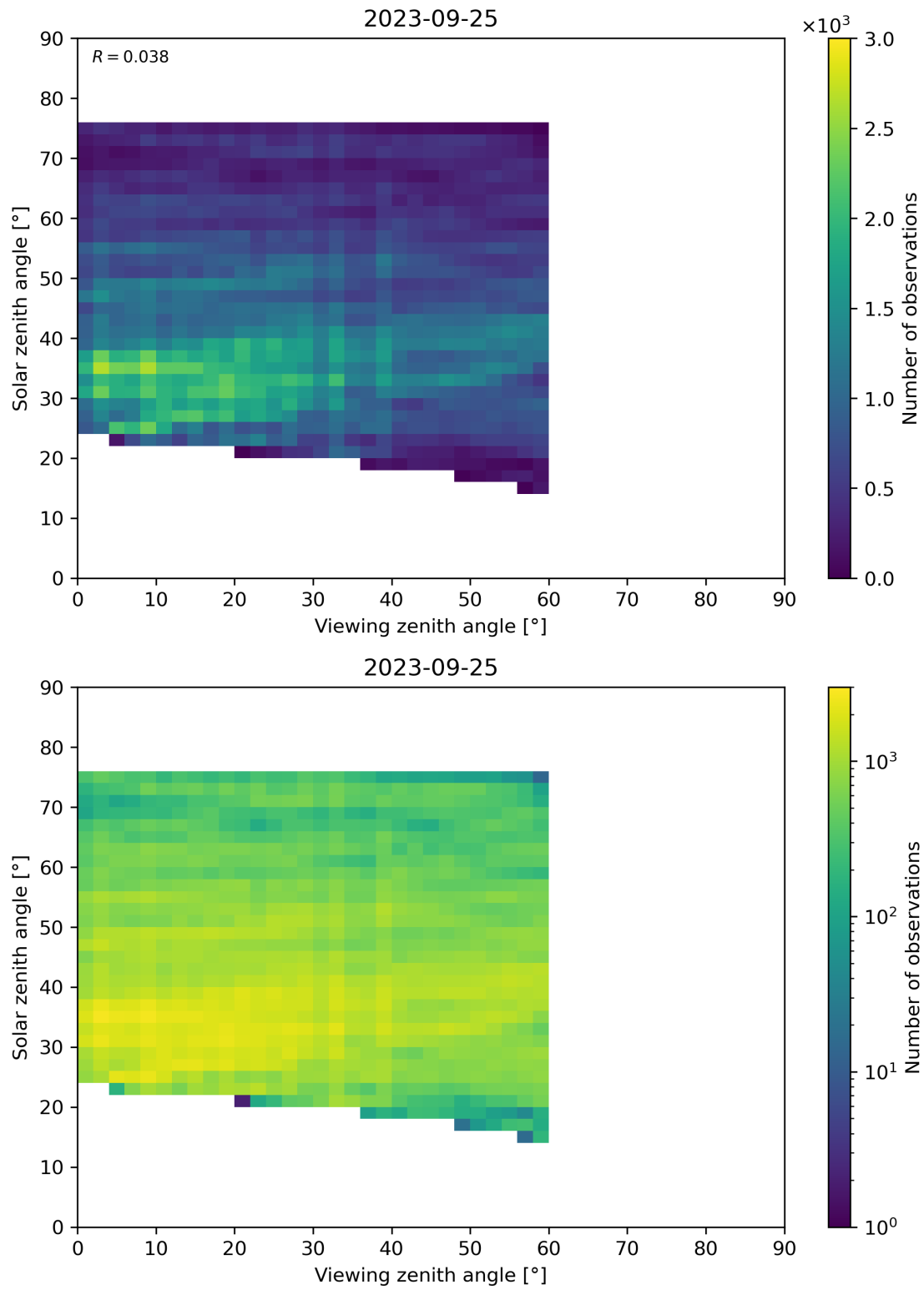
Figure 115: Scatter density plot of “Viewing zenith angle” against “Solar zenith angle” for 2023-09-24 to 2023-09-26.
