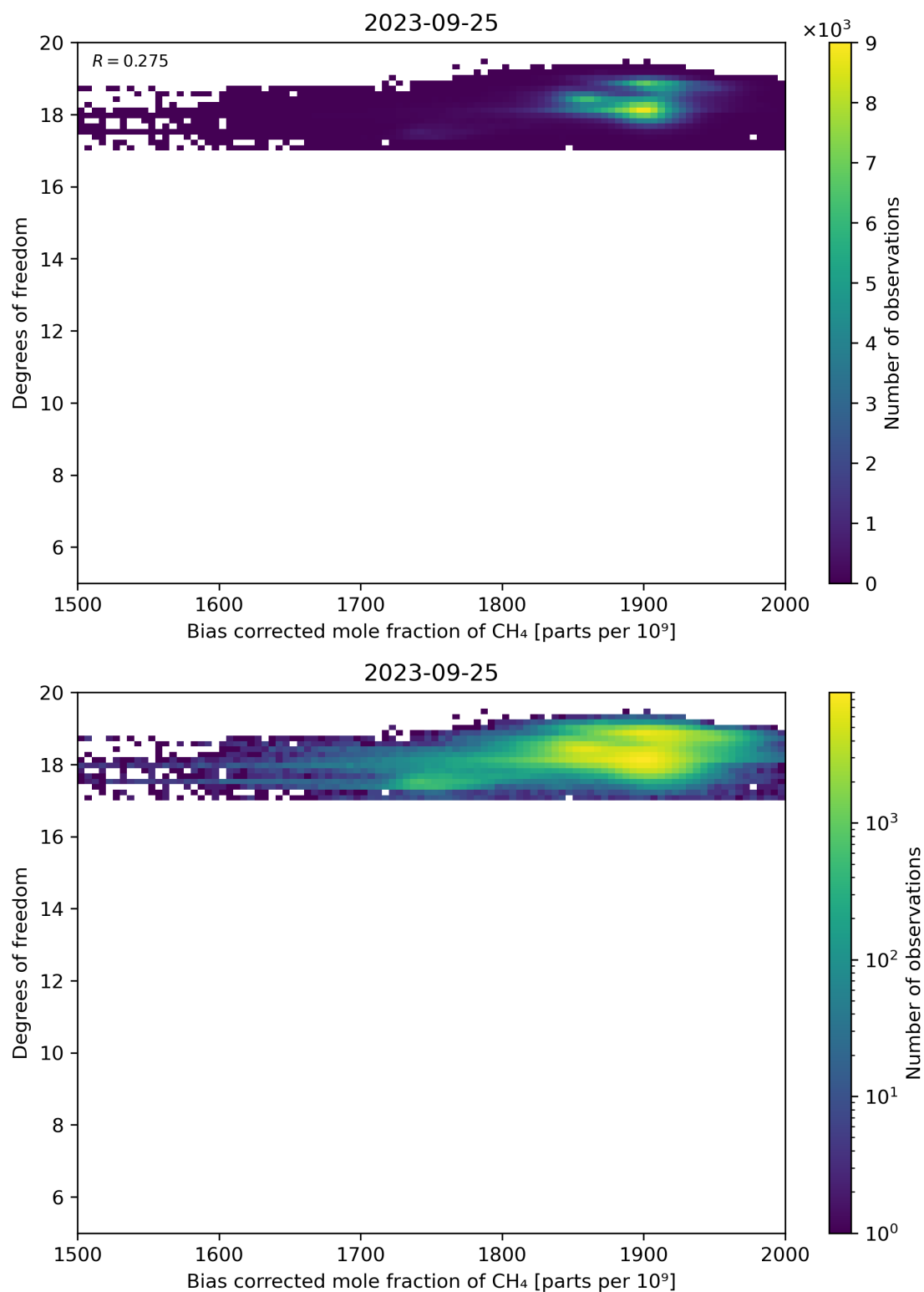
Figure 65: Scatter density plot of “Bias corrected mole fraction of CH 4 ” against “Degrees of freedom” for 2023-09-24 to 2023-09-26.
