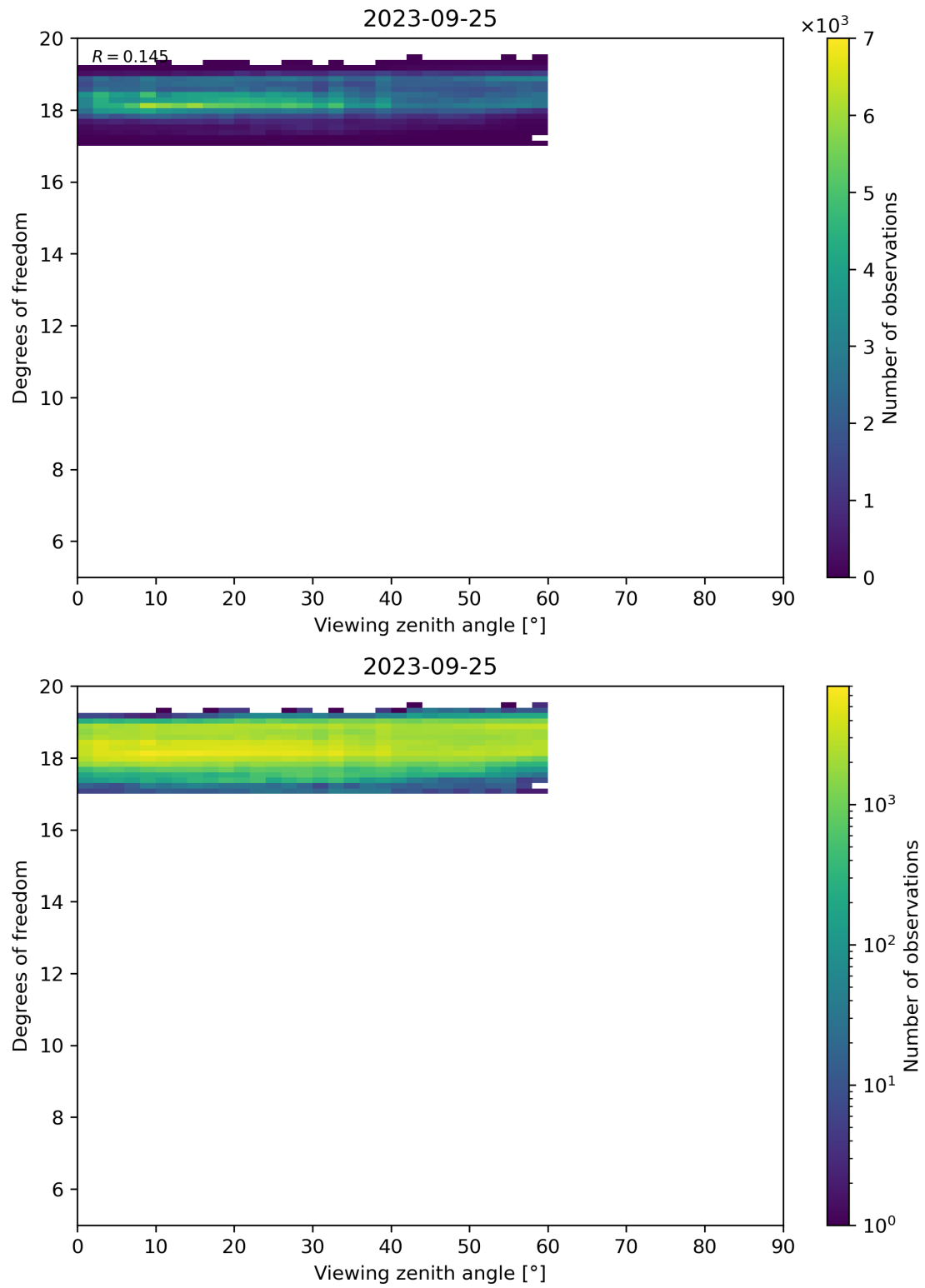
Figure 107: Scatter density plot of “Viewing zenith angle” against “Degrees of freedom” for 2023-09-24 to 2023-09-26.
