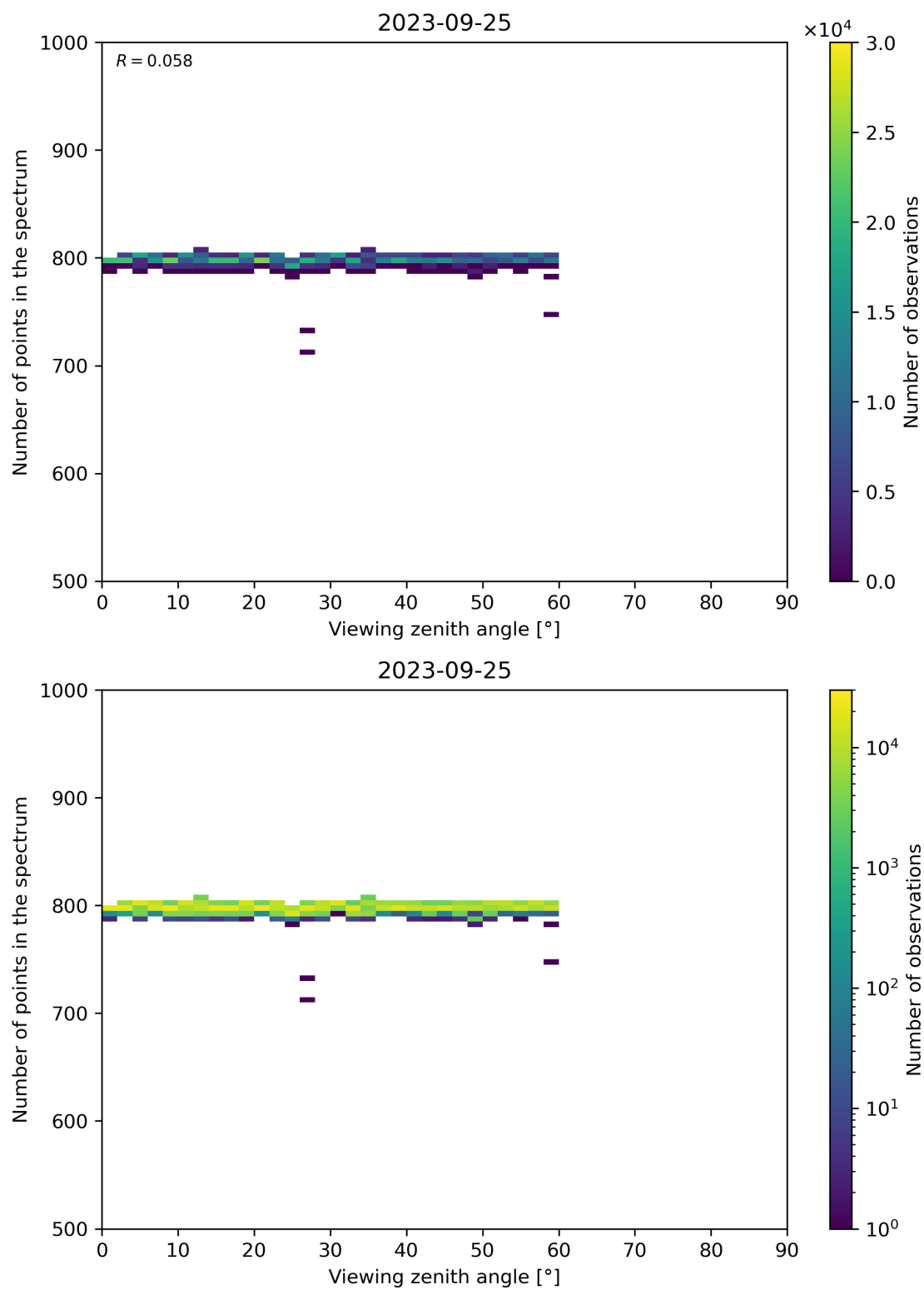
Figure 114: Scatter density plot of “Viewing zenith angle” against “Number of points in the spectrum” for 2023-09-24 to 2023-09-26.
