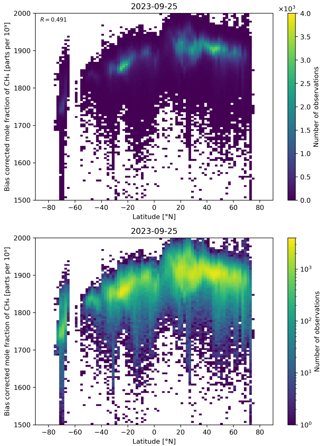
Figure 58: Scatter density plot of “Latitude” against “Bias corrected mole fraction of CH 4 ” for 2023-09-24 to 2023-09-26.
