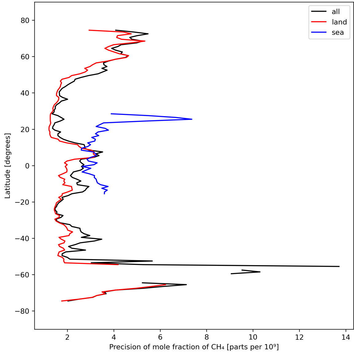
Figure 13: Zonal average of “Precision of mole fraction of CH 4 ” for 2023-09-24 to 2023-09-26.
