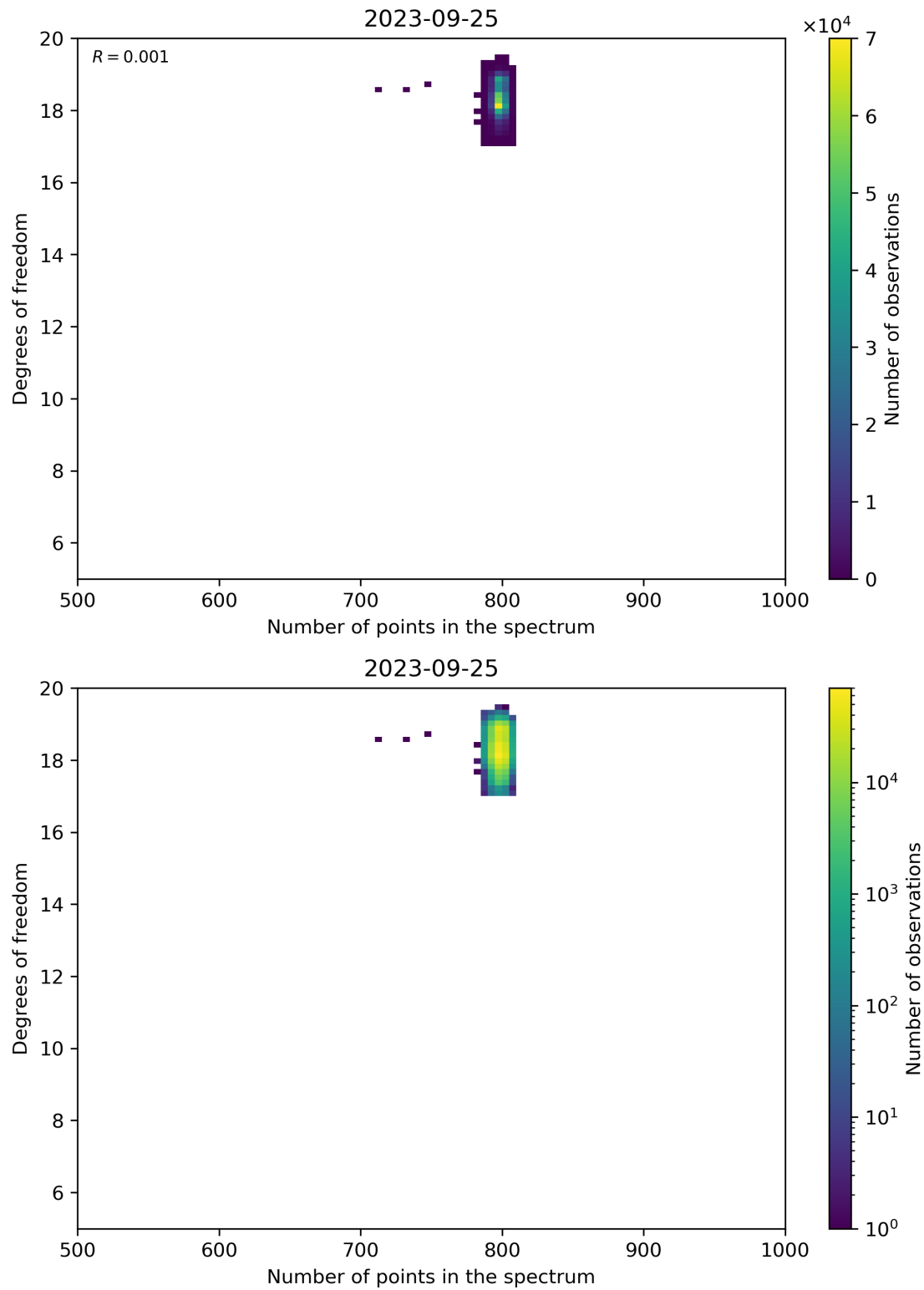
Figure 90: Scatter density plot of “Number of points in the spectrum” against “Degrees of freedom” for 2023-09-24 to 2023-09-26.
