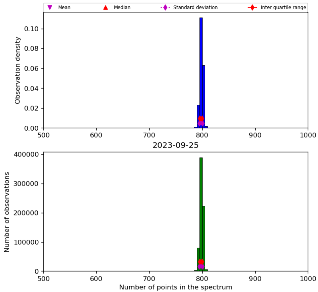
Figure 26: Histogram of “Number of points in the spectrum” for 2023-09-24 to 2023-09-26
