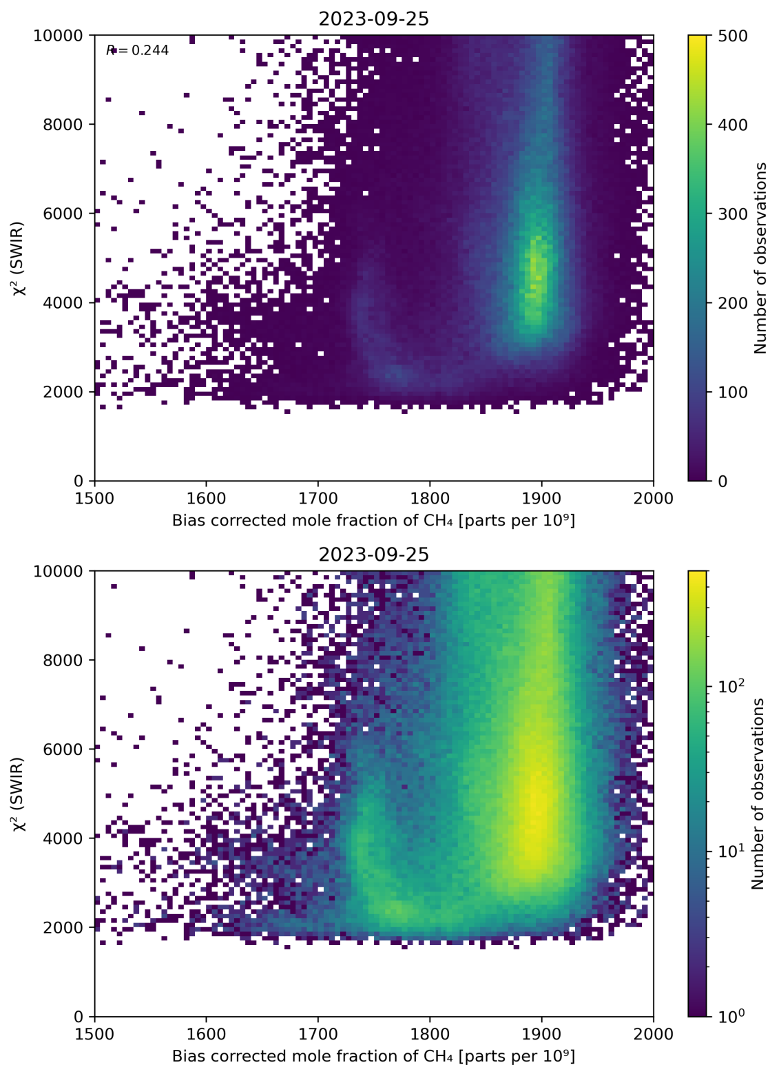
Figure 64: Scatter density plot of “Bias corrected mole fraction of CH 4 ” against “ \chi^2 (SWIR)” for 2023-09-24 to 2023-09-26.
