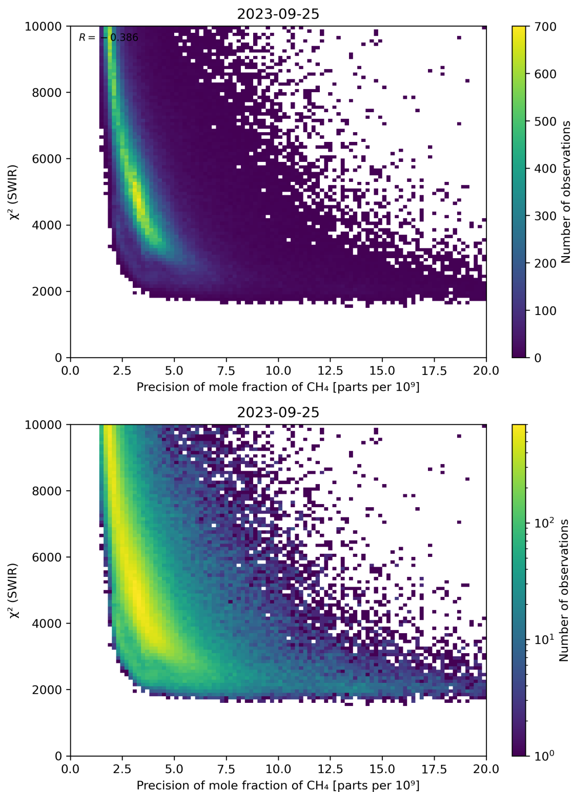
Figure 79: Scatter density plot of “Precision of mole fraction of CH 4 ” against “ \chi^2 (SWIR)” for 2023-09-24 to 2023-09-26.
