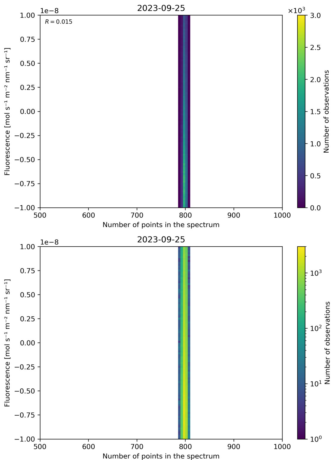
Figure 91: Scatter density plot of “Number of points in the spectrum” against “Fluorescence” for 2023-09-24 to 2023-09-26.
