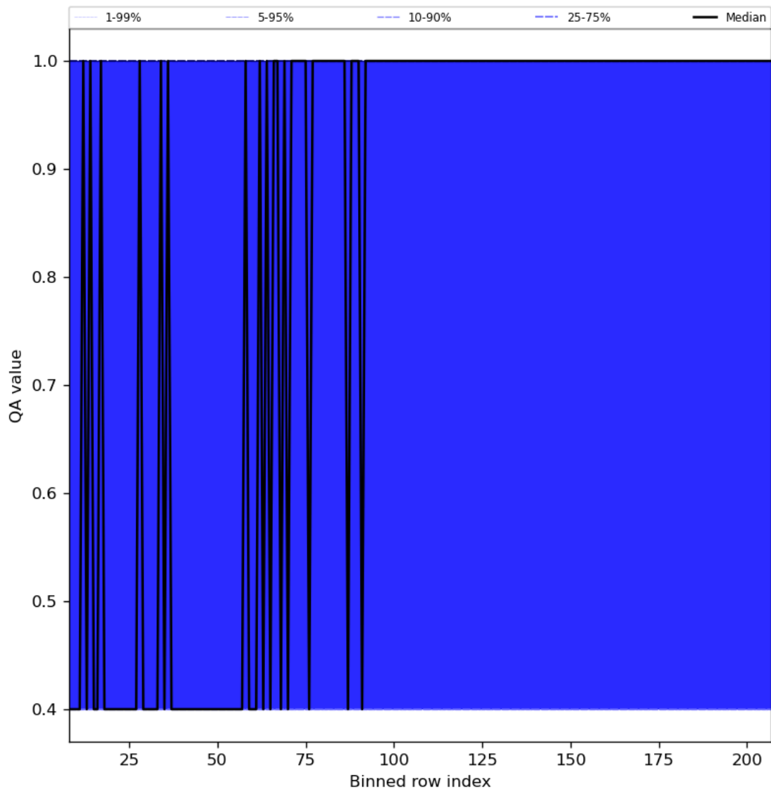
Figure 33: Along track statistics of “QA value” for 2023-09-24 to 2023-09-26
