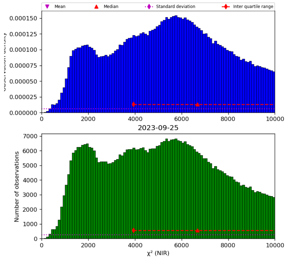
Figure 29: Histogram of “ \chi^2 (NIR)” for 2023-09-24 to 2023-09-26
