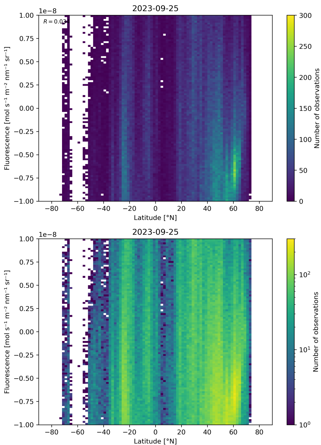
Figure 56: Scatter density plot of “Latitude” against “Fluorescence” for 2023-09-24 to 2023-09-26.
