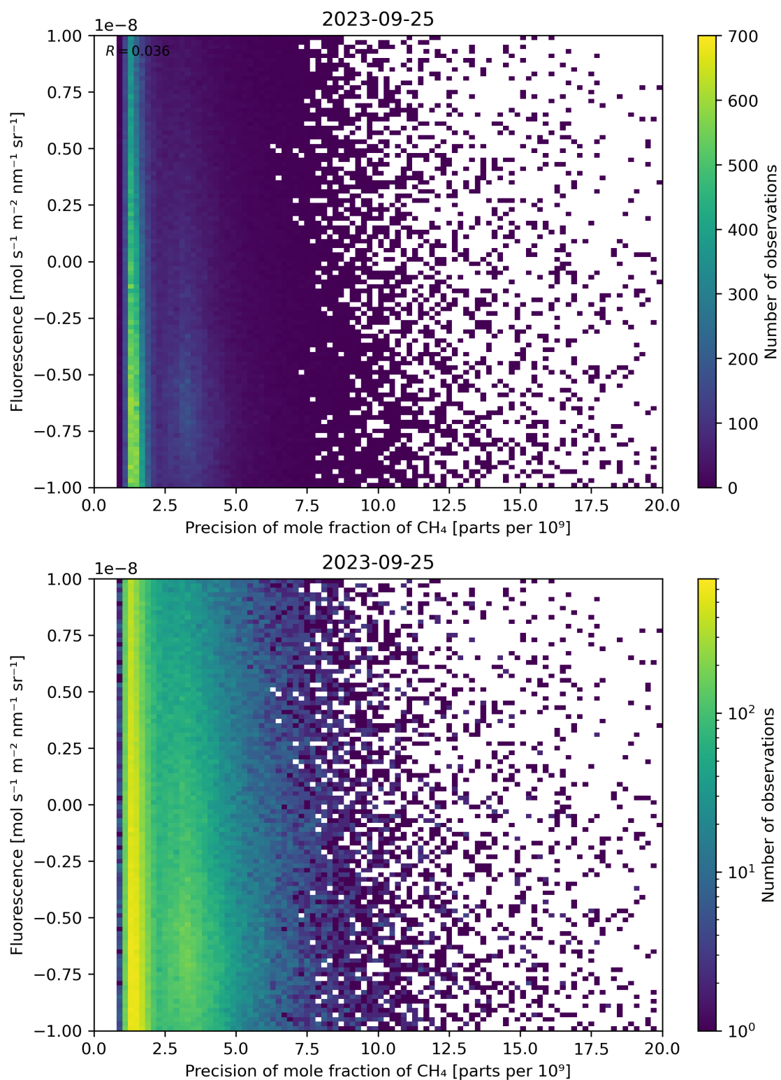
Figure 81: Scatter density plot of “Precision of mole fraction of \text{CH}_4 ” against “Fluorescence” for 2023-09-24 to 2023-09-26.
