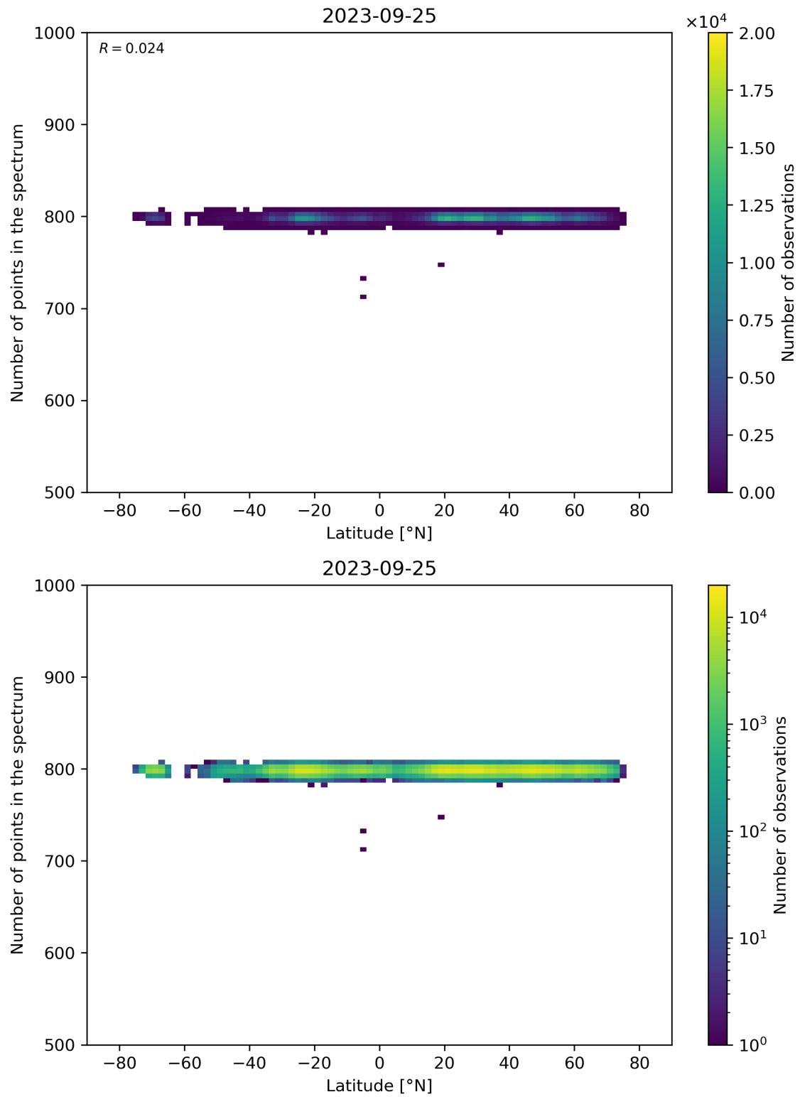
Figure 61: Scatter density plot of “Latitude” against “Number of points in the spectrum” for 2023-09-24 to 2023-09-26.
