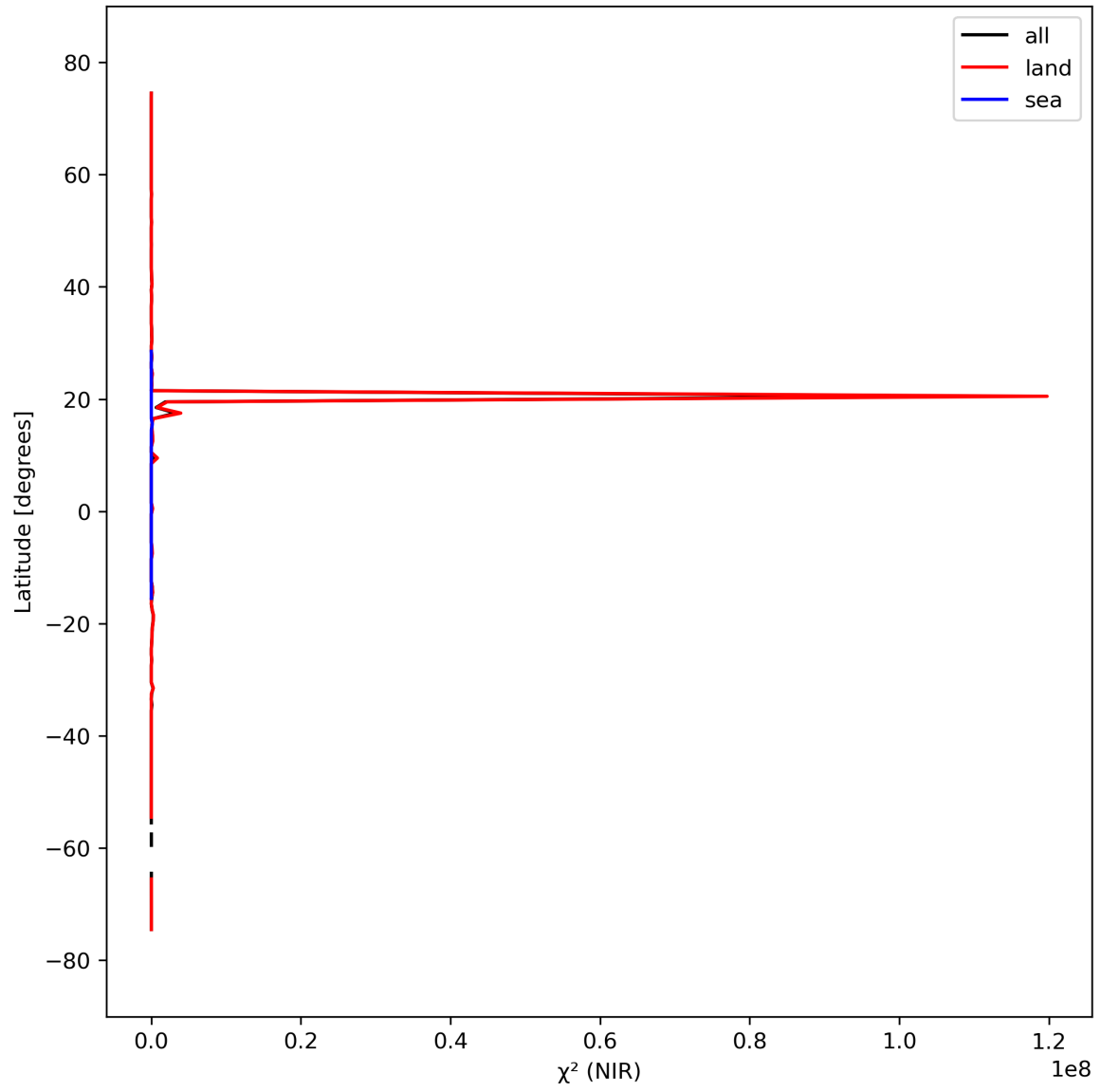
Figure 18: Zonal average of “ \chi^2 (NIR)” for 2023-09-24 to 2023-09-26.
