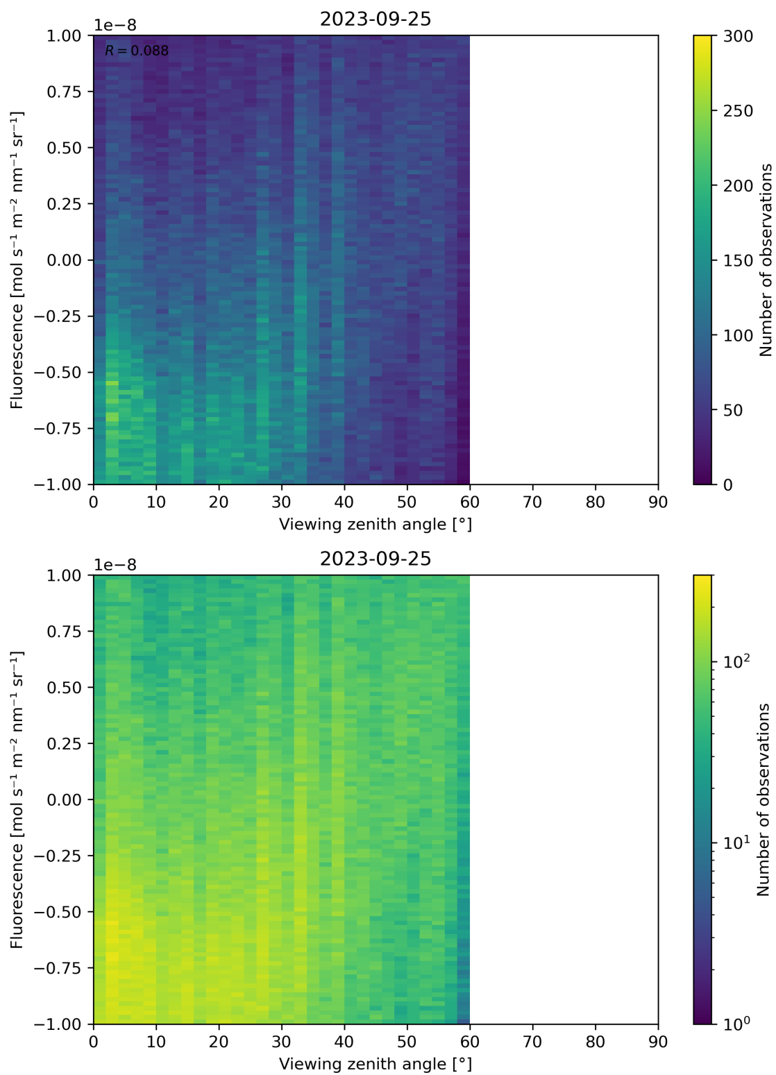
Figure 108: Scatter density plot of “Viewing zenith angle” against “Fluorescence” for 2023-09-24 to 2023-09-26.
