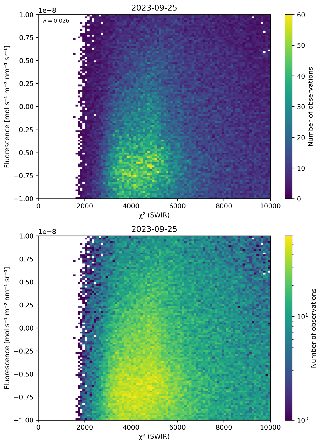
Figure 49: Scatter density plot of “ \chi^2 (SWIR)” against “Fluorescence” for 2023-09-24 to 2023-09-26.
