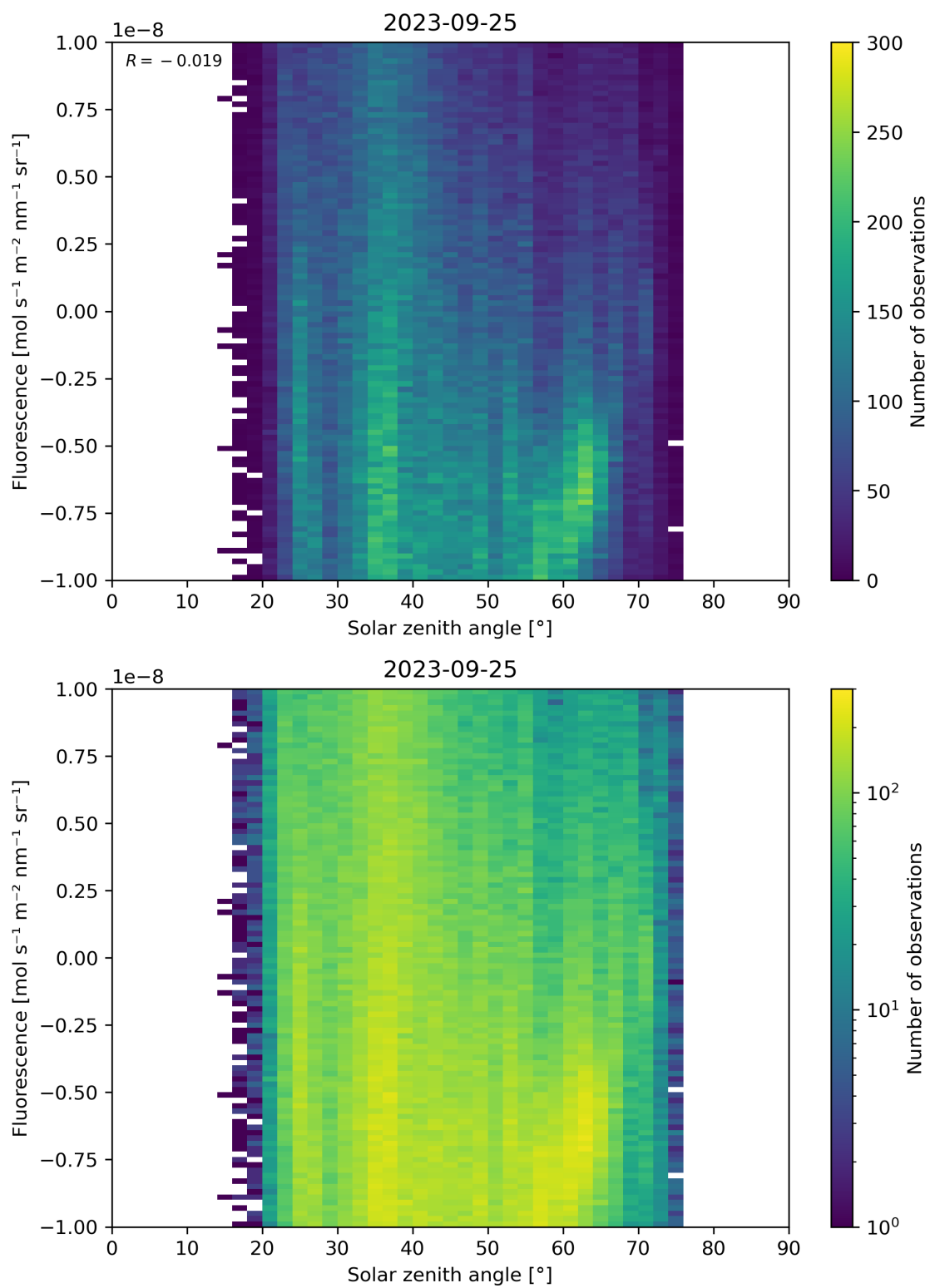
Figure 97: Scatter density plot of “Solar zenith angle” against “Fluorescence” for 2023-09-24 to 2023-09-26.
