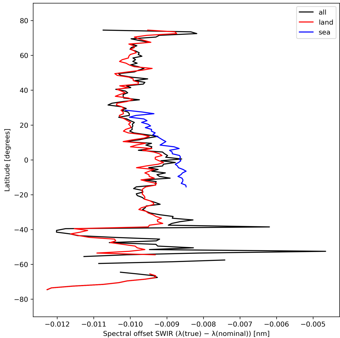
Figure 16: Zonal average of “Spectral offset SWIR ( \lambda(\text{true}) - \lambda(\text{nominal}) )” for 2023-09-24 to 2023-09-26.
