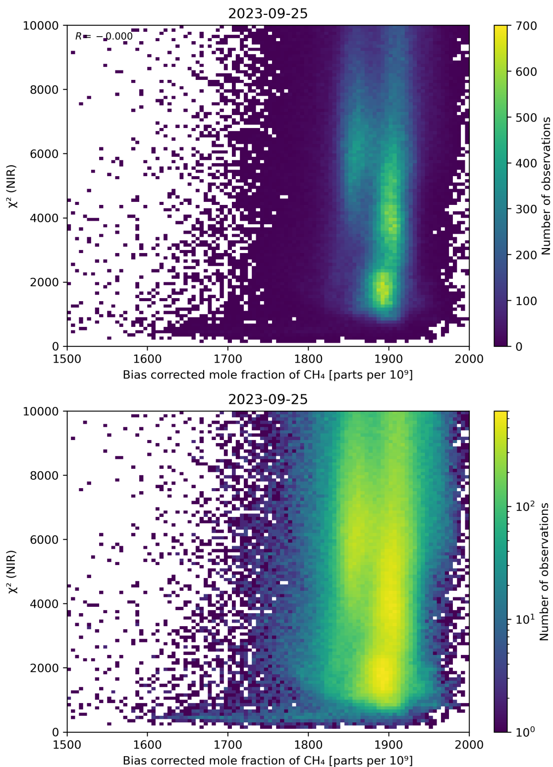
Figure 63: Scatter density plot of “Bias corrected mole fraction of CH 4 ” against “ \chi^2 (NIR)” for 2023-09-24 to 2023-09-26.
