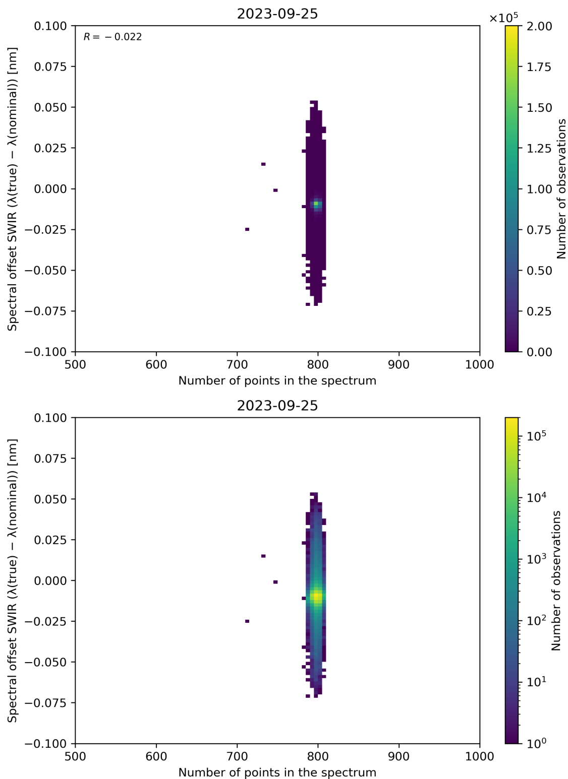
Figure 93: Scatter density plot of “Number of points in the spectrum” against “Spectral offset SWIR ( \lambda(\text{true}) - \lambda(\text{nominal}) )” for 2023-09-24 to 2023-09-26.
