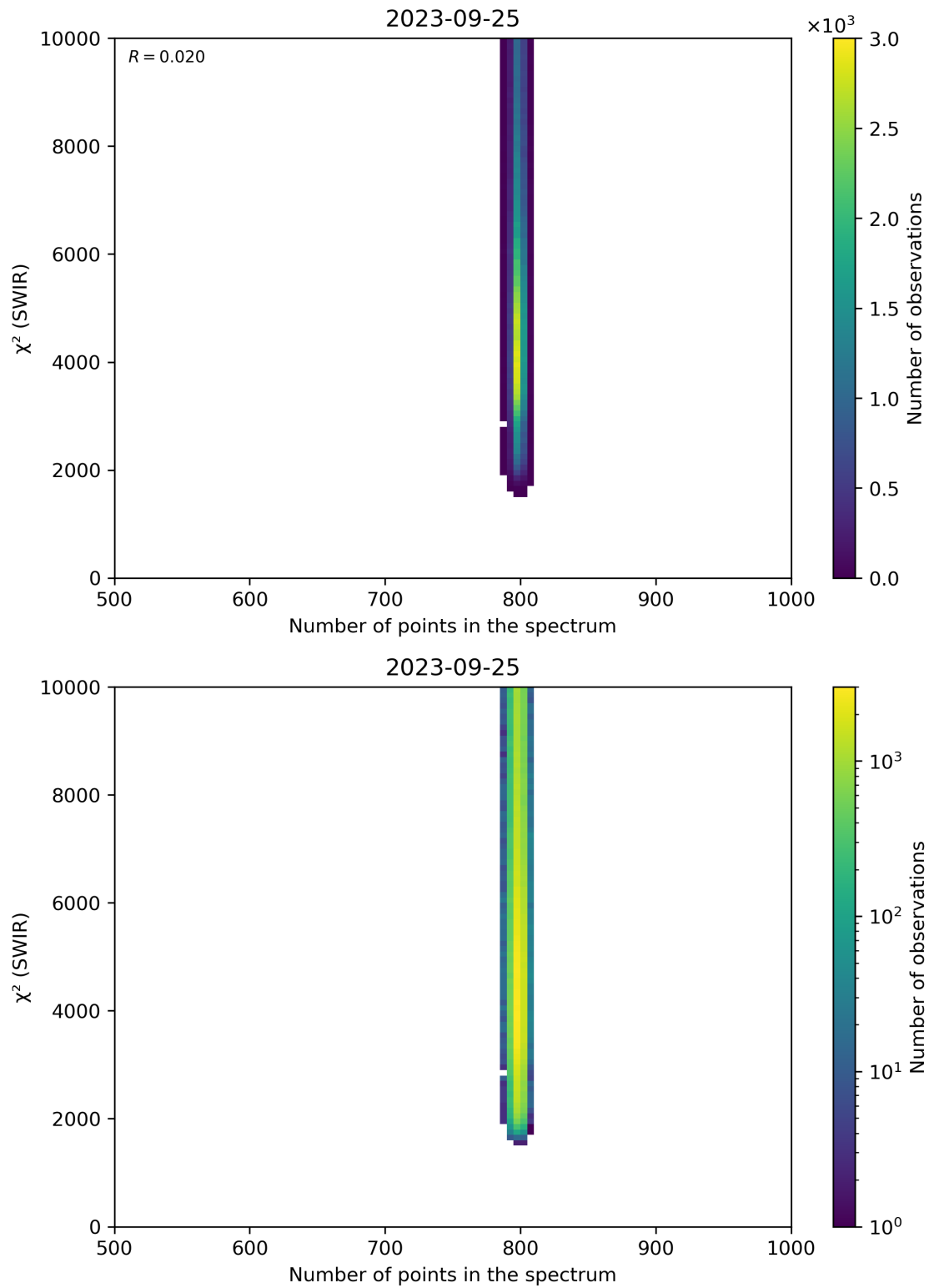
Figure 89: Scatter density plot of “Number of points in the spectrum” against “ \chi^2 (SWIR)” for 2023-09-24 to 2023-09-26.
