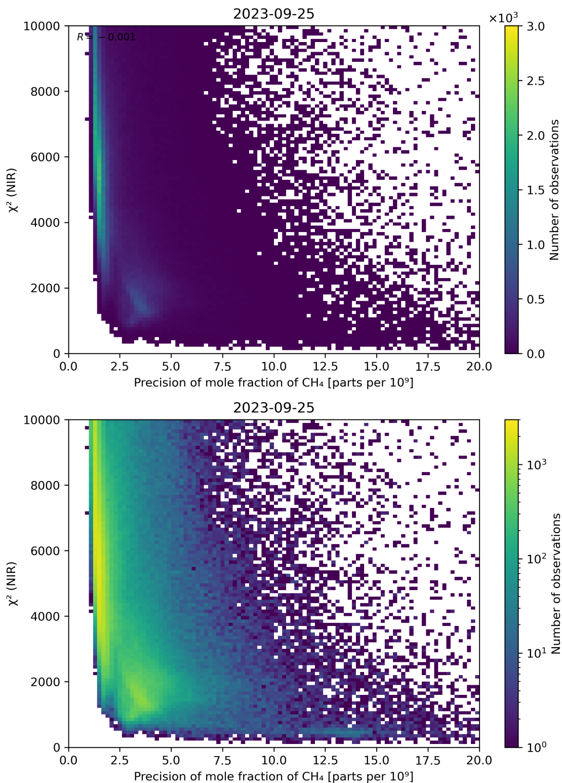
Figure 78: Scatter density plot of “Precision of mole fraction of \text{CH}_4 ” against “ \chi^2 (NIR)” for 2023-09-24 to 2023-09-26.
