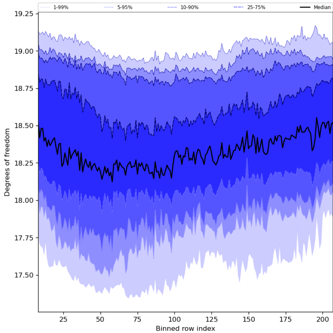
Figure 41: Along track statistics of “Degrees of freedom” for 2023-09-24 to 2023-09-26
