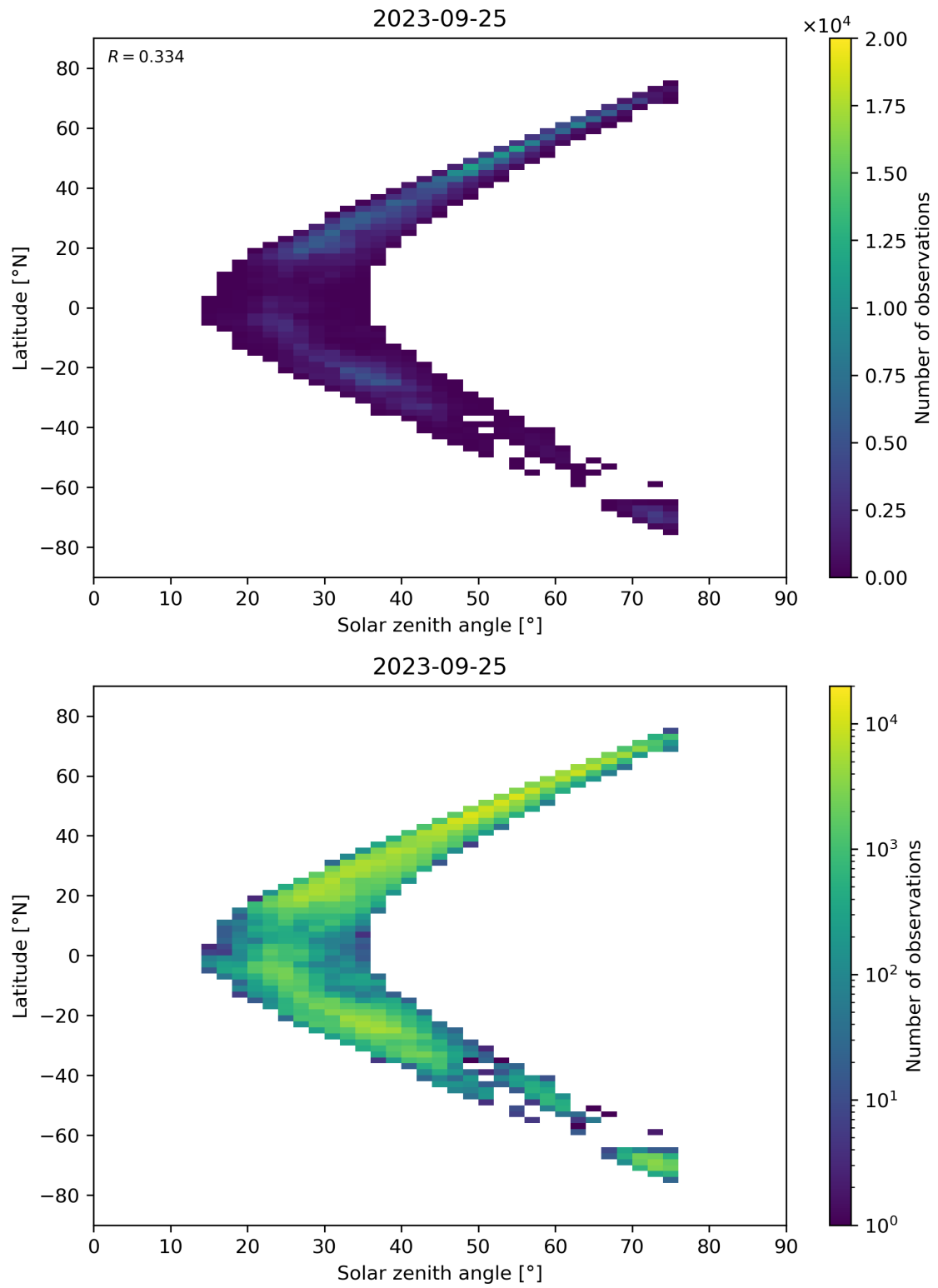
Figure 98: Scatter density plot of “Solar zenith angle” against “Latitude” for 2023-09-24 to 2023-09-26.
