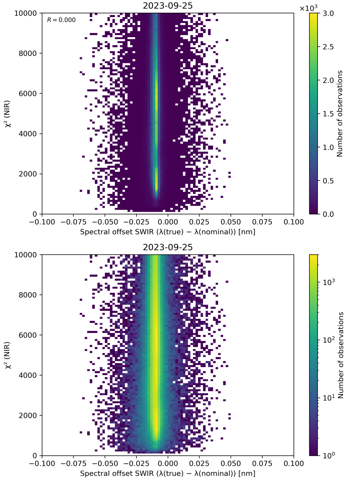
Figure 117: Scatter density plot of “Spectral offset SWIR ( \lambda(\text{true}) - \lambda(\text{nominal}) )” against “ \chi^2 (NIR)” for 2023-09-24 to 2023-09-26.
