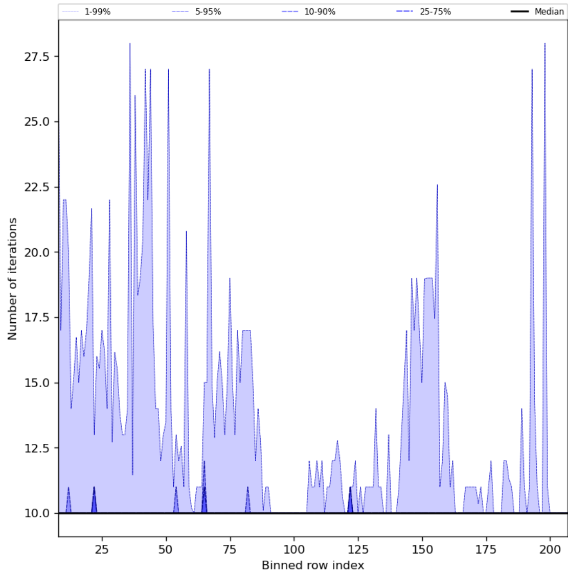
Figure 42: Along track statistics of “Number of iterations” for 2023-09-24 to 2023-09-26
