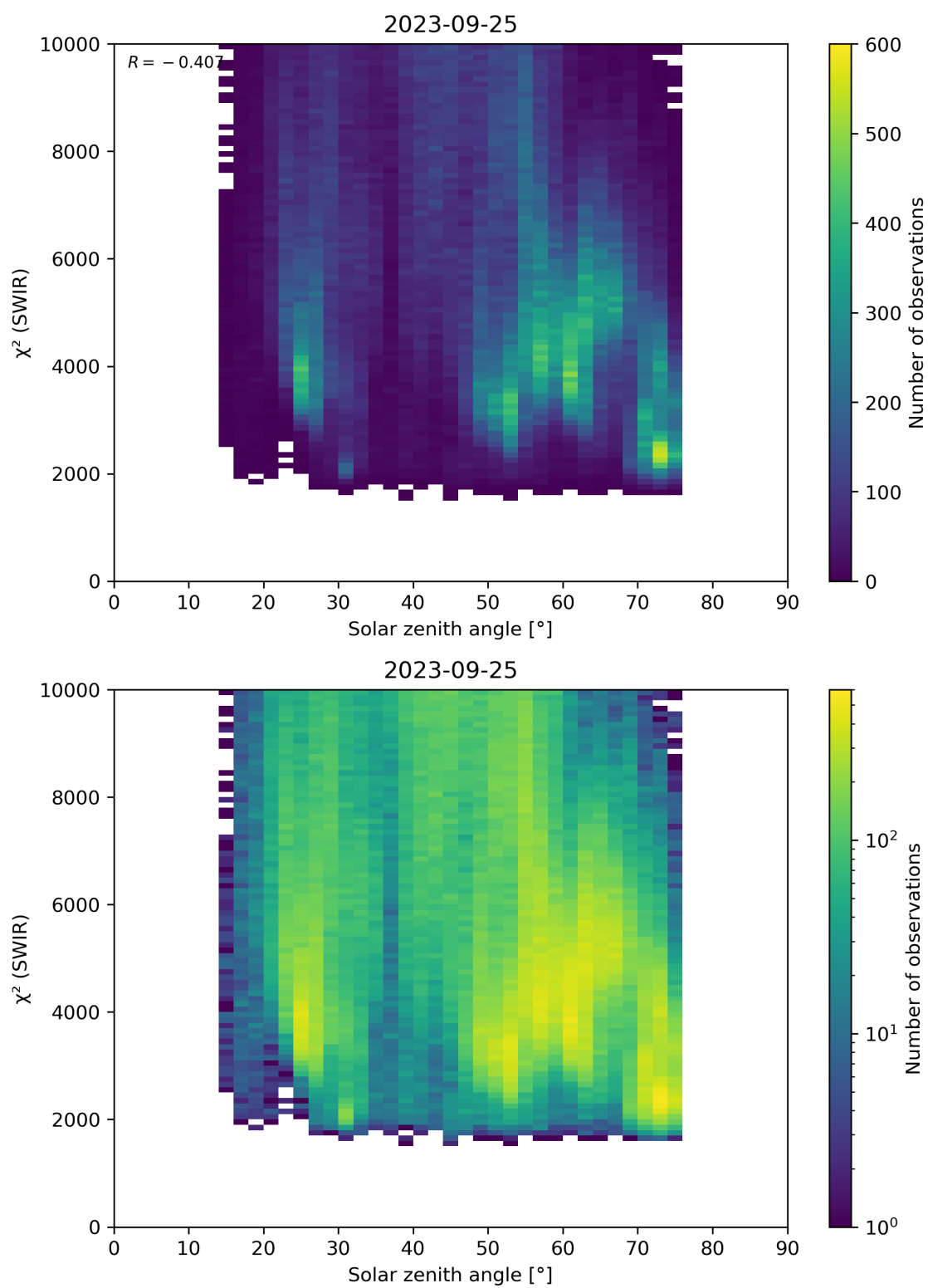
Figure 95: Scatter density plot of “Solar zenith angle” against “ \chi^2 (SWIR)” for 2023-09-24 to 2023-09-26.
