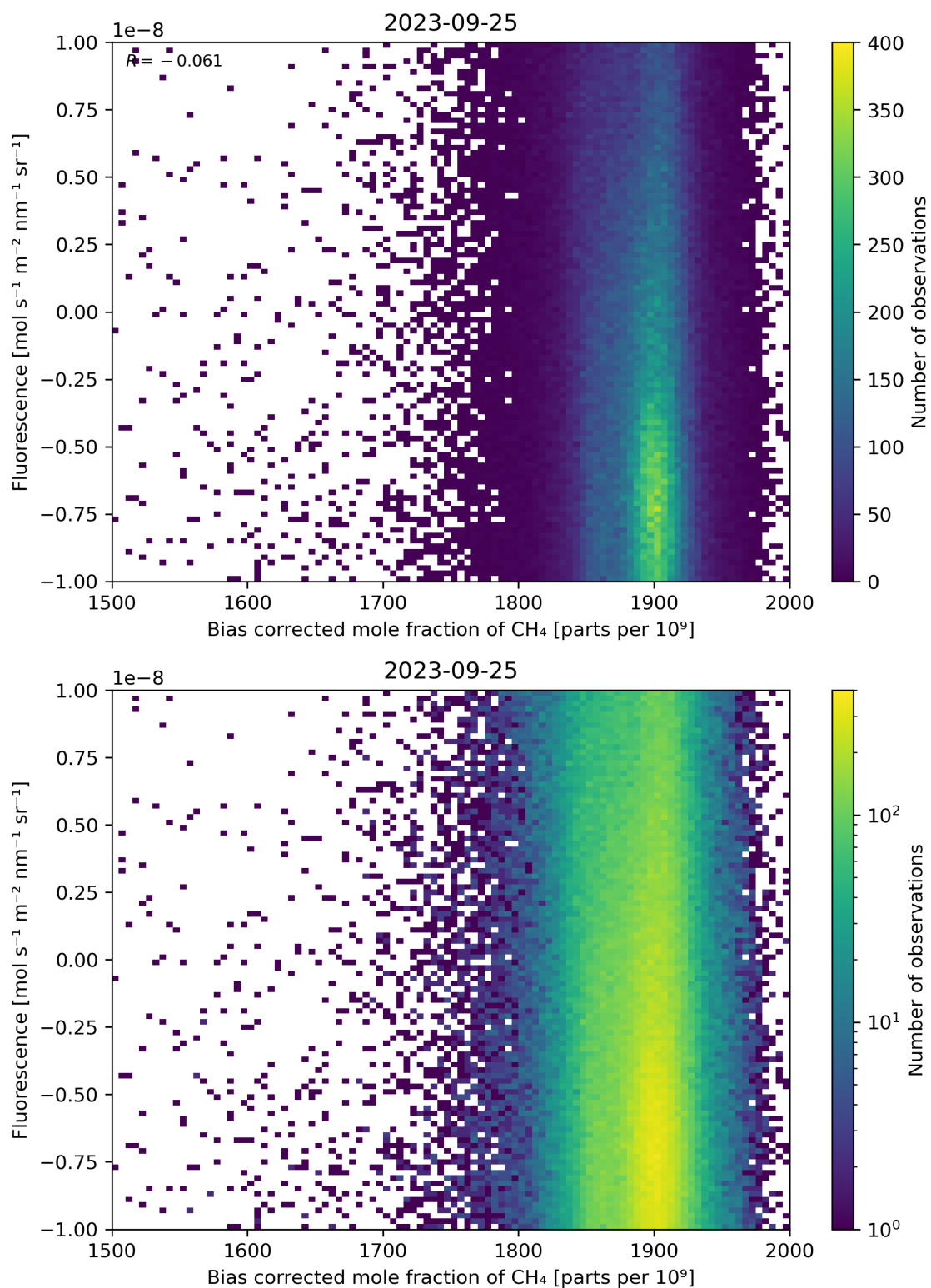
Figure 66: Scatter density plot of “Bias corrected mole fraction of \text{CH}_4 ” against “Fluorescence” for 2023-09-24 to 2023-09-26.
