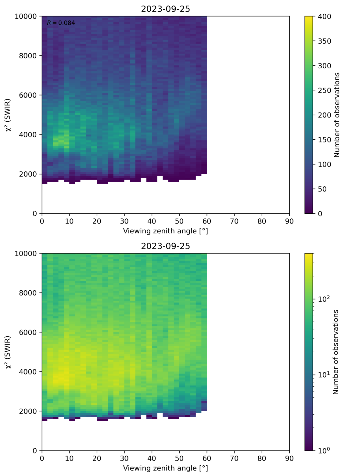
Figure 106: Scatter density plot of “Viewing zenith angle” against “ \chi^2 (SWIR)” for 2023-09-24 to 2023-09-26.
