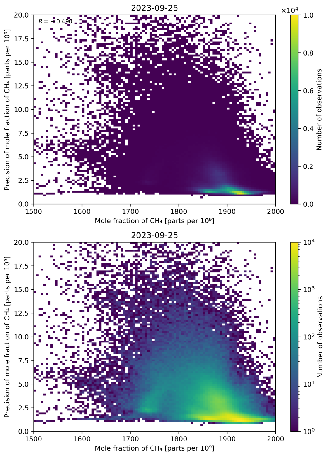
Figure 75: Scatter density plot of “Mole fraction of CH 4 ” against “Precision of mole fraction of CH 4 ” for 2023-09-24 to 2023-09-26.
