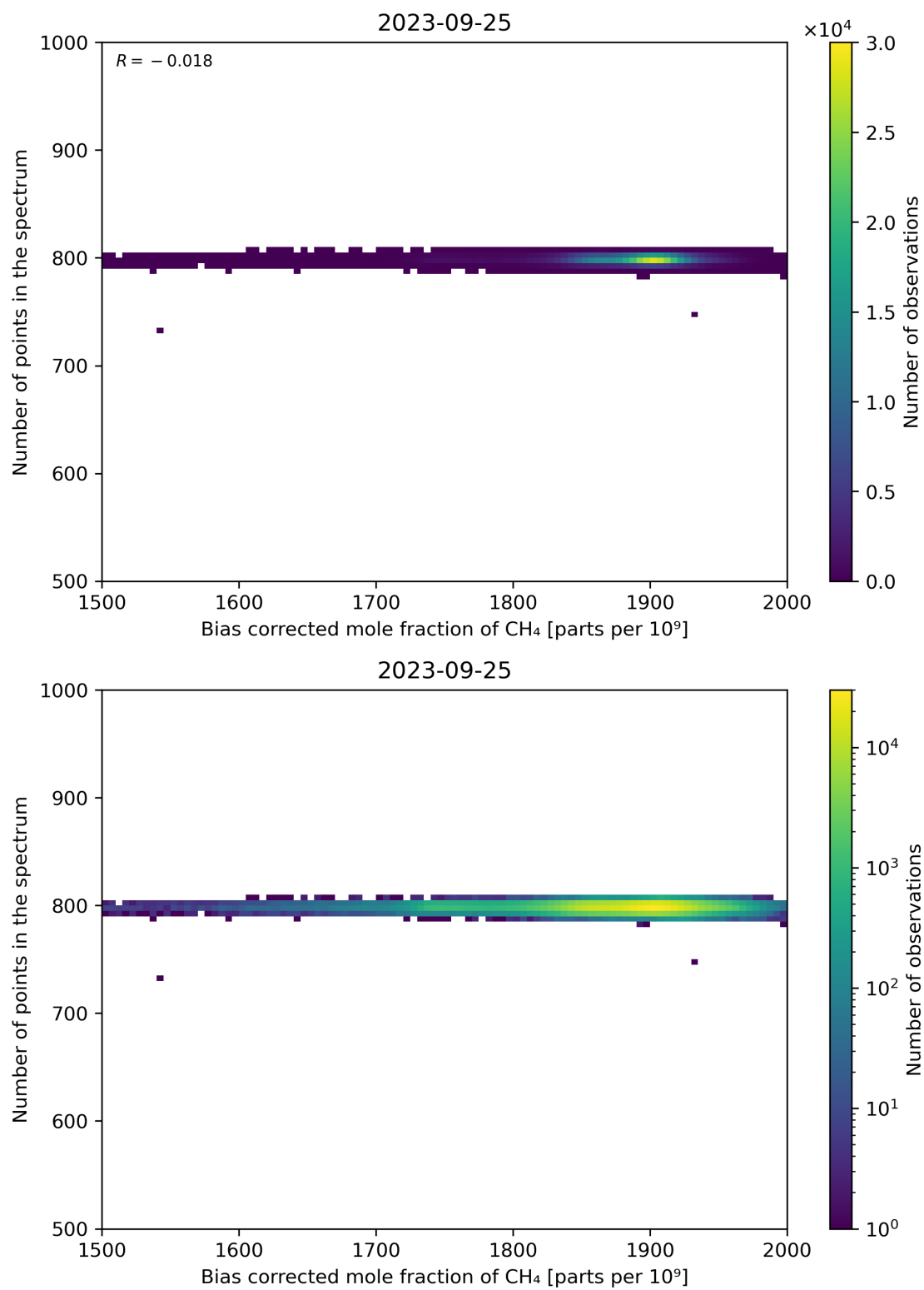
Figure 68: Scatter density plot of “Bias corrected mole fraction of CH 4 ” against “Number of points in the spectrum” for 2023-09-24 to 2023-09-26.
