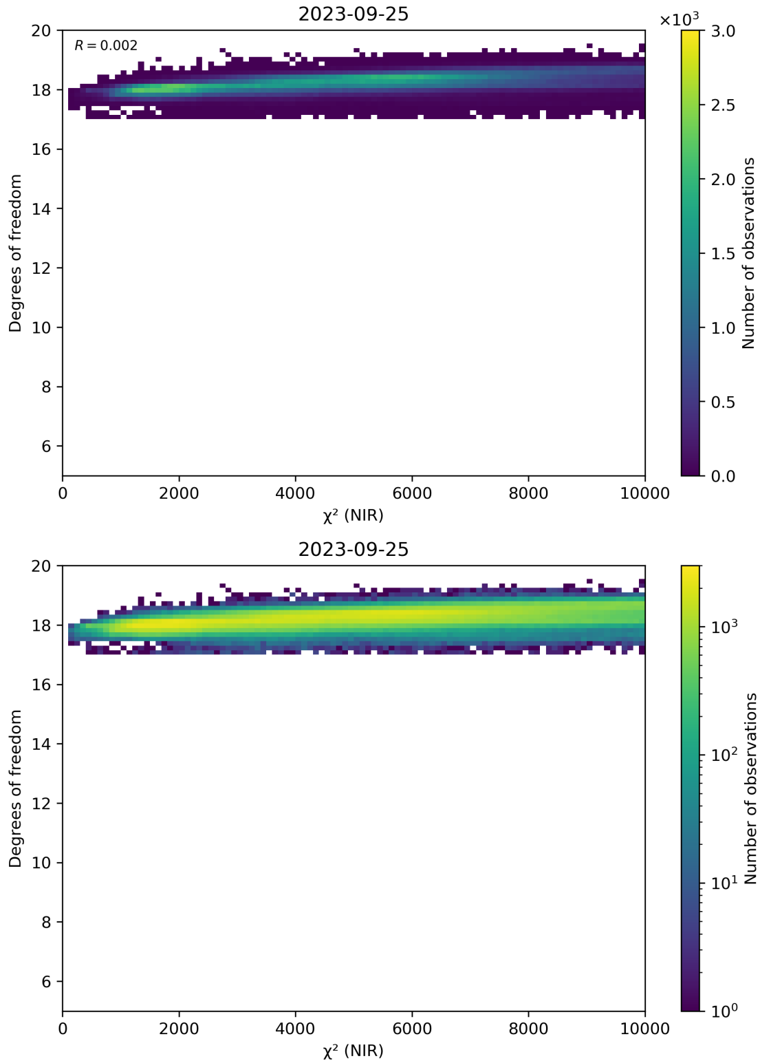
Figure 44: Scatter density plot of “ \chi^2 (NIR)” against “Degrees of freedom” for 2023-09-24 to 2023-09-26.
