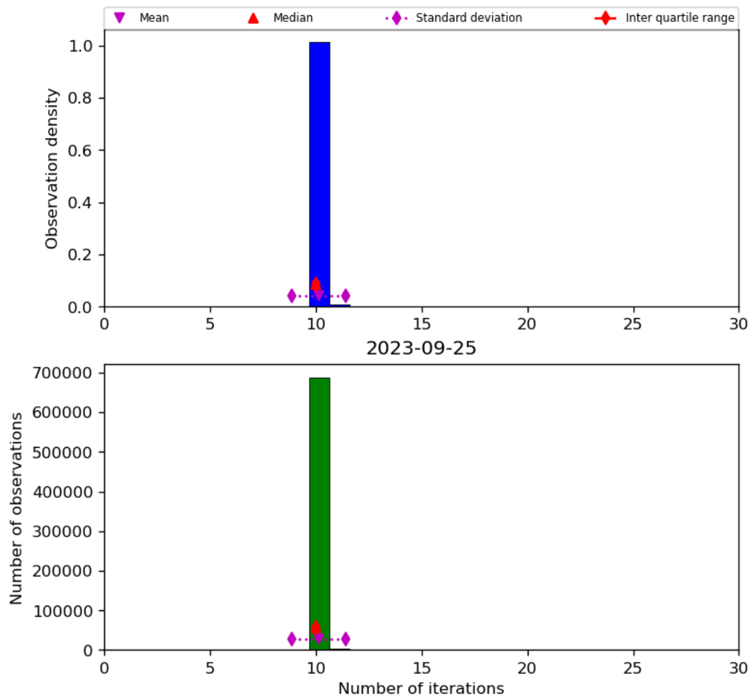
Figure 31: Histogram of “Number of iterations” for 2023-09-24 to 2023-09-26
