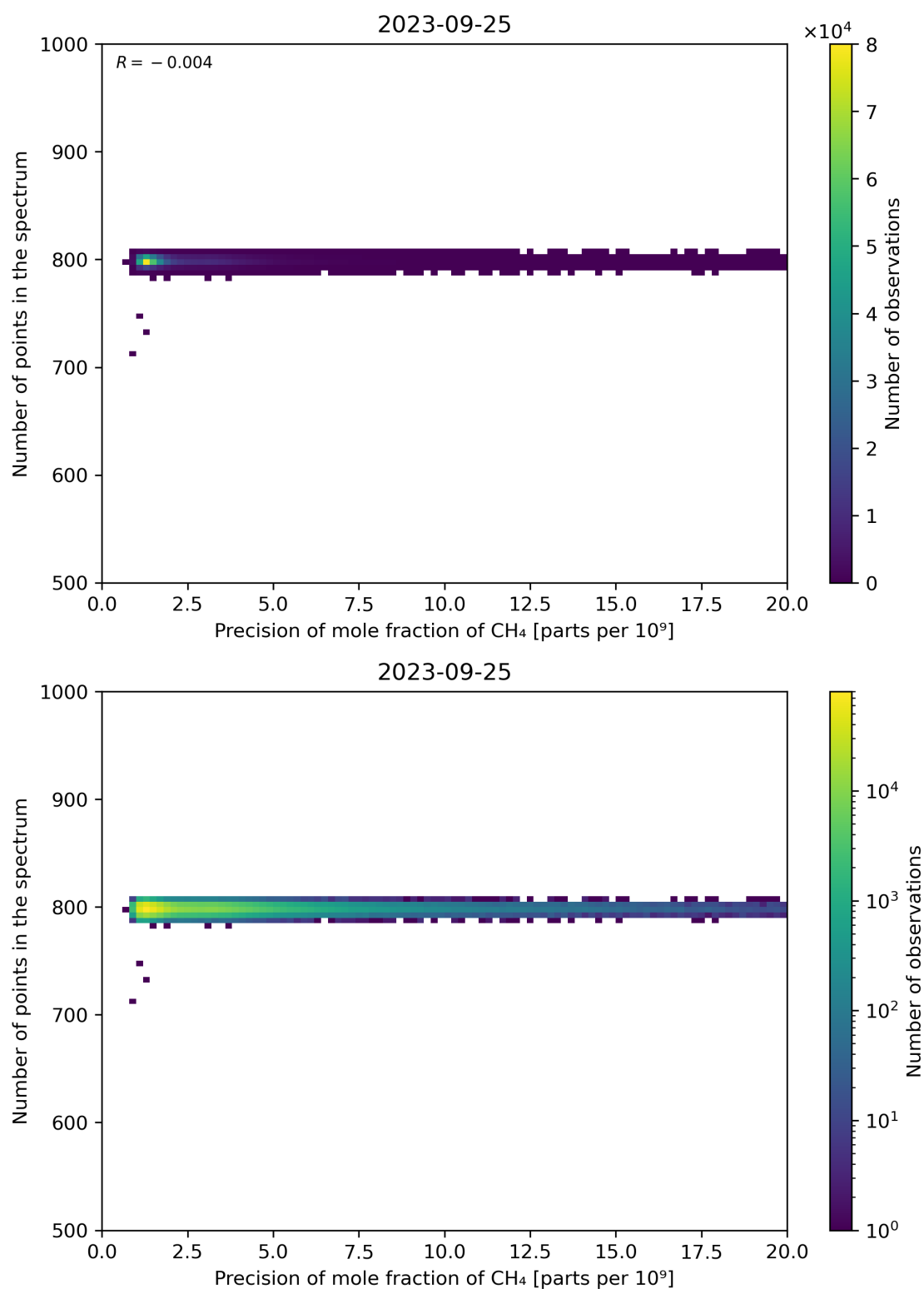
Figure 84: Scatter density plot of “Precision of mole fraction of CH 4 ” against “Number of points in the spectrum” for 2023-09-24 to 2023-09-26.
