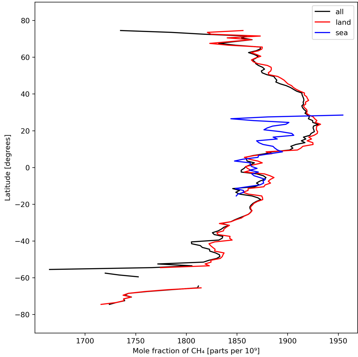
Figure 12: Zonal average of “Mole fraction of CH 4 ” for 2023-09-24 to 2023-09-26.
