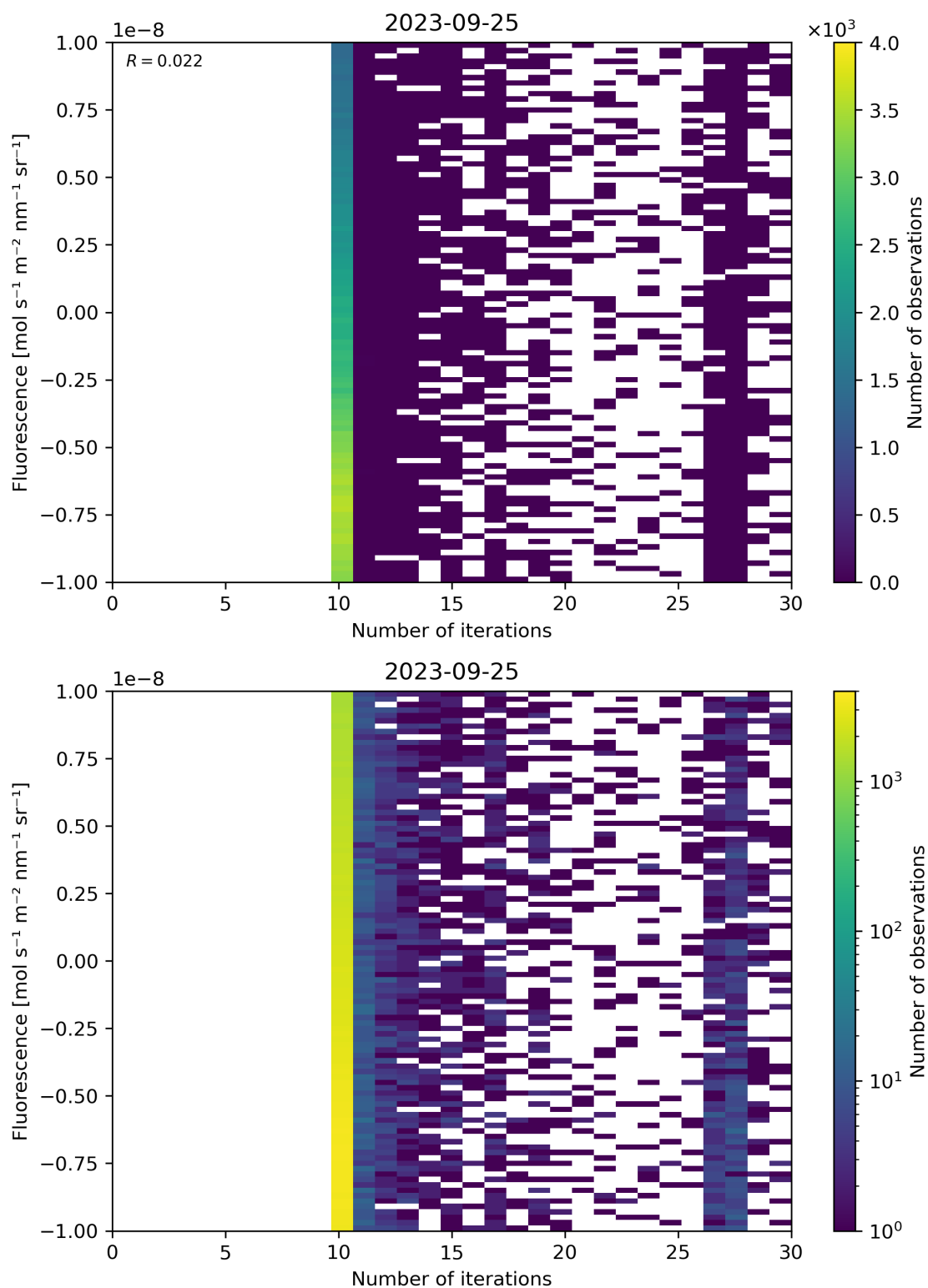
Figure 87: Scatter density plot of “Number of iterations” against “Fluorescence” for 2023-09-24 to 2023-09-26.
