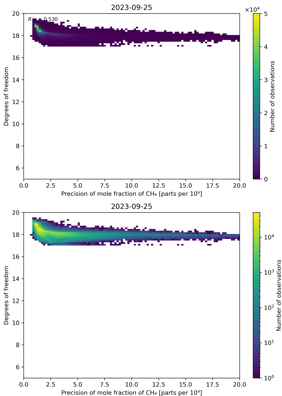
Figure 80: Scatter density plot of “Precision of mole fraction of CH 4 ” against “Degrees of freedom” for 2023-09-24 to 2023-09-26.
