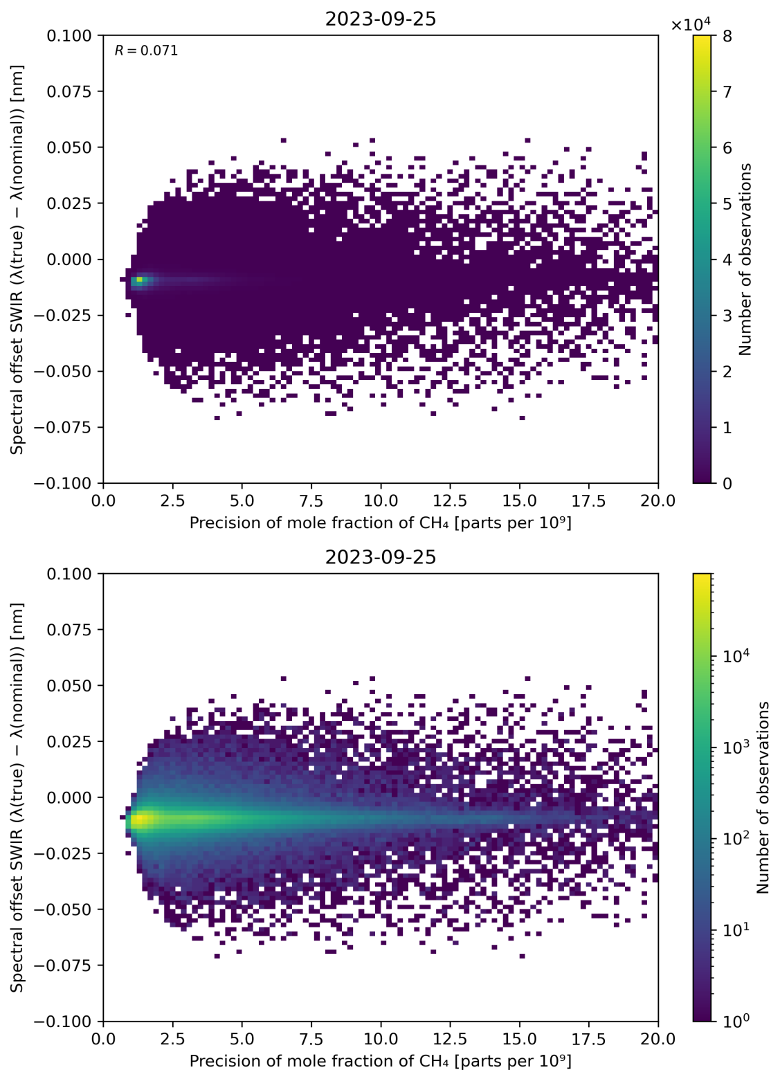
Figure 85: Scatter density plot of “Precision of mole fraction of CH 4 ” against “Spectral offset SWIR ( \lambda(\text{true}) - \lambda(\text{nominal}) )” for 2023-09-24 to 2023-09-26.
