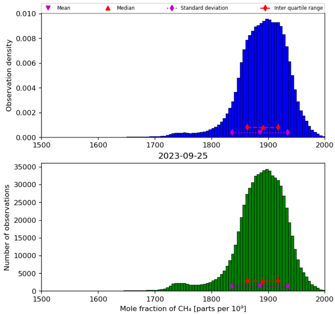
Figure 23: Histogram of “Mole fraction of CH 4 ” for 2023-09-24 to 2023-09-26
