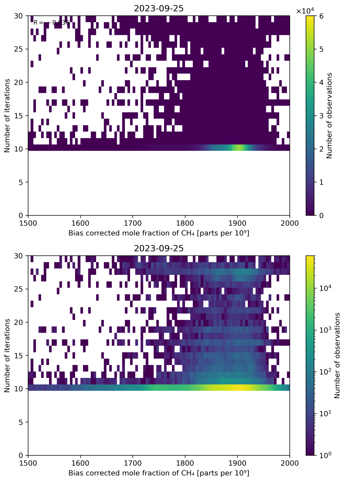
Figure 67: Scatter density plot of “Bias corrected mole fraction of CH 4 ” against “Number of iterations” for 2023-09-24 to 2023-09-26.
