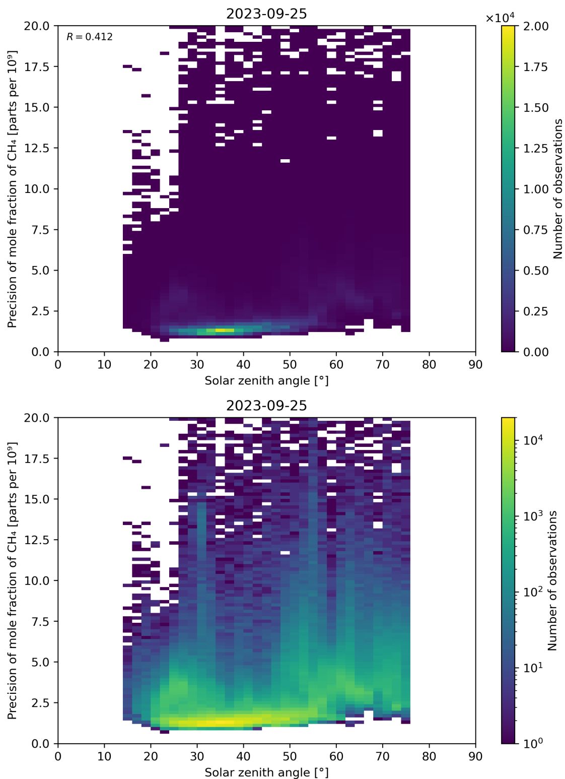
Figure 101: Scatter density plot of “Solar zenith angle” against “Precision of mole fraction of \text{CH}_4 ” for 2023-09-24 to 2023-09-26.
