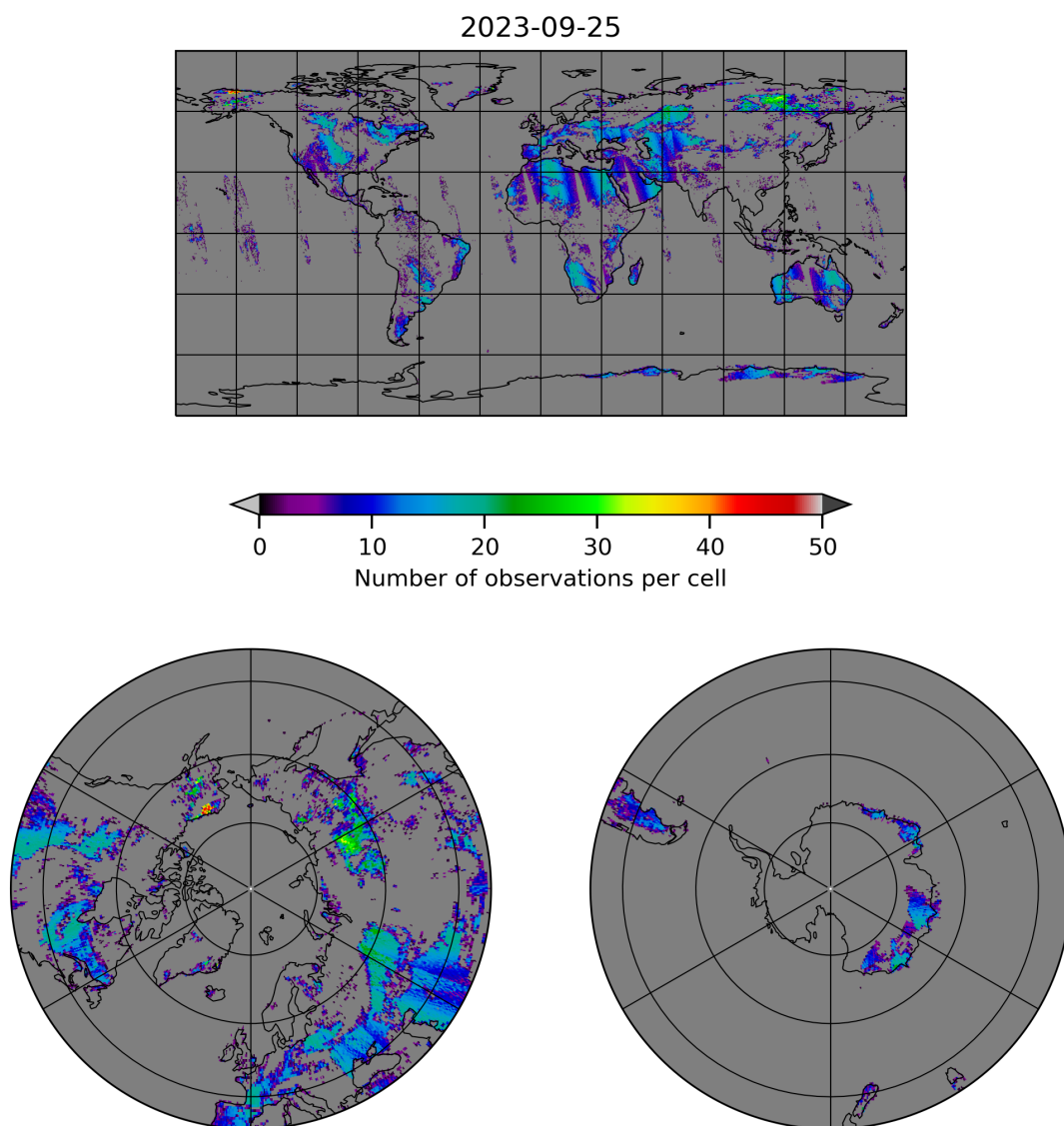
Figure 10: Map of the number of observations for 2023-09-24 to 2023-09-26
