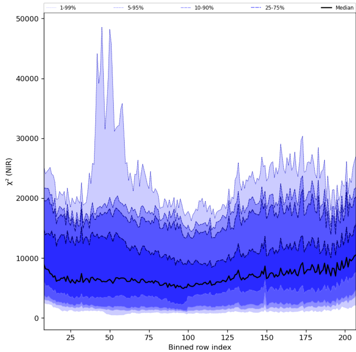
Figure 40: Along track statistics of “ \chi^2 (NIR)” for 2023-09-24 to 2023-09-26
