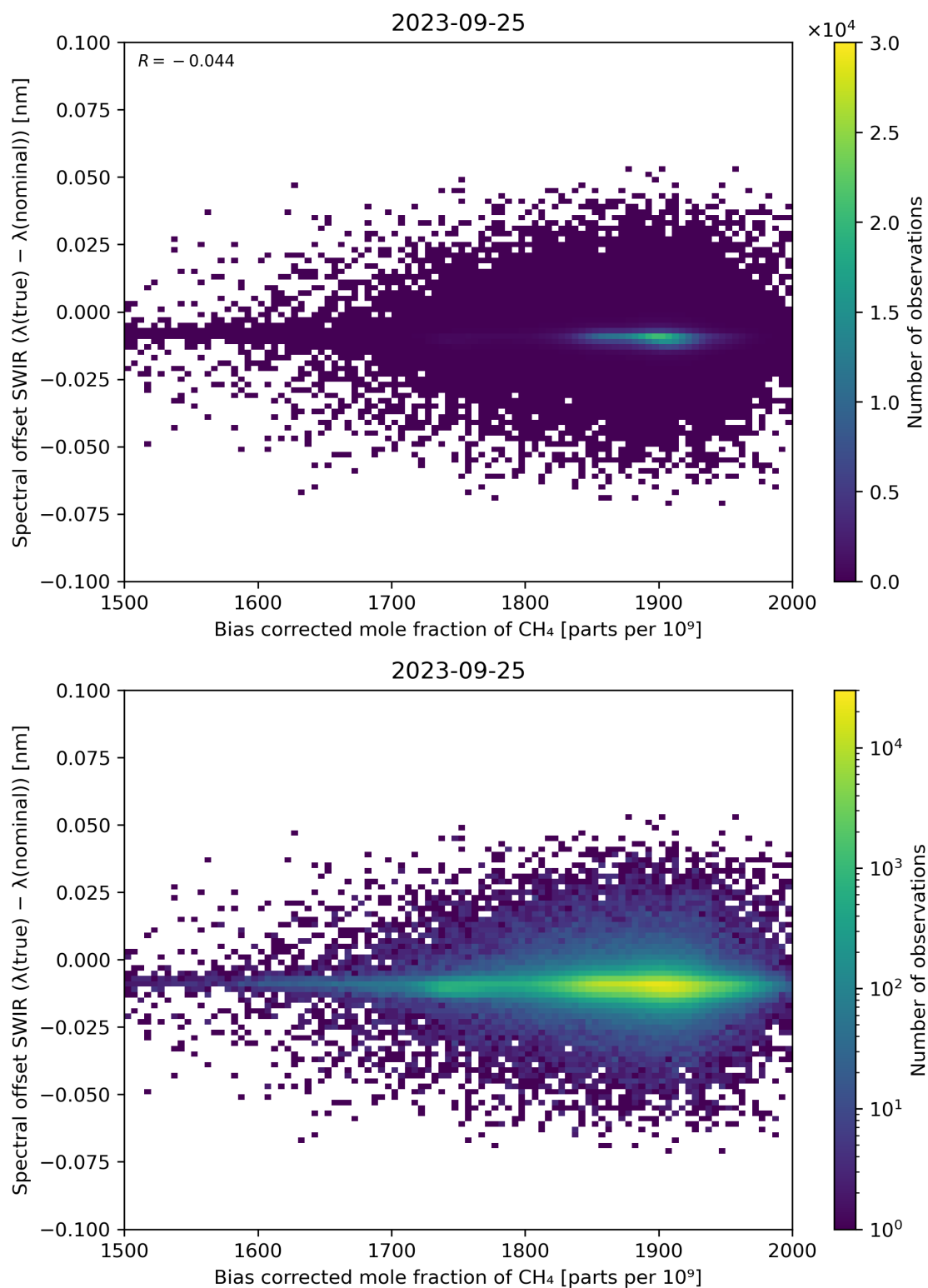
Figure 69: Scatter density plot of “Bias corrected mole fraction of \text{CH}_4 ” against “Spectral offset SWIR ( \lambda(\text{true}) - \lambda(\text{nominal}) )” for 2023-09-24 to 2023-09-26.
