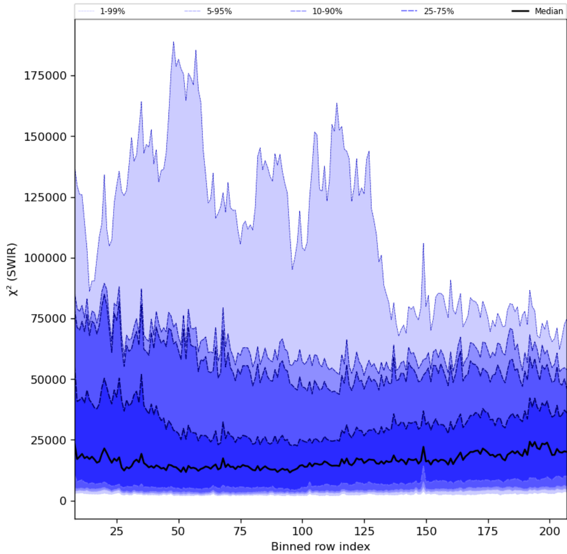
Figure 39: Along track statistics of “ \chi^2 (SWIR)” for 2023-09-24 to 2023-09-26
