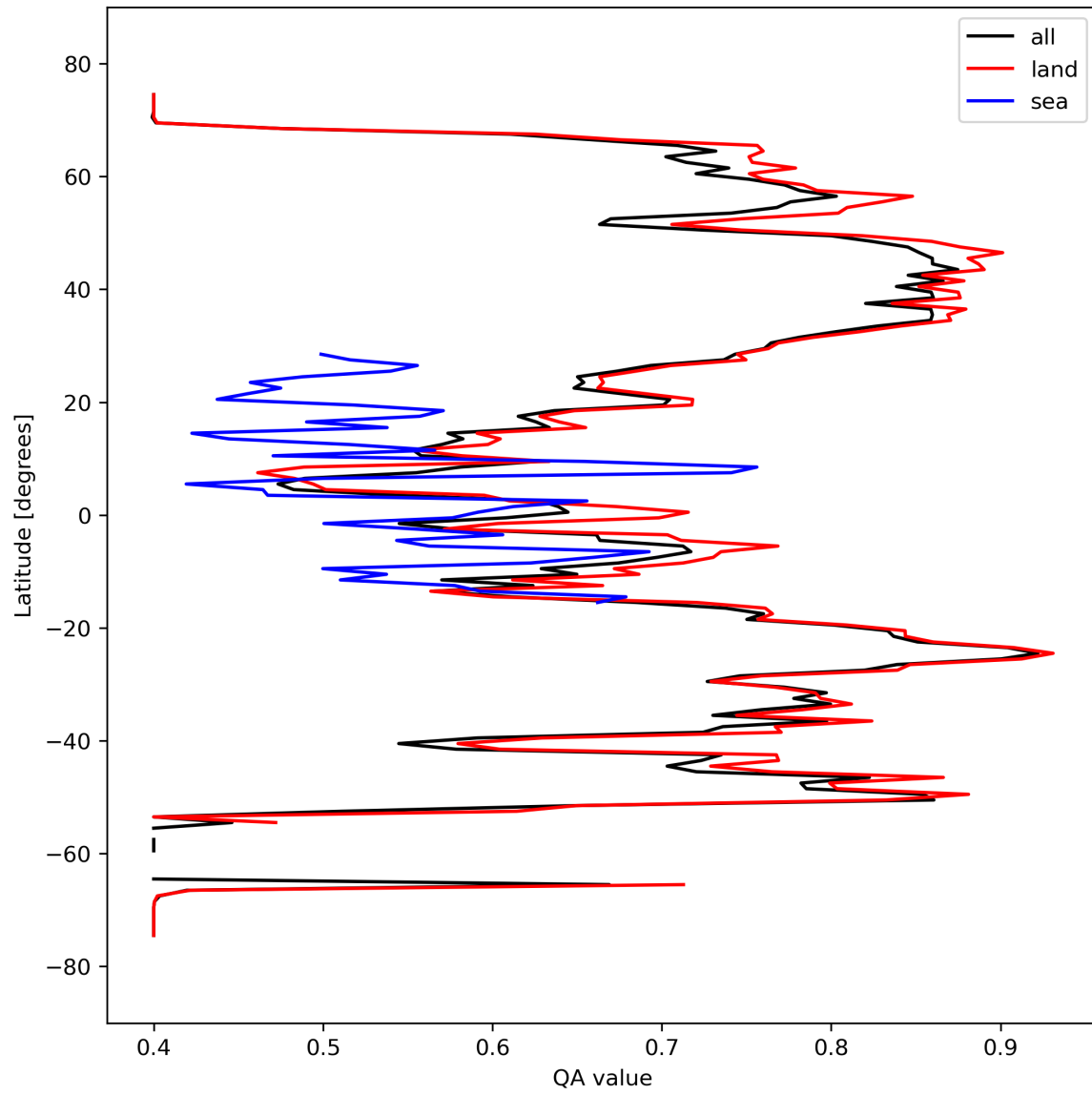
Figure 11: Zonal average of “QA value” for 2023-09-24 to 2023-09-26.
