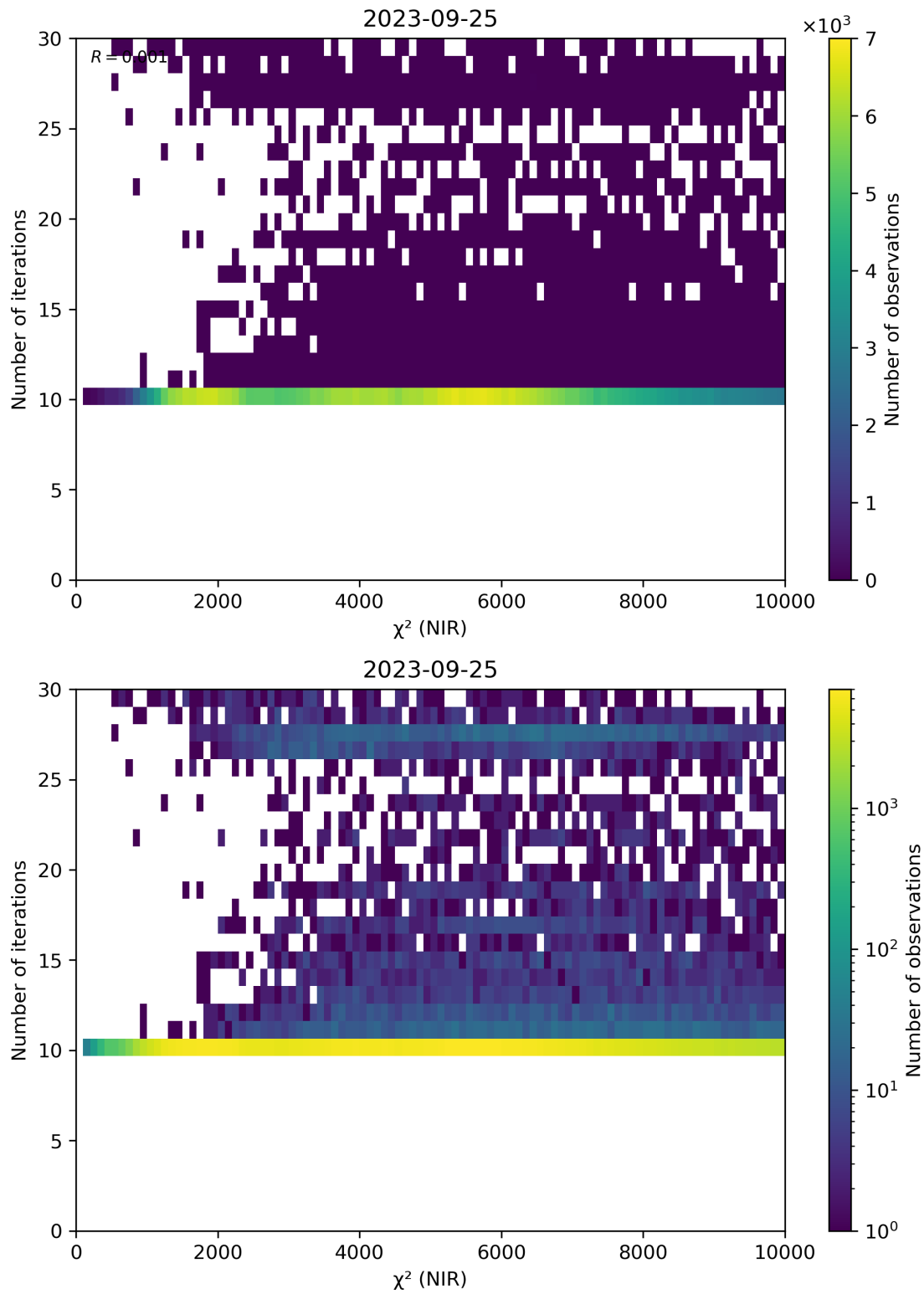
Figure 46: Scatter density plot of “ \chi^2 (NIR)” against “Number of iterations” for 2023-09-24 to 2023-09-26.
