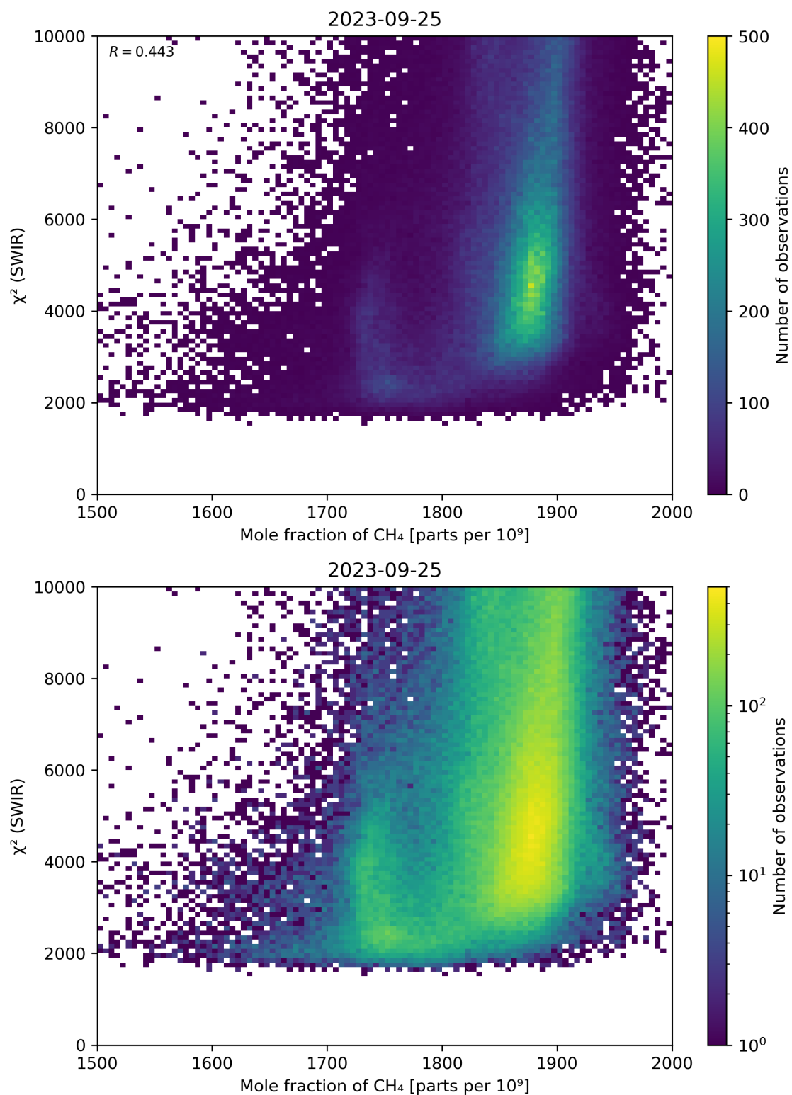
Figure 71: Scatter density plot of “Mole fraction of CH 4 ” against “ \chi^2 (SWIR)” for 2023-09-24 to 2023-09-26.
