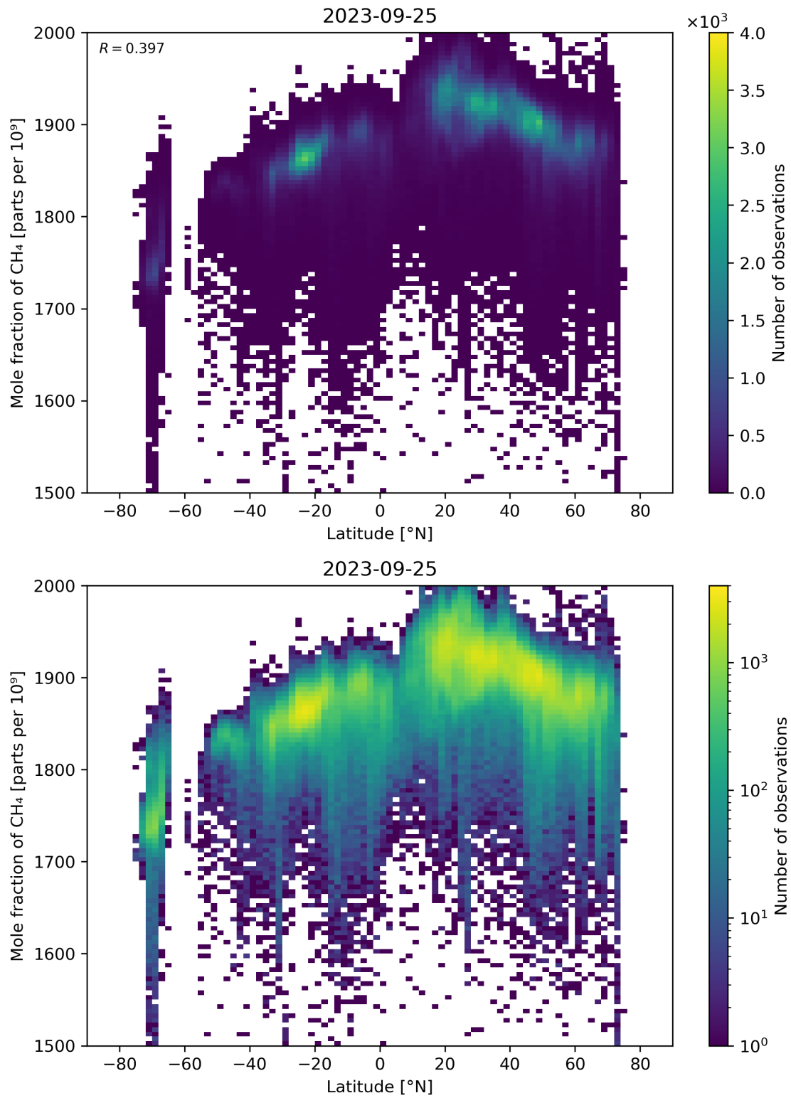
Figure 57: Scatter density plot of “Latitude” against “Mole fraction of CH 4 ” for 2023-09-24 to 2023-09-26.
