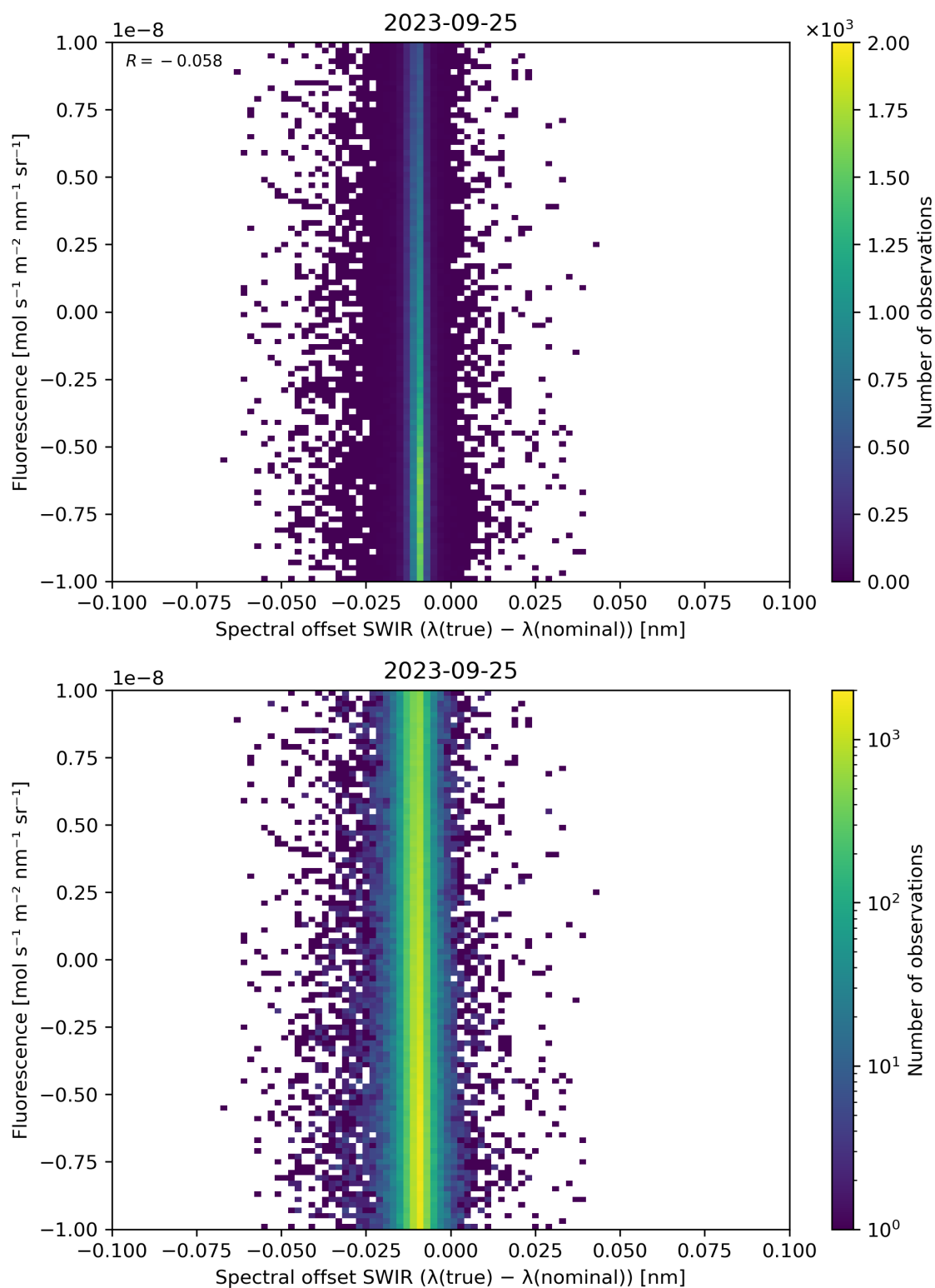
Figure 120: Scatter density plot of “Spectral offset SWIR ( \lambda(\text{true}) - \lambda(\text{nominal}) )” against “Fluorescence” for 2023-09-24 to 2023-09-26.
