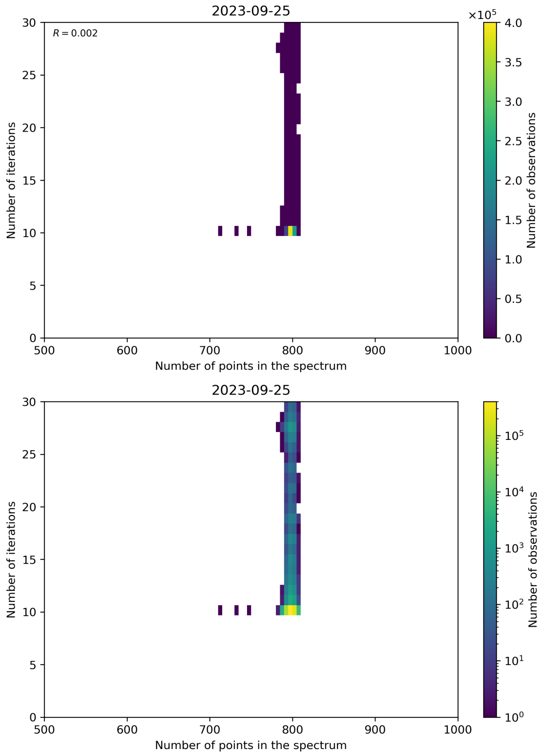
Figure 92: Scatter density plot of “Number of points in the spectrum” against “Number of iterations” for 2023-09-24 to 2023-09-26.
