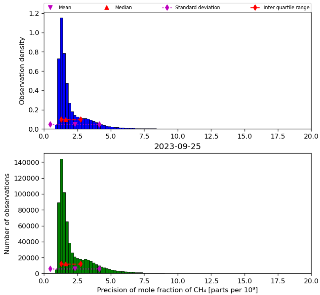
Figure 24: Histogram of “Precision of mole fraction of CH 4 ” for 2023-09-24 to 2023-09-26
