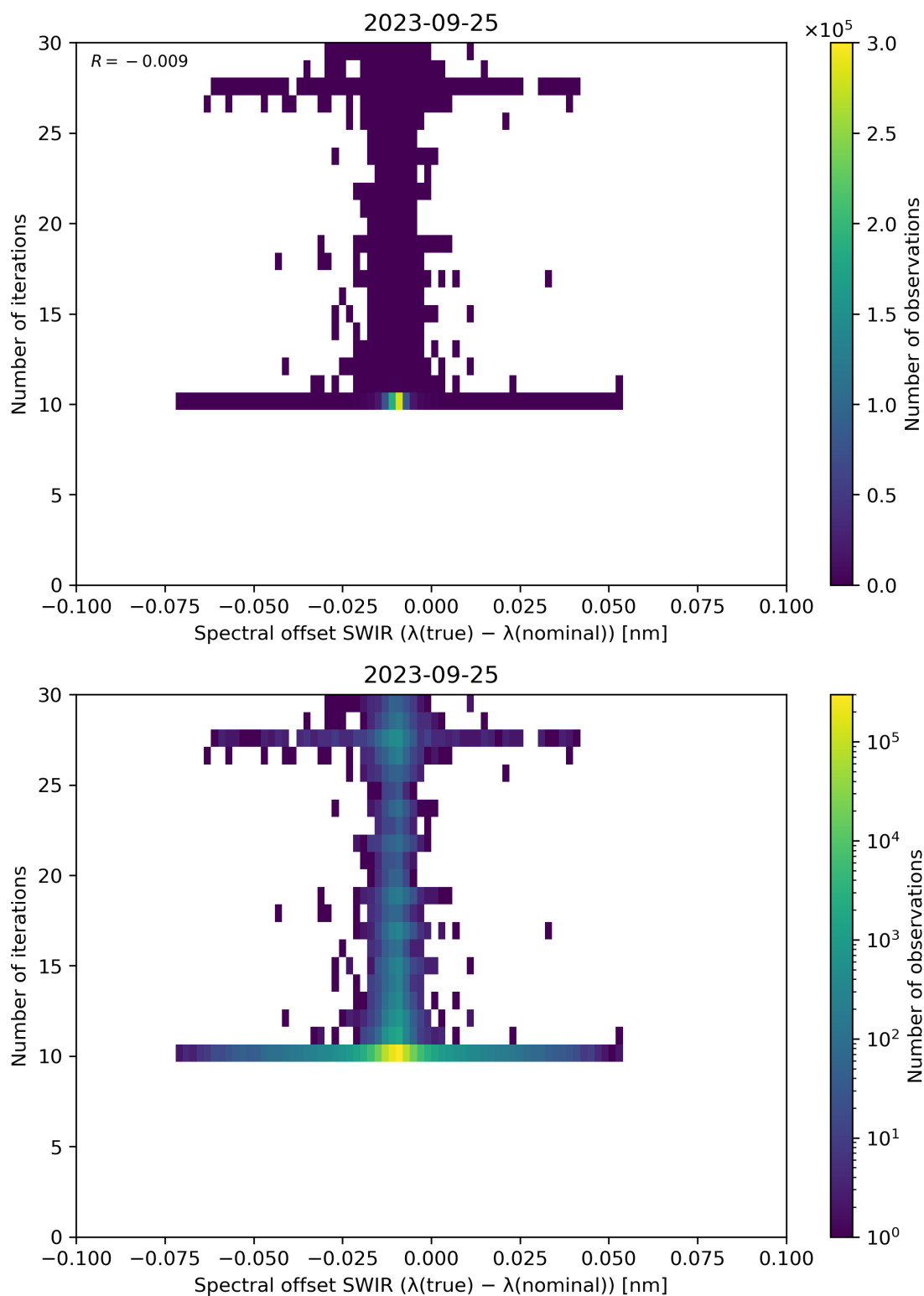
Figure 121: Scatter density plot of “Spectral offset SWIR ( \lambda(\text{true}) - \lambda(\text{nominal}) )” against “Number of iterations” for 2023-09-24 to 2023-09-26.
