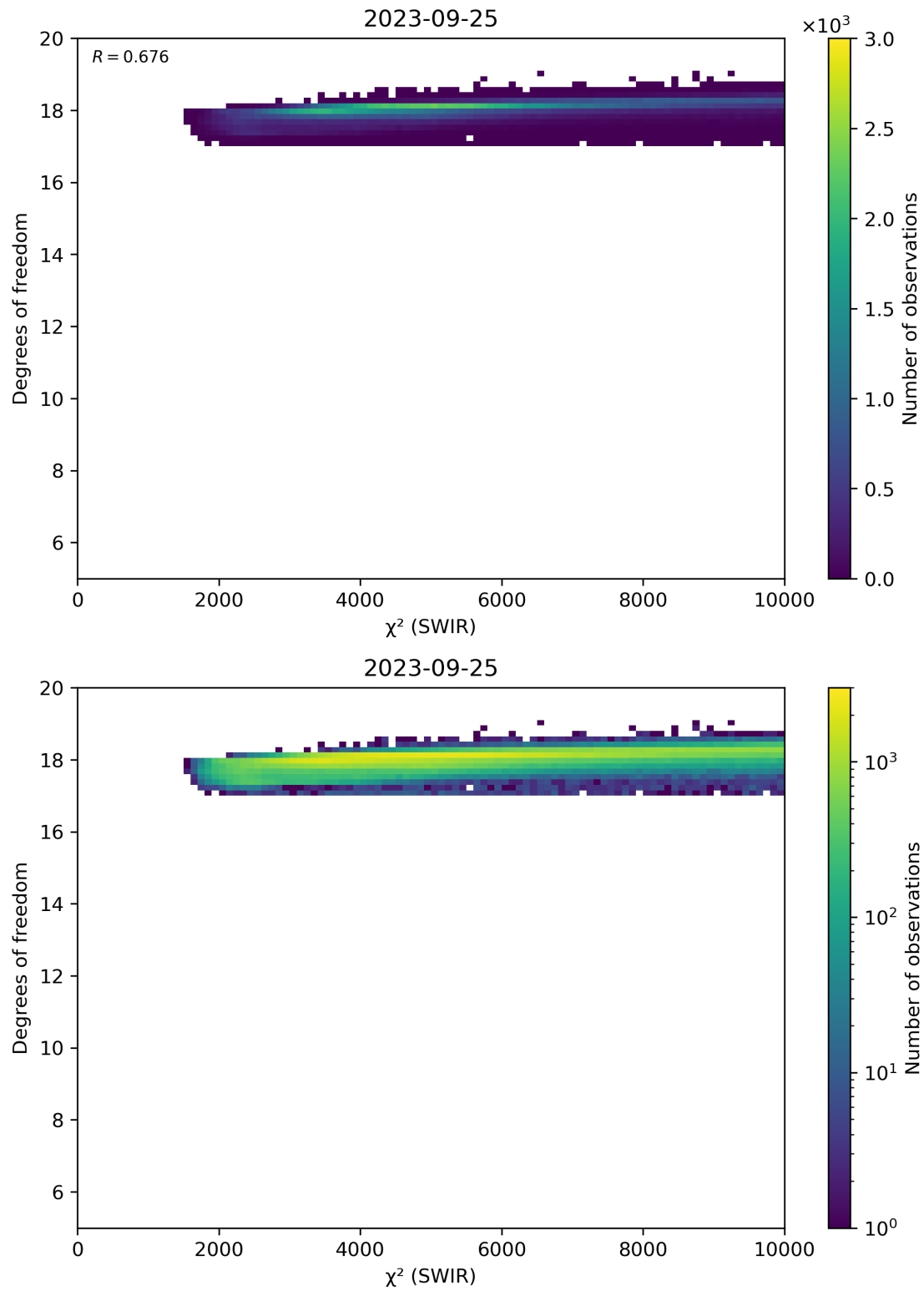
Figure 48: Scatter density plot of “ \chi^2 (SWIR)” against “Degrees of freedom” for 2023-09-24 to 2023-09-26.
