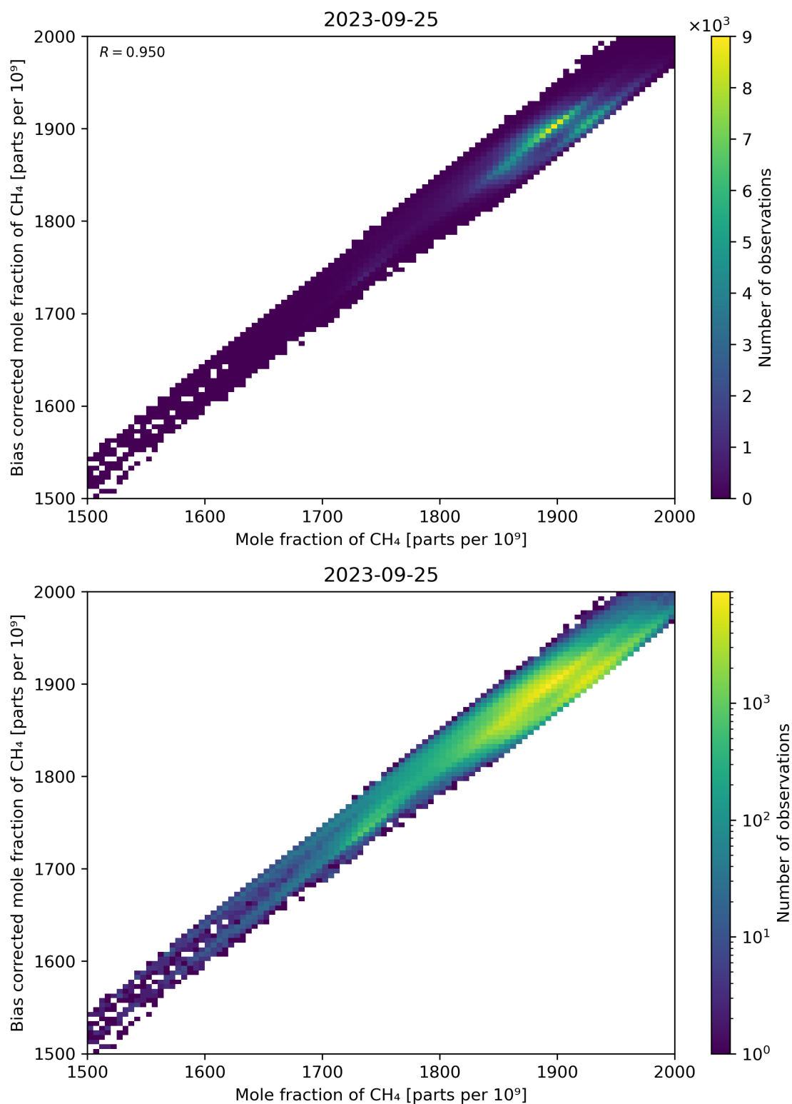
Figure 74: Scatter density plot of “Mole fraction of CH 4 ” against “Bias corrected mole fraction of CH 4 ” for 2023-09-24 to 2023-09-26.
