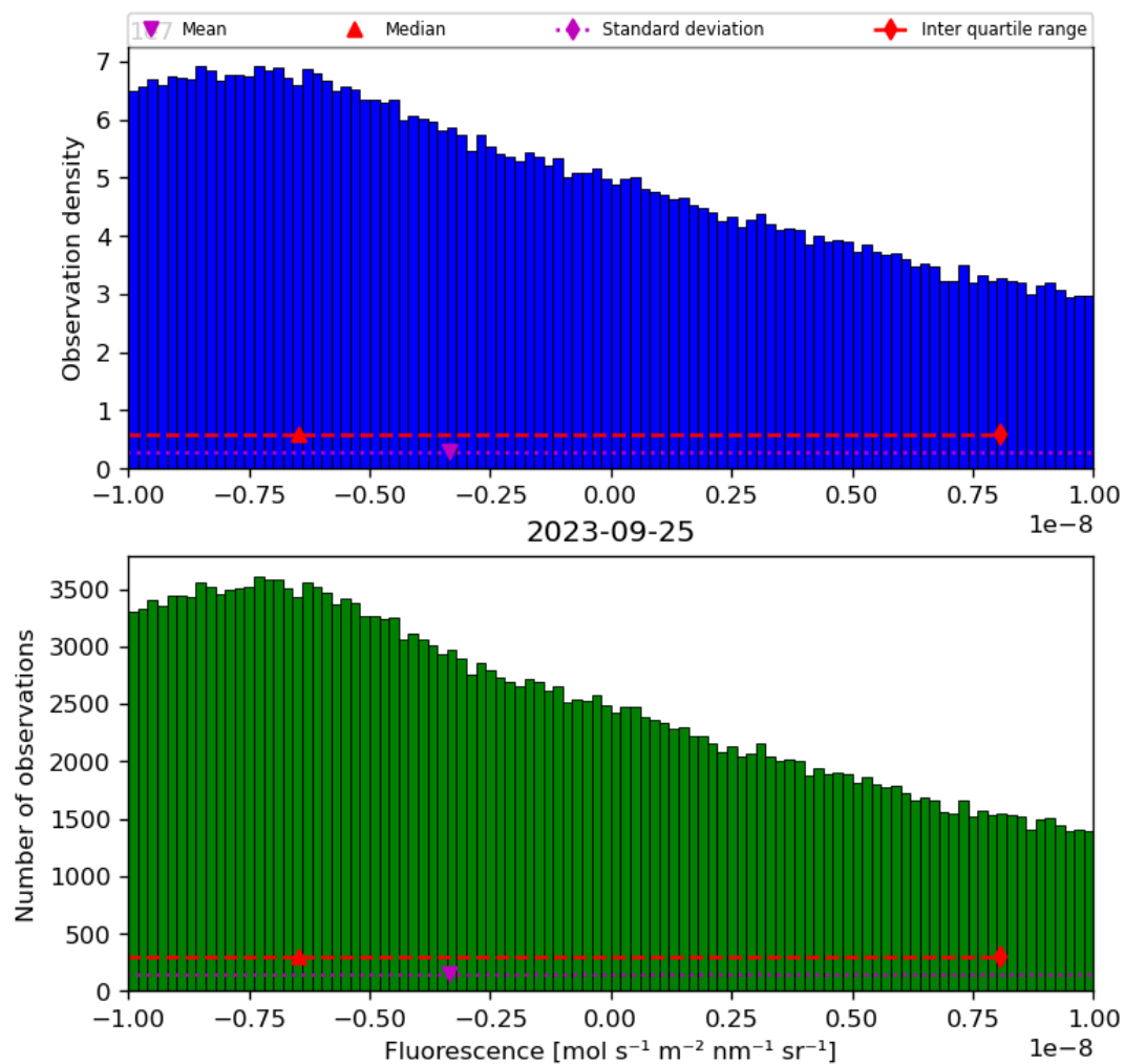
Figure 32: Histogram of “Fluorescence” for 2023-09-24 to 2023-09-26
