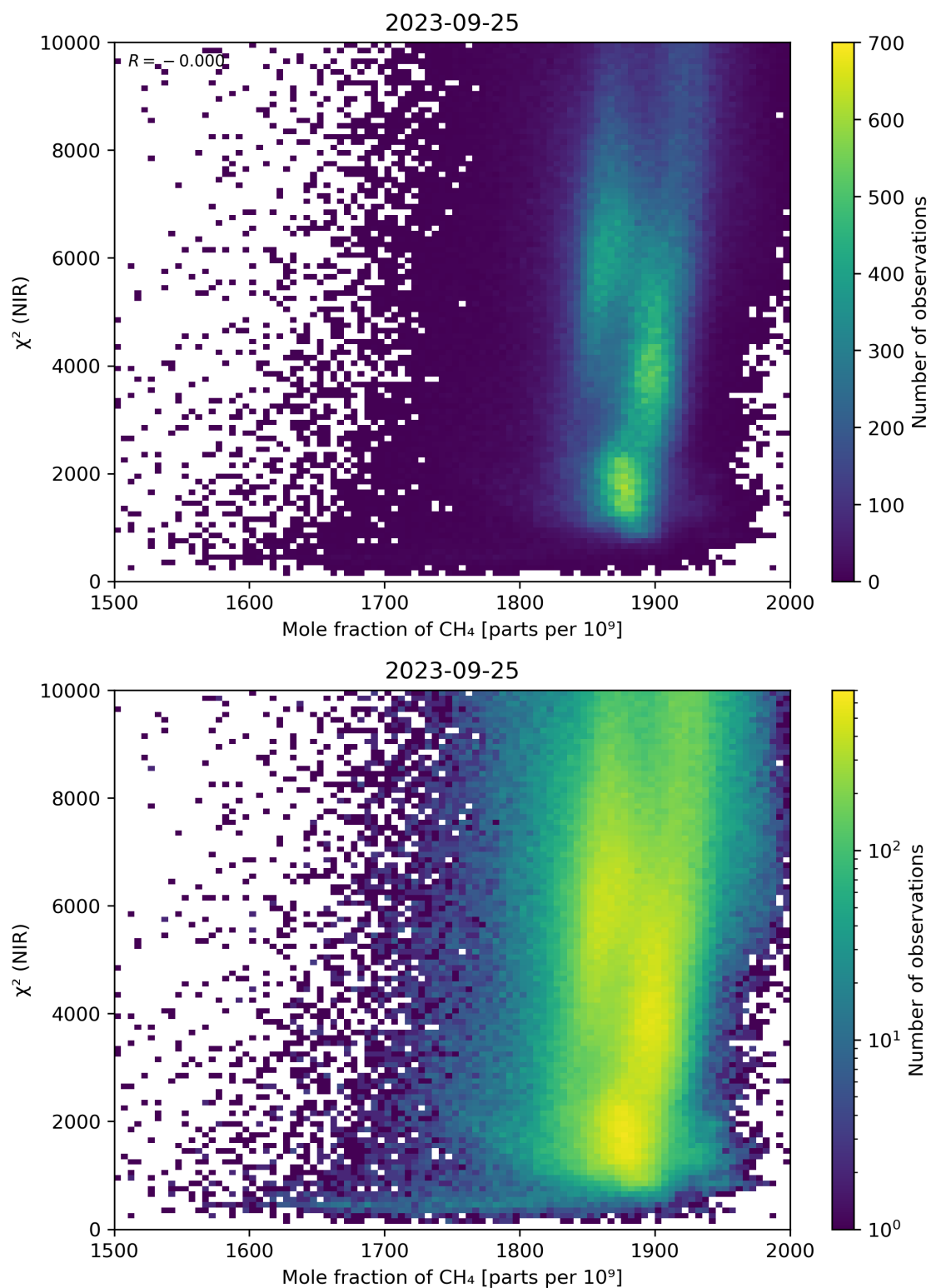
Figure 70: Scatter density plot of “Mole fraction of CH 4 ” against “ \chi^2 (NIR)” for 2023-09-24 to 2023-09-26.
