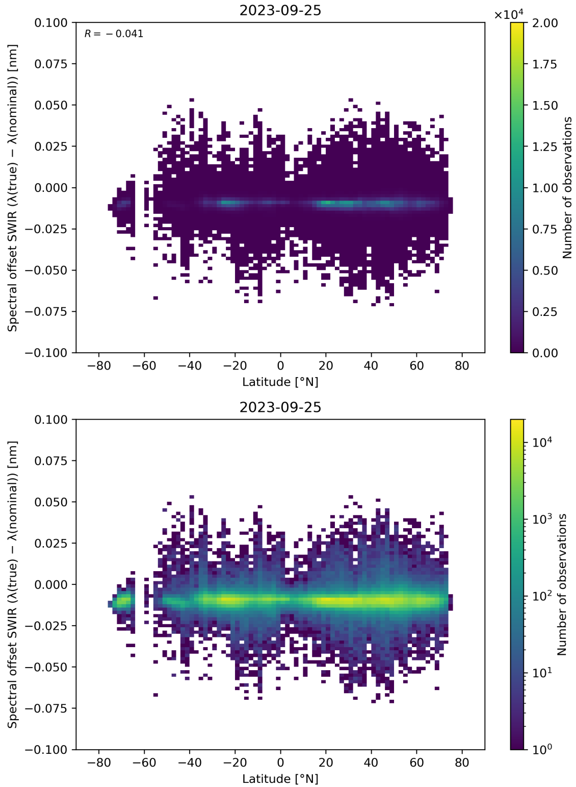
Figure 62: Scatter density plot of “Latitude” against “Spectral offset SWIR ( \lambda(\text{true}) - \lambda(\text{nominal}) )” for 2023-09-24 to 2023-09-26.
