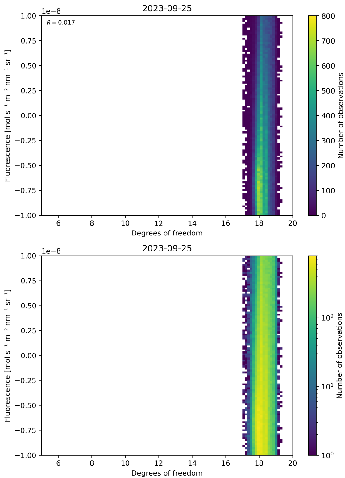
Figure 51: Scatter density plot of “Degrees of freedom” against “Fluorescence” for 2023-09-24 to 2023-09-26.
