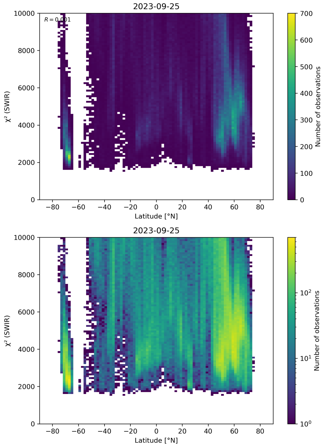
Figure 54: Scatter density plot of “Latitude” against “ \chi^2 (SWIR)” for 2023-09-24 to 2023-09-26.
