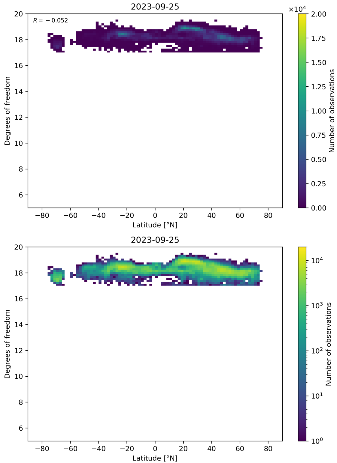
Figure 55: Scatter density plot of “Latitude” against “Degrees of freedom” for 2023-09-24 to 2023-09-26.
