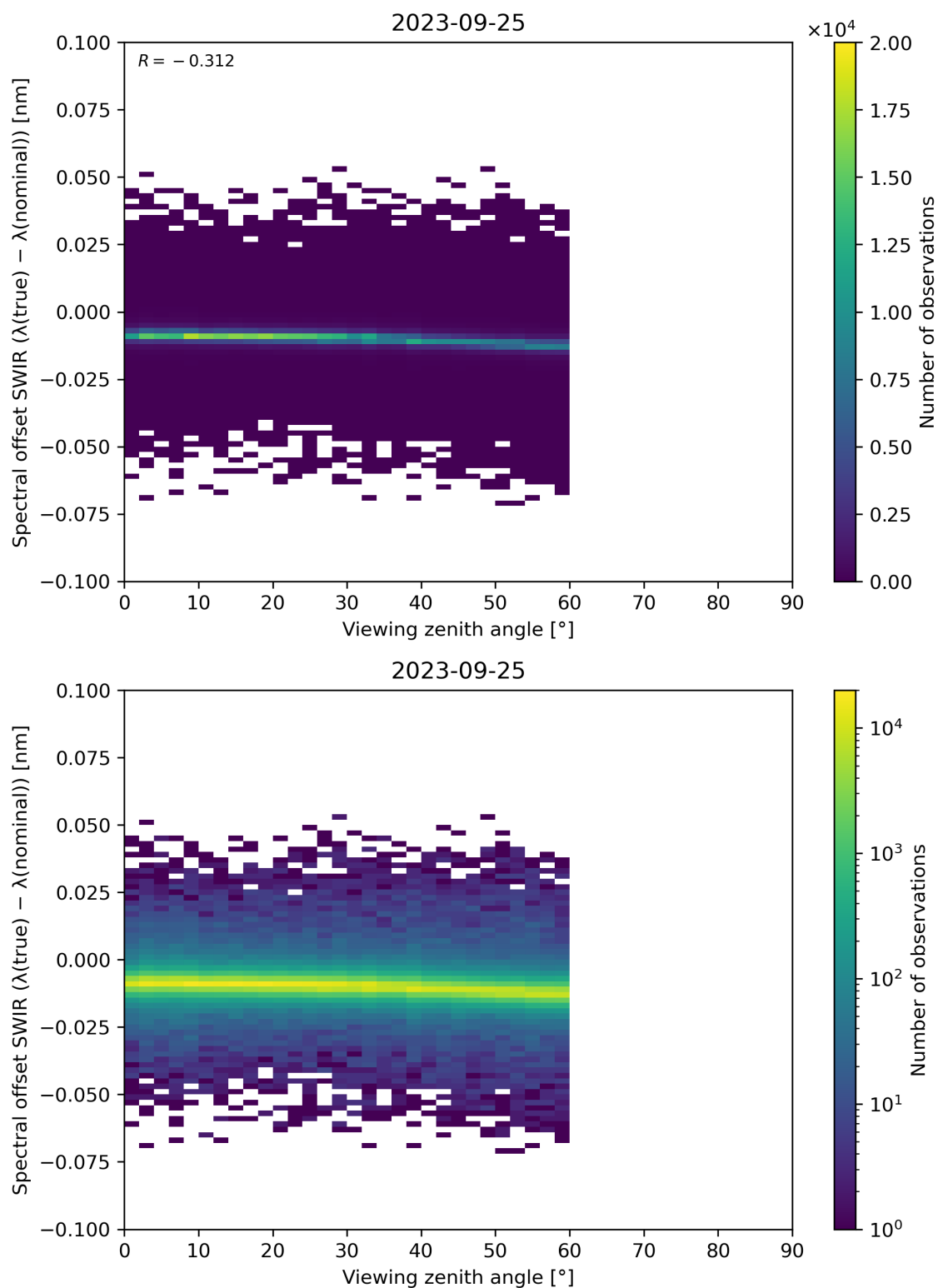
Figure 116: Scatter density plot of “Viewing zenith angle” against “Spectral offset SWIR ( \lambda(\text{true}) - \lambda(\text{nominal}) )” for 2023-09-24 to 2023-09-26.
