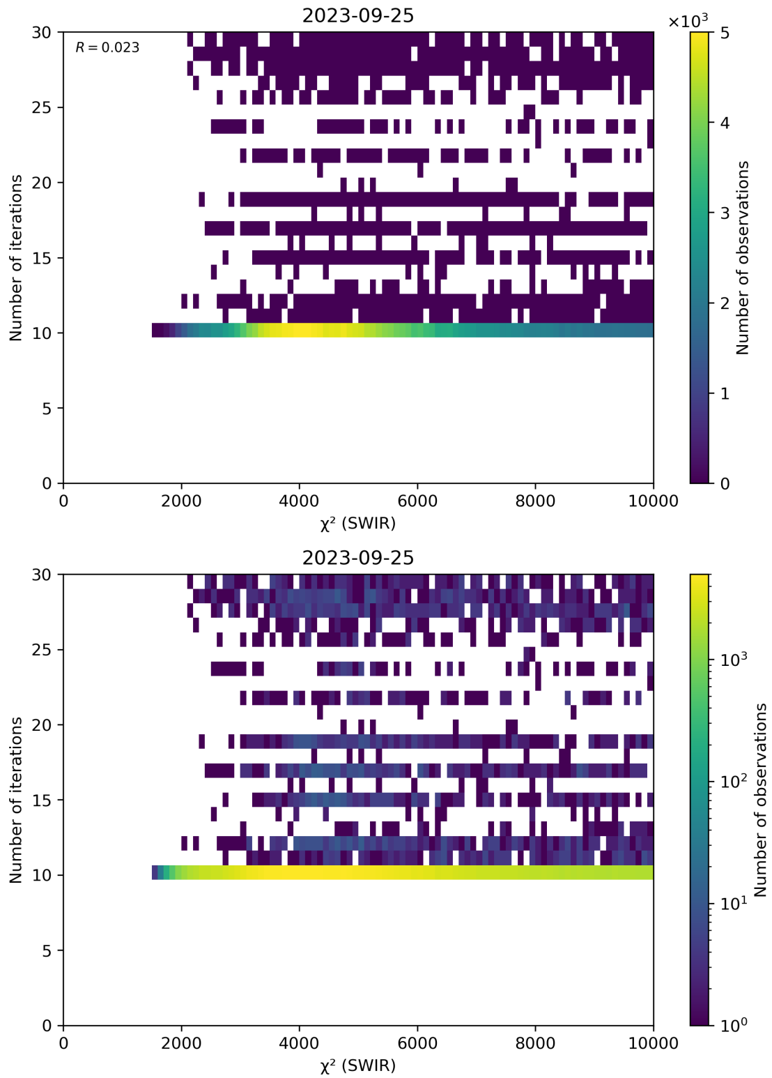
Figure 50: Scatter density plot of “ \chi^2 (SWIR)” against “Number of iterations” for 2023-09-24 to 2023-09-26.
