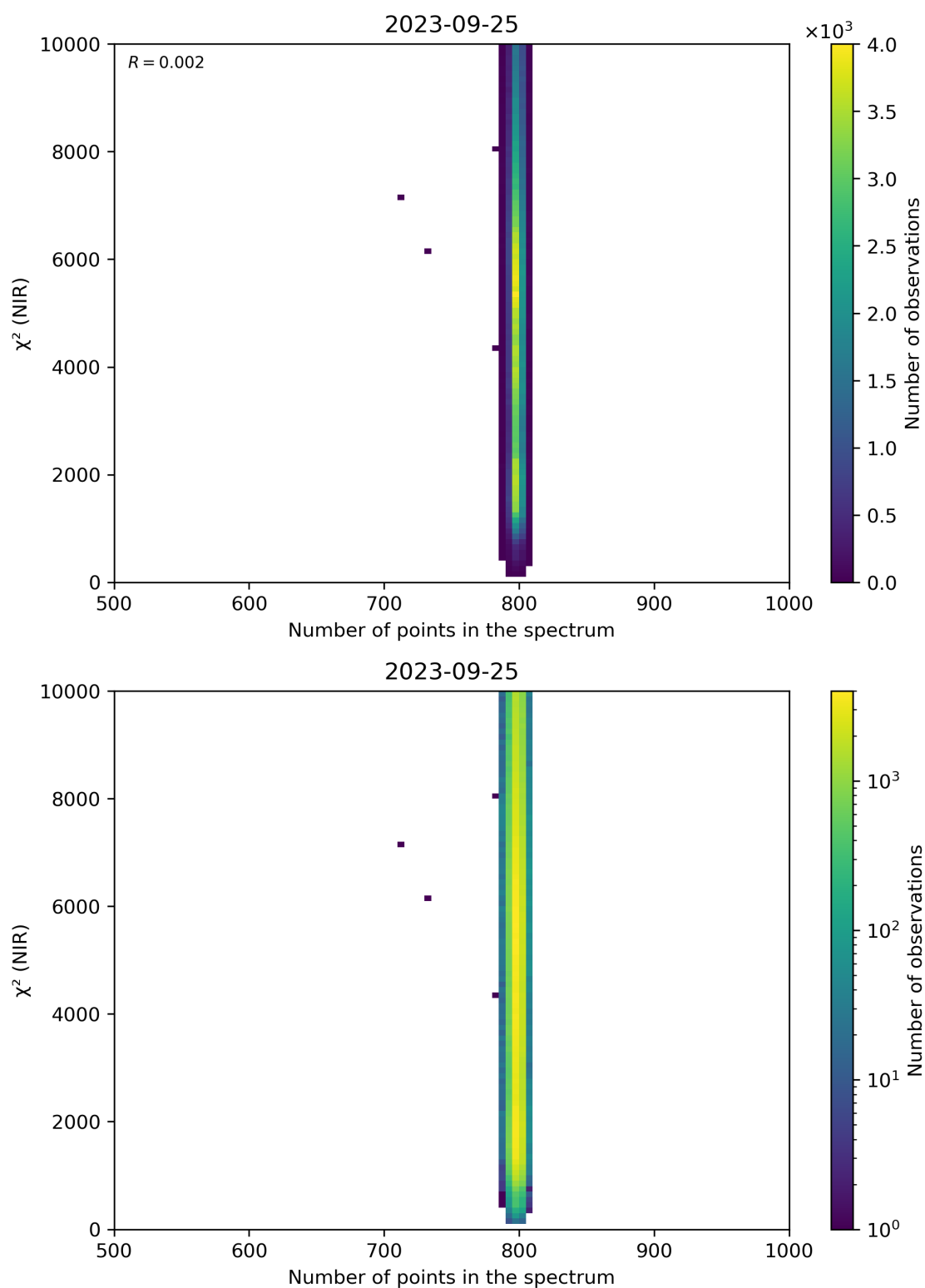
Figure 88: Scatter density plot of “Number of points in the spectrum” against “ \chi^2 (NIR)” for 2023-09-24 to 2023-09-26.
