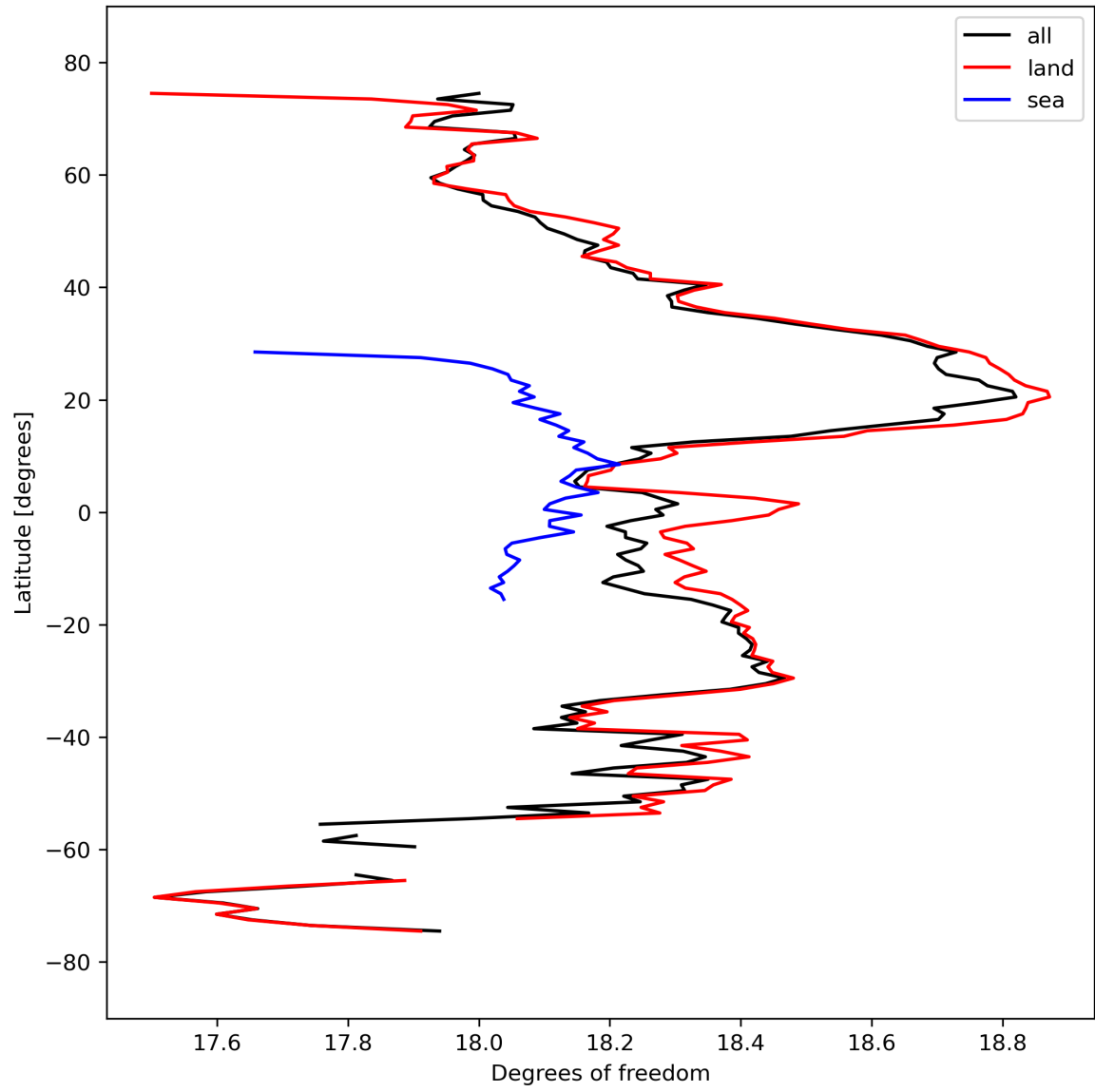
Figure 19: Zonal average of “Degrees of freedom” for 2023-09-24 to 2023-09-26.
