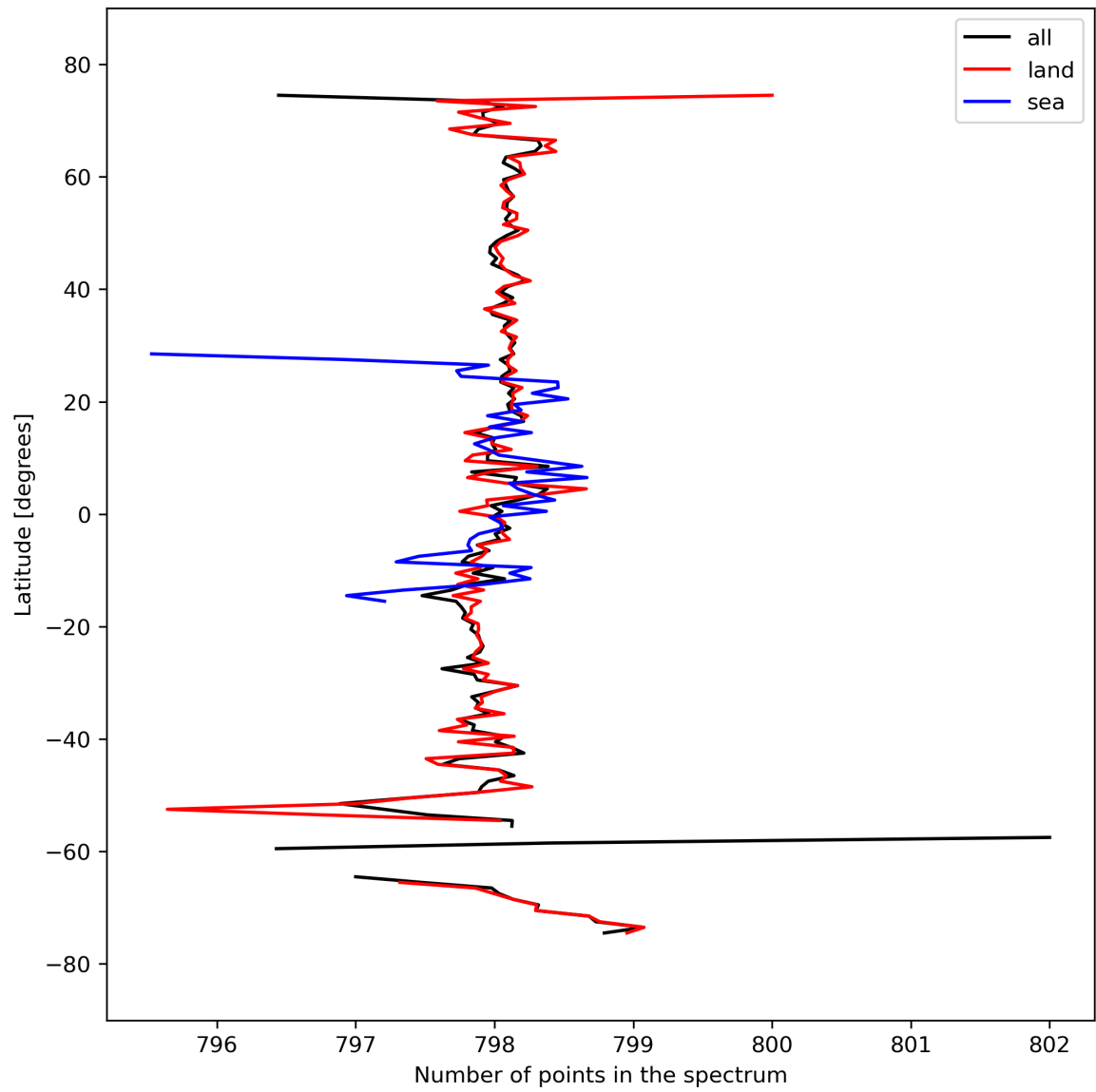
Figure 15: Zonal average of “Number of points in the spectrum” for 2023-09-24 to 2023-09-26.
