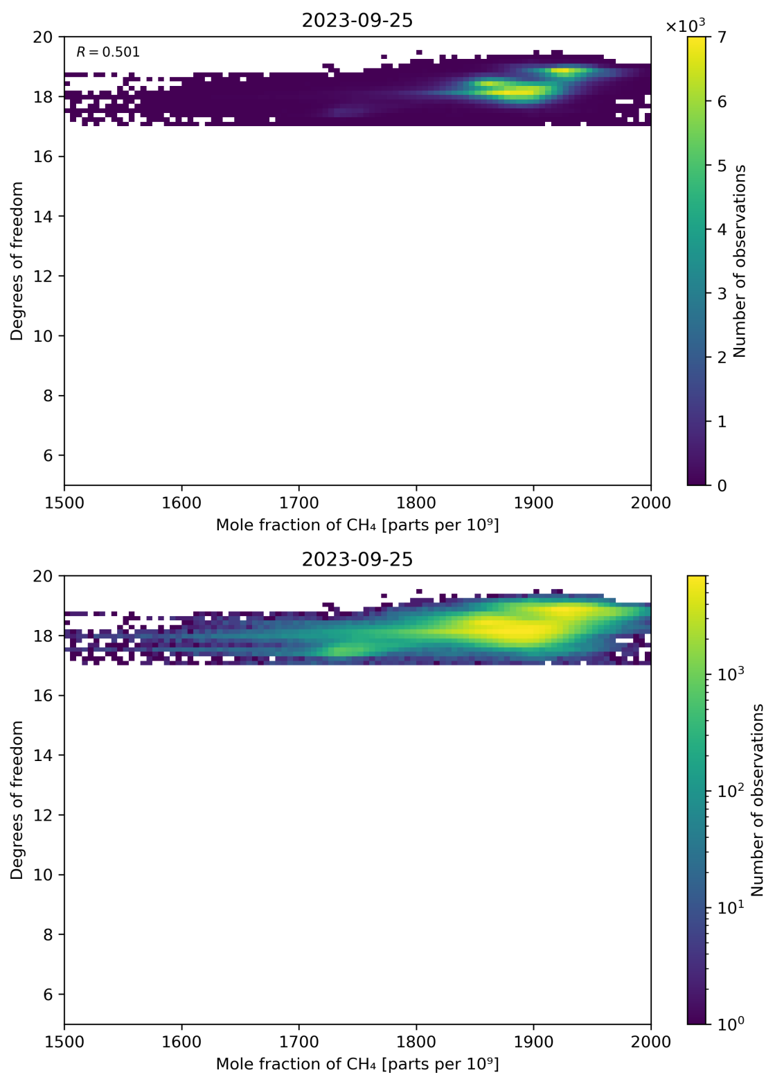
Figure 72: Scatter density plot of “Mole fraction of CH 4 ” against “Degrees of freedom” for 2023-09-24 to 2023-09-26.
