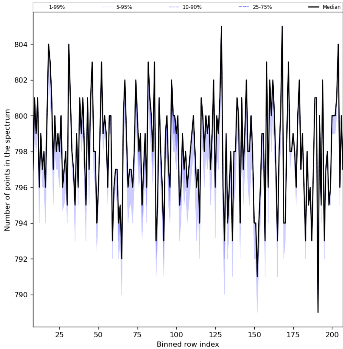
Figure 37: Along track statistics of “Number of points in the spectrum” for 2023-09-24 to 2023-09-26
