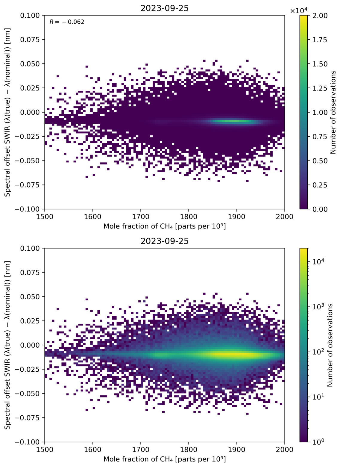
Figure 86: Scatter density plot of “Mole fraction of CH 4 ” against “Spectral offset SWIR ( \lambda(\text{true}) - \lambda(\text{nominal}) )” for 2023-09-24 to 2023-09-26.
