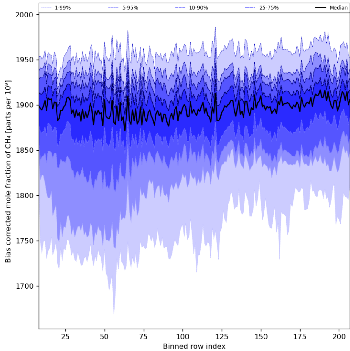
Figure 36: Along track statistics of “Bias corrected mole fraction of CH 4 ” for 2023-09-24 to 2023-09-26
