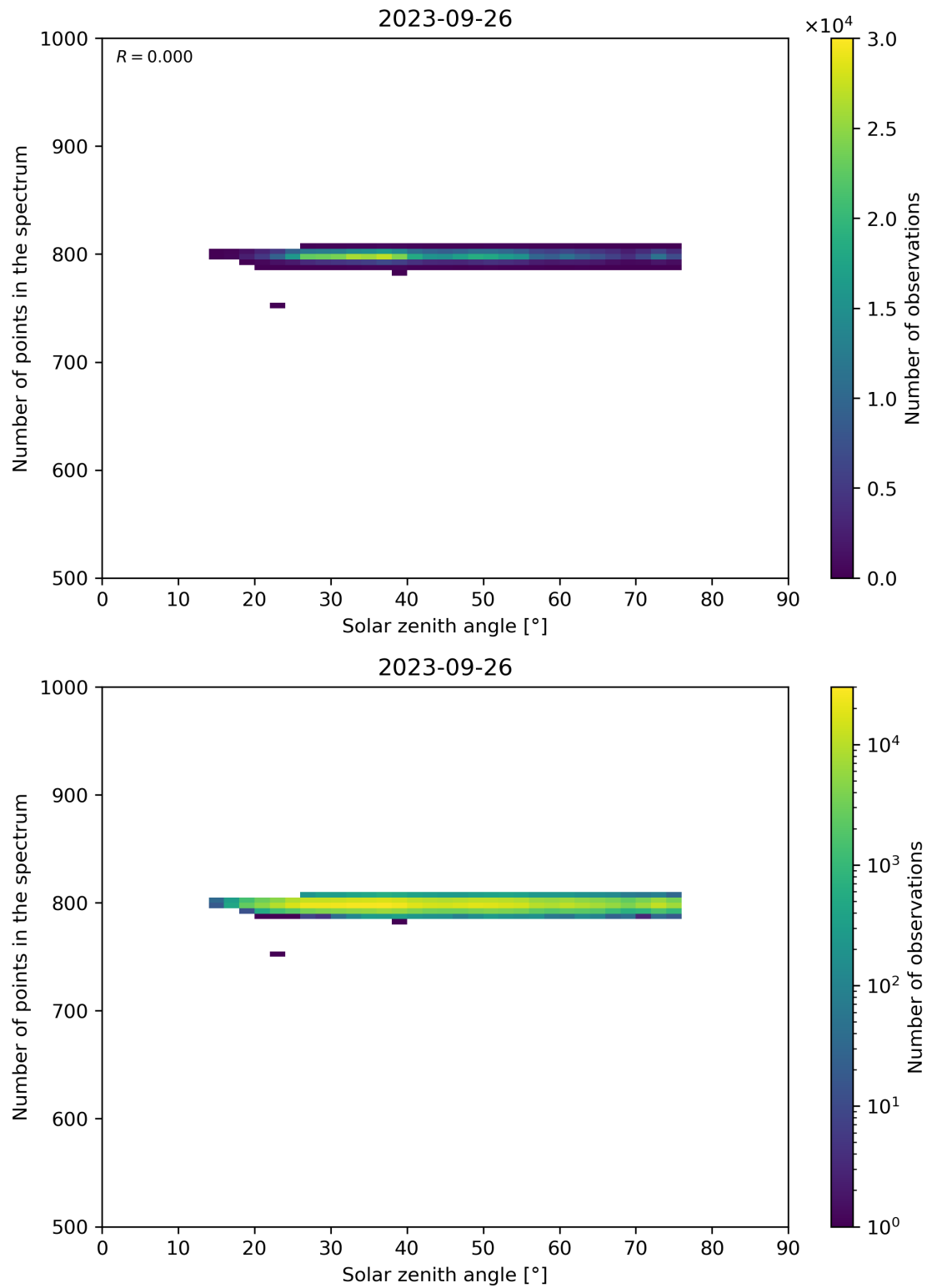
Figure 103: Scatter density plot of “Solar zenith angle” against “Number of points in the spectrum” for 2023-09-26 to 2023-09-27.
