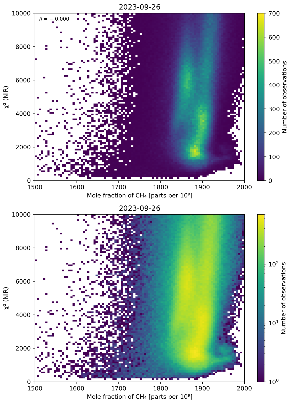
Figure 70: Scatter density plot of “Mole fraction of CH 4 ” against “ \chi^2 (NIR)” for 2023-09-26 to 2023-09-27.
