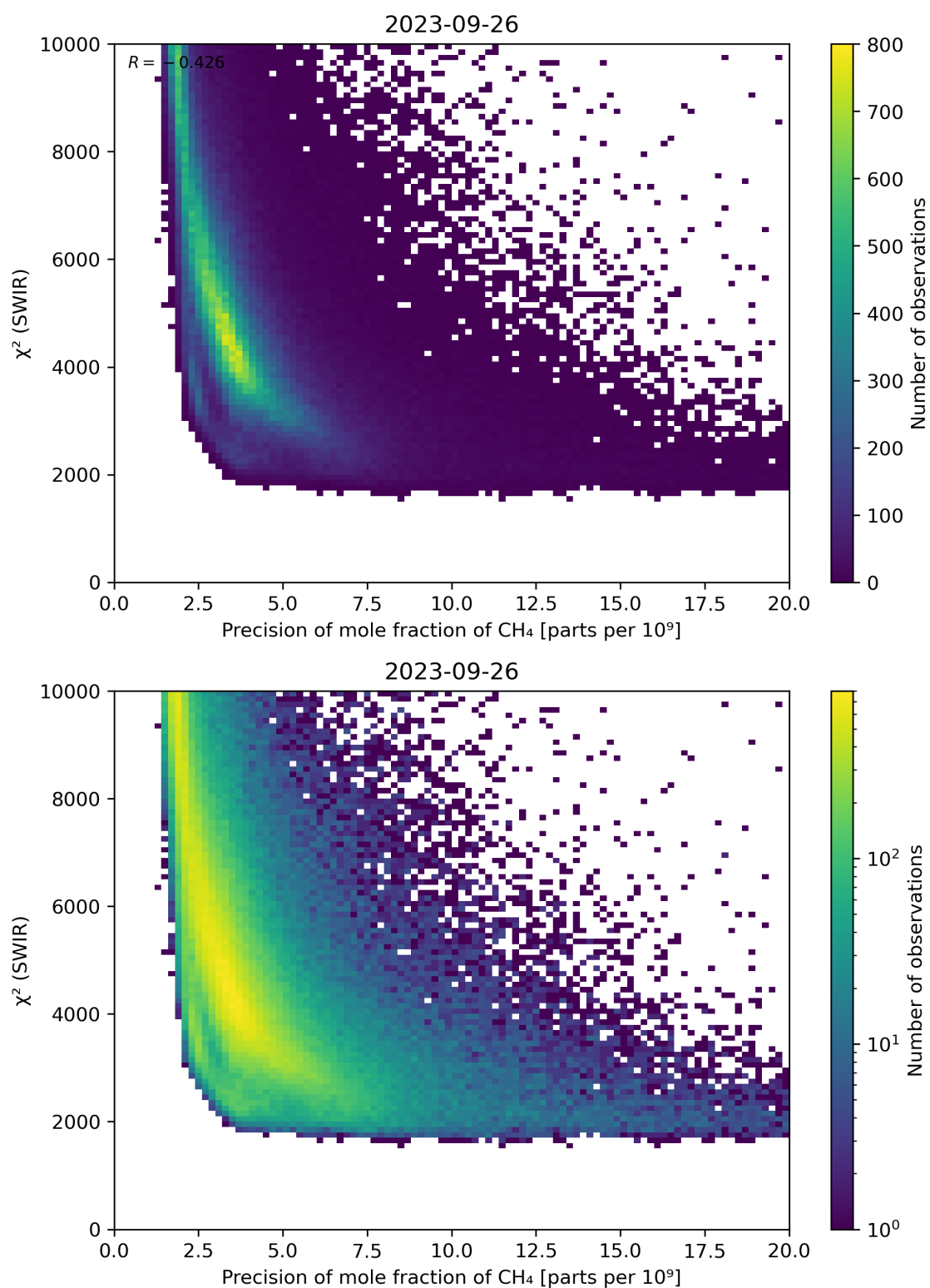
Figure 79: Scatter density plot of “Precision of mole fraction of \text{CH}_4 ” against “ \chi^2 (SWIR)” for 2023-09-26 to 2023-09-27.
