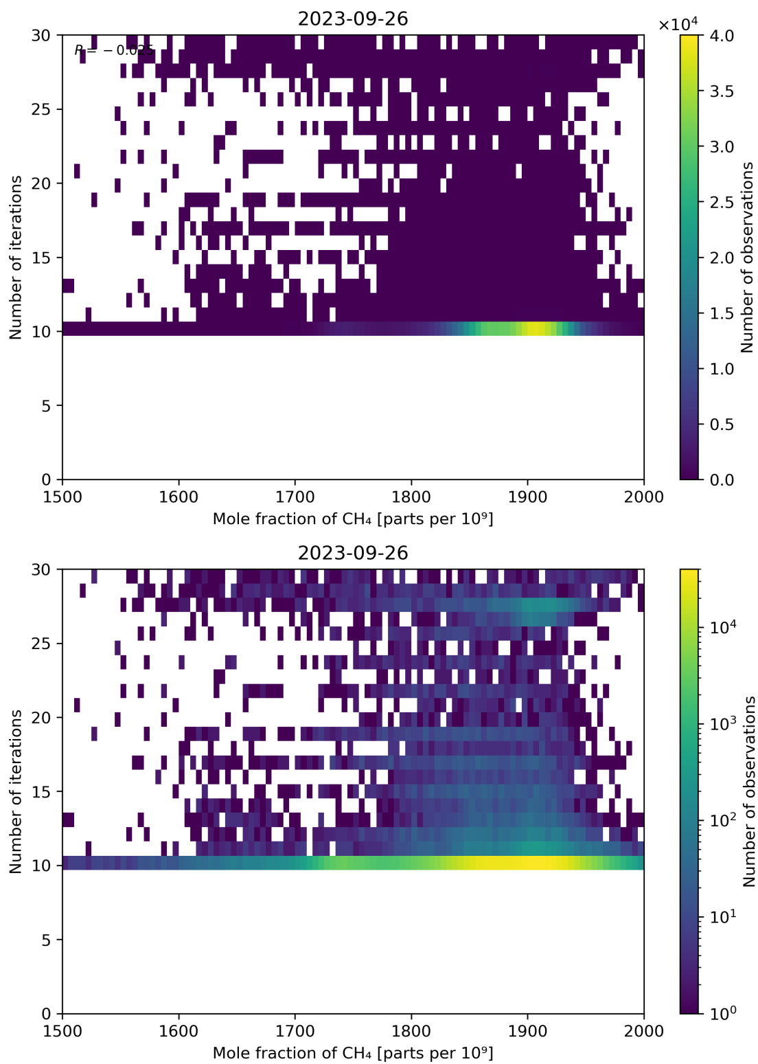
Figure 76: Scatter density plot of “Mole fraction of CH 4 ” against “Number of iterations” for 2023-09-26 to 2023-09-27.
