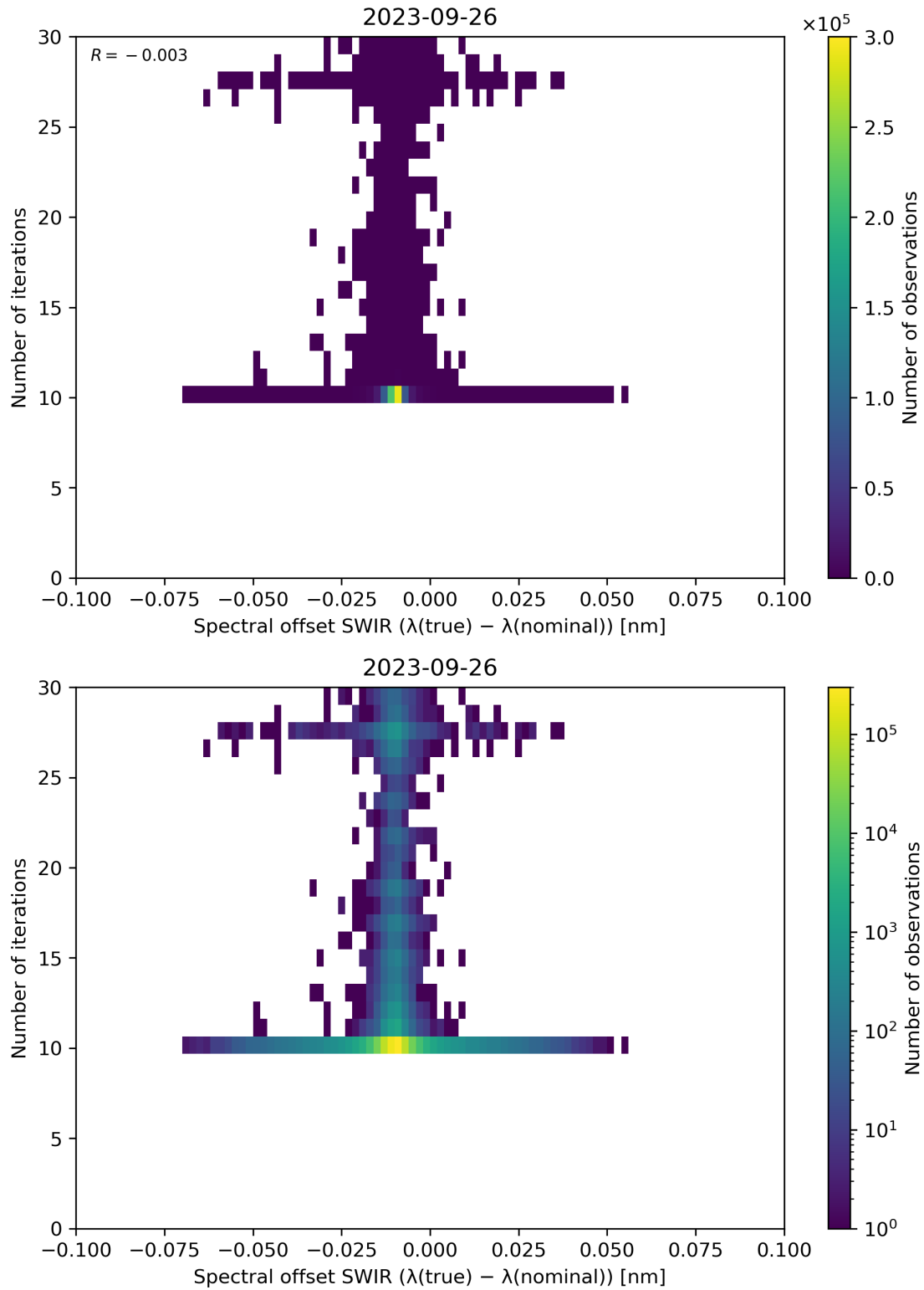
Figure 121: Scatter density plot of “Spectral offset SWIR ( \lambda(\text{true}) - \lambda(\text{nominal}) )” against “Number of iterations” for 2023-09-26 to 2023-09-27.
