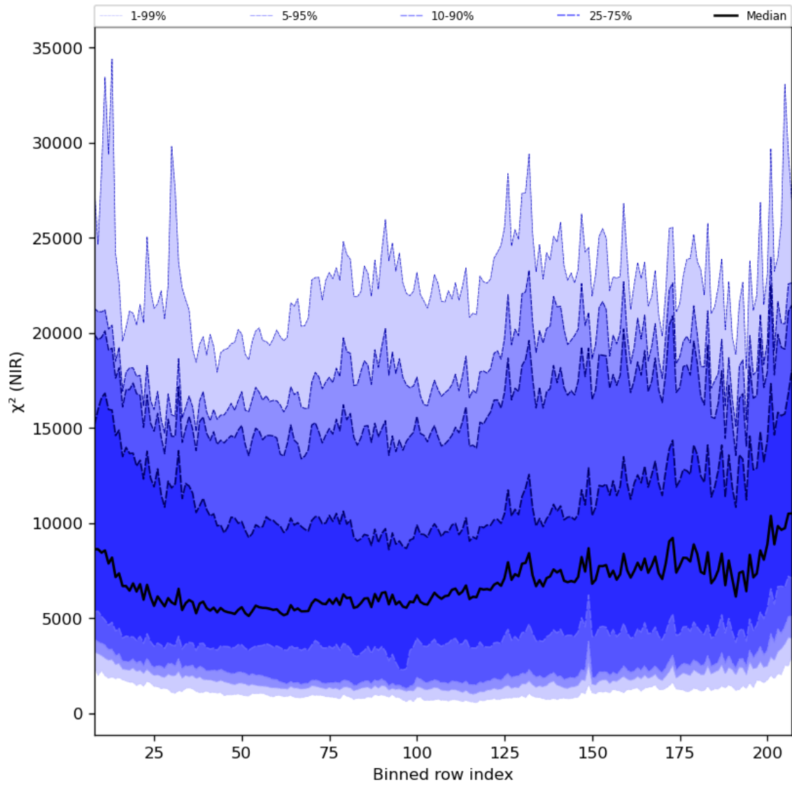
Figure 40: Along track statistics of “ \chi^2 (NIR)” for 2023-09-26 to 2023-09-27
