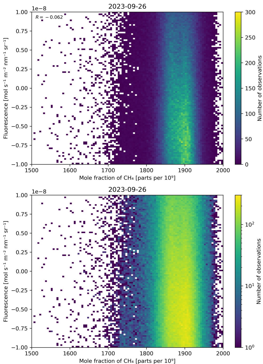
Figure 73: Scatter density plot of “Mole fraction of \text{CH}_4 ” against “Fluorescence” for 2023-09-26 to 2023-09-27.
