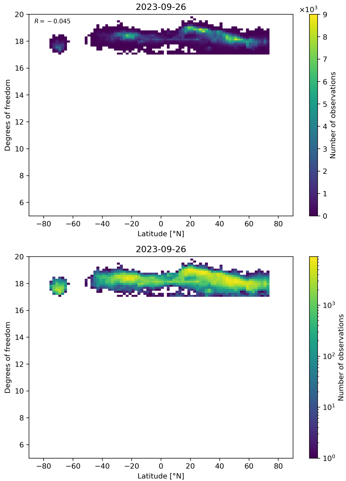
Figure 55: Scatter density plot of “Latitude” against “Degrees of freedom” for 2023-09-26 to 2023-09-27.
