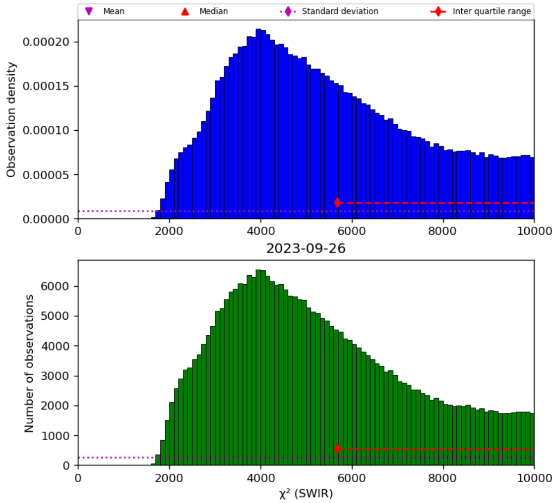
Figure 28: Histogram of “ \chi^2 (SWIR)” for 2023-09-26 to 2023-09-27
