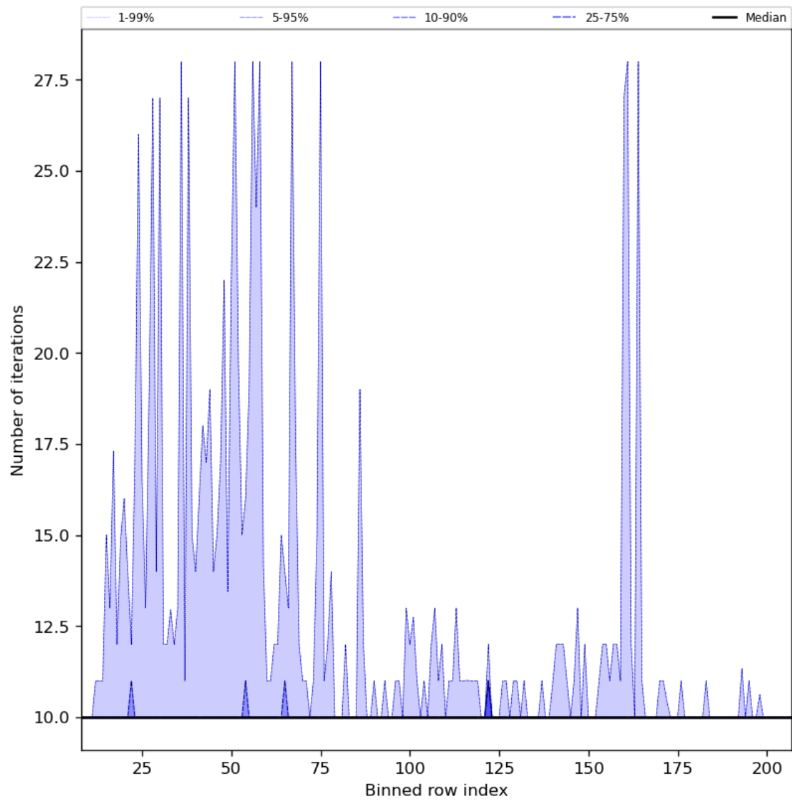
Figure 42: Along track statistics of “Number of iterations” for 2023-09-26 to 2023-09-27
