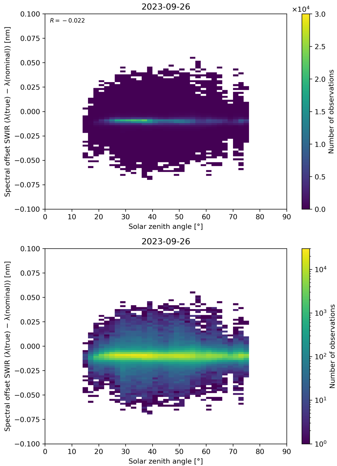
Figure 104: Scatter density plot of “Solar zenith angle” against “Spectral offset SWIR ( \lambda(\text{true}) - \lambda(\text{nominal}) )” for 2023-09-26 to 2023-09-27.
