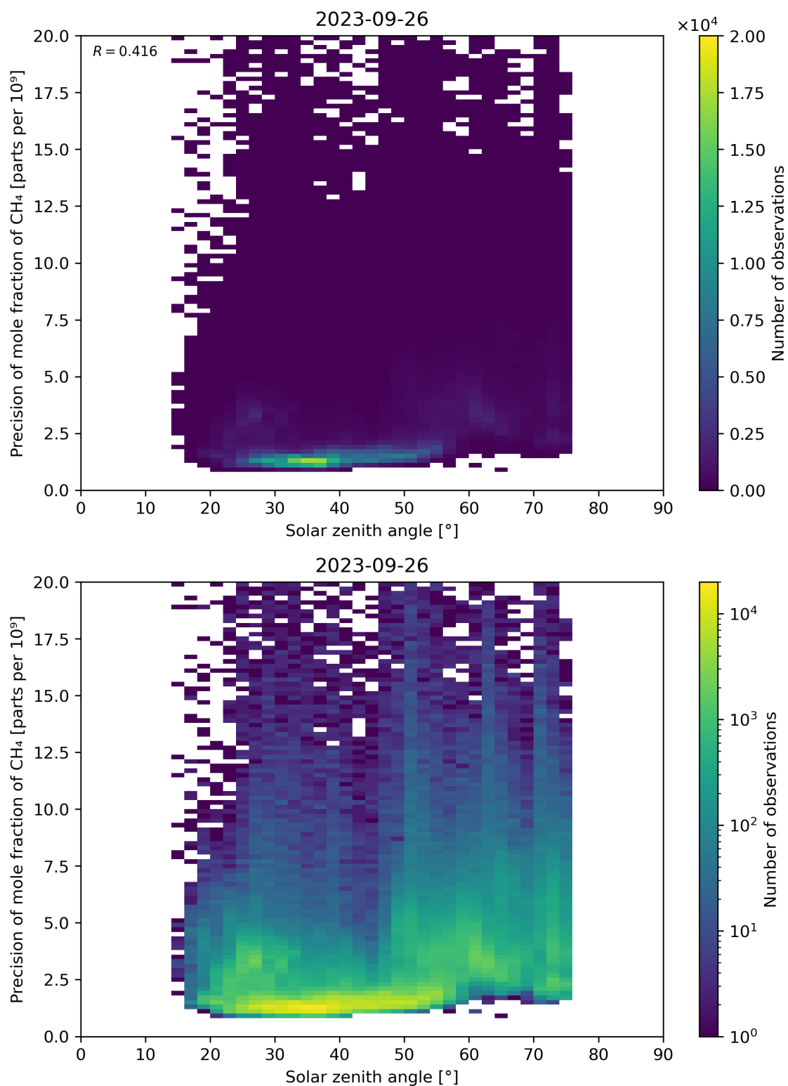
Figure 101: Scatter density plot of “Solar zenith angle” against “Precision of mole fraction of CH 4 ” for 2023-09-26 to 2023-09-27.
