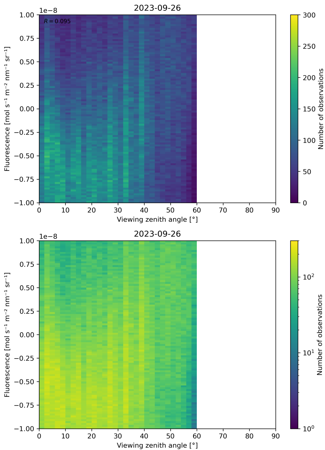
Figure 108: Scatter density plot of “Viewing zenith angle” against “Fluorescence” for 2023-09-26 to 2023-09-27.
