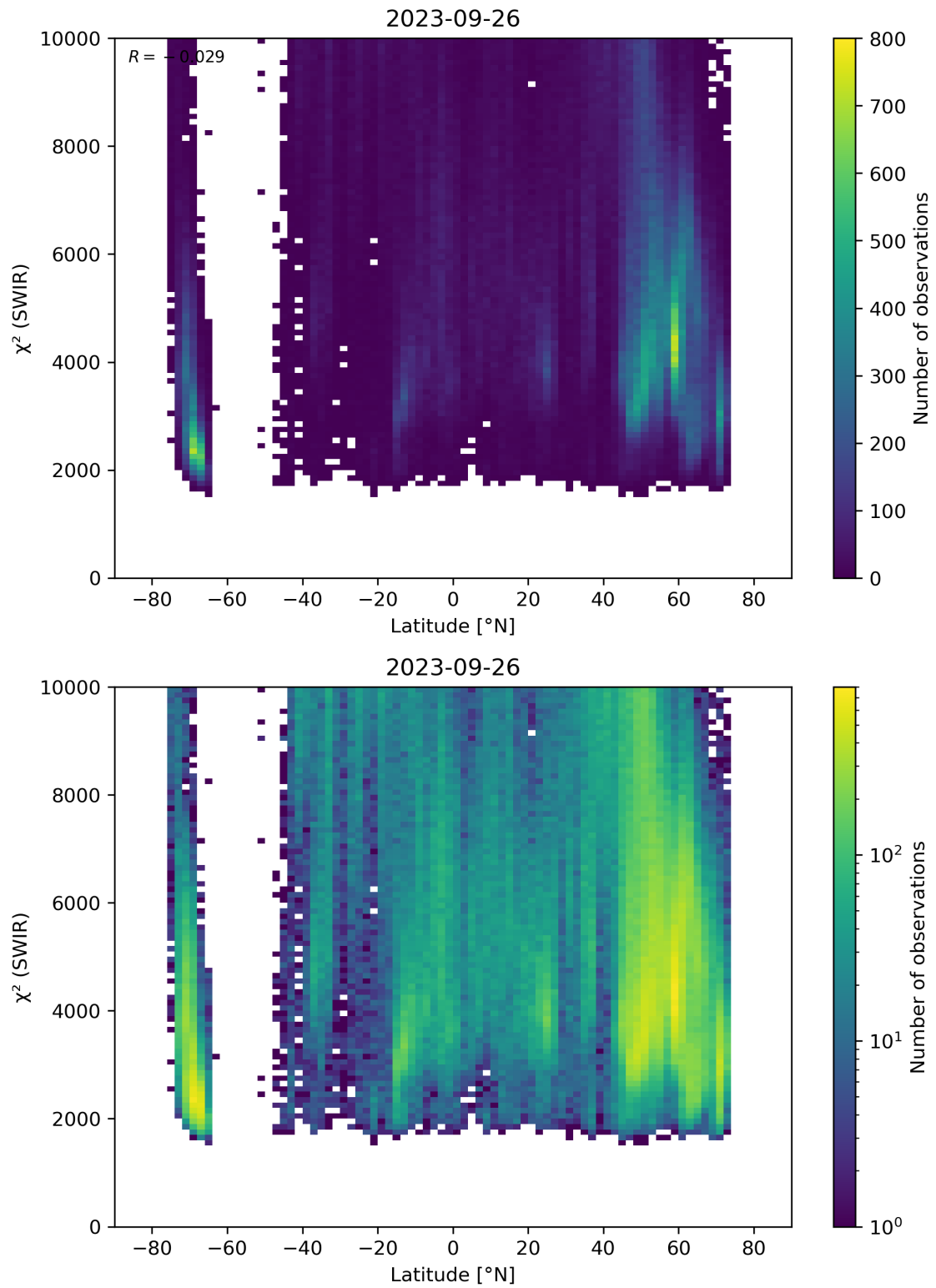
Figure 54: Scatter density plot of “Latitude” against “ \chi^2 (SWIR)” for 2023-09-26 to 2023-09-27.
