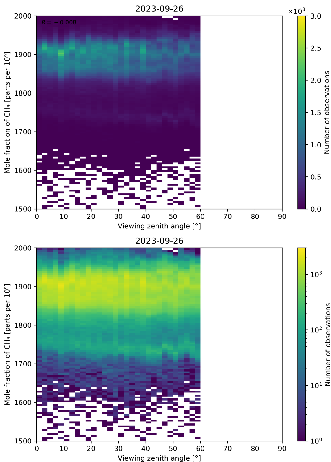
Figure 110: Scatter density plot of “Viewing zenith angle” against “Mole fraction of CH 4 ” for 2023-09-26 to 2023-09-27.
