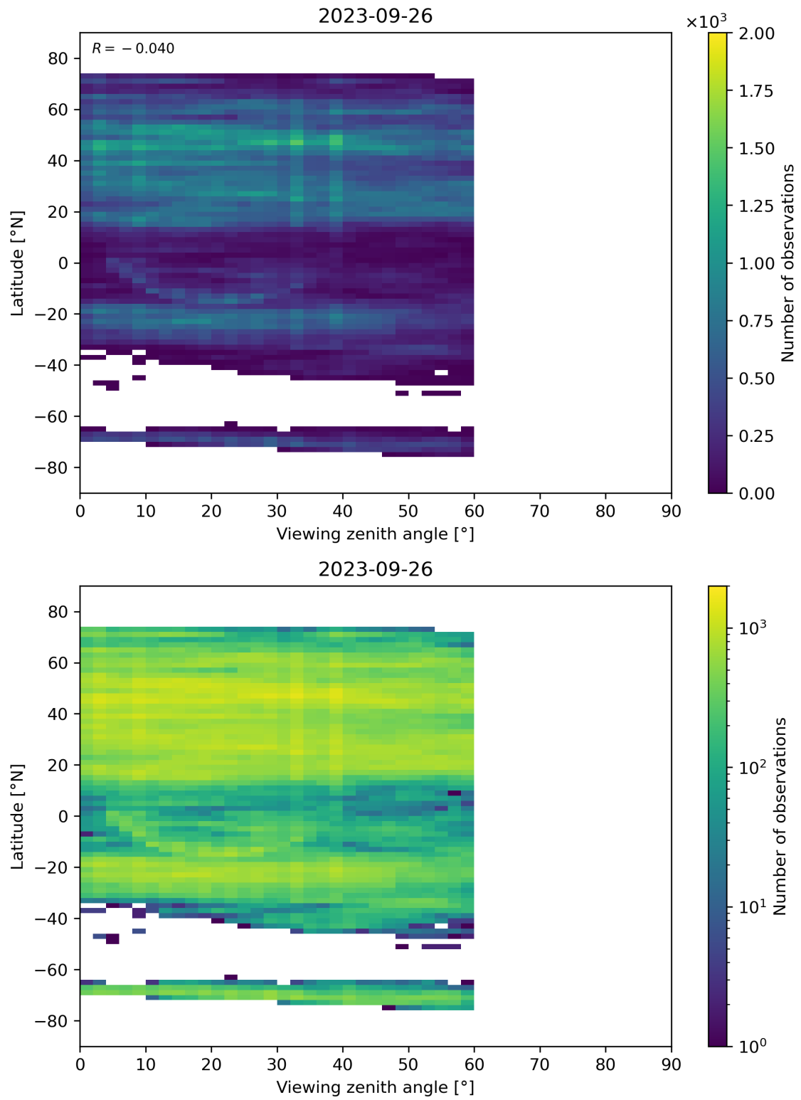
Figure 109: Scatter density plot of “Viewing zenith angle” against “Latitude” for 2023-09-26 to 2023-09-27.
