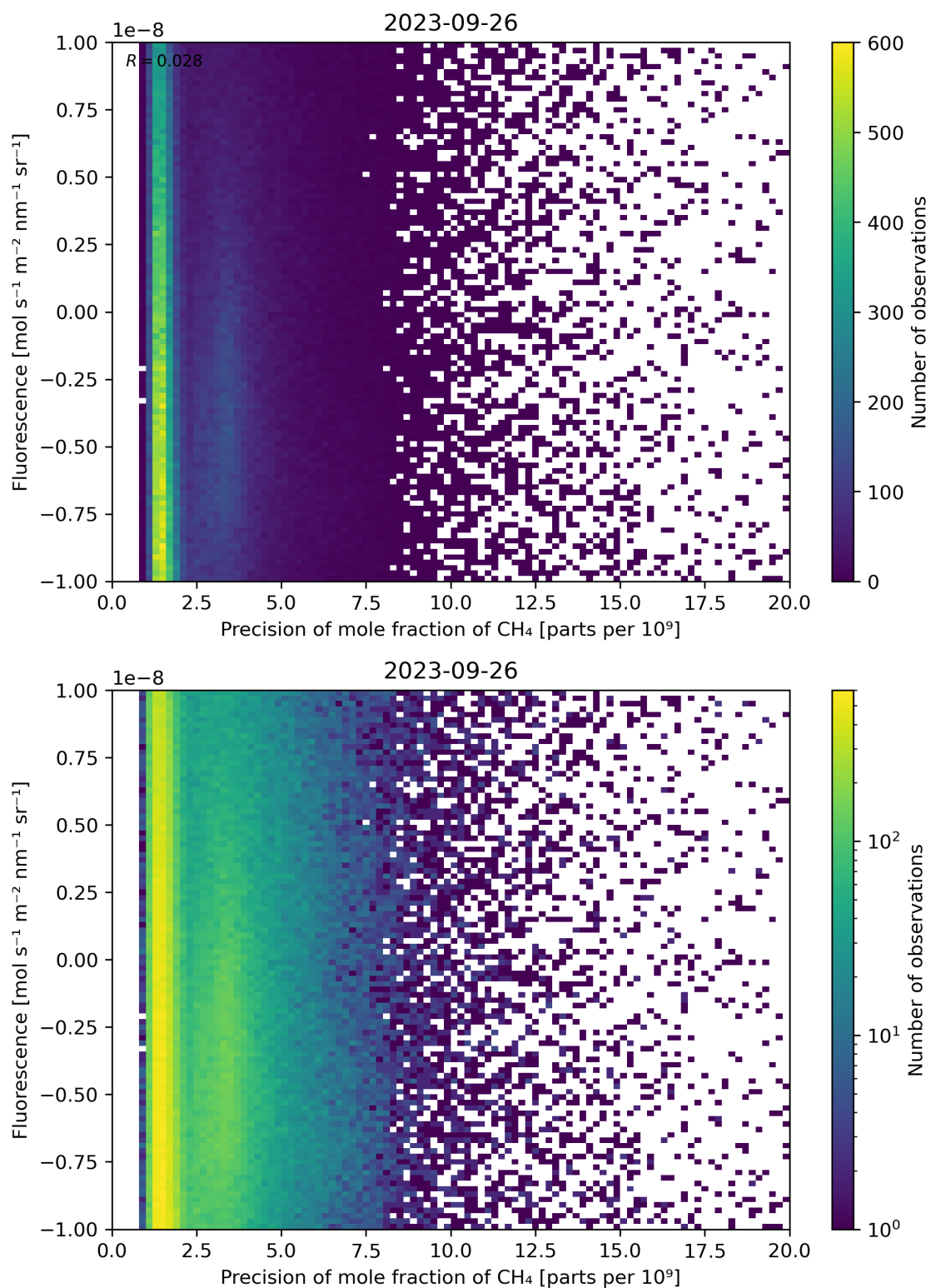
Figure 81: Scatter density plot of “Precision of mole fraction of \text{CH}_4 ” against “Fluorescence” for 2023-09-26 to 2023-09-27.
