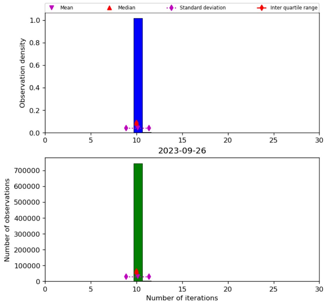
Figure 31: Histogram of “Number of iterations” for 2023-09-26 to 2023-09-27
