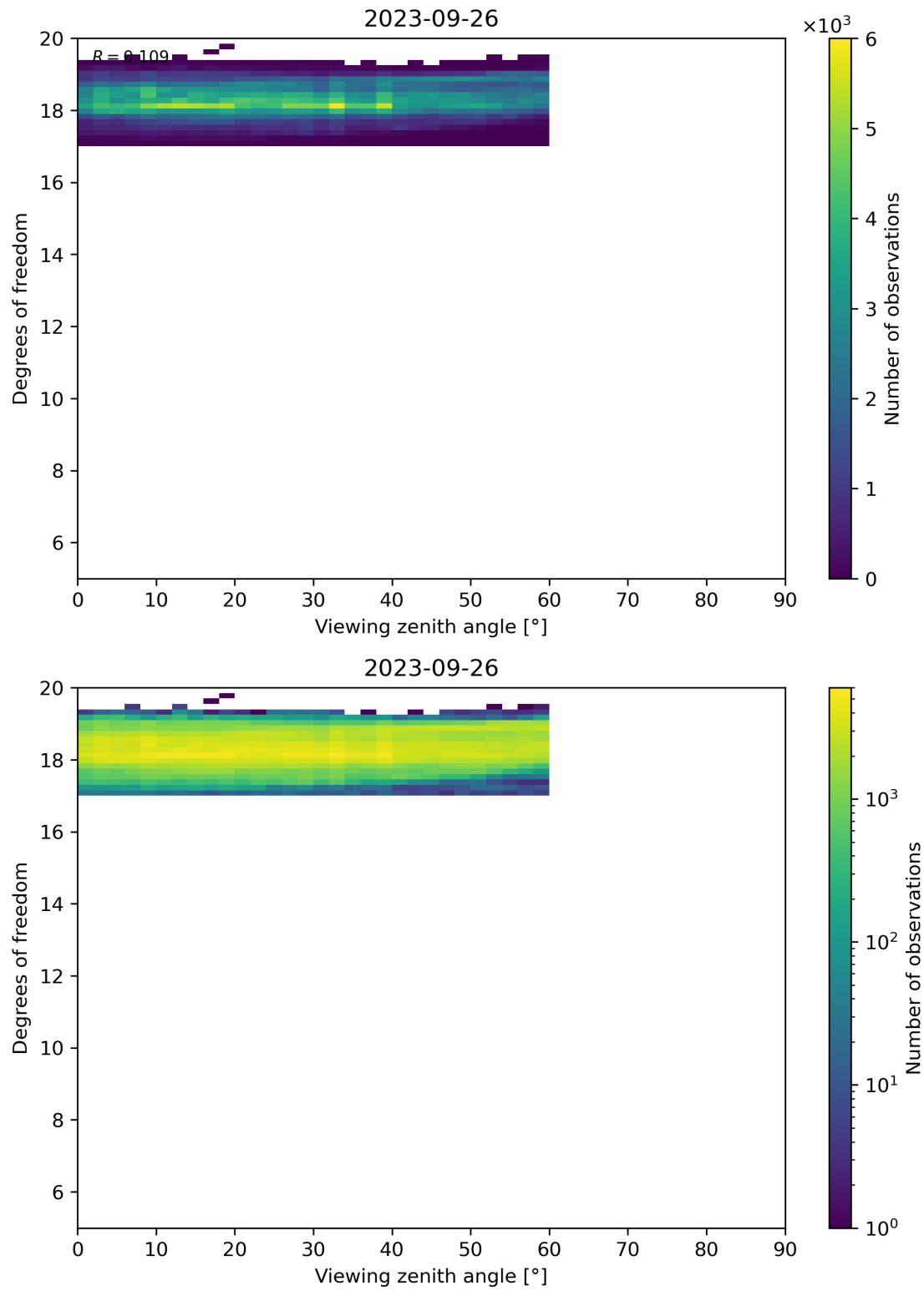
Figure 107: Scatter density plot of “Viewing zenith angle” against “Degrees of freedom” for 2023-09-26 to 2023-09-27.
