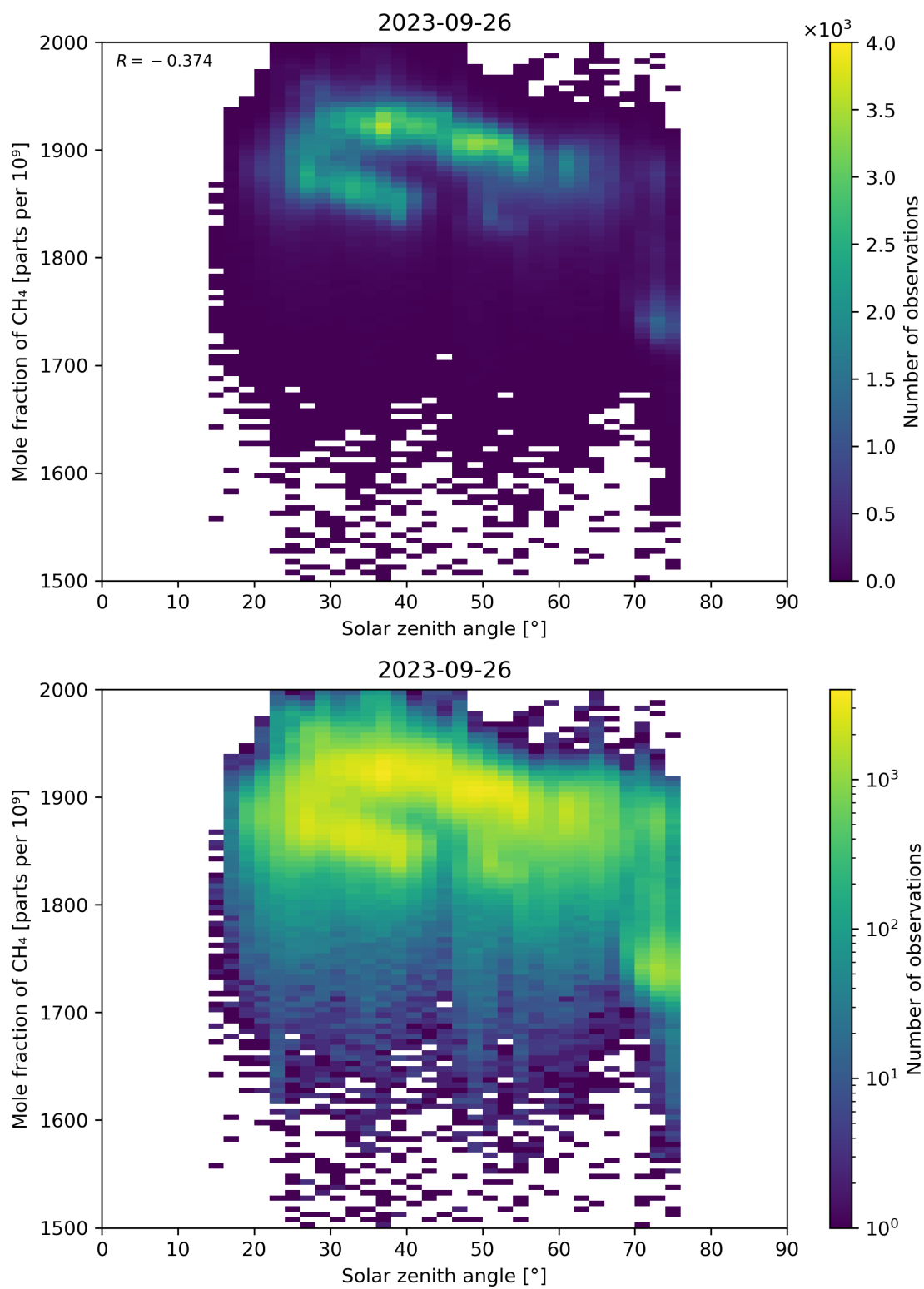
Figure 99: Scatter density plot of “Solar zenith angle” against “Mole fraction of \text{CH}_4 ” for 2023-09-26 to 2023-09-27.
