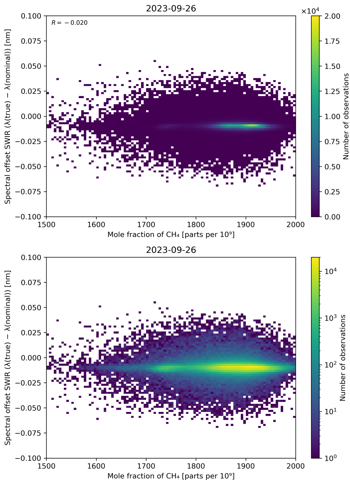
Figure 86: Scatter density plot of “Mole fraction of CH 4 ” against “Spectral offset SWIR ( \lambda(\text{true}) - \lambda(\text{nominal}) )” for 2023-09-26 to 2023-09-27.
