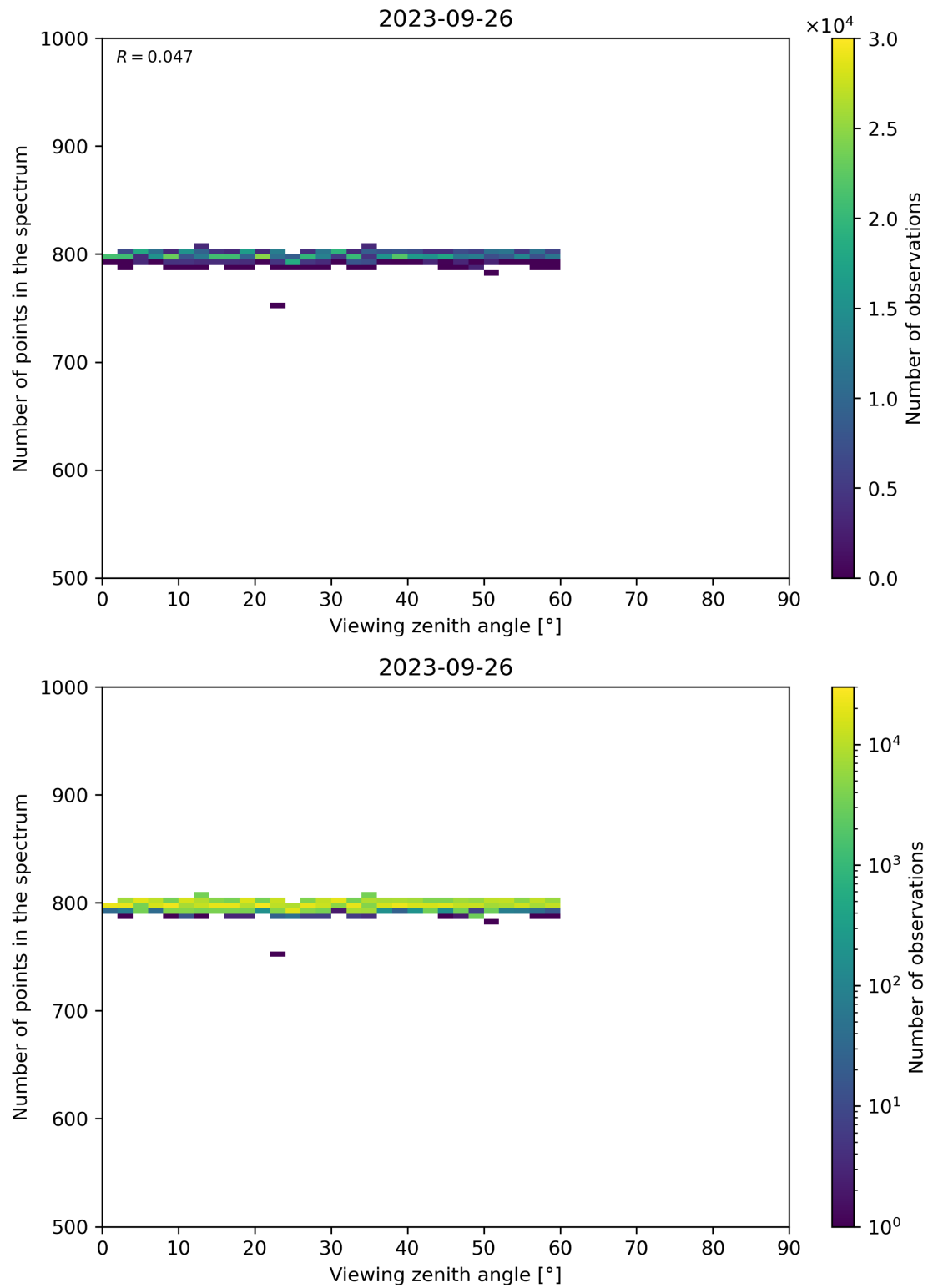
Figure 114: Scatter density plot of “Viewing zenith angle” against “Number of points in the spectrum” for 2023-09-26 to 2023-09-27.
