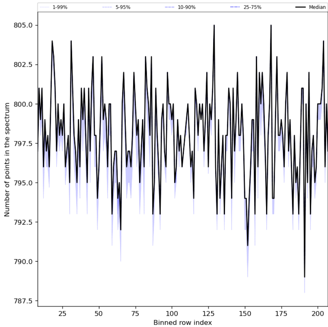
Figure 37: Along track statistics of “Number of points in the spectrum” for 2023-09-26 to 2023-09-27
