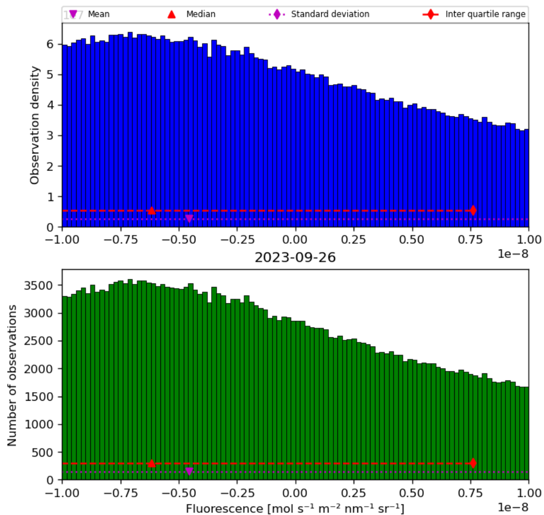
Figure 32: Histogram of “Fluorescence” for 2023-09-26 to 2023-09-27
