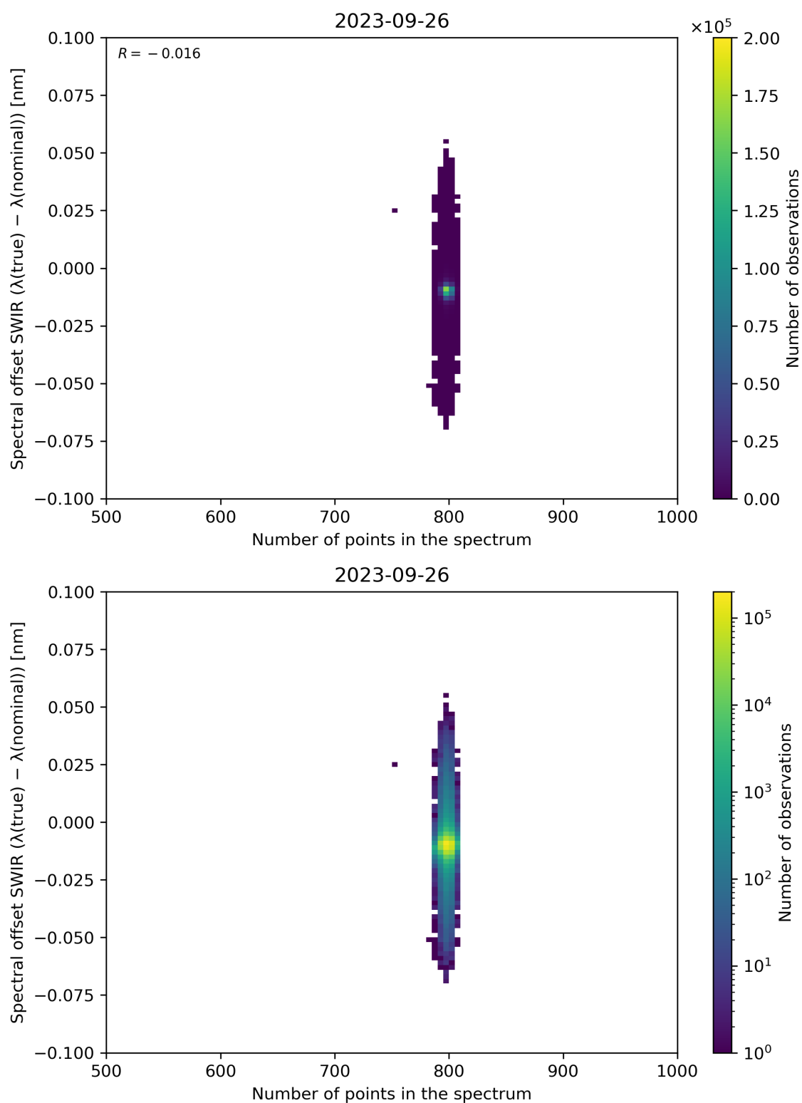
Figure 93: Scatter density plot of “Number of points in the spectrum” against “Spectral offset SWIR ( \lambda(\text{true}) - \lambda(\text{nominal}) )” for 2023-09-26 to 2023-09-27.
