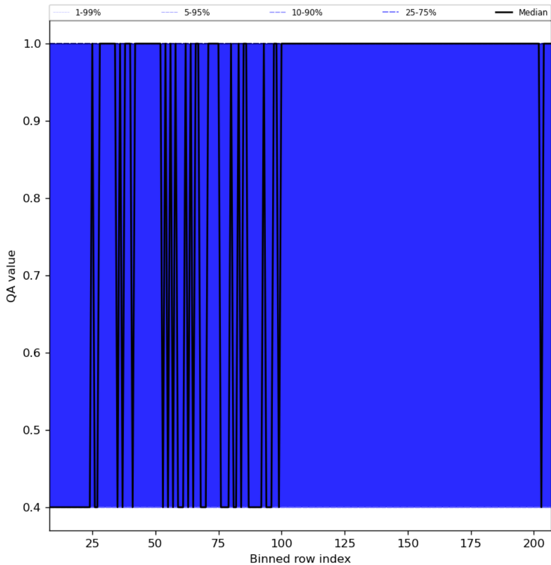
Figure 33: Along track statistics of “QA value” for 2023-09-26 to 2023-09-27
