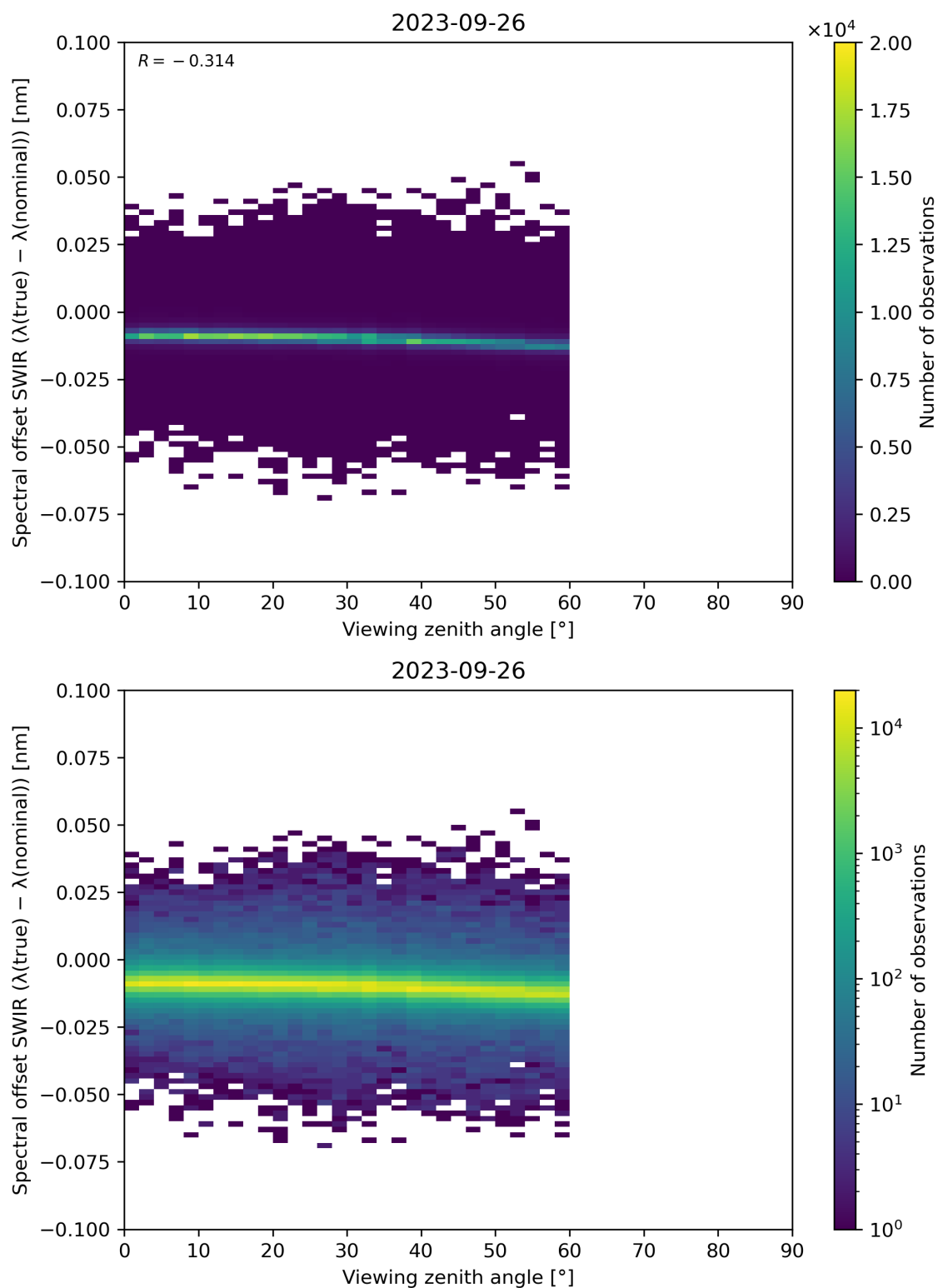
Figure 116: Scatter density plot of “Viewing zenith angle” against “Spectral offset SWIR ( \lambda(\text{true}) - \lambda(\text{nominal}) )” for 2023-09-26 to 2023-09-27.
