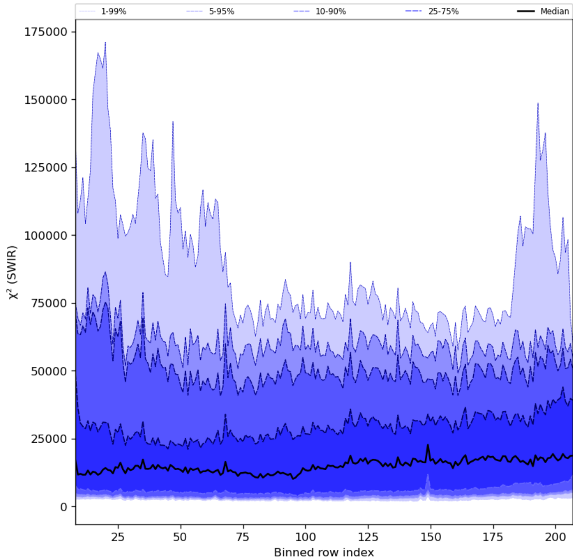
Figure 39: Along track statistics of “ \chi^2 (SWIR)” for 2023-09-26 to 2023-09-27
