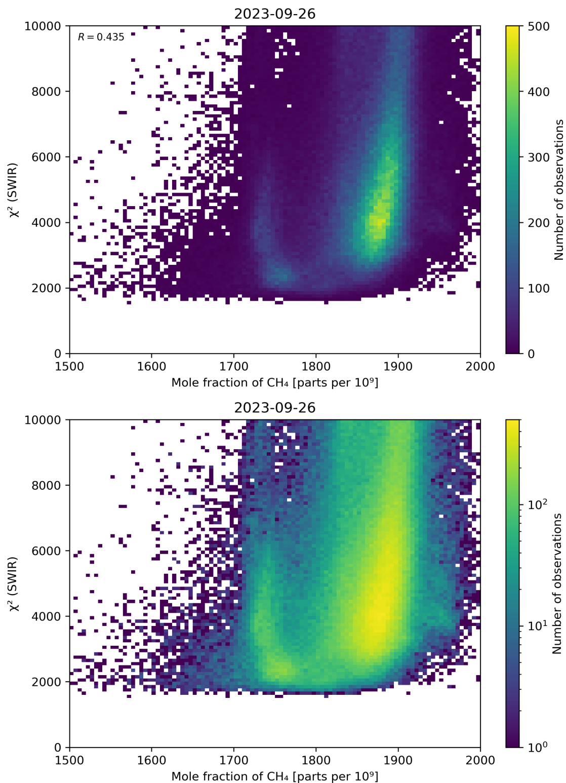
Figure 71: Scatter density plot of “Mole fraction of \text{CH}_4 ” against “ \chi^2 (SWIR)” for 2023-09-26 to 2023-09-27.
