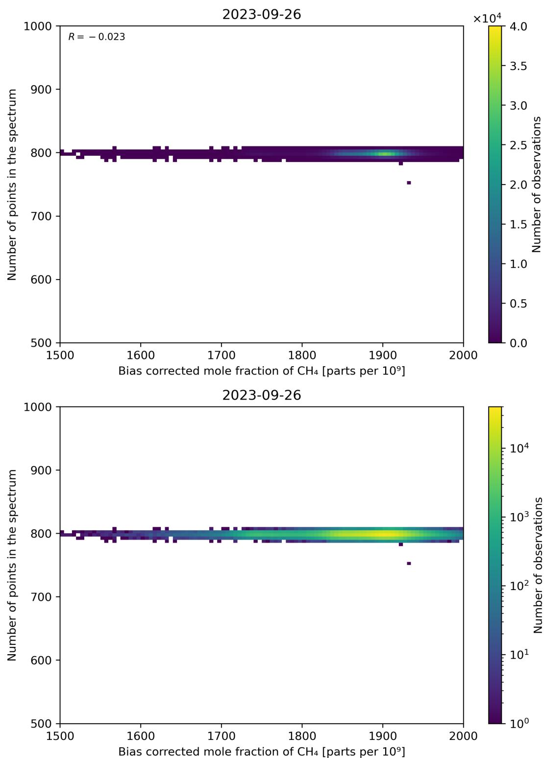
Figure 68: Scatter density plot of “Bias corrected mole fraction of CH 4 ” against “Number of points in the spectrum” for 2023-09-26 to 2023-09-27.
