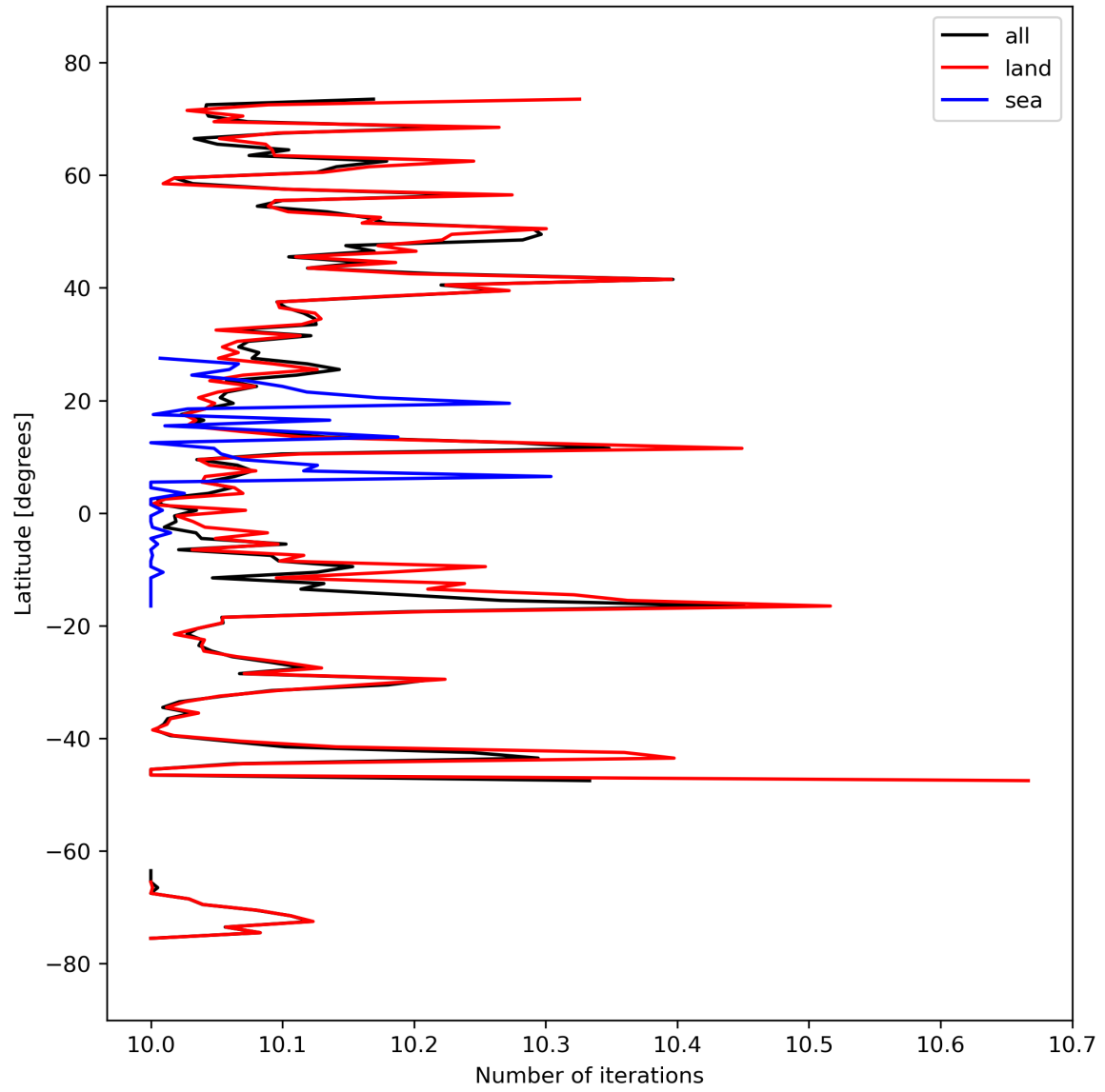
Figure 20: Zonal average of “Number of iterations” for 2023-09-26 to 2023-09-27.
