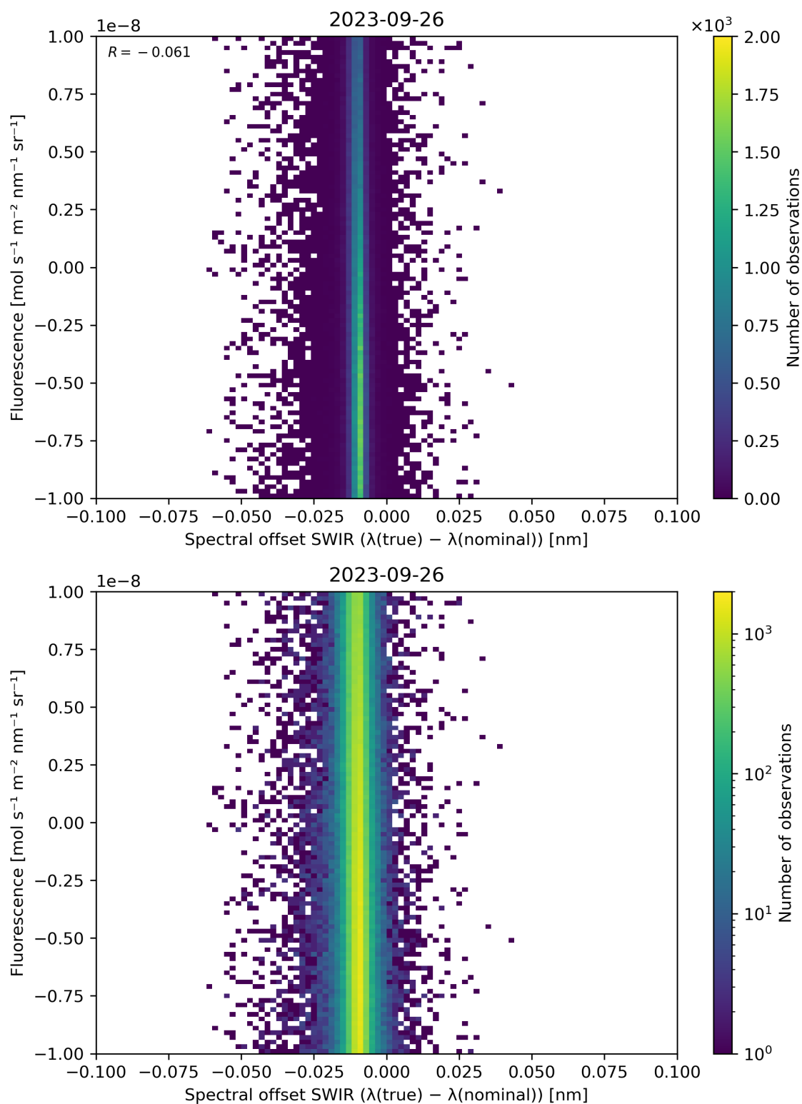
Figure 120: Scatter density plot of “Spectral offset SWIR ( \lambda(\text{true}) - \lambda(\text{nominal}) )” against “Fluorescence” for 2023-09-26 to 2023-09-27.
