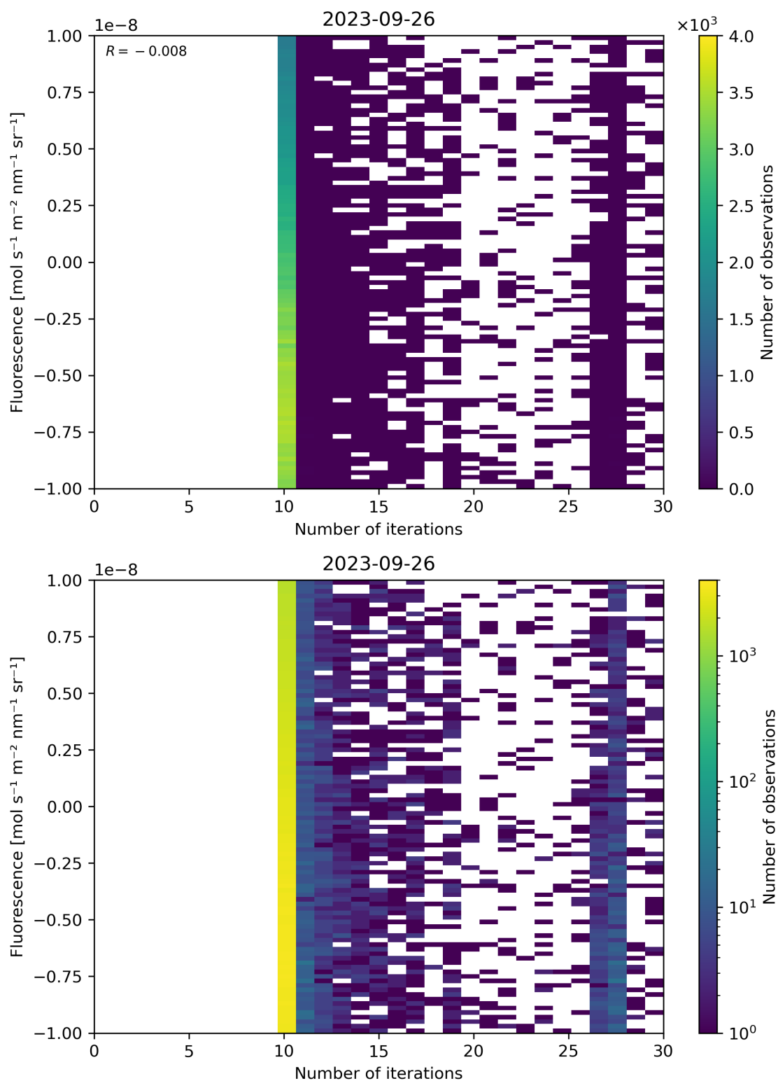
Figure 87: Scatter density plot of “Number of iterations” against “Fluorescence” for 2023-09-26 to 2023-09-27.
