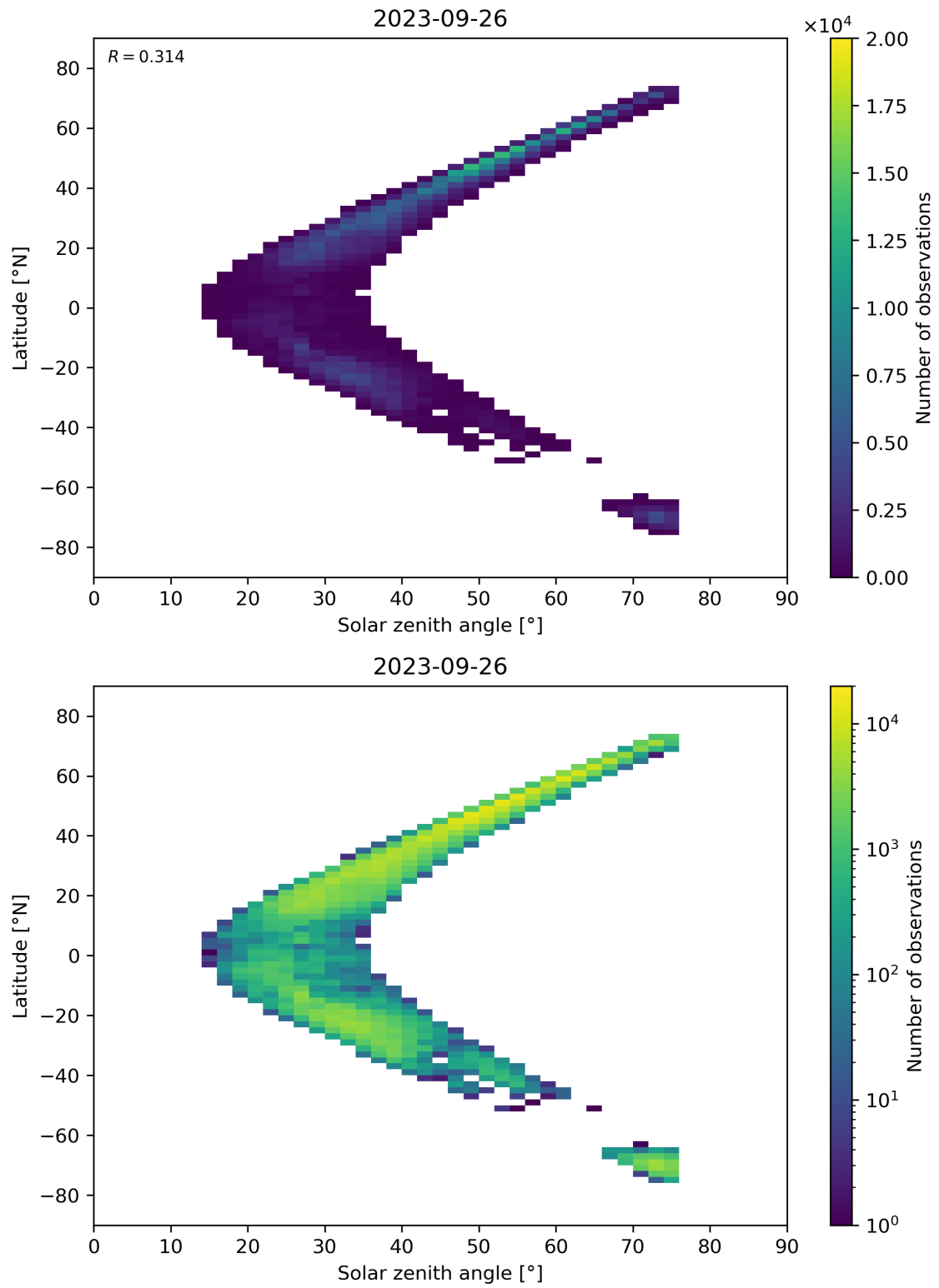
Figure 98: Scatter density plot of “Solar zenith angle” against “Latitude” for 2023-09-26 to 2023-09-27.
