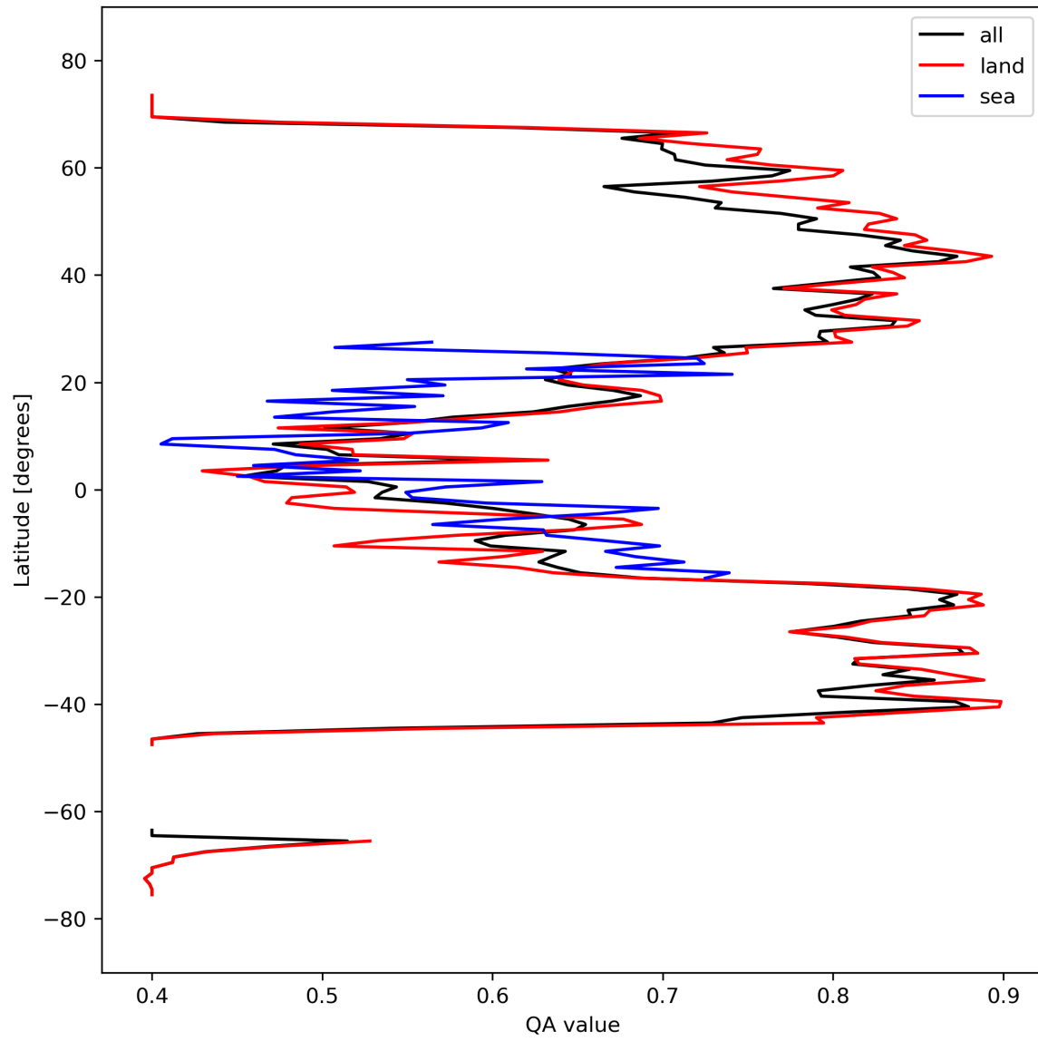
Figure 11: Zonal average of “QA value” for 2023-09-26 to 2023-09-27.
