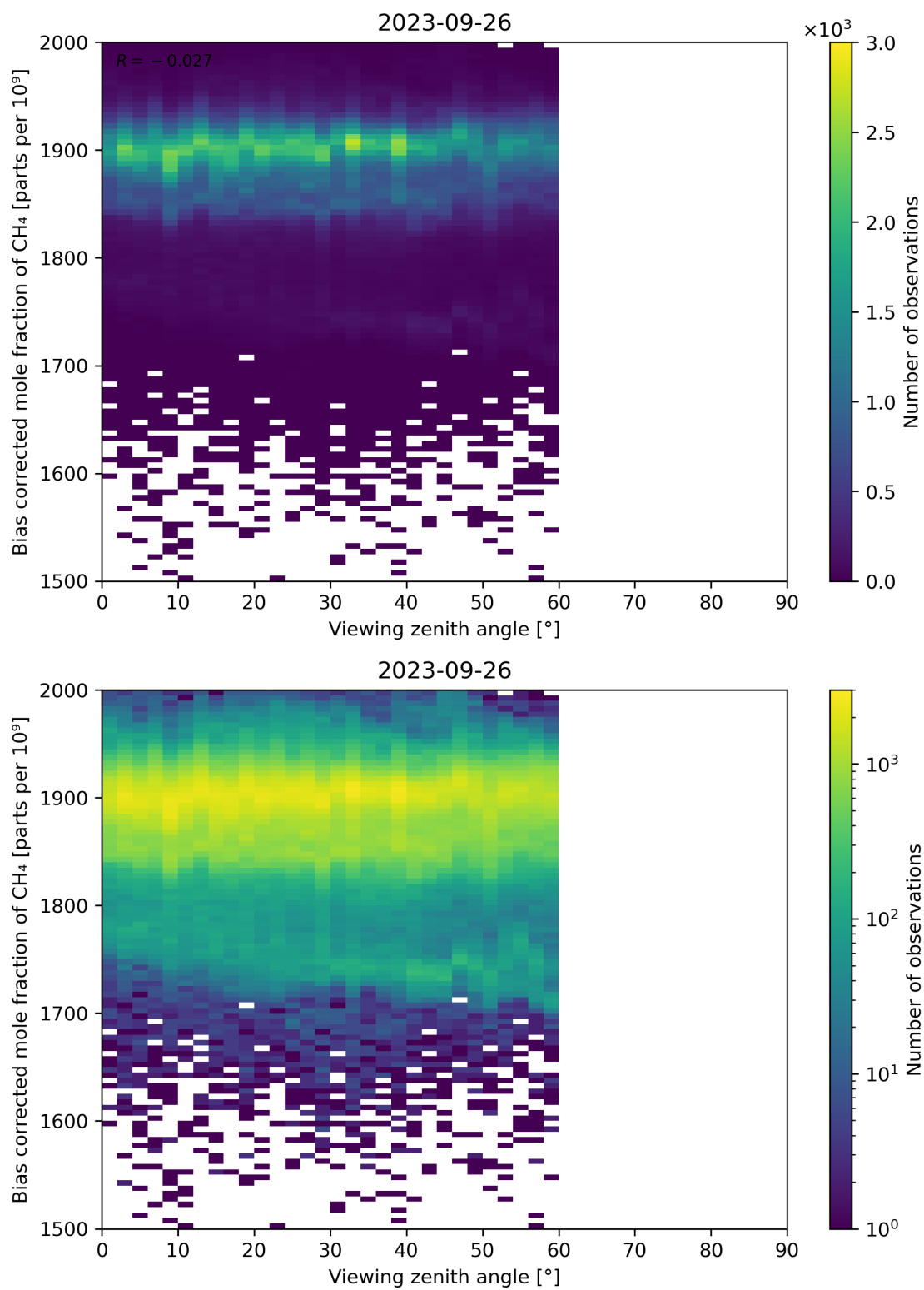
Figure 111: Scatter density plot of “Viewing zenith angle” against “Bias corrected mole fraction of CH 4 ” for 2023-09-26 to 2023-09-27.
