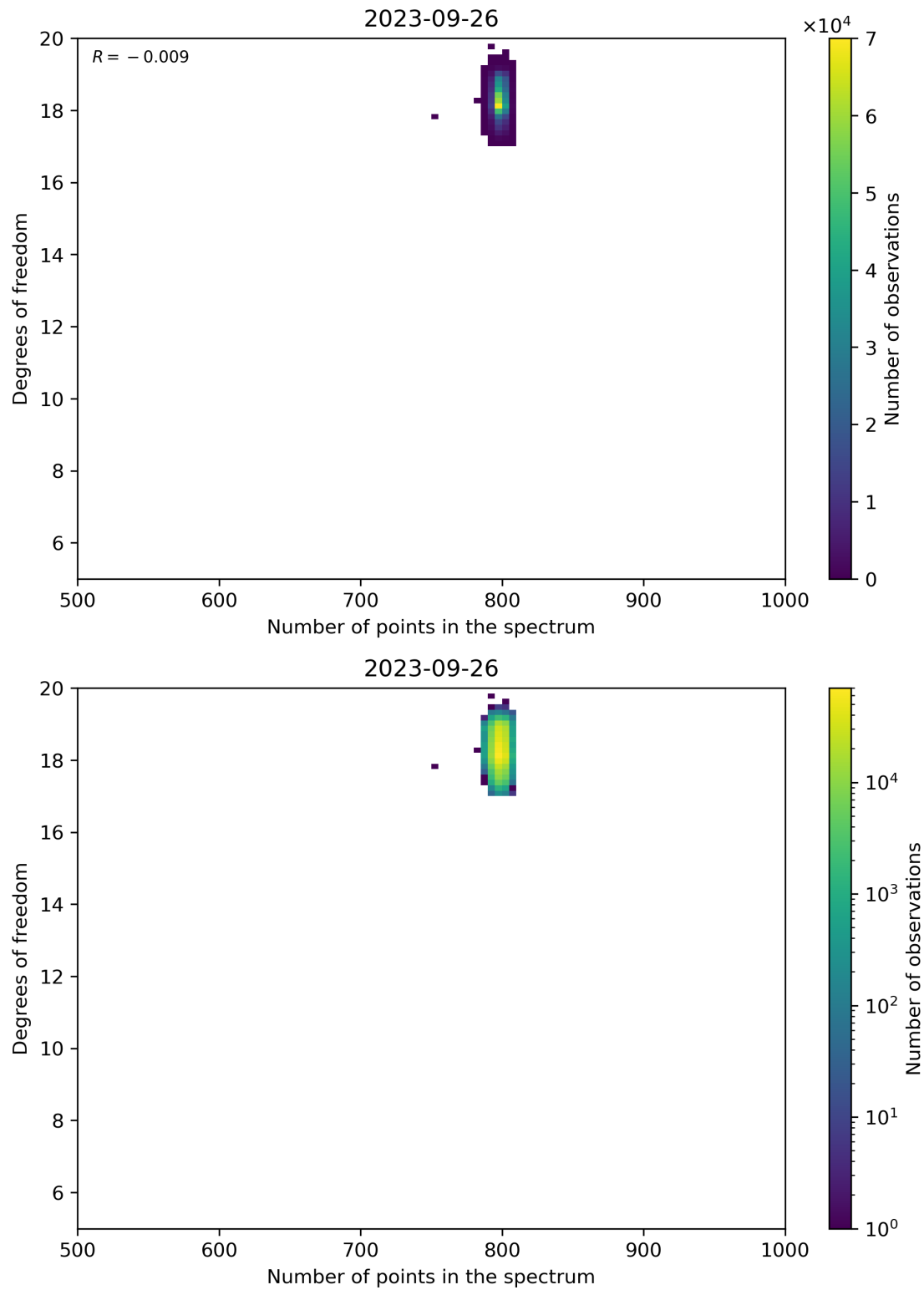
Figure 90: Scatter density plot of “Number of points in the spectrum” against “Degrees of freedom” for 2023-09-26 to 2023-09-27.
