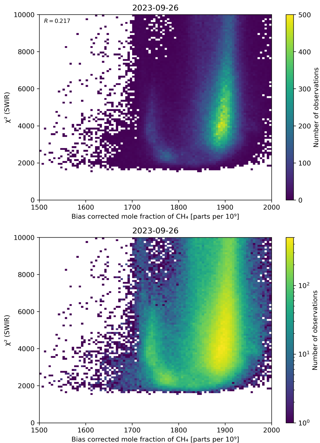
Figure 64: Scatter density plot of “Bias corrected mole fraction of \text{CH}_4 ” against “ \chi^2 (SWIR)” for 2023-09-26 to 2023-09-27.
