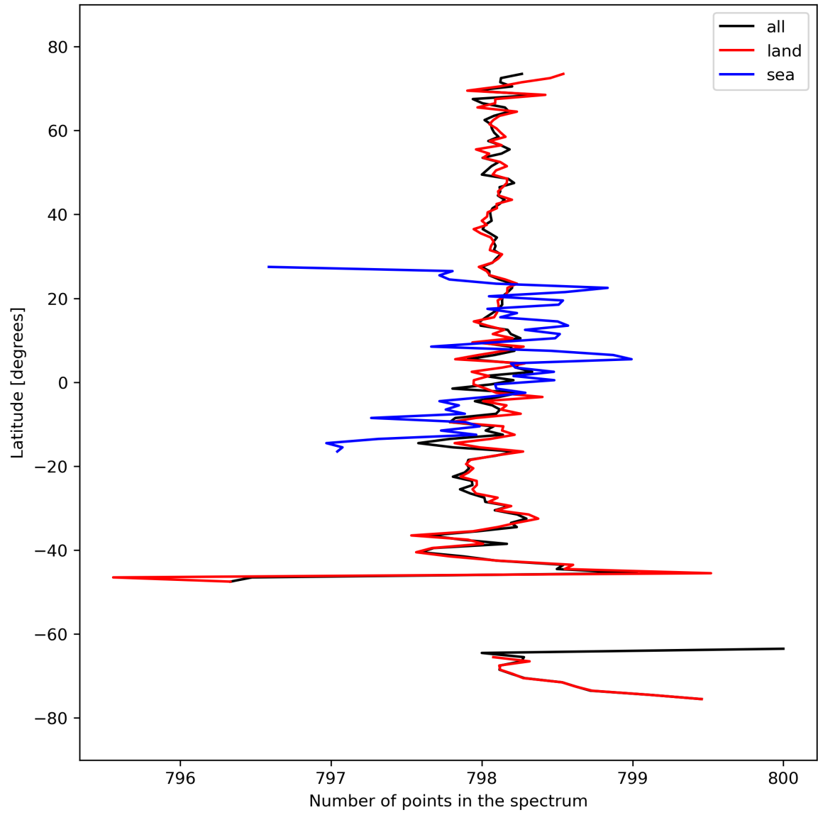
Figure 15: Zonal average of “Number of points in the spectrum” for 2023-09-26 to 2023-09-27.
