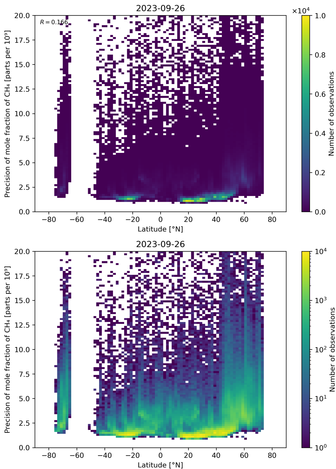
Figure 59: Scatter density plot of “Latitude” against “Precision of mole fraction of \text{CH}_4 ” for 2023-09-26 to 2023-09-27.
