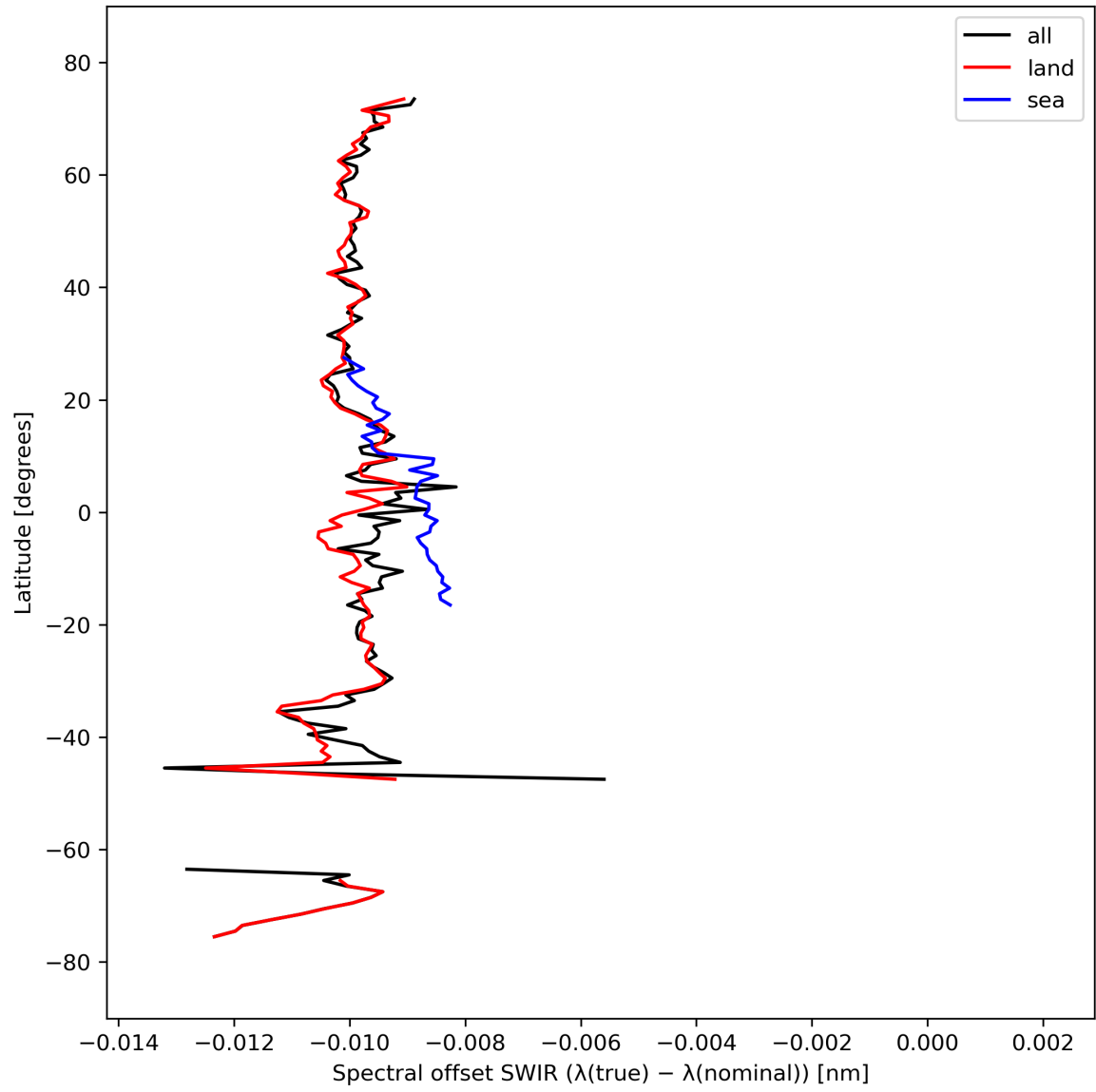
Figure 16: Zonal average of “Spectral offset SWIR ( \lambda(\text{true}) - \lambda(\text{nominal}) )” for 2023-09-26 to 2023-09-27.
