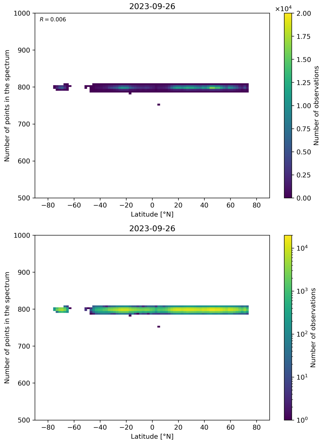
Figure 61: Scatter density plot of “Latitude” against “Number of points in the spectrum” for 2023-09-26 to 2023-09-27.
