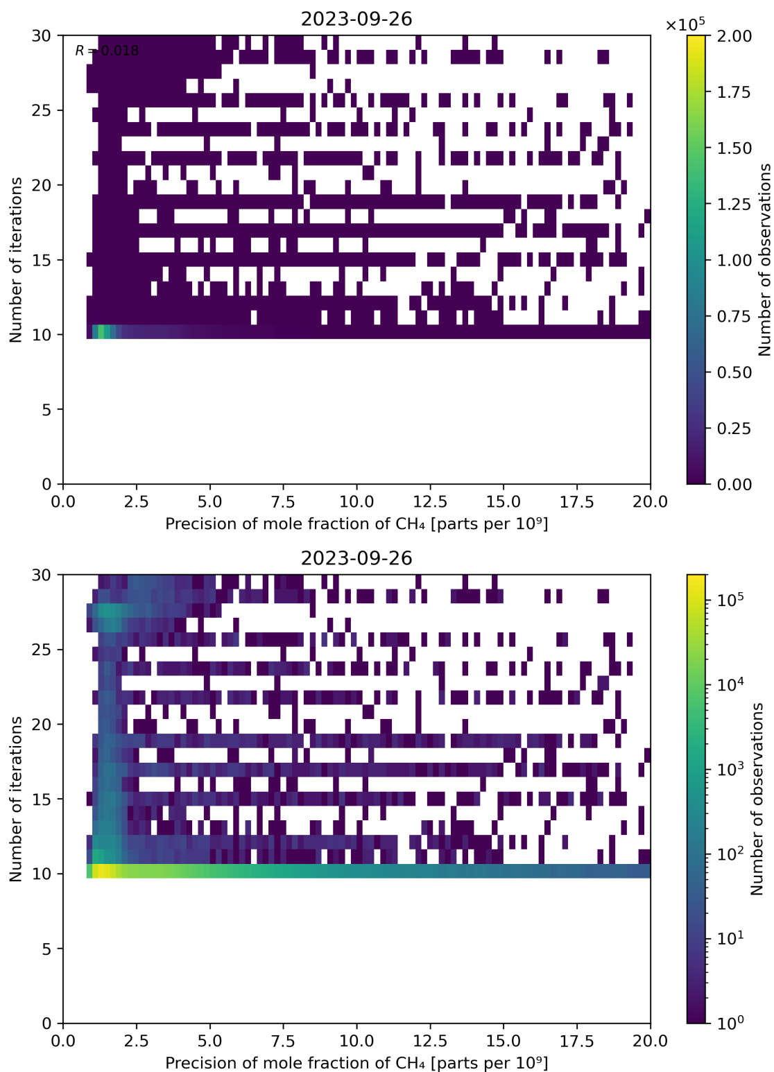
Figure 83: Scatter density plot of “Precision of mole fraction of CH 4 ” against “Number of iterations” for 2023-09-26 to 2023-09-27.
