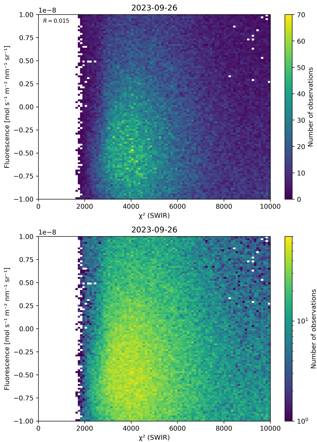
Figure 49: Scatter density plot of “ \chi^2 (SWIR)” against “Fluorescence” for 2023-09-26 to 2023-09-27.
