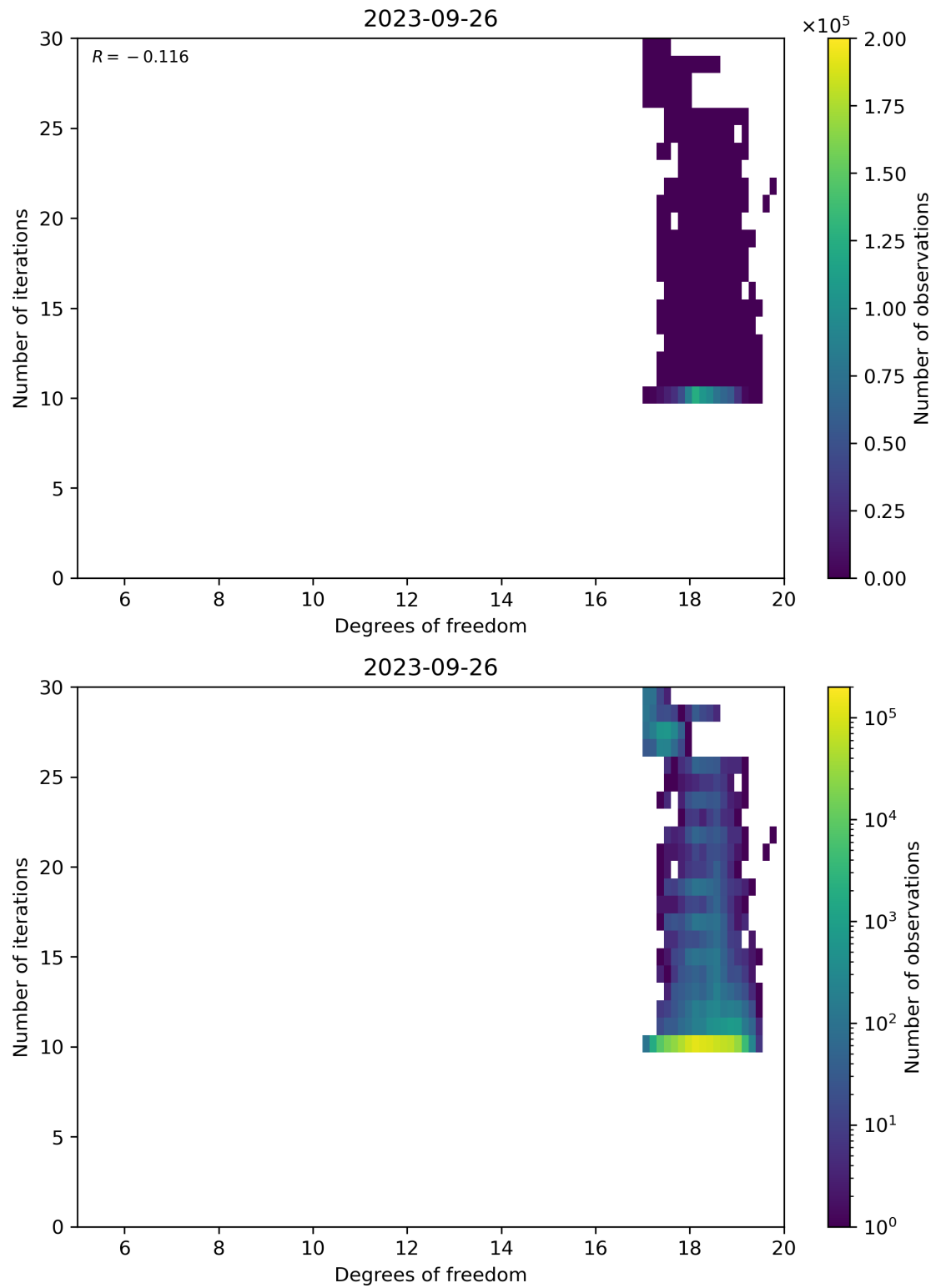
Figure 52: Scatter density plot of “Degrees of freedom” against “Number of iterations” for 2023-09-26 to 2023-09-27.
