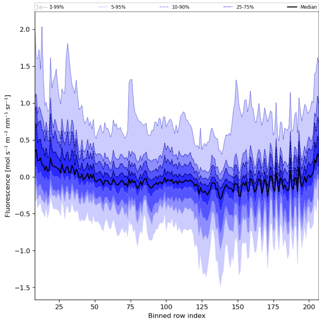
Figure 43: Along track statistics of “Fluorescence” for 2023-09-26 to 2023-09-27
