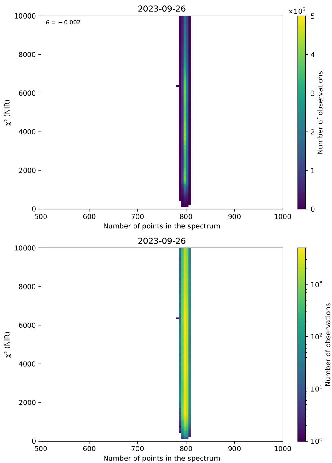
Figure 88: Scatter density plot of “Number of points in the spectrum” against “ \chi^2 (NIR)” for 2023-09-26 to 2023-09-27.
