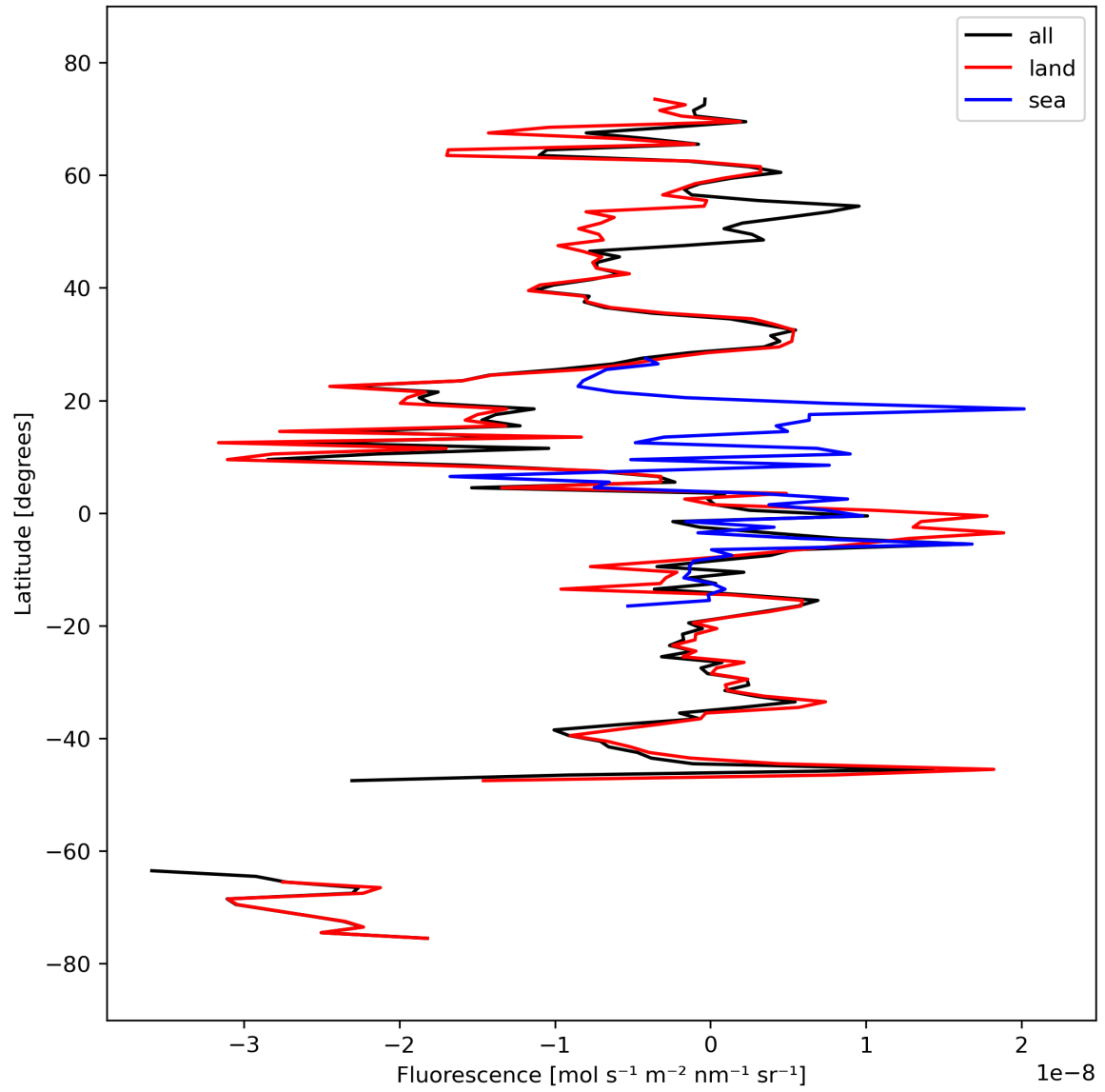
Figure 21: Zonal average of “Fluorescence” for 2023-09-26 to 2023-09-27.
