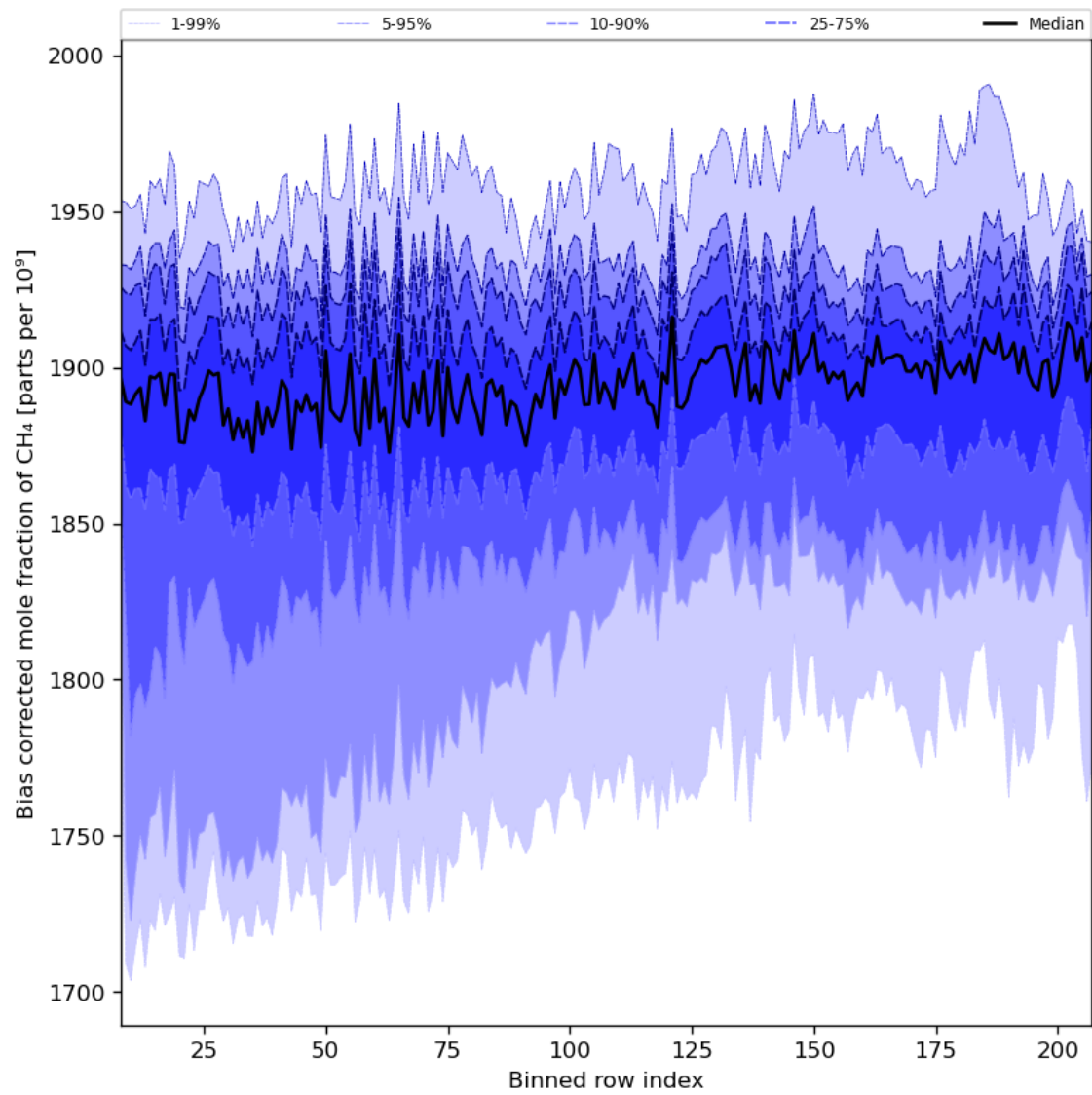
Figure 36: Along track statistics of “Bias corrected mole fraction of CH 4 ” for 2023-09-26 to 2023-09-27
