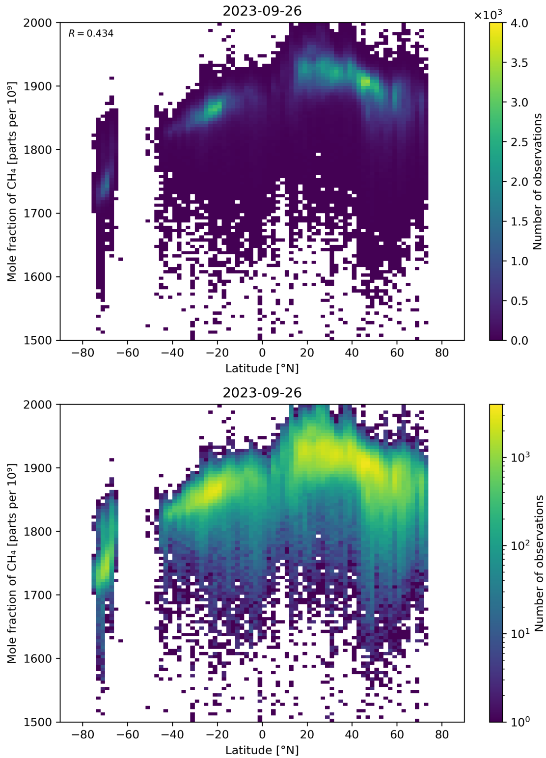
Figure 57: Scatter density plot of “Latitude” against “Mole fraction of CH 4 ” for 2023-09-26 to 2023-09-27.
