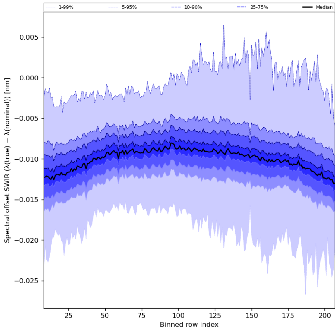
Figure 38: Along track statistics of “Spectral offset SWIR ( \lambda(\text{true}) - \lambda(\text{nominal}) )” for 2023-09-26 to 2023-09-27
