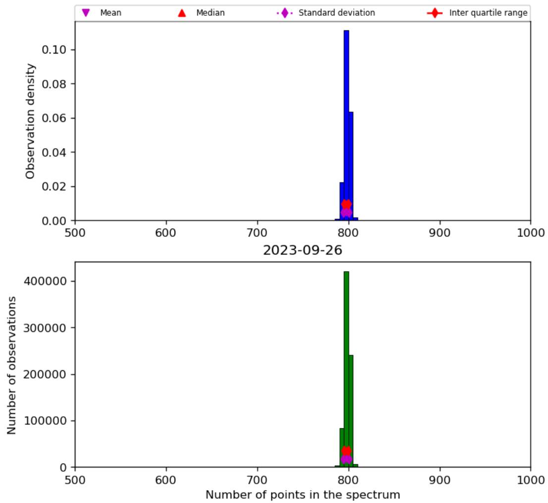
Figure 26: Histogram of “Number of points in the spectrum” for 2023-09-26 to 2023-09-27
