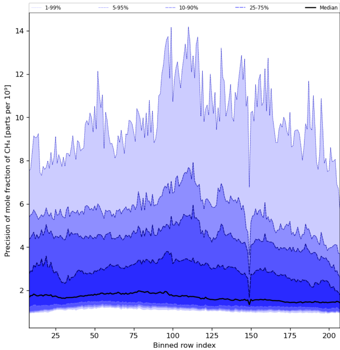
Figure 35: Along track statistics of “Precision of mole fraction of CH 4 ” for 2023-09-26 to 2023-09-27
