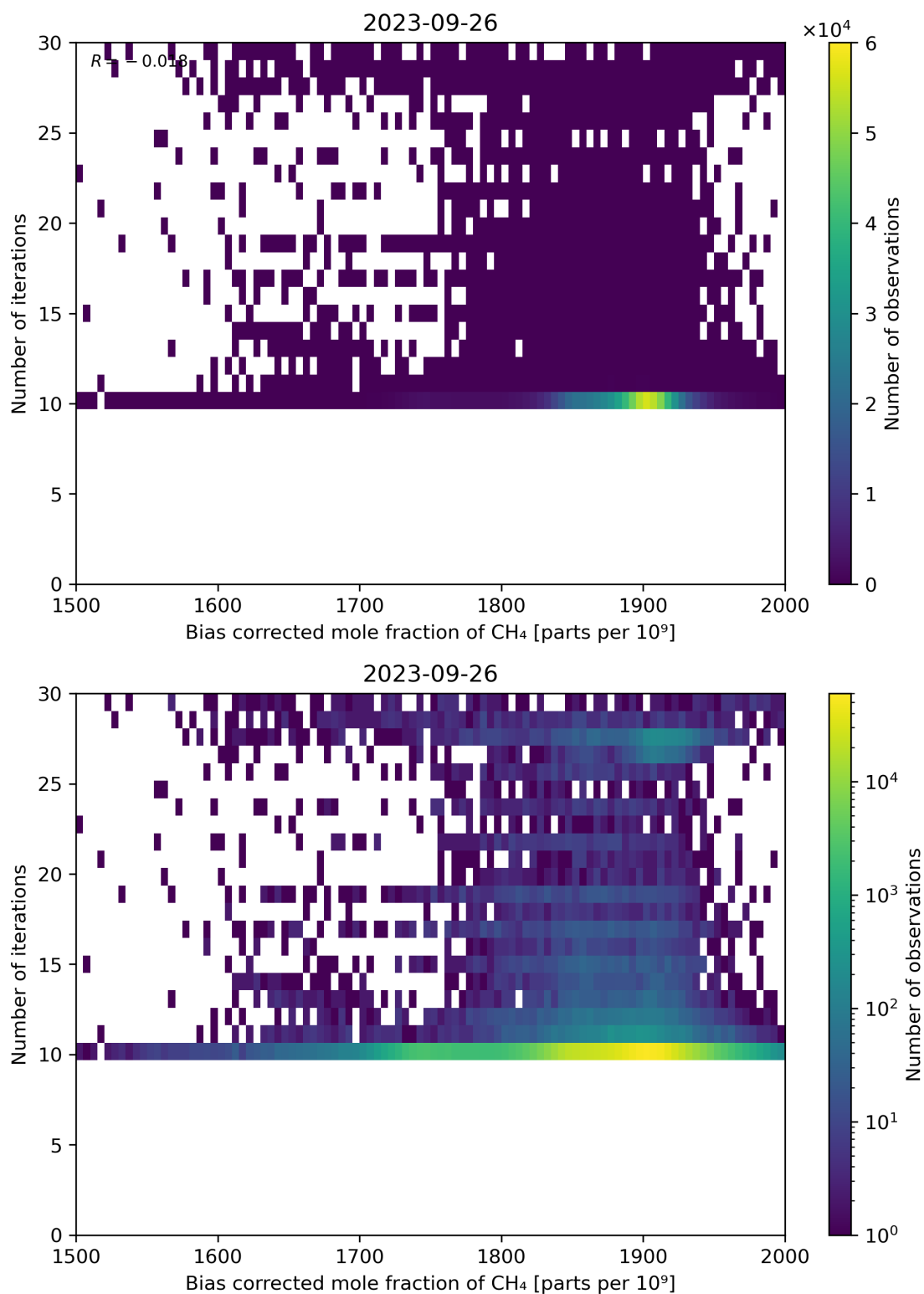
Figure 67: Scatter density plot of “Bias corrected mole fraction of CH 4 ” against “Number of iterations” for 2023-09-26 to 2023-09-27.
