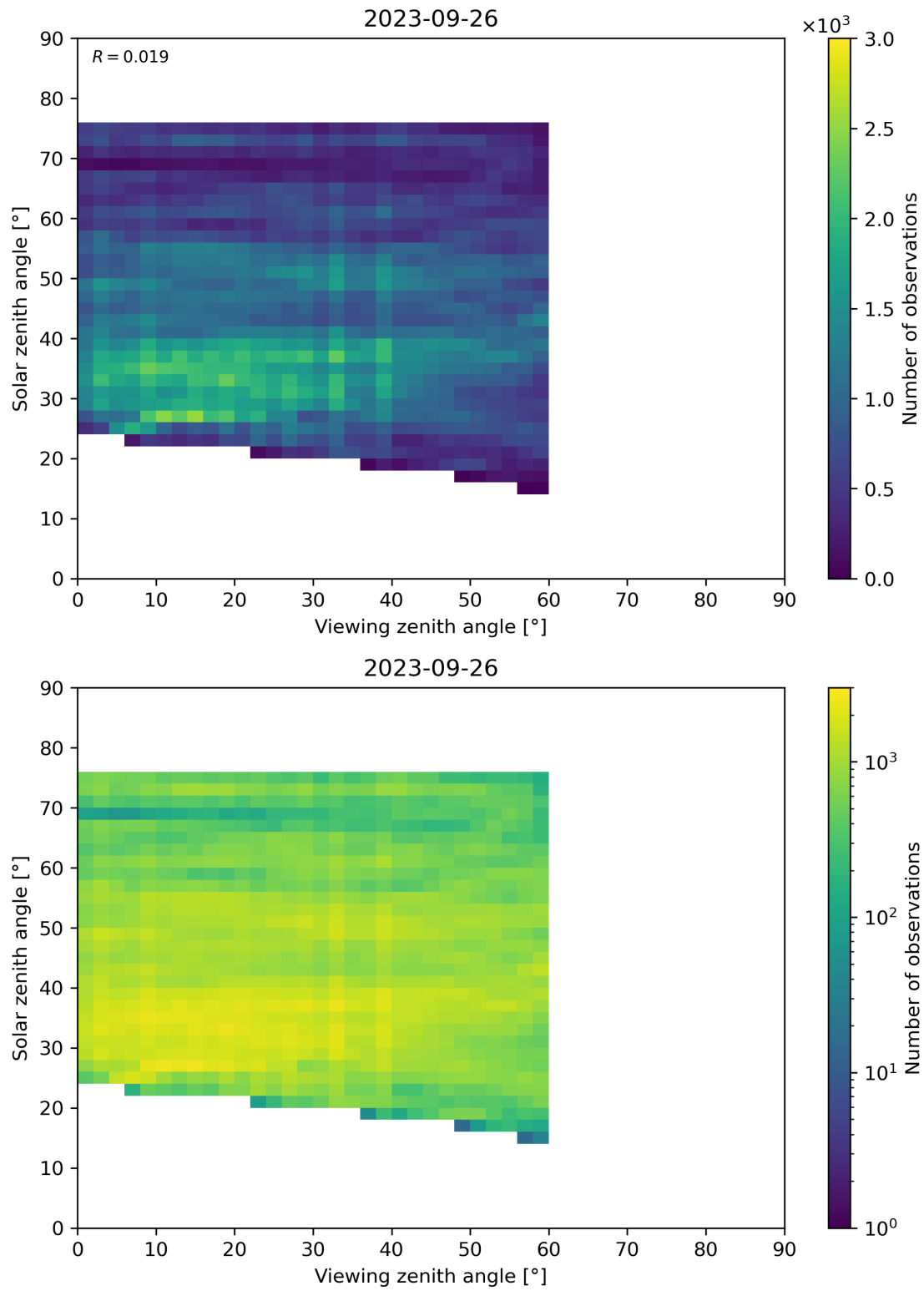
Figure 115: Scatter density plot of “Viewing zenith angle” against “Solar zenith angle” for 2023-09-26 to 2023-09-27.
