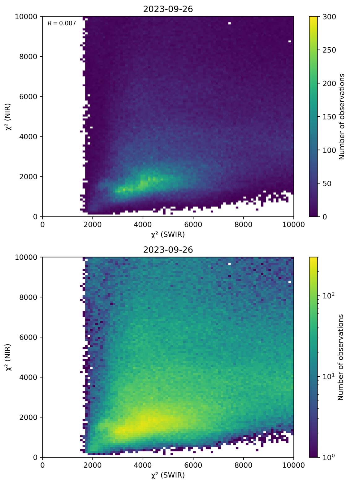
Figure 47: Scatter density plot of “ \chi^2 (SWIR)” against “ \chi^2 (NIR)” for 2023-09-26 to 2023-09-27.
