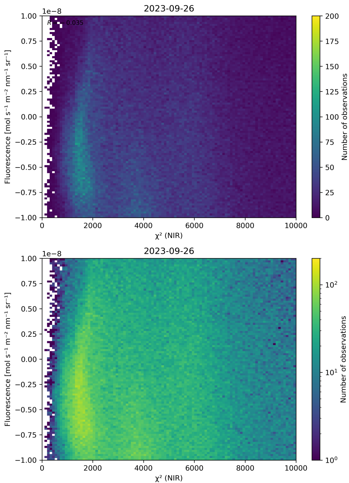
Figure 45: Scatter density plot of “ \chi^2 (NIR)” against “Fluorescence” for 2023-09-26 to 2023-09-27.
