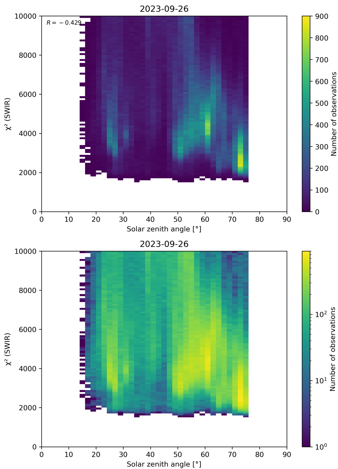
Figure 95: Scatter density plot of “Solar zenith angle” against “ \chi^2 (SWIR)” for 2023-09-26 to 2023-09-27.
