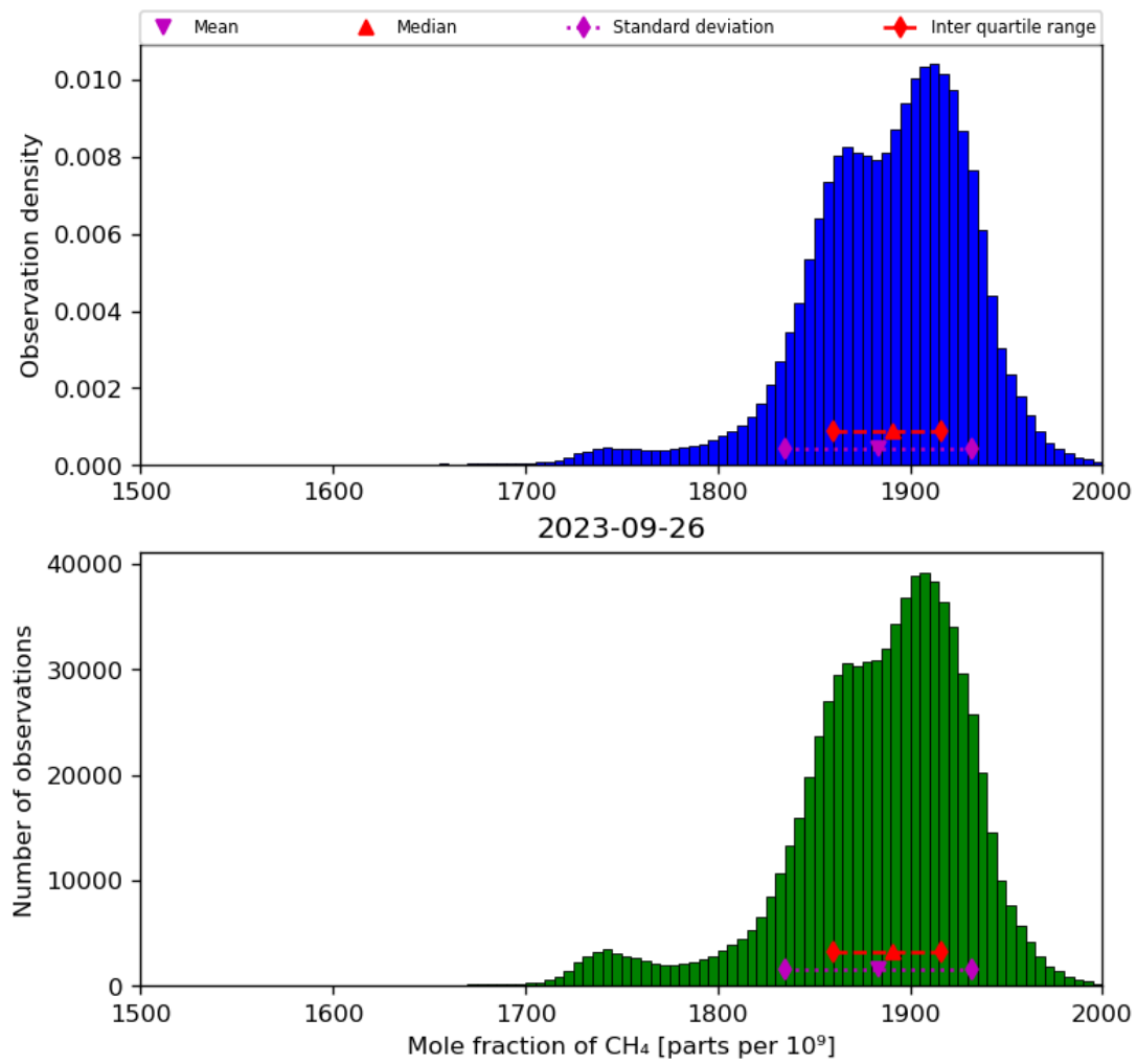
Figure 23: Histogram of “Mole fraction of CH 4 ” for 2023-09-26 to 2023-09-27
