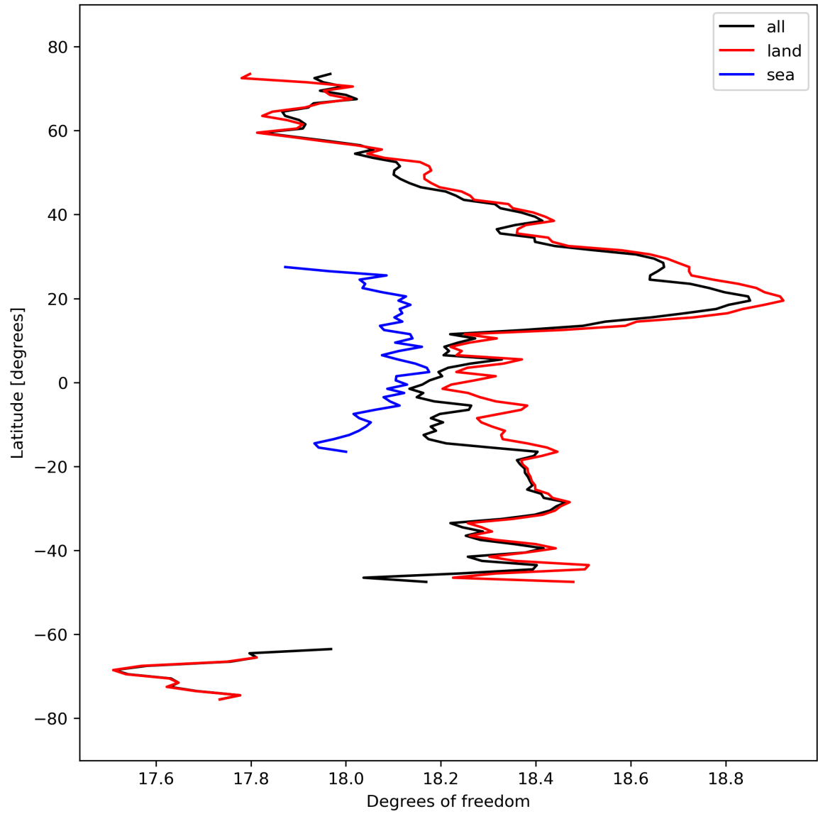
Figure 19: Zonal average of “Degrees of freedom” for 2023-09-26 to 2023-09-27.
