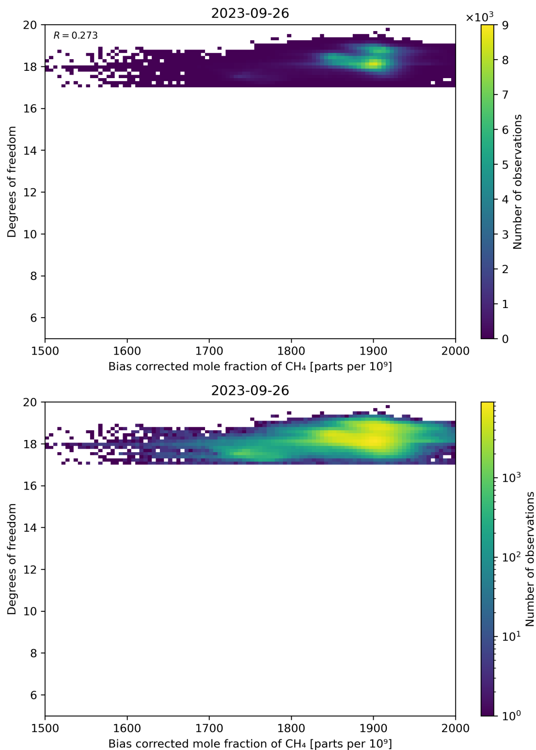
Figure 65: Scatter density plot of “Bias corrected mole fraction of CH 4 ” against “Degrees of freedom” for 2023-09-26 to 2023-09-27.
