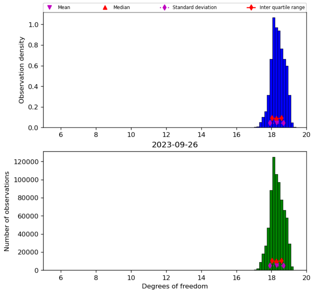
Figure 30: Histogram of “Degrees of freedom” for 2023-09-26 to 2023-09-27
