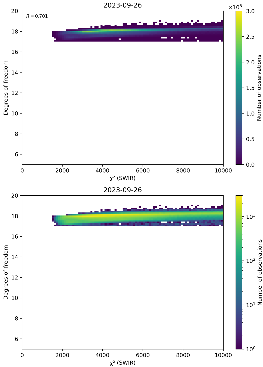
Figure 48: Scatter density plot of “ \chi^2 (SWIR)” against “Degrees of freedom” for 2023-09-26 to 2023-09-27.
