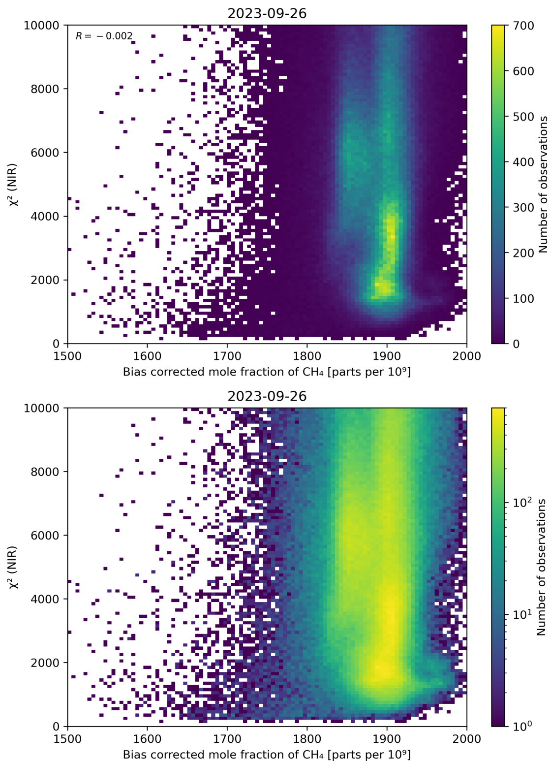
Figure 63: Scatter density plot of “Bias corrected mole fraction of CH 4 ” against “ \chi^2 (NIR)” for 2023-09-26 to 2023-09-27.
