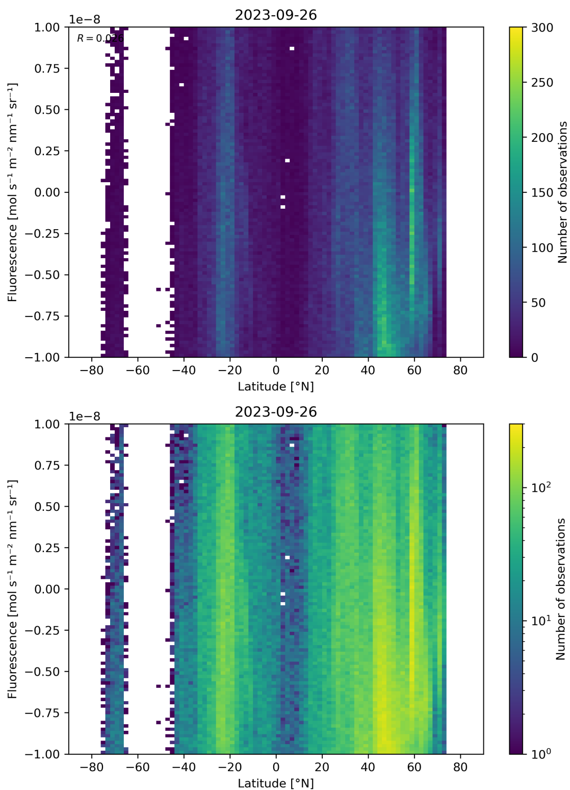
Figure 56: Scatter density plot of “Latitude” against “Fluorescence” for 2023-09-26 to 2023-09-27.
