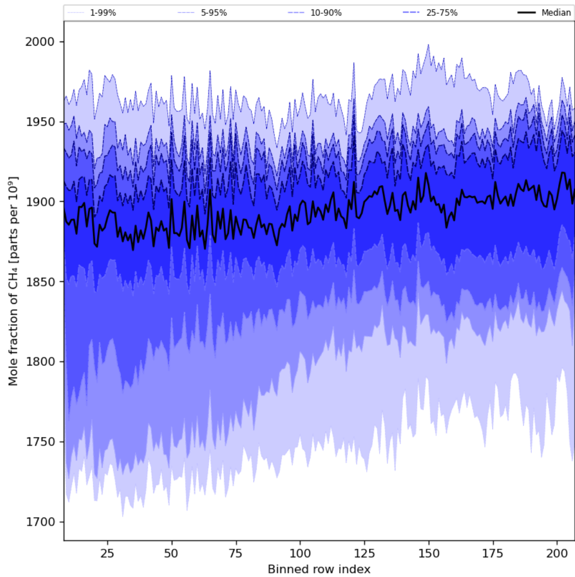
Figure 34: Along track statistics of “Mole fraction of CH 4 ” for 2023-09-26 to 2023-09-27
