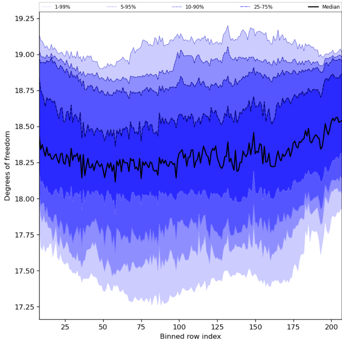
Figure 41: Along track statistics of “Degrees of freedom” for 2023-09-26 to 2023-09-27
