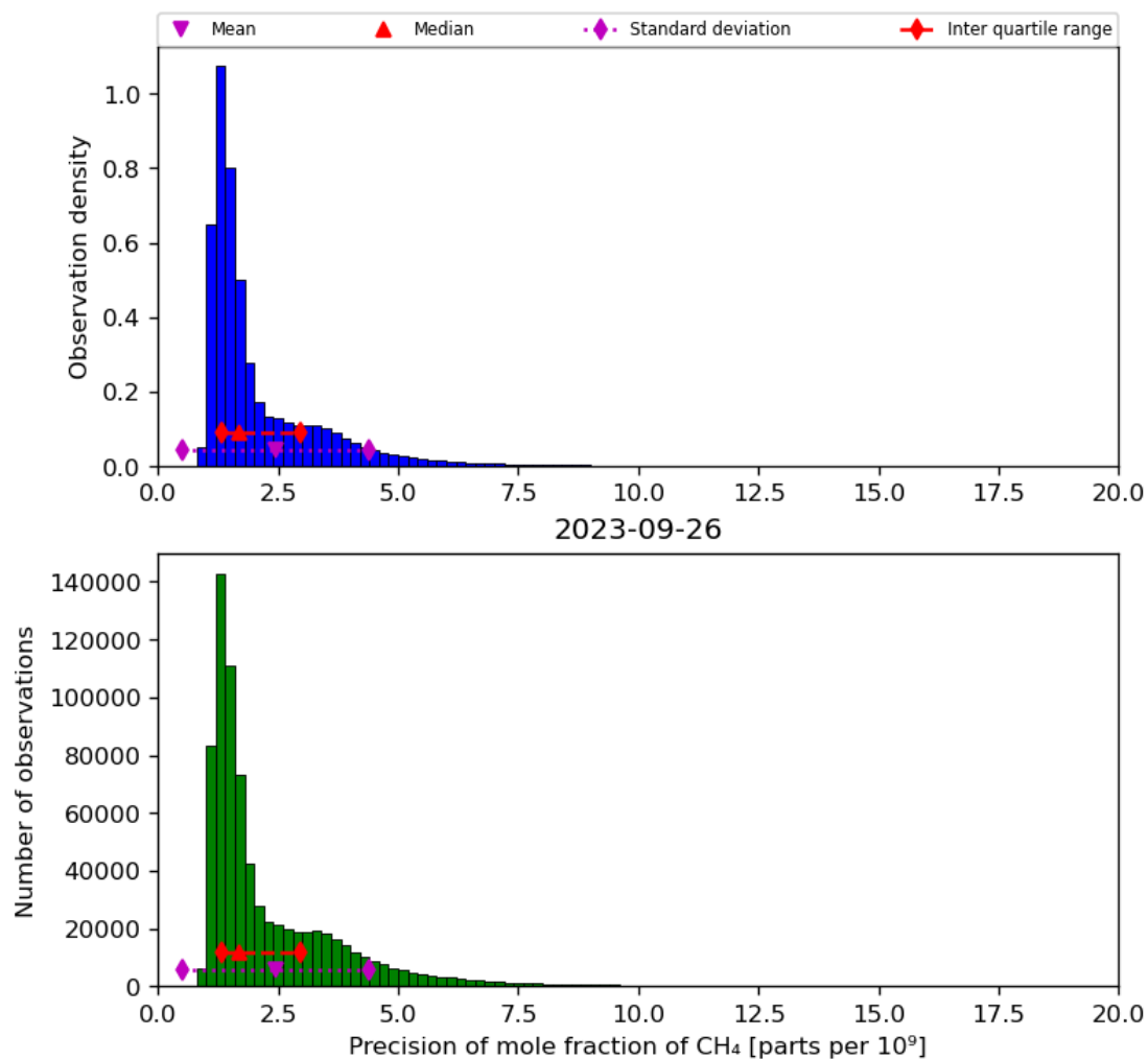
Figure 24: Histogram of “Precision of mole fraction of CH 4 ” for 2023-09-26 to 2023-09-27
