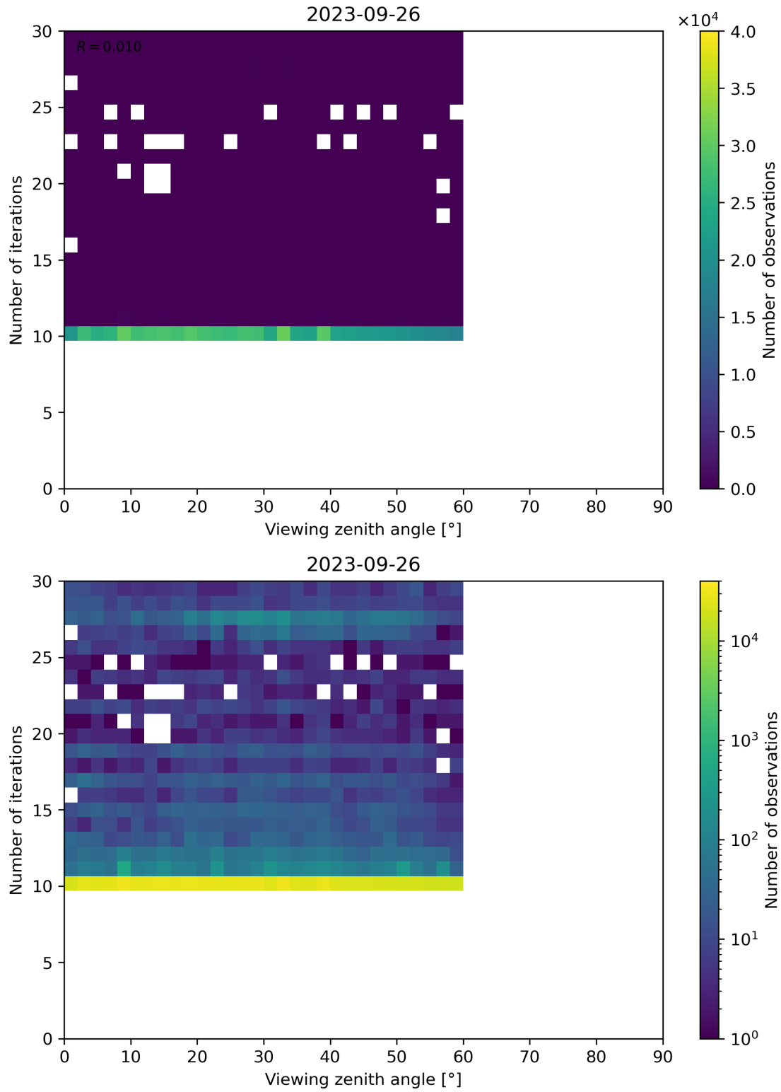
Figure 113: Scatter density plot of “Viewing zenith angle” against “Number of iterations” for 2023-09-26 to 2023-09-27.
