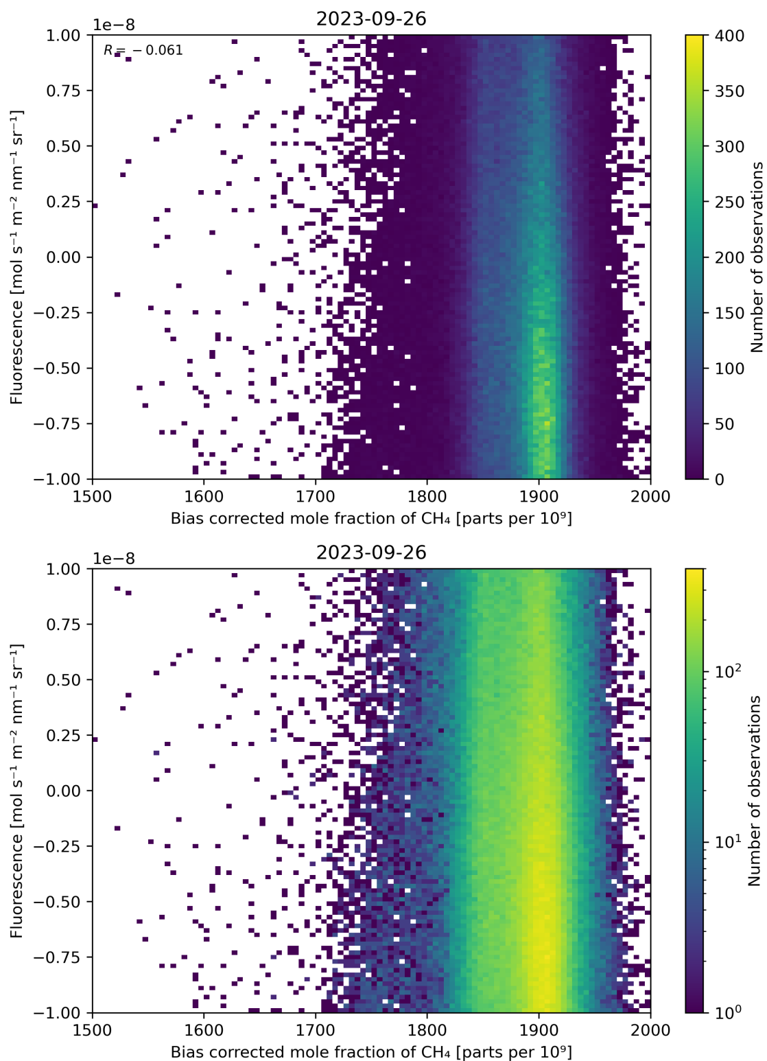
Figure 66: Scatter density plot of “Bias corrected mole fraction of \text{CH}_4 ” against “Fluorescence” for 2023-09-26 to 2023-09-27.
