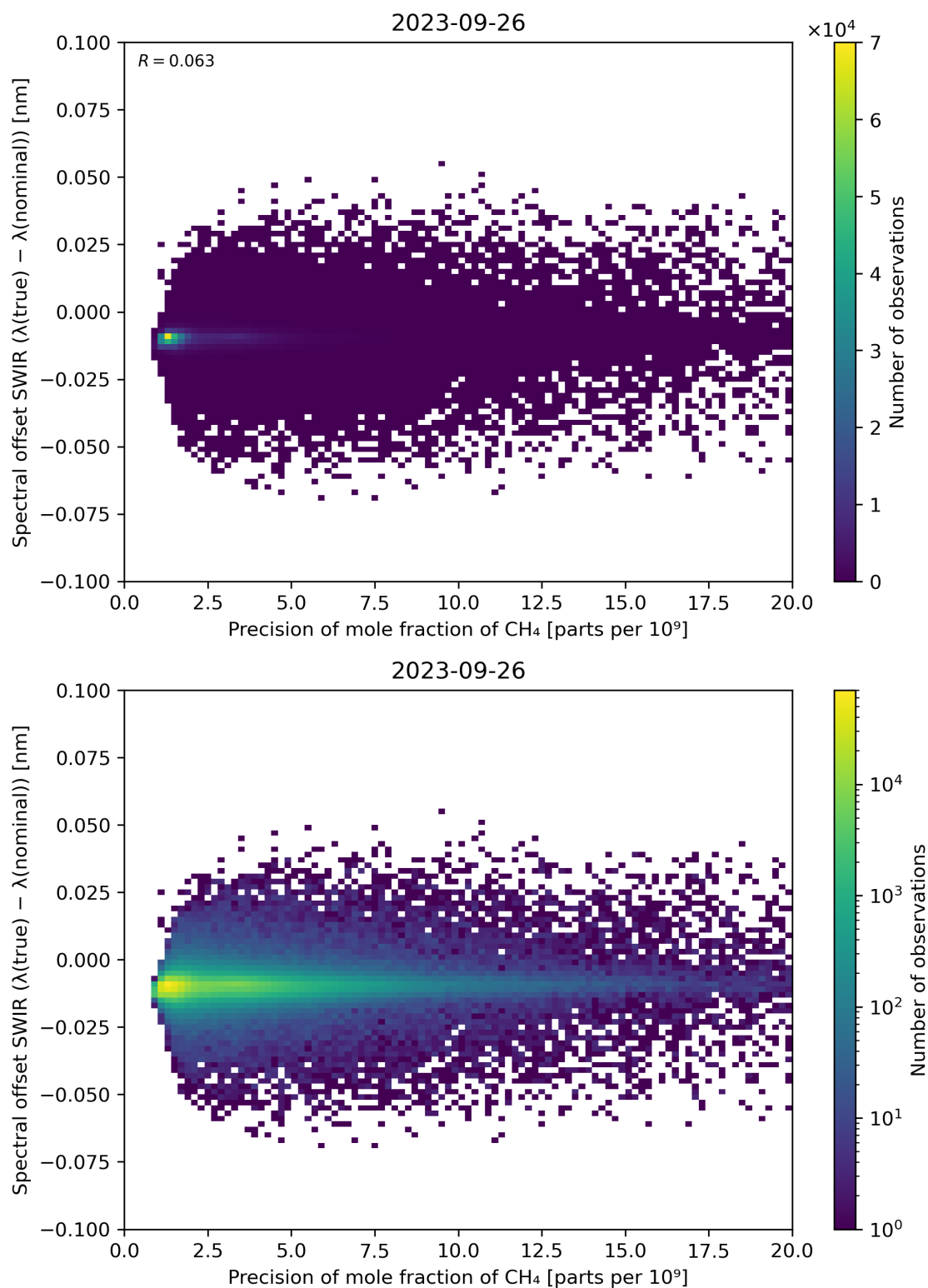
Figure 85: Scatter density plot of “Precision of mole fraction of CH 4 ” against “Spectral offset SWIR ( \lambda(\text{true}) - \lambda(\text{nominal}) )” for 2023-09-26 to 2023-09-27.
