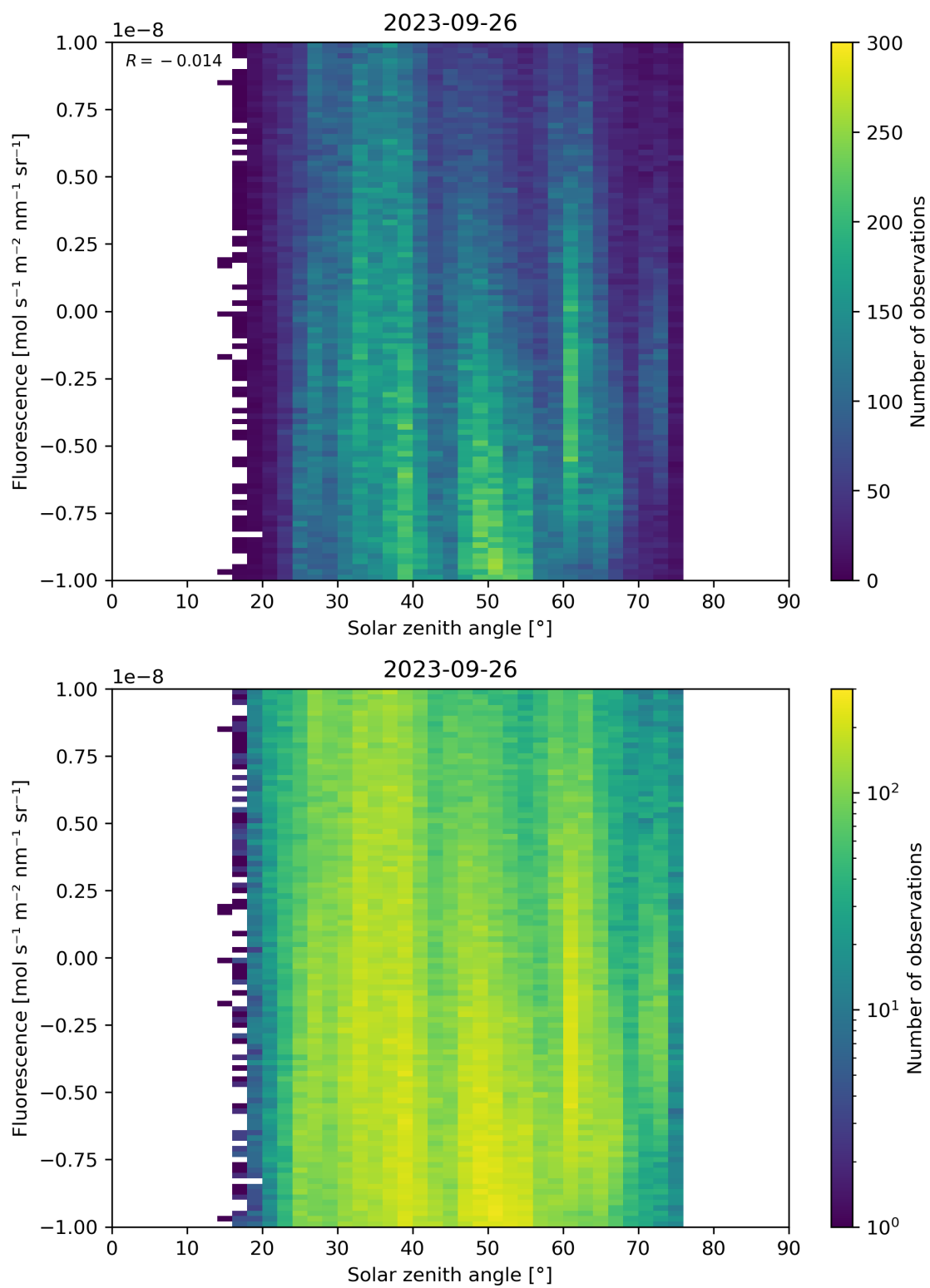
Figure 97: Scatter density plot of “Solar zenith angle” against “Fluorescence” for 2023-09-26 to 2023-09-27.
