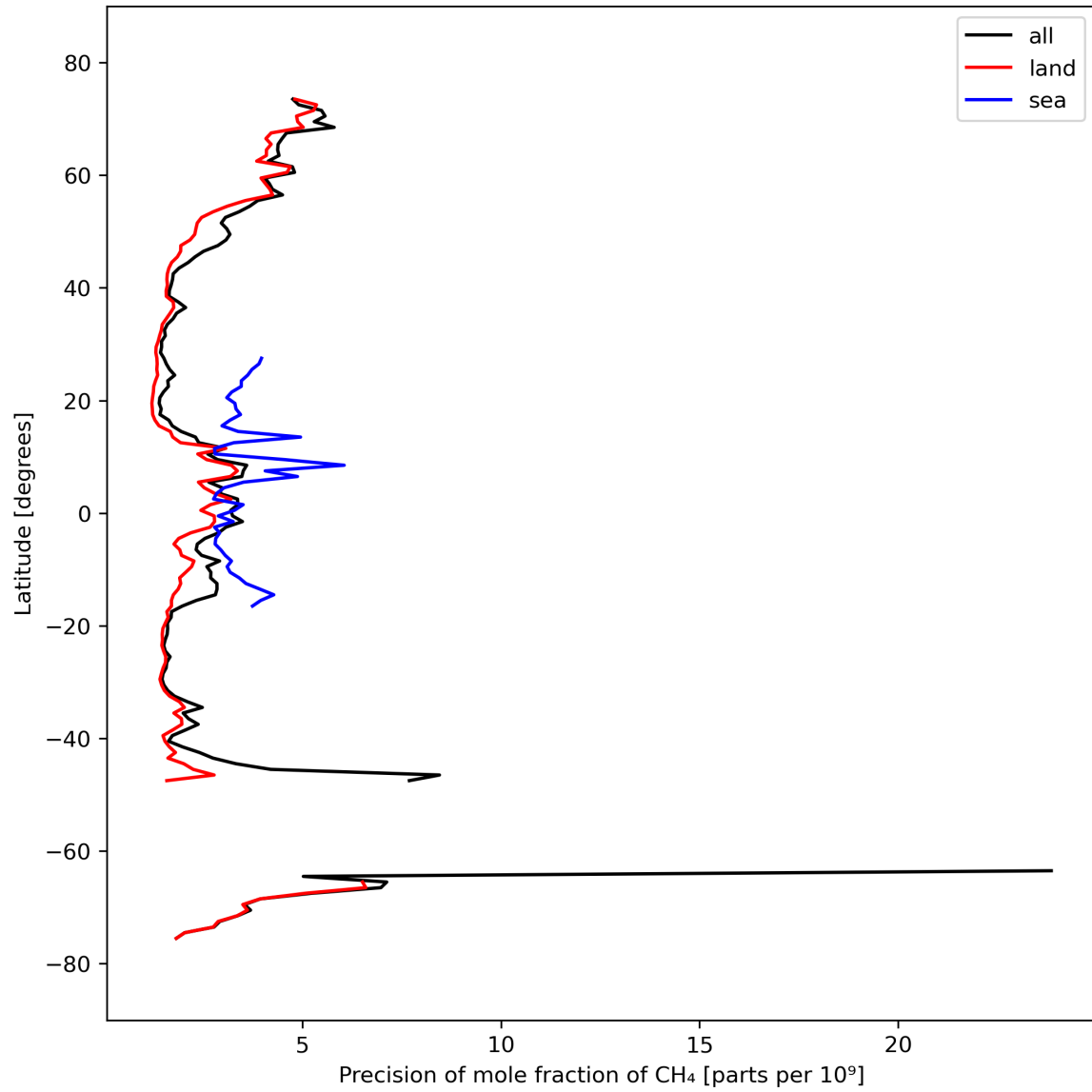
Figure 13: Zonal average of “Precision of mole fraction of \text{CH}_4 ” for 2023-09-26 to 2023-09-27.
