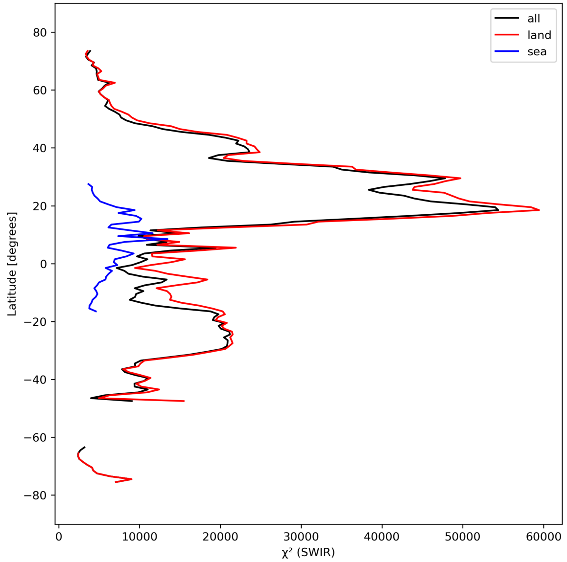
Figure 17: Zonal average of “ \chi^2 (SWIR)” for 2023-09-26 to 2023-09-27.
