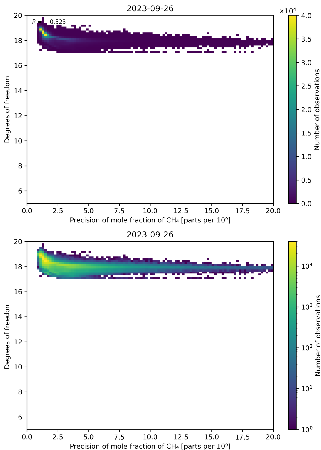
Figure 80: Scatter density plot of “Precision of mole fraction of CH 4 ” against “Degrees of freedom” for 2023-09-26 to 2023-09-27.
