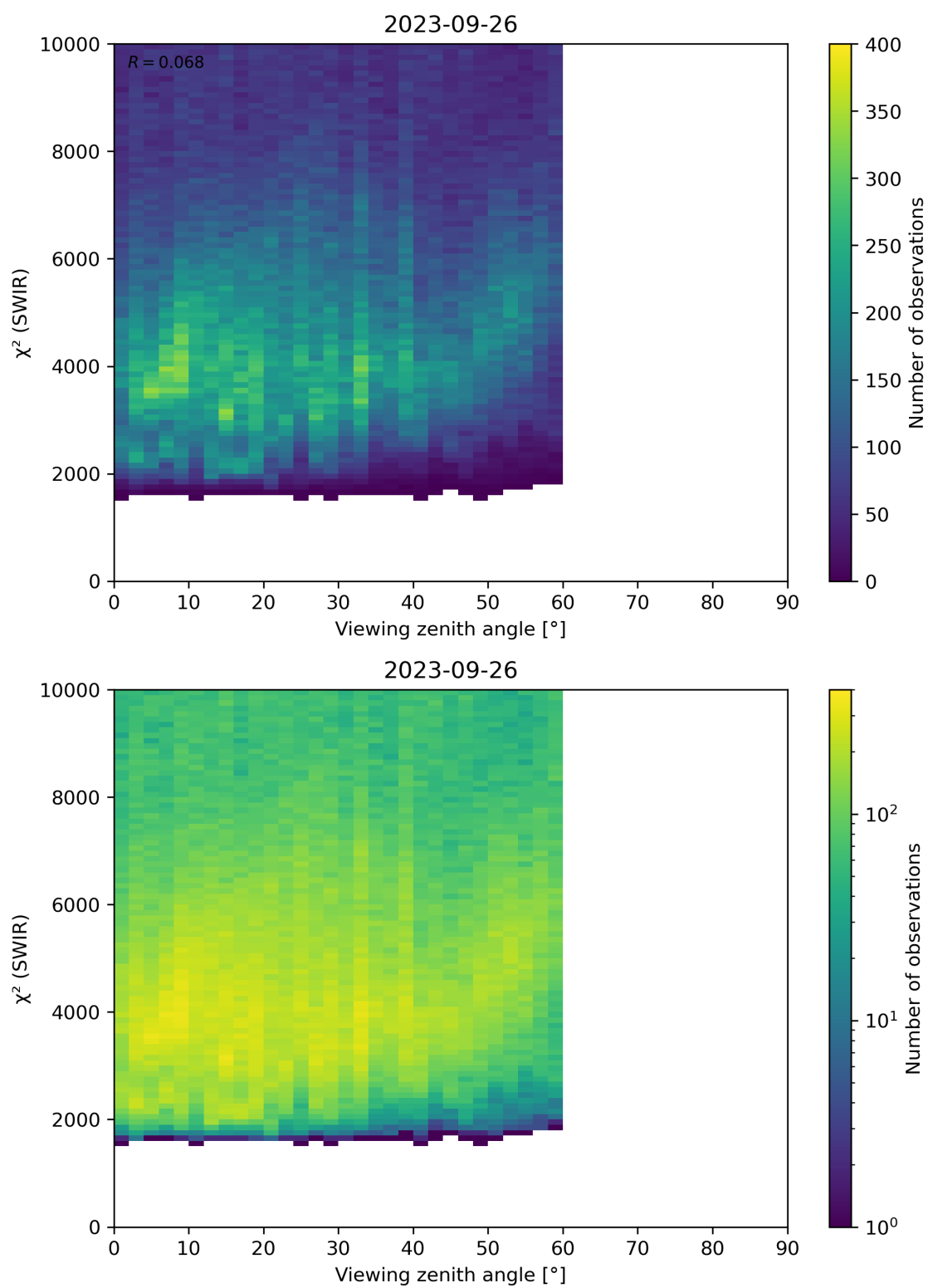
Figure 106: Scatter density plot of “Viewing zenith angle” against “ \chi^2 (SWIR)” for 2023-09-26 to 2023-09-27.
