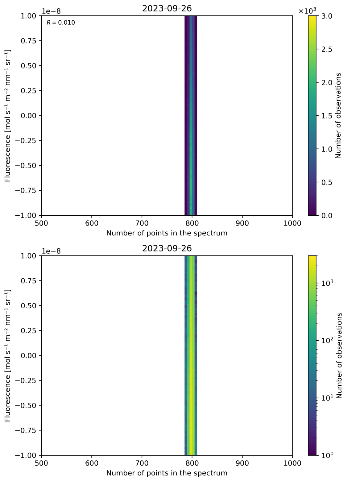
Figure 91: Scatter density plot of “Number of points in the spectrum” against “Fluorescence” for 2023-09-26 to 2023-09-27.
