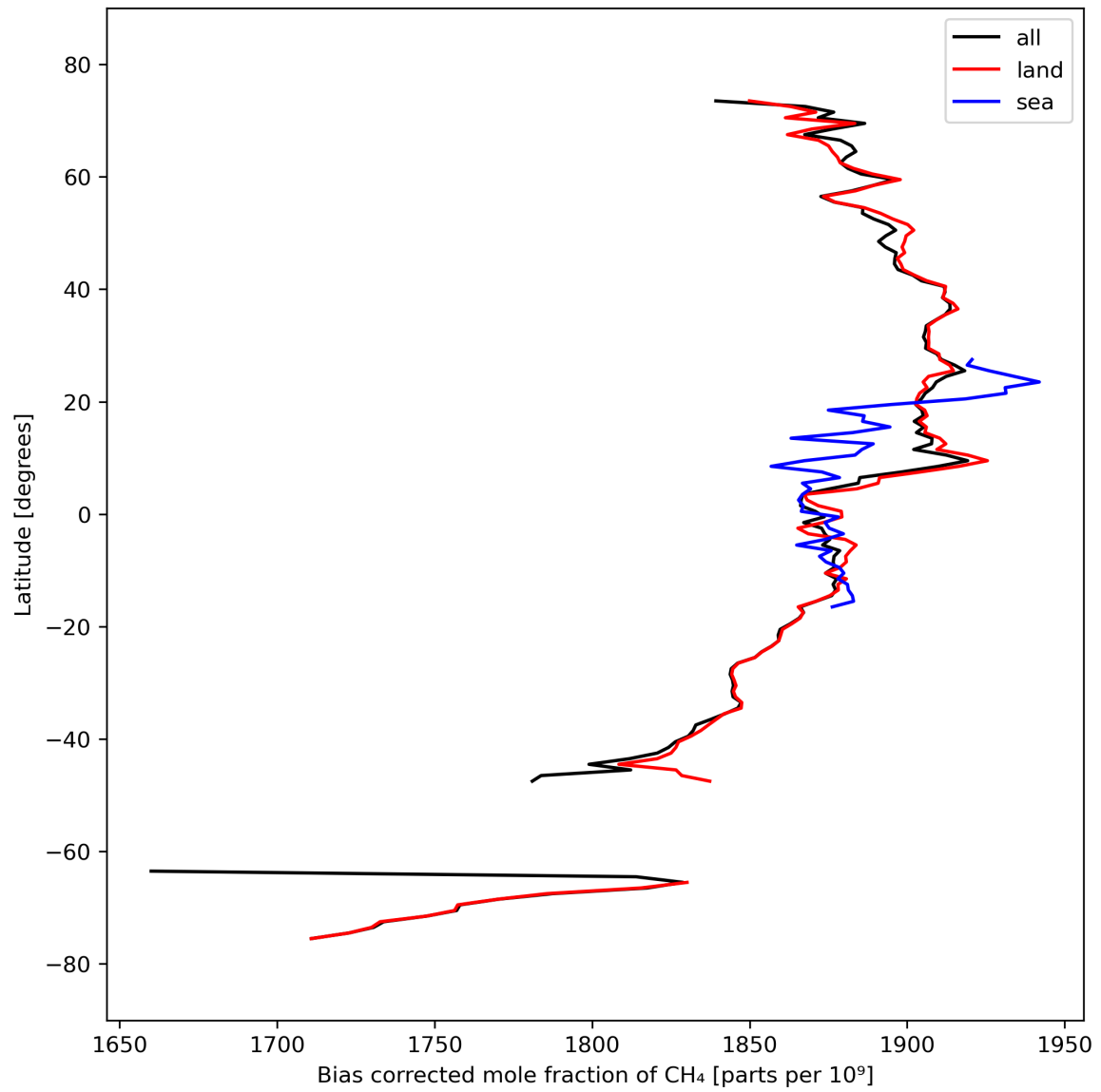
Figure 14: Zonal average of “Bias corrected mole fraction of \text{CH}_4 ” for 2023-09-26 to 2023-09-27.
