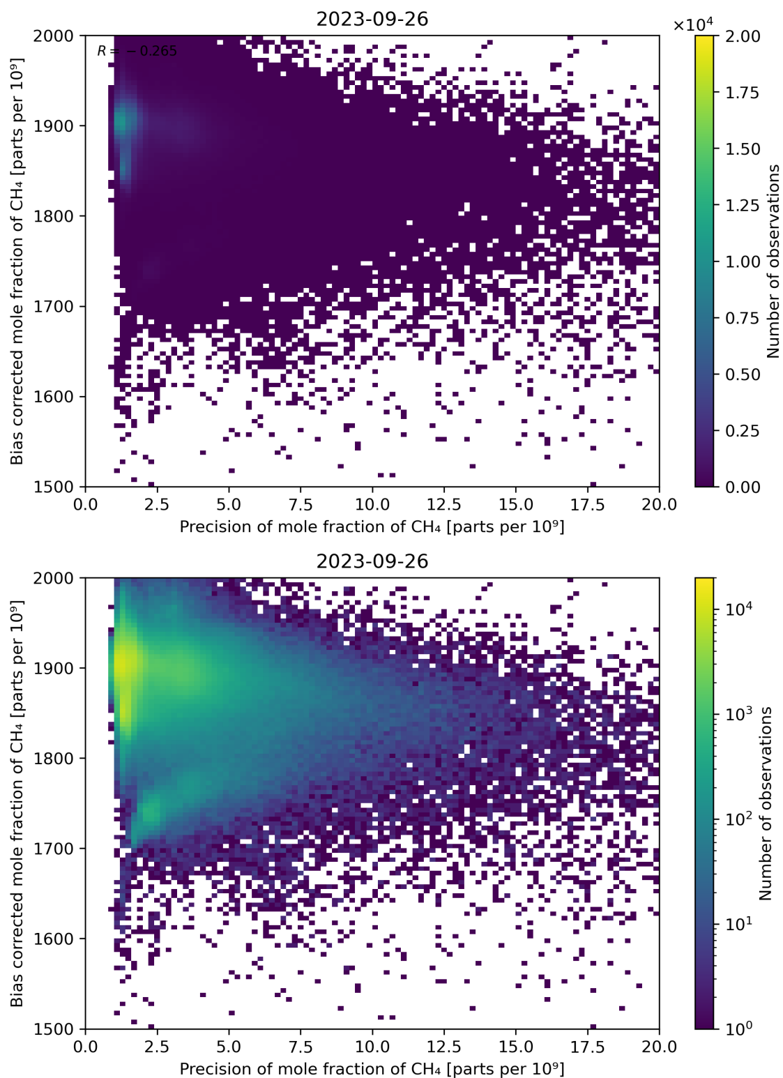
Figure 82: Scatter density plot of “Precision of mole fraction of CH 4 ” against “Bias corrected mole fraction of CH 4 ” for 2023-09-26 to 2023-09-27.
