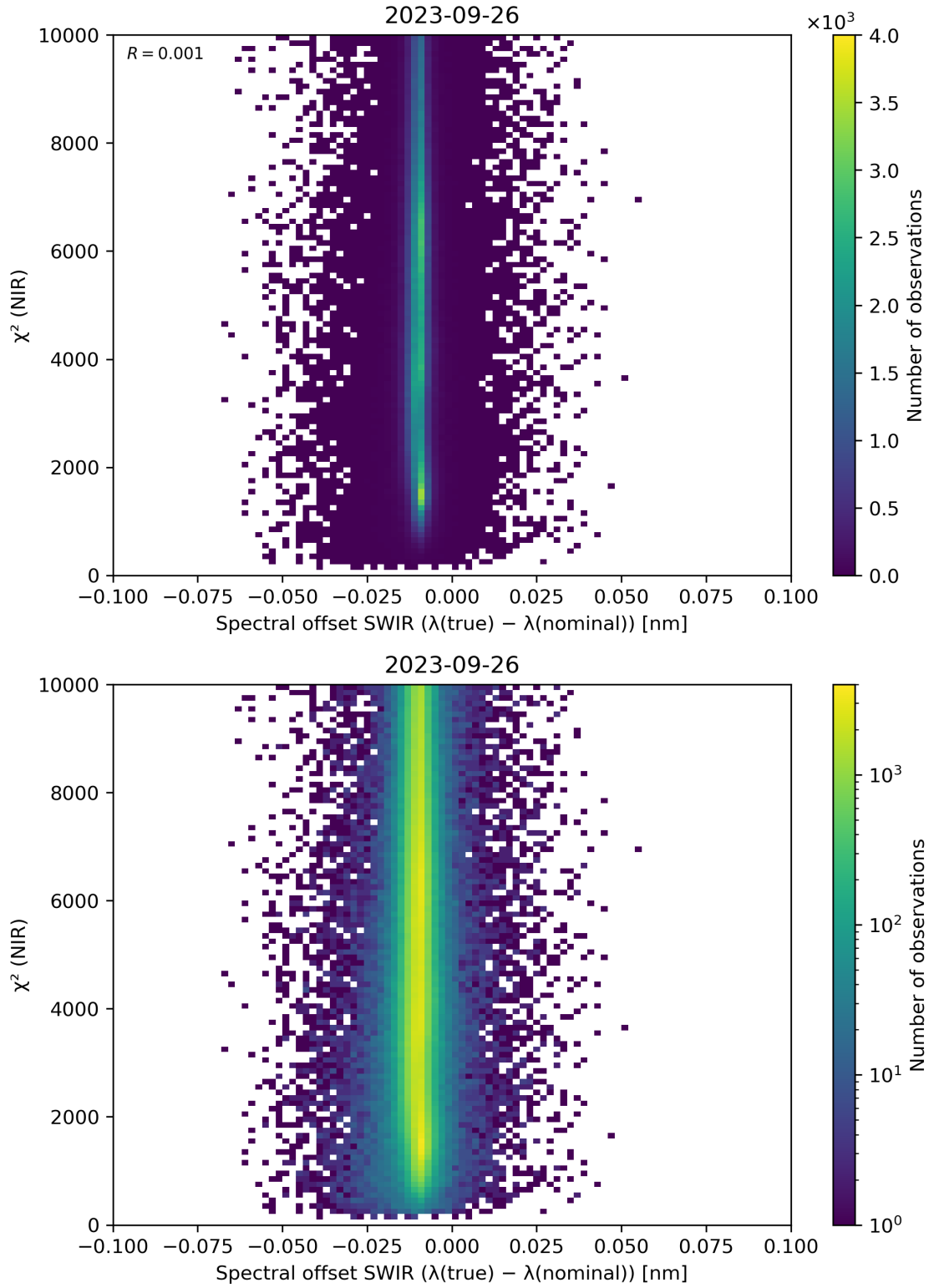
Figure 117: Scatter density plot of “Spectral offset SWIR ( \lambda(\text{true}) - \lambda(\text{nominal}) )” against “ \chi^2 (NIR)” for 2023-09-26 to 2023-09-27.
