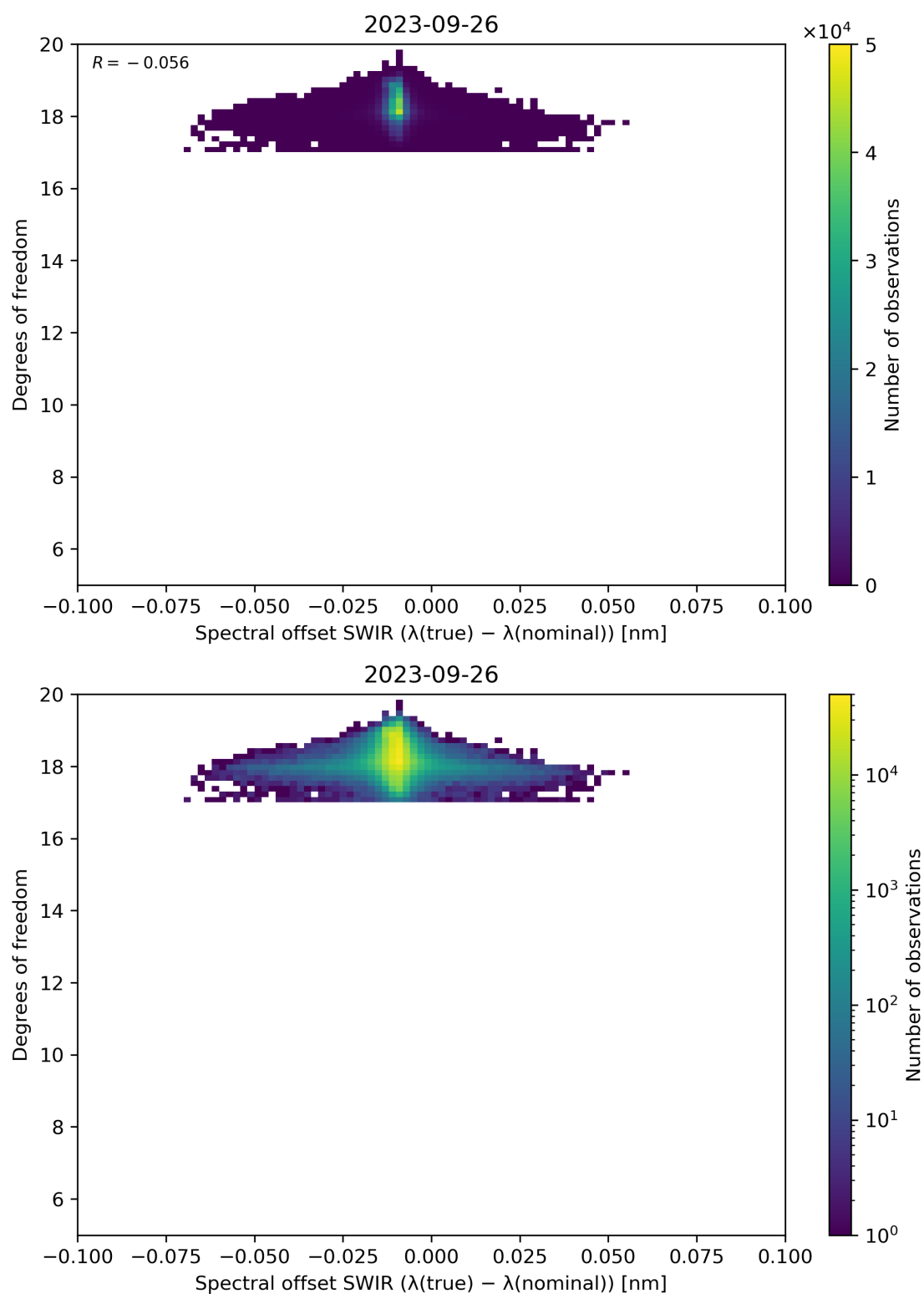
Figure 119: Scatter density plot of “Spectral offset SWIR ( \lambda(\text{true}) - \lambda(\text{nominal}) )” against “Degrees of freedom” for 2023-09-26 to 2023-09-27.
