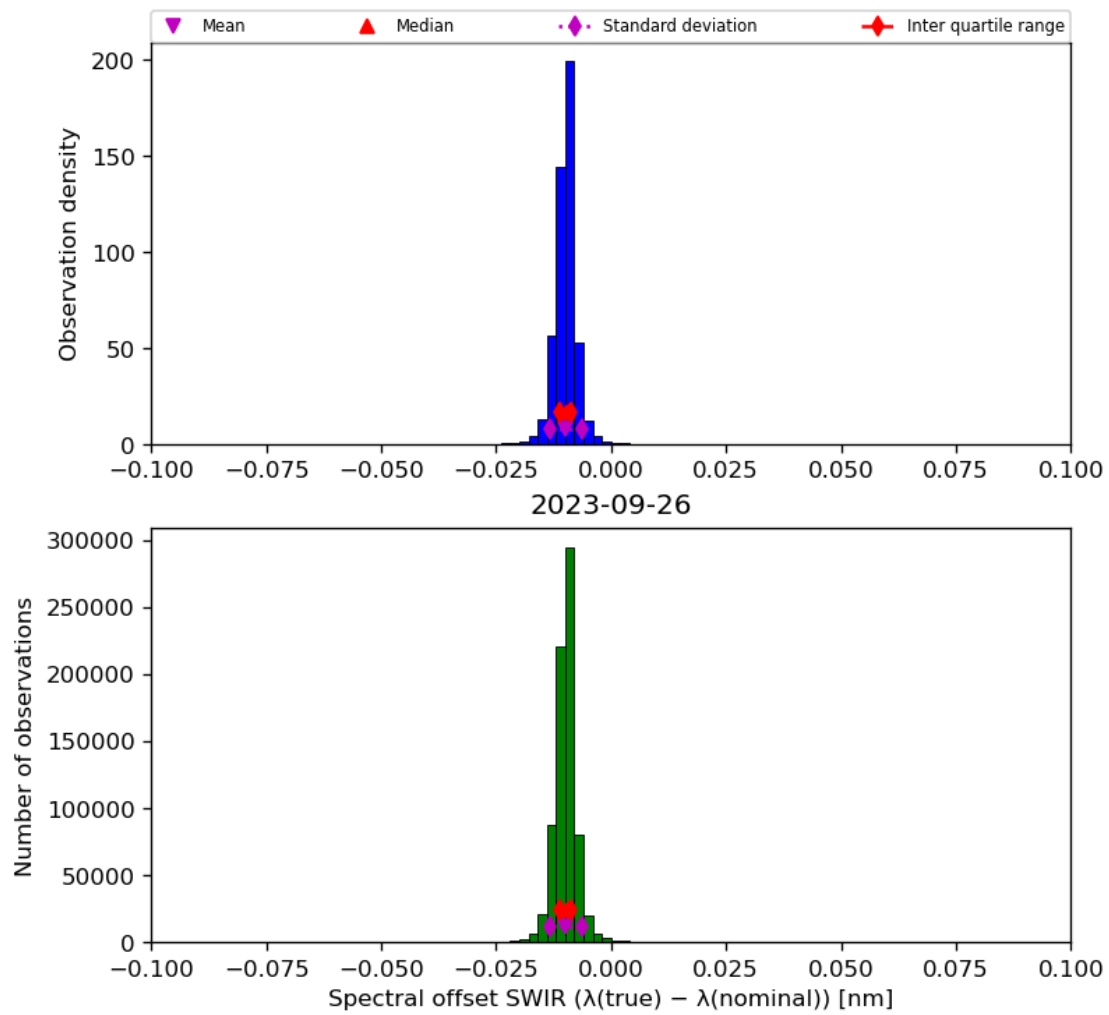
Figure 27: Histogram of “Spectral offset SWIR ( \lambda(\text{true}) - \lambda(\text{nominal}) )” for 2023-09-26 to 2023-09-27
