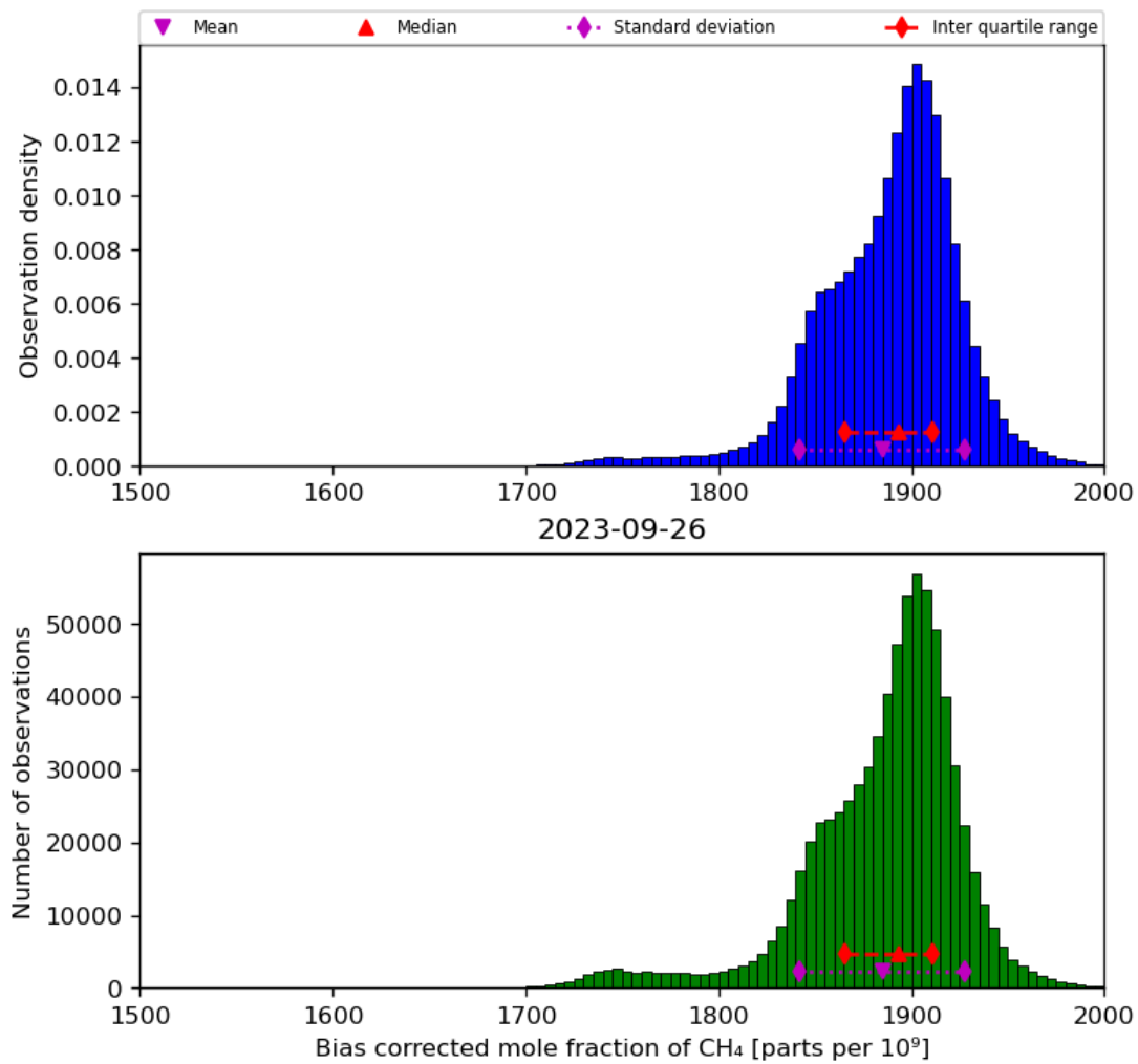
Figure 25: Histogram of “Bias corrected mole fraction of CH 4 ” for 2023-09-26 to 2023-09-27
