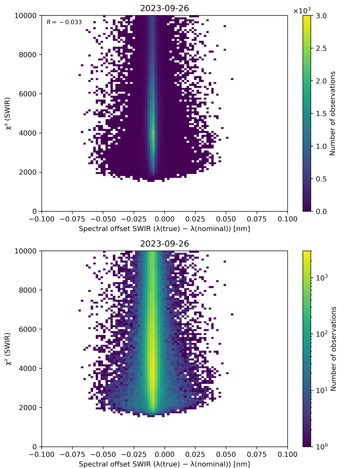
Figure 118: Scatter density plot of “Spectral offset SWIR ( \lambda(\text{true}) - \lambda(\text{nominal}) )” against “ \chi^2 (SWIR)” for 2023-09-26 to 2023-09-27.
