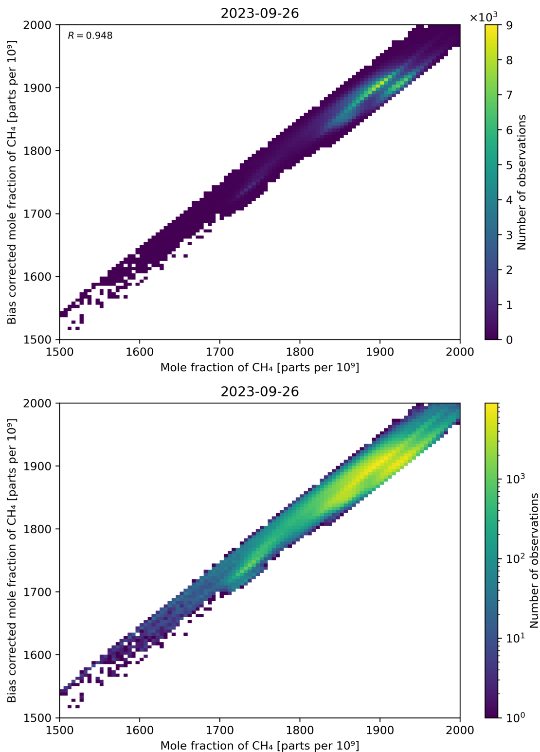
Figure 74: Scatter density plot of “Mole fraction of CH 4 ” against “Bias corrected mole fraction of CH 4 ” for 2023-09-26 to 2023-09-27.
