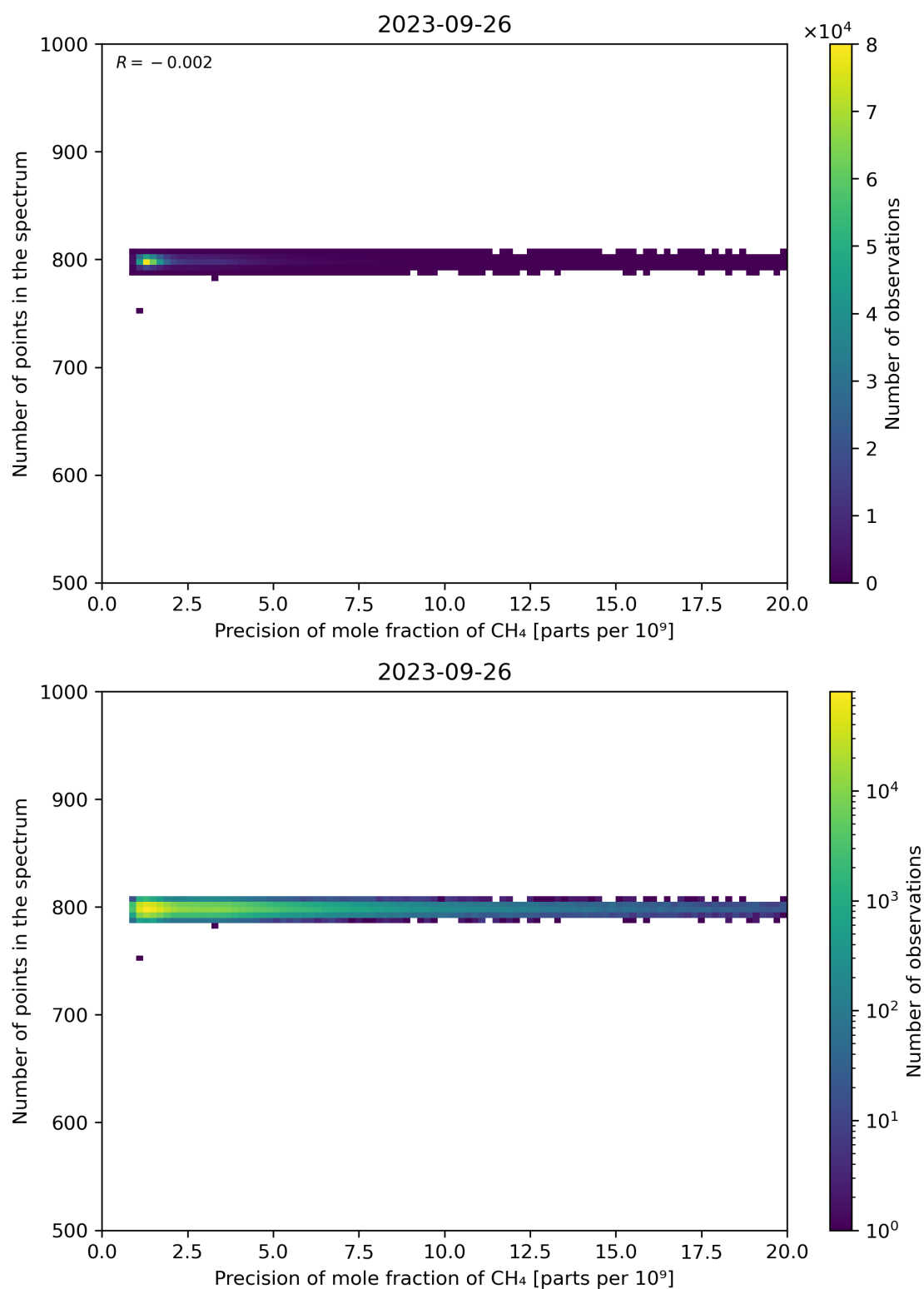
Figure 84: Scatter density plot of “Precision of mole fraction of CH 4 ” against “Number of points in the spectrum” for 2023-09-26 to 2023-09-27.
