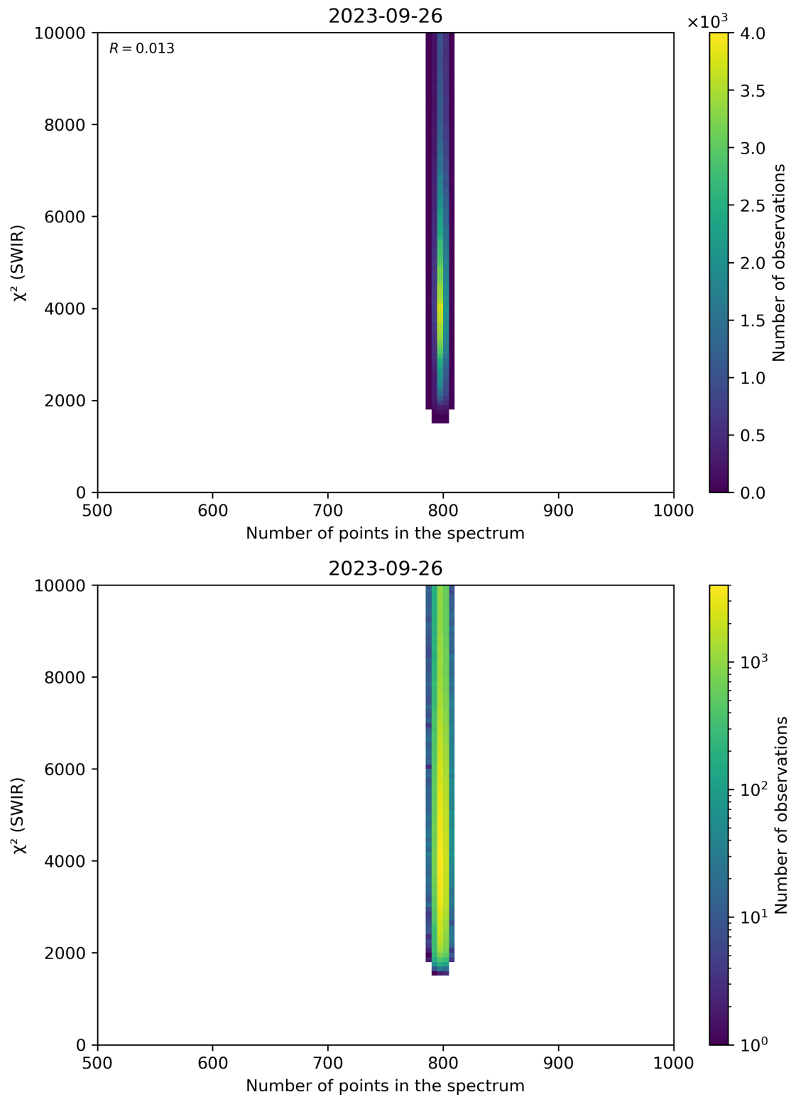
Figure 89: Scatter density plot of “Number of points in the spectrum” against “ \chi^2 (SWIR)” for 2023-09-26 to 2023-09-27.
