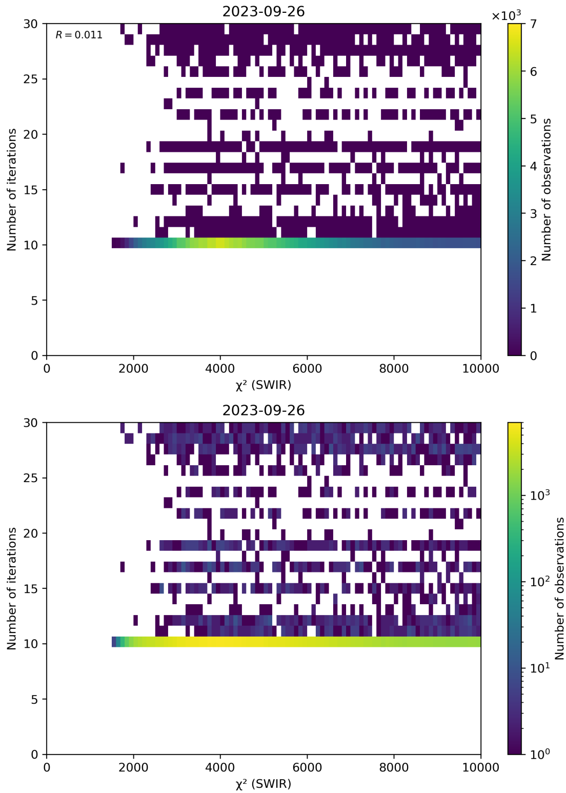
Figure 50: Scatter density plot of “ \chi^2 (SWIR)” against “Number of iterations” for 2023-09-26 to 2023-09-27.
