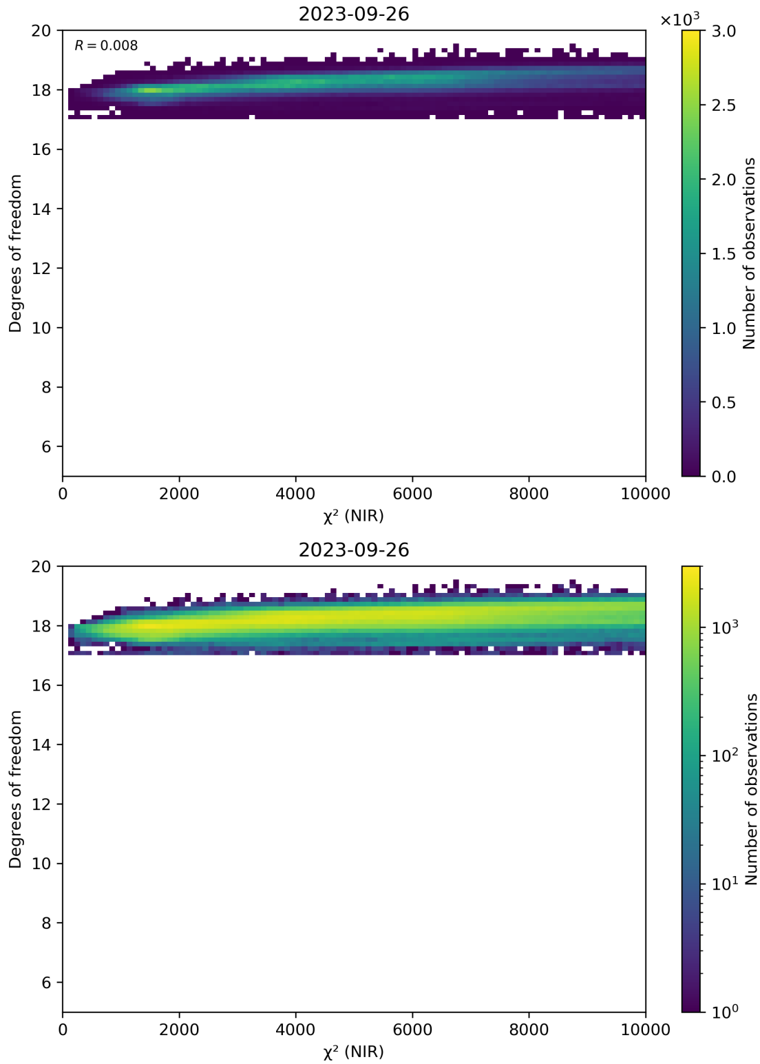
Figure 44: Scatter density plot of “ \chi^2 (NIR)” against “Degrees of freedom” for 2023-09-26 to 2023-09-27.
