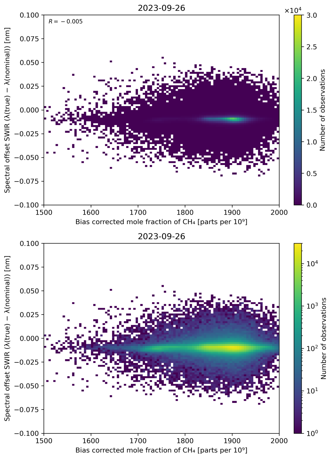
Figure 69: Scatter density plot of “Bias corrected mole fraction of \text{CH}_4 ” against “Spectral offset SWIR ( \lambda(\text{true}) - \lambda(\text{nominal}) )” for 2023-09-26 to 2023-09-27.
