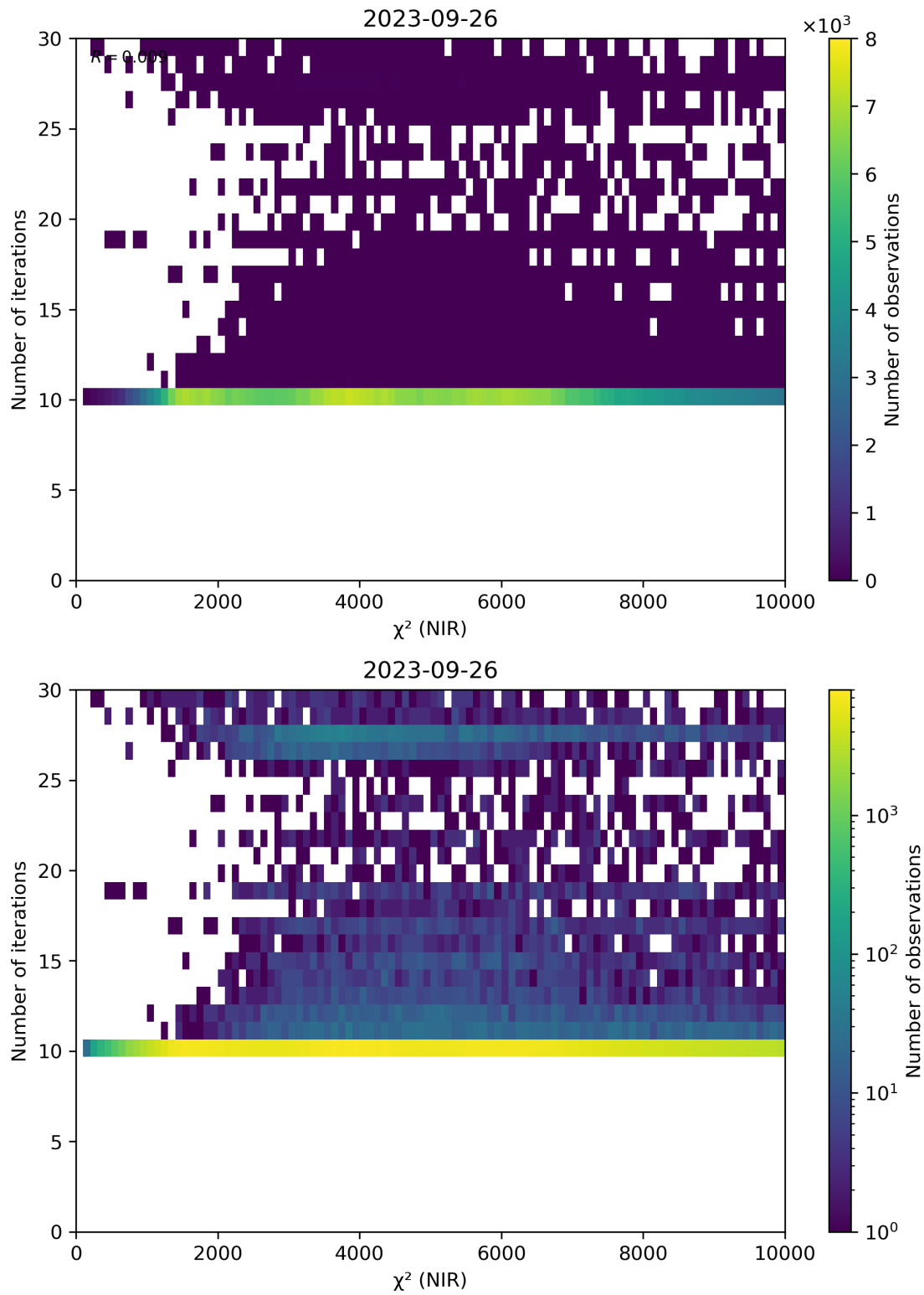
Figure 46: Scatter density plot of “ \chi^2 (NIR)” against “Number of iterations” for 2023-09-26 to 2023-09-27.
