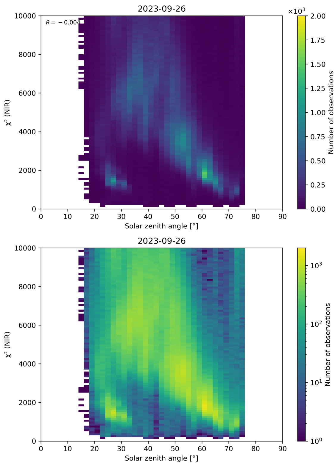
Figure 94: Scatter density plot of “Solar zenith angle” against “ \chi^2 (NIR)” for 2023-09-26 to 2023-09-27.
