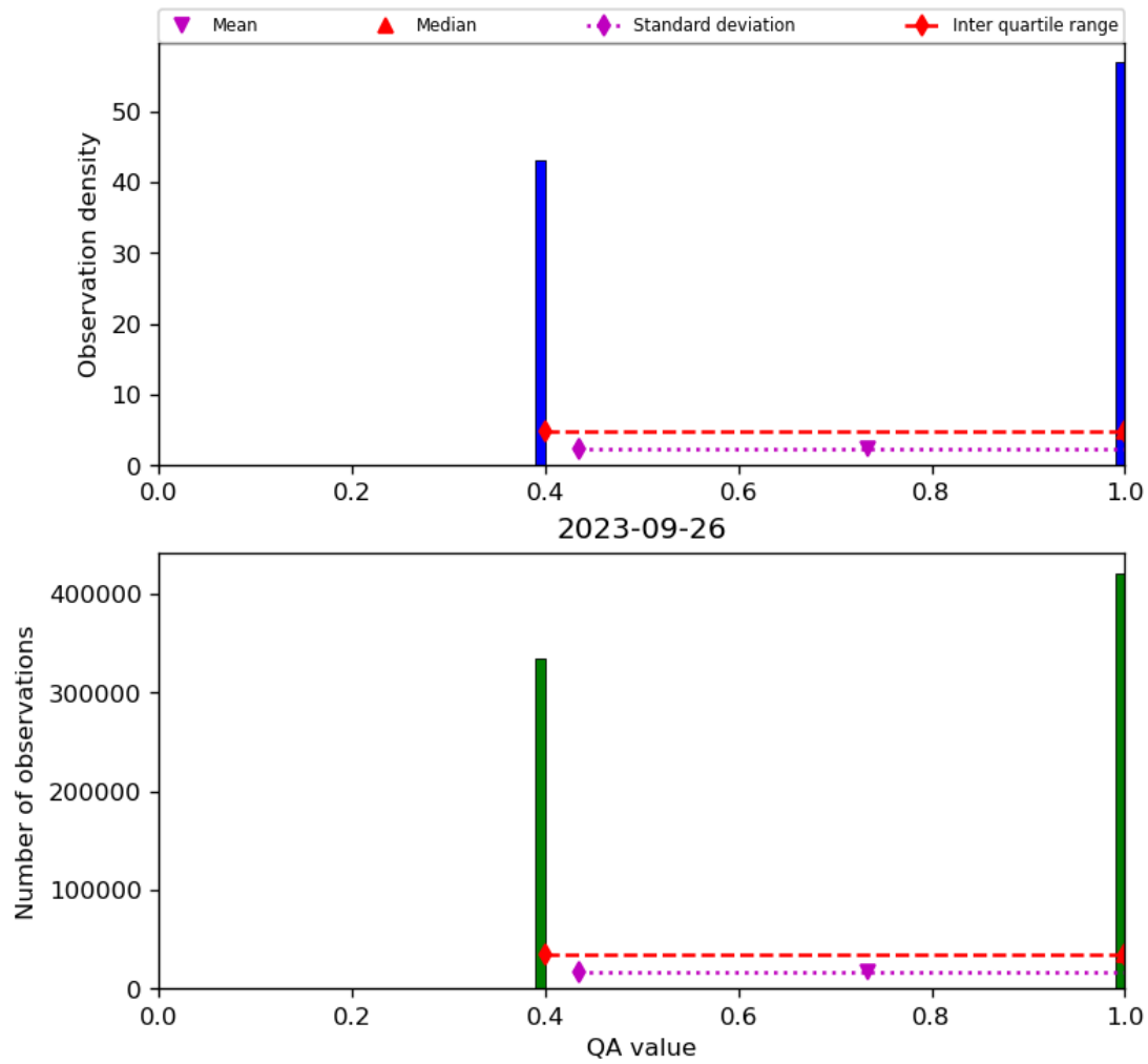
Figure 22: Histogram of “QA value” for 2023-09-26 to 2023-09-27
