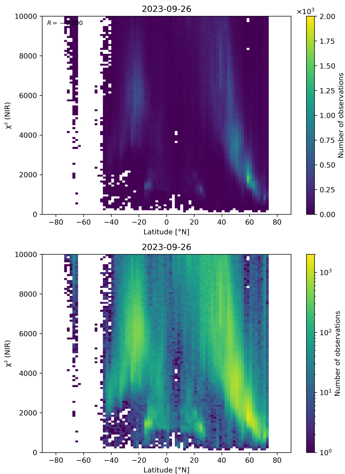
Figure 53: Scatter density plot of “Latitude” against “ \chi^2 (NIR)” for 2023-09-26 to 2023-09-27.
