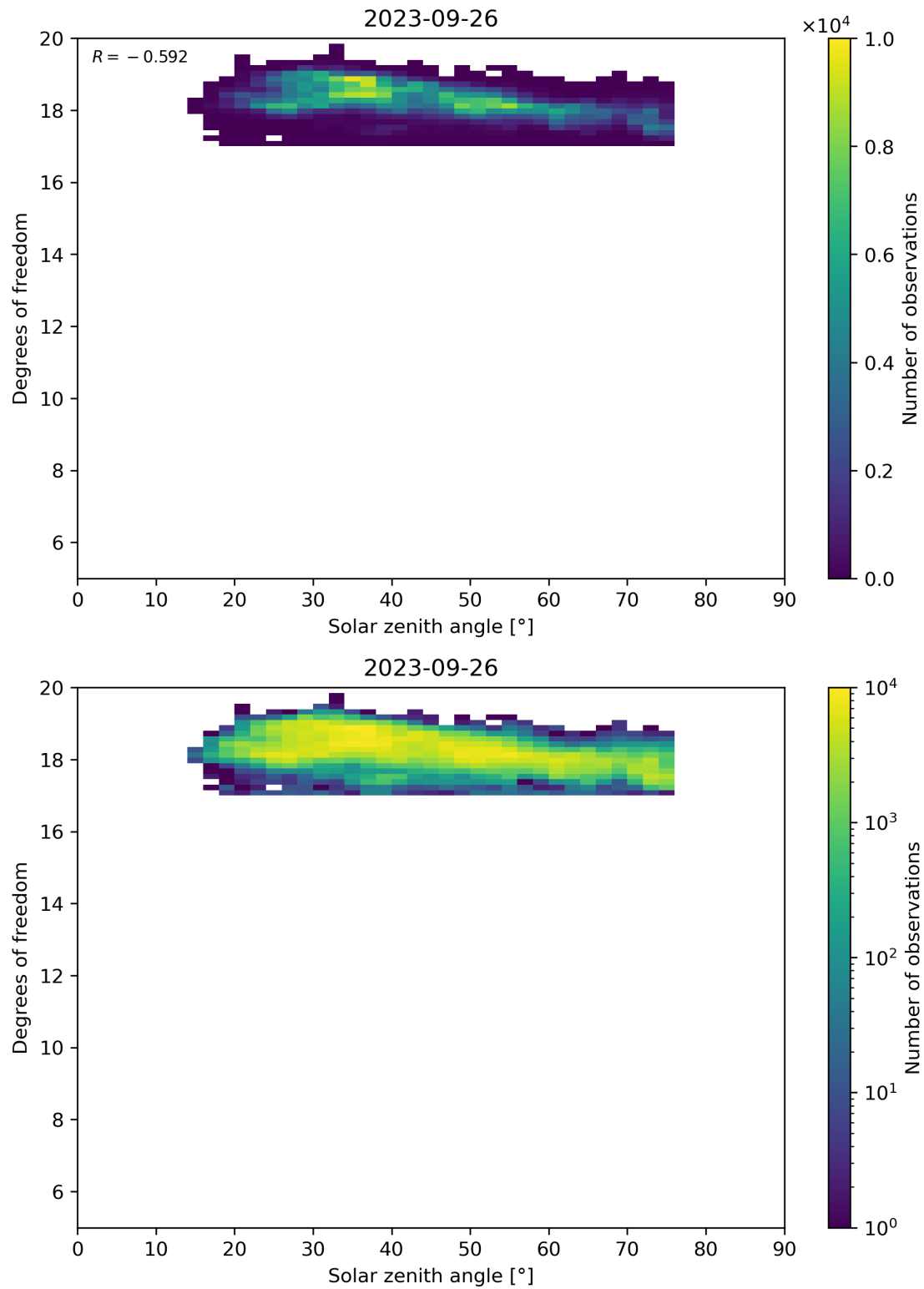
Figure 96: Scatter density plot of “Solar zenith angle” against “Degrees of freedom” for 2023-09-26 to 2023-09-27.
