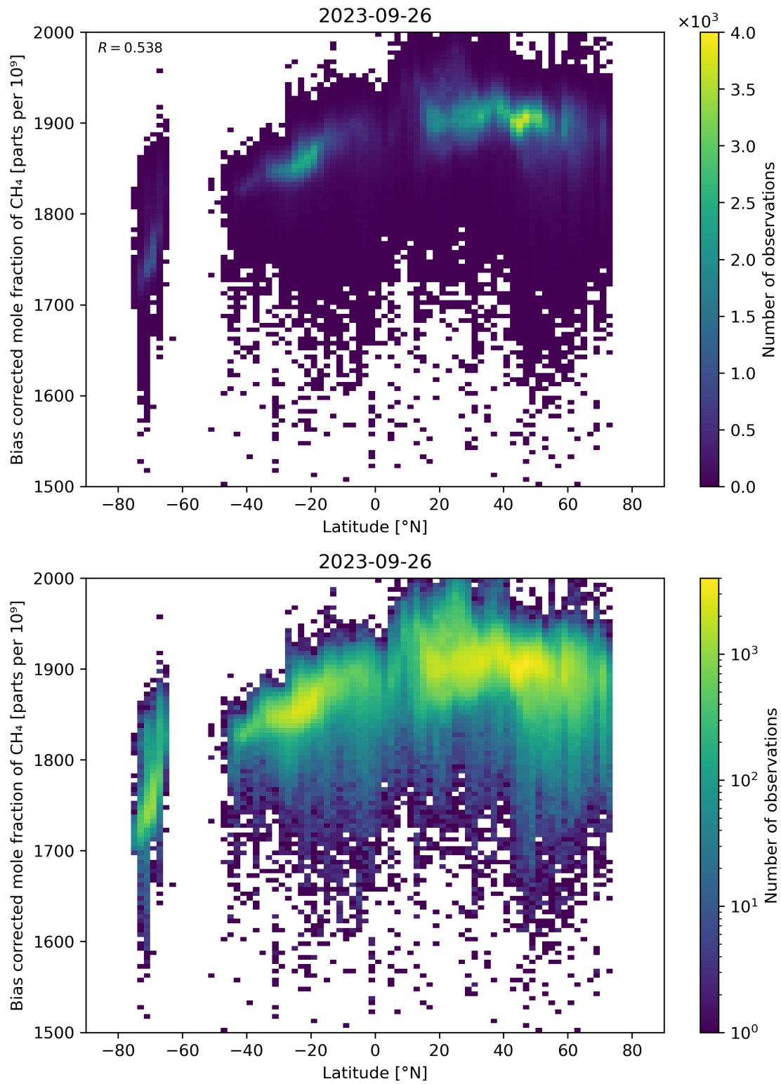
Figure 58: Scatter density plot of “Latitude” against “Bias corrected mole fraction of CH 4 ” for 2023-09-26 to 2023-09-27.
