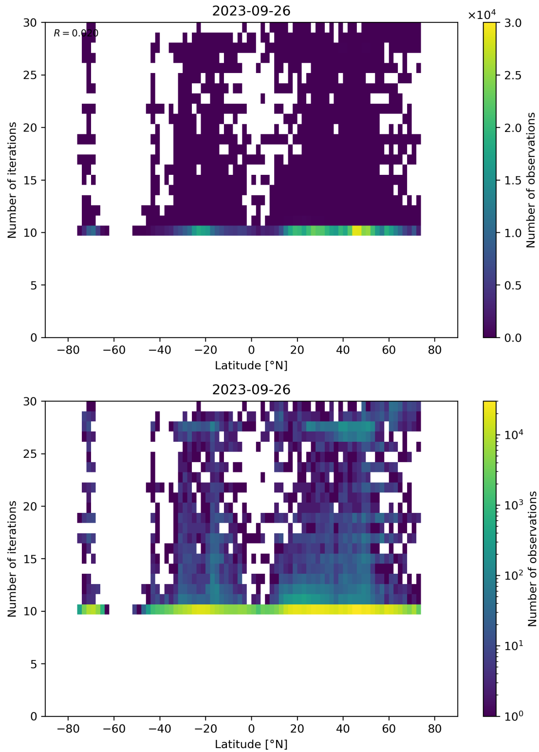
Figure 60: Scatter density plot of “Latitude” against “Number of iterations” for 2023-09-26 to 2023-09-27.
