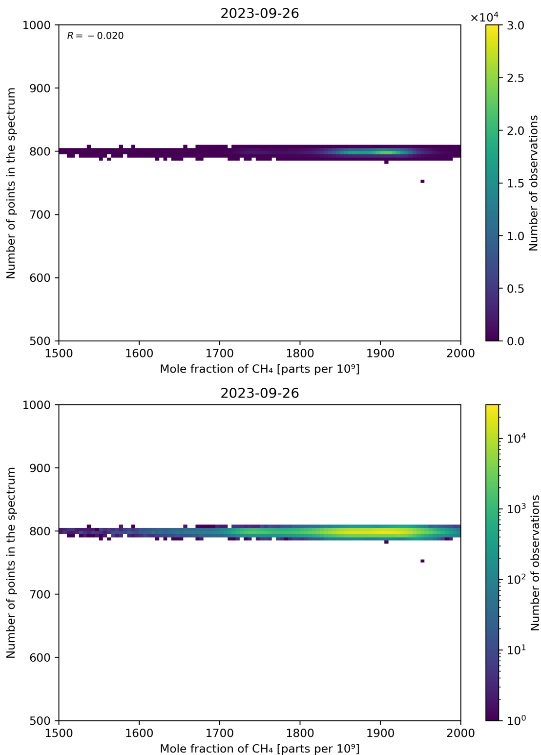
Figure 77: Scatter density plot of “Mole fraction of CH 4 ” against “Number of points in the spectrum” for 2023-09-26 to 2023-09-27.
