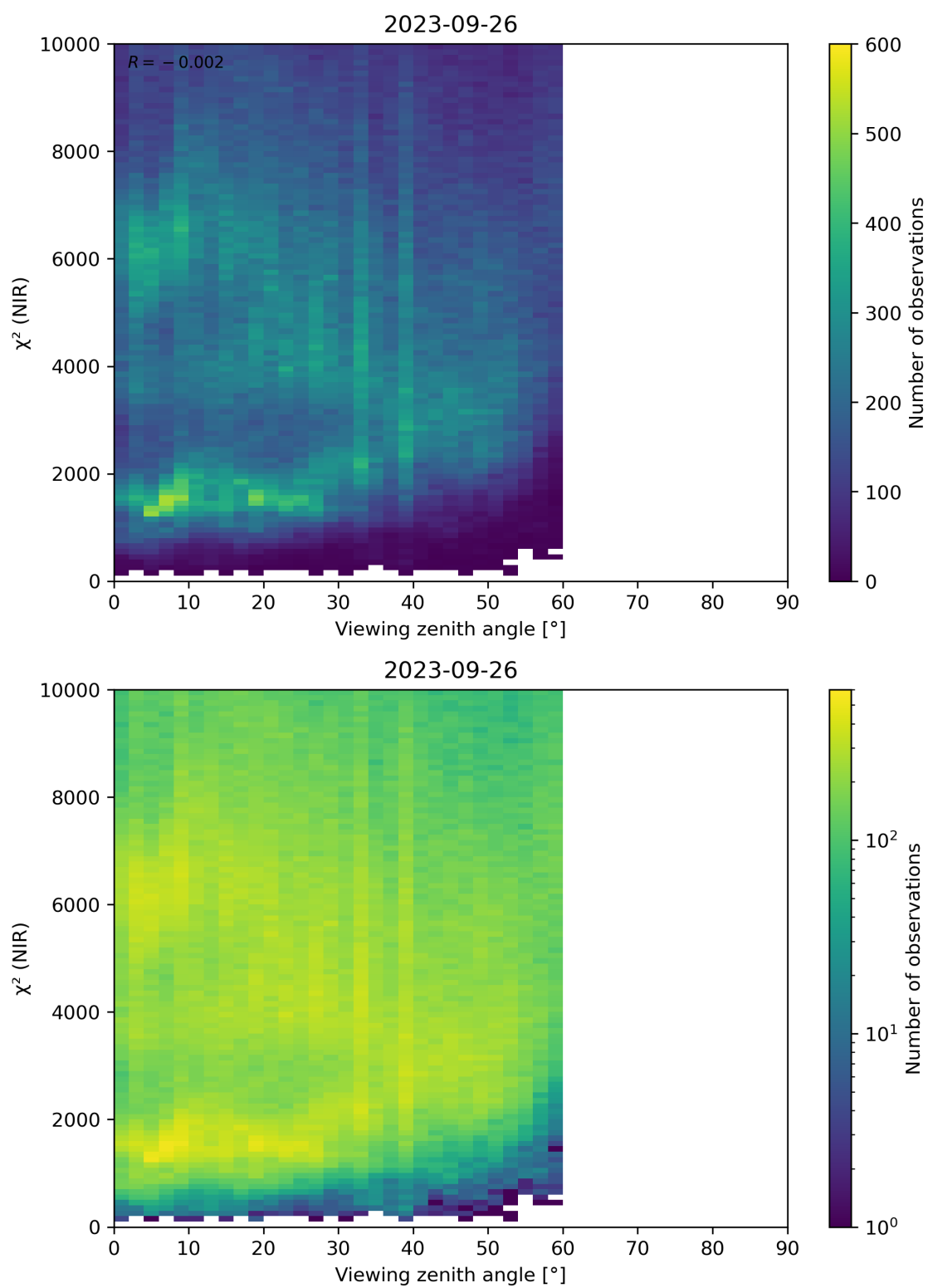
Figure 105: Scatter density plot of “Viewing zenith angle” against “ \chi^2 (NIR)” for 2023-09-26 to 2023-09-27.
