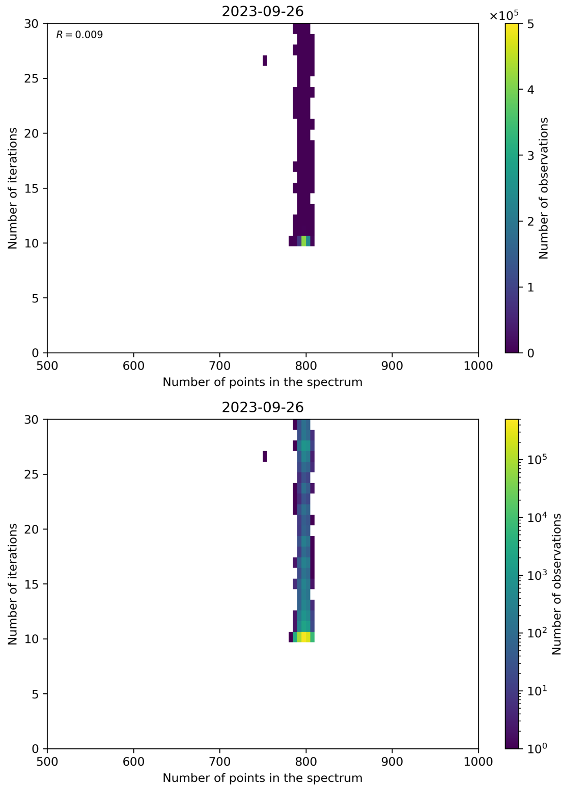
Figure 92: Scatter density plot of “Number of points in the spectrum” against “Number of iterations” for 2023-09-26 to 2023-09-27.
