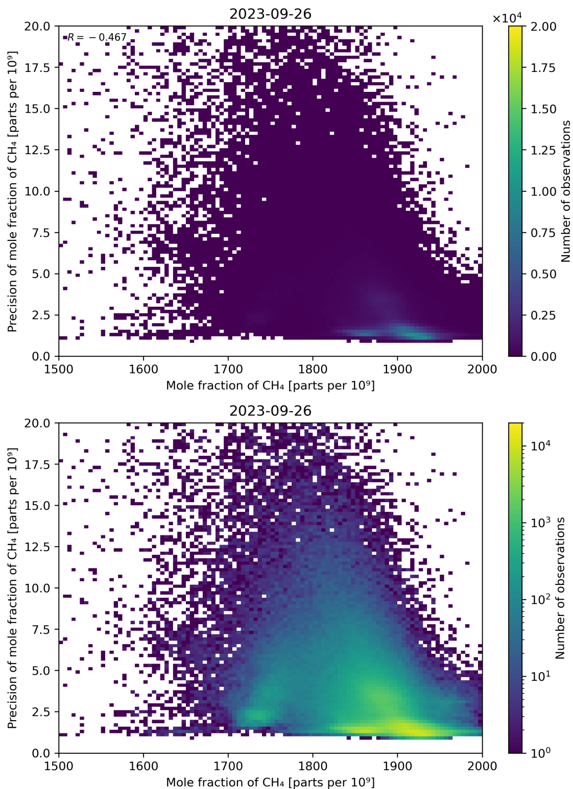
Figure 75: Scatter density plot of “Mole fraction of CH 4 ” against “Precision of mole fraction of CH 4 ” for 2023-09-26 to 2023-09-27.
