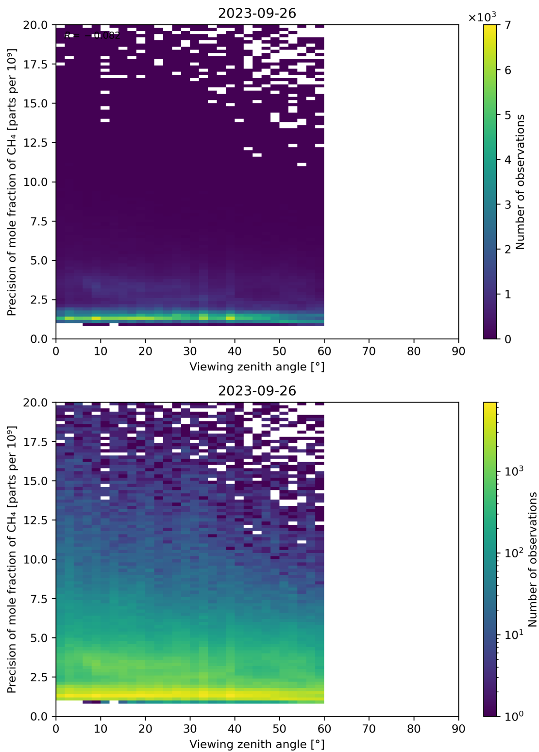
Figure 112: Scatter density plot of “Viewing zenith angle” against “Precision of mole fraction of CH 4 ” for 2023-09-26 to 2023-09-27.
