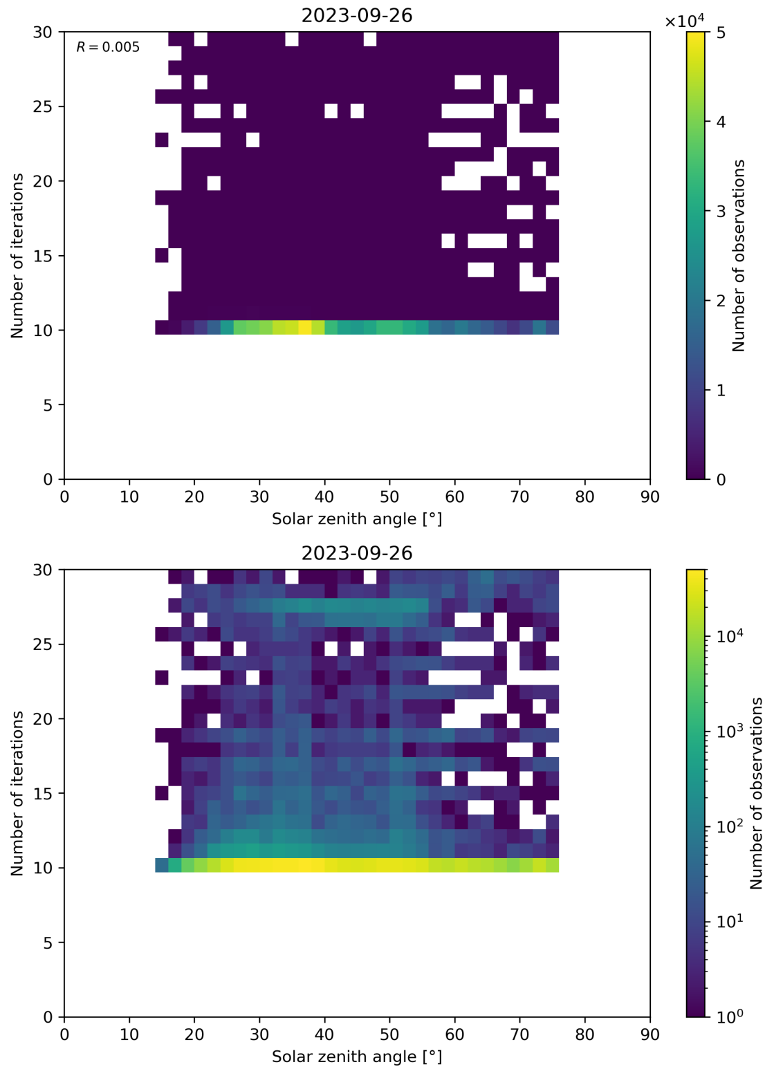
Figure 102: Scatter density plot of “Solar zenith angle” against “Number of iterations” for 2023-09-26 to 2023-09-27.
