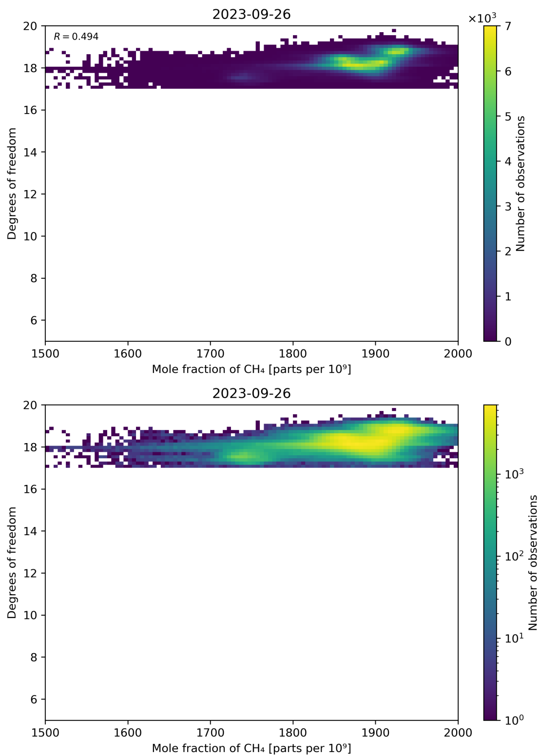
Figure 72: Scatter density plot of “Mole fraction of CH 4 ” against “Degrees of freedom” for 2023-09-26 to 2023-09-27.
