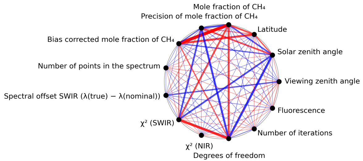
Figure 1: Map of correlation graph for 2023-09-26 to 2023-09-27.
