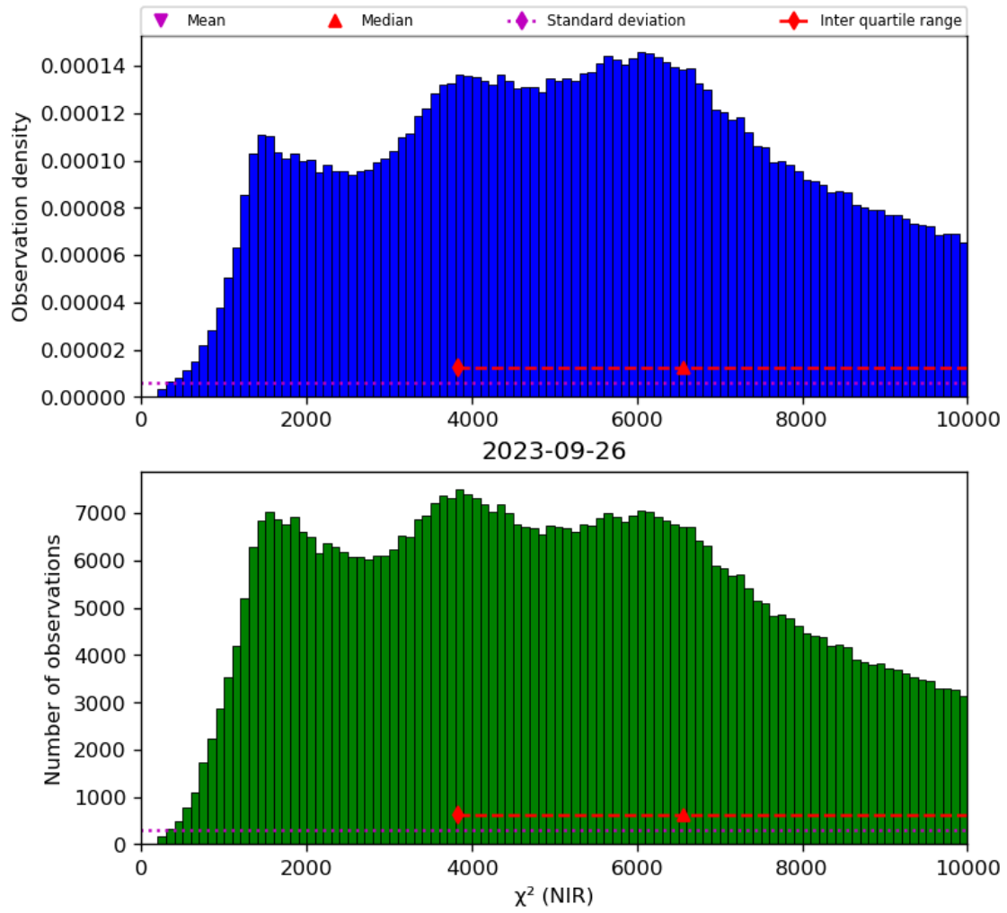
Figure 29: Histogram of “ \chi^2 (NIR)” for 2023-09-26 to 2023-09-27
