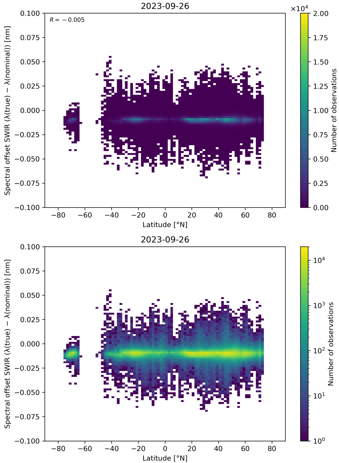
Figure 62: Scatter density plot of “Latitude” against “Spectral offset SWIR ( \lambda(\text{true}) - \lambda(\text{nominal}) )” for 2023-09-26 to 2023-09-27.
