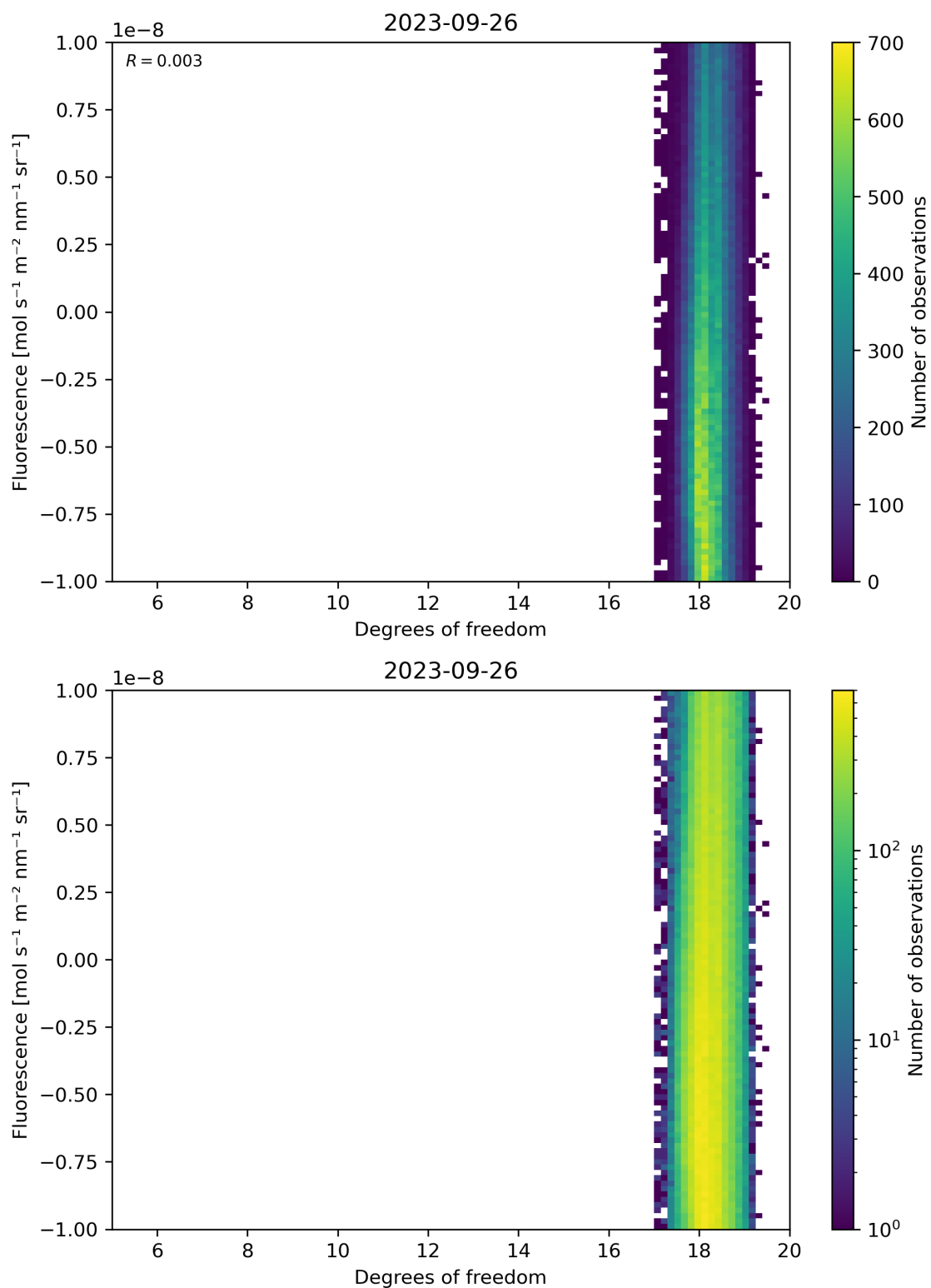
Figure 51: Scatter density plot of “Degrees of freedom” against “Fluorescence” for 2023-09-26 to 2023-09-27.
