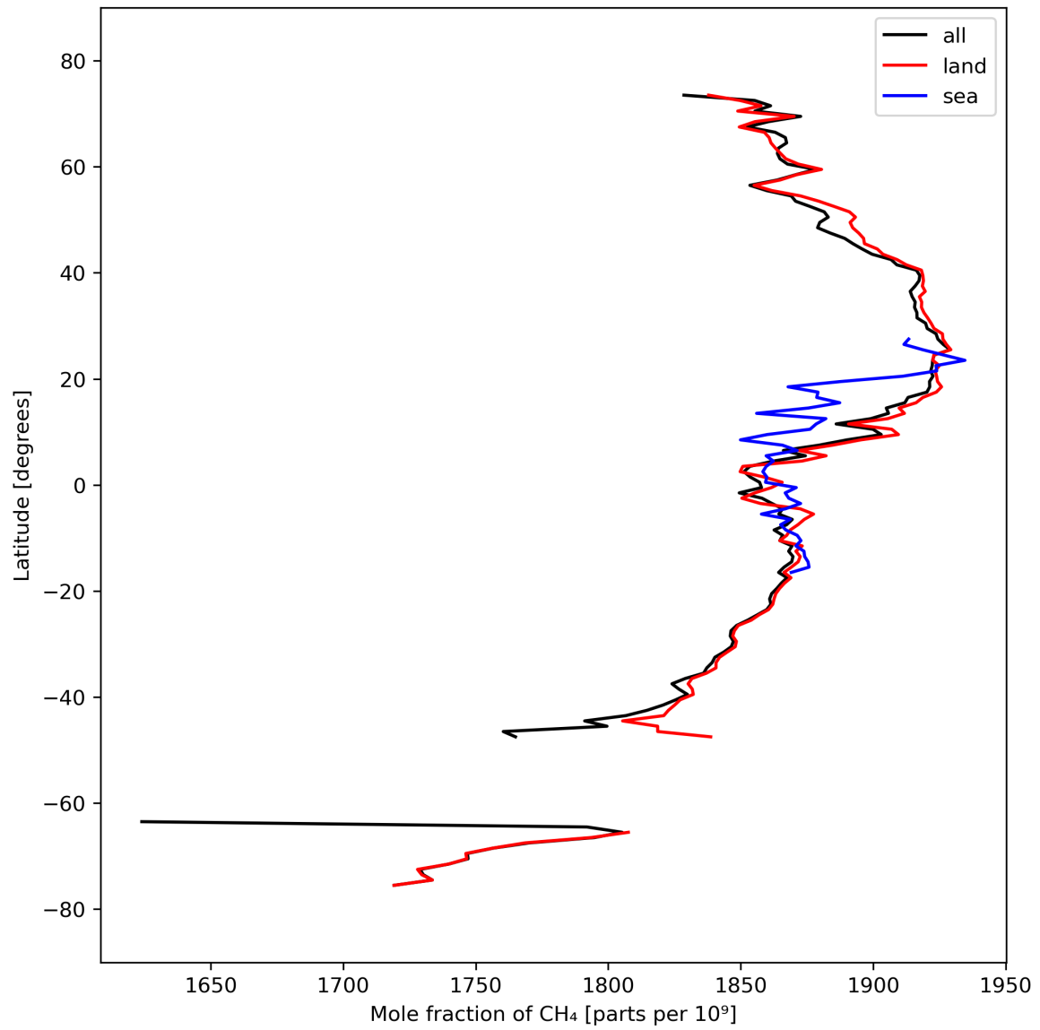
Figure 12: Zonal average of “Mole fraction of \text{CH}_4 ” for 2023-09-26 to 2023-09-27.
