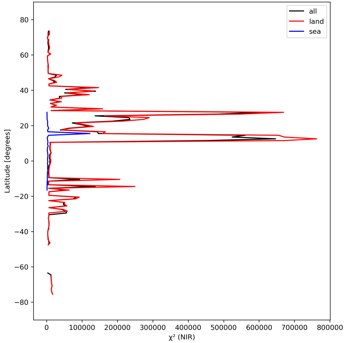
Figure 18: Zonal average of “ \chi^2 (NIR)” for 2023-09-26 to 2023-09-27.
