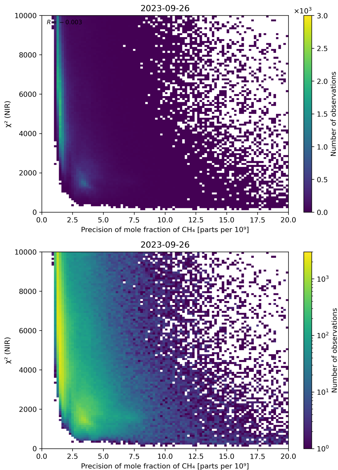
Figure 78: Scatter density plot of “Precision of mole fraction of \text{CH}_4 ” against “ \chi^2 (NIR)” for 2023-09-26 to 2023-09-27.
