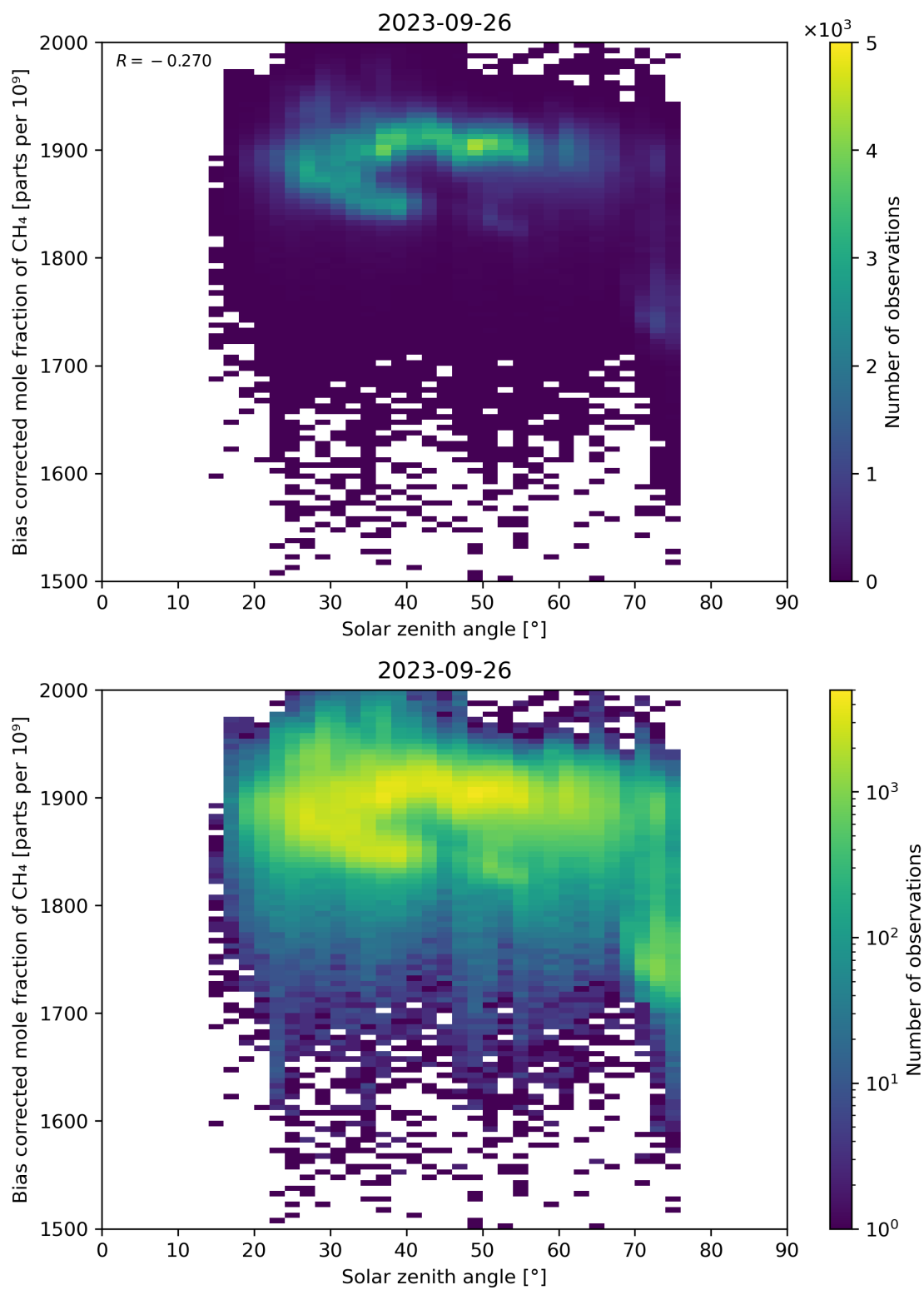
Figure 100: Scatter density plot of “Solar zenith angle” against “Bias corrected mole fraction of CH 4 ” for 2023-09-26 to 2023-09-27.
