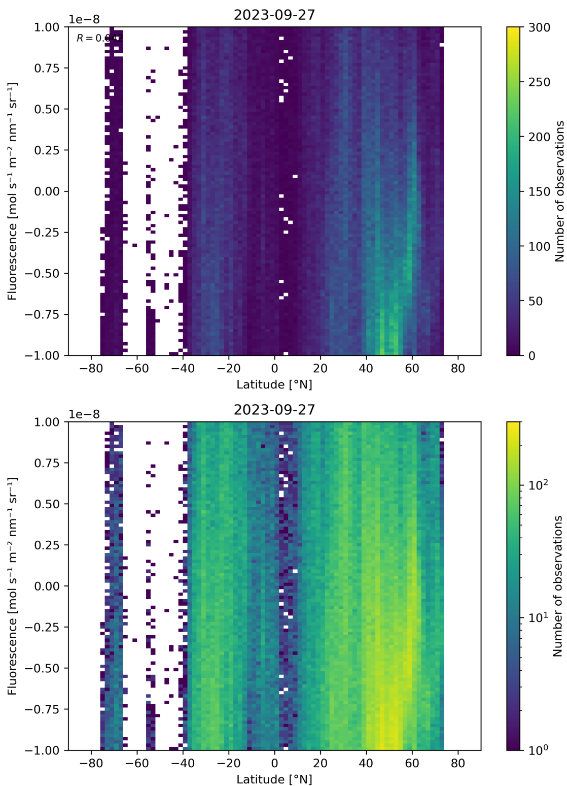
Figure 56: Scatter density plot of “Latitude” against “Fluorescence” for 2023-09-26 to 2023-09-28.
