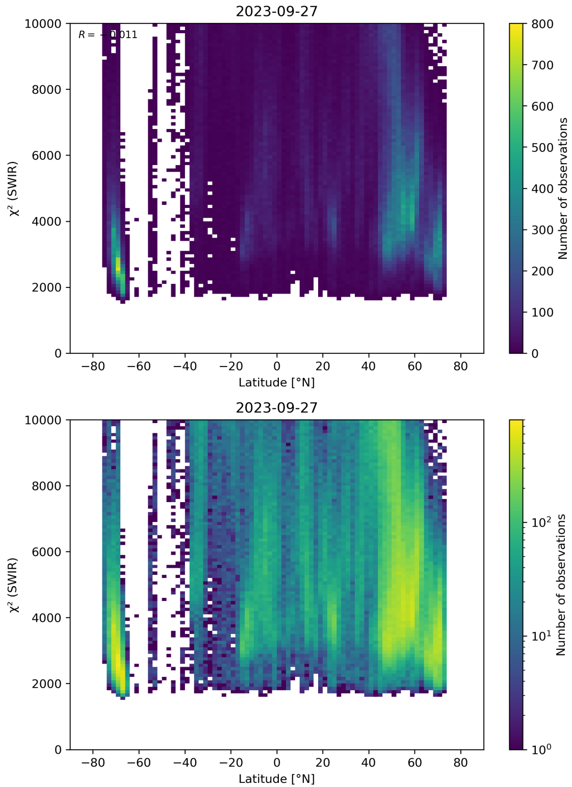
Figure 54: Scatter density plot of “Latitude” against “ \chi^2 (SWIR)” for 2023-09-26 to 2023-09-28.
