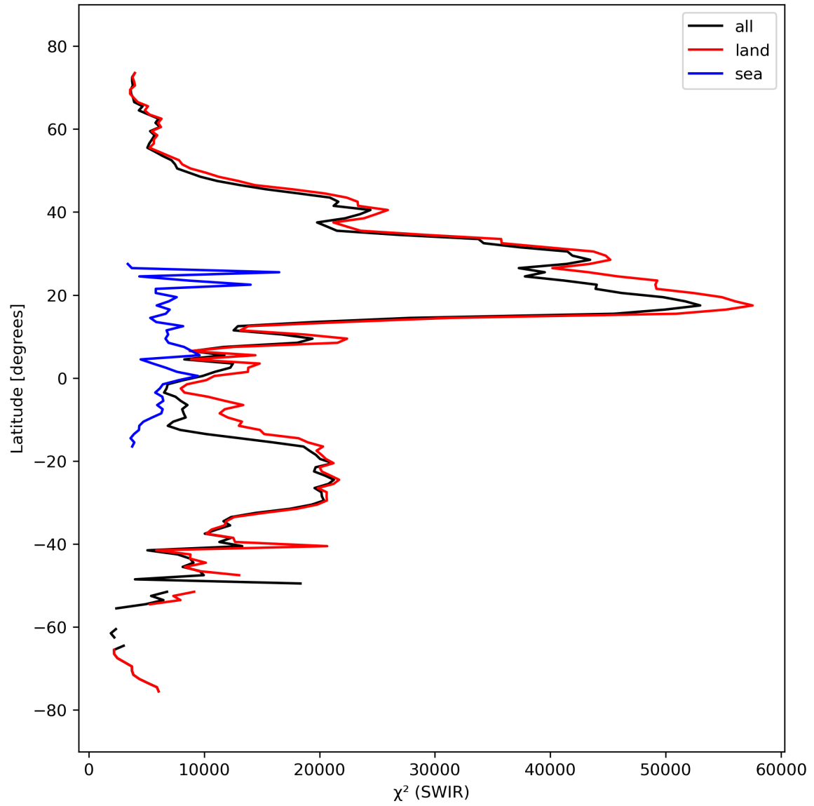
Figure 17: Zonal average of “ \chi^2 (SWIR)” for 2023-09-26 to 2023-09-28.
