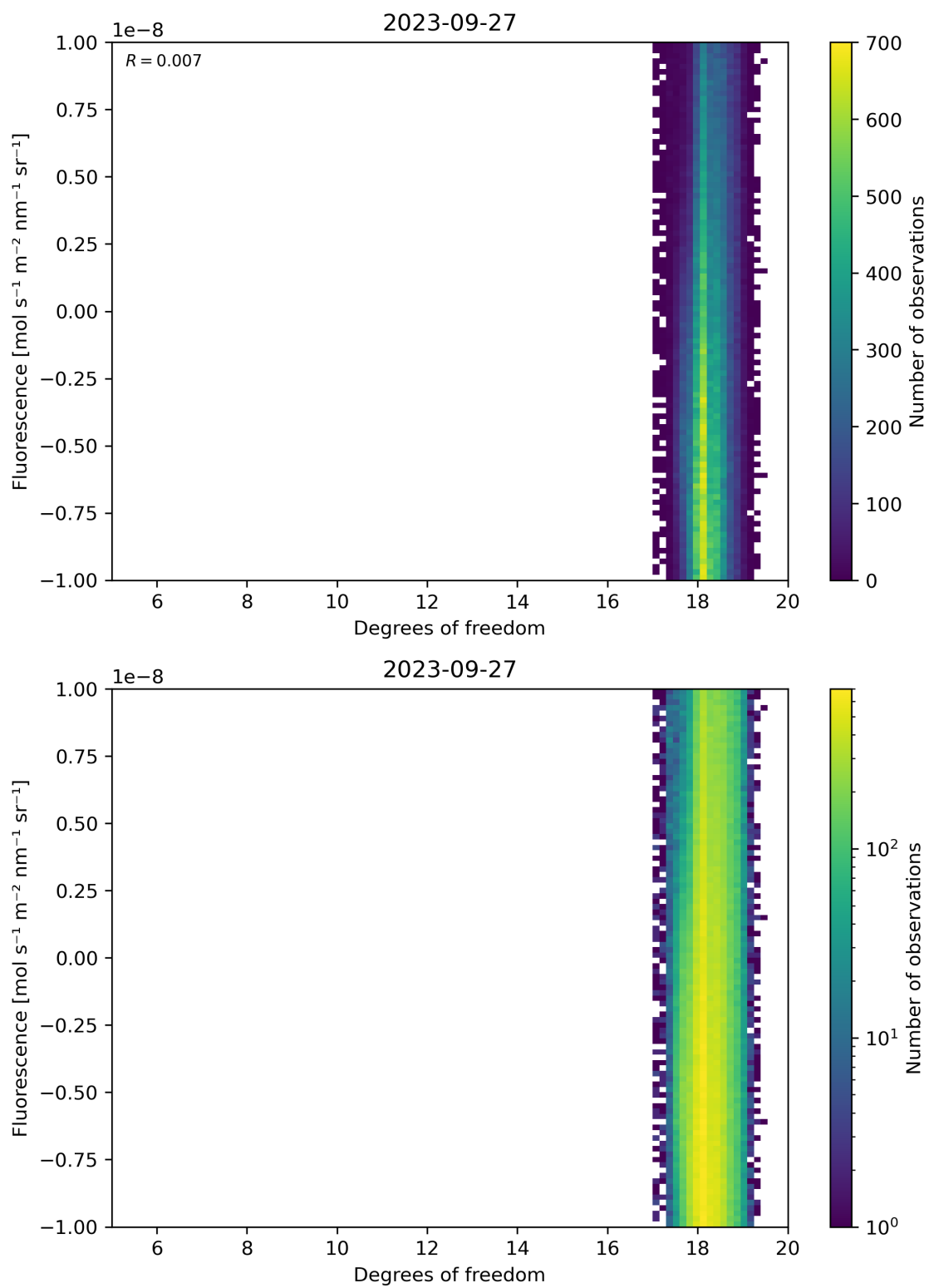
Figure 51: Scatter density plot of “Degrees of freedom” against “Fluorescence” for 2023-09-26 to 2023-09-28.
