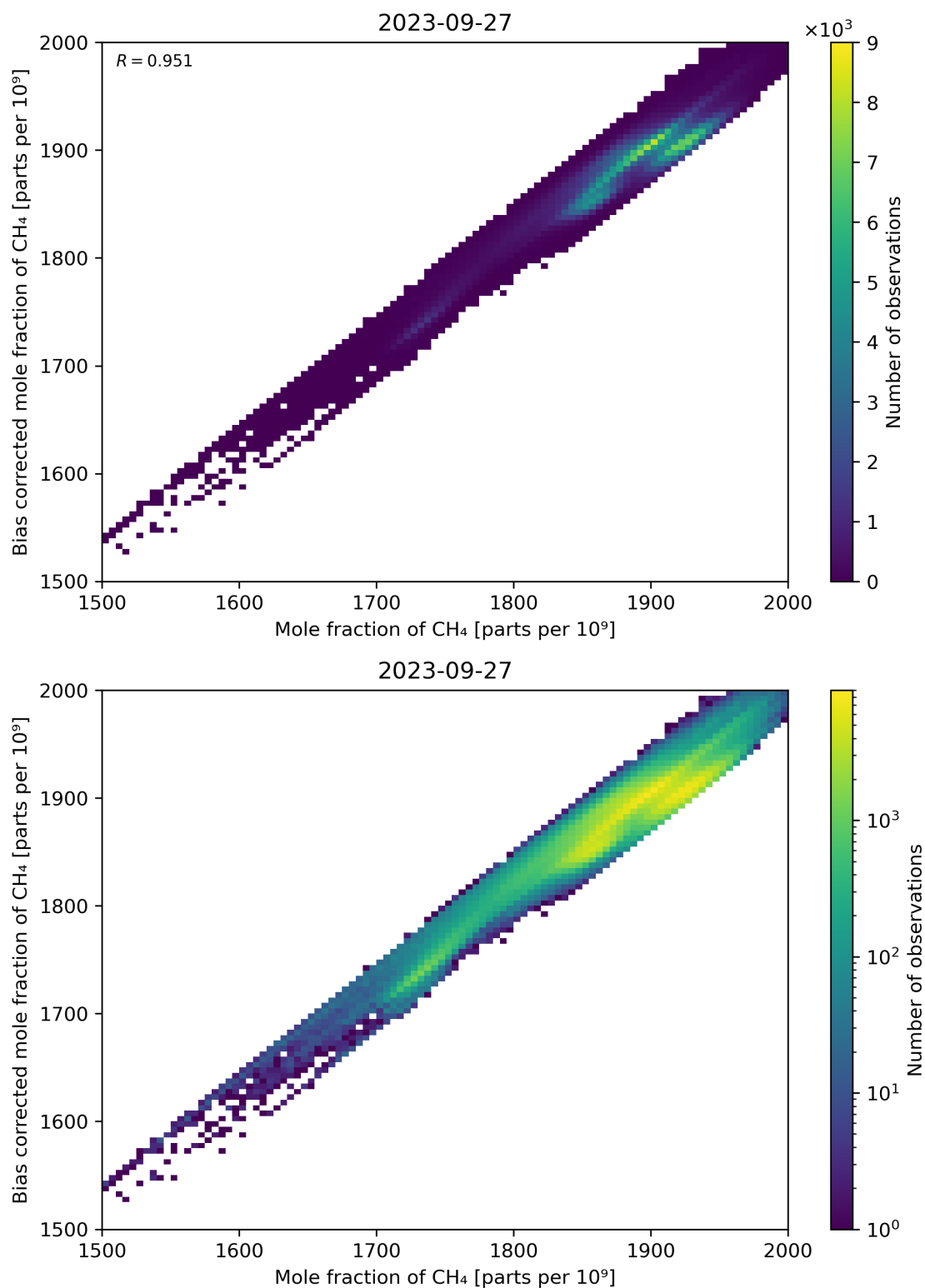
Figure 74: Scatter density plot of “Mole fraction of CH 4 ” against “Bias corrected mole fraction of CH 4 ” for 2023-09-26 to 2023-09-28.
