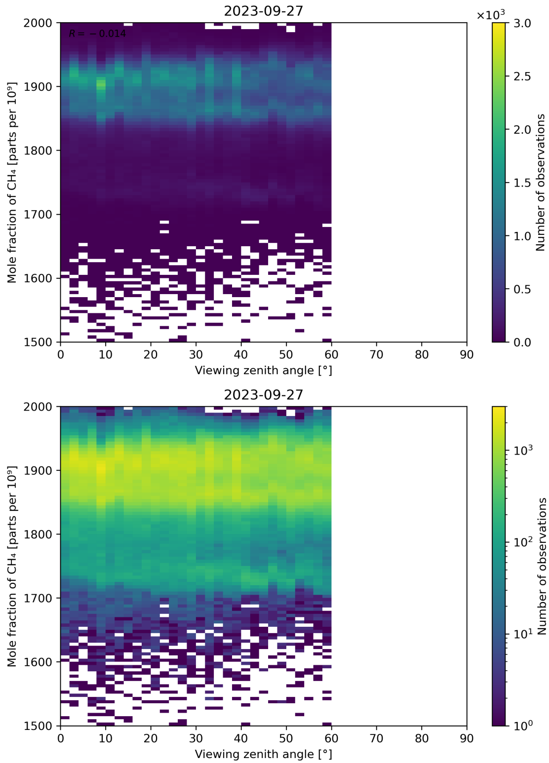
Figure 110: Scatter density plot of “Viewing zenith angle” against “Mole fraction of CH 4 ” for 2023-09-26 to 2023-09-28.
