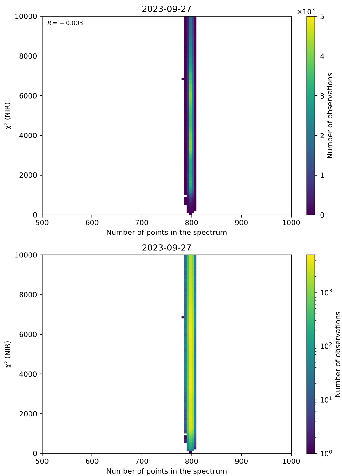
Figure 88: Scatter density plot of “Number of points in the spectrum” against “ \chi^2 (NIR)” for 2023-09-26 to 2023-09-28.
