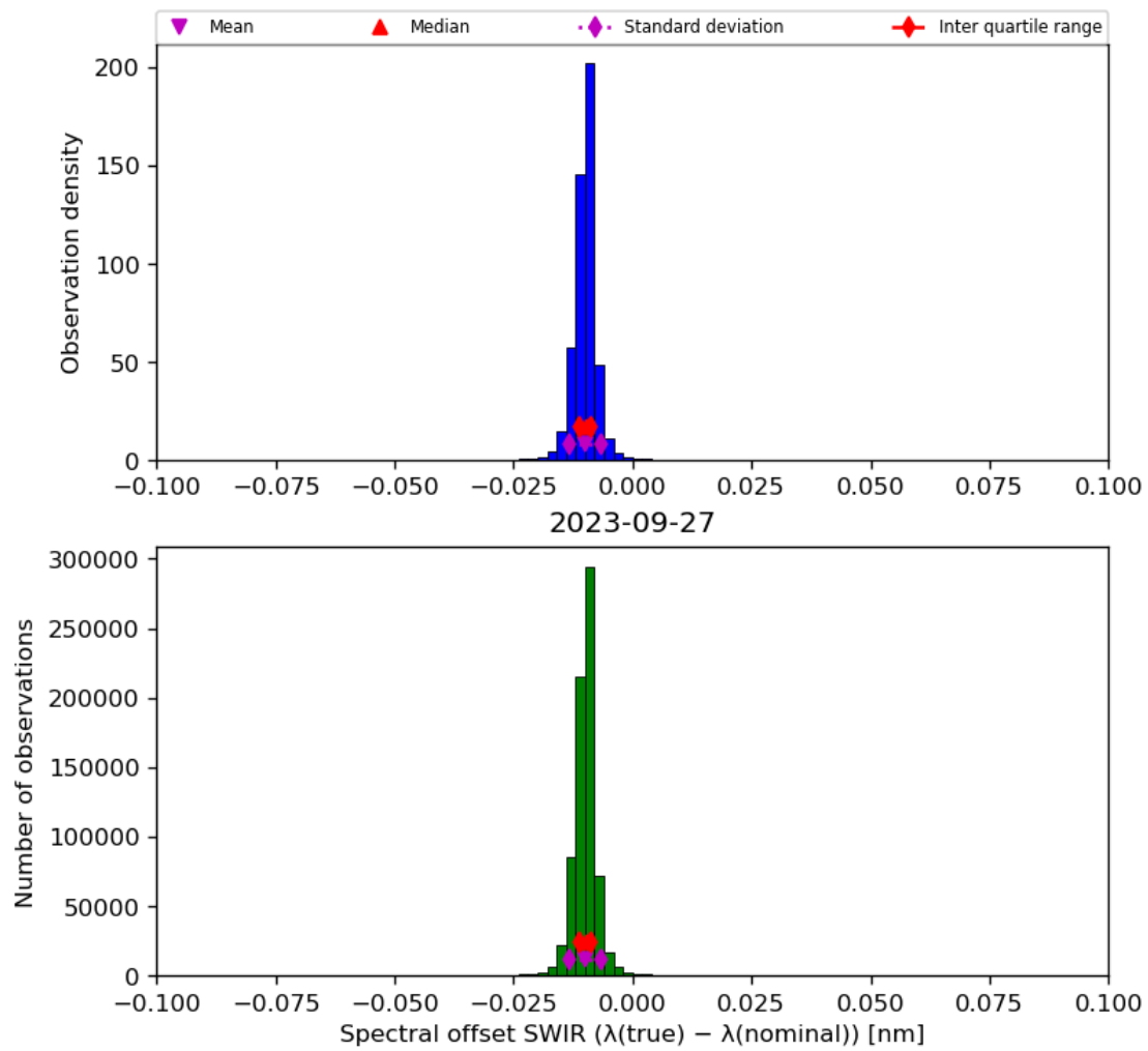
Figure 27: Histogram of “Spectral offset SWIR ( \lambda(\text{true}) - \lambda(\text{nominal}) )” for 2023-09-26 to 2023-09-28
