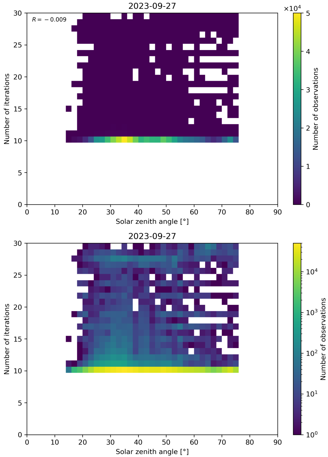
Figure 102: Scatter density plot of “Solar zenith angle” against “Number of iterations” for 2023-09-26 to 2023-09-28.
