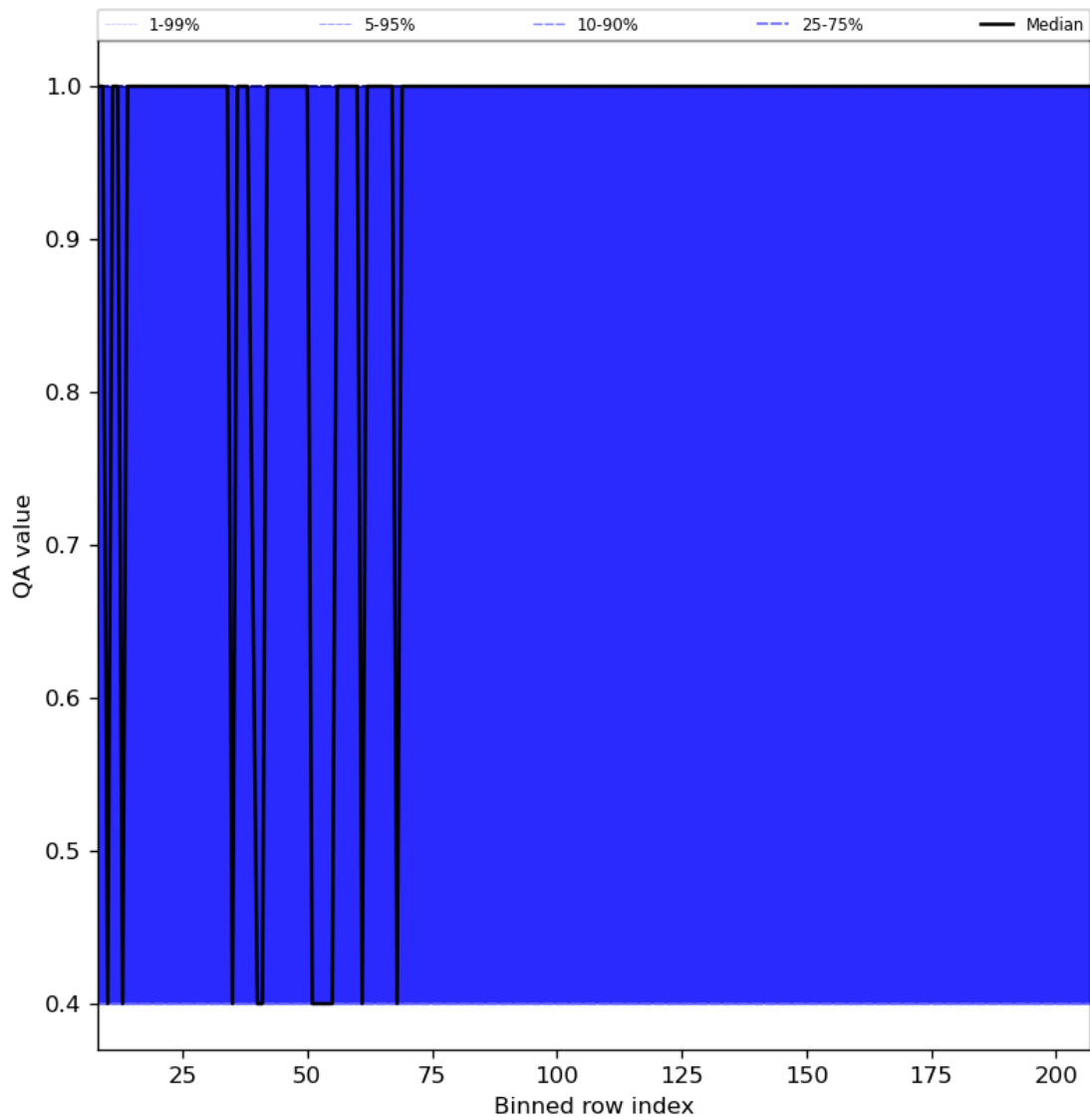
Figure 33: Along track statistics of “QA value” for 2023-09-26 to 2023-09-28
