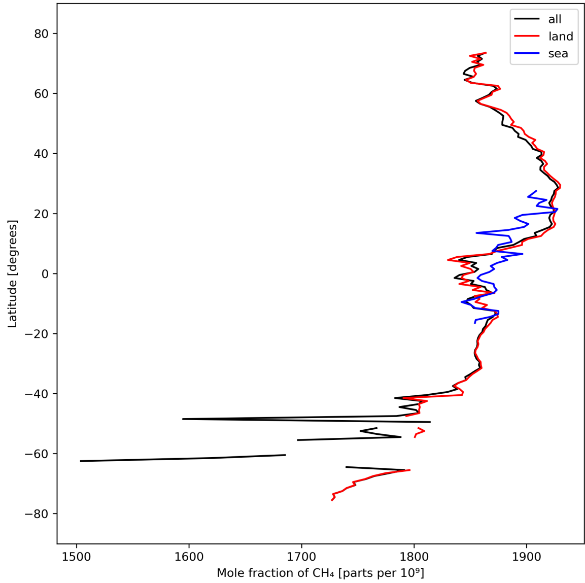
Figure 12: Zonal average of “Mole fraction of \text{CH}_4 ” for 2023-09-26 to 2023-09-28.
