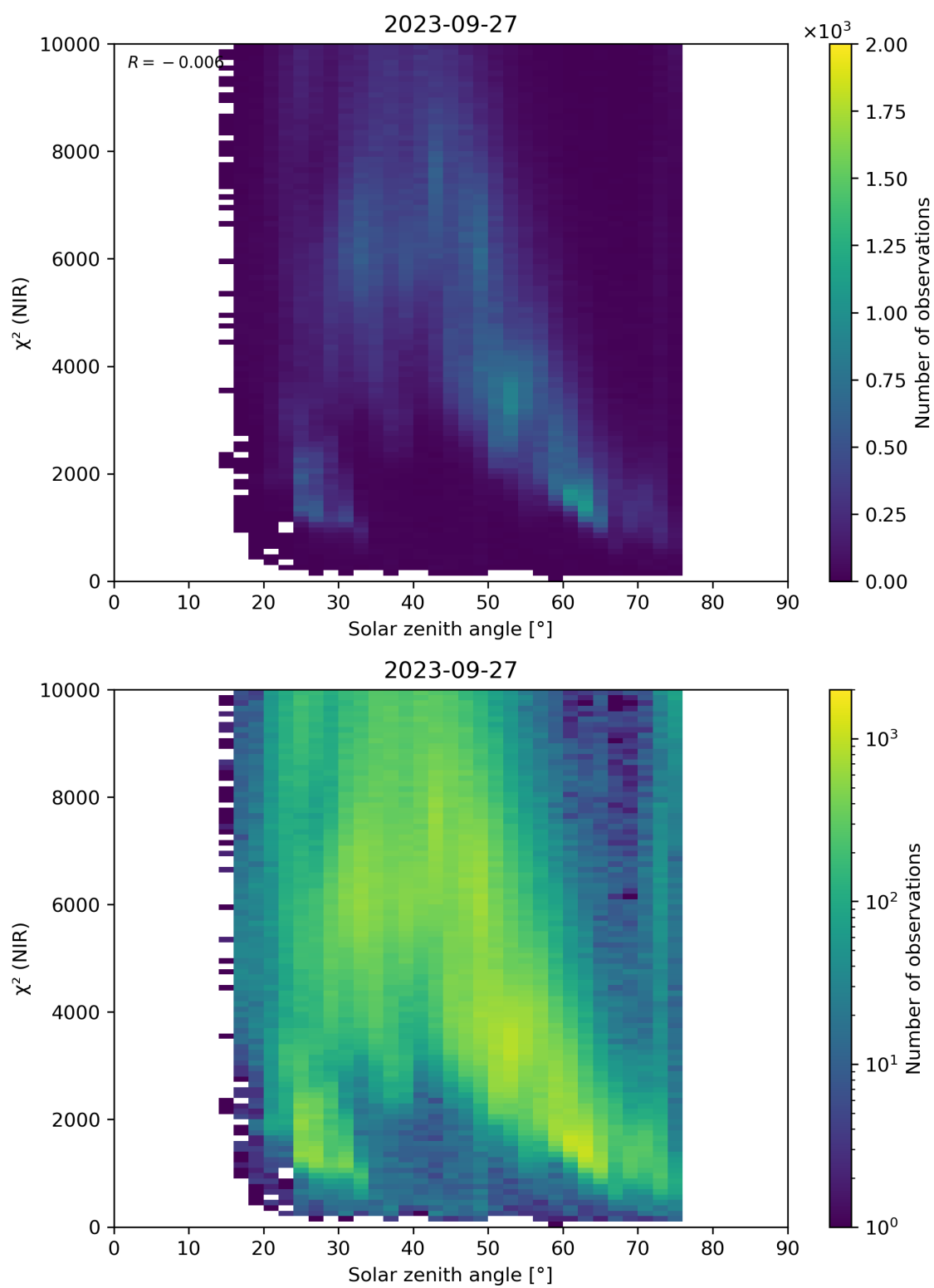
Figure 94: Scatter density plot of “Solar zenith angle” against “ \chi^2 (NIR)” for 2023-09-26 to 2023-09-28.
