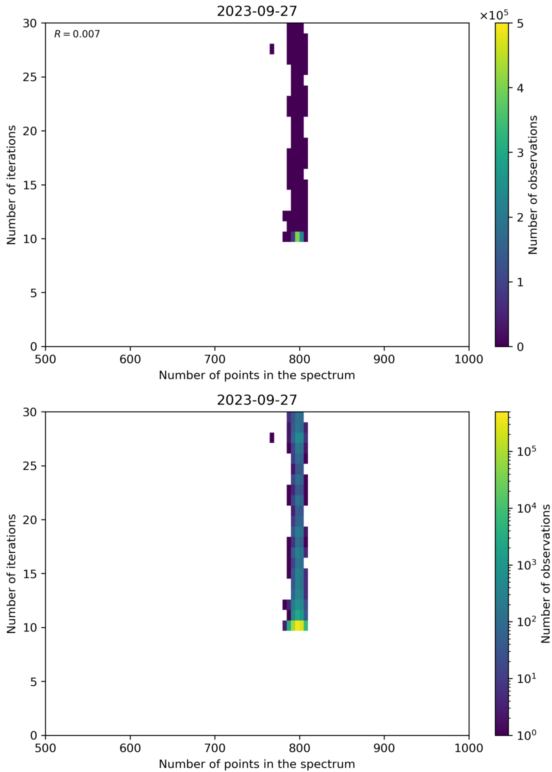
Figure 92: Scatter density plot of “Number of points in the spectrum” against “Number of iterations” for 2023-09-26 to 2023-09-28.
