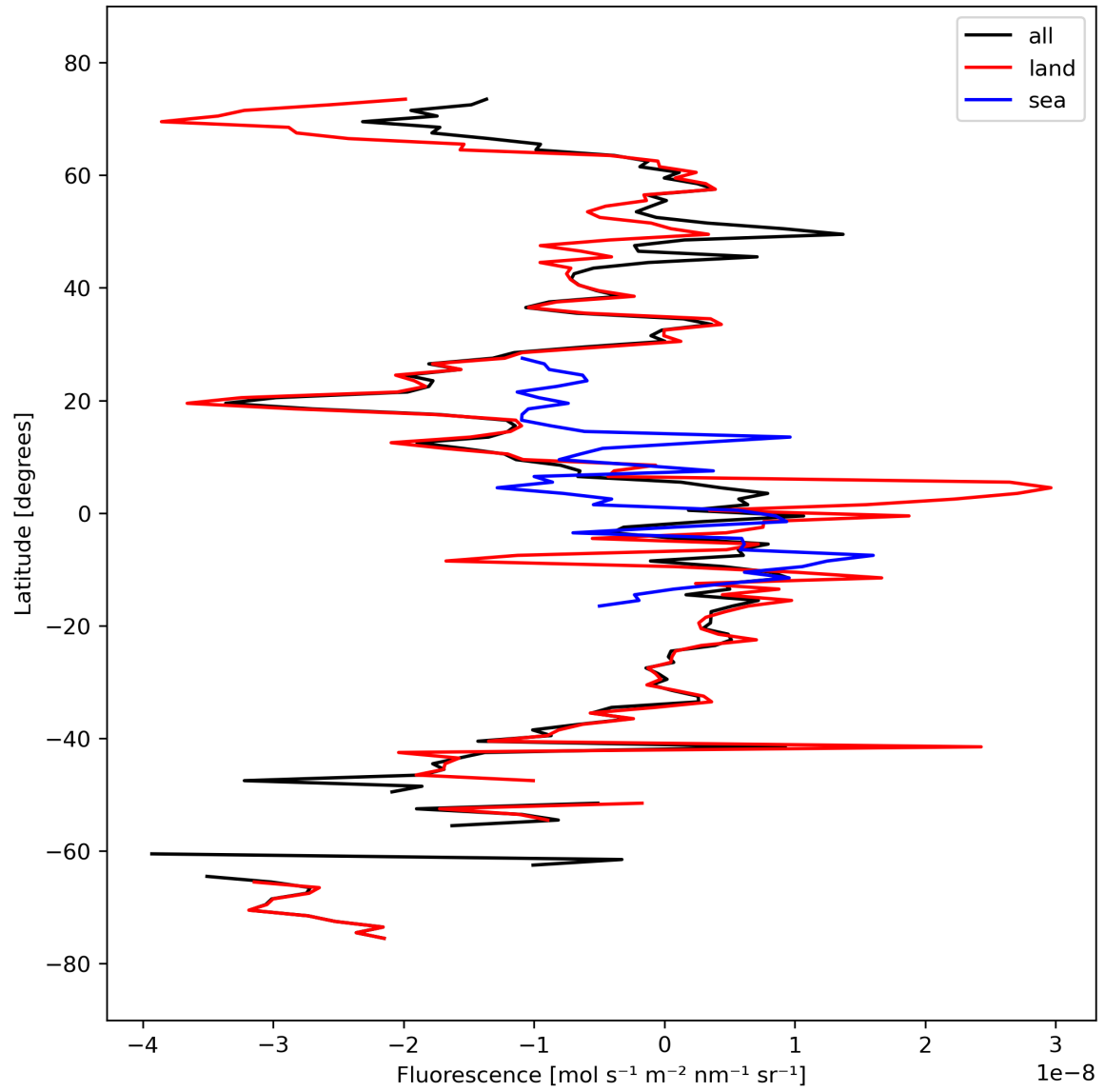
Figure 21: Zonal average of “Fluorescence” for 2023-09-26 to 2023-09-28.
