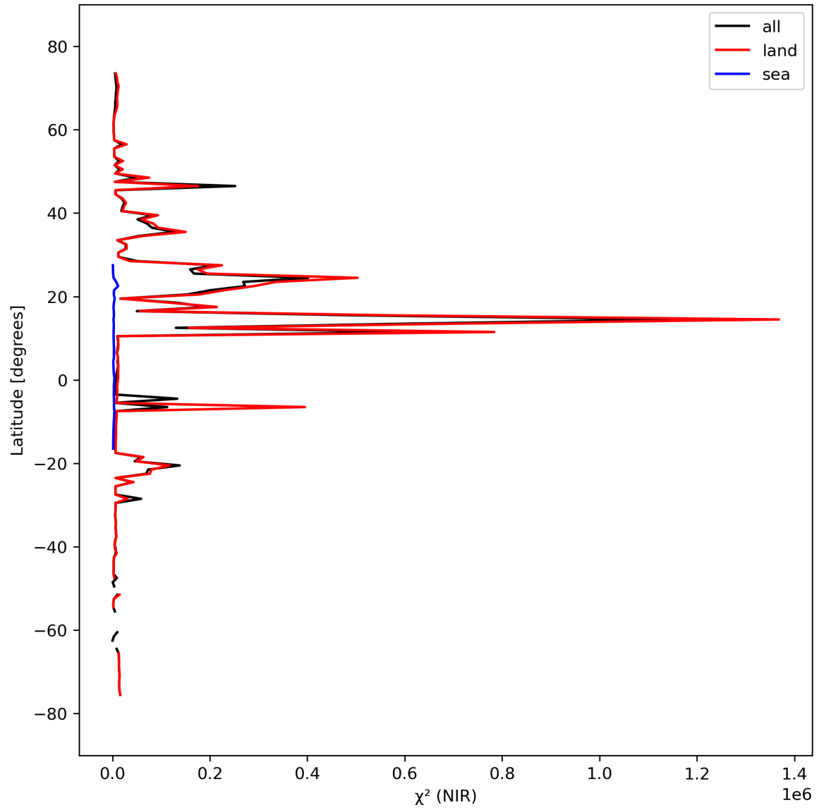
Figure 18: Zonal average of “ \chi^2 (NIR)” for 2023-09-26 to 2023-09-28.
