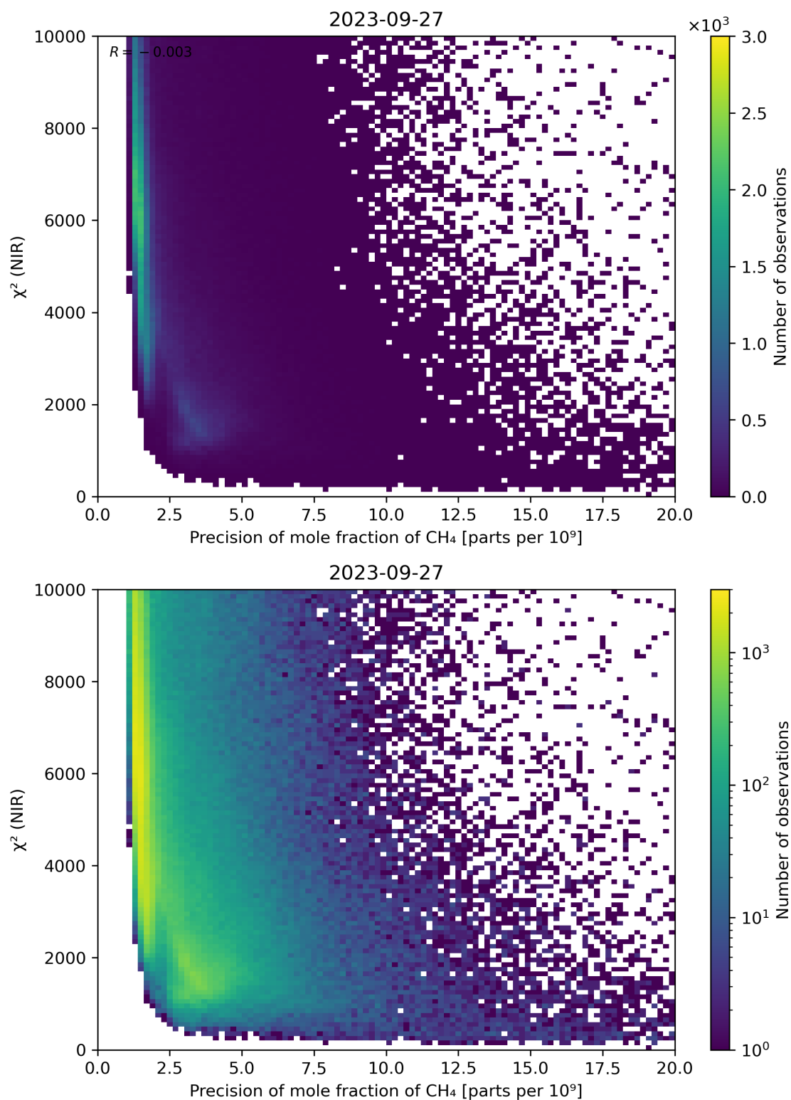
Figure 78: Scatter density plot of “Precision of mole fraction of \text{CH}_4 ” against “ \chi^2 (NIR)” for 2023-09-26 to 2023-09-28.
