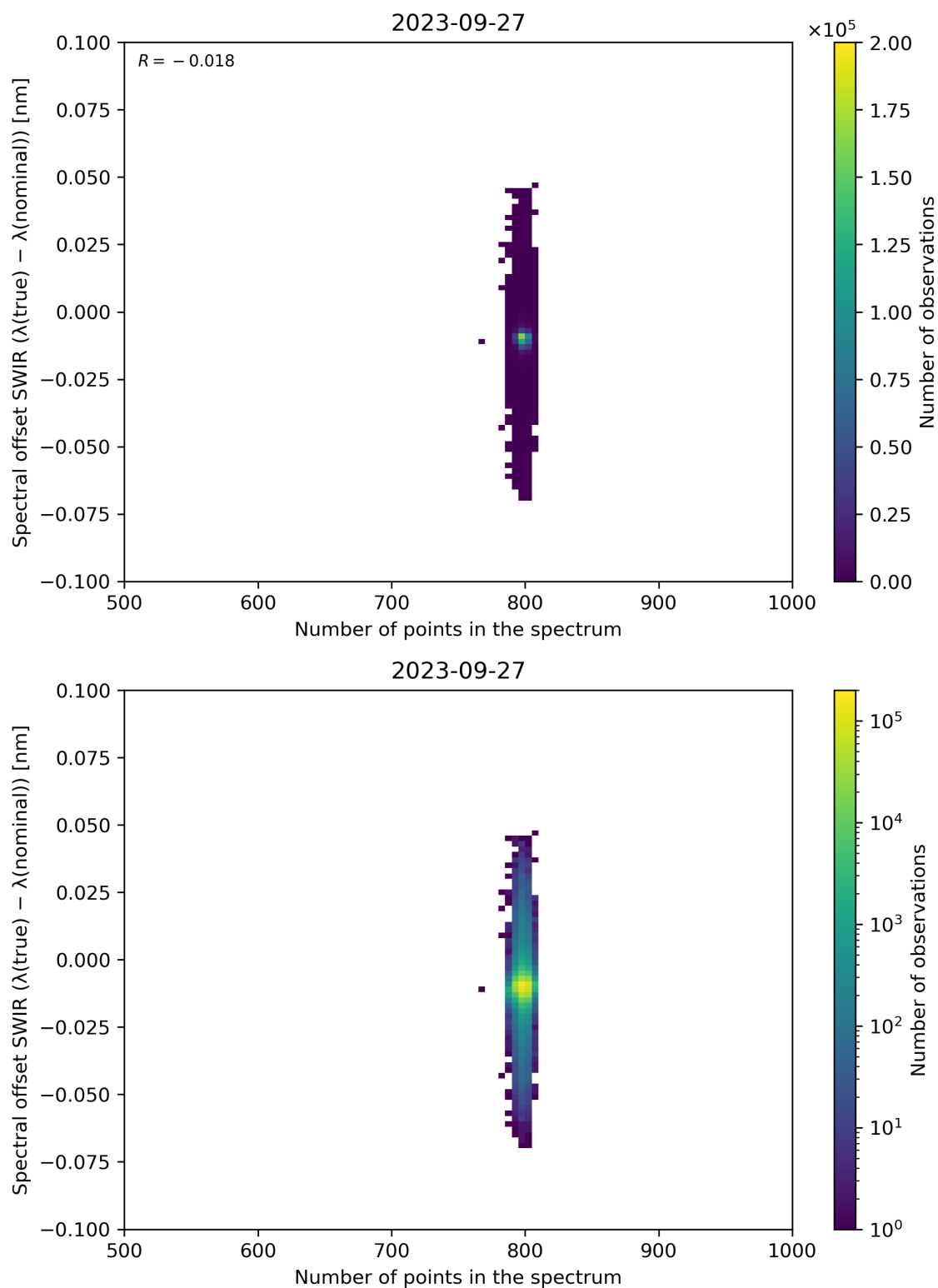
Figure 93: Scatter density plot of “Number of points in the spectrum” against “Spectral offset SWIR ( \lambda(\text{true}) - \lambda(\text{nominal}) )” for 2023-09-26 to 2023-09-28.
