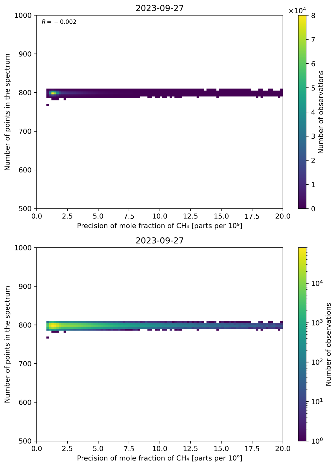
Figure 84: Scatter density plot of “Precision of mole fraction of CH 4 ” against “Number of points in the spectrum” for 2023-09-26 to 2023-09-28.
