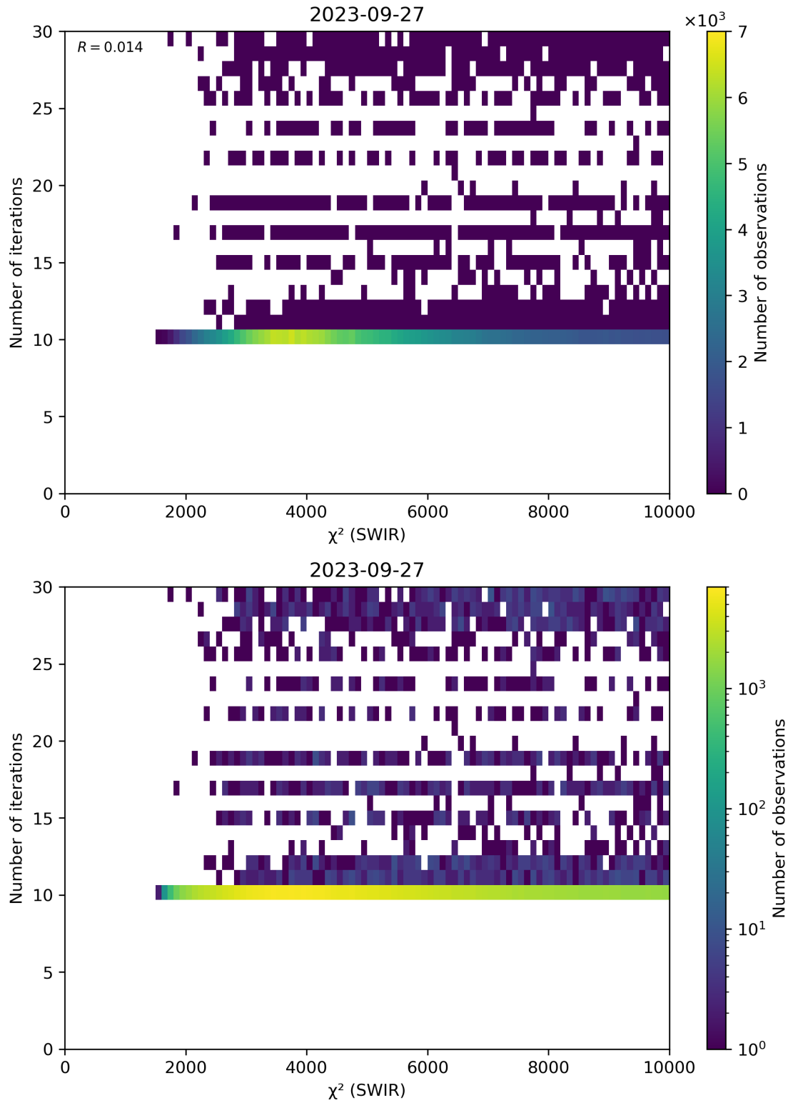
Figure 50: Scatter density plot of “ \chi^2 (SWIR)” against “Number of iterations” for 2023-09-26 to 2023-09-28.
