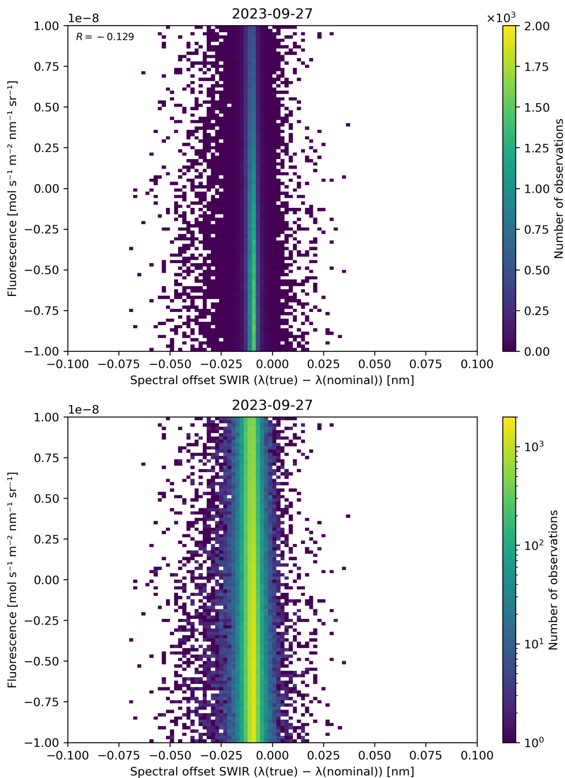
Figure 120: Scatter density plot of “Spectral offset SWIR ( \lambda(\text{true}) - \lambda(\text{nominal}) )” against “Fluorescence” for 2023-09-26 to 2023-09-28.
