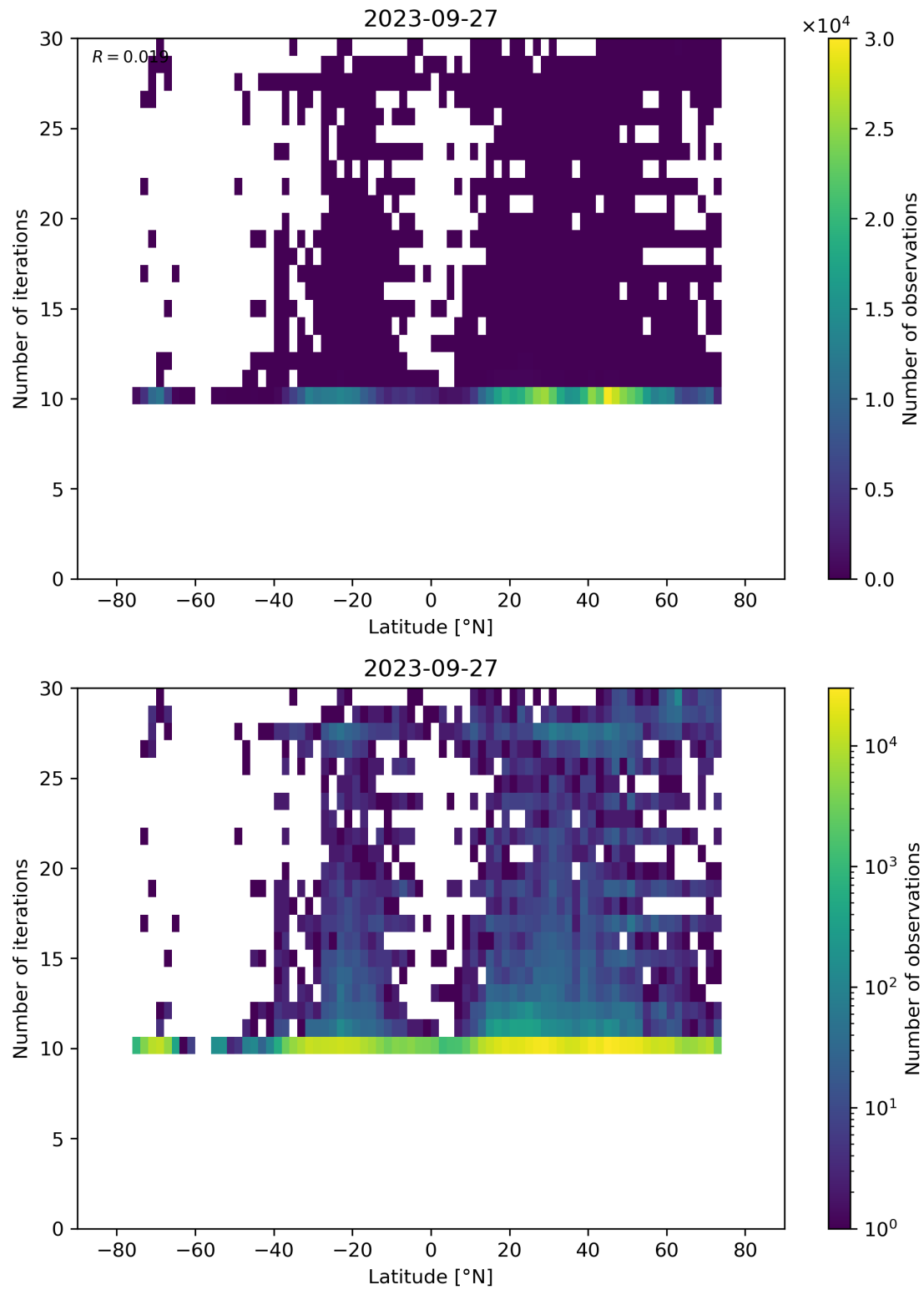
Figure 60: Scatter density plot of “Latitude” against “Number of iterations” for 2023-09-26 to 2023-09-28.
