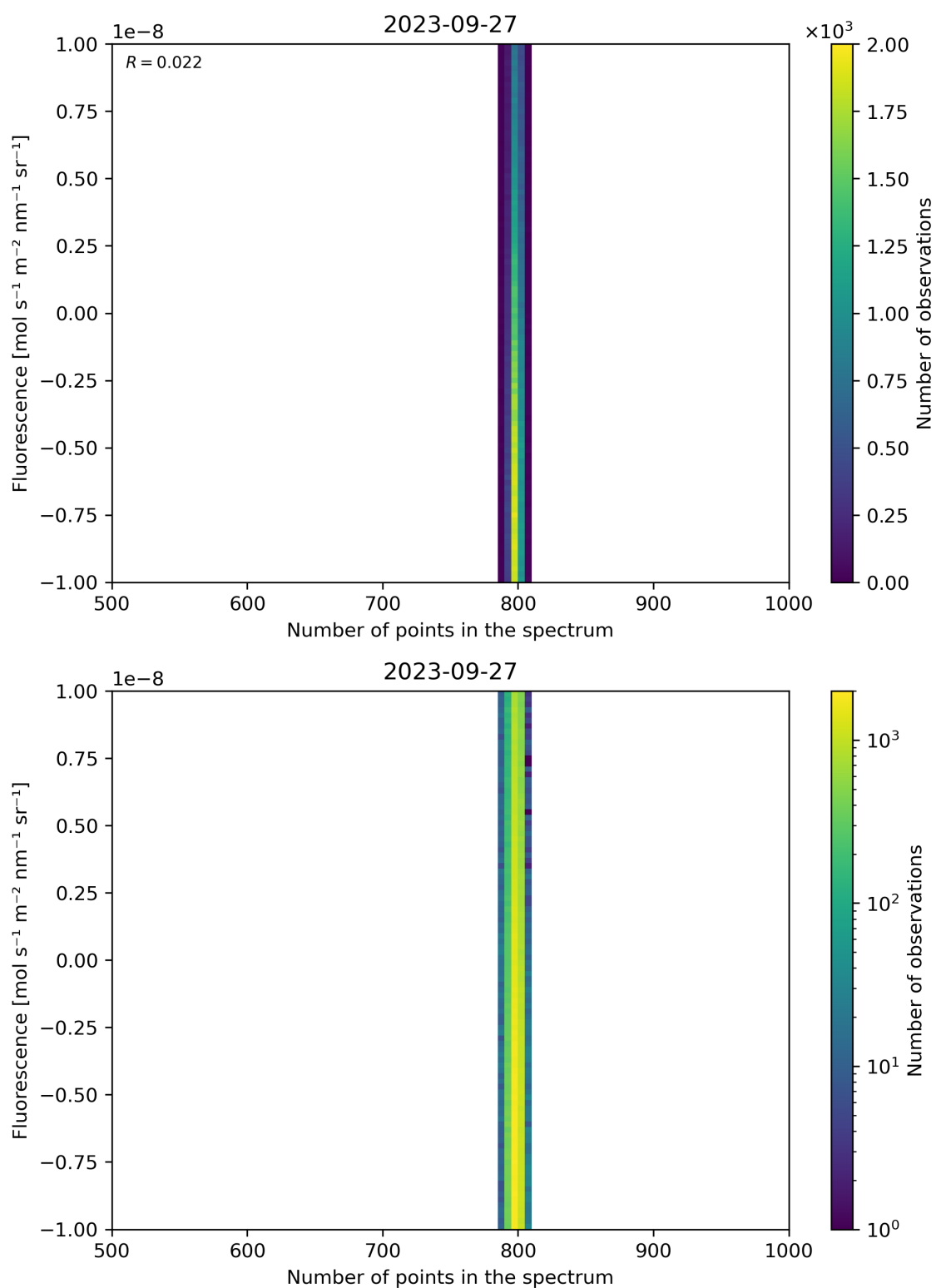
Figure 91: Scatter density plot of “Number of points in the spectrum” against “Fluorescence” for 2023-09-26 to 2023-09-28.
