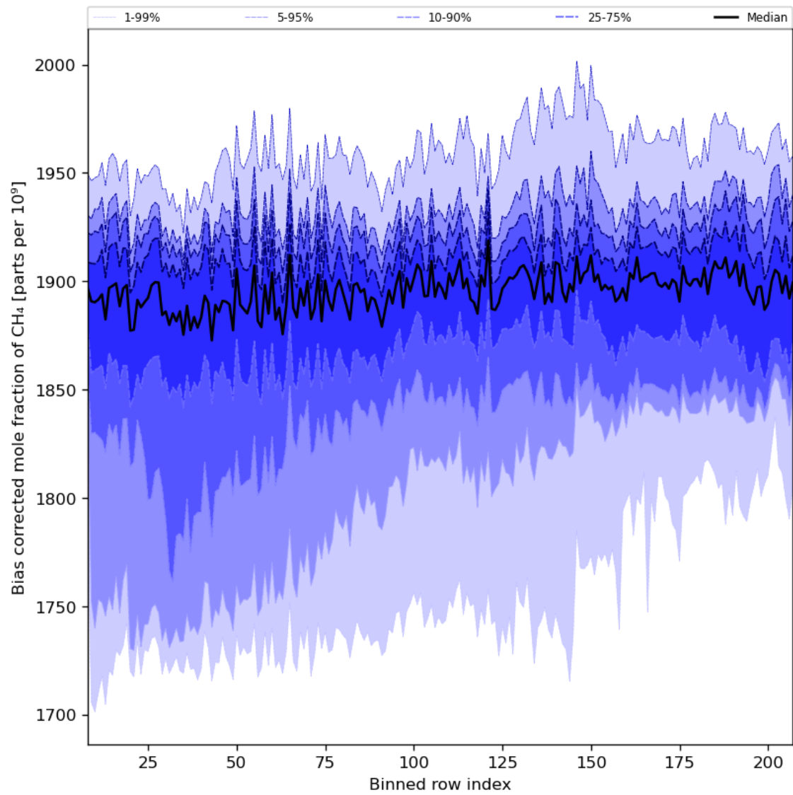
Figure 36: Along track statistics of “Bias corrected mole fraction of CH 4 ” for 2023-09-26 to 2023-09-28
