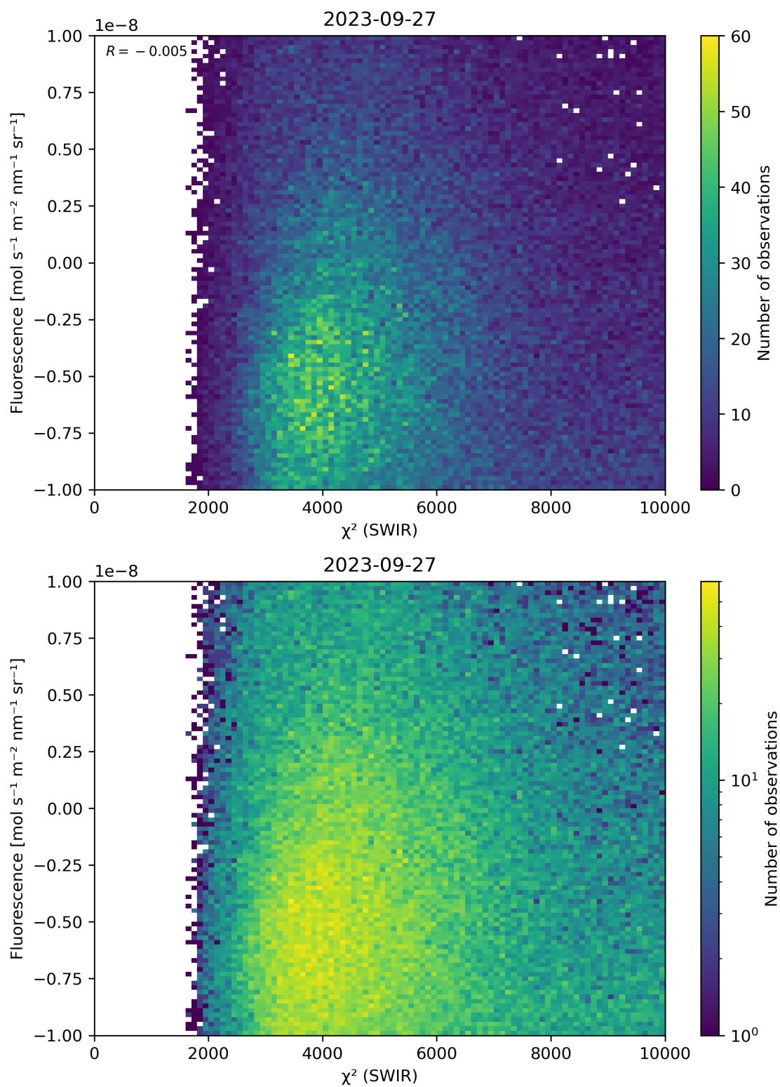
Figure 49: Scatter density plot of “ \chi^2 (SWIR)” against “Fluorescence” for 2023-09-26 to 2023-09-28.
