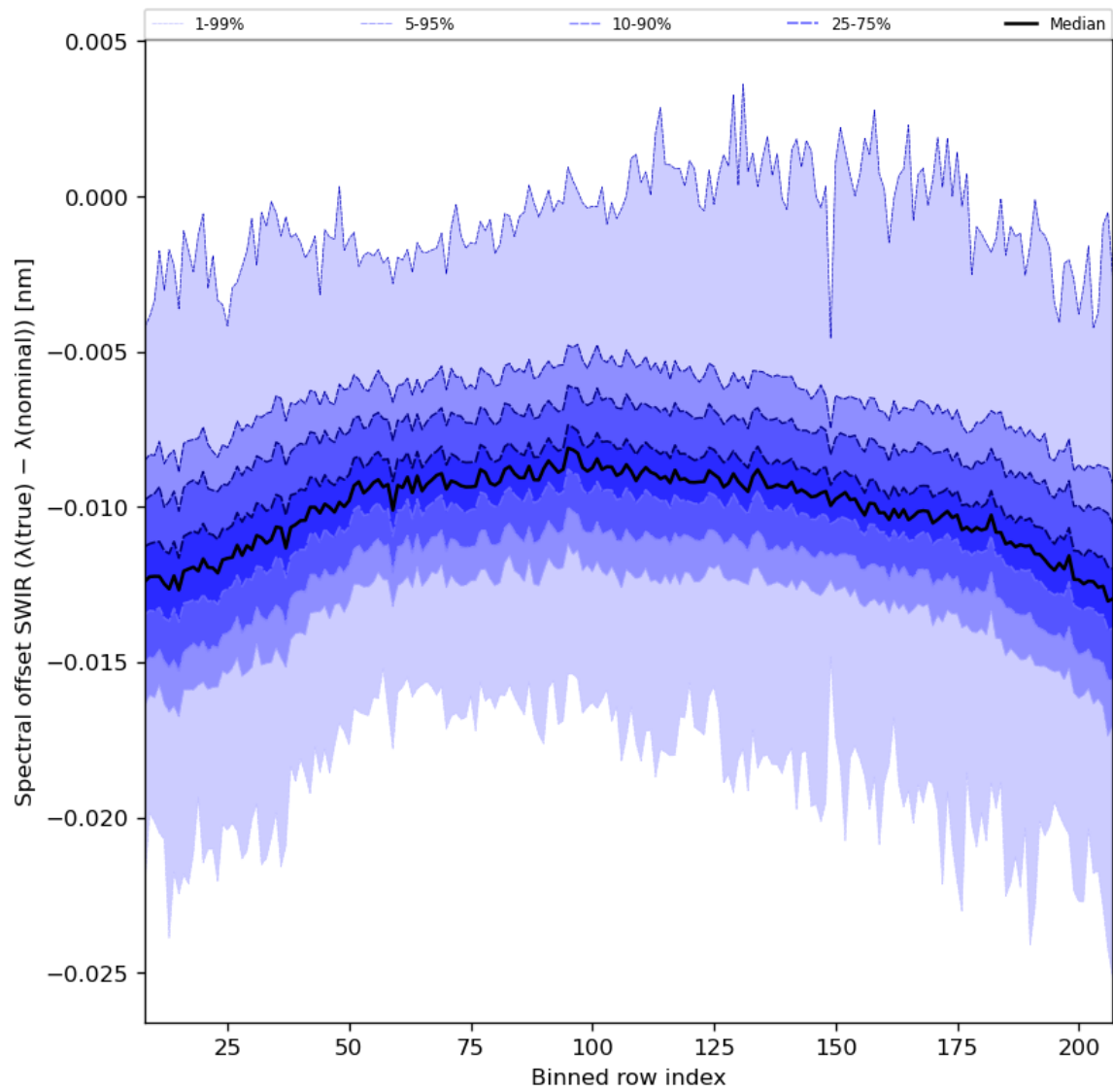
Figure 38: Along track statistics of “Spectral offset SWIR ( \lambda(\text{true}) - \lambda(\text{nominal}) )” for 2023-09-26 to 2023-09-28
