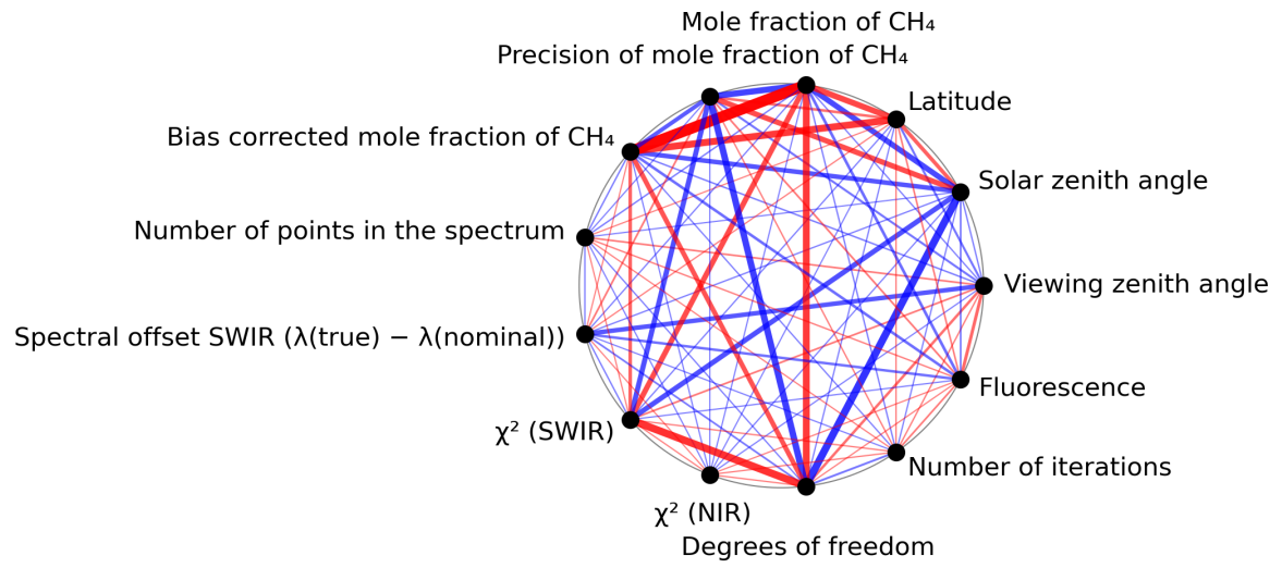
Figure 1: Map of correlation graph for 2023-09-26 to 2023-09-28.
