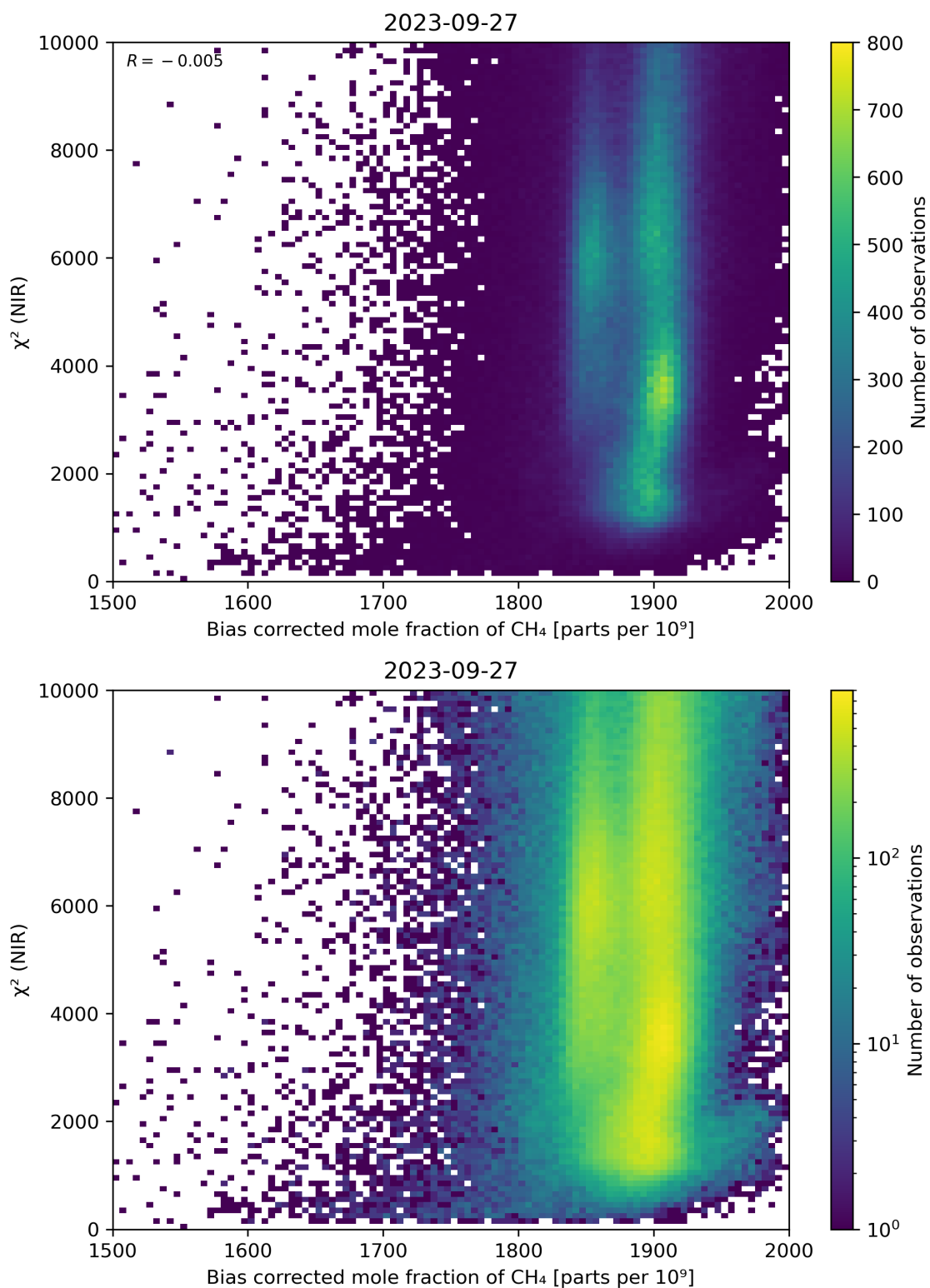
Figure 63: Scatter density plot of “Bias corrected mole fraction of CH 4 ” against “ \chi^2 (NIR)” for 2023-09-26 to 2023-09-28.
