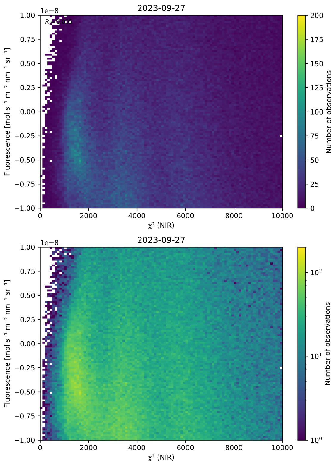
Figure 45: Scatter density plot of “ \chi^2 (NIR)” against “Fluorescence” for 2023-09-26 to 2023-09-28.
