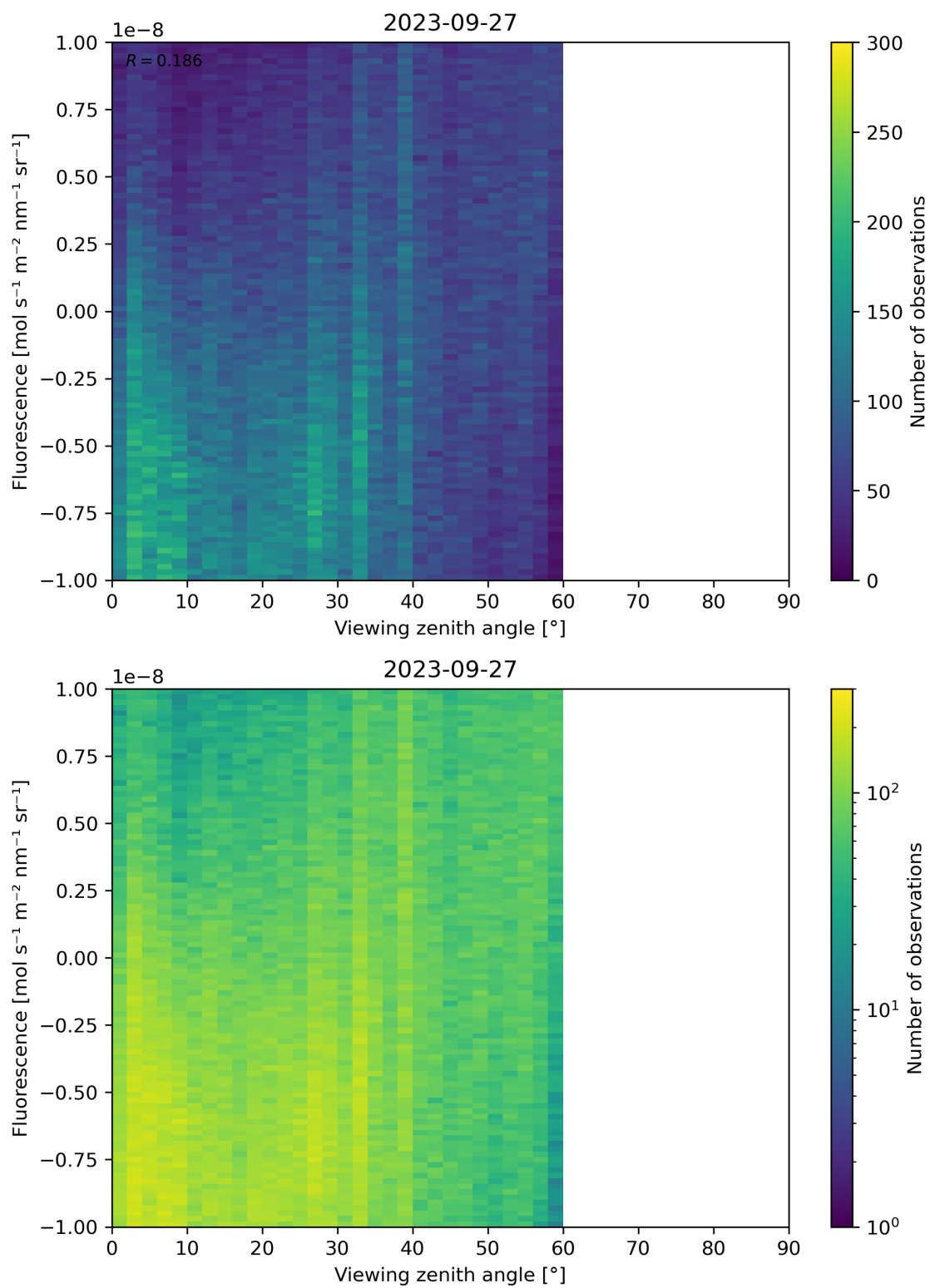
Figure 108: Scatter density plot of “Viewing zenith angle” against “Fluorescence” for 2023-09-26 to 2023-09-28.
