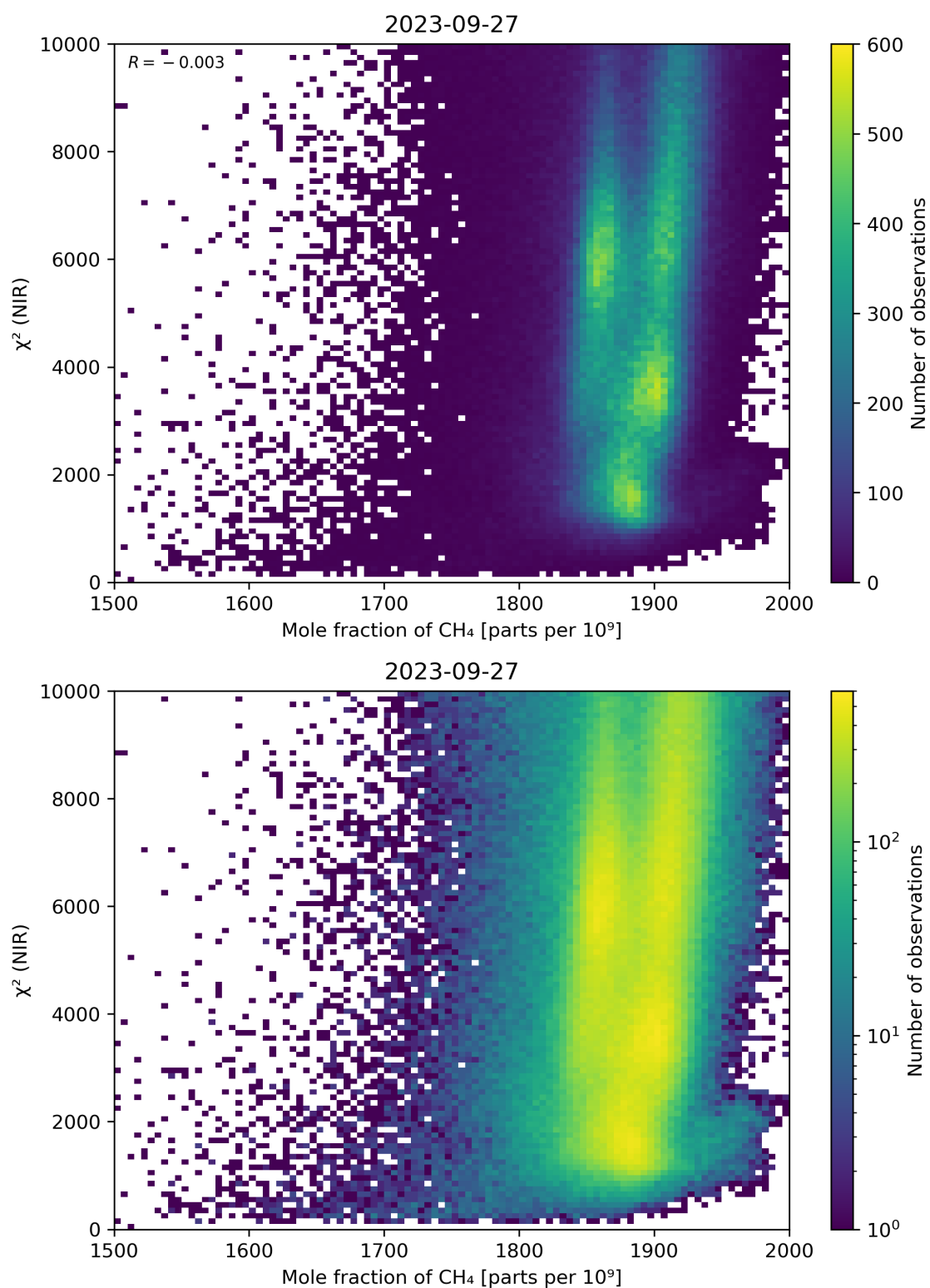
Figure 70: Scatter density plot of “Mole fraction of CH 4 ” against “ \chi^2 (NIR)” for 2023-09-26 to 2023-09-28.
