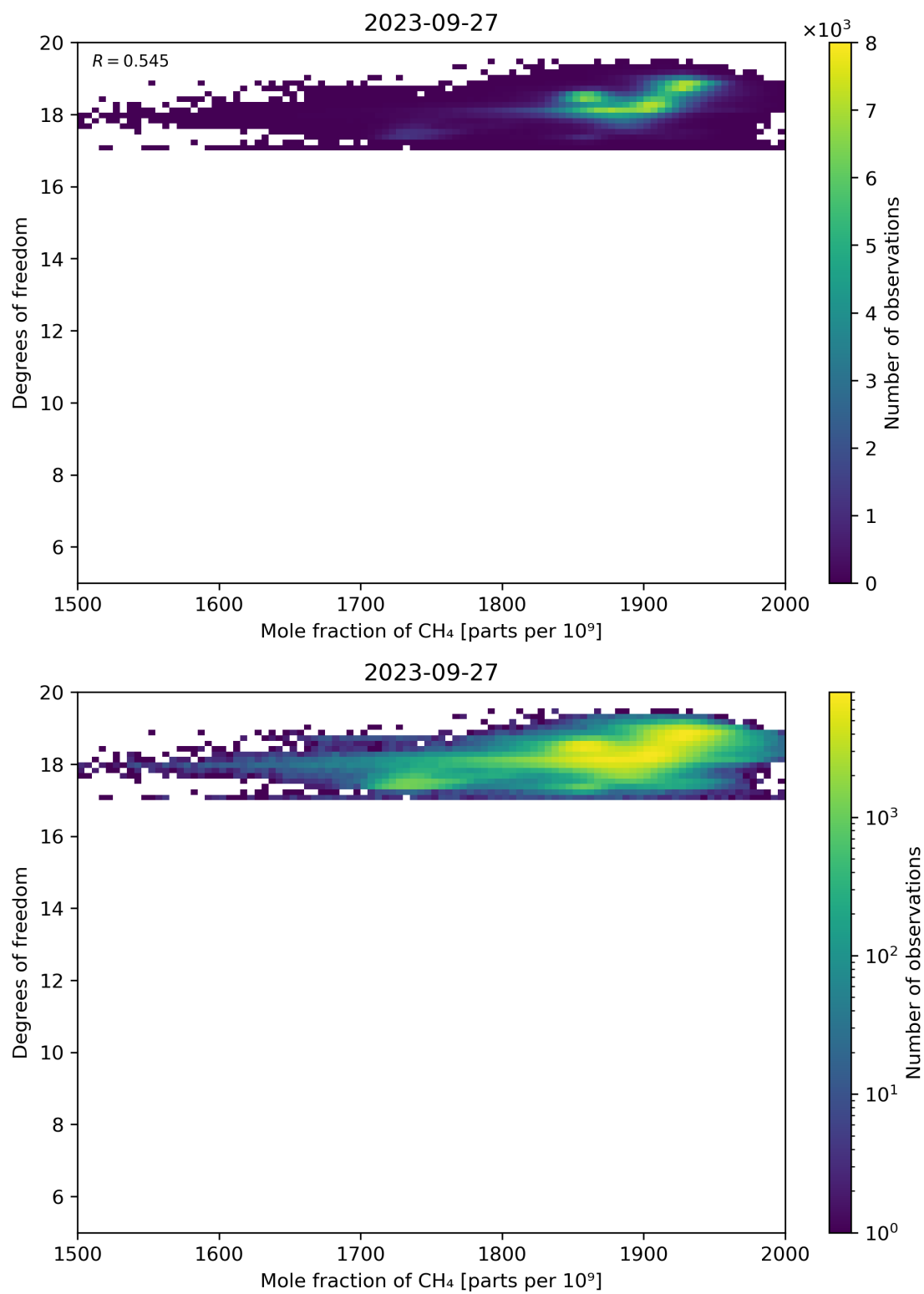
Figure 72: Scatter density plot of “Mole fraction of CH 4 ” against “Degrees of freedom” for 2023-09-26 to 2023-09-28.
