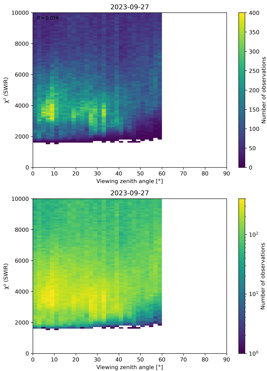
Figure 106: Scatter density plot of “Viewing zenith angle” against “ \chi^2 (SWIR)” for 2023-09-26 to 2023-09-28.
