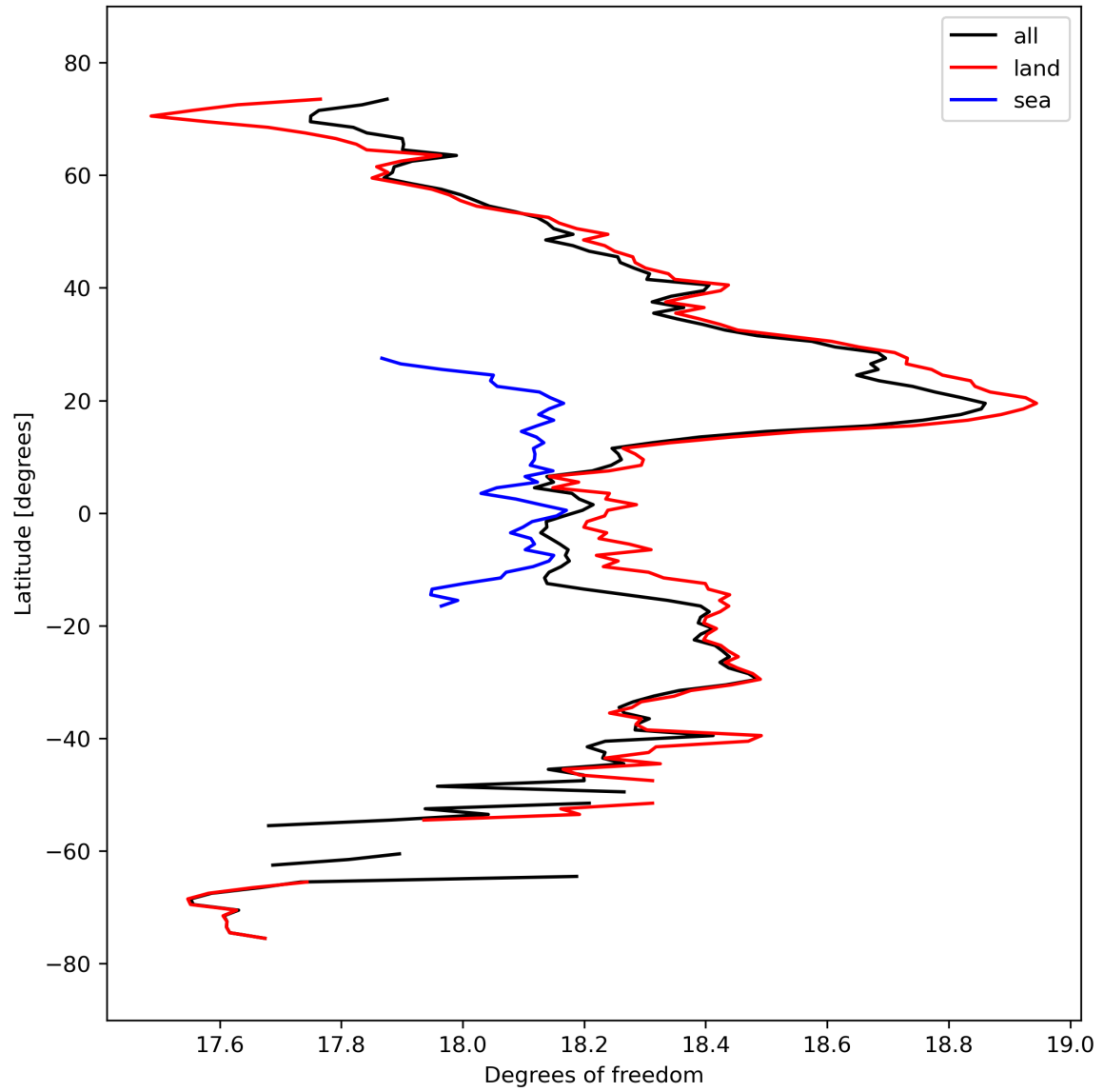
Figure 19: Zonal average of “Degrees of freedom” for 2023-09-26 to 2023-09-28.
