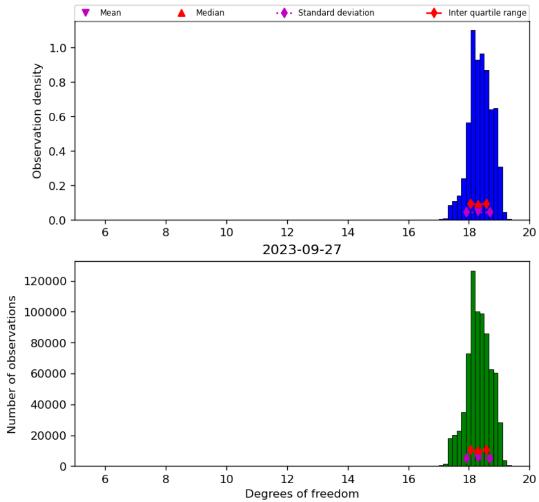
Figure 30: Histogram of “Degrees of freedom” for 2023-09-26 to 2023-09-28
