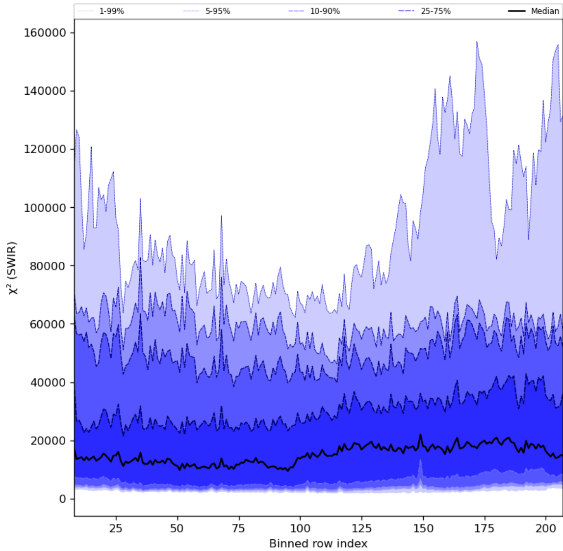
Figure 39: Along track statistics of “ \chi^2 (SWIR)” for 2023-09-26 to 2023-09-28
