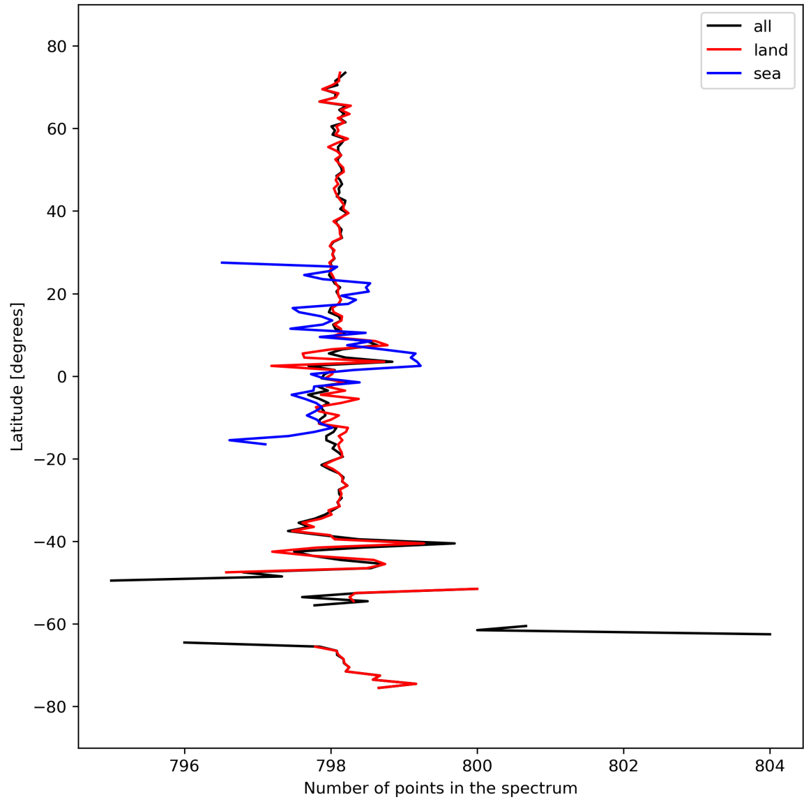
Figure 15: Zonal average of “Number of points in the spectrum” for 2023-09-26 to 2023-09-28.
