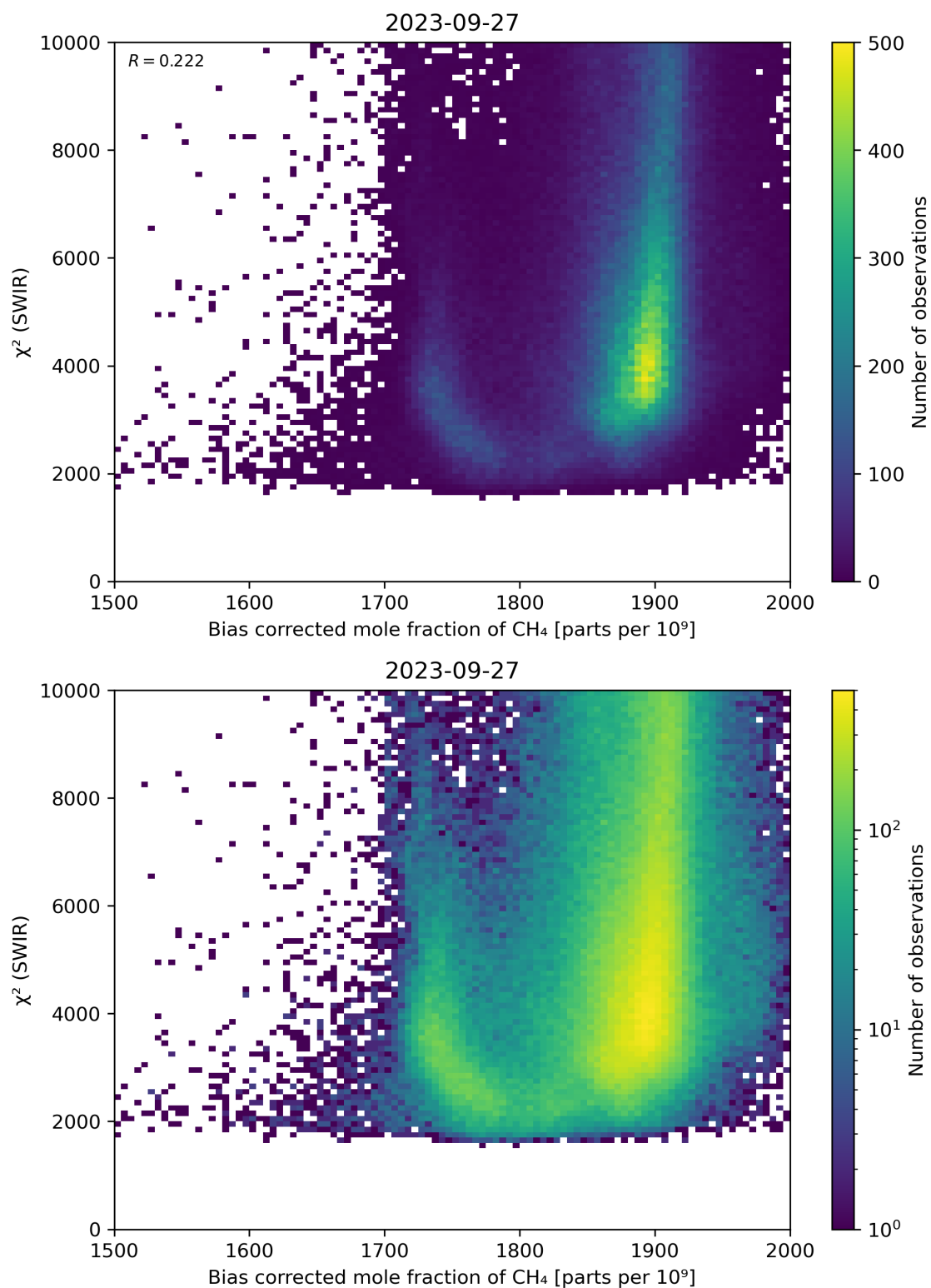
Figure 64: Scatter density plot of “Bias corrected mole fraction of \text{CH}_4 ” against “ \chi^2 (SWIR)” for 2023-09-26 to 2023-09-28.
